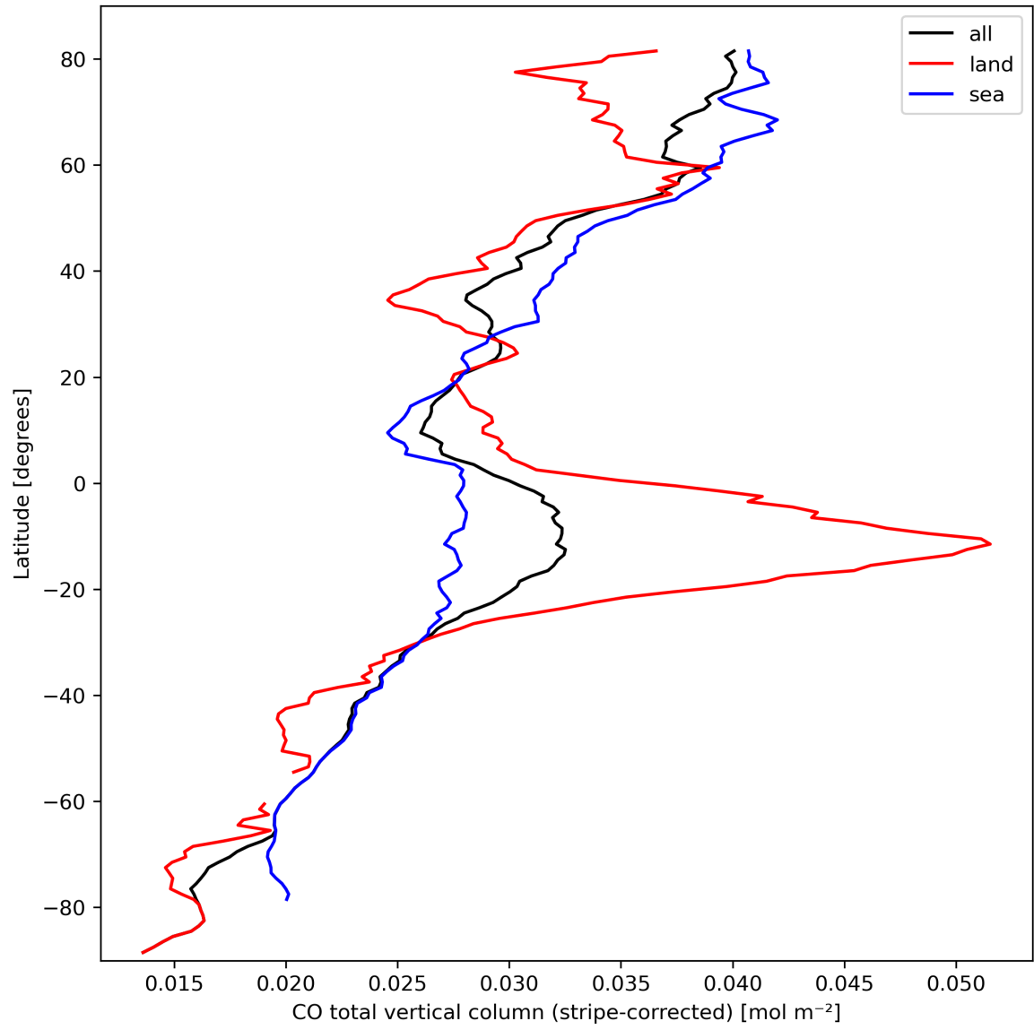
Figure 11: Zonal average of “CO total vertical column (stripe-corrected)” for 2023-10-01 to 2023-10-03.
