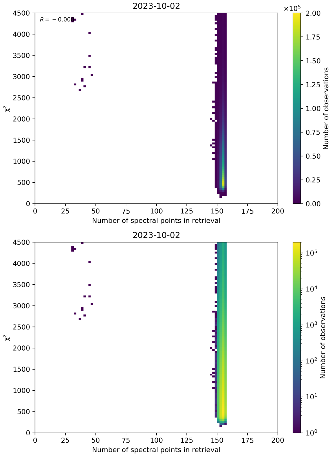
Figure 58: Scatter density plot of “Number of spectral points in retrieval” against “ \chi^2 ” for 2023-10-01 to 2023-10-03.
