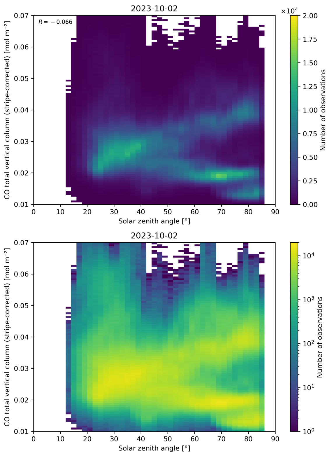
Figure 62: Scatter density plot of “Solar zenith angle” against “CO total vertical column (stripe-corrected)” for 2023-10-01 to 2023-10-03.
