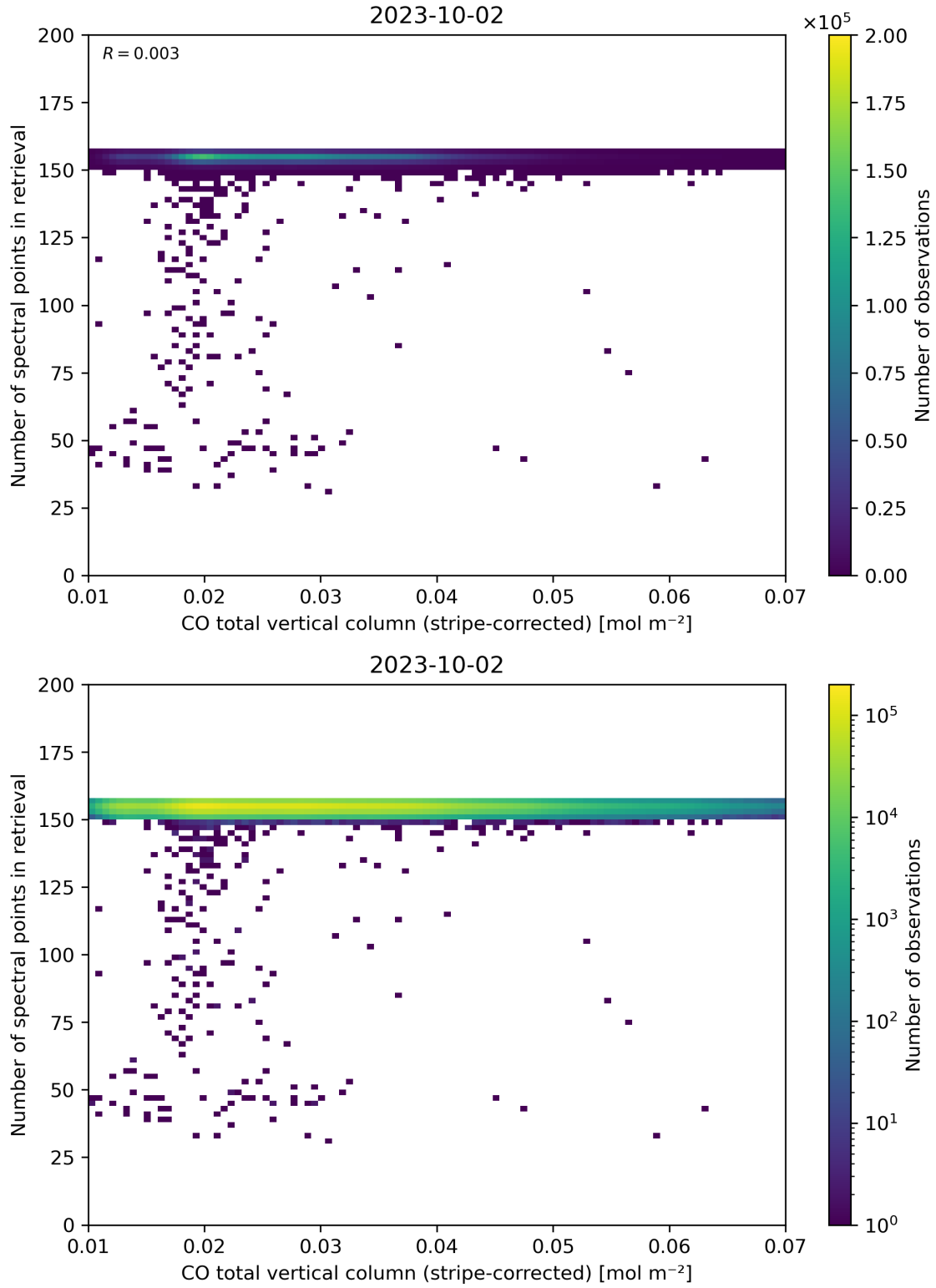
Figure 40: Scatter density plot of “CO total vertical column (stripe-corrected)” against “Number of spectral points in retrieval” for 2023-10-01 to 2023-10-03.
