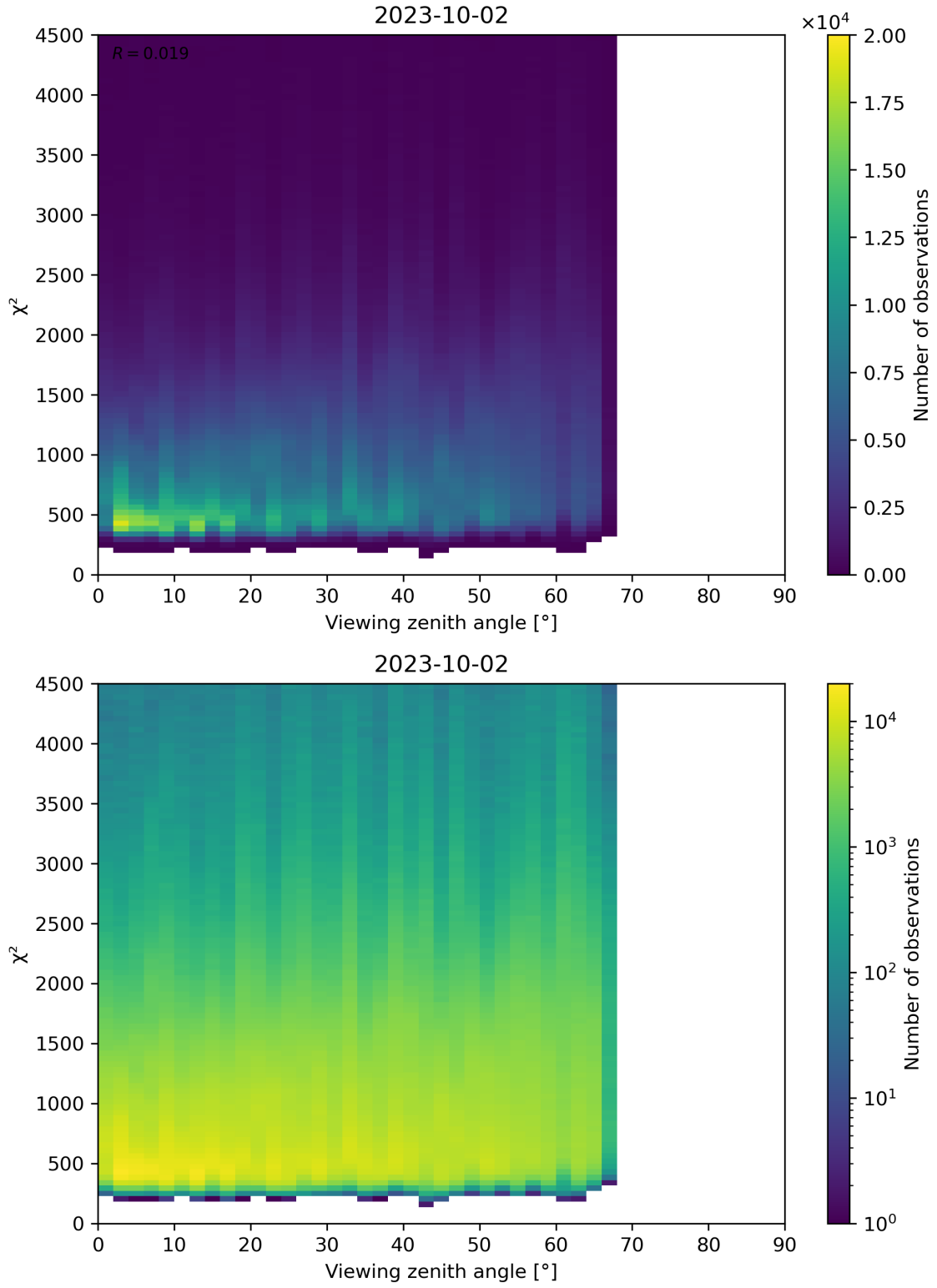
Figure 72: Scatter density plot of “Viewing zenith angle” against “ \chi^2 ” for 2023-10-01 to 2023-10-03.
