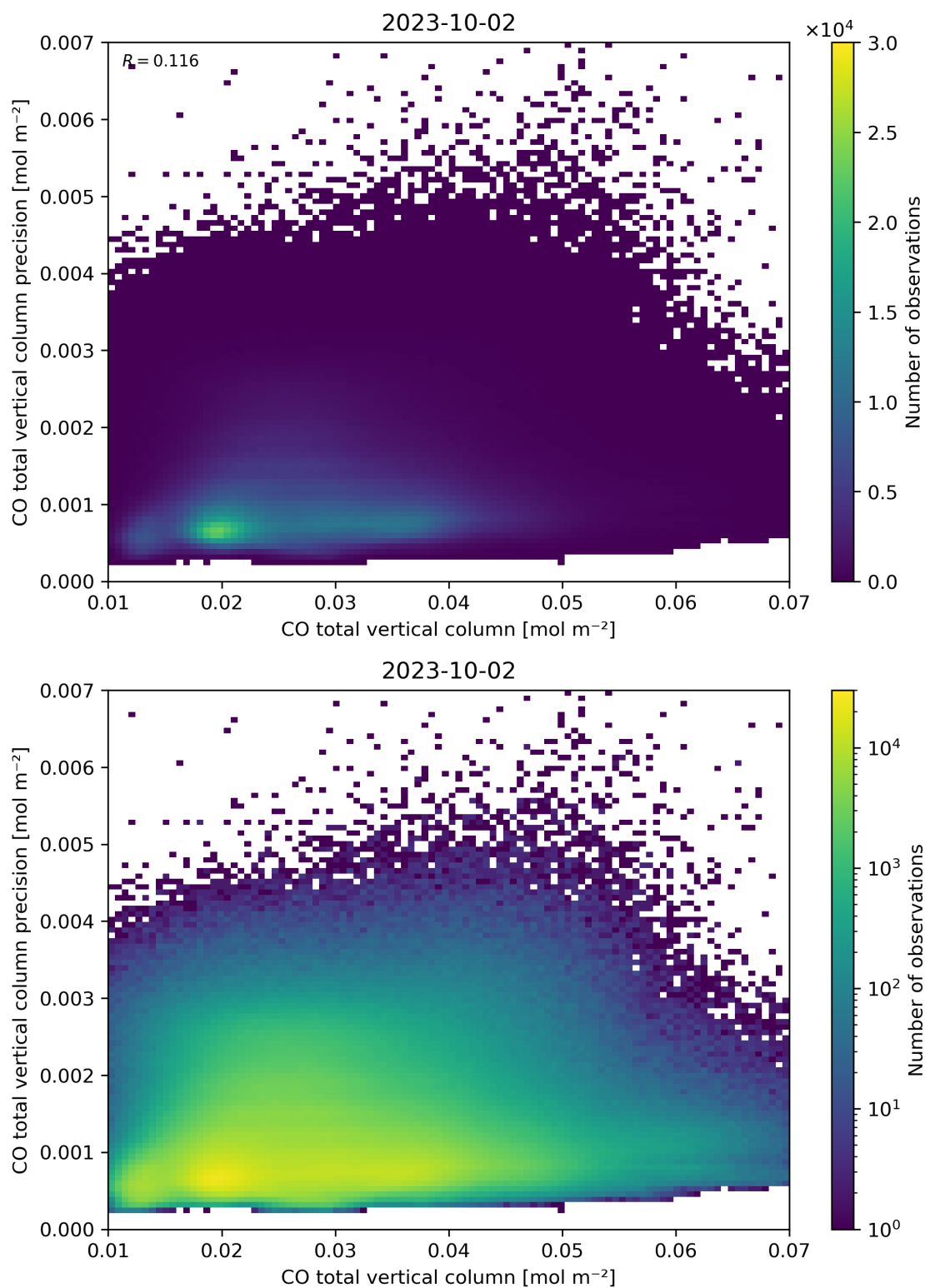
Figure 34: Scatter density plot of “CO total vertical column” against “CO total vertical column precision” for 2023-10-01 to 2023-10-03.
