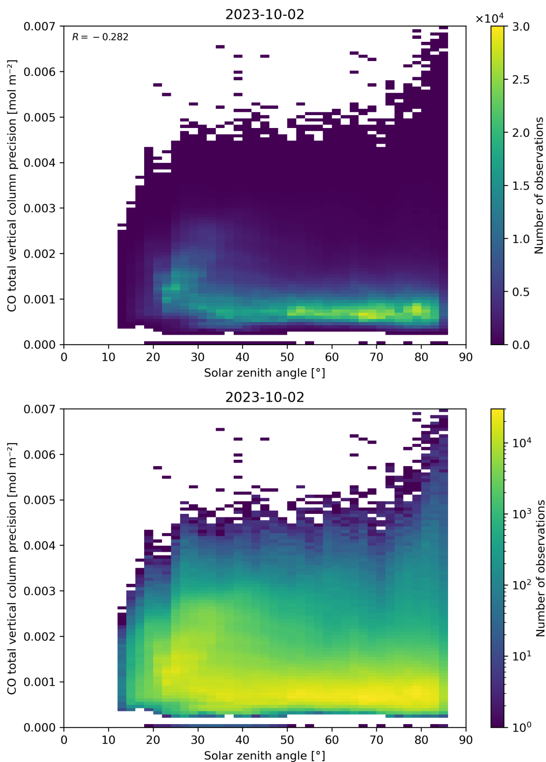
Figure 63: Scatter density plot of “Solar zenith angle” against “CO total vertical column precision” for 2023-10-01 to 2023-10-03.
