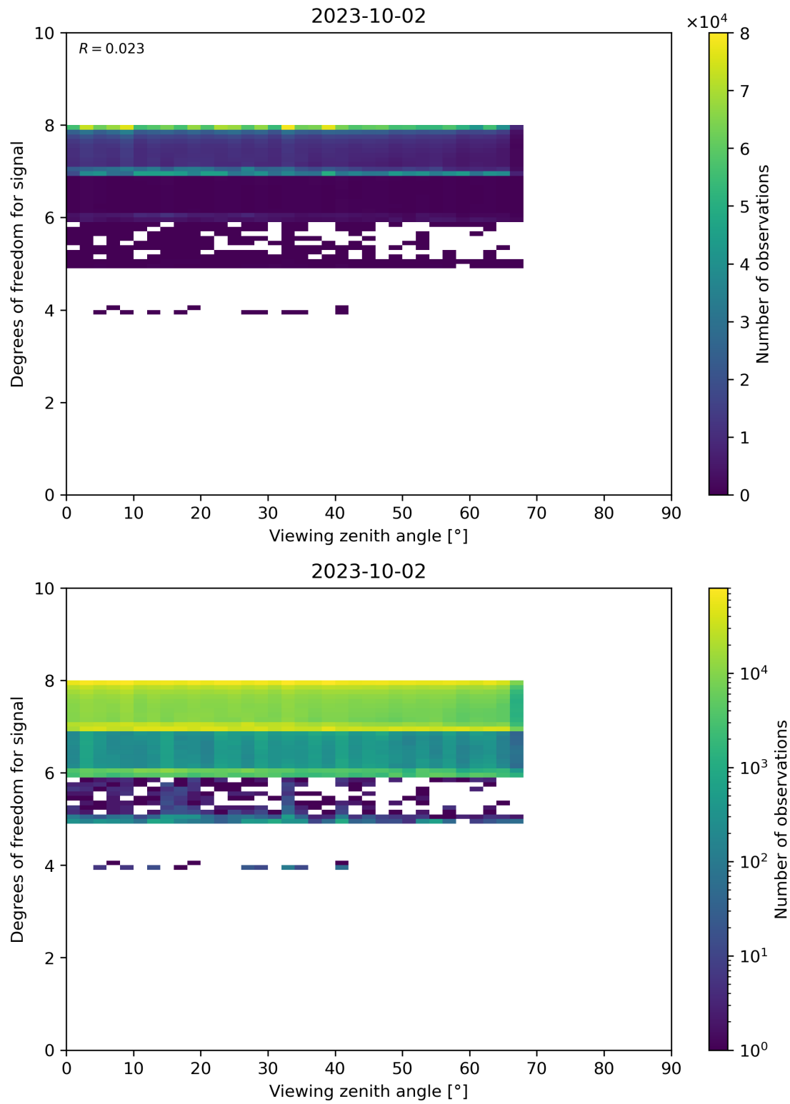
Figure 73: Scatter density plot of “Viewing zenith angle” against “Degrees of freedom for signal” for 2023-10-01 to 2023-10-03.
