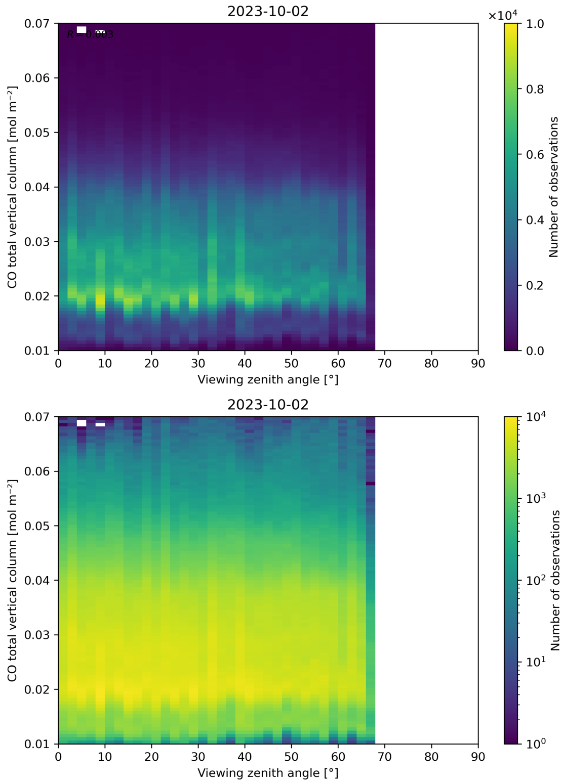
Figure 69: Scatter density plot of “Viewing zenith angle” against “CO total vertical column” for 2023-10-01 to 2023-10-03.
