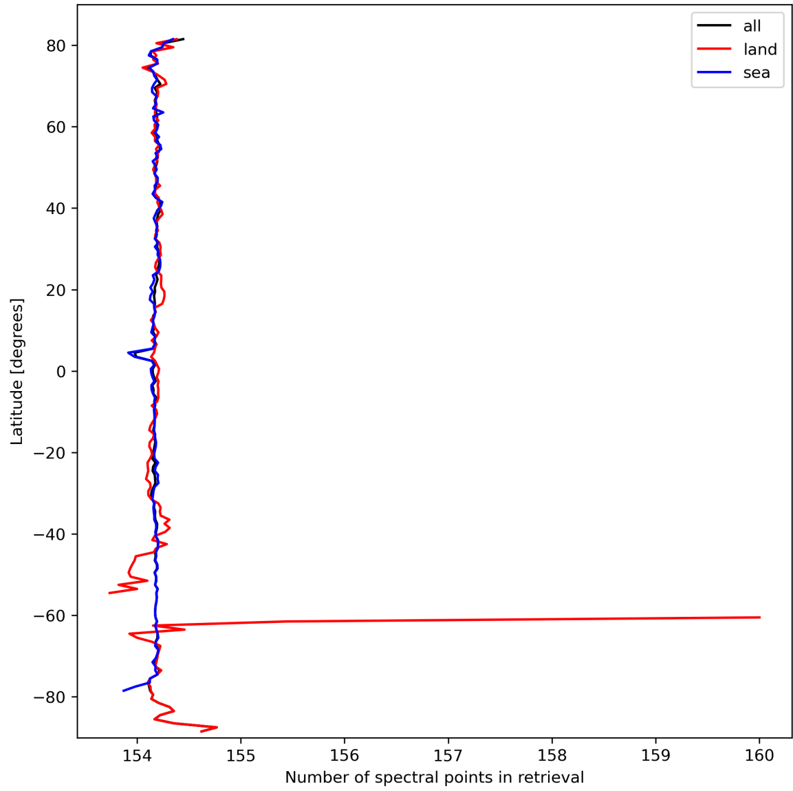
Figure 13: Zonal average of “Number of spectral points in retrieval” for 2023-10-01 to 2023-10-03.
