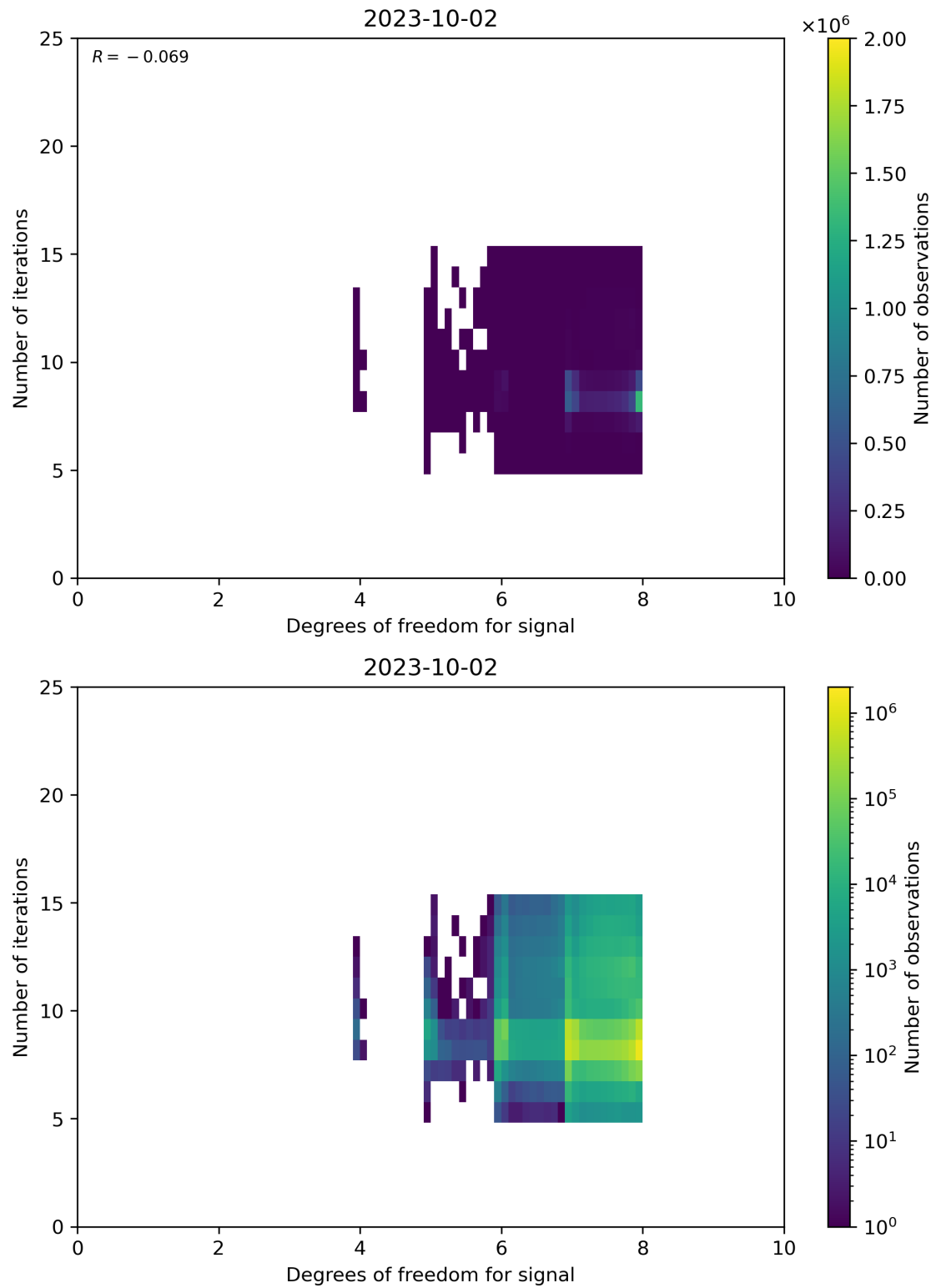
Figure 50: Scatter density plot of “Degrees of freedom for signal” against “Number of iterations” for 2023-10-01 to 2023-10-03.
