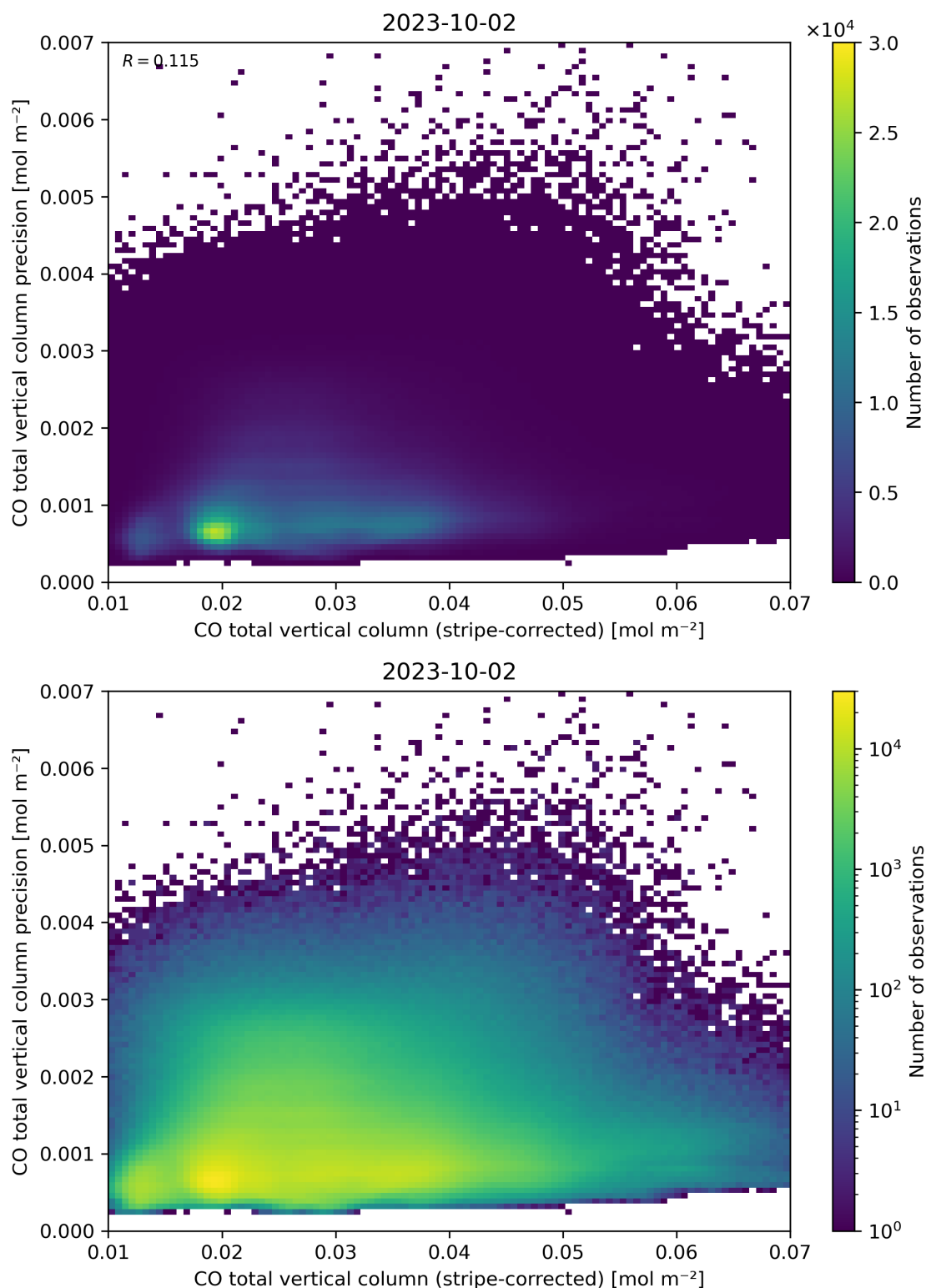
Figure 36: Scatter density plot of “CO total vertical column (stripe-corrected)” against “CO total vertical column precision” for 2023-10-01 to 2023-10-03.
