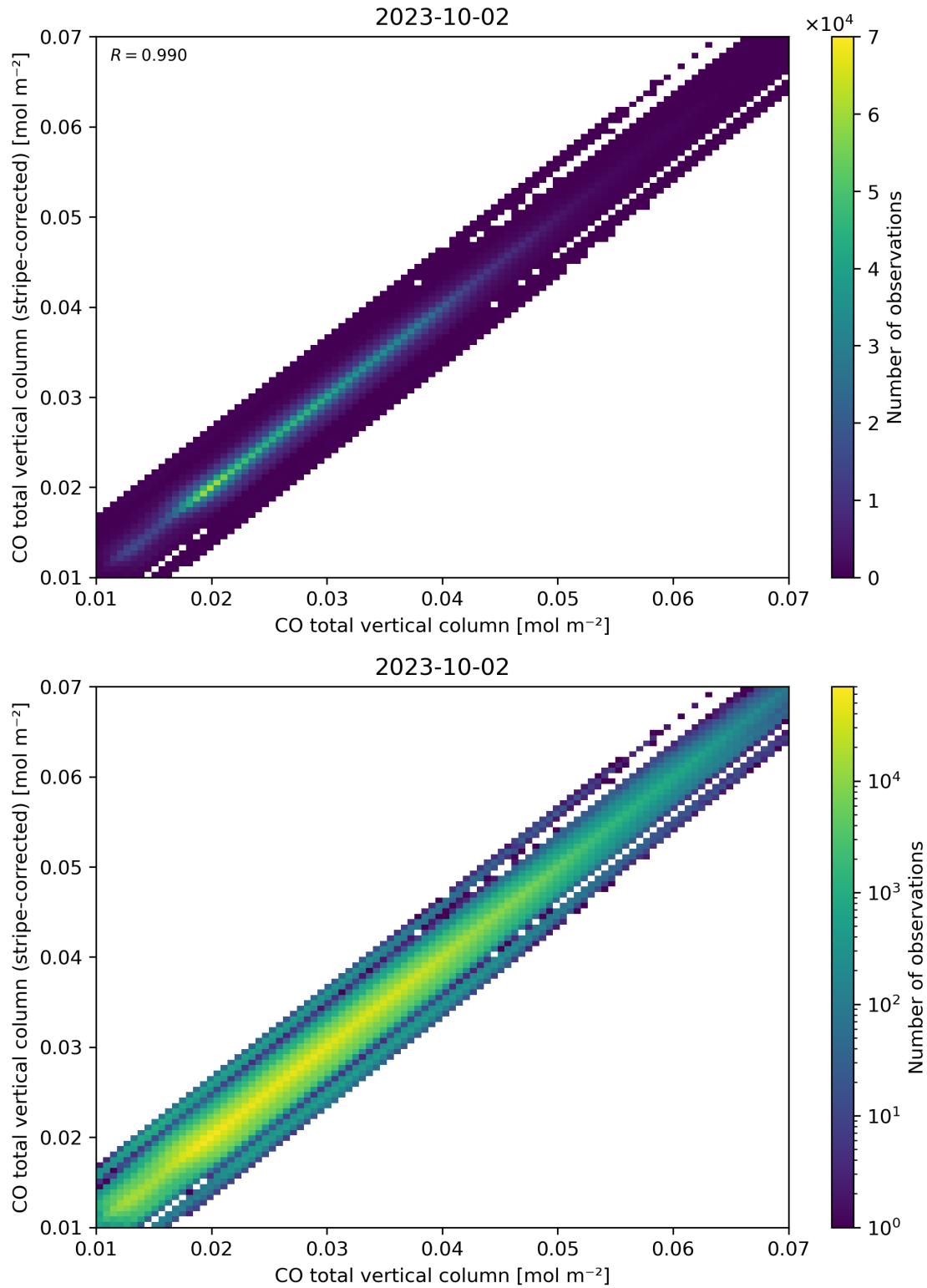
Figure 33: Scatter density plot of “CO total vertical column” against “CO total vertical column (stripe-corrected)” for 2023-10-01 to 2023-10-03.
