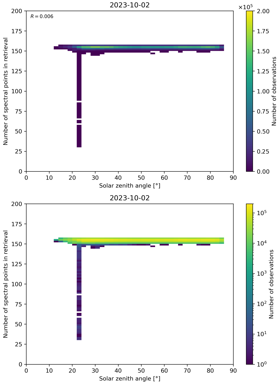
Figure 68: Scatter density plot of “Solar zenith angle” against “Number of spectral points in retrieval” for 2023-10-01 to 2023-10-03.
