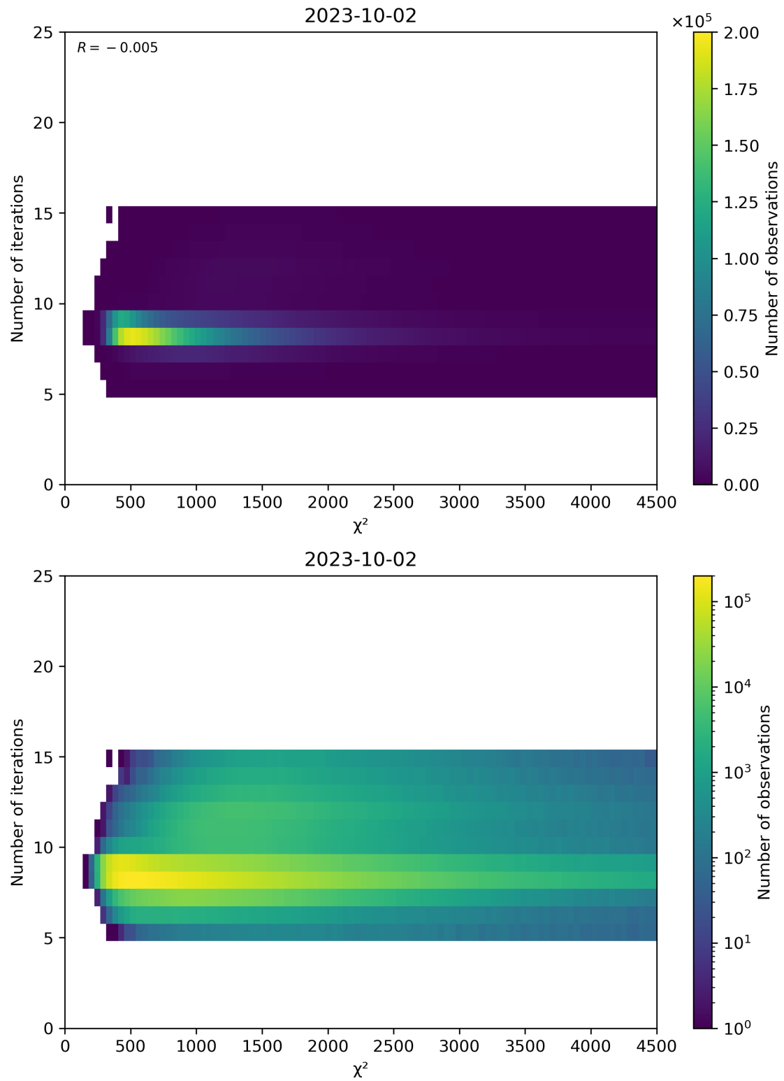
Figure 49: Scatter density plot of “ \chi^2 ” against “Number of iterations” for 2023-10-01 to 2023-10-03.
