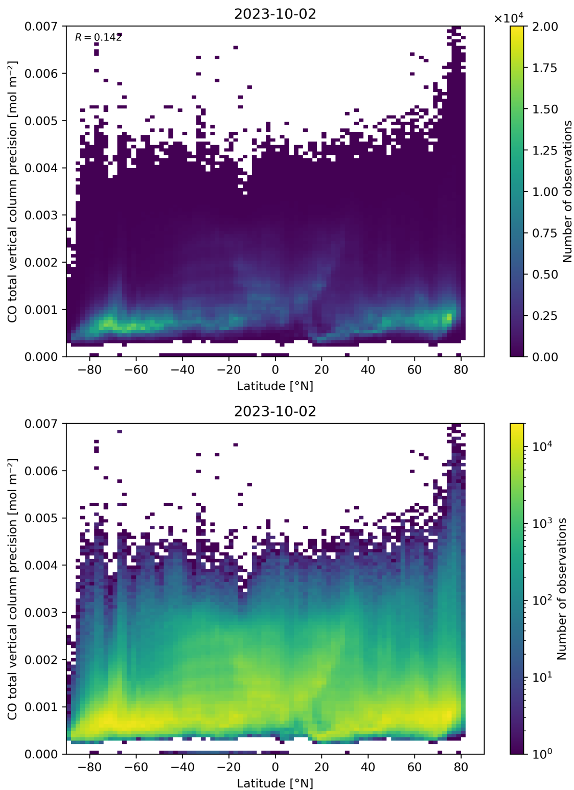
Figure 53: Scatter density plot of “Latitude” against “CO total vertical column precision” for 2023-10-01 to 2023-10-03.
