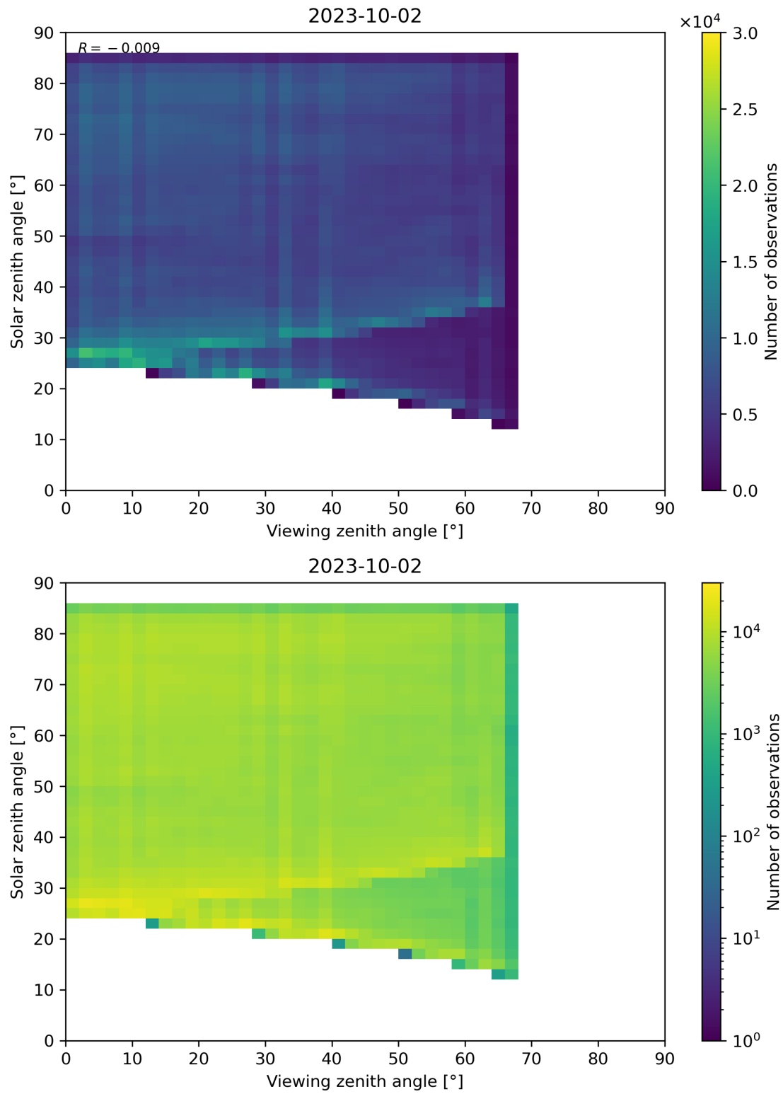
Figure 77: Scatter density plot of “Viewing zenith angle” against “Solar zenith angle” for 2023-10-01 to 2023-10-03.
