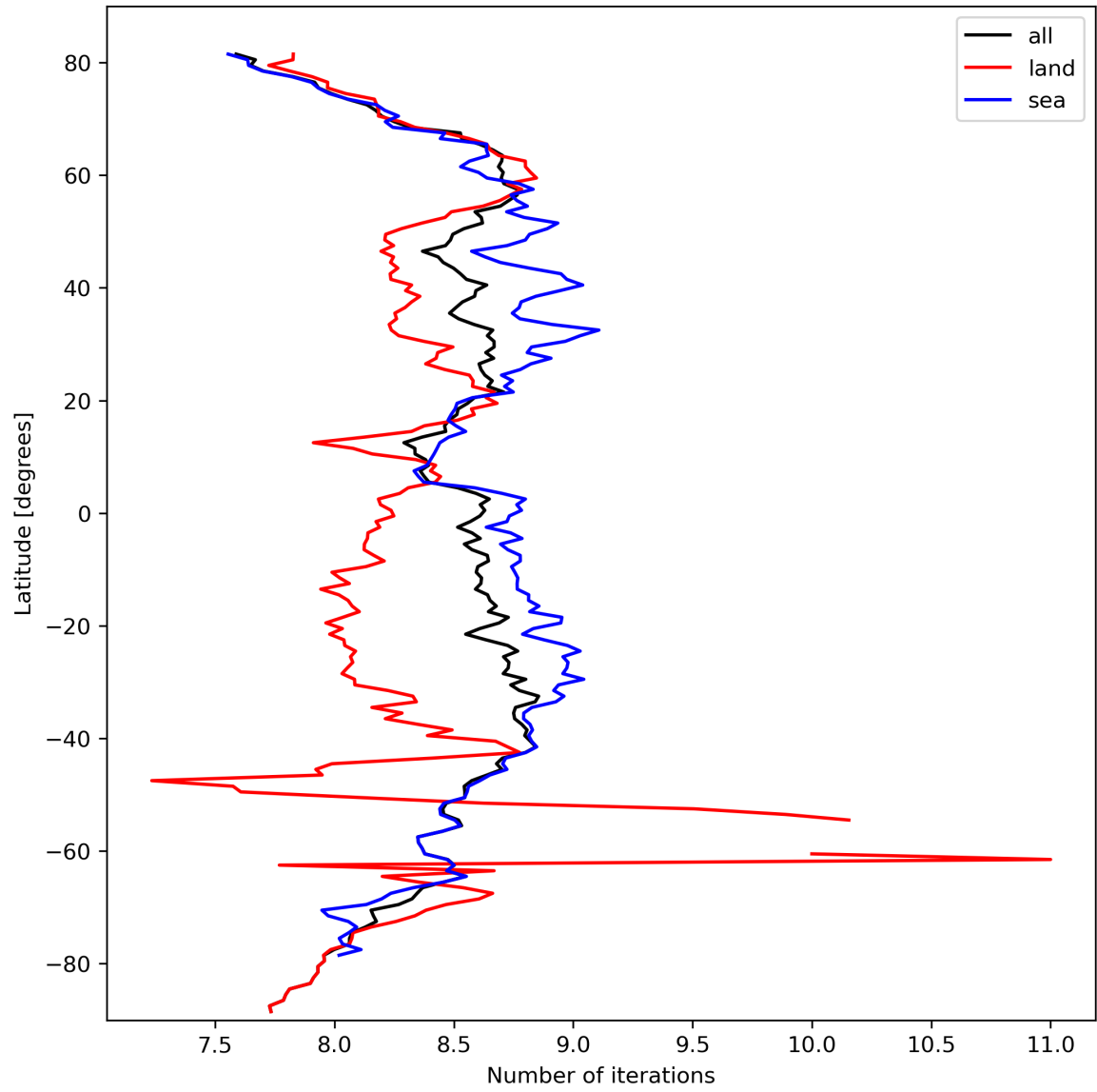
Figure 16: Zonal average of “Number of iterations” for 2023-10-01 to 2023-10-03.
