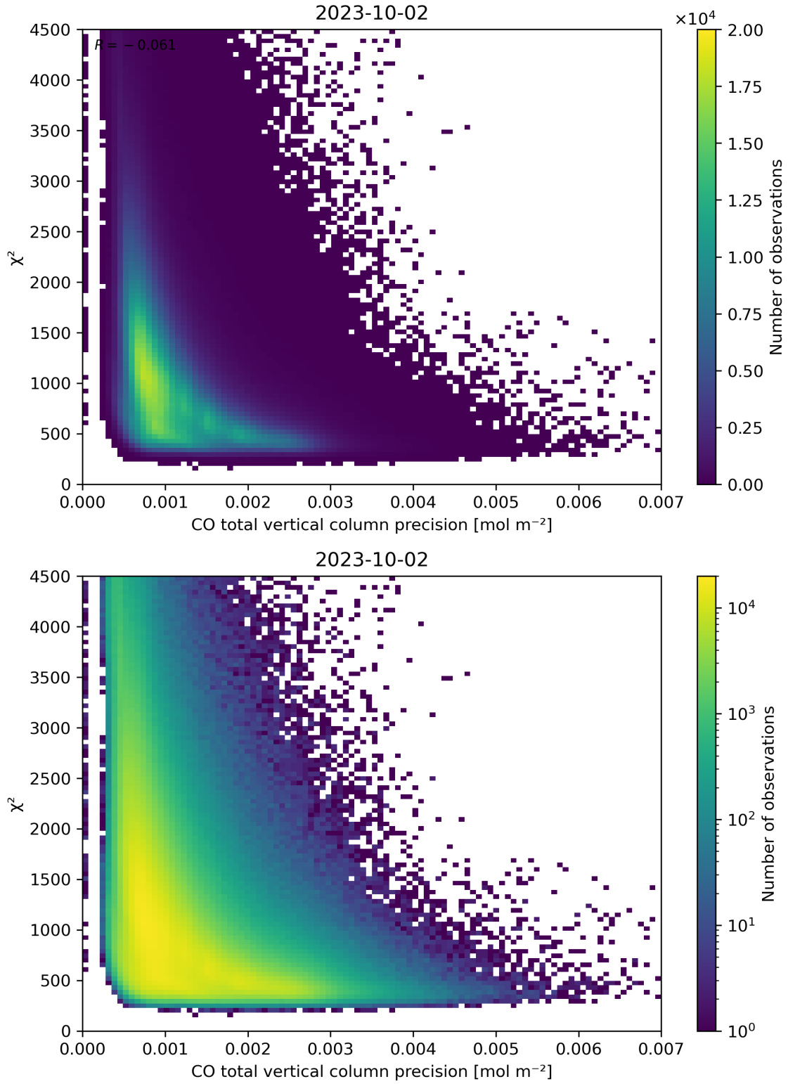
Figure 44: Scatter density plot of “CO total vertical column precision” against “ \chi^2 ” for 2023-10-01 to 2023-10-03.
