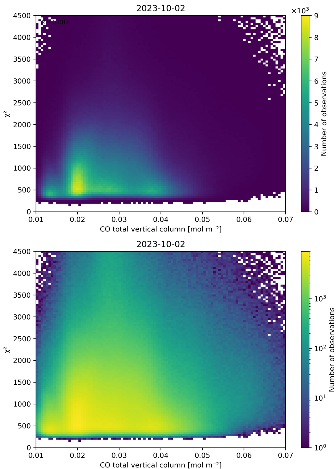
Figure 35: Scatter density plot of “CO total vertical column” against “ \chi^2 ” for 2023-10-01 to 2023-10-03.
