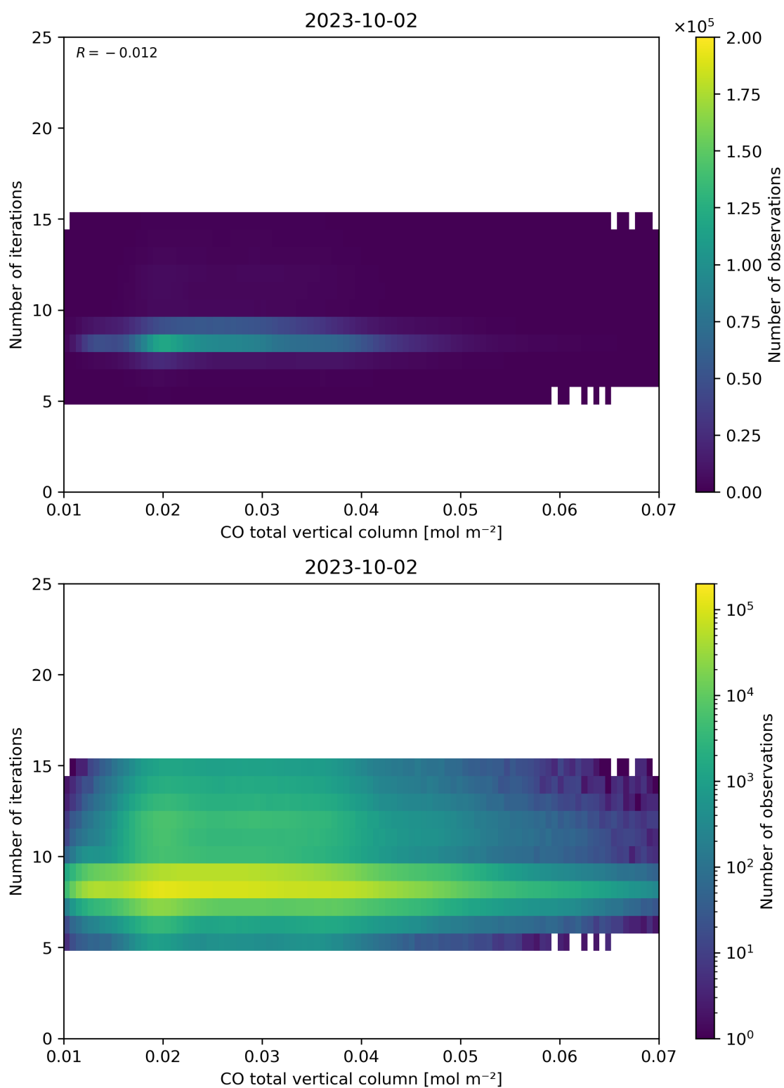
Figure 42: Scatter density plot of “CO total vertical column” against “Number of iterations” for 2023-10-01 to 2023-10-03.
