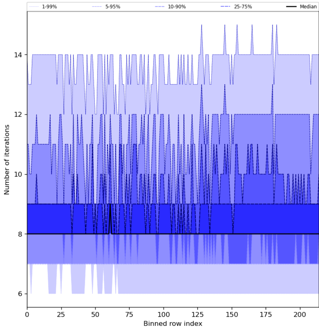
Figure 32: Along track statistics of “Number of iterations” for 2023-10-01 to 2023-10-03
