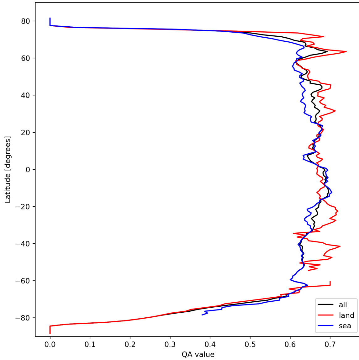
Figure 9: Zonal average of “QA value” for 2023-10-01 to 2023-10-03.
