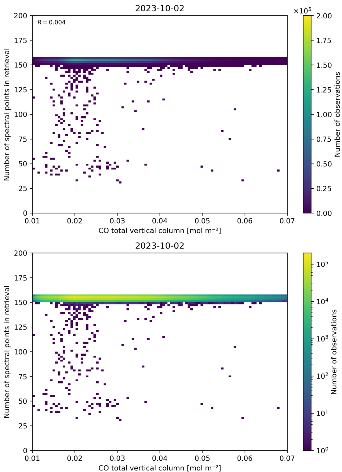
Figure 43: Scatter density plot of “CO total vertical column” against “Number of spectral points in retrieval” for 2023-10-01 to 2023-10-03.
