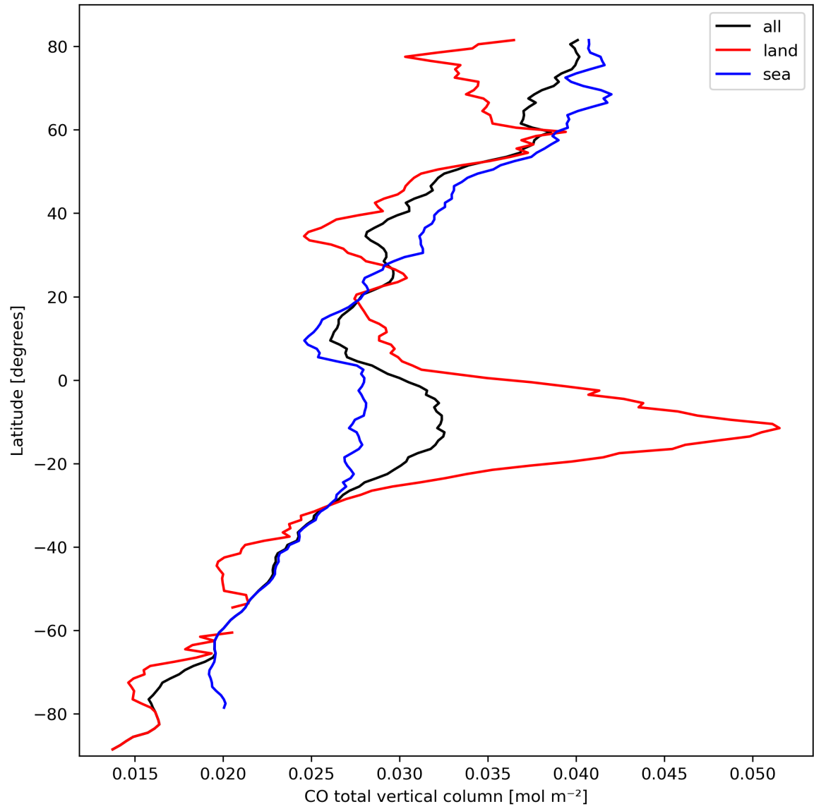
Figure 10: Zonal average of “CO total vertical column” for 2023-10-01 to 2023-10-03.
