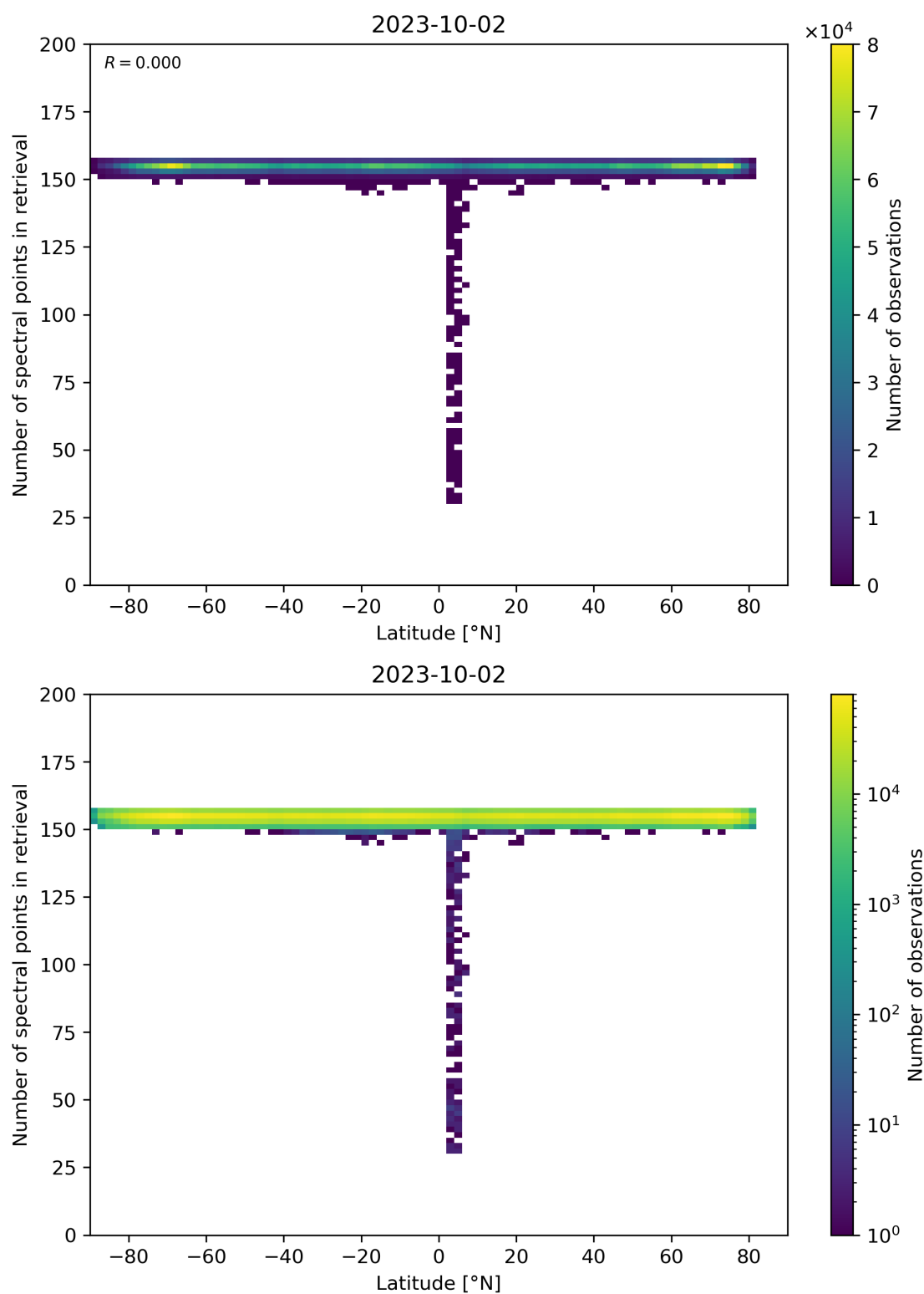
Figure 57: Scatter density plot of “Latitude” against “Number of spectral points in retrieval” for 2023-10-01 to 2023-10-03.
