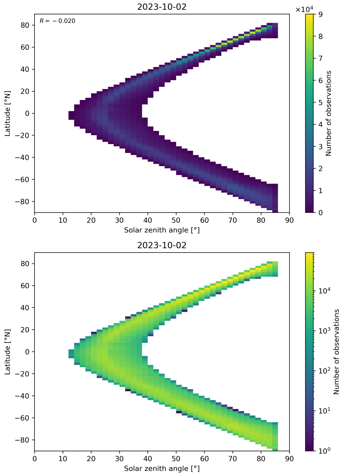
Figure 66: Scatter density plot of “Solar zenith angle” against “Latitude” for 2023-10-01 to 2023-10-03.
