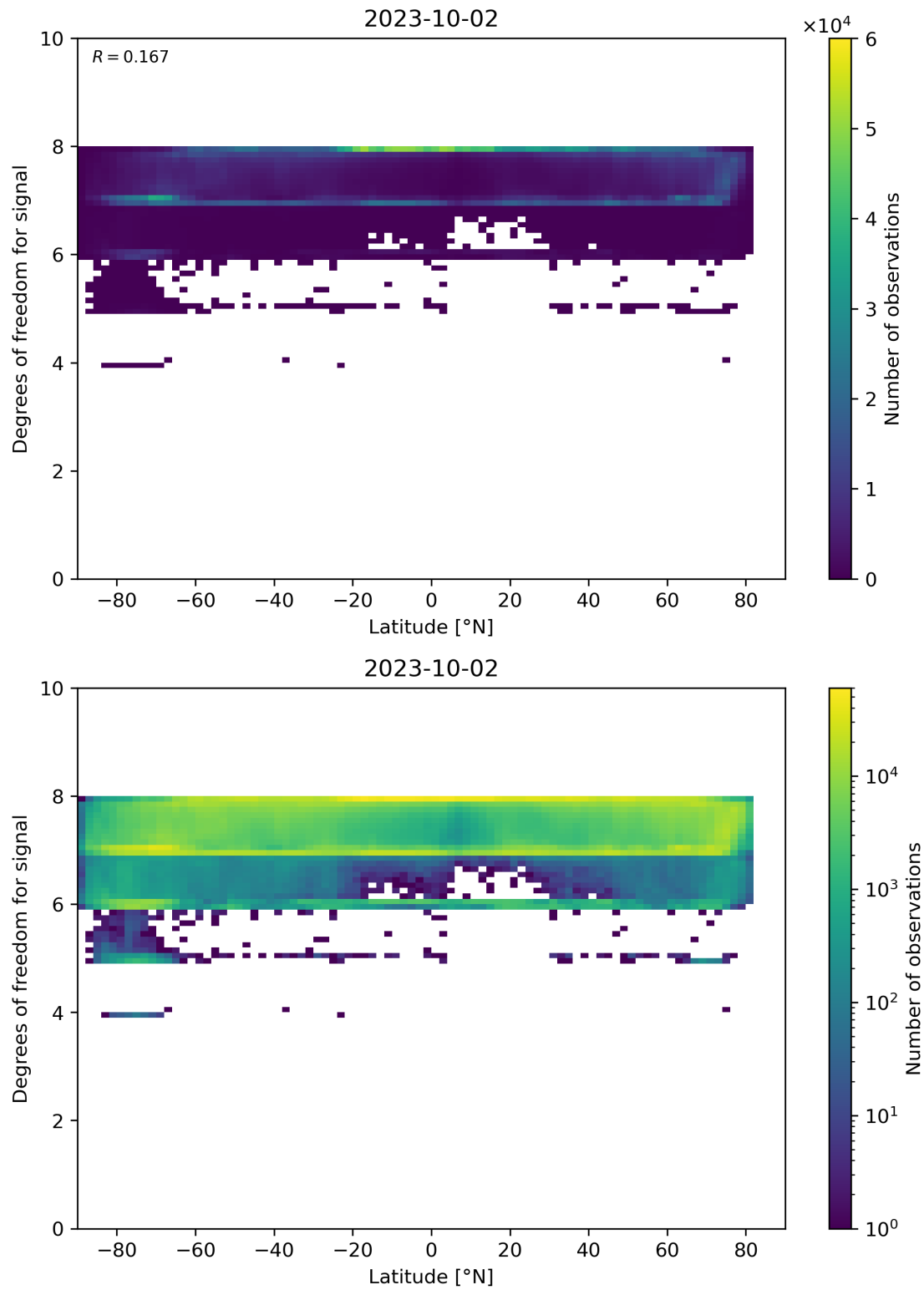
Figure 55: Scatter density plot of “Latitude” against “Degrees of freedom for signal” for 2023-10-01 to 2023-10-03.
