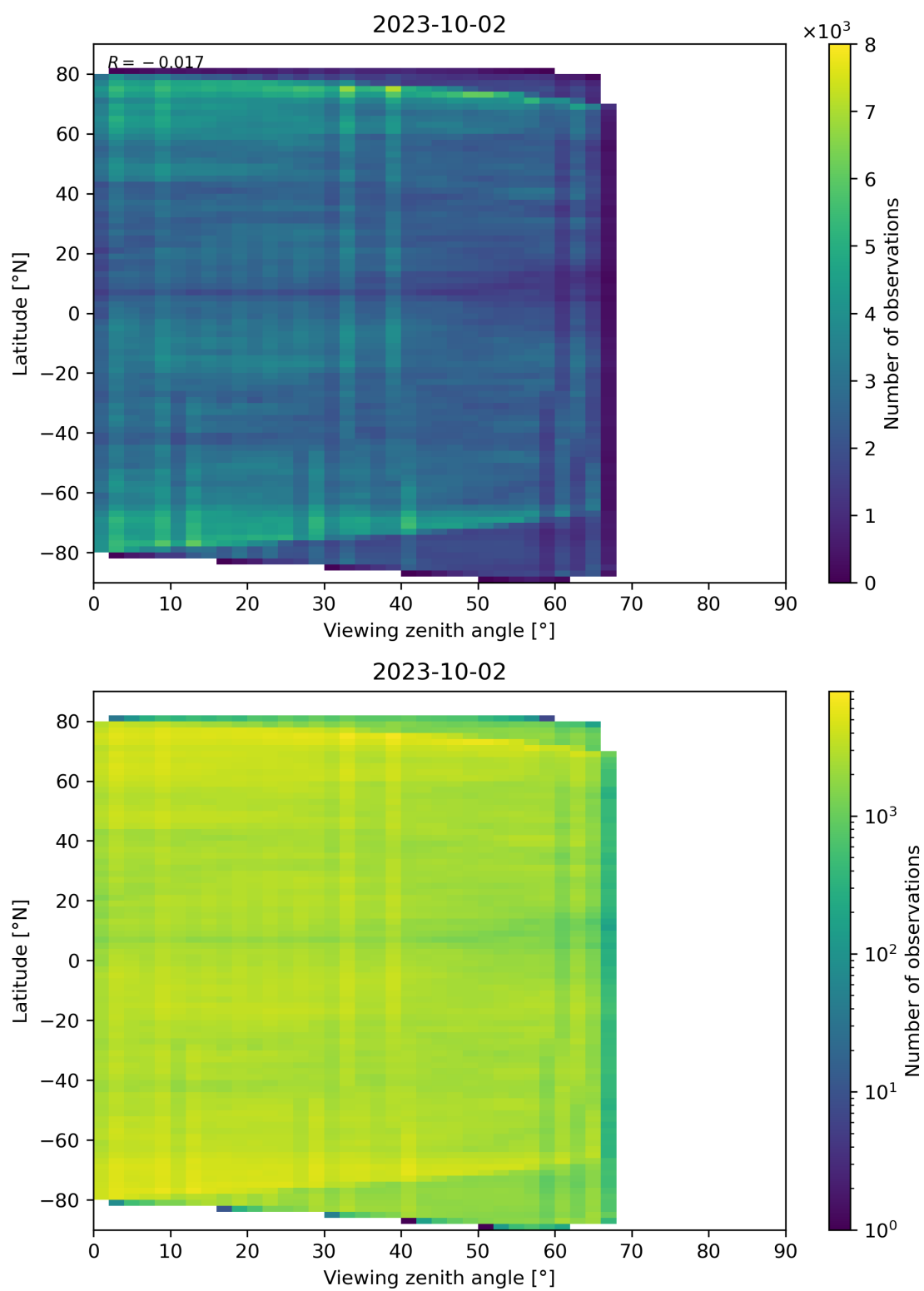
Figure 74: Scatter density plot of “Viewing zenith angle” against “Latitude” for 2023-10-01 to 2023-10-03.
