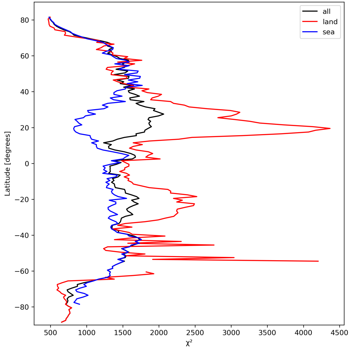
Figure 14: Zonal average of “ \chi^2 ” for 2023-10-01 to 2023-10-03.
