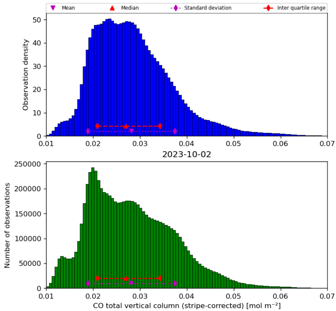
Figure 19: Histogram of “CO total vertical column (stripe-corrected)” for 2023-10-01 to 2023-10-03
