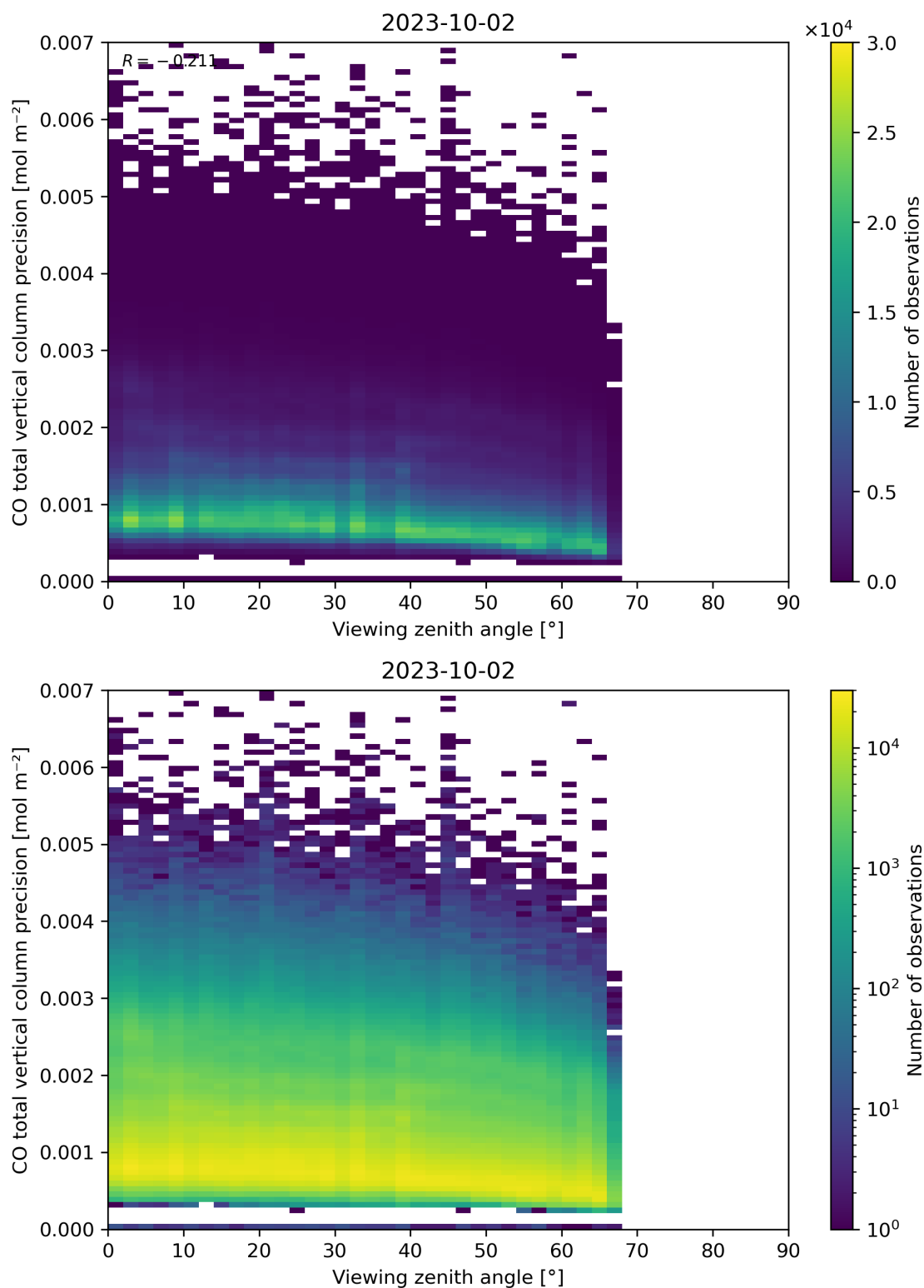
Figure 71: Scatter density plot of “Viewing zenith angle” against “CO total vertical column precision” for 2023-10-01 to 2023-10-03.
