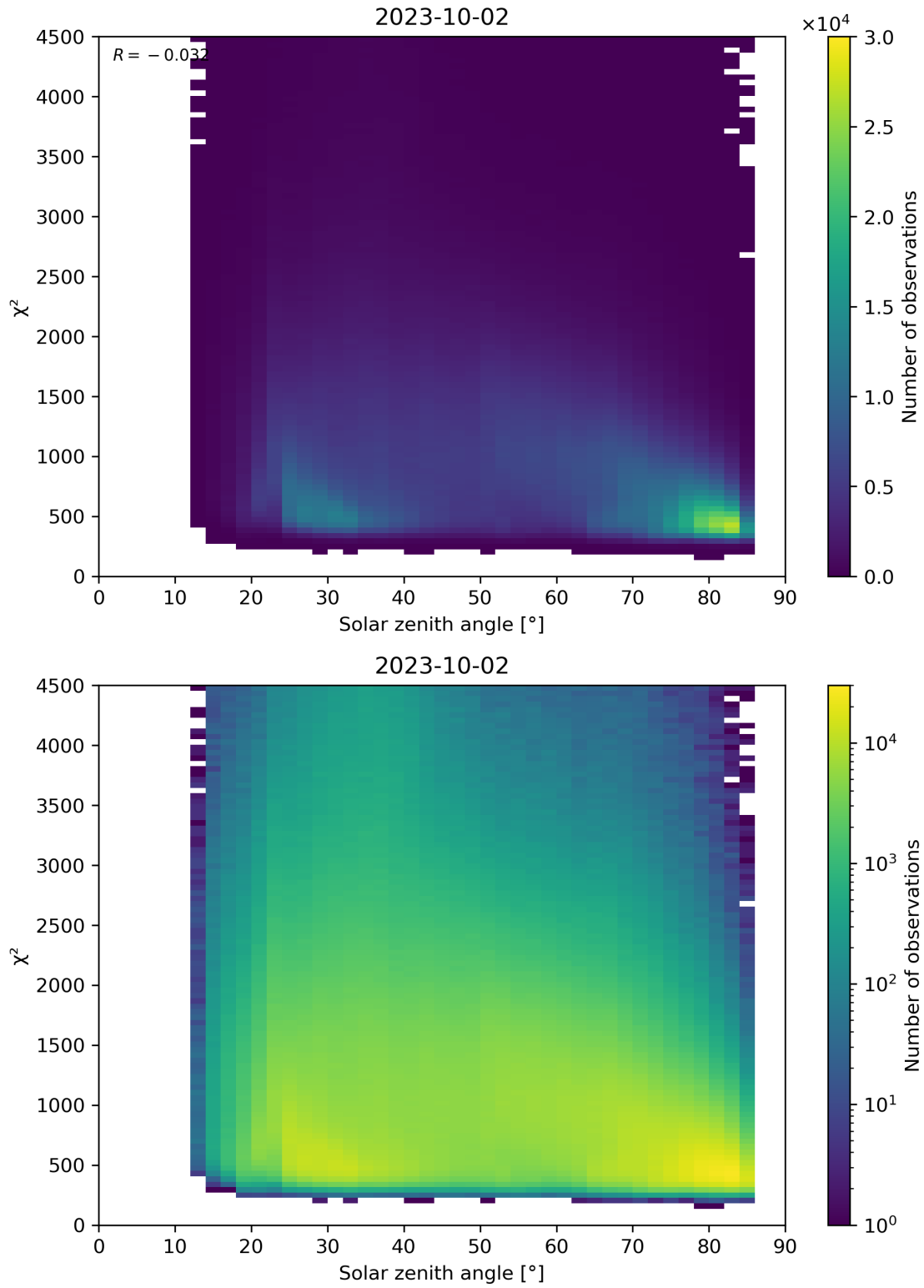
Figure 64: Scatter density plot of “Solar zenith angle” against “ \chi^2 ” for 2023-10-01 to 2023-10-03.
