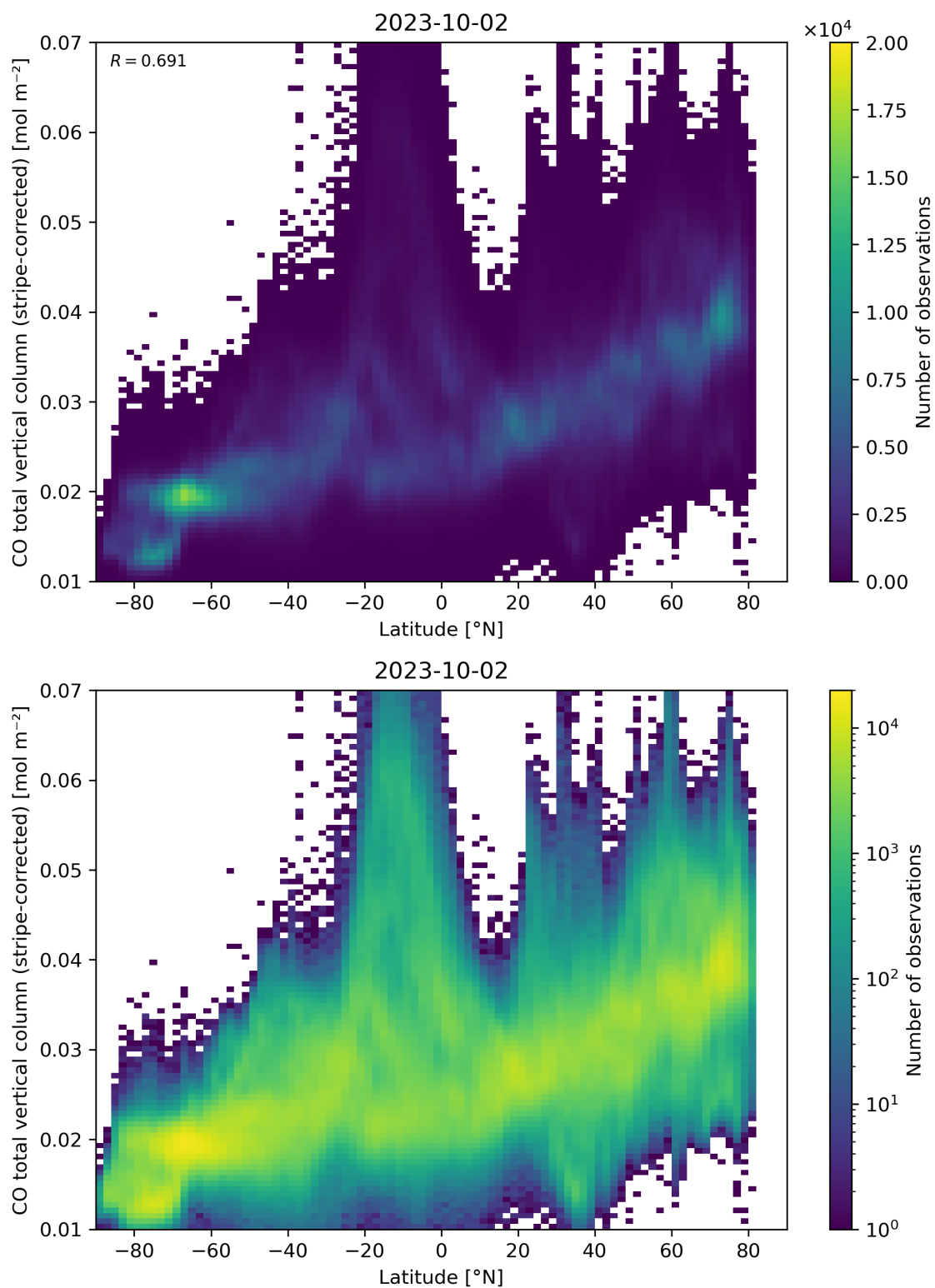
Figure 52: Scatter density plot of “Latitude” against “CO total vertical column (stripe-corrected)” for 2023-10-01 to 2023-10-03.
