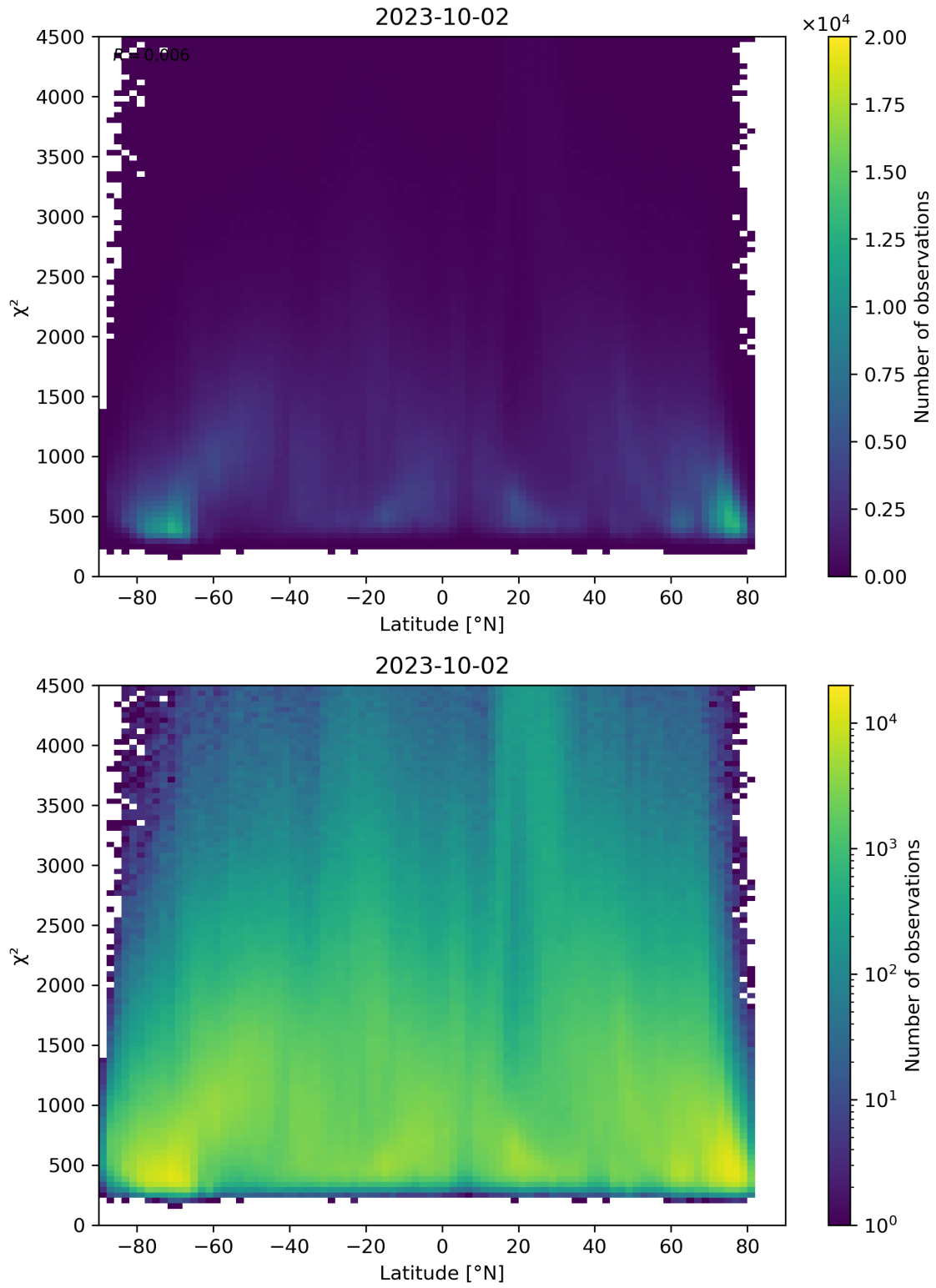
Figure 54: Scatter density plot of “Latitude” against “ \chi^2 ” for 2023-10-01 to 2023-10-03.
