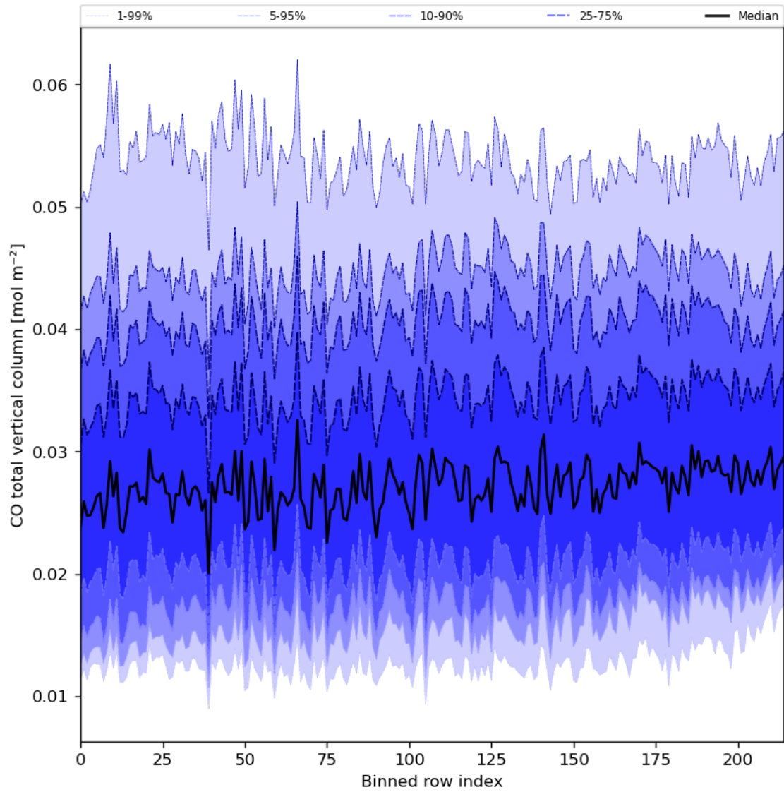
Figure 26: Along track statistics of “CO total vertical column” for 2023-10-01 to 2023-10-03
