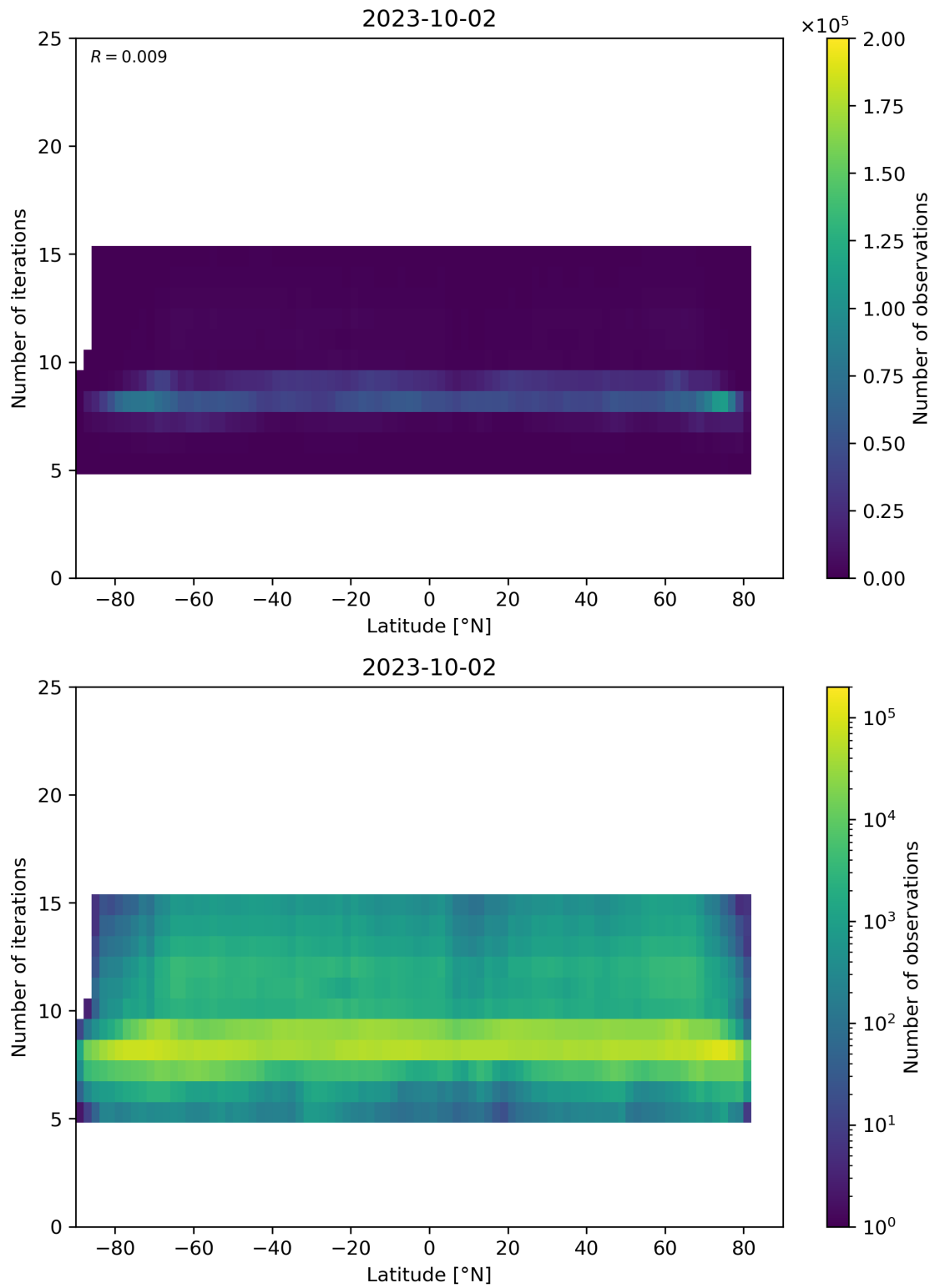
Figure 56: Scatter density plot of “Latitude” against “Number of iterations” for 2023-10-01 to 2023-10-03.
