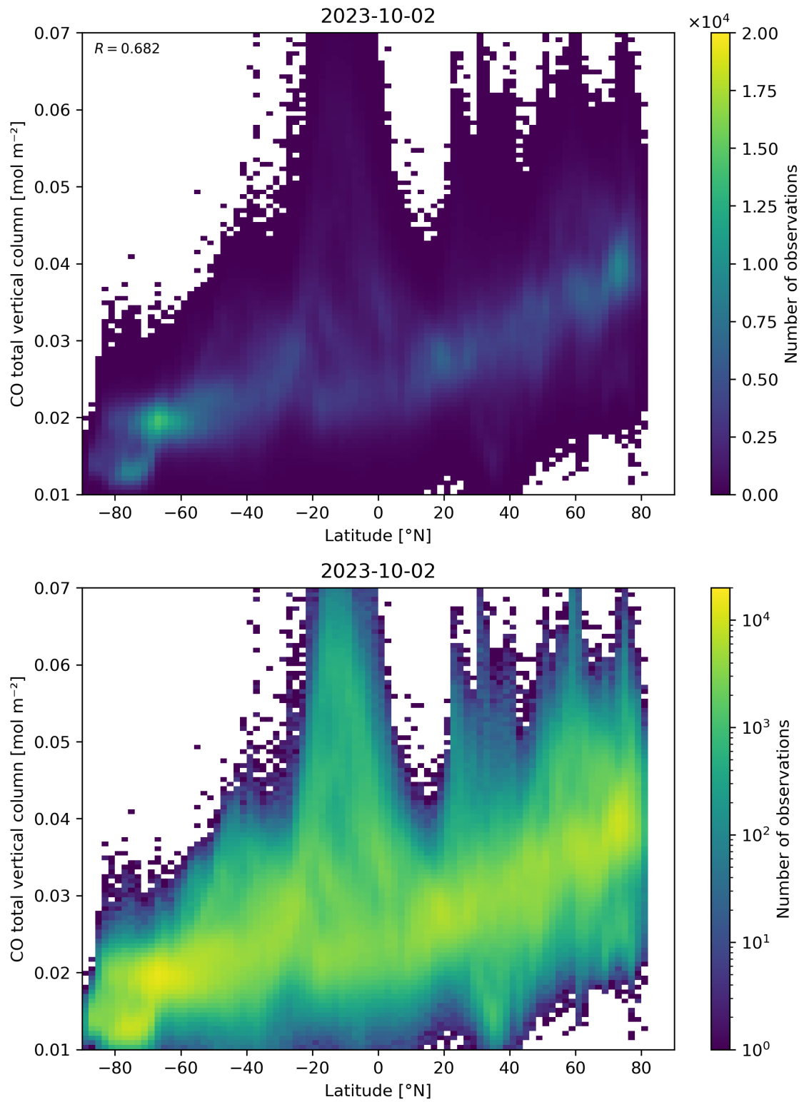
Figure 51: Scatter density plot of “Latitude” against “CO total vertical column” for 2023-10-01 to 2023-10-03.
