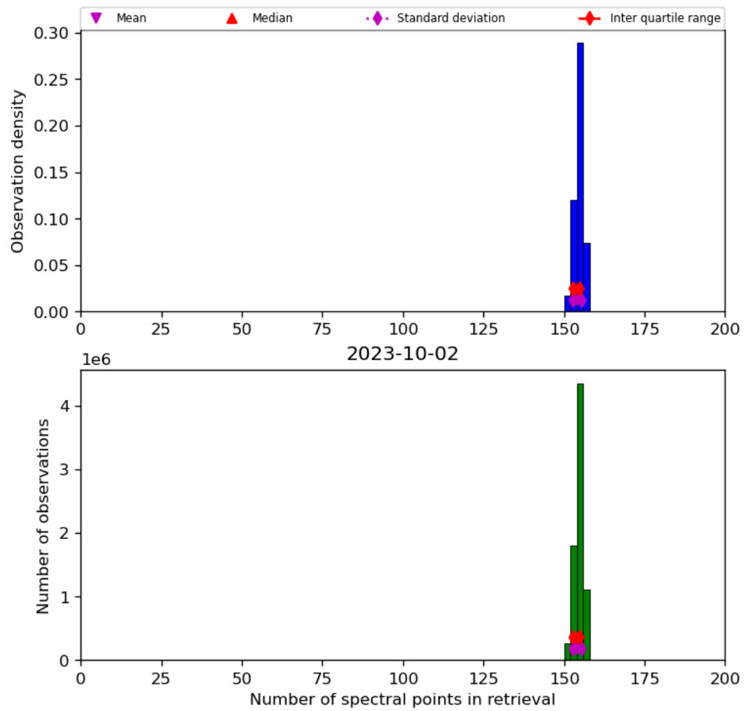
Figure 21: Histogram of “Number of spectral points in retrieval” for 2023-10-01 to 2023-10-03
