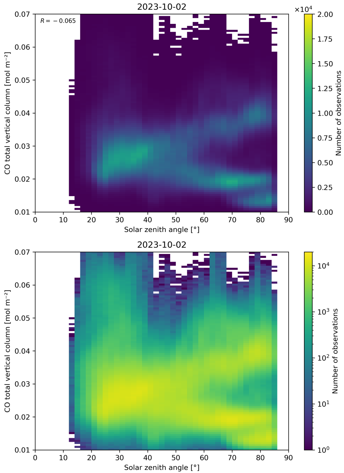
Figure 61: Scatter density plot of “Solar zenith angle” against “CO total vertical column” for 2023-10-01 to 2023-10-03.
