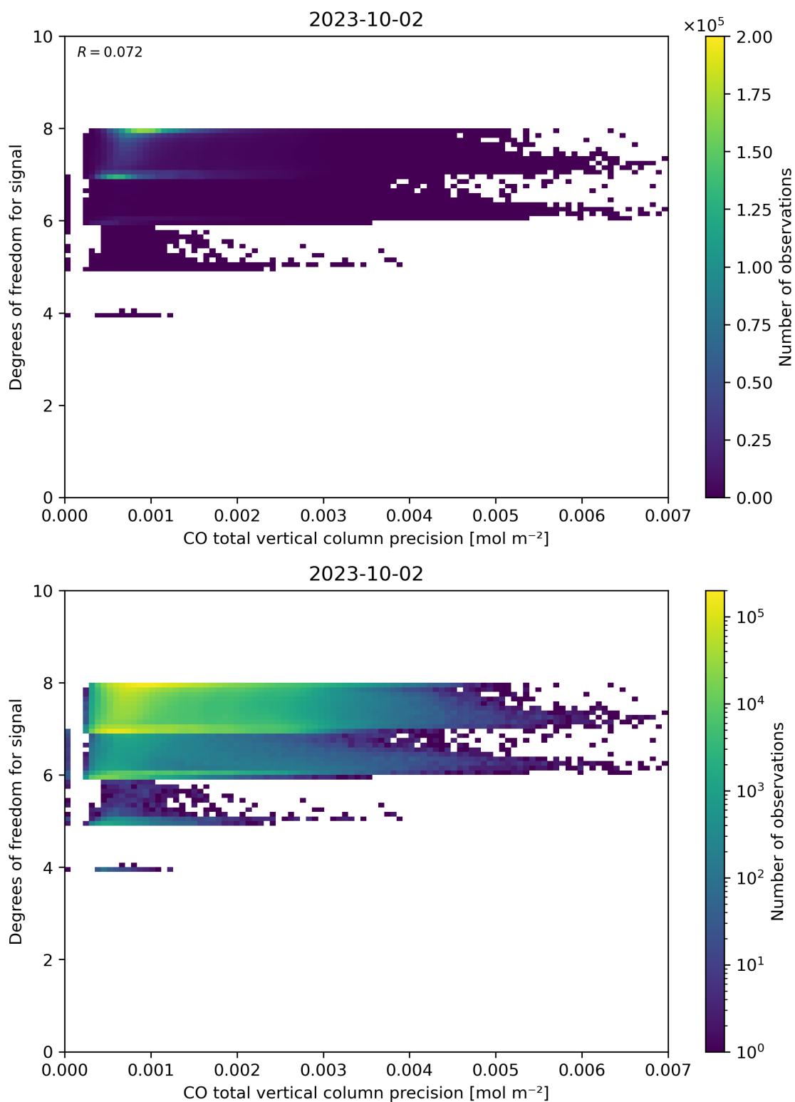
Figure 45: Scatter density plot of “CO total vertical column precision” against “Degrees of freedom for signal” for 2023-10-01 to 2023-10-03.
