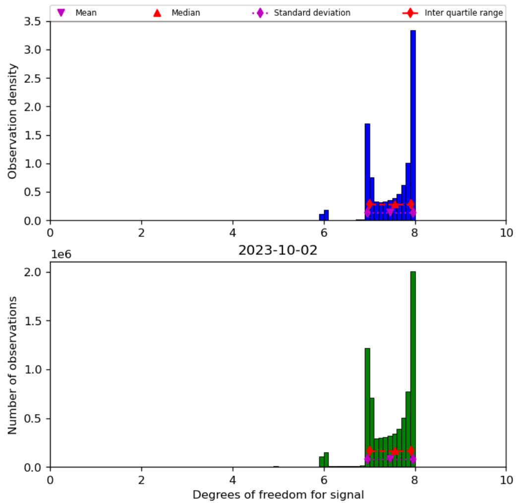
Figure 23: Histogram of “Degrees of freedom for signal” for 2023-10-01 to 2023-10-03
