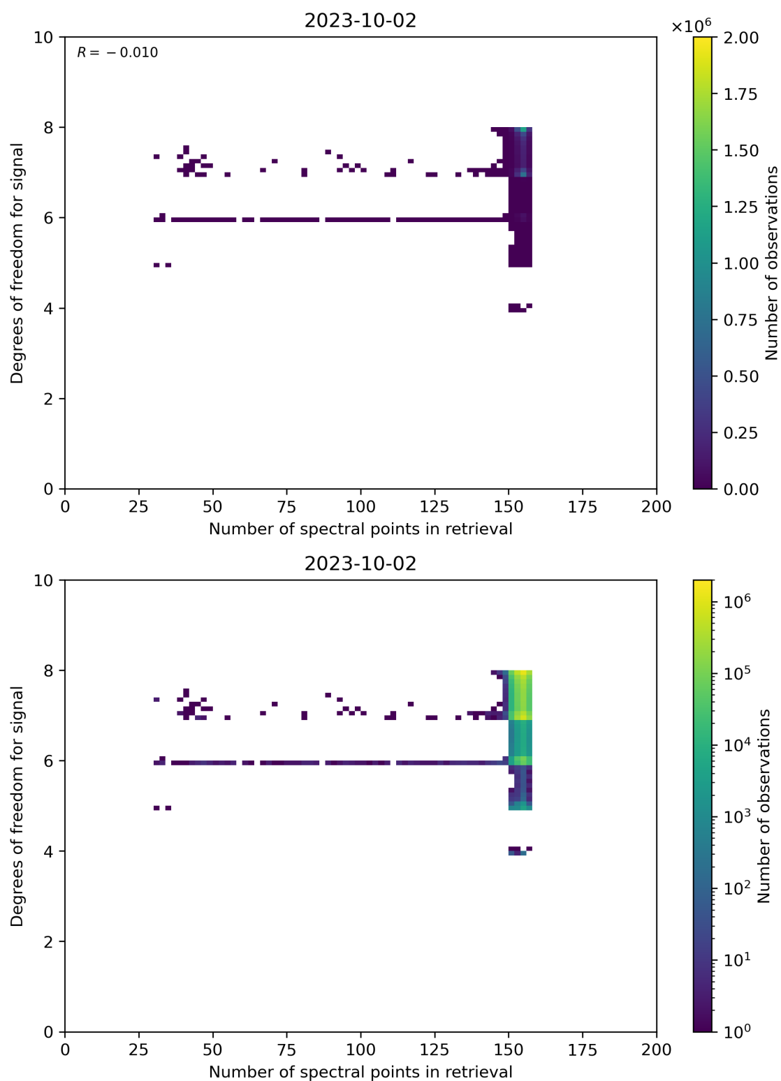
Figure 59: Scatter density plot of “Number of spectral points in retrieval” against “Degrees of freedom for signal” for 2023-10-01 to 2023-10-03.
