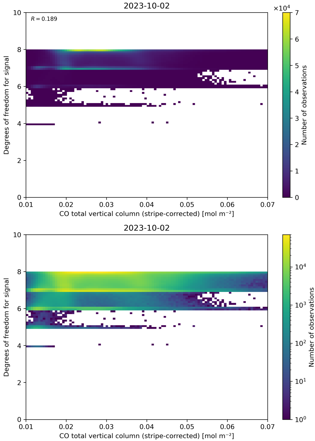
Figure 38: Scatter density plot of “CO total vertical column (stripe-corrected)” against “Degrees of freedom for signal” for 2023-10-01 to 2023-10-03.
