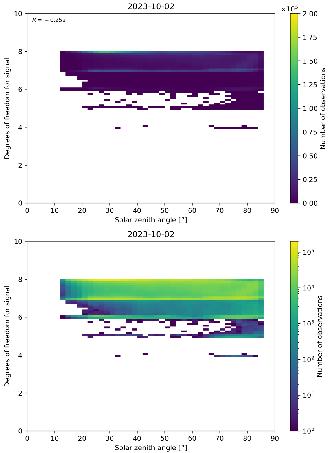
Figure 65: Scatter density plot of “Solar zenith angle” against “Degrees of freedom for signal” for 2023-10-01 to 2023-10-03.
