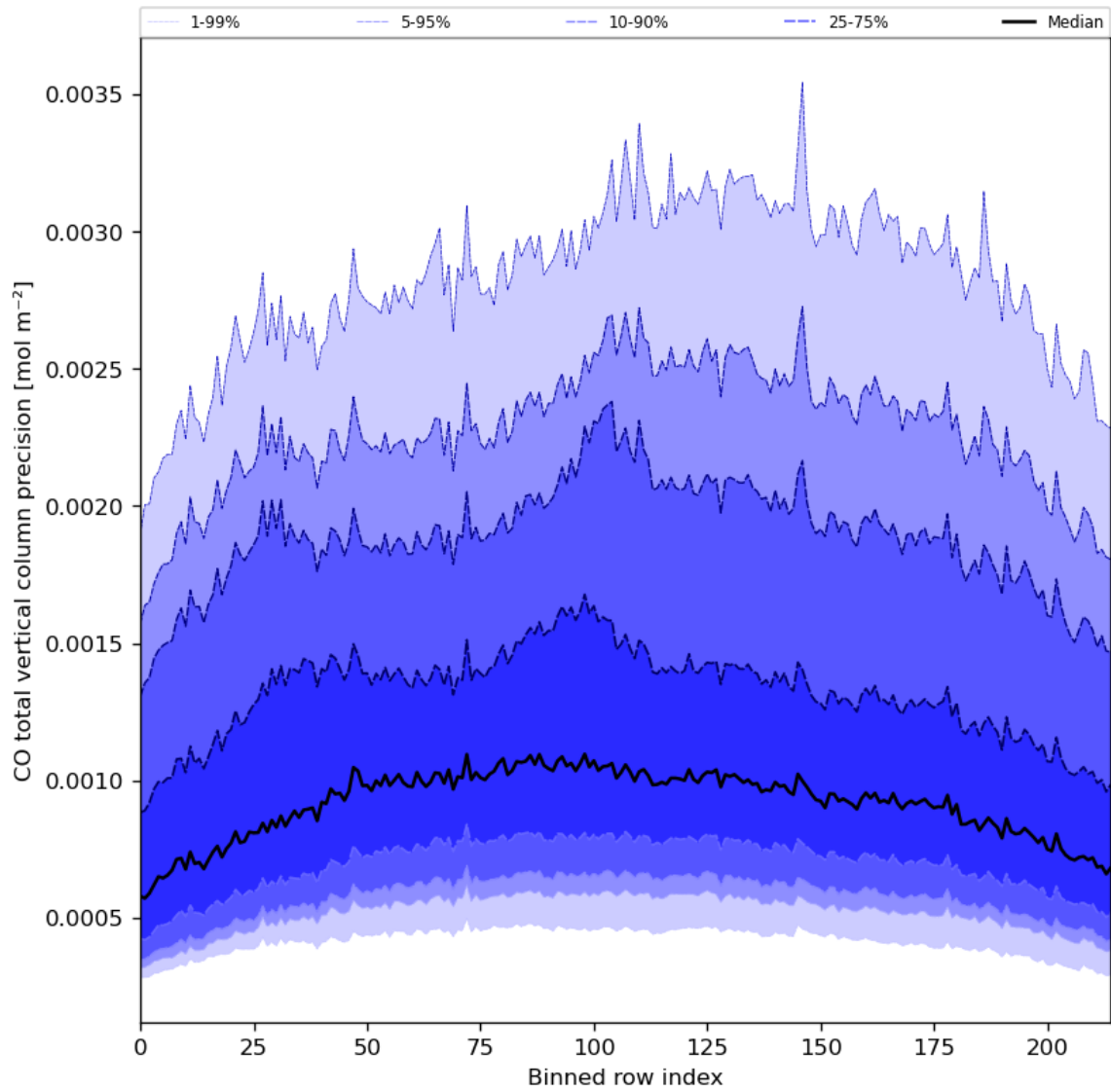
Figure 28: Along track statistics of “CO total vertical column precision” for 2023-10-01 to 2023-10-03
