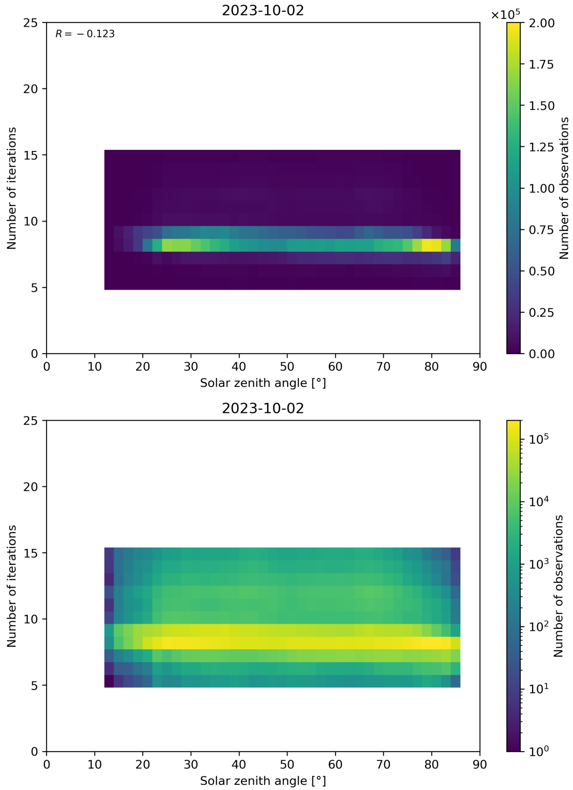
Figure 67: Scatter density plot of “Solar zenith angle” against “Number of iterations” for 2023-10-01 to 2023-10-03.
