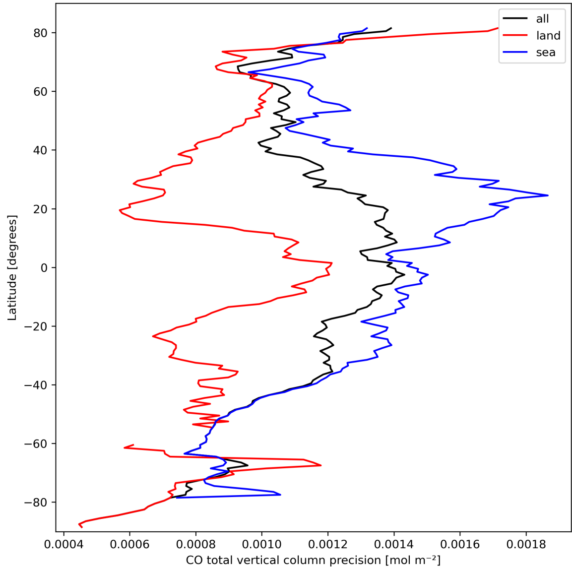
Figure 12: Zonal average of “CO total vertical column precision” for 2023-10-01 to 2023-10-03.
