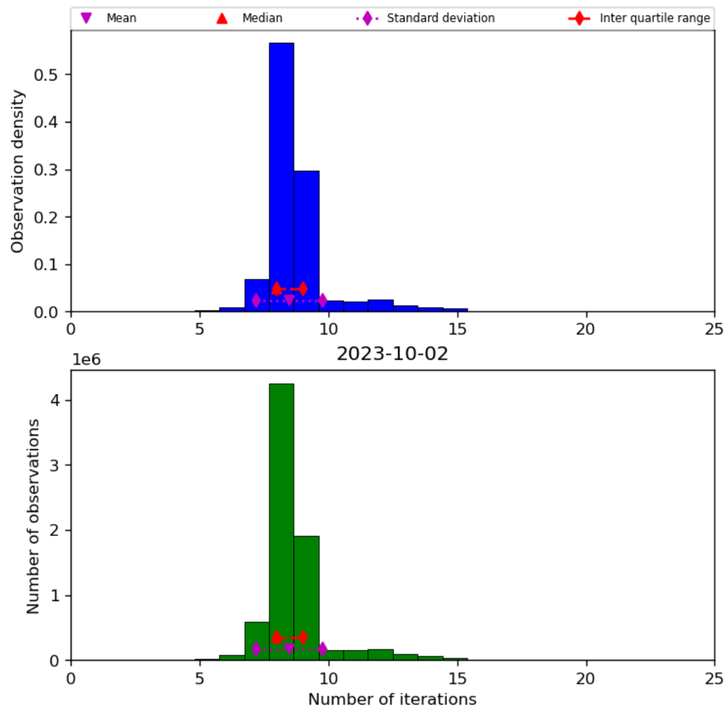
Figure 24: Histogram of “Number of iterations” for 2023-10-01 to 2023-10-03
