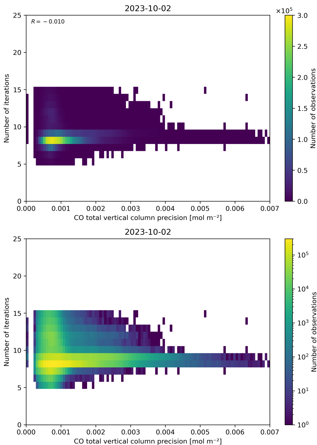
Figure 46: Scatter density plot of “CO total vertical column precision” against “Number of iterations” for 2023-10-01 to 2023-10-03.
