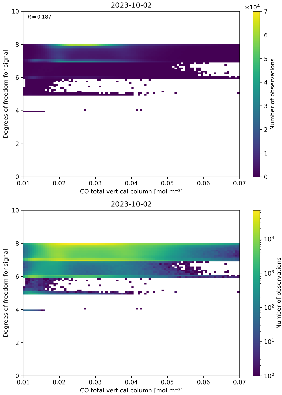
Figure 41: Scatter density plot of “CO total vertical column” against “Degrees of freedom for signal” for 2023-10-01 to 2023-10-03.
