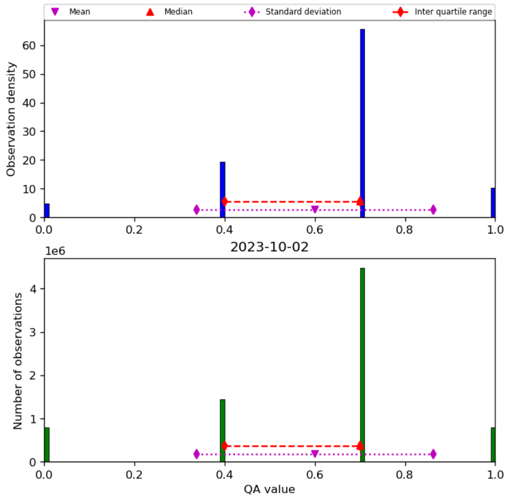
Figure 17: Histogram of “QA value” for 2023-10-01 to 2023-10-03
