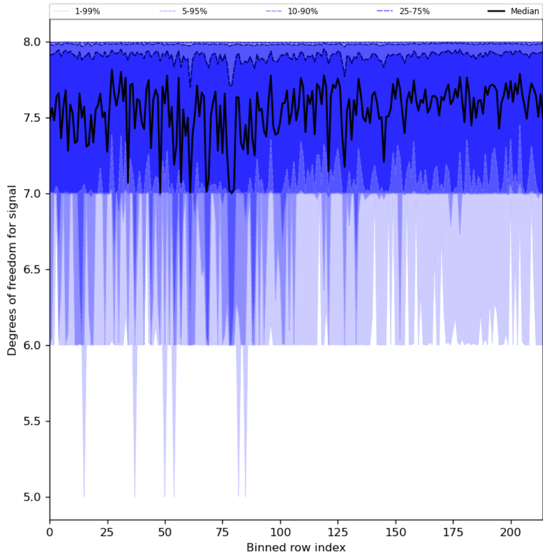
Figure 31: Along track statistics of “Degrees of freedom for signal” for 2023-10-01 to 2023-10-03
