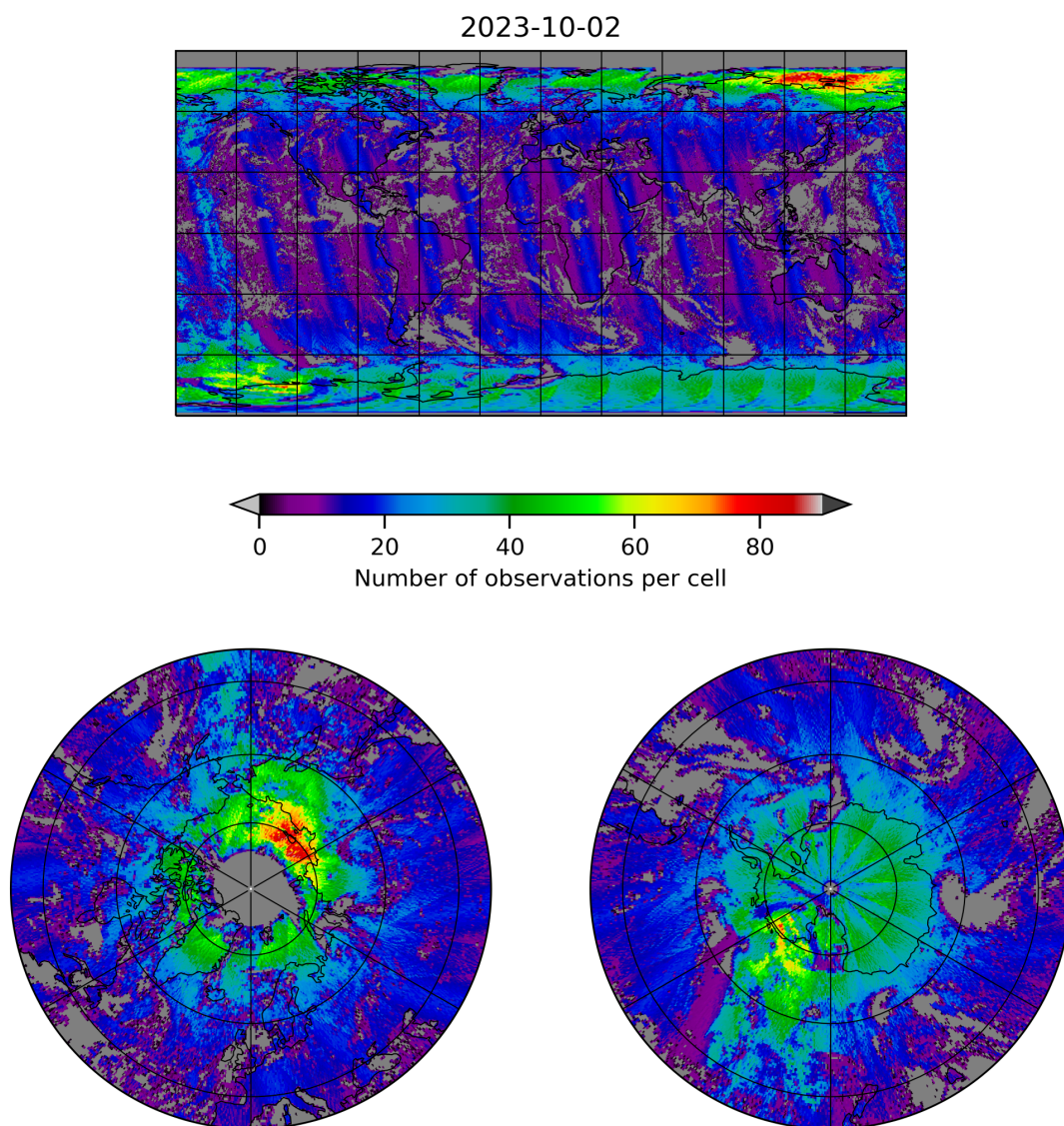
Figure 8: Map of the number of observations for 2023-10-01 to 2023-10-03
