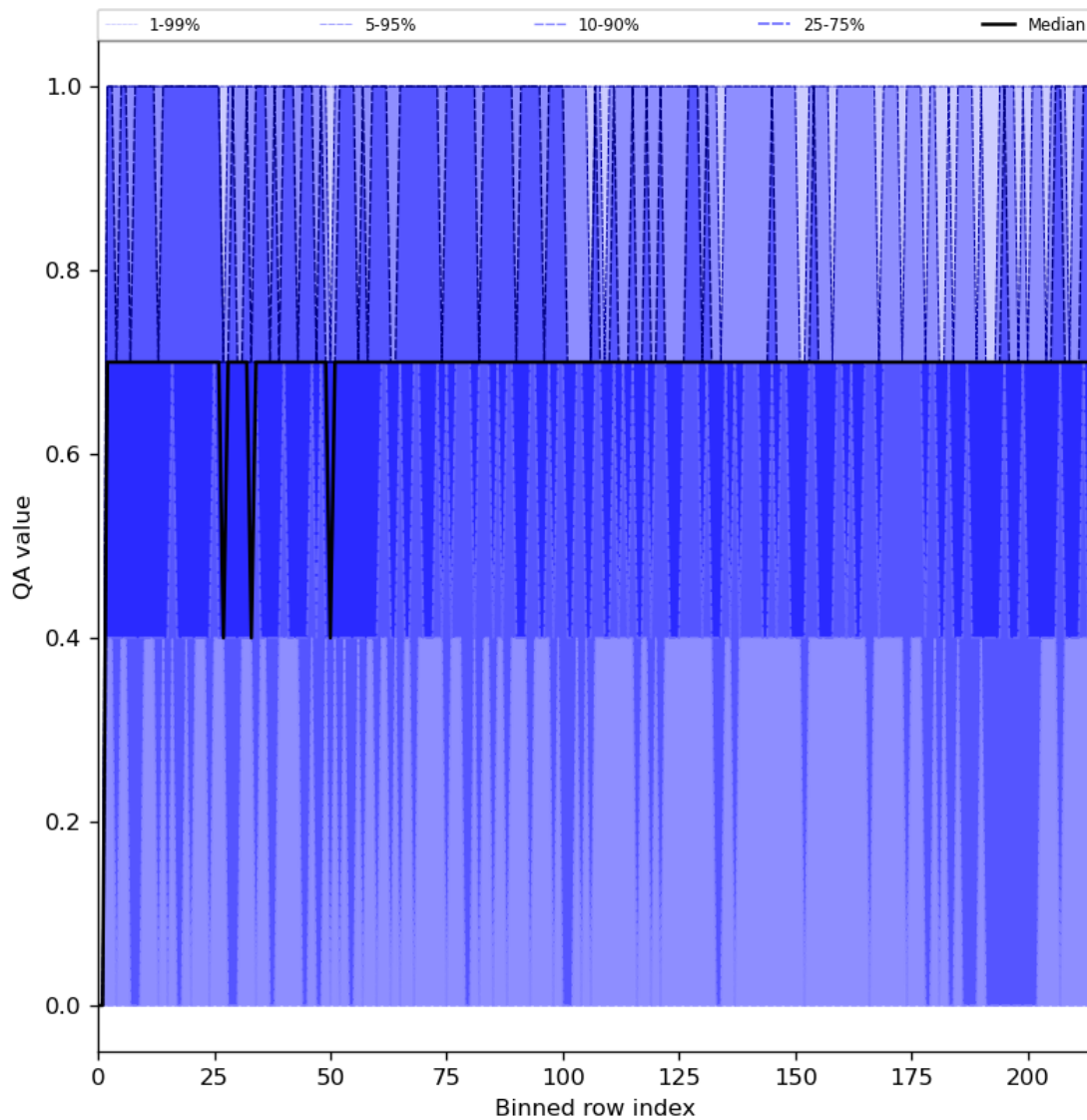
Figure 25: Along track statistics of “QA value” for 2023-10-01 to 2023-10-03
