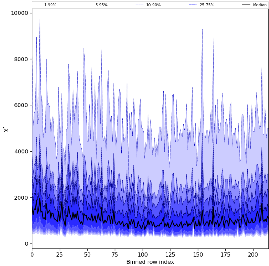
Figure 30: Along track statistics of “ \chi^2 ” for 2023-10-01 to 2023-10-03
