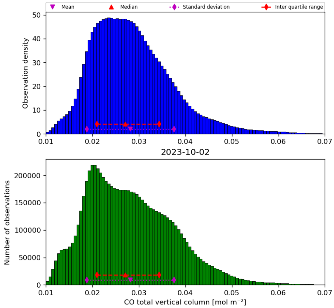
Figure 18: Histogram of “CO total vertical column” for 2023-10-01 to 2023-10-03
