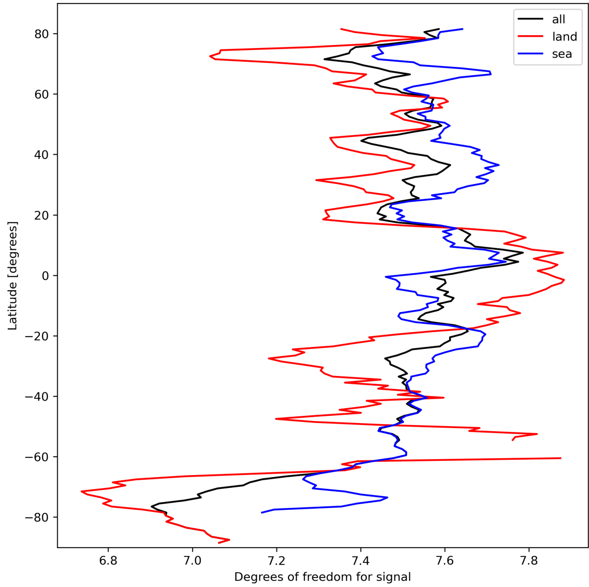
Figure 15: Zonal average of “Degrees of freedom for signal” for 2023-10-01 to 2023-10-03.
