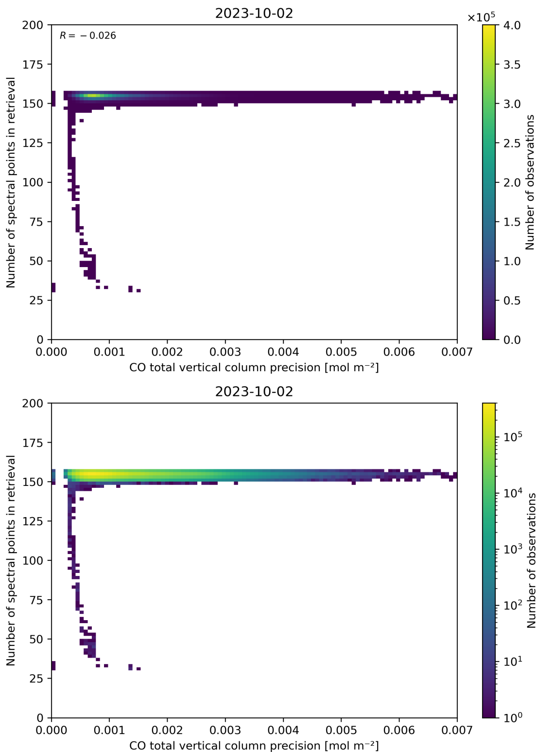
Figure 47: Scatter density plot of “CO total vertical column precision” against “Number of spectral points in retrieval” for 2023-10-01 to 2023-10-03.
