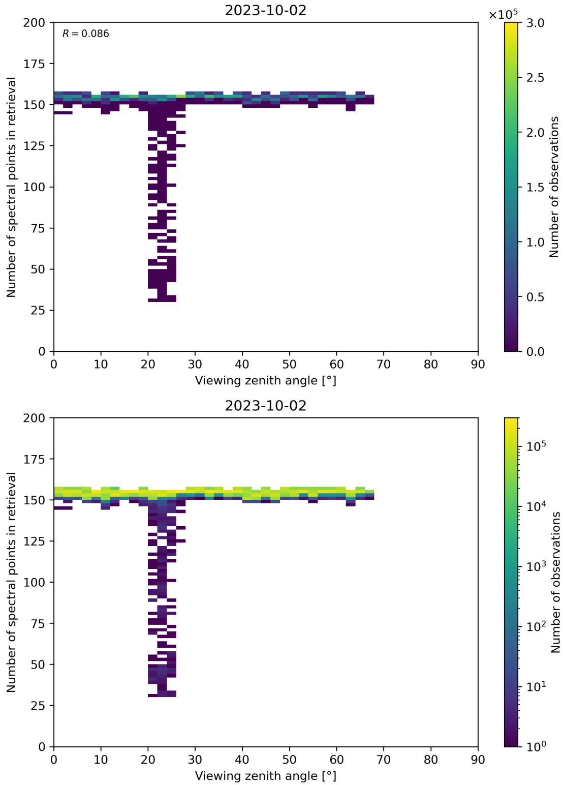
Figure 76: Scatter density plot of “Viewing zenith angle” against “Number of spectral points in retrieval” for 2023-10-01 to 2023-10-03.
