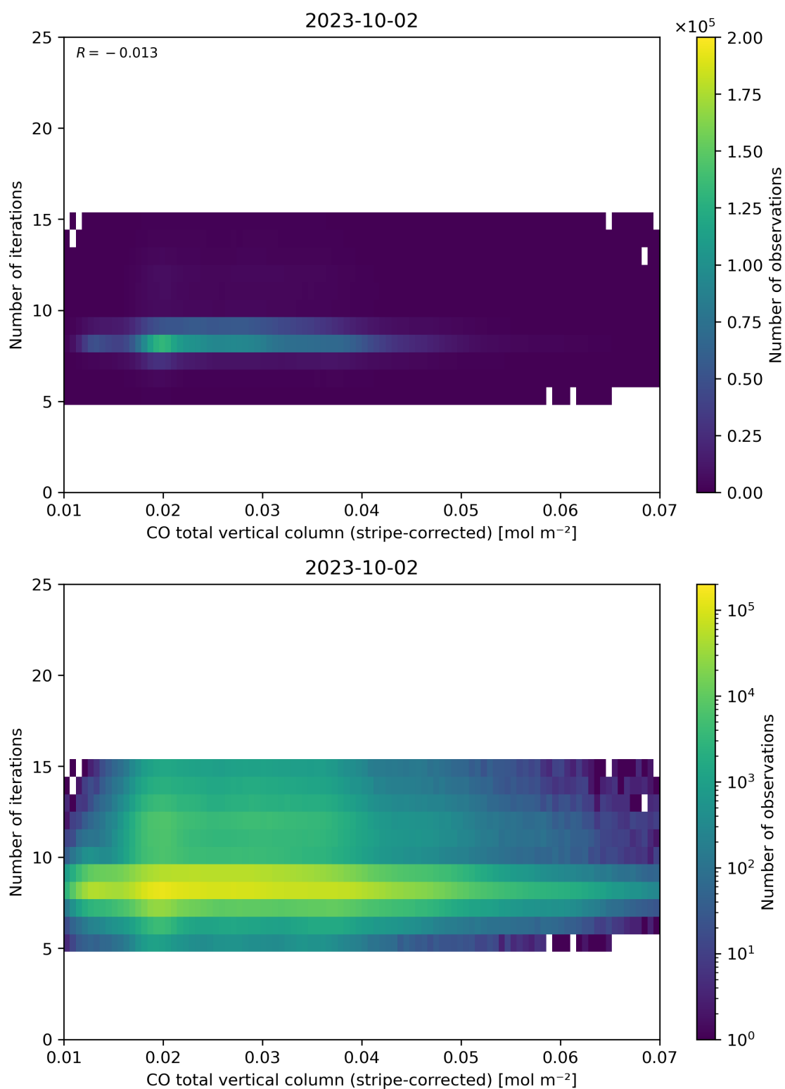
Figure 39: Scatter density plot of “CO total vertical column (stripe-corrected)” against “Number of iterations” for 2023-10-01 to 2023-10-03.
