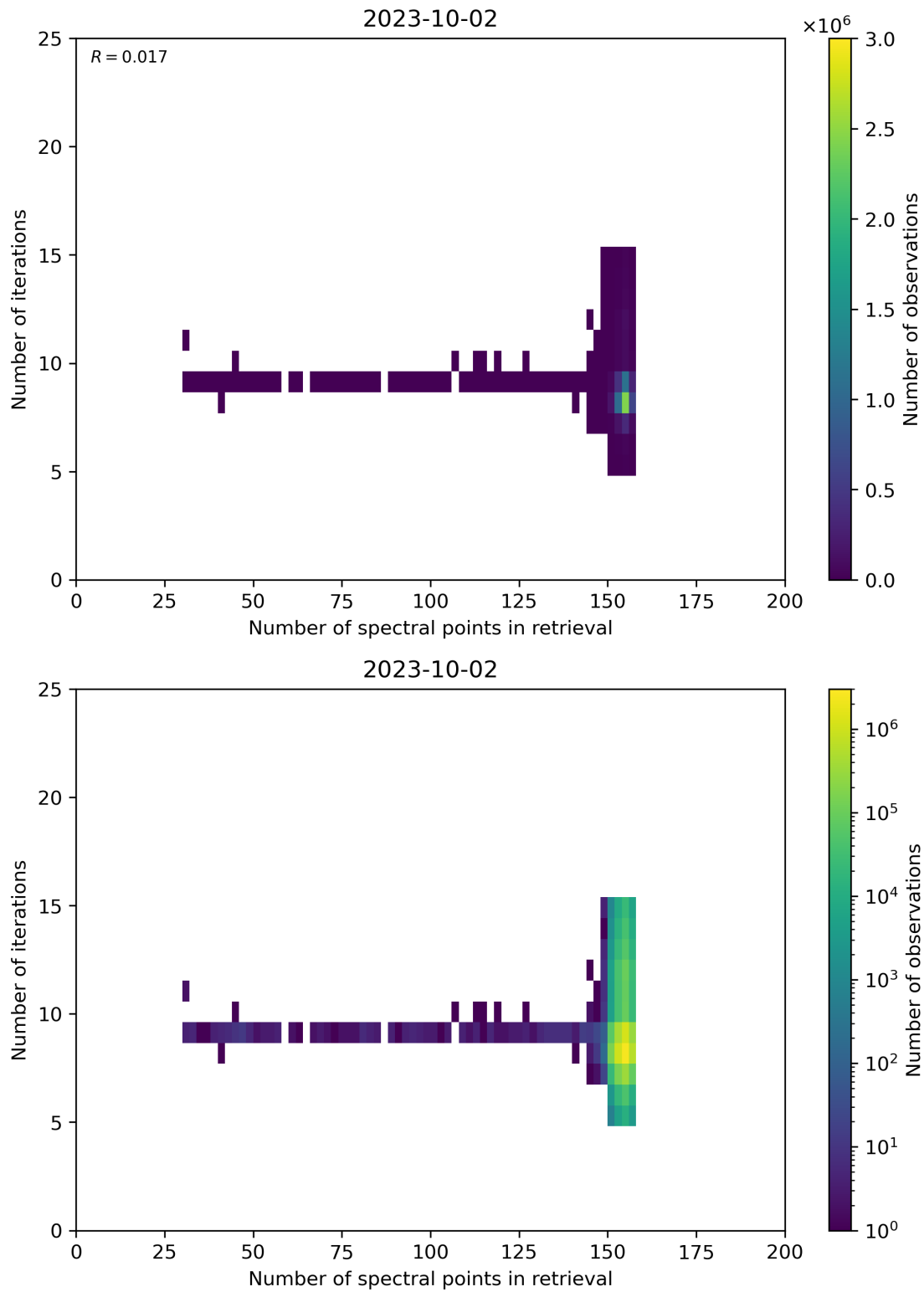
Figure 60: Scatter density plot of “Number of spectral points in retrieval” against “Number of iterations” for 2023-10-01 to 2023-10-03.
