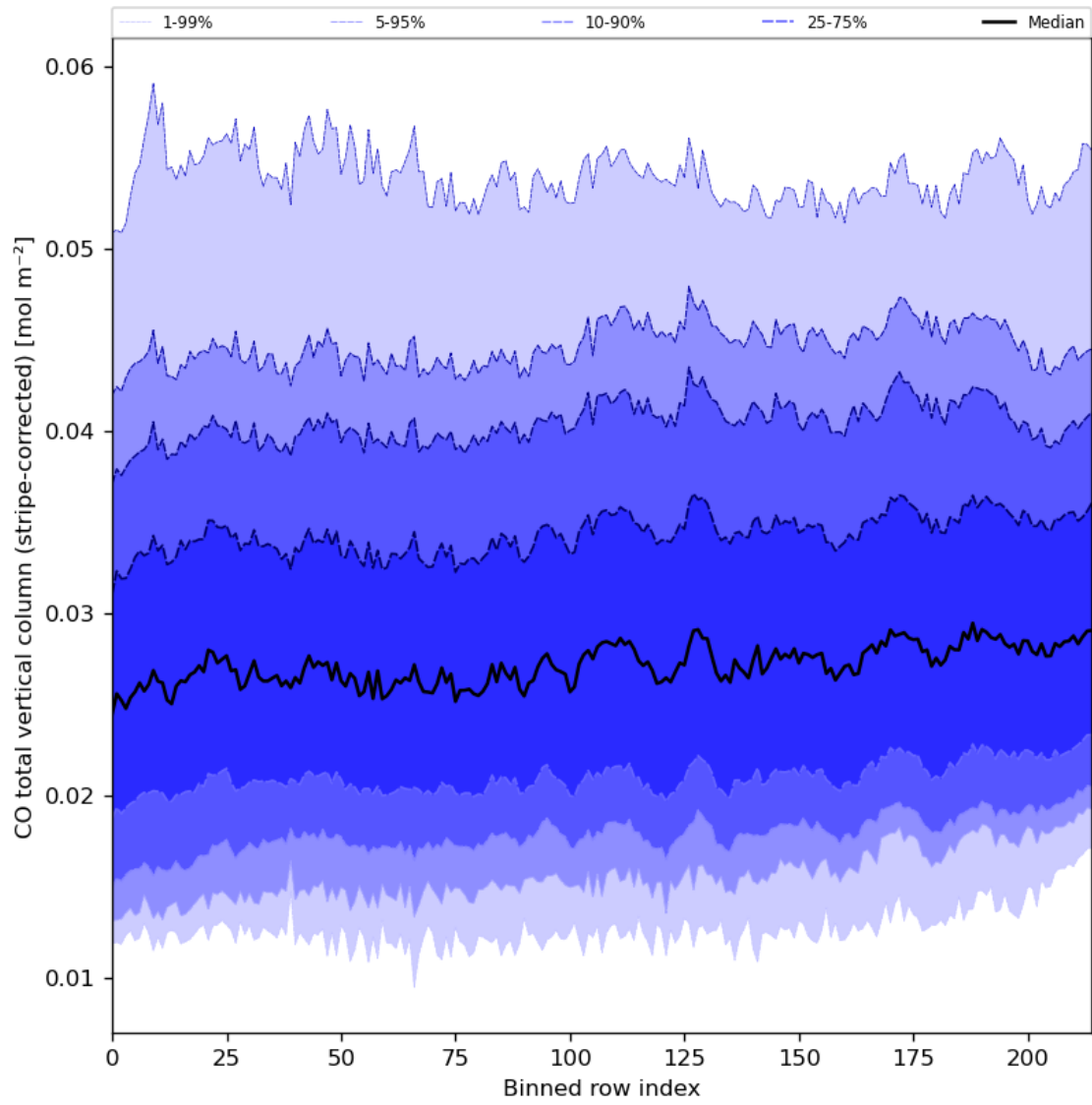
Figure 27: Along track statistics of “CO total vertical column (stripe-corrected)” for 2023-10-01 to 2023-10-03
