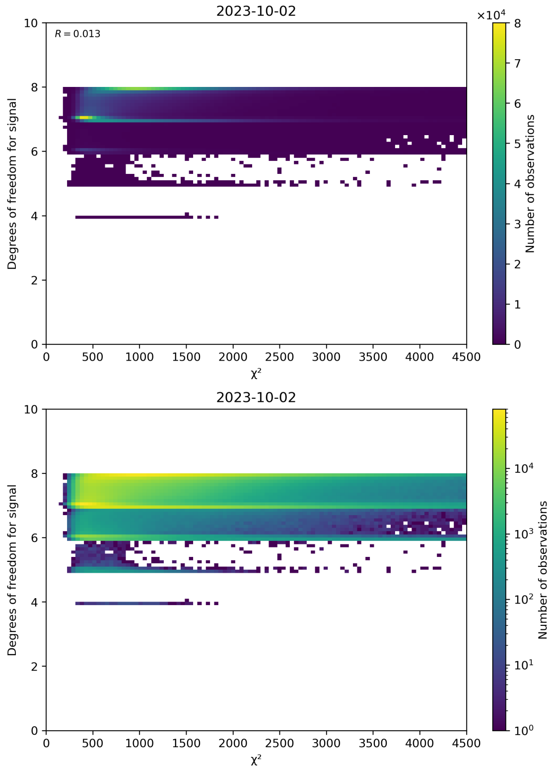
Figure 48: Scatter density plot of “ \chi^2 ” against “Degrees of freedom for signal” for 2023-10-01 to 2023-10-03.
