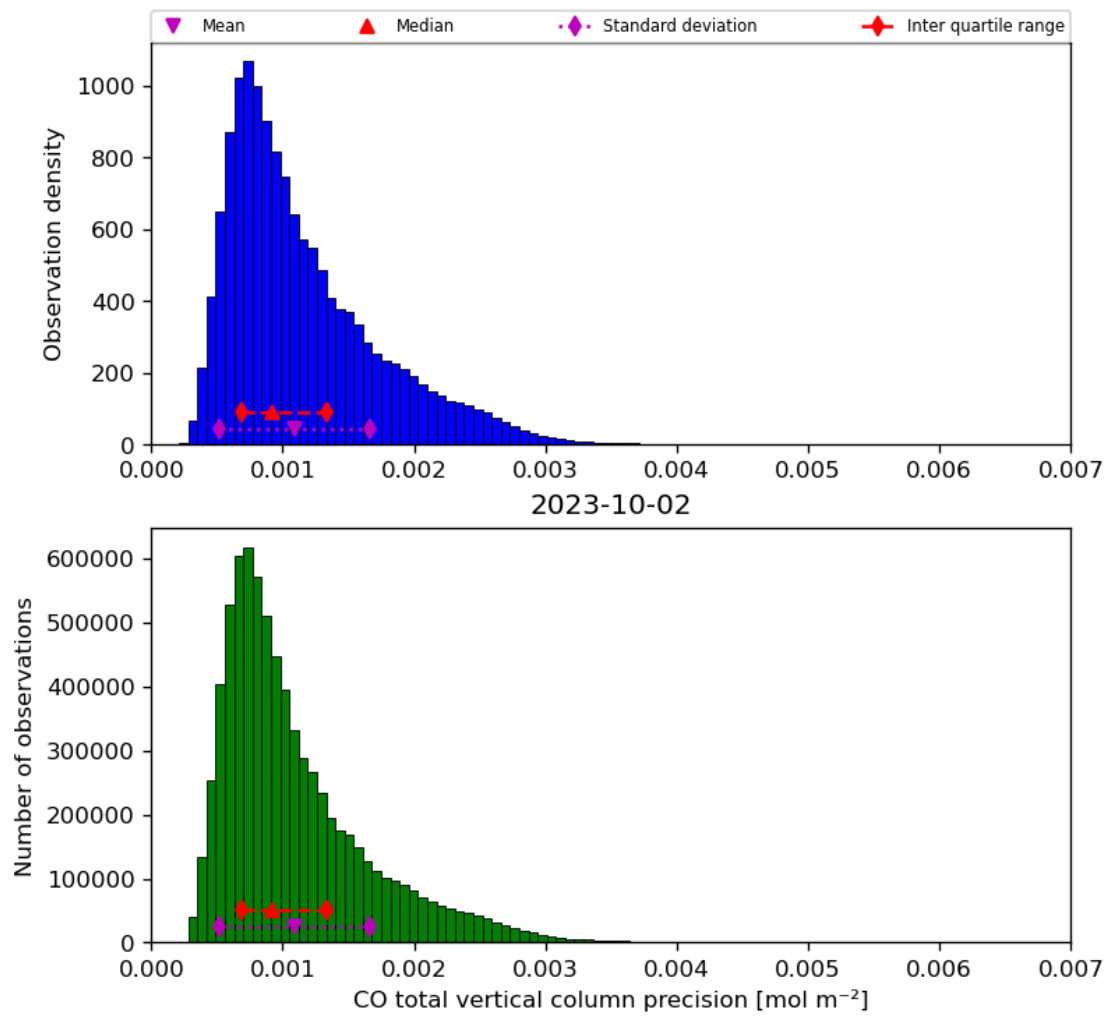
Figure 20: Histogram of “CO total vertical column precision” for 2023-10-01 to 2023-10-03
