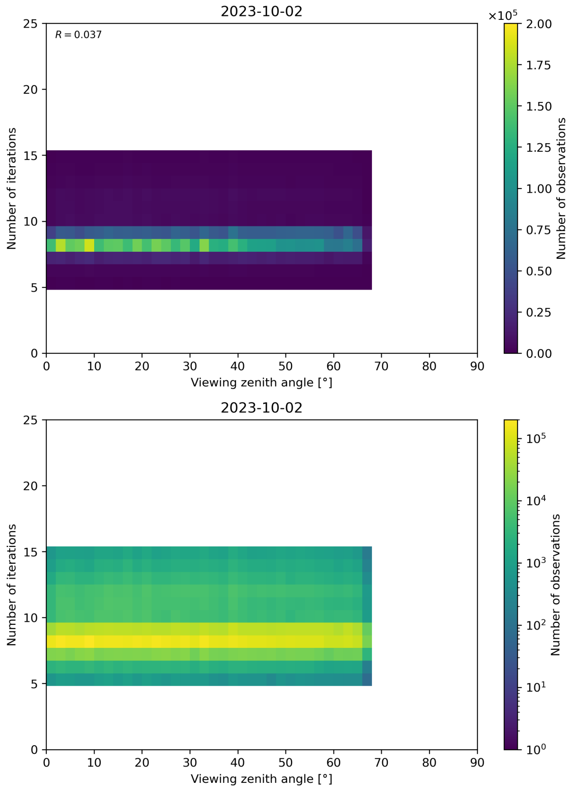
Figure 75: Scatter density plot of “Viewing zenith angle” against “Number of iterations” for 2023-10-01 to 2023-10-03.
