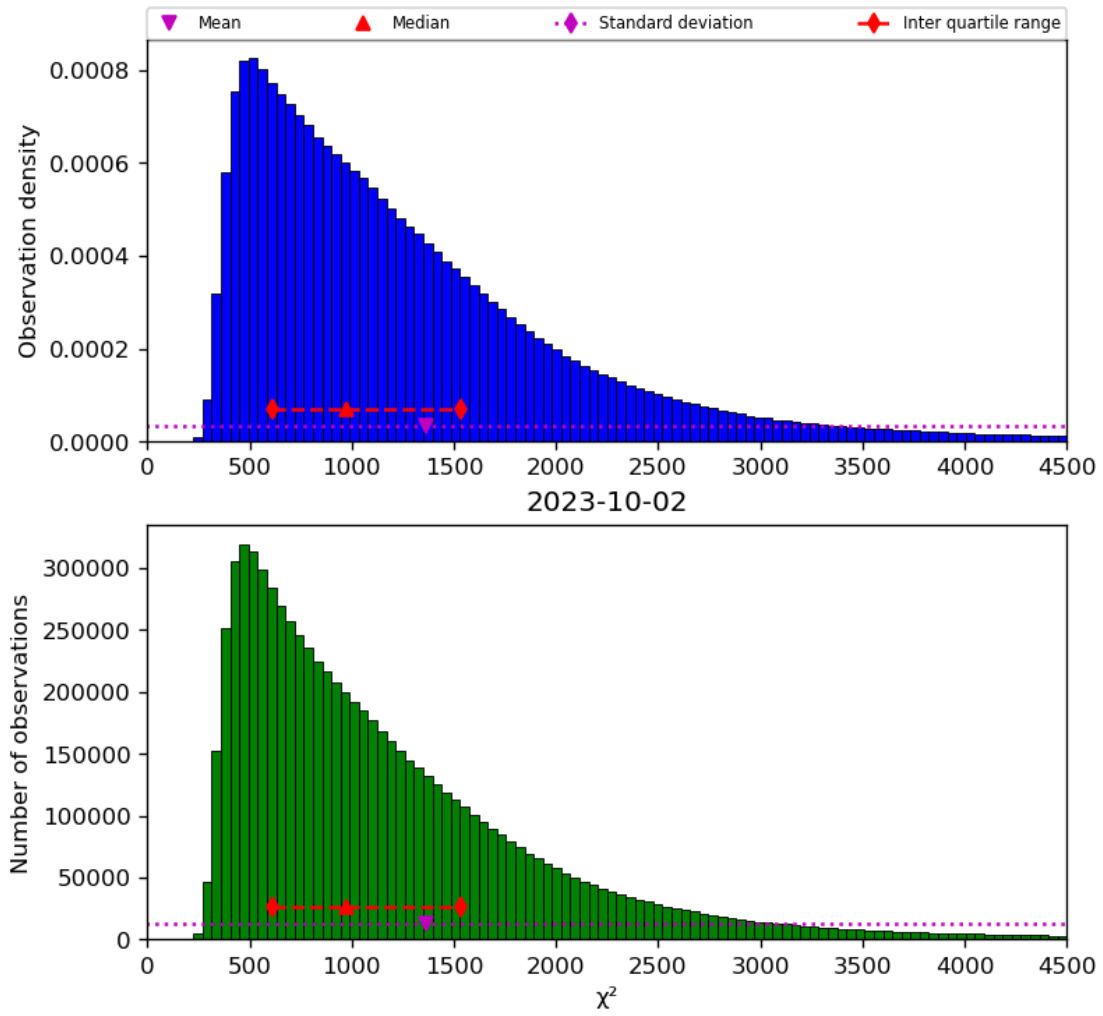
Figure 22: Histogram of “ \chi^2 ” for 2023-10-01 to 2023-10-03
