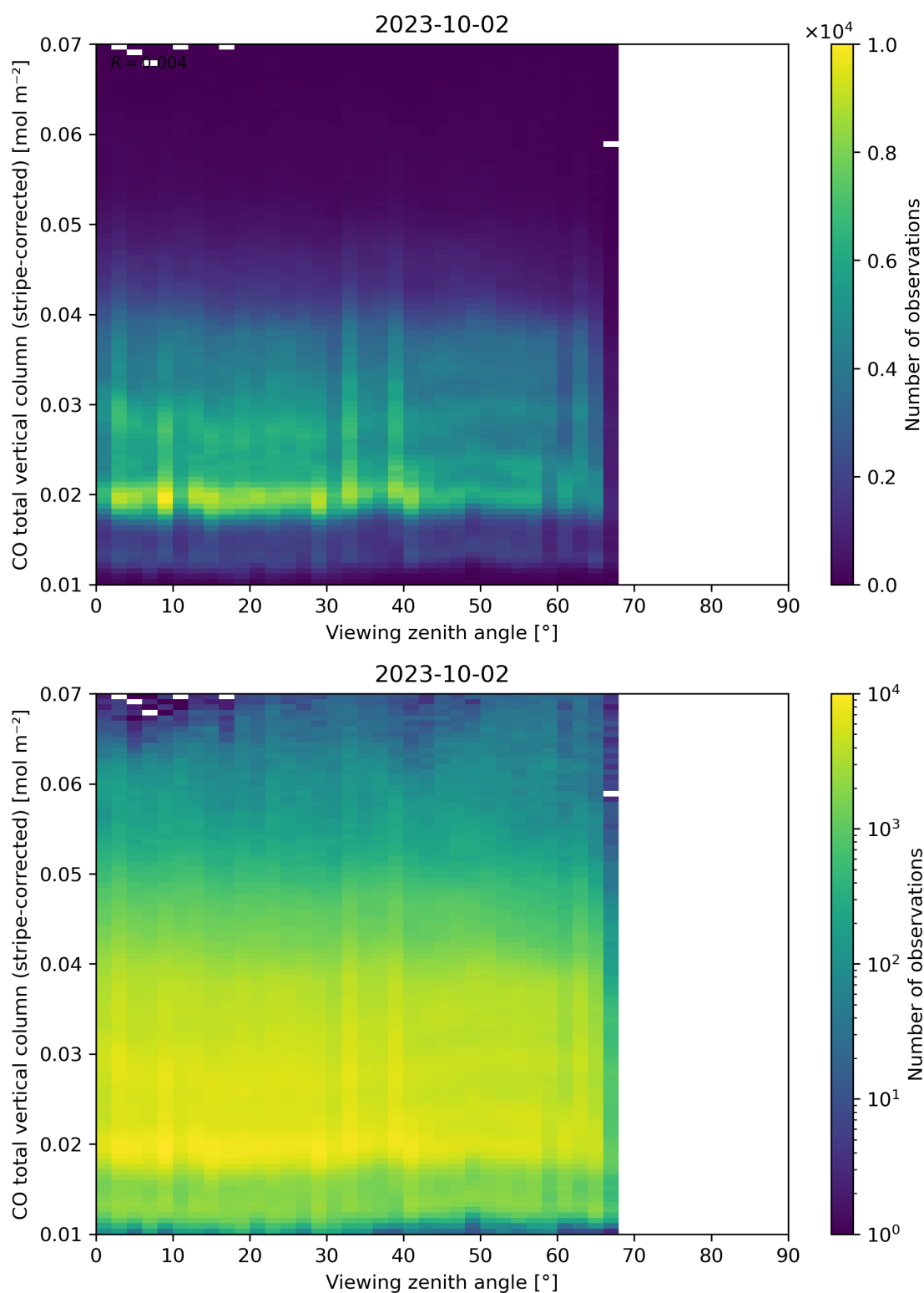
Figure 70: Scatter density plot of “Viewing zenith angle” against “CO total vertical column (stripe-corrected)” for 2023-10-01 to 2023-10-03.
