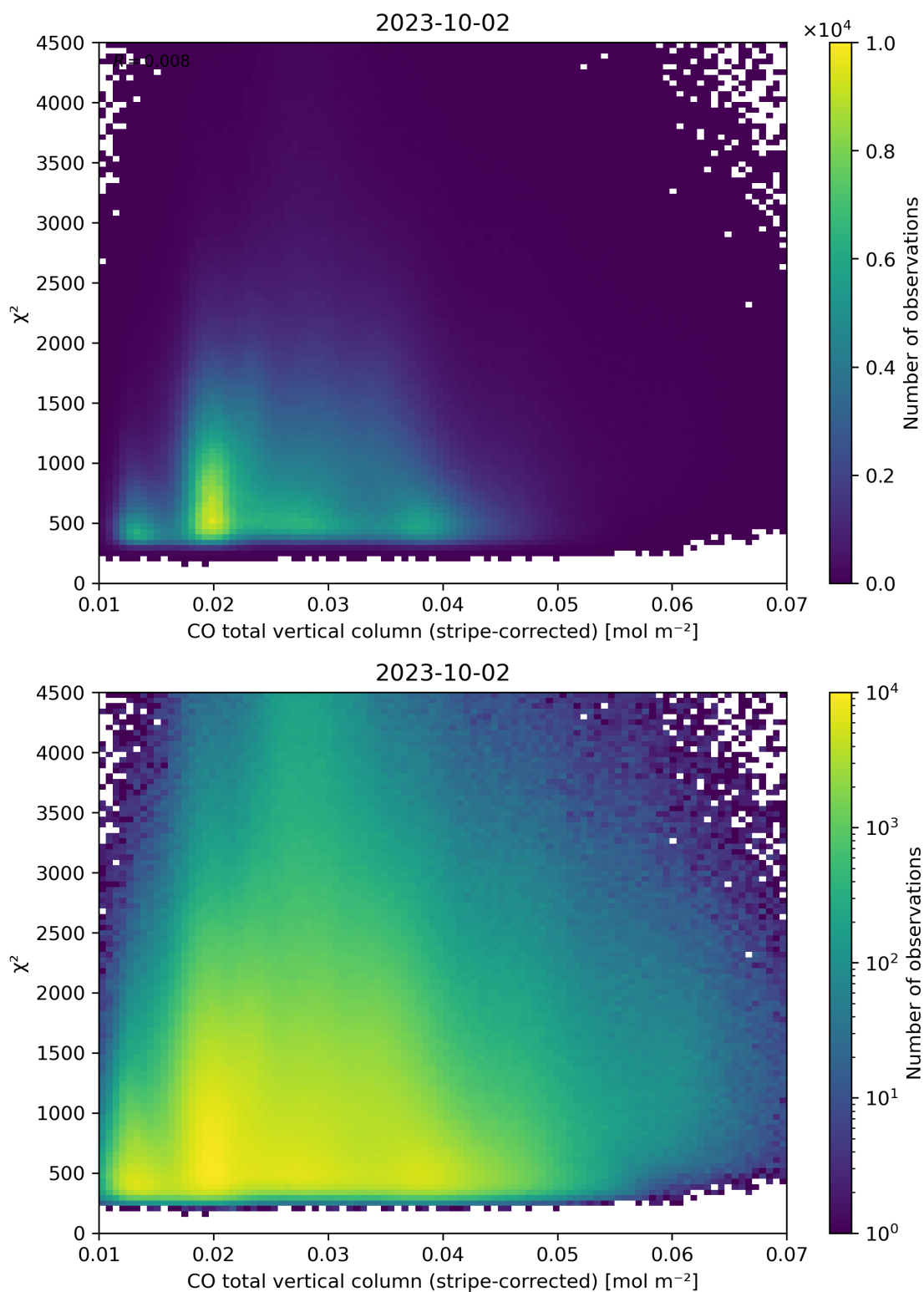
Figure 37: Scatter density plot of “CO total vertical column (stripe-corrected)” against “ \chi^2 ” for 2023-10-01 to 2023-10-03.
