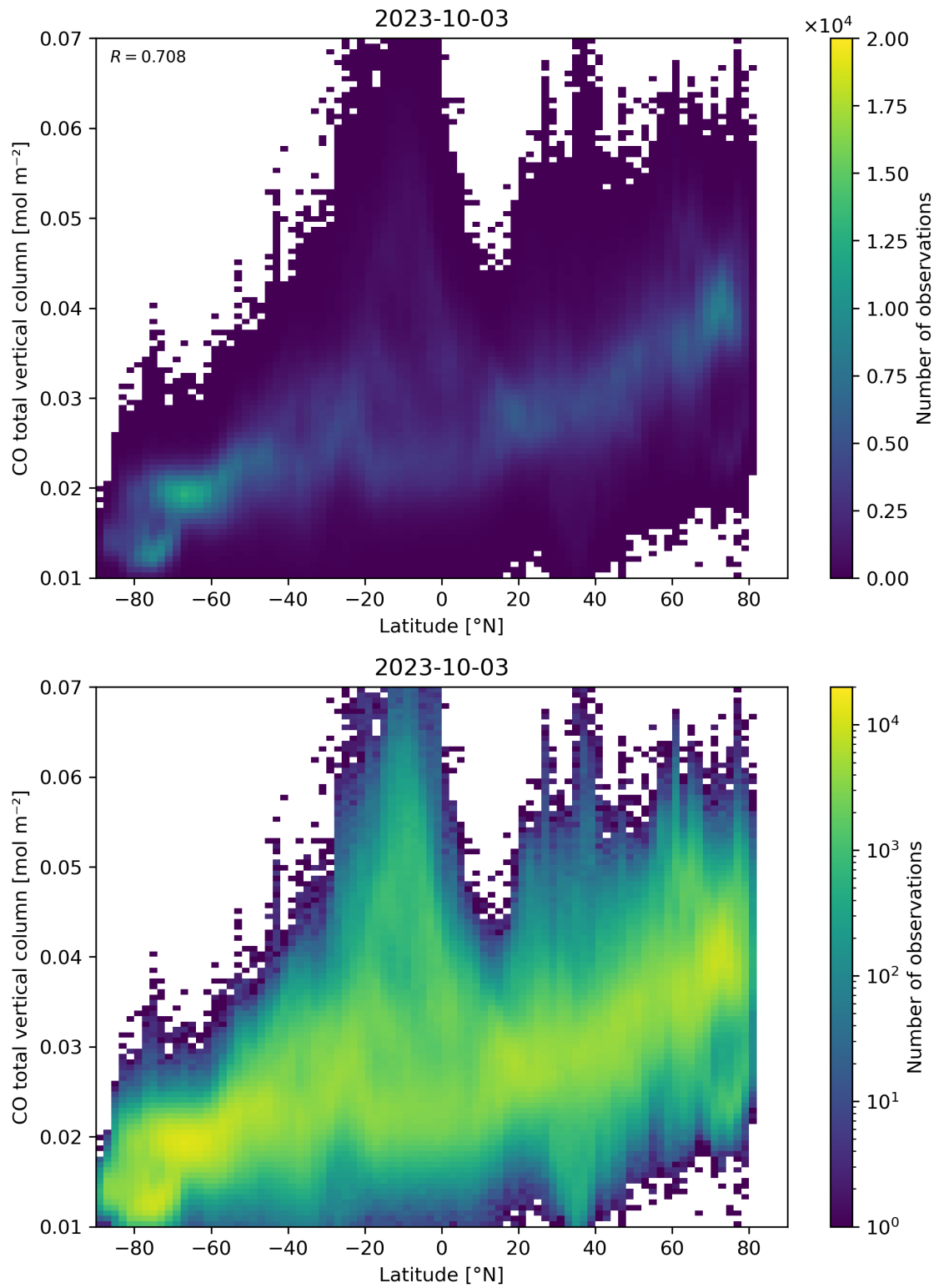
Figure 51: Scatter density plot of “Latitude” against “CO total vertical column” for 2023-10-02 to 2023-10-04.
