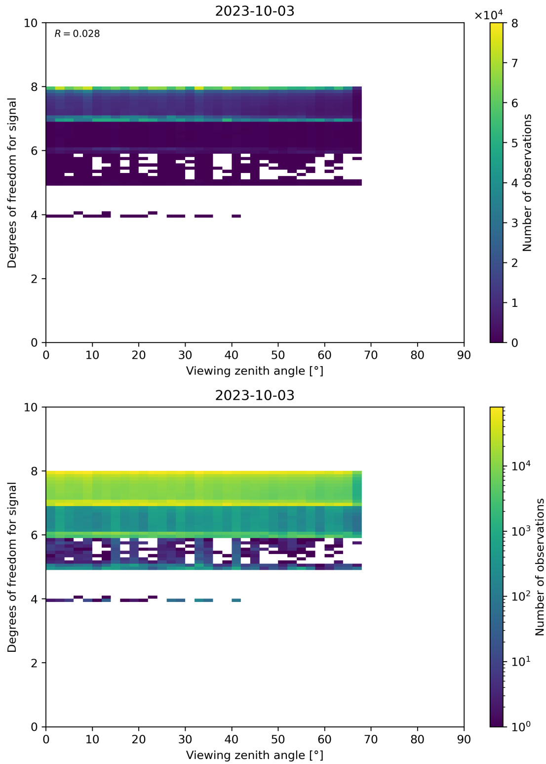
Figure 73: Scatter density plot of “Viewing zenith angle” against “Degrees of freedom for signal” for 2023-10-02 to 2023-10-04.
