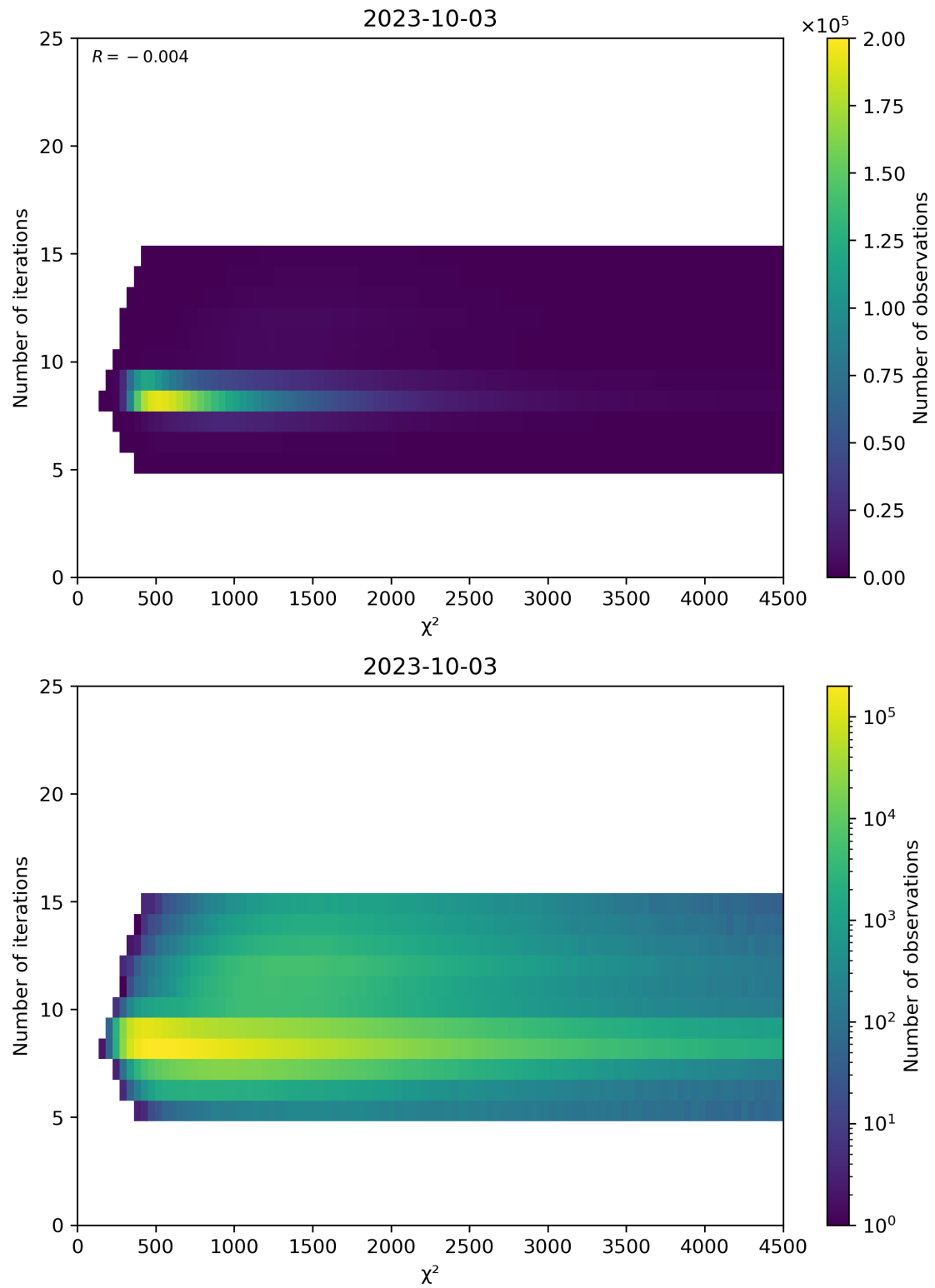
Figure 49: Scatter density plot of “ \chi^2 ” against “Number of iterations” for 2023-10-02 to 2023-10-04.
