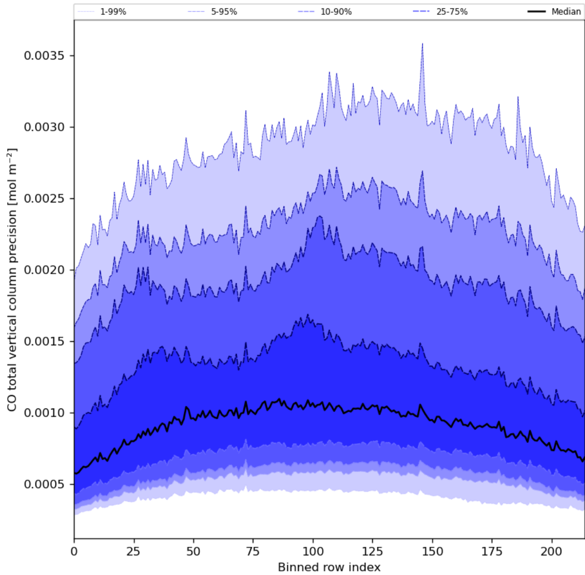
Figure 28: Along track statistics of “CO total vertical column precision” for 2023-10-02 to 2023-10-04
