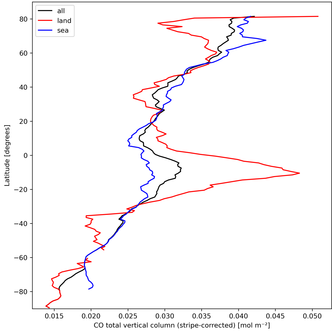
Figure 11: Zonal average of “CO total vertical column (stripe-corrected)” for 2023-10-02 to 2023-10-04.
