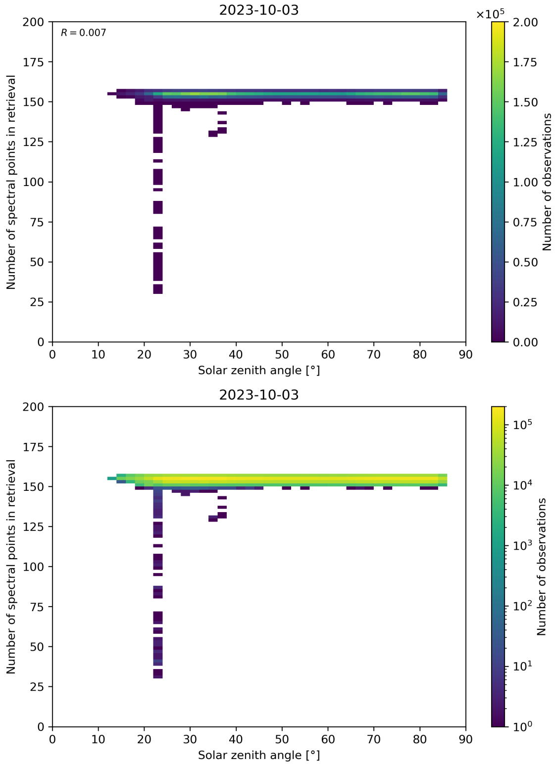
Figure 68: Scatter density plot of “Solar zenith angle” against “Number of spectral points in retrieval” for 2023-10-02 to 2023-10-04.
