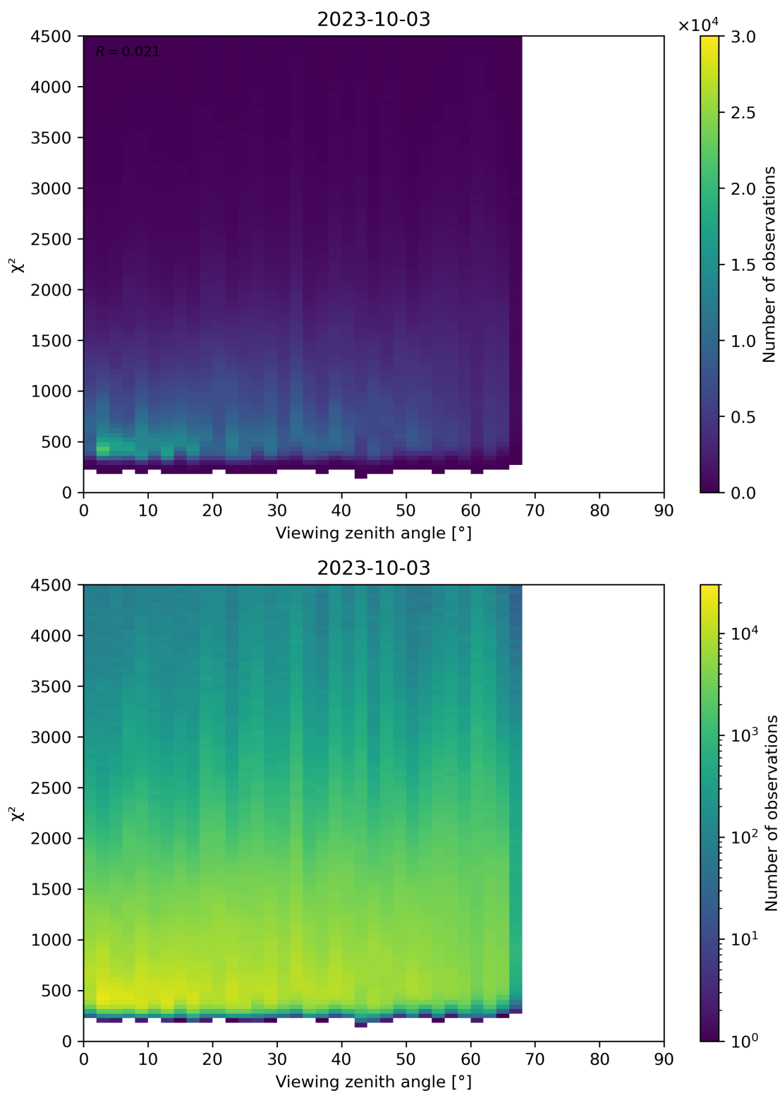
Figure 72: Scatter density plot of “Viewing zenith angle” against “ \chi^2 ” for 2023-10-02 to 2023-10-04.
