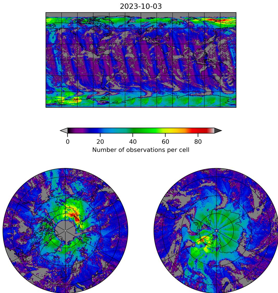
Figure 8: Map of the number of observations for 2023-10-02 to 2023-10-04
