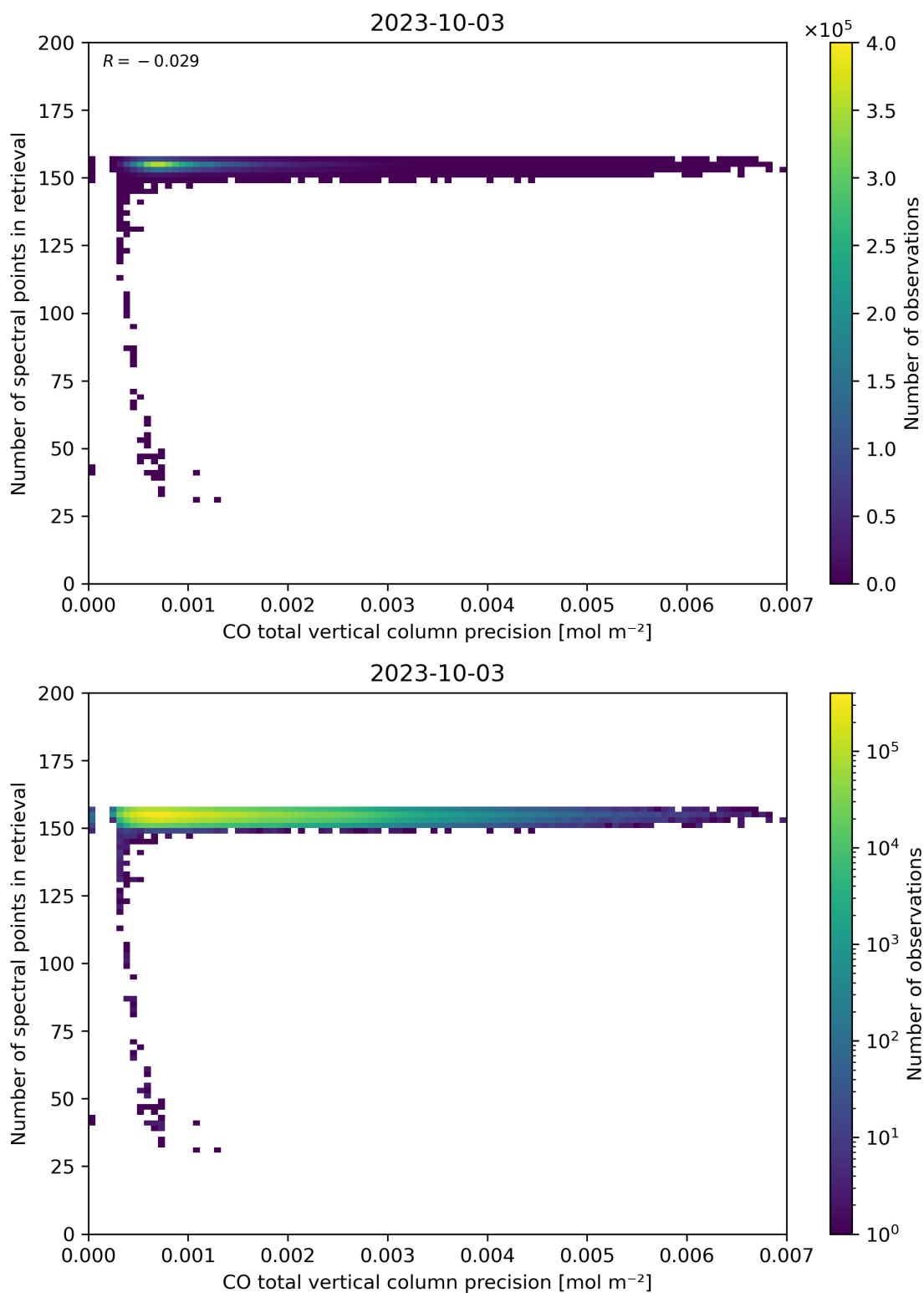
Figure 47: Scatter density plot of “CO total vertical column precision” against “Number of spectral points in retrieval” for 2023-10-02 to 2023-10-04.
