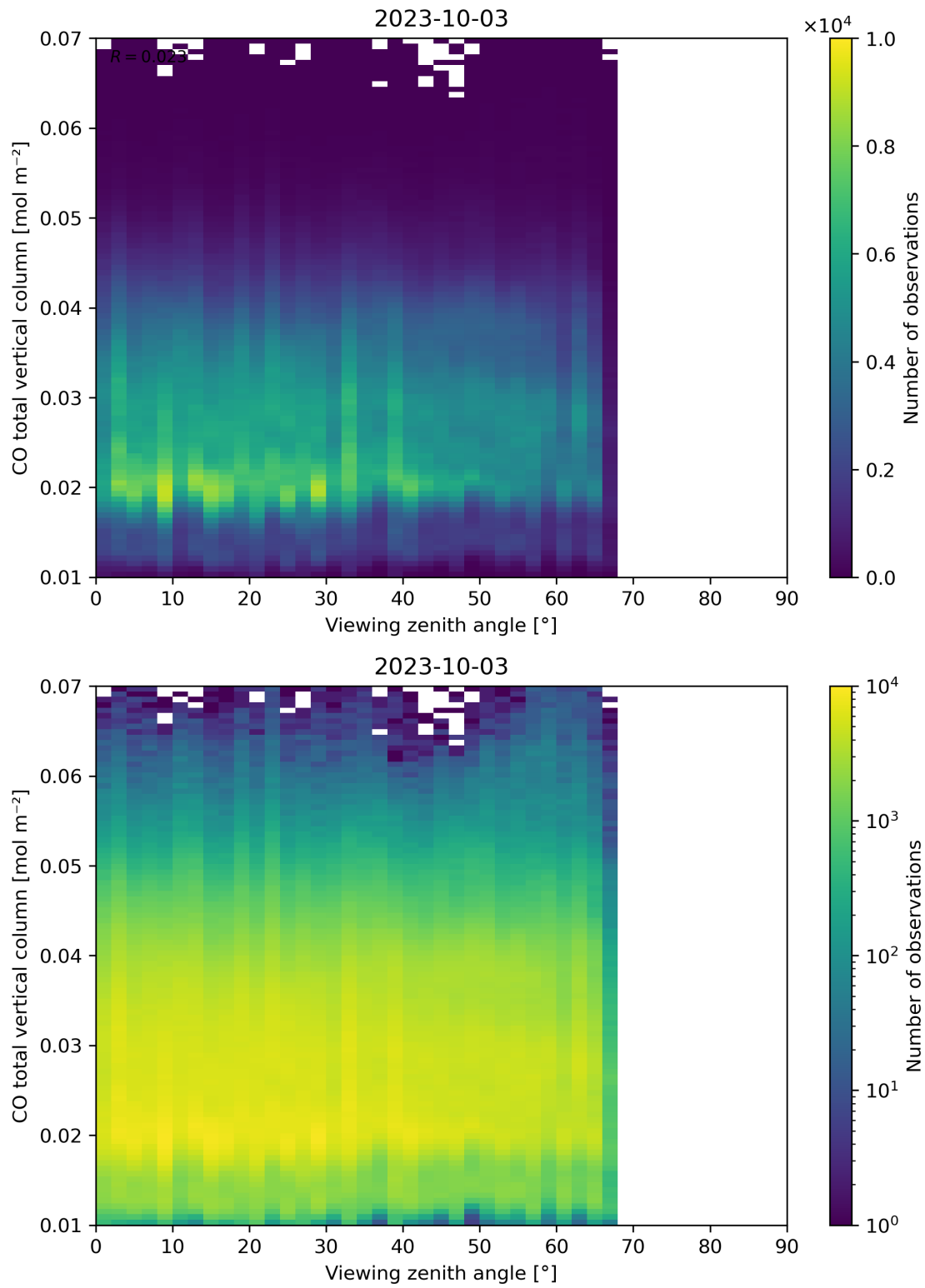
Figure 69: Scatter density plot of “Viewing zenith angle” against “CO total vertical column” for 2023-10-02 to 2023-10-04.
