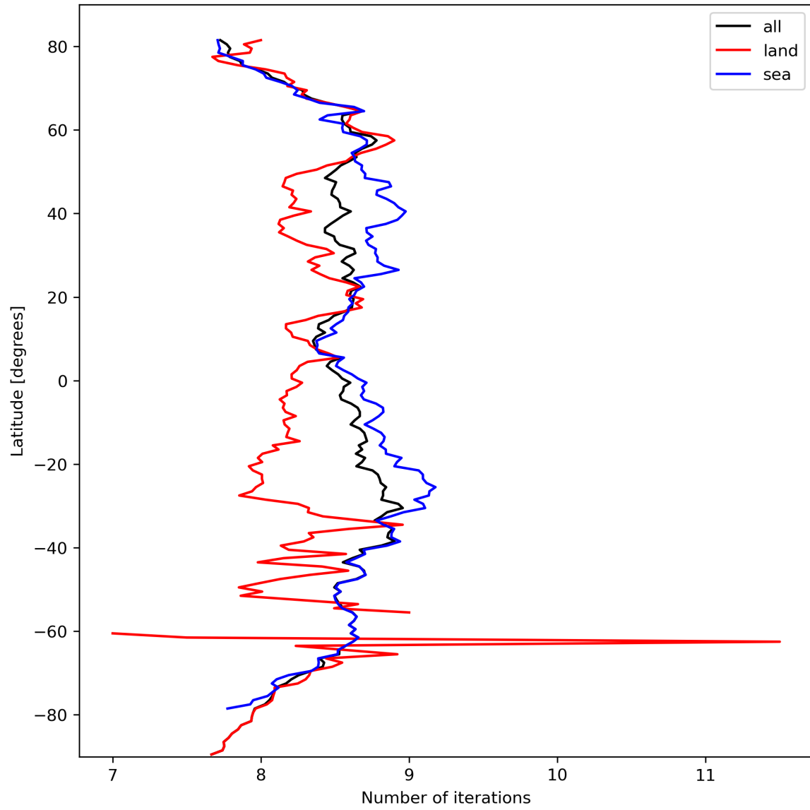
Figure 16: Zonal average of “Number of iterations” for 2023-10-02 to 2023-10-04.
