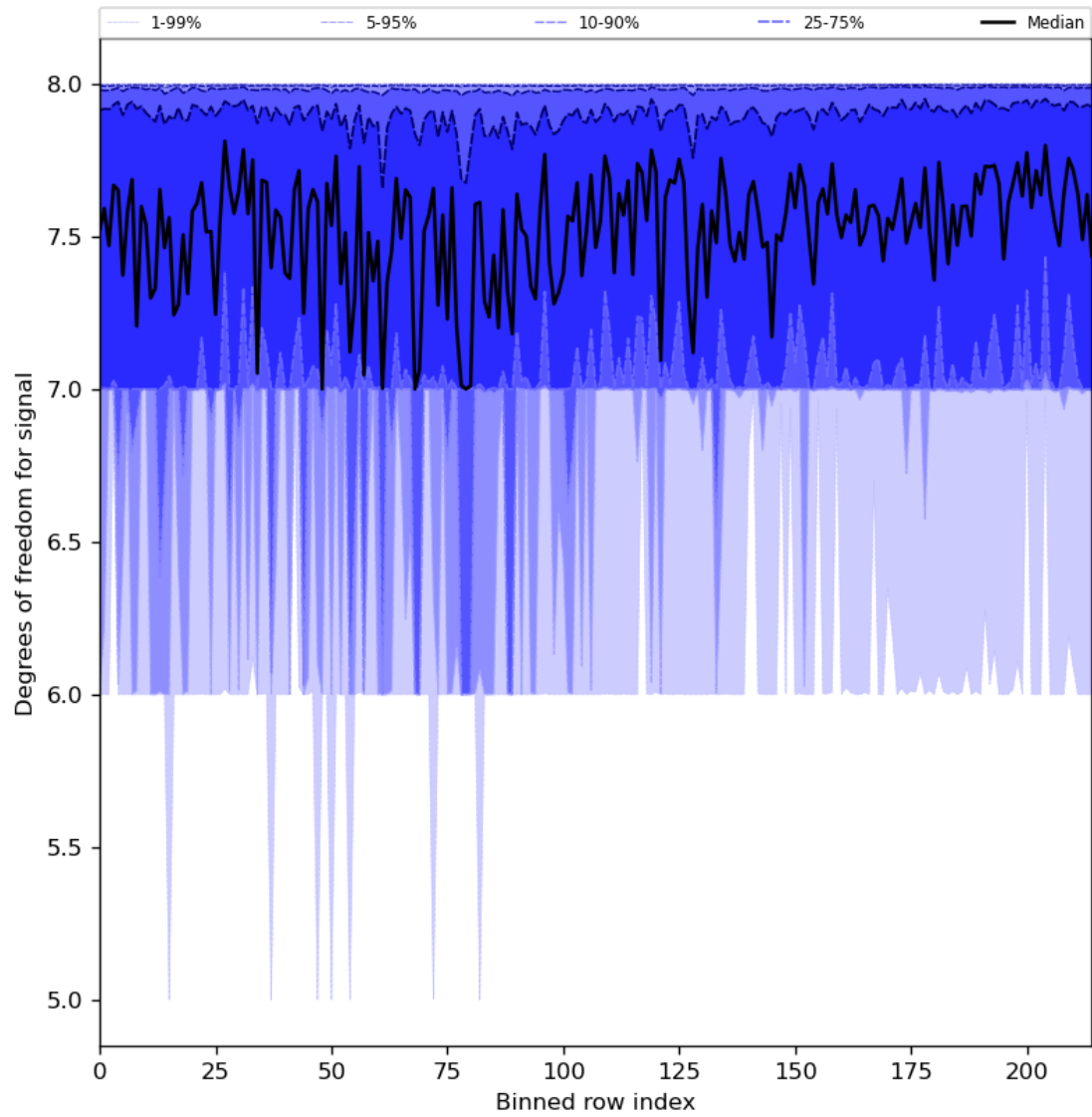
Figure 31: Along track statistics of “Degrees of freedom for signal” for 2023-10-02 to 2023-10-04
