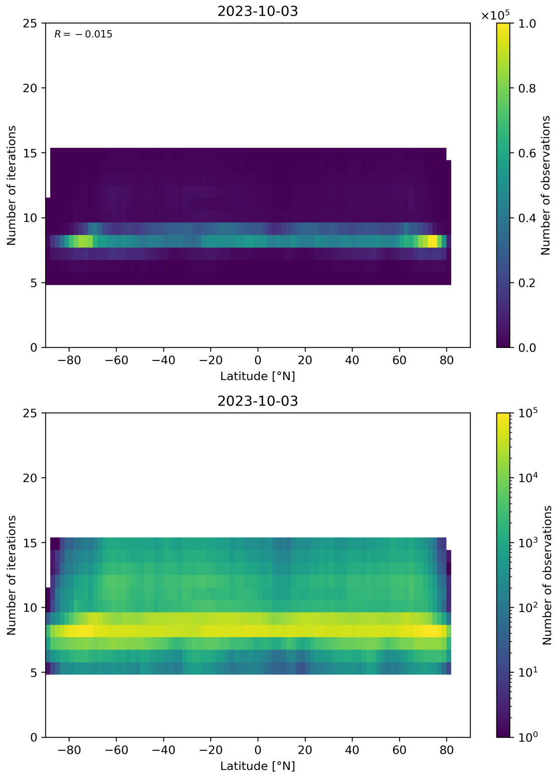
Figure 56: Scatter density plot of “Latitude” against “Number of iterations” for 2023-10-02 to 2023-10-04.
