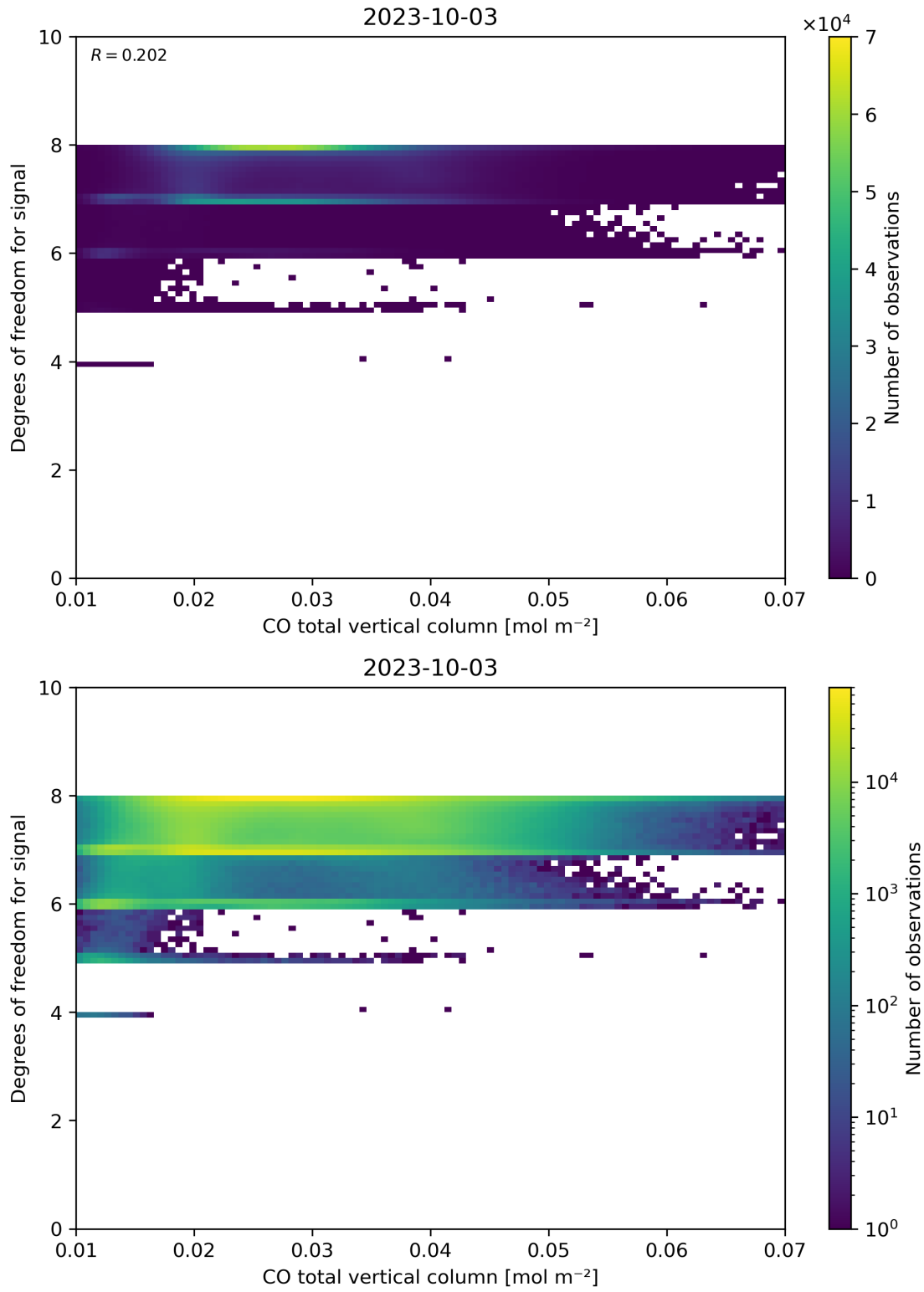
Figure 41: Scatter density plot of “CO total vertical column” against “Degrees of freedom for signal” for 2023-10-02 to 2023-10-04.
