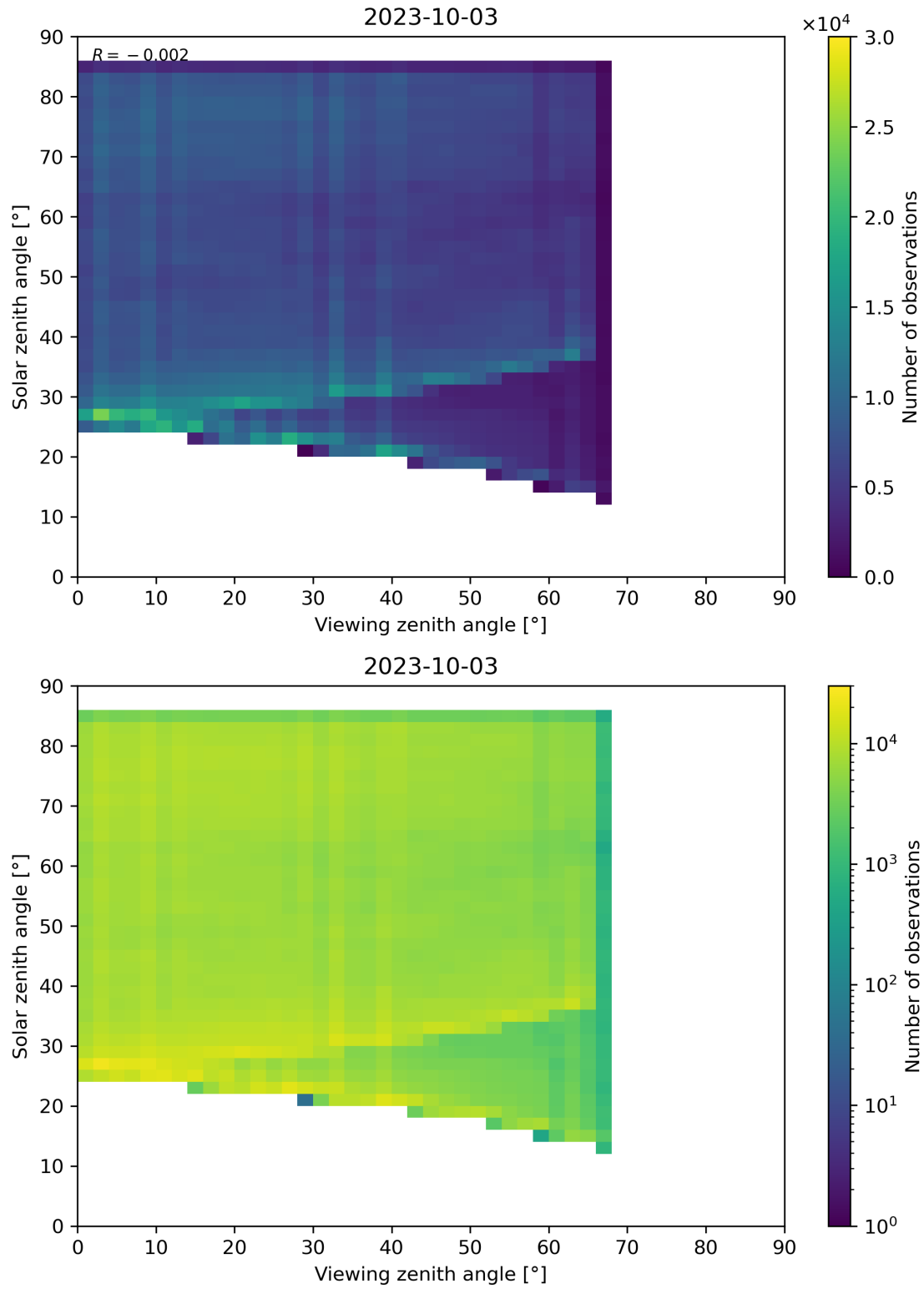
Figure 77: Scatter density plot of “Viewing zenith angle” against “Solar zenith angle” for 2023-10-02 to 2023-10-04.
