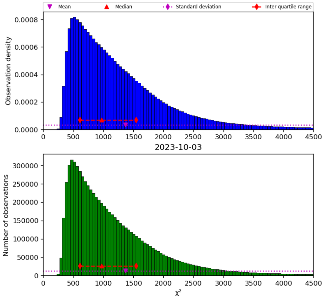
Figure 22: Histogram of " \chi^2 " for 2023-10-02 to 2023-10-04
