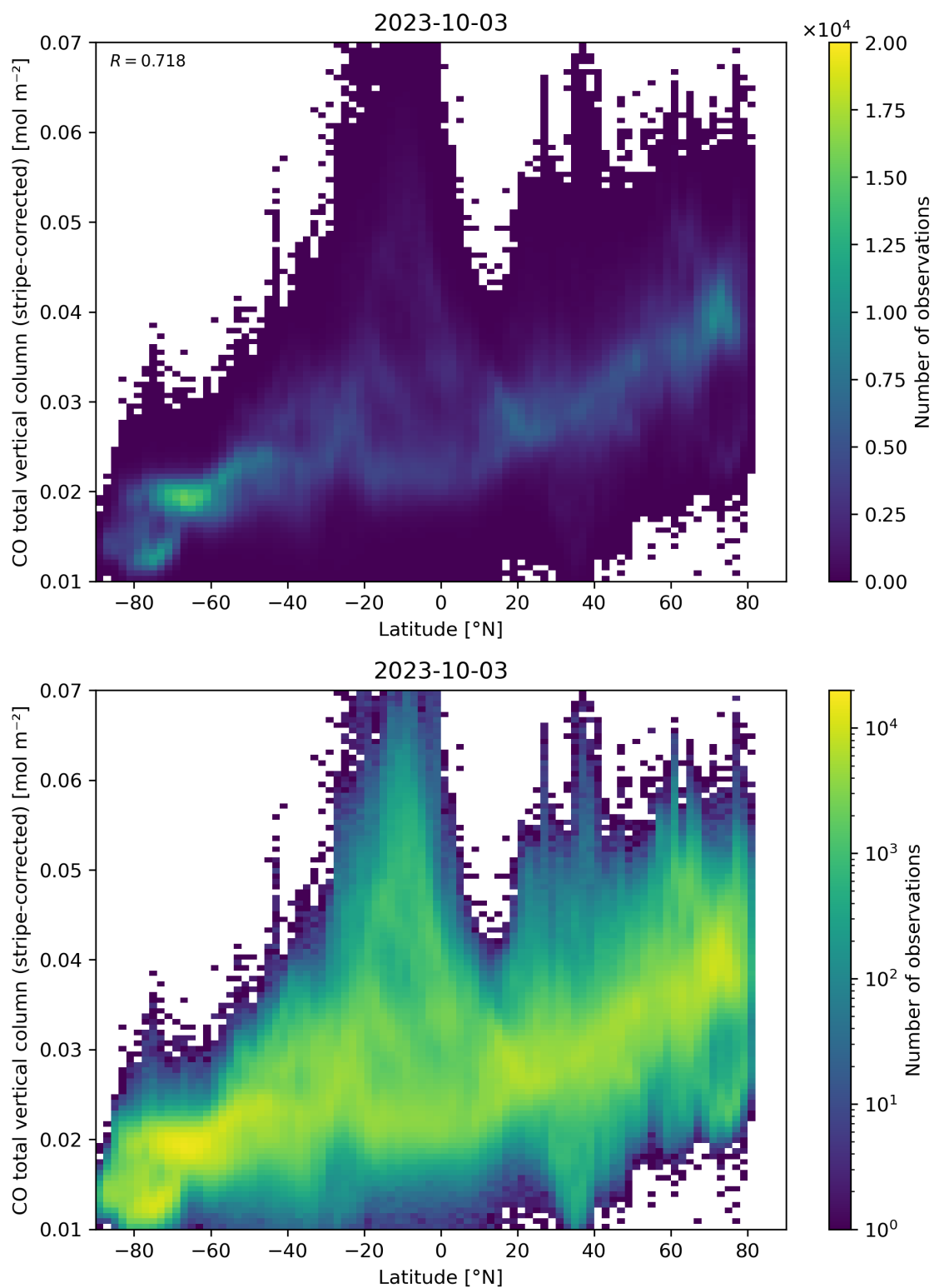
Figure 52: Scatter density plot of “Latitude” against “CO total vertical column (stripe-corrected)” for 2023-10-02 to 2023-10-04.
