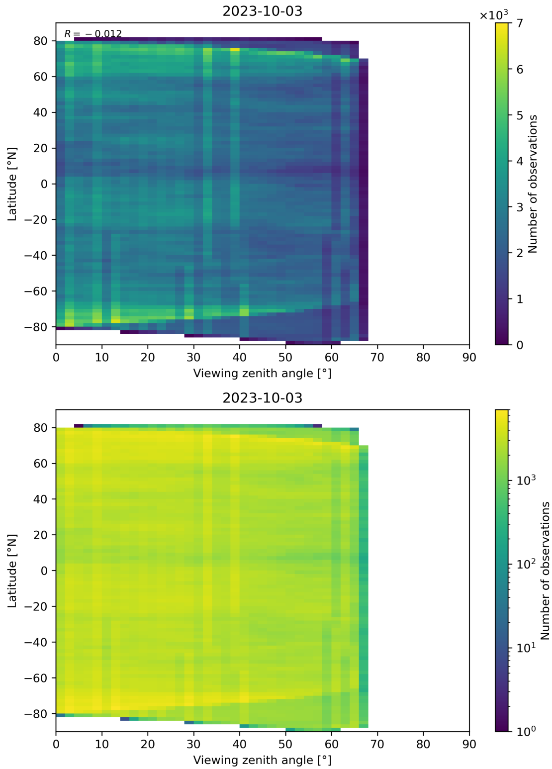
Figure 74: Scatter density plot of “Viewing zenith angle” against “Latitude” for 2023-10-02 to 2023-10-04.
