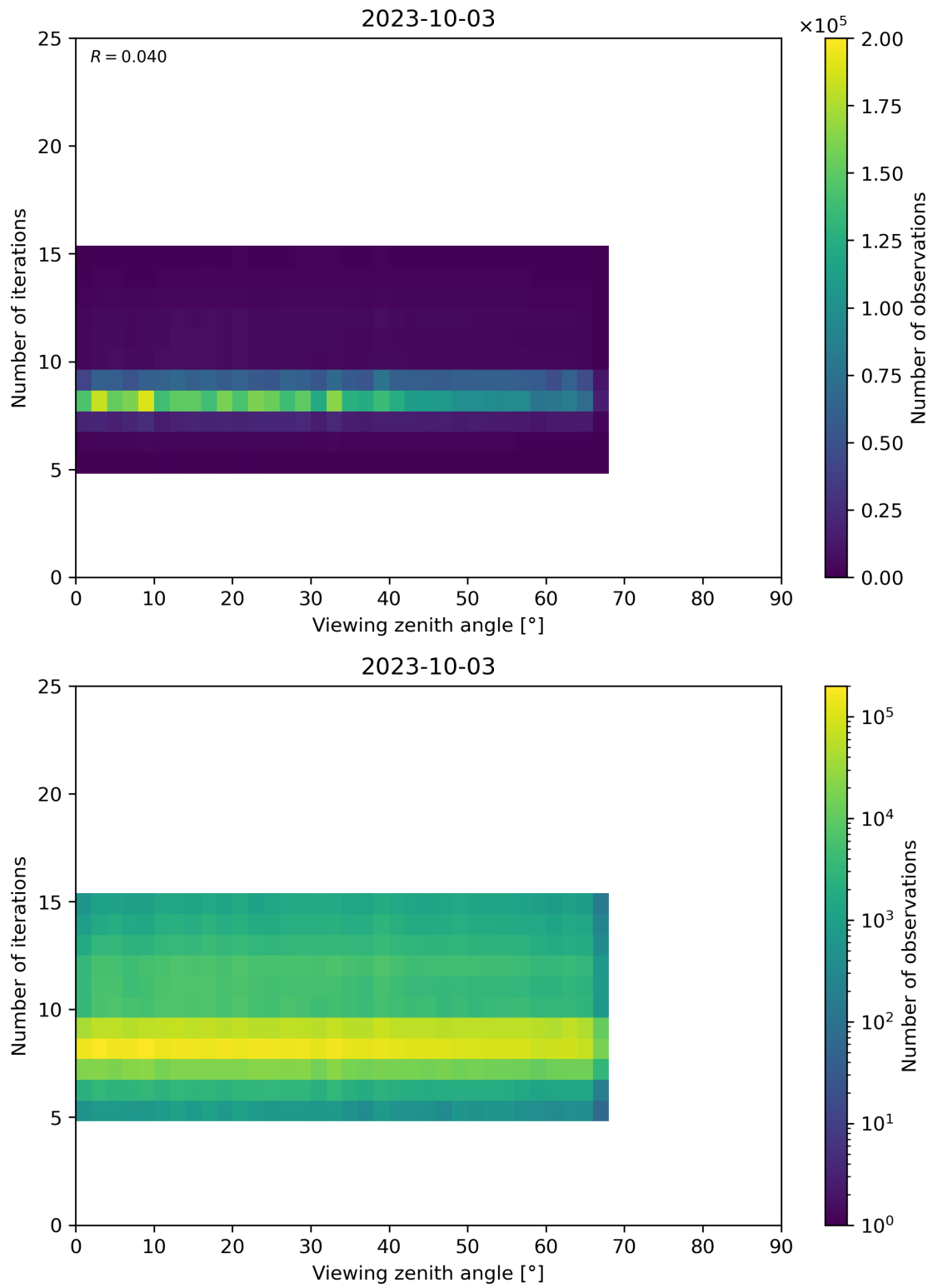
Figure 75: Scatter density plot of “Viewing zenith angle” against “Number of iterations” for 2023-10-02 to 2023-10-04.
