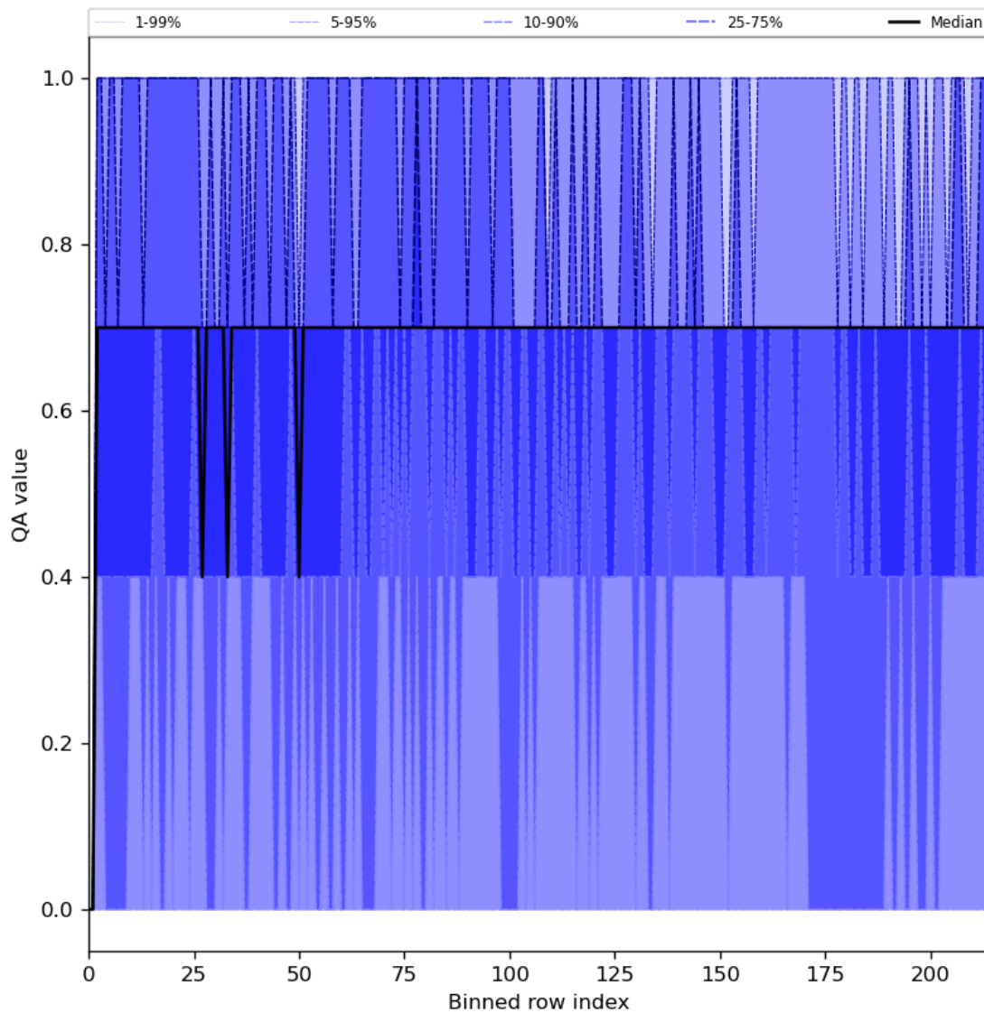
Figure 25: Along track statistics of “QA value” for 2023-10-02 to 2023-10-04
