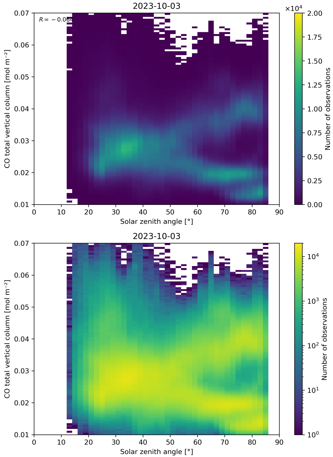
Figure 61: Scatter density plot of “Solar zenith angle” against “CO total vertical column” for 2023-10-02 to 2023-10-04.
