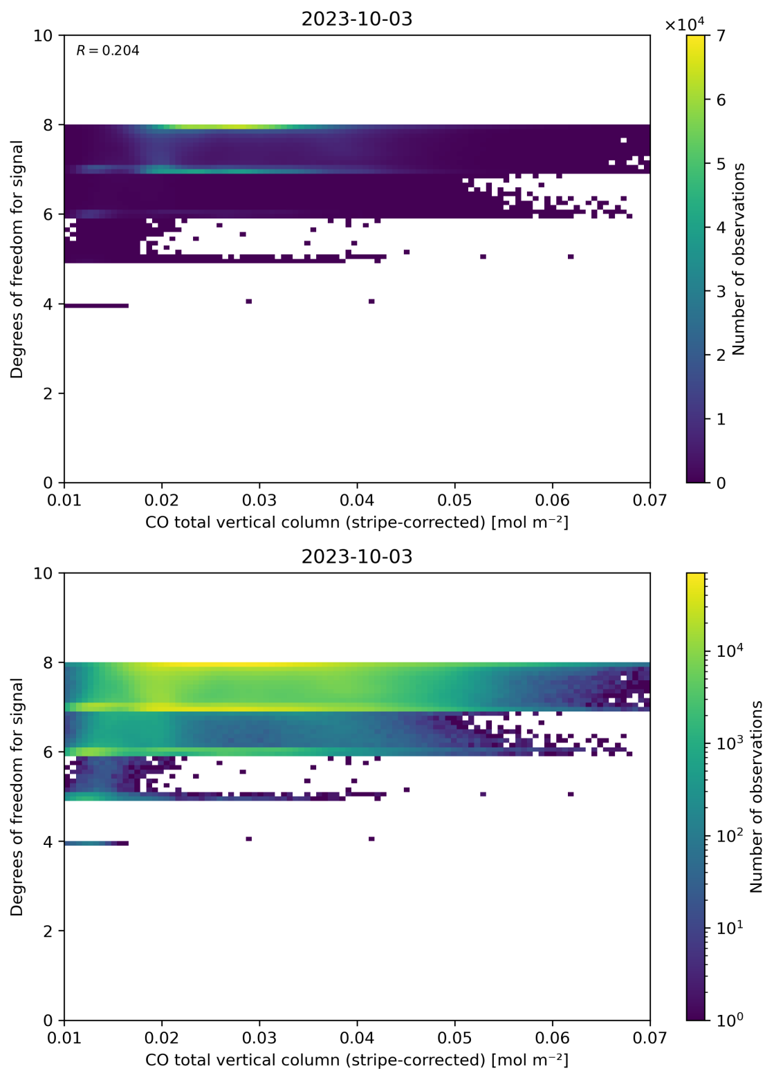
Figure 38: Scatter density plot of “CO total vertical column (stripe-corrected)” against “Degrees of freedom for signal” for 2023-10-02 to 2023-10-04.
