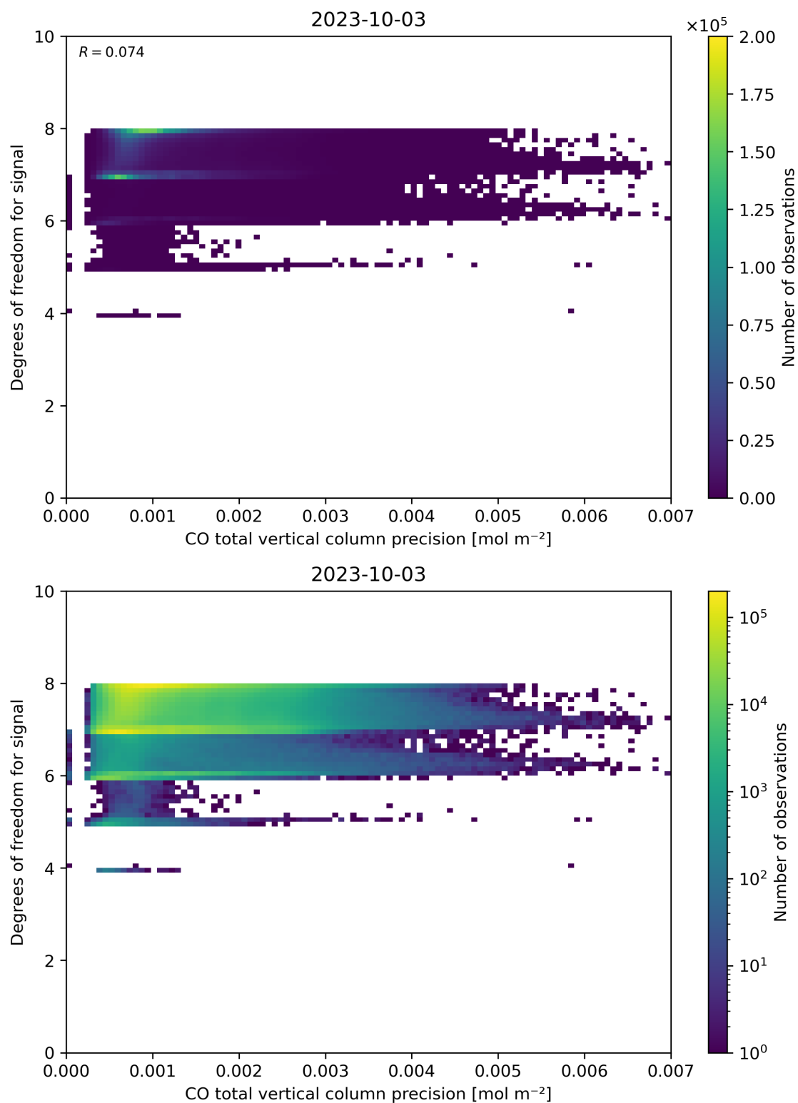
Figure 45: Scatter density plot of “CO total vertical column precision” against “Degrees of freedom for signal” for 2023-10-02 to 2023-10-04.
