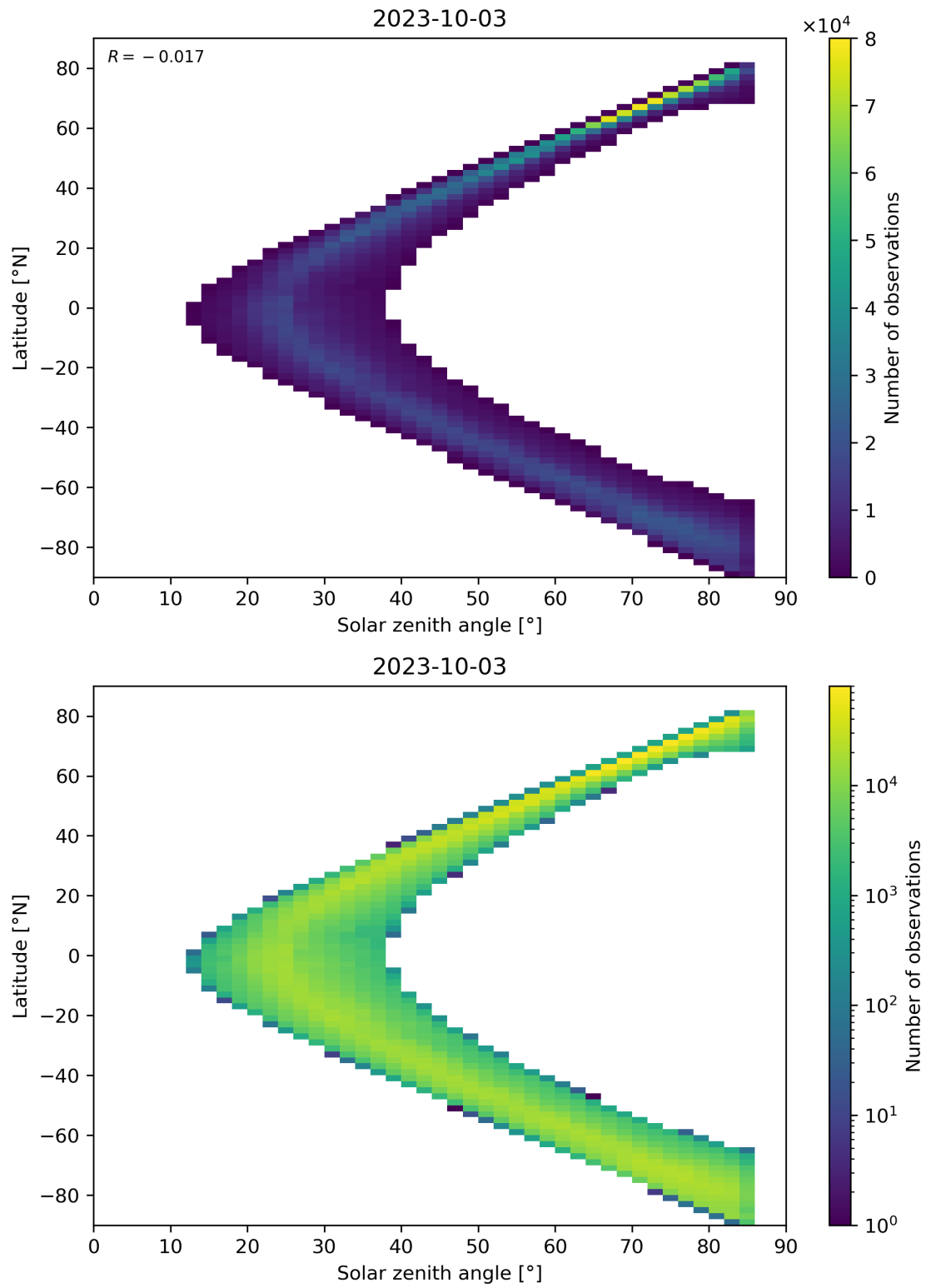
Figure 66: Scatter density plot of “Solar zenith angle” against “Latitude” for 2023-10-02 to 2023-10-04.
