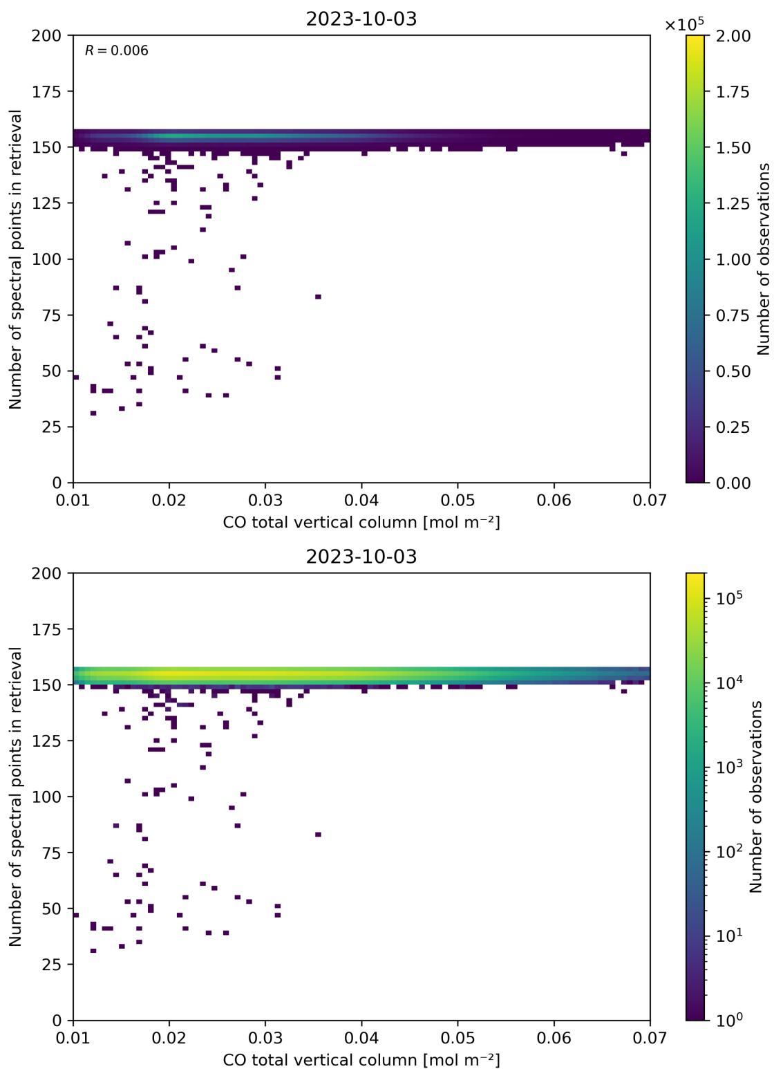
Figure 43: Scatter density plot of “CO total vertical column” against “Number of spectral points in retrieval” for 2023-10-02 to 2023-10-04.
