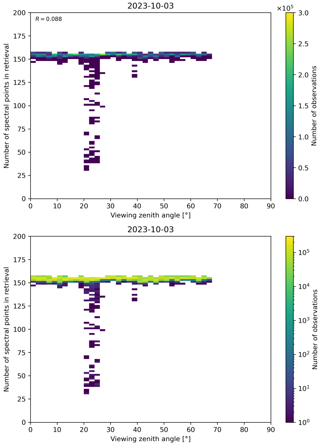
Figure 76: Scatter density plot of “Viewing zenith angle” against “Number of spectral points in retrieval” for 2023-10-02 to 2023-10-04.
