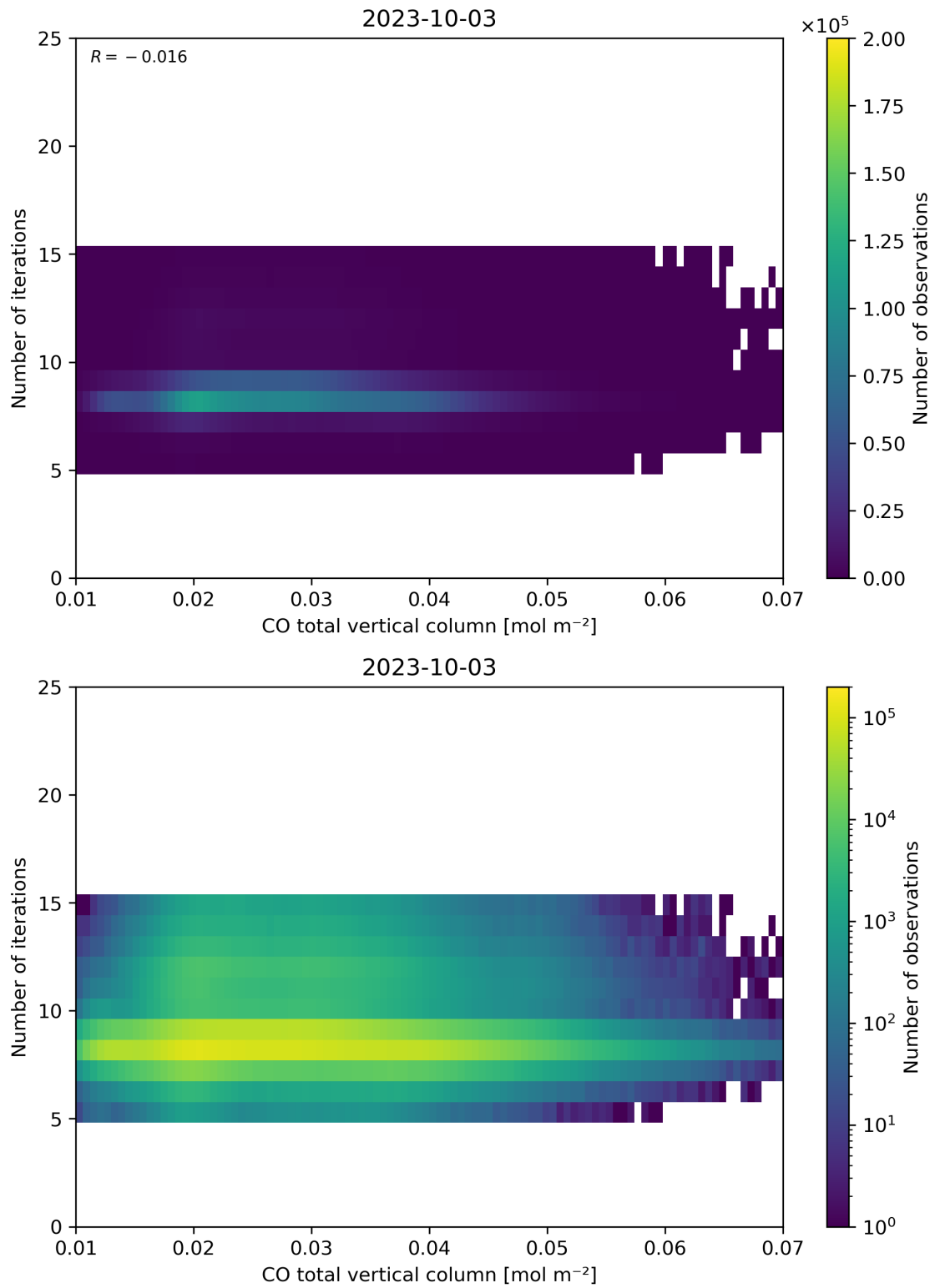
Figure 42: Scatter density plot of “CO total vertical column” against “Number of iterations” for 2023-10-02 to 2023-10-04.
