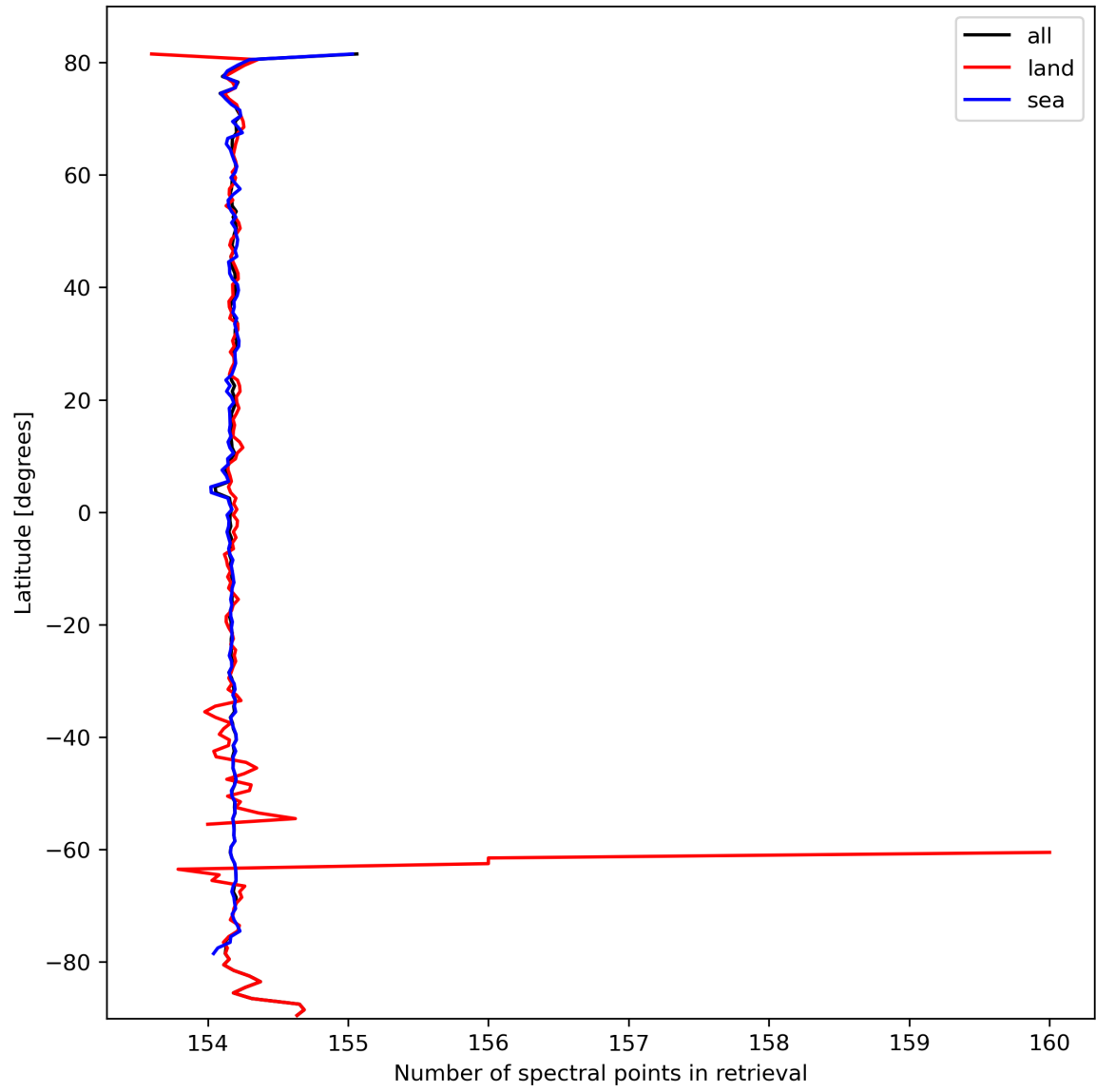
Figure 13: Zonal average of “Number of spectral points in retrieval” for 2023-10-02 to 2023-10-04.
