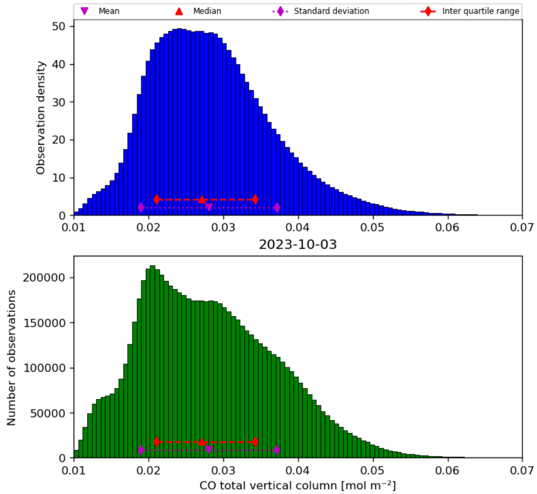
Figure 18: Histogram of “CO total vertical column” for 2023-10-02 to 2023-10-04
