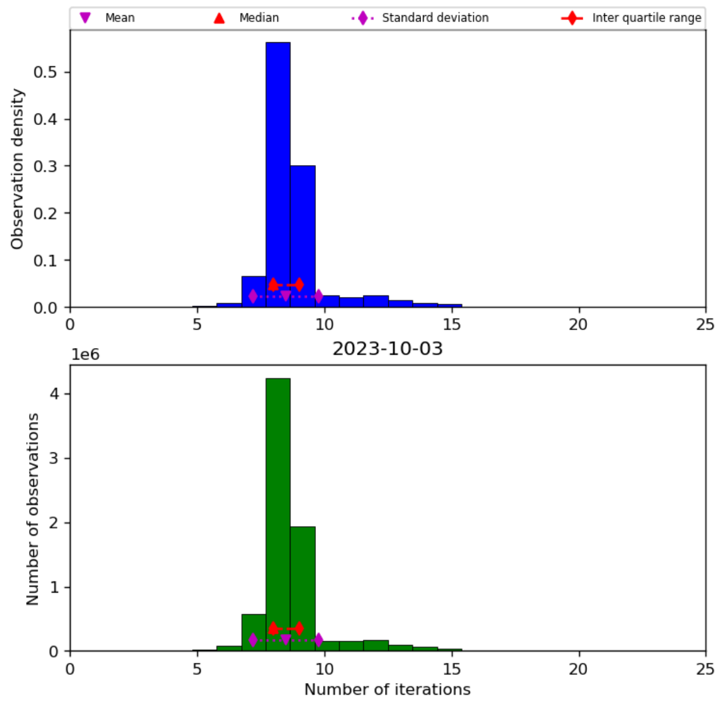
Figure 24: Histogram of “Number of iterations” for 2023-10-02 to 2023-10-04
