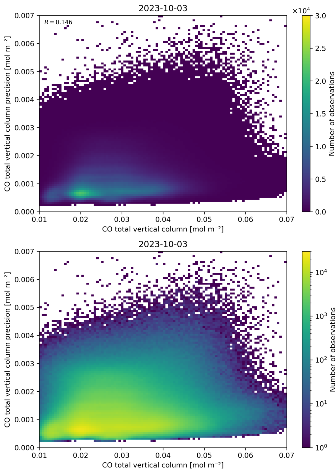
Figure 34: Scatter density plot of “CO total vertical column” against “CO total vertical column precision” for 2023-10-02 to 2023-10-04.
