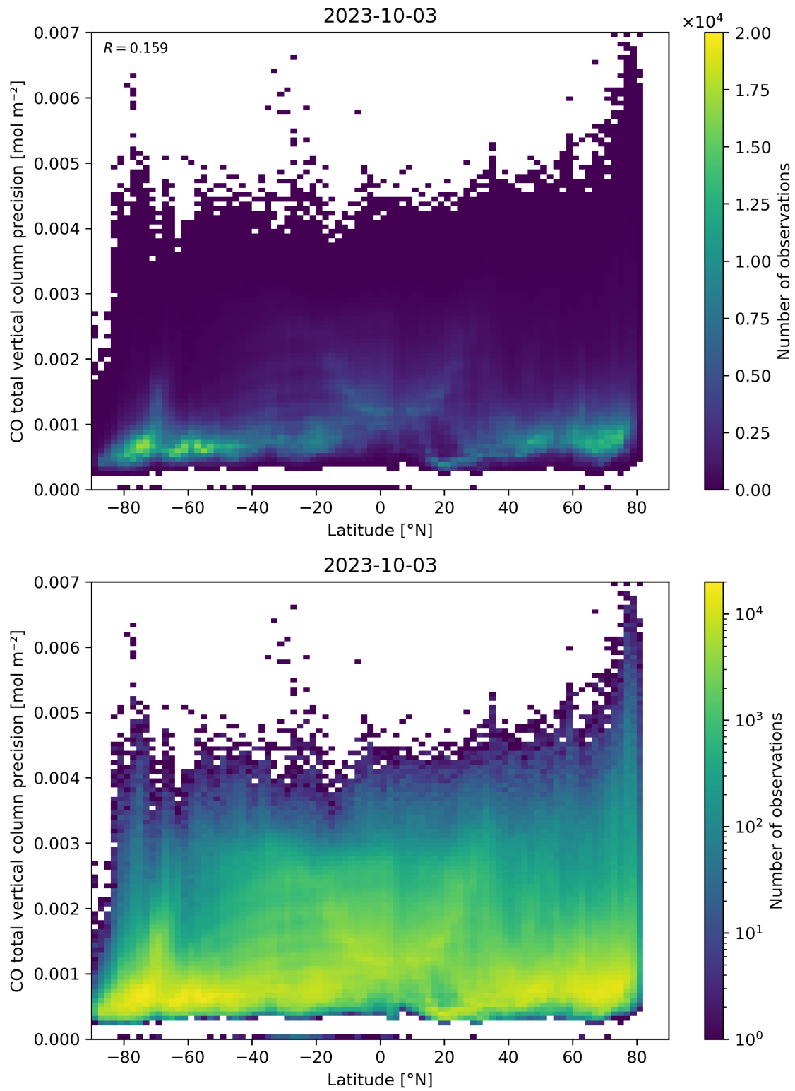
Figure 53: Scatter density plot of “Latitude” against “CO total vertical column precision” for 2023-10-02 to 2023-10-04.
