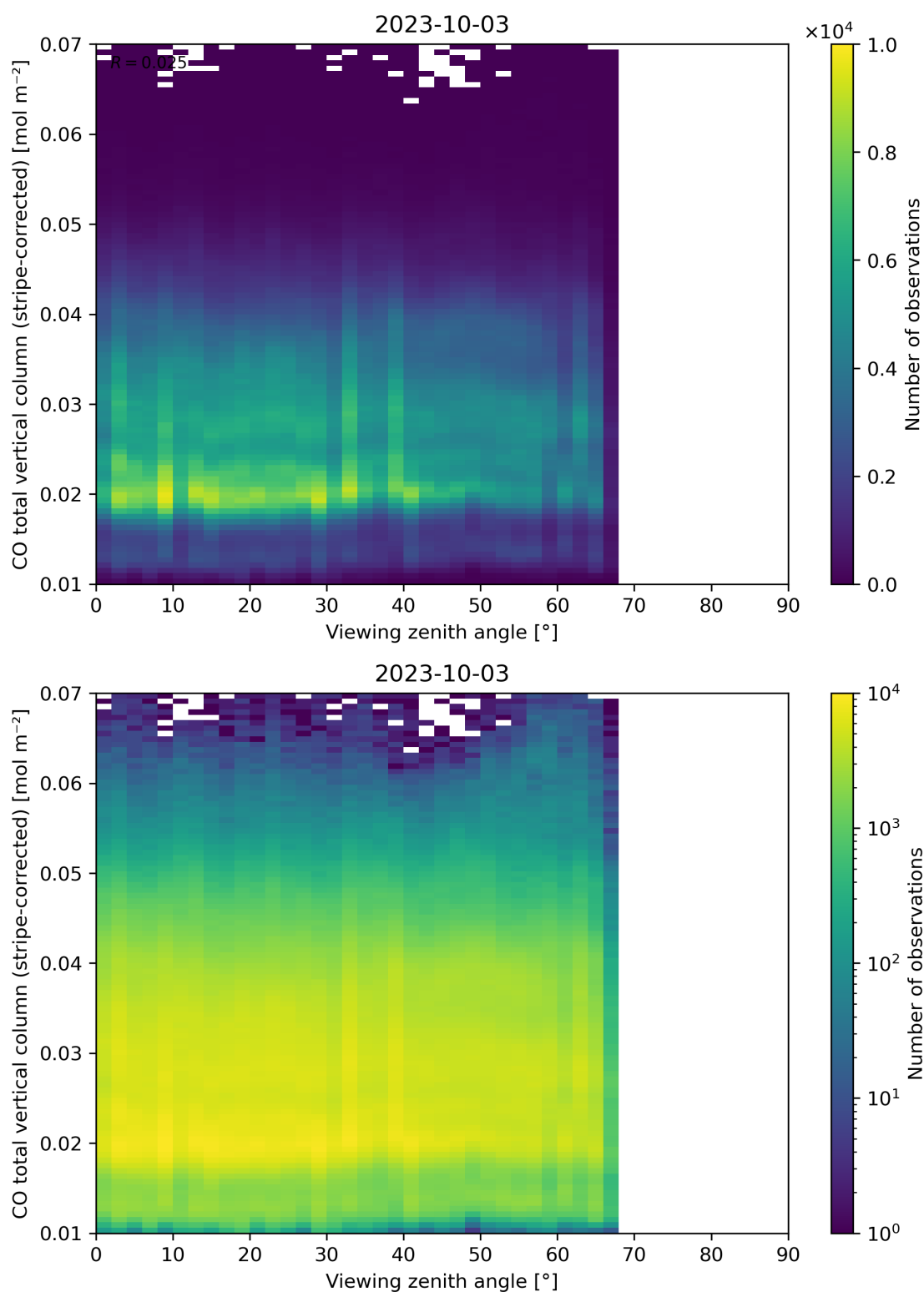
Figure 70: Scatter density plot of “Viewing zenith angle” against “CO total vertical column (stripe-corrected)” for 2023-10-02 to 2023-10-04.
