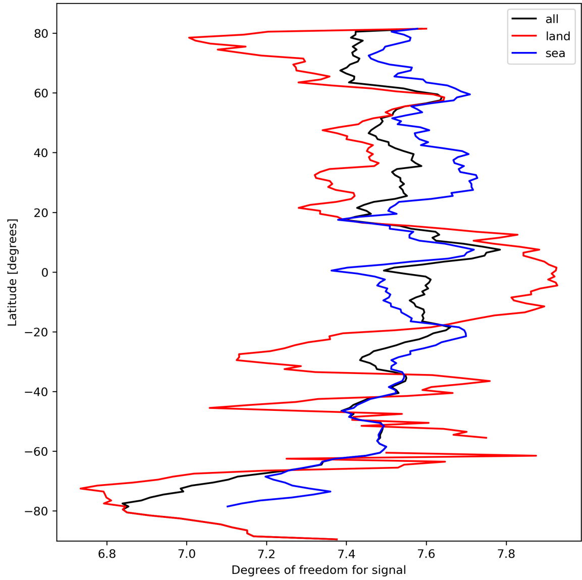
Figure 15: Zonal average of “Degrees of freedom for signal” for 2023-10-02 to 2023-10-04.
