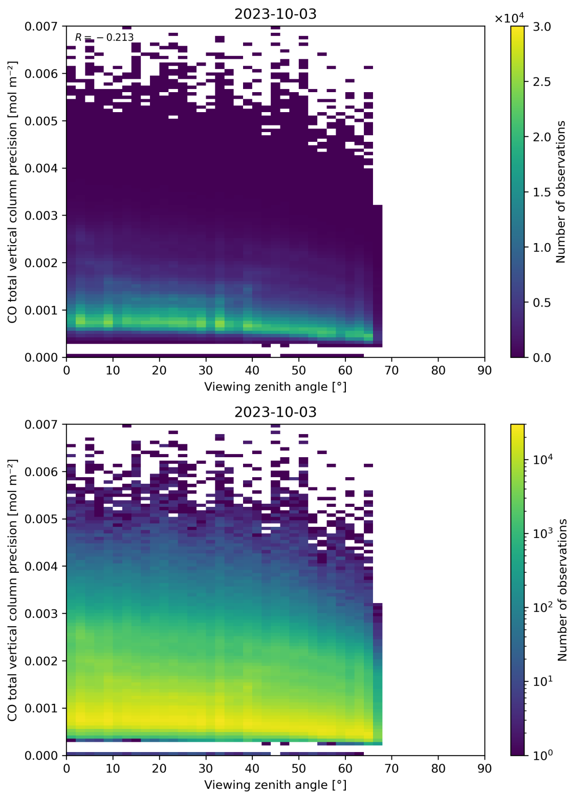
Figure 71: Scatter density plot of “Viewing zenith angle” against “CO total vertical column precision” for 2023-10-02 to 2023-10-04.
