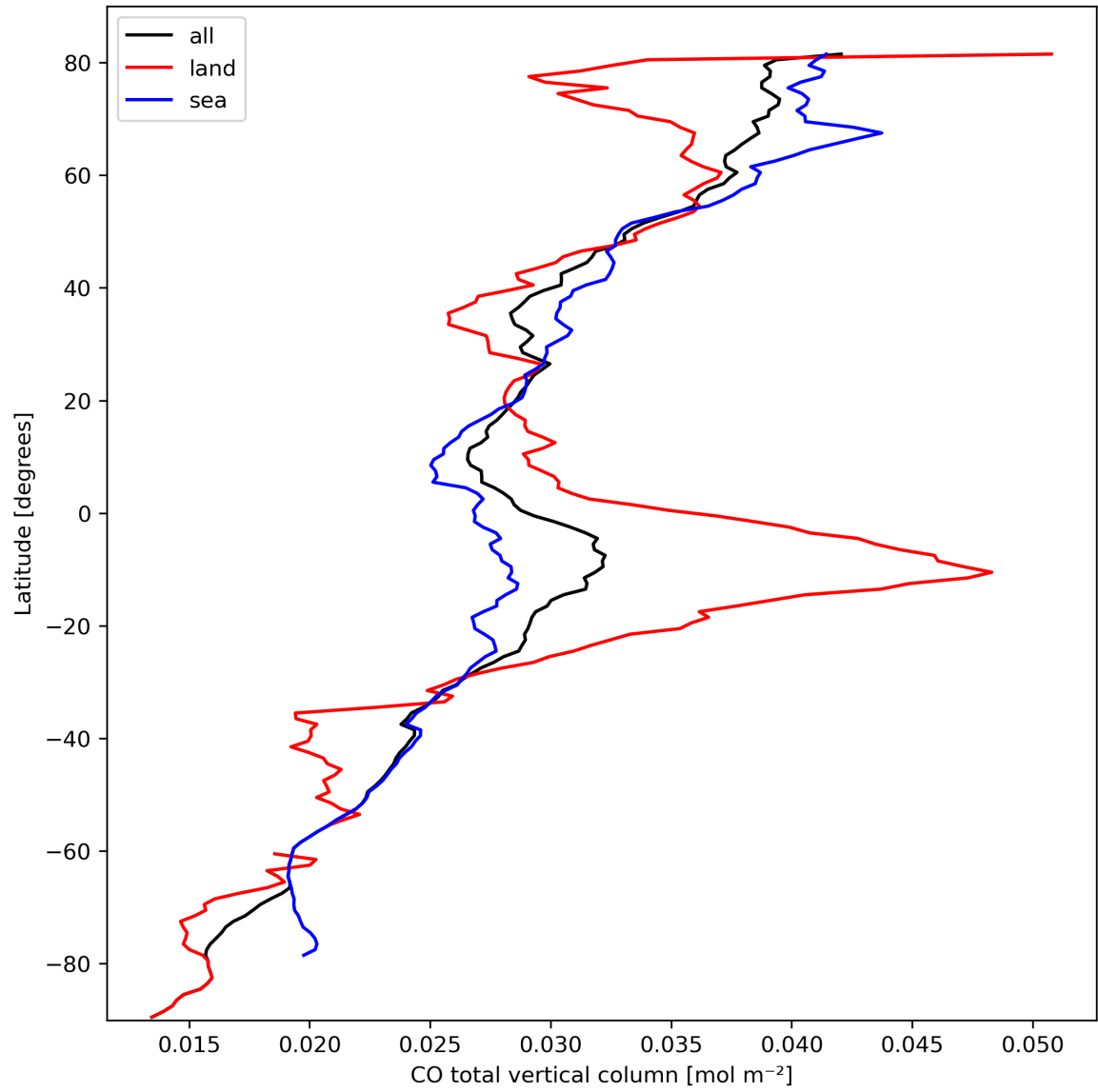
Figure 10: Zonal average of “CO total vertical column” for 2023-10-02 to 2023-10-04.
