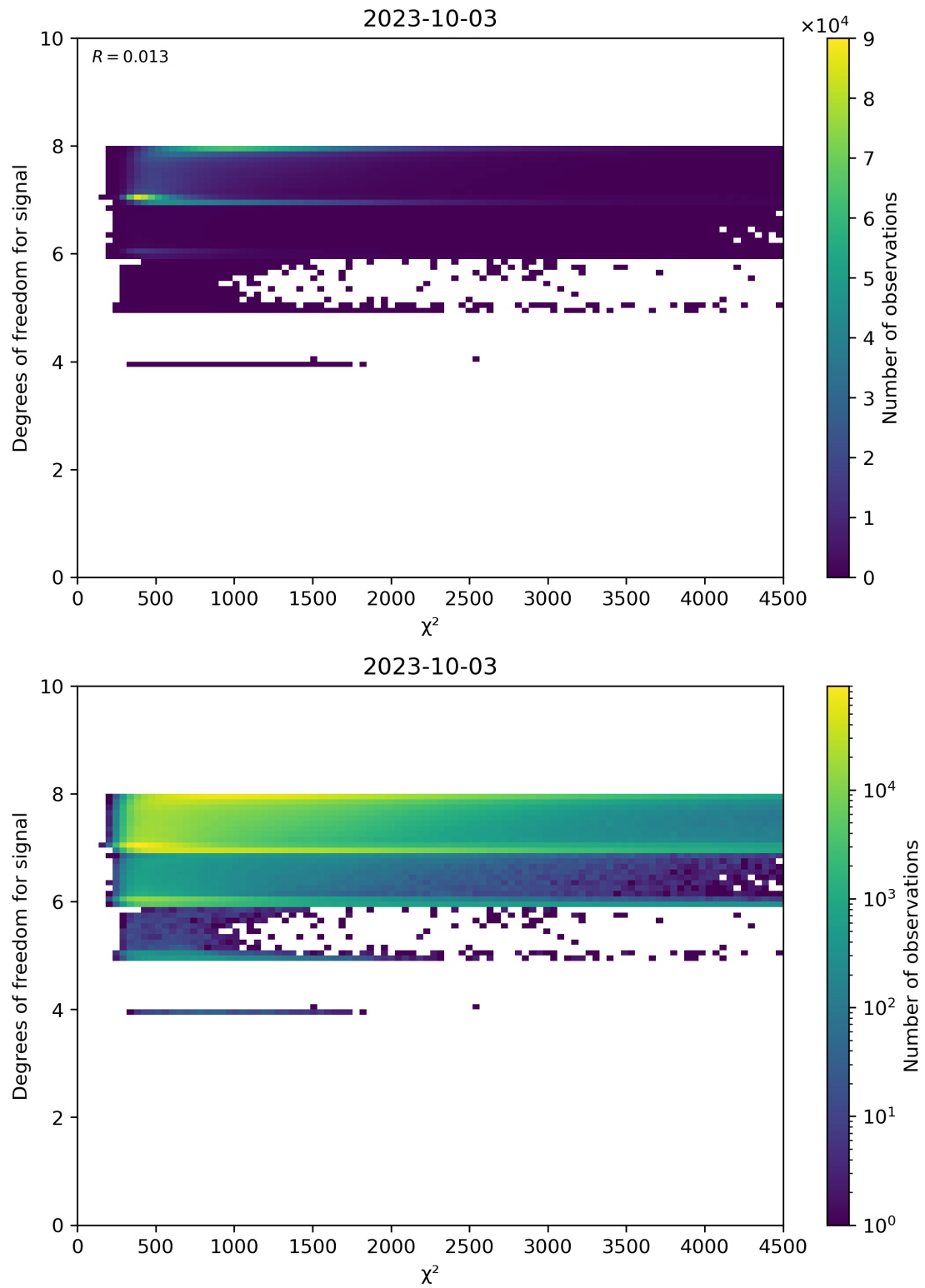
Figure 48: Scatter density plot of “ \chi^2 ” against “Degrees of freedom for signal” for 2023-10-02 to 2023-10-04.
