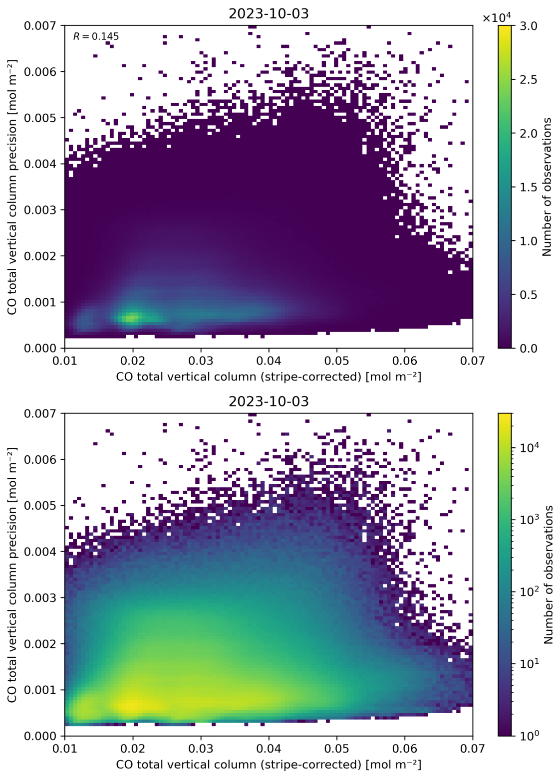
Figure 36: Scatter density plot of “CO total vertical column (stripe-corrected)” against “CO total vertical column precision” for 2023-10-02 to 2023-10-04.
