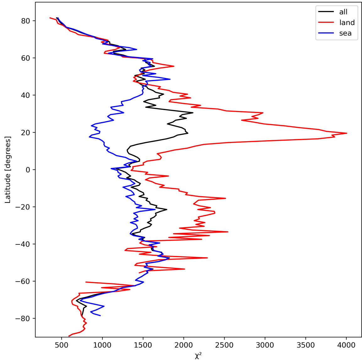
Figure 14: Zonal average of “ \chi^2 ” for 2023-10-02 to 2023-10-04.
