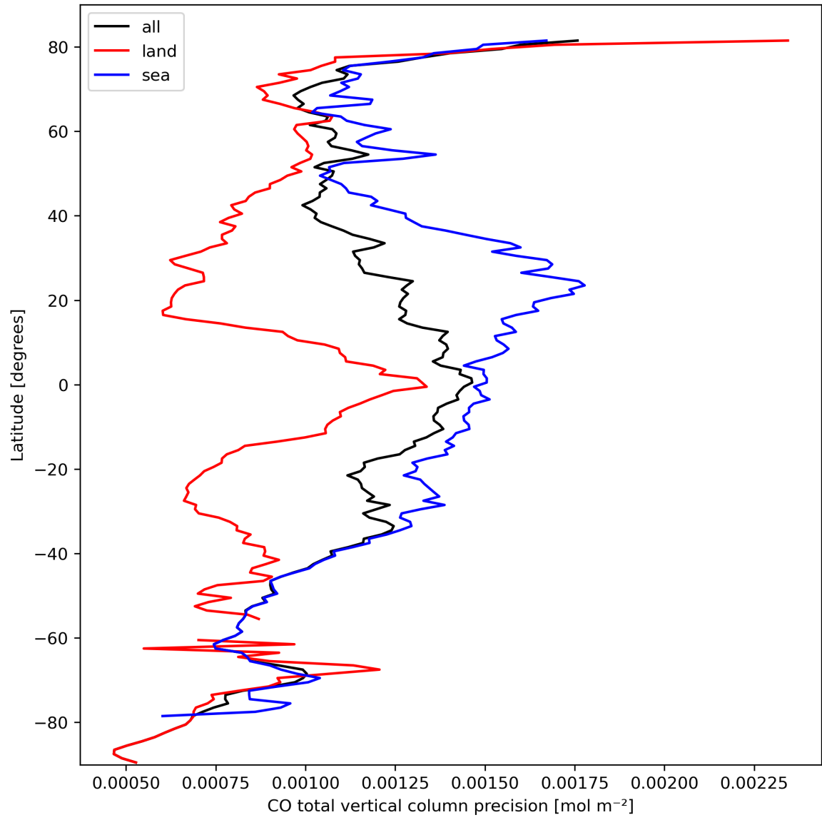
Figure 12: Zonal average of “CO total vertical column precision” for 2023-10-02 to 2023-10-04.
