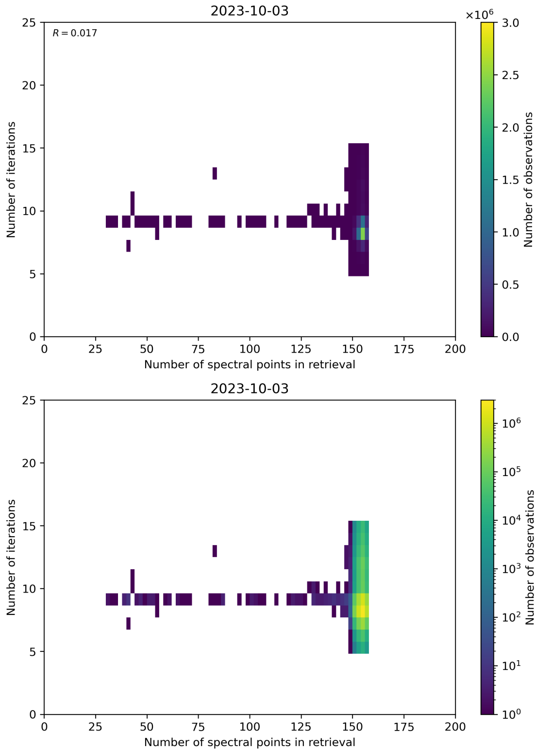
Figure 60: Scatter density plot of “Number of spectral points in retrieval” against “Number of iterations” for 2023-10-02 to 2023-10-04.
