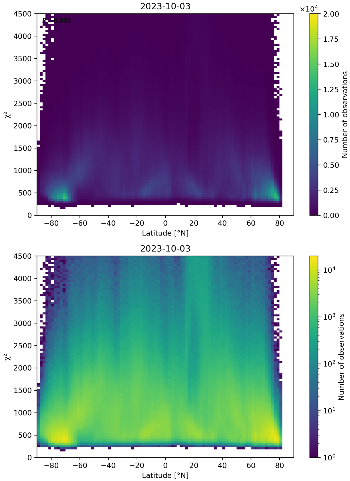
Figure 54: Scatter density plot of “Latitude” against “ \chi^2 ” for 2023-10-02 to 2023-10-04.
