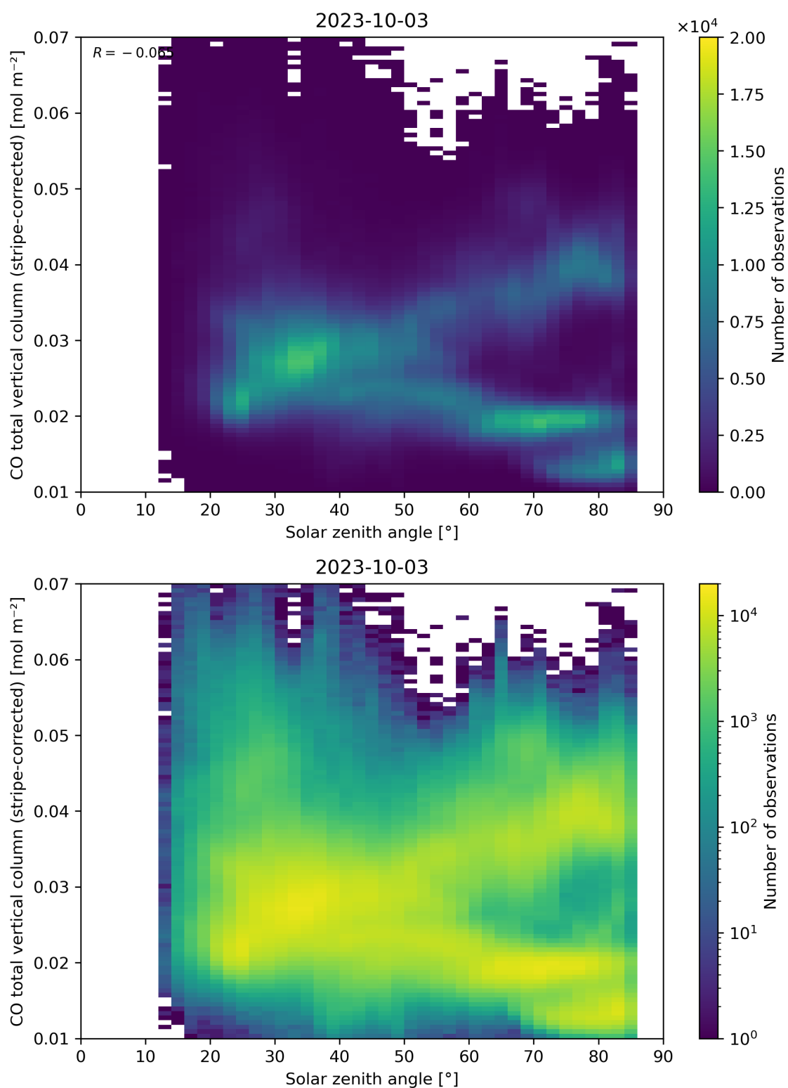
Figure 62: Scatter density plot of “Solar zenith angle” against “CO total vertical column (stripe-corrected)” for 2023-10-02 to 2023-10-04.
