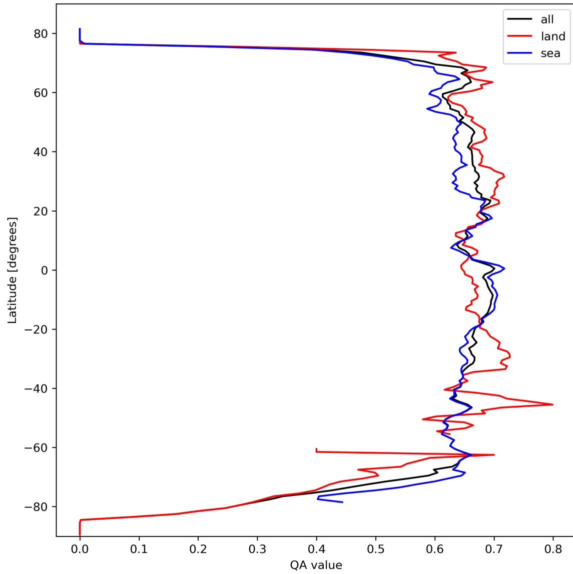
Figure 9: Zonal average of “QA value” for 2023-10-02 to 2023-10-04.
