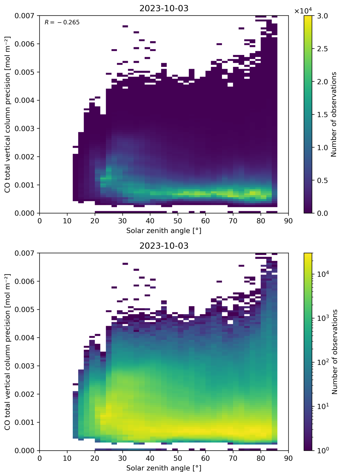
Figure 63: Scatter density plot of “Solar zenith angle” against “CO total vertical column precision” for 2023-10-02 to 2023-10-04.
