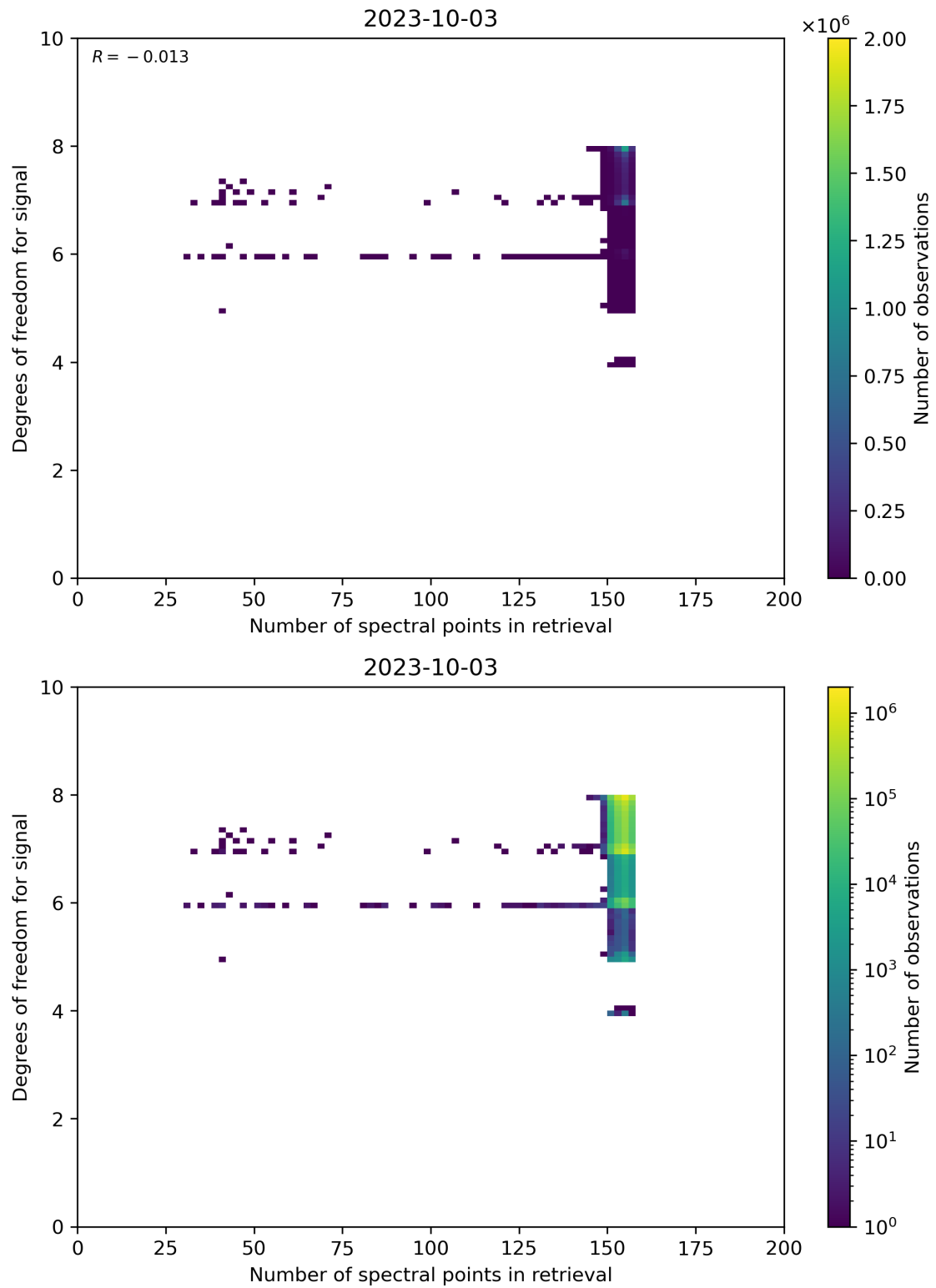
Figure 59: Scatter density plot of “Number of spectral points in retrieval” against “Degrees of freedom for signal” for 2023-10-02 to 2023-10-04.
