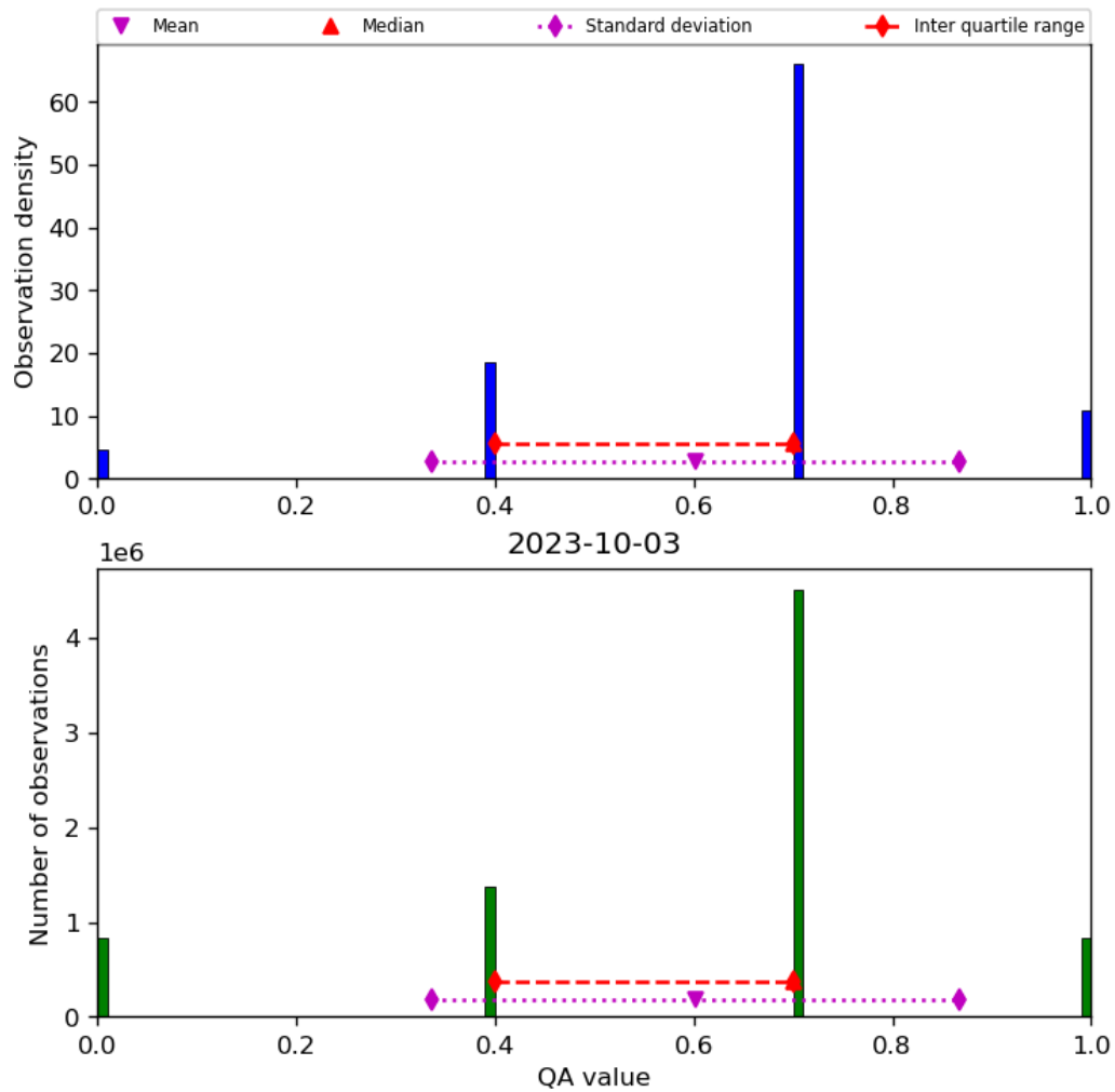
Figure 17: Histogram of "QA value" for 2023-10-02 to 2023-10-04
