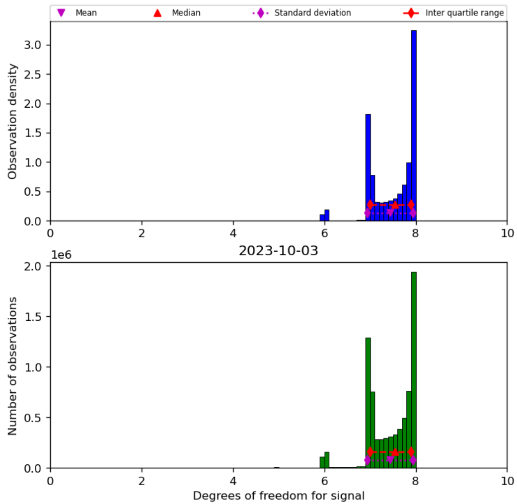
Figure 23: Histogram of “Degrees of freedom for signal” for 2023-10-02 to 2023-10-04
