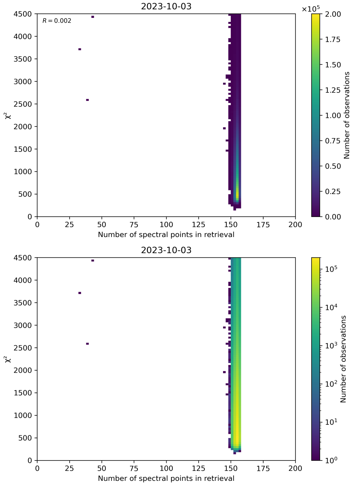
Figure 58: Scatter density plot of “Number of spectral points in retrieval” against “ \chi^2 ” for 2023-10-02 to 2023-10-04.
