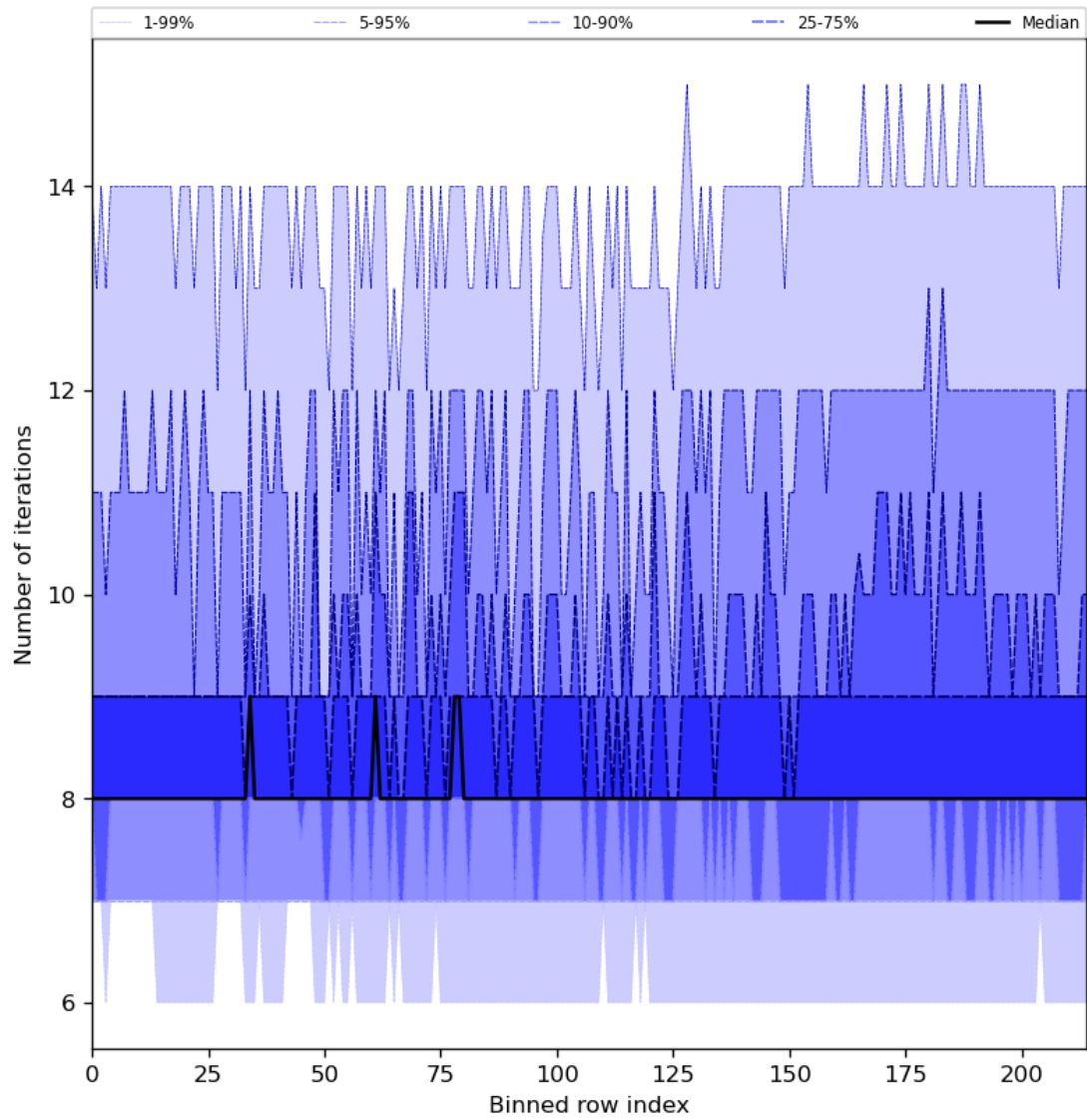
Figure 32: Along track statistics of “Number of iterations” for 2023-10-02 to 2023-10-04
