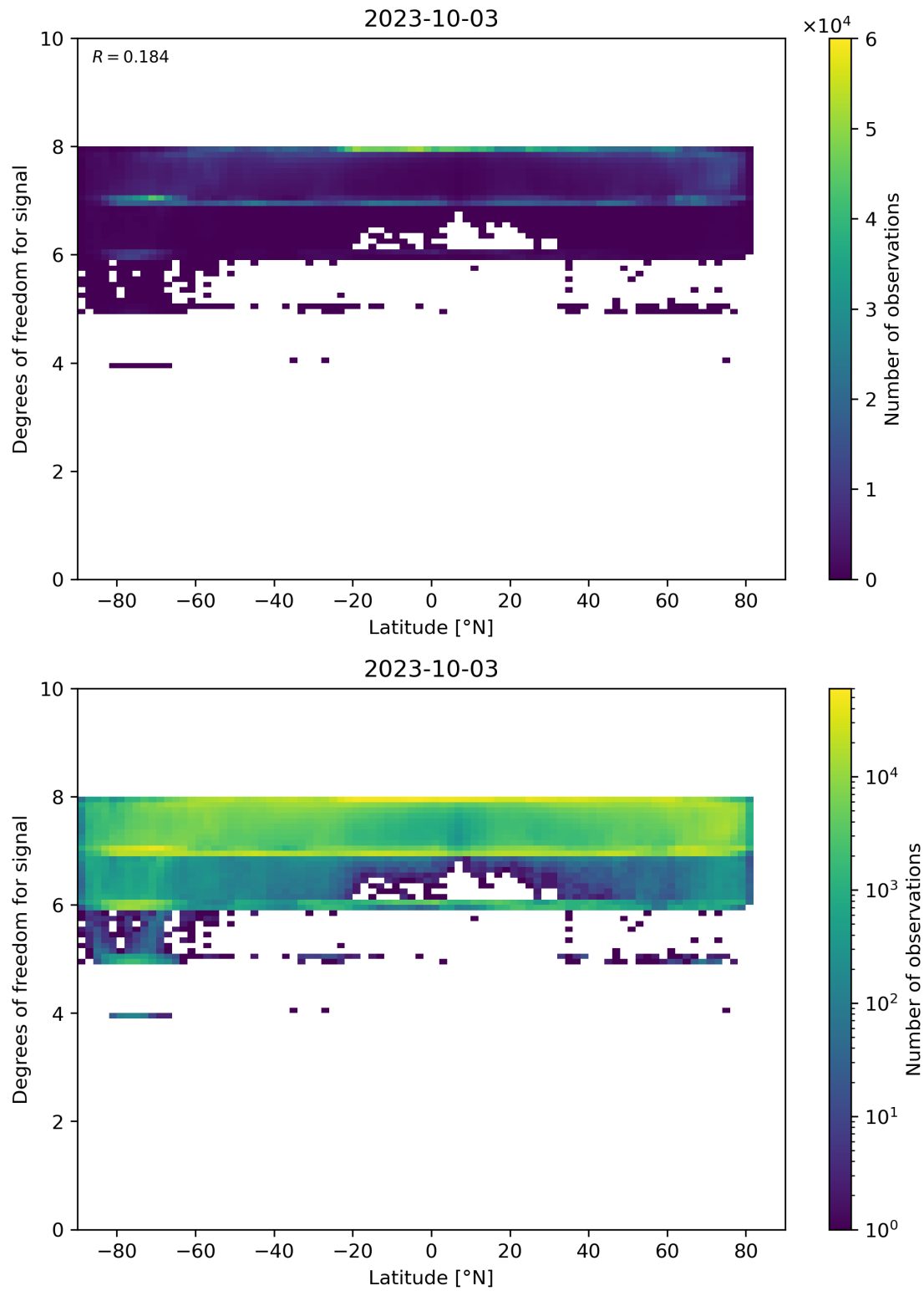
Figure 55: Scatter density plot of “Latitude” against “Degrees of freedom for signal” for 2023-10-02 to 2023-10-04.
