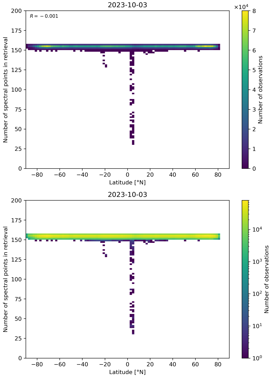
Figure 57: Scatter density plot of “Latitude” against “Number of spectral points in retrieval” for 2023-10-02 to 2023-10-04.
