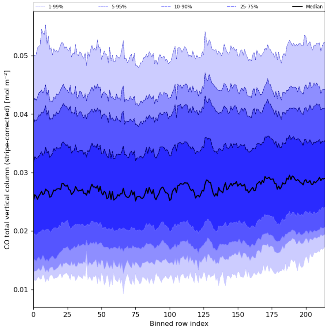
Figure 27: Along track statistics of “CO total vertical column (stripe-corrected)” for 2023-10-02 to 2023-10-04
