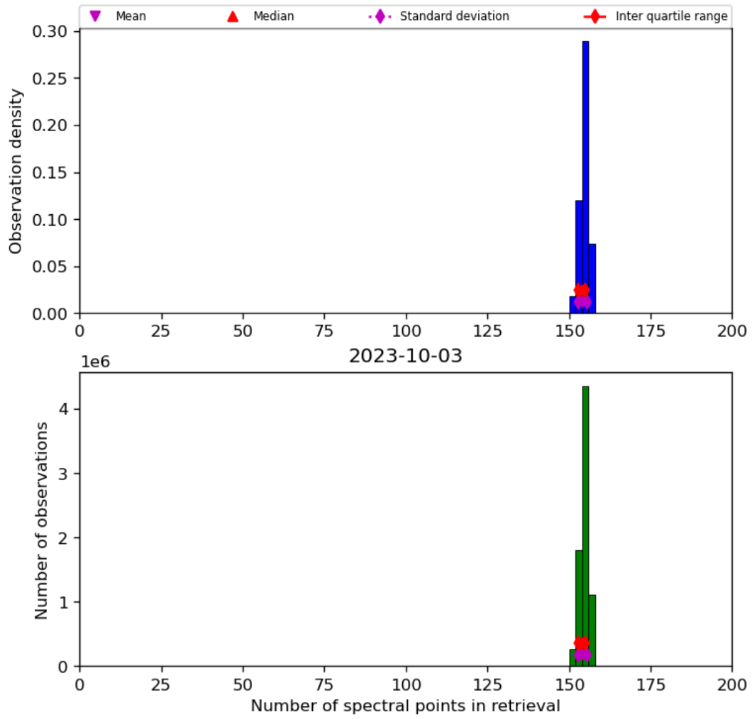
Figure 21: Histogram of “Number of spectral points in retrieval” for 2023-10-02 to 2023-10-04
