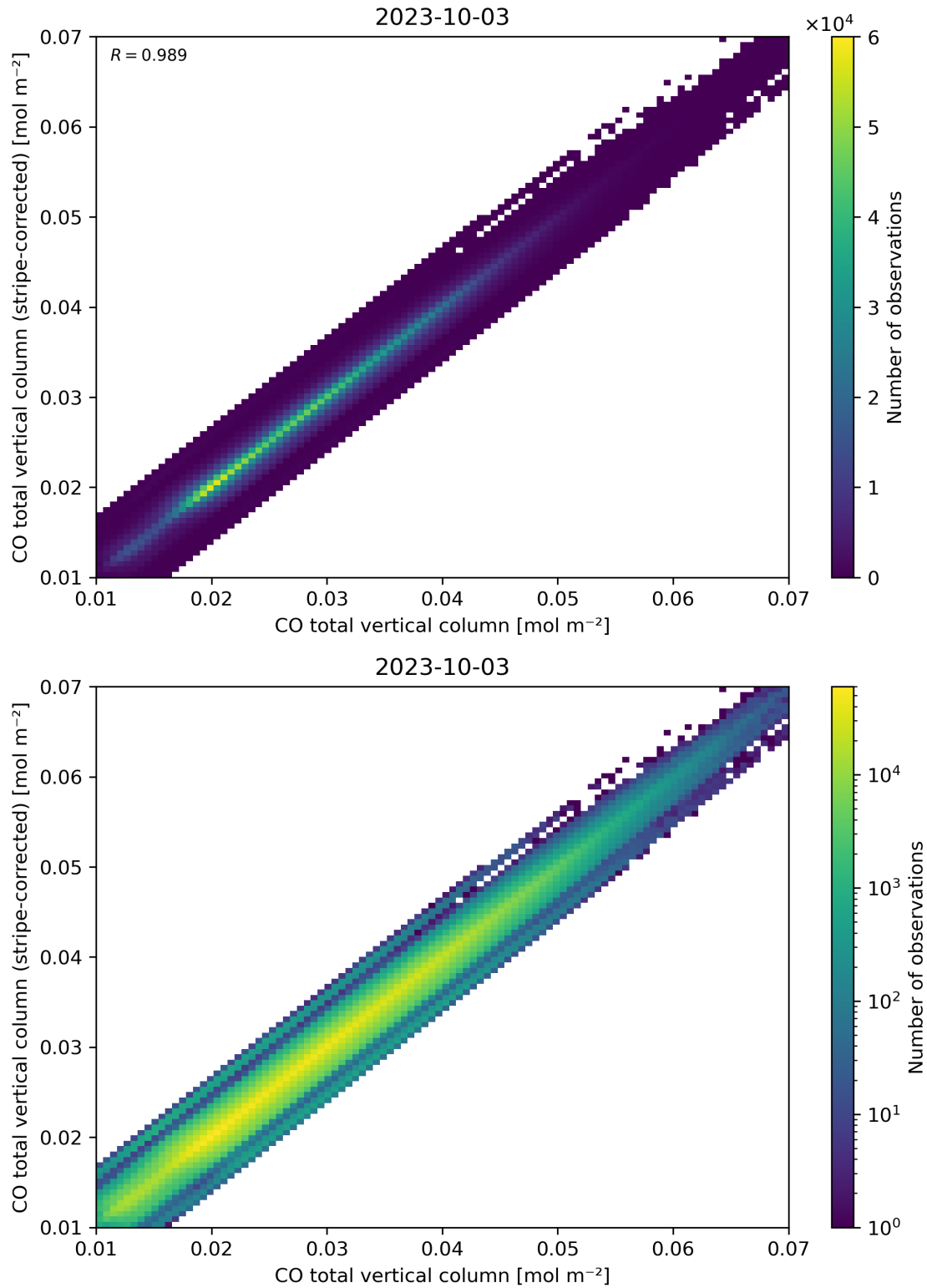
Figure 33: Scatter density plot of “CO total vertical column” against “CO total vertical column (stripe-corrected)” for 2023-10-02 to 2023-10-04.
