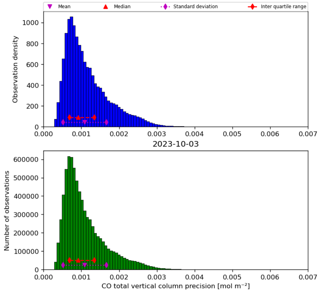
Figure 20: Histogram of “CO total vertical column precision” for 2023-10-02 to 2023-10-04
