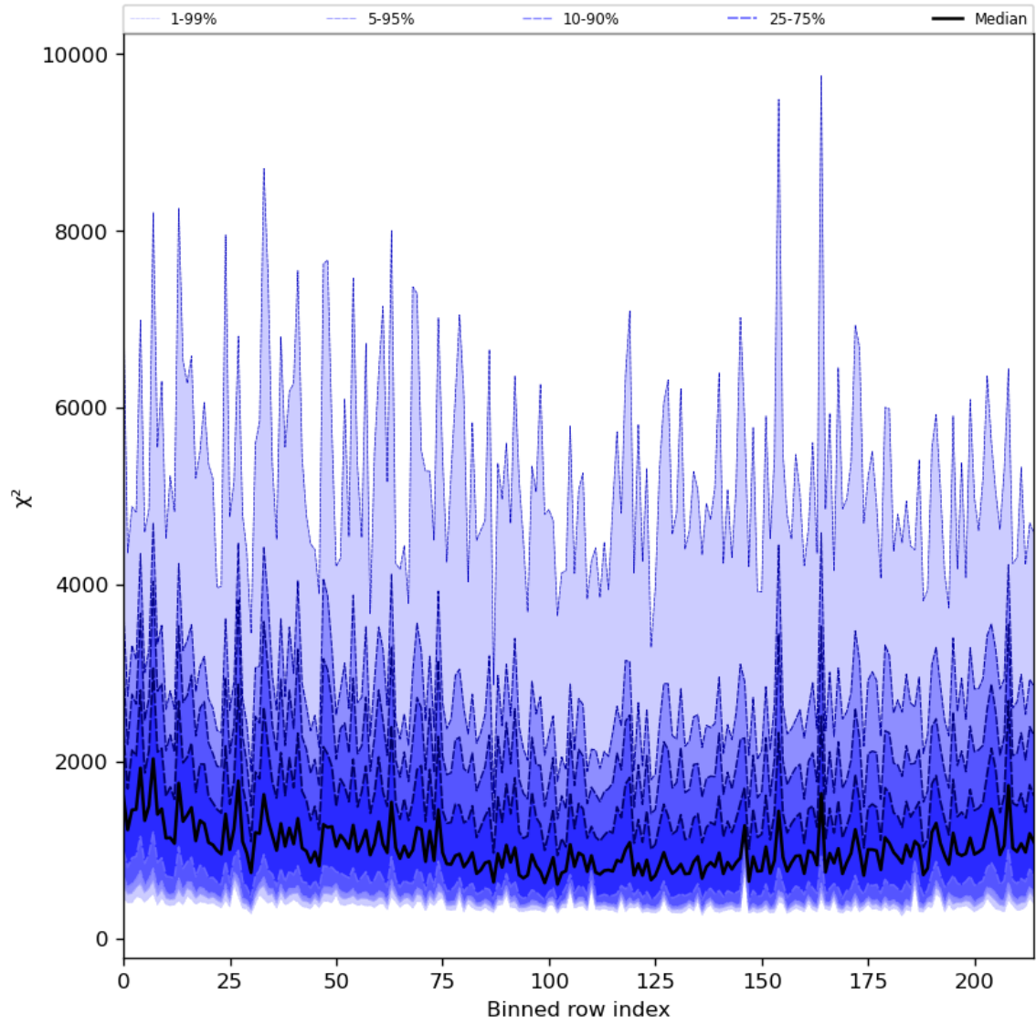
Figure 30: Along track statistics of “ \chi^2 ” for 2023-10-02 to 2023-10-04
