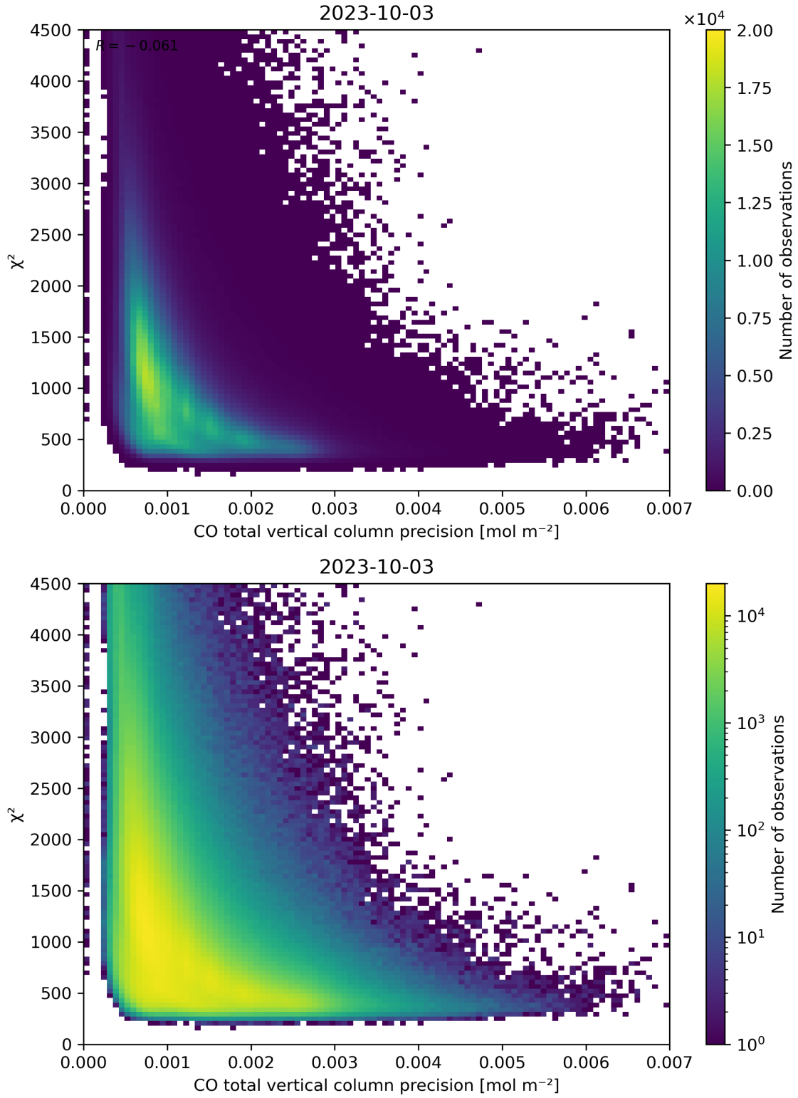
Figure 44: Scatter density plot of “CO total vertical column precision” against “ \chi^2 ” for 2023-10-02 to 2023-10-04.
