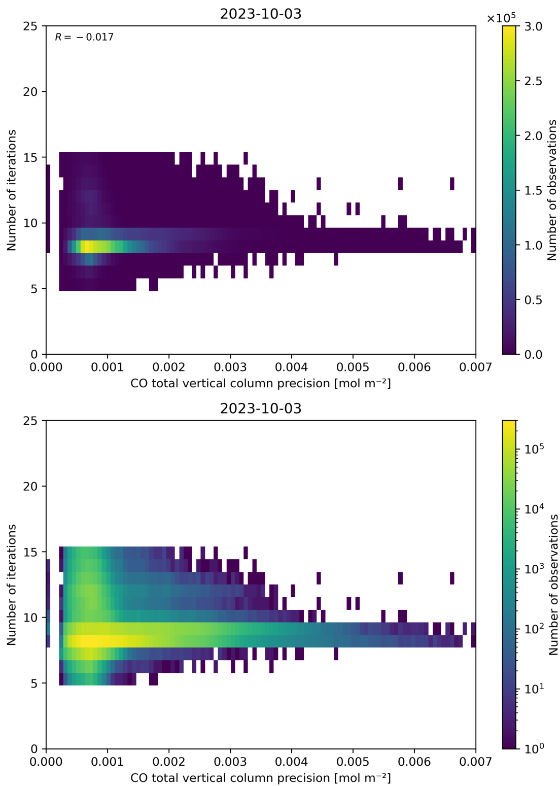
Figure 46: Scatter density plot of “CO total vertical column precision” against “Number of iterations” for 2023-10-02 to 2023-10-04.
