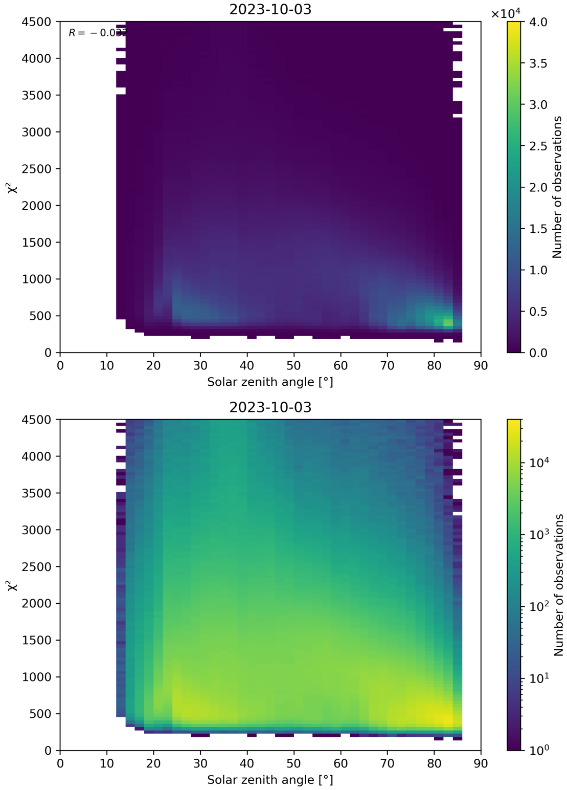
Figure 64: Scatter density plot of “Solar zenith angle” against “ \chi^2 ” for 2023-10-02 to 2023-10-04.
