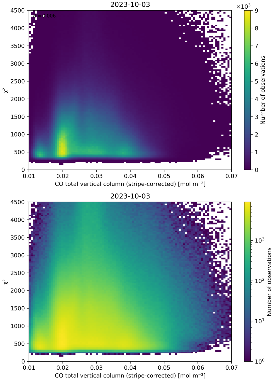
Figure 37: Scatter density plot of “CO total vertical column (stripe-corrected)” against “ \chi^2 ” for 2023-10-02 to 2023-10-04.
