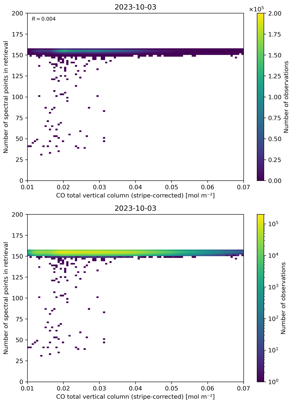
Figure 40: Scatter density plot of “CO total vertical column (stripe-corrected)” against “Number of spectral points in retrieval” for 2023-10-02 to 2023-10-04.
