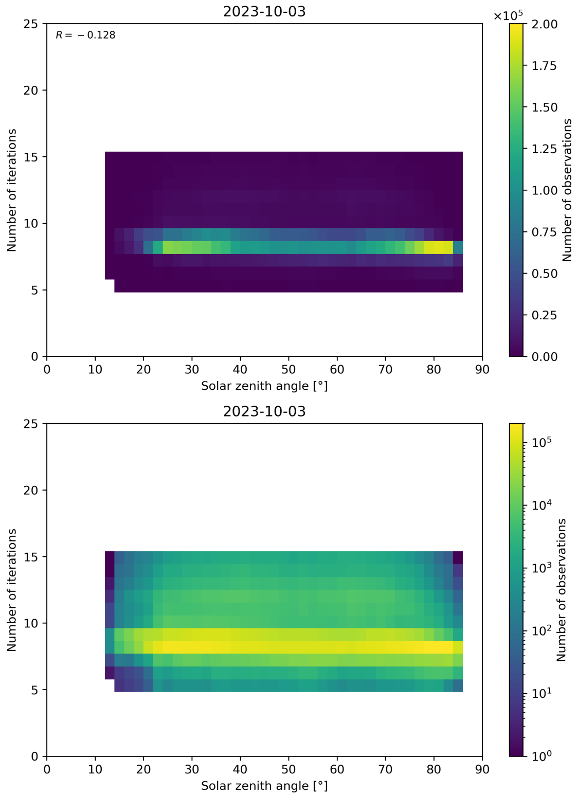
Figure 67: Scatter density plot of “Solar zenith angle” against “Number of iterations” for 2023-10-02 to 2023-10-04.
