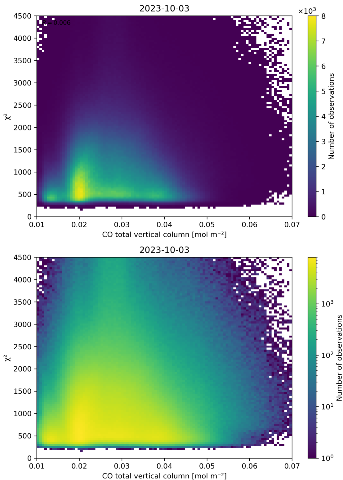
Figure 35: Scatter density plot of “CO total vertical column” against “ \chi^2 ” for 2023-10-02 to 2023-10-04.
