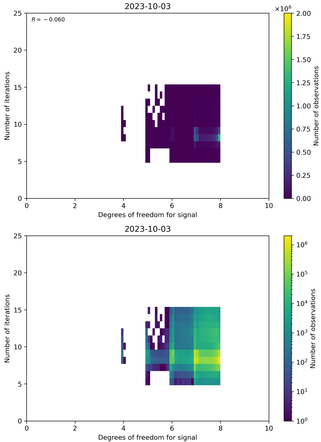
Figure 50: Scatter density plot of “Degrees of freedom for signal” against “Number of iterations” for 2023-10-02 to 2023-10-04.
