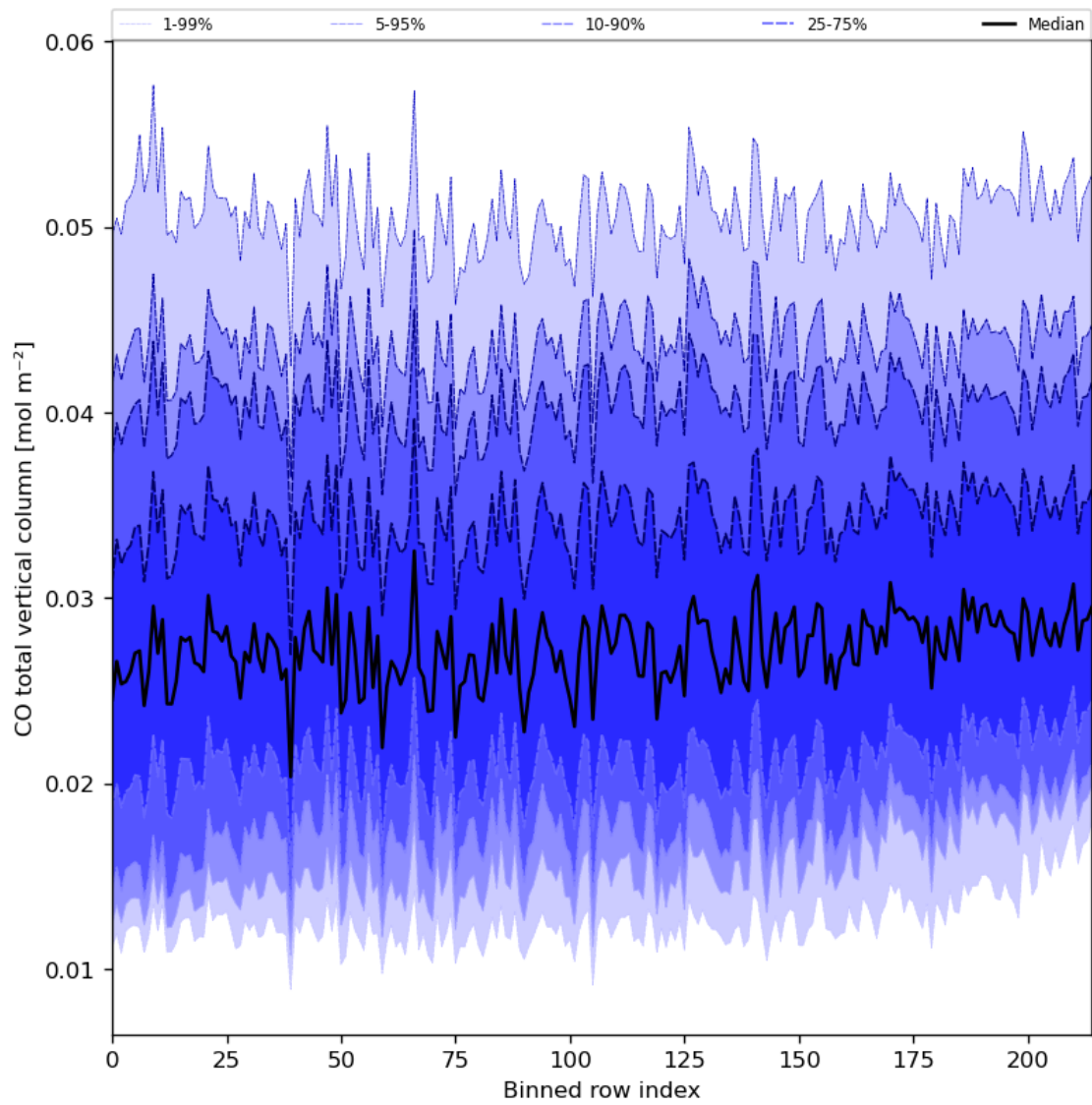
Figure 26: Along track statistics of “CO total vertical column” for 2023-10-02 to 2023-10-04
