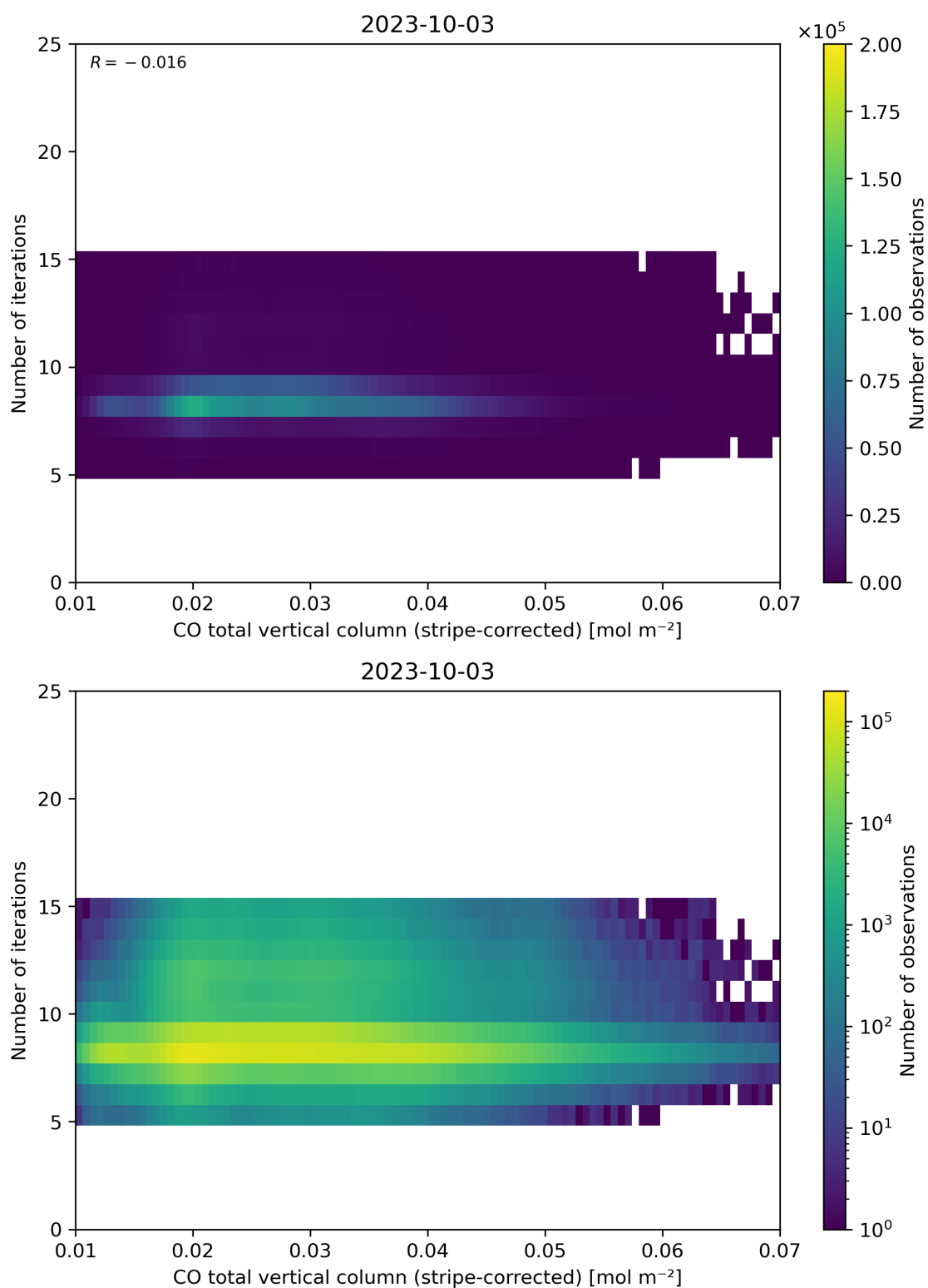
Figure 39: Scatter density plot of “CO total vertical column (stripe-corrected)” against “Number of iterations” for 2023-10-02 to 2023-10-04.
