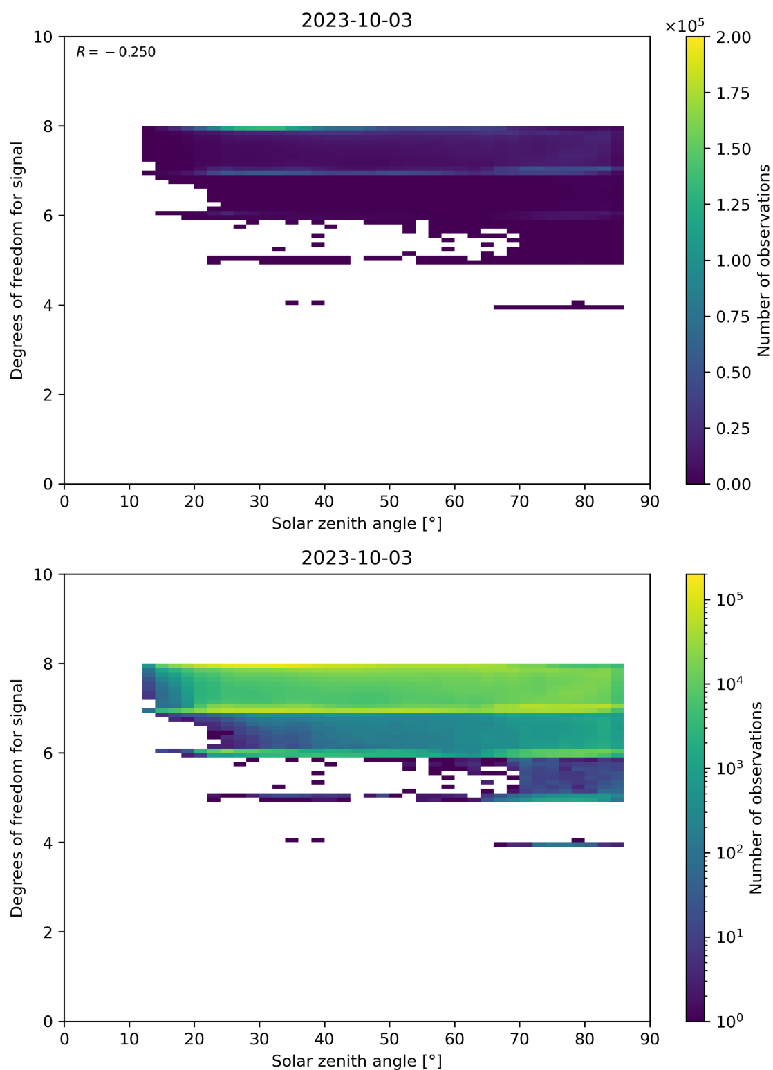
Figure 65: Scatter density plot of “Solar zenith angle” against “Degrees of freedom for signal” for 2023-10-02 to 2023-10-04.
