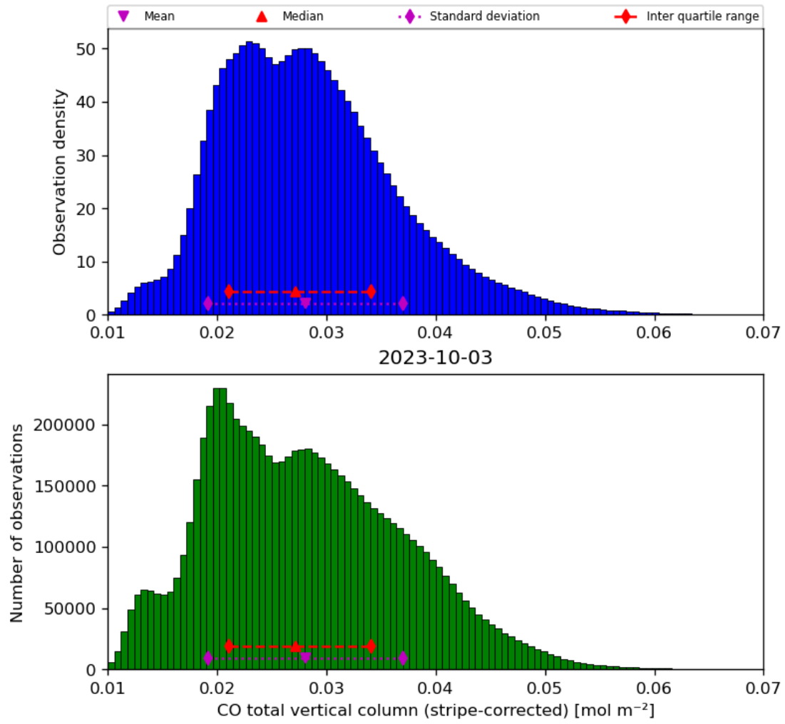
Figure 19: Histogram of “CO total vertical column (stripe-corrected)” for 2023-10-02 to 2023-10-04
