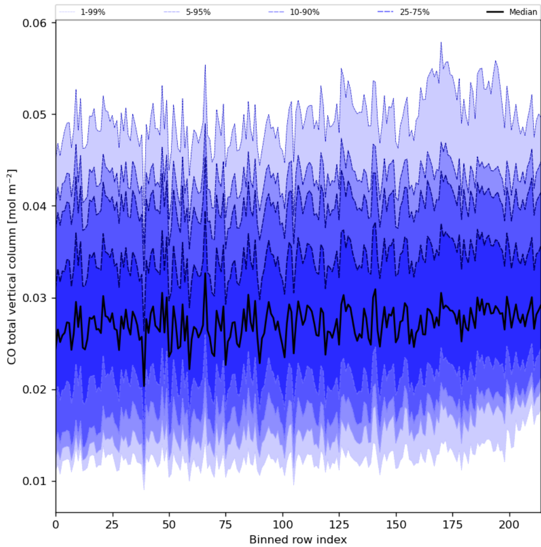
Figure 26: Along track statistics of “CO total vertical column” for 2023-10-03 to 2023-10-05
