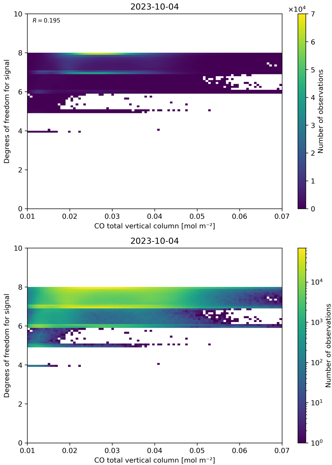
Figure 41: Scatter density plot of “CO total vertical column” against “Degrees of freedom for signal” for 2023-10-03 to 2023-10-05.
