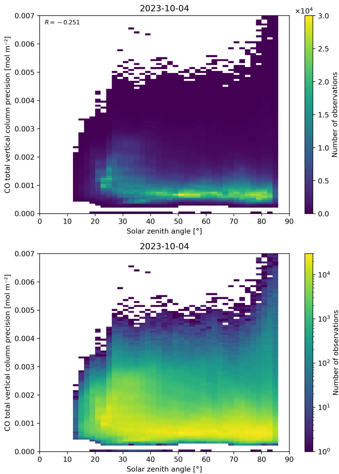
Figure 63: Scatter density plot of “Solar zenith angle” against “CO total vertical column precision” for 2023-10-03 to 2023-10-05.
