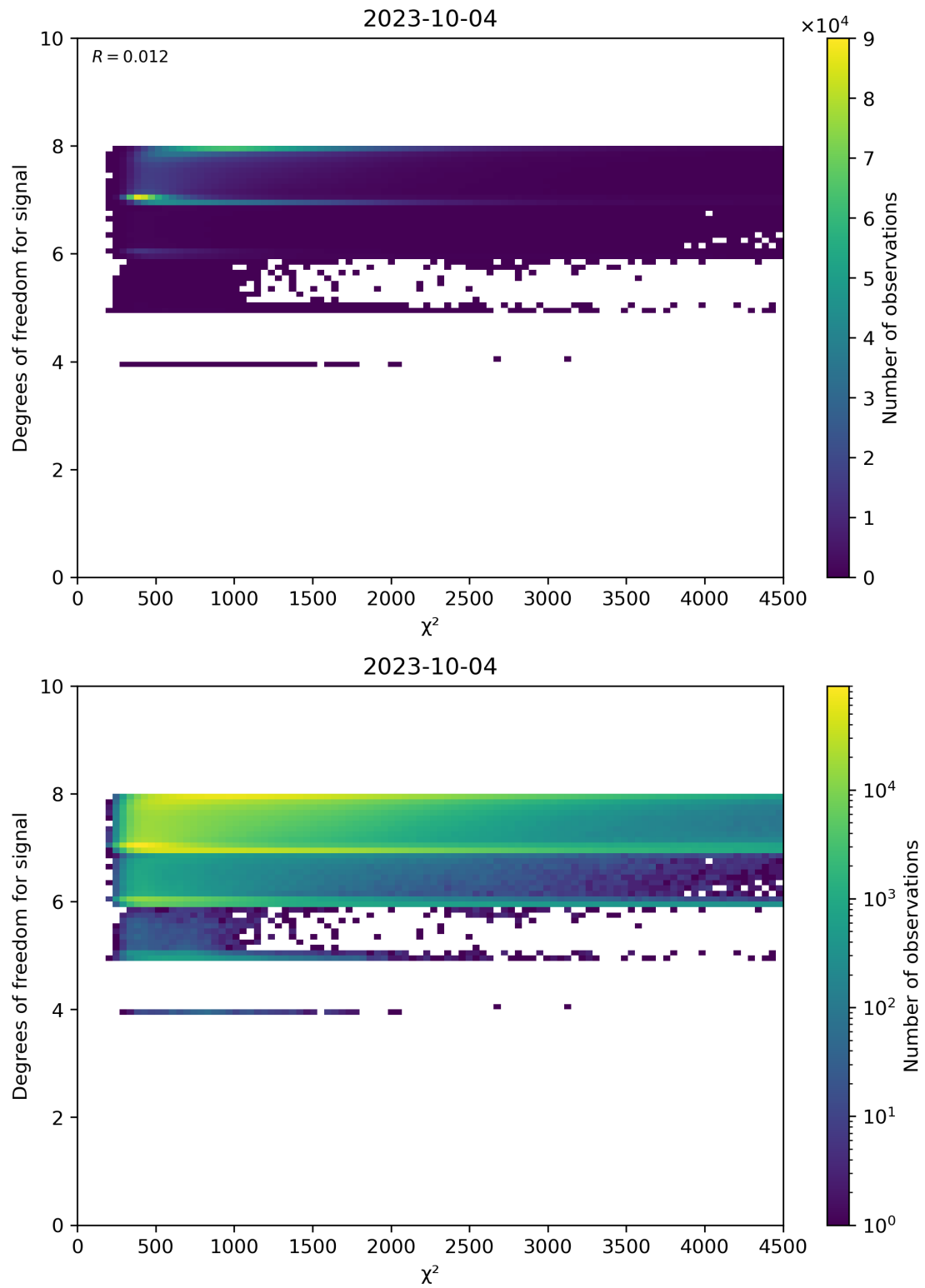
Figure 48: Scatter density plot of “ \chi^2 ” against “Degrees of freedom for signal” for 2023-10-03 to 2023-10-05.
