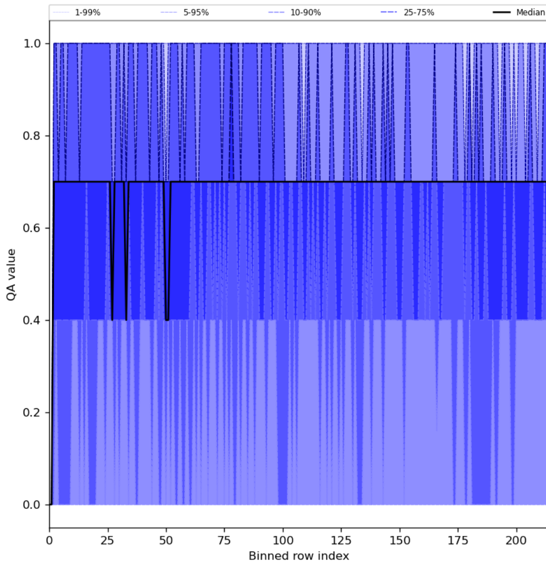
Figure 25: Along track statistics of “QA value” for 2023-10-03 to 2023-10-05
