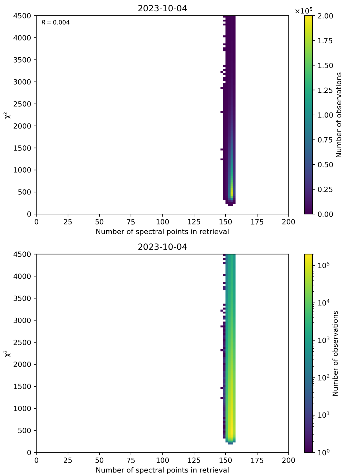
Figure 58: Scatter density plot of “Number of spectral points in retrieval” against “ \chi^2 ” for 2023-10-03 to 2023-10-05.
