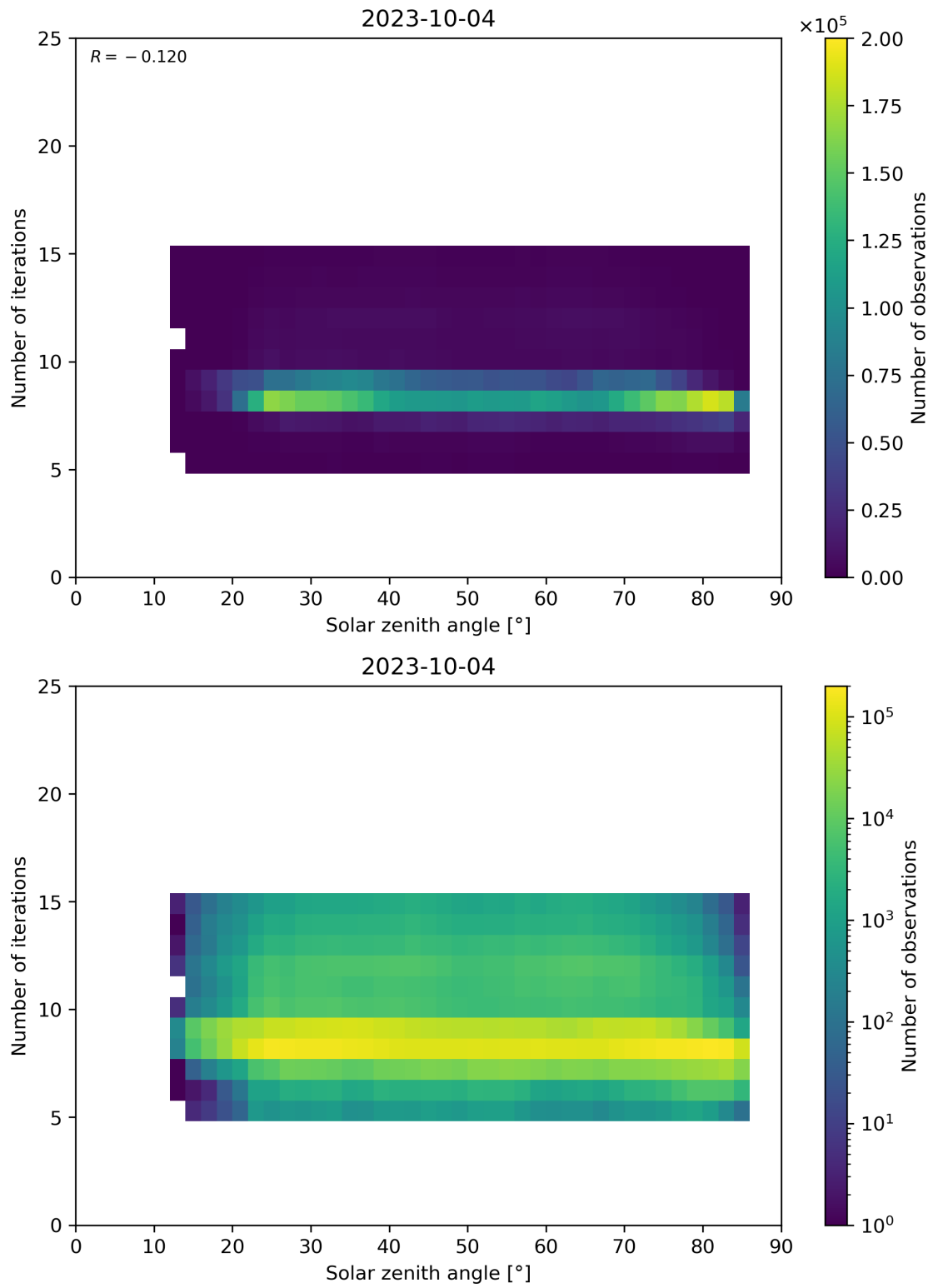
Figure 67: Scatter density plot of “Solar zenith angle” against “Number of iterations” for 2023-10-03 to 2023-10-05.
