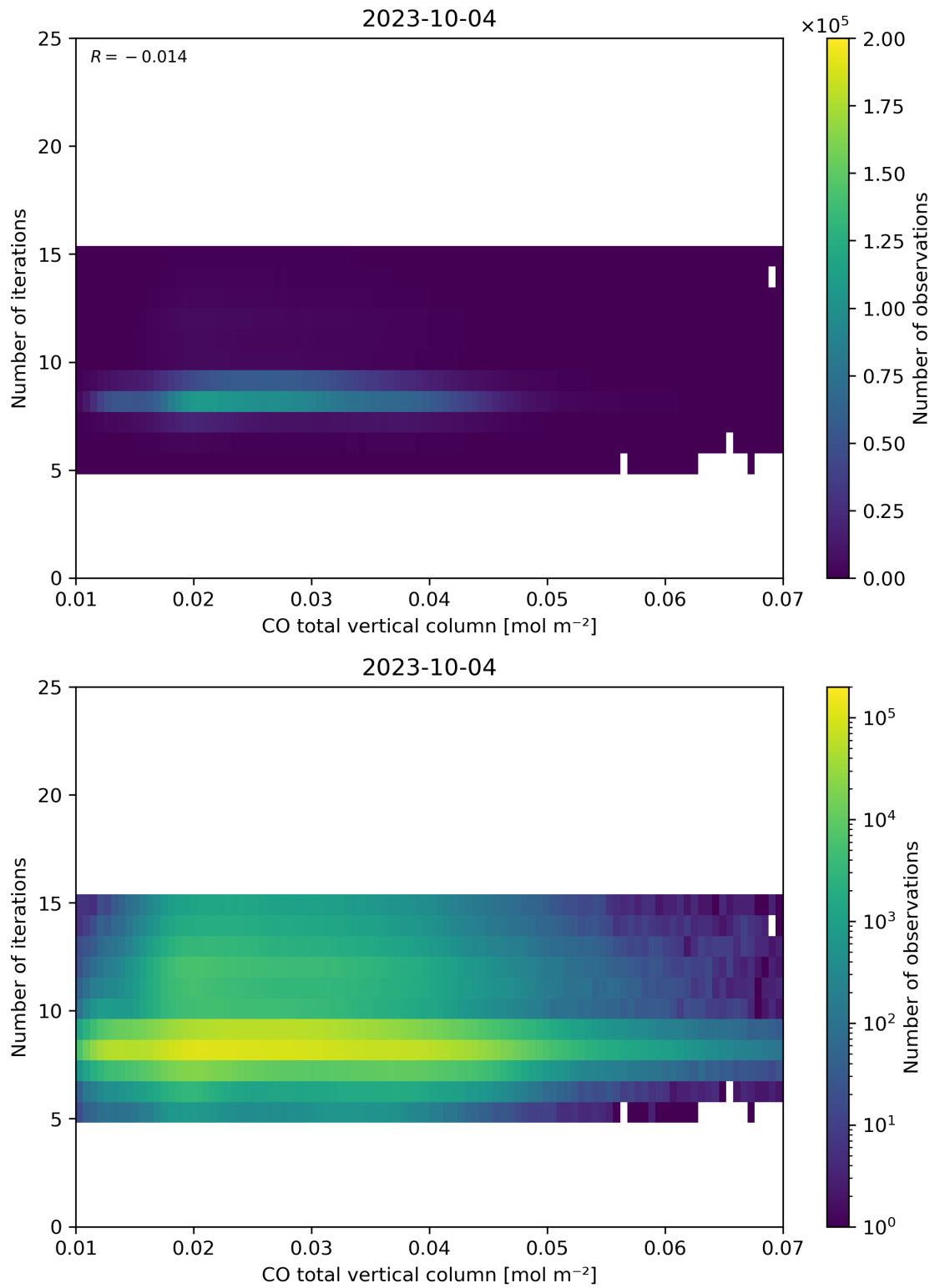
Figure 42: Scatter density plot of “CO total vertical column” against “Number of iterations” for 2023-10-03 to 2023-10-05.
