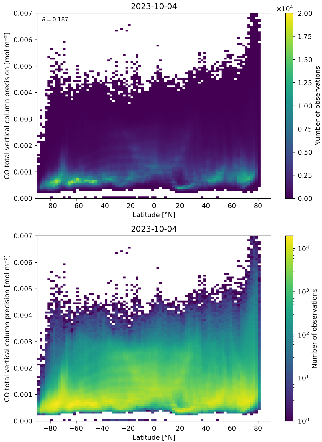
Figure 53: Scatter density plot of “Latitude” against “CO total vertical column precision” for 2023-10-03 to 2023-10-05.
