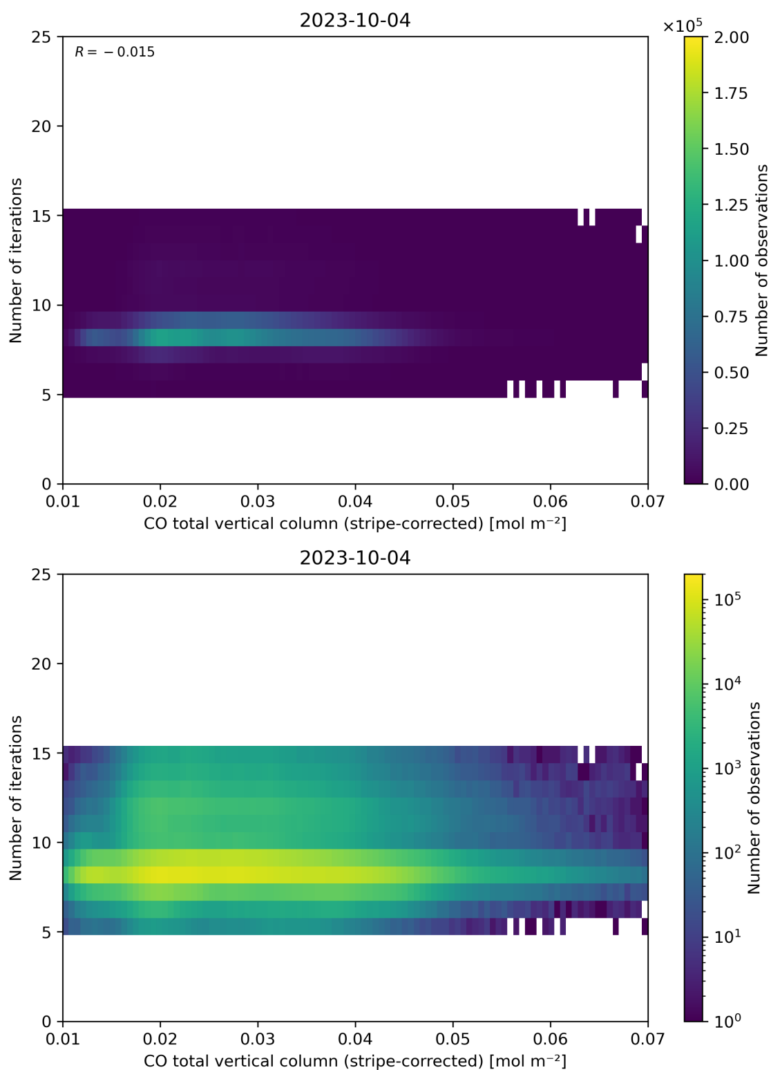
Figure 39: Scatter density plot of “CO total vertical column (stripe-corrected)” against “Number of iterations” for 2023-10-03 to 2023-10-05.
