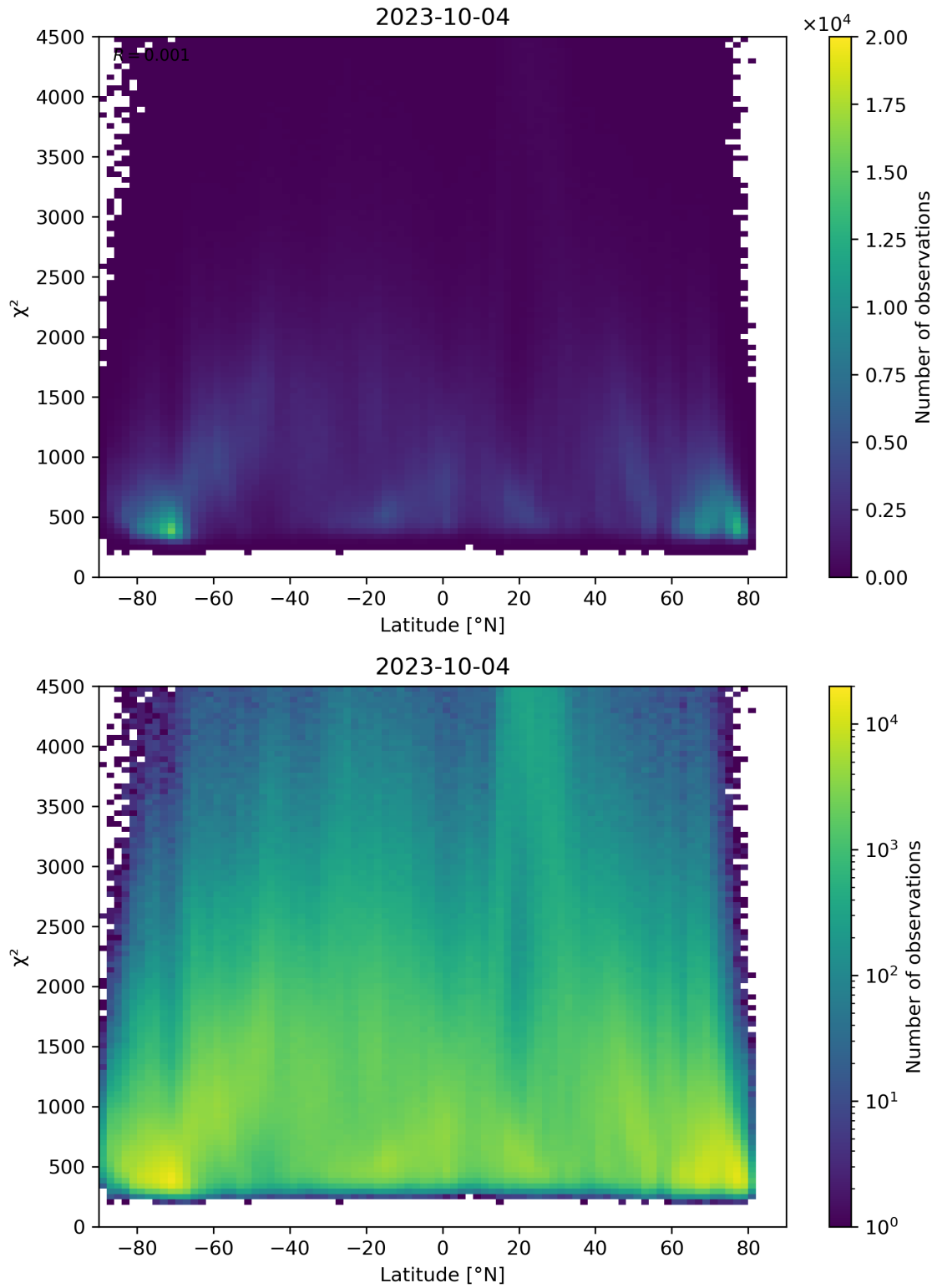
Figure 54: Scatter density plot of “Latitude” against “ \chi^2 ” for 2023-10-03 to 2023-10-05.
