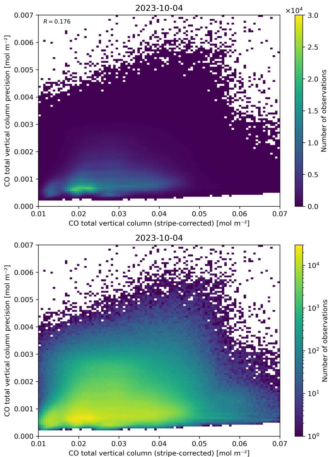
Figure 36: Scatter density plot of “CO total vertical column (stripe-corrected)” against “CO total vertical column precision” for 2023-10-03 to 2023-10-05.
