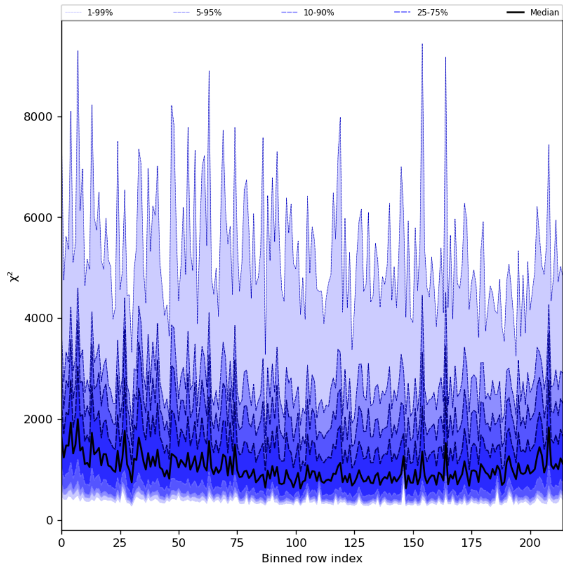
Figure 30: Along track statistics of “ \chi^2 ” for 2023-10-03 to 2023-10-05
