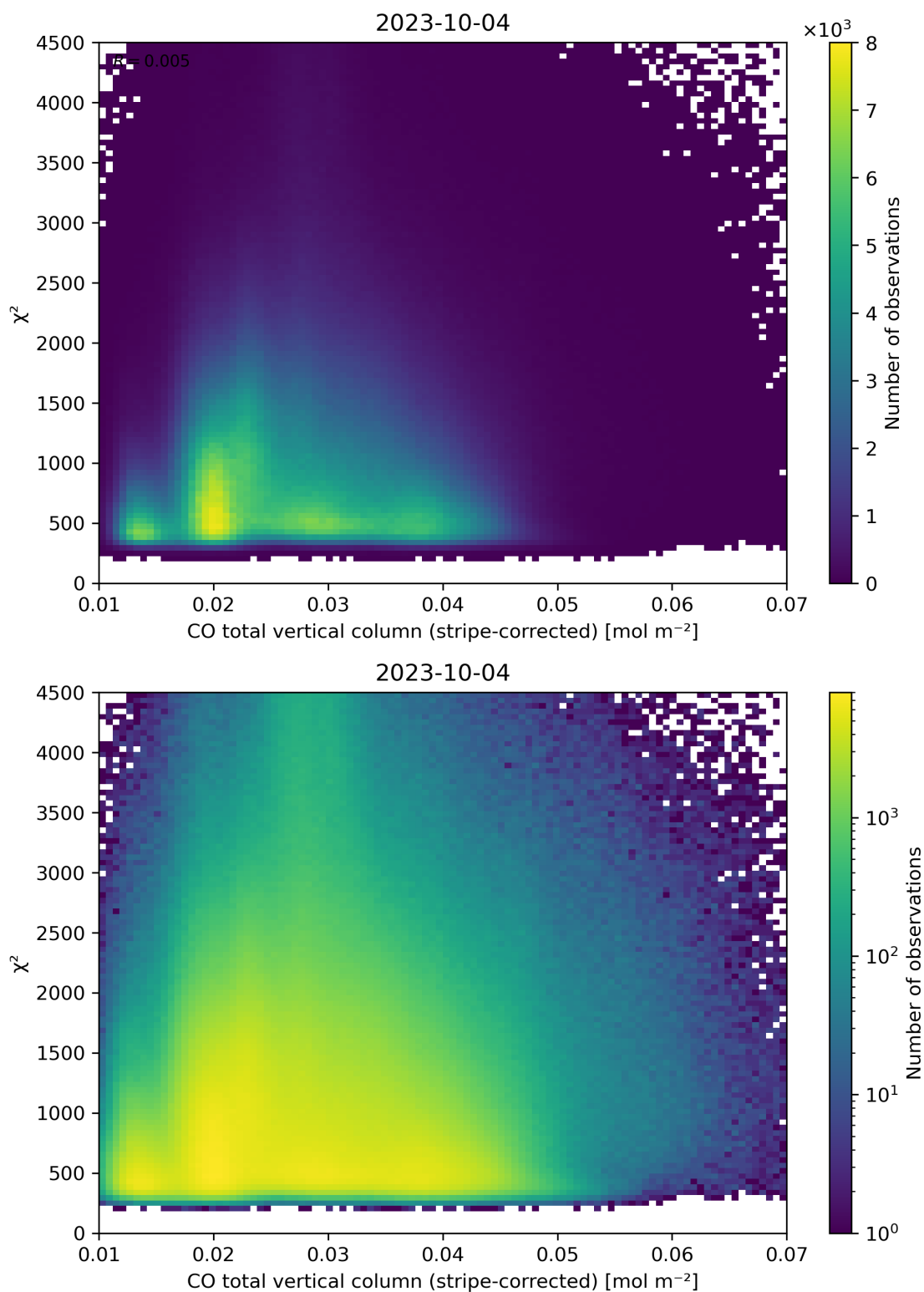
Figure 37: Scatter density plot of “CO total vertical column (stripe-corrected)” against “ \chi^2 ” for 2023-10-03 to 2023-10-05.
