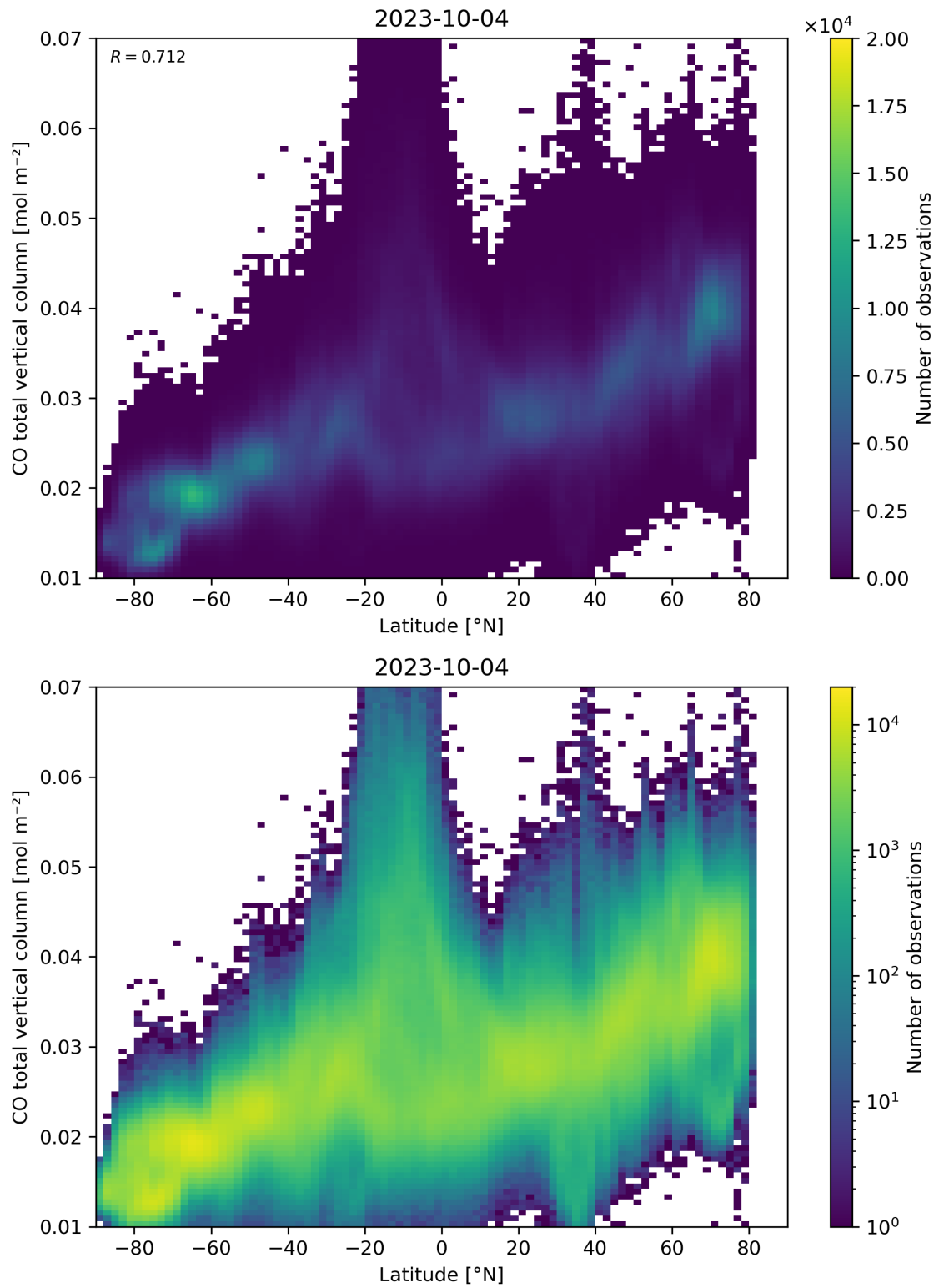
Figure 51: Scatter density plot of “Latitude” against “CO total vertical column” for 2023-10-03 to 2023-10-05.
