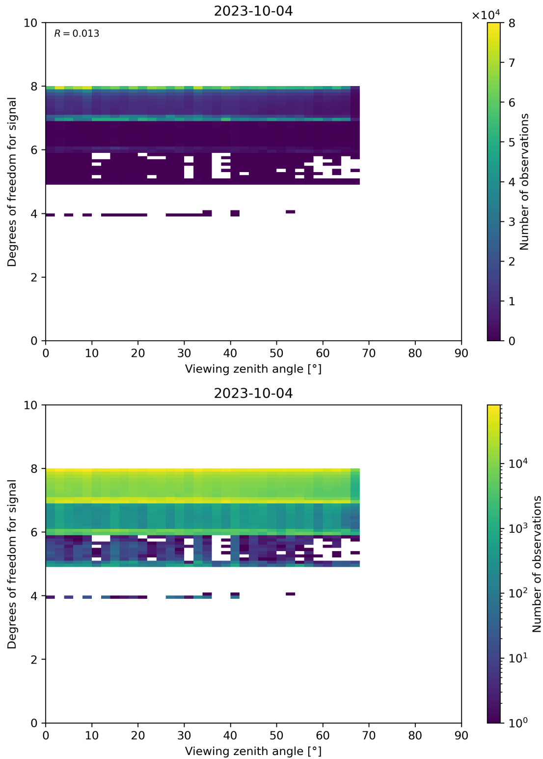
Figure 73: Scatter density plot of “Viewing zenith angle” against “Degrees of freedom for signal” for 2023-10-03 to 2023-10-05.
