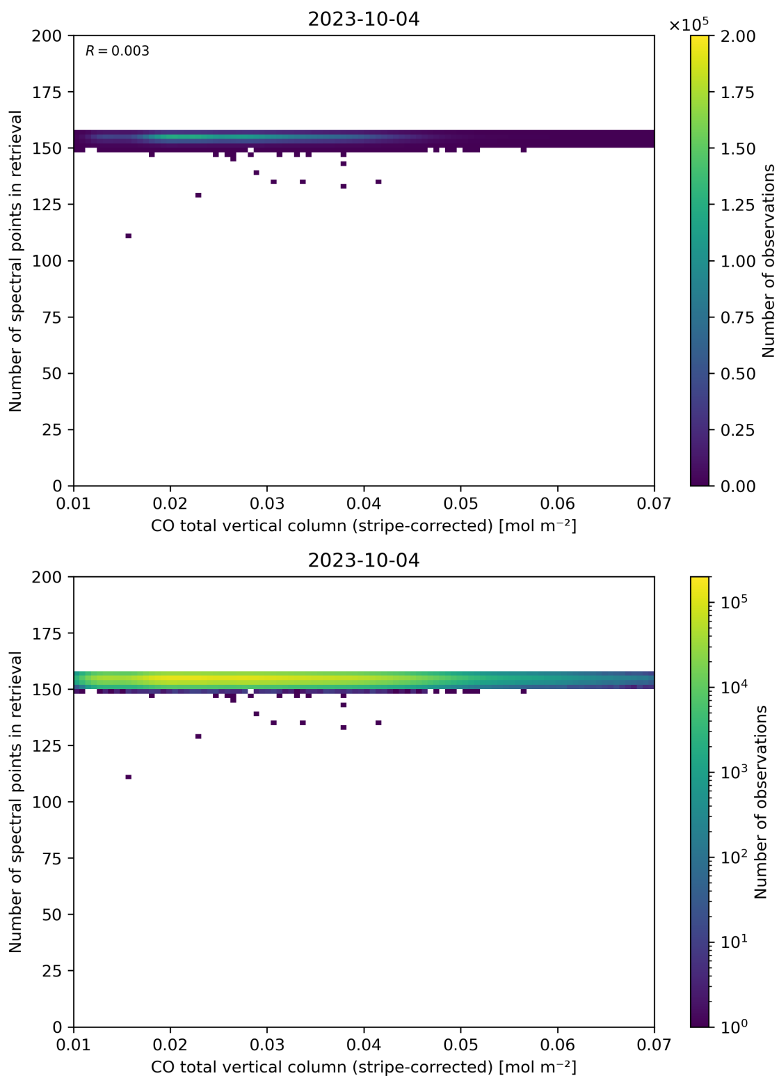
Figure 40: Scatter density plot of “CO total vertical column (stripe-corrected)” against “Number of spectral points in retrieval” for 2023-10-03 to 2023-10-05.
