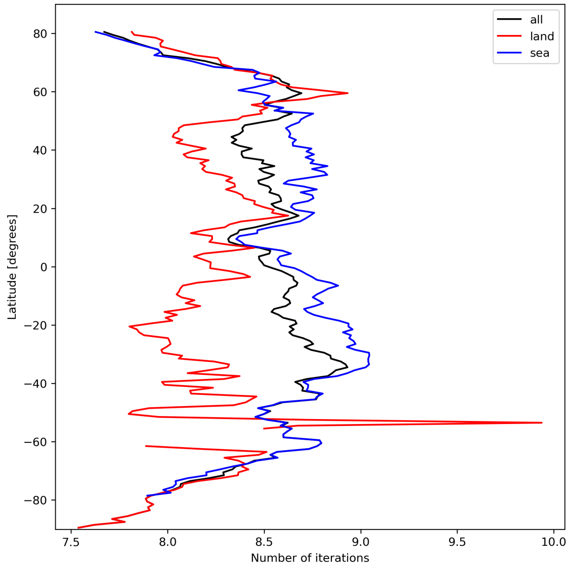
Figure 16: Zonal average of “Number of iterations” for 2023-10-03 to 2023-10-05.
