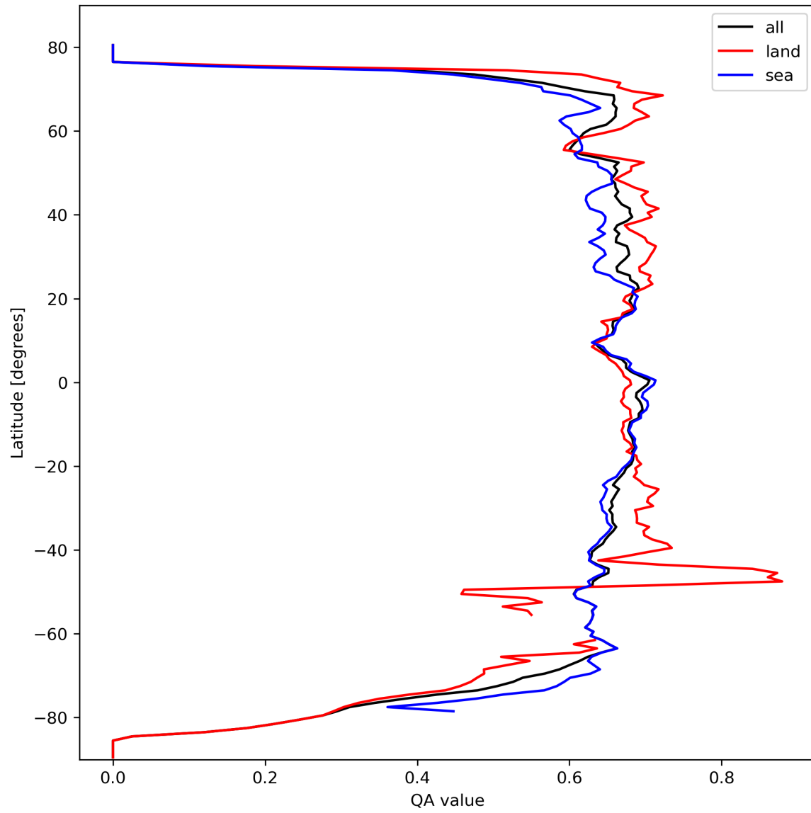
Figure 9: Zonal average of “QA value” for 2023-10-03 to 2023-10-05.
