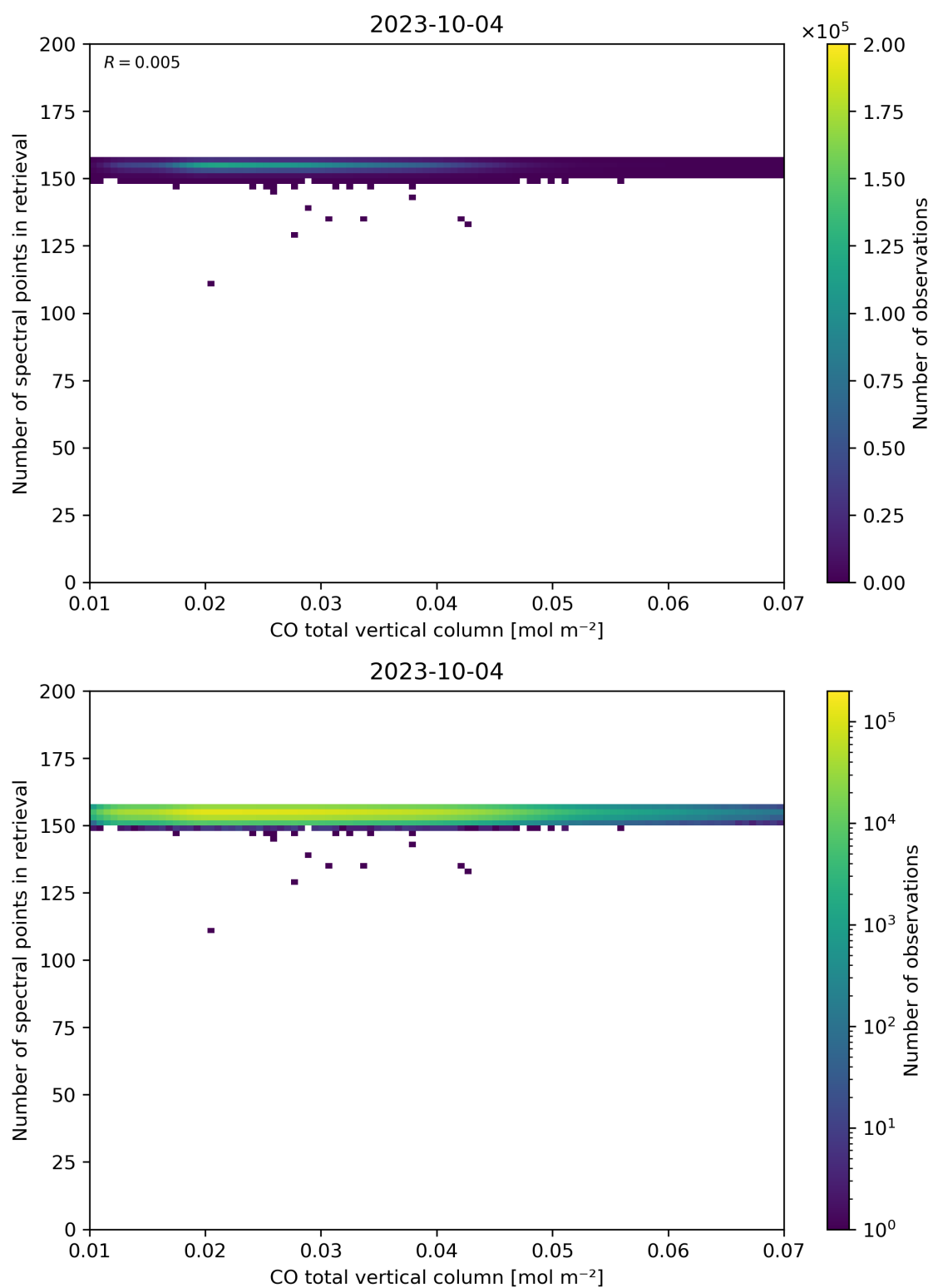
Figure 43: Scatter density plot of “CO total vertical column” against “Number of spectral points in retrieval” for 2023-10-03 to 2023-10-05.
