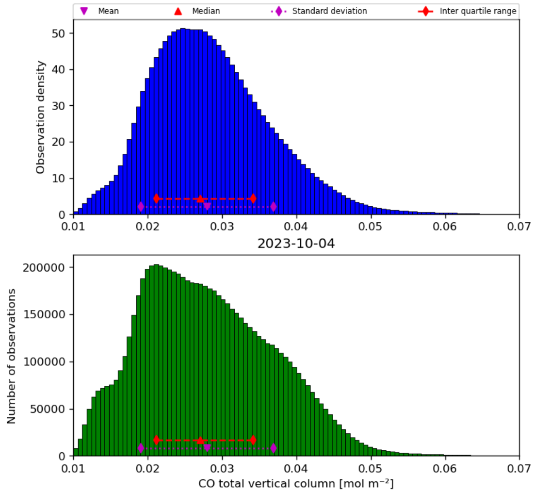
Figure 18: Histogram of “CO total vertical column” for 2023-10-03 to 2023-10-05
