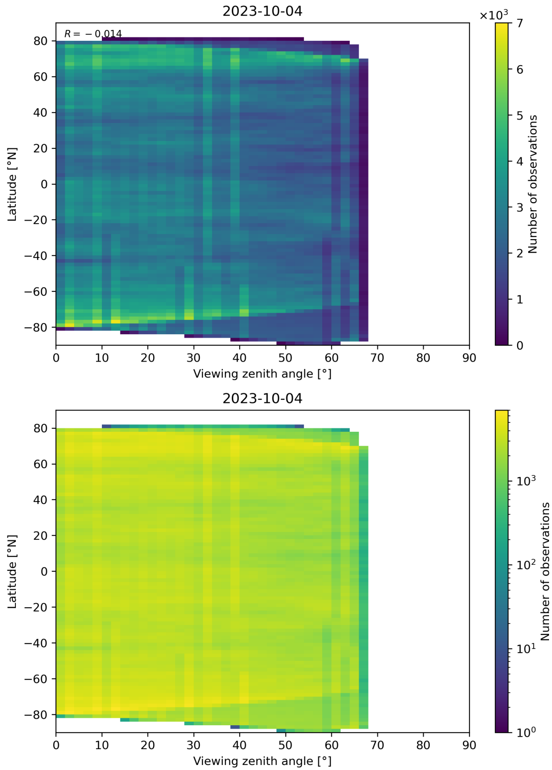
Figure 74: Scatter density plot of “Viewing zenith angle” against “Latitude” for 2023-10-03 to 2023-10-05.
