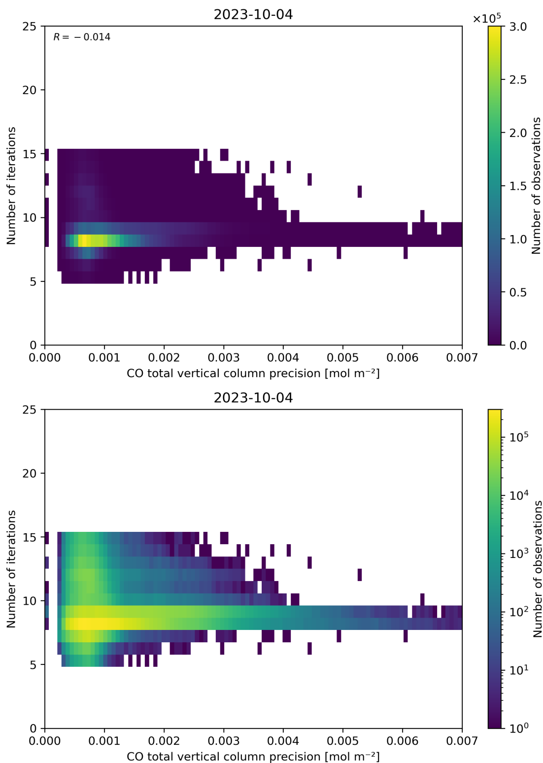
Figure 46: Scatter density plot of “CO total vertical column precision” against “Number of iterations” for 2023-10-03 to 2023-10-05.
