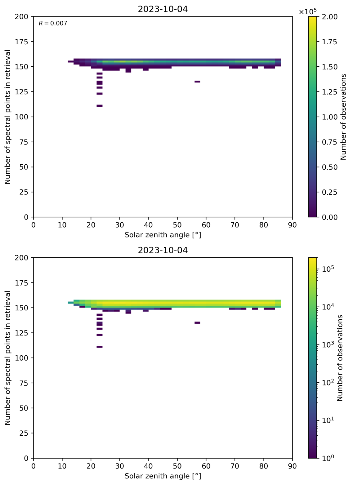
Figure 68: Scatter density plot of “Solar zenith angle” against “Number of spectral points in retrieval” for 2023-10-03 to 2023-10-05.
