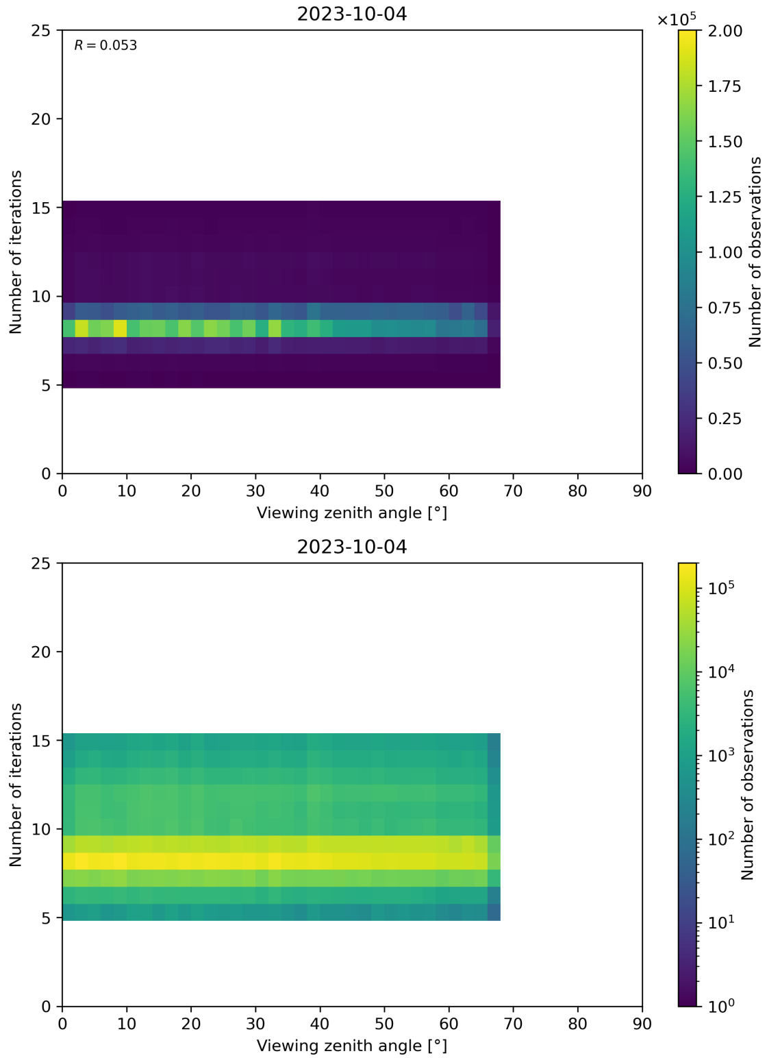
Figure 75: Scatter density plot of “Viewing zenith angle” against “Number of iterations” for 2023-10-03 to 2023-10-05.
