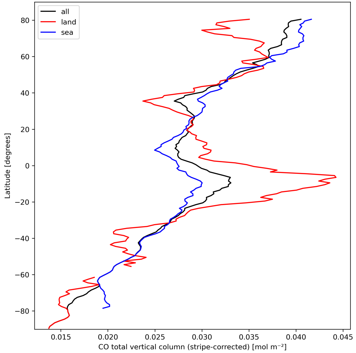
Figure 11: Zonal average of “CO total vertical column (stripe-corrected)” for 2023-10-03 to 2023-10-05.
