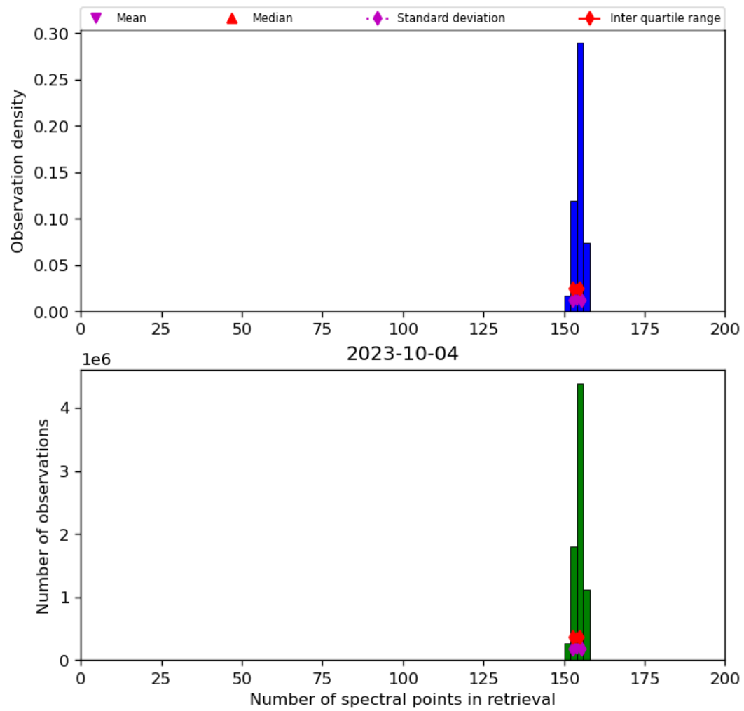
Figure 21: Histogram of “Number of spectral points in retrieval” for 2023-10-03 to 2023-10-05
