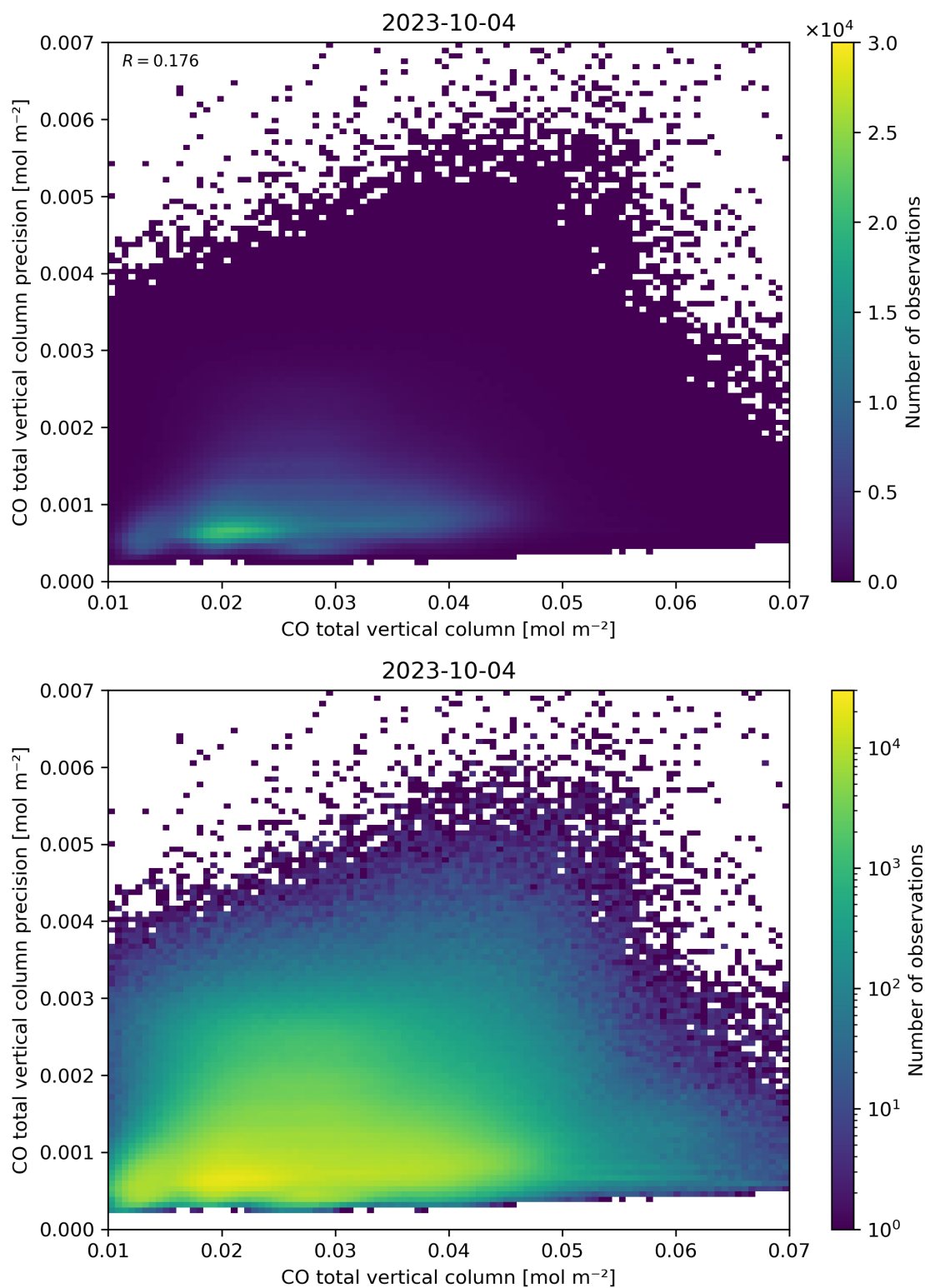
Figure 34: Scatter density plot of “CO total vertical column” against “CO total vertical column precision” for 2023-10-03 to 2023-10-05.
