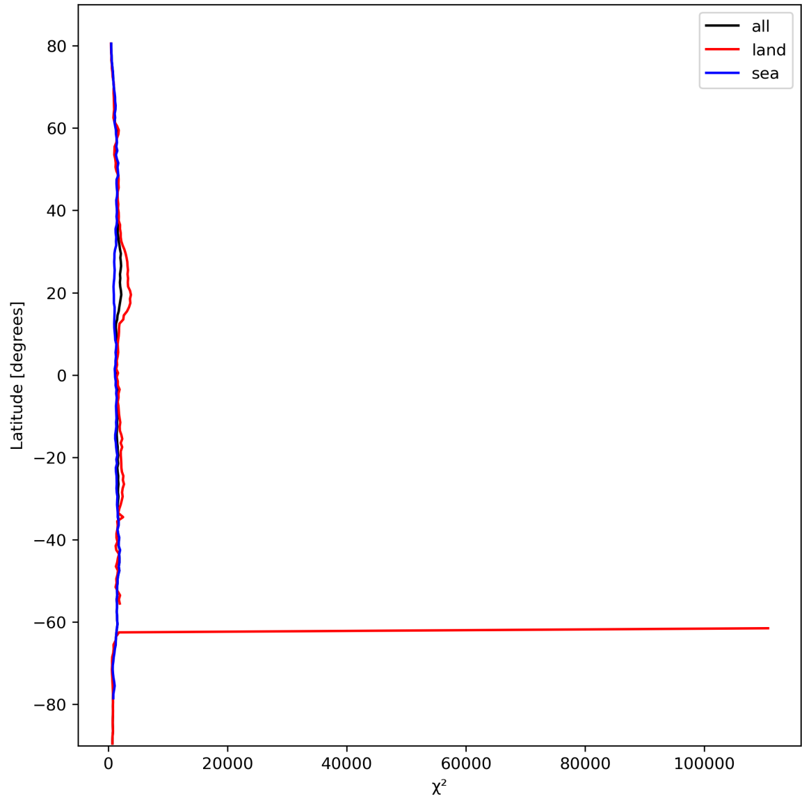
Figure 14: Zonal average of “ \chi^2 ” for 2023-10-03 to 2023-10-05.
