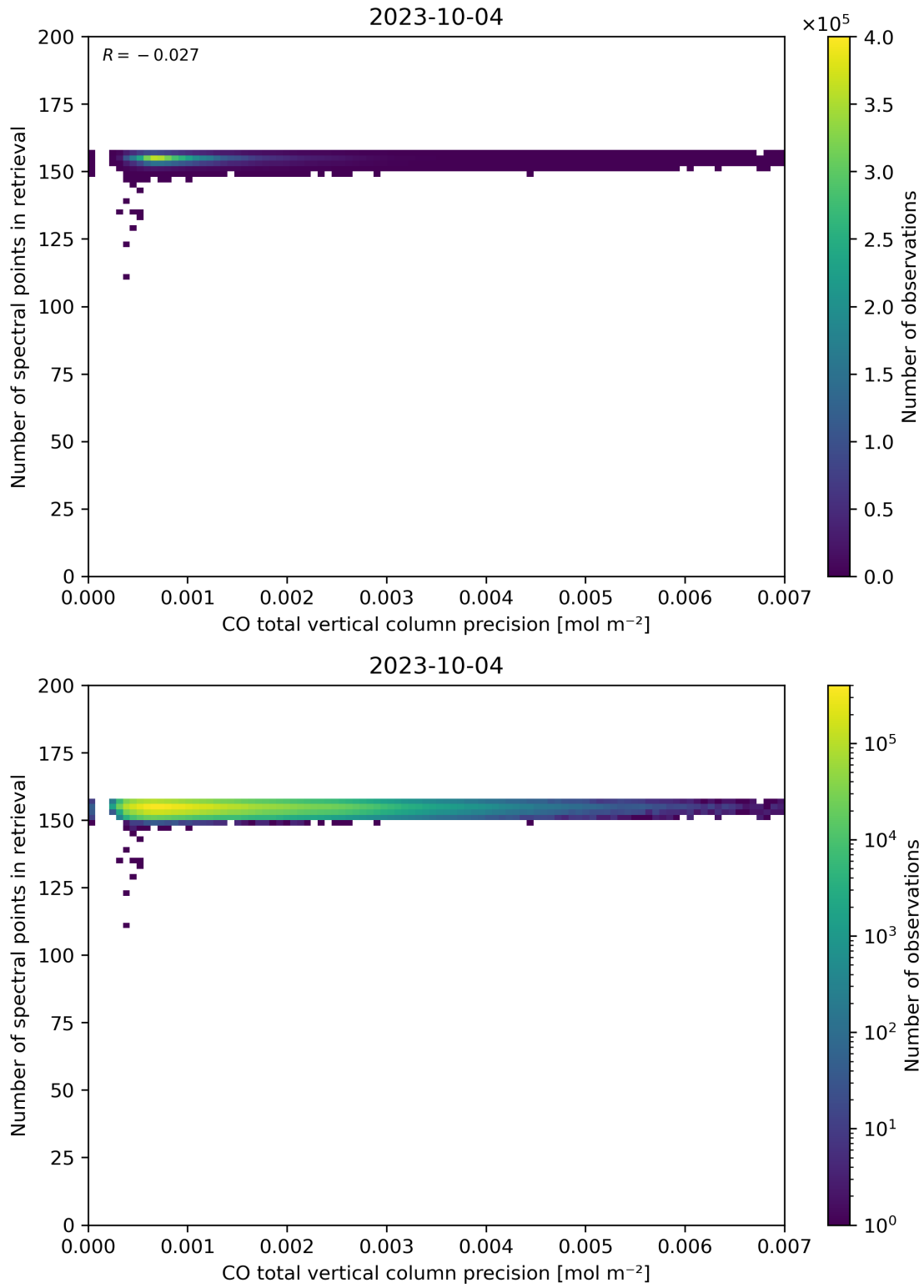
Figure 47: Scatter density plot of “CO total vertical column precision” against “Number of spectral points in retrieval” for 2023-10-03 to 2023-10-05.
