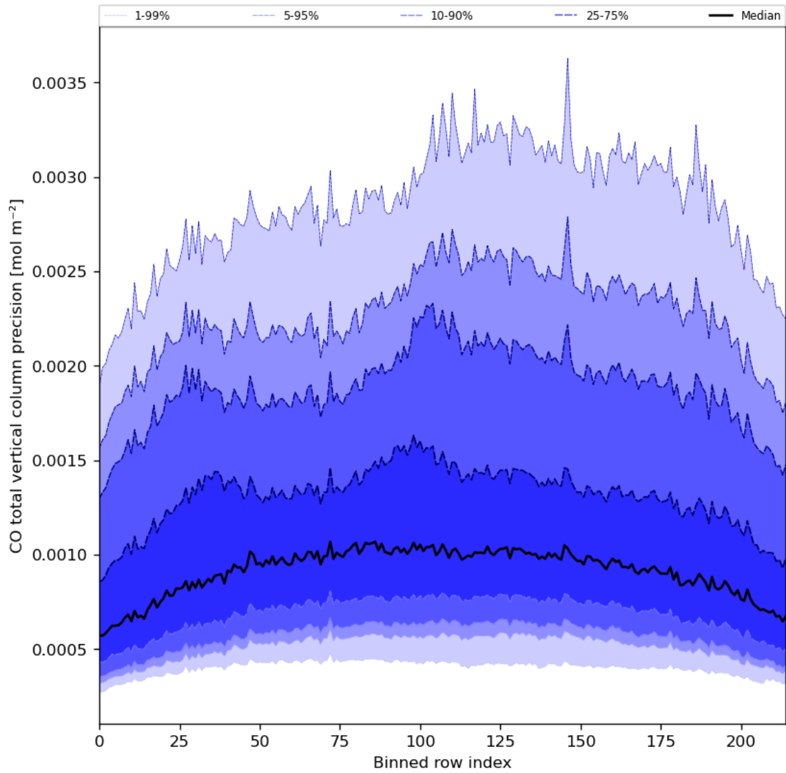
Figure 28: Along track statistics of “CO total vertical column precision” for 2023-10-03 to 2023-10-05
