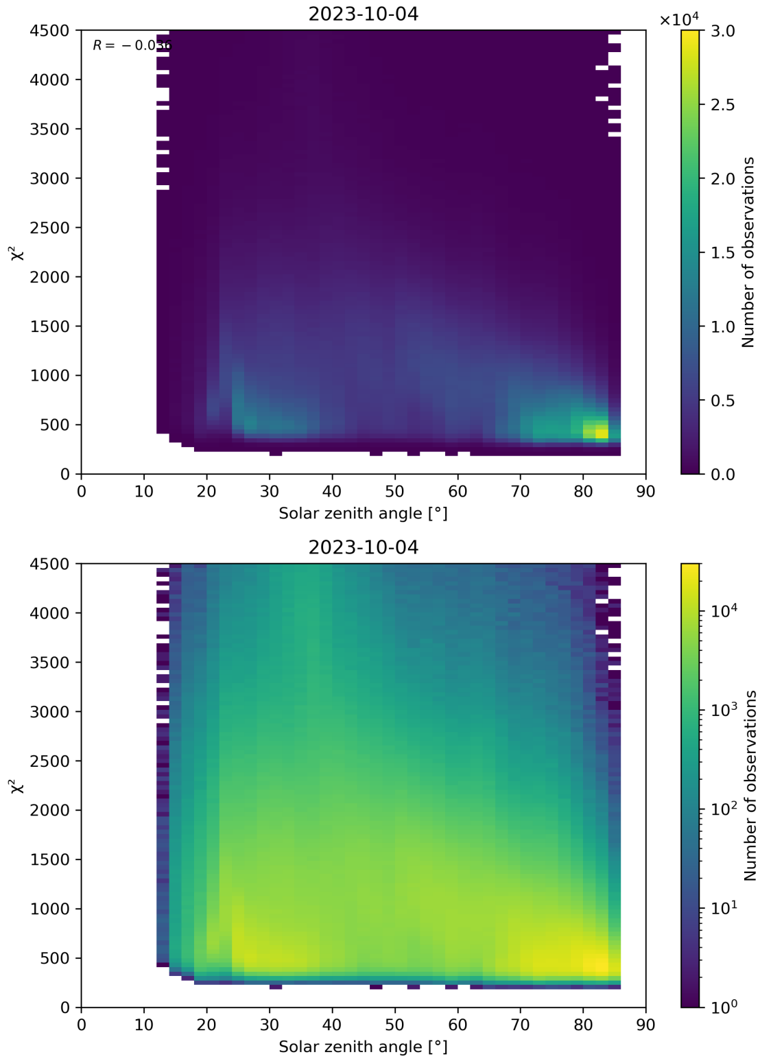
Figure 64: Scatter density plot of “Solar zenith angle” against “ \chi^2 ” for 2023-10-03 to 2023-10-05.
