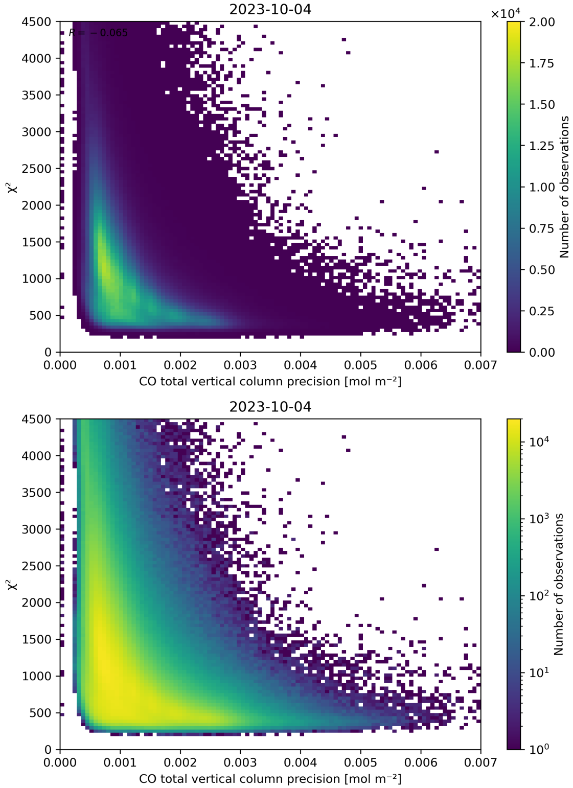
Figure 44: Scatter density plot of “CO total vertical column precision” against “ \chi^2 ” for 2023-10-03 to 2023-10-05.
