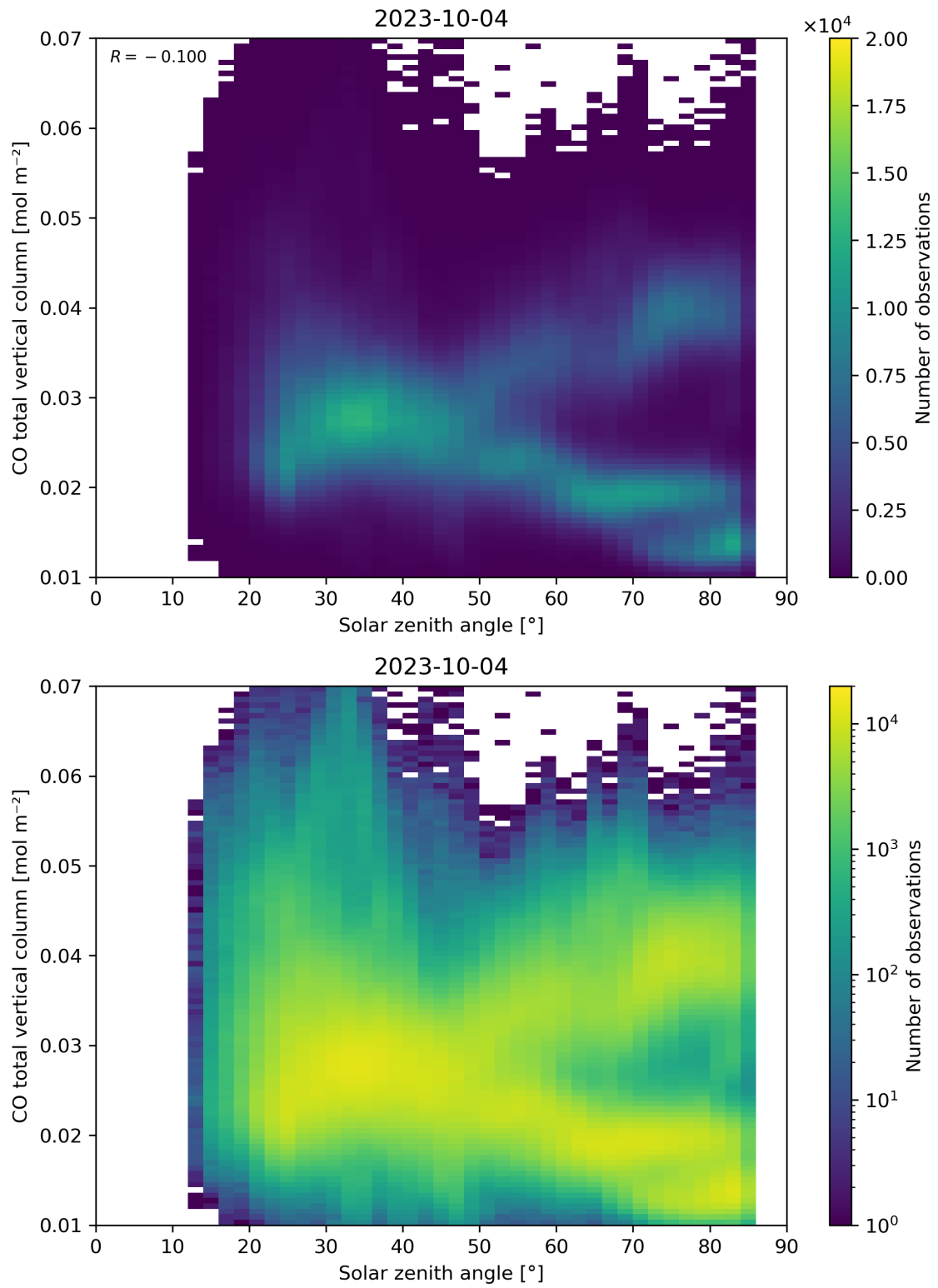
Figure 61: Scatter density plot of “Solar zenith angle” against “CO total vertical column” for 2023-10-03 to 2023-10-05.
