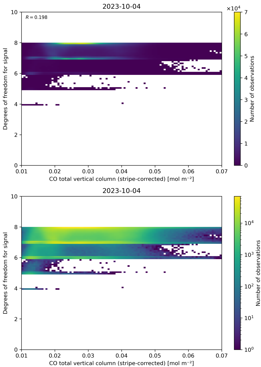
Figure 38: Scatter density plot of “CO total vertical column (stripe-corrected)” against “Degrees of freedom for signal” for 2023-10-03 to 2023-10-05.
