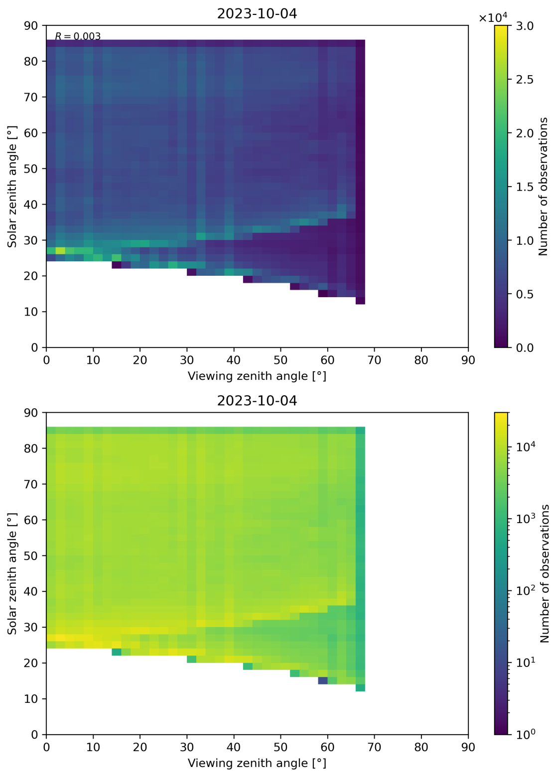
Figure 77: Scatter density plot of “Viewing zenith angle” against “Solar zenith angle” for 2023-10-03 to 2023-10-05.
