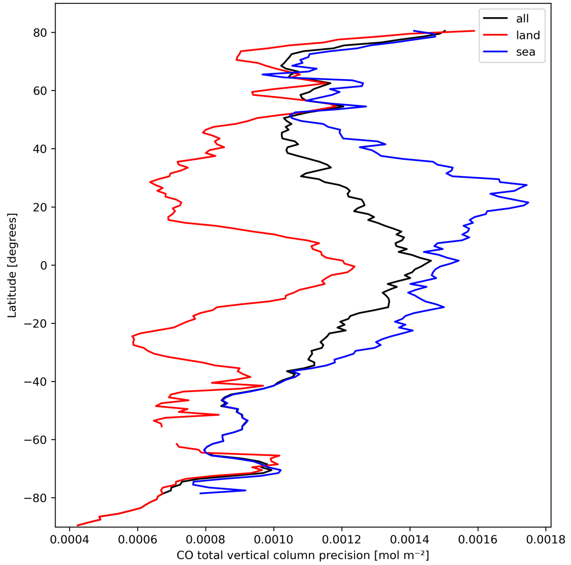
Figure 12: Zonal average of “CO total vertical column precision” for 2023-10-03 to 2023-10-05.
