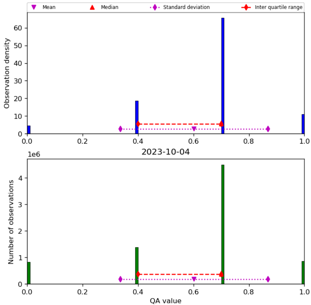
Figure 17: Histogram of "QA value" for 2023-10-03 to 2023-10-05
