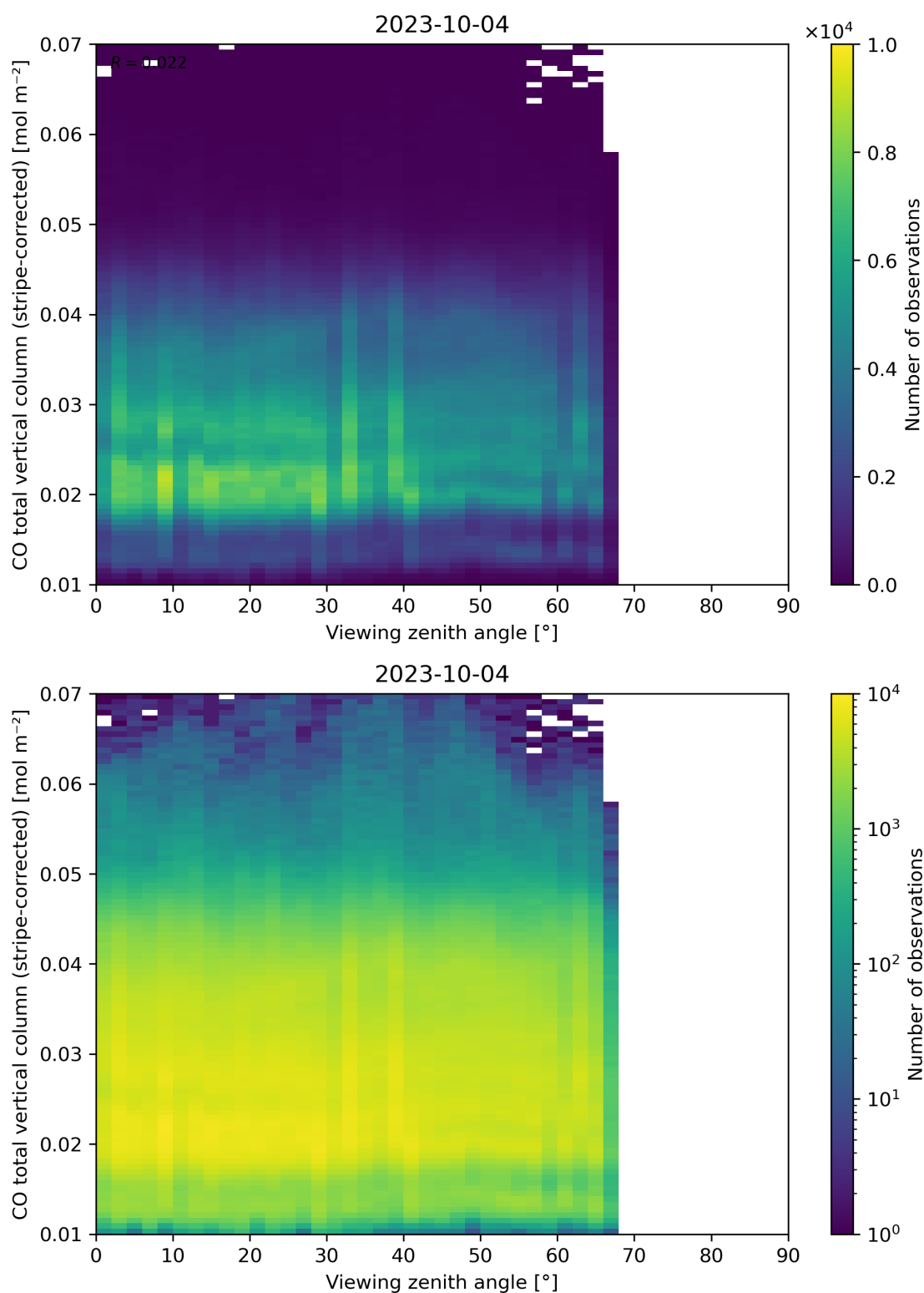
Figure 70: Scatter density plot of “Viewing zenith angle” against “CO total vertical column (stripe-corrected)” for 2023-10-03 to 2023-10-05.
