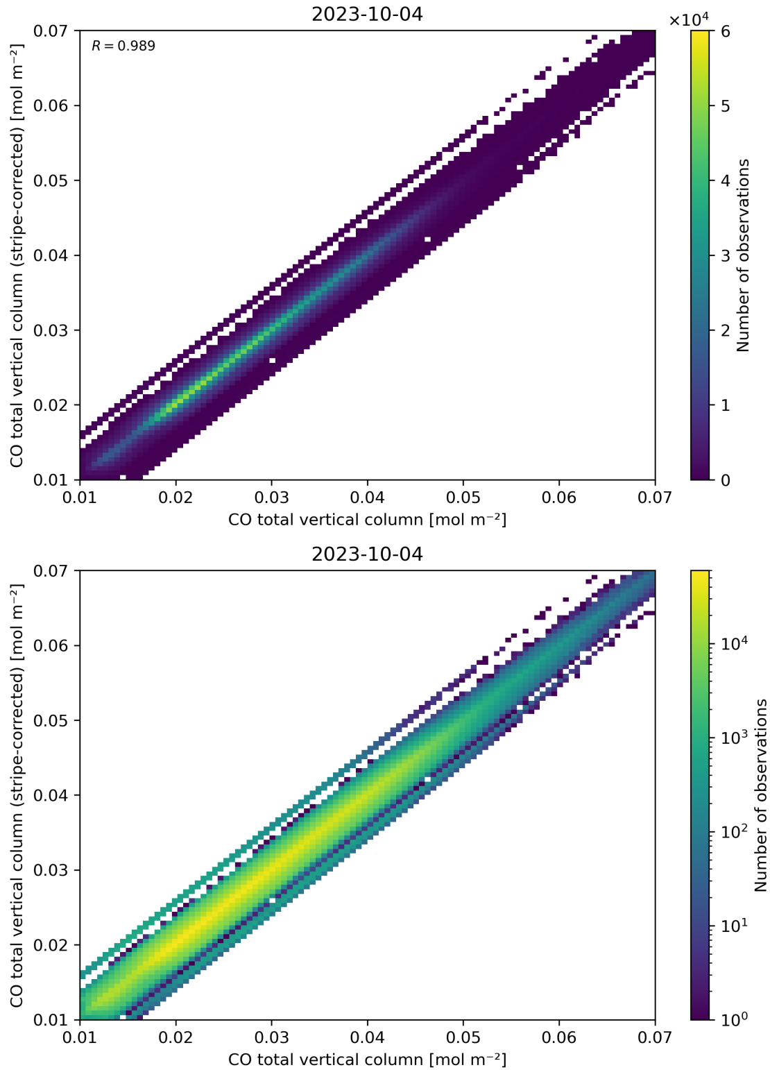
Figure 33: Scatter density plot of “CO total vertical column” against “CO total vertical column (stripe-corrected)” for 2023-10-03 to 2023-10-05.
