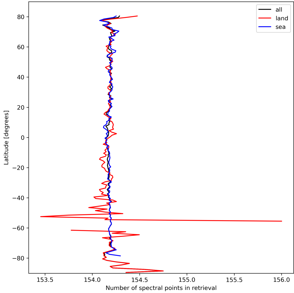
Figure 13: Zonal average of “Number of spectral points in retrieval” for 2023-10-03 to 2023-10-05.
