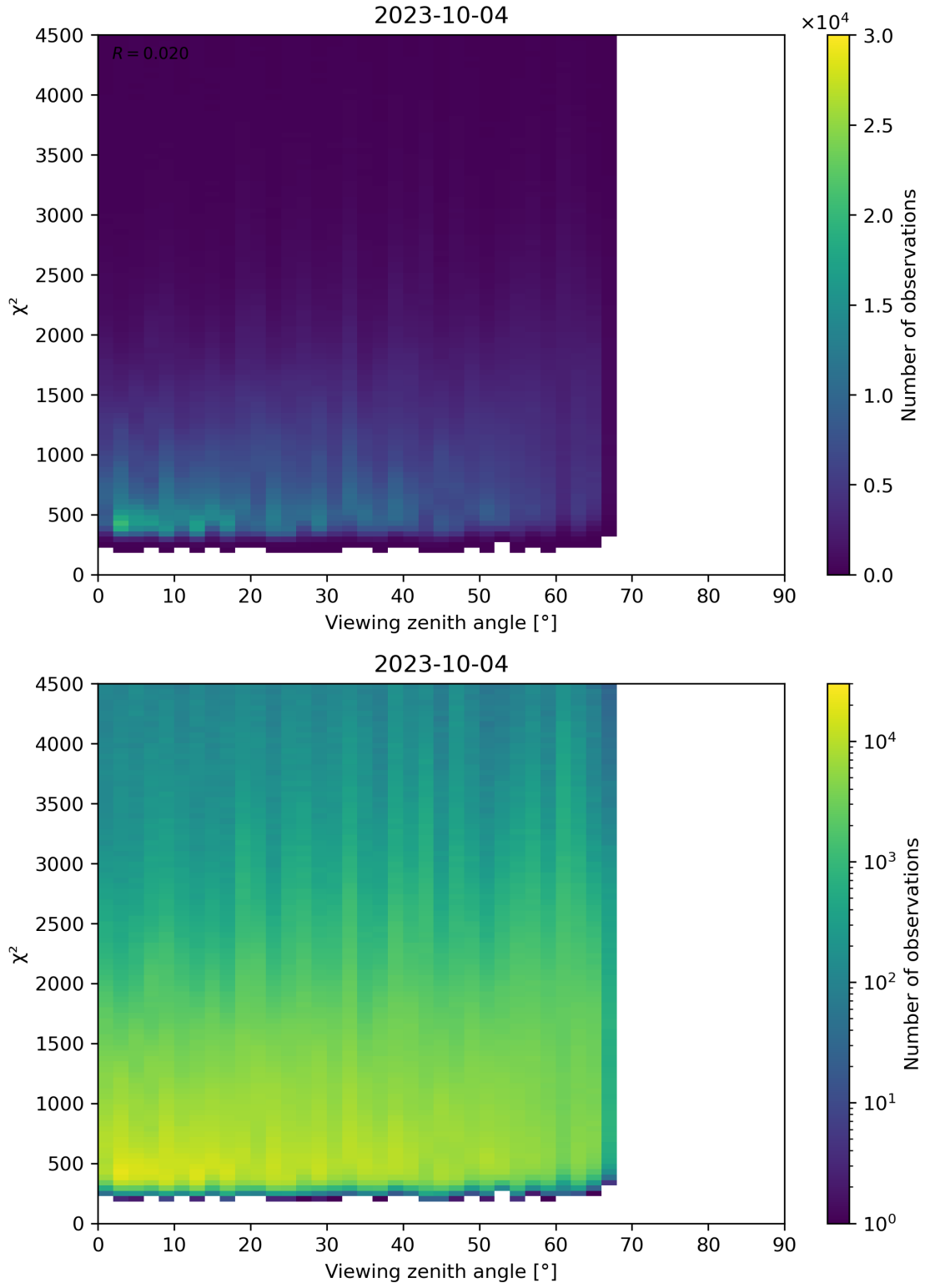
Figure 72: Scatter density plot of “Viewing zenith angle” against “ \chi^2 ” for 2023-10-03 to 2023-10-05.
