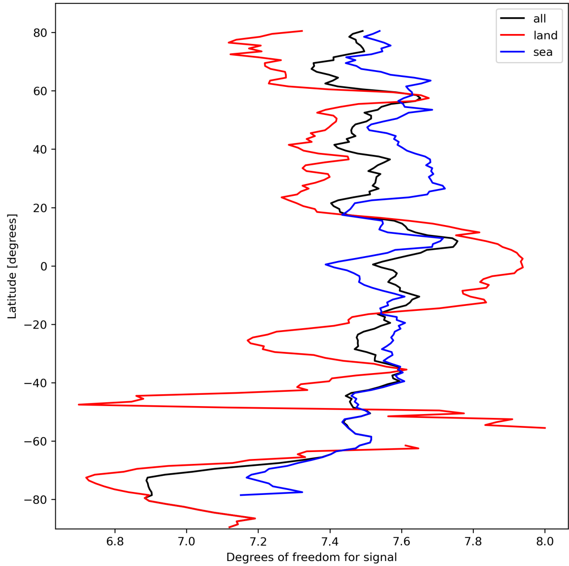
Figure 15: Zonal average of “Degrees of freedom for signal” for 2023-10-03 to 2023-10-05.
