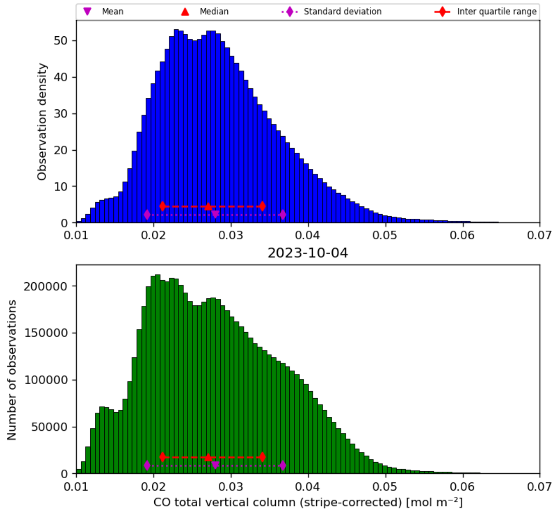
Figure 19: Histogram of “CO total vertical column (stripe-corrected)” for 2023-10-03 to 2023-10-05
