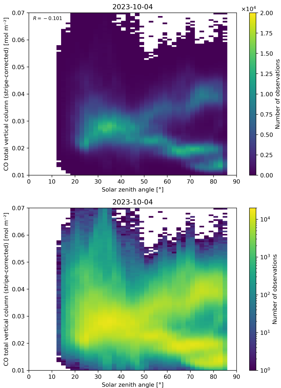
Figure 62: Scatter density plot of “Solar zenith angle” against “CO total vertical column (stripe-corrected)” for 2023-10-03 to 2023-10-05.
