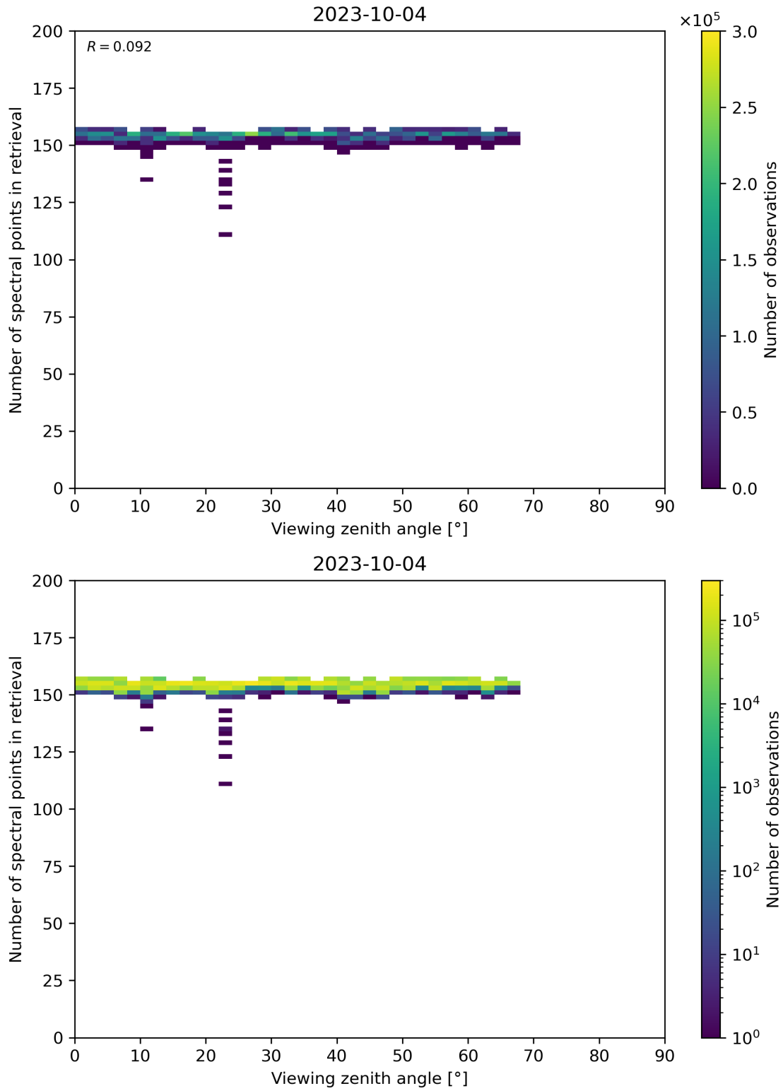
Figure 76: Scatter density plot of “Viewing zenith angle” against “Number of spectral points in retrieval” for 2023-10-03 to 2023-10-05.
