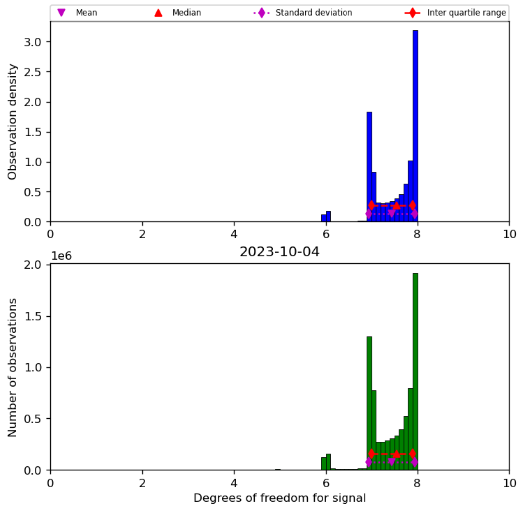
Figure 23: Histogram of “Degrees of freedom for signal” for 2023-10-03 to 2023-10-05
