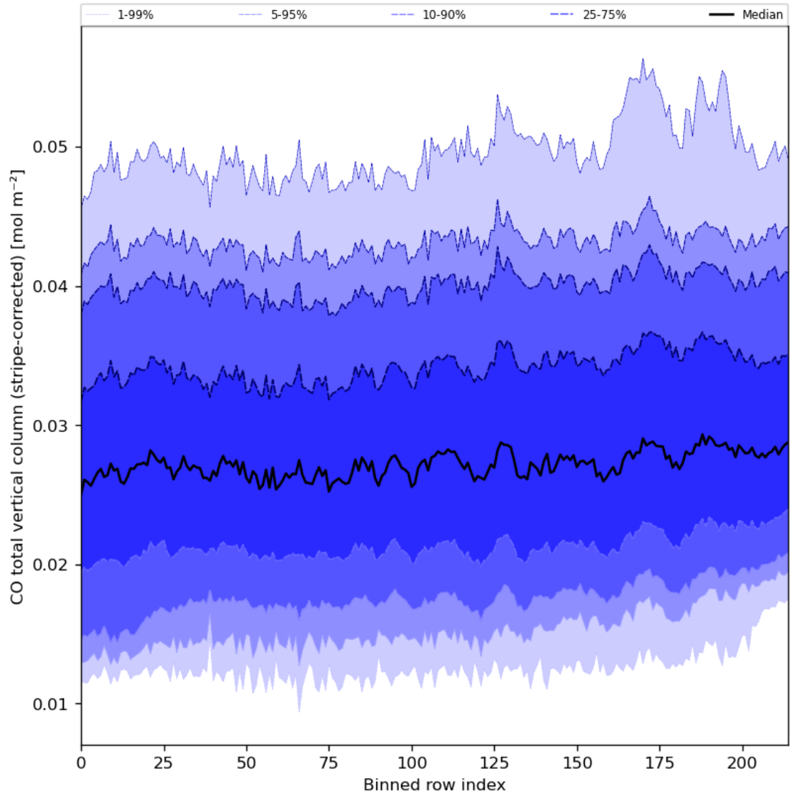
Figure 27: Along track statistics of “CO total vertical column (stripe-corrected)” for 2023-10-03 to 2023-10-05
