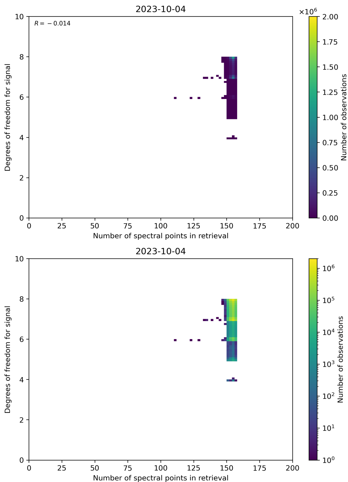
Figure 59: Scatter density plot of “Number of spectral points in retrieval” against “Degrees of freedom for signal” for 2023-10-03 to 2023-10-05.
