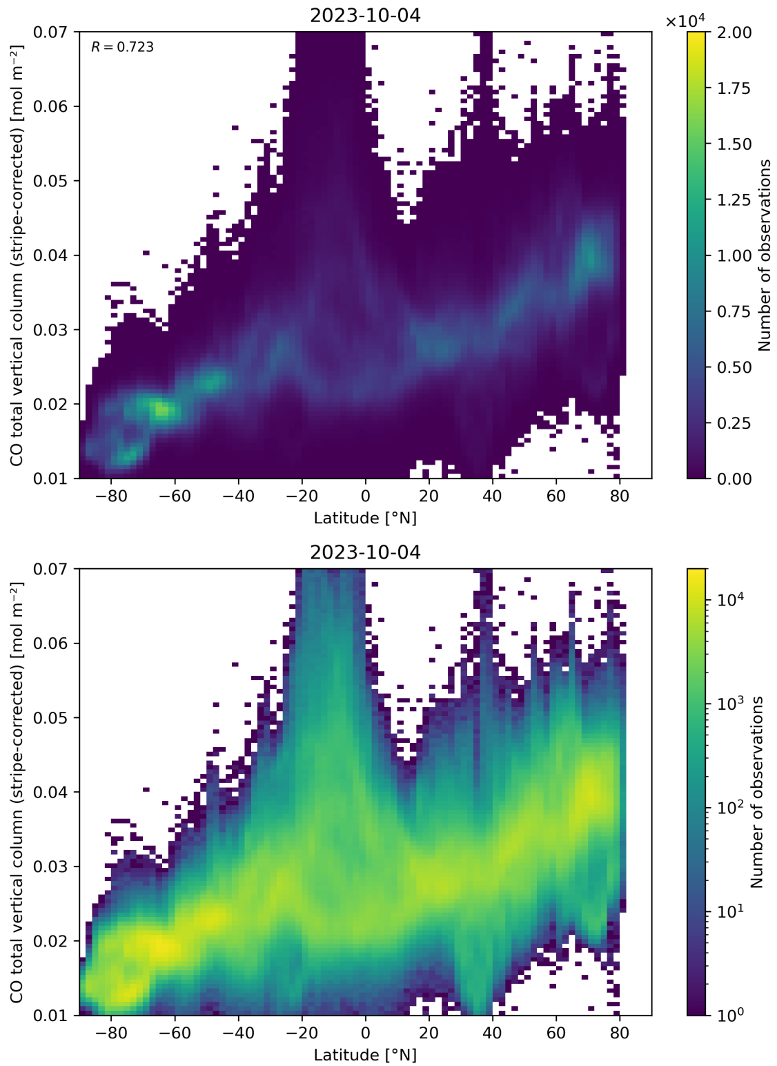
Figure 52: Scatter density plot of “Latitude” against “CO total vertical column (stripe-corrected)” for 2023-10-03 to 2023-10-05.
