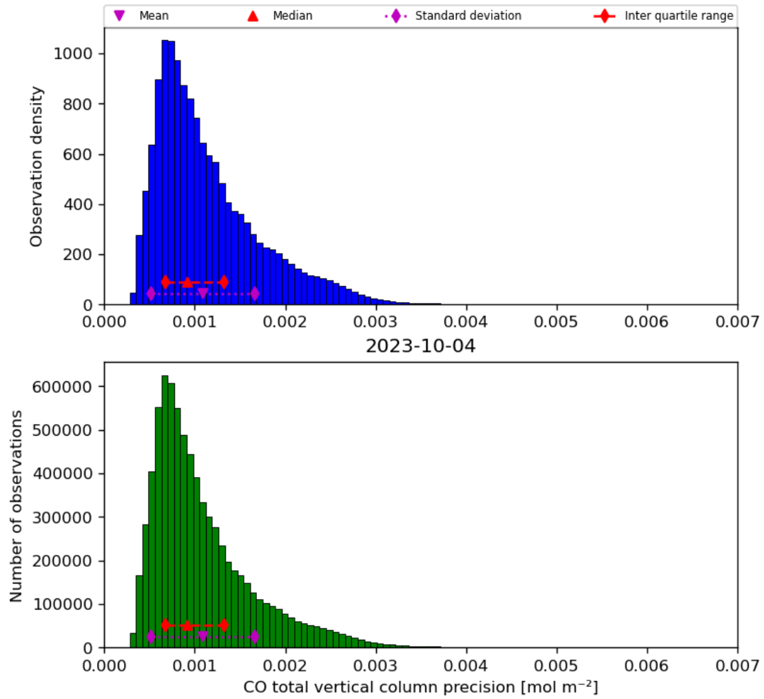
Figure 20: Histogram of “CO total vertical column precision” for 2023-10-03 to 2023-10-05
