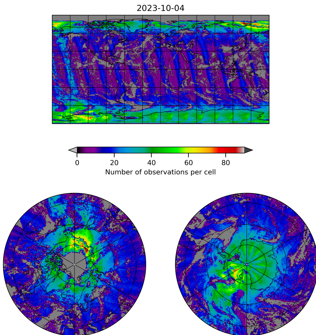
Figure 8: Map of the number of observations for 2023-10-03 to 2023-10-05
