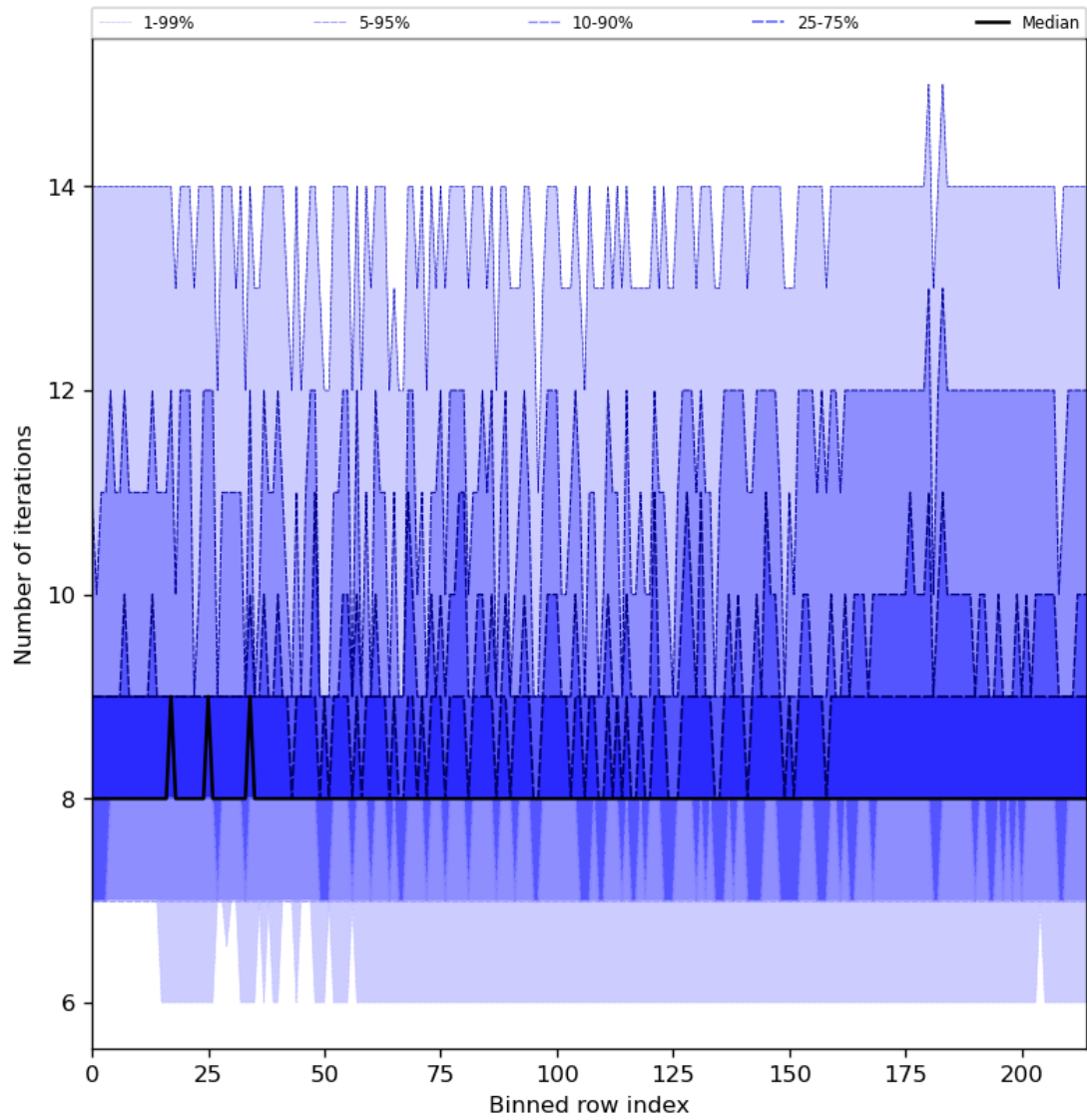
Figure 32: Along track statistics of “Number of iterations” for 2023-10-03 to 2023-10-05
