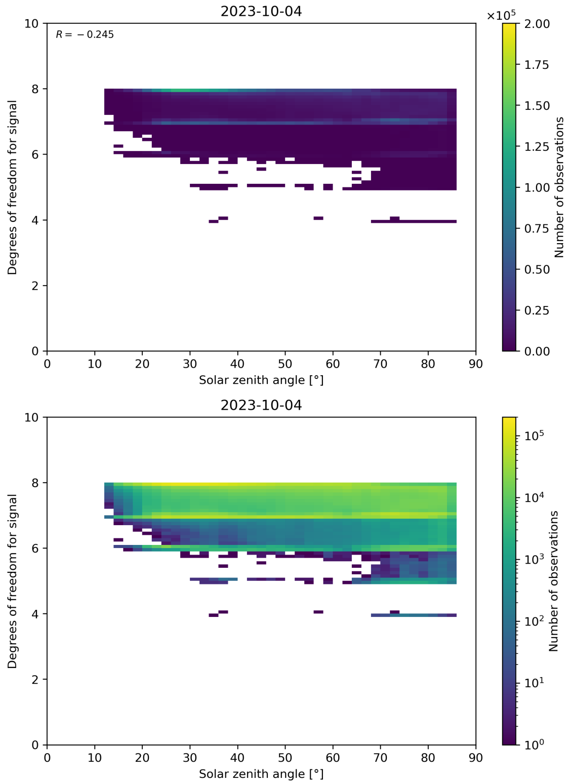
Figure 65: Scatter density plot of “Solar zenith angle” against “Degrees of freedom for signal” for 2023-10-03 to 2023-10-05.
