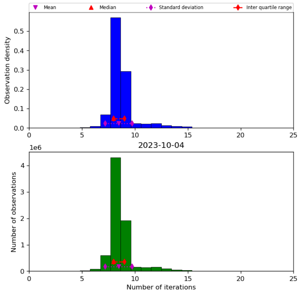
Figure 24: Histogram of “Number of iterations” for 2023-10-03 to 2023-10-05
