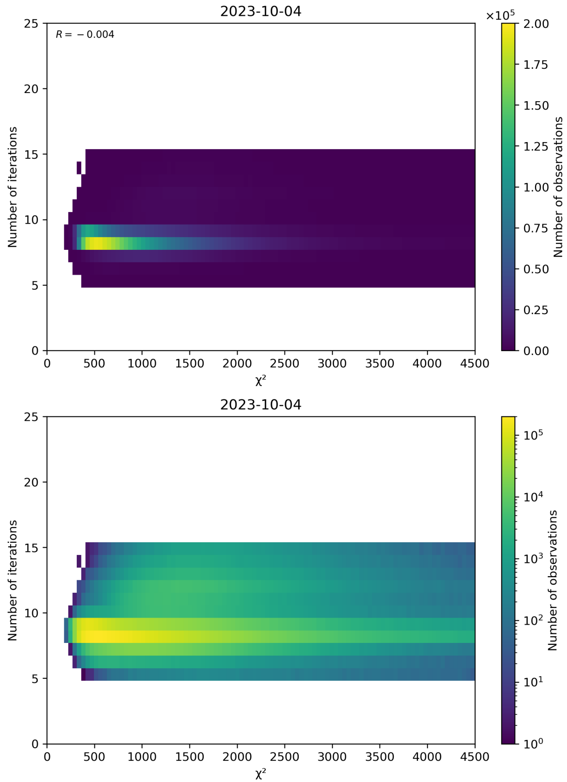
Figure 49: Scatter density plot of “ \chi^2 ” against “Number of iterations” for 2023-10-03 to 2023-10-05.
