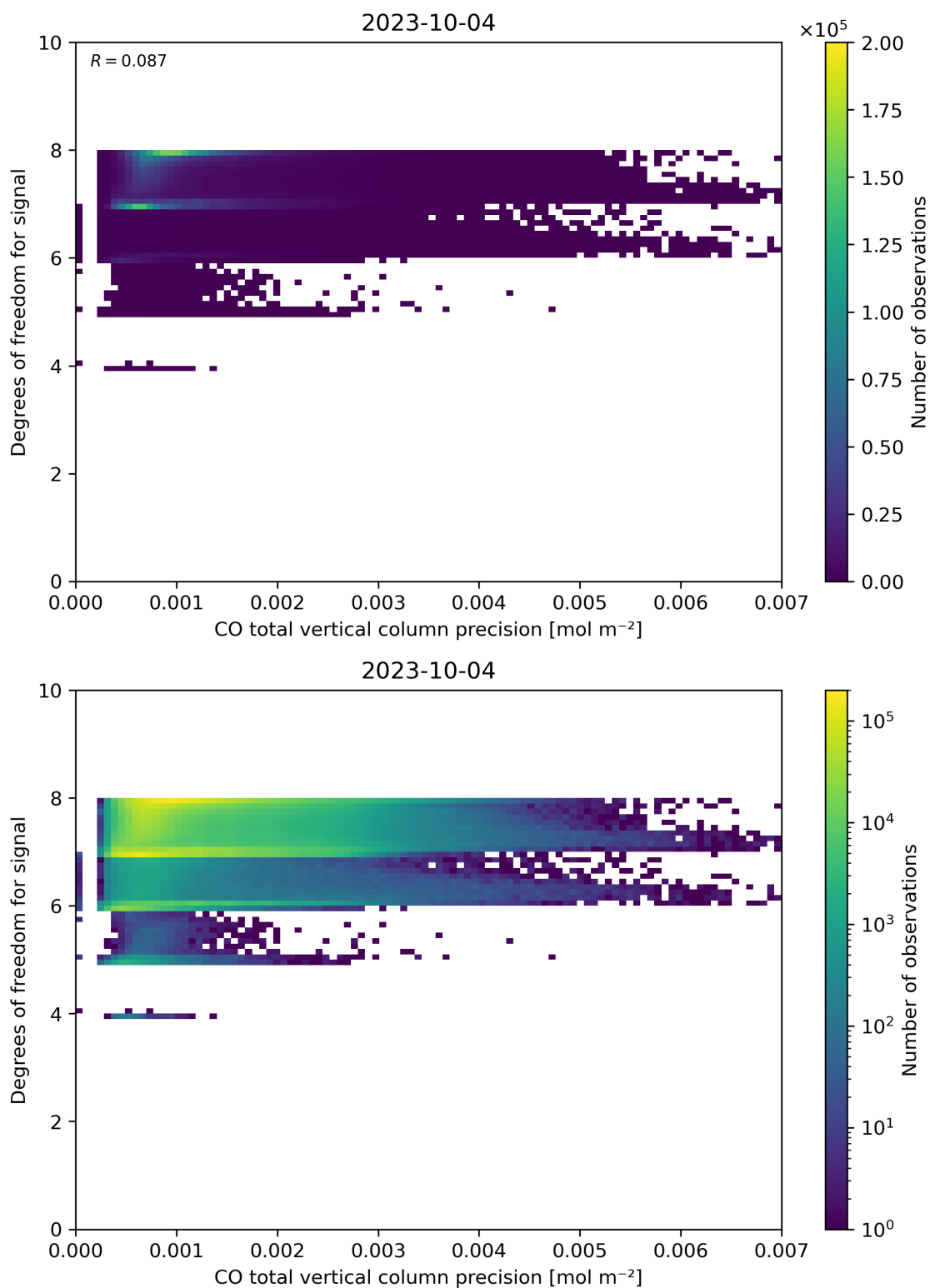
Figure 45: Scatter density plot of “CO total vertical column precision” against “Degrees of freedom for signal” for 2023-10-03 to 2023-10-05.
