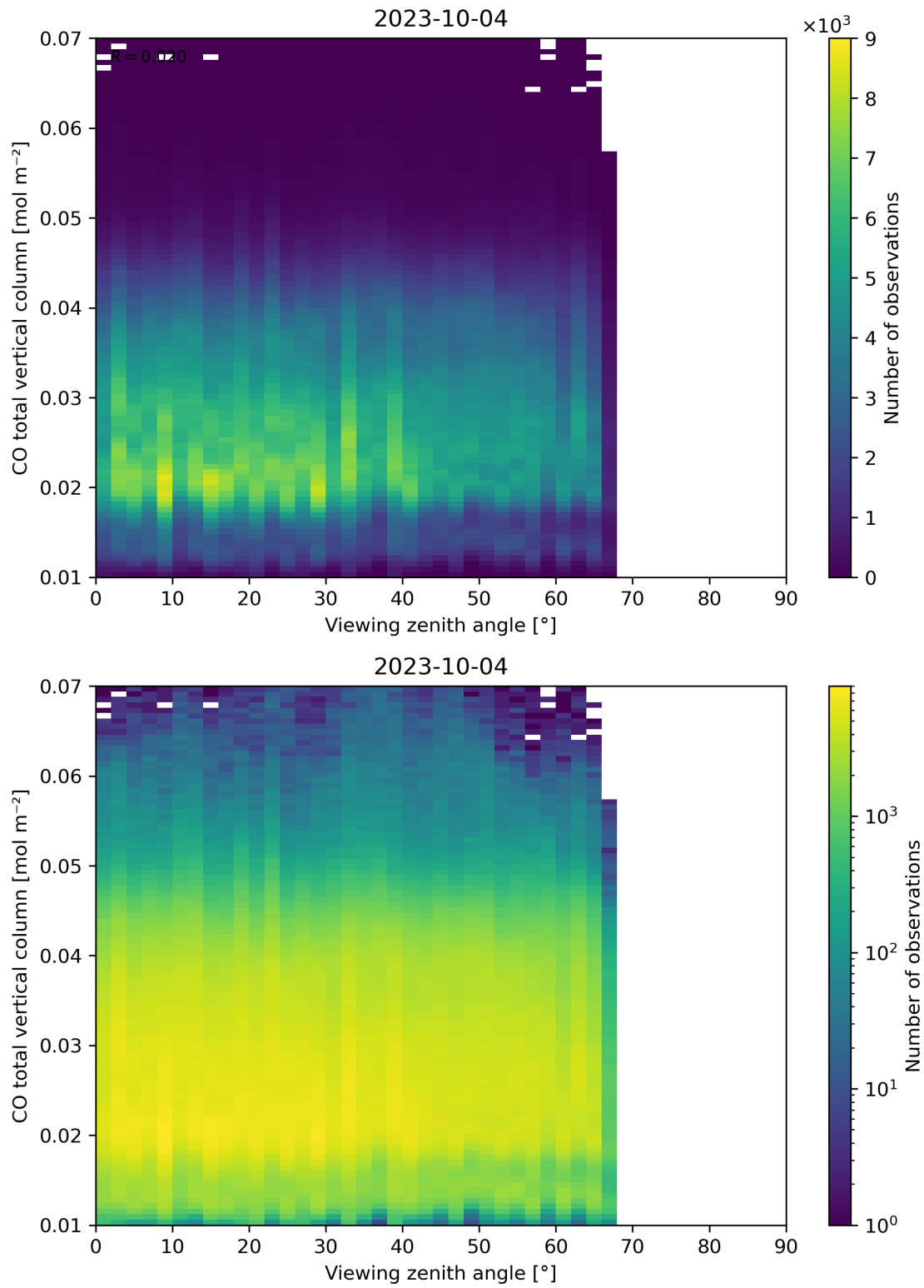
Figure 69: Scatter density plot of “Viewing zenith angle” against “CO total vertical column” for 2023-10-03 to 2023-10-05.
