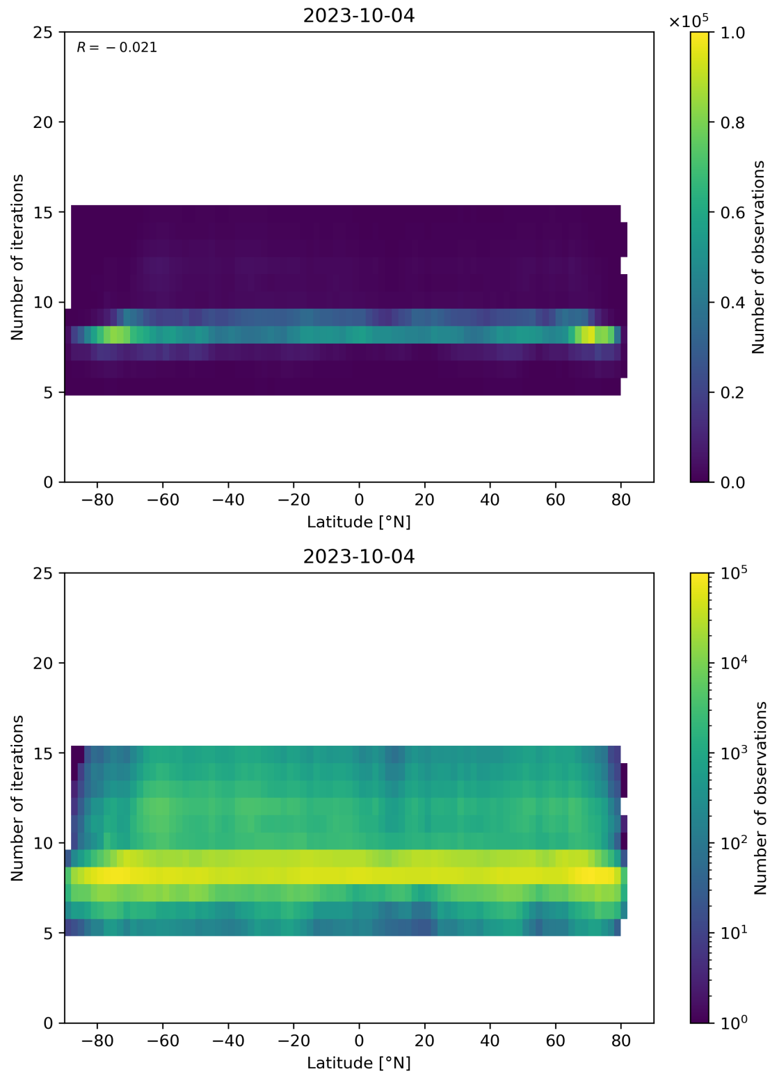
Figure 56: Scatter density plot of “Latitude” against “Number of iterations” for 2023-10-03 to 2023-10-05.
