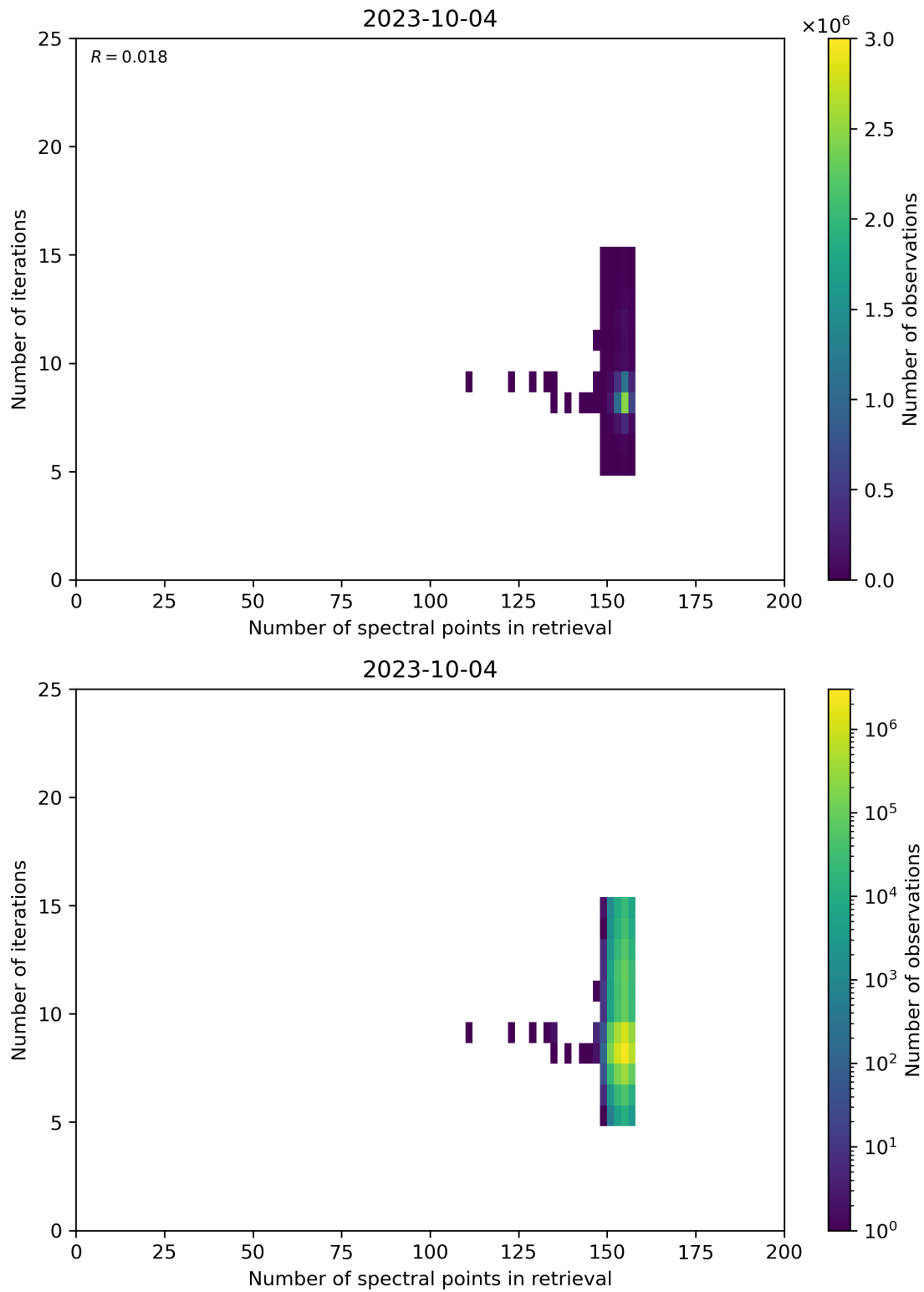
Figure 60: Scatter density plot of “Number of spectral points in retrieval” against “Number of iterations” for 2023-10-03 to 2023-10-05.
