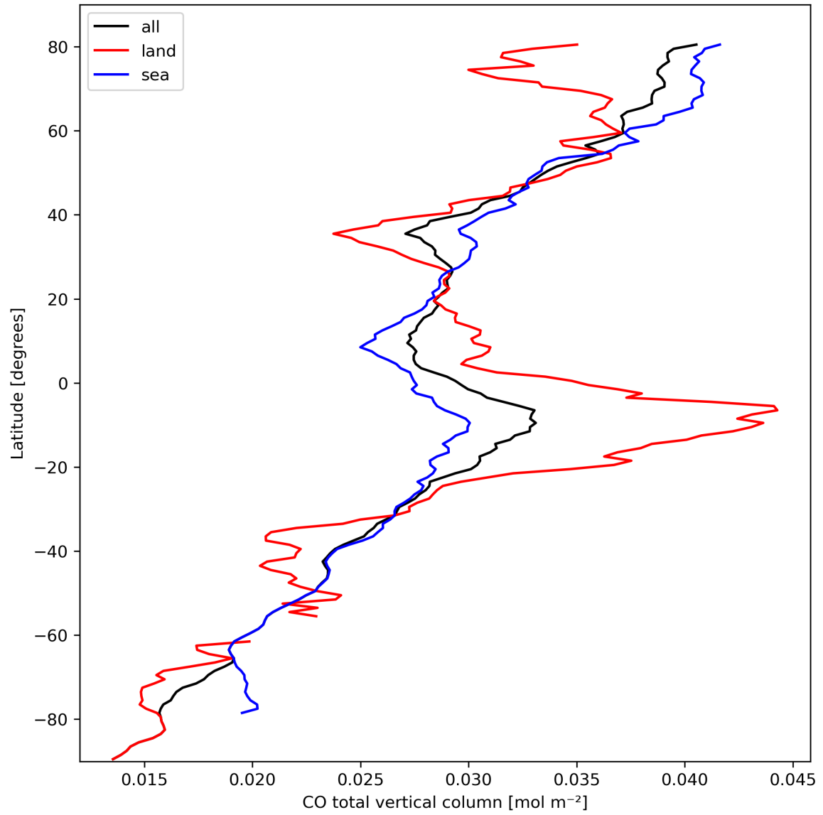
Figure 10: Zonal average of “CO total vertical column” for 2023-10-03 to 2023-10-05.
