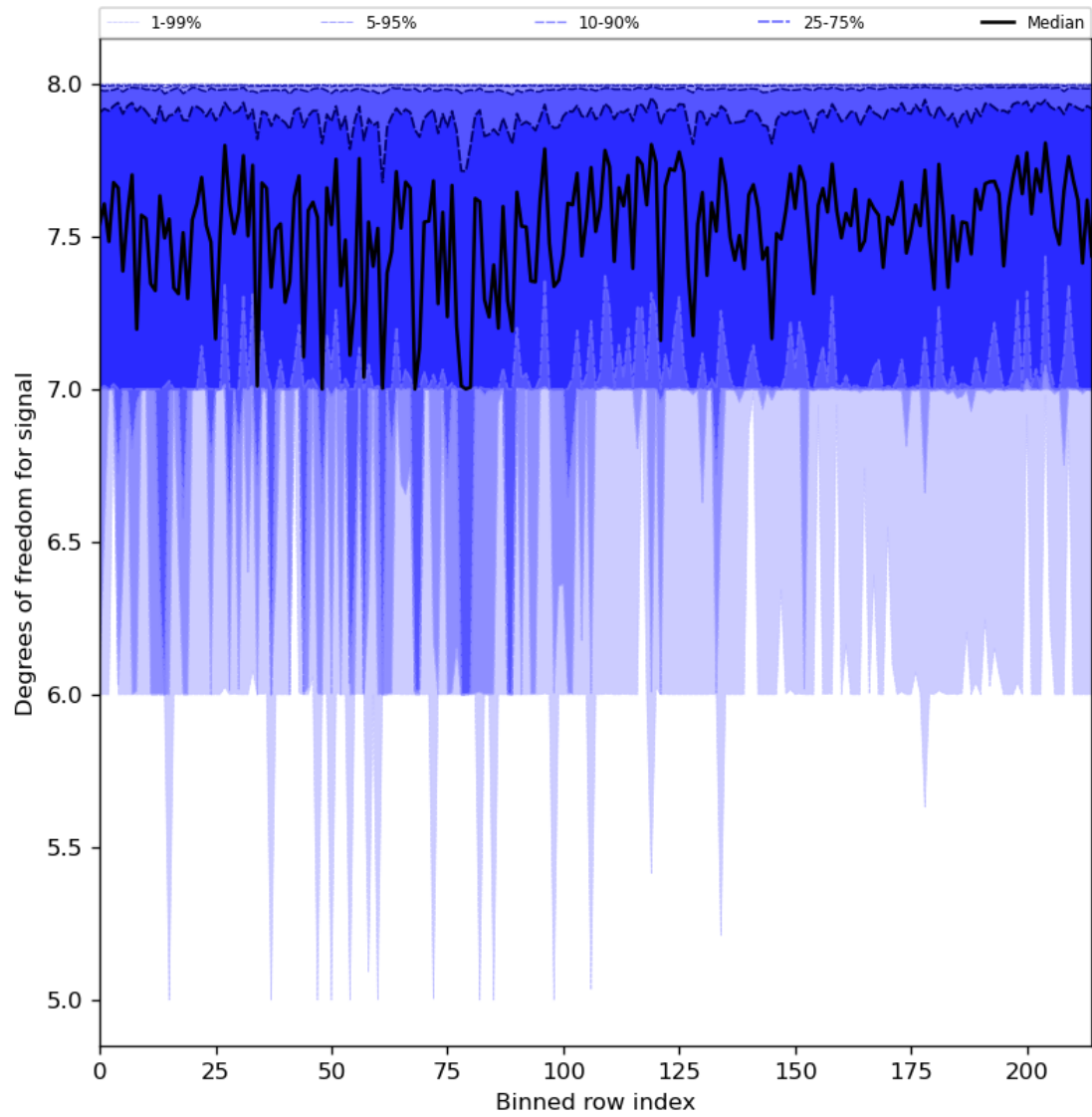
Figure 31: Along track statistics of “Degrees of freedom for signal” for 2023-10-03 to 2023-10-05
