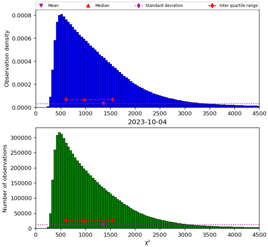
Figure 22: Histogram of “ \chi^2 ” for 2023-10-03 to 2023-10-05
