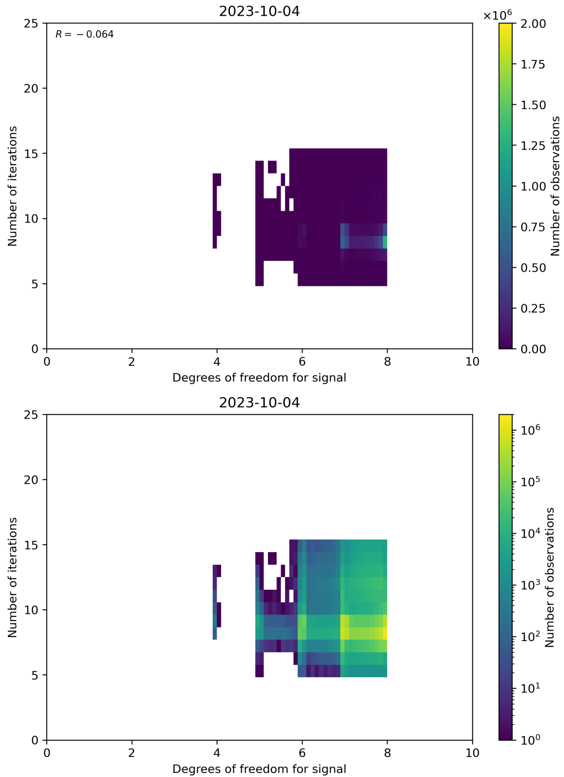
Figure 50: Scatter density plot of “Degrees of freedom for signal” against “Number of iterations” for 2023-10-03 to 2023-10-05.
