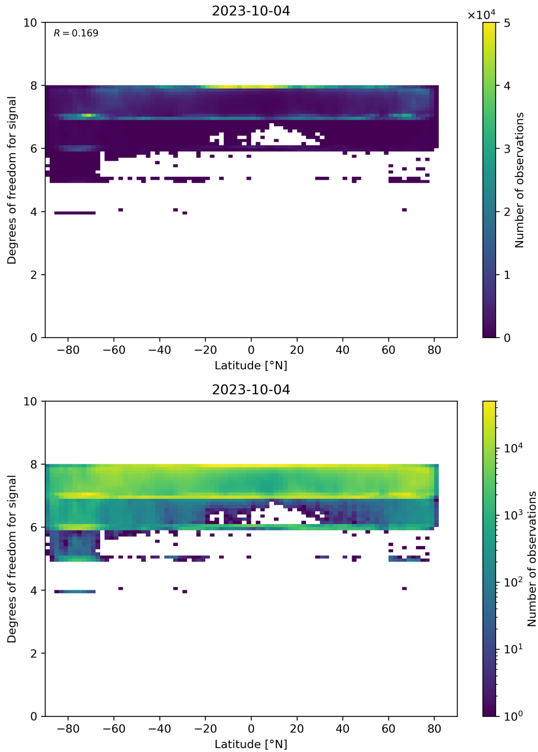
Figure 55: Scatter density plot of “Latitude” against “Degrees of freedom for signal” for 2023-10-03 to 2023-10-05.
