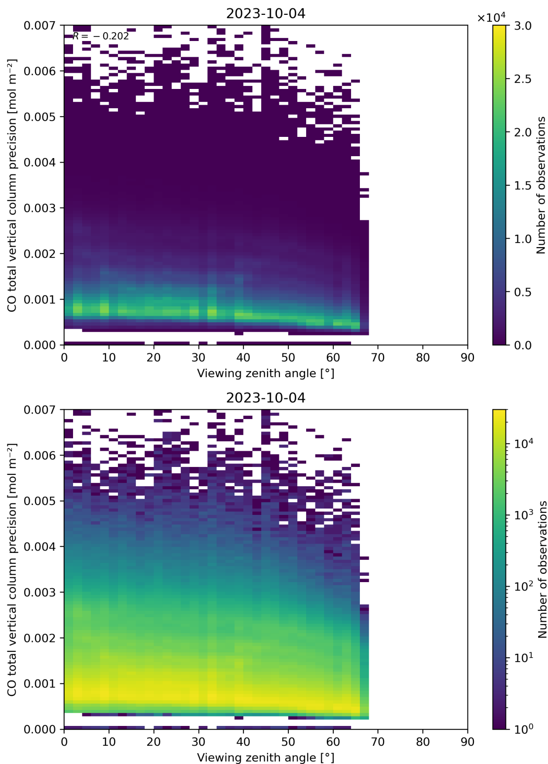
Figure 71: Scatter density plot of “Viewing zenith angle” against “CO total vertical column precision” for 2023-10-03 to 2023-10-05.
