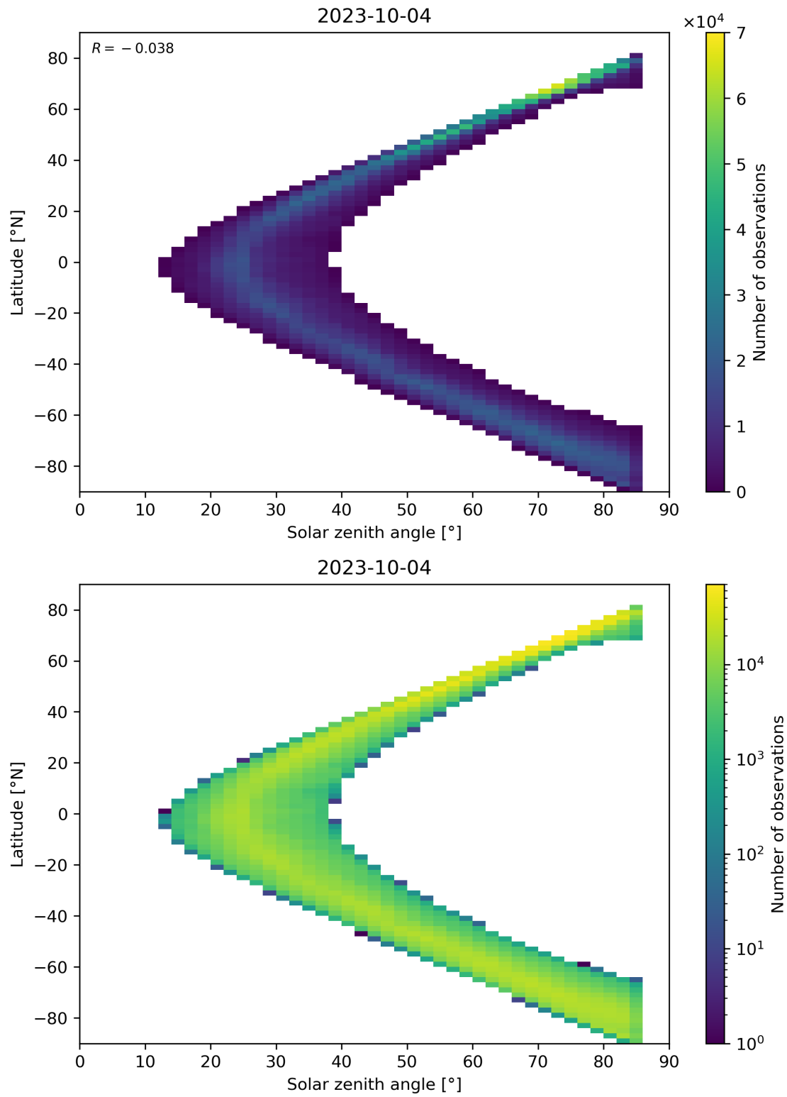
Figure 66: Scatter density plot of “Solar zenith angle” against “Latitude” for 2023-10-03 to 2023-10-05.
