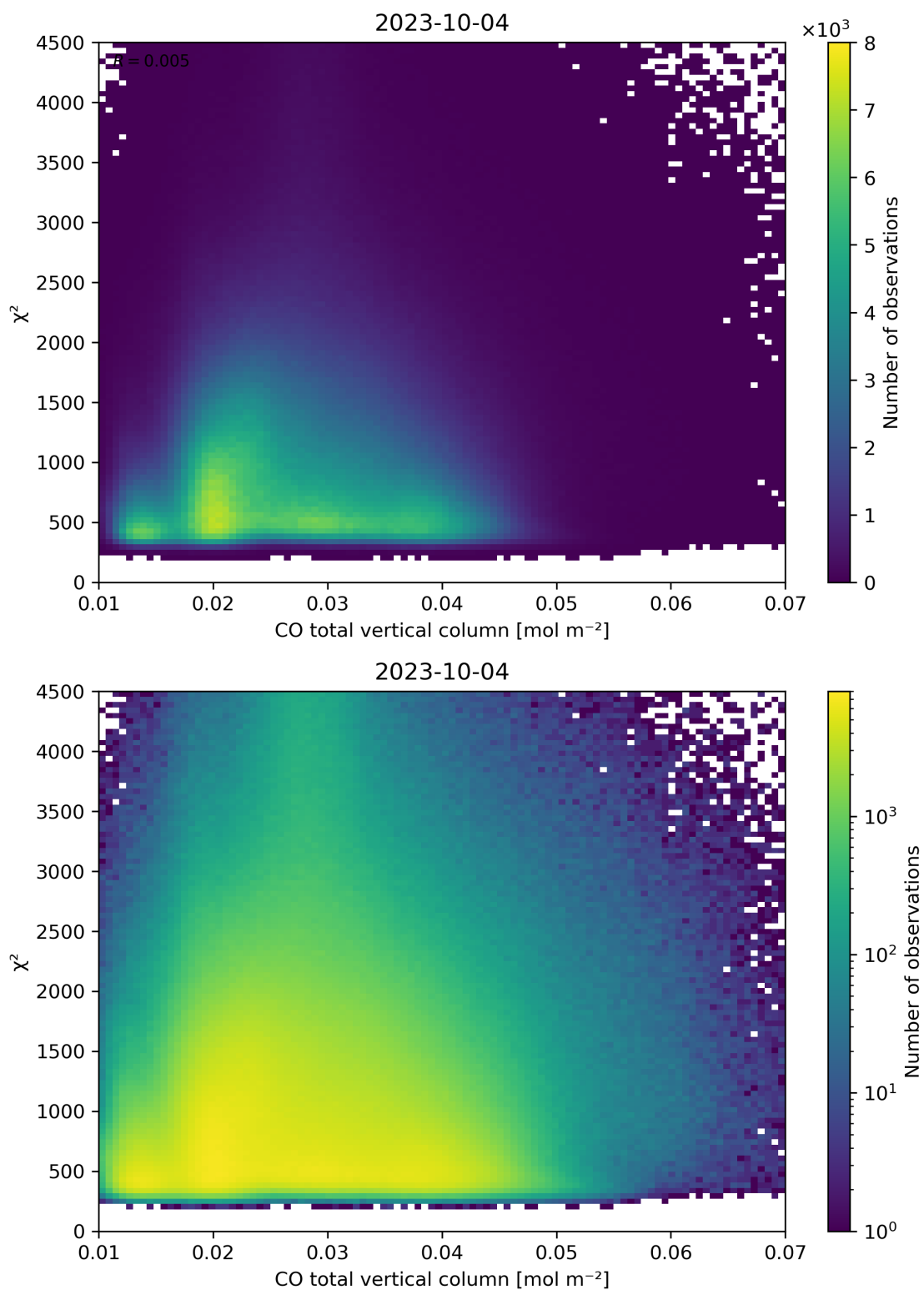
Figure 35: Scatter density plot of “CO total vertical column” against “ \chi^2 ” for 2023-10-03 to 2023-10-05.
