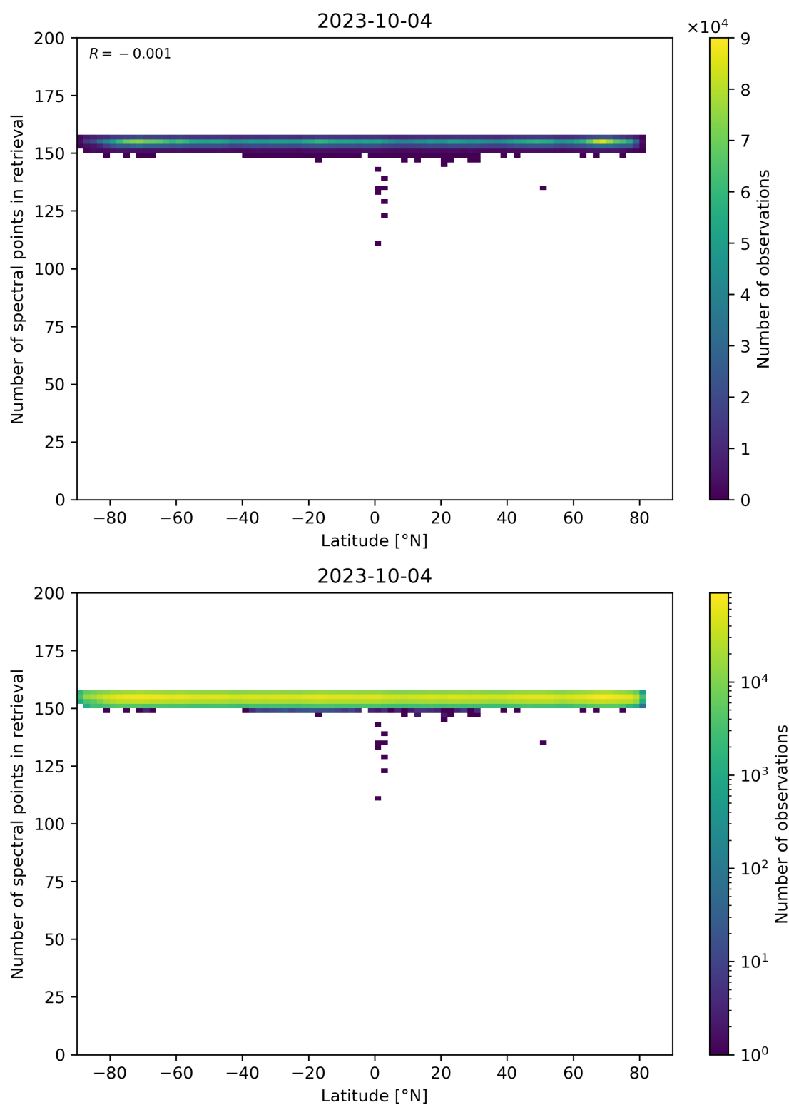
Figure 57: Scatter density plot of “Latitude” against “Number of spectral points in retrieval” for 2023-10-03 to 2023-10-05.
