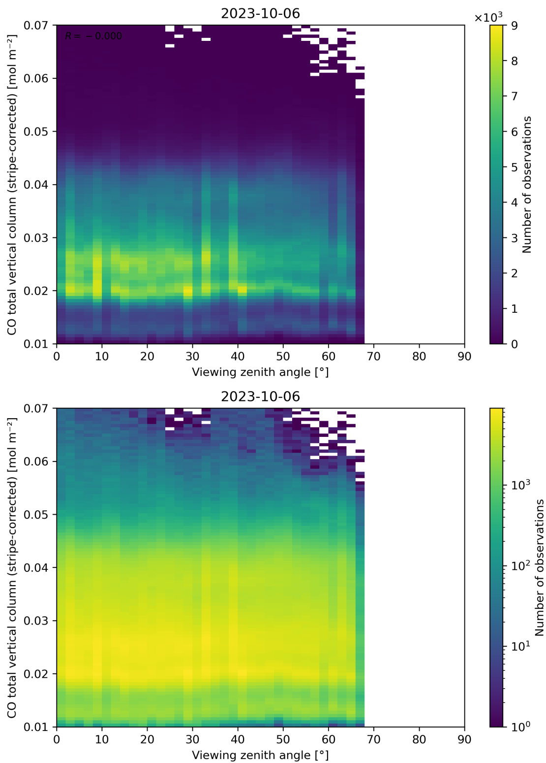
Figure 70: Scatter density plot of “Viewing zenith angle” against “CO total vertical column (stripe-corrected)” for 2023-10-06 to 2023-10-07.
