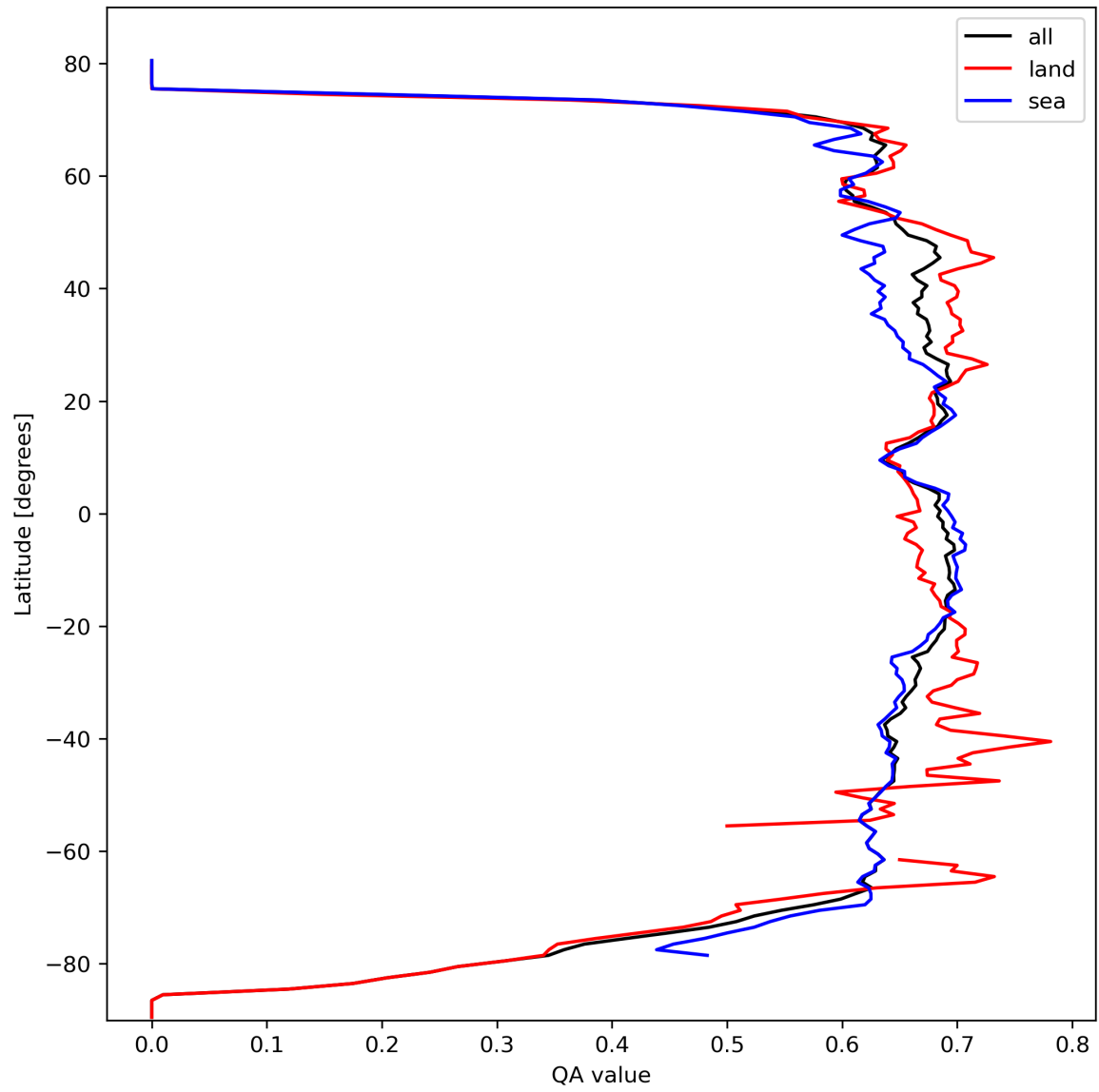
Figure 9: Zonal average of “QA value” for 2023-10-06 to 2023-10-07.
