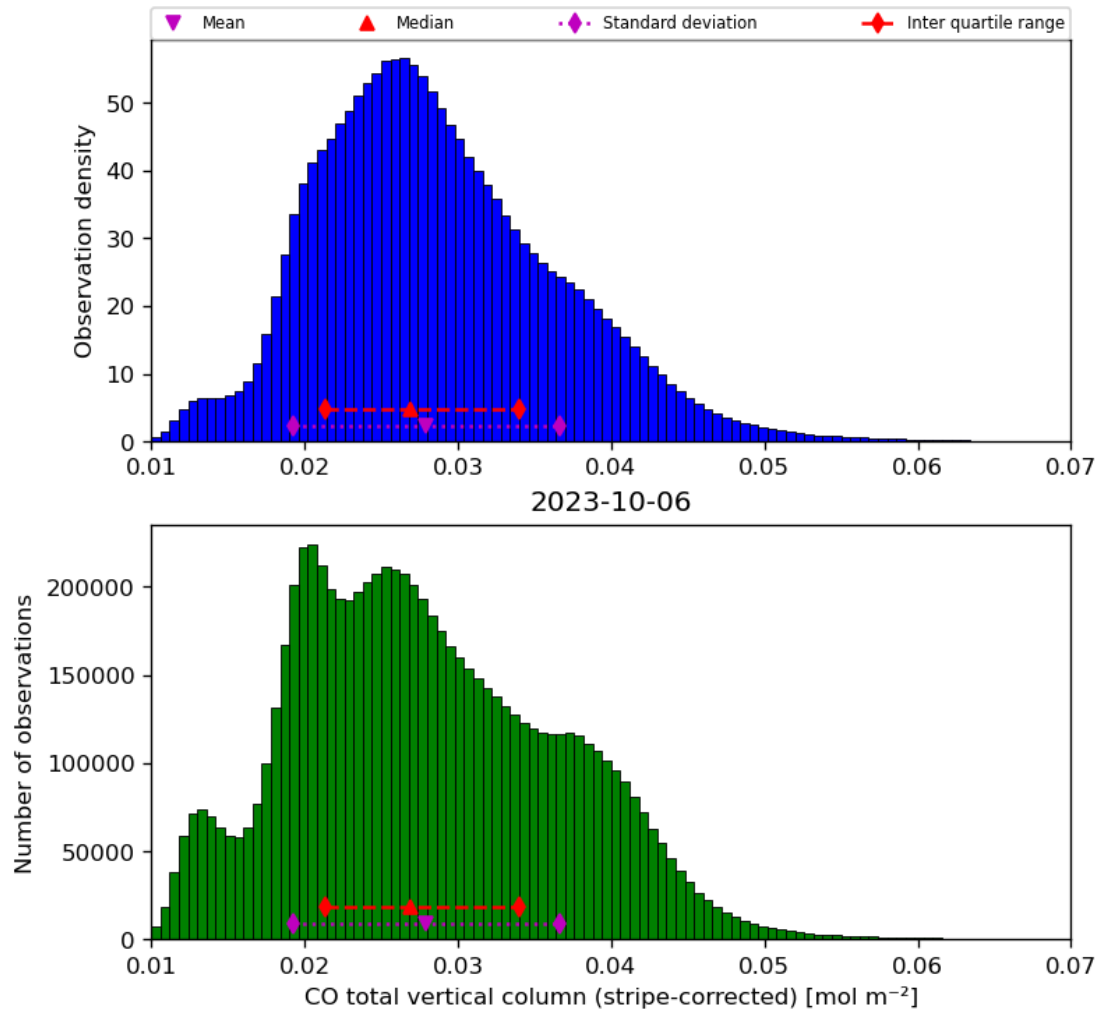
Figure 19: Histogram of “CO total vertical column (stripe-corrected)” for 2023-10-06 to 2023-10-07
