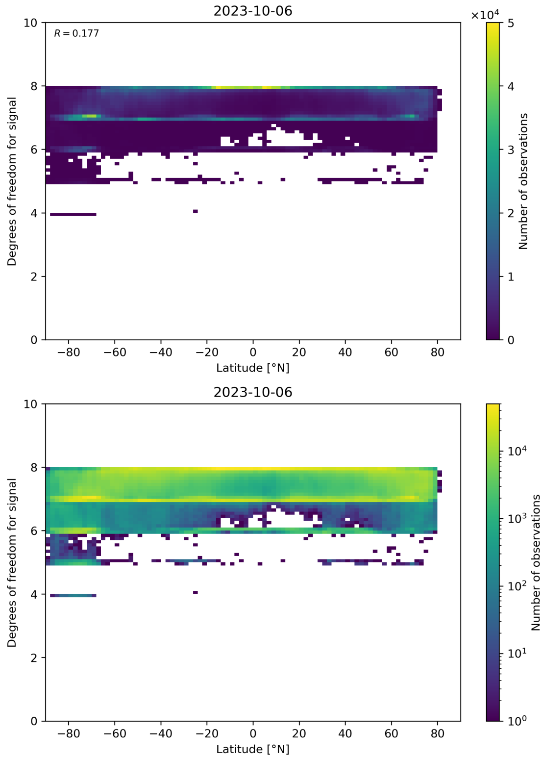
Figure 55: Scatter density plot of “Latitude” against “Degrees of freedom for signal” for 2023-10-06 to 2023-10-07.
