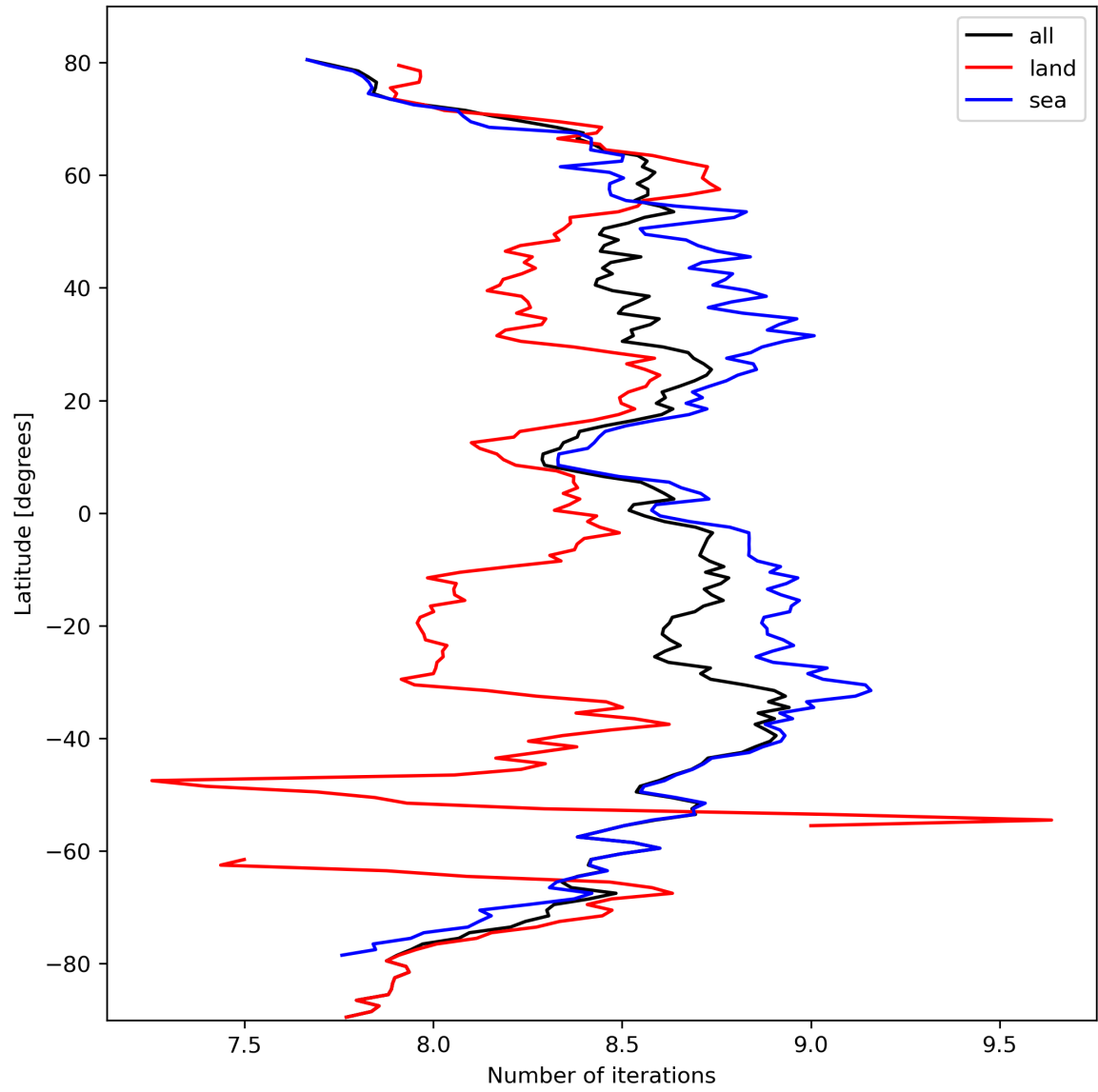
Figure 16: Zonal average of “Number of iterations” for 2023-10-06 to 2023-10-07.
