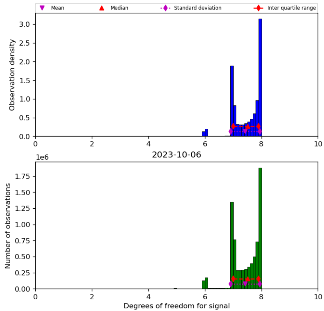
Figure 23: Histogram of “Degrees of freedom for signal” for 2023-10-06 to 2023-10-07
