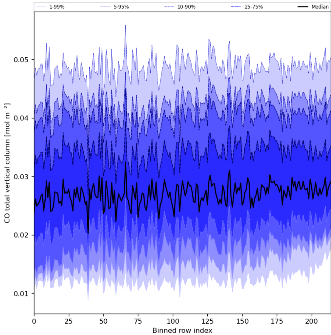
Figure 26: Along track statistics of “CO total vertical column” for 2023-10-06 to 2023-10-07
