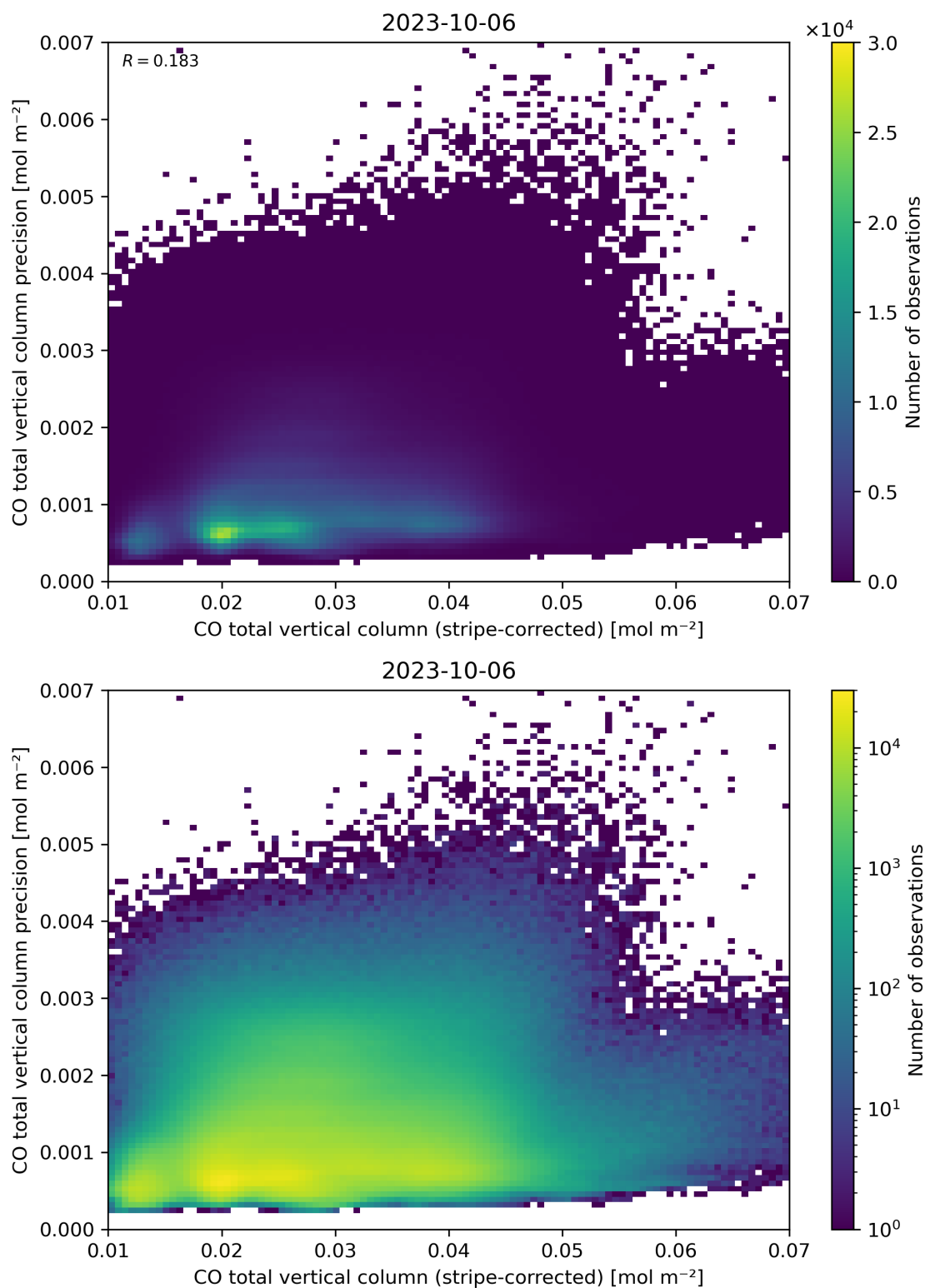
Figure 36: Scatter density plot of “CO total vertical column (stripe-corrected)” against “CO total vertical column precision” for 2023-10-06 to 2023-10-07.
