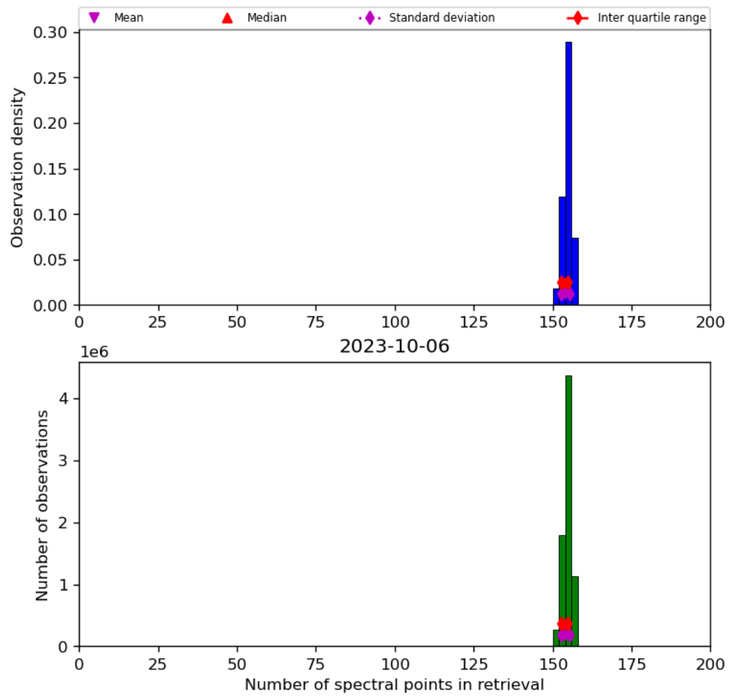
Figure 21: Histogram of “Number of spectral points in retrieval” for 2023-10-06 to 2023-10-07
