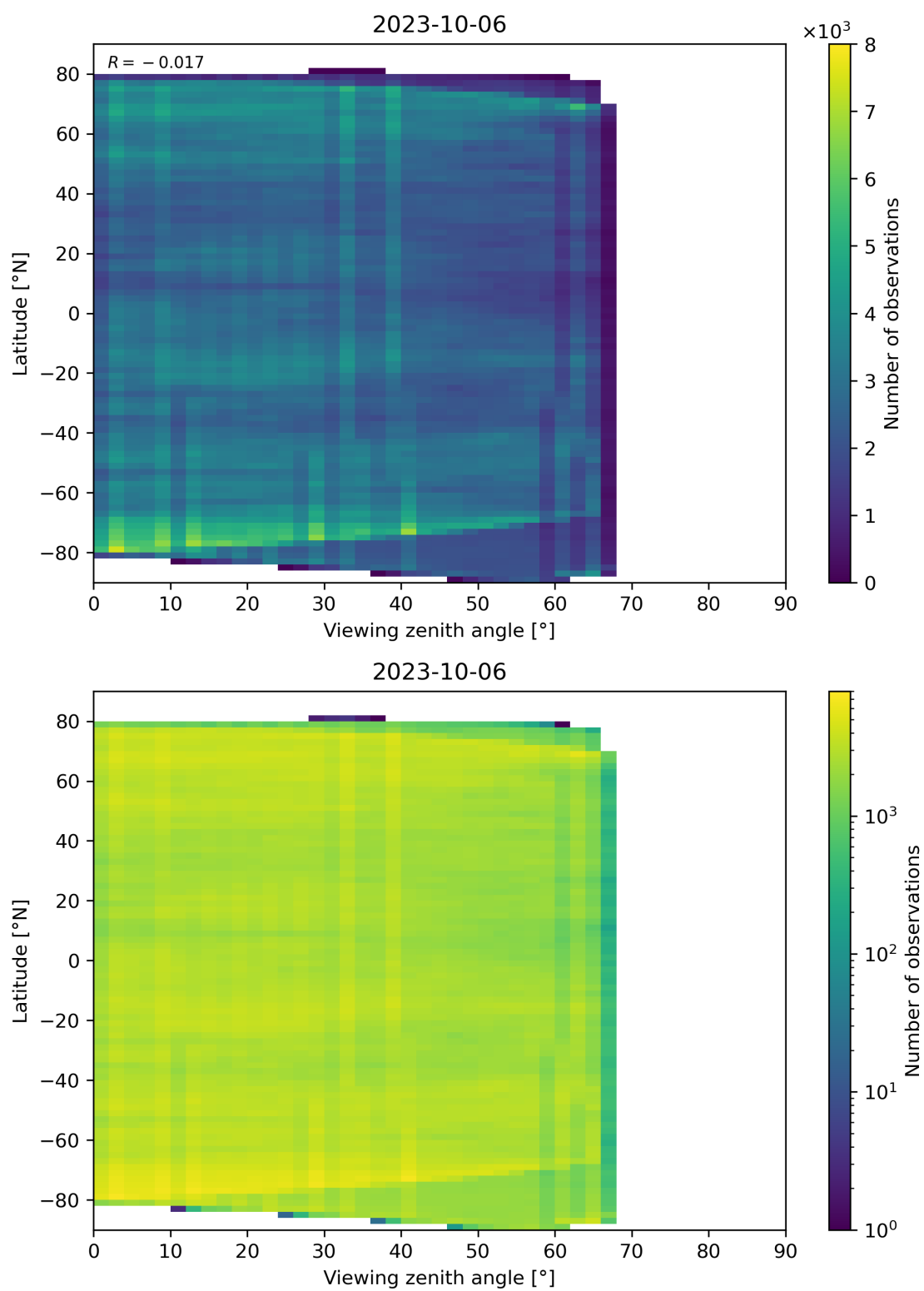
Figure 74: Scatter density plot of “Viewing zenith angle” against “Latitude” for 2023-10-06 to 2023-10-07.
