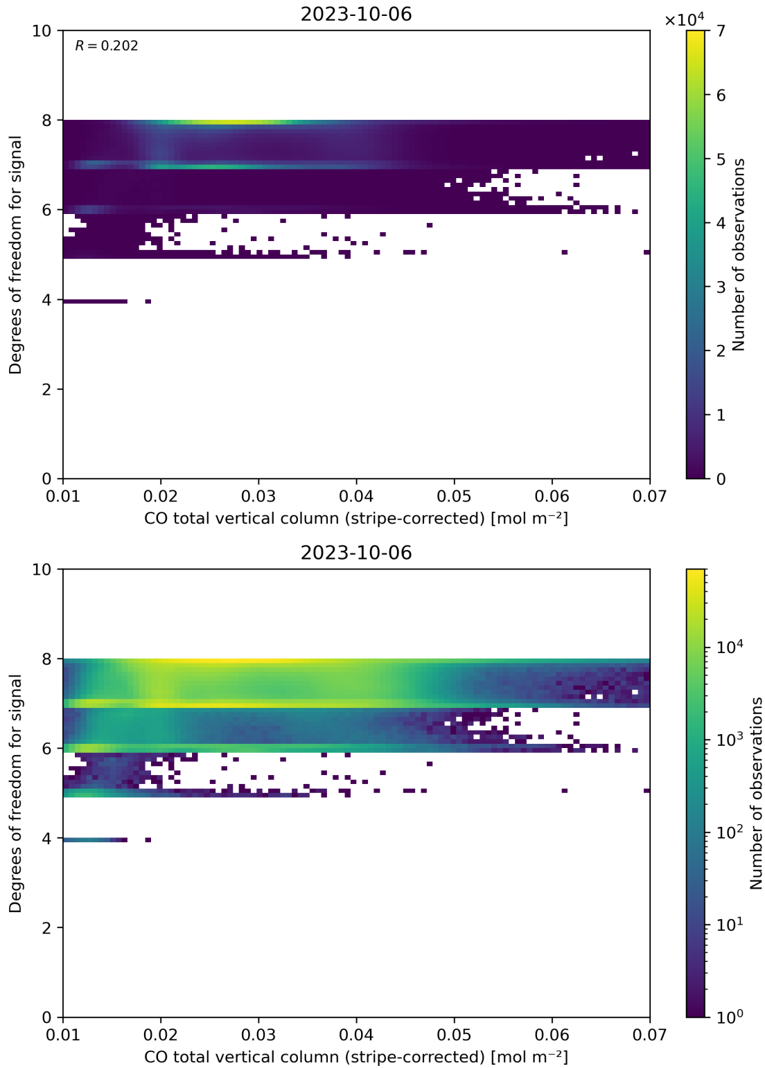
Figure 38: Scatter density plot of “CO total vertical column (stripe-corrected)” against “Degrees of freedom for signal” for 2023-10-06 to 2023-10-07.
