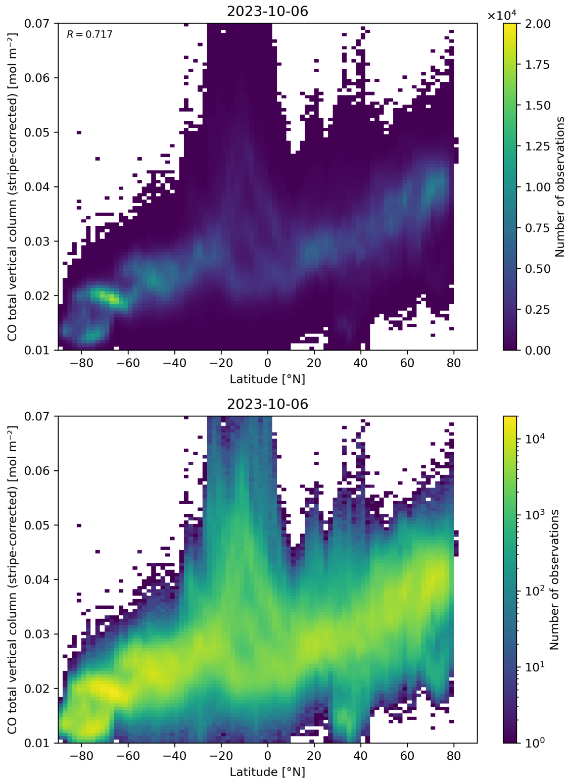
Figure 52: Scatter density plot of “Latitude” against “CO total vertical column (stripe-corrected)” for 2023-10-06 to 2023-10-07.
