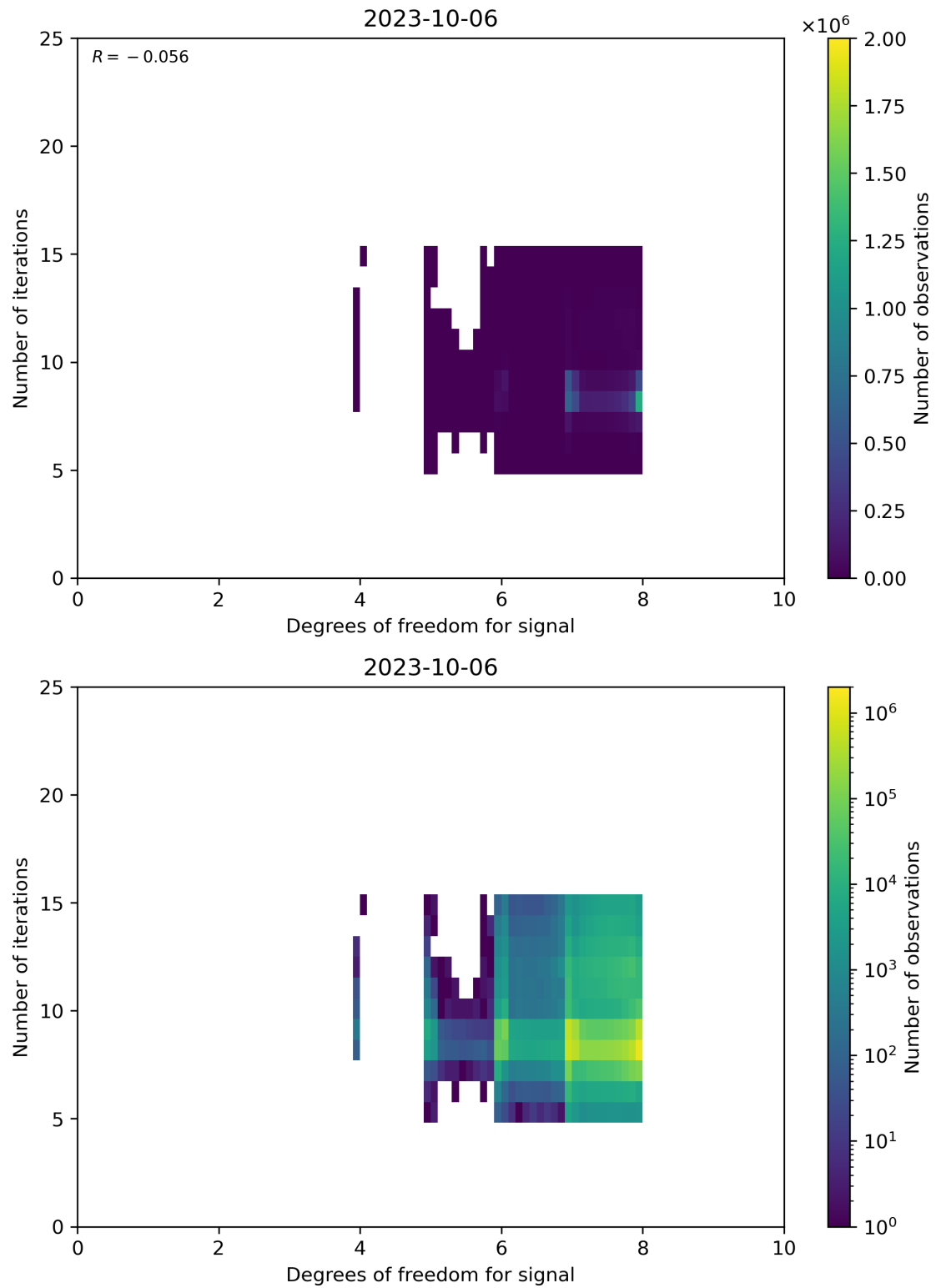
Figure 50: Scatter density plot of “Degrees of freedom for signal” against “Number of iterations” for 2023-10-06 to 2023-10-07.
