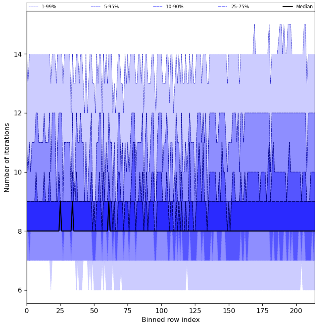
Figure 32: Along track statistics of “Number of iterations” for 2023-10-06 to 2023-10-07
