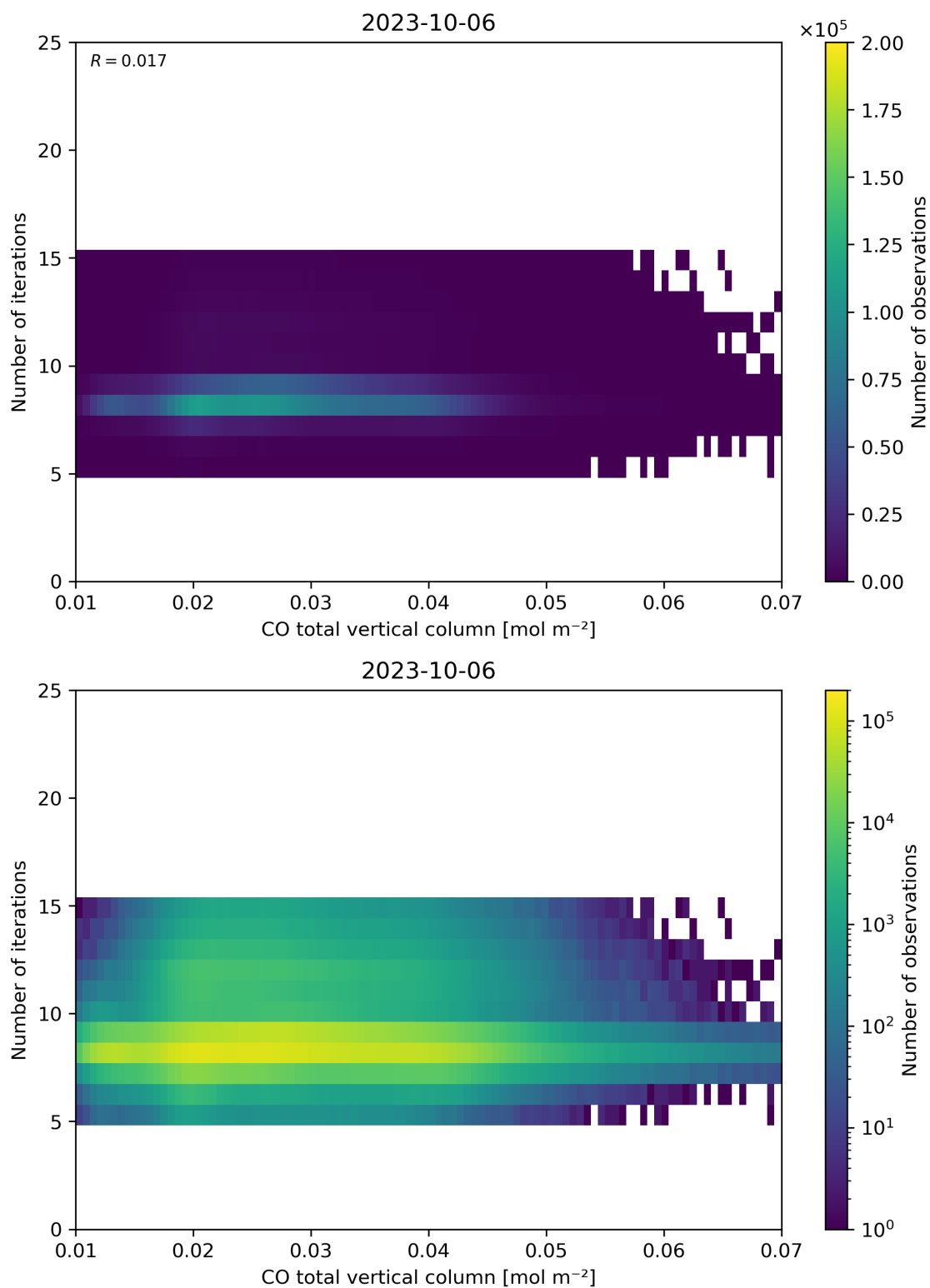
Figure 42: Scatter density plot of “CO total vertical column” against “Number of iterations” for 2023-10-06 to 2023-10-07.
