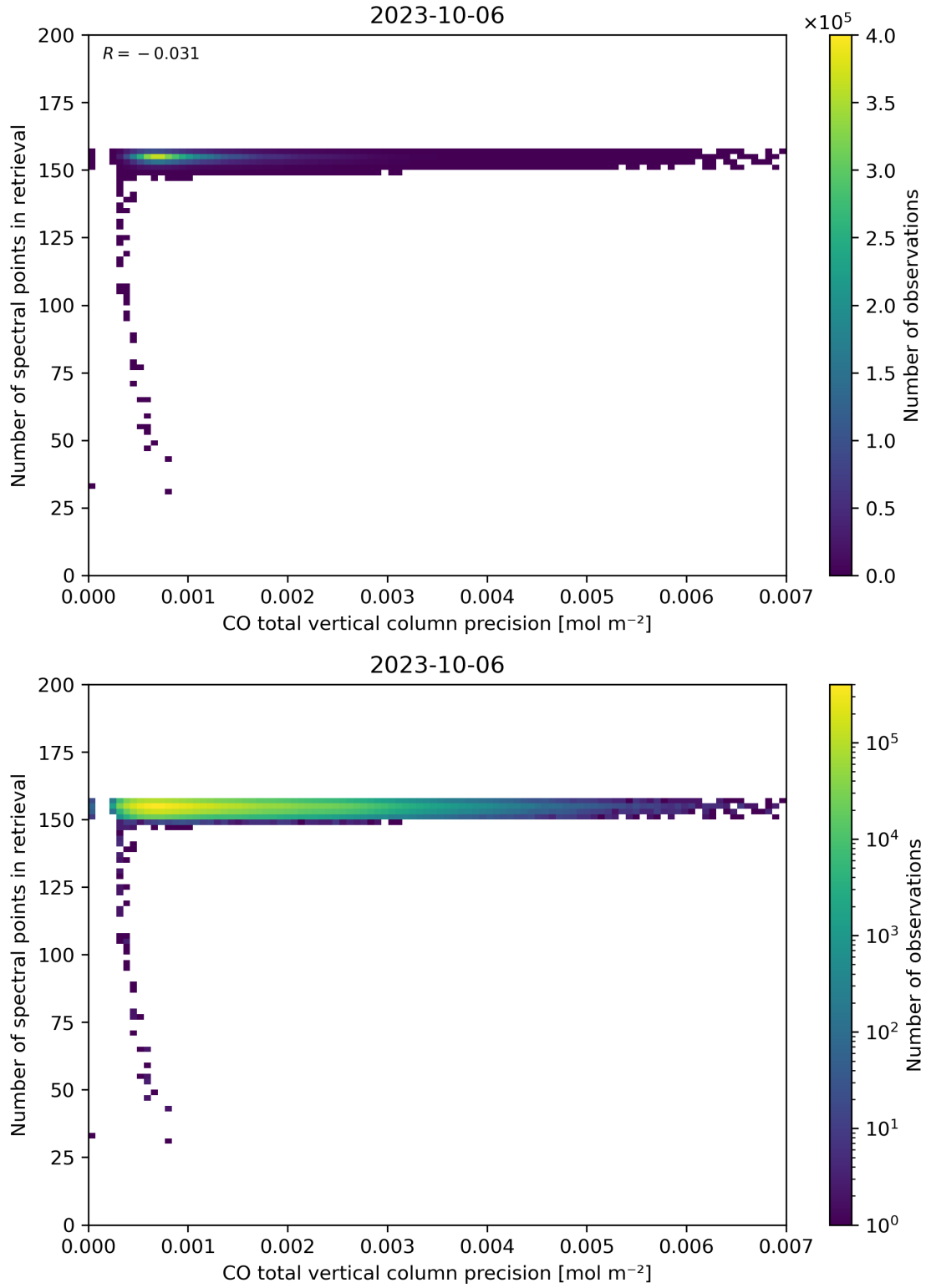
Figure 47: Scatter density plot of “CO total vertical column precision” against “Number of spectral points in retrieval” for 2023-10-06 to 2023-10-07.
