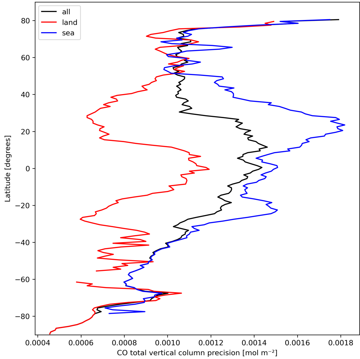
Figure 12: Zonal average of “CO total vertical column precision” for 2023-10-06 to 2023-10-07.
