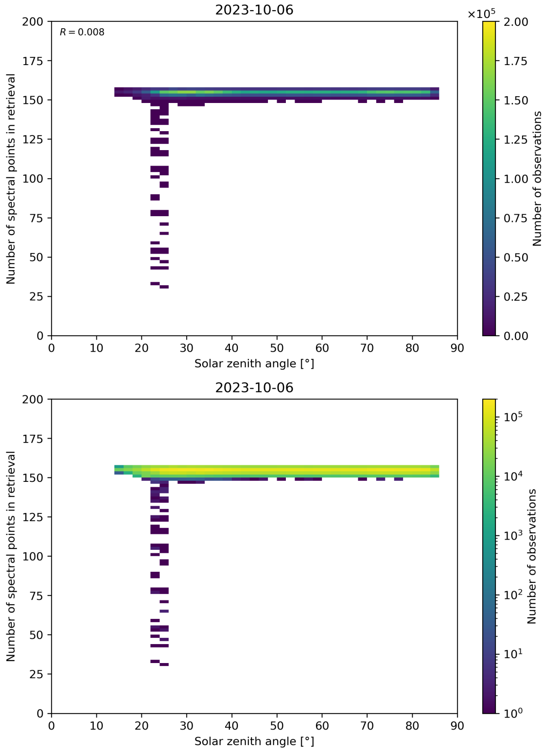
Figure 68: Scatter density plot of “Solar zenith angle” against “Number of spectral points in retrieval” for 2023-10-06 to 2023-10-07.
