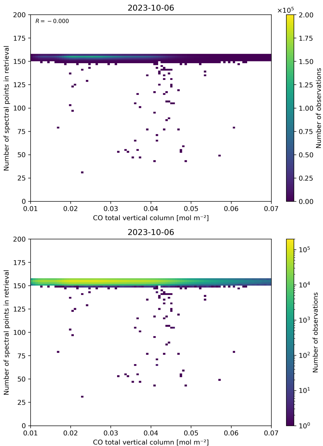
Figure 43: Scatter density plot of “CO total vertical column” against “Number of spectral points in retrieval” for 2023-10-06 to 2023-10-07.
