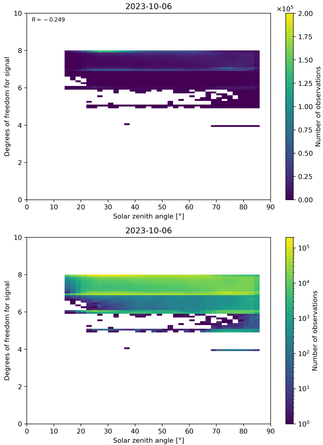
Figure 65: Scatter density plot of “Solar zenith angle” against “Degrees of freedom for signal” for 2023-10-06 to 2023-10-07.
