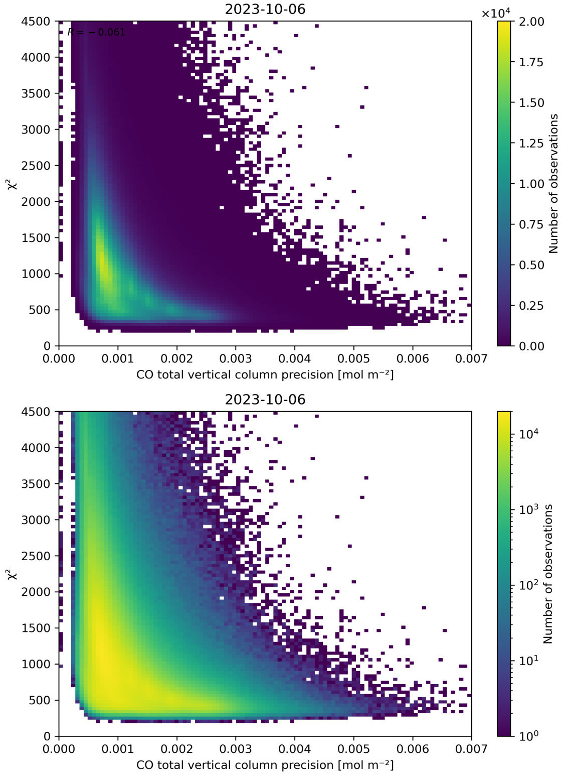
Figure 44: Scatter density plot of “CO total vertical column precision” against “ \chi^2 ” for 2023-10-06 to 2023-10-07.
