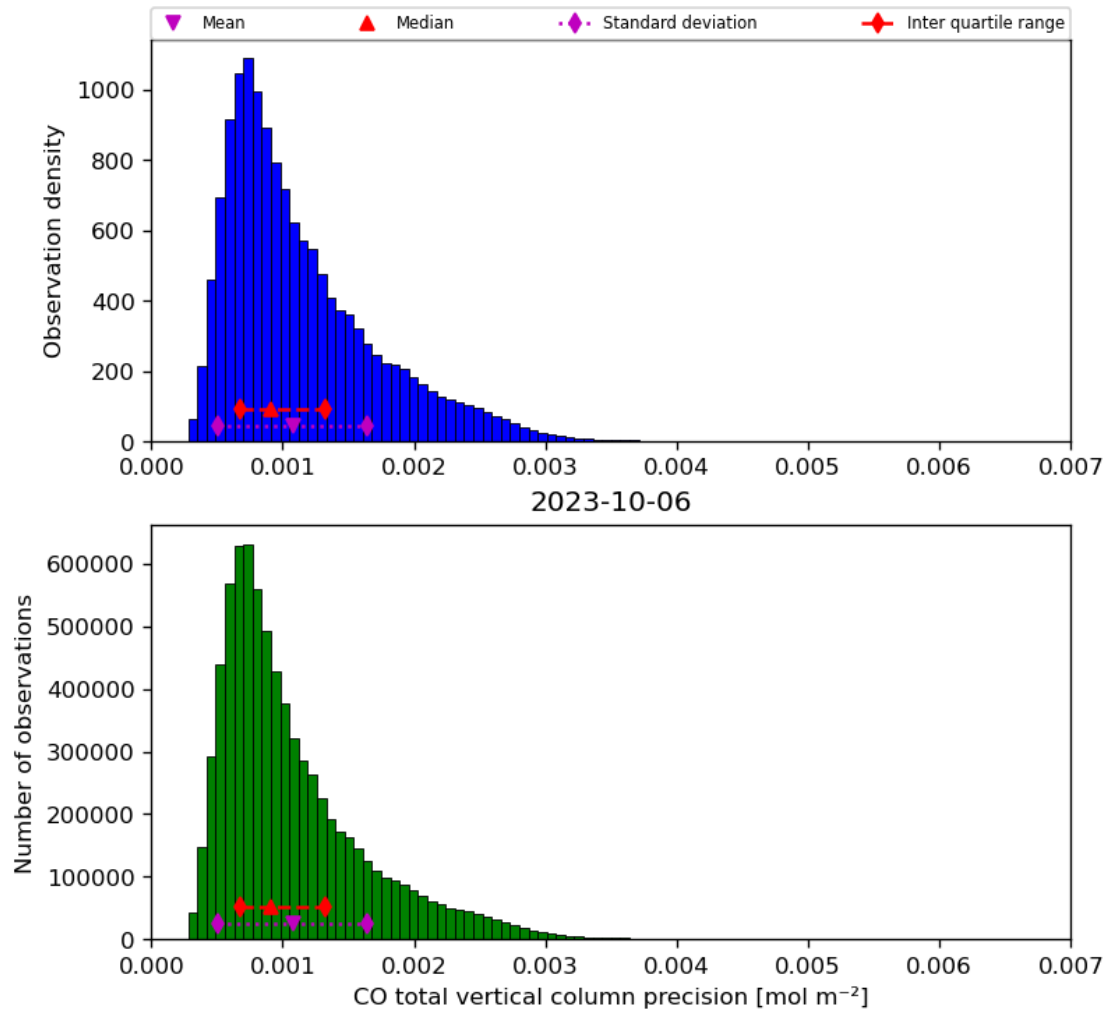
Figure 20: Histogram of “CO total vertical column precision” for 2023-10-06 to 2023-10-07
