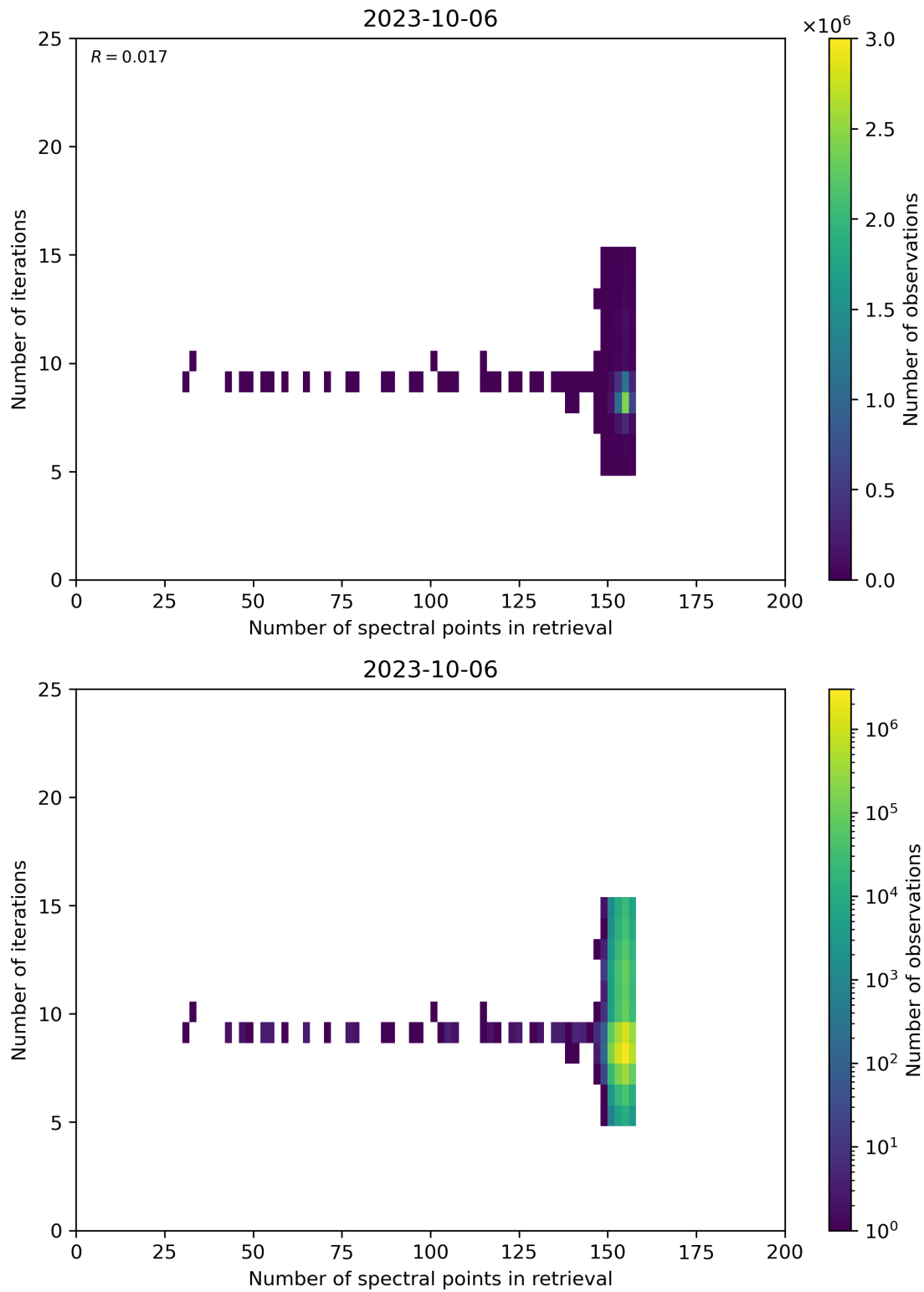
Figure 60: Scatter density plot of “Number of spectral points in retrieval” against “Number of iterations” for 2023-10-06 to 2023-10-07.
