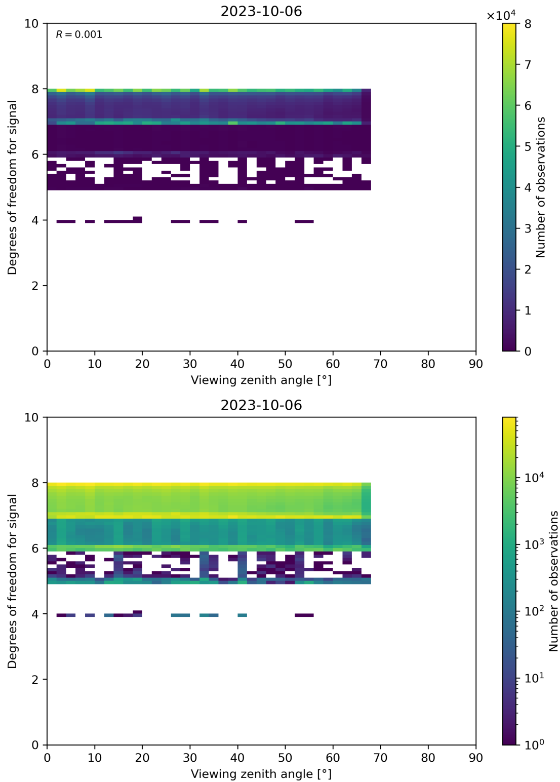
Figure 73: Scatter density plot of “Viewing zenith angle” against “Degrees of freedom for signal” for 2023-10-06 to 2023-10-07.
