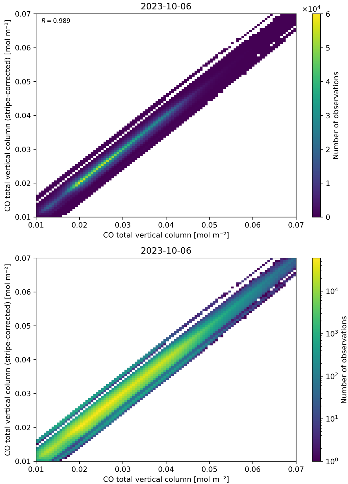
Figure 33: Scatter density plot of “CO total vertical column” against “CO total vertical column (stripe-corrected)” for 2023-10-06 to 2023-10-07.
