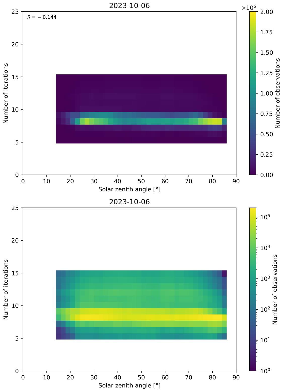
Figure 67: Scatter density plot of “Solar zenith angle” against “Number of iterations” for 2023-10-06 to 2023-10-07.
