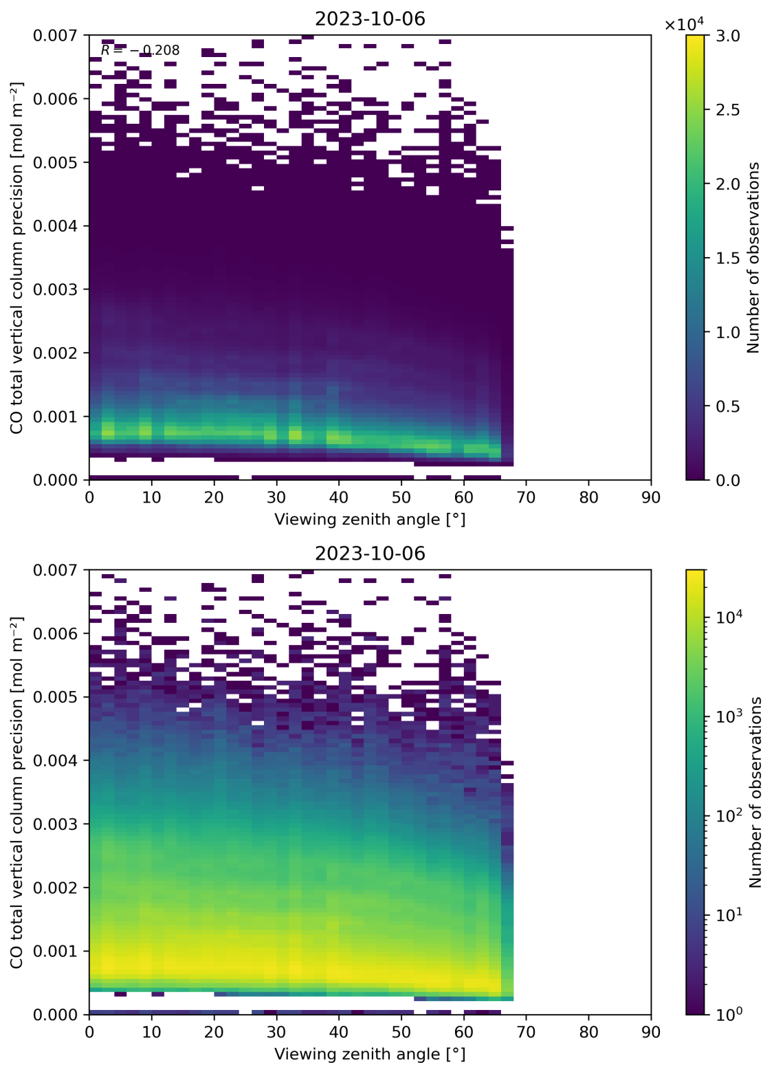
Figure 71: Scatter density plot of “Viewing zenith angle” against “CO total vertical column precision” for 2023-10-06 to 2023-10-07.
