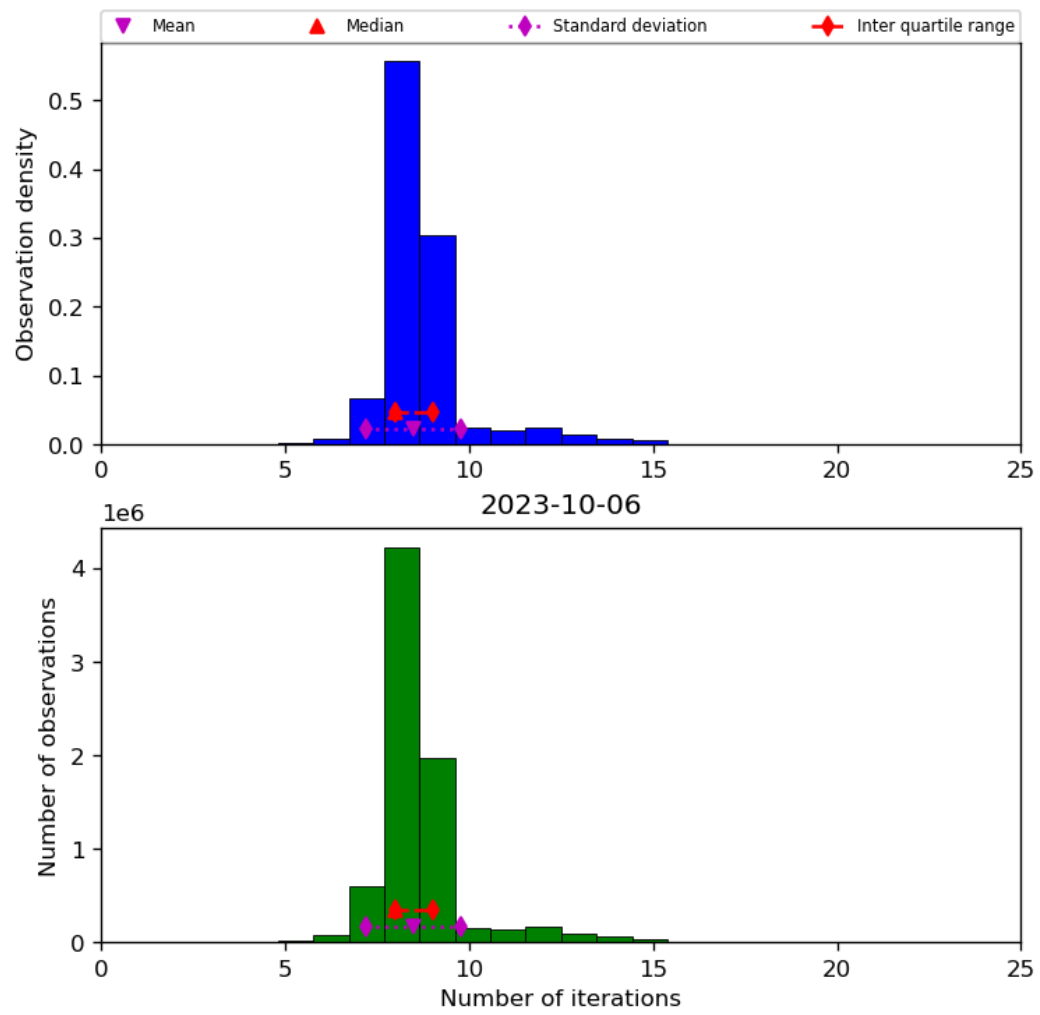
Figure 24: Histogram of “Number of iterations” for 2023-10-06 to 2023-10-07
