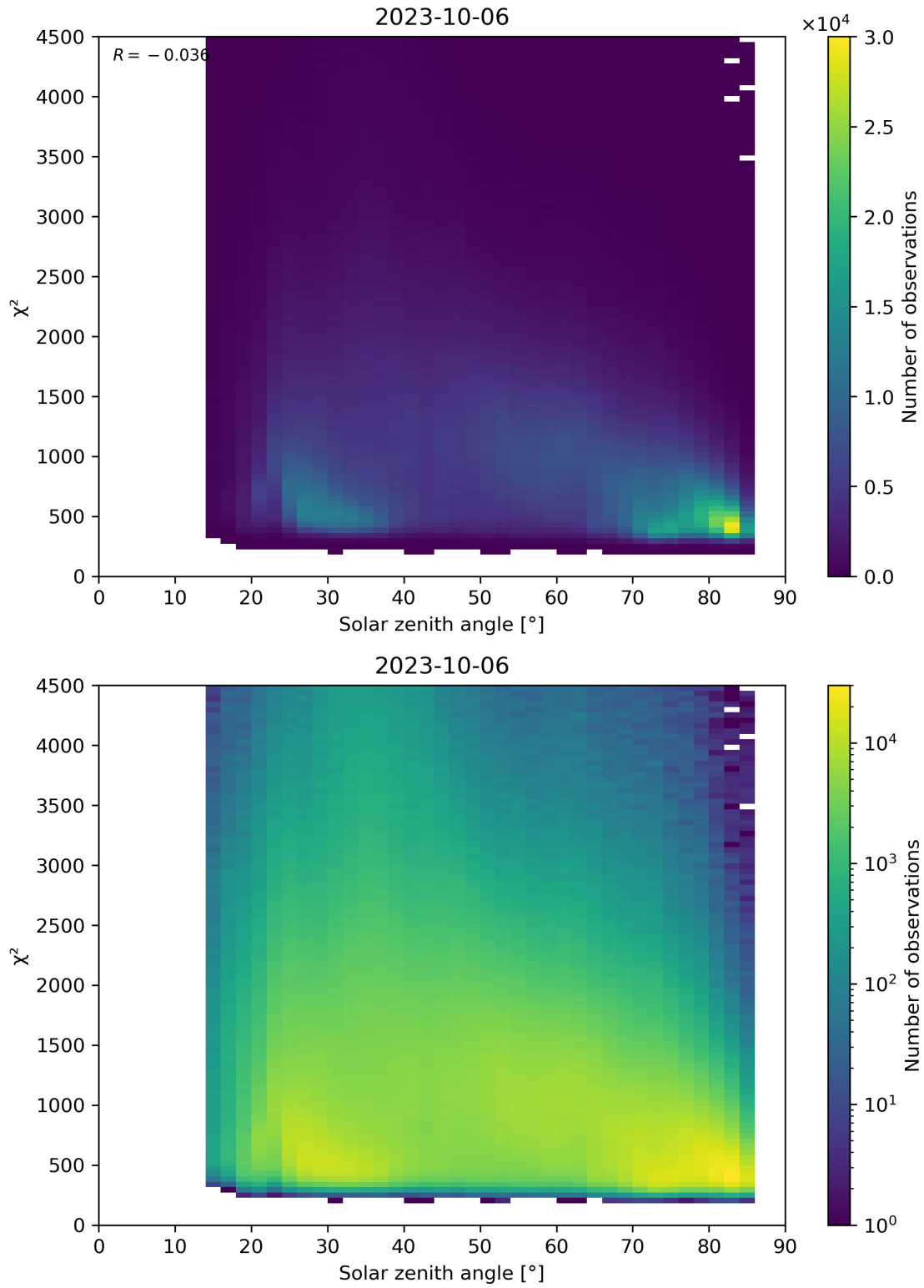
Figure 64: Scatter density plot of “Solar zenith angle” against “ \chi^2 ” for 2023-10-06 to 2023-10-07.
