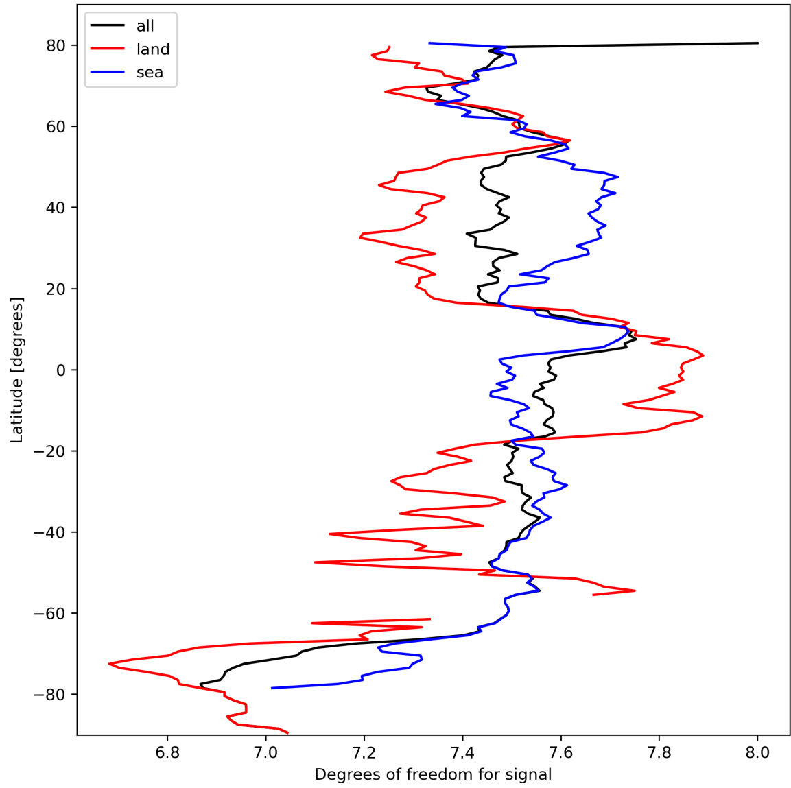
Figure 15: Zonal average of “Degrees of freedom for signal” for 2023-10-06 to 2023-10-07.
