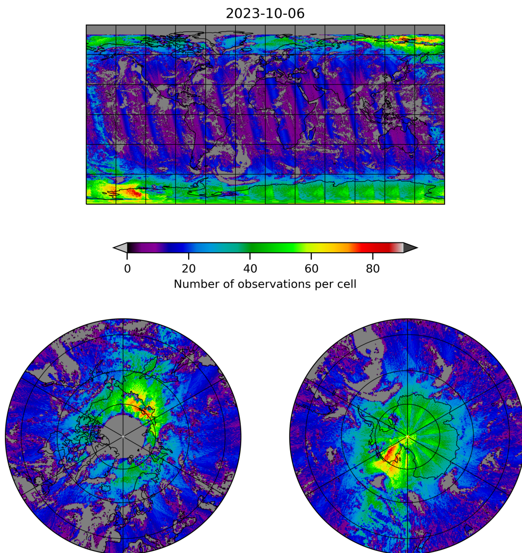
Figure 8: Map of the number of observations for 2023-10-06 to 2023-10-07
