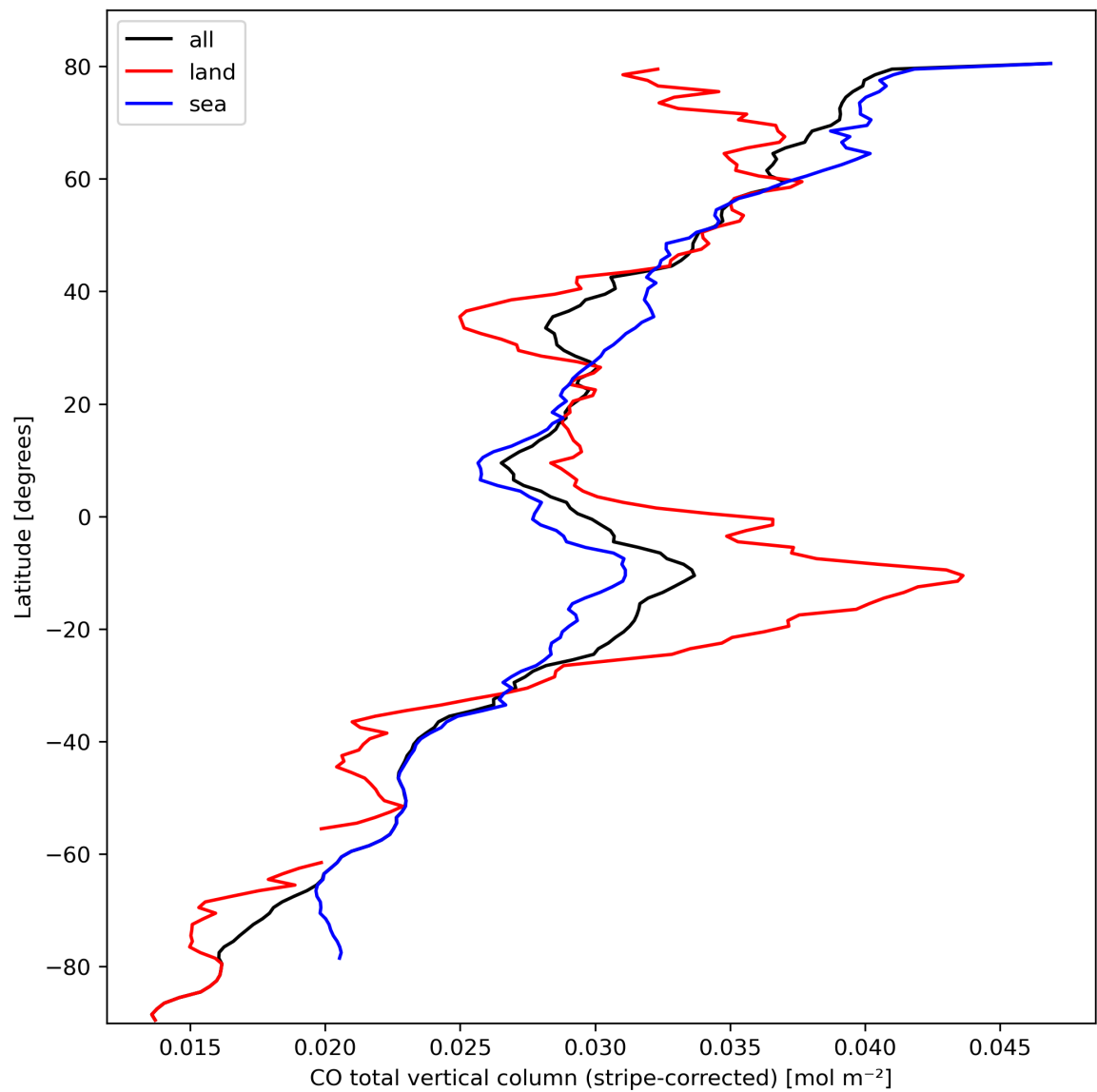
Figure 11: Zonal average of “CO total vertical column (stripe-corrected)” for 2023-10-06 to 2023-10-07.
