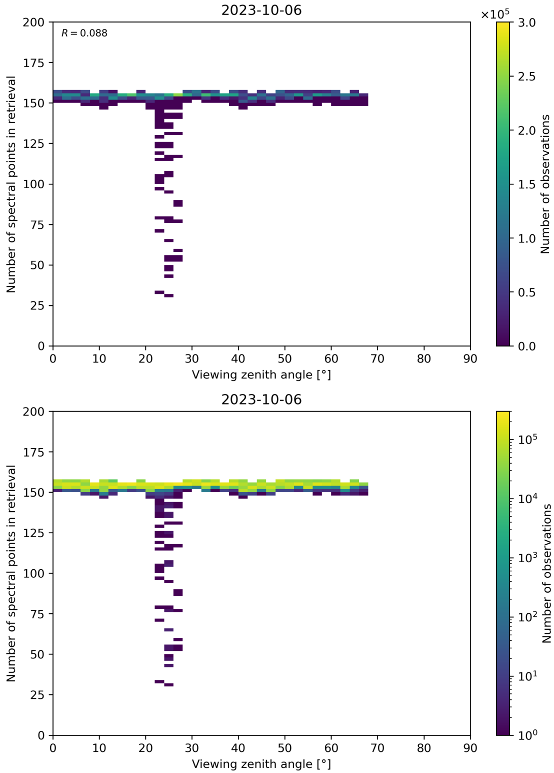
Figure 76: Scatter density plot of “Viewing zenith angle” against “Number of spectral points in retrieval” for 2023-10-06 to 2023-10-07.
