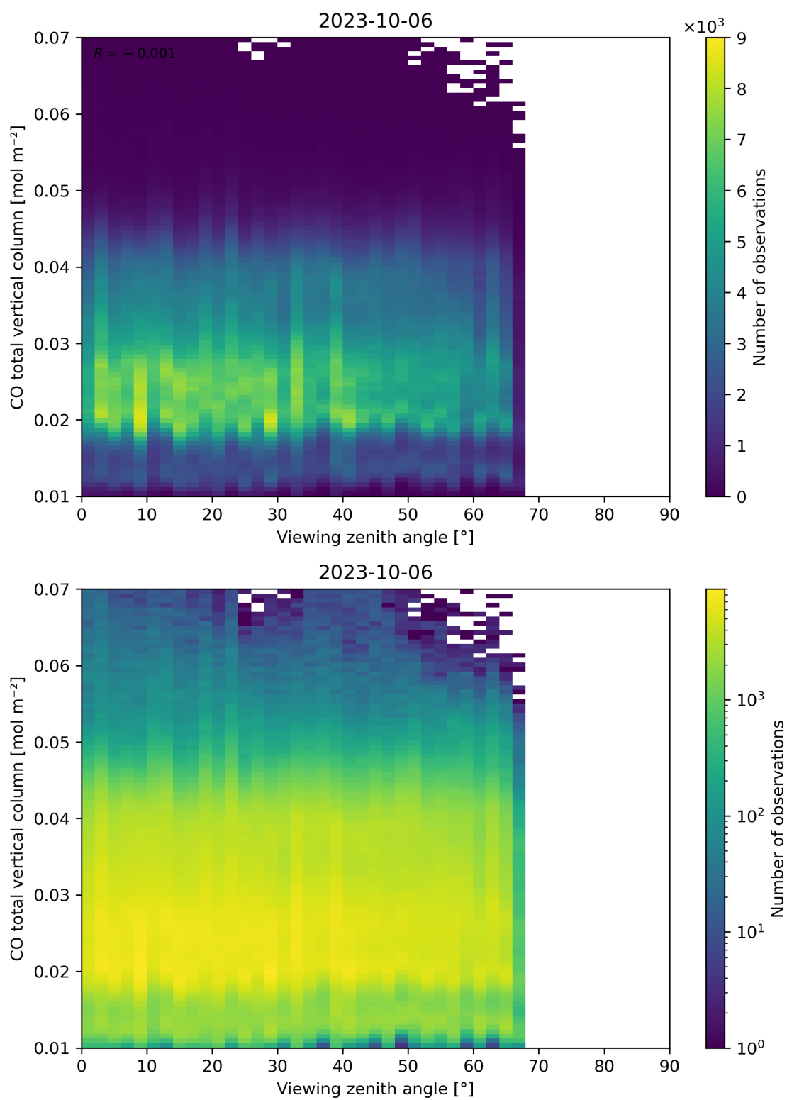
Figure 69: Scatter density plot of “Viewing zenith angle” against “CO total vertical column” for 2023-10-06 to 2023-10-07.
