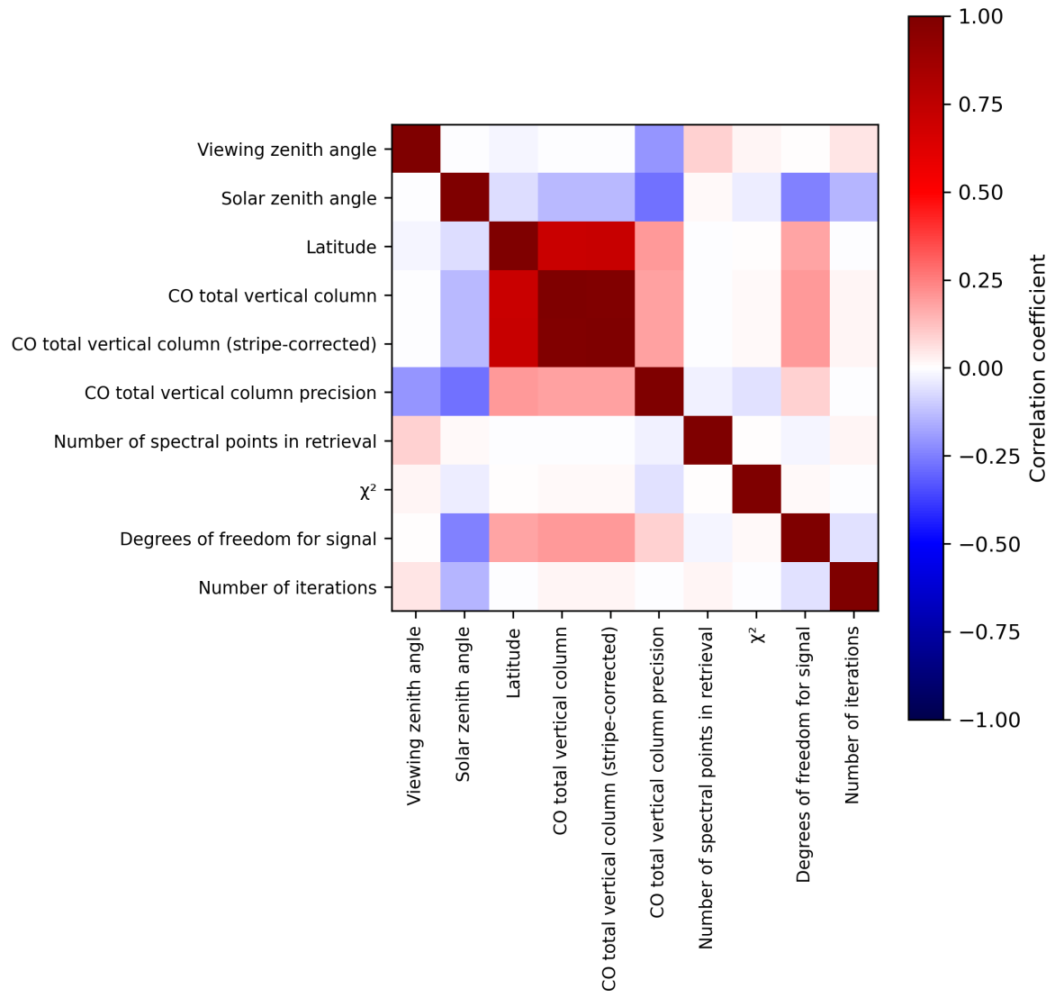
Figure 2: Map of correlation matrix for 2023-10-06 to 2023-10-07.
