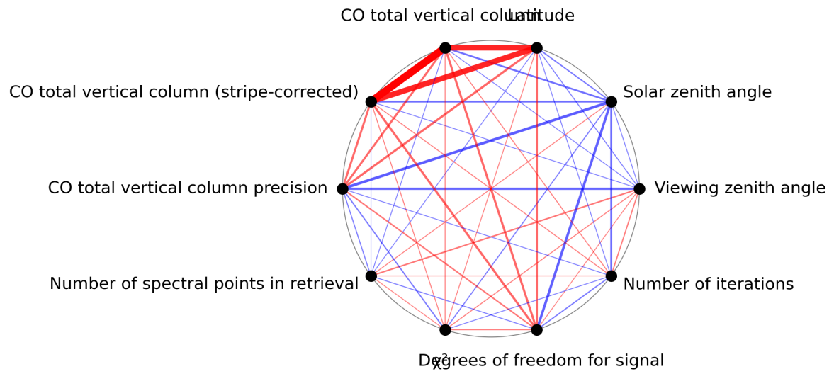
Figure 1: Map of correlation graph for 2023-10-06 to 2023-10-07.
