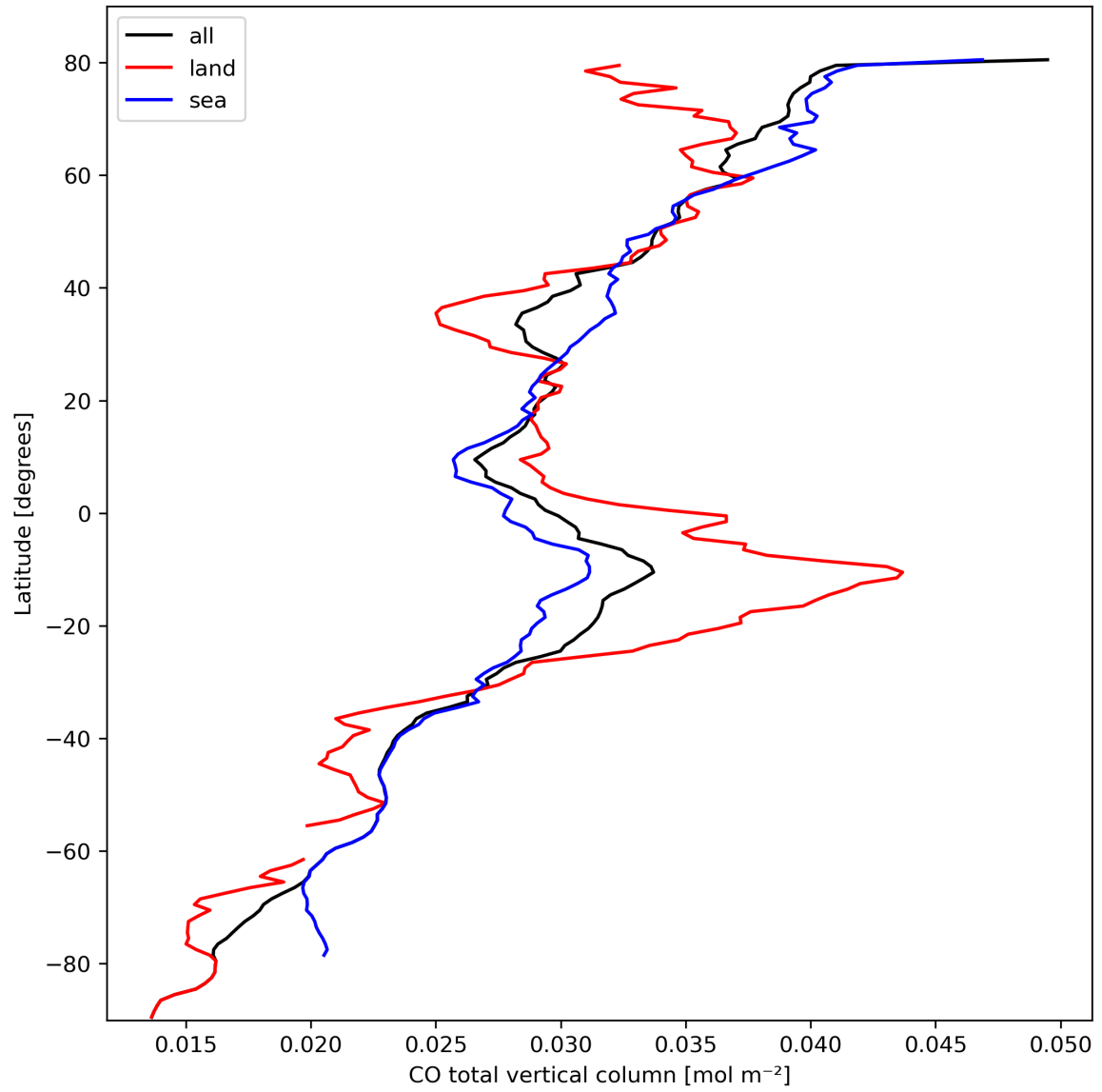
Figure 10: Zonal average of “CO total vertical column” for 2023-10-06 to 2023-10-07.
