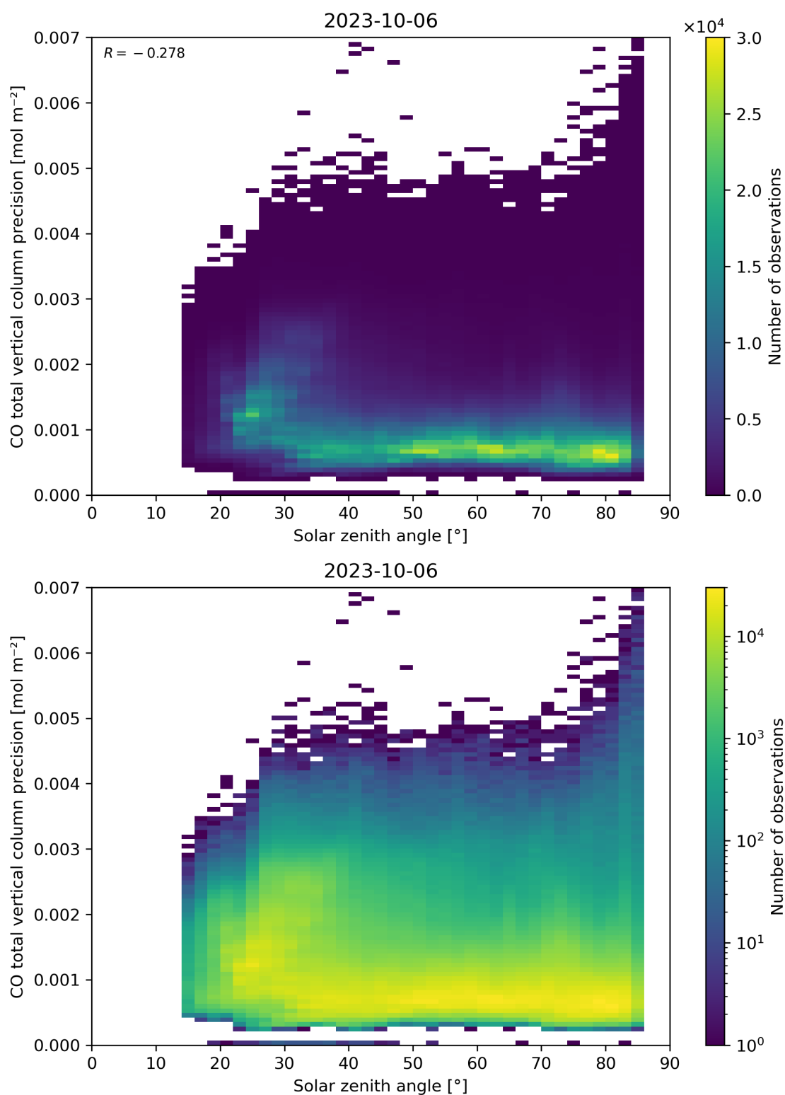
Figure 63: Scatter density plot of “Solar zenith angle” against “CO total vertical column precision” for 2023-10-06 to 2023-10-07.
