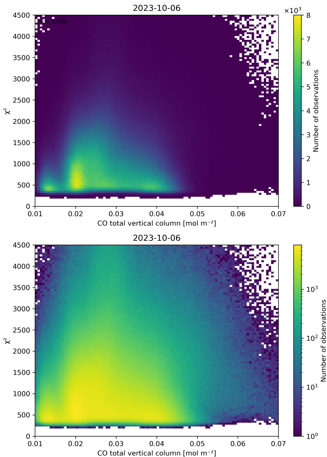
Figure 35: Scatter density plot of “CO total vertical column” against “ \chi^2 ” for 2023-10-06 to 2023-10-07.
