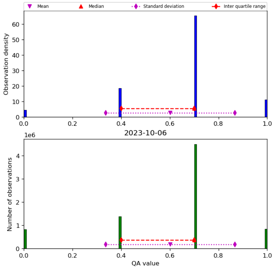
Figure 17: Histogram of “QA value” for 2023-10-06 to 2023-10-07
