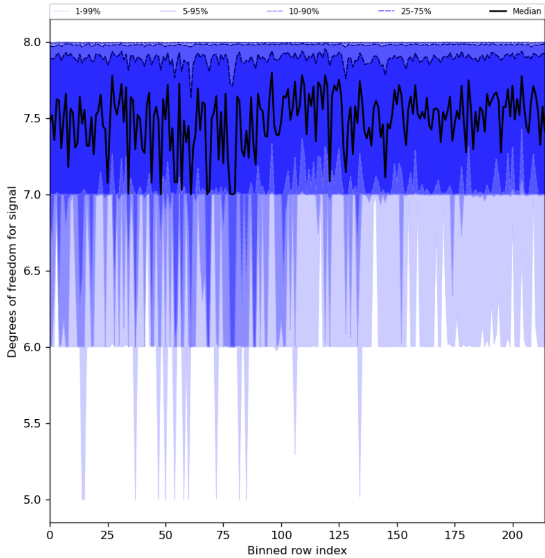
Figure 31: Along track statistics of “Degrees of freedom for signal” for 2023-10-06 to 2023-10-07
