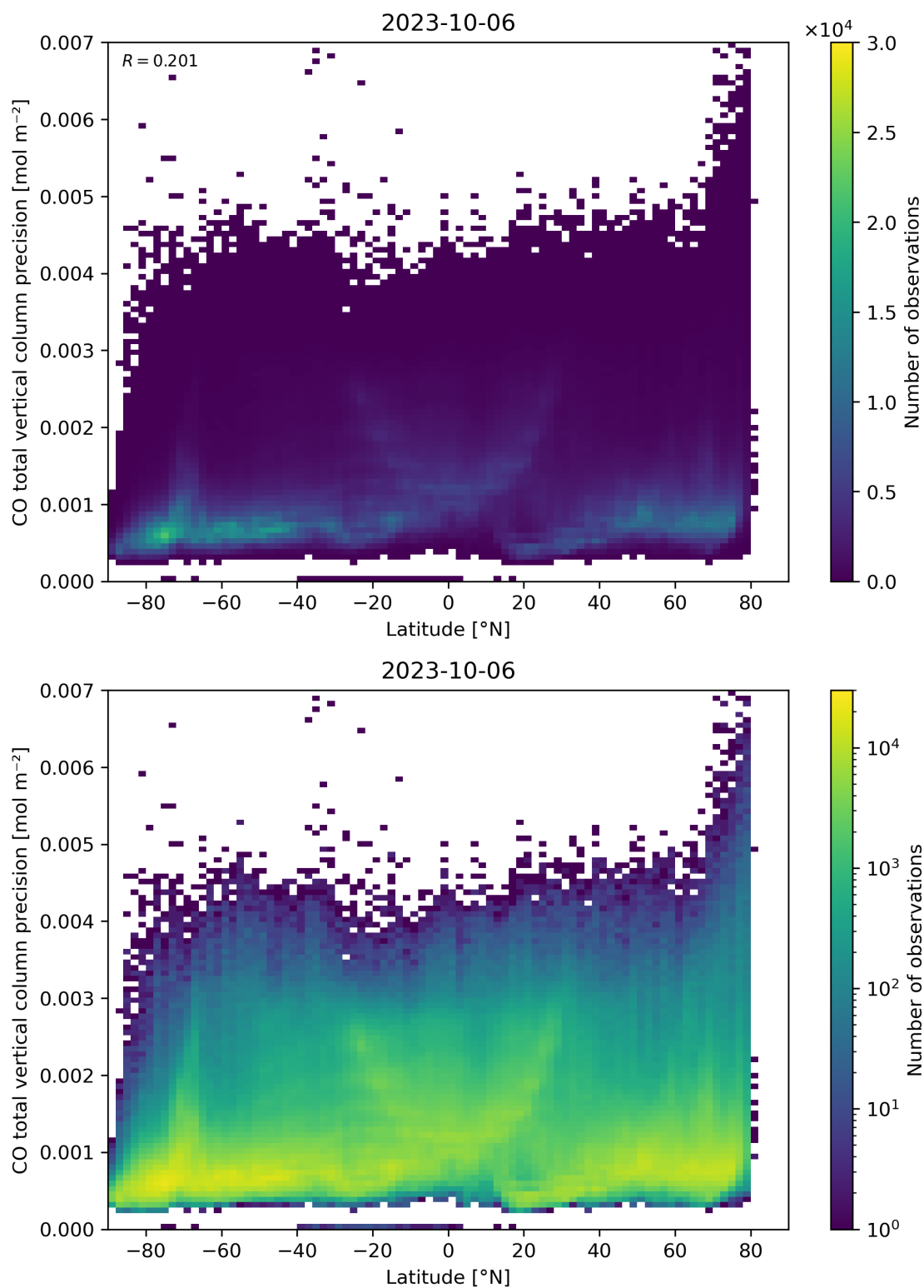
Figure 53: Scatter density plot of “Latitude” against “CO total vertical column precision” for 2023-10-06 to 2023-10-07.
