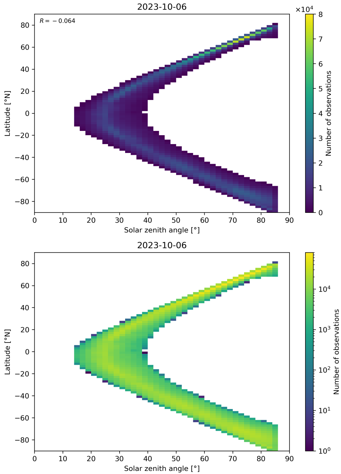
Figure 66: Scatter density plot of “Solar zenith angle” against “Latitude” for 2023-10-06 to 2023-10-07.
