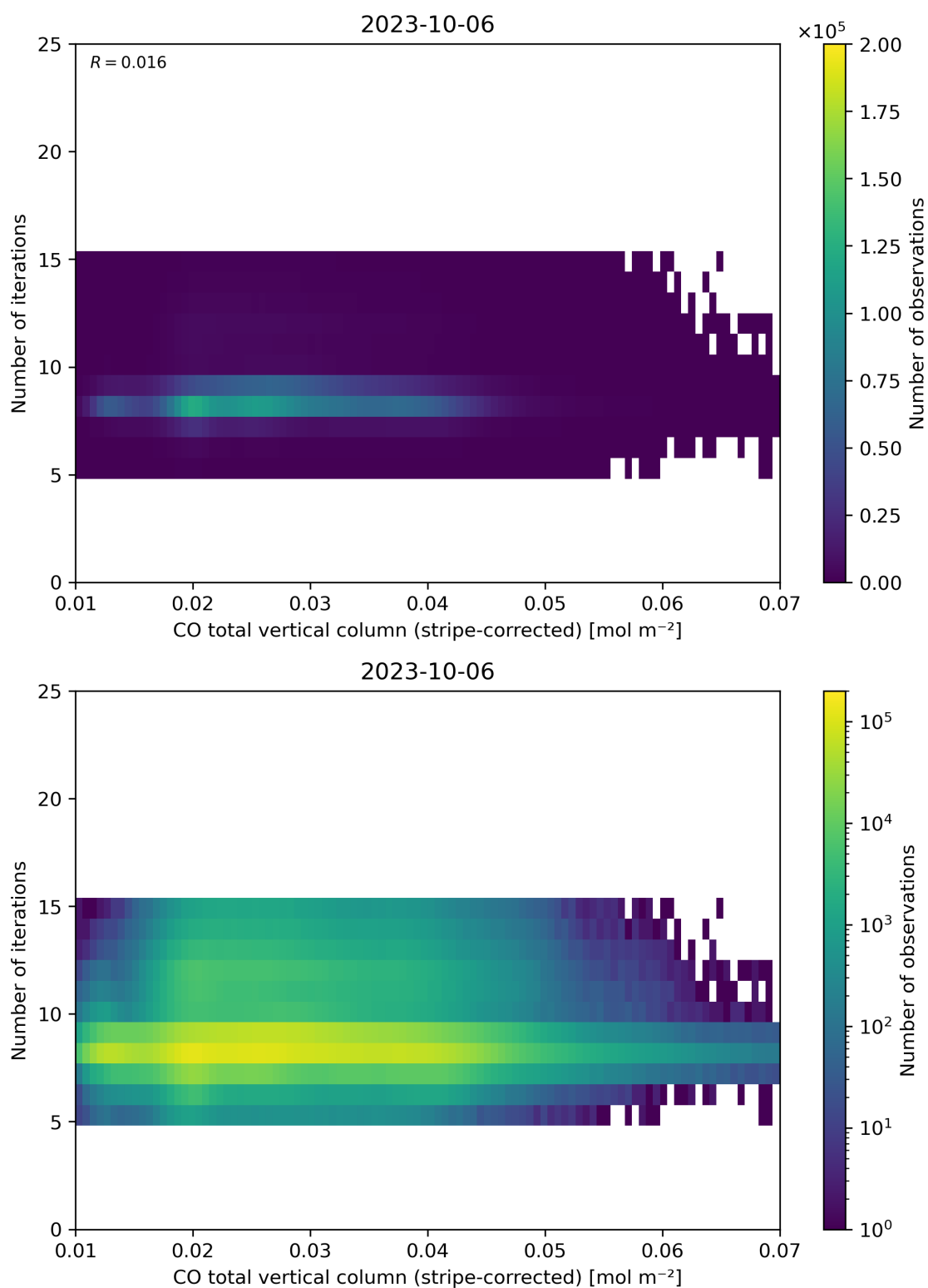
Figure 39: Scatter density plot of “CO total vertical column (stripe-corrected)” against “Number of iterations” for 2023-10-06 to 2023-10-07.
