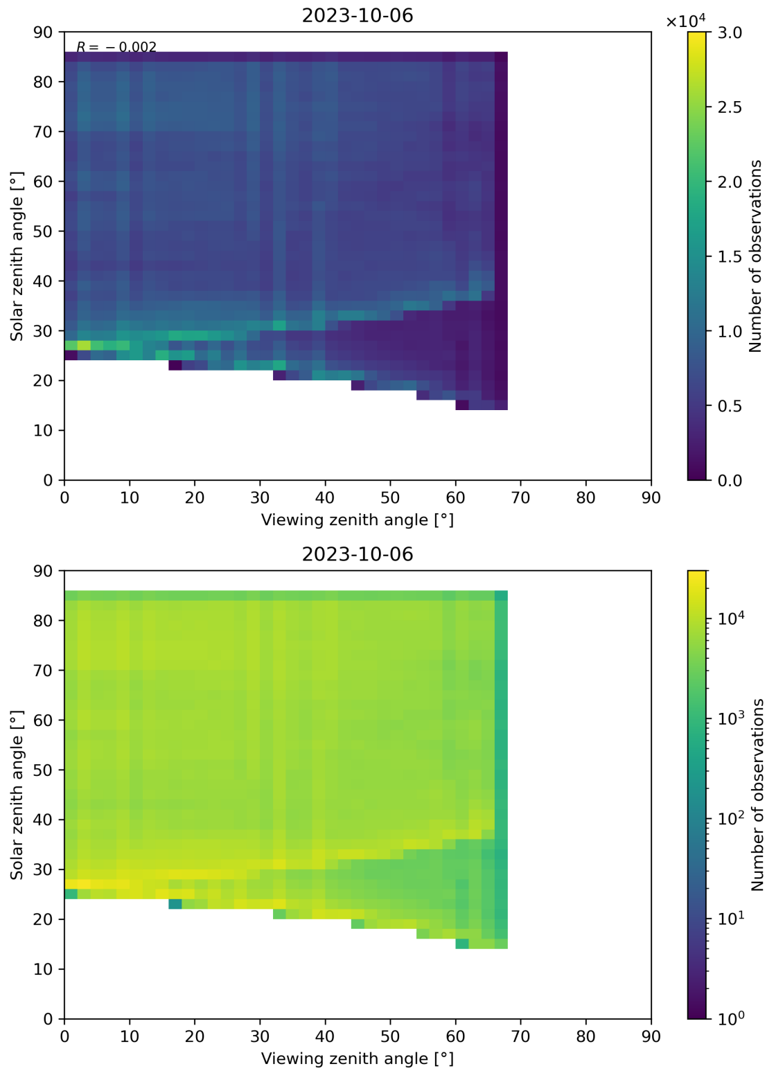
Figure 77: Scatter density plot of “Viewing zenith angle” against “Solar zenith angle” for 2023-10-06 to 2023-10-07.
