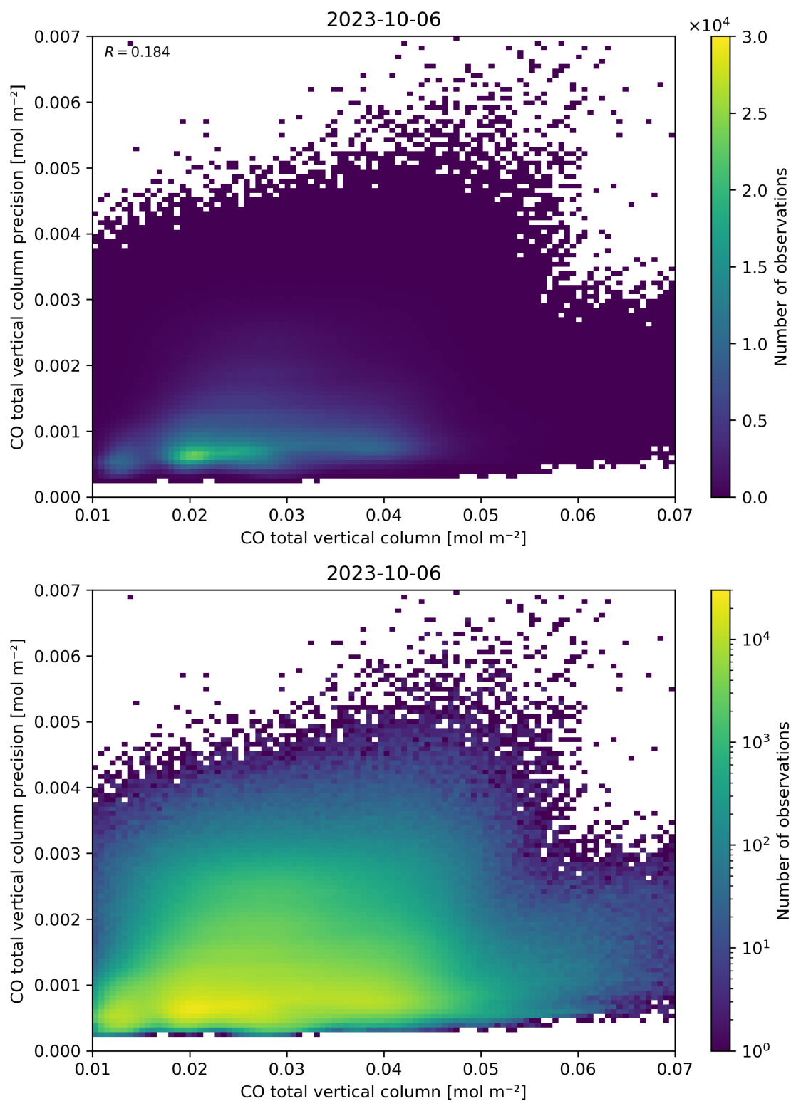
Figure 34: Scatter density plot of “CO total vertical column” against “CO total vertical column precision” for 2023-10-06 to 2023-10-07.
