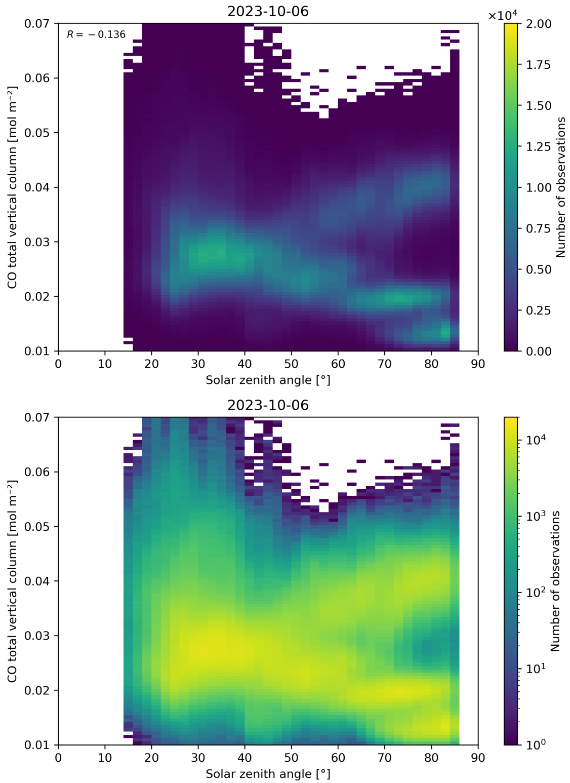
Figure 61: Scatter density plot of “Solar zenith angle” against “CO total vertical column” for 2023-10-06 to 2023-10-07.
