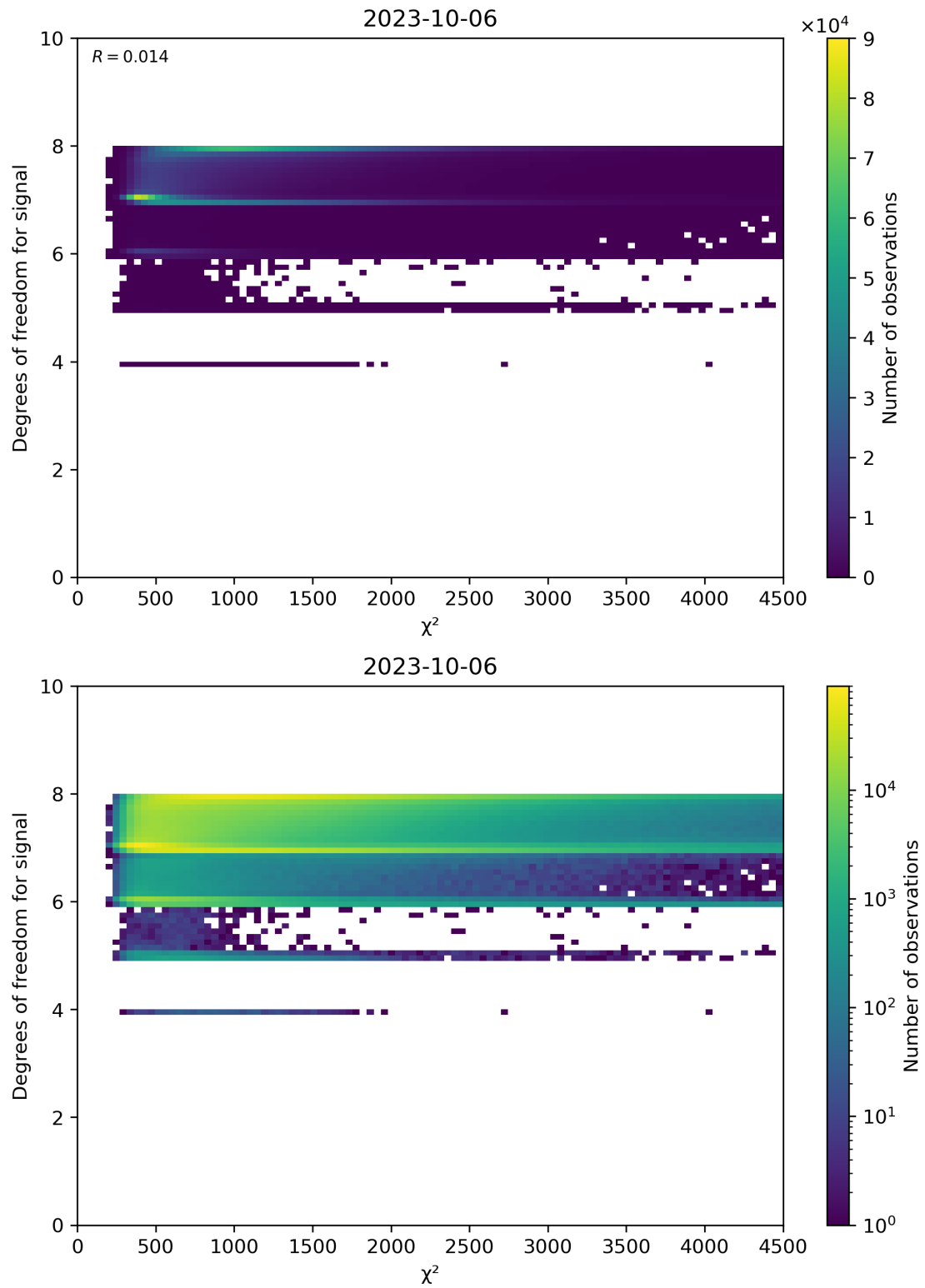
Figure 48: Scatter density plot of “ \chi^2 ” against “Degrees of freedom for signal” for 2023-10-06 to 2023-10-07.
