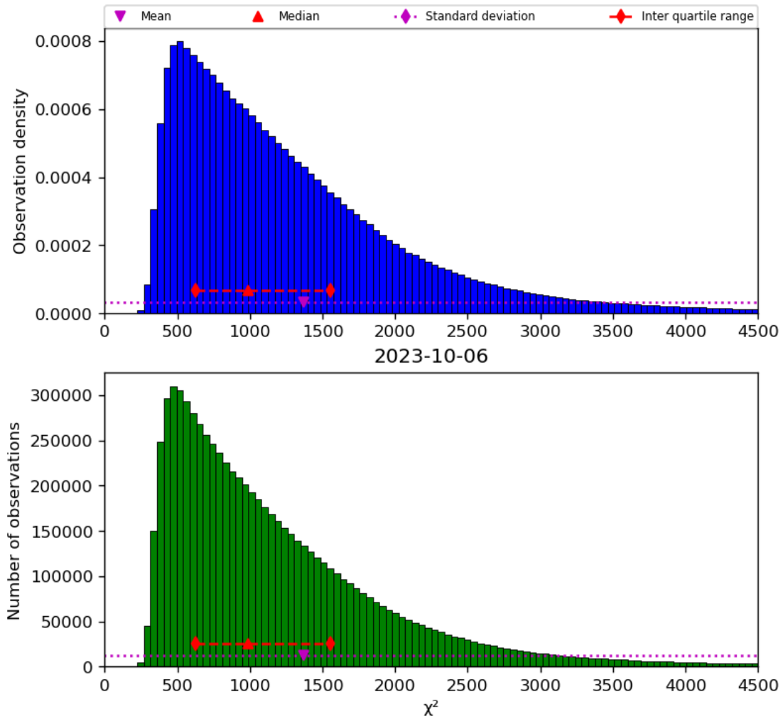
Figure 22: Histogram of " \chi^2 " for 2023-10-06 to 2023-10-07
