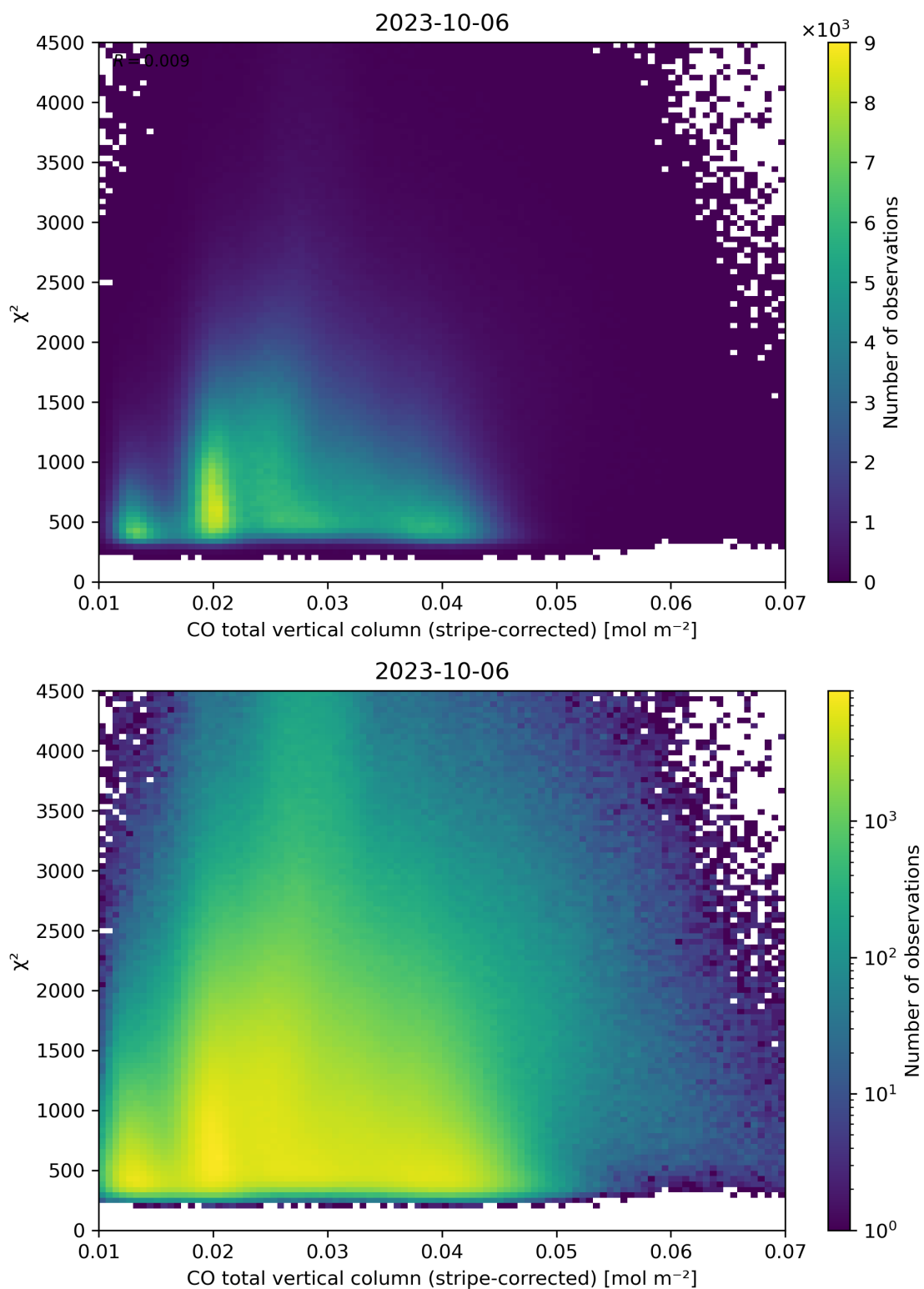
Figure 37: Scatter density plot of “CO total vertical column (stripe-corrected)” against “ \chi^2 ” for 2023-10-06 to 2023-10-07.
