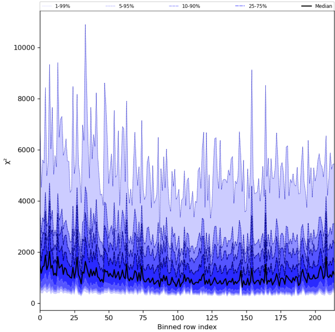
Figure 30: Along track statistics of “ \chi^2 ” for 2023-10-06 to 2023-10-07
