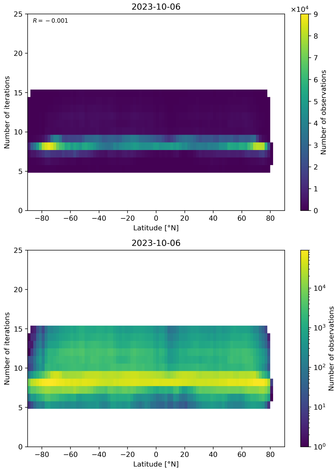
Figure 56: Scatter density plot of “Latitude” against “Number of iterations” for 2023-10-06 to 2023-10-07.
