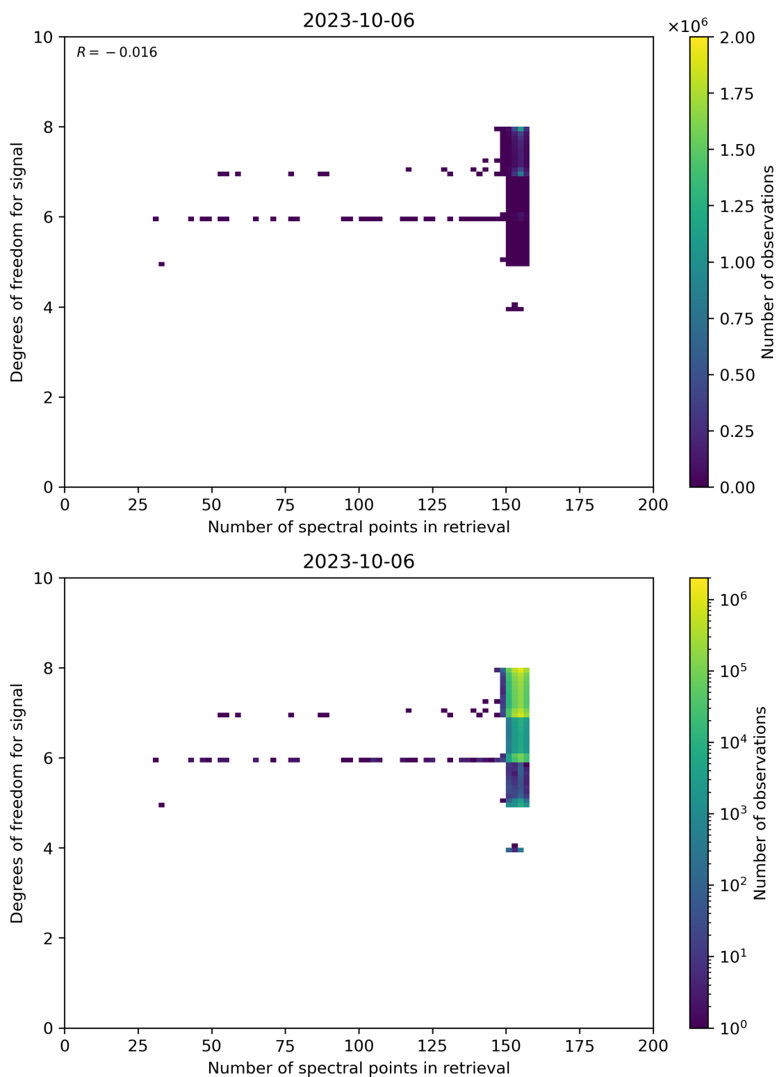
Figure 59: Scatter density plot of “Number of spectral points in retrieval” against “Degrees of freedom for signal” for 2023-10-06 to 2023-10-07.
