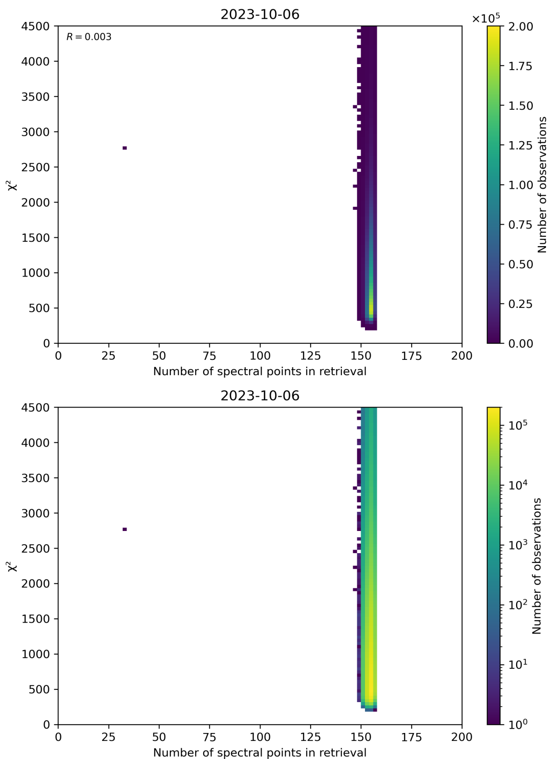
Figure 58: Scatter density plot of “Number of spectral points in retrieval” against “ \chi^2 ” for 2023-10-06 to 2023-10-07.
