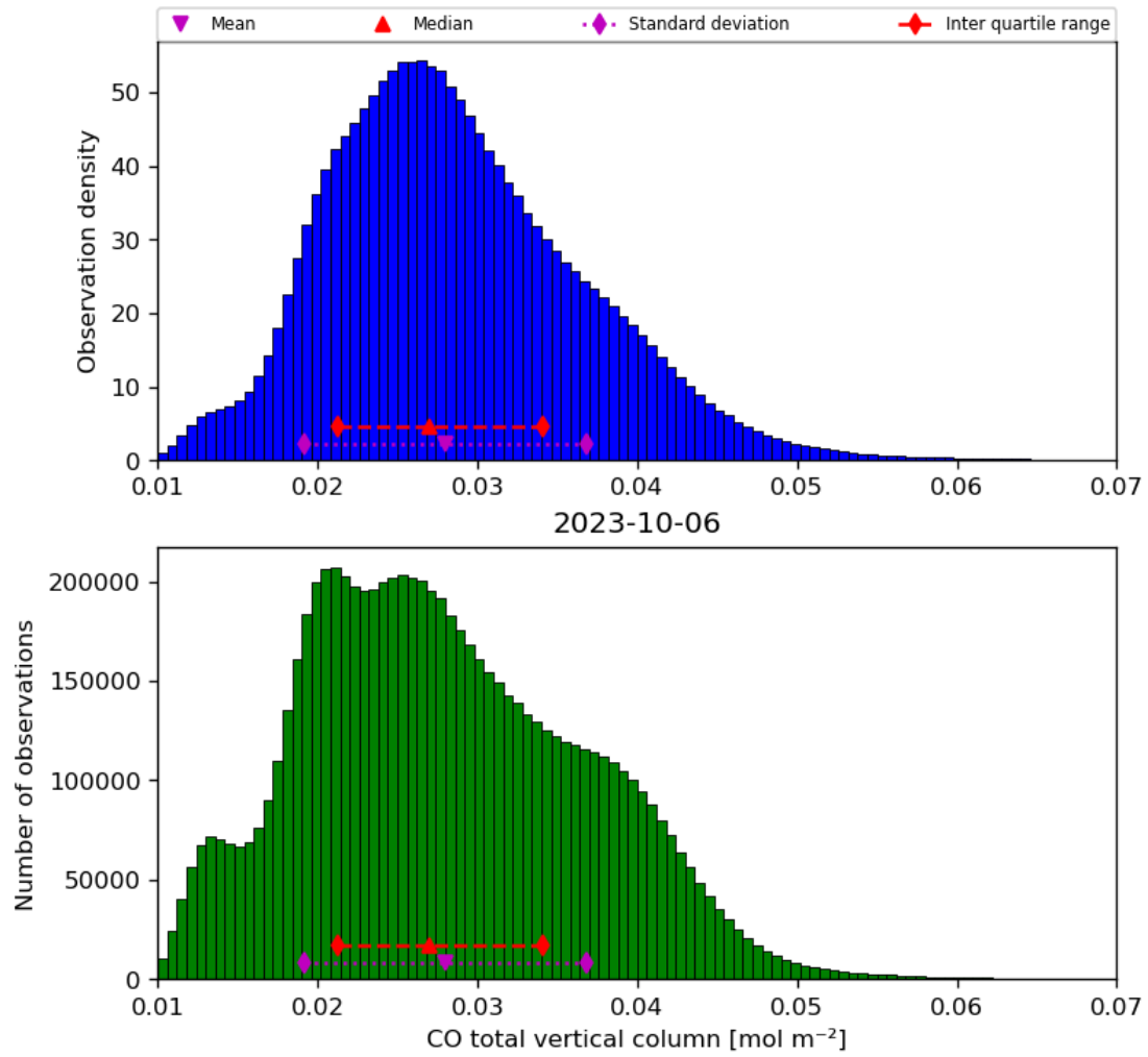
Figure 18: Histogram of “CO total vertical column” for 2023-10-06 to 2023-10-07
