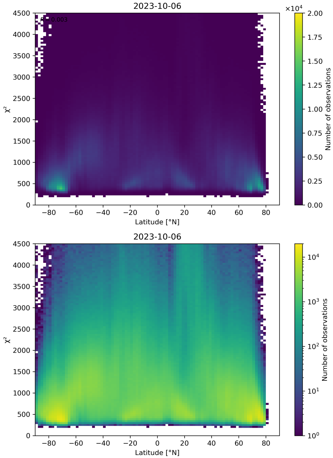
Figure 54: Scatter density plot of “Latitude” against “ \chi^2 ” for 2023-10-06 to 2023-10-07.
