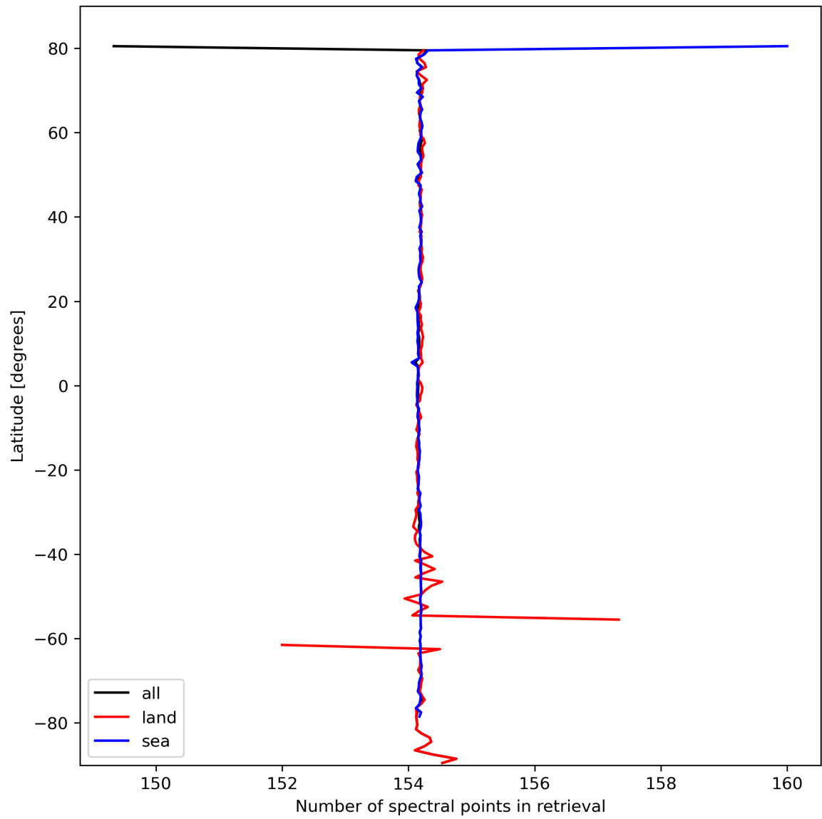
Figure 13: Zonal average of “Number of spectral points in retrieval” for 2023-10-06 to 2023-10-07.
