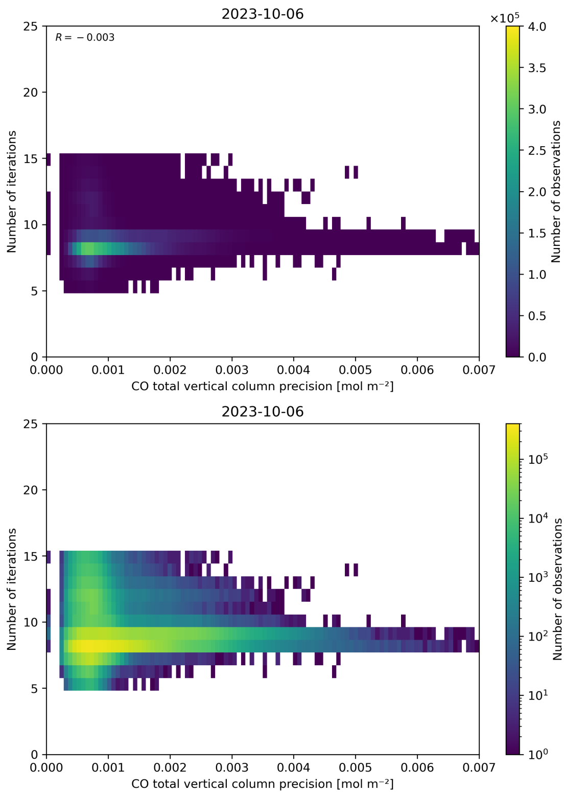
Figure 46: Scatter density plot of “CO total vertical column precision” against “Number of iterations” for 2023-10-06 to 2023-10-07.
