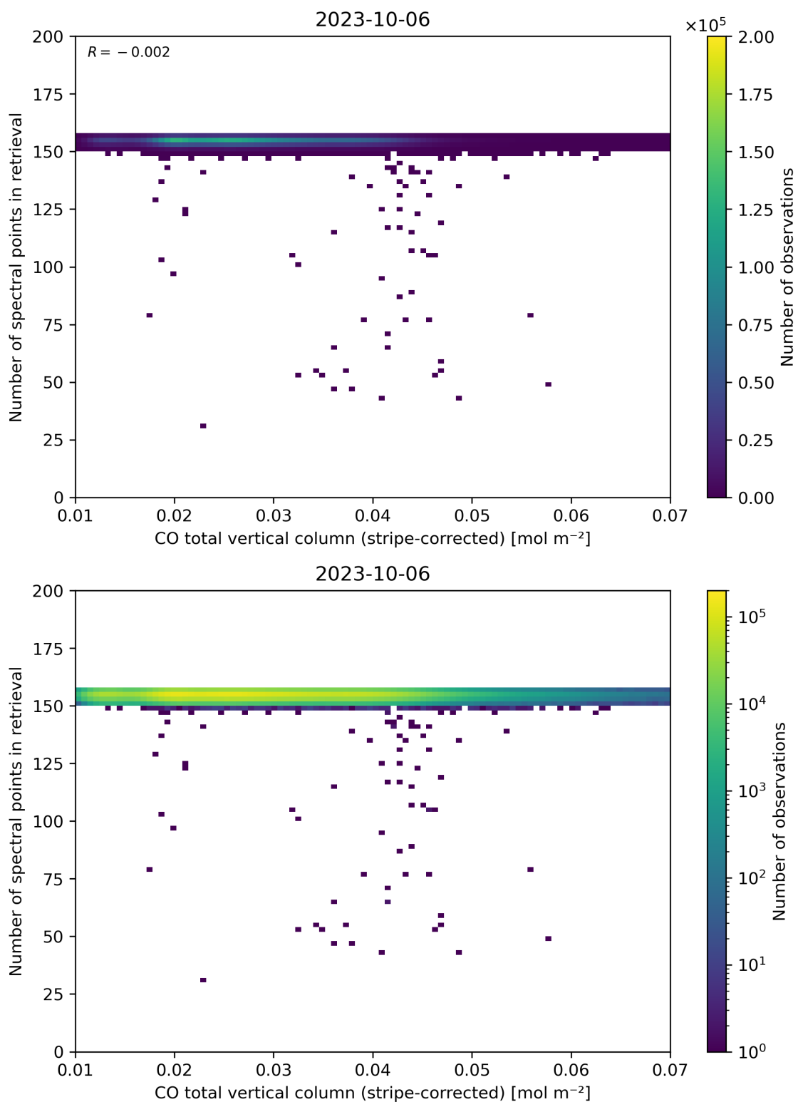
Figure 40: Scatter density plot of “CO total vertical column (stripe-corrected)” against “Number of spectral points in retrieval” for 2023-10-06 to 2023-10-07.
