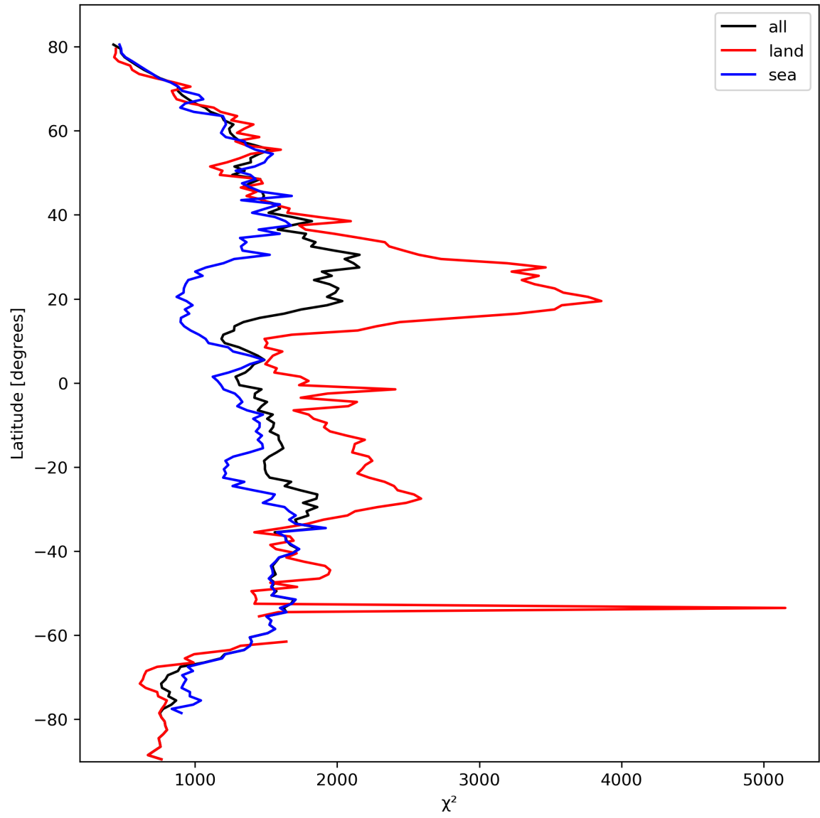
Figure 14: Zonal average of “ \chi^2 ” for 2023-10-06 to 2023-10-07.
