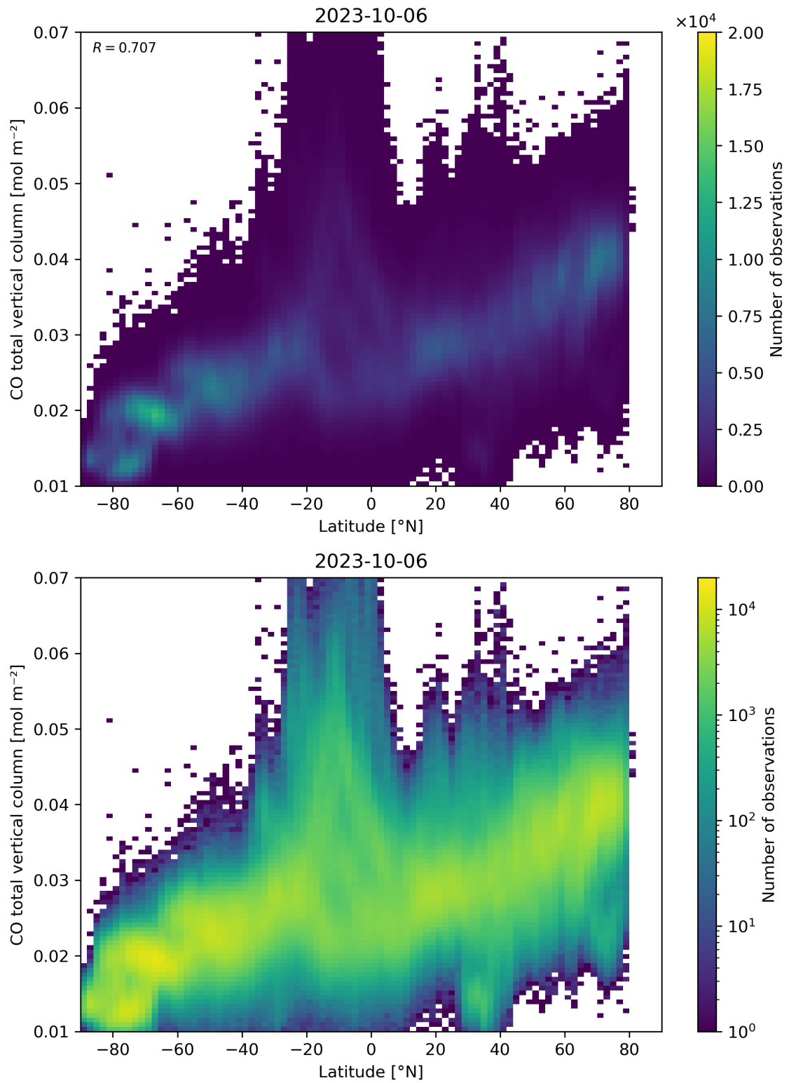
Figure 51: Scatter density plot of “Latitude” against “CO total vertical column” for 2023-10-06 to 2023-10-07.
