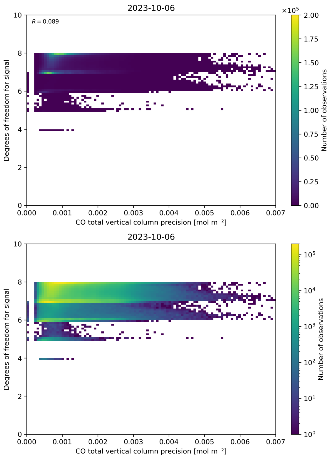
Figure 45: Scatter density plot of “CO total vertical column precision” against “Degrees of freedom for signal” for 2023-10-06 to 2023-10-07.
