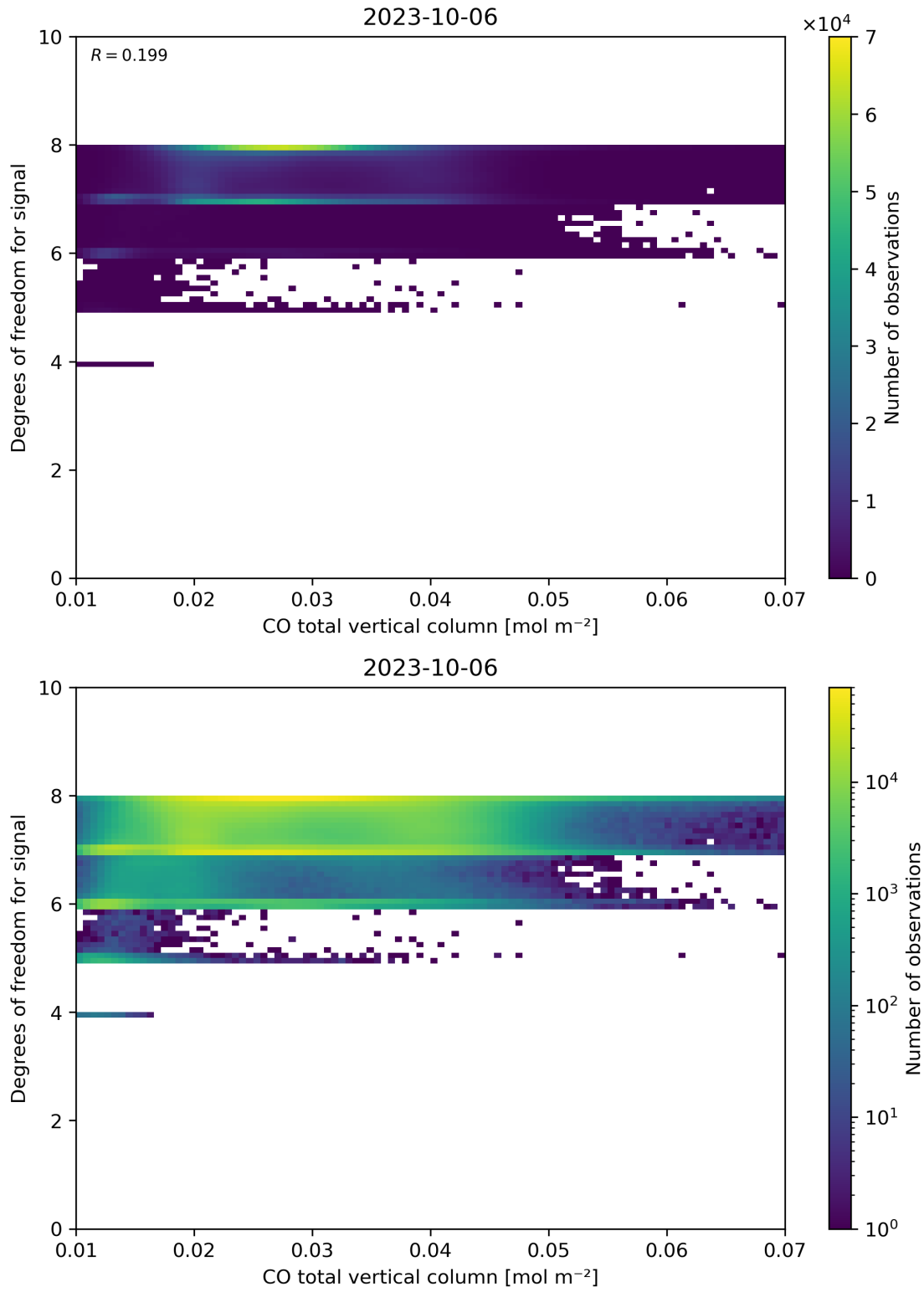
Figure 41: Scatter density plot of “CO total vertical column” against “Degrees of freedom for signal” for 2023-10-06 to 2023-10-07.
