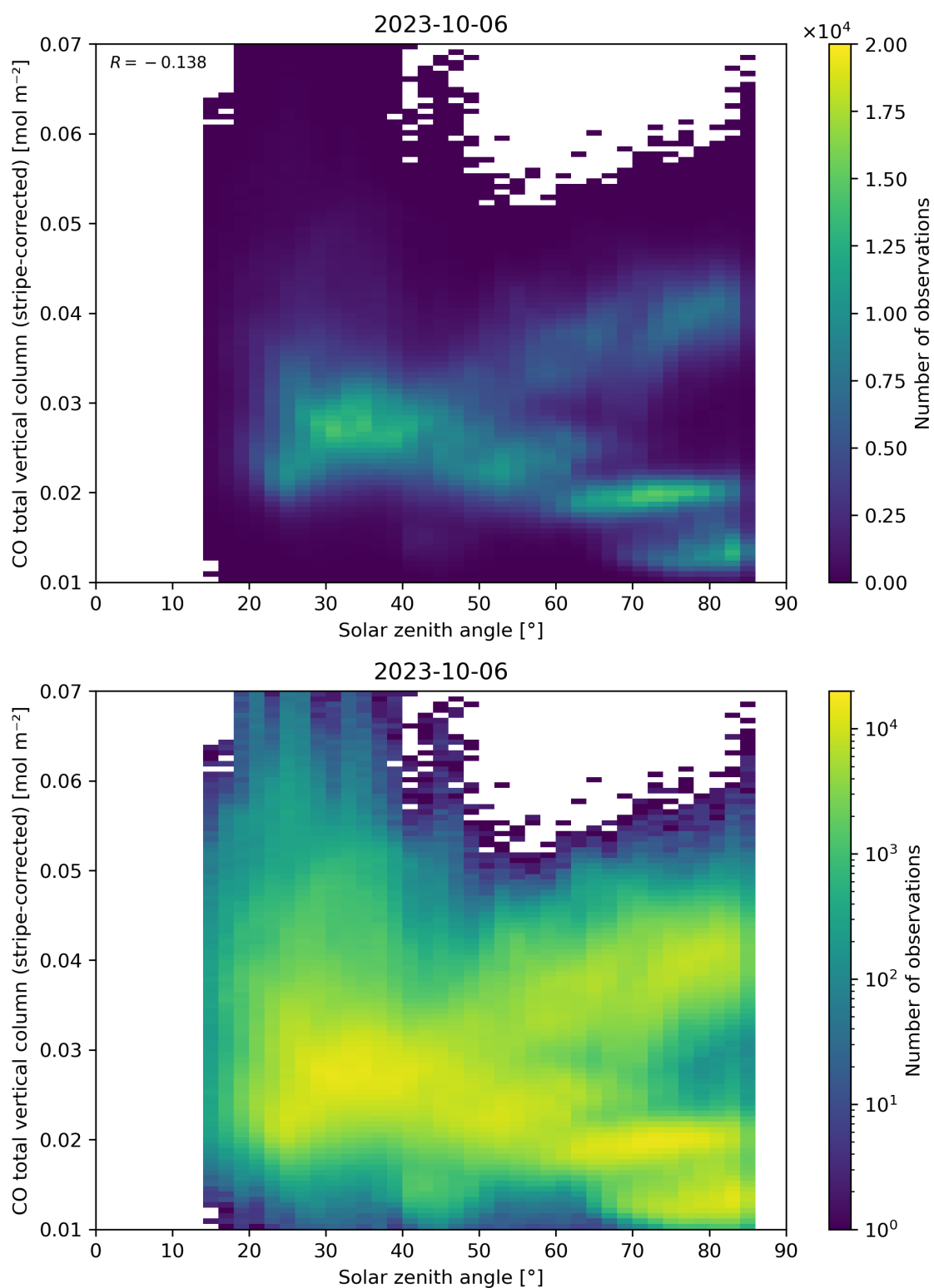
Figure 62: Scatter density plot of “Solar zenith angle” against “CO total vertical column (stripe-corrected)” for 2023-10-06 to 2023-10-07.
