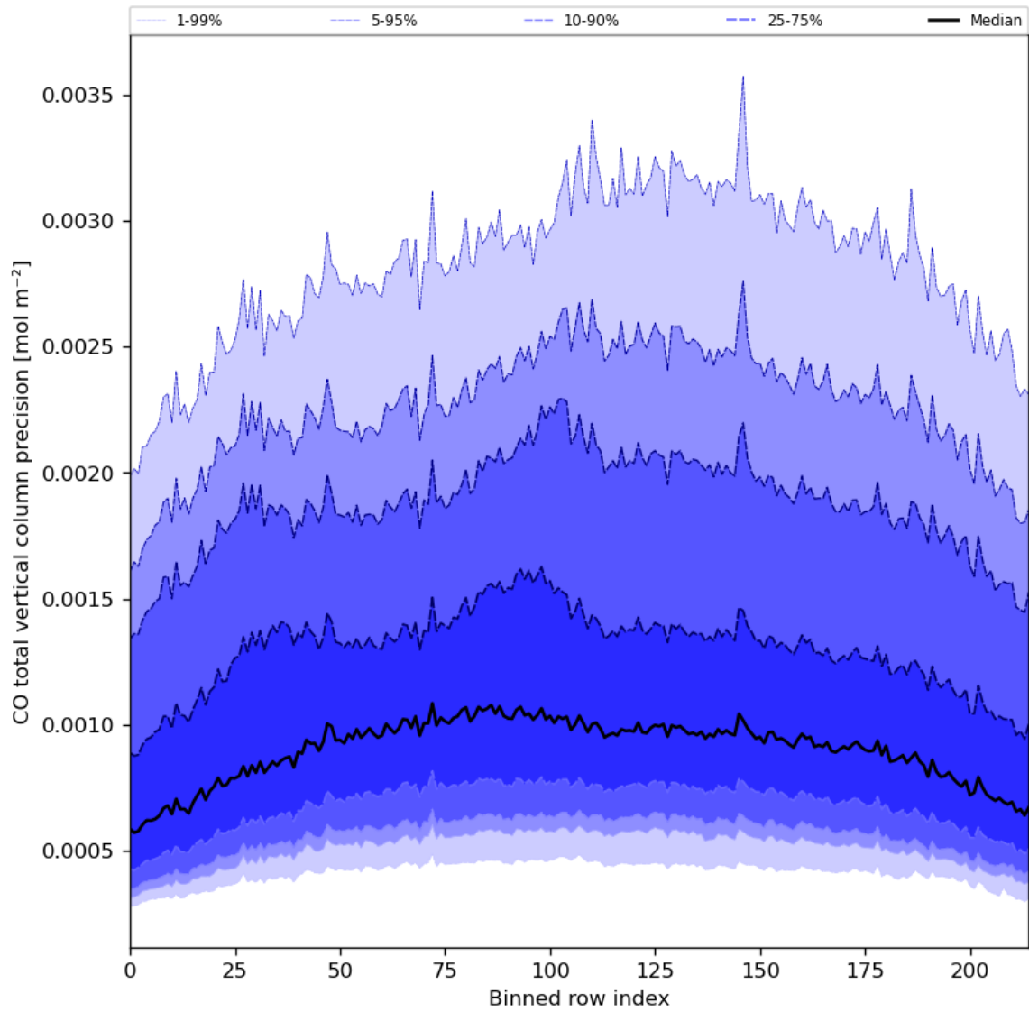
Figure 28: Along track statistics of “CO total vertical column precision” for 2023-10-06 to 2023-10-07
