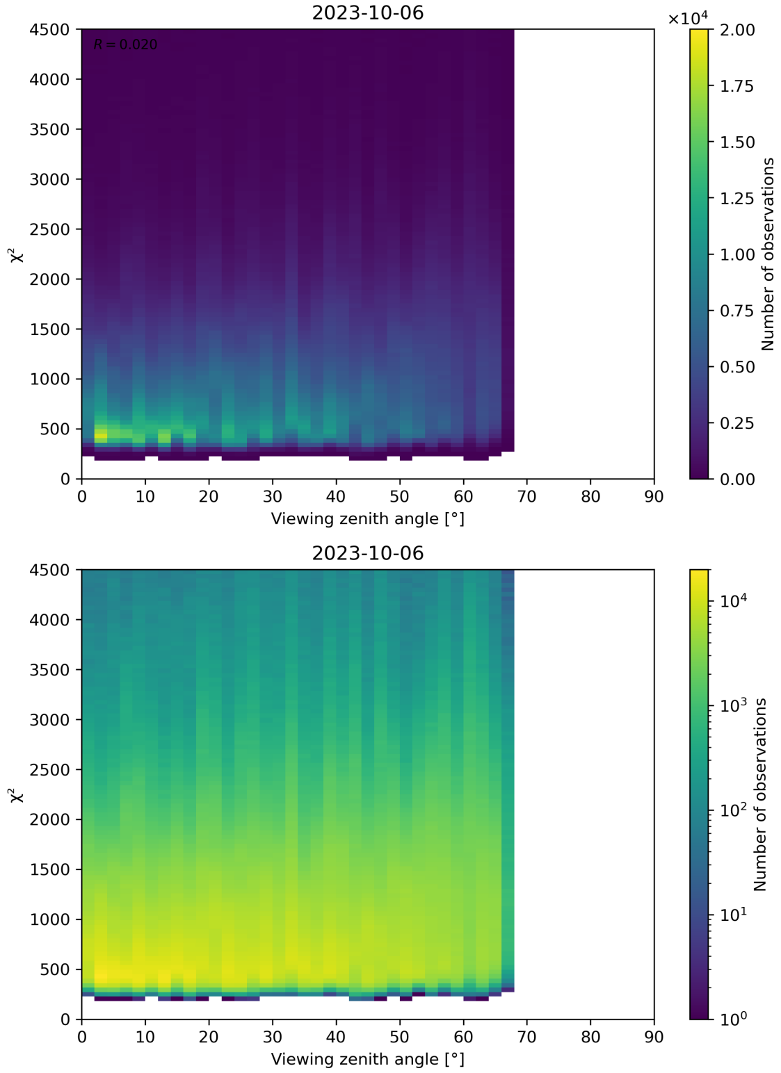
Figure 72: Scatter density plot of “Viewing zenith angle” against “ \chi^2 ” for 2023-10-06 to 2023-10-07.
