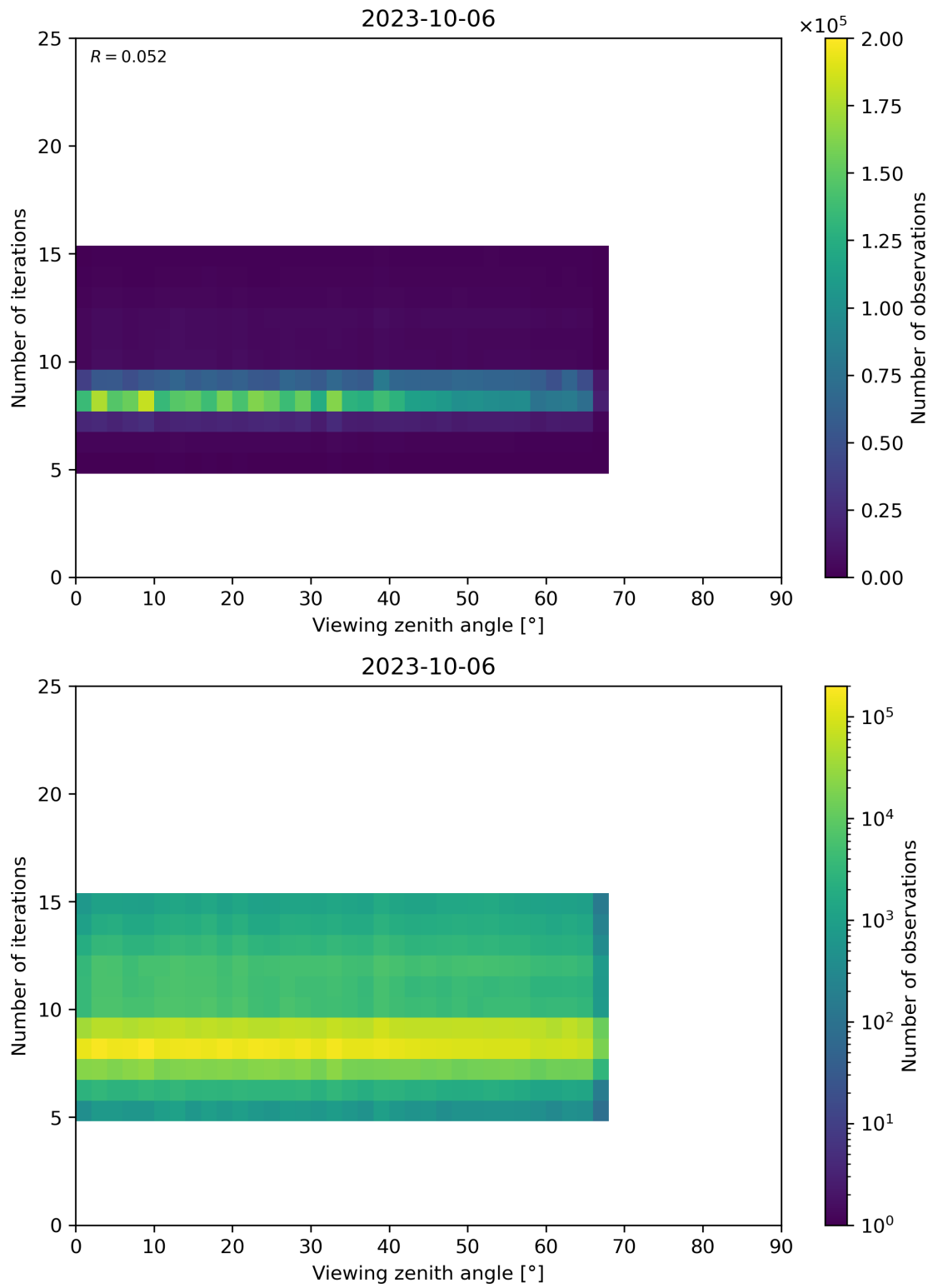
Figure 75: Scatter density plot of “Viewing zenith angle” against “Number of iterations” for 2023-10-06 to 2023-10-07.
