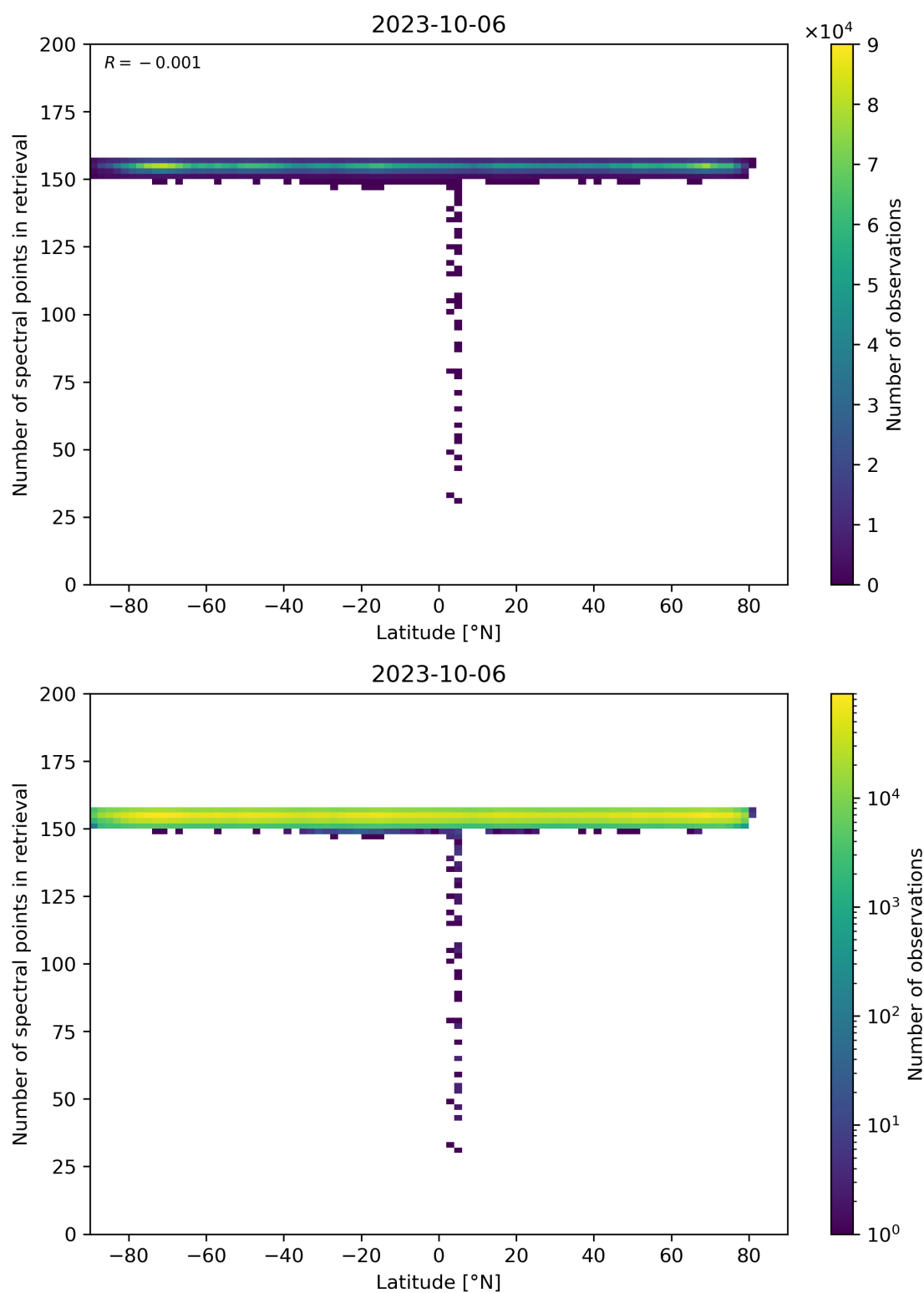
Figure 57: Scatter density plot of “Latitude” against “Number of spectral points in retrieval” for 2023-10-06 to 2023-10-07.
