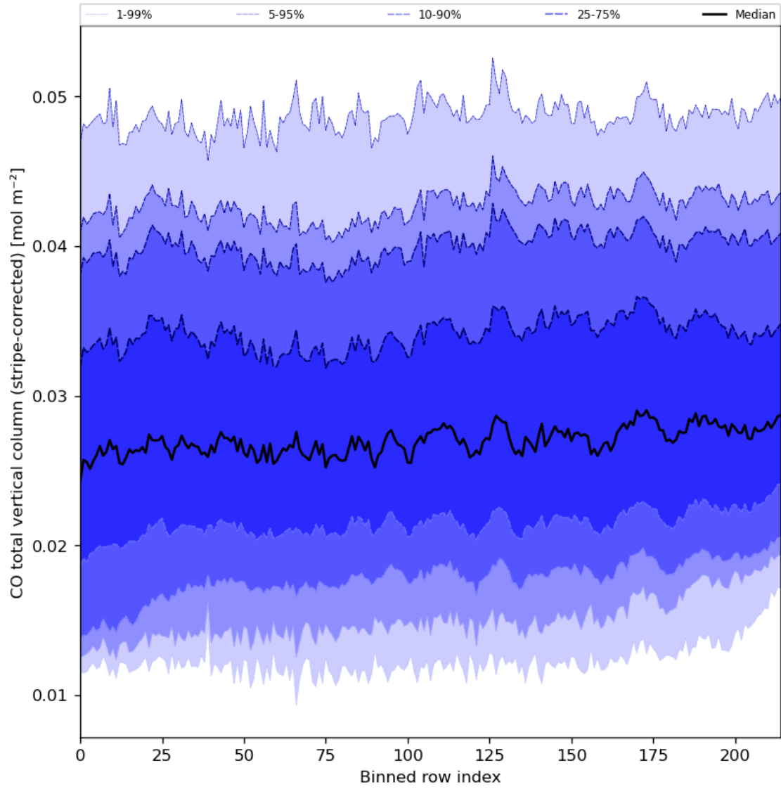
Figure 27: Along track statistics of “CO total vertical column (stripe-corrected)” for 2023-10-06 to 2023-10-07
