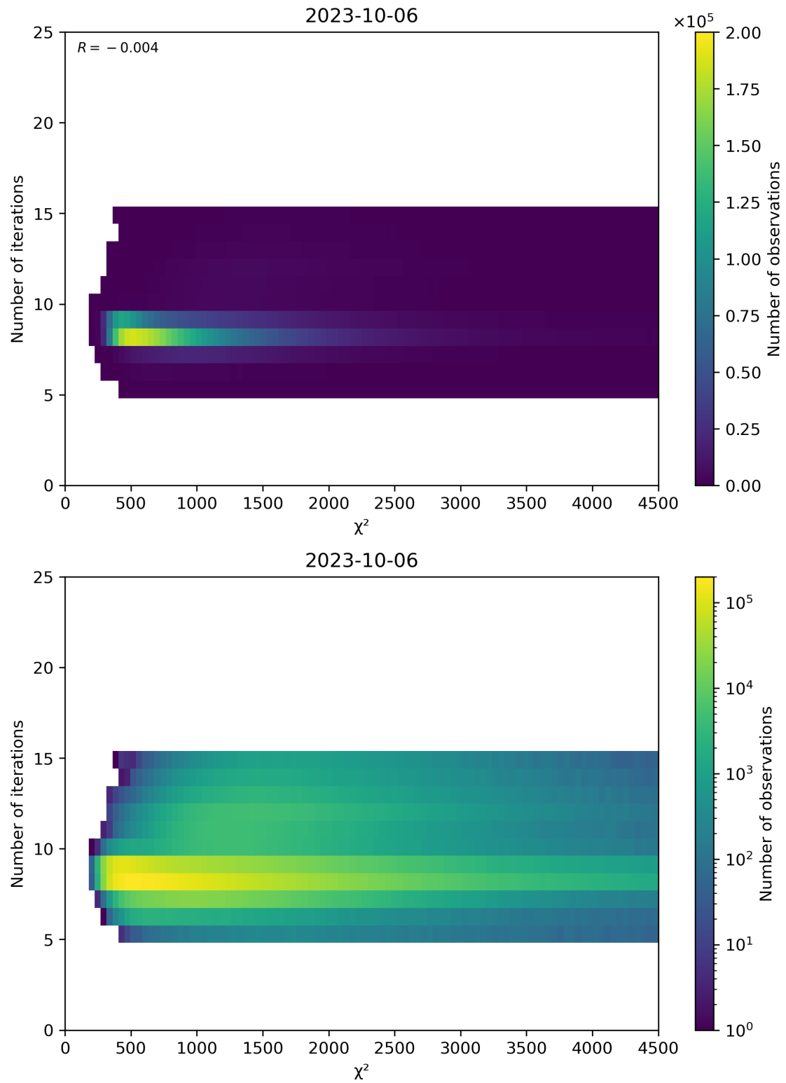
Figure 49: Scatter density plot of “ \chi^2 ” against “Number of iterations” for 2023-10-06 to 2023-10-07.
