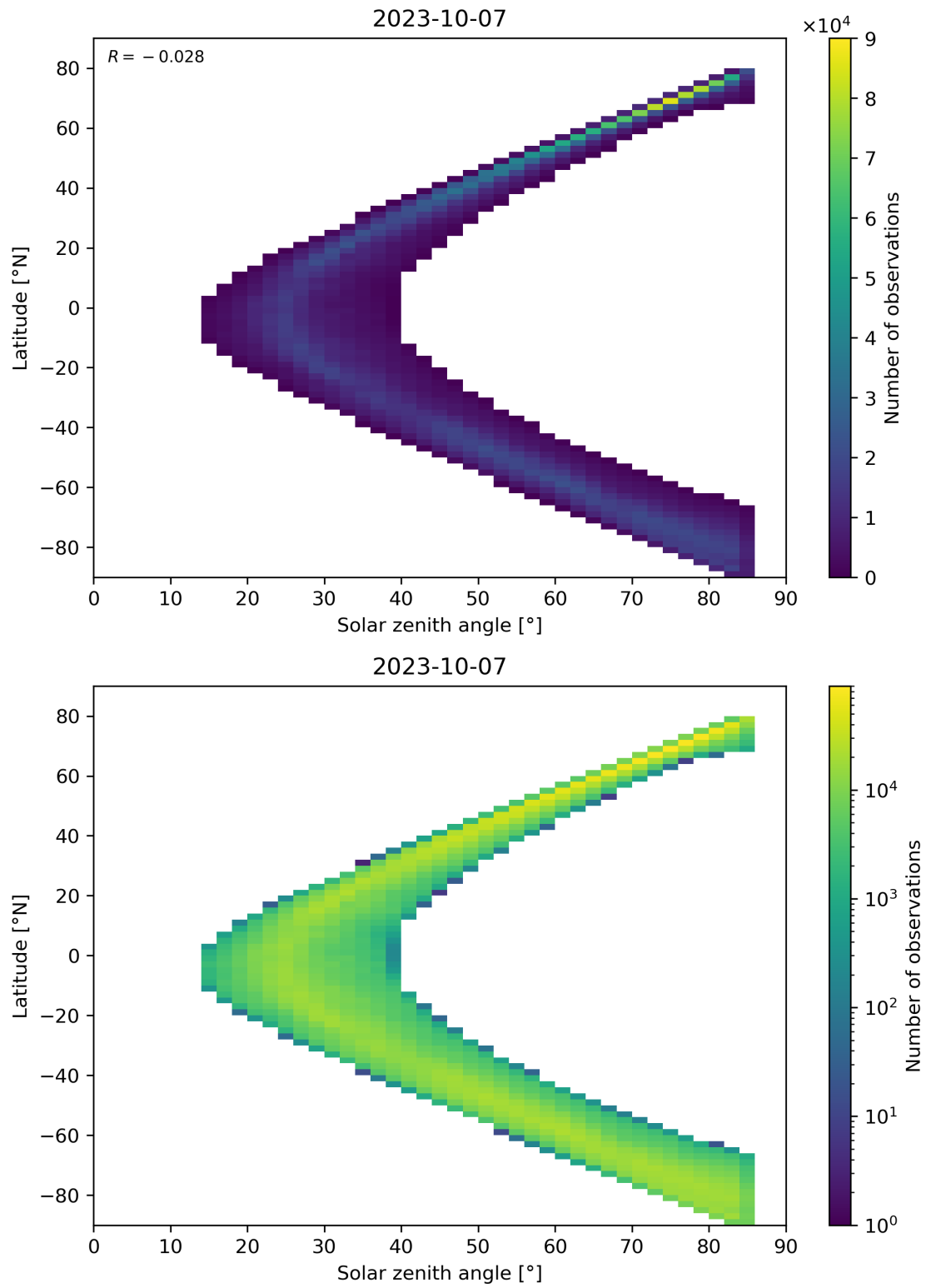
Figure 66: Scatter density plot of “Solar zenith angle” against “Latitude” for 2023-10-06 to 2023-10-08.
