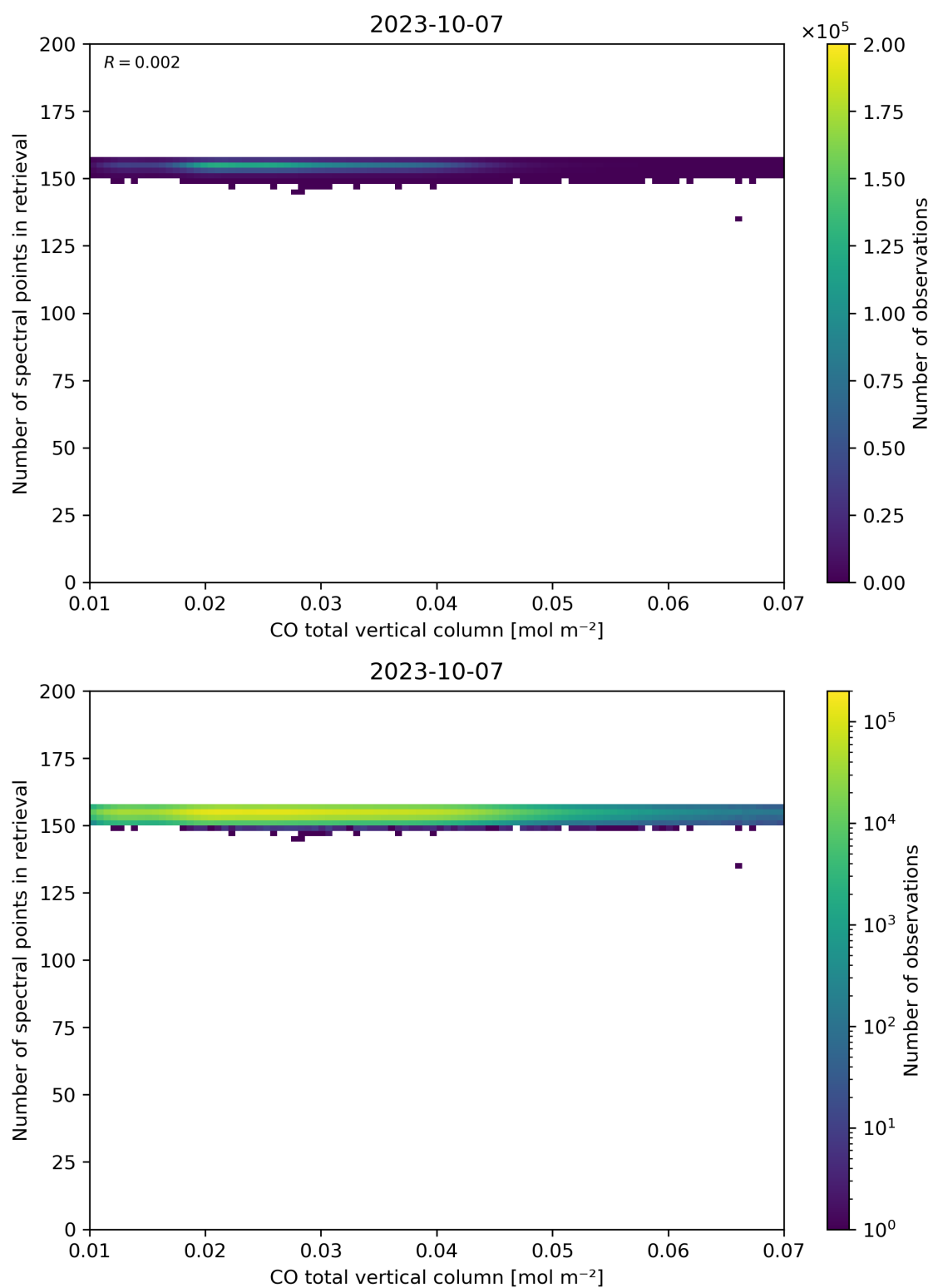
Figure 43: Scatter density plot of “CO total vertical column” against “Number of spectral points in retrieval” for 2023-10-06 to 2023-10-08.
