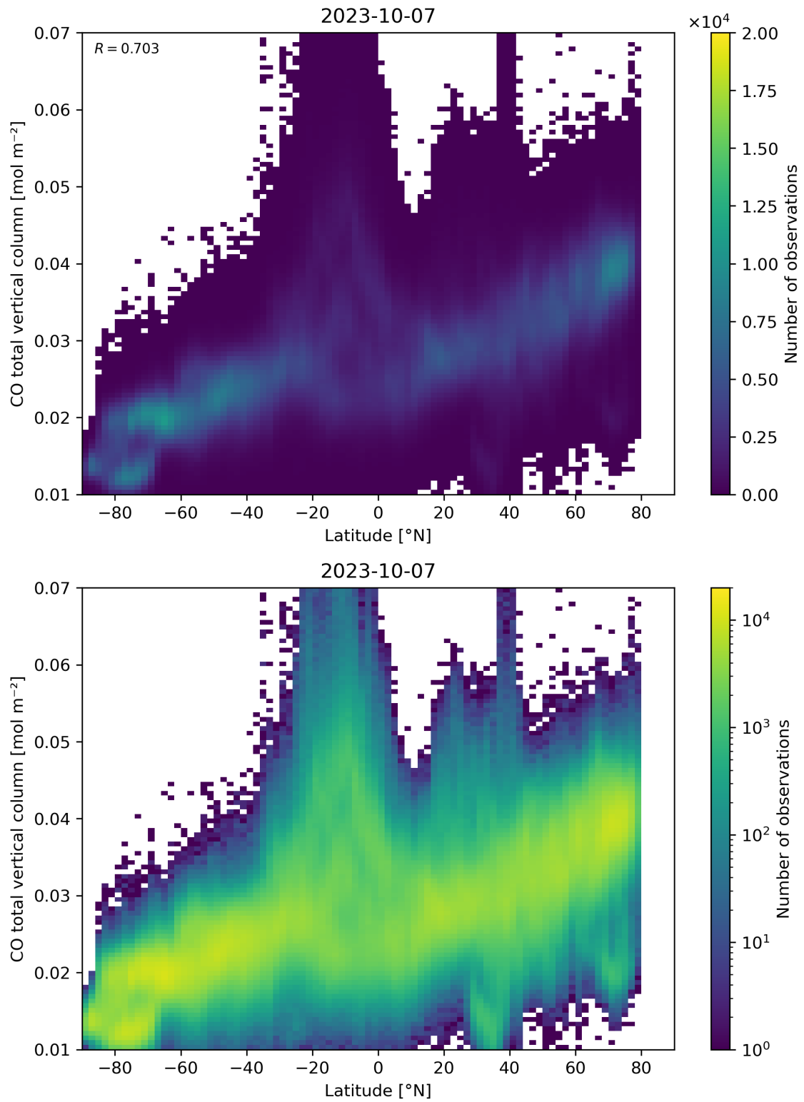
Figure 51: Scatter density plot of “Latitude” against “CO total vertical column” for 2023-10-06 to 2023-10-08.
