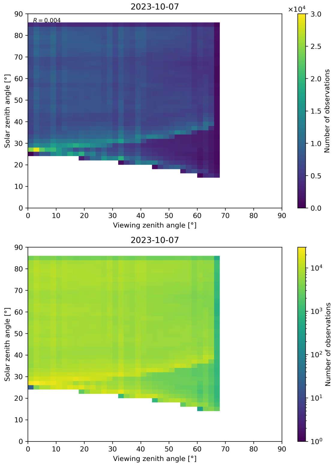
Figure 77: Scatter density plot of “Viewing zenith angle” against “Solar zenith angle” for 2023-10-06 to 2023-10-08.
