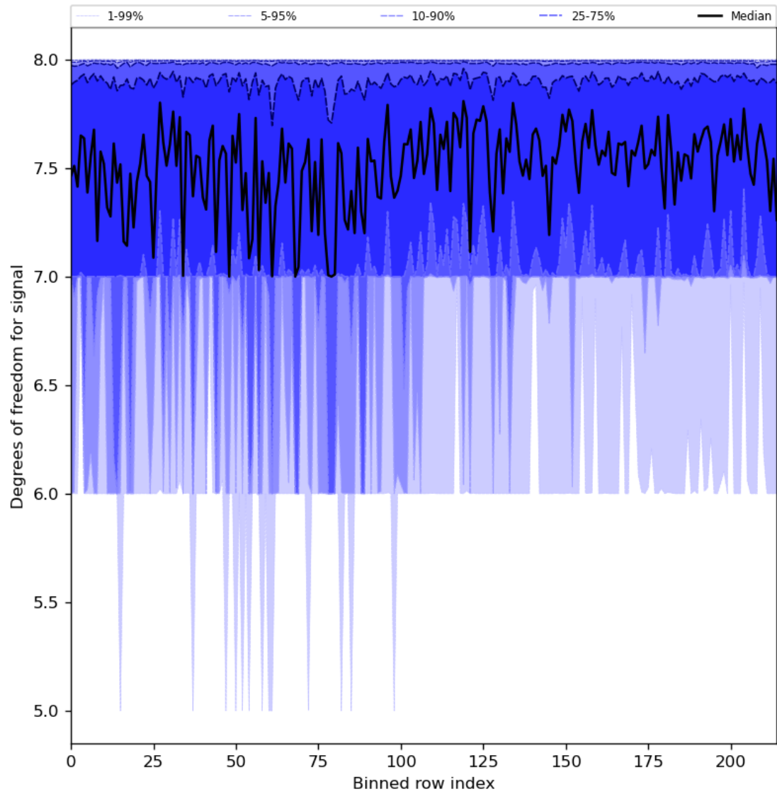
Figure 31: Along track statistics of “Degrees of freedom for signal” for 2023-10-06 to 2023-10-08
