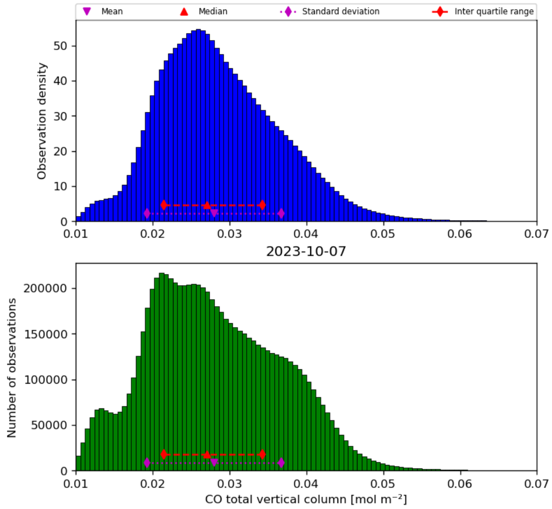
Figure 18: Histogram of “CO total vertical column” for 2023-10-06 to 2023-10-08
