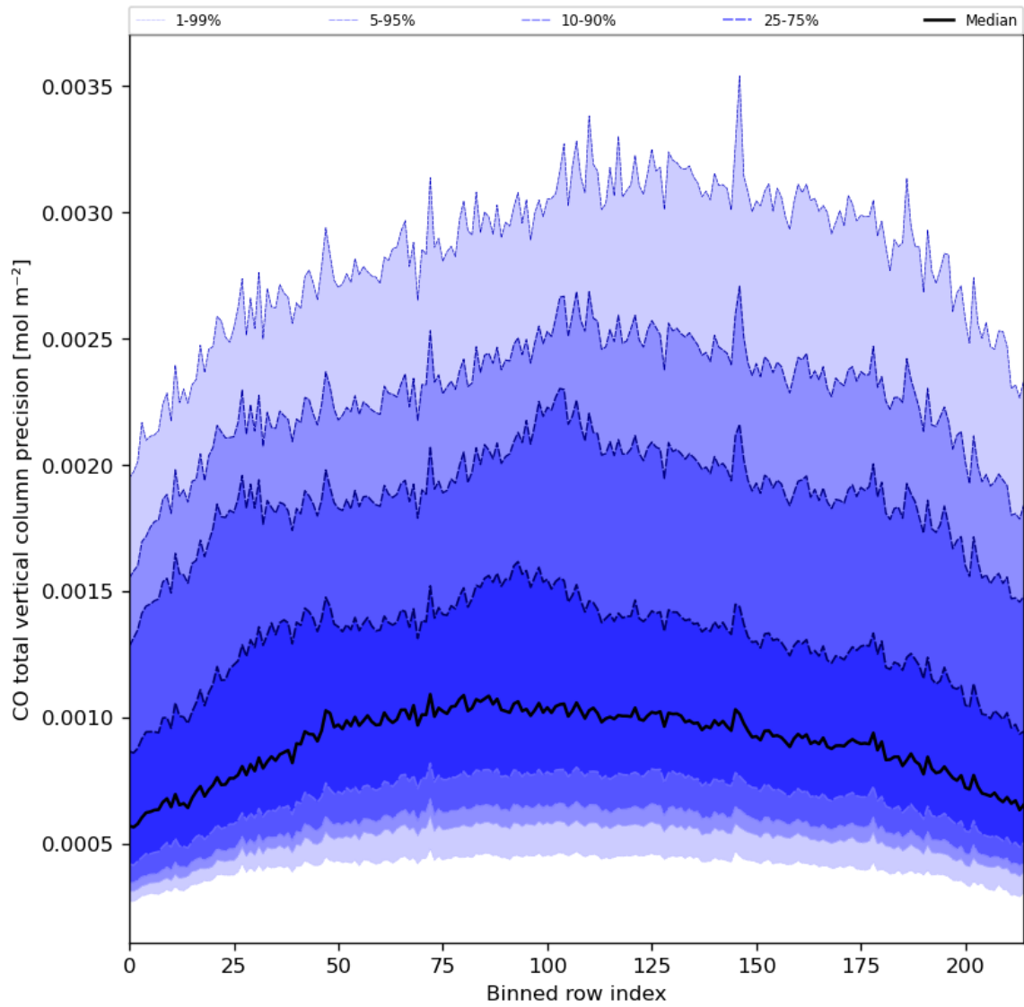
Figure 28: Along track statistics of “CO total vertical column precision” for 2023-10-06 to 2023-10-08
