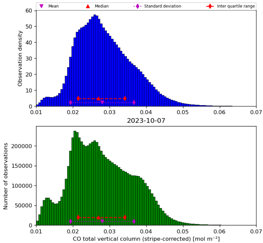
Figure 19: Histogram of “CO total vertical column (stripe-corrected)” for 2023-10-06 to 2023-10-08
