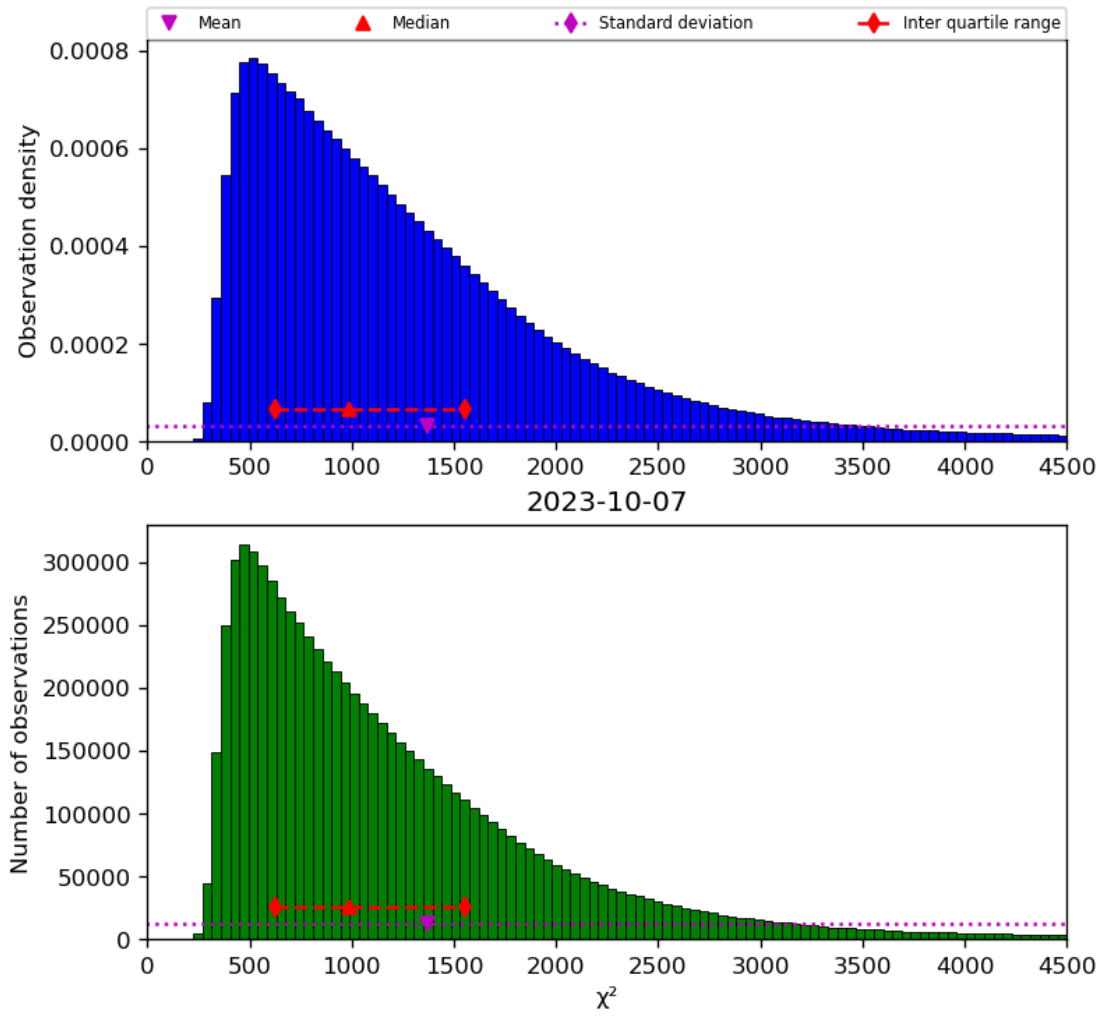
Figure 22: Histogram of “ \chi^2 ” for 2023-10-06 to 2023-10-08
