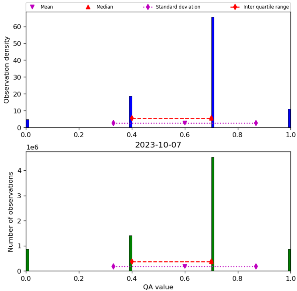
Figure 17: Histogram of “QA value” for 2023-10-06 to 2023-10-08
