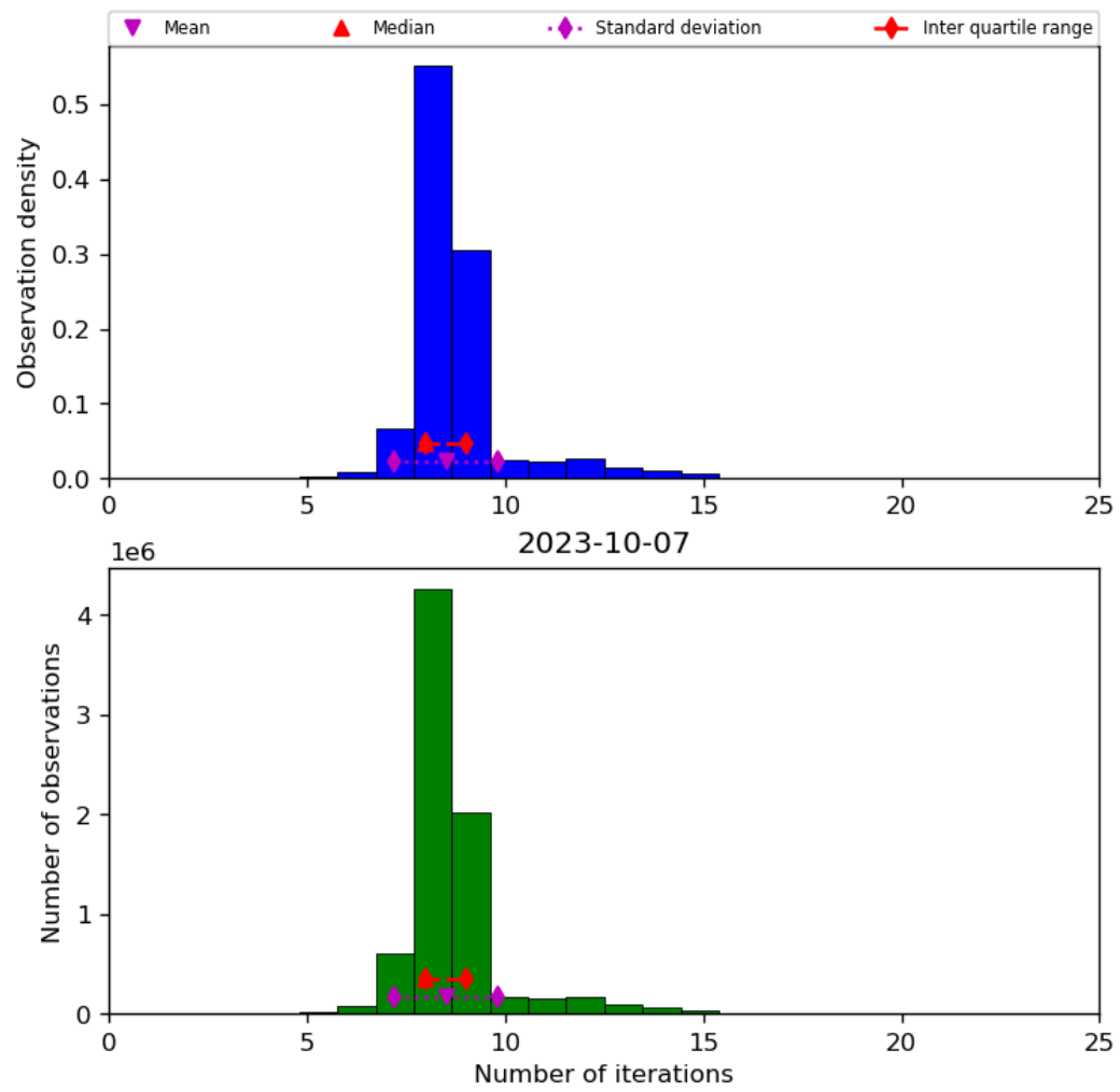
Figure 24: Histogram of “Number of iterations” for 2023-10-06 to 2023-10-08
