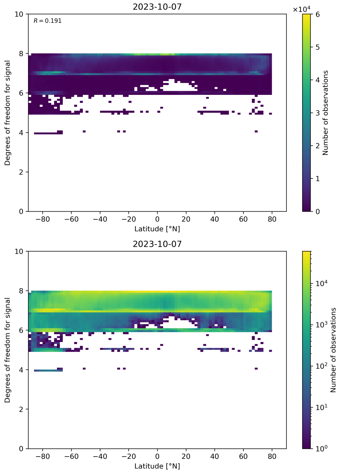
Figure 55: Scatter density plot of “Latitude” against “Degrees of freedom for signal” for 2023-10-06 to 2023-10-08.
