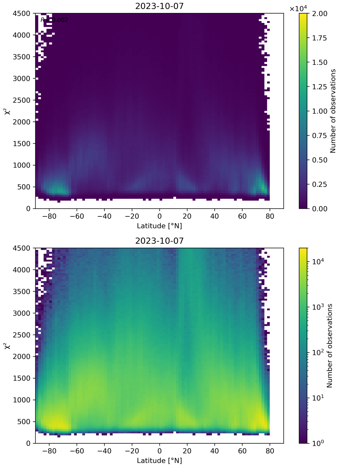
Figure 54: Scatter density plot of “Latitude” against “ \chi^2 ” for 2023-10-06 to 2023-10-08.
