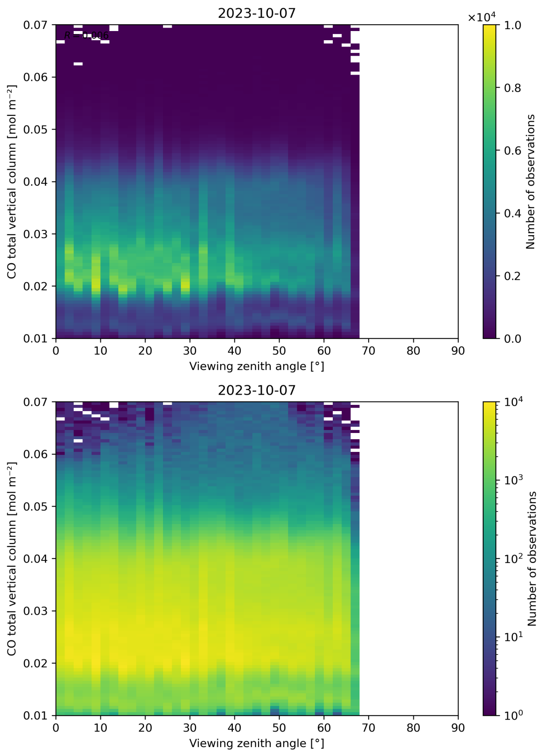
Figure 69: Scatter density plot of “Viewing zenith angle” against “CO total vertical column” for 2023-10-06 to 2023-10-08.
