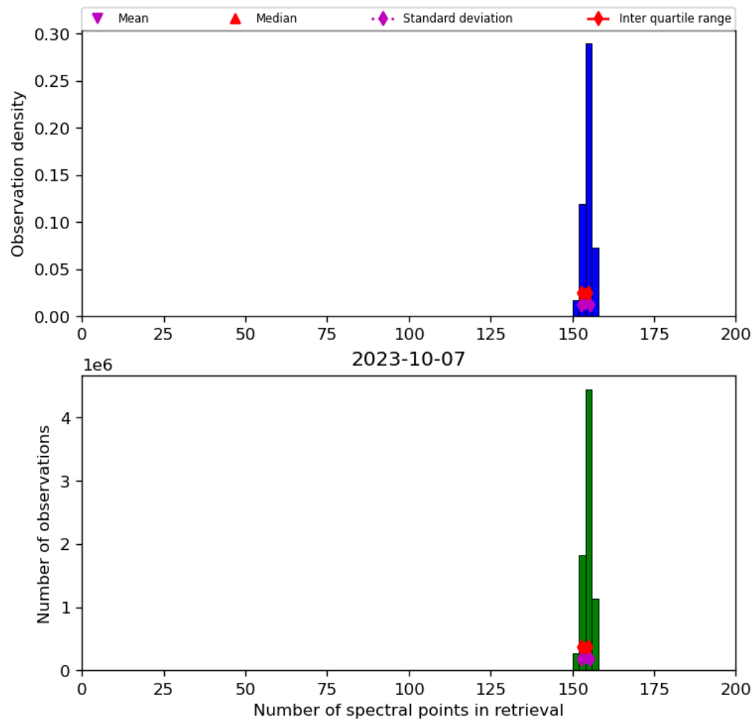
Figure 21: Histogram of “Number of spectral points in retrieval” for 2023-10-06 to 2023-10-08
