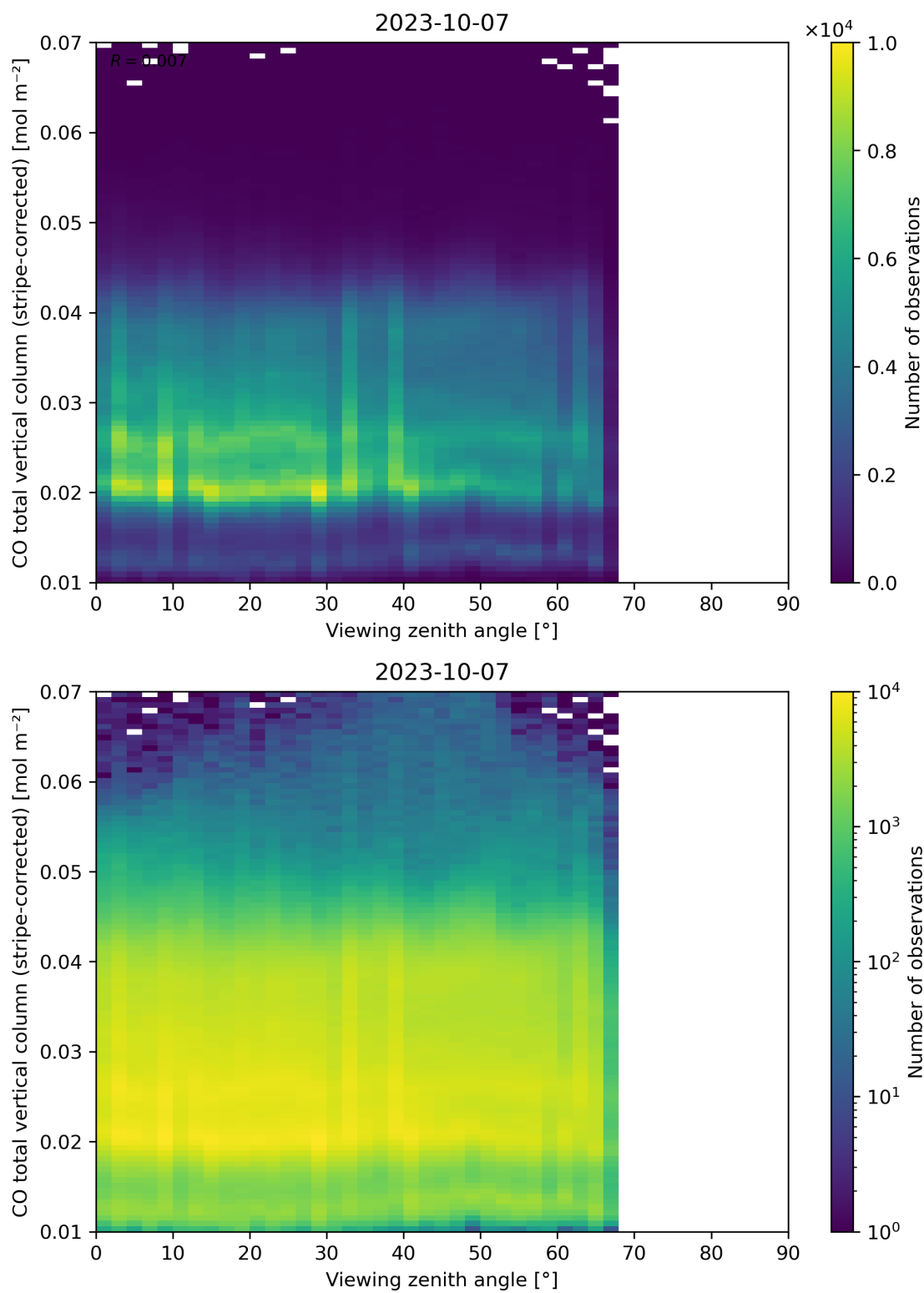
Figure 70: Scatter density plot of “Viewing zenith angle” against “CO total vertical column (stripe-corrected)” for 2023-10-06 to 2023-10-08.
