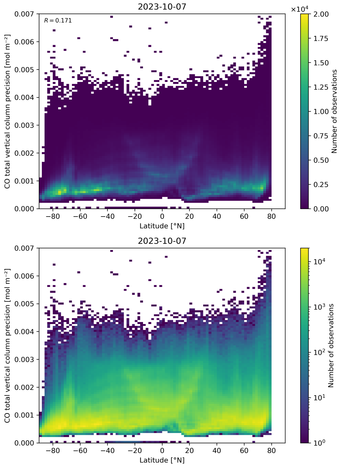
Figure 53: Scatter density plot of “Latitude” against “CO total vertical column precision” for 2023-10-06 to 2023-10-08.
