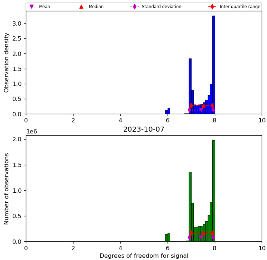
Figure 23: Histogram of “Degrees of freedom for signal” for 2023-10-06 to 2023-10-08
