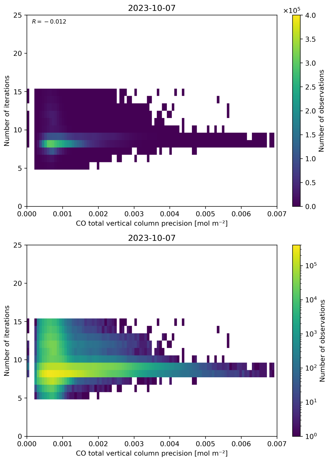
Figure 46: Scatter density plot of “CO total vertical column precision” against “Number of iterations” for 2023-10-06 to 2023-10-08.
