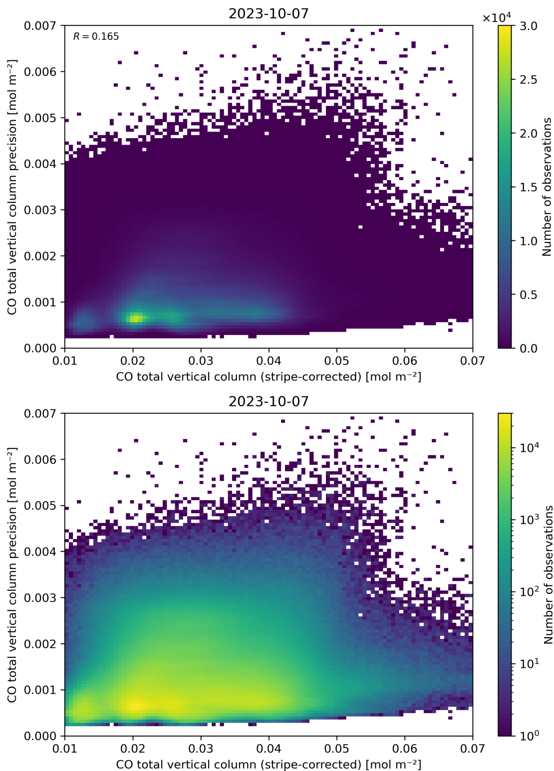
Figure 36: Scatter density plot of “CO total vertical column (stripe-corrected)” against “CO total vertical column precision” for 2023-10-06 to 2023-10-08.
