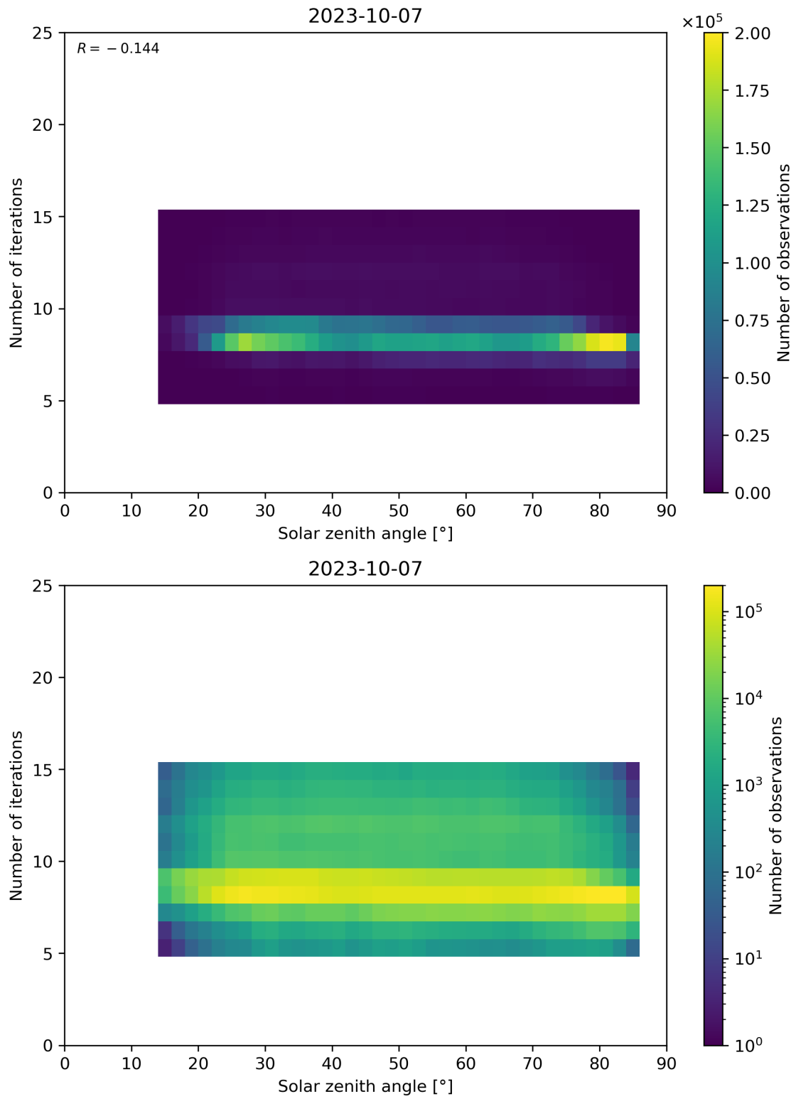
Figure 67: Scatter density plot of “Solar zenith angle” against “Number of iterations” for 2023-10-06 to 2023-10-08.
