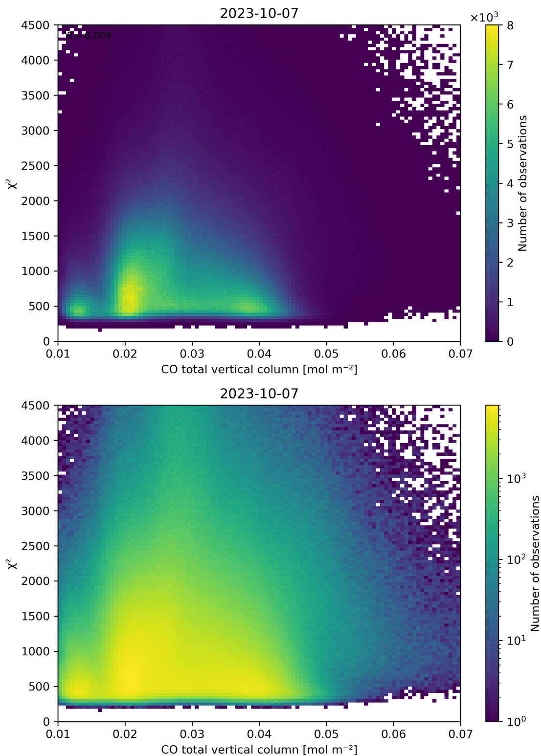
Figure 35: Scatter density plot of “CO total vertical column” against “ \chi^2 ” for 2023-10-06 to 2023-10-08.
