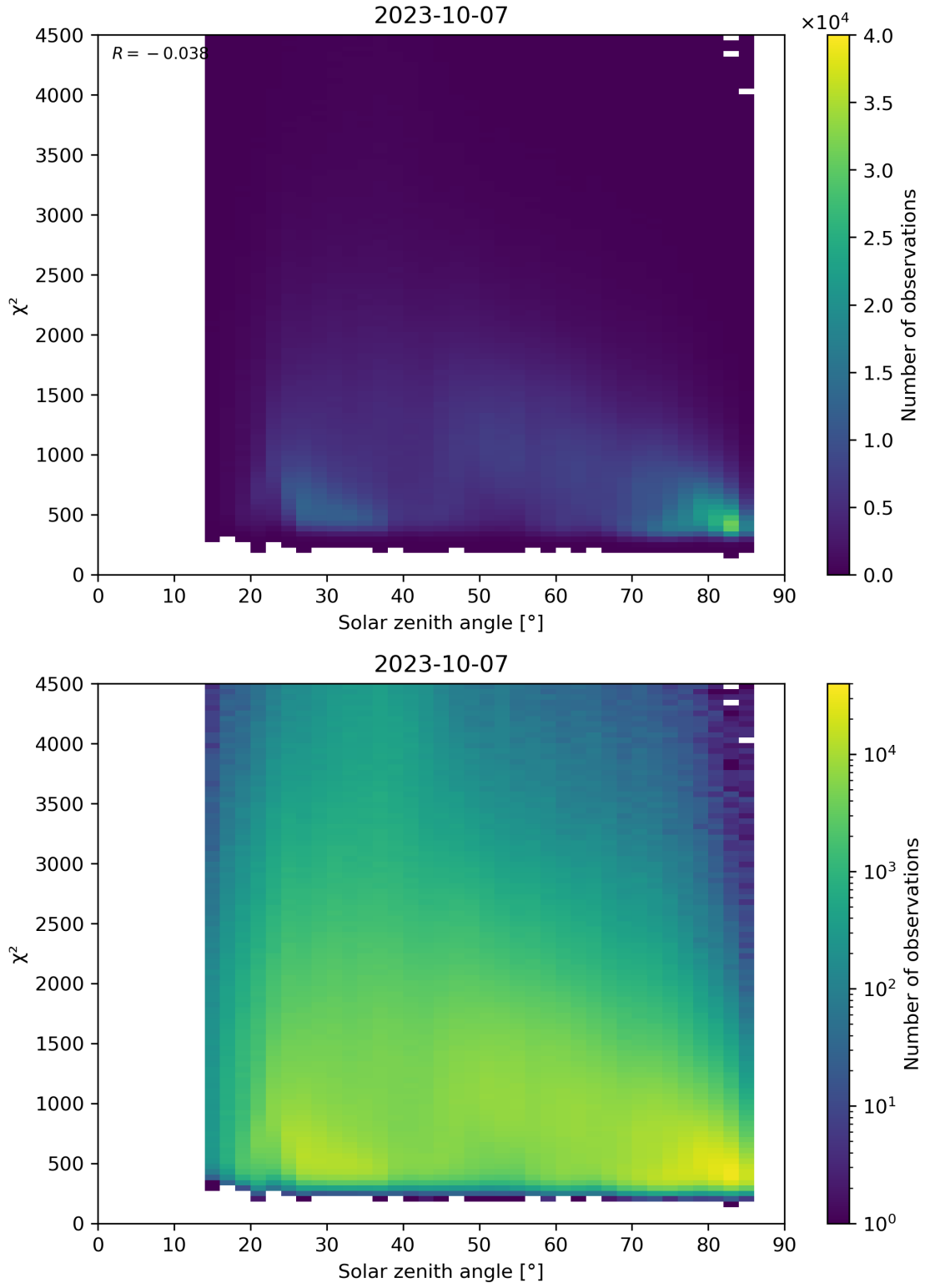
Figure 64: Scatter density plot of “Solar zenith angle” against “ \chi^2 ” for 2023-10-06 to 2023-10-08.
