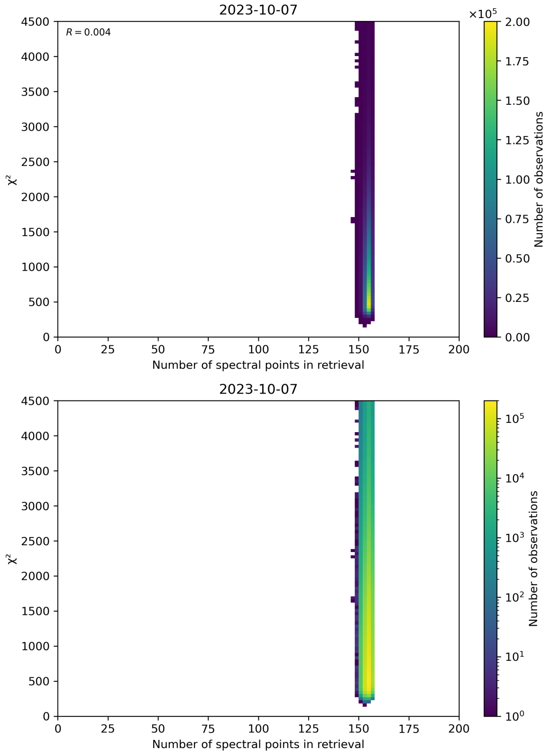
Figure 58: Scatter density plot of “Number of spectral points in retrieval” against “ \chi^2 ” for 2023-10-06 to 2023-10-08.
