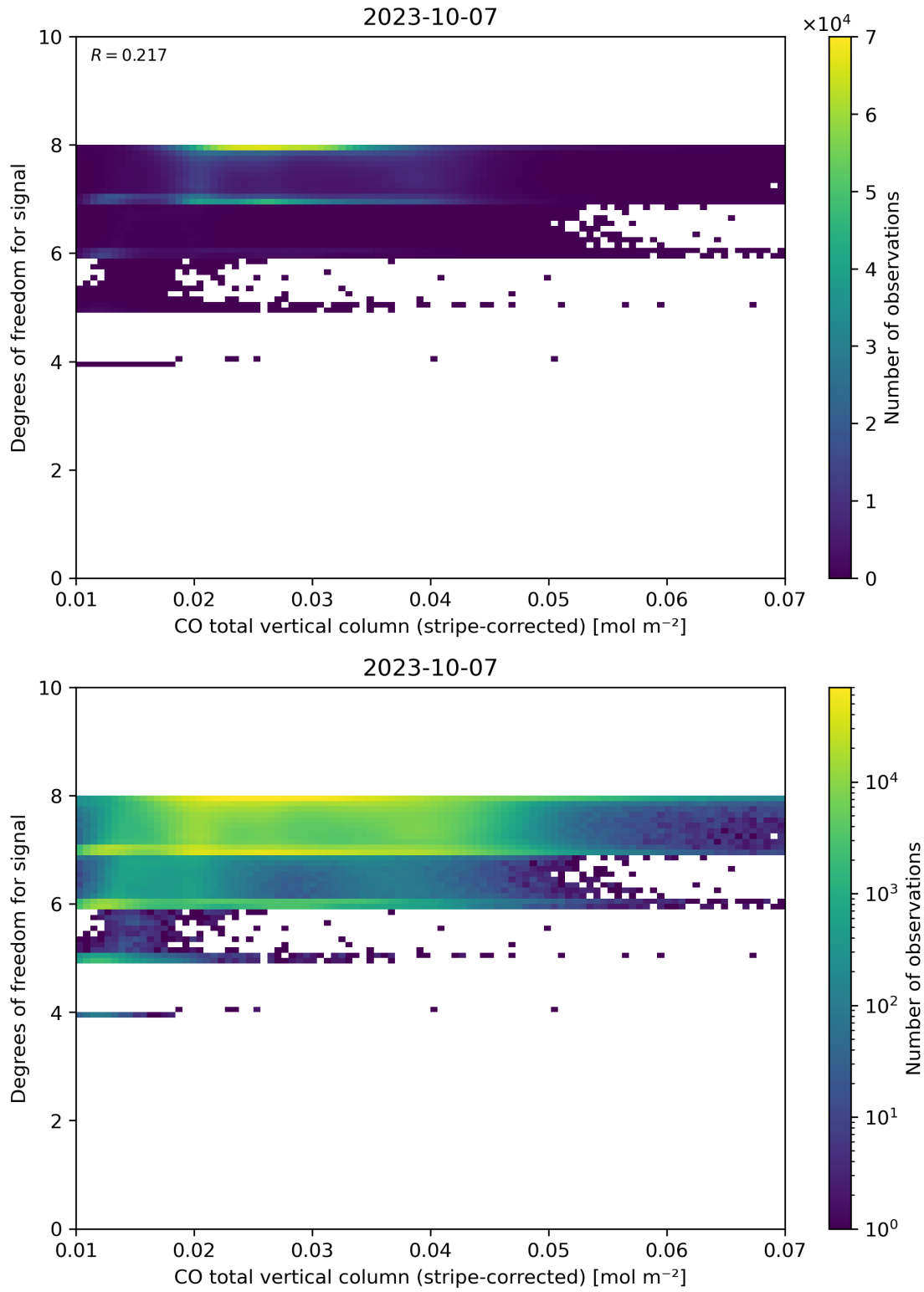
Figure 38: Scatter density plot of “CO total vertical column (stripe-corrected)” against “Degrees of freedom for signal” for 2023-10-06 to 2023-10-08.
