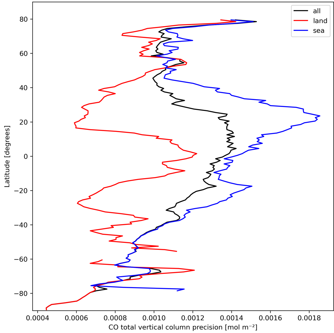
Figure 12: Zonal average of “CO total vertical column precision” for 2023-10-06 to 2023-10-08.
