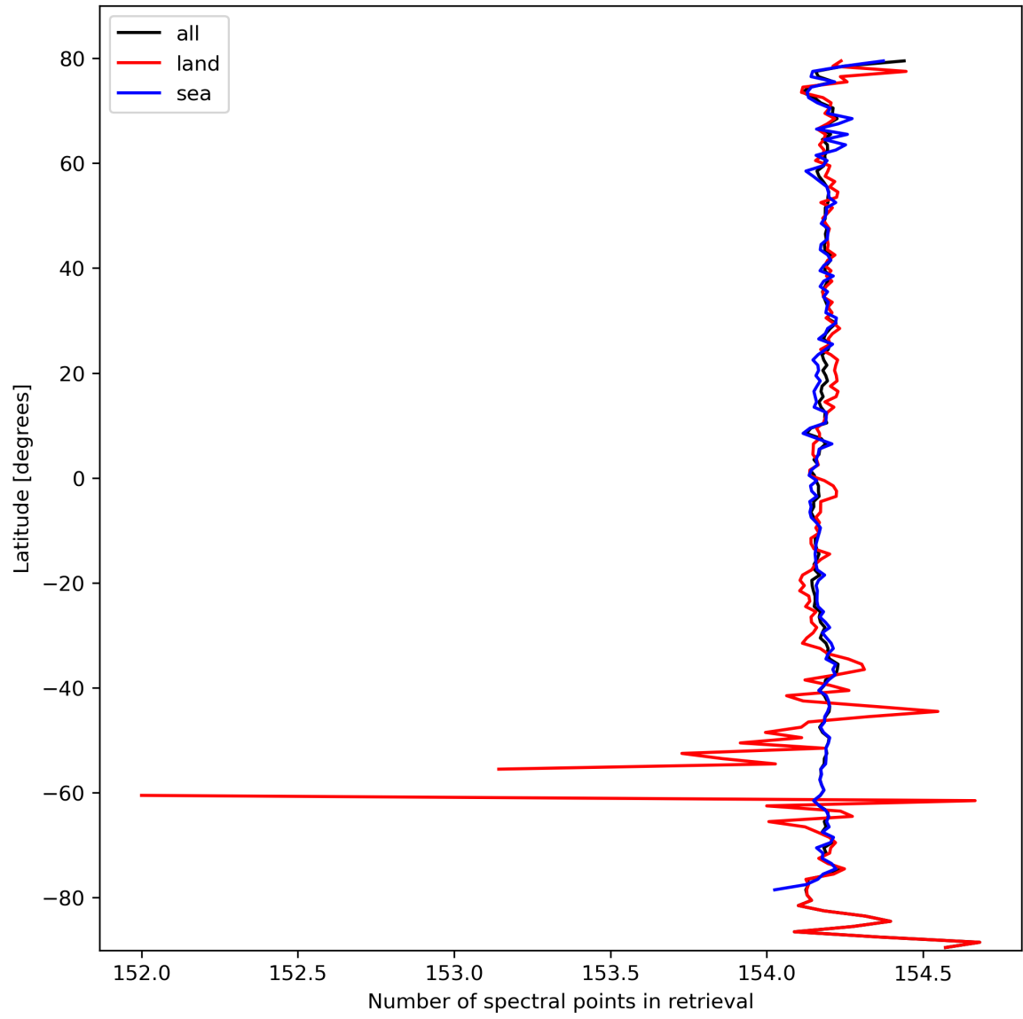
Figure 13: Zonal average of “Number of spectral points in retrieval” for 2023-10-06 to 2023-10-08.
