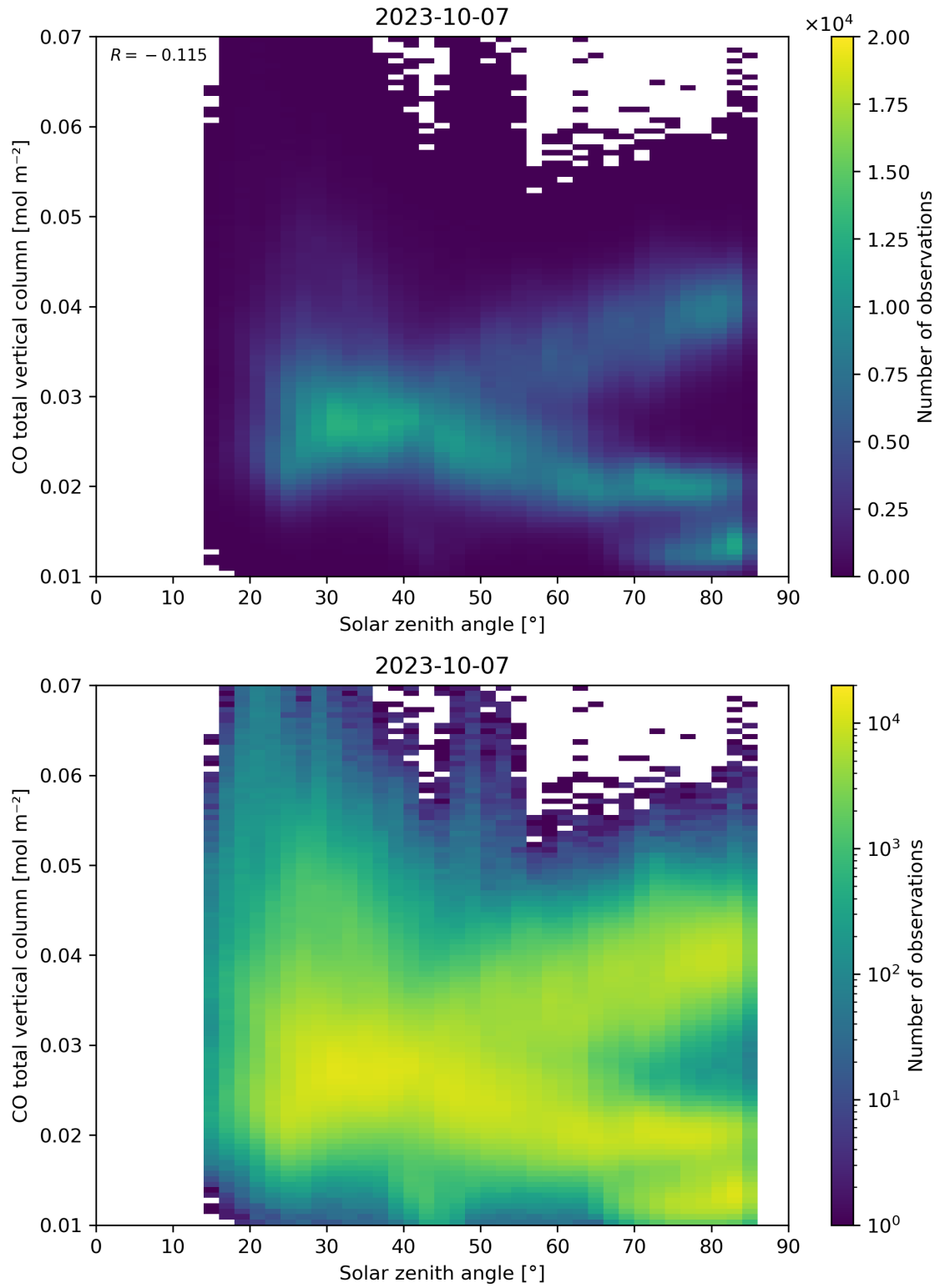
Figure 61: Scatter density plot of “Solar zenith angle” against “CO total vertical column” for 2023-10-06 to 2023-10-08.
