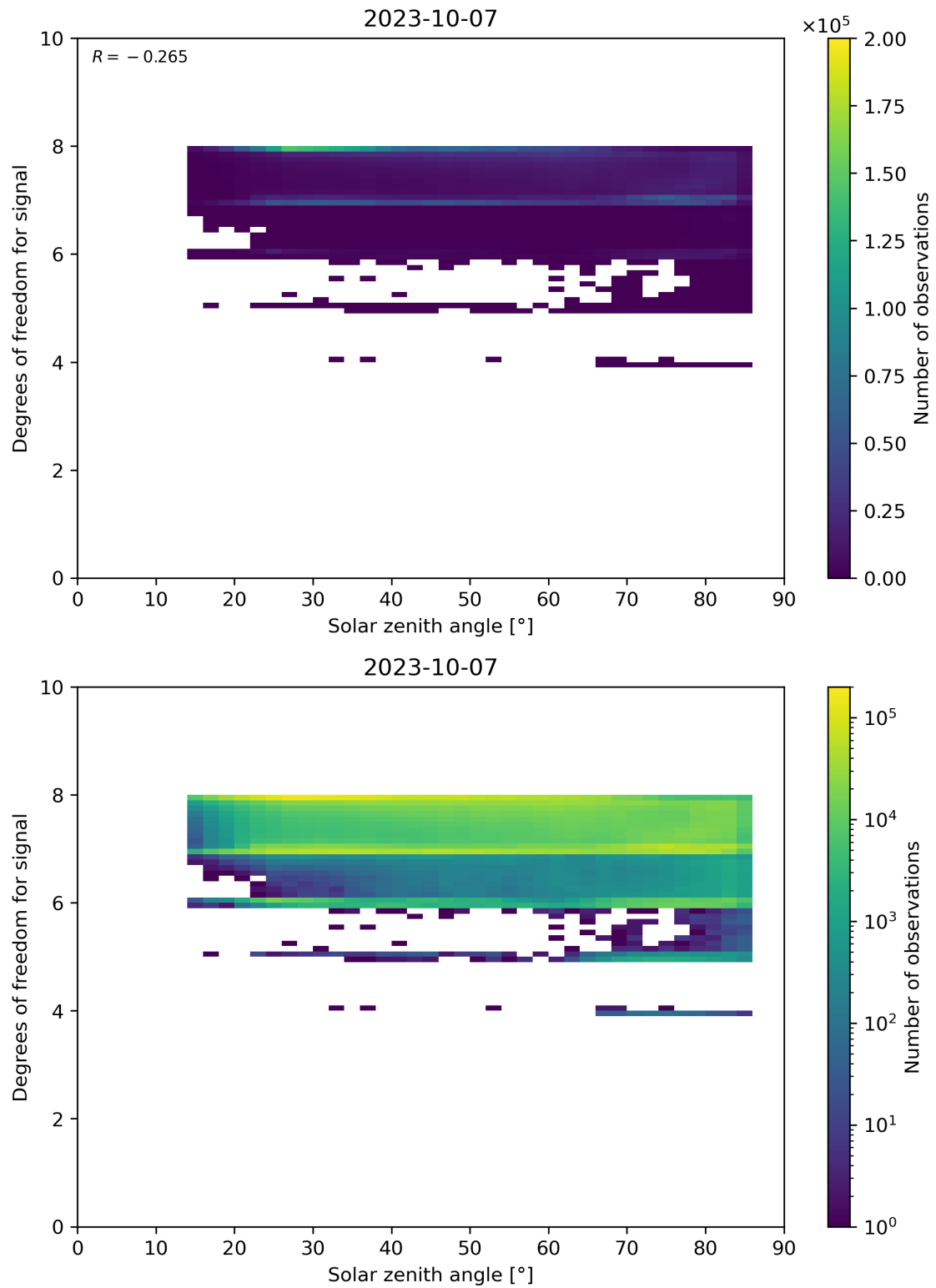
Figure 65: Scatter density plot of “Solar zenith angle” against “Degrees of freedom for signal” for 2023-10-06 to 2023-10-08.
