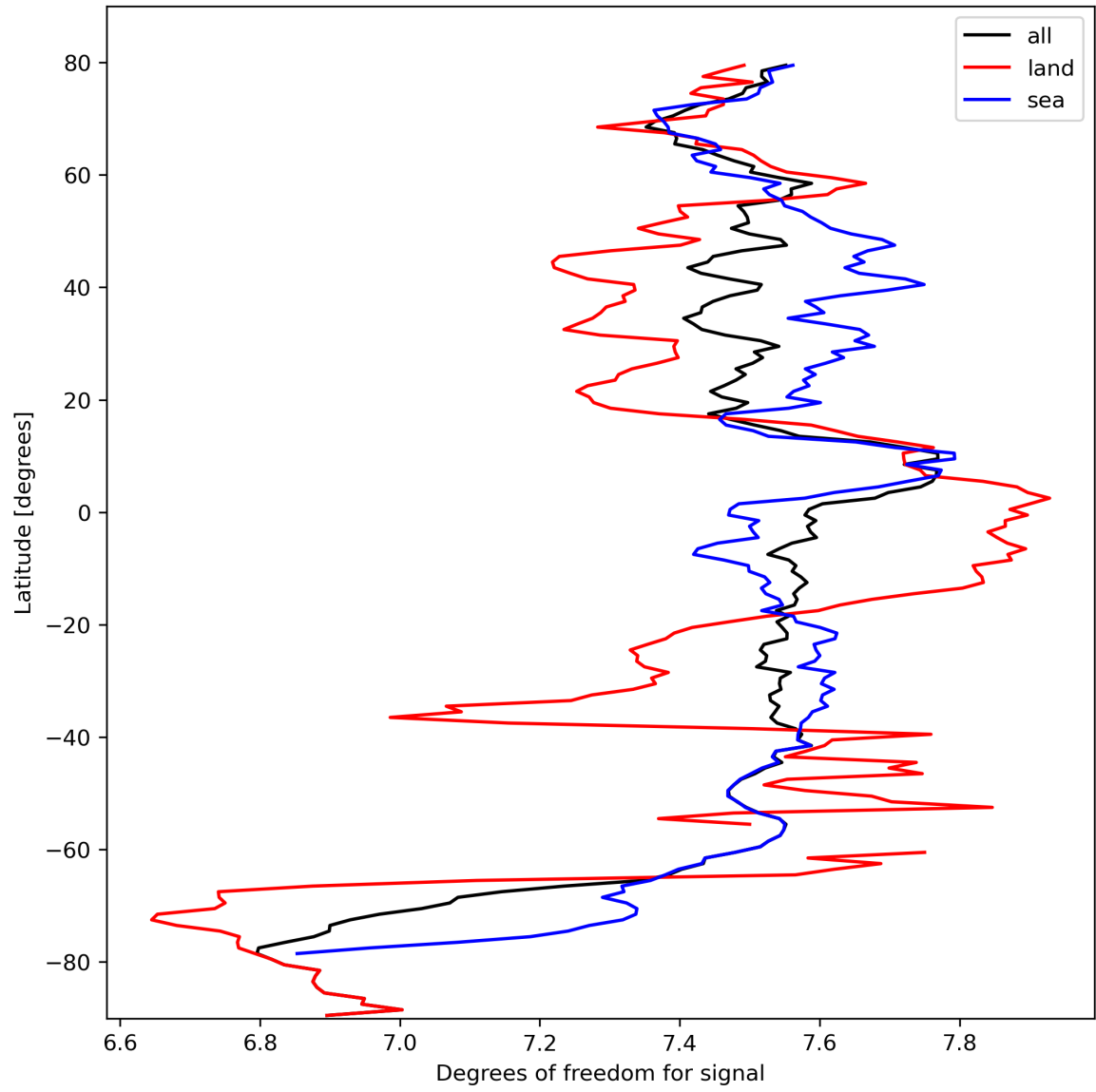
Figure 15: Zonal average of “Degrees of freedom for signal” for 2023-10-06 to 2023-10-08.
