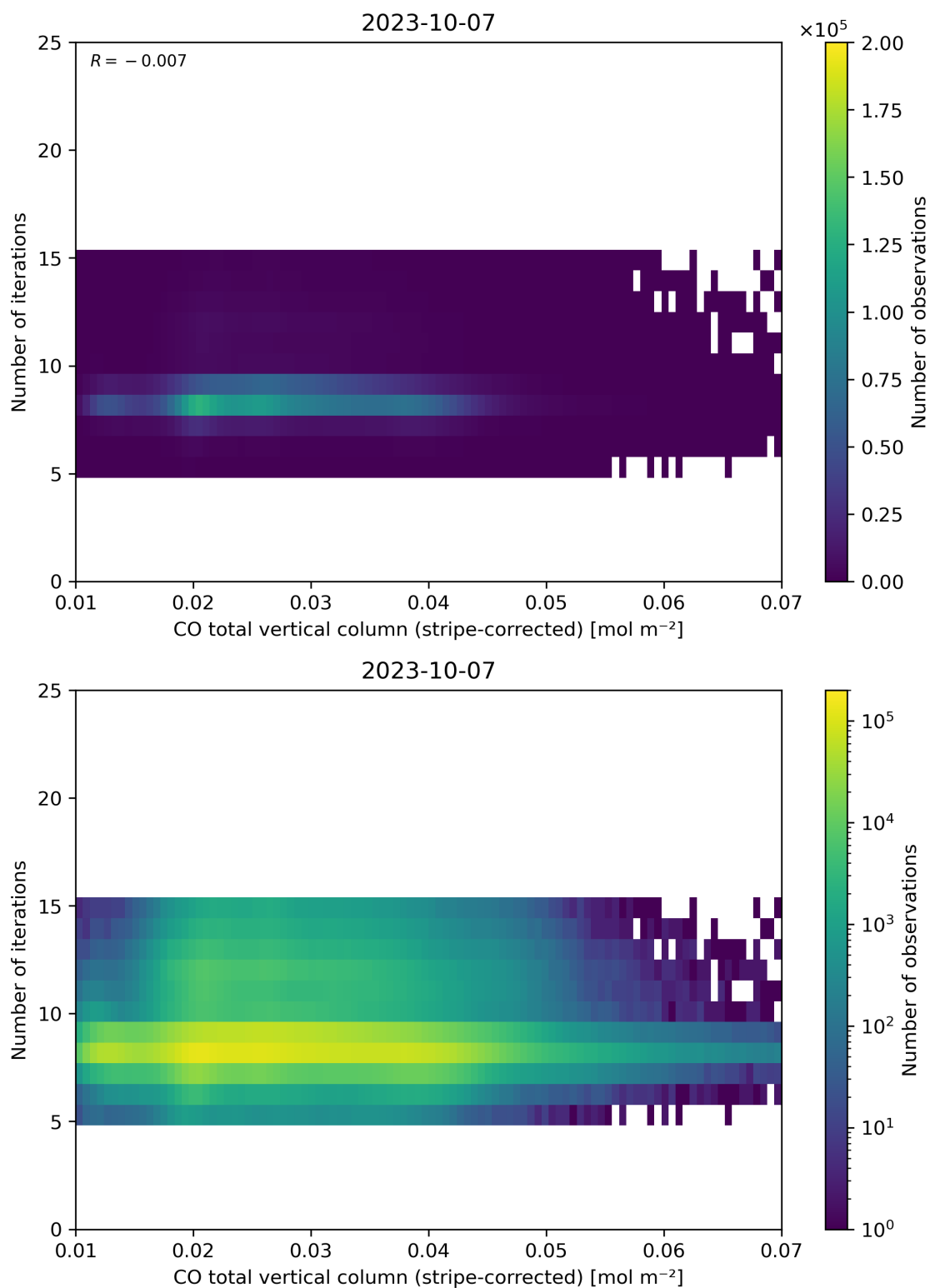
Figure 39: Scatter density plot of “CO total vertical column (stripe-corrected)” against “Number of iterations” for 2023-10-06 to 2023-10-08.
