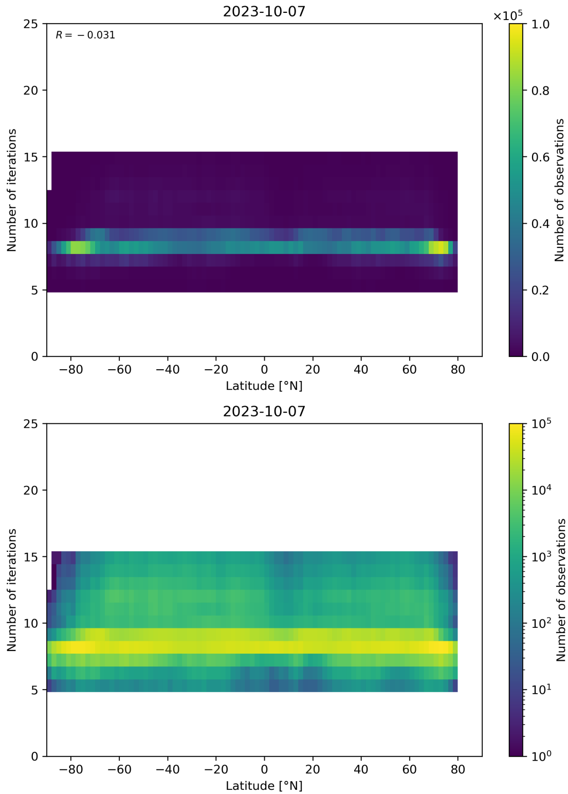
Figure 56: Scatter density plot of “Latitude” against “Number of iterations” for 2023-10-06 to 2023-10-08.
