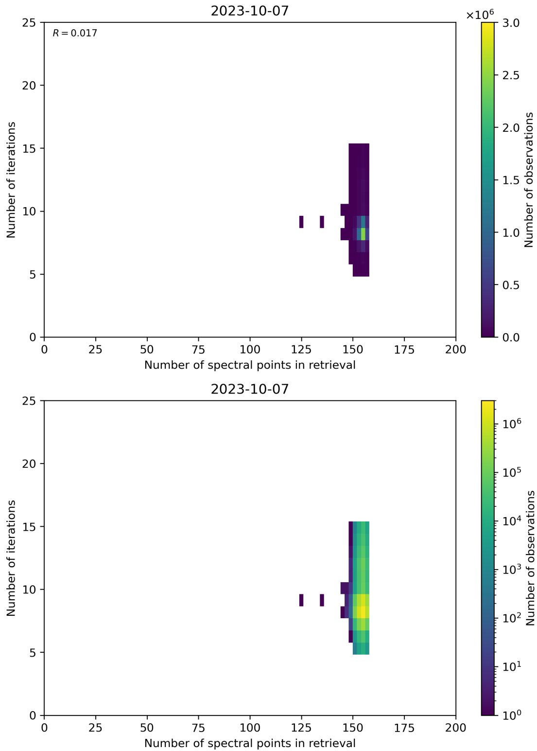
Figure 60: Scatter density plot of “Number of spectral points in retrieval” against “Number of iterations” for 2023-10-06 to 2023-10-08.
