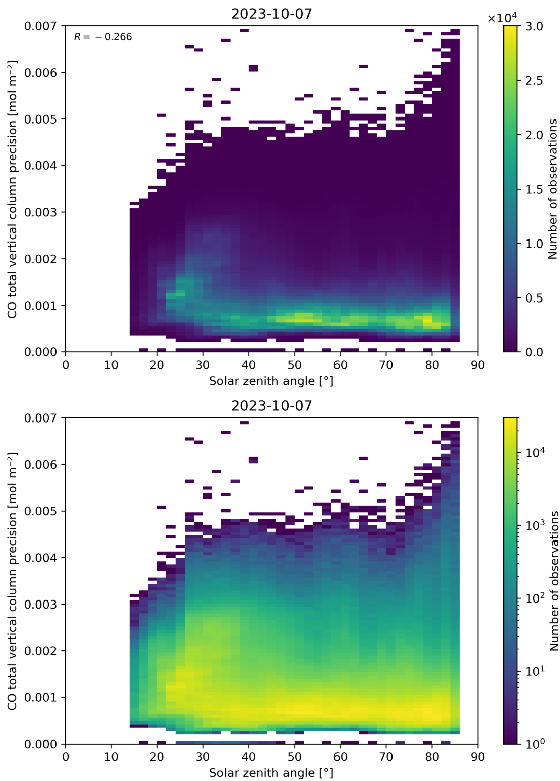
Figure 63: Scatter density plot of “Solar zenith angle” against “CO total vertical column precision” for 2023-10-06 to 2023-10-08.
