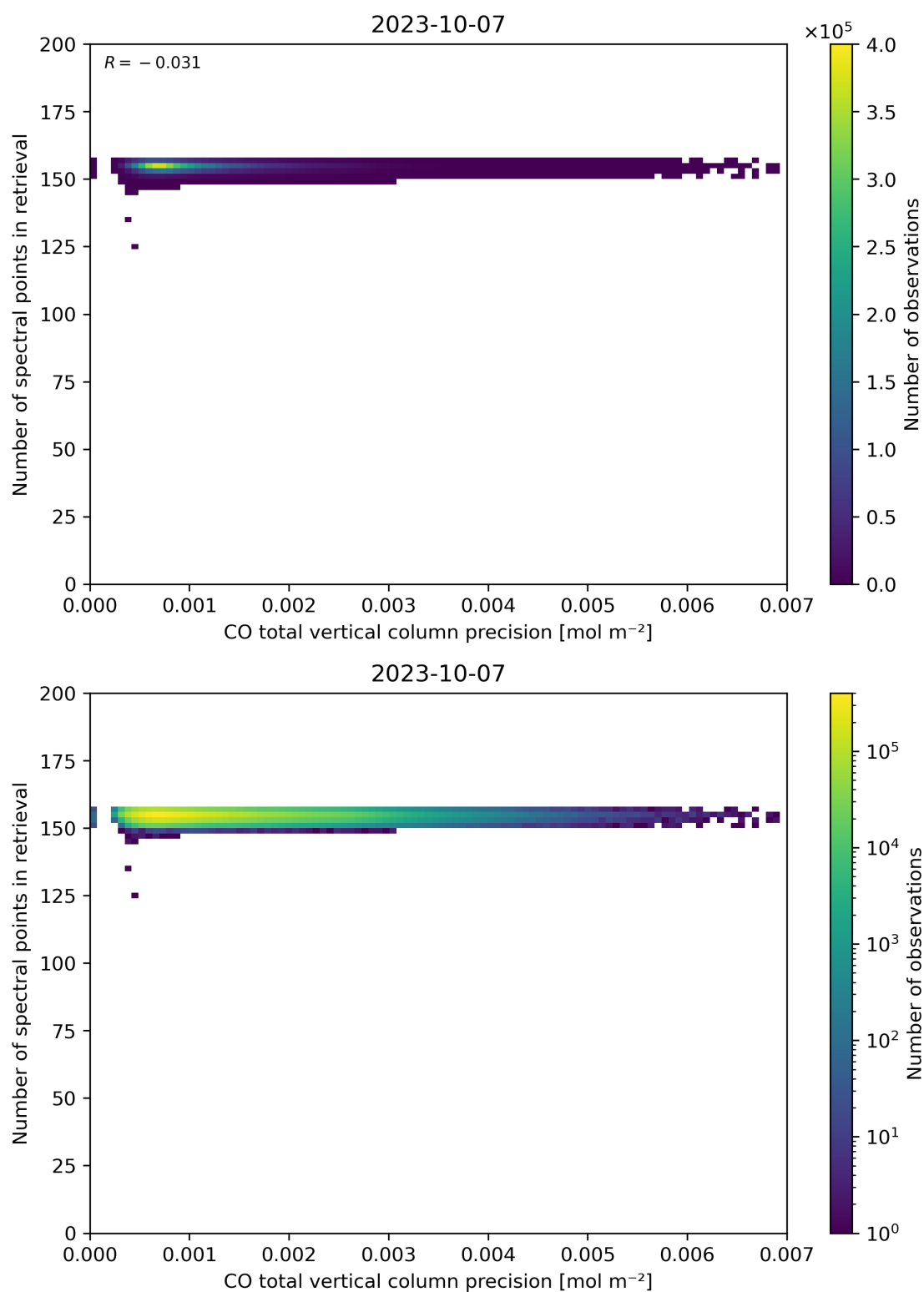
Figure 47: Scatter density plot of “CO total vertical column precision” against “Number of spectral points in retrieval” for 2023-10-06 to 2023-10-08.
