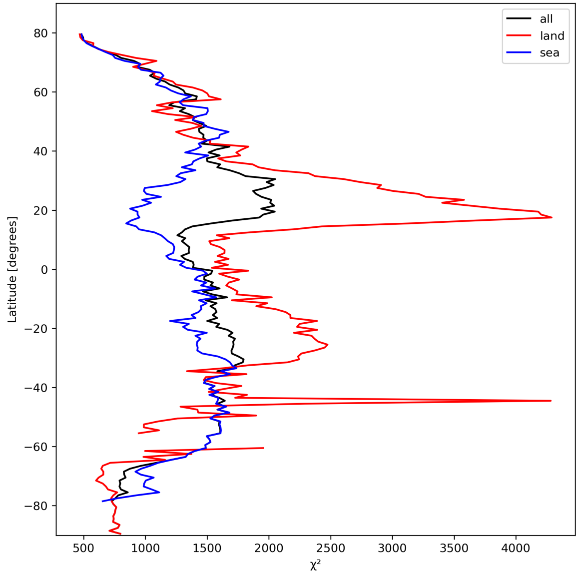
Figure 14: Zonal average of “ \chi^2 ” for 2023-10-06 to 2023-10-08.
