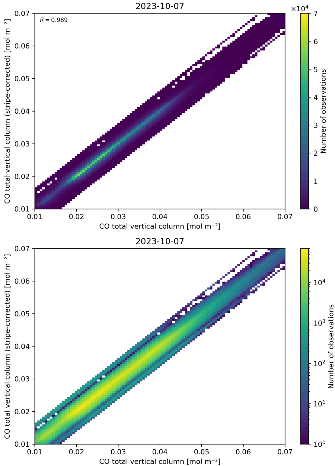
Figure 33: Scatter density plot of “CO total vertical column” against “CO total vertical column (stripe-corrected)” for 2023-10-06 to 2023-10-08.
