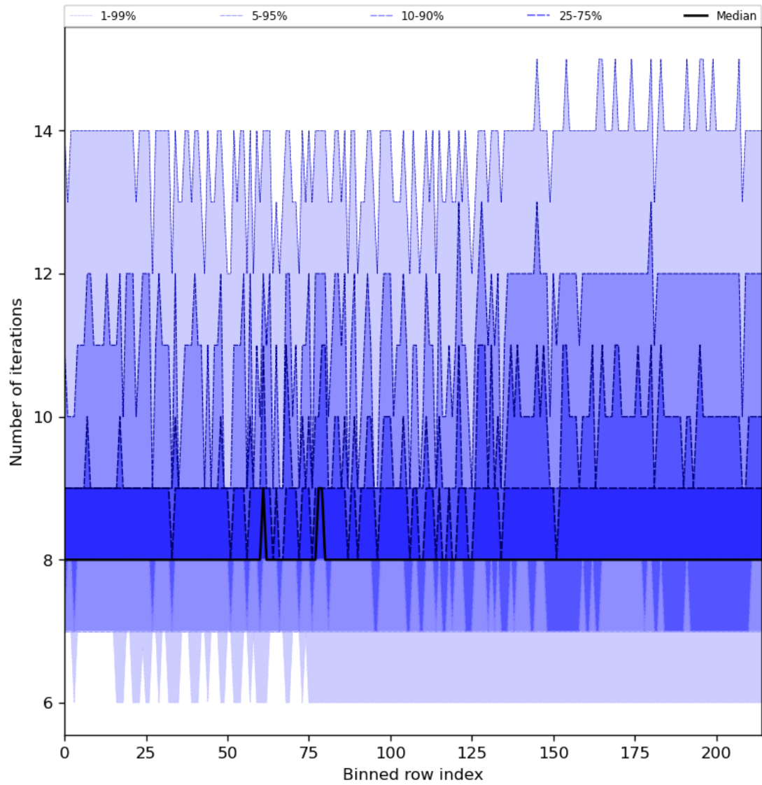
Figure 32: Along track statistics of “Number of iterations” for 2023-10-06 to 2023-10-08
