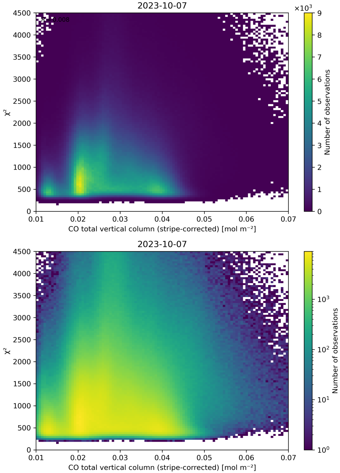
Figure 37: Scatter density plot of “CO total vertical column (stripe-corrected)” against “ \chi^2 ” for 2023-10-06 to 2023-10-08.
