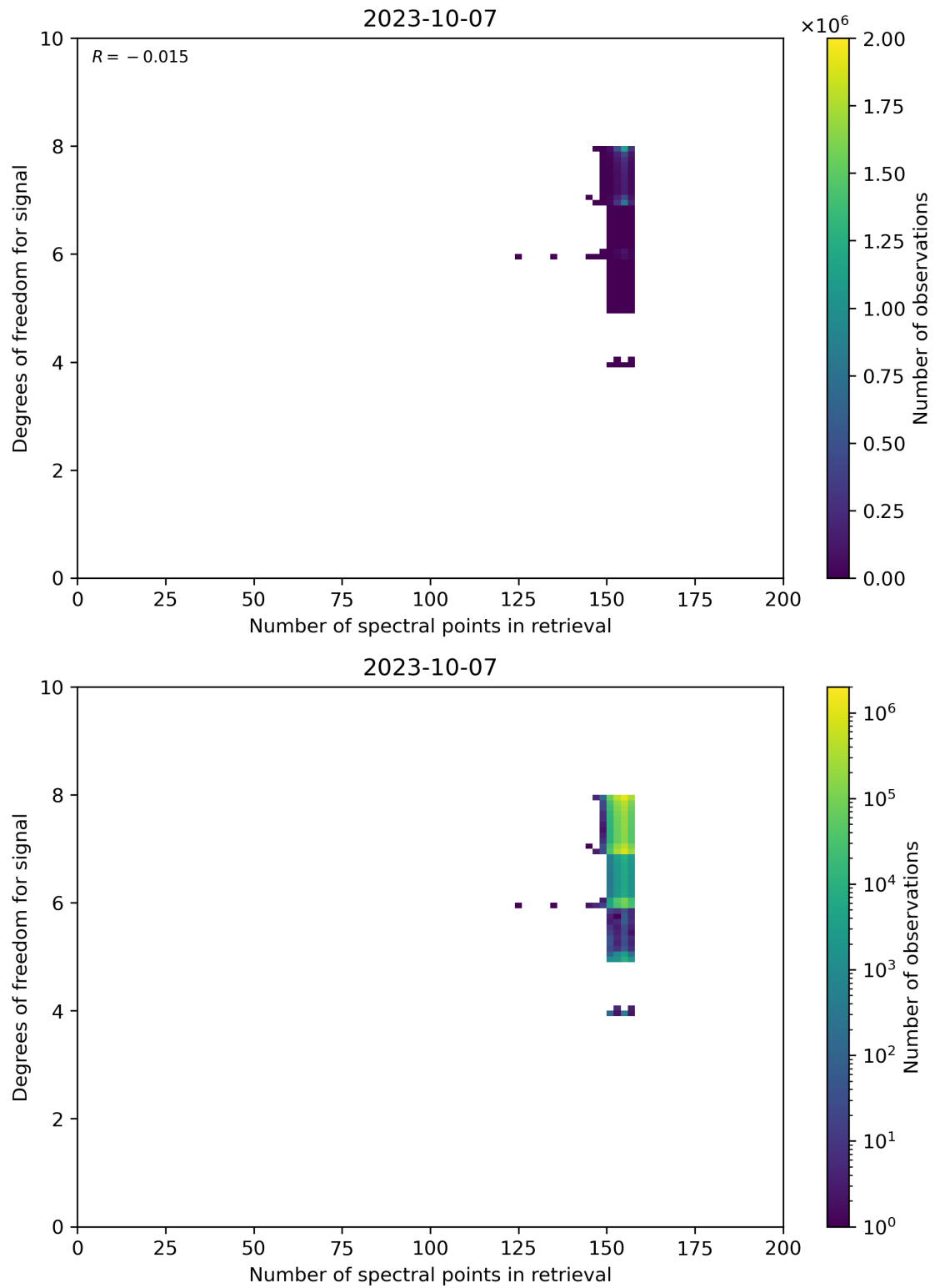
Figure 59: Scatter density plot of “Number of spectral points in retrieval” against “Degrees of freedom for signal” for 2023-10-06 to 2023-10-08.
