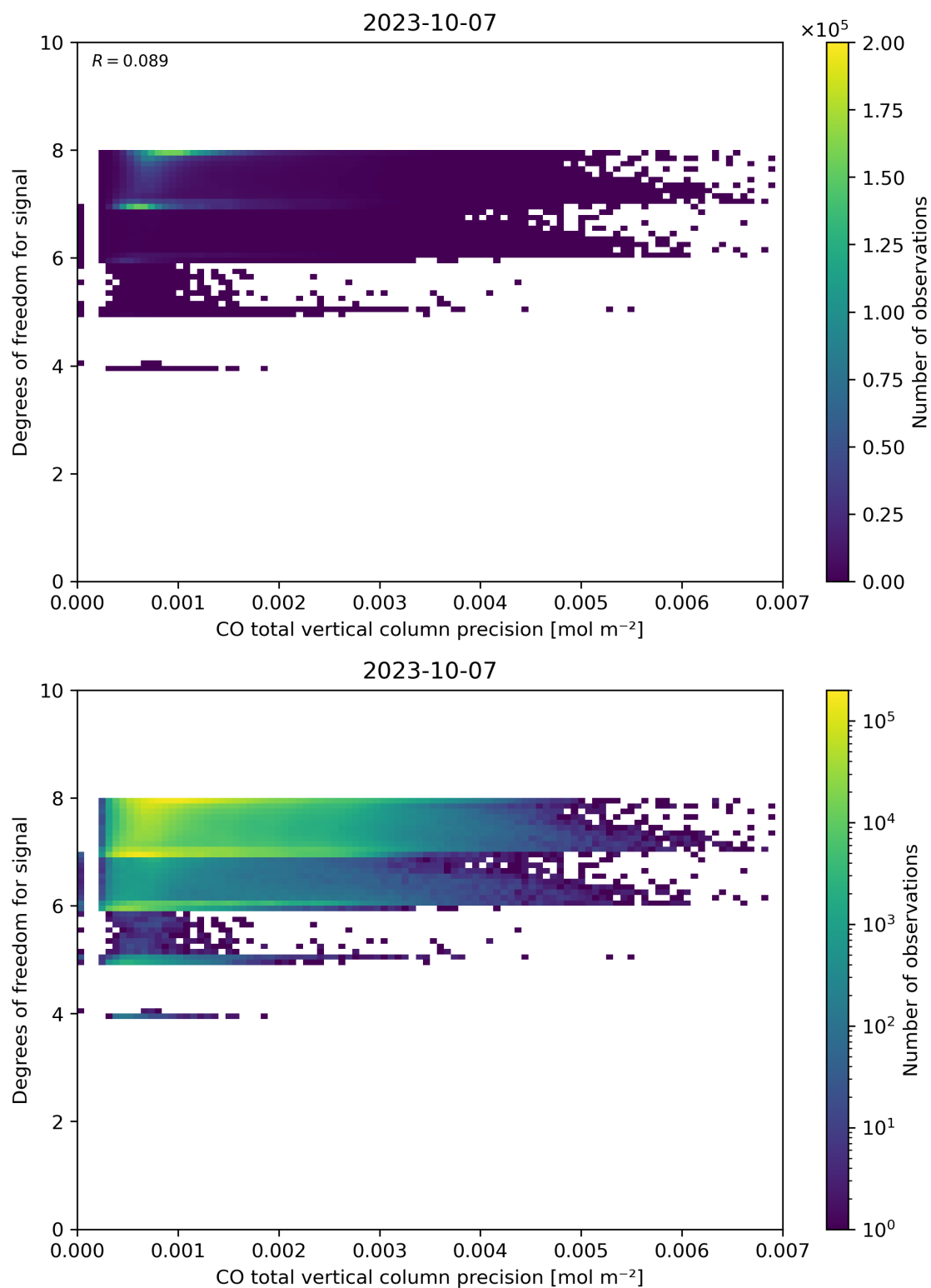
Figure 45: Scatter density plot of “CO total vertical column precision” against “Degrees of freedom for signal” for 2023-10-06 to 2023-10-08.
