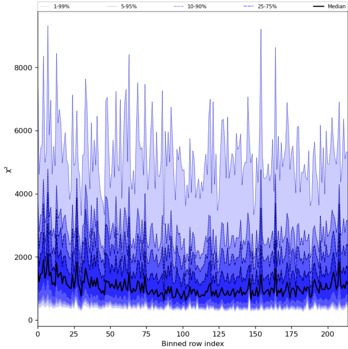
Figure 30: Along track statistics of “ \chi^2 ” for 2023-10-06 to 2023-10-08
