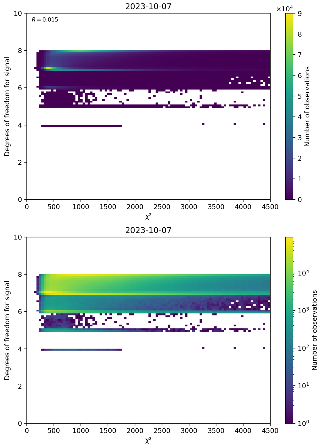
Figure 48: Scatter density plot of " \chi^2 " against "Degrees of freedom for signal" for 2023-10-06 to 2023-10-08.
