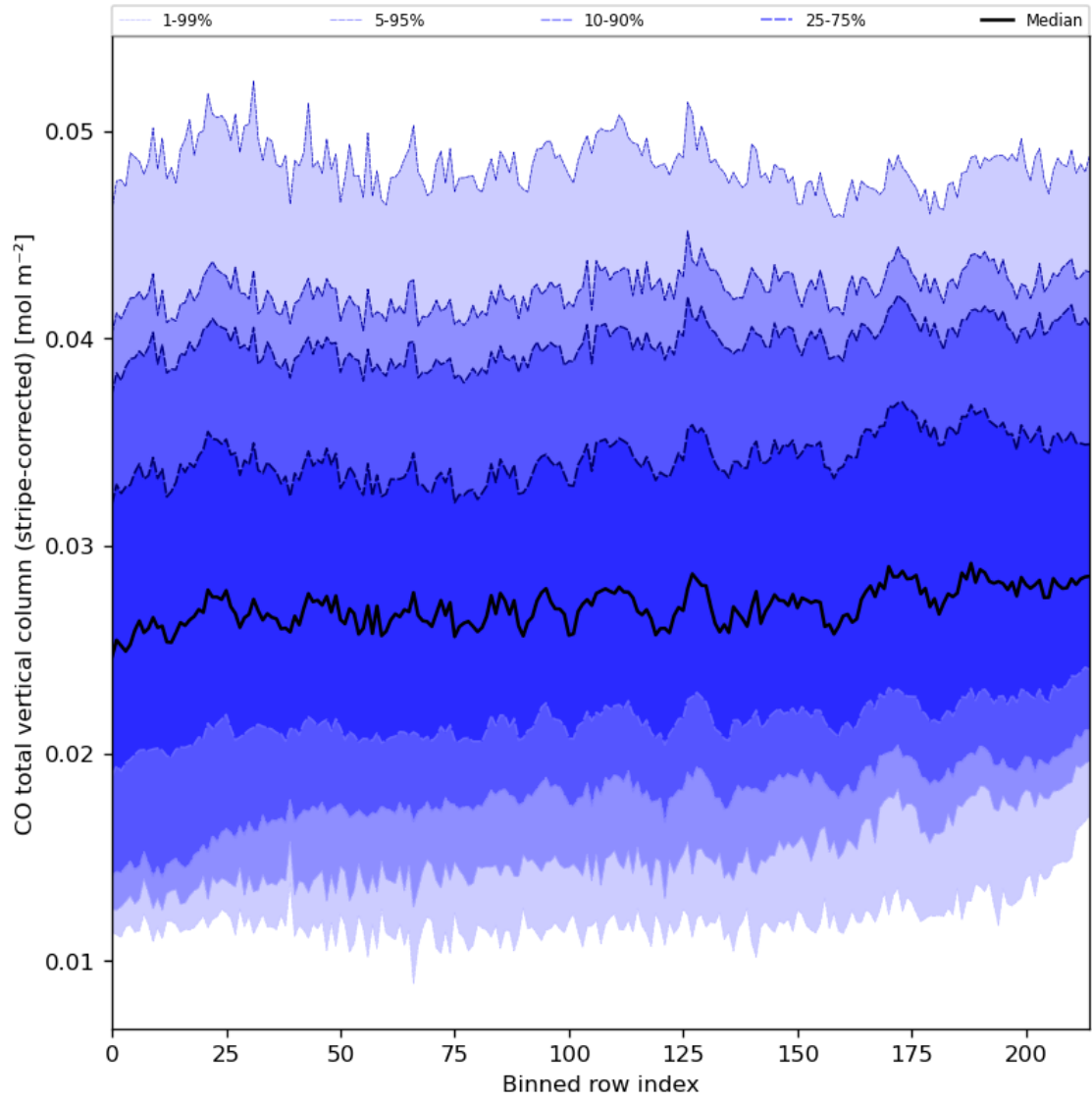
Figure 27: Along track statistics of “CO total vertical column (stripe-corrected)” for 2023-10-06 to 2023-10-08
