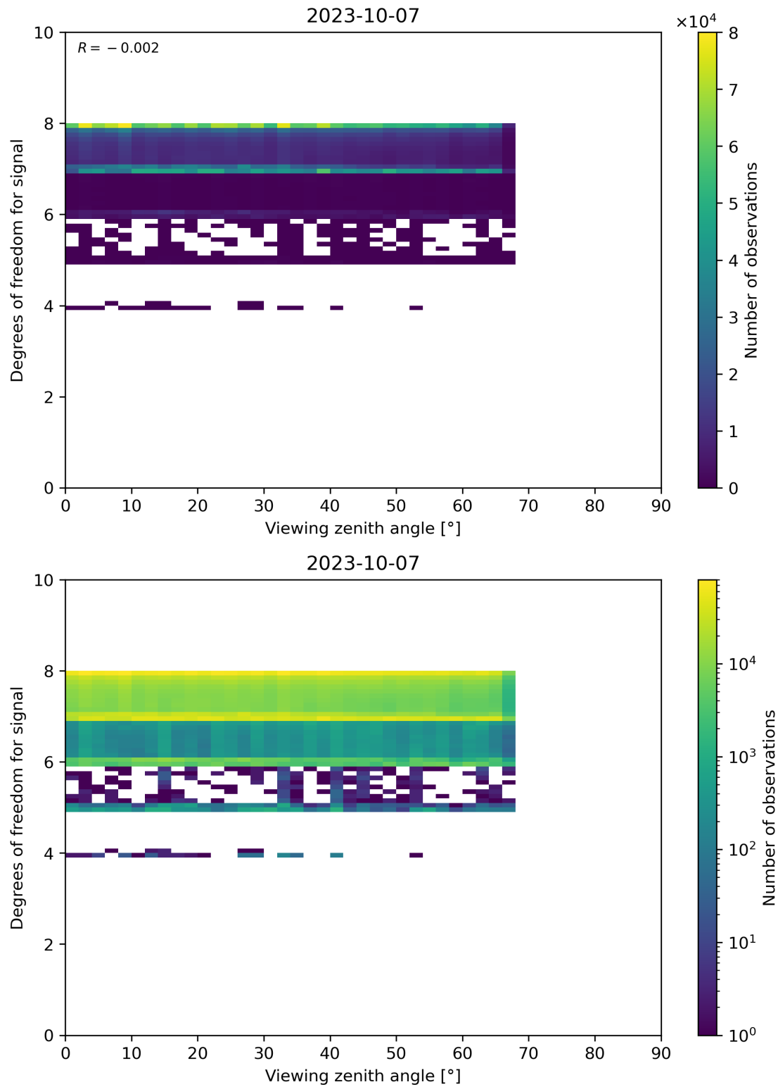
Figure 73: Scatter density plot of “Viewing zenith angle” against “Degrees of freedom for signal” for 2023-10-06 to 2023-10-08.
