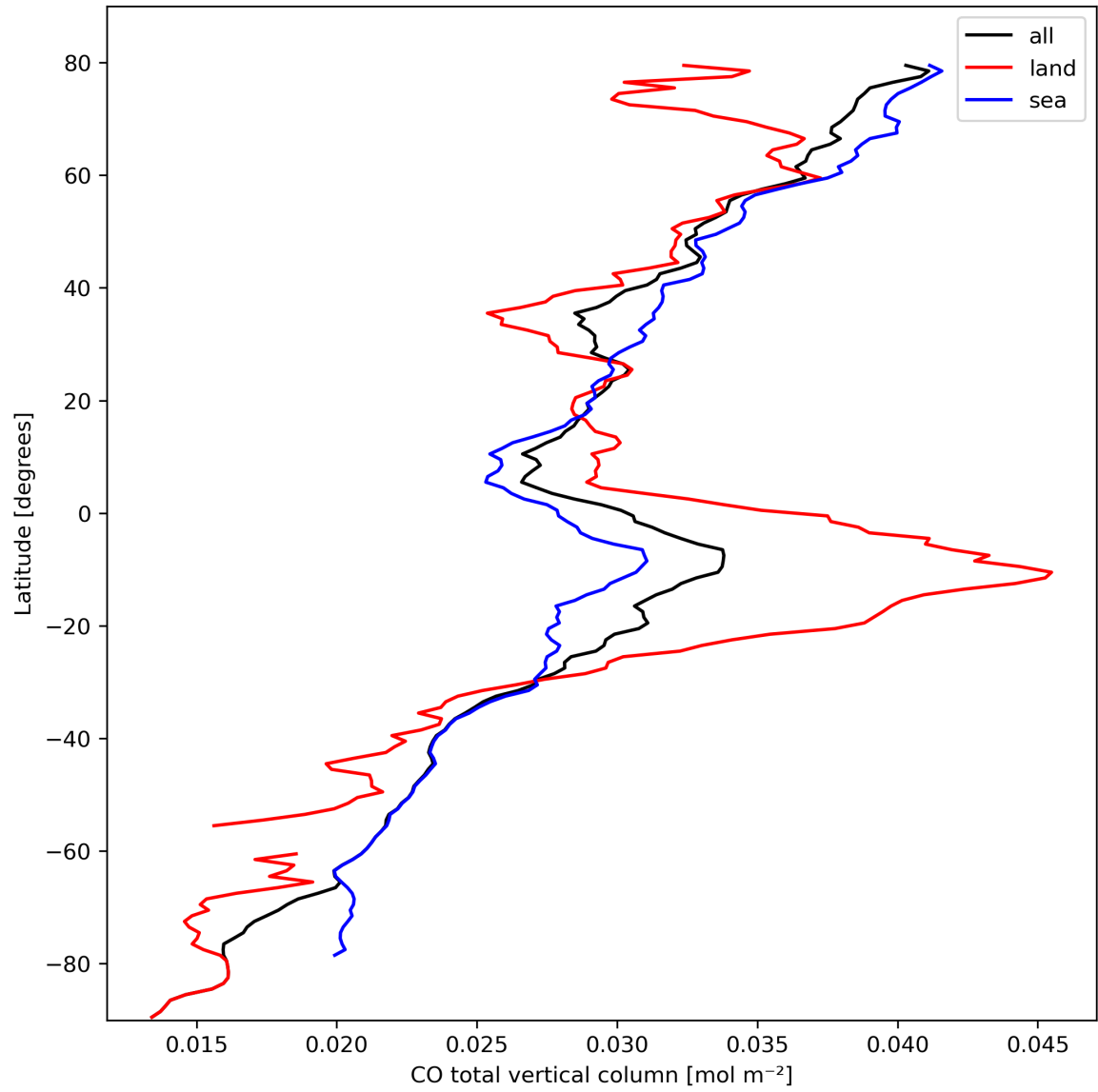
Figure 10: Zonal average of “CO total vertical column” for 2023-10-06 to 2023-10-08.
