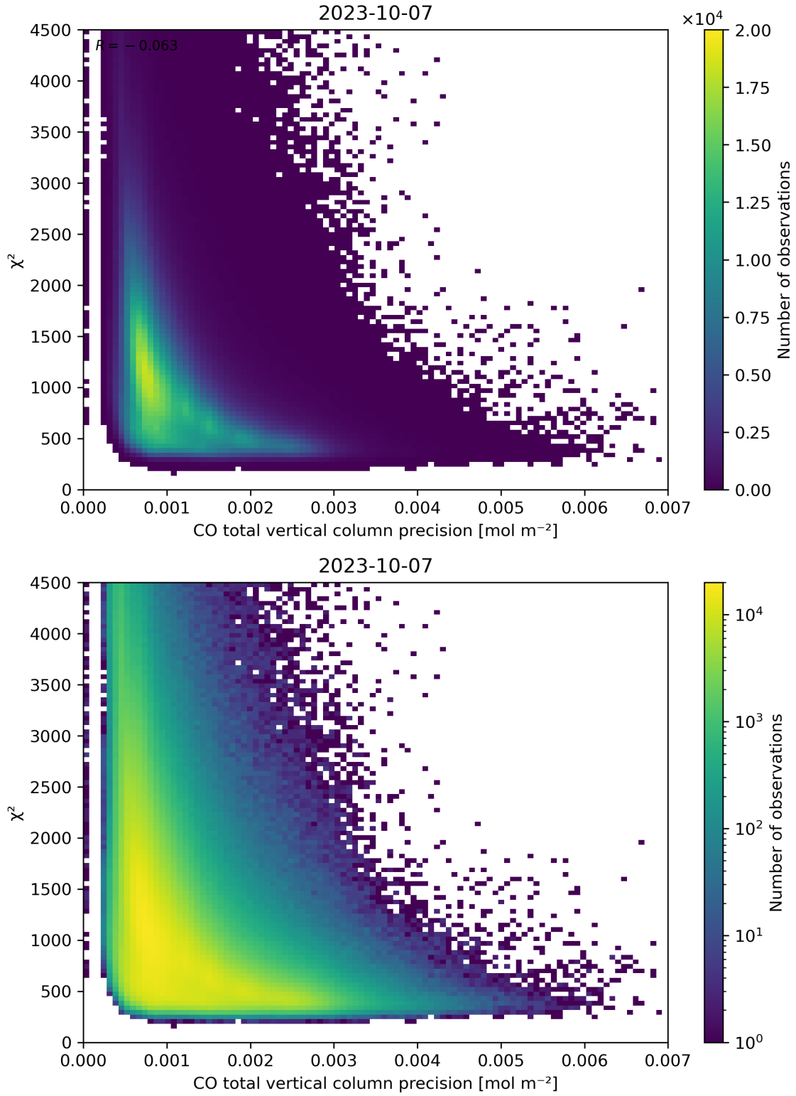
Figure 44: Scatter density plot of “CO total vertical column precision” against “ \chi^2 ” for 2023-10-06 to 2023-10-08.
