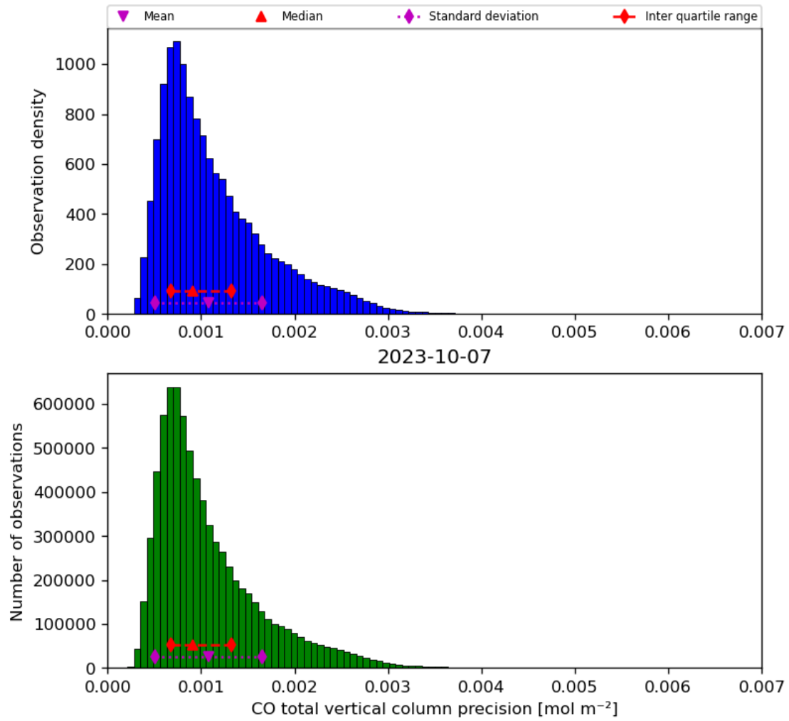
Figure 20: Histogram of “CO total vertical column precision” for 2023-10-06 to 2023-10-08
