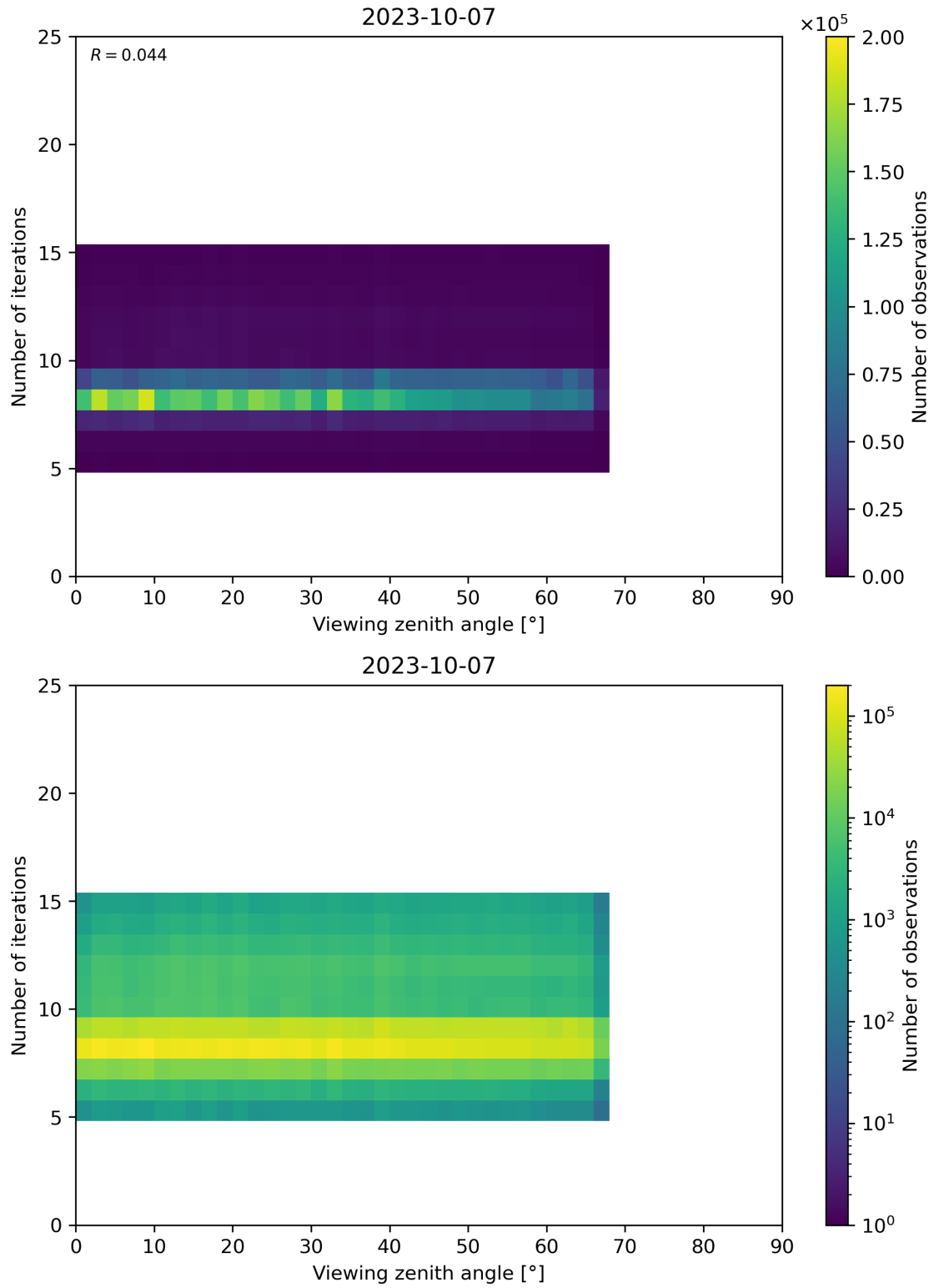
Figure 75: Scatter density plot of “Viewing zenith angle” against “Number of iterations” for 2023-10-06 to 2023-10-08.
