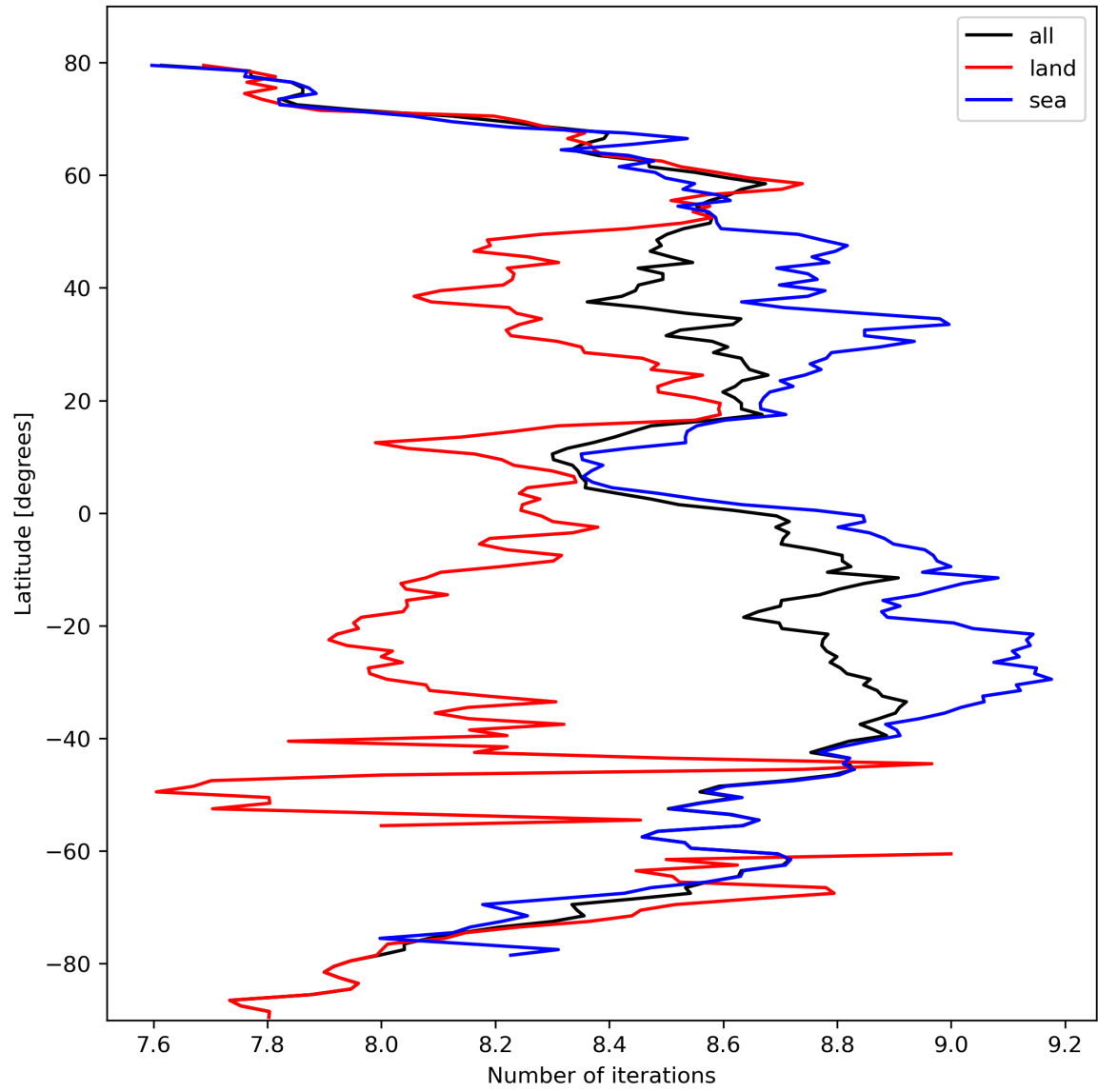
Figure 16: Zonal average of “Number of iterations” for 2023-10-06 to 2023-10-08.
