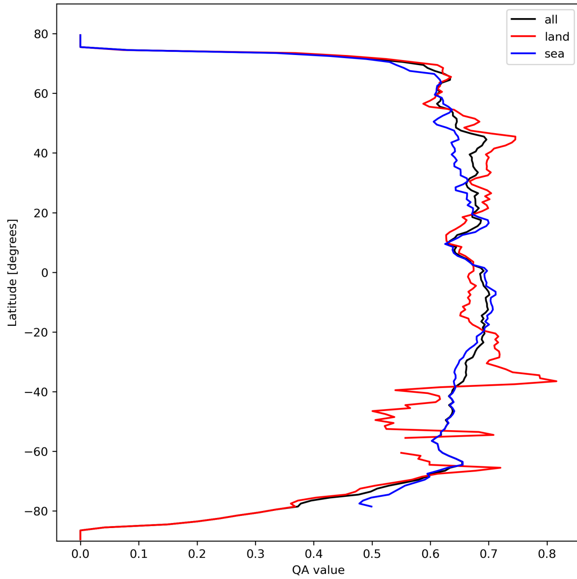
Figure 9: Zonal average of “QA value” for 2023-10-06 to 2023-10-08.
