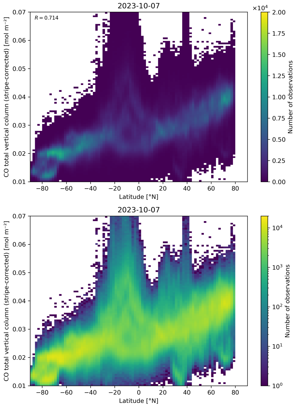
Figure 52: Scatter density plot of “Latitude” against “CO total vertical column (stripe-corrected)” for 2023-10-06 to 2023-10-08.
