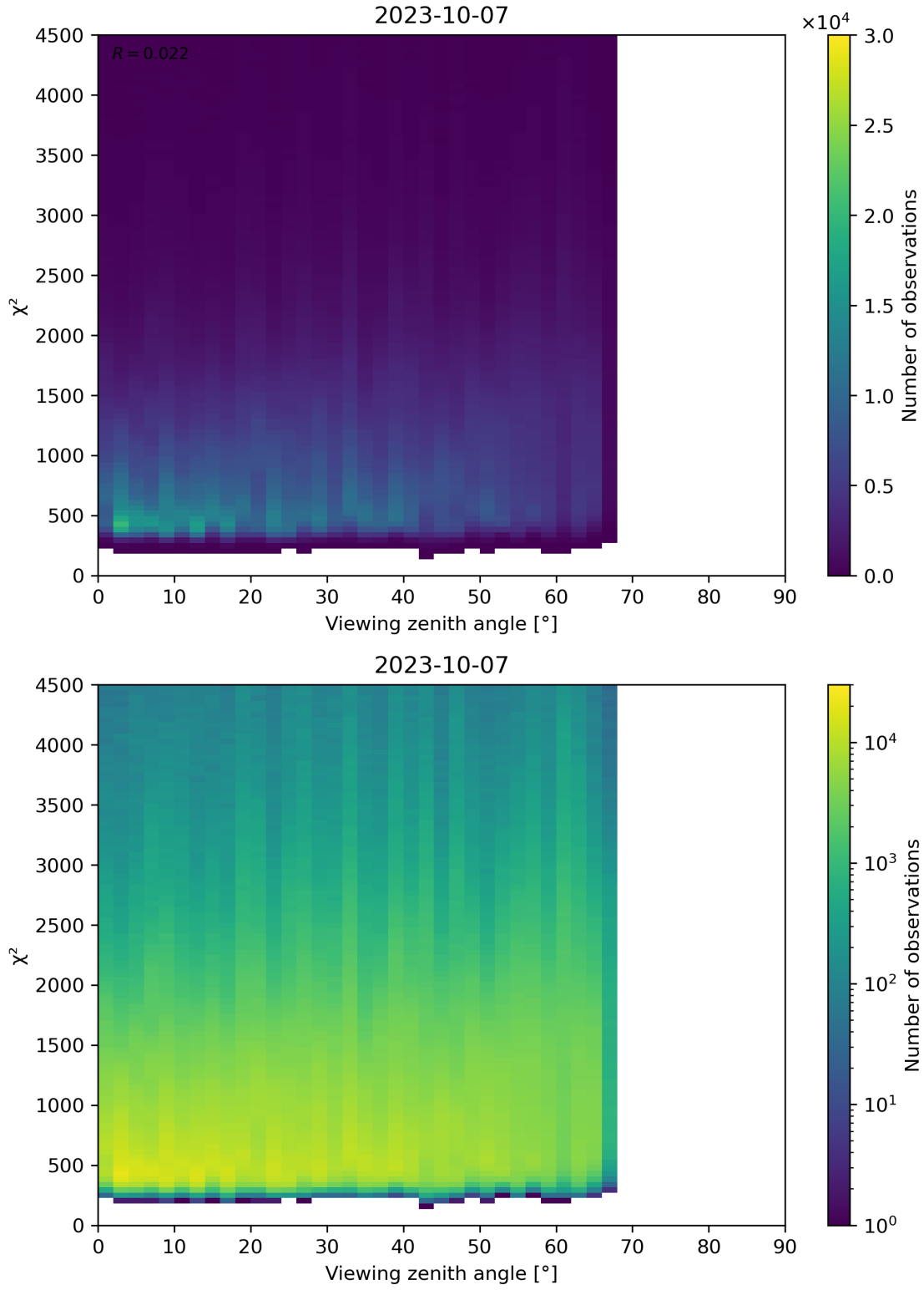
Figure 72: Scatter density plot of “Viewing zenith angle” against “ \chi^2 ” for 2023-10-06 to 2023-10-08.
