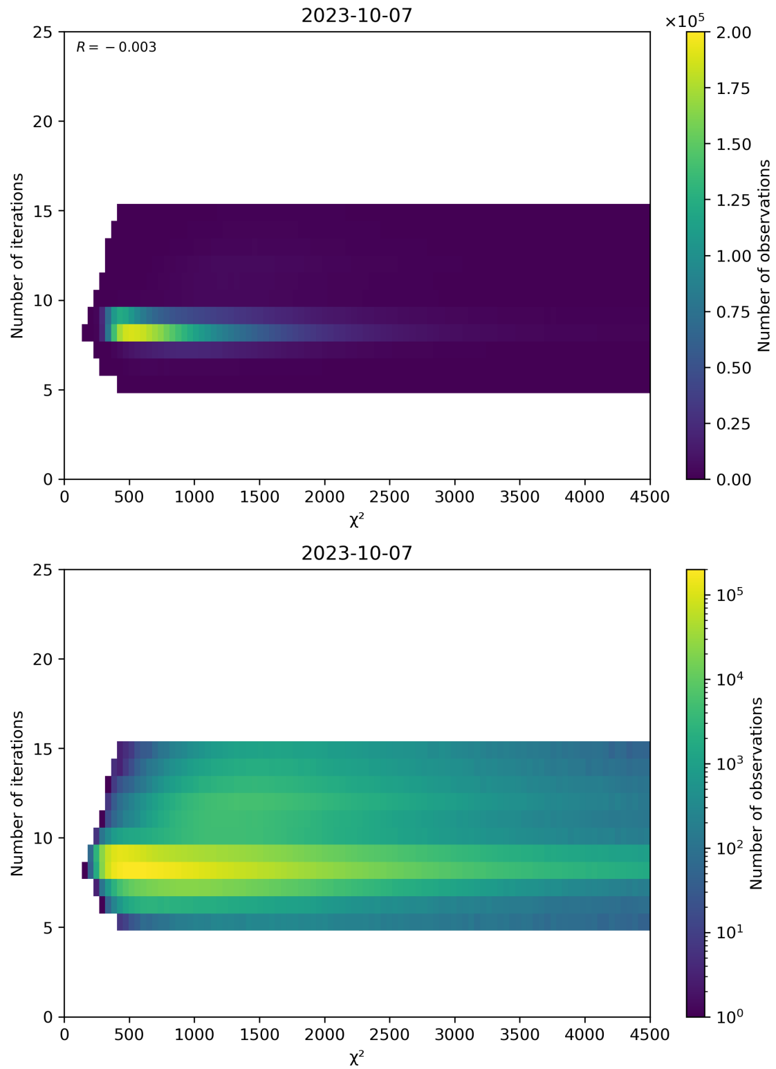
Figure 49: Scatter density plot of “ \chi^2 ” against “Number of iterations” for 2023-10-06 to 2023-10-08.
