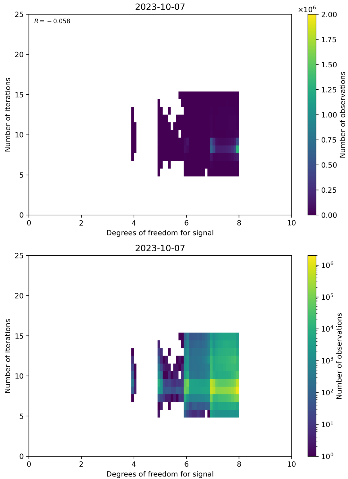
Figure 50: Scatter density plot of “Degrees of freedom for signal” against “Number of iterations” for 2023-10-06 to 2023-10-08.
