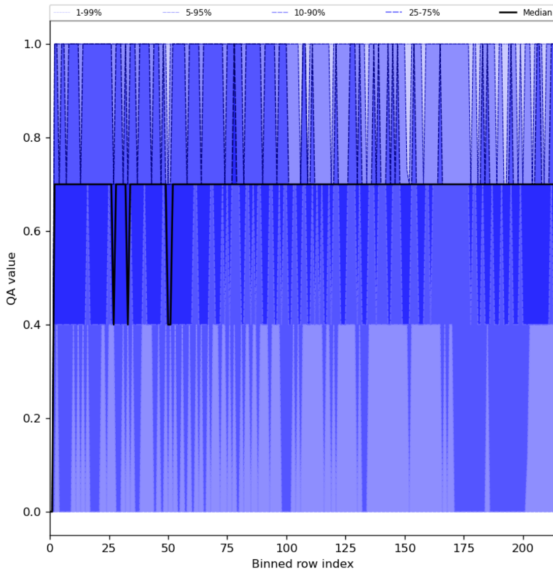
Figure 25: Along track statistics of “QA value” for 2023-10-06 to 2023-10-08
