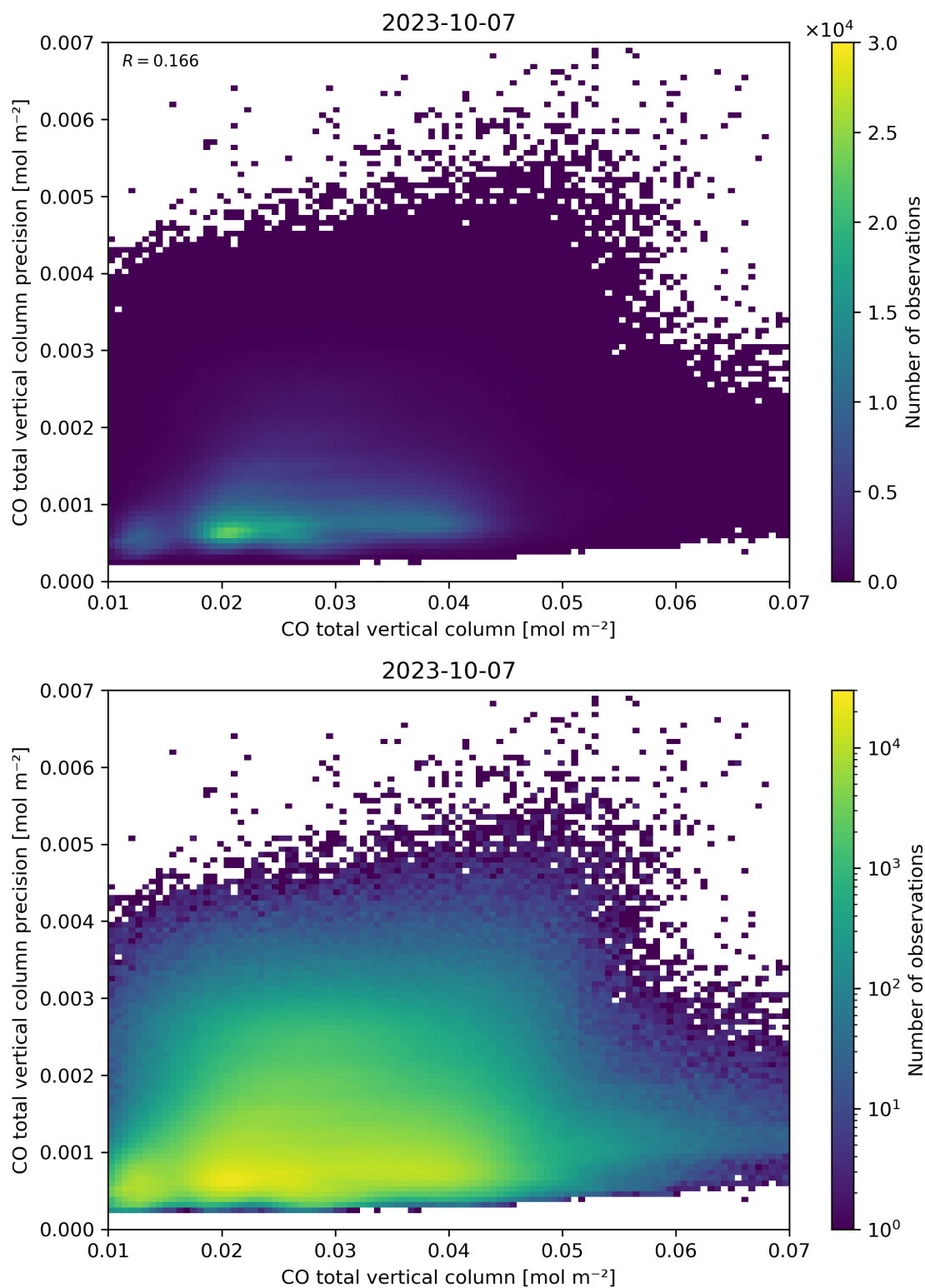
Figure 34: Scatter density plot of “CO total vertical column” against “CO total vertical column precision” for 2023-10-06 to 2023-10-08.
