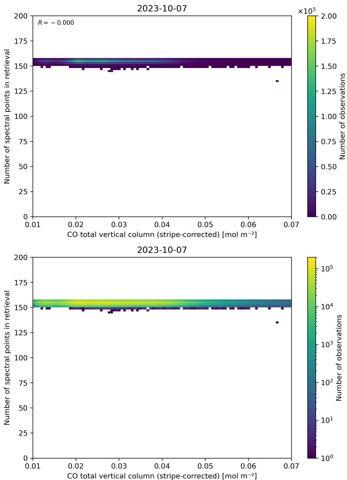
Figure 40: Scatter density plot of “CO total vertical column (stripe-corrected)” against “Number of spectral points in retrieval” for 2023-10-06 to 2023-10-08.
