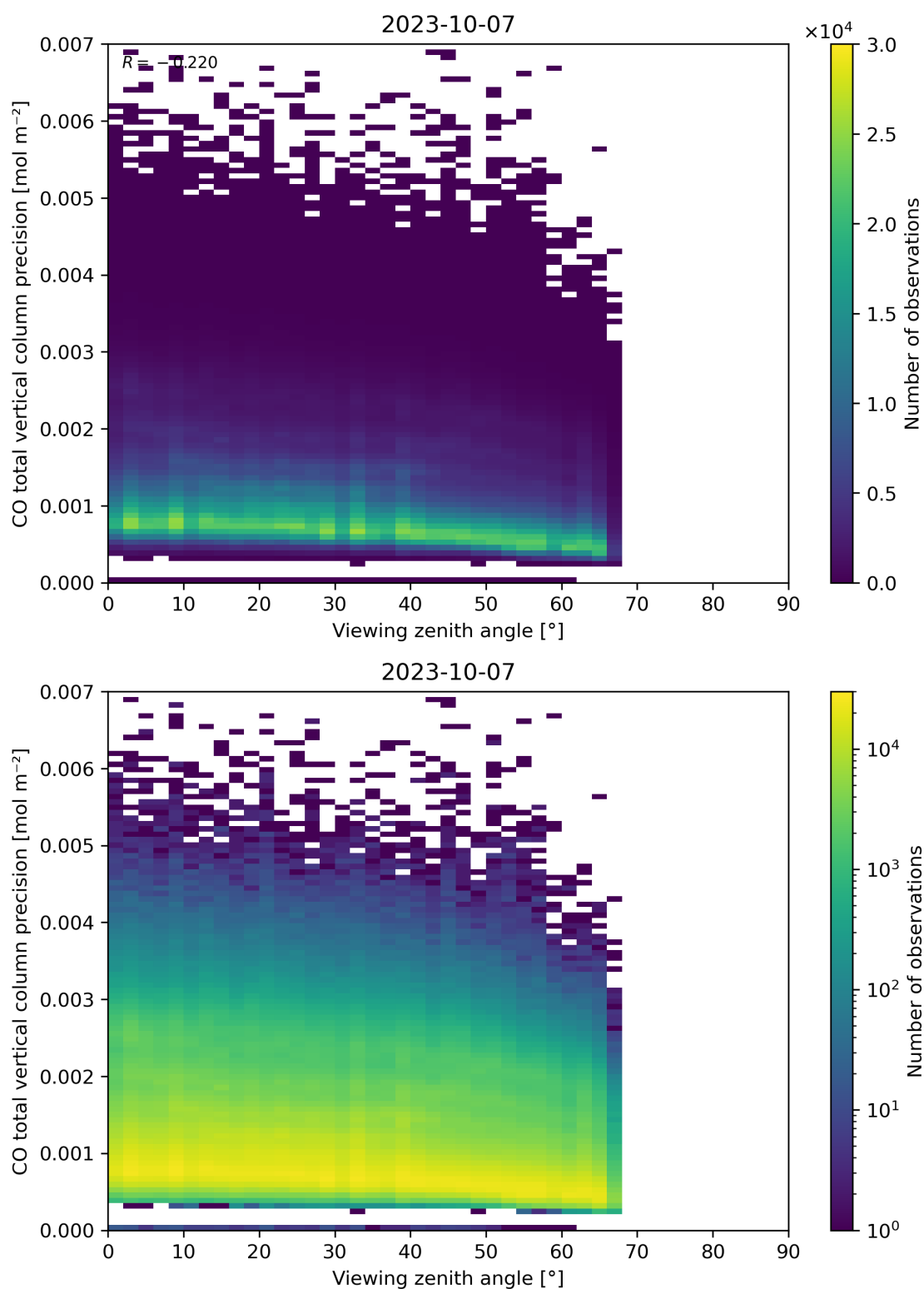
Figure 71: Scatter density plot of “Viewing zenith angle” against “CO total vertical column precision” for 2023-10-06 to 2023-10-08.
