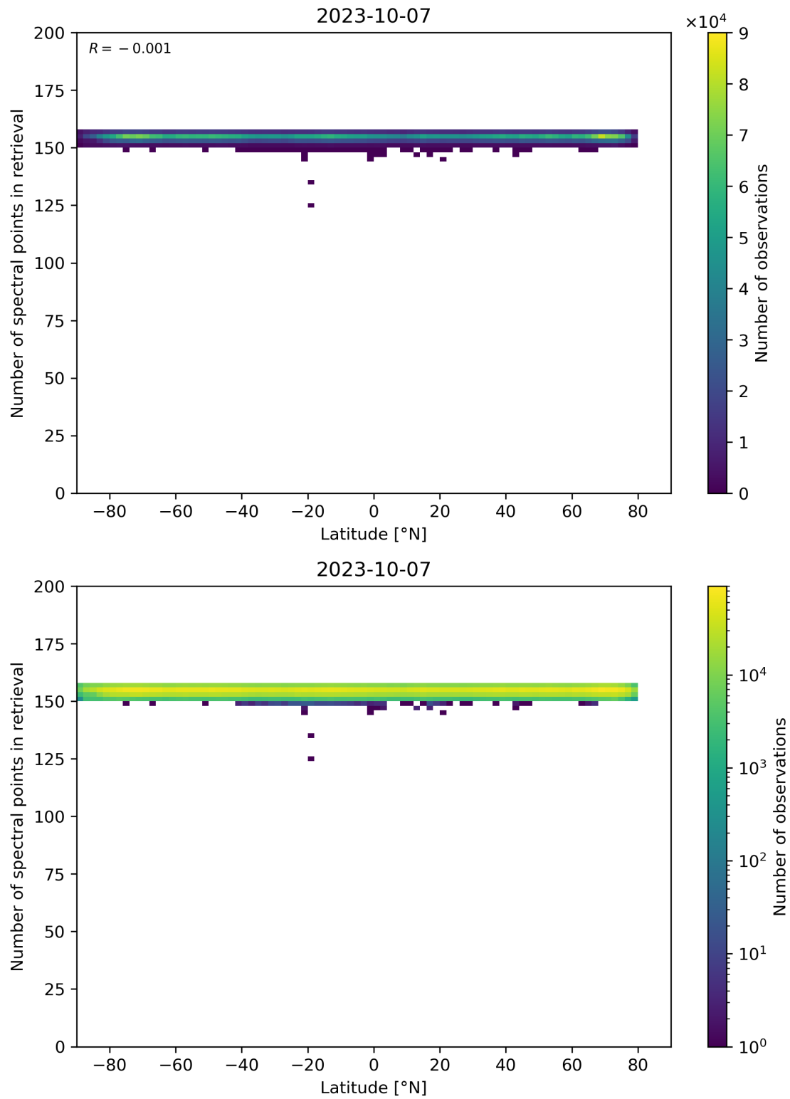
Figure 57: Scatter density plot of “Latitude” against “Number of spectral points in retrieval” for 2023-10-06 to 2023-10-08.
