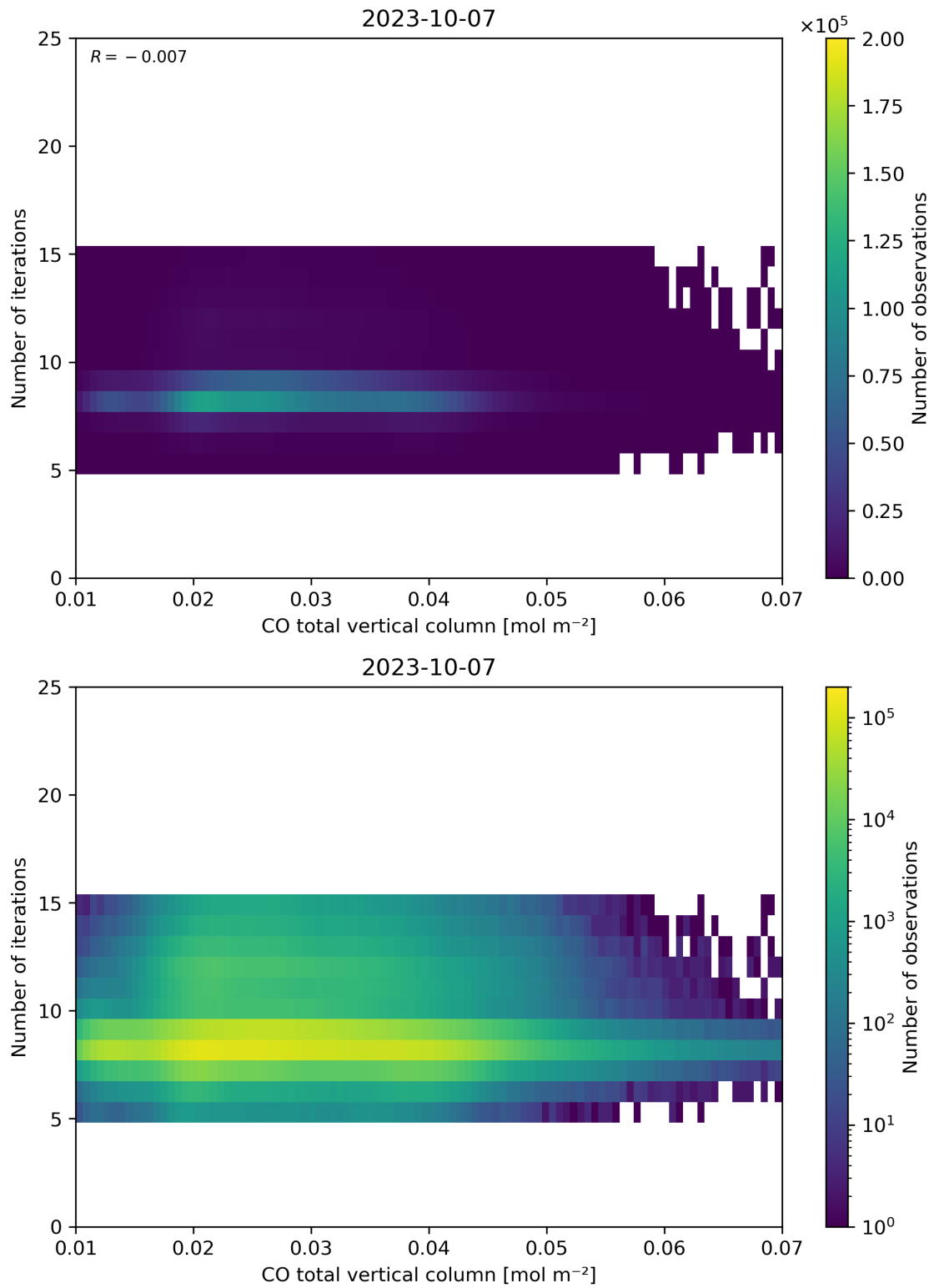
Figure 42: Scatter density plot of “CO total vertical column” against “Number of iterations” for 2023-10-06 to 2023-10-08.
