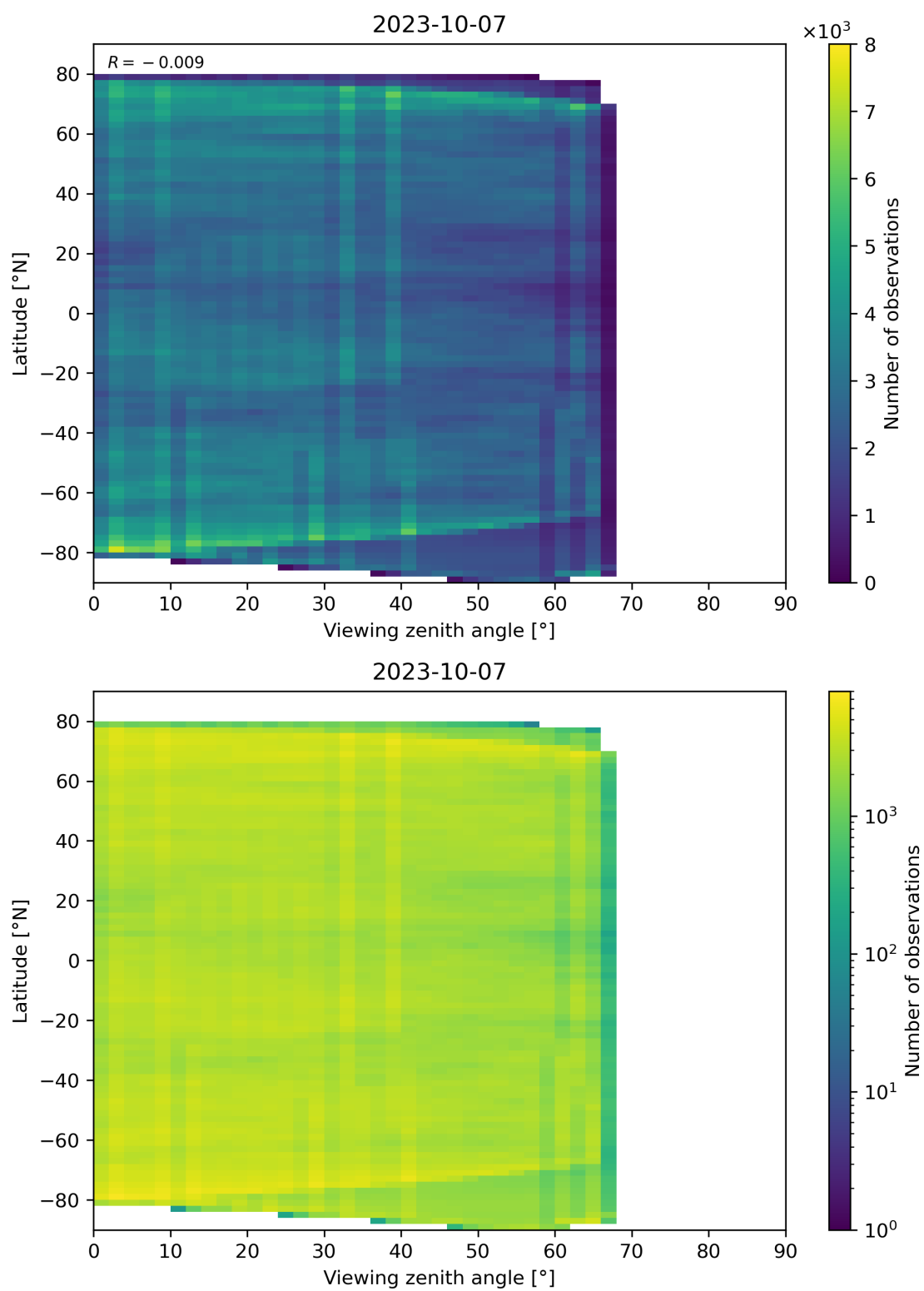
Figure 74: Scatter density plot of “Viewing zenith angle” against “Latitude” for 2023-10-06 to 2023-10-08.
