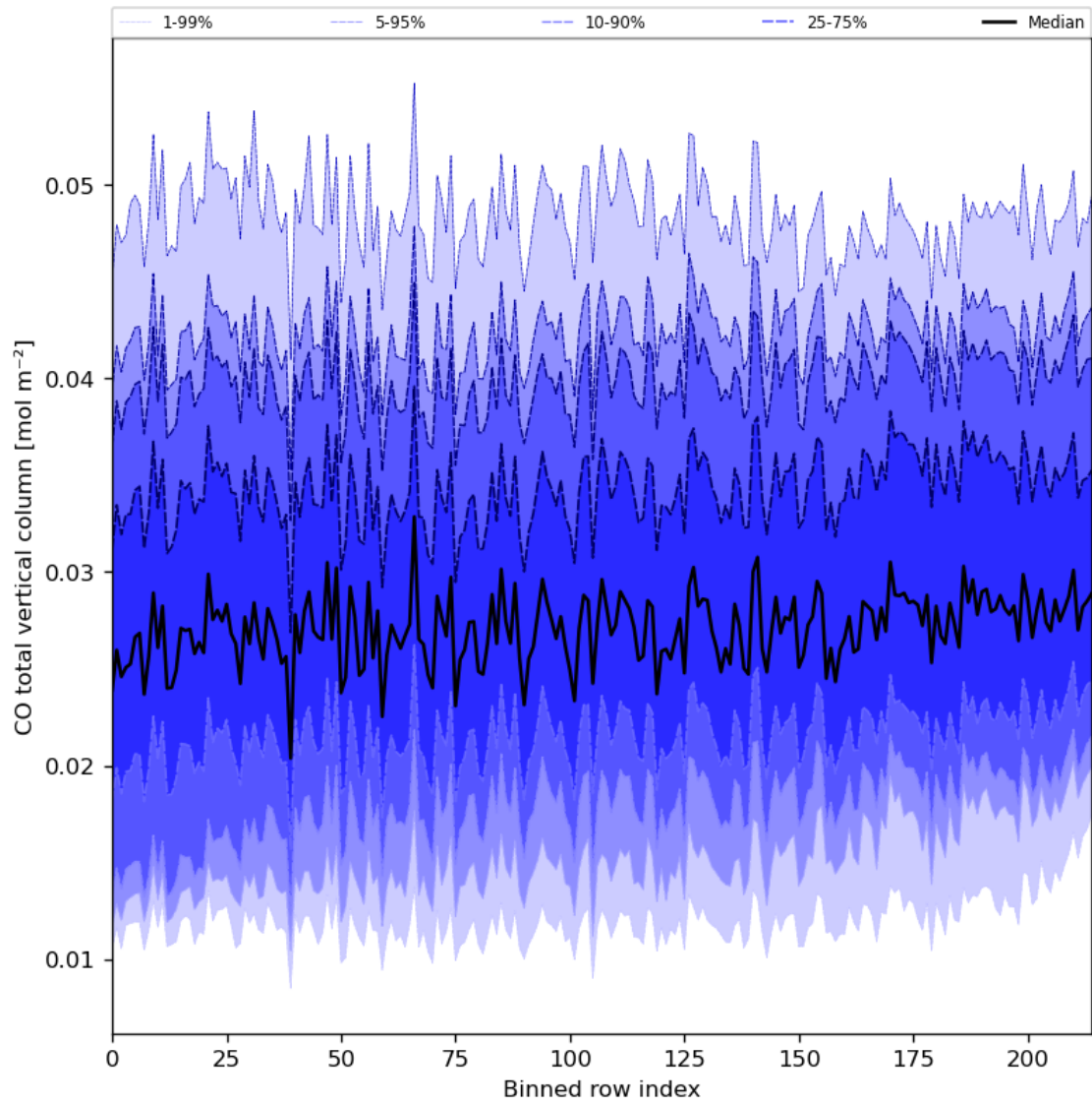
Figure 26: Along track statistics of “CO total vertical column” for 2023-10-06 to 2023-10-08
