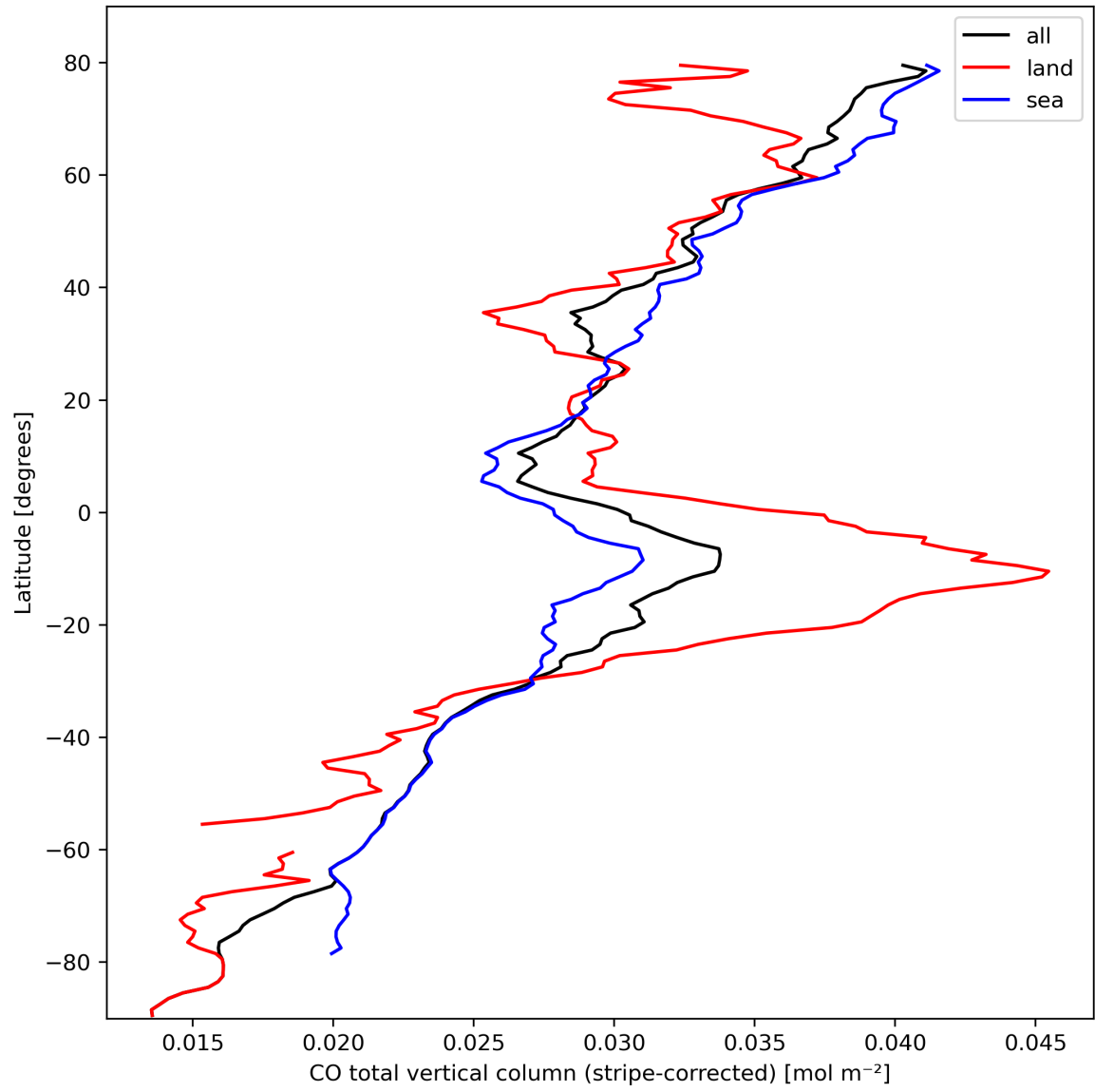
Figure 11: Zonal average of “CO total vertical column (stripe-corrected)” for 2023-10-06 to 2023-10-08.
