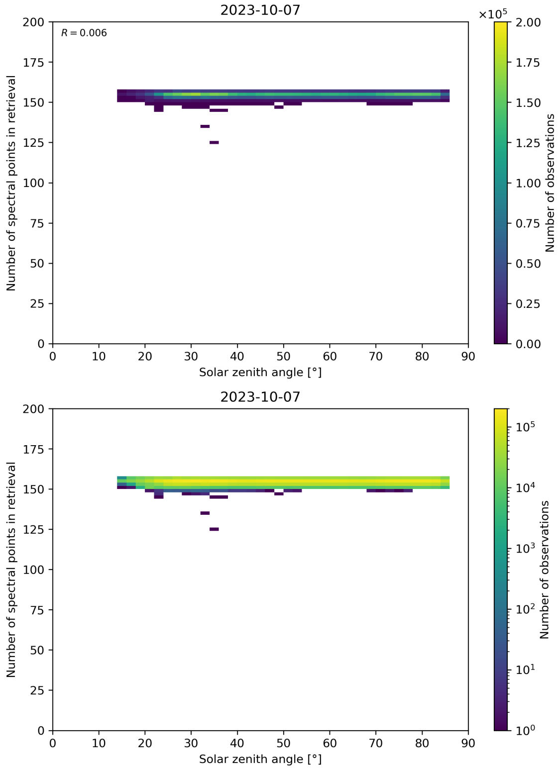
Figure 68: Scatter density plot of “Solar zenith angle” against “Number of spectral points in retrieval” for 2023-10-06 to 2023-10-08.
