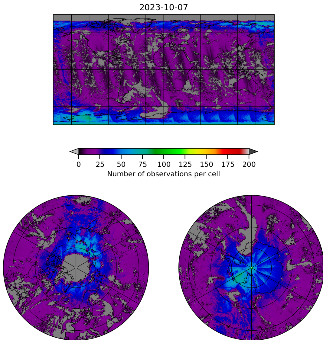
Figure 8: Map of the number of observations for 2023-10-06 to 2023-10-08
