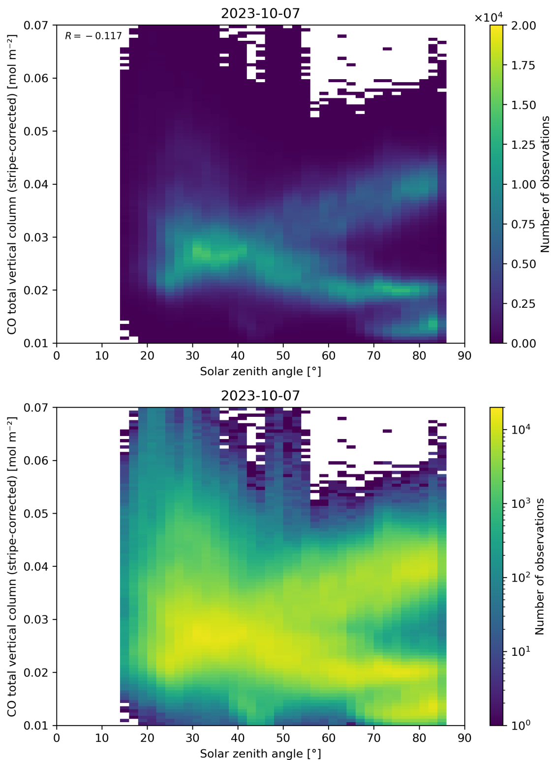
Figure 62: Scatter density plot of “Solar zenith angle” against “CO total vertical column (stripe-corrected)” for 2023-10-06 to 2023-10-08.
