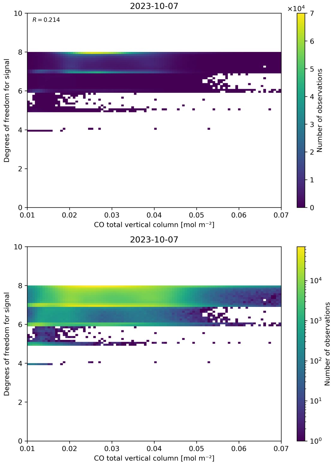
Figure 41: Scatter density plot of “CO total vertical column” against “Degrees of freedom for signal” for 2023-10-06 to 2023-10-08.
