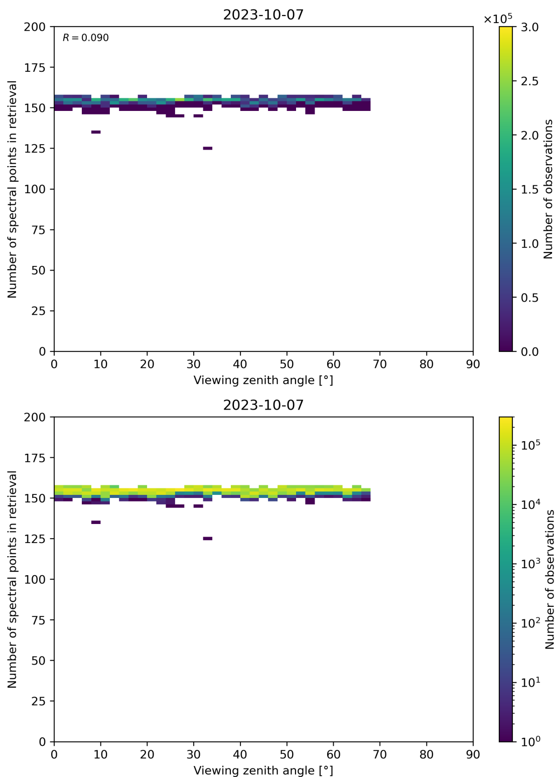
Figure 76: Scatter density plot of “Viewing zenith angle” against “Number of spectral points in retrieval” for 2023-10-06 to 2023-10-08.
