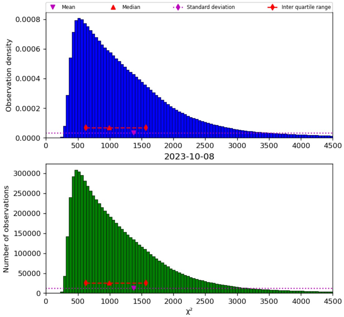
Figure 22: Histogram of “ \chi^2 ” for 2023-10-07 to 2023-10-09
