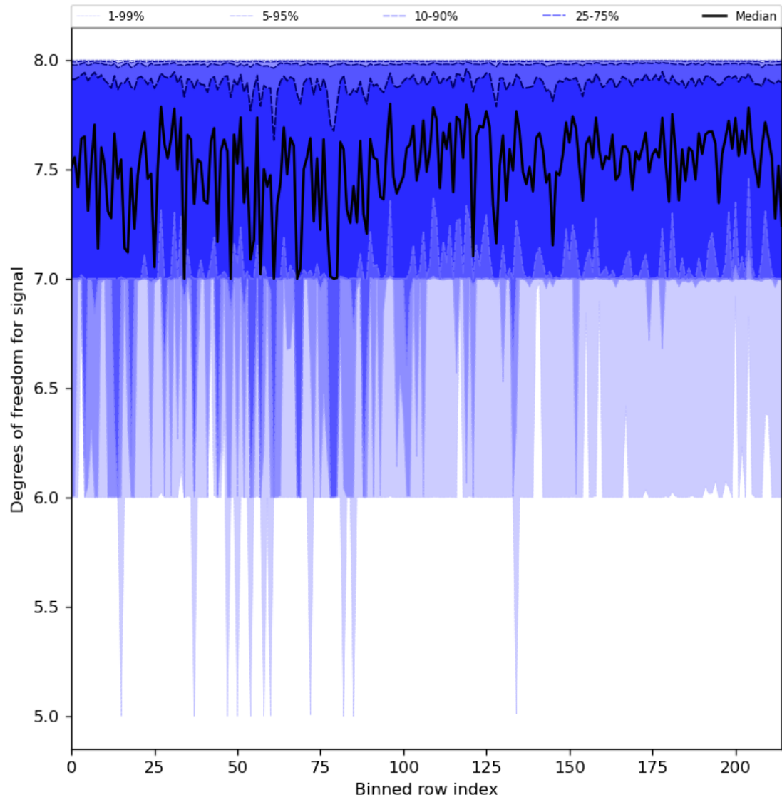
Figure 31: Along track statistics of “Degrees of freedom for signal” for 2023-10-07 to 2023-10-09
