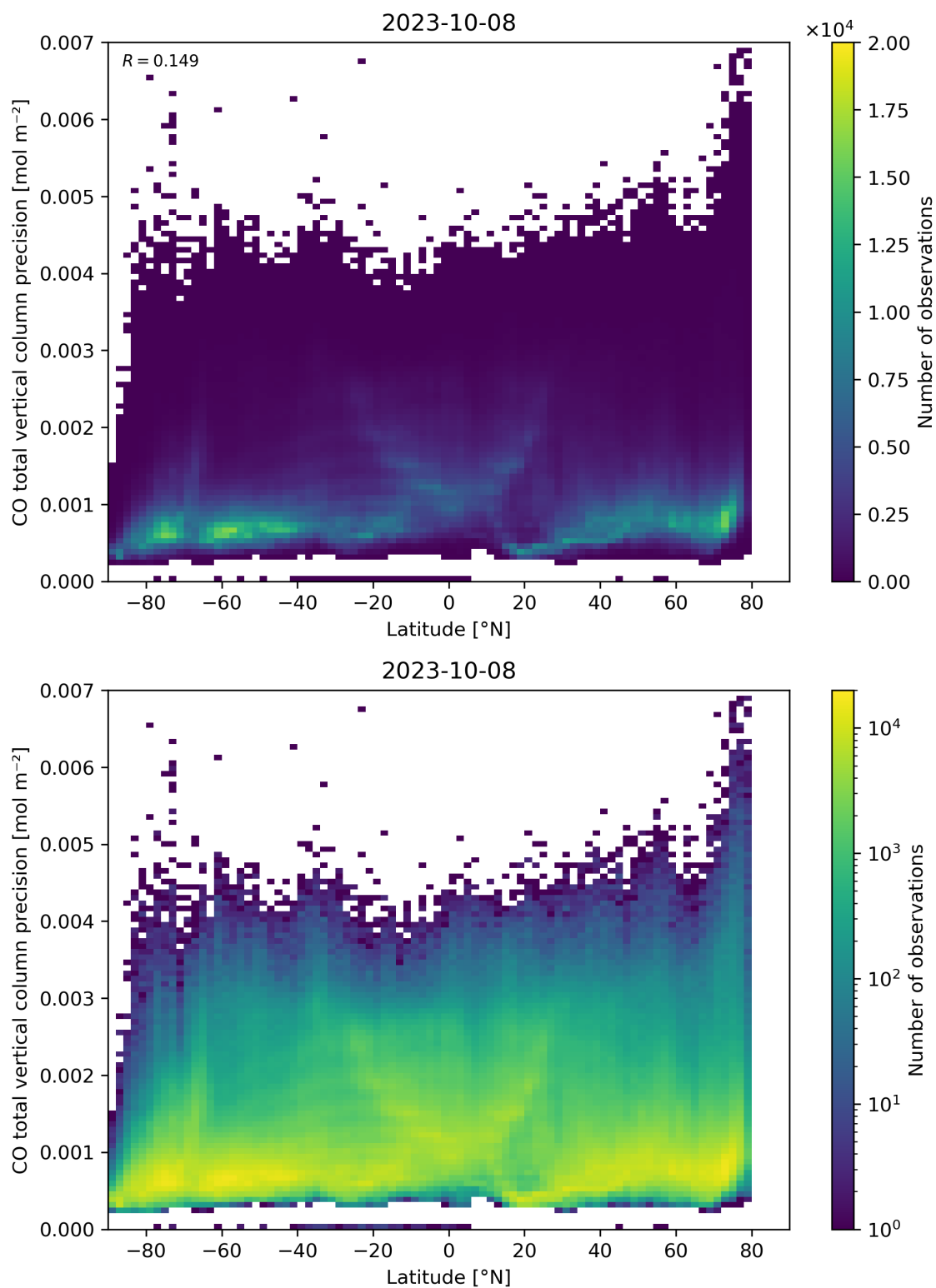
Figure 53: Scatter density plot of “Latitude” against “CO total vertical column precision” for 2023-10-07 to 2023-10-09.
