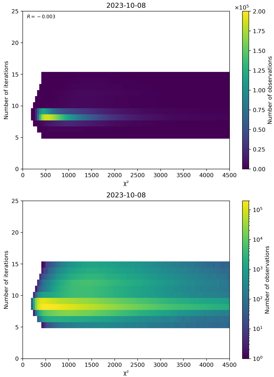
Figure 49: Scatter density plot of “ \chi^2 ” against “Number of iterations” for 2023-10-07 to 2023-10-09.
