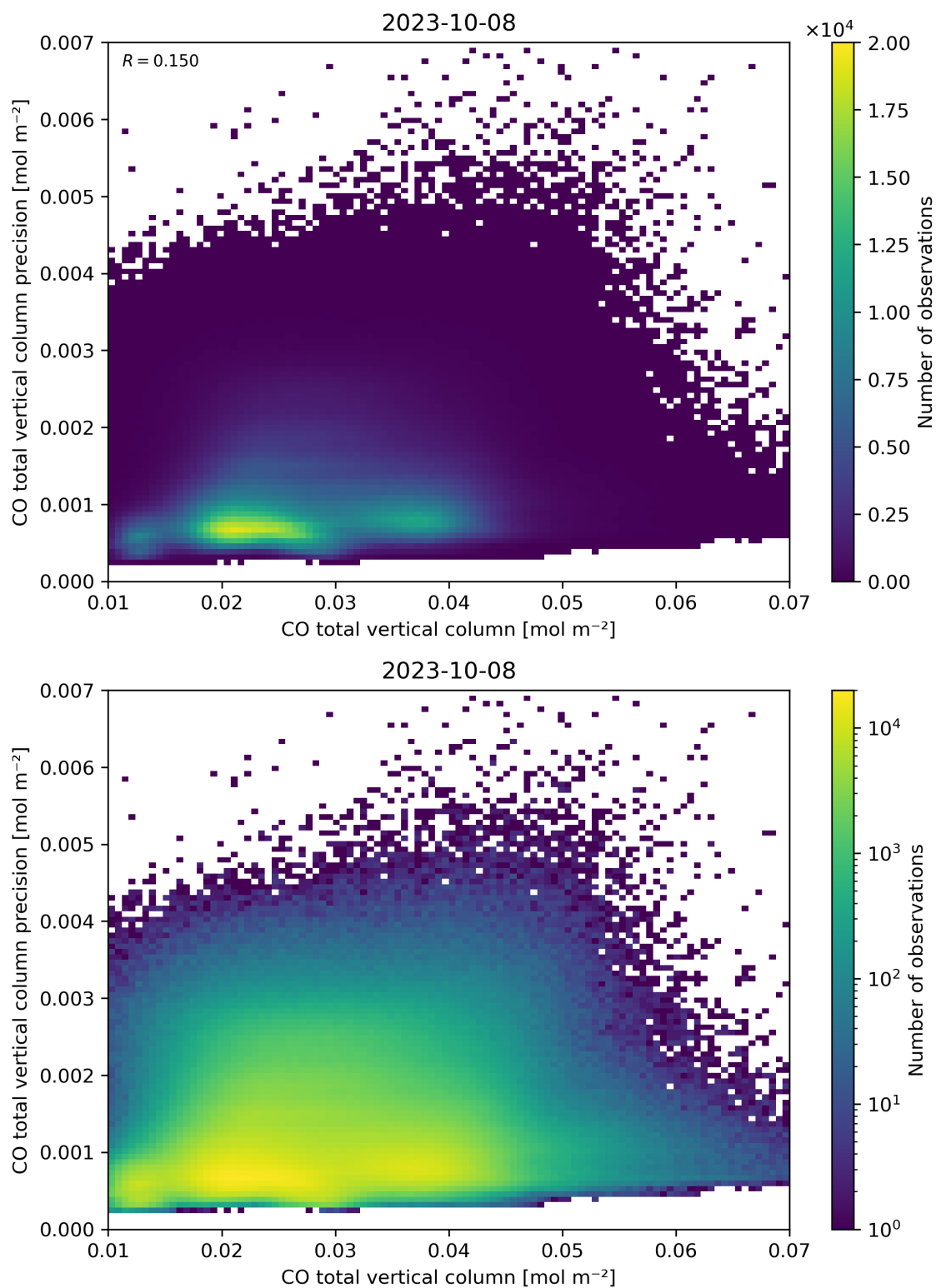
Figure 34: Scatter density plot of “CO total vertical column” against “CO total vertical column precision” for 2023-10-07 to 2023-10-09.
