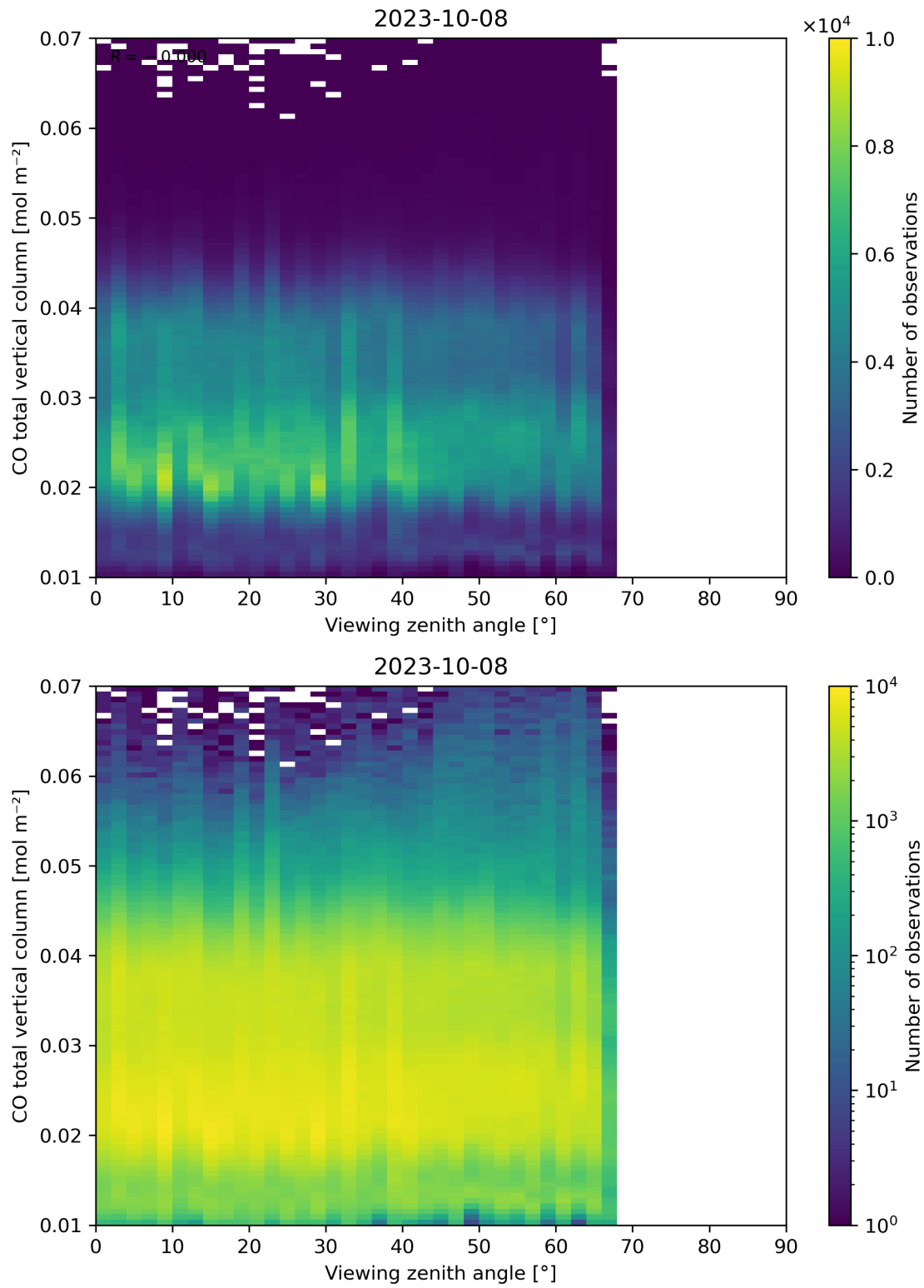
Figure 69: Scatter density plot of “Viewing zenith angle” against “CO total vertical column” for 2023-10-07 to 2023-10-09.
