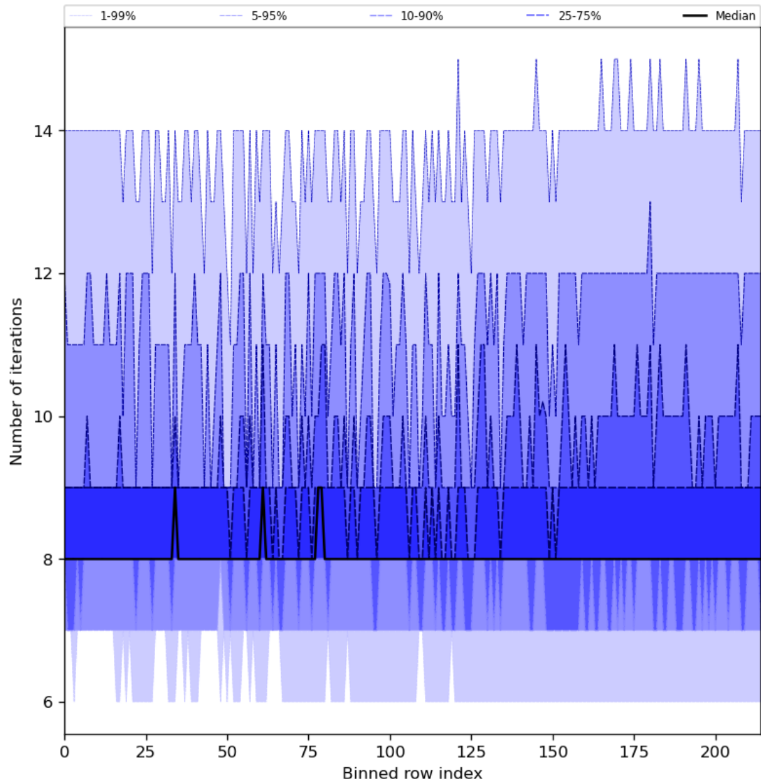
Figure 32: Along track statistics of “Number of iterations” for 2023-10-07 to 2023-10-09
