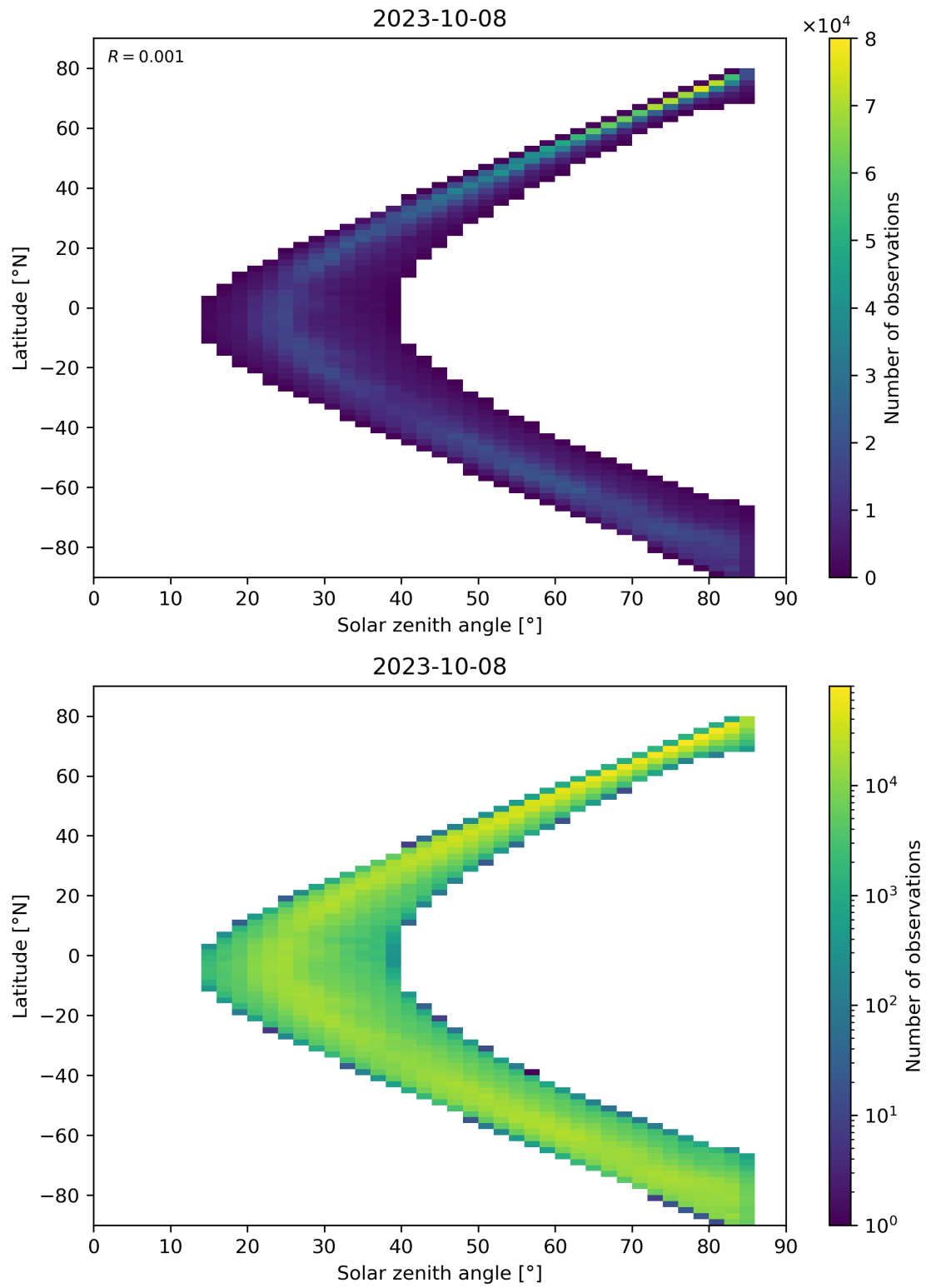
Figure 66: Scatter density plot of “Solar zenith angle” against “Latitude” for 2023-10-07 to 2023-10-09.
