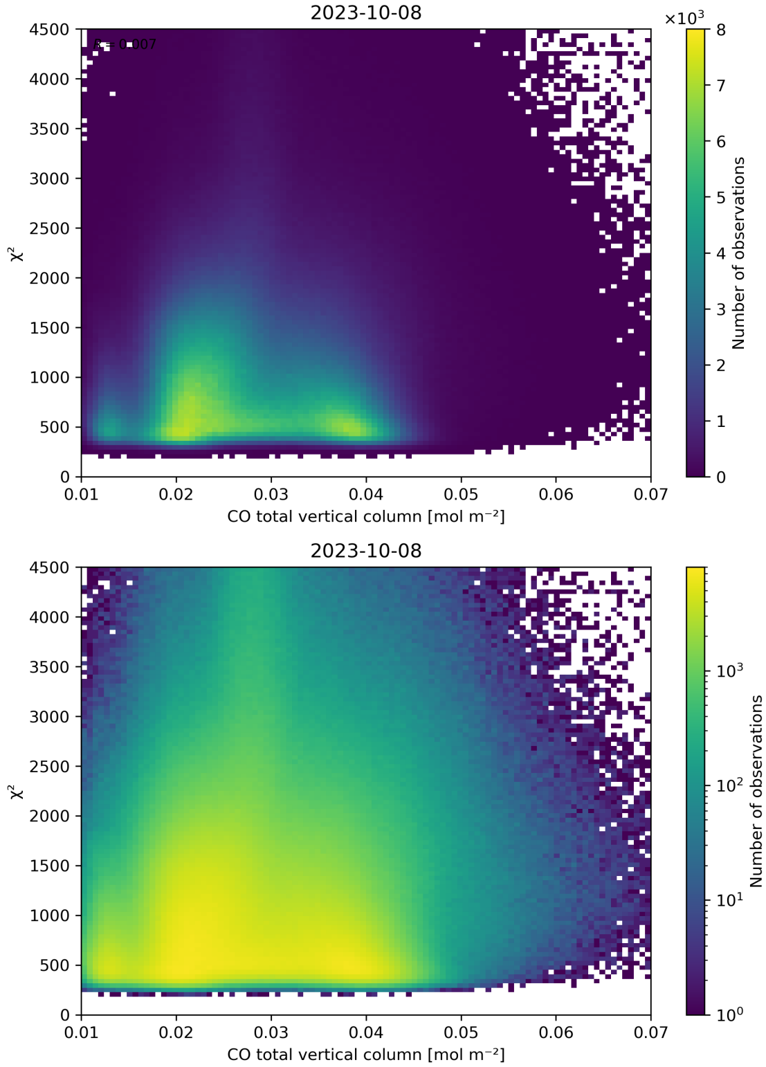
Figure 35: Scatter density plot of “CO total vertical column” against “ \chi^2 ” for 2023-10-07 to 2023-10-09.
