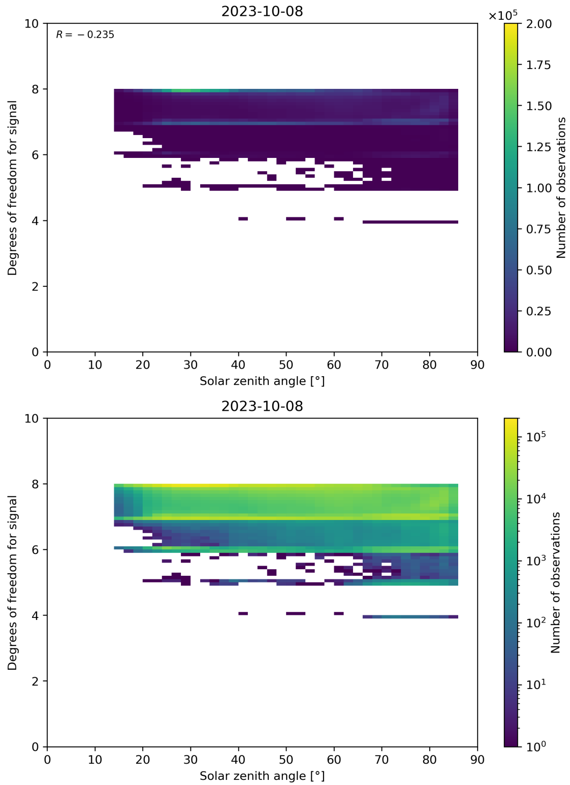
Figure 65: Scatter density plot of “Solar zenith angle” against “Degrees of freedom for signal” for 2023-10-07 to 2023-10-09.
