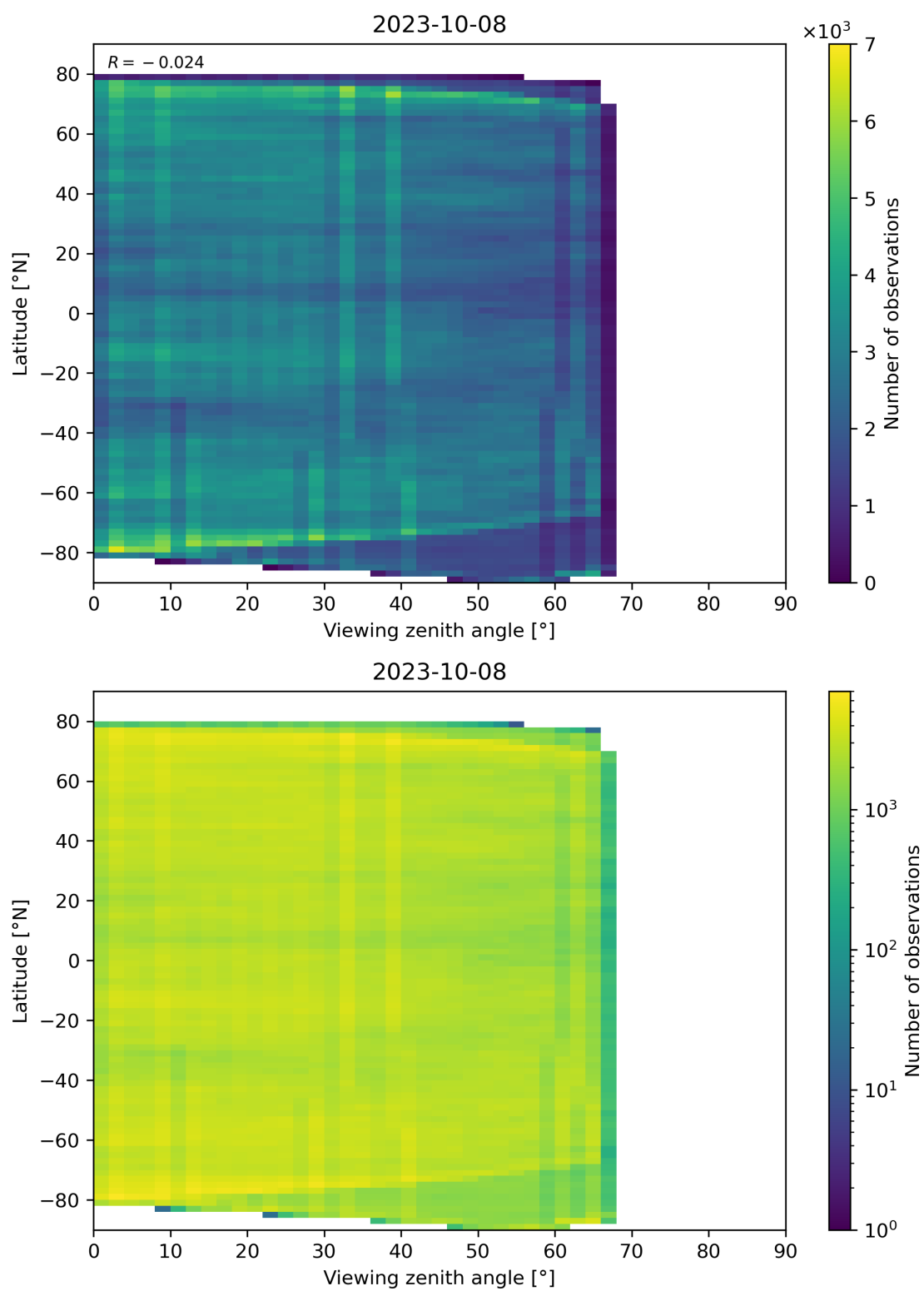
Figure 74: Scatter density plot of “Viewing zenith angle” against “Latitude” for 2023-10-07 to 2023-10-09.
