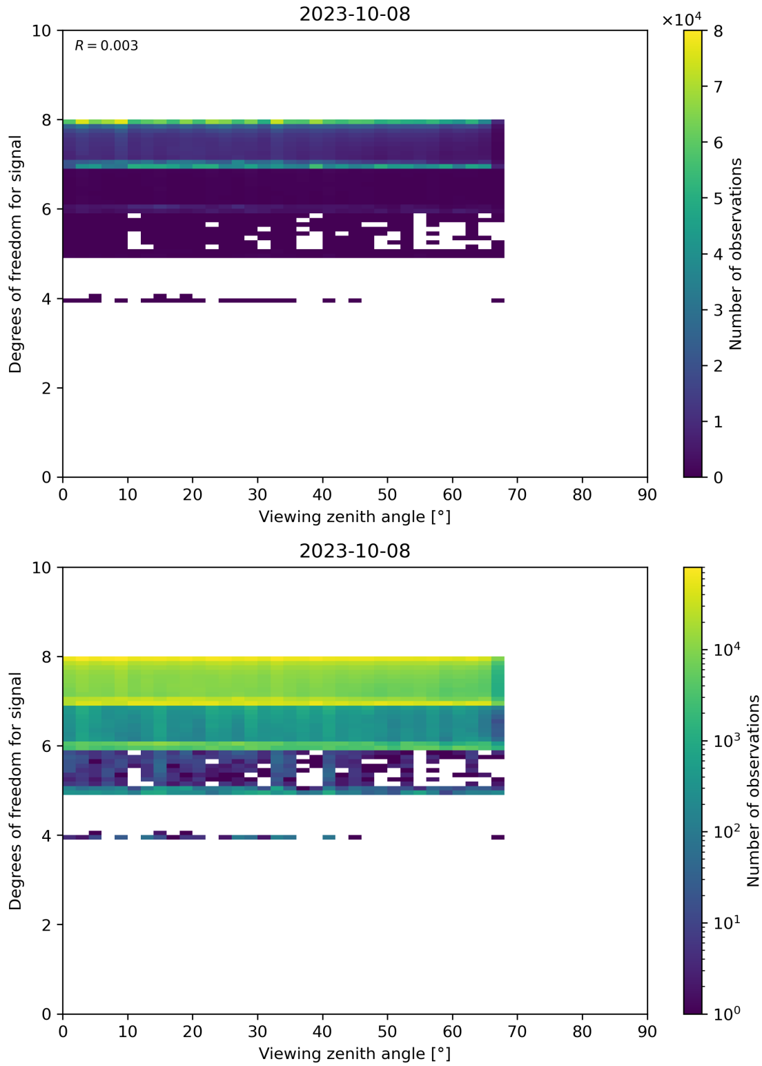
Figure 73: Scatter density plot of “Viewing zenith angle” against “Degrees of freedom for signal” for 2023-10-07 to 2023-10-09.
