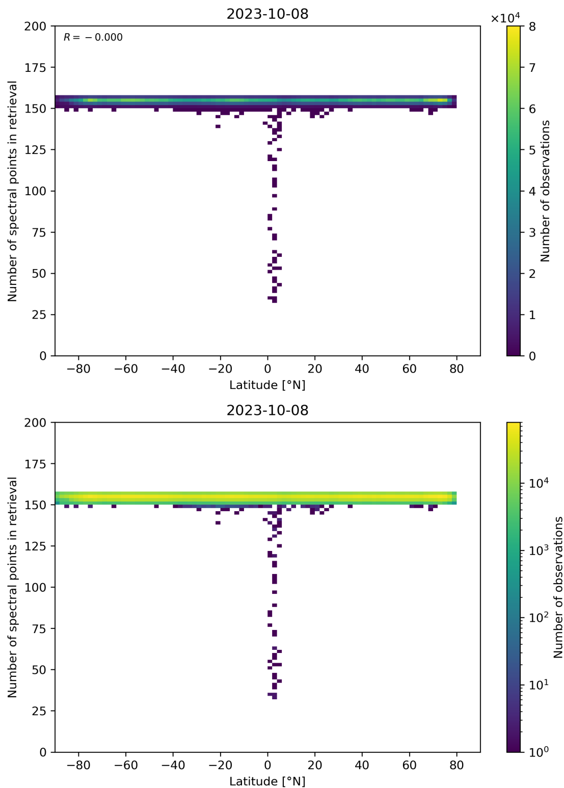
Figure 57: Scatter density plot of “Latitude” against “Number of spectral points in retrieval” for 2023-10-07 to 2023-10-09.
