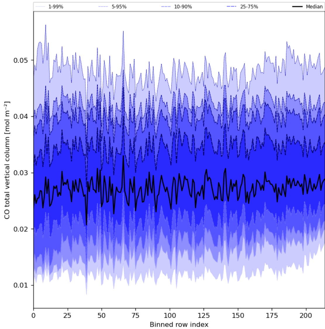
Figure 26: Along track statistics of “CO total vertical column” for 2023-10-07 to 2023-10-09
