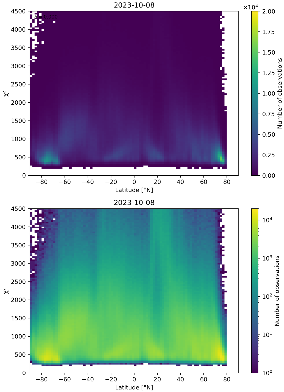
Figure 54: Scatter density plot of “Latitude” against “ \chi^2 ” for 2023-10-07 to 2023-10-09.
