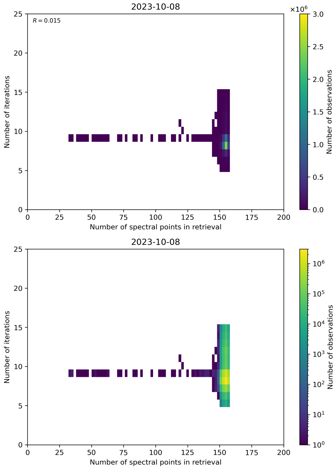
Figure 60: Scatter density plot of “Number of spectral points in retrieval” against “Number of iterations” for 2023-10-07 to 2023-10-09.
