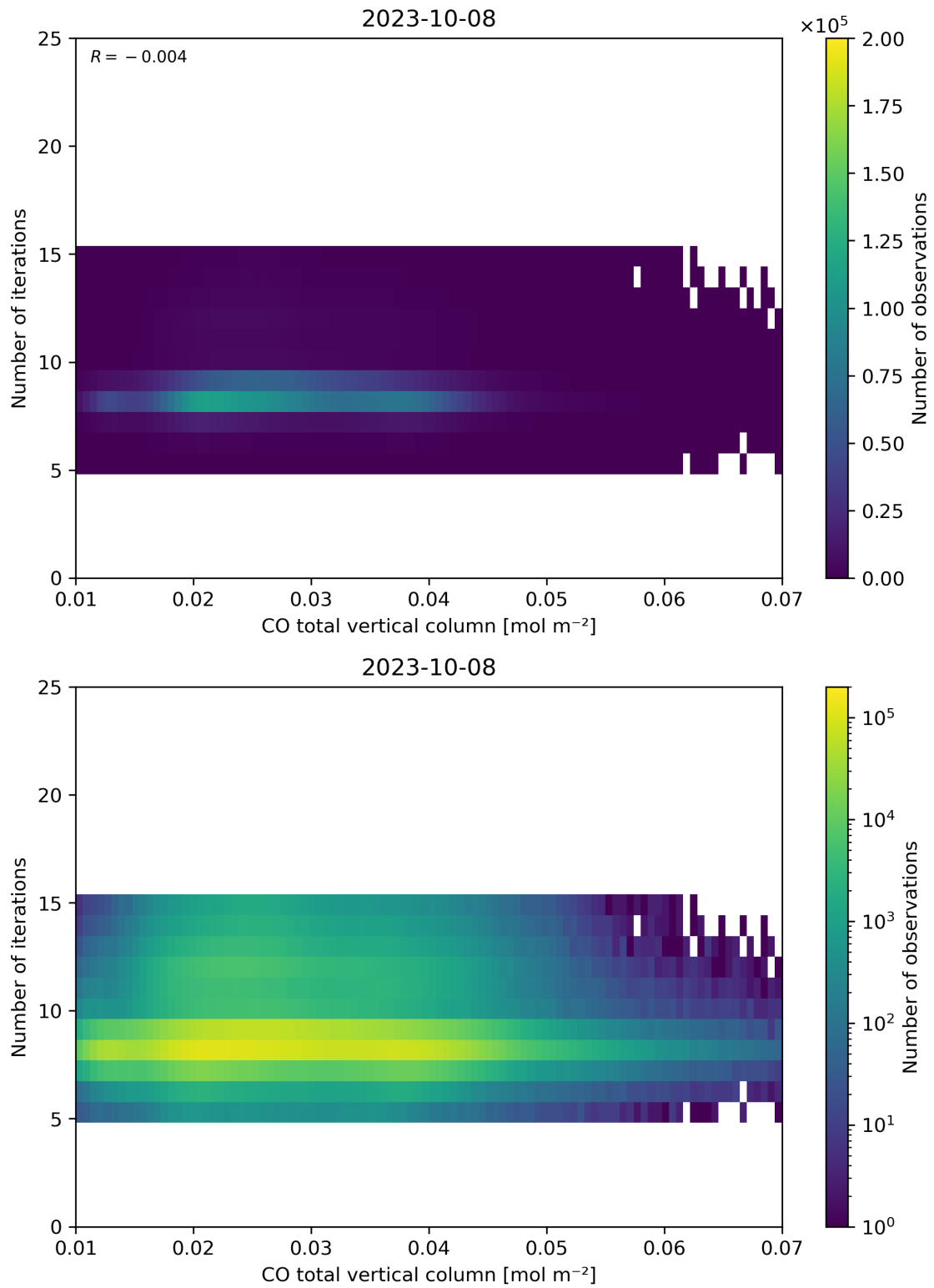
Figure 42: Scatter density plot of “CO total vertical column” against “Number of iterations” for 2023-10-07 to 2023-10-09.
