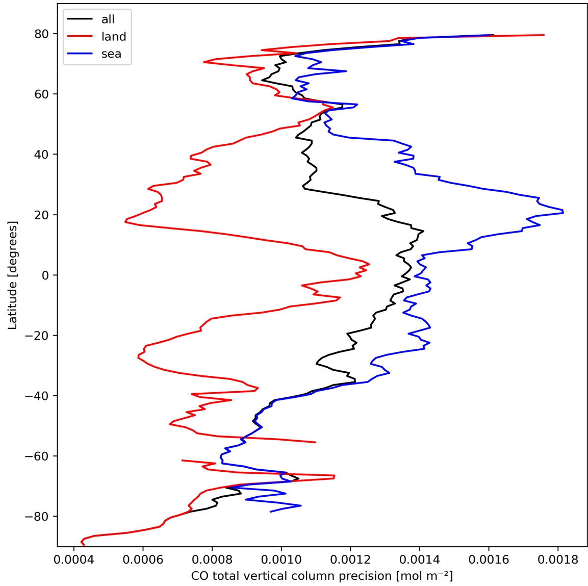
Figure 12: Zonal average of “CO total vertical column precision” for 2023-10-07 to 2023-10-09.
