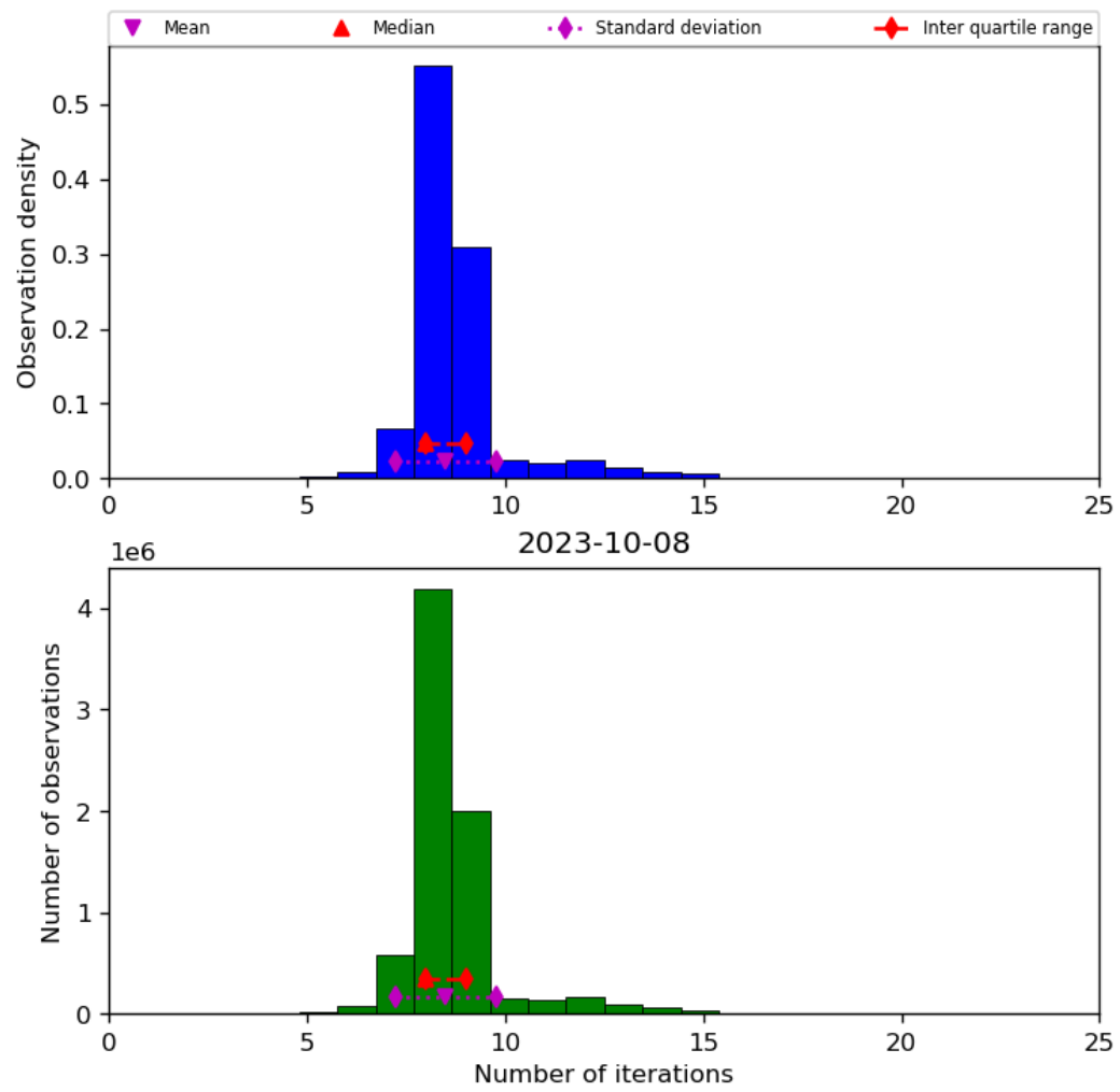
Figure 24: Histogram of “Number of iterations” for 2023-10-07 to 2023-10-09
