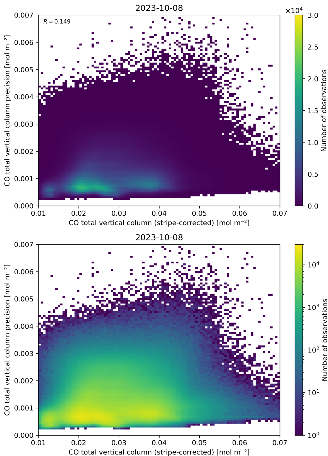
Figure 36: Scatter density plot of “CO total vertical column (stripe-corrected)” against “CO total vertical column precision” for 2023-10-07 to 2023-10-09.
