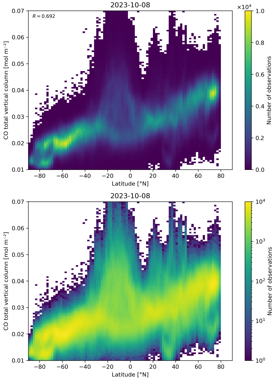
Figure 51: Scatter density plot of “Latitude” against “CO total vertical column” for 2023-10-07 to 2023-10-09.
