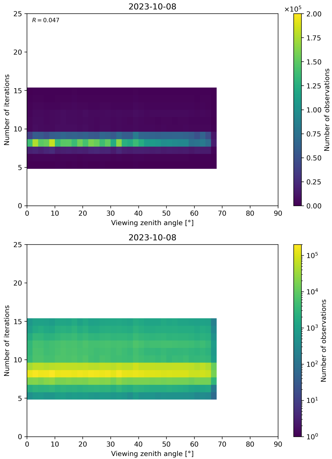
Figure 75: Scatter density plot of “Viewing zenith angle” against “Number of iterations” for 2023-10-07 to 2023-10-09.
