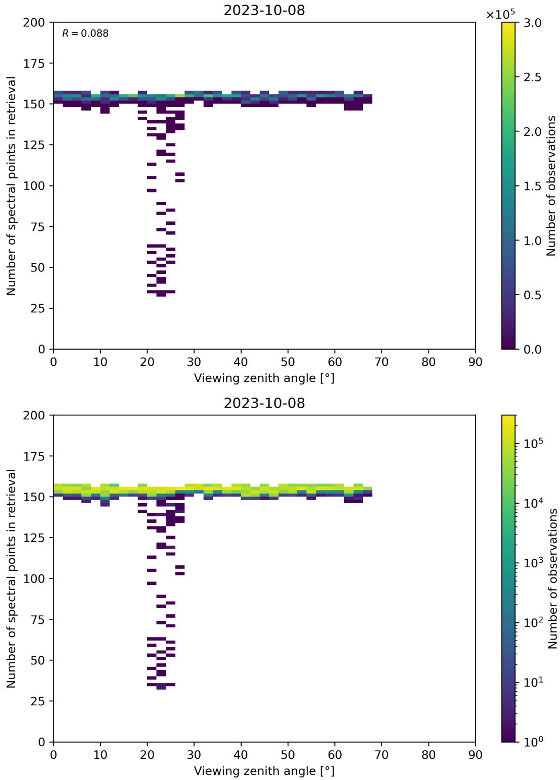
Figure 76: Scatter density plot of “Viewing zenith angle” against “Number of spectral points in retrieval” for 2023-10-07 to 2023-10-09.
