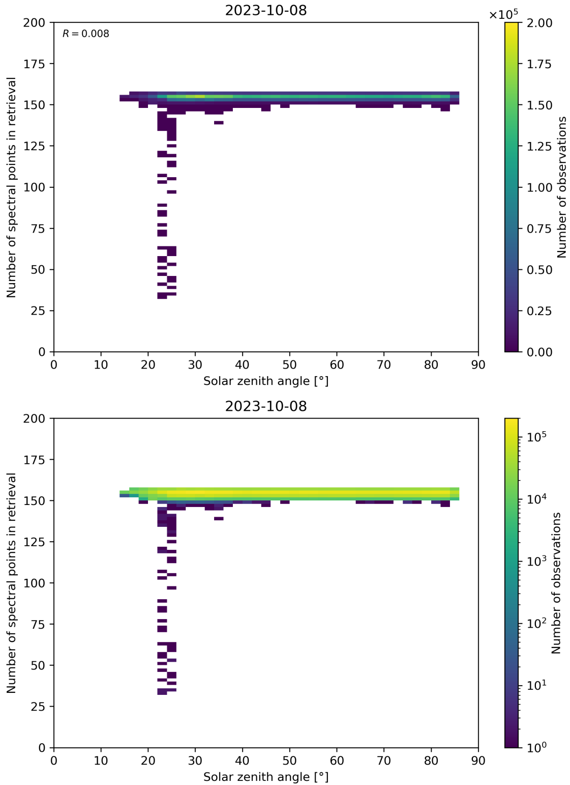
Figure 68: Scatter density plot of “Solar zenith angle” against “Number of spectral points in retrieval” for 2023-10-07 to 2023-10-09.
