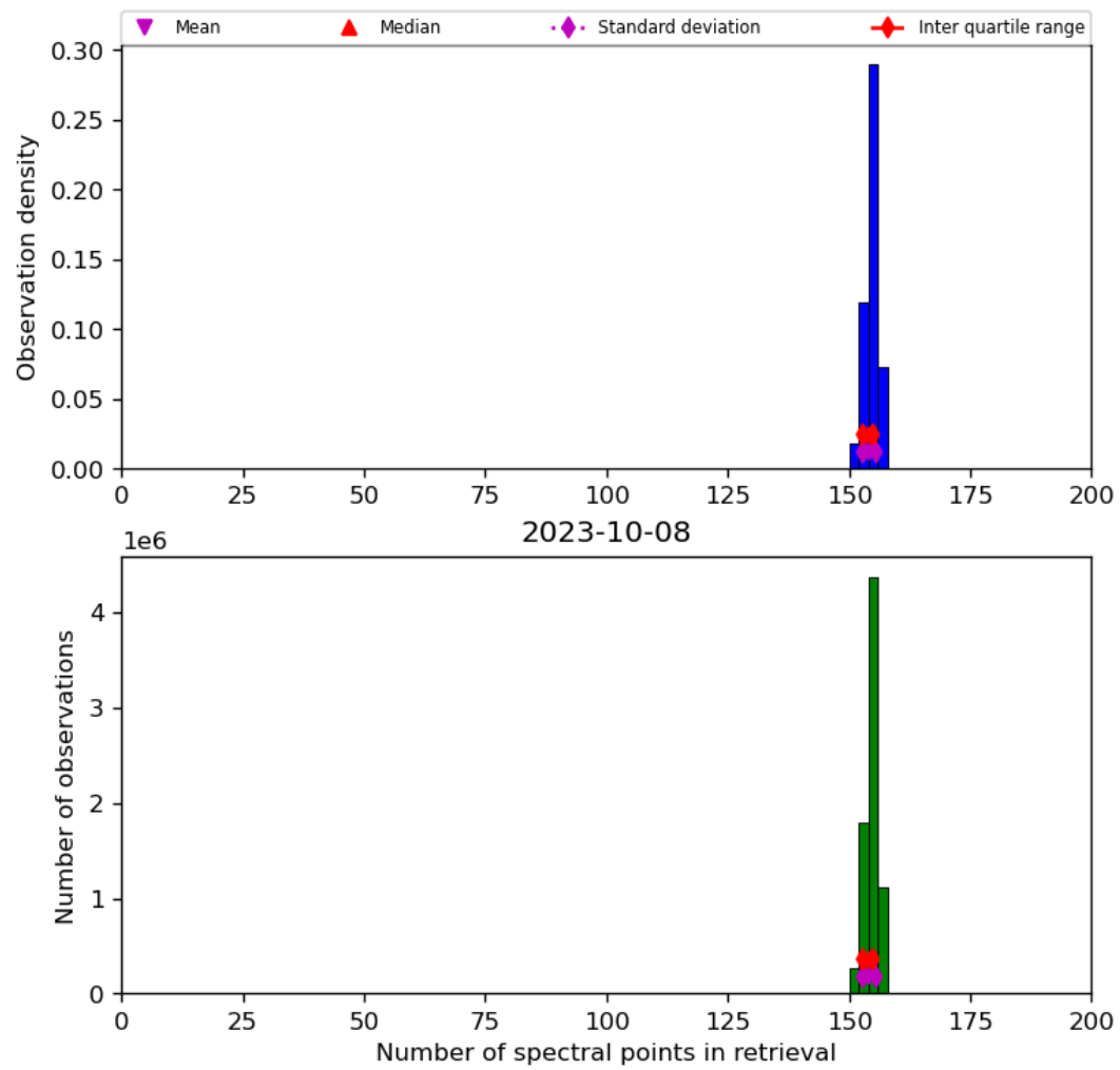
Figure 21: Histogram of “Number of spectral points in retrieval” for 2023-10-07 to 2023-10-09
