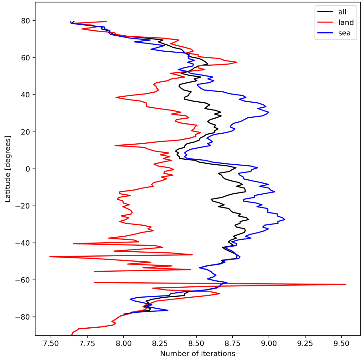
Figure 16: Zonal average of “Number of iterations” for 2023-10-07 to 2023-10-09.
