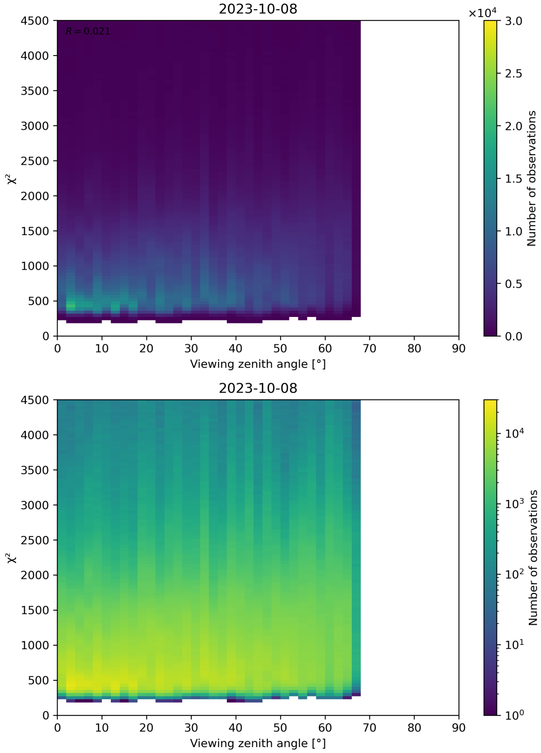
Figure 72: Scatter density plot of “Viewing zenith angle” against “ \chi^2 ” for 2023-10-07 to 2023-10-09.
