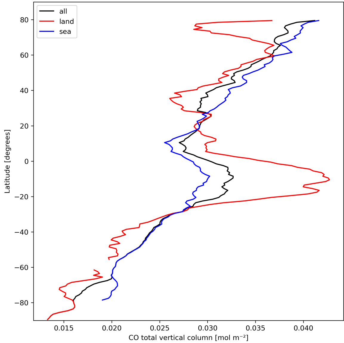
Figure 10: Zonal average of “CO total vertical column” for 2023-10-07 to 2023-10-09.
