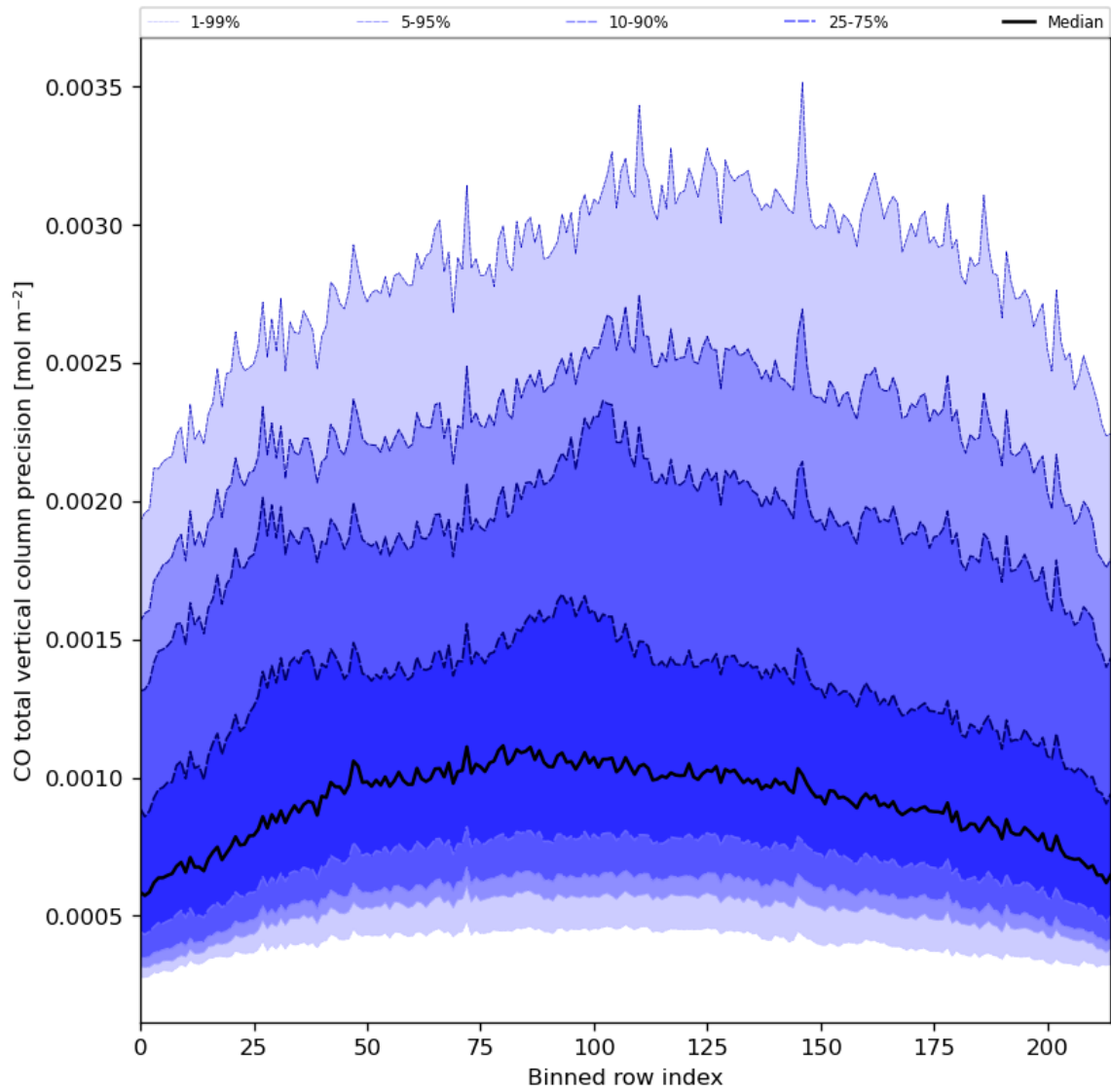
Figure 28: Along track statistics of “CO total vertical column precision” for 2023-10-07 to 2023-10-09
