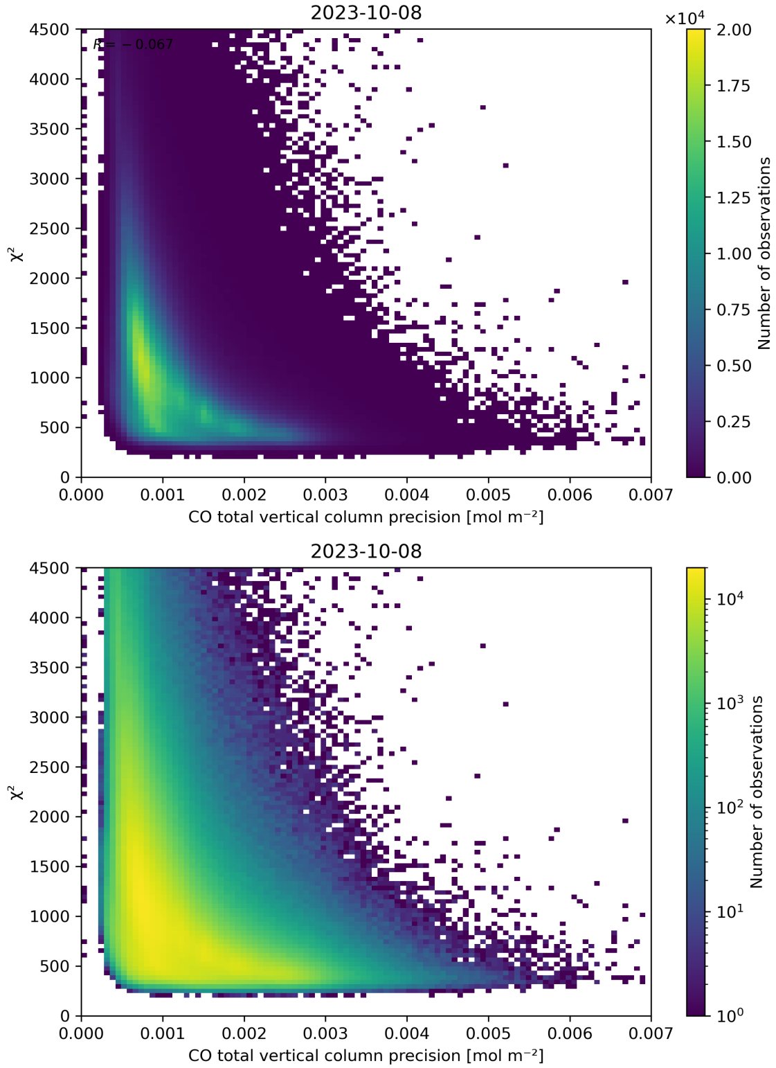
Figure 44: Scatter density plot of “CO total vertical column precision” against “ \chi^2 ” for 2023-10-07 to 2023-10-09.
