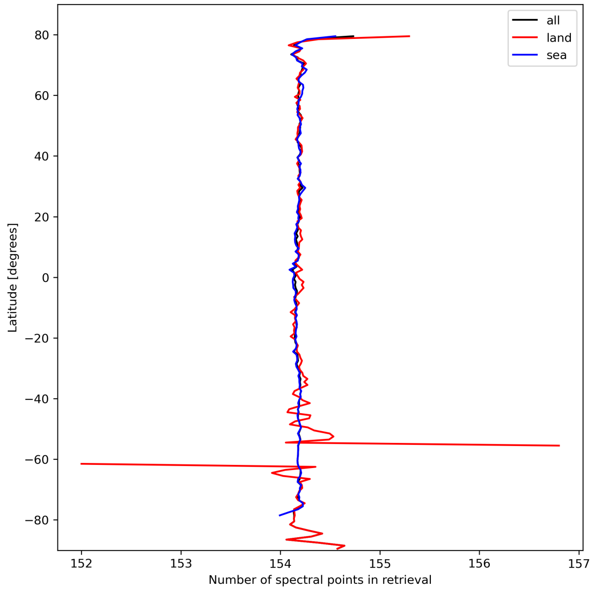
Figure 13: Zonal average of “Number of spectral points in retrieval” for 2023-10-07 to 2023-10-09.
