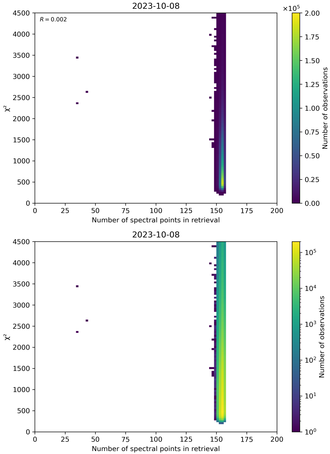
Figure 58: Scatter density plot of “Number of spectral points in retrieval” against “ \chi^2 ” for 2023-10-07 to 2023-10-09.
