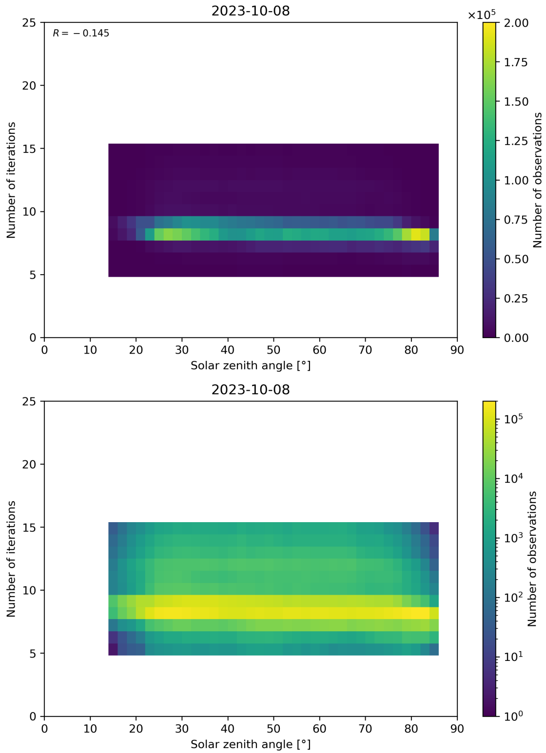
Figure 67: Scatter density plot of “Solar zenith angle” against “Number of iterations” for 2023-10-07 to 2023-10-09.
