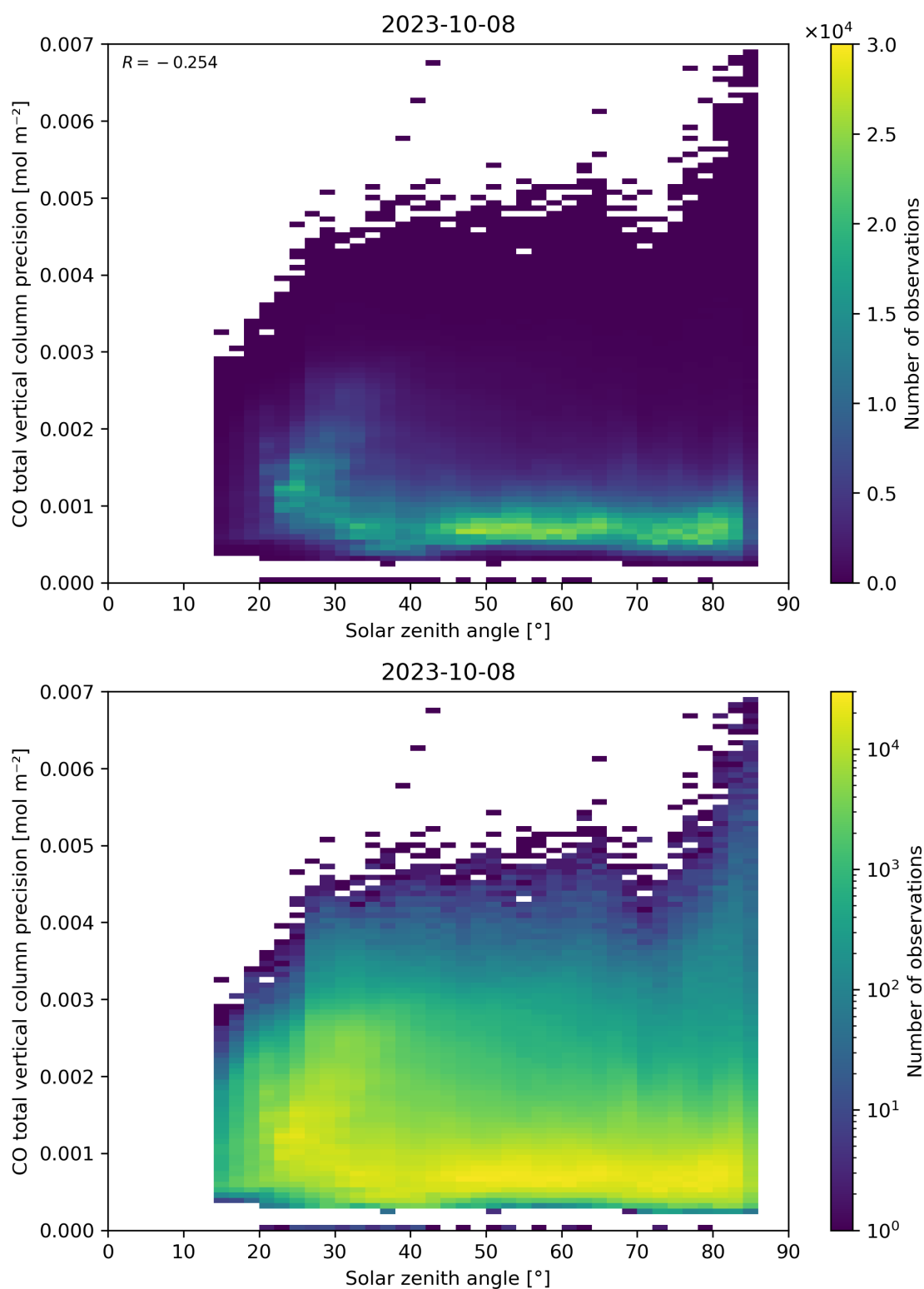
Figure 63: Scatter density plot of “Solar zenith angle” against “CO total vertical column precision” for 2023-10-07 to 2023-10-09.
