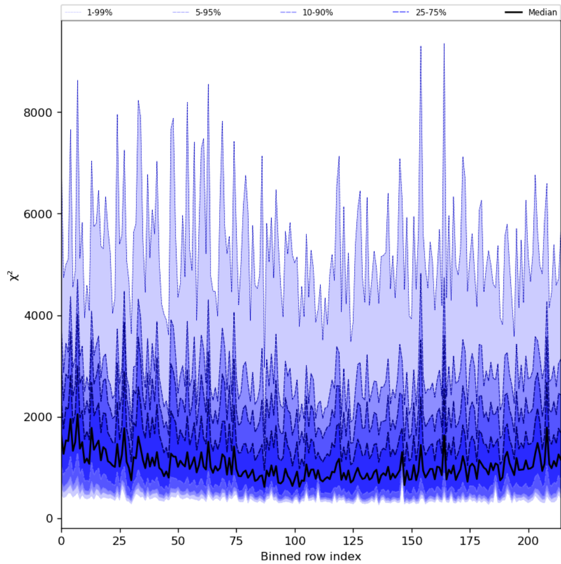
Figure 30: Along track statistics of “ \chi^2 ” for 2023-10-07 to 2023-10-09
