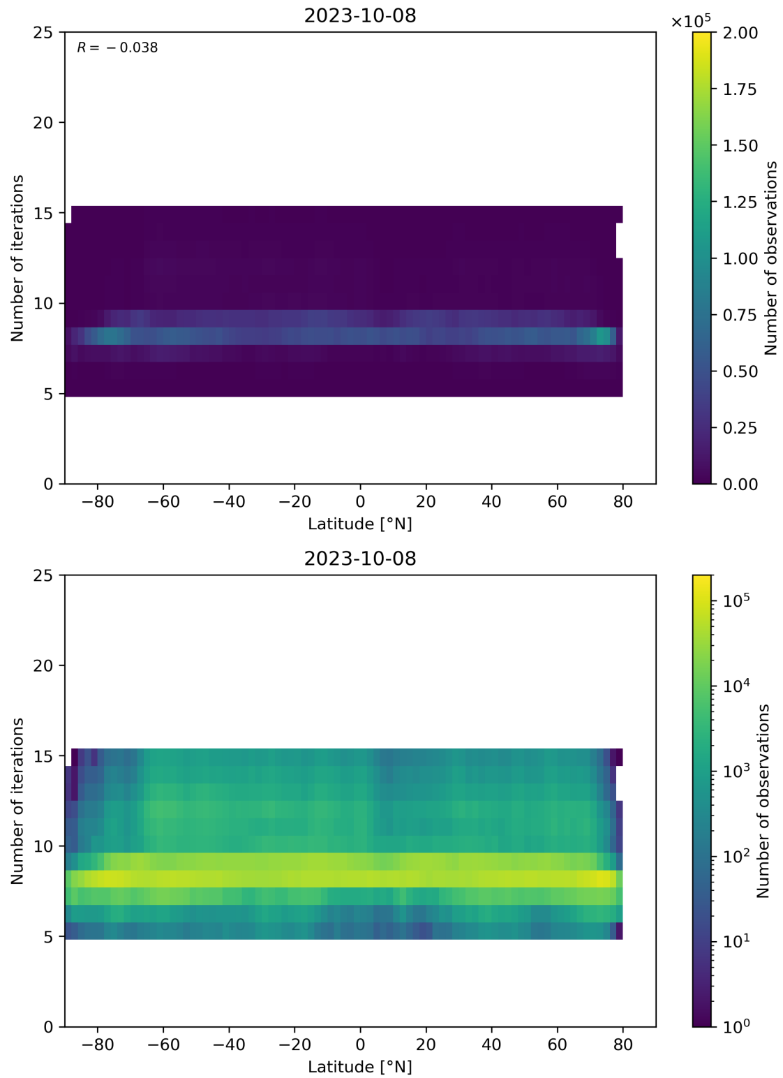
Figure 56: Scatter density plot of “Latitude” against “Number of iterations” for 2023-10-07 to 2023-10-09.
