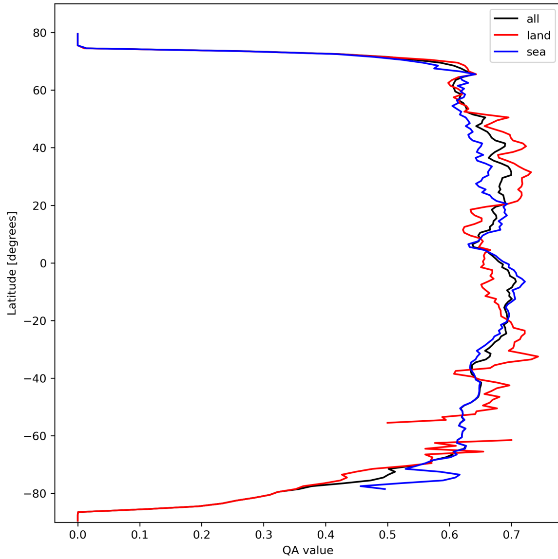
Figure 9: Zonal average of “QA value” for 2023-10-07 to 2023-10-09.
