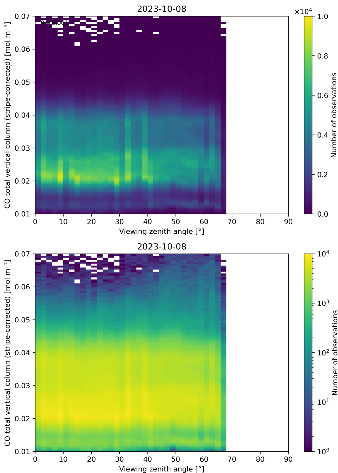
Figure 70: Scatter density plot of “Viewing zenith angle” against “CO total vertical column (stripe-corrected)” for 2023-10-07 to 2023-10-09.
