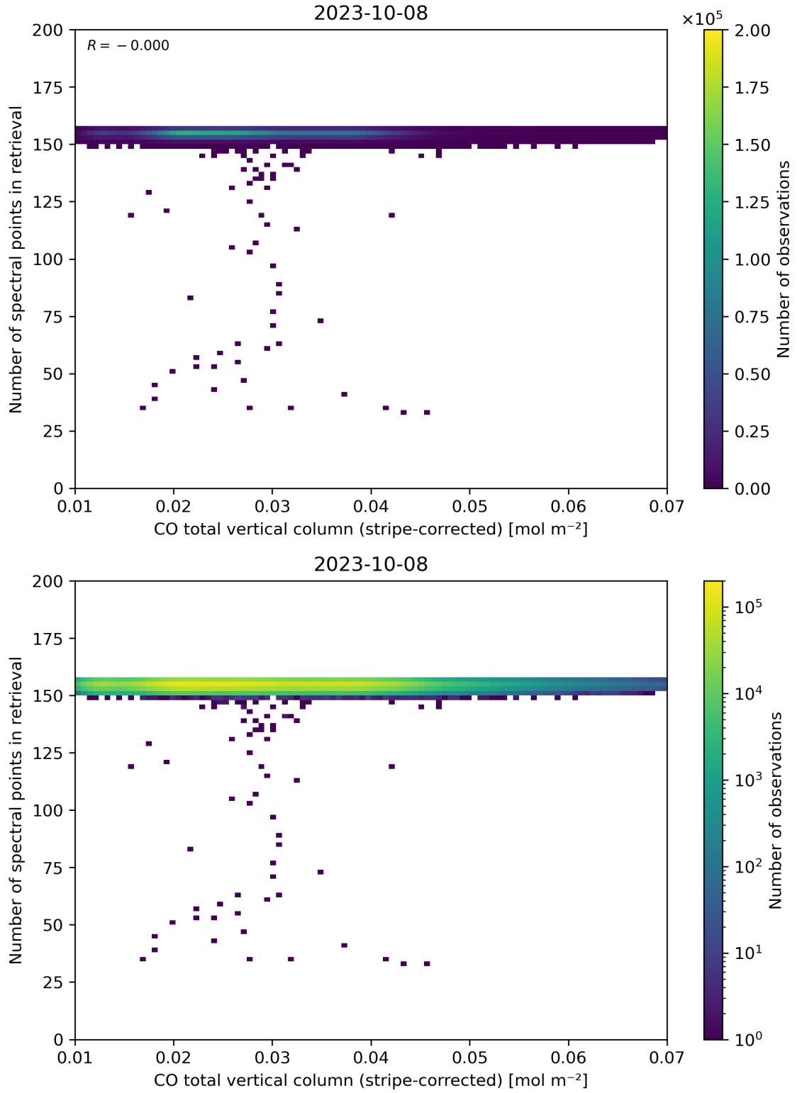
Figure 40: Scatter density plot of “CO total vertical column (stripe-corrected)” against “Number of spectral points in retrieval” for 2023-10-07 to 2023-10-09.
