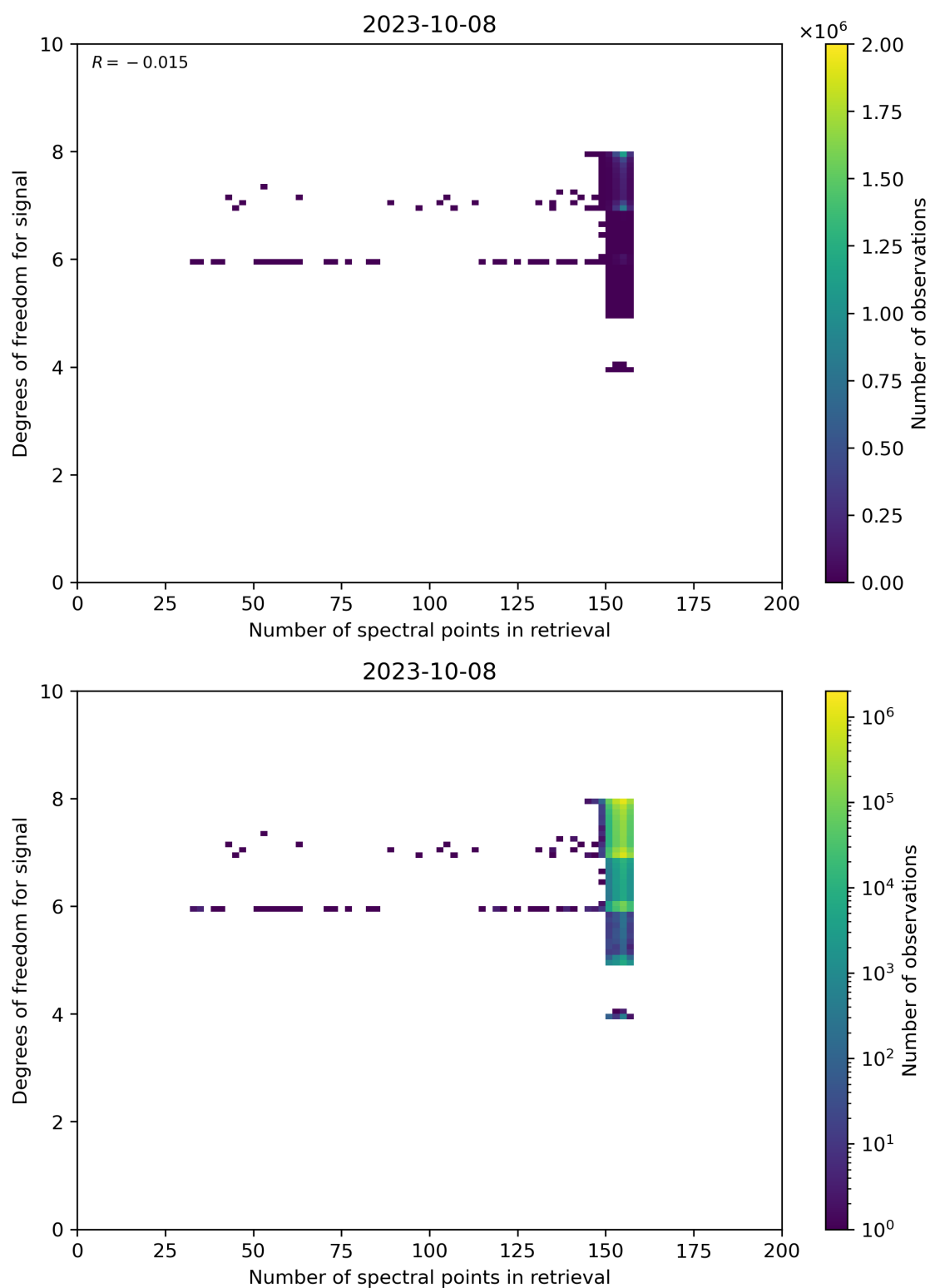
Figure 59: Scatter density plot of “Number of spectral points in retrieval” against “Degrees of freedom for signal” for 2023-10-07 to 2023-10-09.
