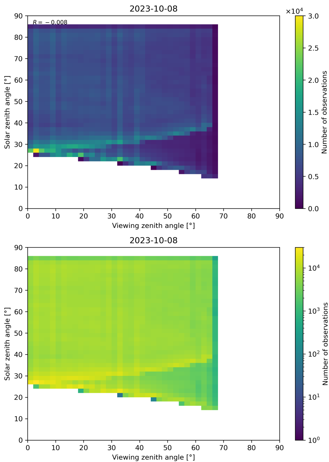
Figure 77: Scatter density plot of “Viewing zenith angle” against “Solar zenith angle” for 2023-10-07 to 2023-10-09.
