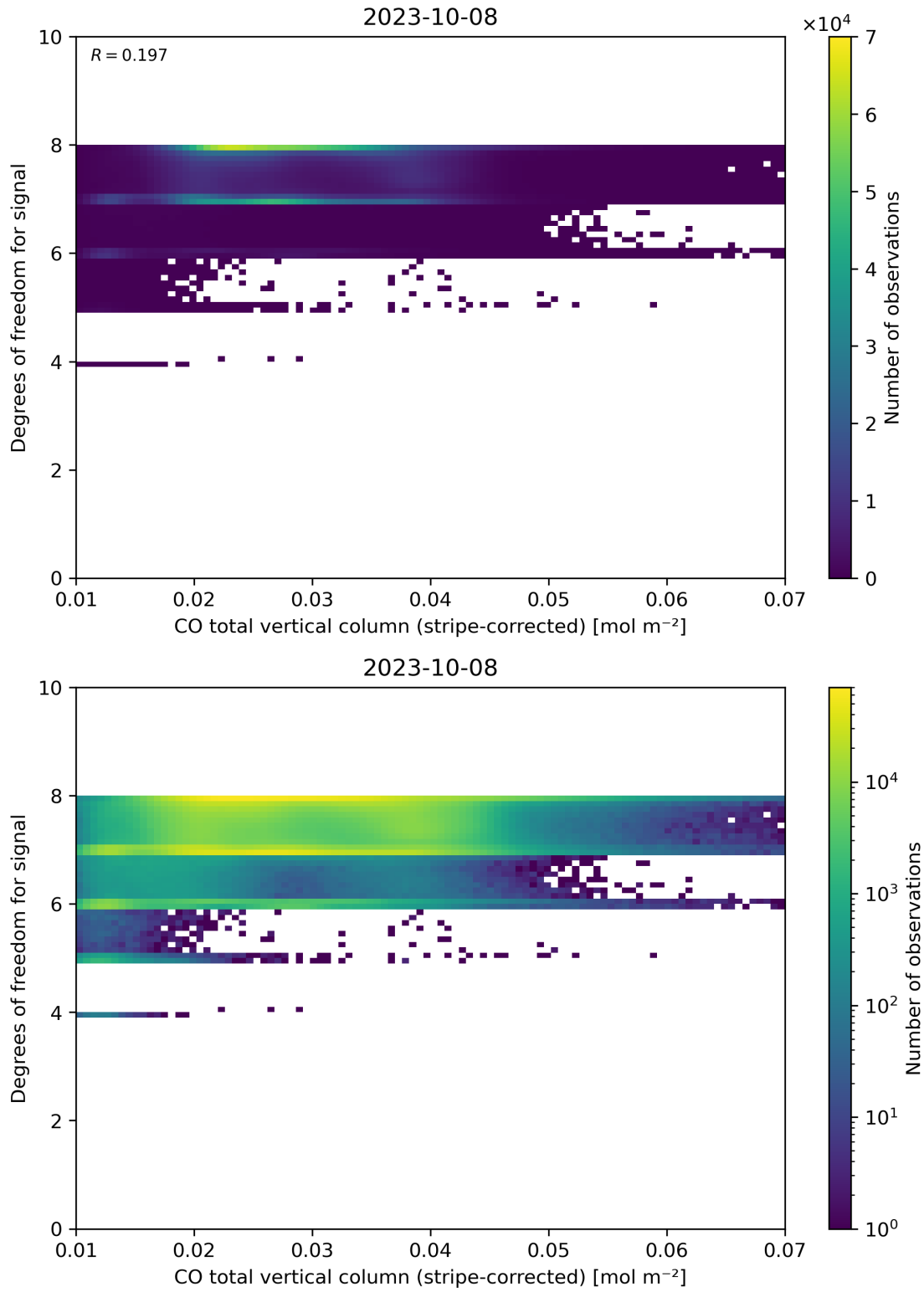
Figure 38: Scatter density plot of “CO total vertical column (stripe-corrected)” against “Degrees of freedom for signal” for 2023-10-07 to 2023-10-09.
