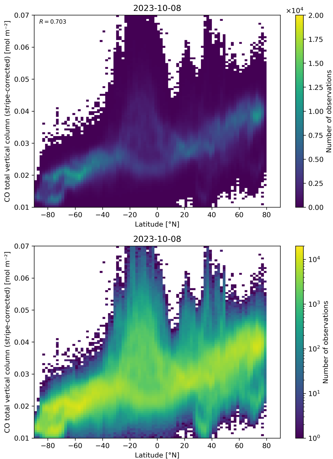
Figure 52: Scatter density plot of “Latitude” against “CO total vertical column (stripe-corrected)” for 2023-10-07 to 2023-10-09.
