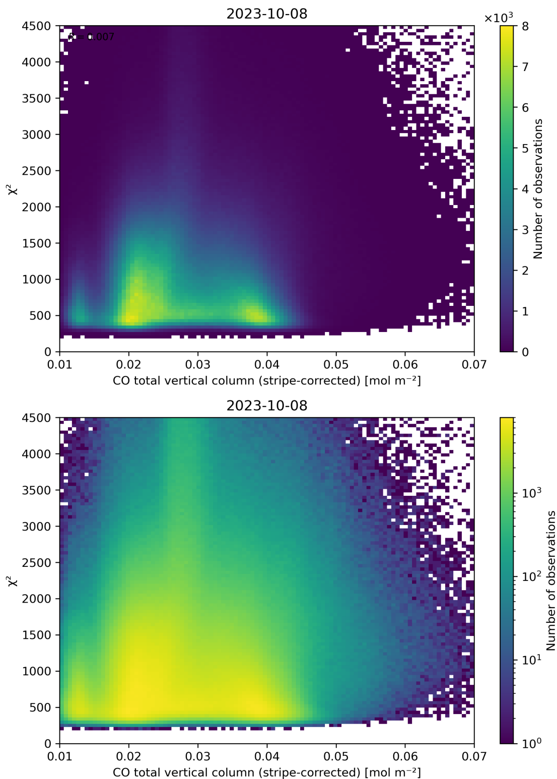
Figure 37: Scatter density plot of “CO total vertical column (stripe-corrected)” against “ \chi^2 ” for 2023-10-07 to 2023-10-09.
