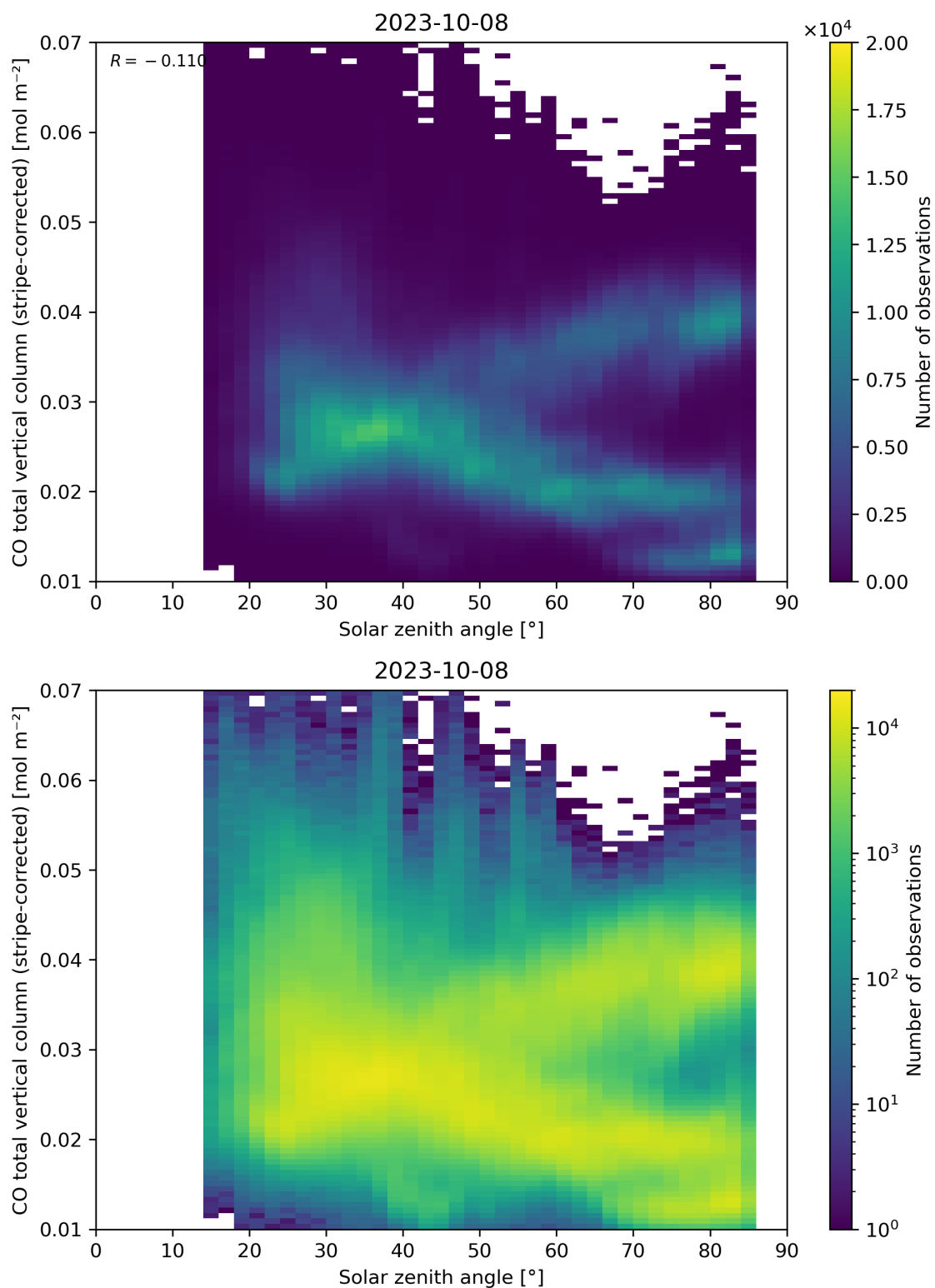
Figure 62: Scatter density plot of “Solar zenith angle” against “CO total vertical column (stripe-corrected)” for 2023-10-07 to 2023-10-09.
