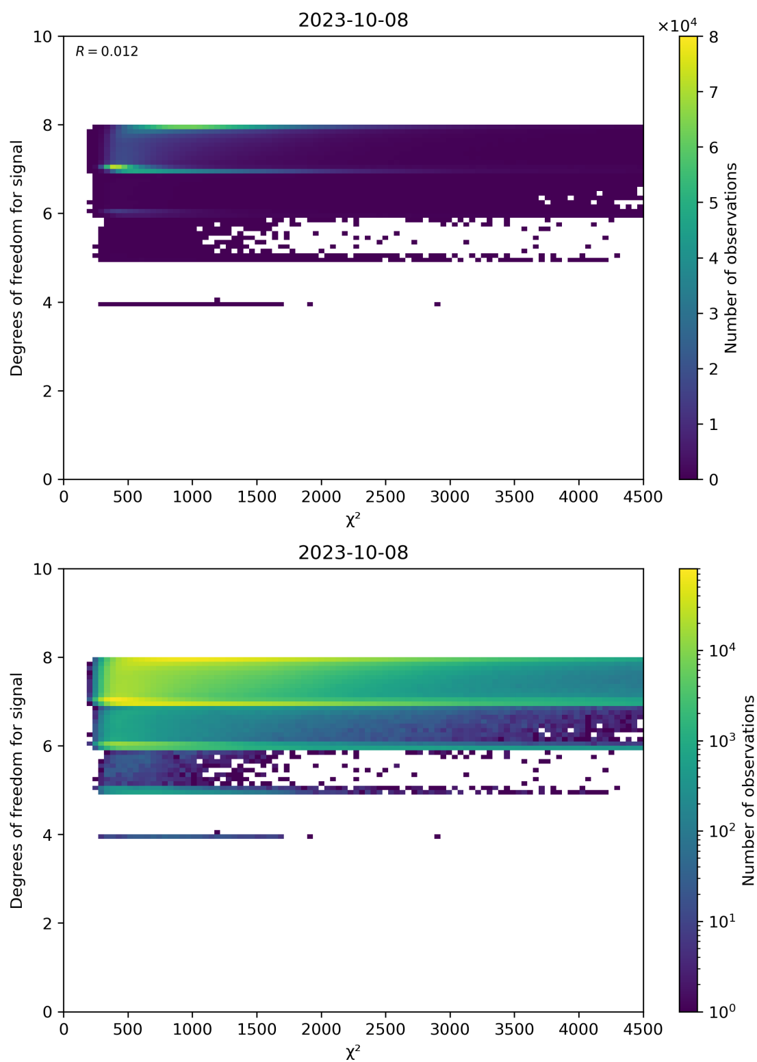
Figure 48: Scatter density plot of “ \chi^2 ” against “Degrees of freedom for signal” for 2023-10-07 to 2023-10-09.
