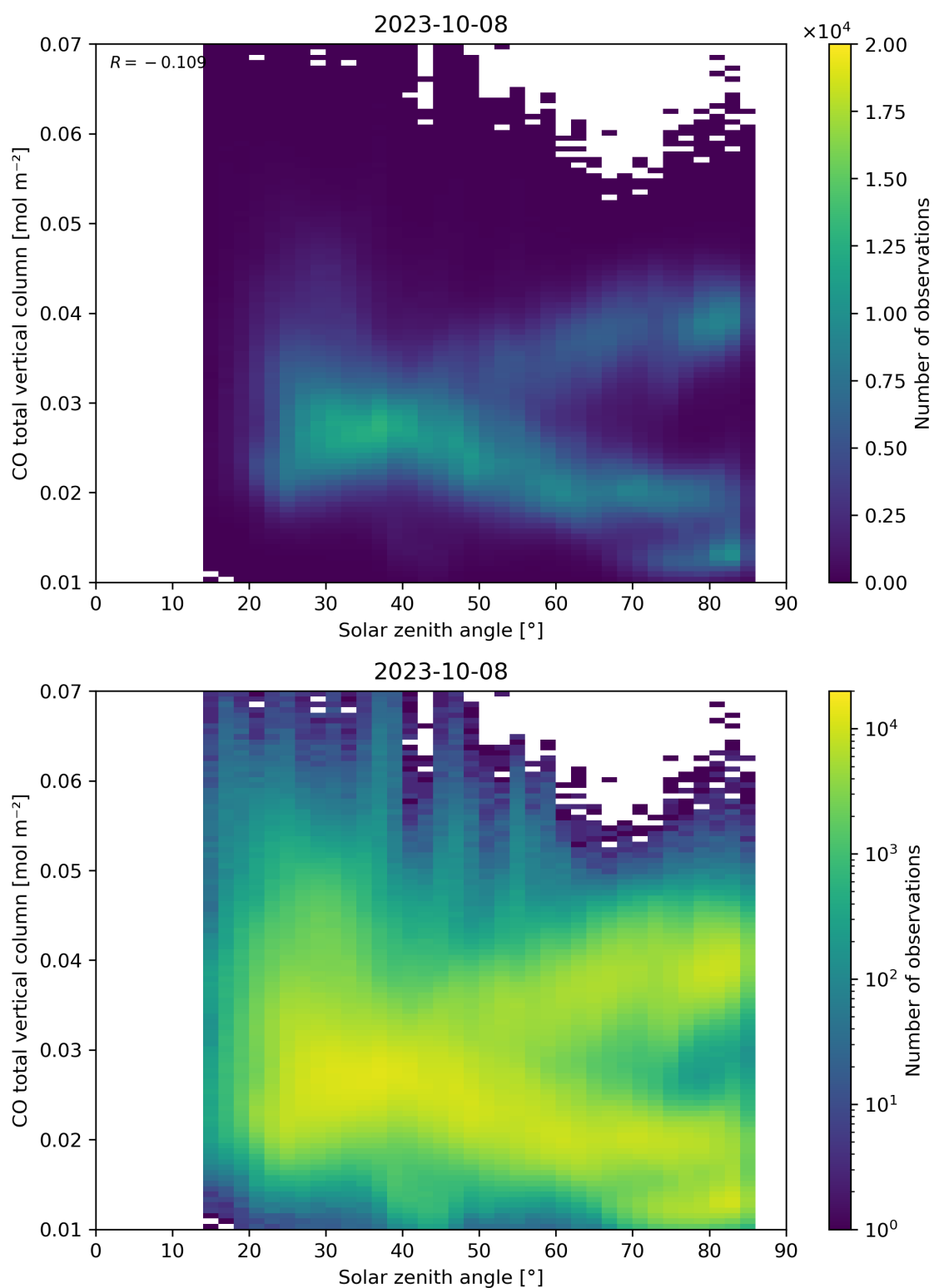
Figure 61: Scatter density plot of “Solar zenith angle” against “CO total vertical column” for 2023-10-07 to 2023-10-09.
