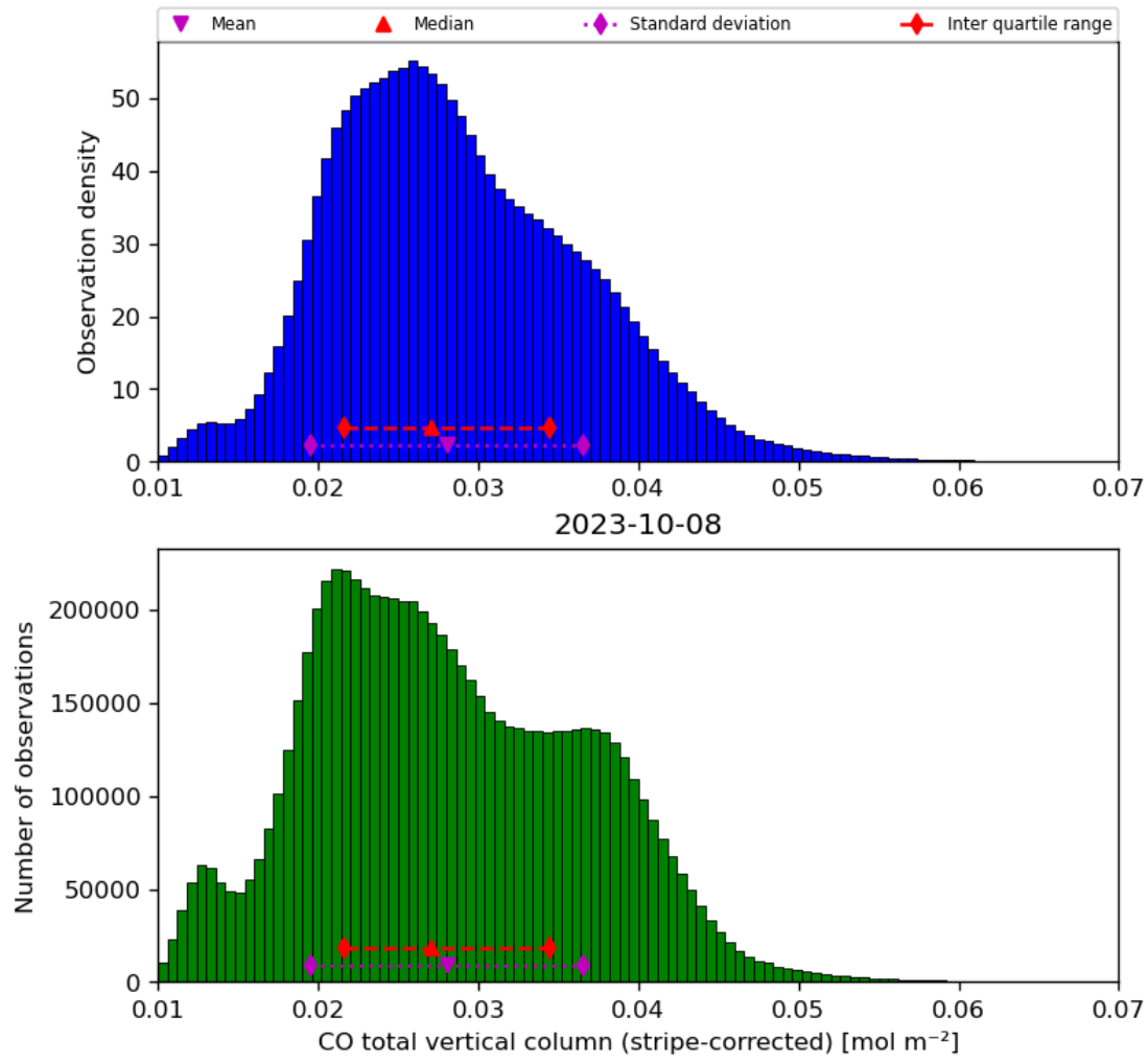
Figure 19: Histogram of “CO total vertical column (stripe-corrected)” for 2023-10-07 to 2023-10-09
