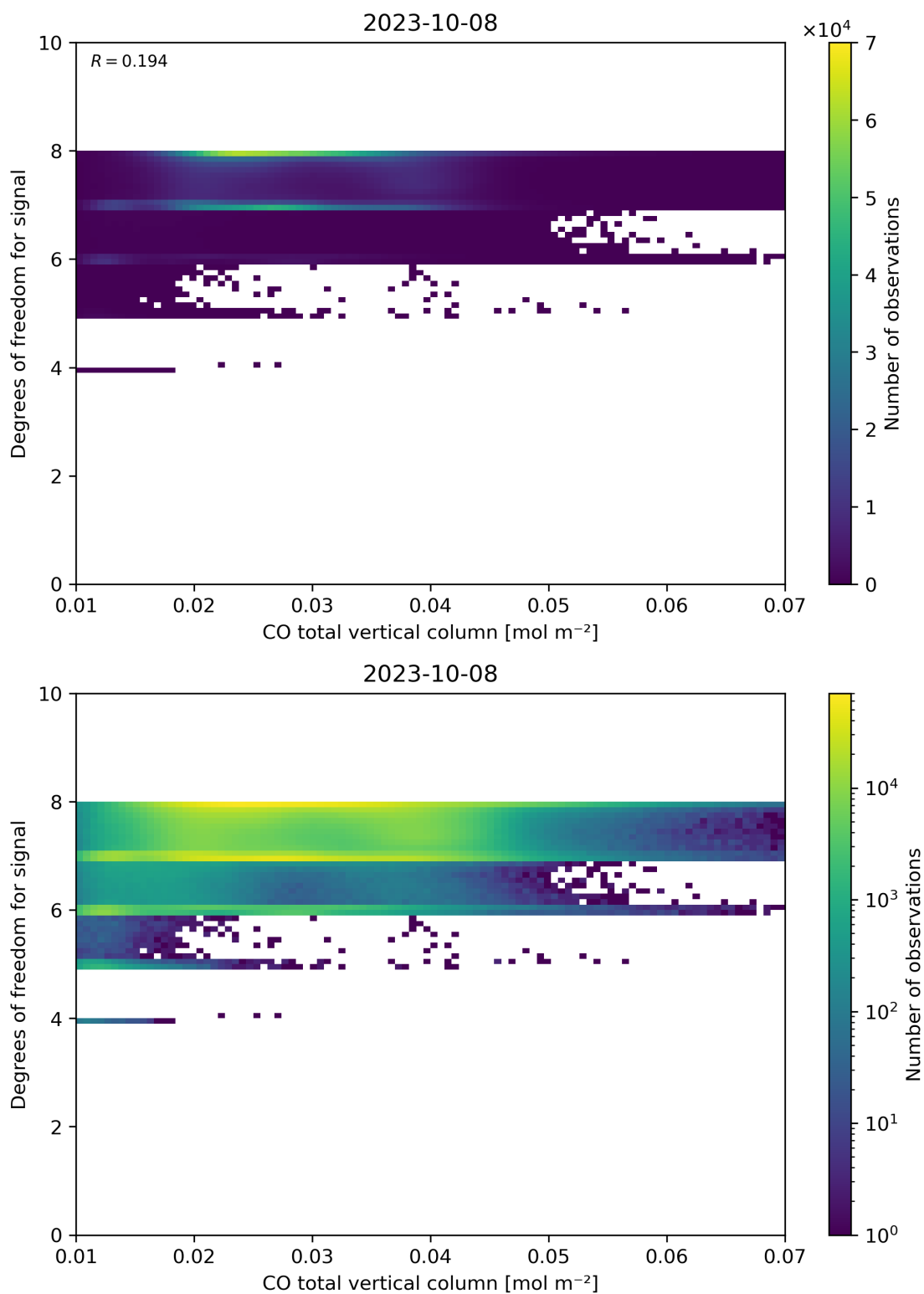
Figure 41: Scatter density plot of “CO total vertical column” against “Degrees of freedom for signal” for 2023-10-07 to 2023-10-09.
