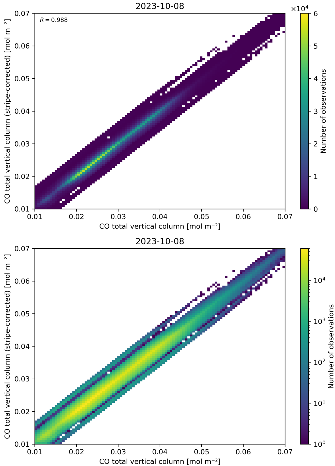
Figure 33: Scatter density plot of “CO total vertical column” against “CO total vertical column (stripe-corrected)” for 2023-10-07 to 2023-10-09.
