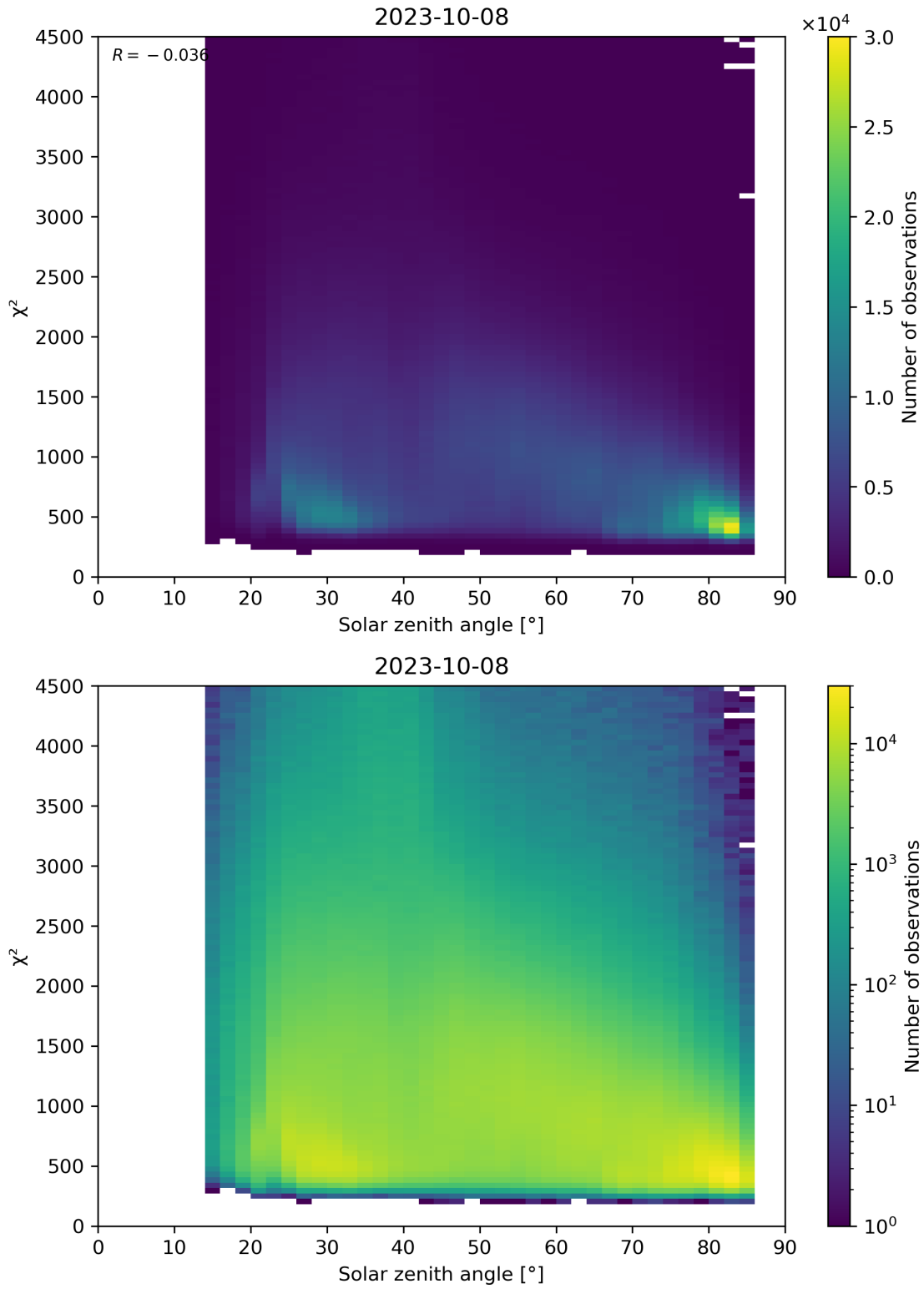
Figure 64: Scatter density plot of “Solar zenith angle” against “ \chi^2 ” for 2023-10-07 to 2023-10-09.
