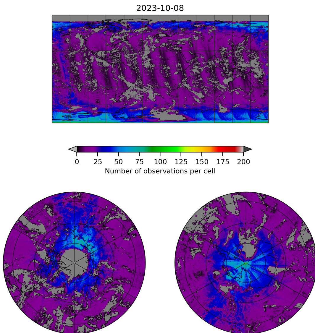
Figure 8: Map of the number of observations for 2023-10-07 to 2023-10-09
