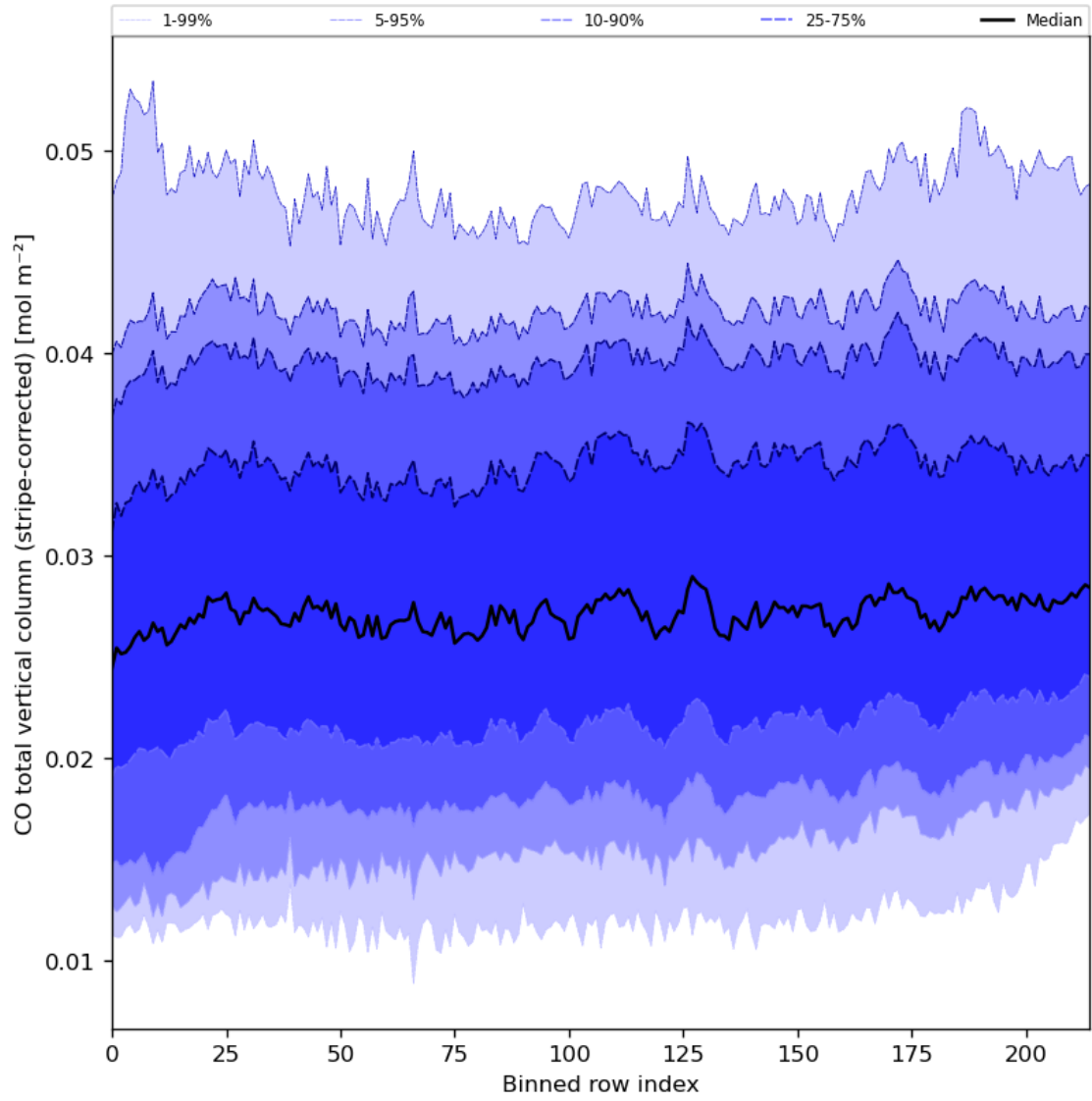
Figure 27: Along track statistics of “CO total vertical column (stripe-corrected)” for 2023-10-07 to 2023-10-09
