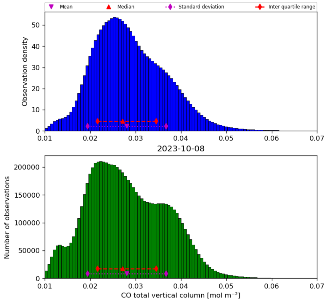
Figure 18: Histogram of “CO total vertical column” for 2023-10-07 to 2023-10-09
