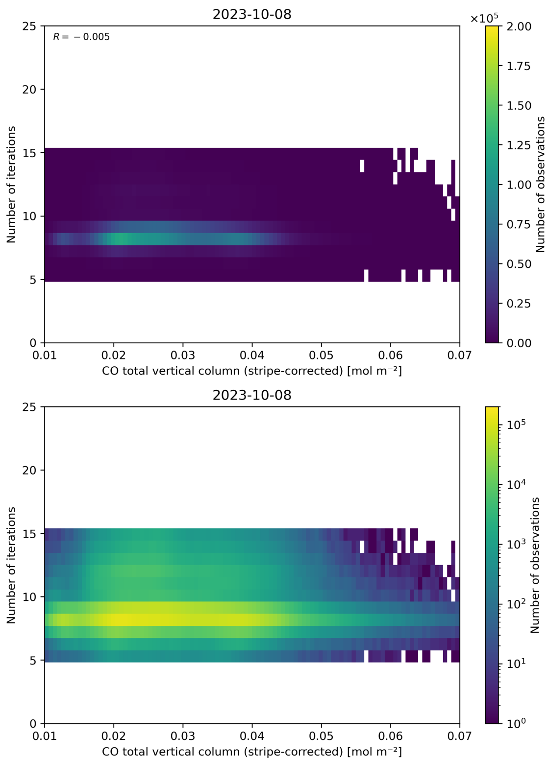
Figure 39: Scatter density plot of “CO total vertical column (stripe-corrected)” against “Number of iterations” for 2023-10-07 to 2023-10-09.
