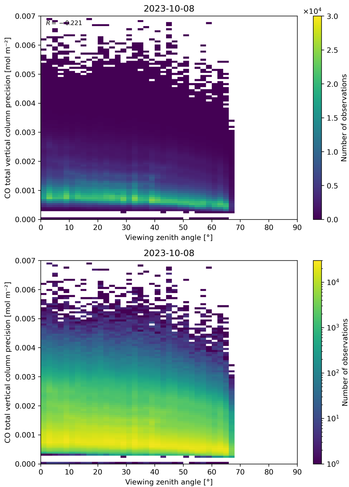
Figure 71: Scatter density plot of “Viewing zenith angle” against “CO total vertical column precision” for 2023-10-07 to 2023-10-09.
