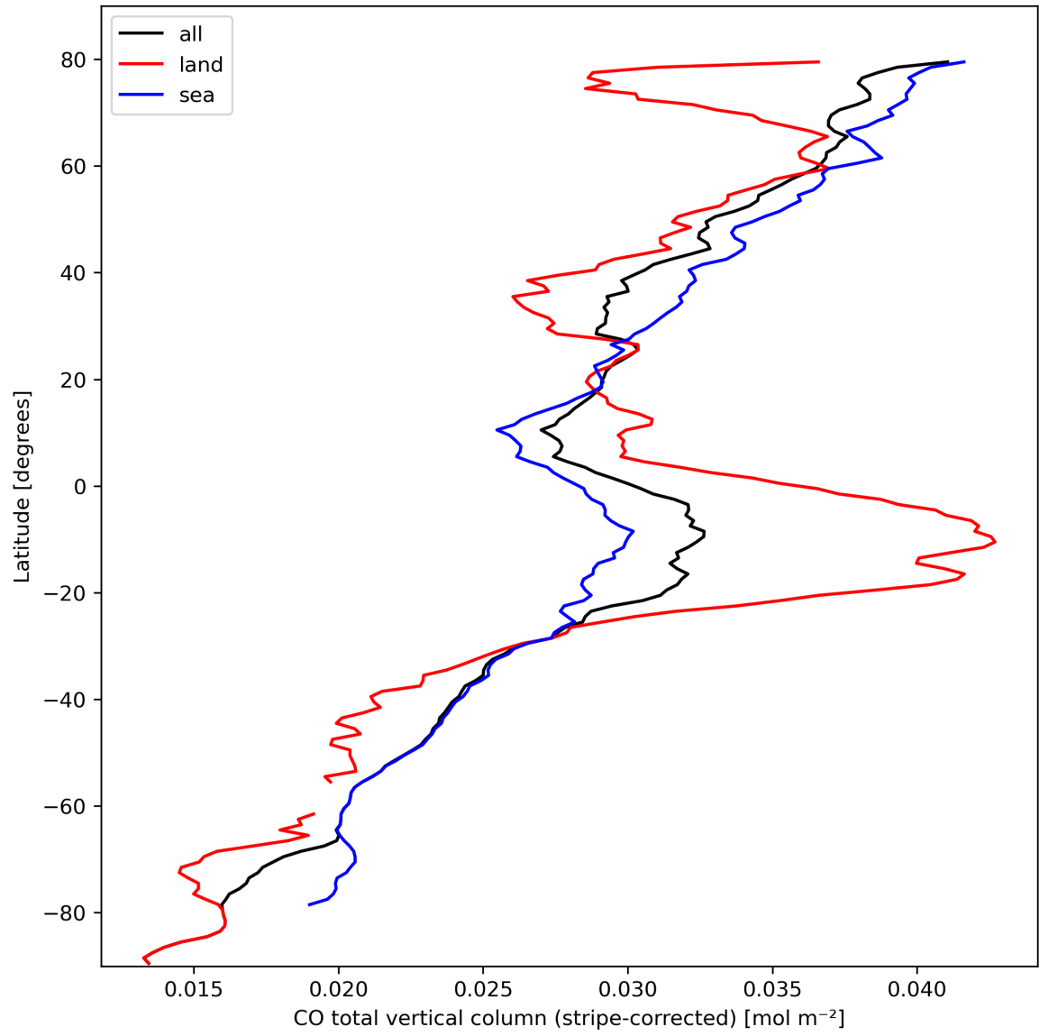
Figure 11: Zonal average of “CO total vertical column (stripe-corrected)” for 2023-10-07 to 2023-10-09.
