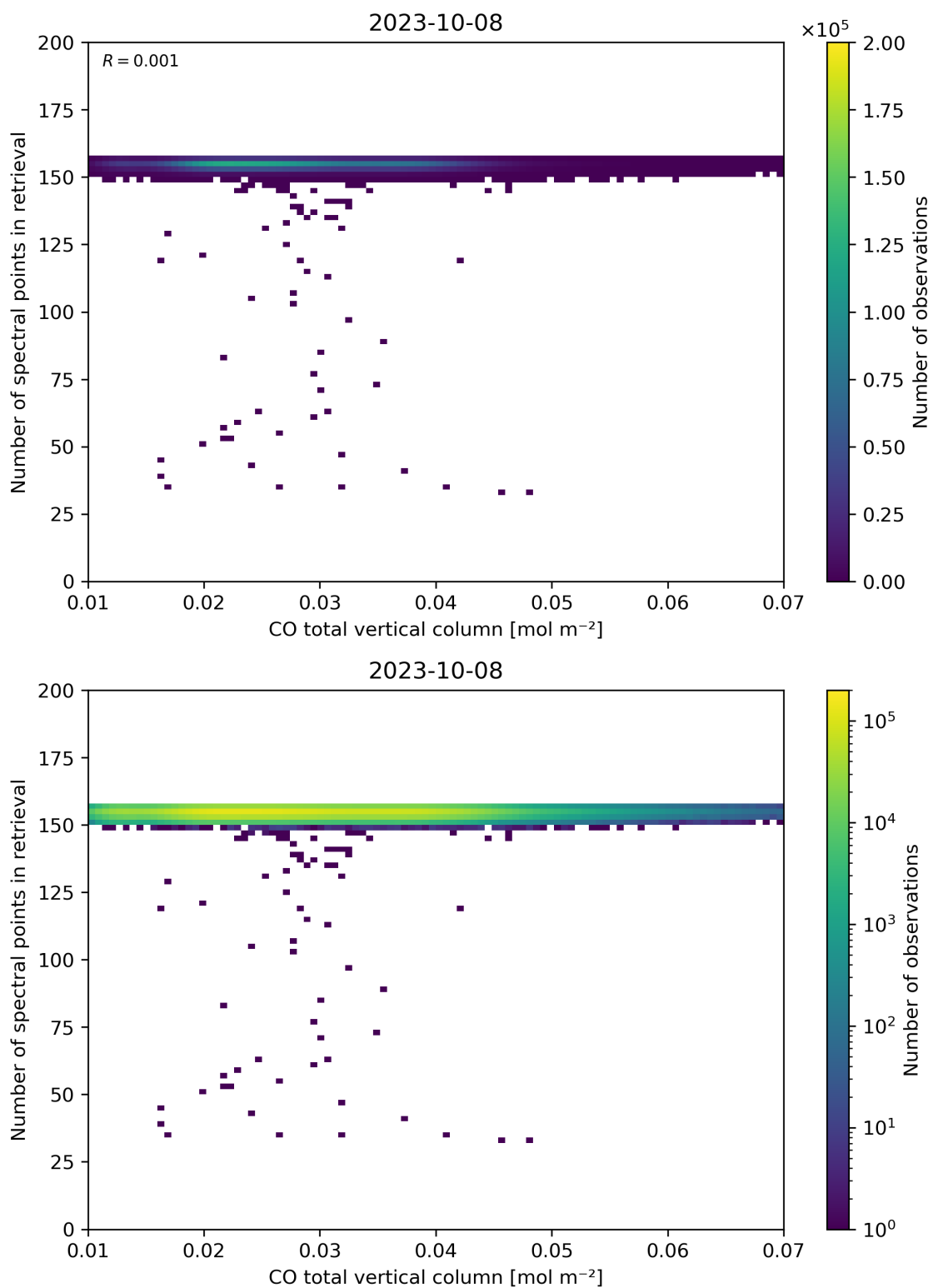
Figure 43: Scatter density plot of “CO total vertical column” against “Number of spectral points in retrieval” for 2023-10-07 to 2023-10-09.
