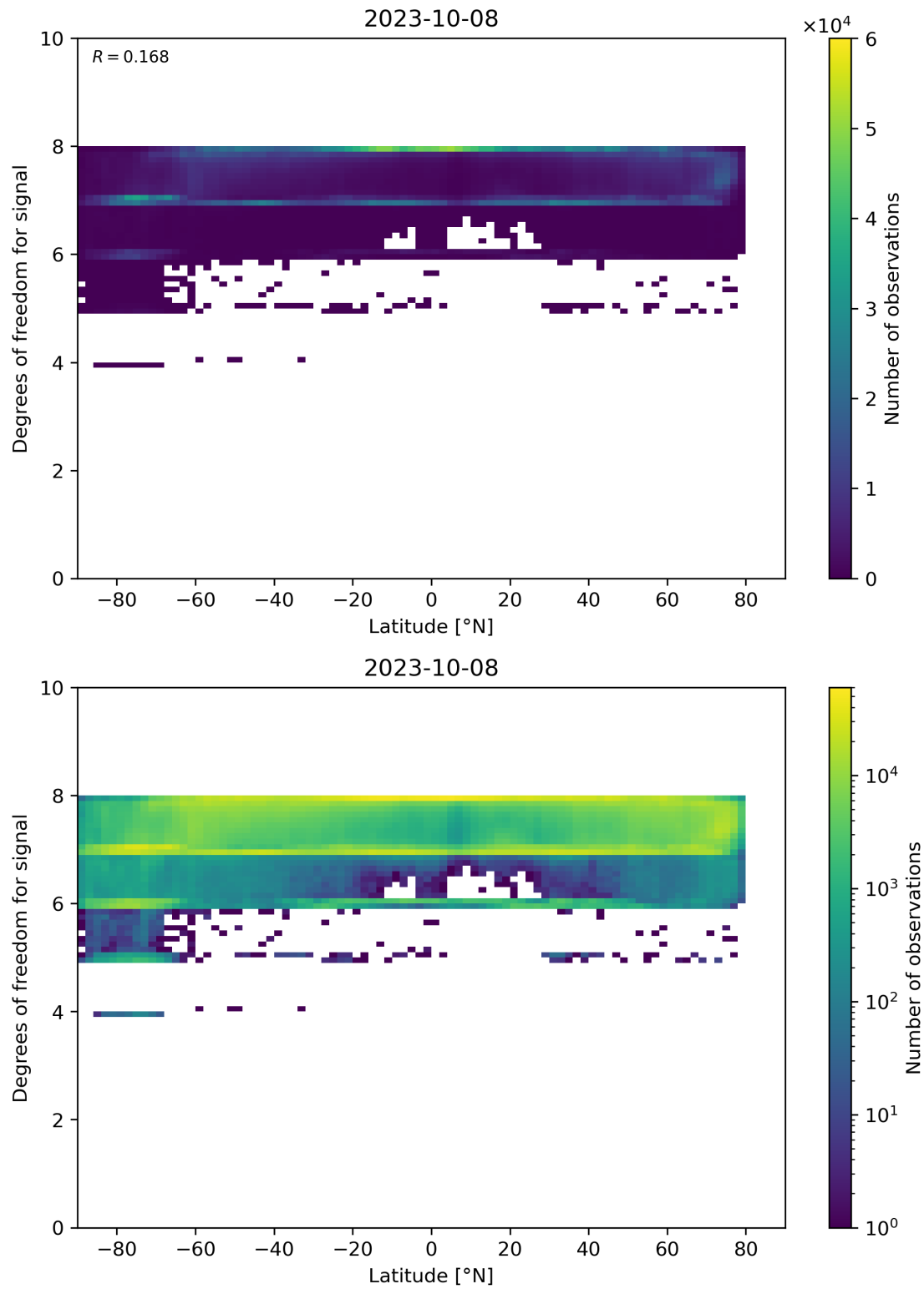
Figure 55: Scatter density plot of “Latitude” against “Degrees of freedom for signal” for 2023-10-07 to 2023-10-09.
