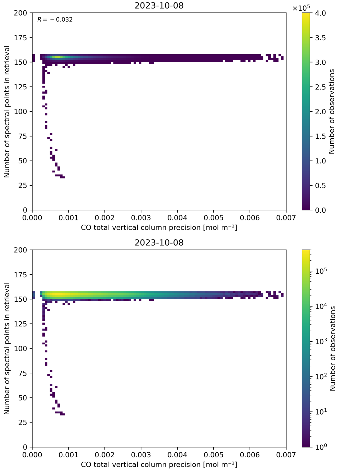
Figure 47: Scatter density plot of “CO total vertical column precision” against “Number of spectral points in retrieval” for 2023-10-07 to 2023-10-09.
