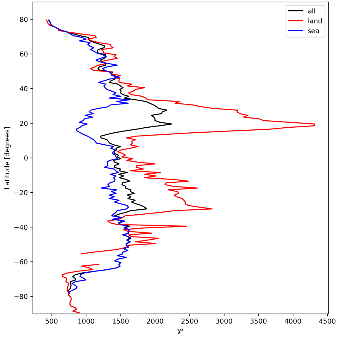
Figure 14: Zonal average of “ \chi^2 ” for 2023-10-07 to 2023-10-09.
