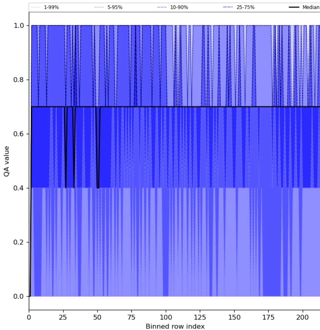
Figure 25: Along track statistics of “QA value” for 2023-10-07 to 2023-10-09
