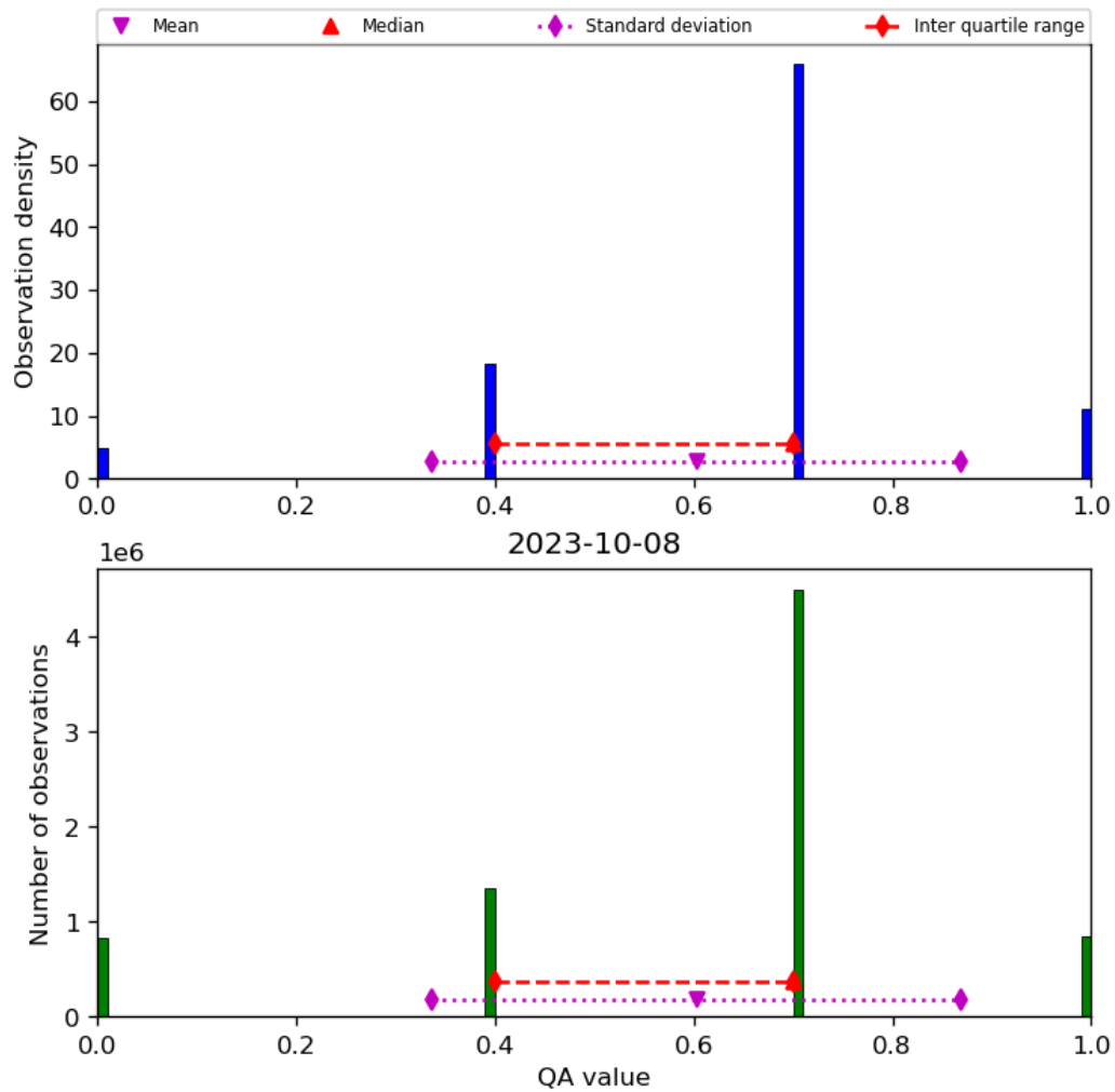
Figure 17: Histogram of “QA value” for 2023-10-07 to 2023-10-09
