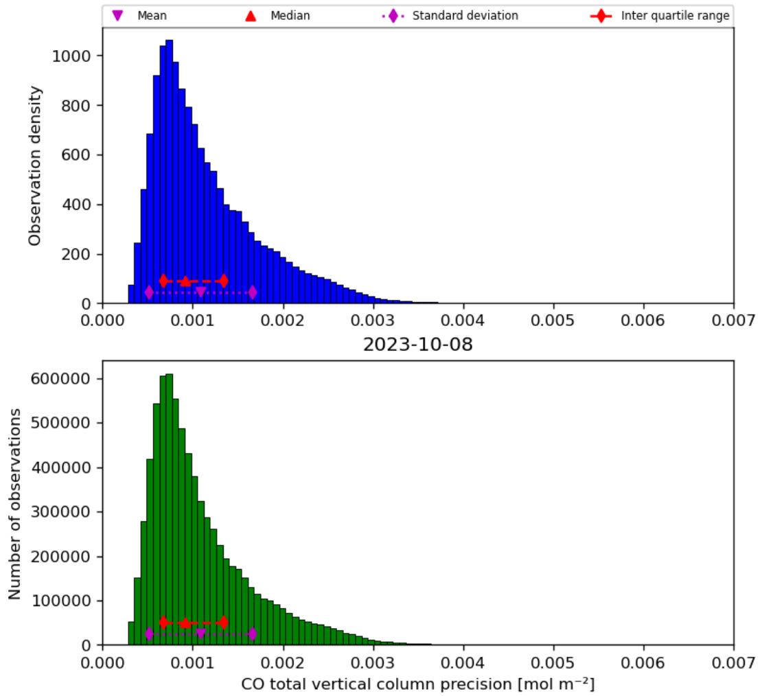
Figure 20: Histogram of “CO total vertical column precision” for 2023-10-07 to 2023-10-09
