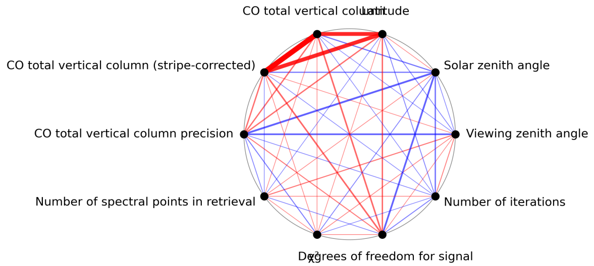
Figure 1: Map of correlation graph for 2023-10-07 to 2023-10-09.
