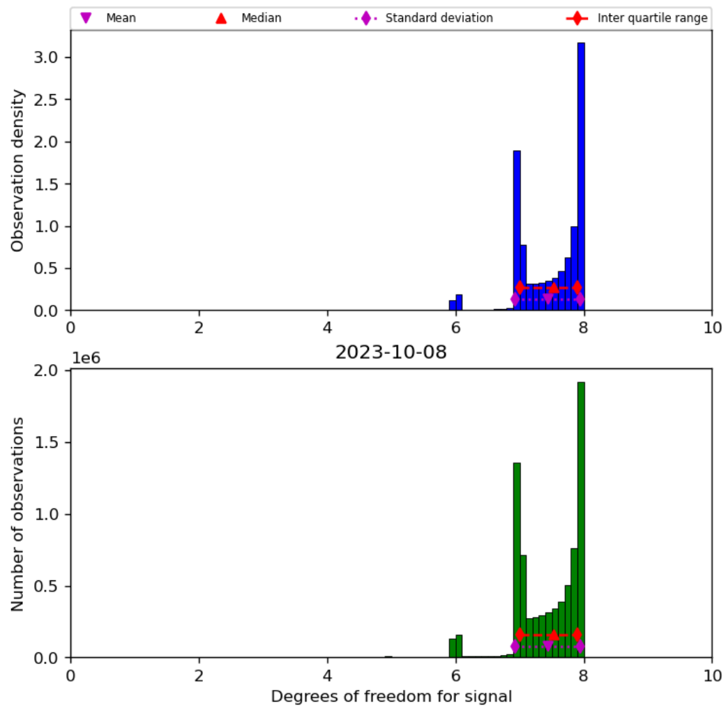
Figure 23: Histogram of “Degrees of freedom for signal” for 2023-10-07 to 2023-10-09
