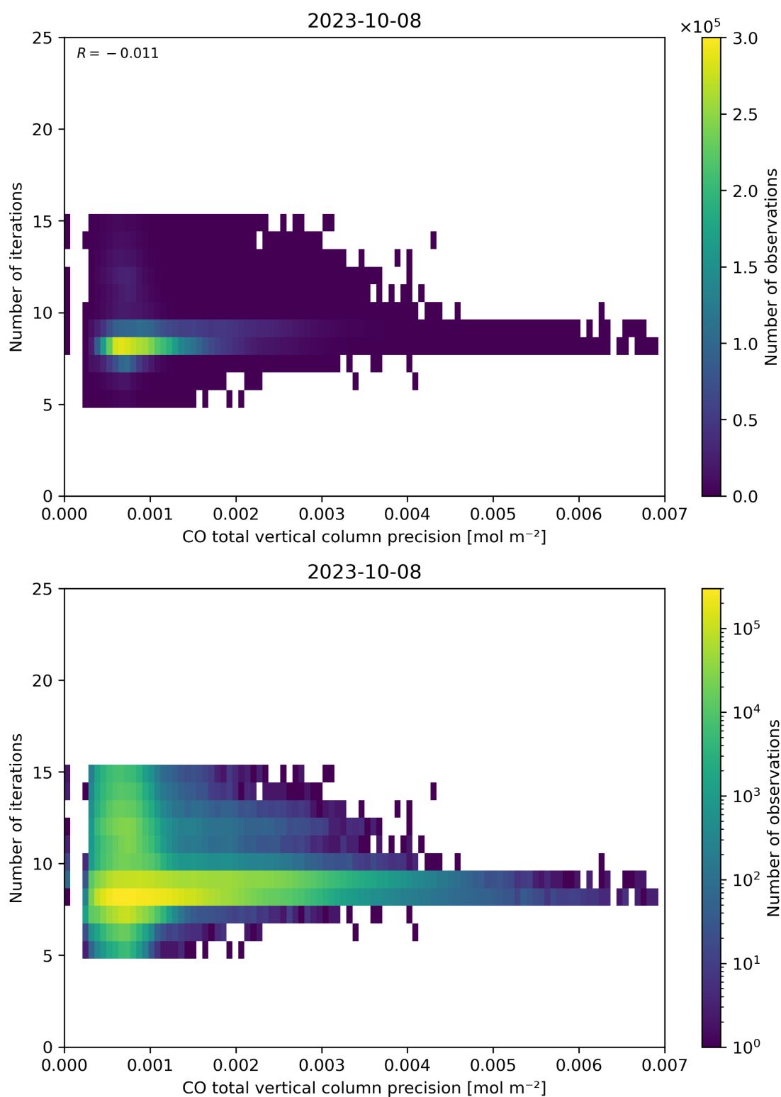
Figure 46: Scatter density plot of “CO total vertical column precision” against “Number of iterations” for 2023-10-07 to 2023-10-09.
