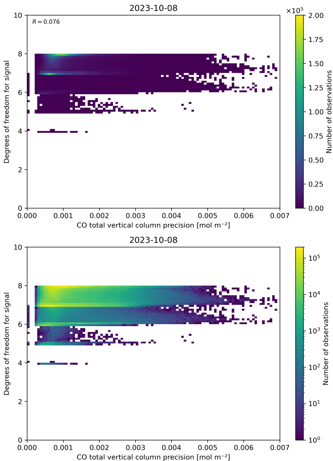
Figure 45: Scatter density plot of “CO total vertical column precision” against “Degrees of freedom for signal” for 2023-10-07 to 2023-10-09.
