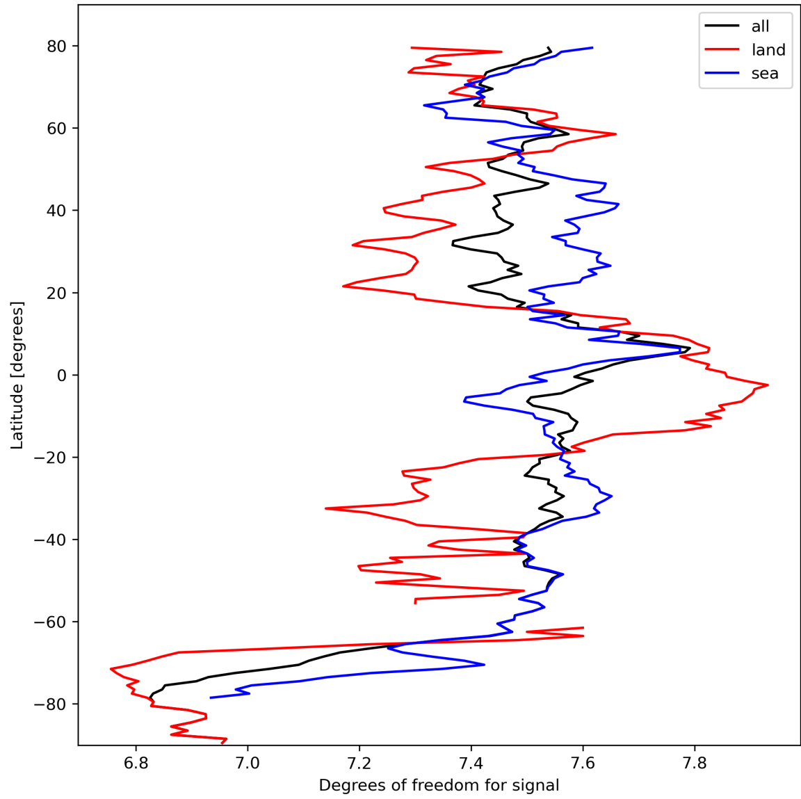
Figure 15: Zonal average of “Degrees of freedom for signal” for 2023-10-07 to 2023-10-09.
