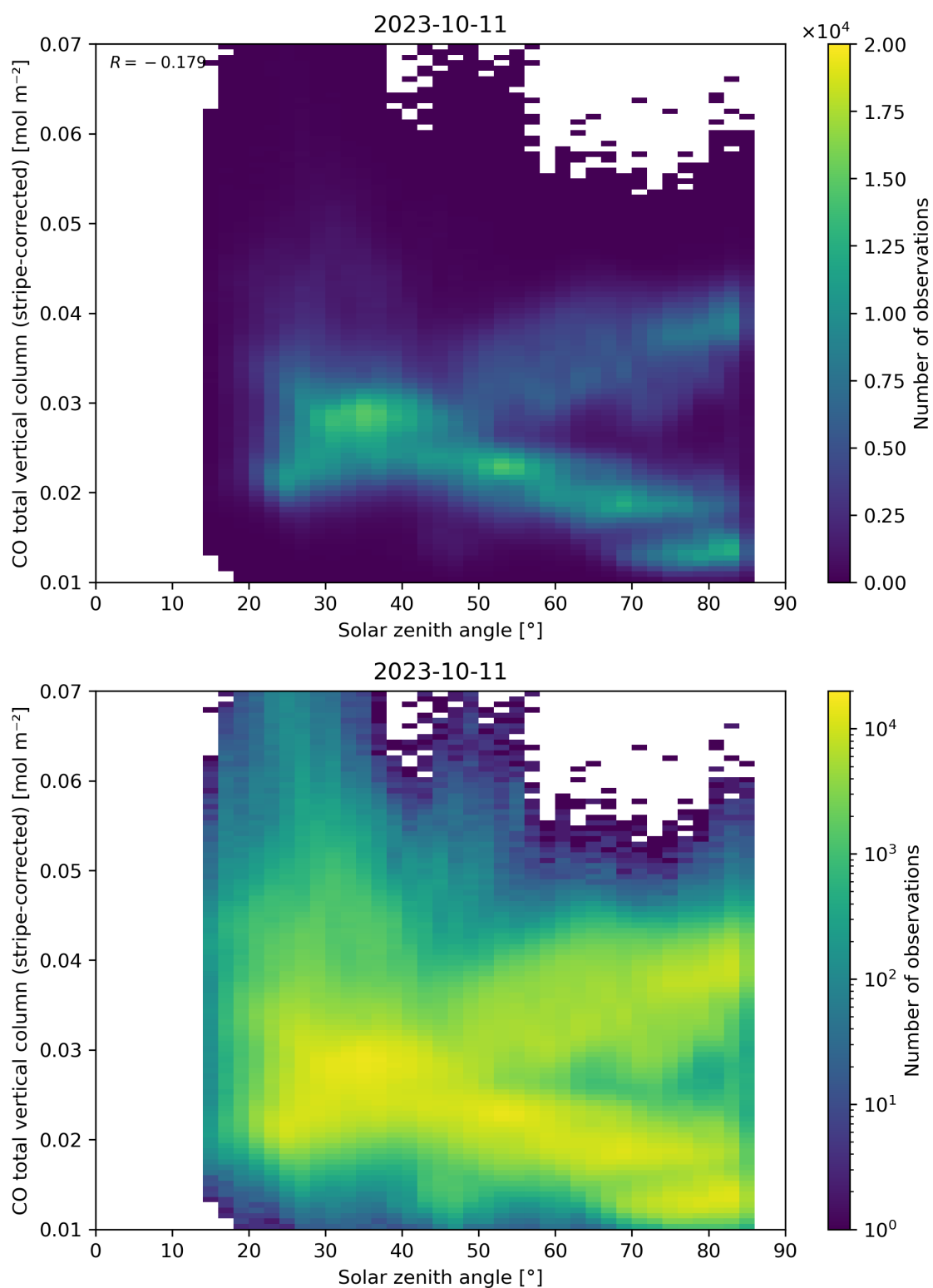
Figure 62: Scatter density plot of “Solar zenith angle” against “CO total vertical column (stripe-corrected)” for 2023-10-10 to 2023-10-12.
