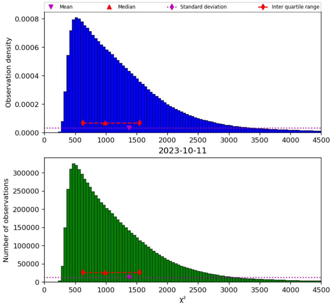
Figure 22: Histogram of “ \chi^2 ” for 2023-10-10 to 2023-10-12
