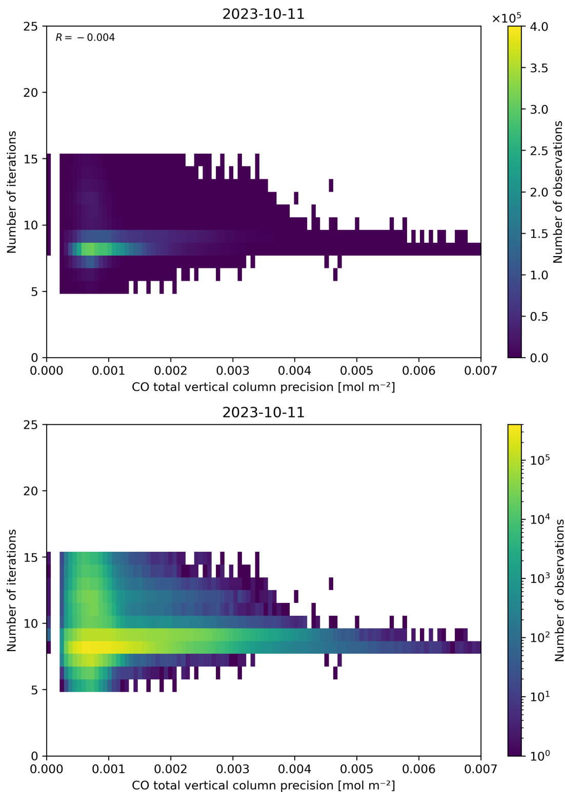
Figure 46: Scatter density plot of “CO total vertical column precision” against “Number of iterations” for 2023-10-10 to 2023-10-12.
