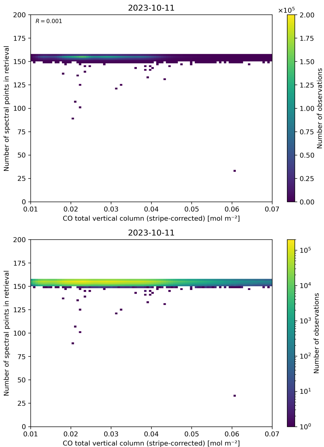
Figure 40: Scatter density plot of “CO total vertical column (stripe-corrected)” against “Number of spectral points in retrieval” for 2023-10-10 to 2023-10-12.
