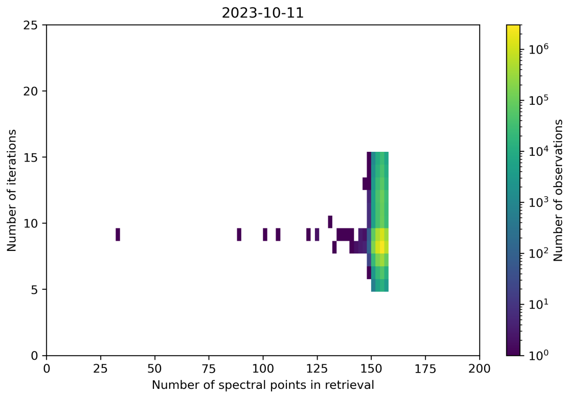
Figure 60: Scatter density plot of “Number of spectral points in retrieval” against “Number of iterations” for 2023-10-10 to 2023-10-12.
