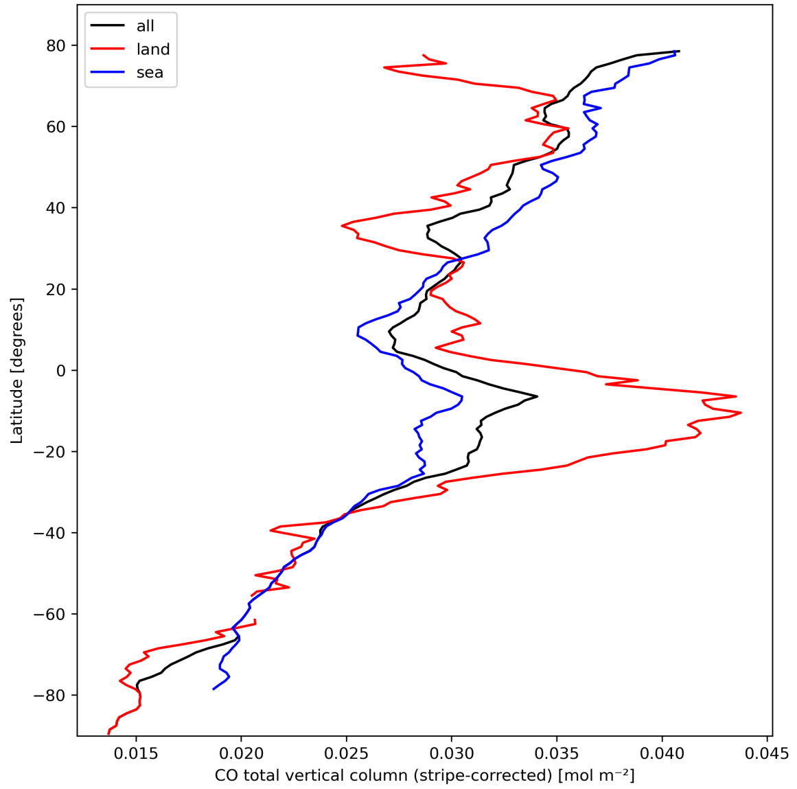
Figure 11: Zonal average of “CO total vertical column (stripe-corrected)” for 2023-10-10 to 2023-10-12.
