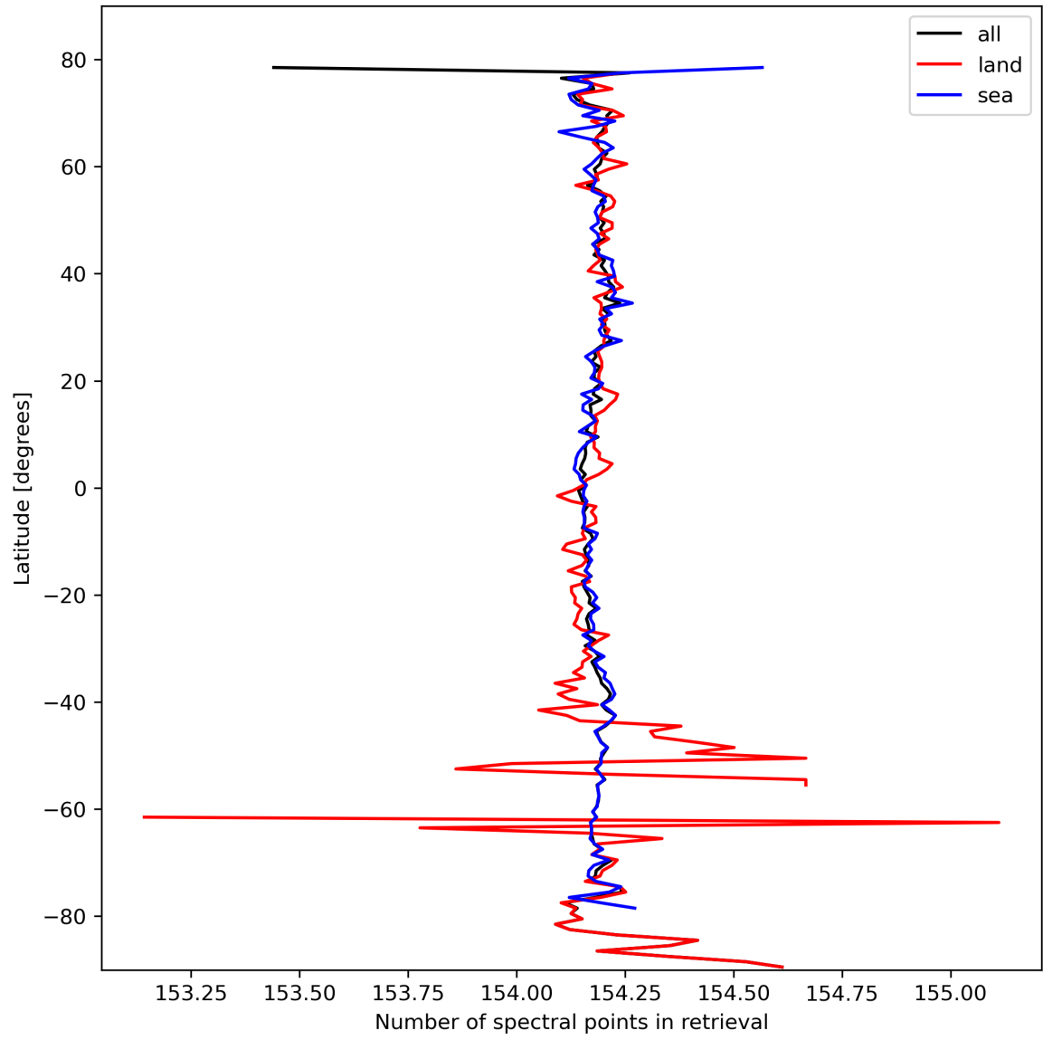
Figure 13: Zonal average of “Number of spectral points in retrieval” for 2023-10-10 to 2023-10-12.
