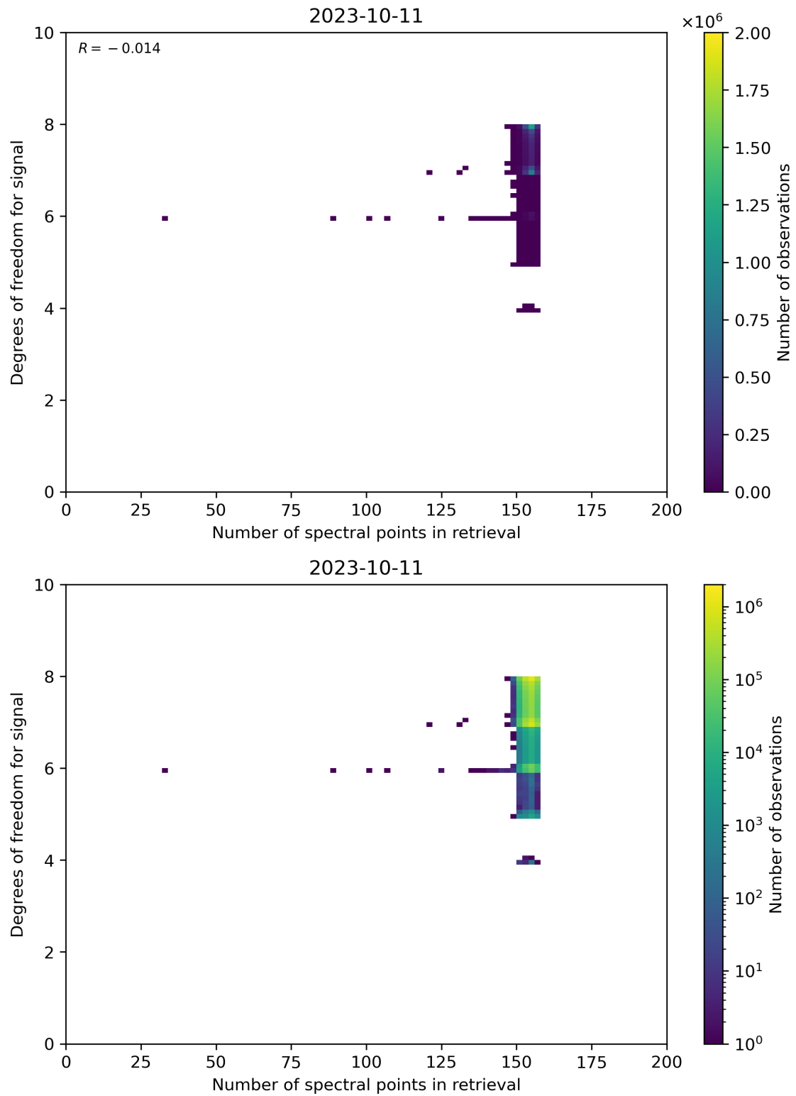
Figure 59: Scatter density plot of “Number of spectral points in retrieval” against “Degrees of freedom for signal” for 2023-10-10 to 2023-10-12.
