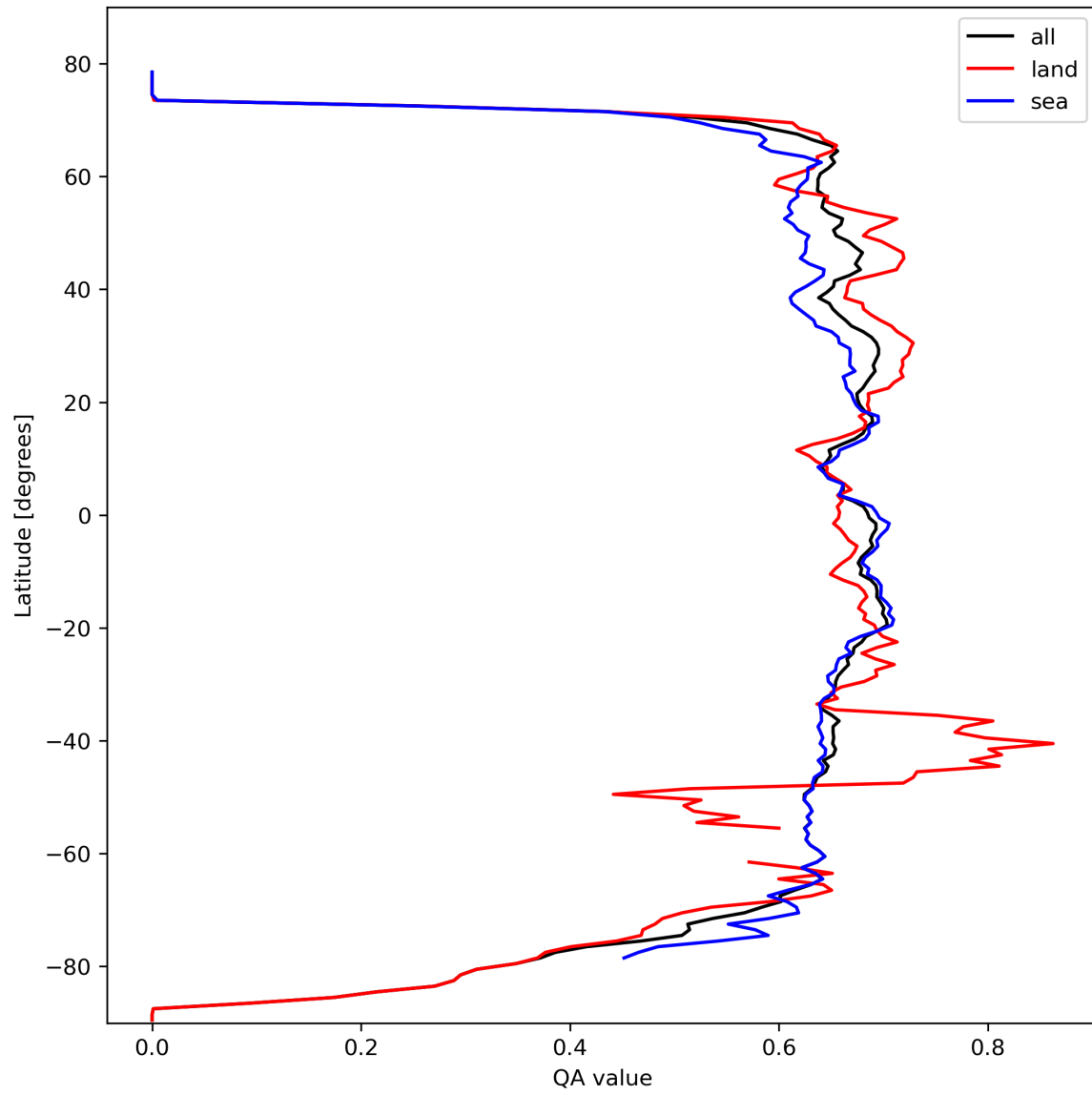
Figure 9: Zonal average of “QA value” for 2023-10-10 to 2023-10-12.
