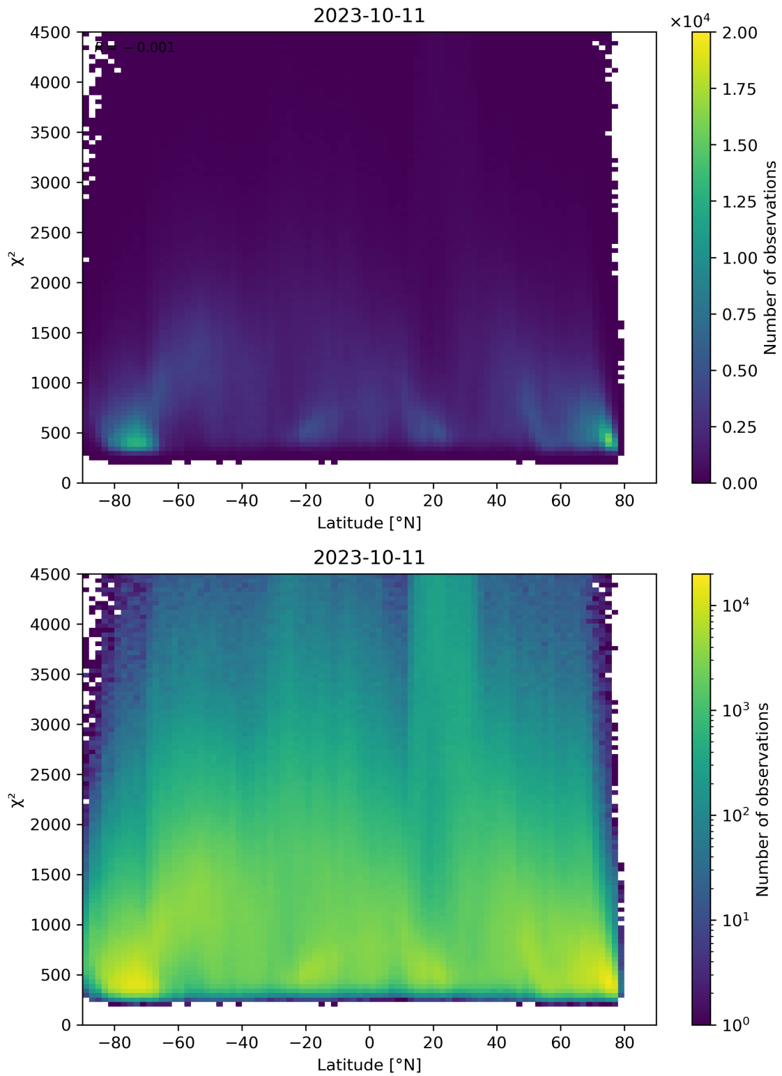
Figure 54: Scatter density plot of “Latitude” against “ \chi^2 ” for 2023-10-10 to 2023-10-12.
