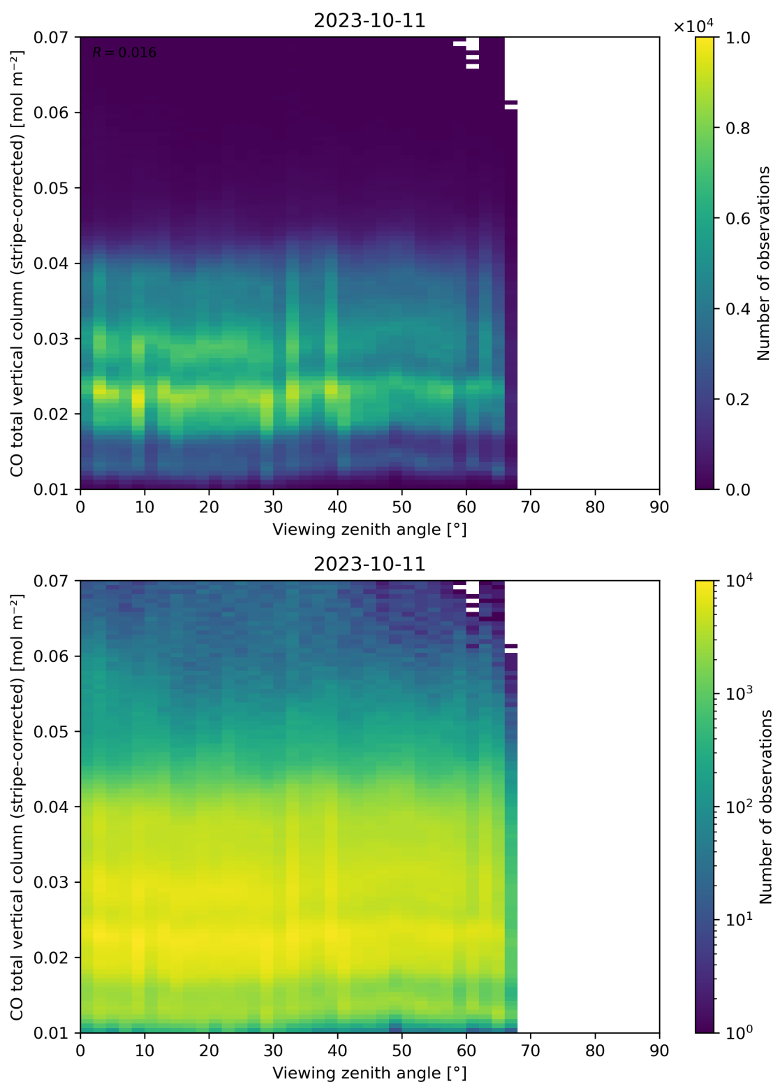
Figure 70: Scatter density plot of “Viewing zenith angle” against “CO total vertical column (stripe-corrected)” for 2023-10-10 to 2023-10-12.
