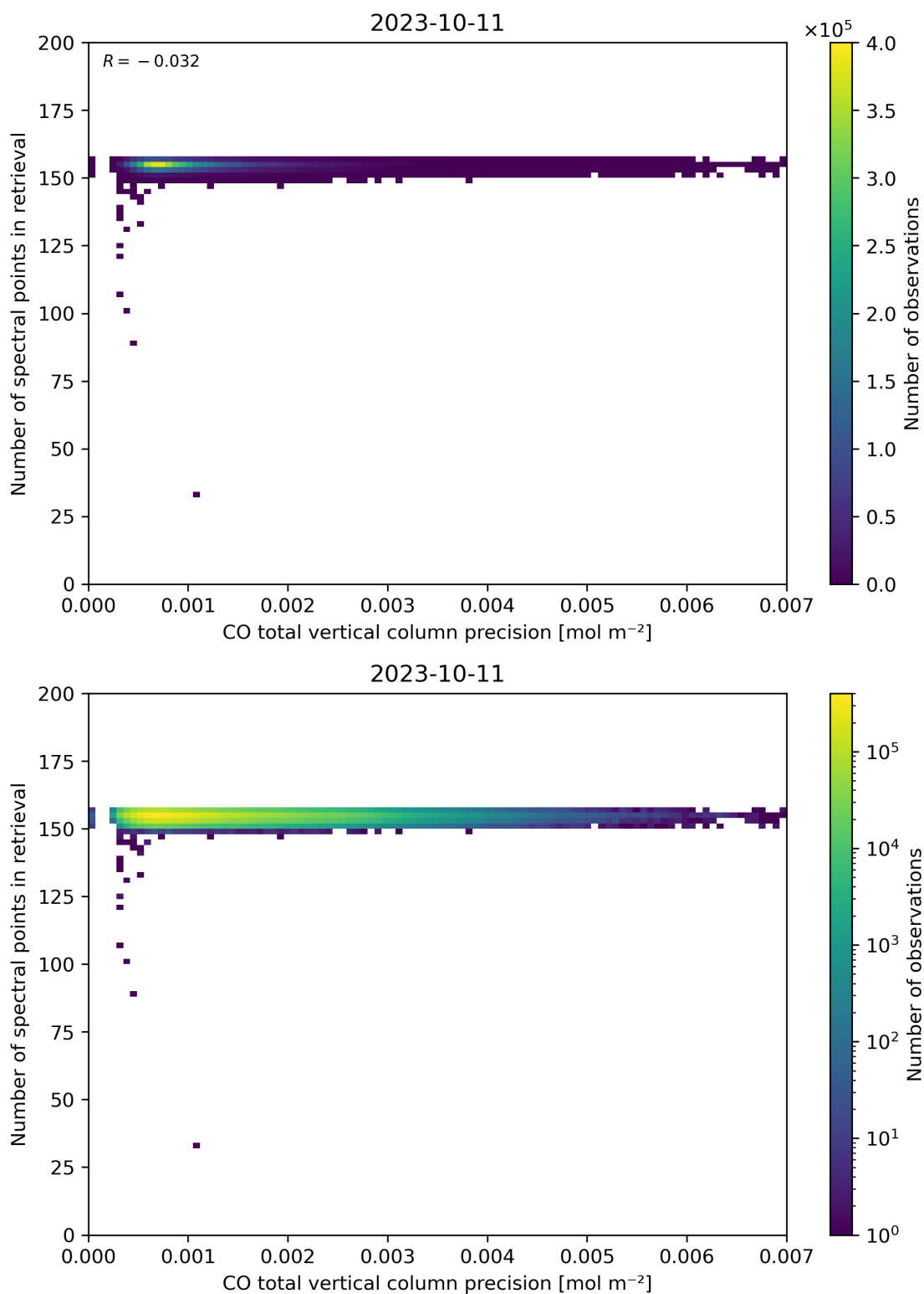
Figure 47: Scatter density plot of “CO total vertical column precision” against “Number of spectral points in retrieval” for 2023-10-10 to 2023-10-12.
