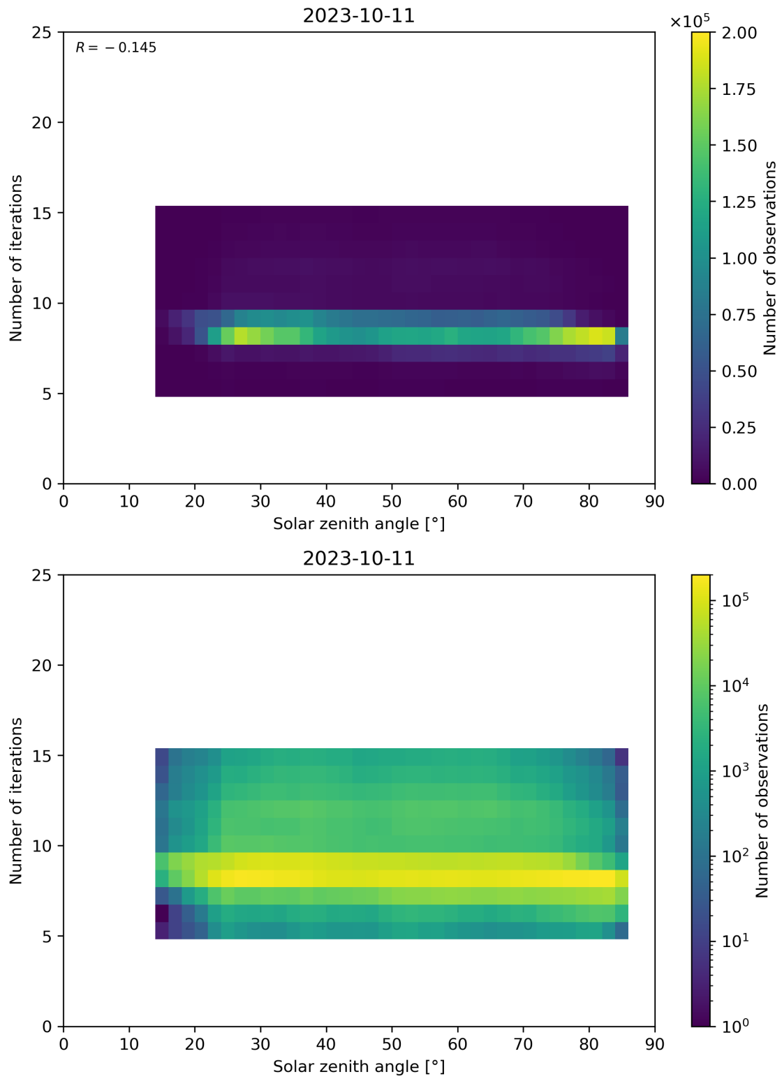
Figure 67: Scatter density plot of “Solar zenith angle” against “Number of iterations” for 2023-10-10 to 2023-10-12.
