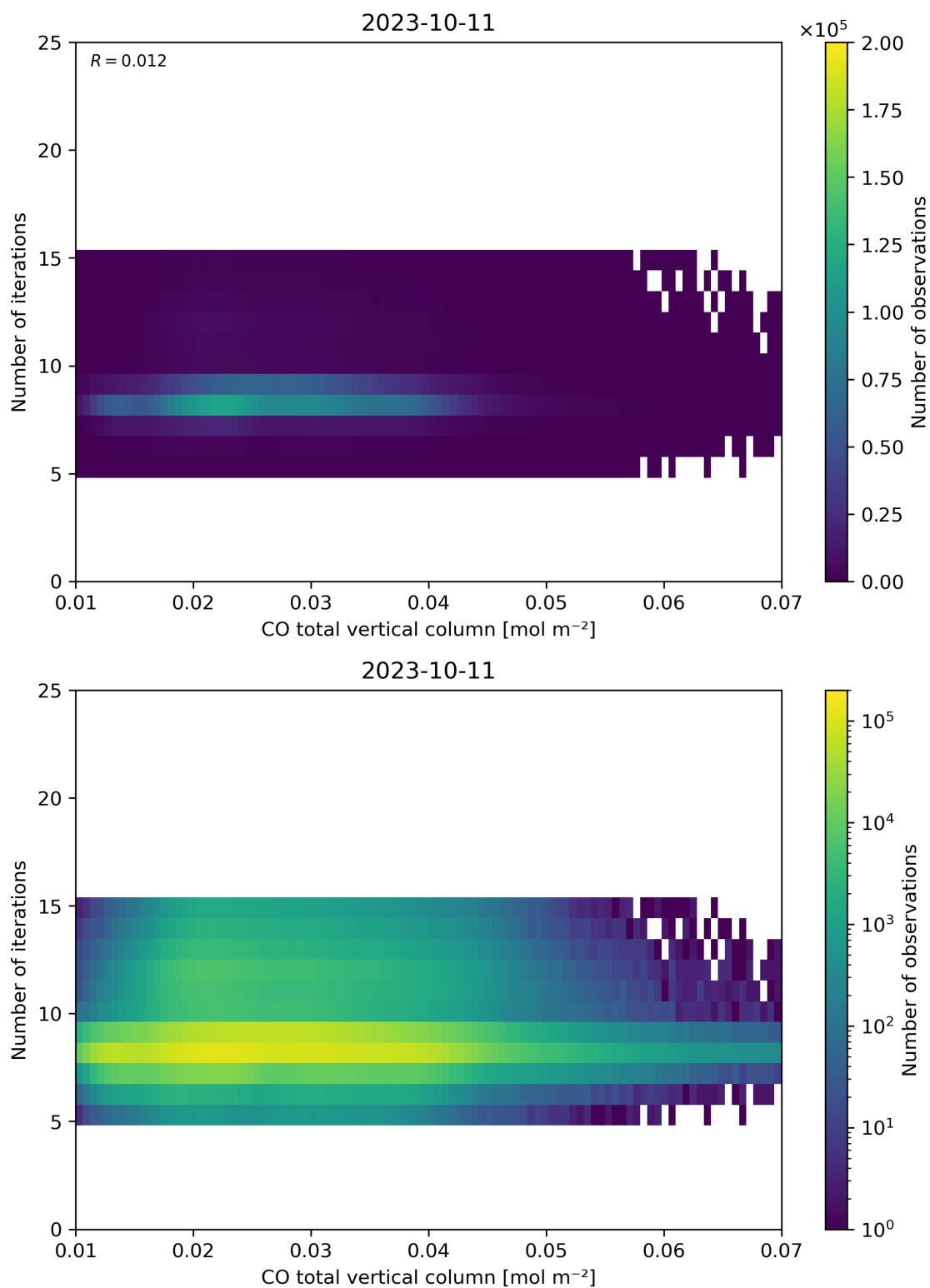
Figure 42: Scatter density plot of “CO total vertical column” against “Number of iterations” for 2023-10-10 to 2023-10-12.
