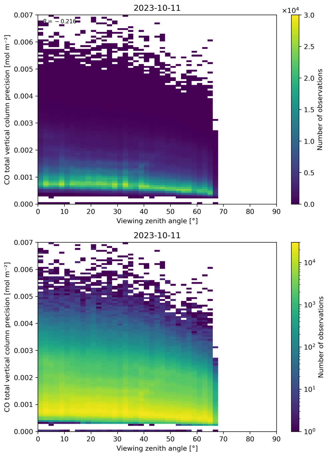
Figure 71: Scatter density plot of “Viewing zenith angle” against “CO total vertical column precision” for 2023-10-10 to 2023-10-12.
