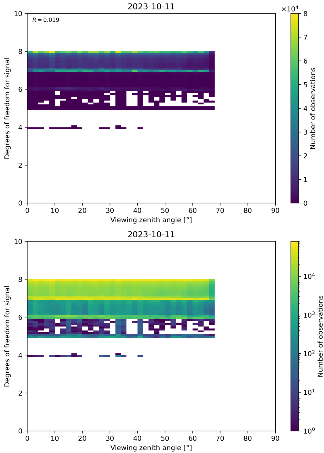
Figure 73: Scatter density plot of “Viewing zenith angle” against “Degrees of freedom for signal” for 2023-10-10 to 2023-10-12.
