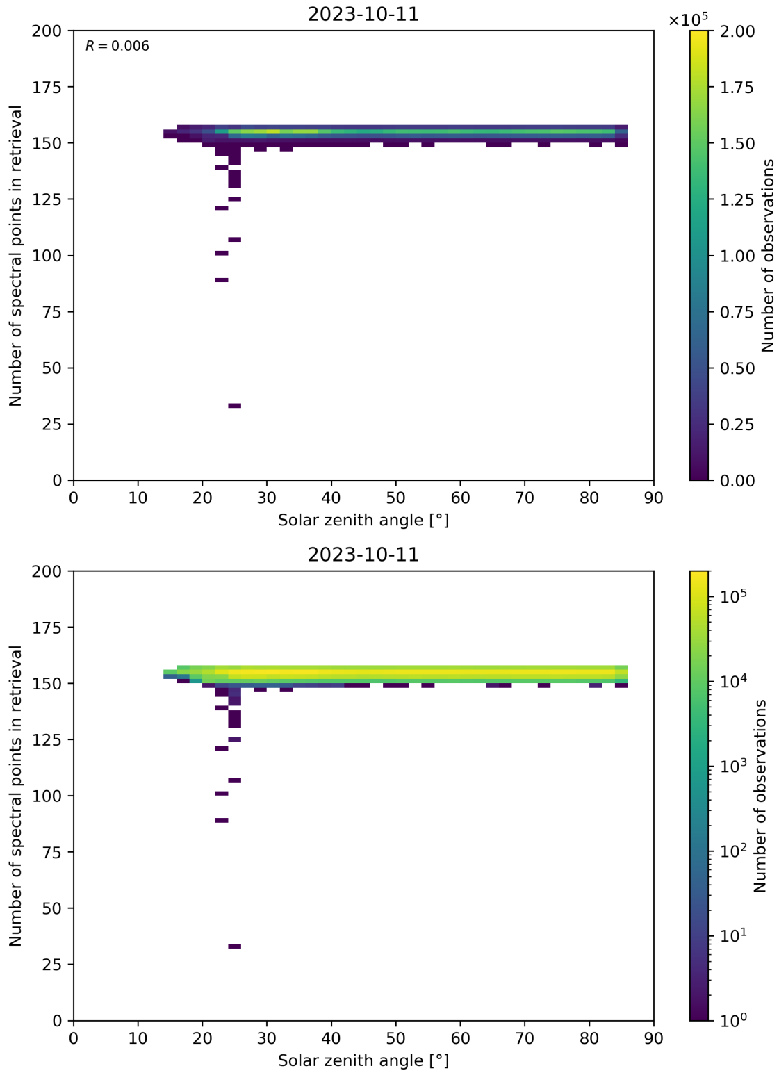
Figure 68: Scatter density plot of “Solar zenith angle” against “Number of spectral points in retrieval” for 2023-10-10 to 2023-10-12.
