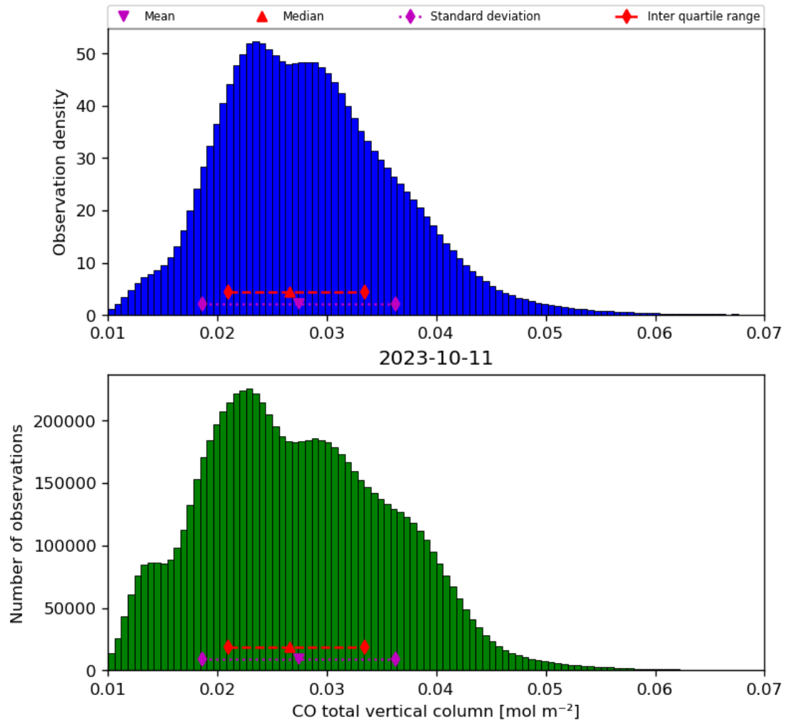
Figure 18: Histogram of “CO total vertical column” for 2023-10-10 to 2023-10-12
