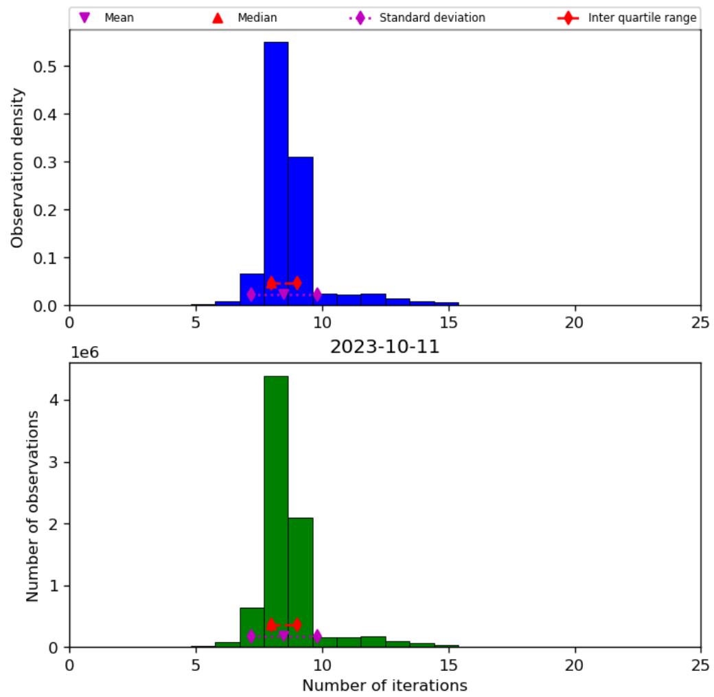
Figure 24: Histogram of “Number of iterations” for 2023-10-10 to 2023-10-12
