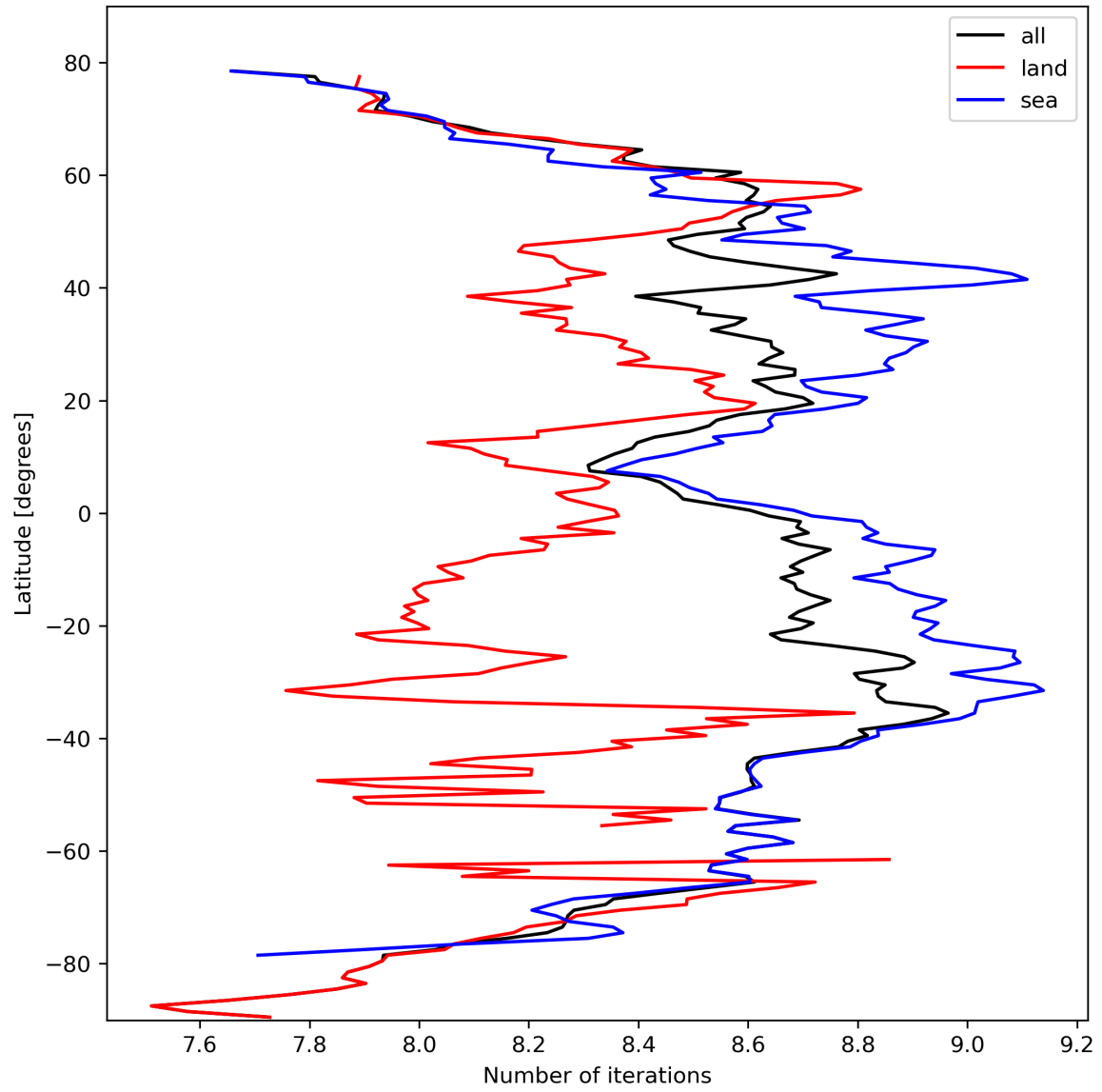
Figure 16: Zonal average of “Number of iterations” for 2023-10-10 to 2023-10-12.
