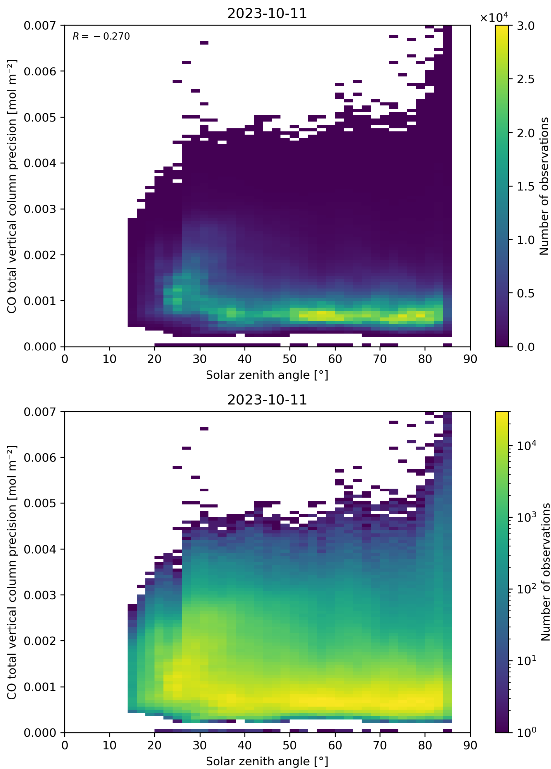
Figure 63: Scatter density plot of “Solar zenith angle” against “CO total vertical column precision” for 2023-10-10 to 2023-10-12.
