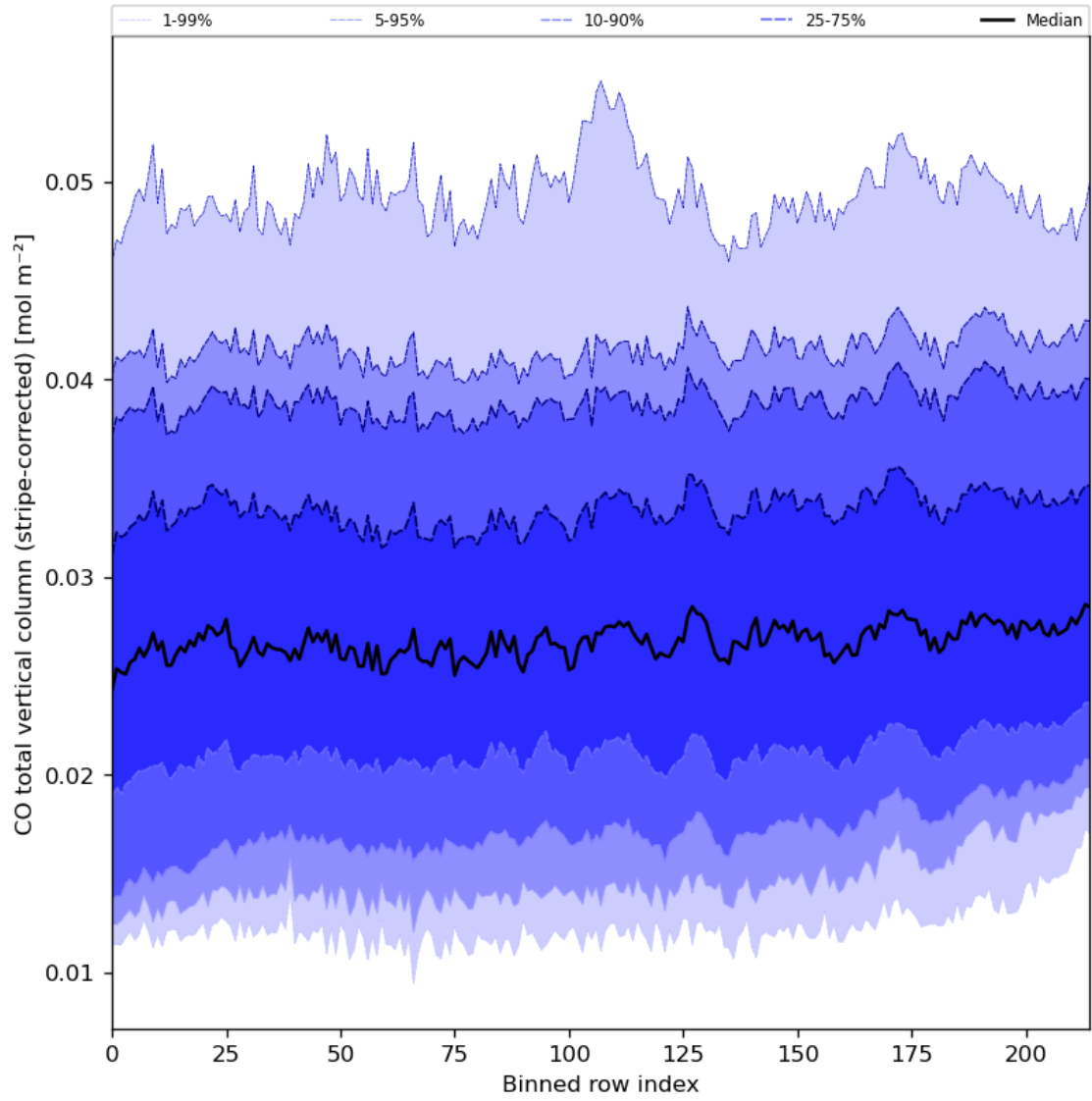
Figure 27: Along track statistics of “CO total vertical column (stripe-corrected)” for 2023-10-10 to 2023-10-12
