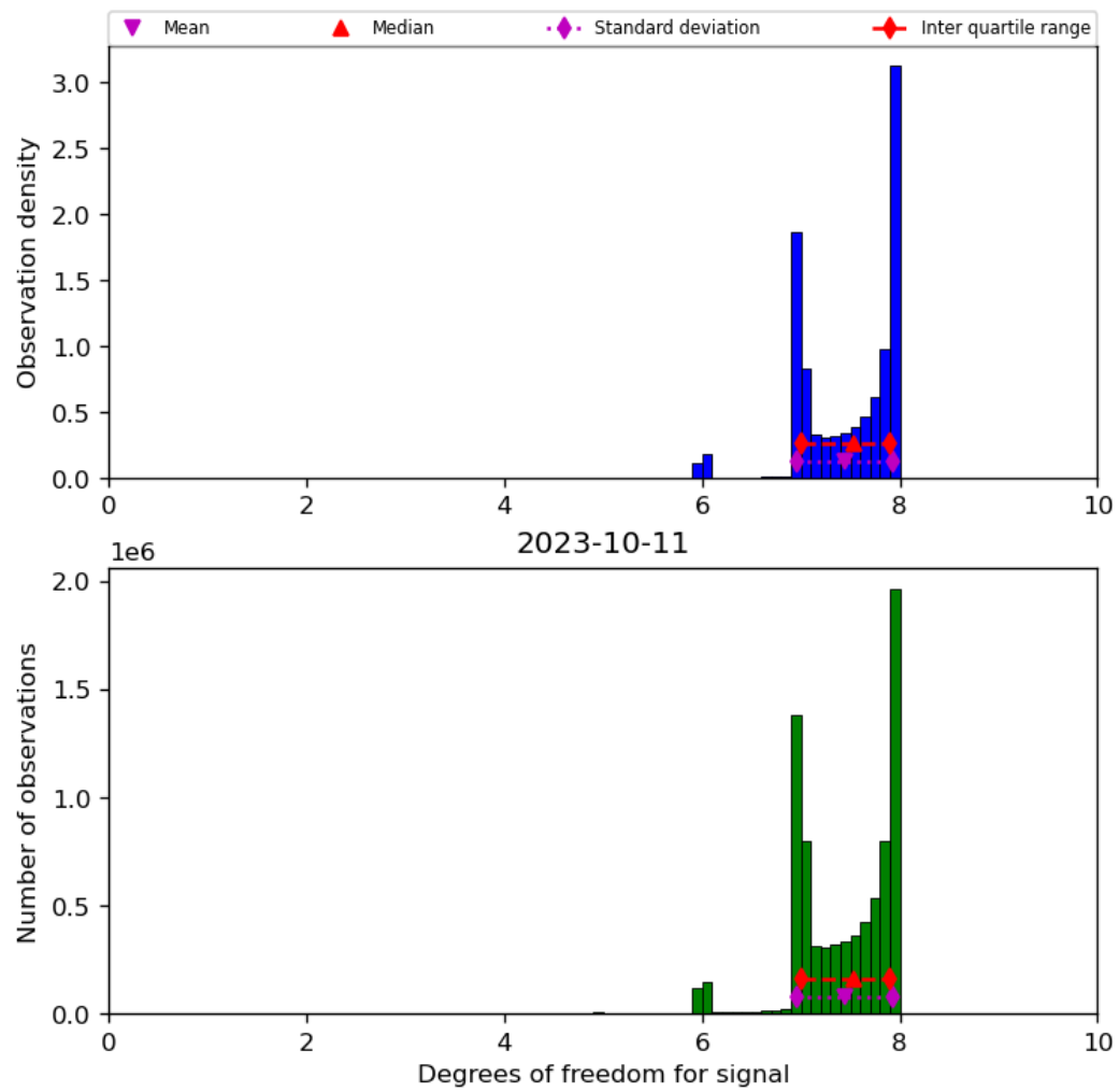
Figure 23: Histogram of “Degrees of freedom for signal” for 2023-10-10 to 2023-10-12
