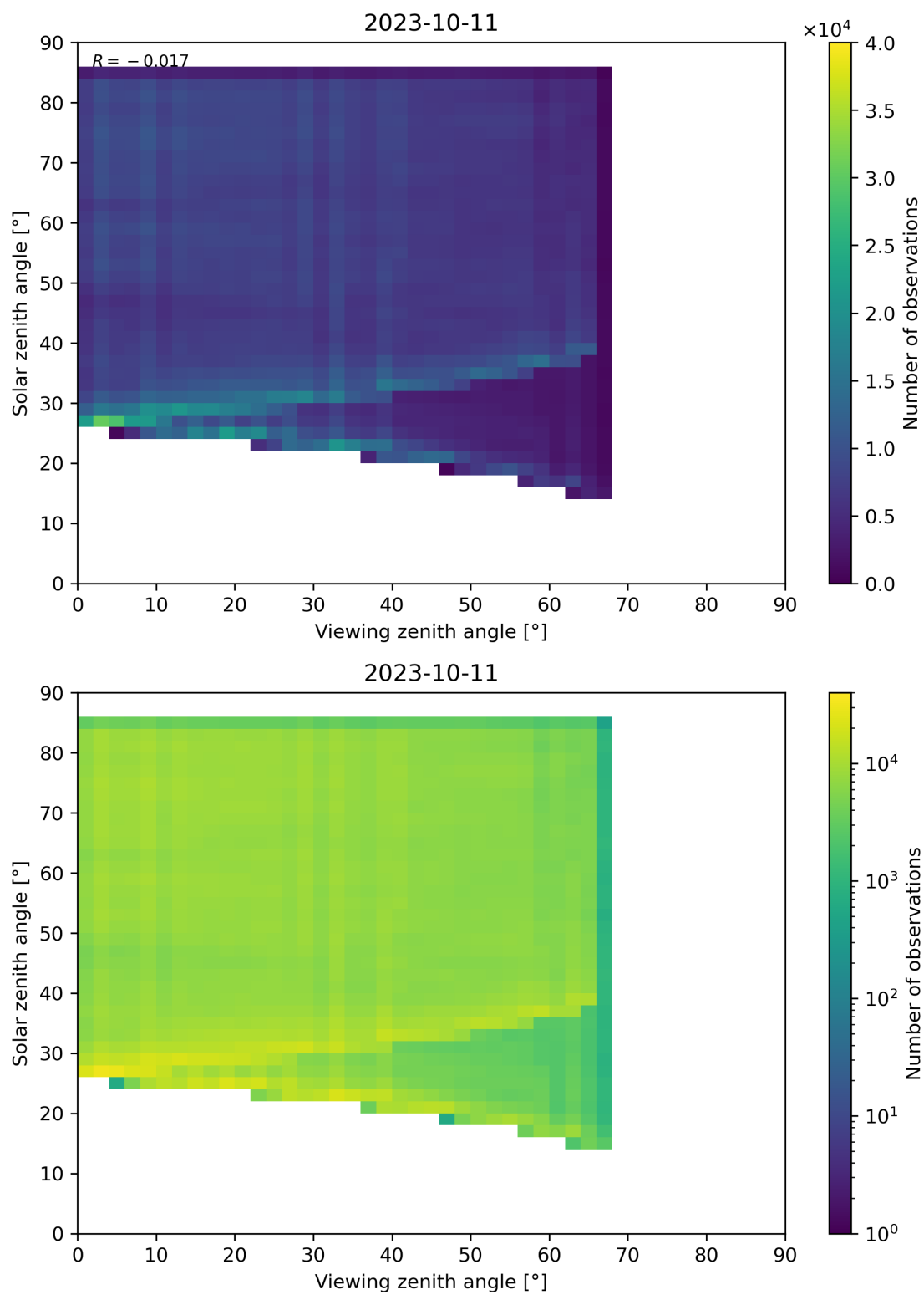
Figure 77: Scatter density plot of “Viewing zenith angle” against “Solar zenith angle” for 2023-10-10 to 2023-10-12.
