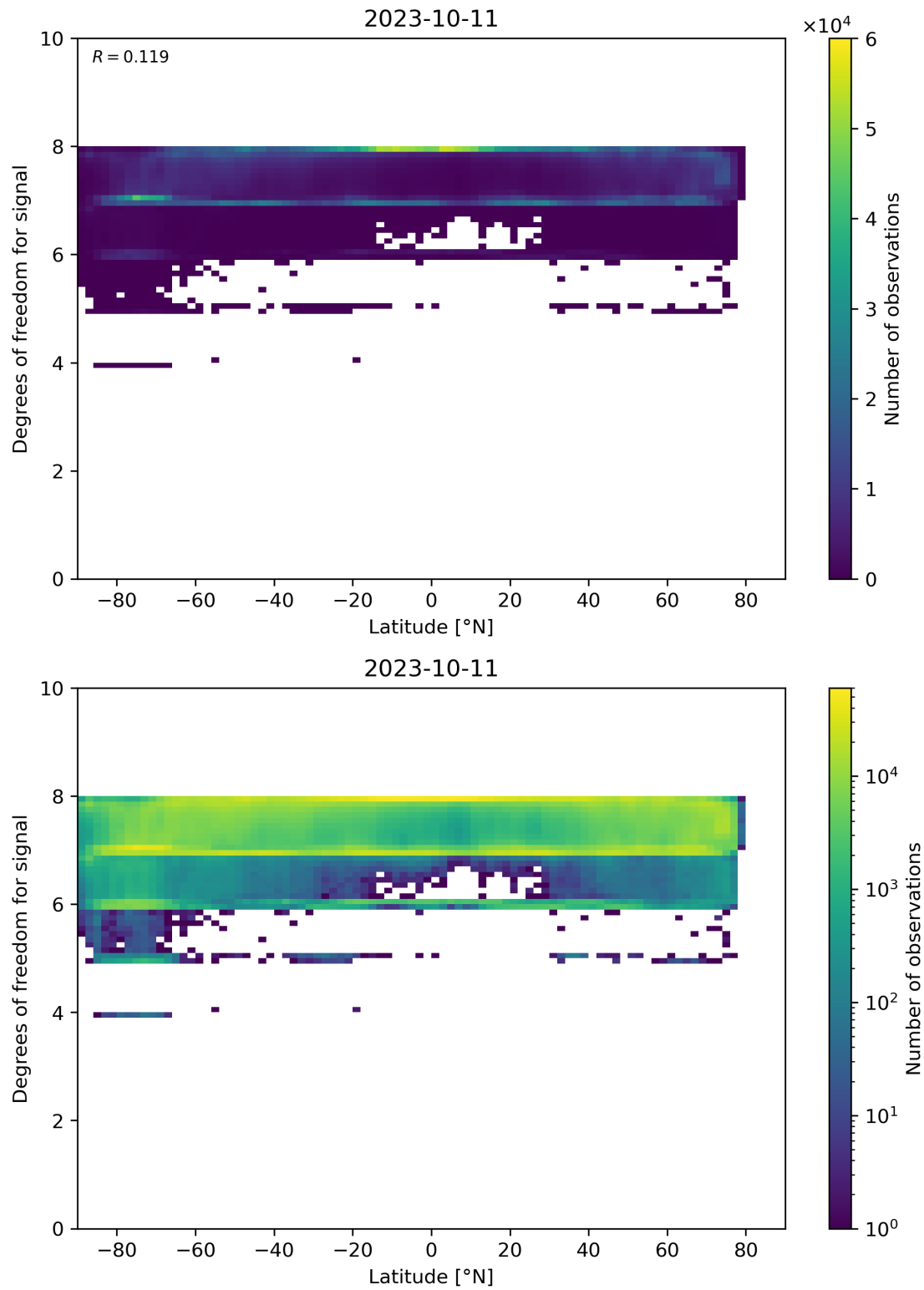
Figure 55: Scatter density plot of “Latitude” against “Degrees of freedom for signal” for 2023-10-10 to 2023-10-12.
