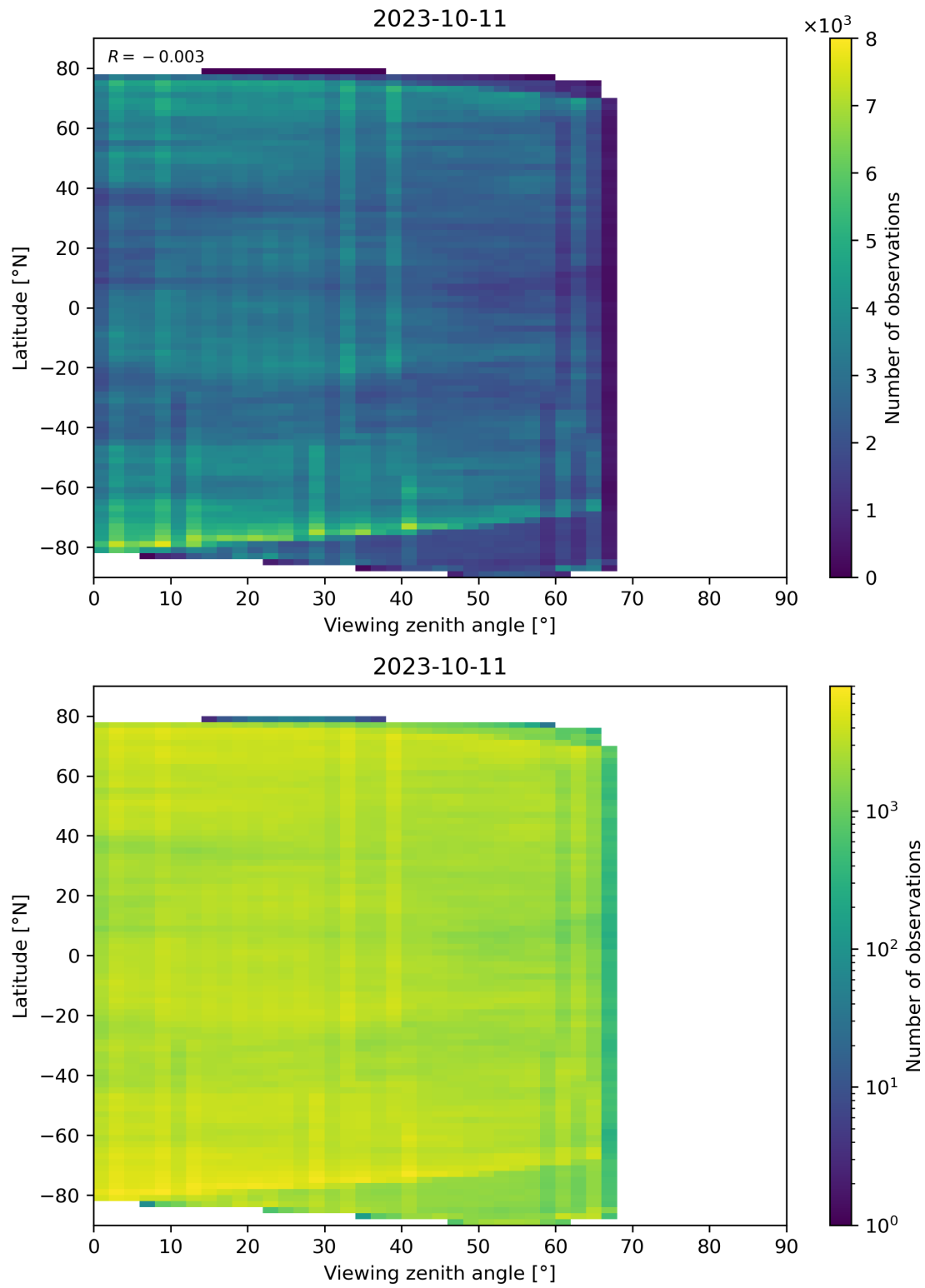
Figure 74: Scatter density plot of “Viewing zenith angle” against “Latitude” for 2023-10-10 to 2023-10-12.
