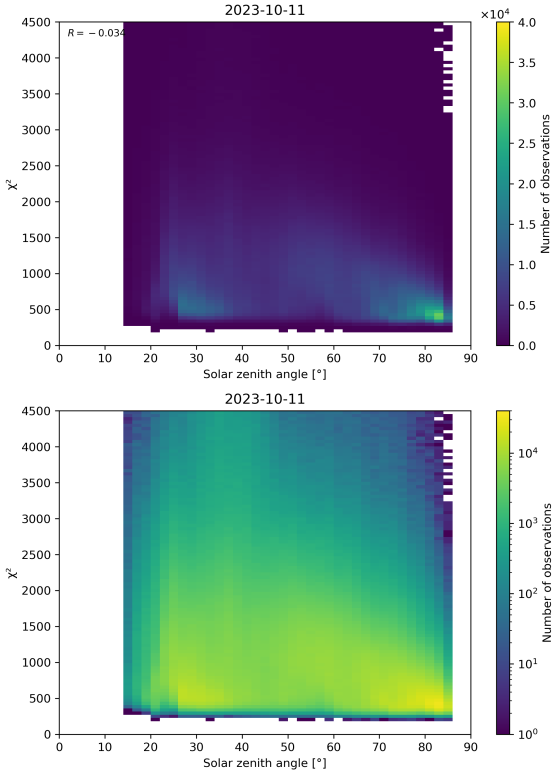
Figure 64: Scatter density plot of “Solar zenith angle” against “ \chi^2 ” for 2023-10-10 to 2023-10-12.
