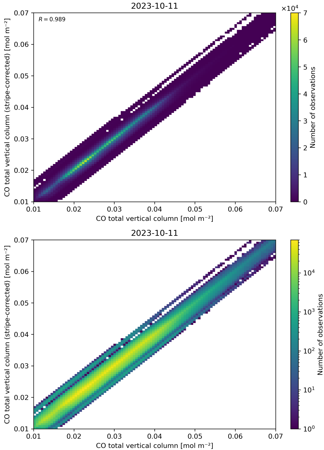
Figure 33: Scatter density plot of “CO total vertical column” against “CO total vertical column (stripe-corrected)” for 2023-10-10 to 2023-10-12.
