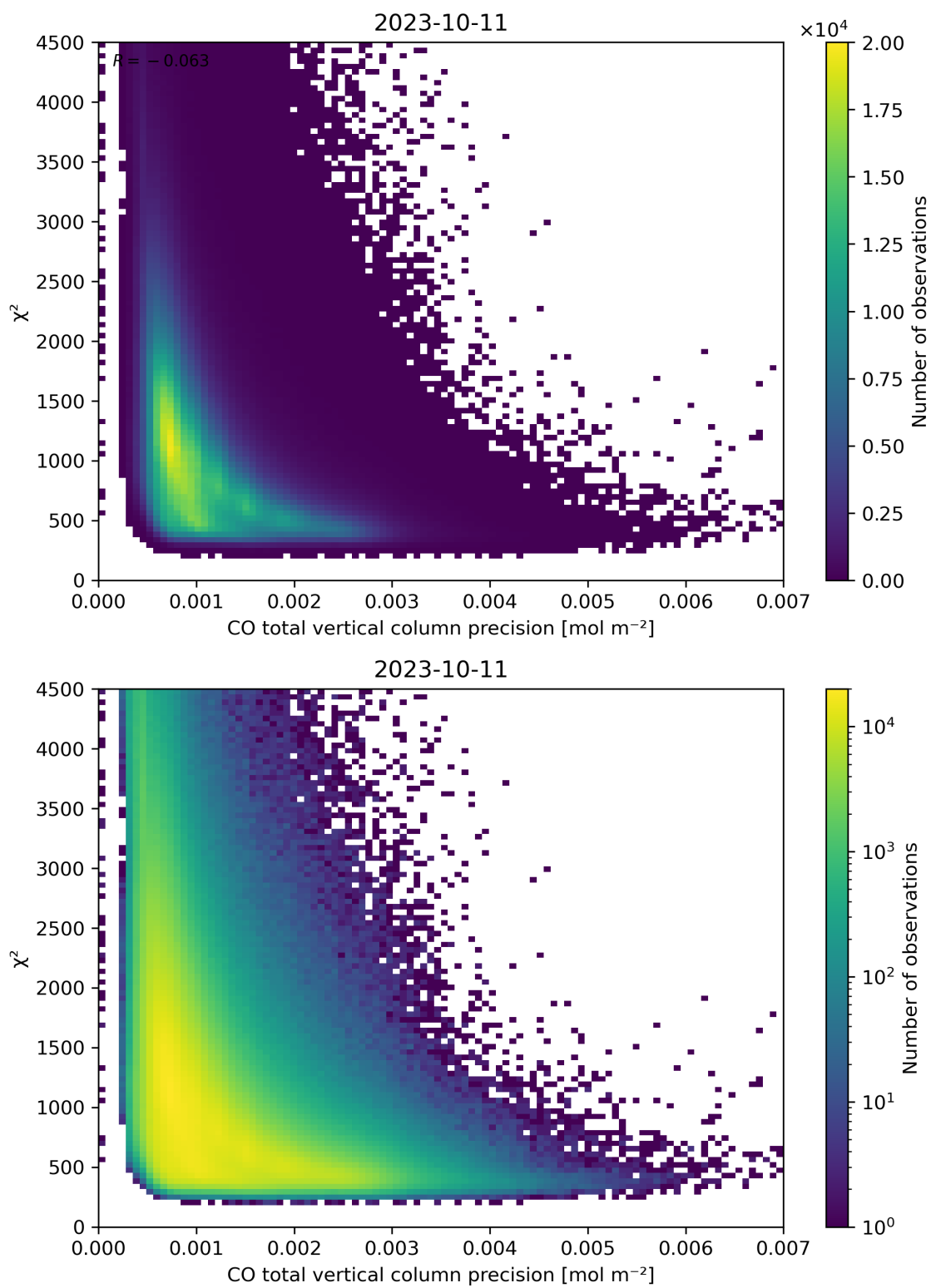
Figure 44: Scatter density plot of “CO total vertical column precision” against “ \chi^2 ” for 2023-10-10 to 2023-10-12.
