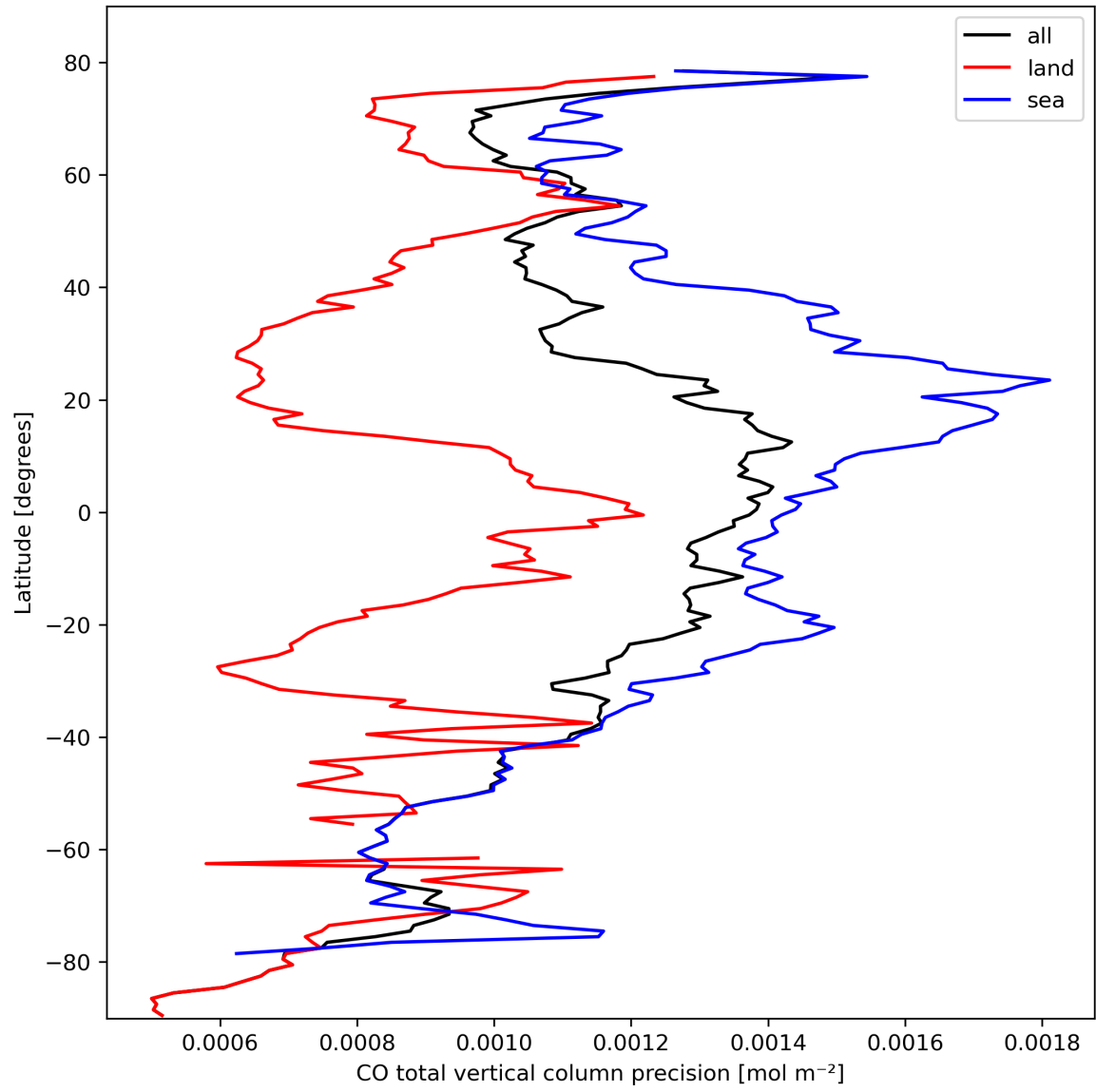
Figure 12: Zonal average of “CO total vertical column precision” for 2023-10-10 to 2023-10-12.
