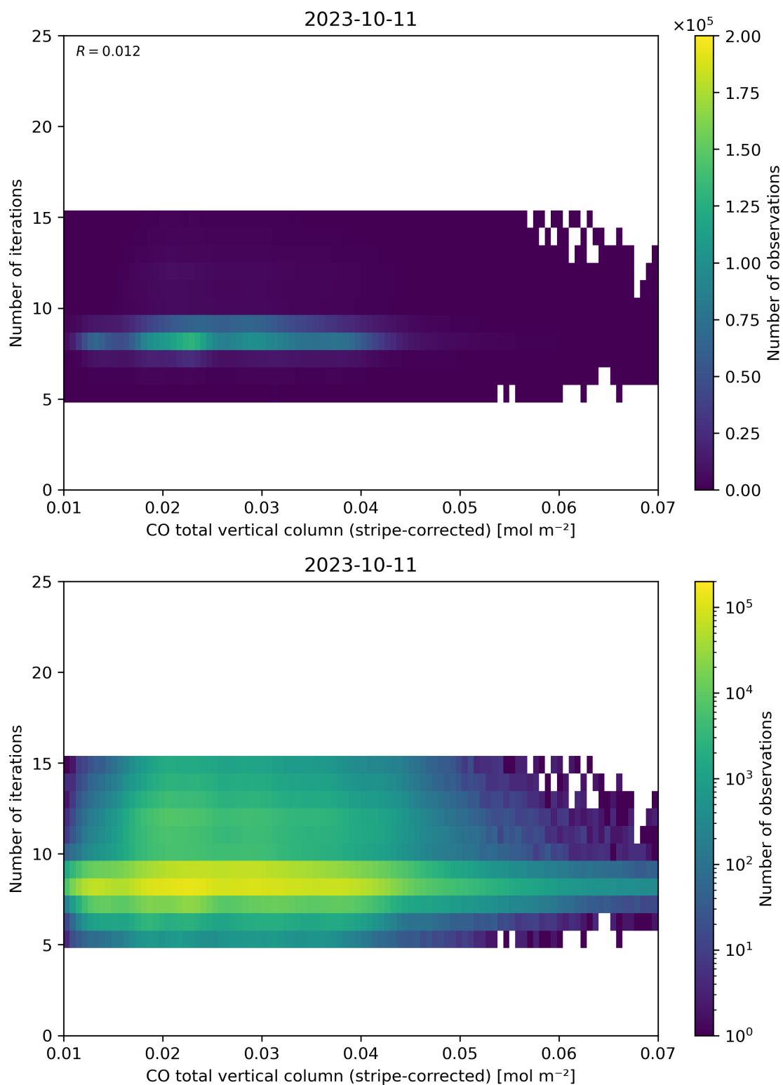
Figure 39: Scatter density plot of “CO total vertical column (stripe-corrected)” against “Number of iterations” for 2023-10-10 to 2023-10-12.
