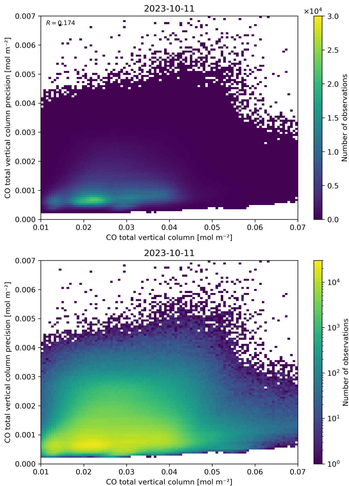
Figure 34: Scatter density plot of “CO total vertical column” against “CO total vertical column precision” for 2023-10-10 to 2023-10-12.
