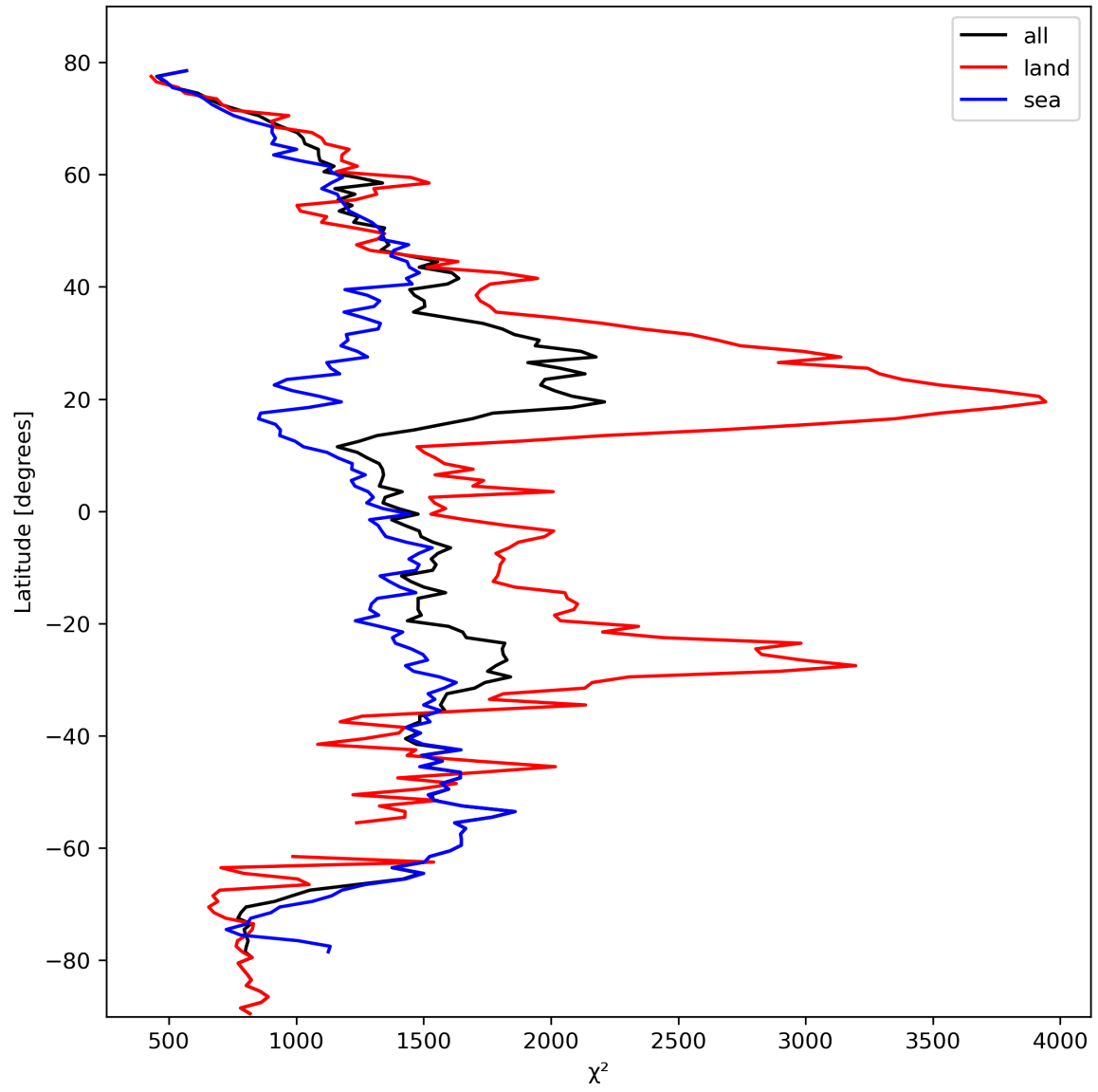
Figure 14: Zonal average of “ \chi^2 ” for 2023-10-10 to 2023-10-12.
