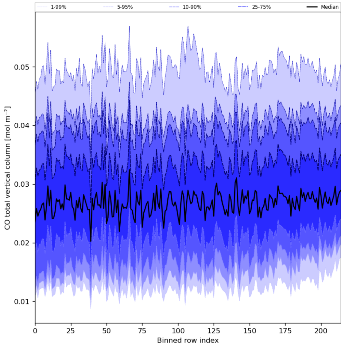
Figure 26: Along track statistics of “CO total vertical column” for 2023-10-10 to 2023-10-12
