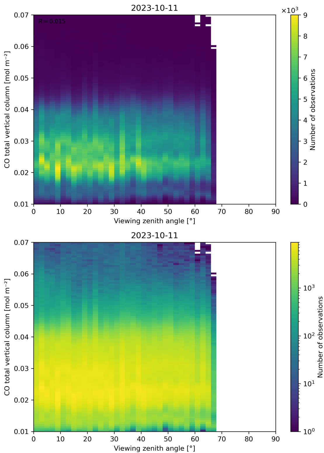
Figure 69: Scatter density plot of “Viewing zenith angle” against “CO total vertical column” for 2023-10-10 to 2023-10-12.
