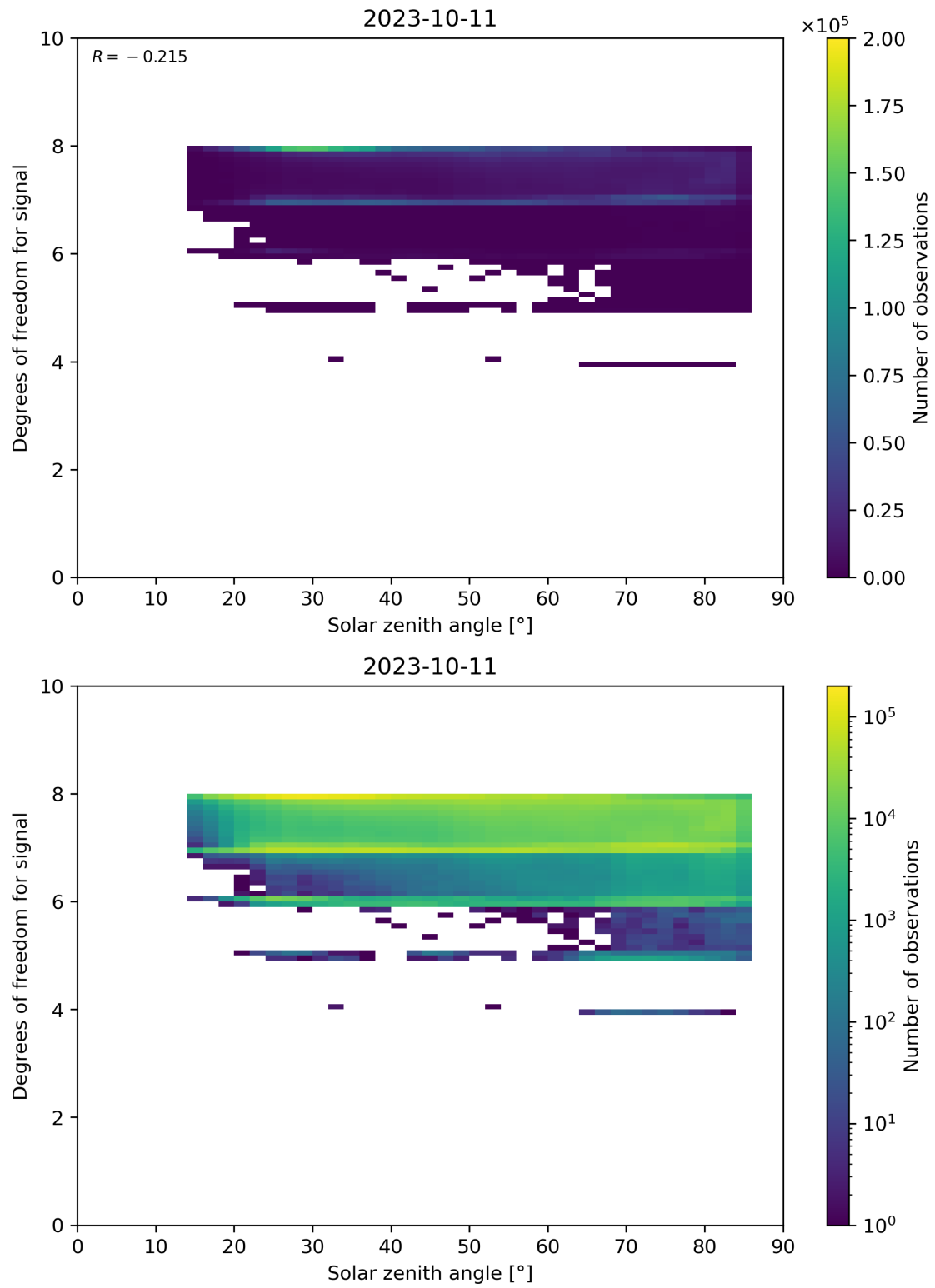
Figure 65: Scatter density plot of “Solar zenith angle” against “Degrees of freedom for signal” for 2023-10-10 to 2023-10-12.
