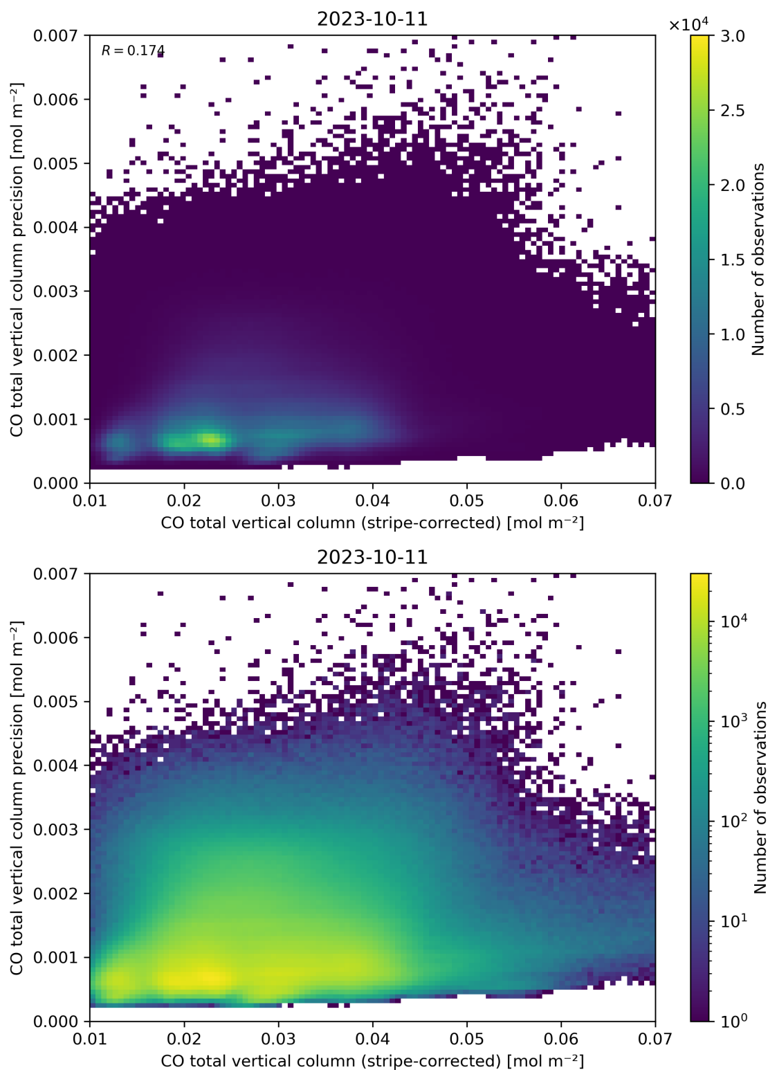
Figure 36: Scatter density plot of “CO total vertical column (stripe-corrected)” against “CO total vertical column precision” for 2023-10-10 to 2023-10-12.
