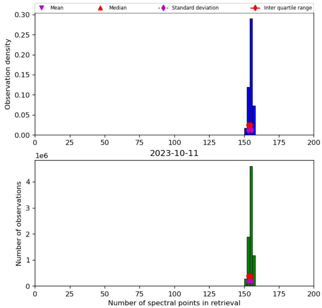
Figure 21: Histogram of “Number of spectral points in retrieval” for 2023-10-10 to 2023-10-12
