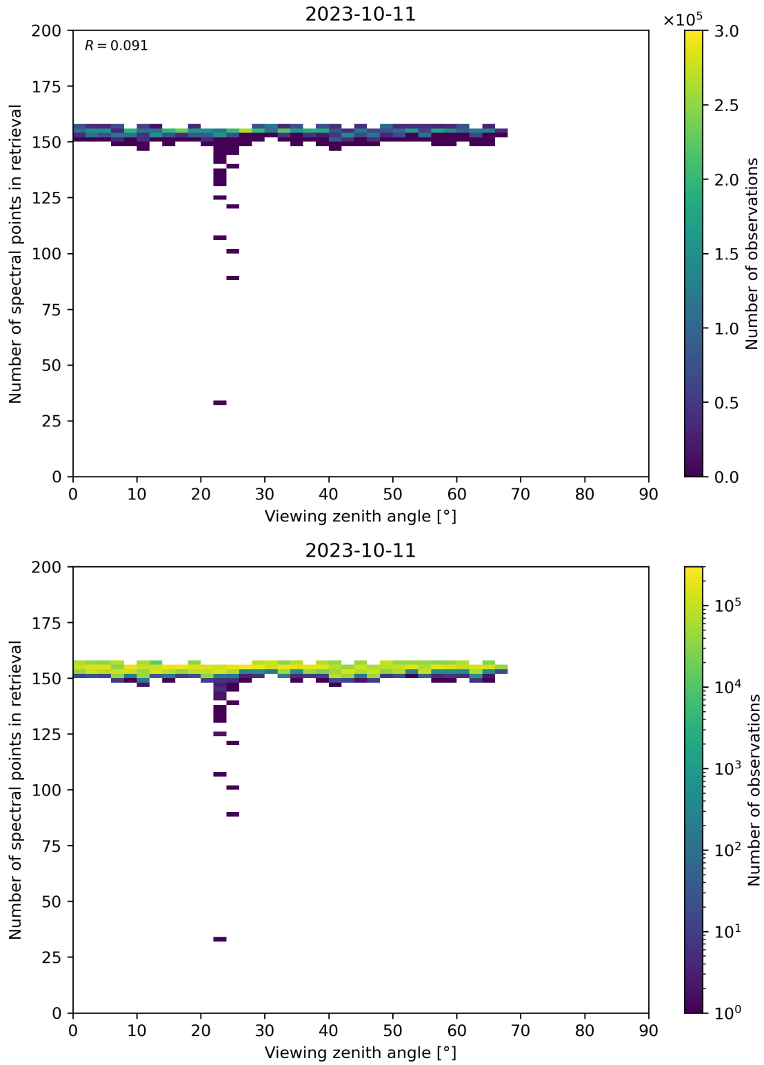
Figure 76: Scatter density plot of “Viewing zenith angle” against “Number of spectral points in retrieval” for 2023-10-10 to 2023-10-12.
