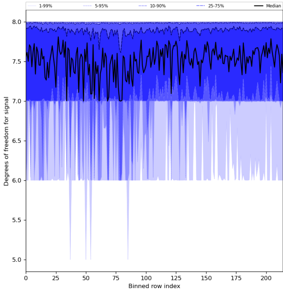
Figure 31: Along track statistics of “Degrees of freedom for signal” for 2023-10-10 to 2023-10-12
