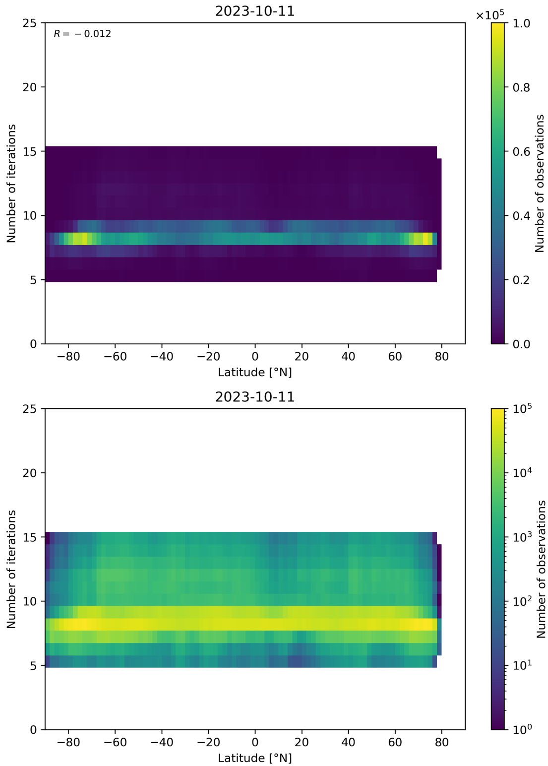
Figure 56: Scatter density plot of “Latitude” against “Number of iterations” for 2023-10-10 to 2023-10-12.
