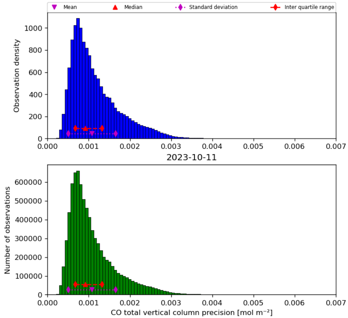
Figure 20: Histogram of “CO total vertical column precision” for 2023-10-10 to 2023-10-12
