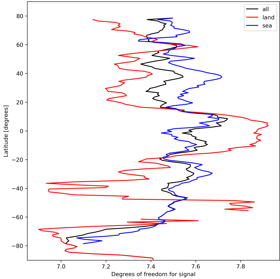
Figure 15: Zonal average of “Degrees of freedom for signal” for 2023-10-10 to 2023-10-12.
