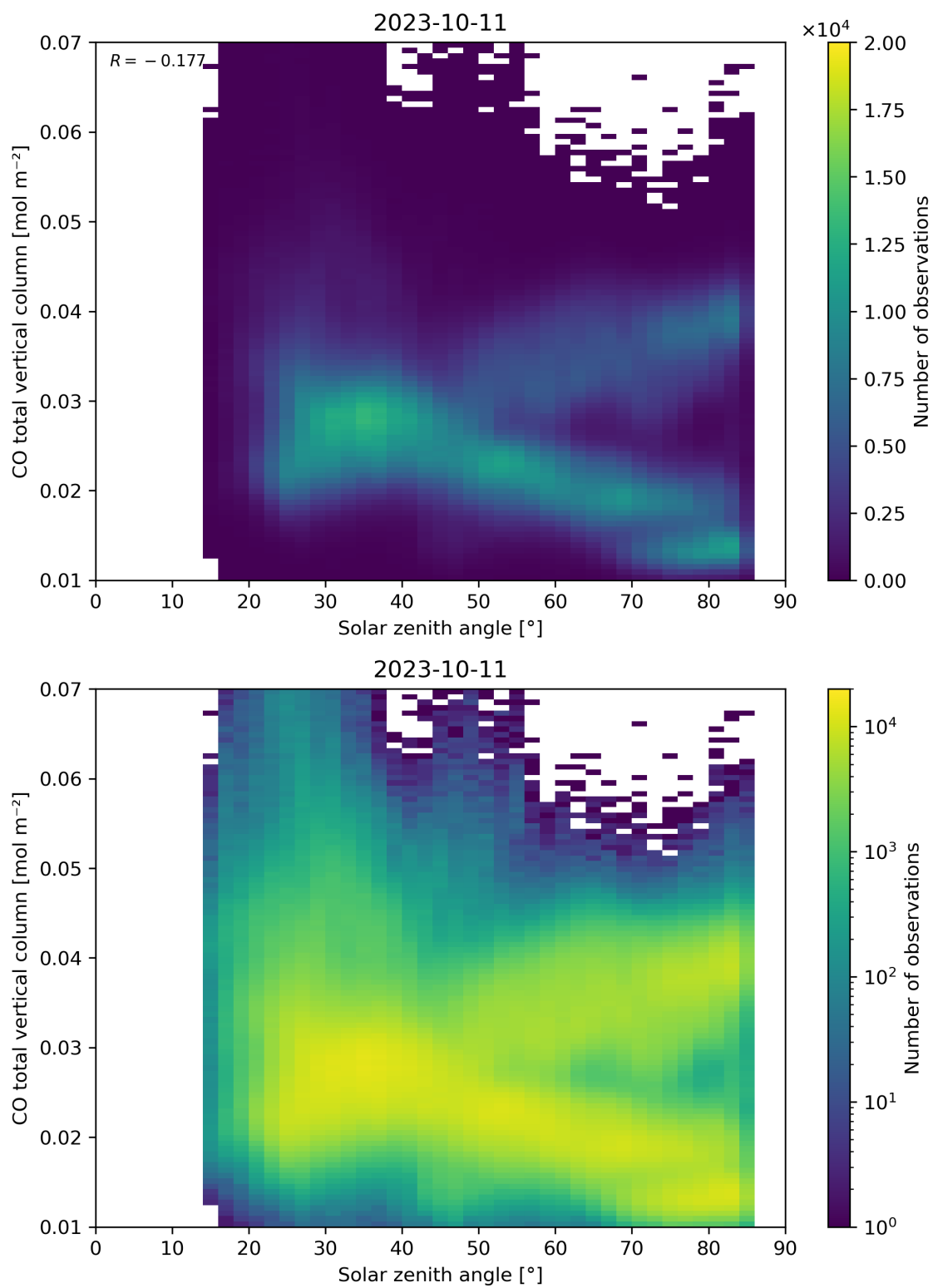
Figure 61: Scatter density plot of “Solar zenith angle” against “CO total vertical column” for 2023-10-10 to 2023-10-12.
