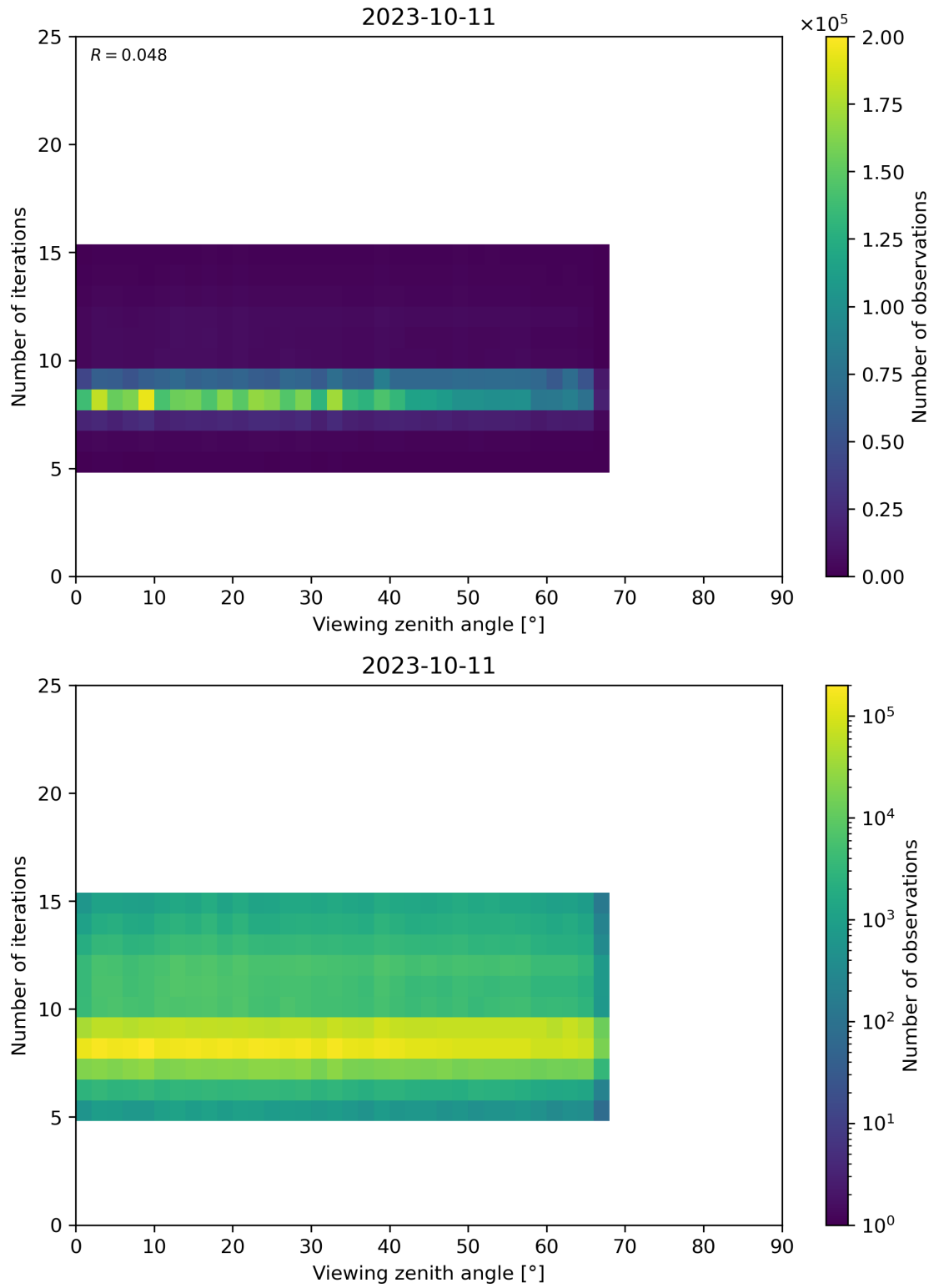
Figure 75: Scatter density plot of “Viewing zenith angle” against “Number of iterations” for 2023-10-10 to 2023-10-12.
