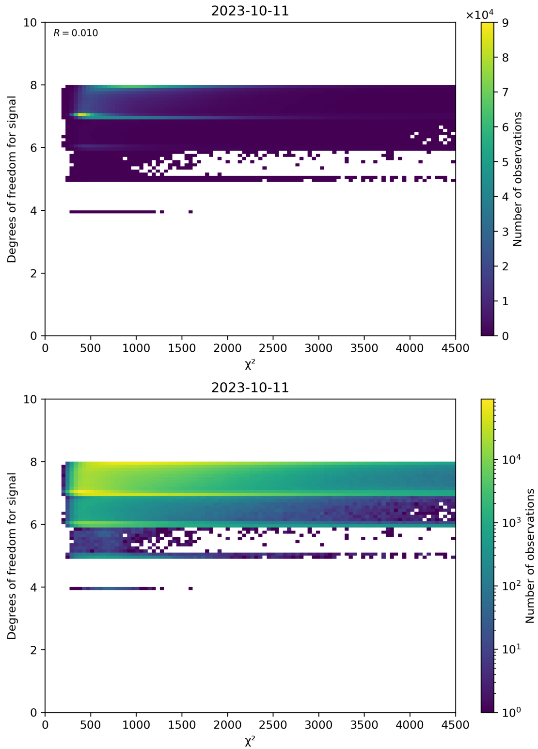
Figure 48: Scatter density plot of “ \chi^2 ” against “Degrees of freedom for signal” for 2023-10-10 to 2023-10-12.
