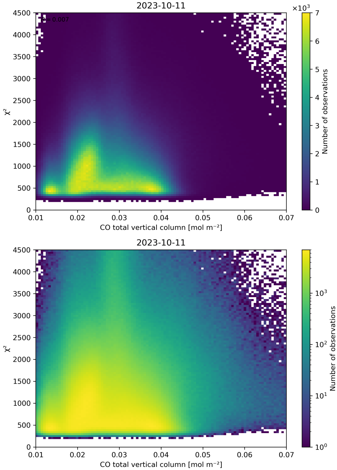
Figure 35: Scatter density plot of “CO total vertical column” against “ \chi^2 ” for 2023-10-10 to 2023-10-12.
