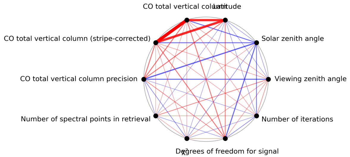
Figure 1: Map of correlation graph for 2023-10-10 to 2023-10-12.
