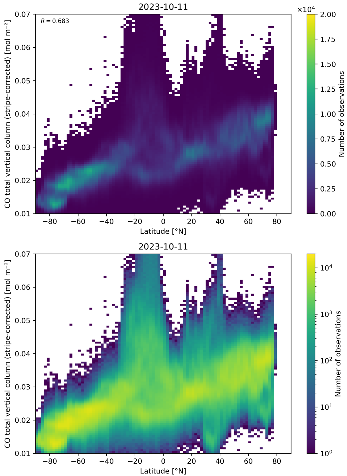
Figure 52: Scatter density plot of “Latitude” against “CO total vertical column (stripe-corrected)” for 2023-10-10 to 2023-10-12.
