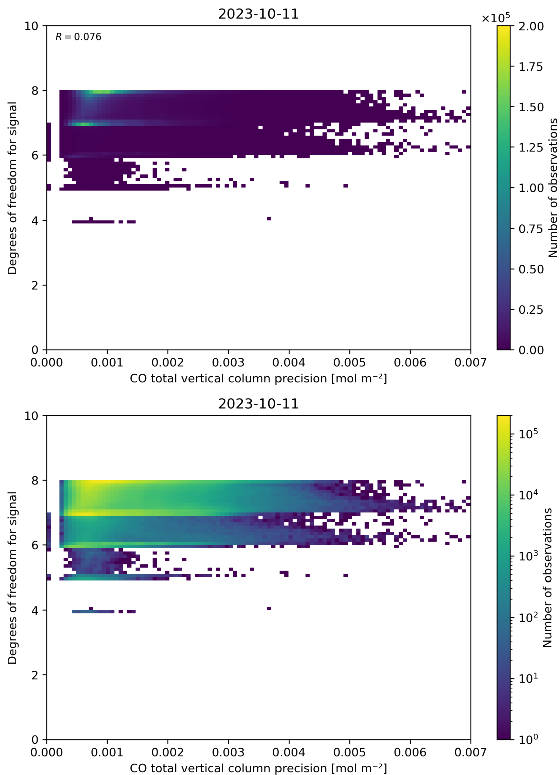
Figure 45: Scatter density plot of “CO total vertical column precision” against “Degrees of freedom for signal” for 2023-10-10 to 2023-10-12.
