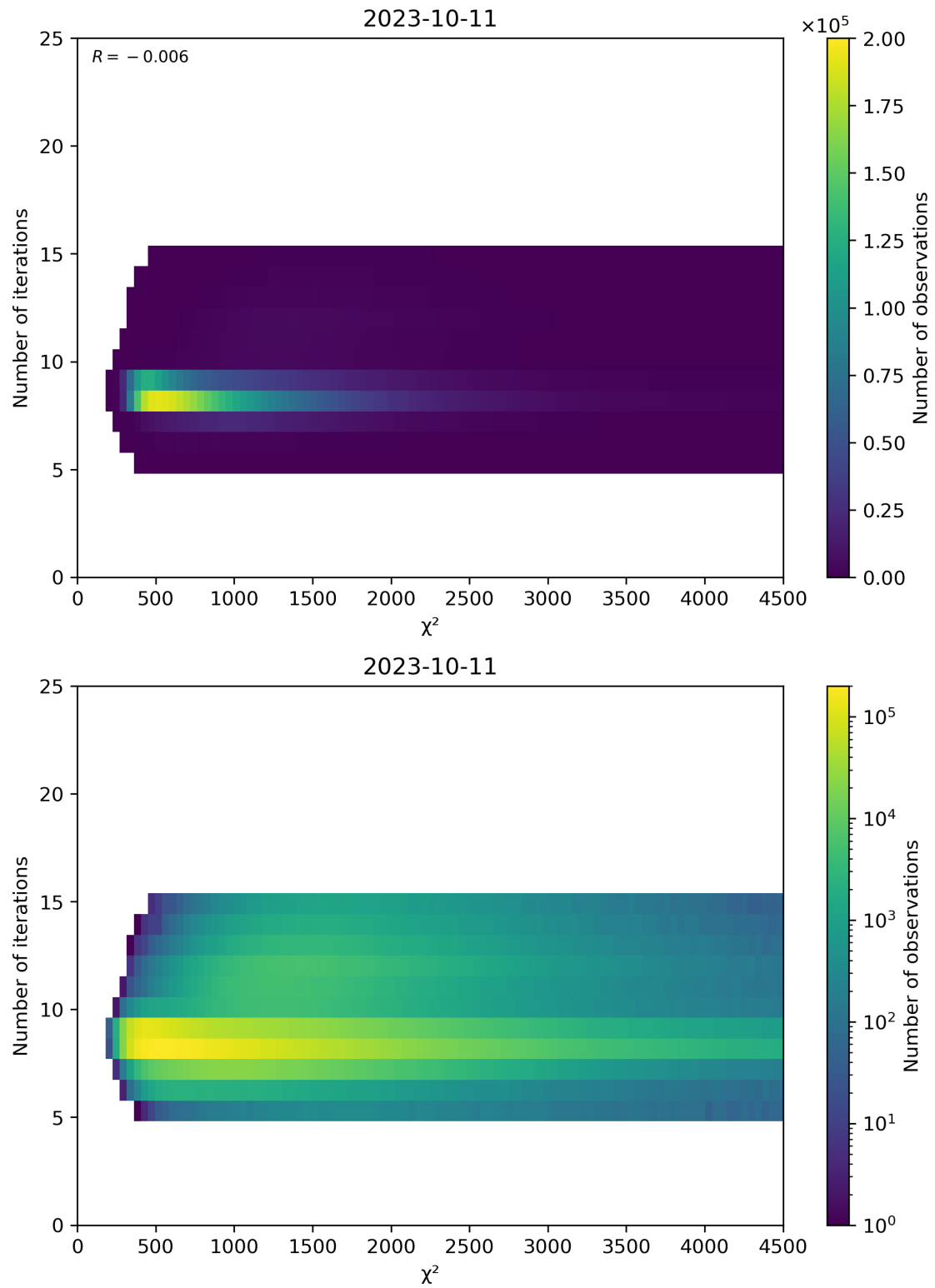
Figure 49: Scatter density plot of “ \chi^2 ” against “Number of iterations” for 2023-10-10 to 2023-10-12.
