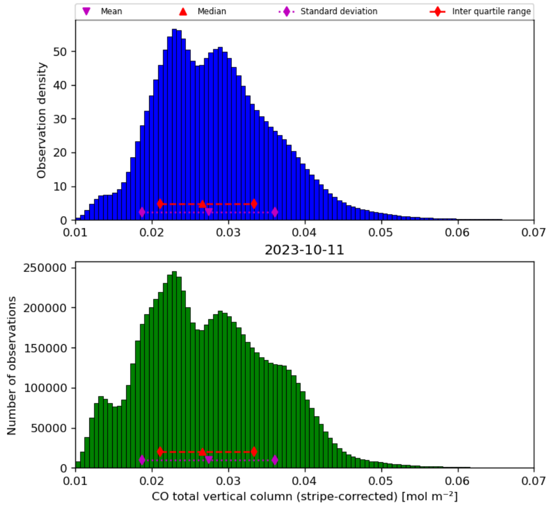
Figure 19: Histogram of “CO total vertical column (stripe-corrected)” for 2023-10-10 to 2023-10-12
