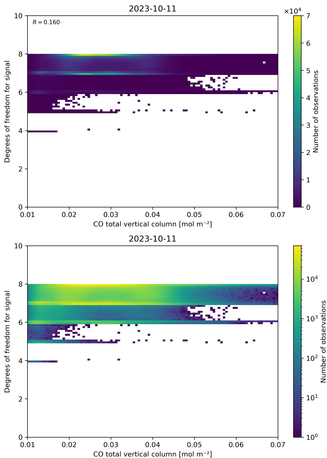
Figure 41: Scatter density plot of “CO total vertical column” against “Degrees of freedom for signal” for 2023-10-10 to 2023-10-12.
