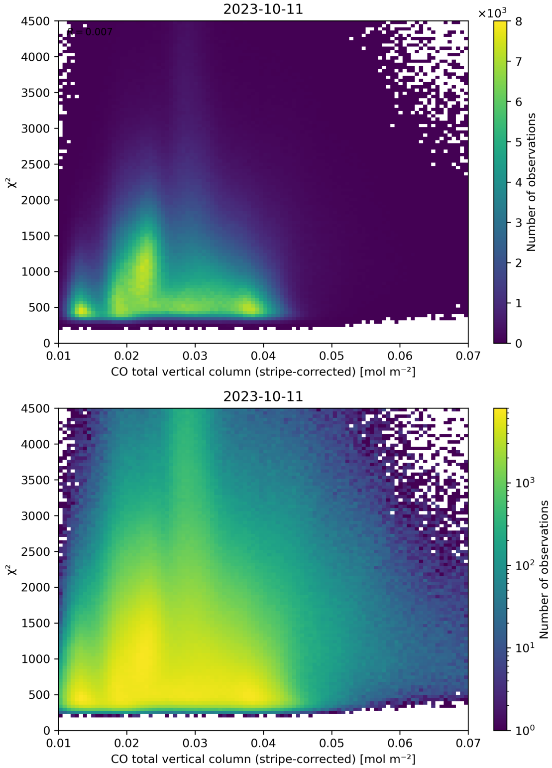
Figure 37: Scatter density plot of “CO total vertical column (stripe-corrected)” against “ \chi^2 ” for 2023-10-10 to 2023-10-12.
