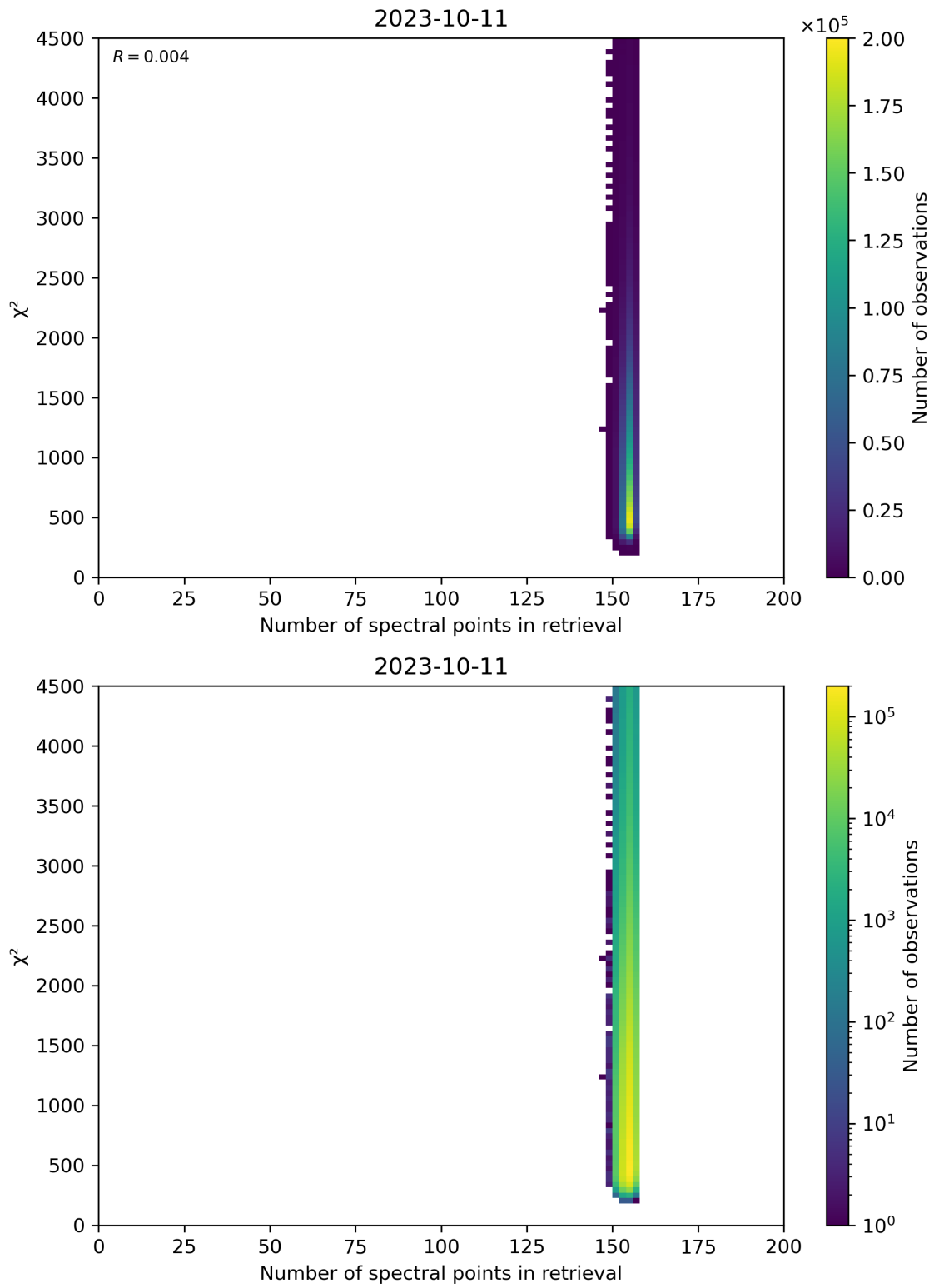
Figure 58: Scatter density plot of “Number of spectral points in retrieval” against “ \chi^2 ” for 2023-10-10 to 2023-10-12.
