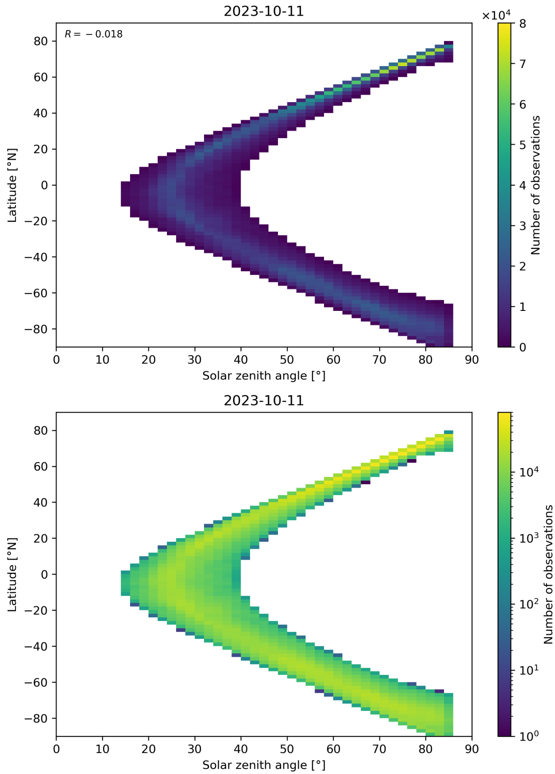
Figure 66: Scatter density plot of “Solar zenith angle” against “Latitude” for 2023-10-10 to 2023-10-12.
