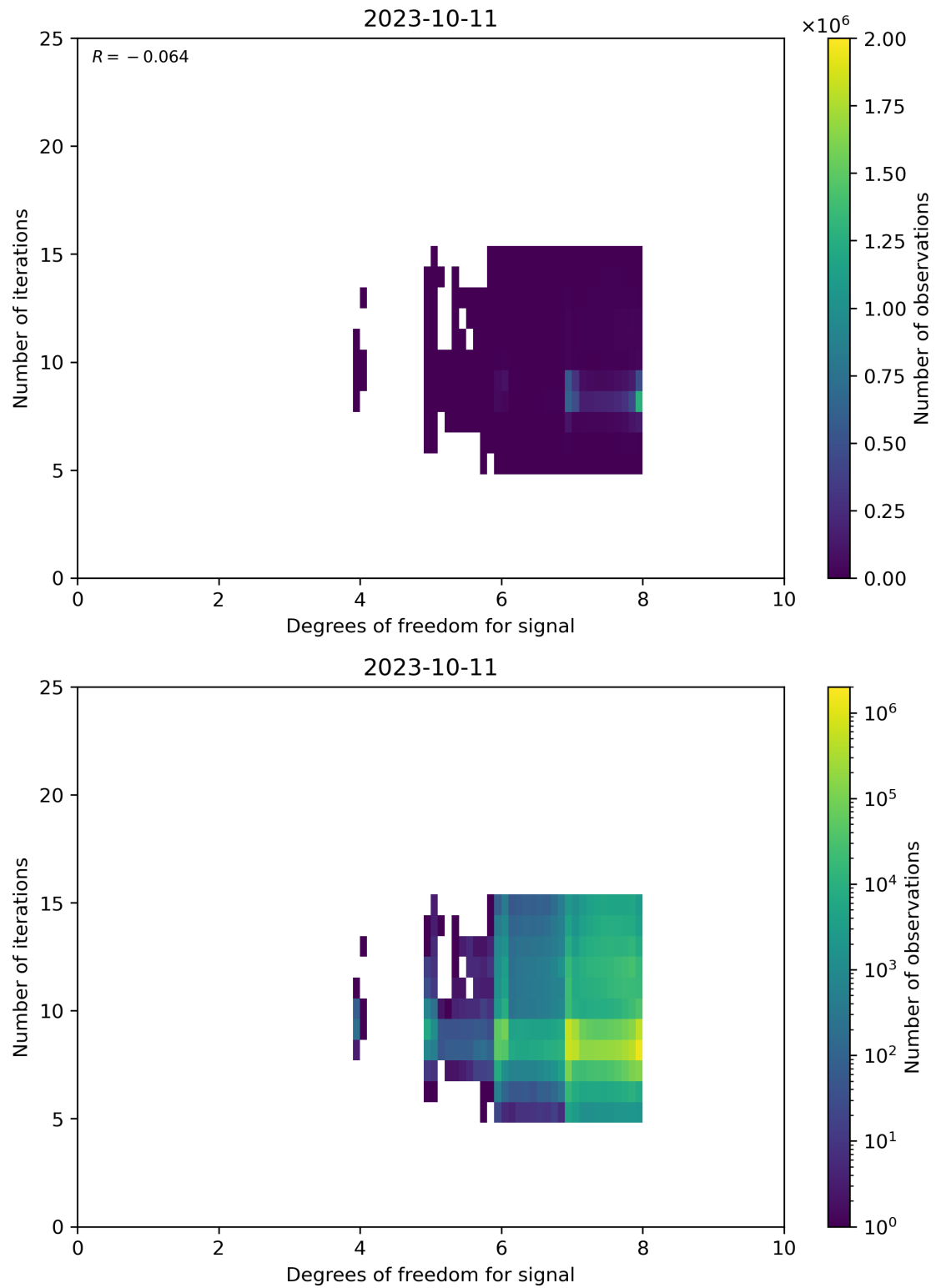
Figure 50: Scatter density plot of “Degrees of freedom for signal” against “Number of iterations” for 2023-10-10 to 2023-10-12.
