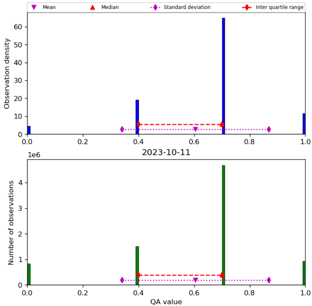
Figure 17: Histogram of “QA value” for 2023-10-10 to 2023-10-12
