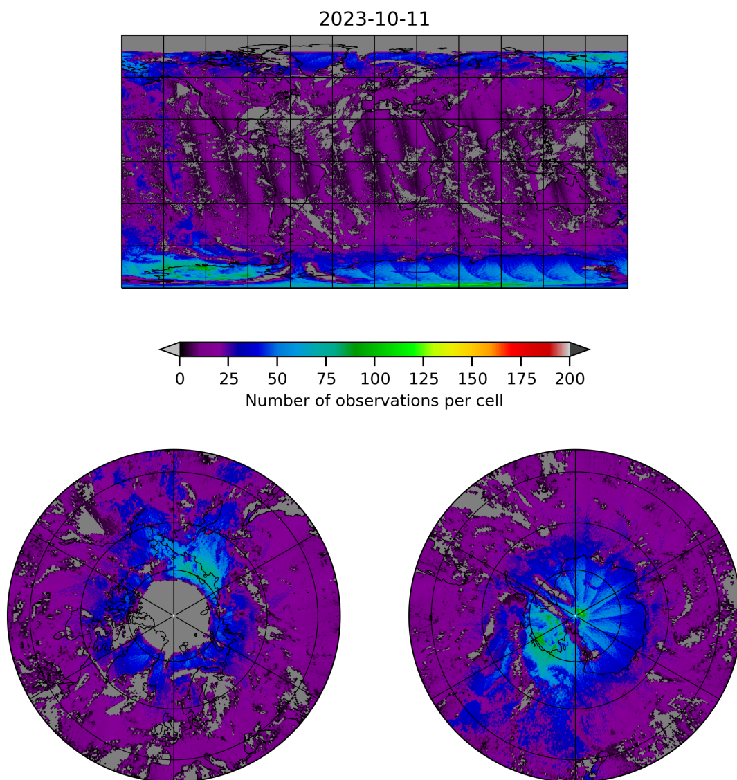
Figure 8: Map of the number of observations for 2023-10-10 to 2023-10-12
