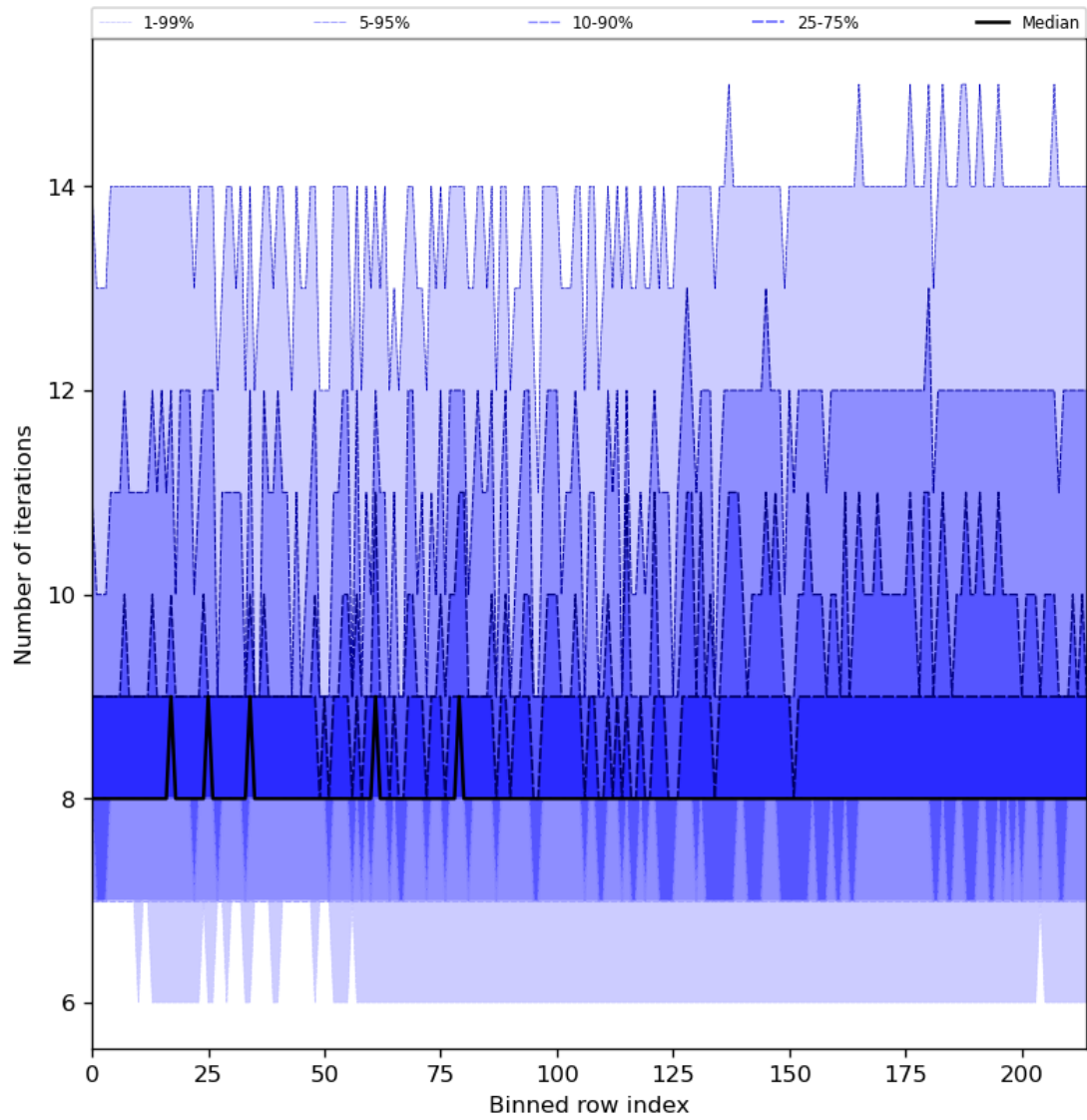
Figure 32: Along track statistics of “Number of iterations” for 2023-10-10 to 2023-10-12
