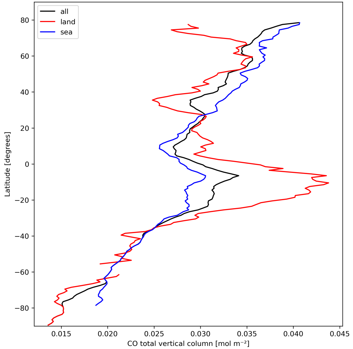
Figure 10: Zonal average of “CO total vertical column” for 2023-10-10 to 2023-10-12.
