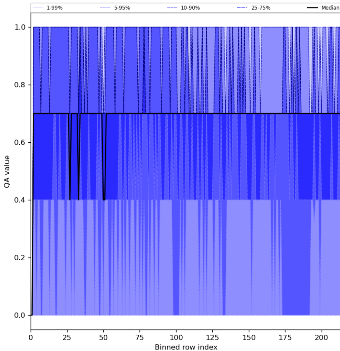
Figure 25: Along track statistics of “QA value” for 2023-10-10 to 2023-10-12
