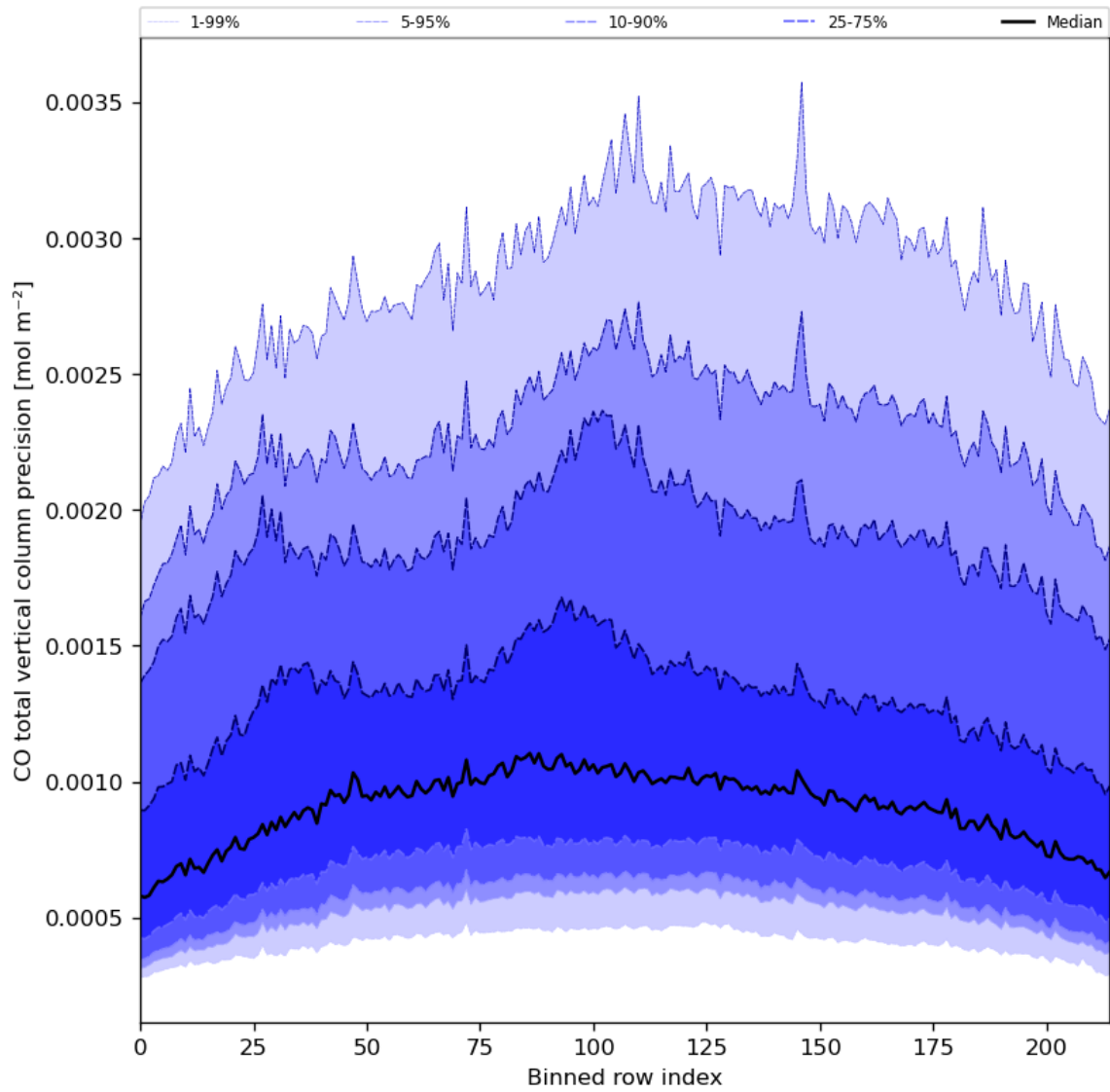
Figure 28: Along track statistics of “CO total vertical column precision” for 2023-10-10 to 2023-10-12
