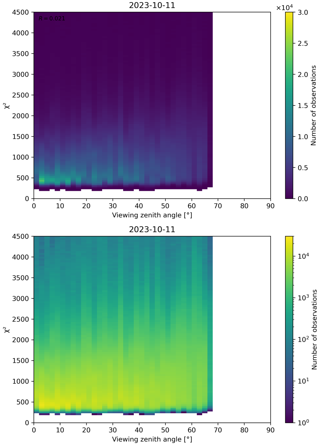
Figure 72: Scatter density plot of “Viewing zenith angle” against “ \chi^2 ” for 2023-10-10 to 2023-10-12.
