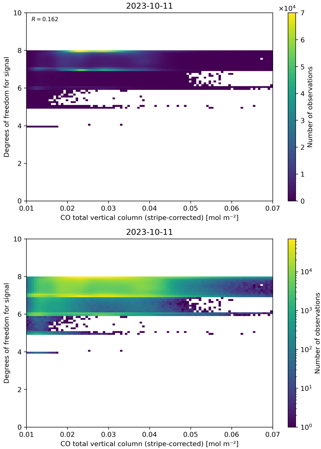
Figure 38: Scatter density plot of “CO total vertical column (stripe-corrected)” against “Degrees of freedom for signal” for 2023-10-10 to 2023-10-12.
