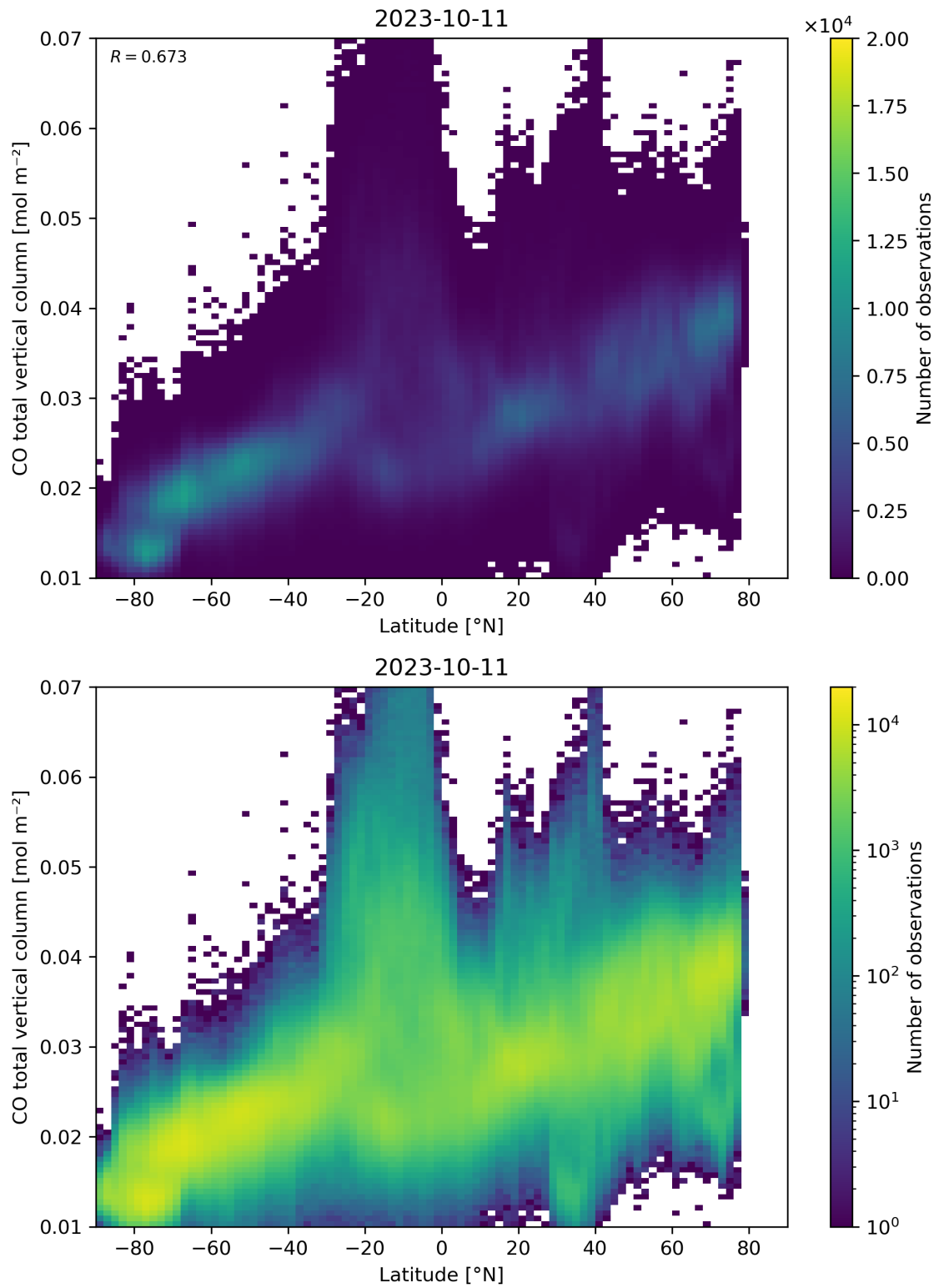
Figure 51: Scatter density plot of “Latitude” against “CO total vertical column” for 2023-10-10 to 2023-10-12.
