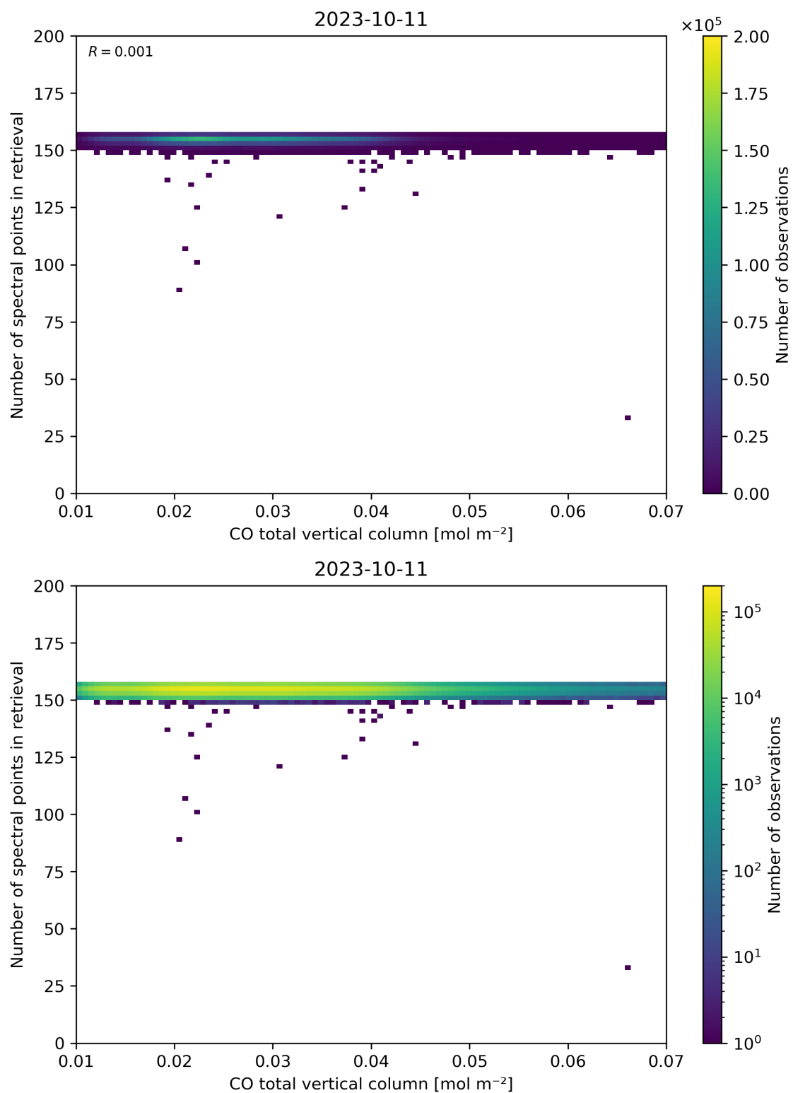
Figure 43: Scatter density plot of “CO total vertical column” against “Number of spectral points in retrieval” for 2023-10-10 to 2023-10-12.
