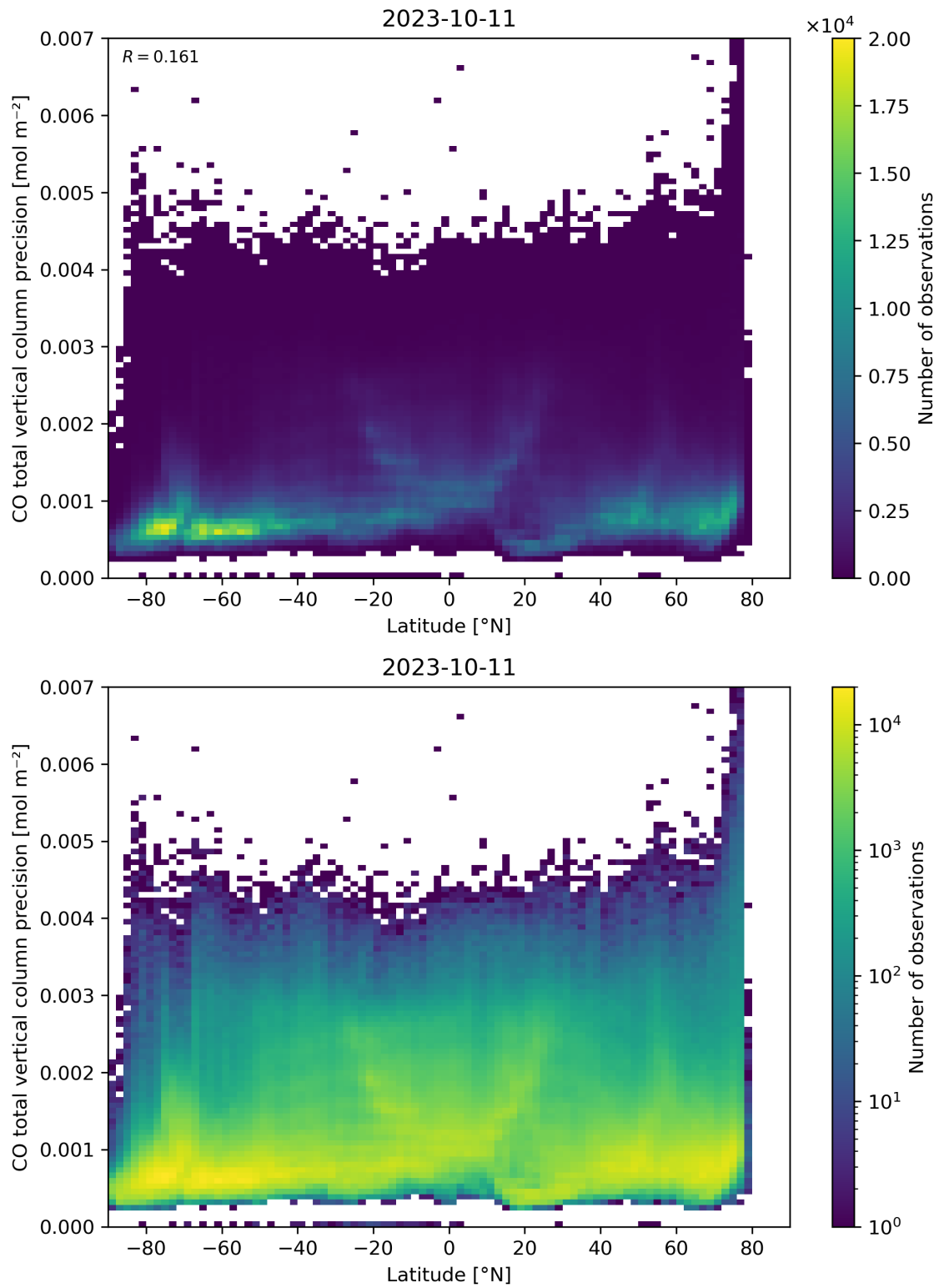
Figure 53: Scatter density plot of “Latitude” against “CO total vertical column precision” for 2023-10-10 to 2023-10-12.
