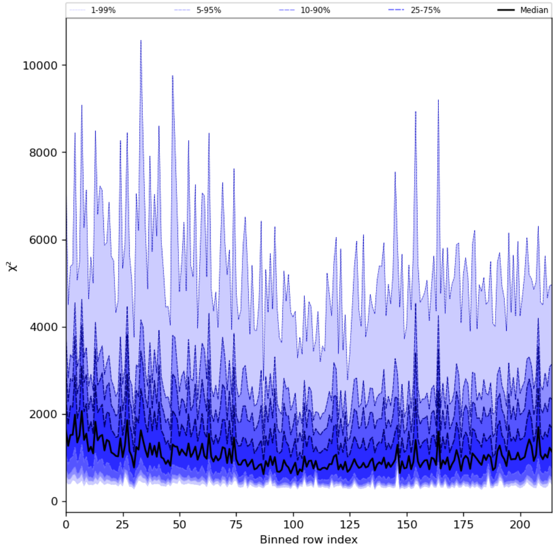
Figure 30: Along track statistics of “ \chi^2 ” for 2023-10-10 to 2023-10-12
