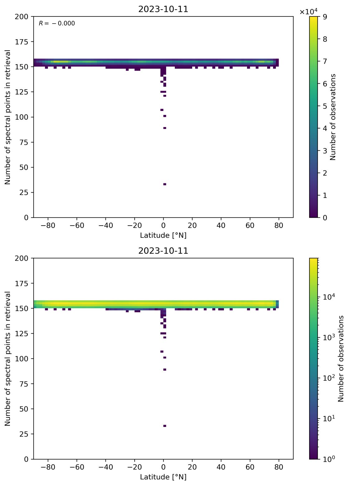
Figure 57: Scatter density plot of “Latitude” against “Number of spectral points in retrieval” for 2023-10-10 to 2023-10-12.
