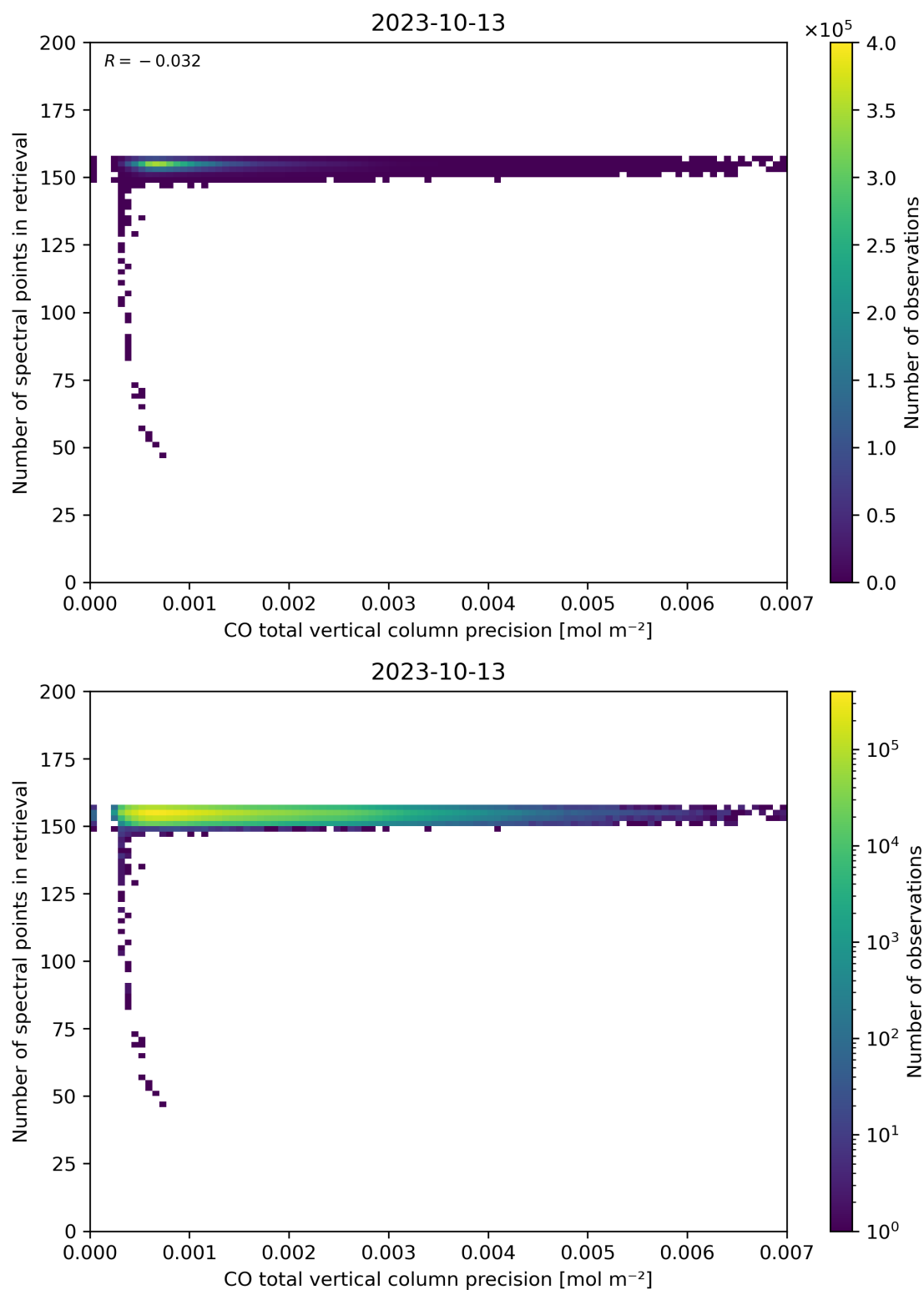
Figure 47: Scatter density plot of “CO total vertical column precision” against “Number of spectral points in retrieval” for 2023-10-12 to 2023-10-14.
