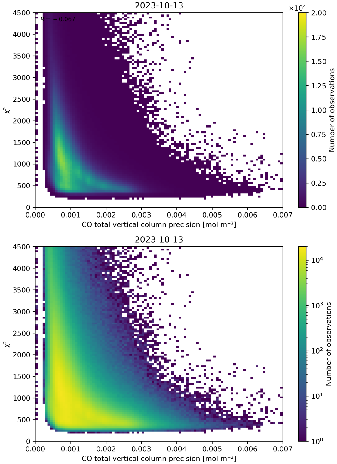
Figure 44: Scatter density plot of “CO total vertical column precision” against “ \chi^2 ” for 2023-10-12 to 2023-10-14.
