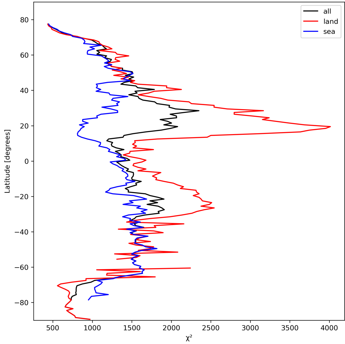
Figure 14: Zonal average of “ \chi^2 ” for 2023-10-12 to 2023-10-14.
