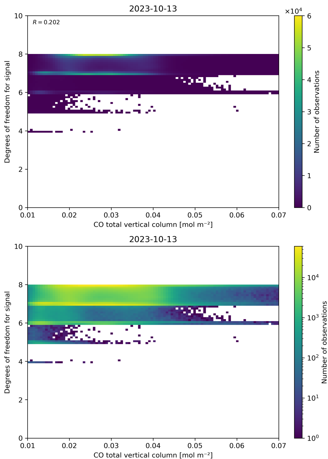
Figure 41: Scatter density plot of “CO total vertical column” against “Degrees of freedom for signal” for 2023-10-12 to 2023-10-14.
