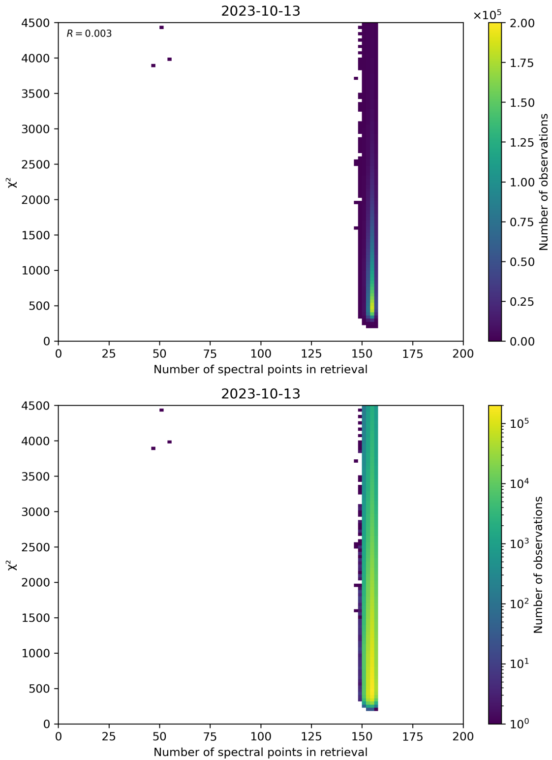
Figure 58: Scatter density plot of “Number of spectral points in retrieval” against “ \chi^2 ” for 2023-10-12 to 2023-10-14.
