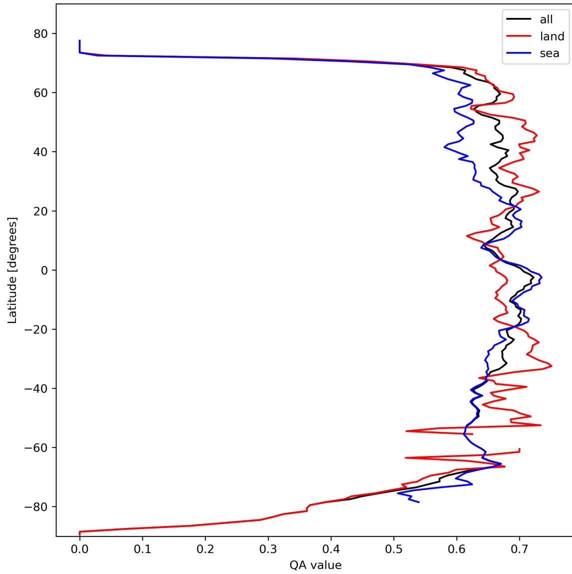
Figure 9: Zonal average of “QA value” for 2023-10-12 to 2023-10-14.
