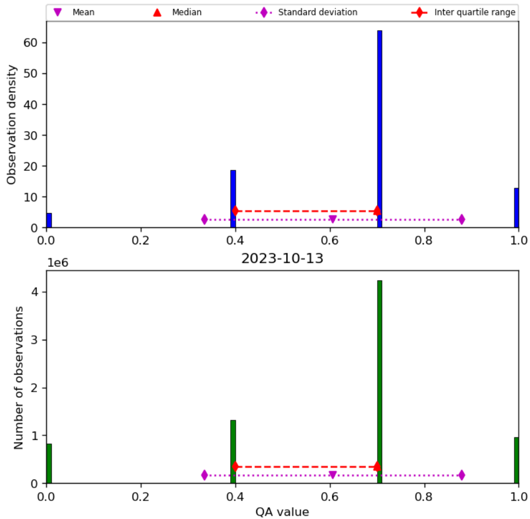
Figure 17: Histogram of “QA value” for 2023-10-12 to 2023-10-14
