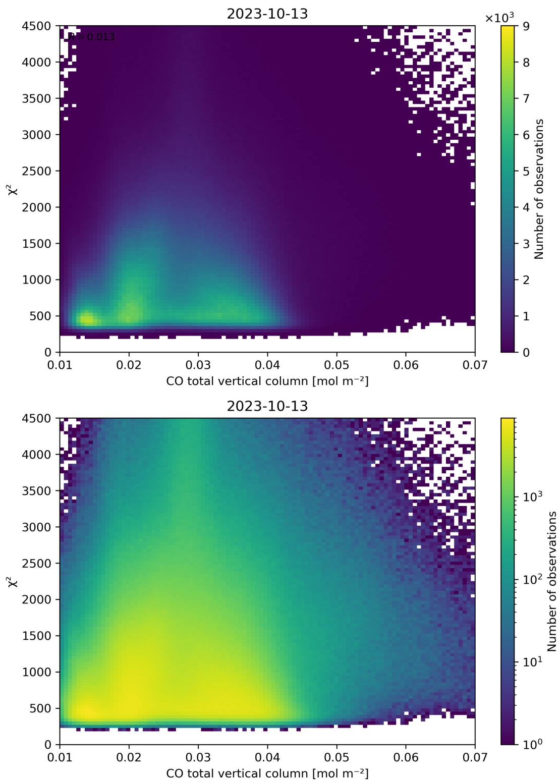
Figure 35: Scatter density plot of “CO total vertical column” against “ \chi^2 ” for 2023-10-12 to 2023-10-14.
