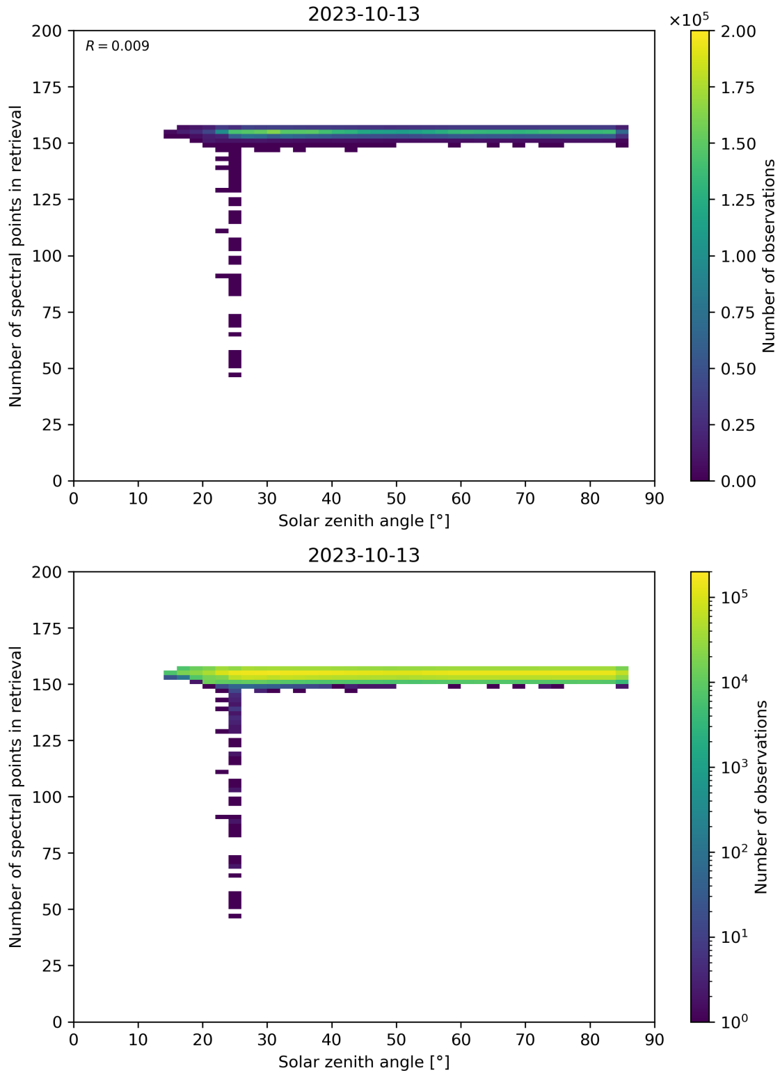
Figure 68: Scatter density plot of “Solar zenith angle” against “Number of spectral points in retrieval” for 2023-10-12 to 2023-10-14.
