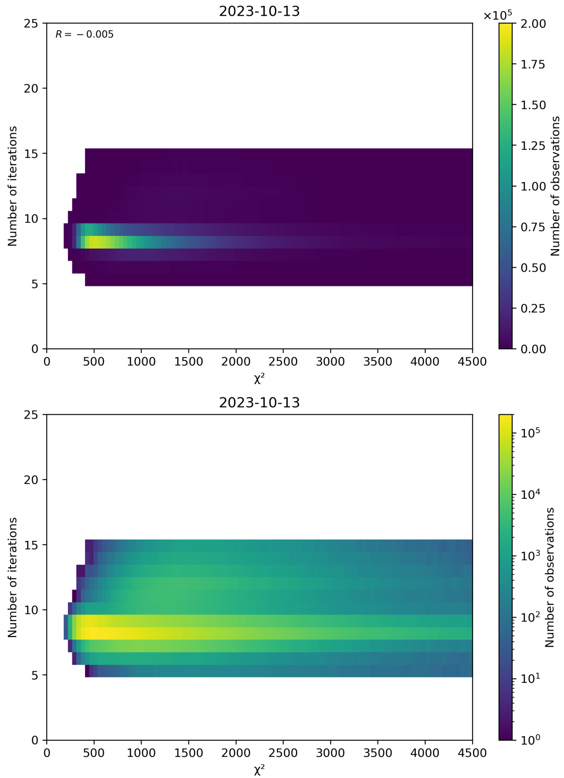
Figure 49: Scatter density plot of “ \chi^2 ” against “Number of iterations” for 2023-10-12 to 2023-10-14.
