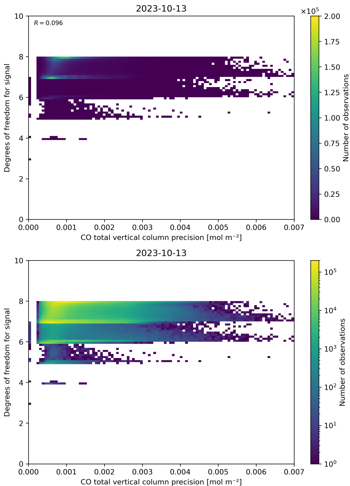
Figure 45: Scatter density plot of “CO total vertical column precision” against “Degrees of freedom for signal” for 2023-10-12 to 2023-10-14.
