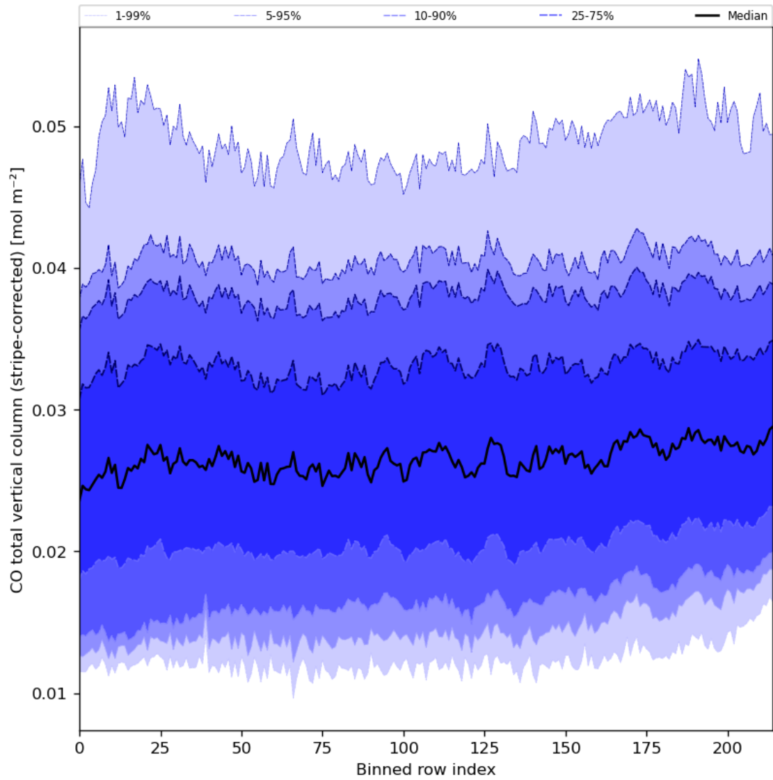
Figure 27: Along track statistics of “CO total vertical column (stripe-corrected)” for 2023-10-12 to 2023-10-14
