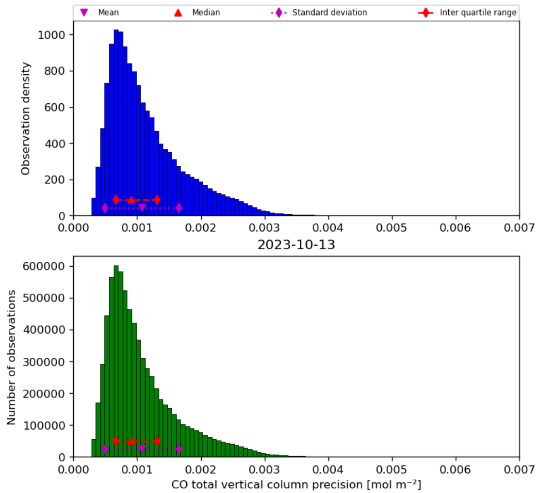
Figure 20: Histogram of “CO total vertical column precision” for 2023-10-12 to 2023-10-14
