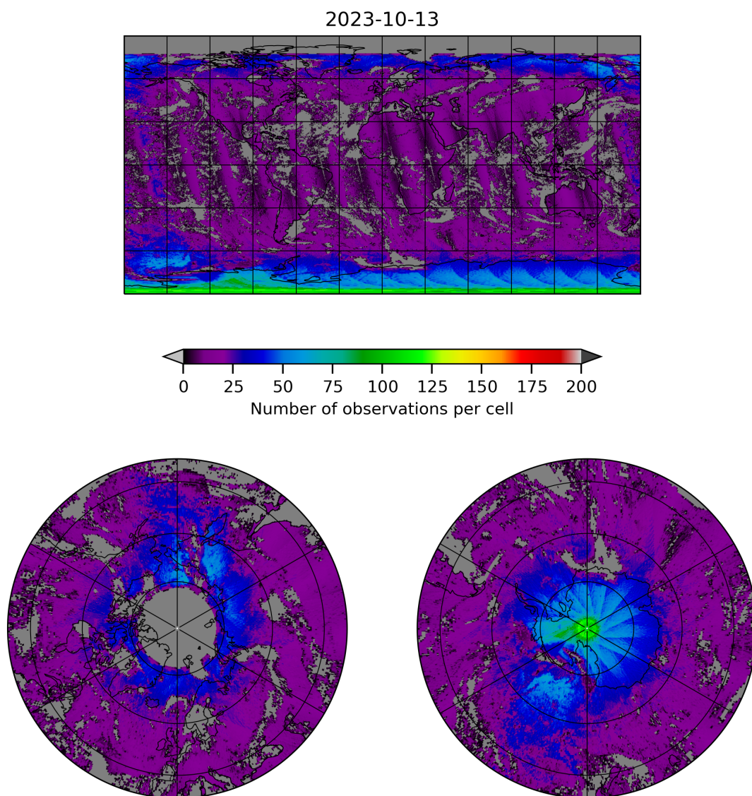
Figure 8: Map of the number of observations for 2023-10-12 to 2023-10-14
