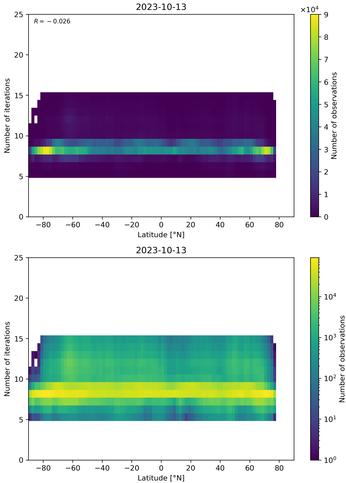
Figure 56: Scatter density plot of “Latitude” against “Number of iterations” for 2023-10-12 to 2023-10-14.
