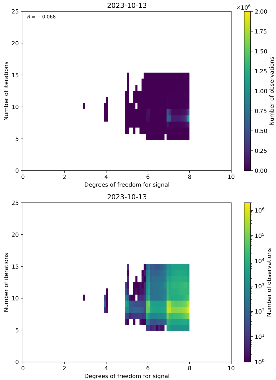
Figure 50: Scatter density plot of “Degrees of freedom for signal” against “Number of iterations” for 2023-10-12 to 2023-10-14.
