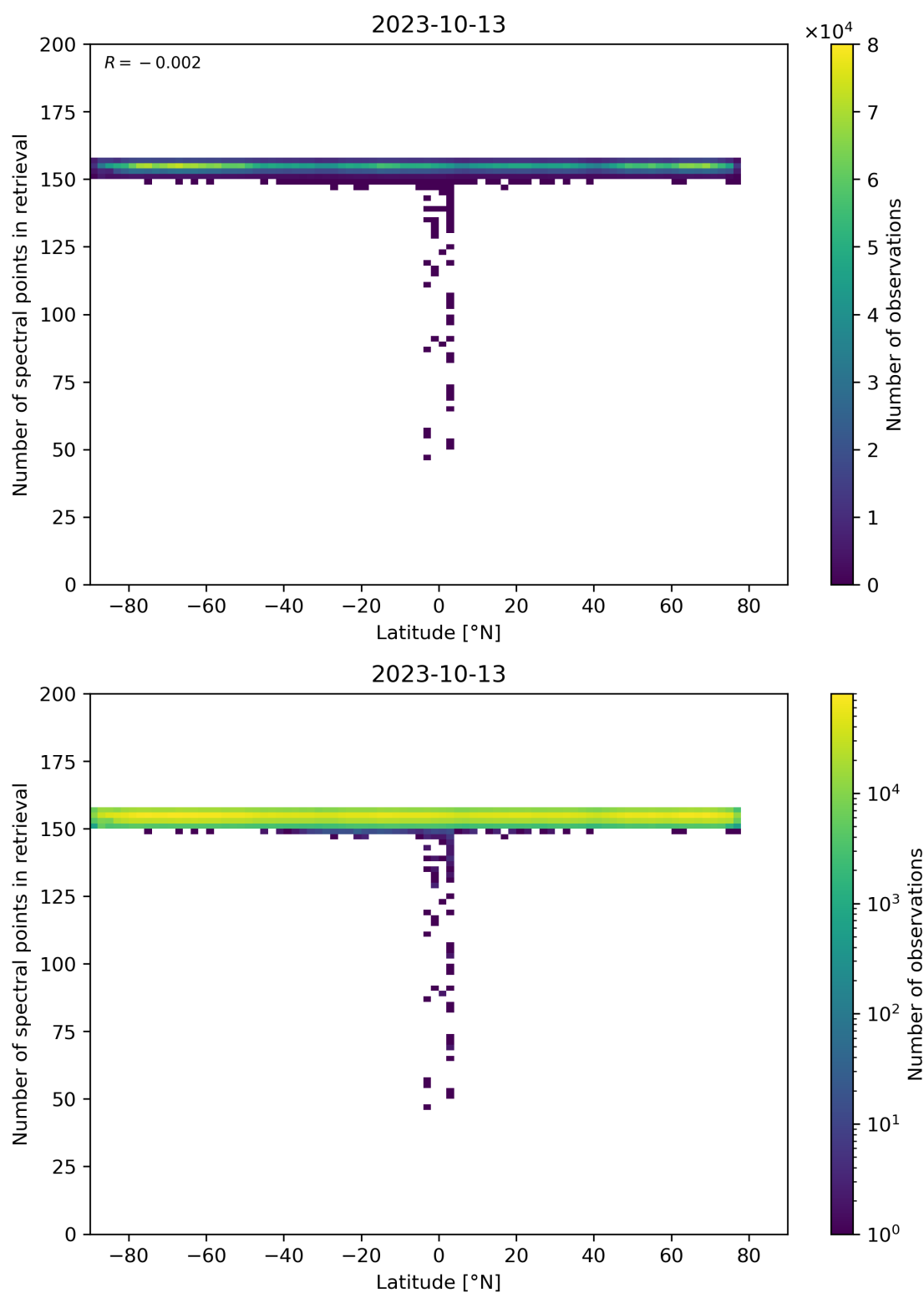
Figure 57: Scatter density plot of “Latitude” against “Number of spectral points in retrieval” for 2023-10-12 to 2023-10-14.
