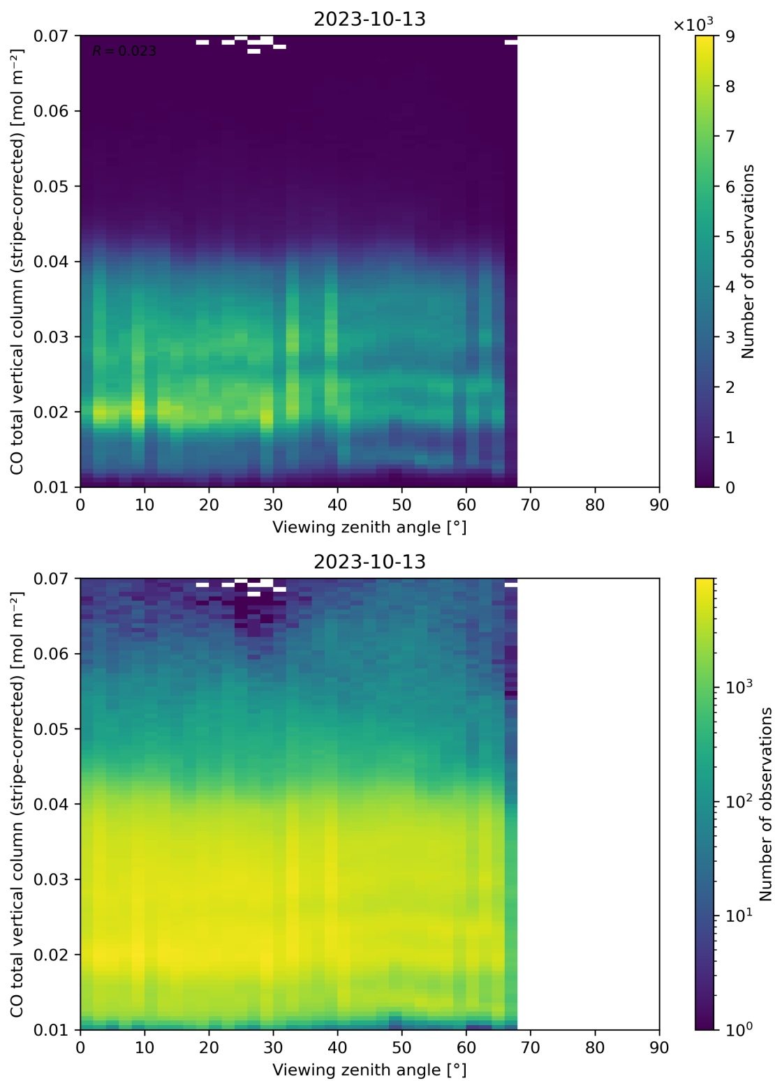
Figure 70: Scatter density plot of “Viewing zenith angle” against “CO total vertical column (stripe-corrected)” for 2023-10-12 to 2023-10-14.
