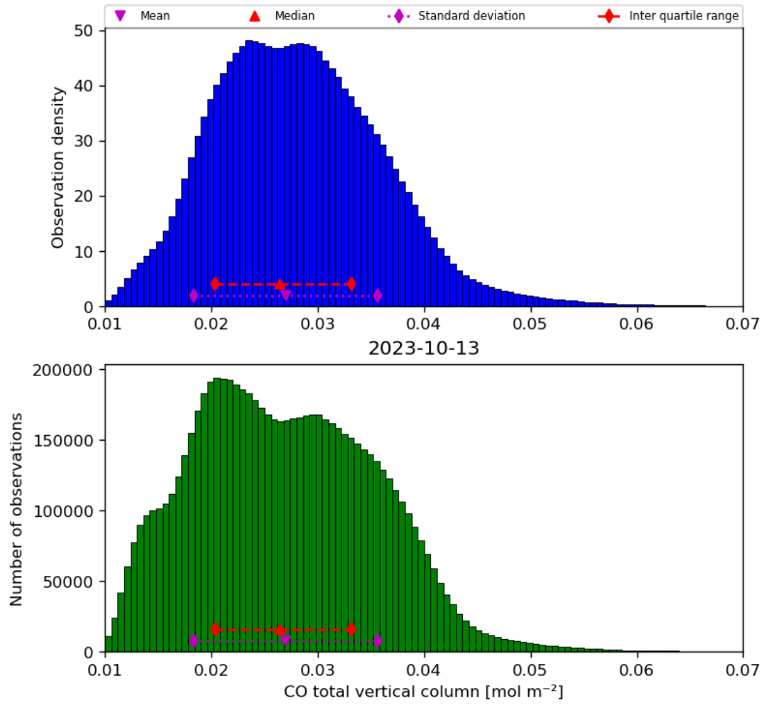
Figure 18: Histogram of “CO total vertical column” for 2023-10-12 to 2023-10-14
