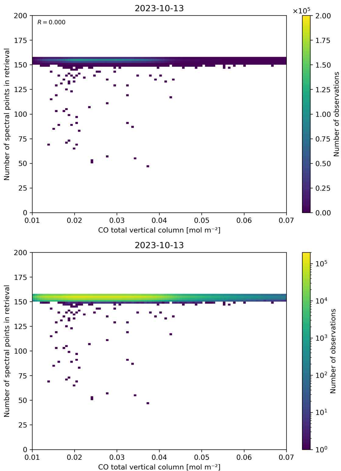
Figure 43: Scatter density plot of “CO total vertical column” against “Number of spectral points in retrieval” for 2023-10-12 to 2023-10-14.
