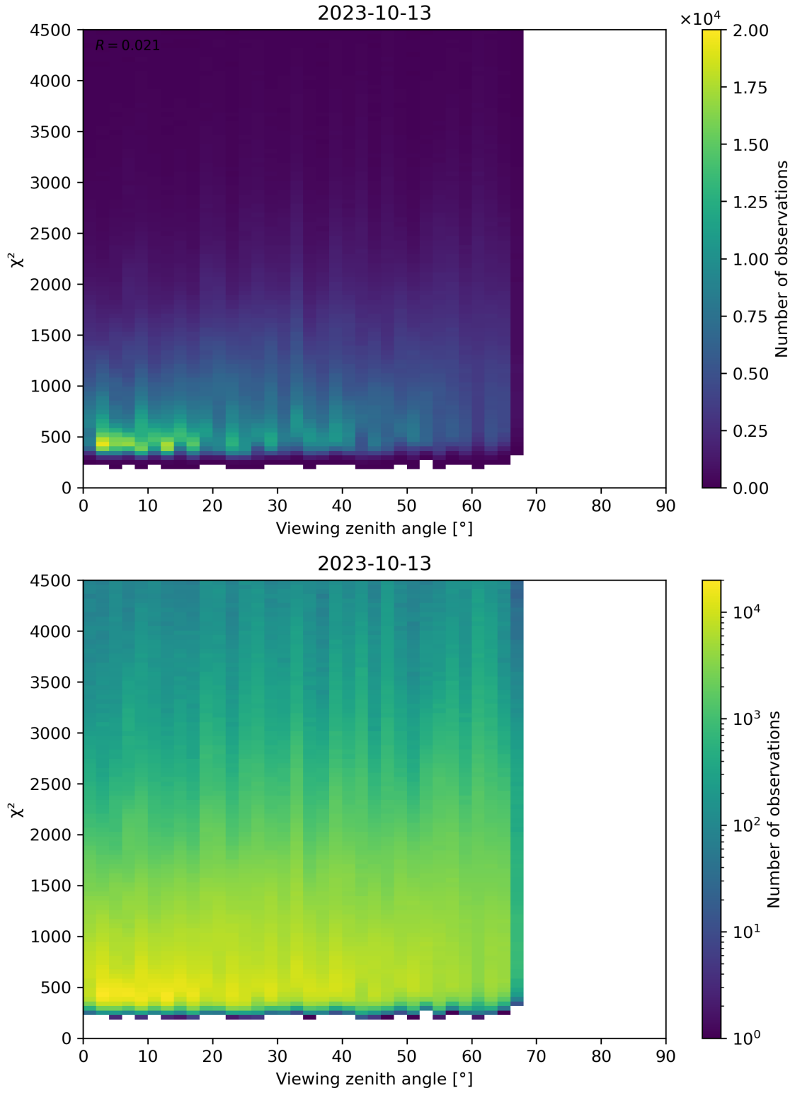
Figure 72: Scatter density plot of “Viewing zenith angle” against “ \chi^2 ” for 2023-10-12 to 2023-10-14.
