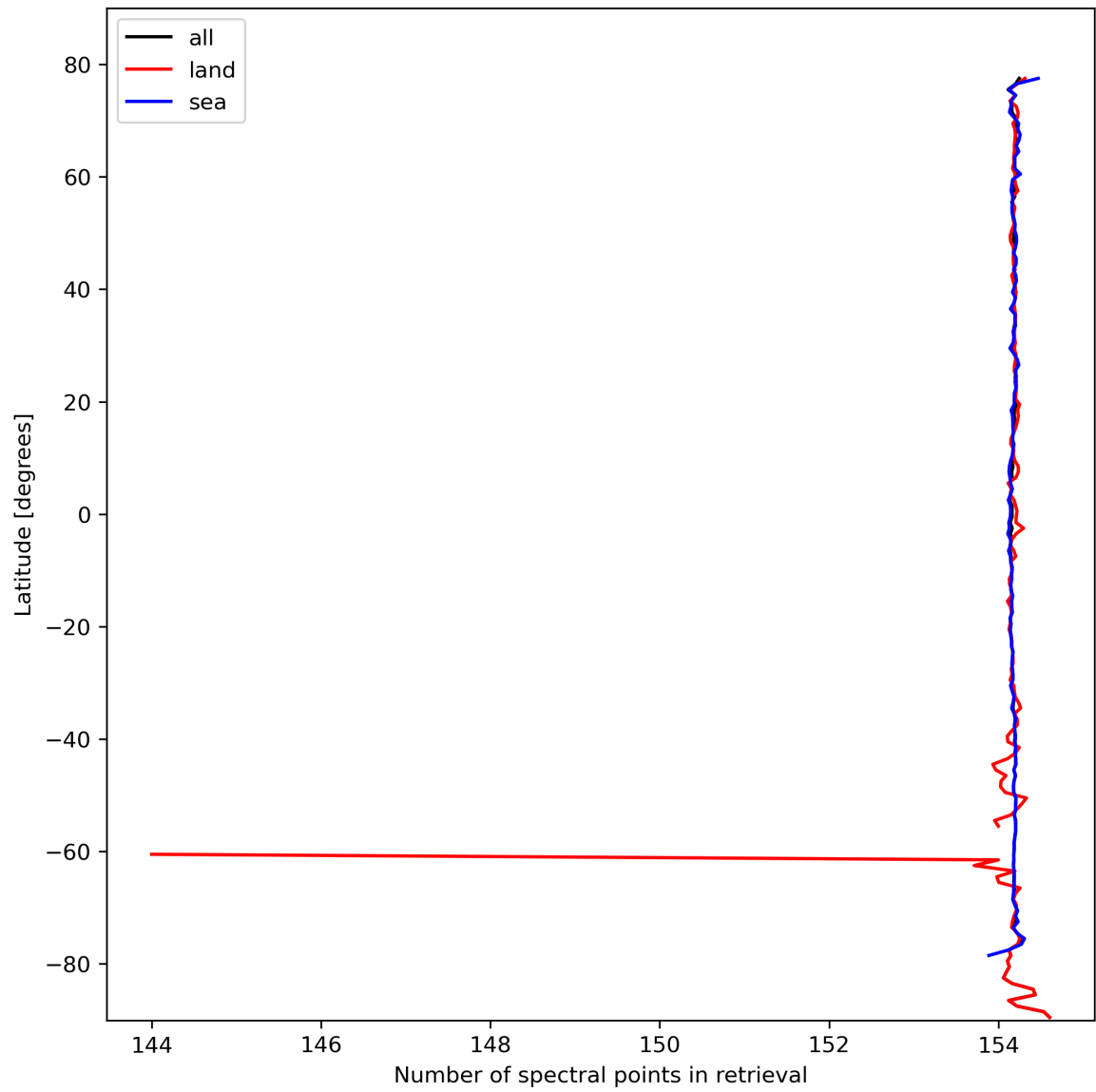
Figure 13: Zonal average of “Number of spectral points in retrieval” for 2023-10-12 to 2023-10-14.
