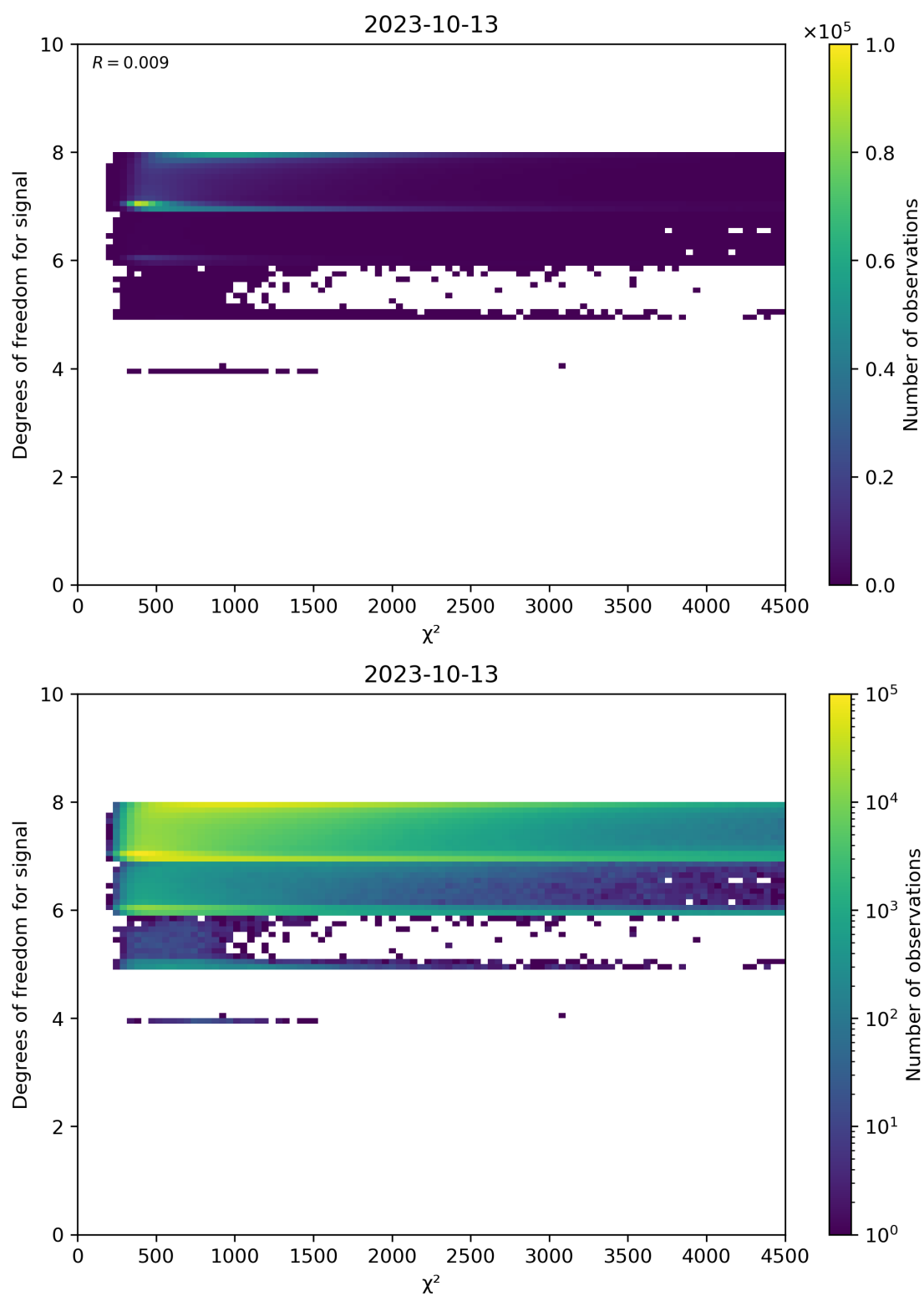
Figure 48: Scatter density plot of “ \chi^2 ” against “Degrees of freedom for signal” for 2023-10-12 to 2023-10-14.
