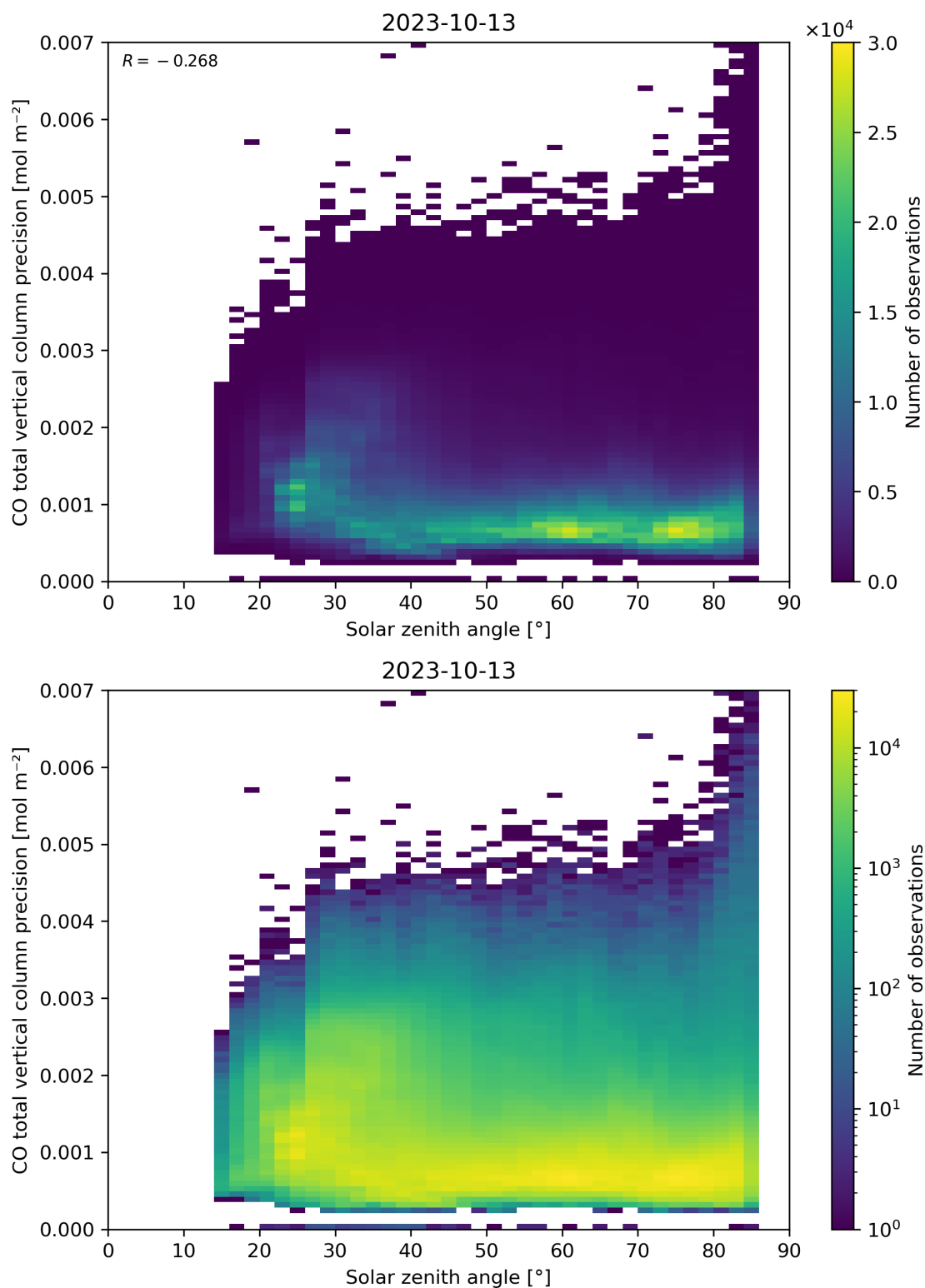
Figure 63: Scatter density plot of “Solar zenith angle” against “CO total vertical column precision” for 2023-10-12 to 2023-10-14.
