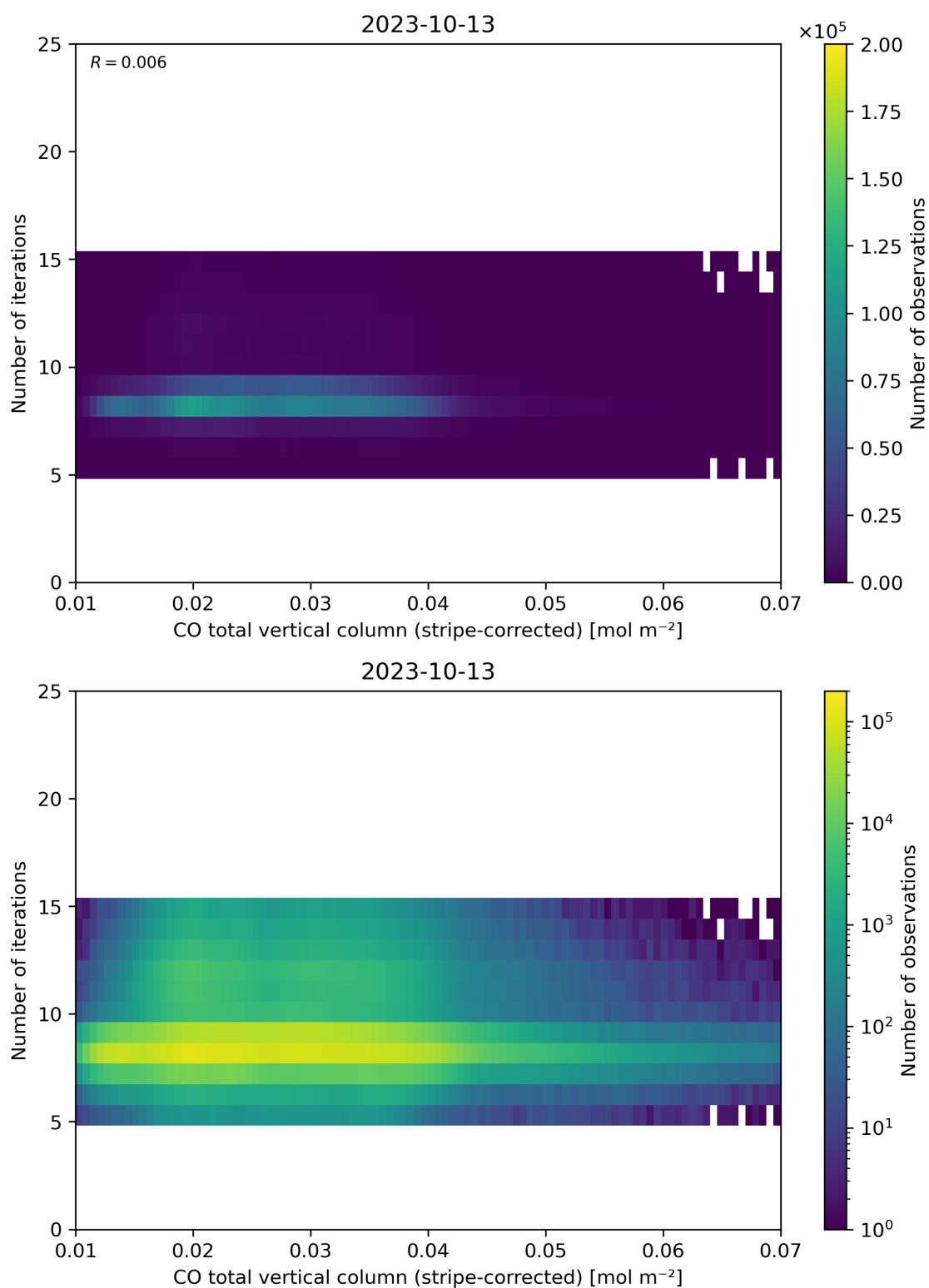
Figure 39: Scatter density plot of “CO total vertical column (stripe-corrected)” against “Number of iterations” for 2023-10-12 to 2023-10-14.
