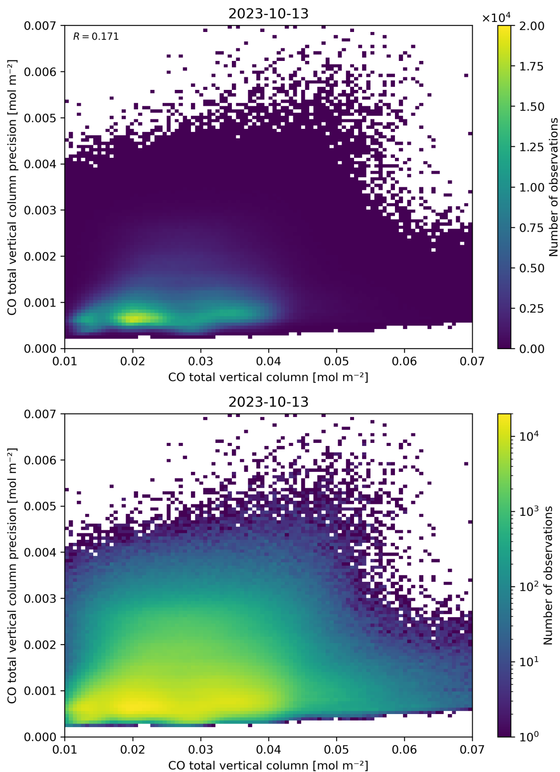
Figure 34: Scatter density plot of “CO total vertical column” against “CO total vertical column precision” for 2023-10-12 to 2023-10-14.
