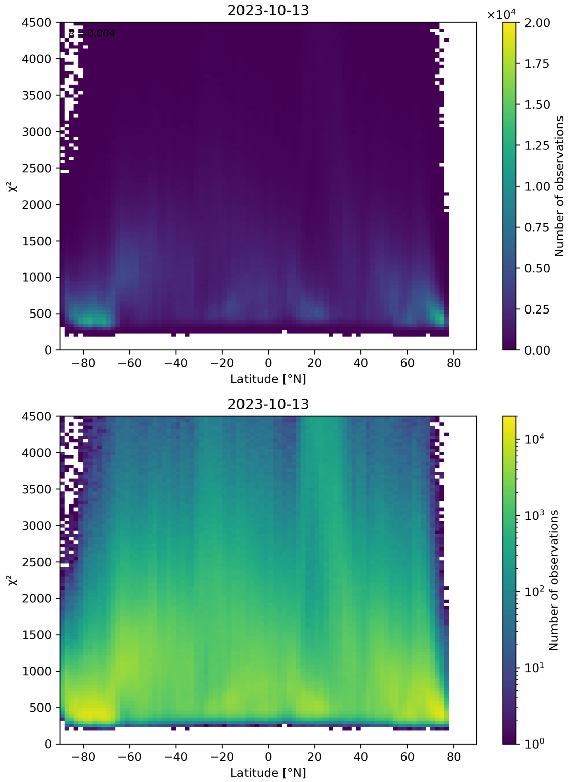
Figure 54: Scatter density plot of “Latitude” against “ \chi^2 ” for 2023-10-12 to 2023-10-14.
