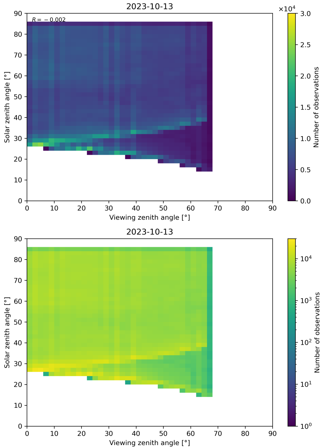
Figure 77: Scatter density plot of “Viewing zenith angle” against “Solar zenith angle” for 2023-10-12 to 2023-10-14.
