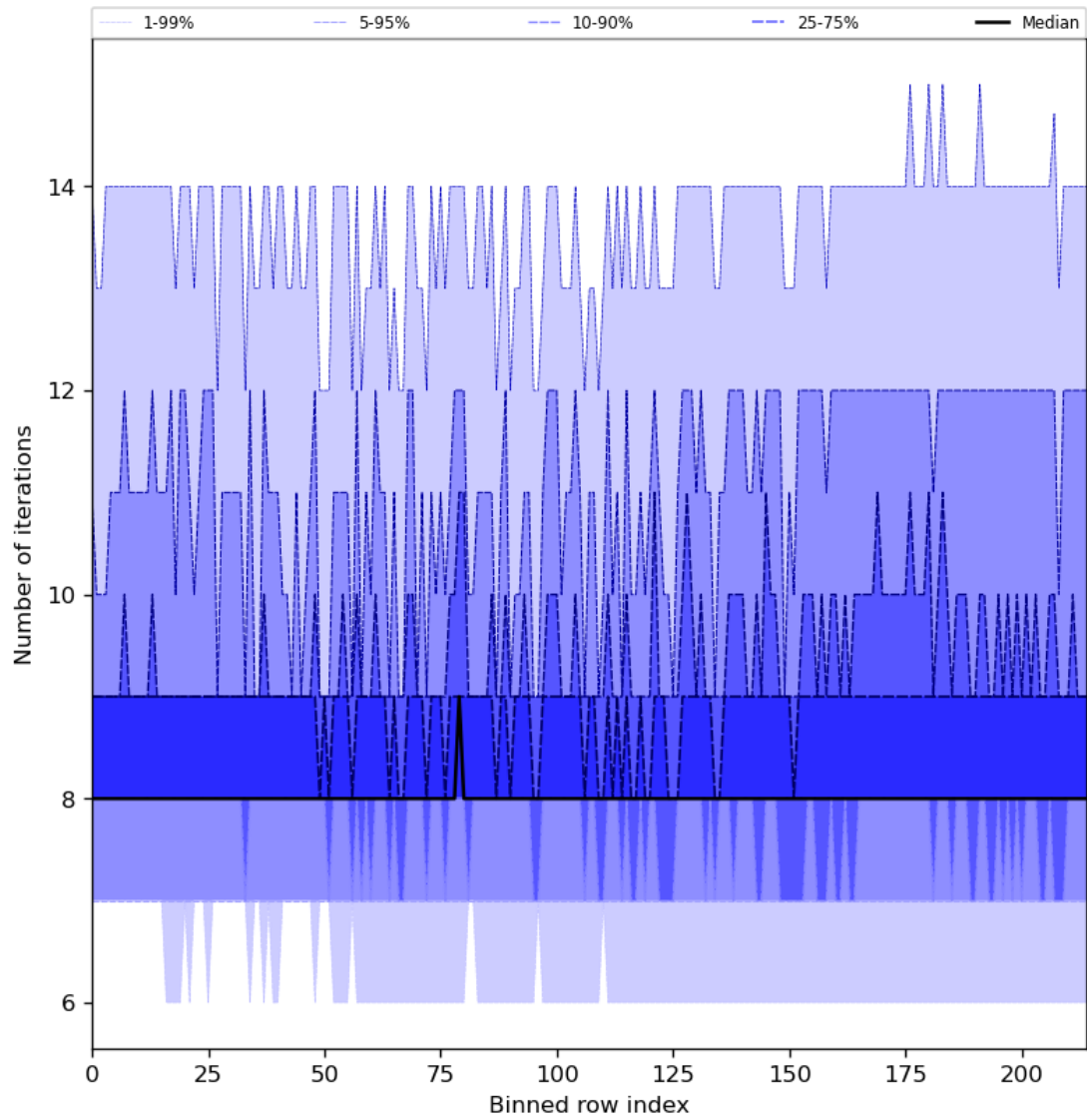
Figure 32: Along track statistics of “Number of iterations” for 2023-10-12 to 2023-10-14
