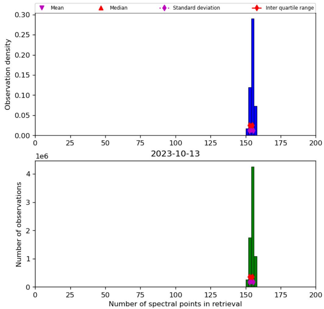
Figure 21: Histogram of “Number of spectral points in retrieval” for 2023-10-12 to 2023-10-14
