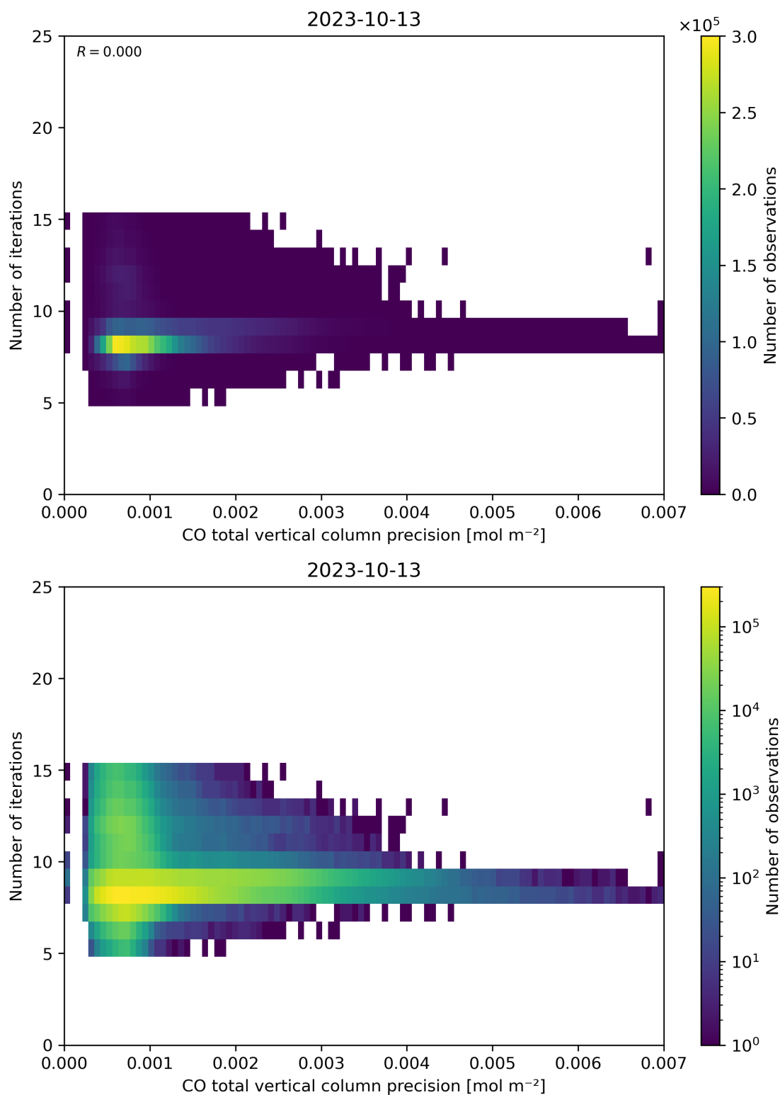
Figure 46: Scatter density plot of “CO total vertical column precision” against “Number of iterations” for 2023-10-12 to 2023-10-14.
