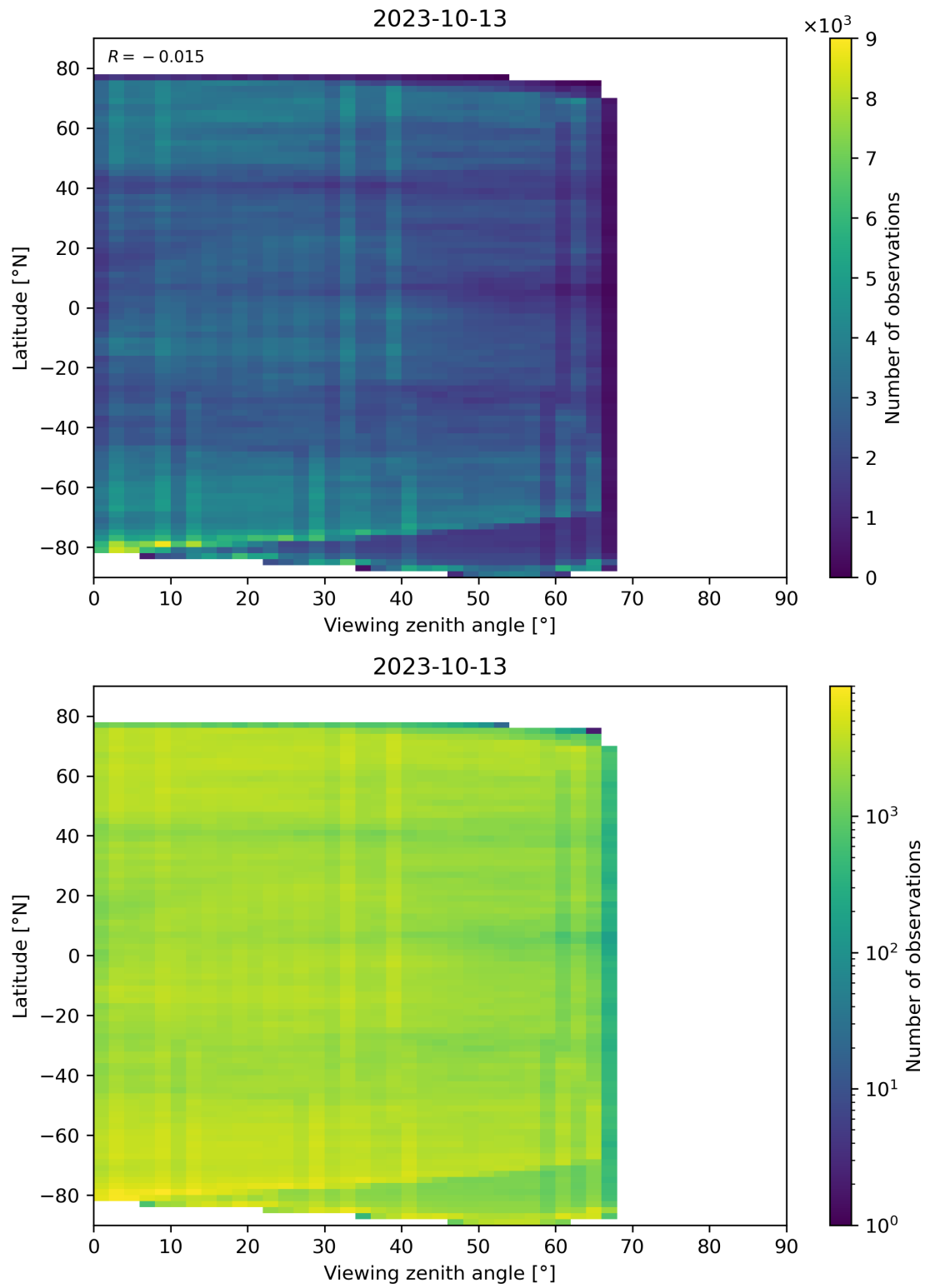
Figure 74: Scatter density plot of “Viewing zenith angle” against “Latitude” for 2023-10-12 to 2023-10-14.
