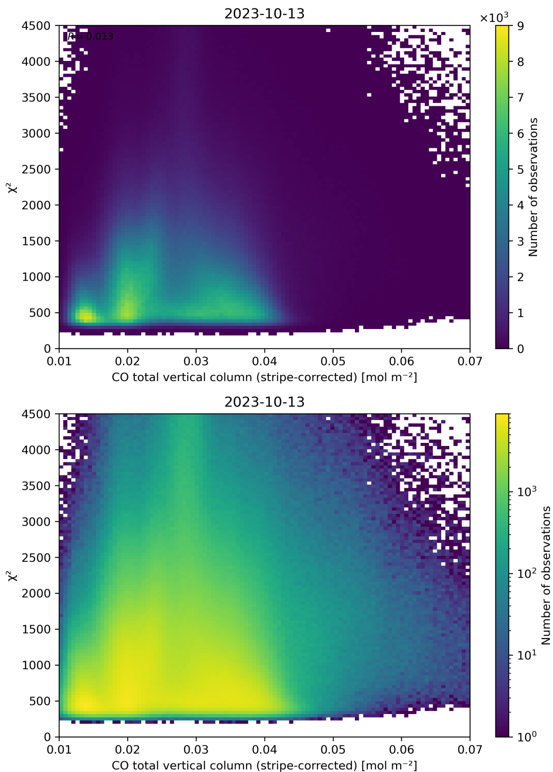
Figure 37: Scatter density plot of “CO total vertical column (stripe-corrected)” against “ \chi^2 ” for 2023-10-12 to 2023-10-14.
