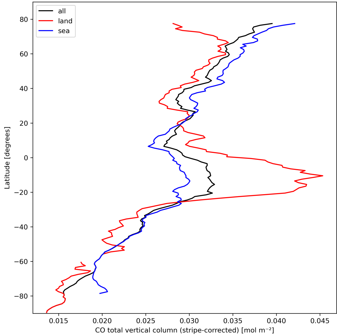
Figure 11: Zonal average of “CO total vertical column (stripe-corrected)” for 2023-10-12 to 2023-10-14.
