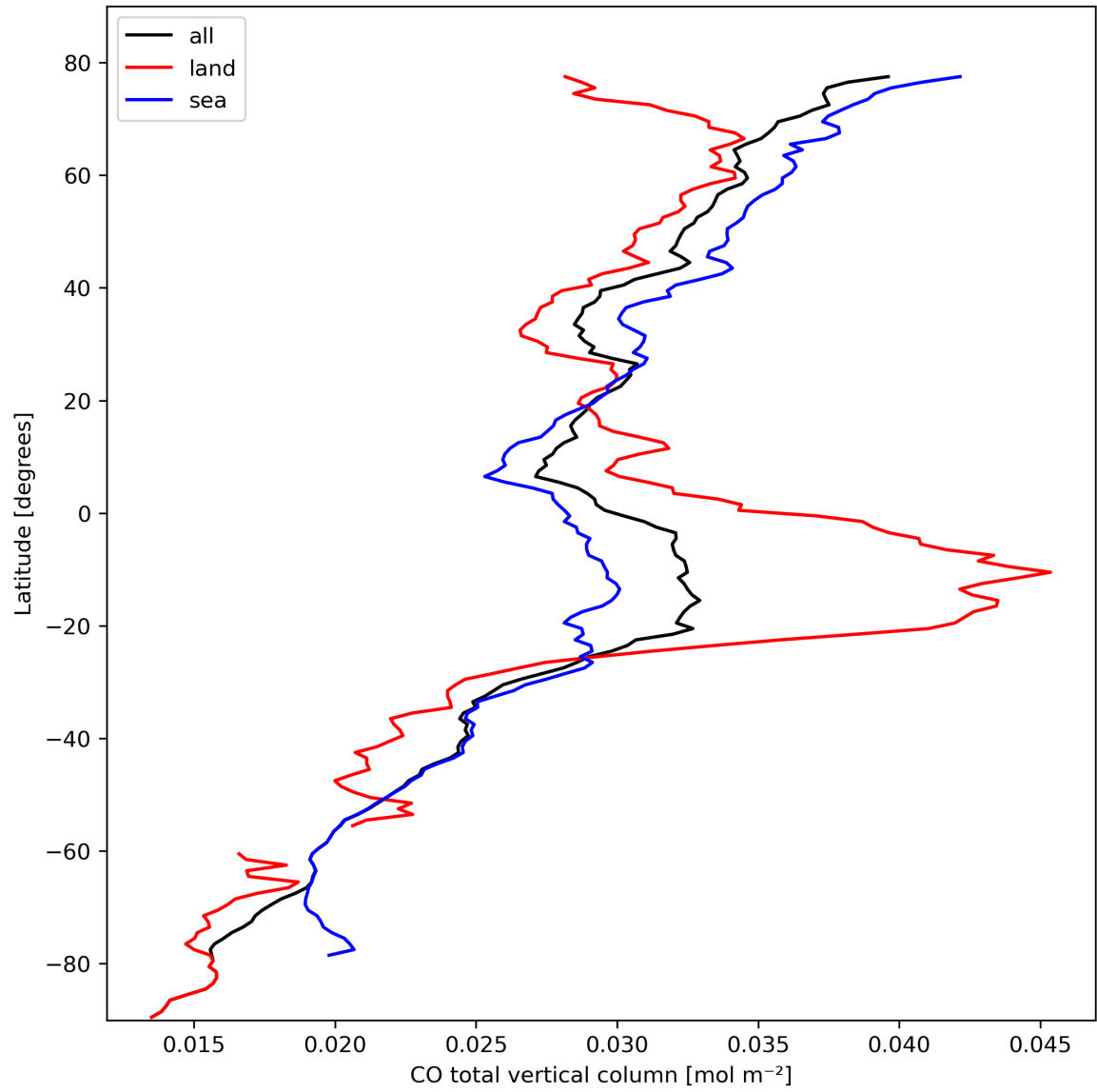
Figure 10: Zonal average of “CO total vertical column” for 2023-10-12 to 2023-10-14.
