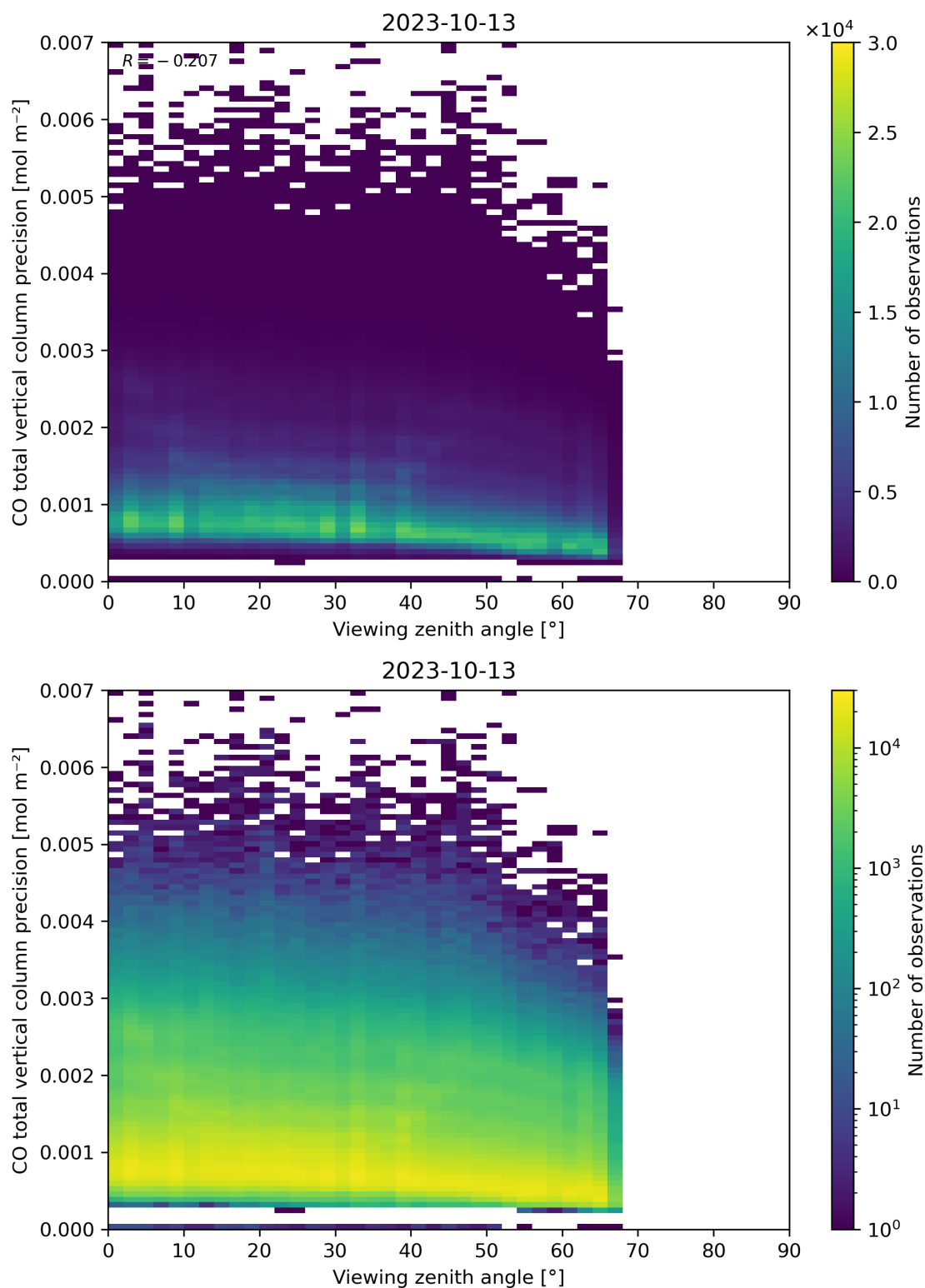
Figure 71: Scatter density plot of “Viewing zenith angle” against “CO total vertical column precision” for 2023-10-12 to 2023-10-14.
