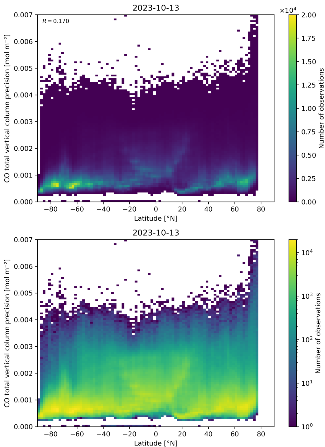
Figure 53: Scatter density plot of “Latitude” against “CO total vertical column precision” for 2023-10-12 to 2023-10-14.
