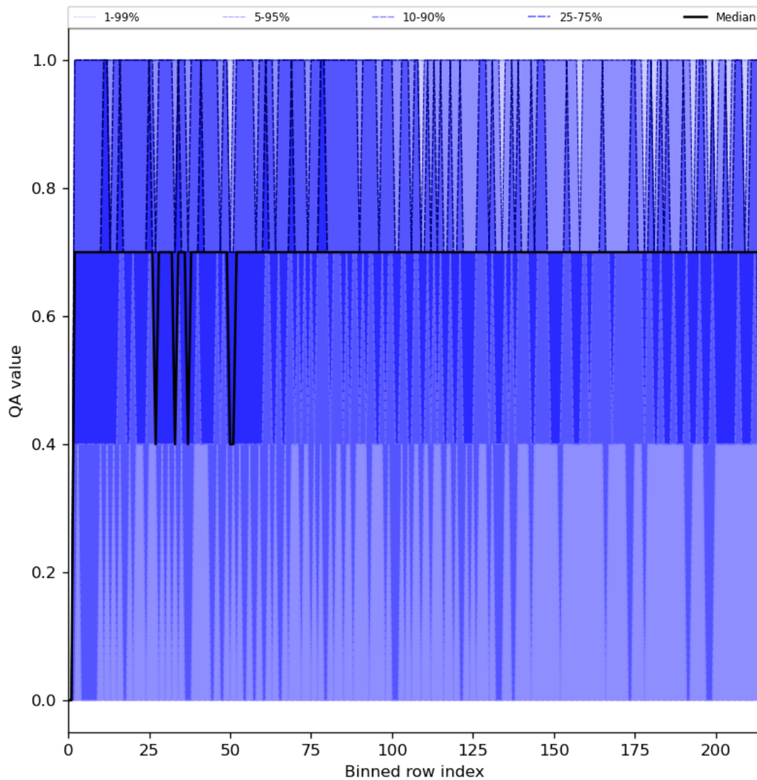
Figure 25: Along track statistics of “QA value” for 2023-10-12 to 2023-10-14
