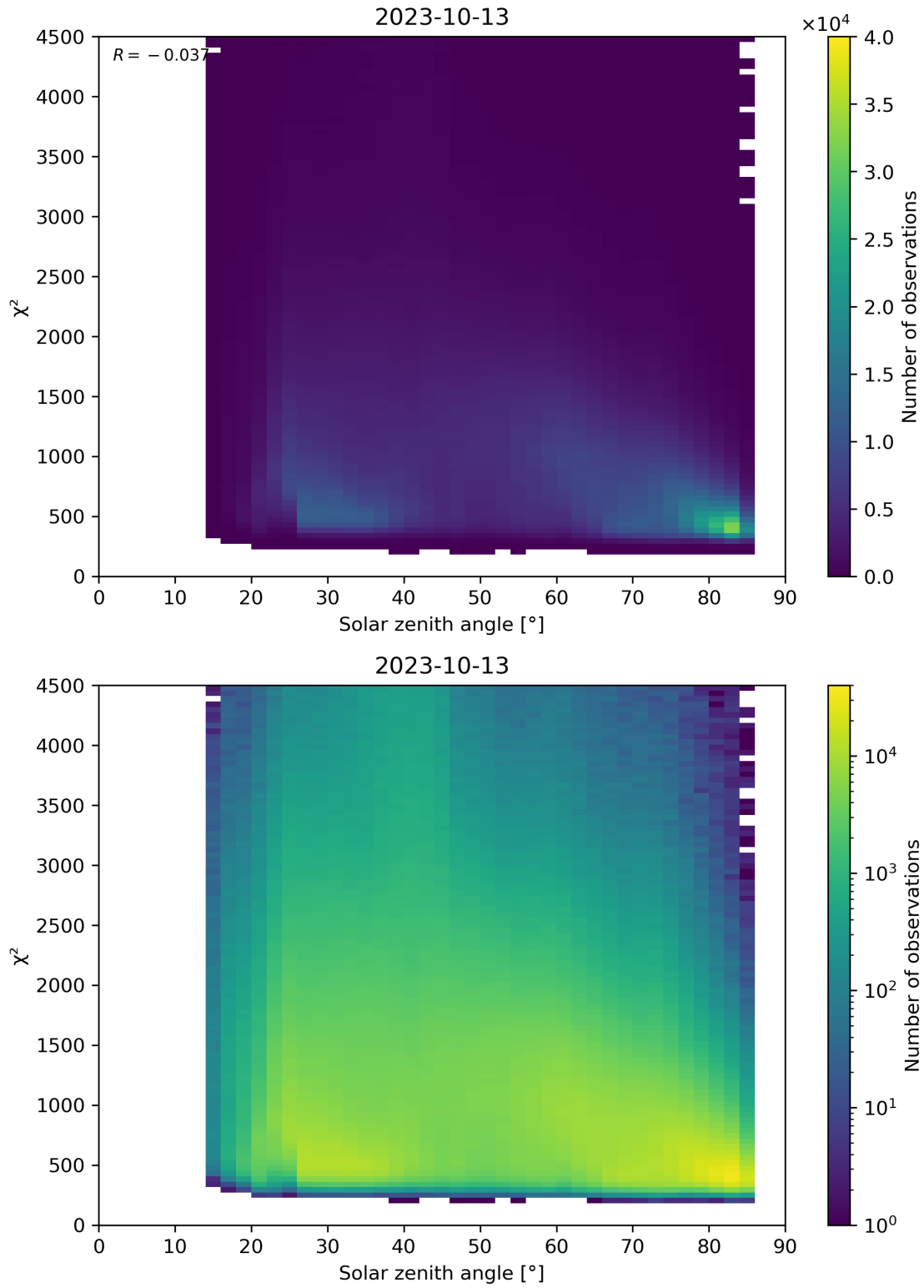
Figure 64: Scatter density plot of “Solar zenith angle” against “ \chi^2 ” for 2023-10-12 to 2023-10-14.
