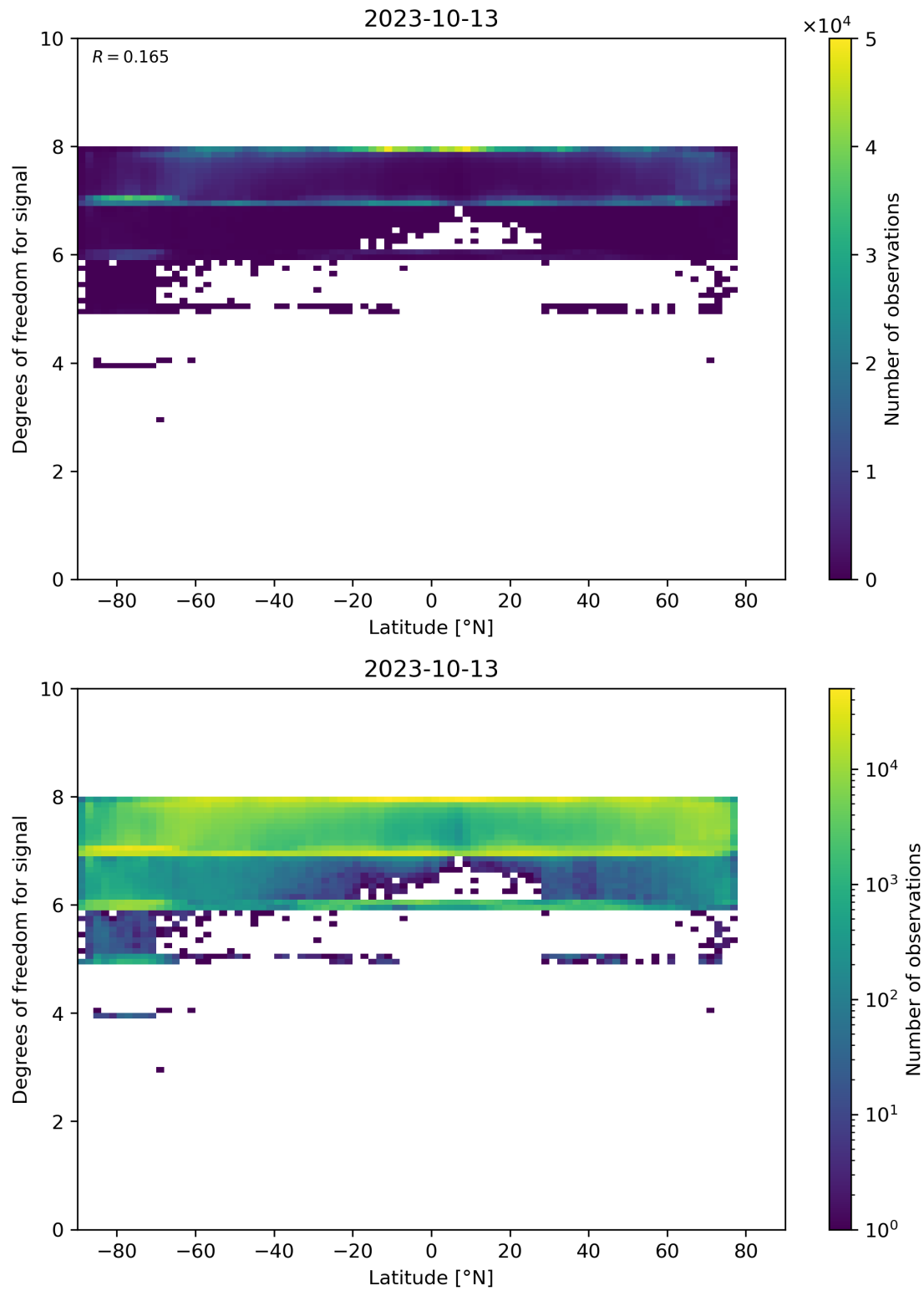
Figure 55: Scatter density plot of “Latitude” against “Degrees of freedom for signal” for 2023-10-12 to 2023-10-14.
