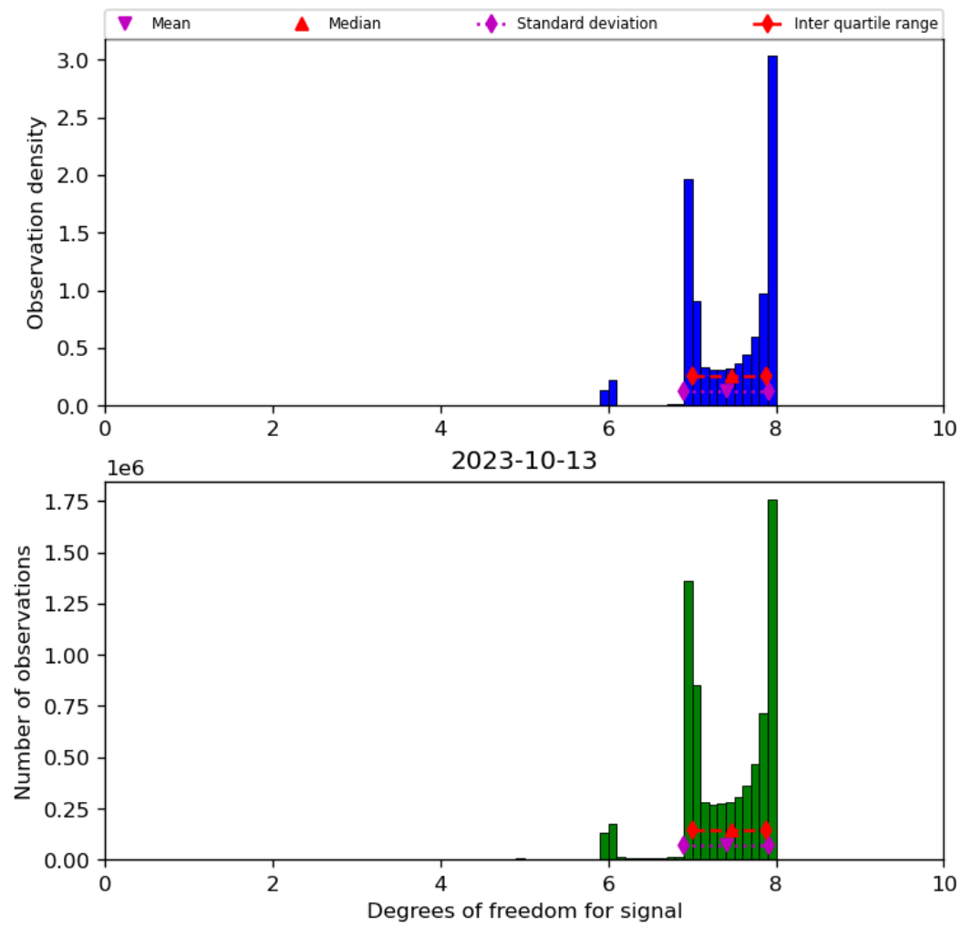
Figure 23: Histogram of “Degrees of freedom for signal” for 2023-10-12 to 2023-10-14
