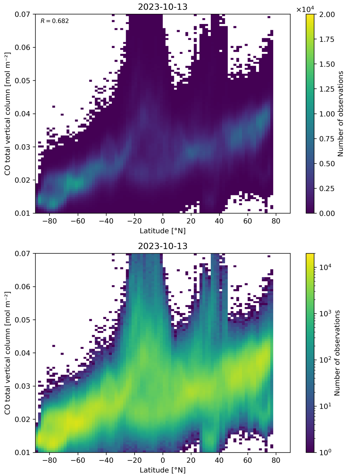
Figure 51: Scatter density plot of “Latitude” against “CO total vertical column” for 2023-10-12 to 2023-10-14.
