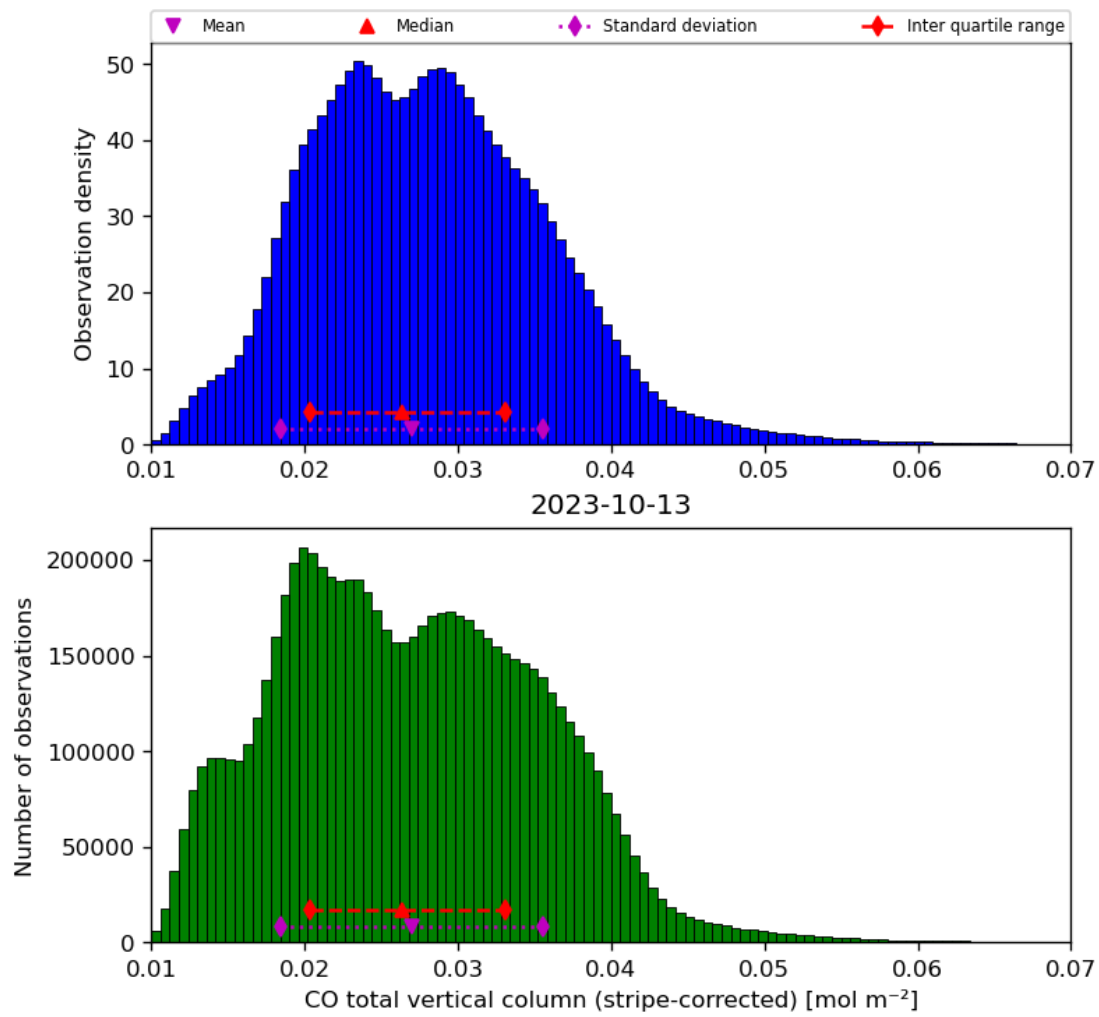
Figure 19: Histogram of “CO total vertical column (stripe-corrected)” for 2023-10-12 to 2023-10-14
