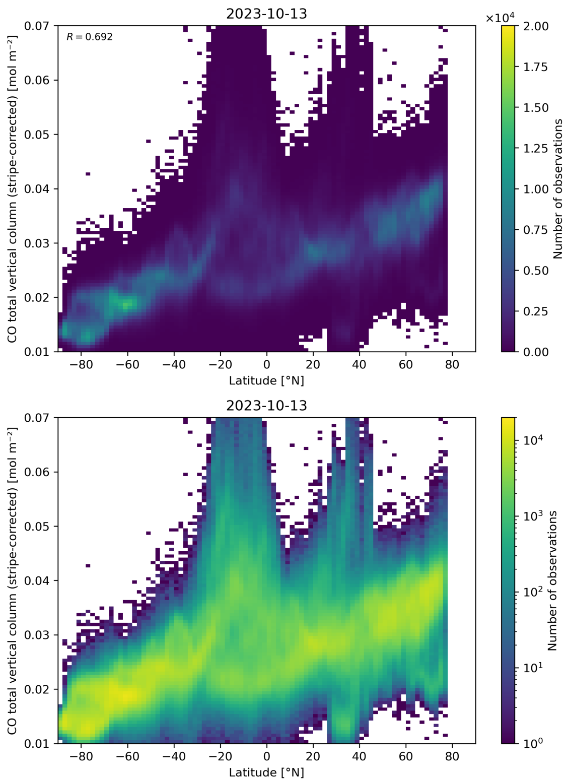
Figure 52: Scatter density plot of “Latitude” against “CO total vertical column (stripe-corrected)” for 2023-10-12 to 2023-10-14.
