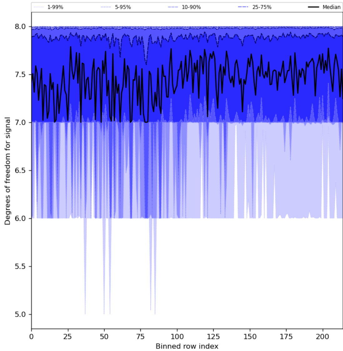
Figure 31: Along track statistics of “Degrees of freedom for signal” for 2023-10-12 to 2023-10-14
