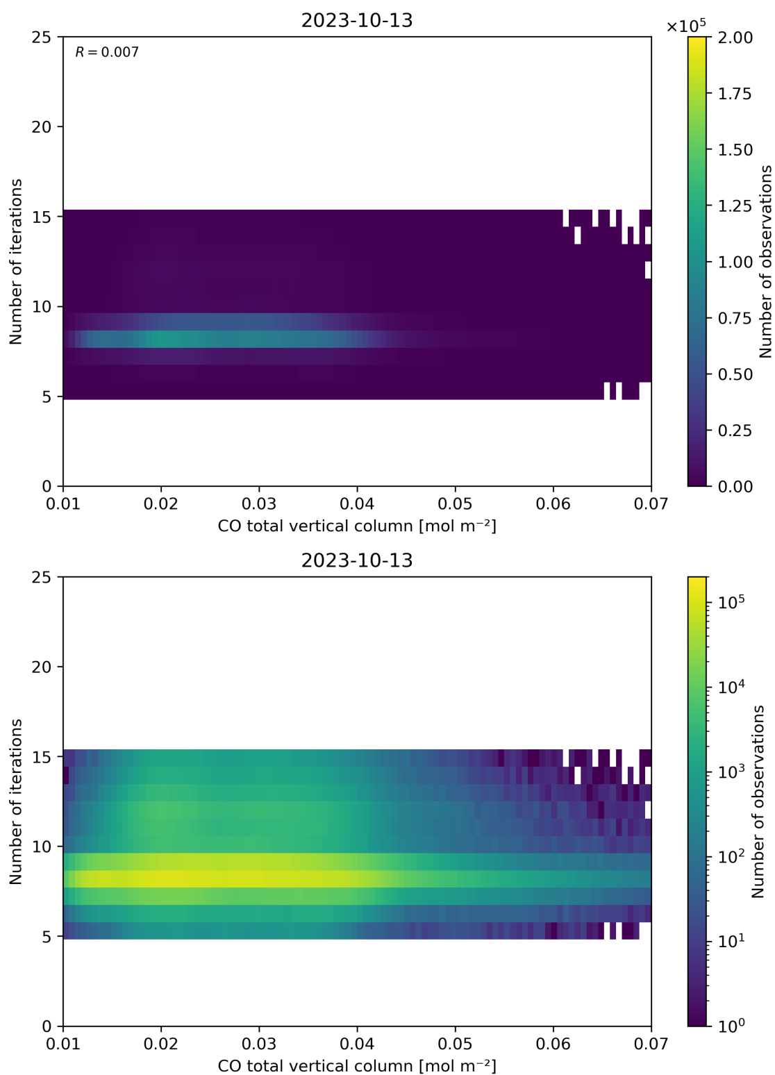
Figure 42: Scatter density plot of “CO total vertical column” against “Number of iterations” for 2023-10-12 to 2023-10-14.
