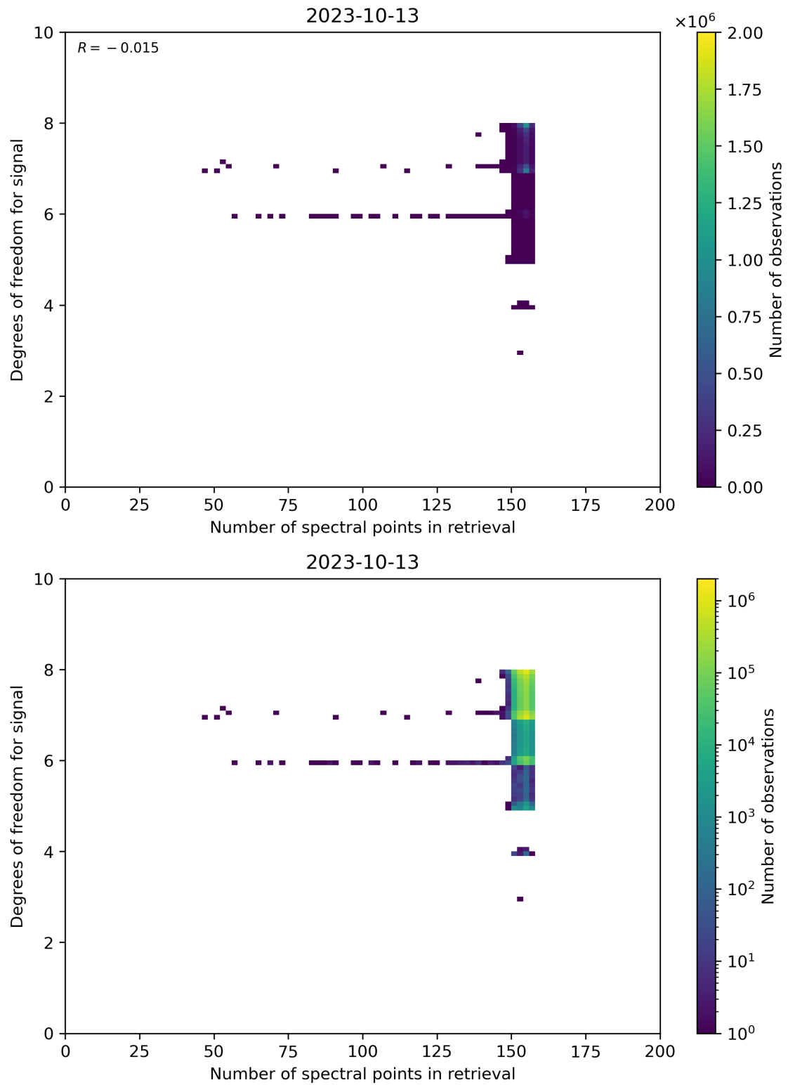
Figure 59: Scatter density plot of “Number of spectral points in retrieval” against “Degrees of freedom for signal” for 2023-10-12 to 2023-10-14.
