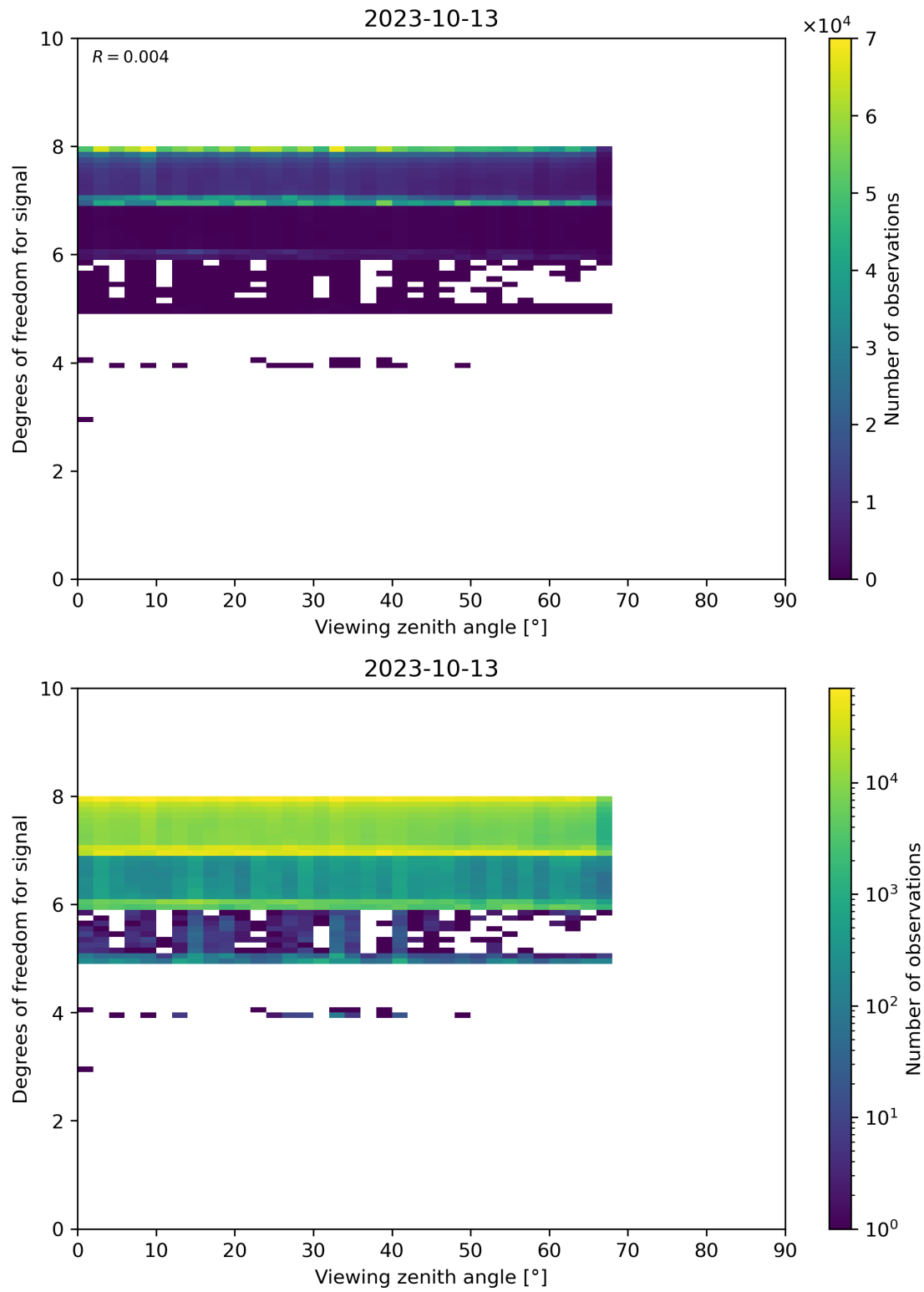
Figure 73: Scatter density plot of “Viewing zenith angle” against “Degrees of freedom for signal” for 2023-10-12 to 2023-10-14.
