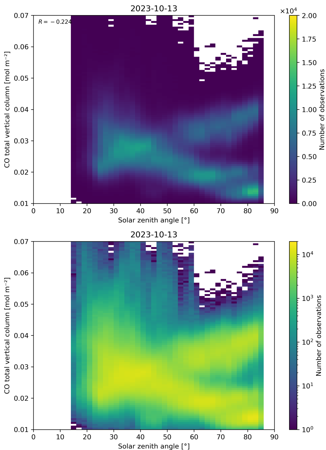
Figure 61: Scatter density plot of “Solar zenith angle” against “CO total vertical column” for 2023-10-12 to 2023-10-14.
