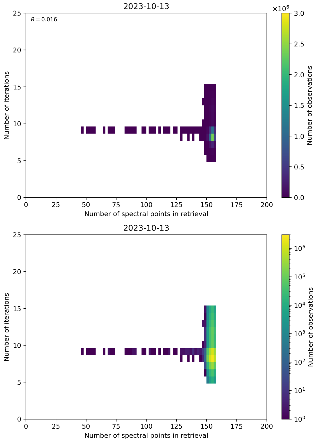
Figure 60: Scatter density plot of “Number of spectral points in retrieval” against “Number of iterations” for 2023-10-12 to 2023-10-14.
