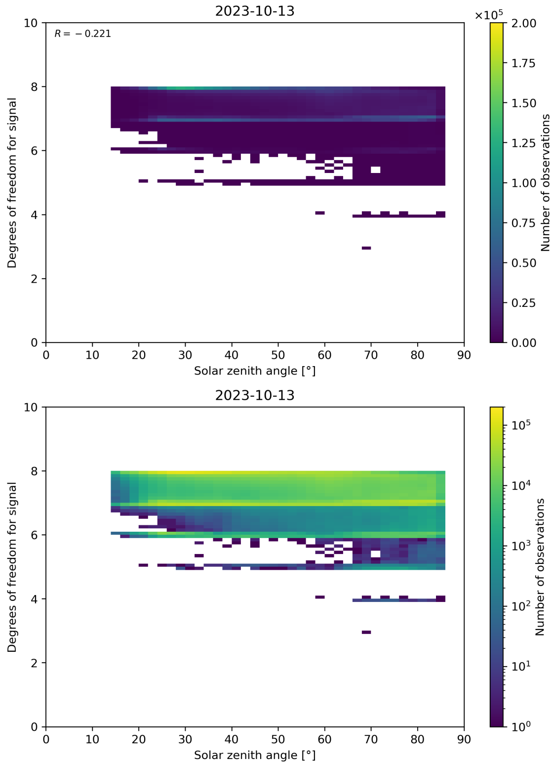
Figure 65: Scatter density plot of “Solar zenith angle” against “Degrees of freedom for signal” for 2023-10-12 to 2023-10-14.
