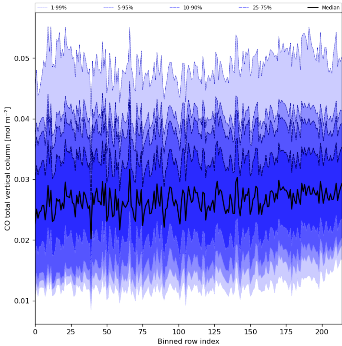
Figure 26: Along track statistics of “CO total vertical column” for 2023-10-12 to 2023-10-14
