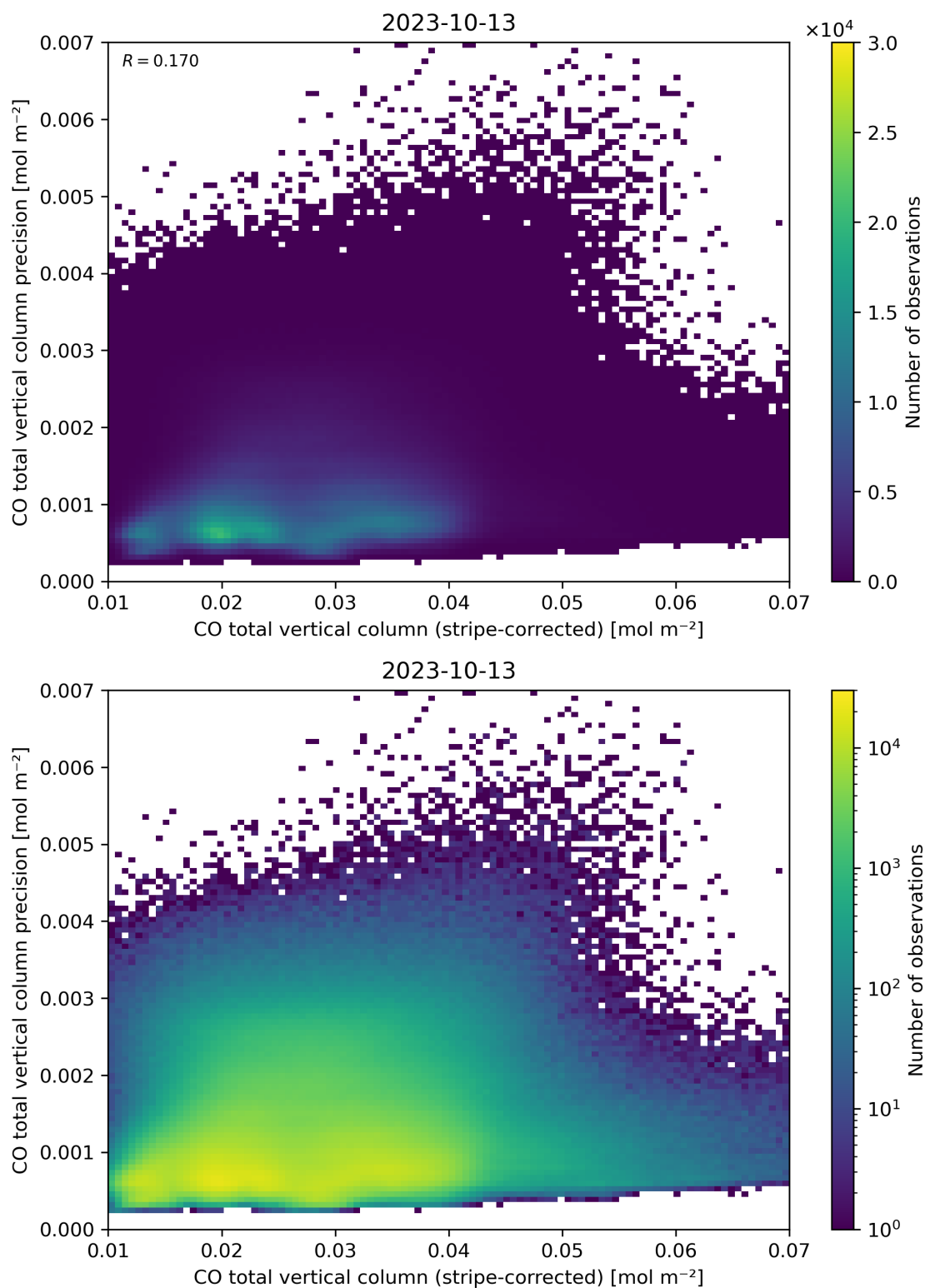
Figure 36: Scatter density plot of “CO total vertical column (stripe-corrected)” against “CO total vertical column precision” for 2023-10-12 to 2023-10-14.
