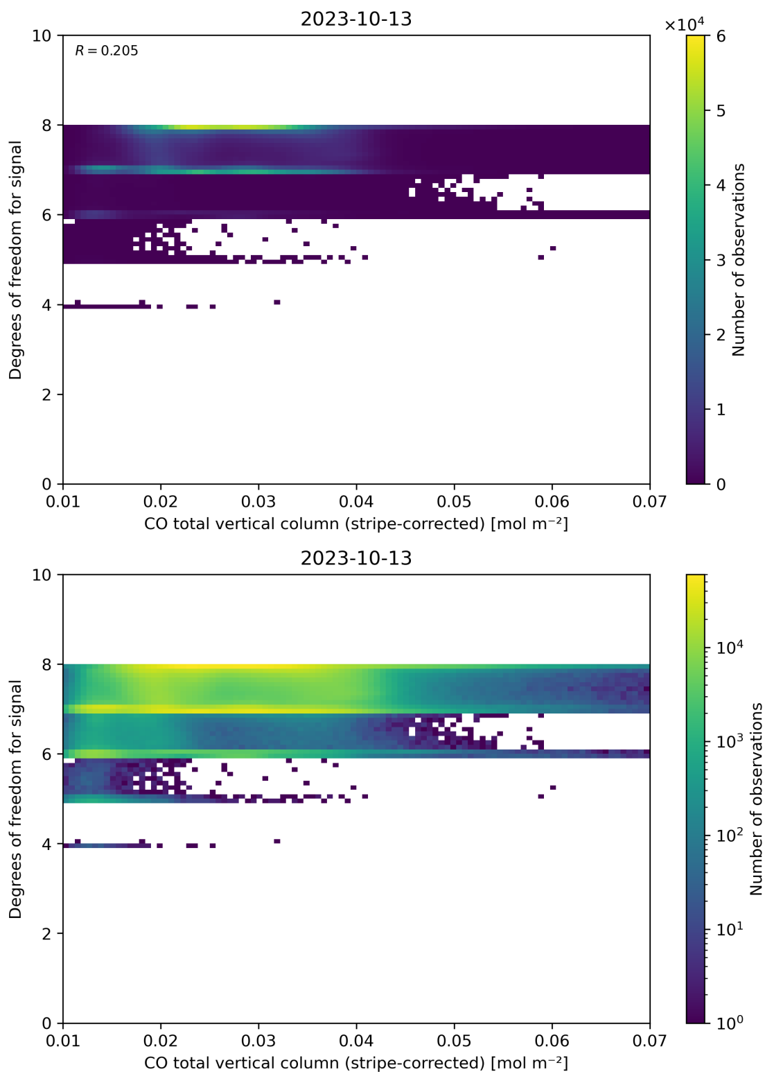
Figure 38: Scatter density plot of “CO total vertical column (stripe-corrected)” against “Degrees of freedom for signal” for 2023-10-12 to 2023-10-14.
