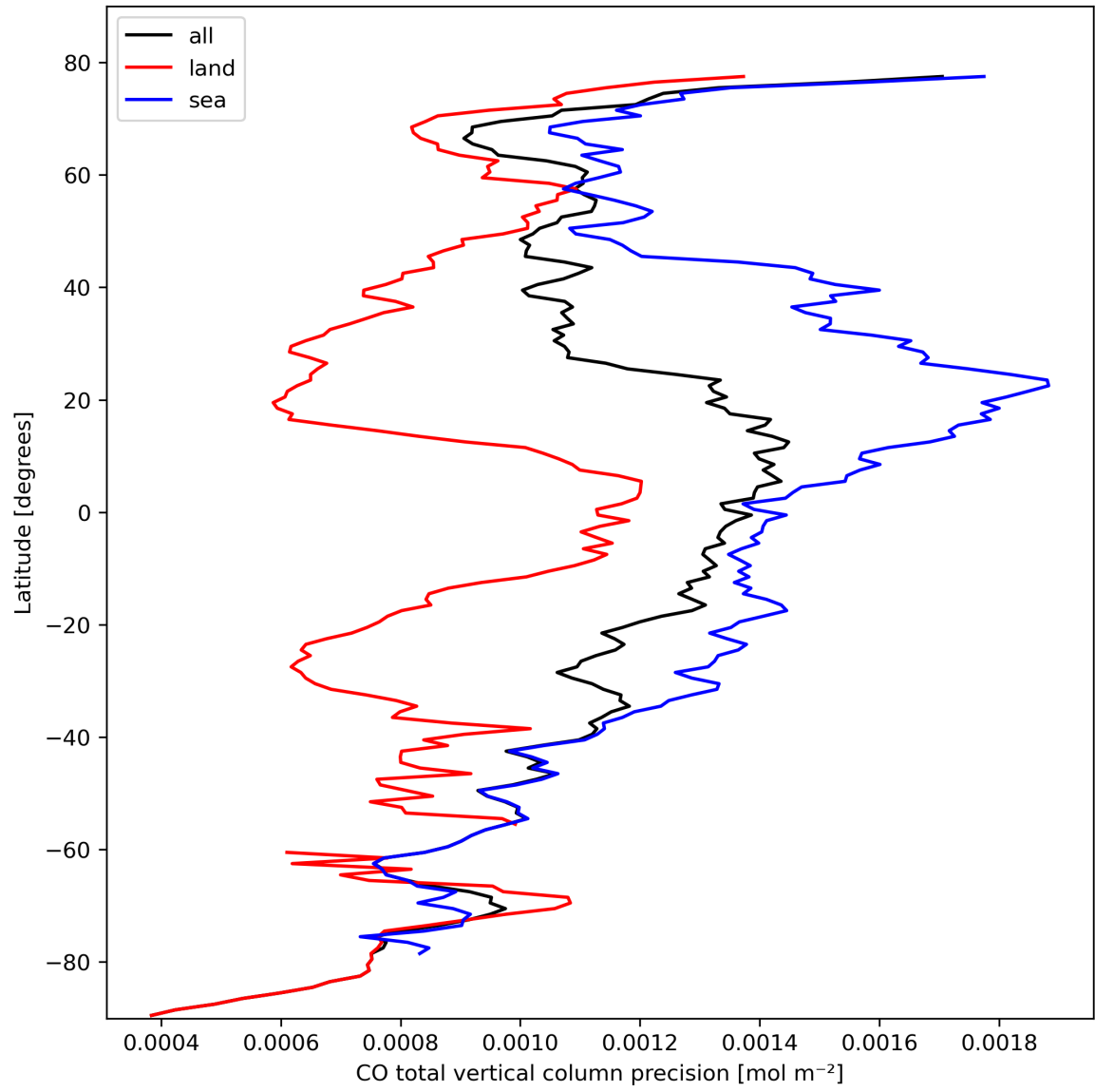
Figure 12: Zonal average of “CO total vertical column precision” for 2023-10-12 to 2023-10-14.
