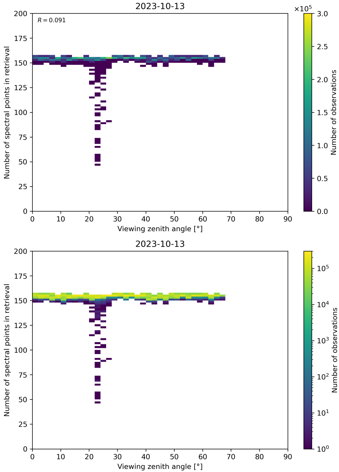
Figure 76: Scatter density plot of “Viewing zenith angle” against “Number of spectral points in retrieval” for 2023-10-12 to 2023-10-14.
