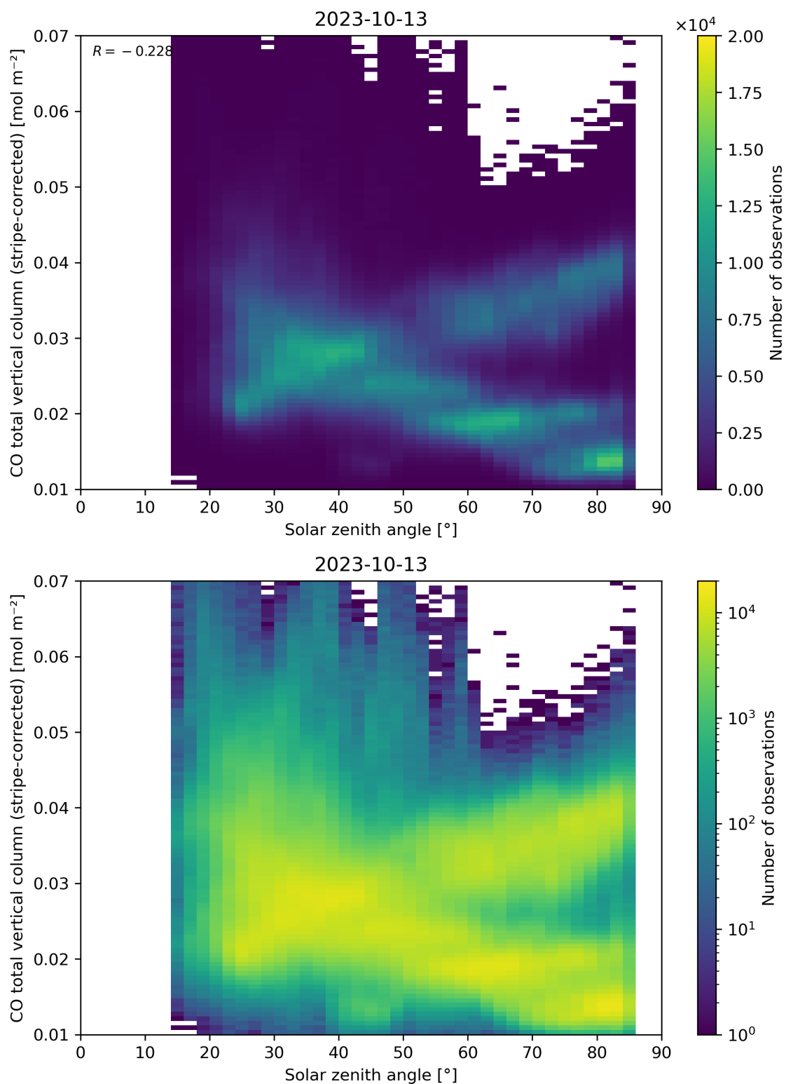
Figure 62: Scatter density plot of “Solar zenith angle” against “CO total vertical column (stripe-corrected)” for 2023-10-12 to 2023-10-14.
