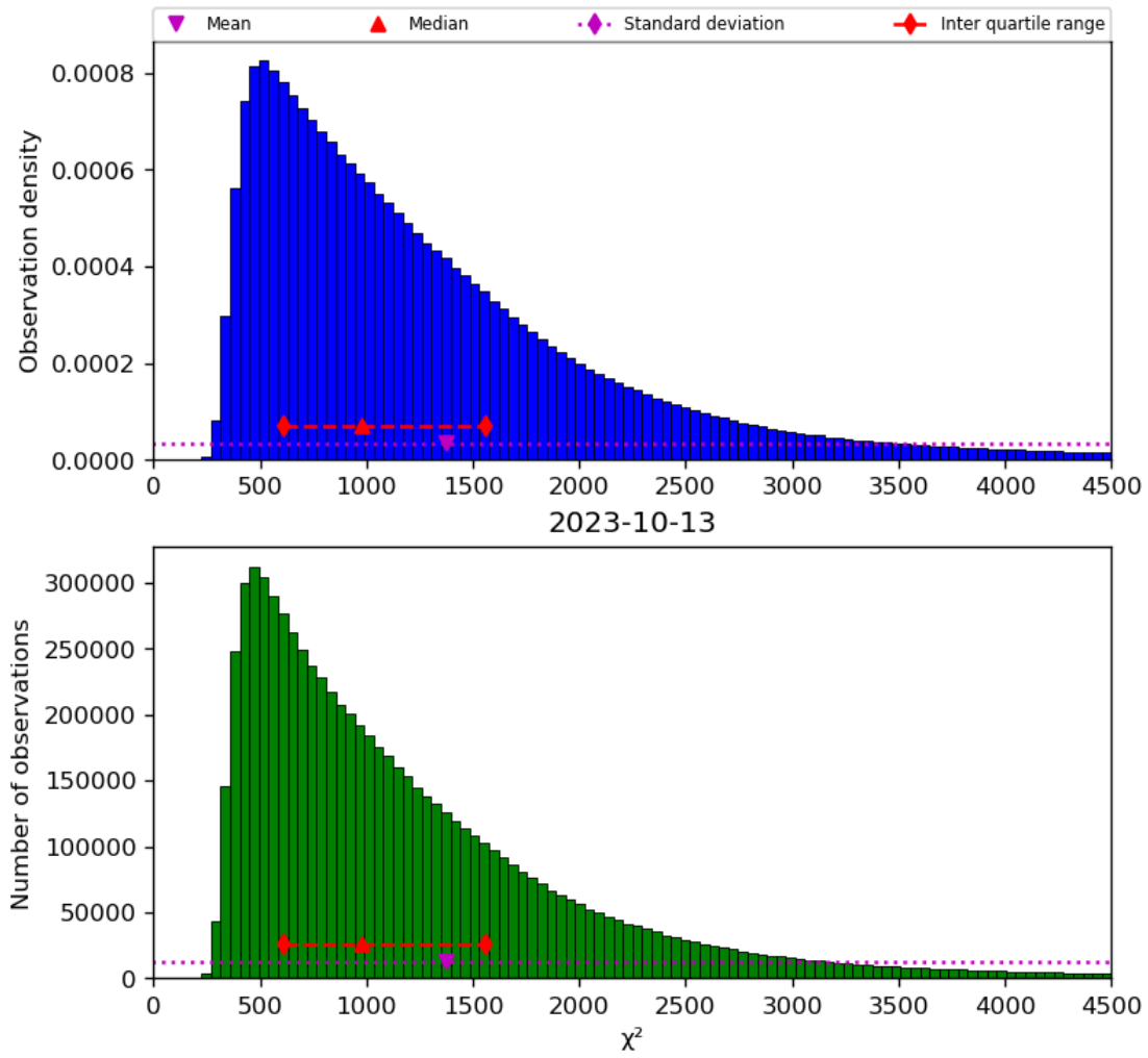
Figure 22: Histogram of “ \chi^2 ” for 2023-10-12 to 2023-10-14
