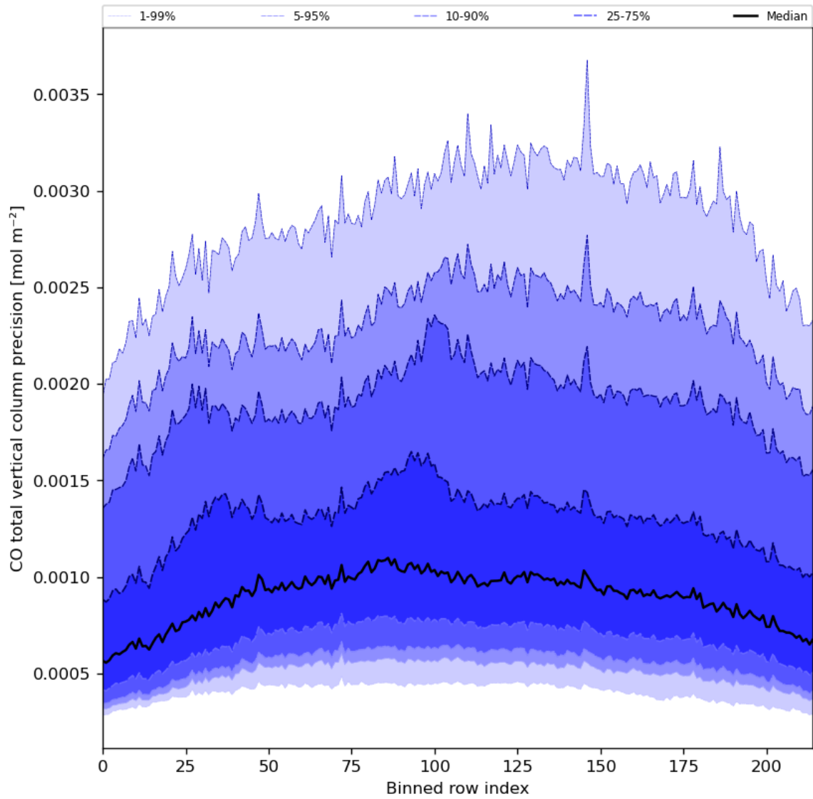
Figure 28: Along track statistics of “CO total vertical column precision” for 2023-10-12 to 2023-10-14
