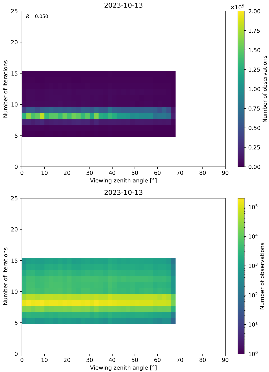
Figure 75: Scatter density plot of “Viewing zenith angle” against “Number of iterations” for 2023-10-12 to 2023-10-14.
