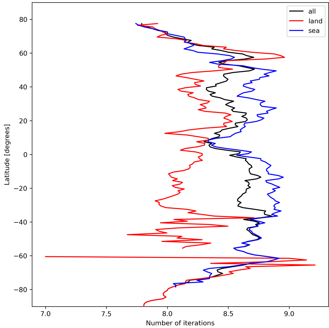
Figure 16: Zonal average of “Number of iterations” for 2023-10-12 to 2023-10-14.
