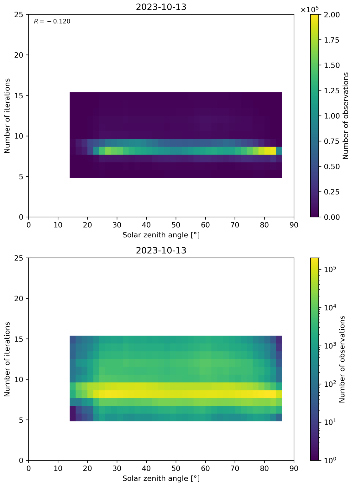
Figure 67: Scatter density plot of “Solar zenith angle” against “Number of iterations” for 2023-10-12 to 2023-10-14.
