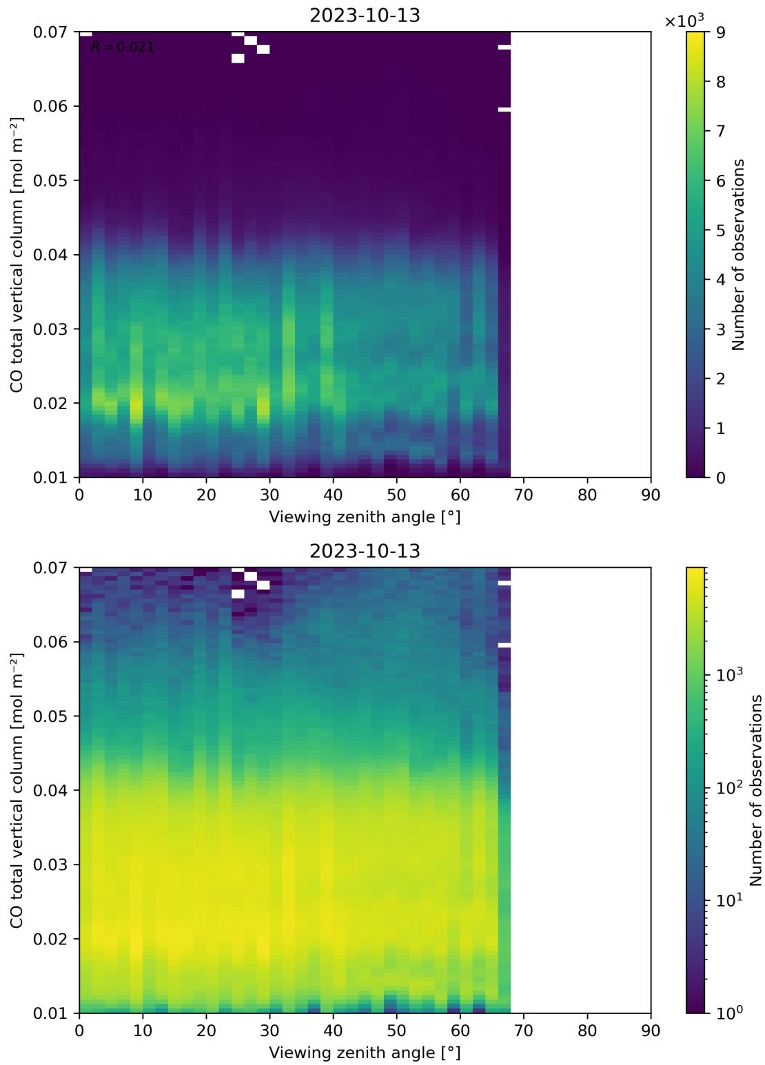
Figure 69: Scatter density plot of “Viewing zenith angle” against “CO total vertical column” for 2023-10-12 to 2023-10-14.
