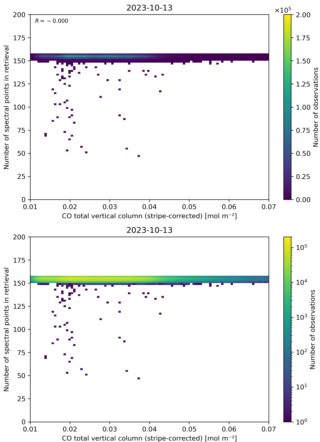
Figure 40: Scatter density plot of “CO total vertical column (stripe-corrected)” against “Number of spectral points in retrieval” for 2023-10-12 to 2023-10-14.
