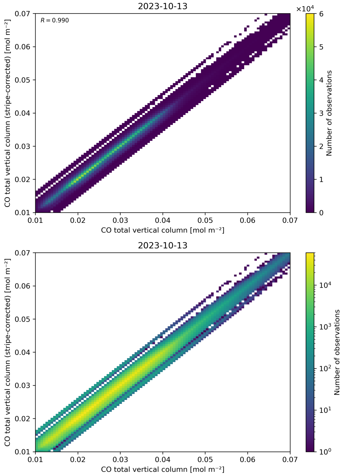
Figure 33: Scatter density plot of “CO total vertical column” against “CO total vertical column (stripe-corrected)” for 2023-10-12 to 2023-10-14.
