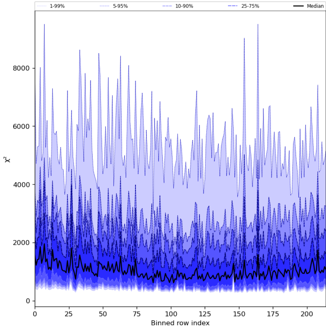
Figure 30: Along track statistics of “ \chi^2 ” for 2023-10-12 to 2023-10-14
