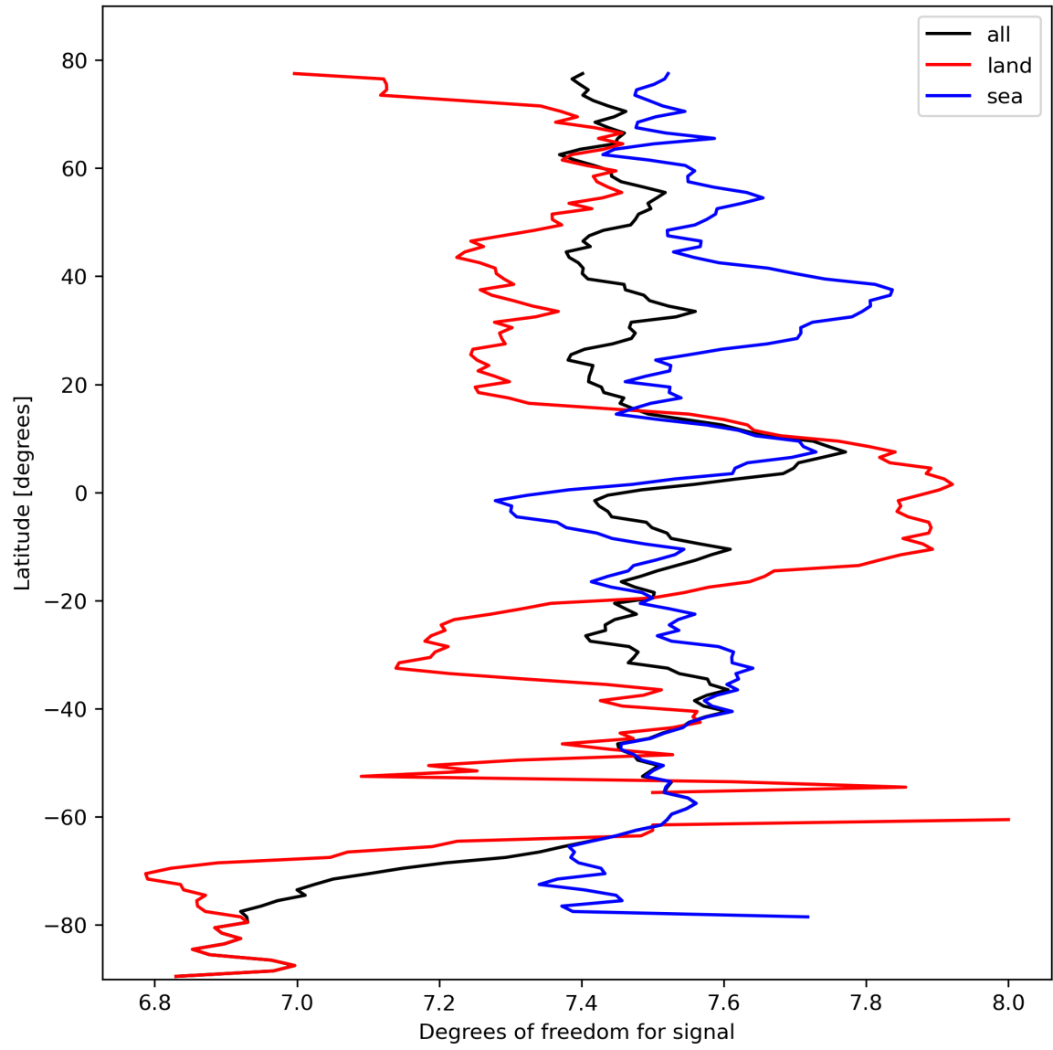
Figure 15: Zonal average of “Degrees of freedom for signal” for 2023-10-12 to 2023-10-14.
