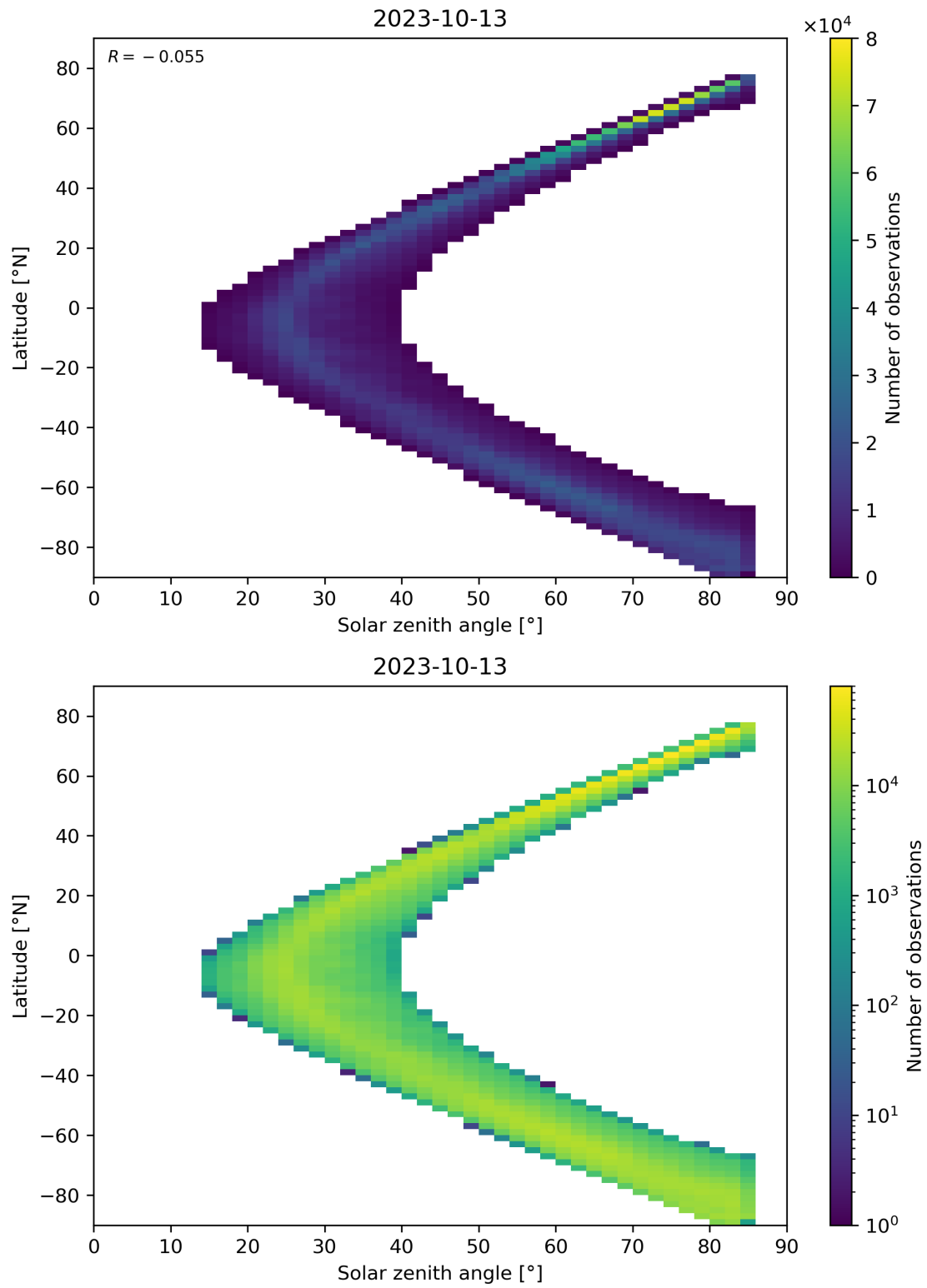
Figure 66: Scatter density plot of “Solar zenith angle” against “Latitude” for 2023-10-12 to 2023-10-14.
