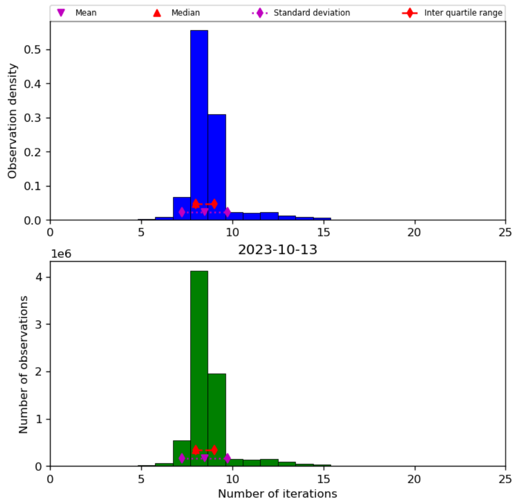
Figure 24: Histogram of “Number of iterations” for 2023-10-12 to 2023-10-14
