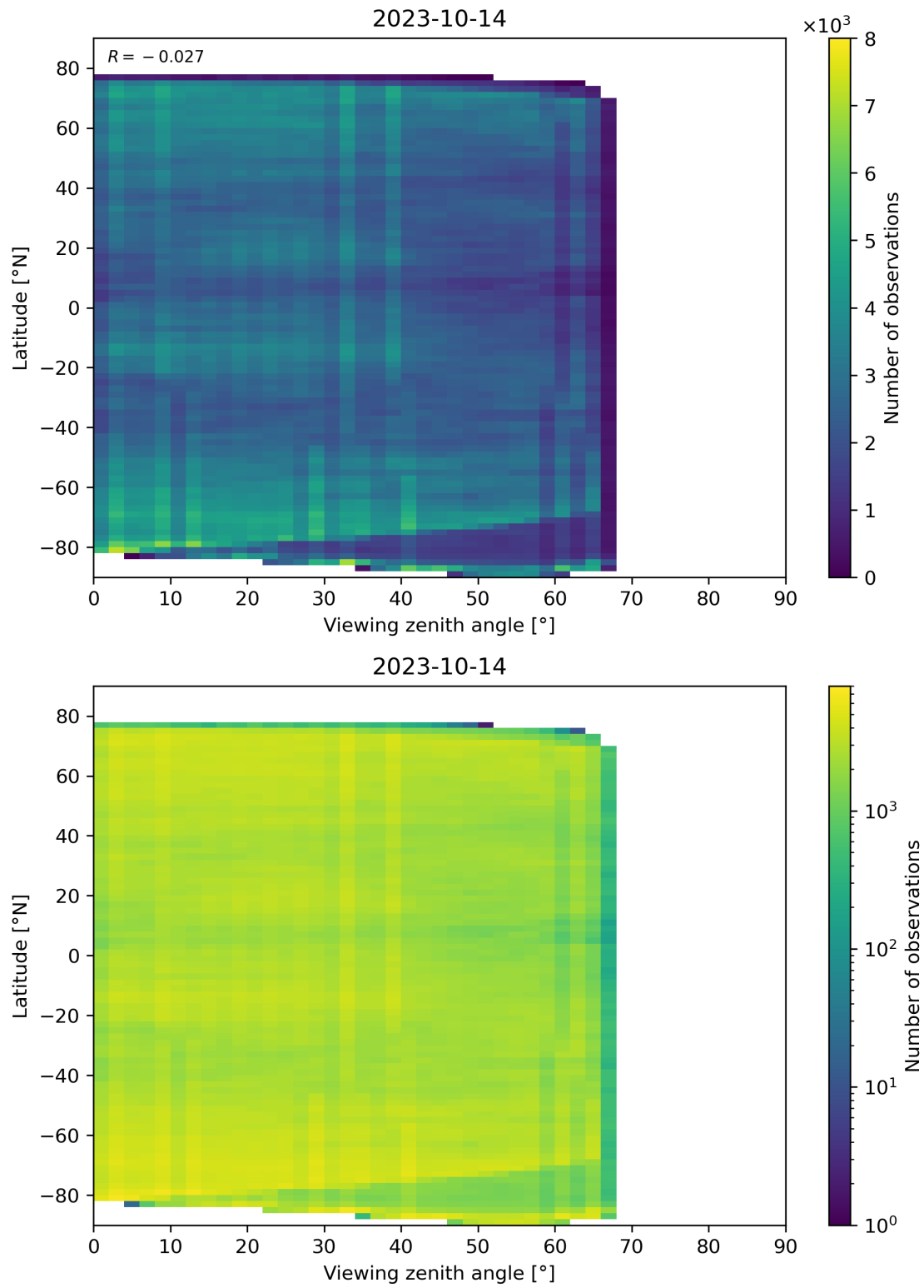
Figure 74: Scatter density plot of “Viewing zenith angle” against “Latitude” for 2023-10-13 to 2023-10-15.
