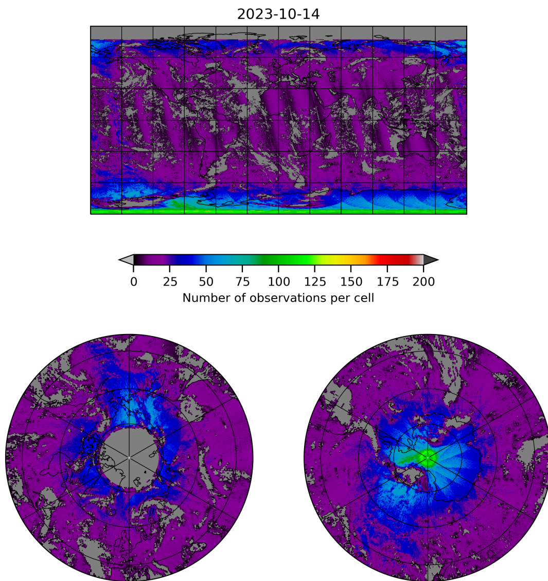
Figure 8: Map of the number of observations for 2023-10-13 to 2023-10-15
