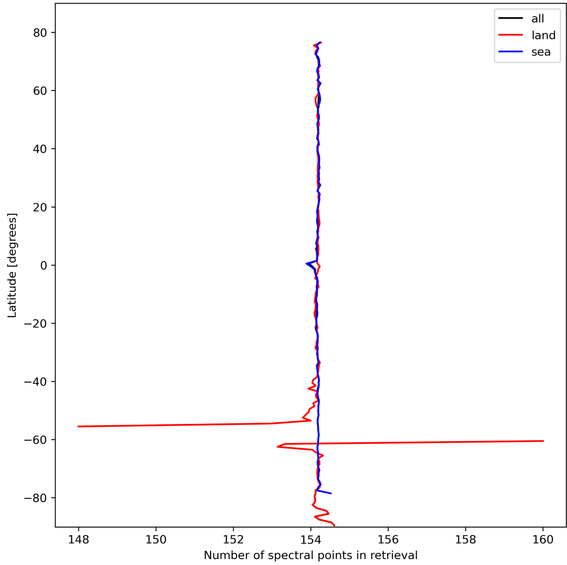
Figure 13: Zonal average of “Number of spectral points in retrieval” for 2023-10-13 to 2023-10-15.
