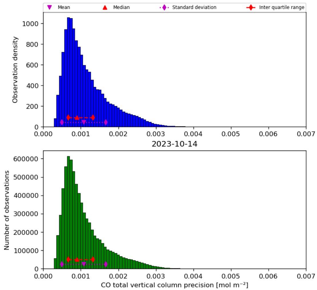
Figure 20: Histogram of “CO total vertical column precision” for 2023-10-13 to 2023-10-15
