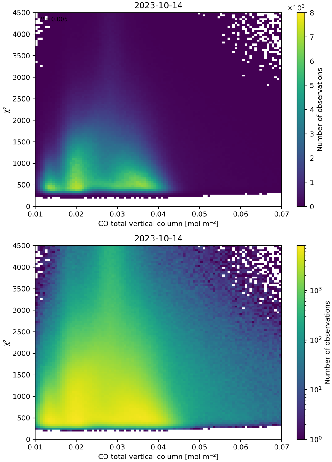
Figure 35: Scatter density plot of “CO total vertical column” against “ \chi^2 ” for 2023-10-13 to 2023-10-15.
