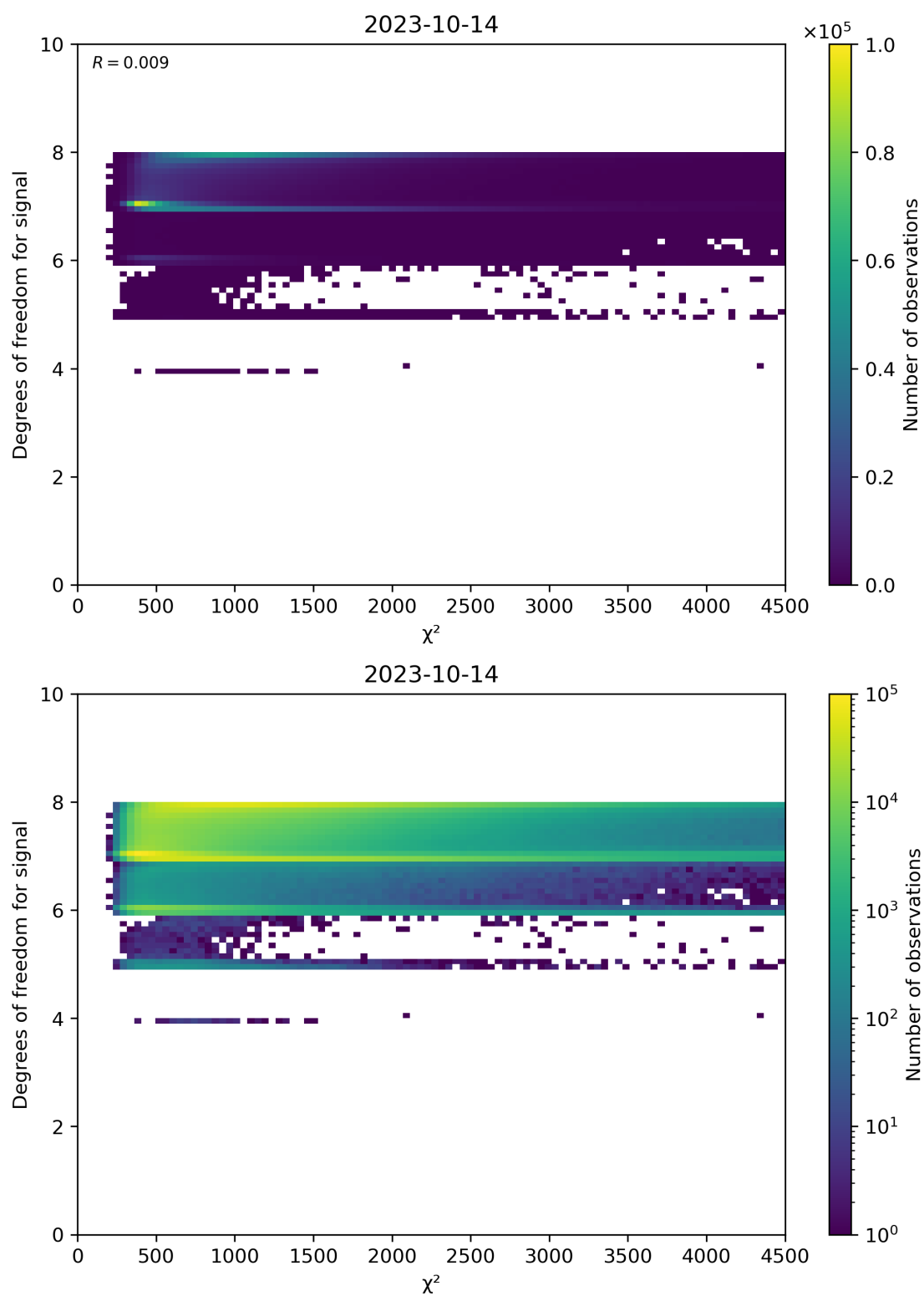
Figure 48: Scatter density plot of “ \chi^2 ” against “Degrees of freedom for signal” for 2023-10-13 to 2023-10-15.
