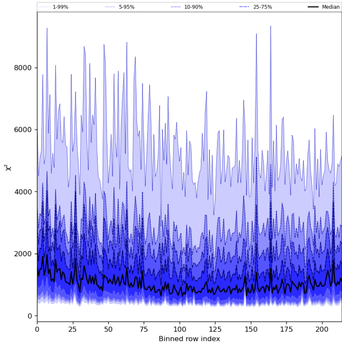
Figure 30: Along track statistics of “ \chi^2 ” for 2023-10-13 to 2023-10-15
