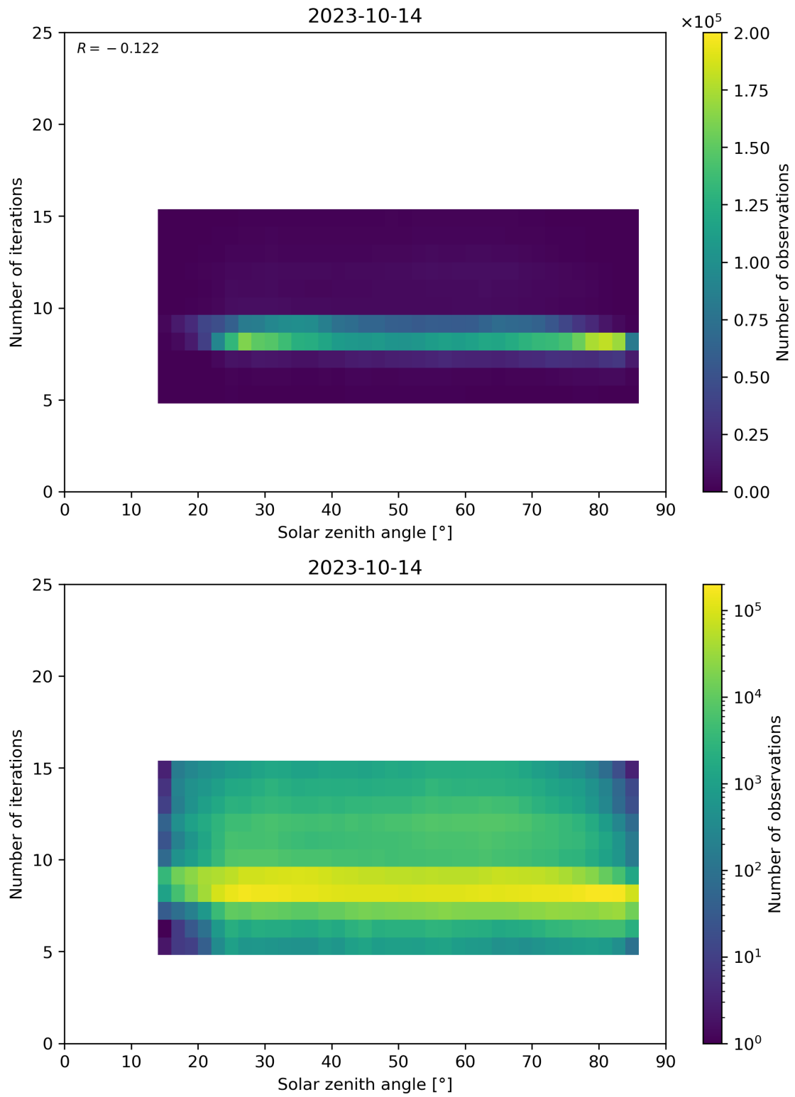
Figure 67: Scatter density plot of “Solar zenith angle” against “Number of iterations” for 2023-10-13 to 2023-10-15.
