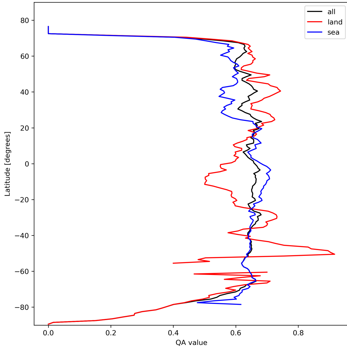
Figure 9: Zonal average of “QA value” for 2023-10-13 to 2023-10-15.
