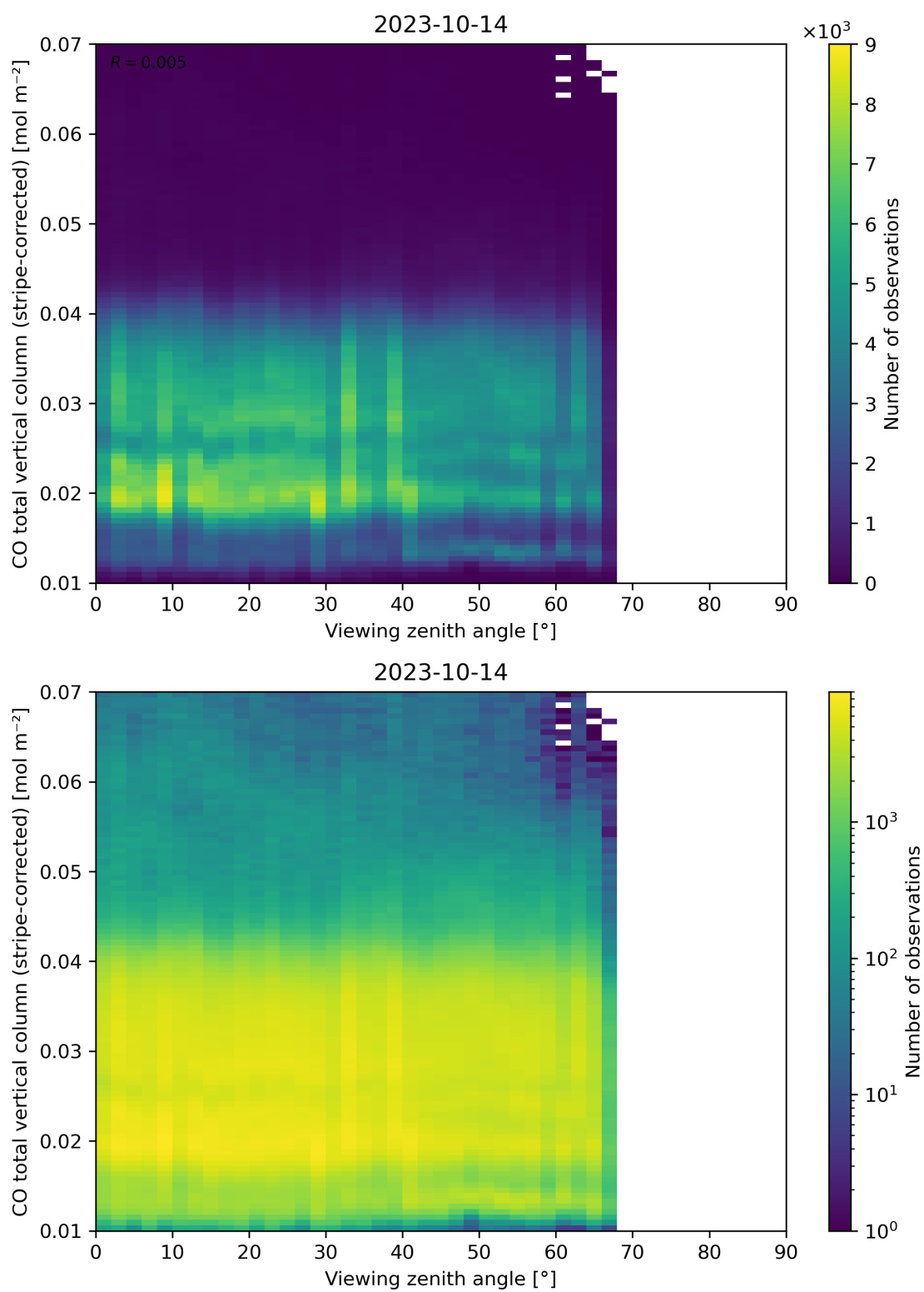
Figure 70: Scatter density plot of “Viewing zenith angle” against “CO total vertical column (stripe-corrected)” for 2023-10-13 to 2023-10-15.
