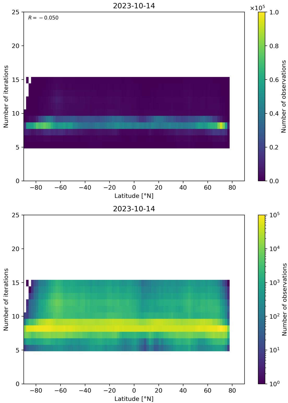
Figure 56: Scatter density plot of “Latitude” against “Number of iterations” for 2023-10-13 to 2023-10-15.
