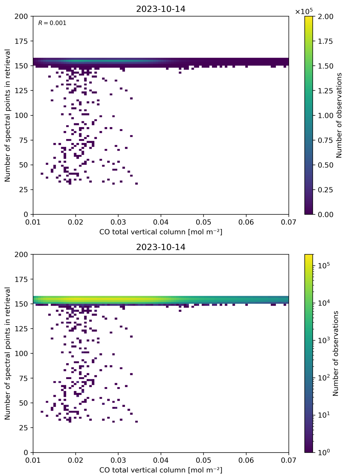
Figure 43: Scatter density plot of “CO total vertical column” against “Number of spectral points in retrieval” for 2023-10-13 to 2023-10-15.
