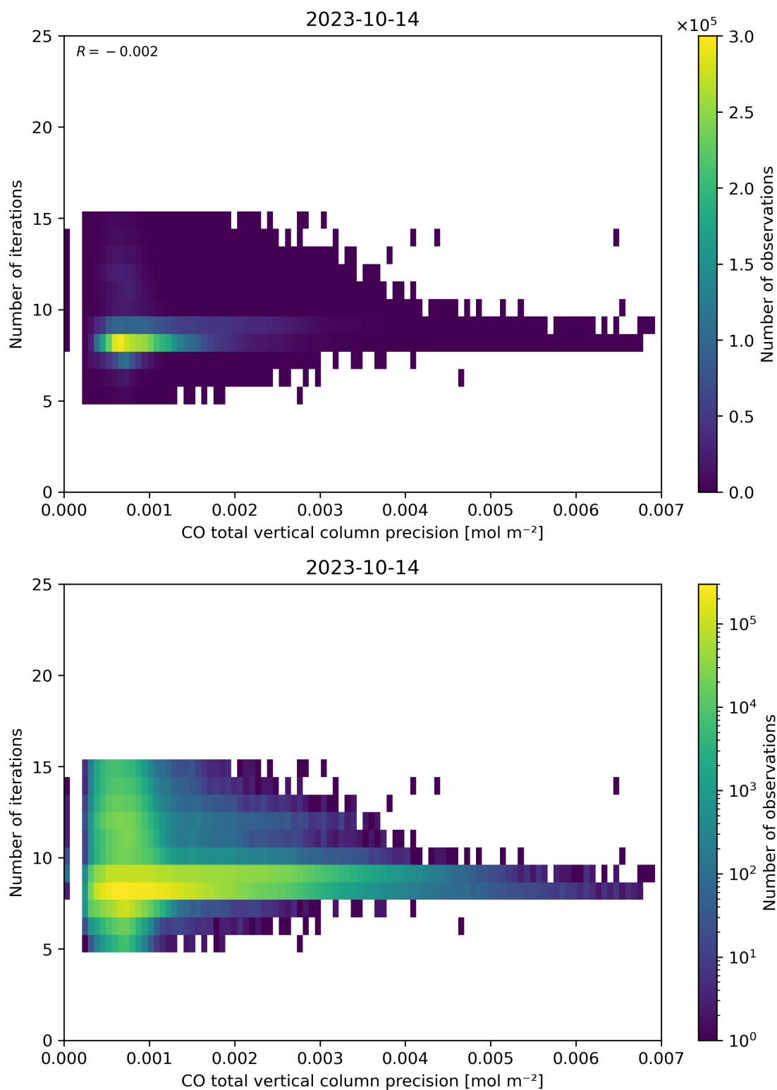
Figure 46: Scatter density plot of “CO total vertical column precision” against “Number of iterations” for 2023-10-13 to 2023-10-15.
