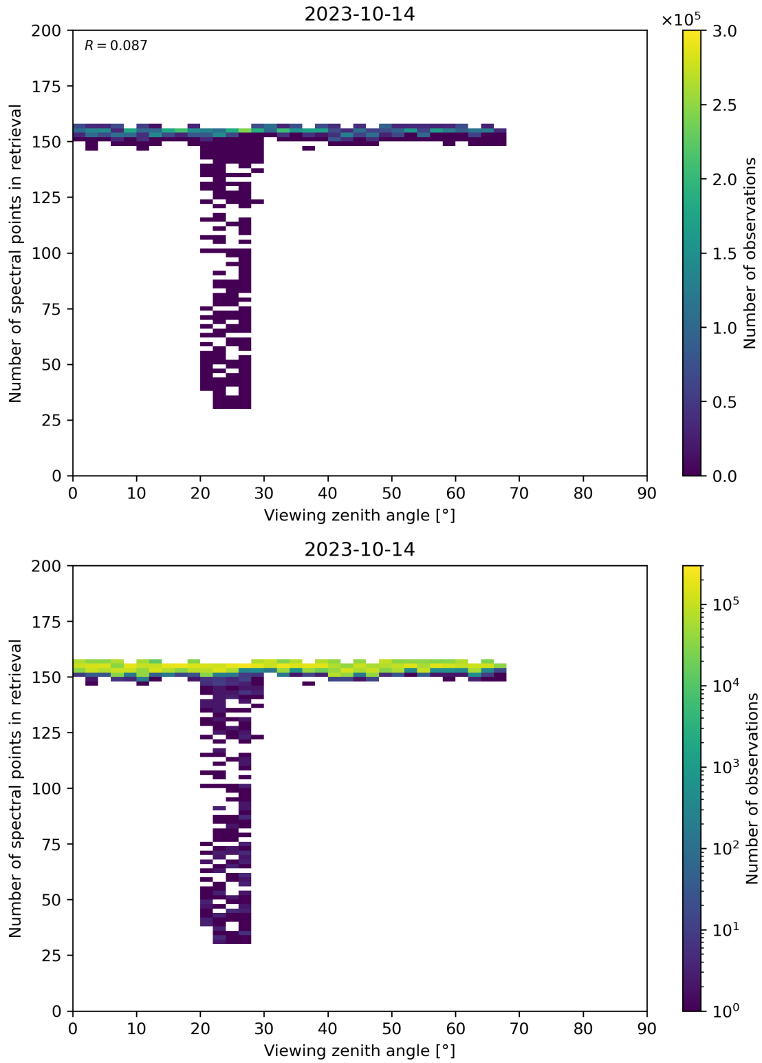
Figure 76: Scatter density plot of “Viewing zenith angle” against “Number of spectral points in retrieval” for 2023-10-13 to 2023-10-15.
