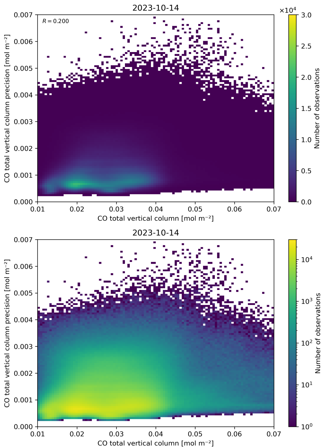
Figure 34: Scatter density plot of “CO total vertical column” against “CO total vertical column precision” for 2023-10-13 to 2023-10-15.
