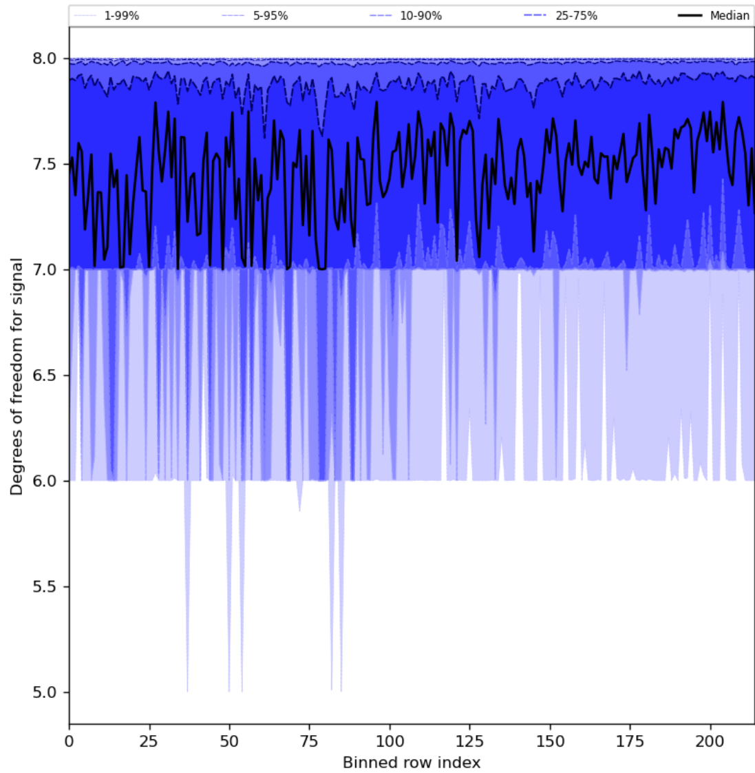
Figure 31: Along track statistics of “Degrees of freedom for signal” for 2023-10-13 to 2023-10-15
