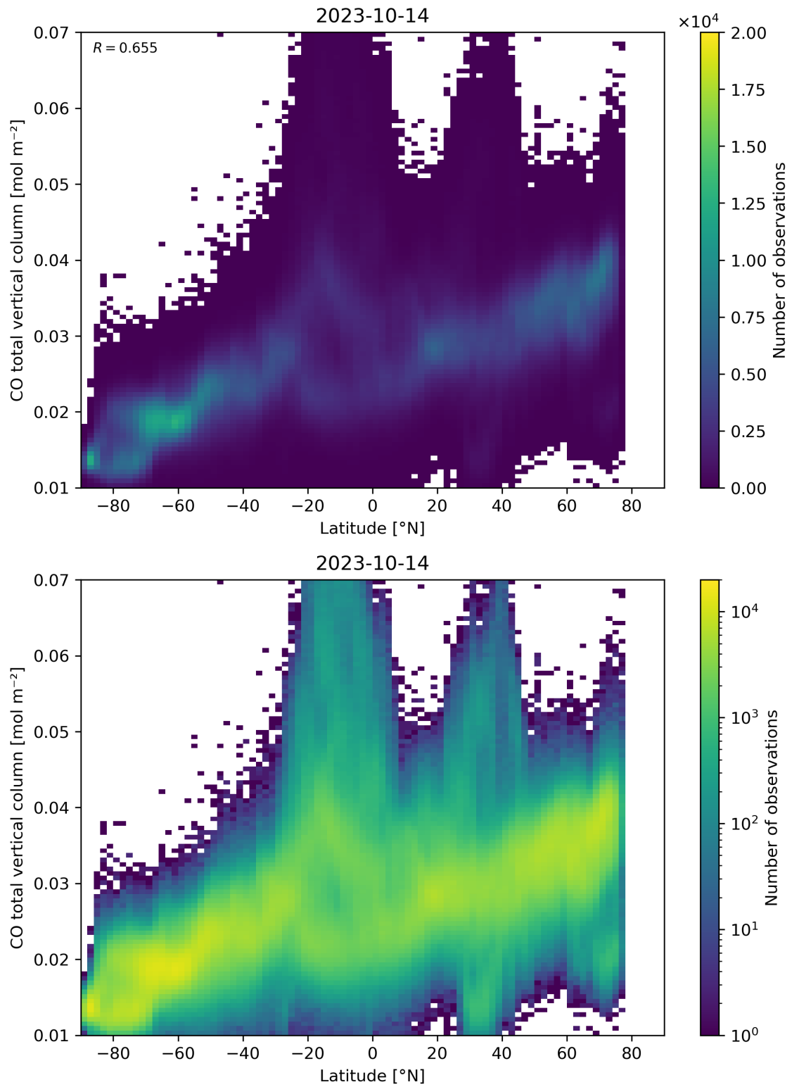
Figure 51: Scatter density plot of “Latitude” against “CO total vertical column” for 2023-10-13 to 2023-10-15.
