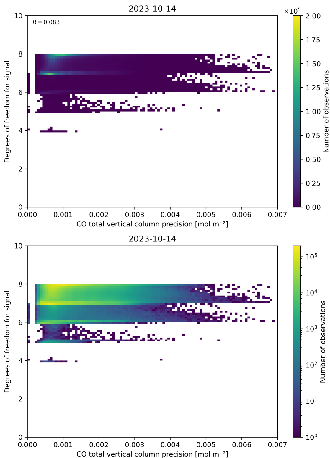
Figure 45: Scatter density plot of “CO total vertical column precision” against “Degrees of freedom for signal” for 2023-10-13 to 2023-10-15.
