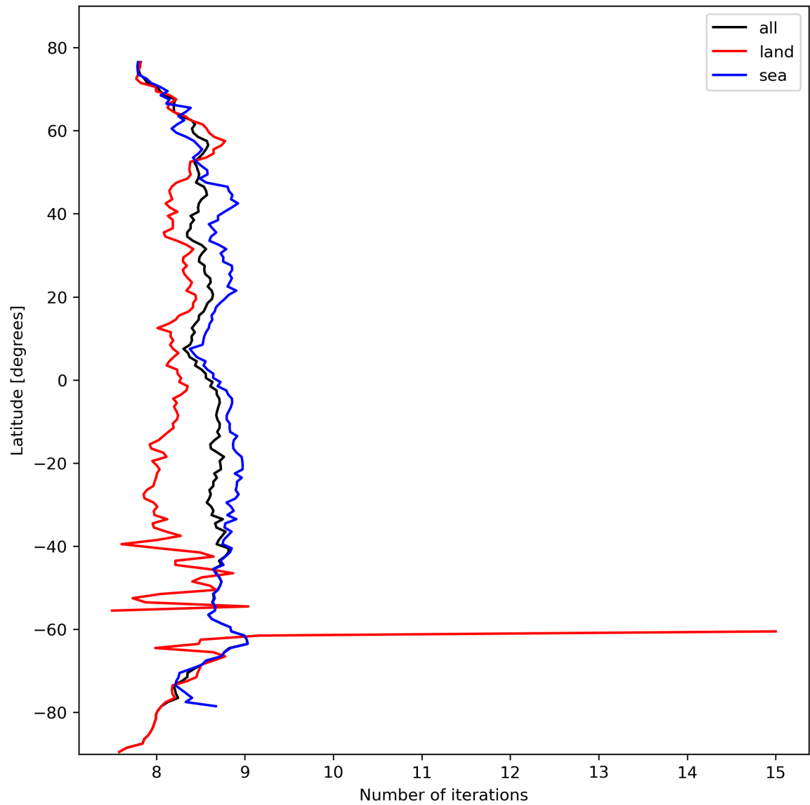
Figure 16: Zonal average of “Number of iterations” for 2023-10-13 to 2023-10-15.
