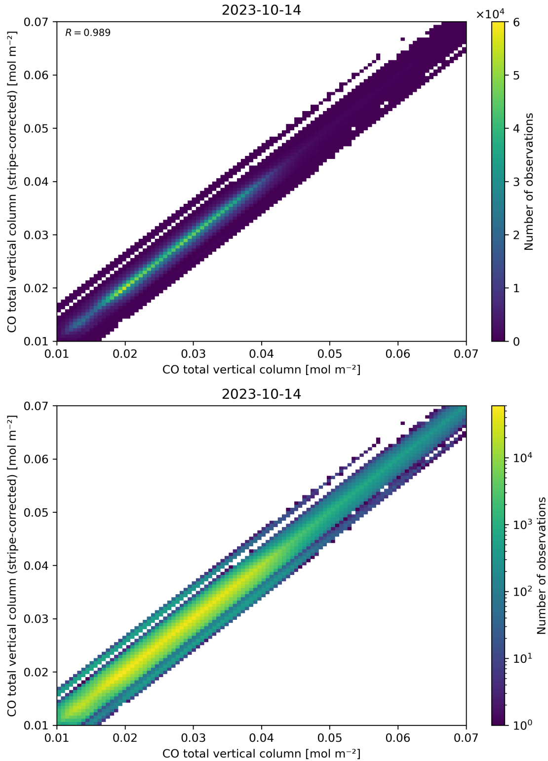
Figure 33: Scatter density plot of “CO total vertical column” against “CO total vertical column (stripe-corrected)” for 2023-10-13 to 2023-10-15.
