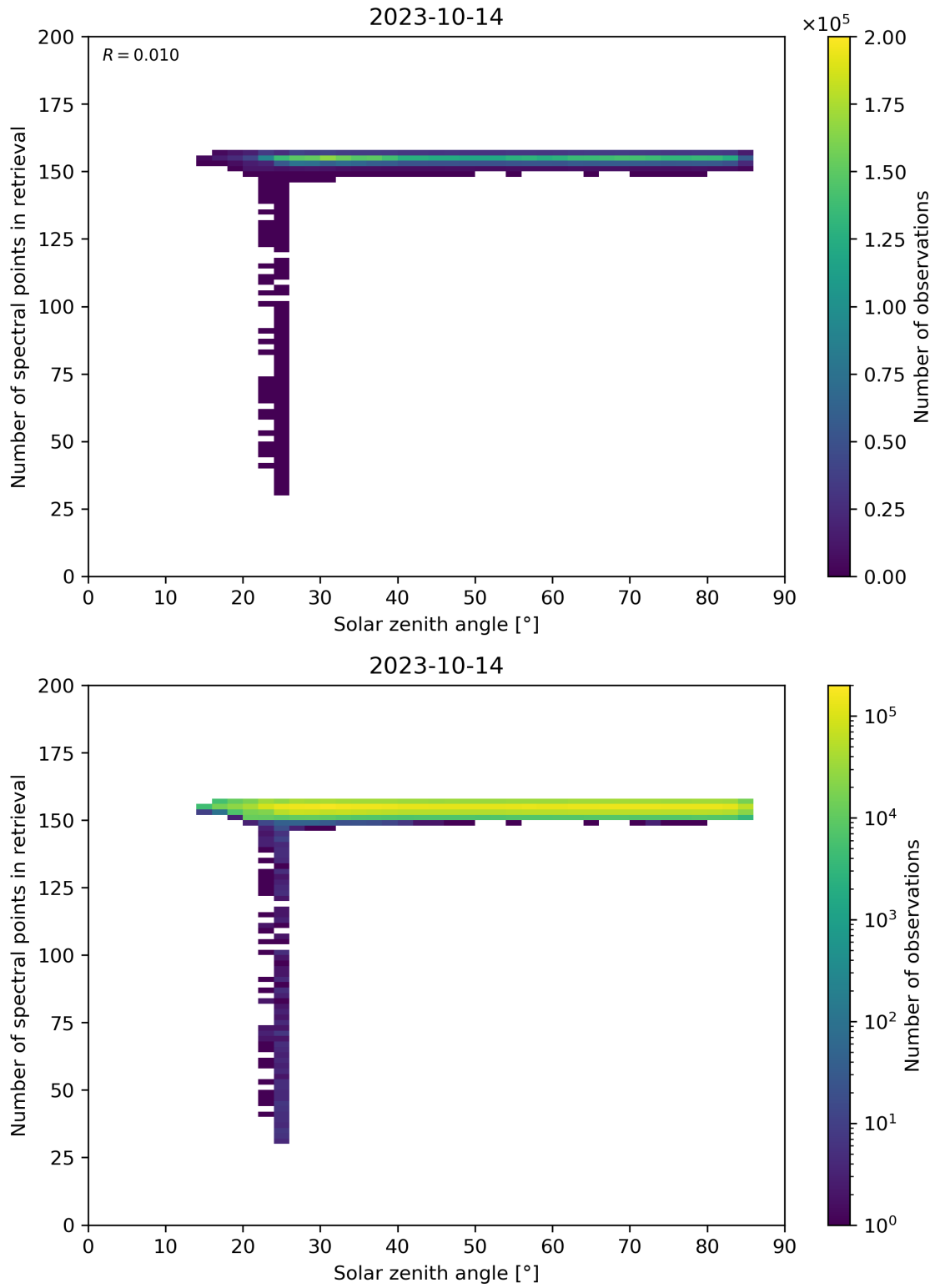
Figure 68: Scatter density plot of “Solar zenith angle” against “Number of spectral points in retrieval” for 2023-10-13 to 2023-10-15.
