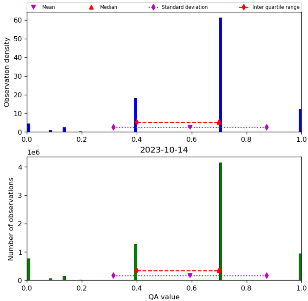
Figure 17: Histogram of “QA value” for 2023-10-13 to 2023-10-15
