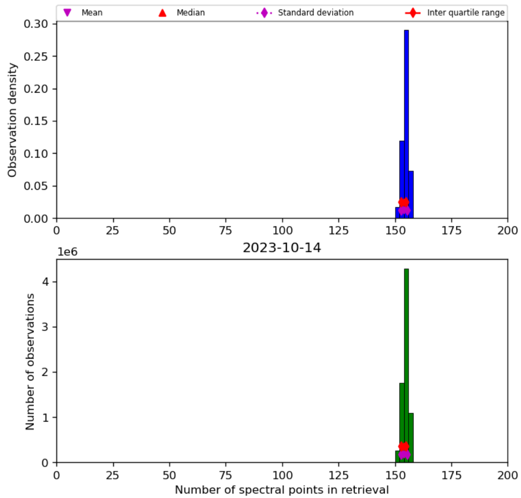
Figure 21: Histogram of “Number of spectral points in retrieval” for 2023-10-13 to 2023-10-15
