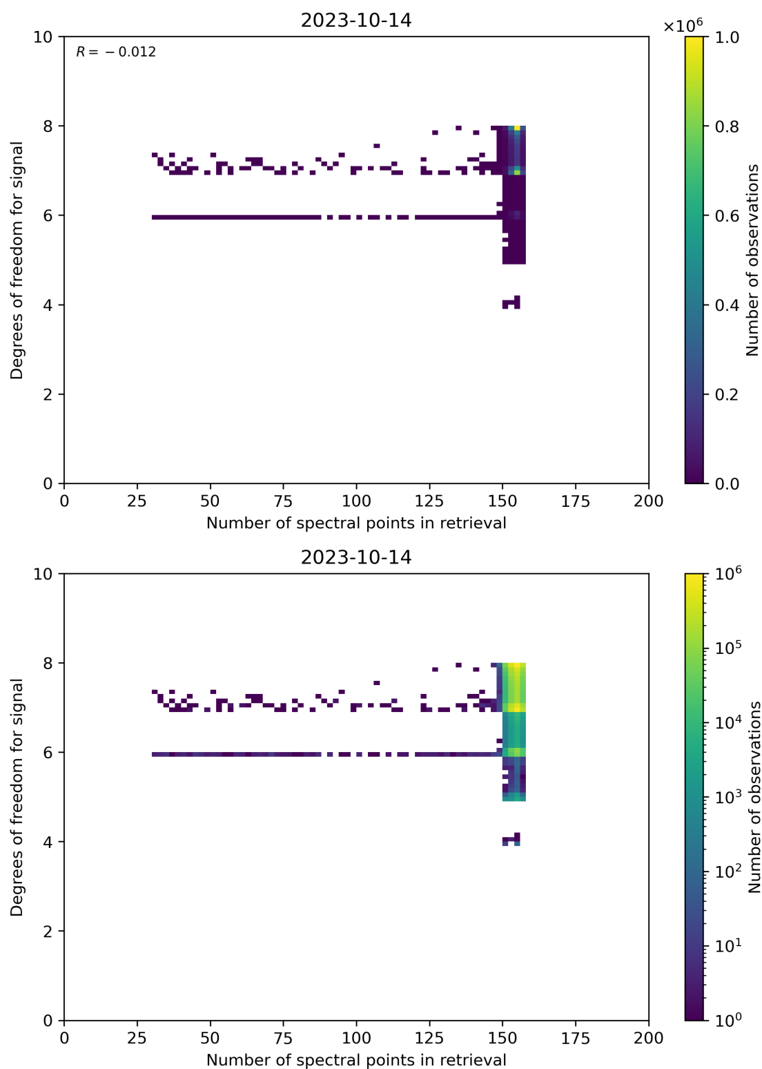
Figure 59: Scatter density plot of “Number of spectral points in retrieval” against “Degrees of freedom for signal” for 2023-10-13 to 2023-10-15.
