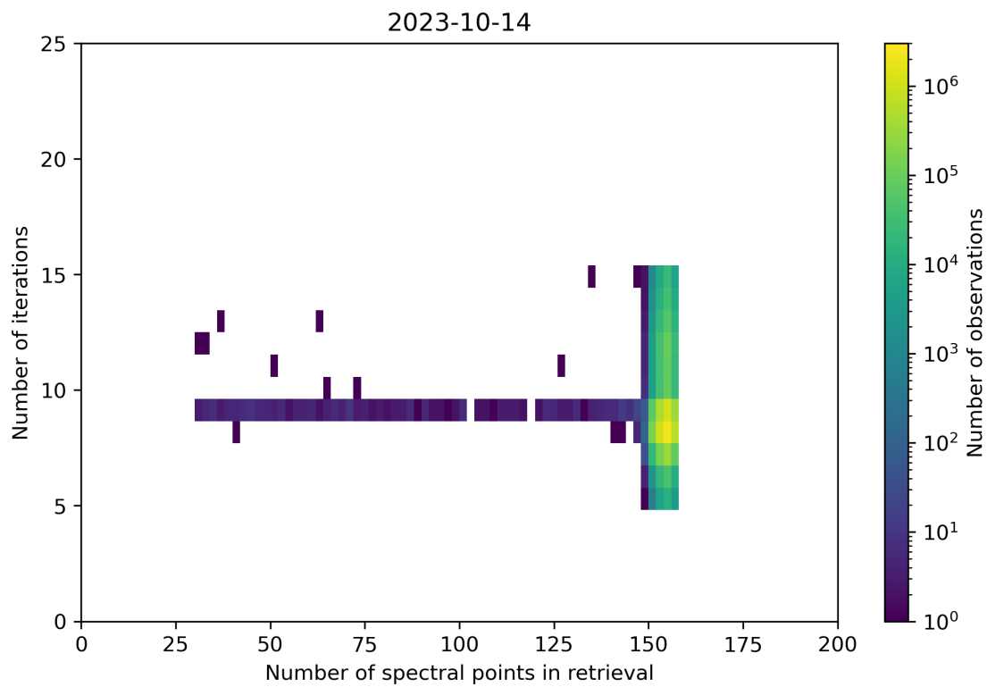
Figure 60: Scatter density plot of “Number of spectral points in retrieval” against “Number of iterations” for 2023-10-13 to 2023-10-15.
