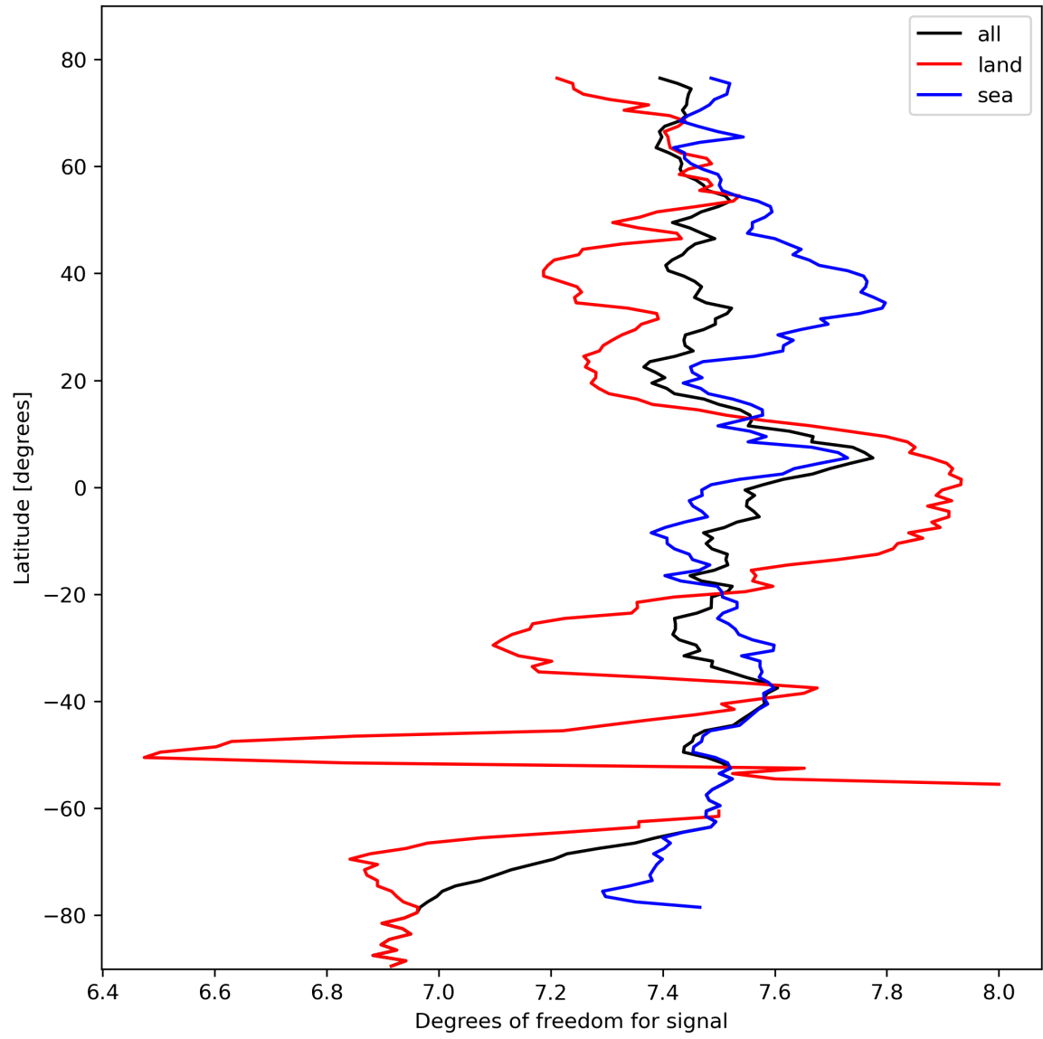
Figure 15: Zonal average of “Degrees of freedom for signal” for 2023-10-13 to 2023-10-15.
