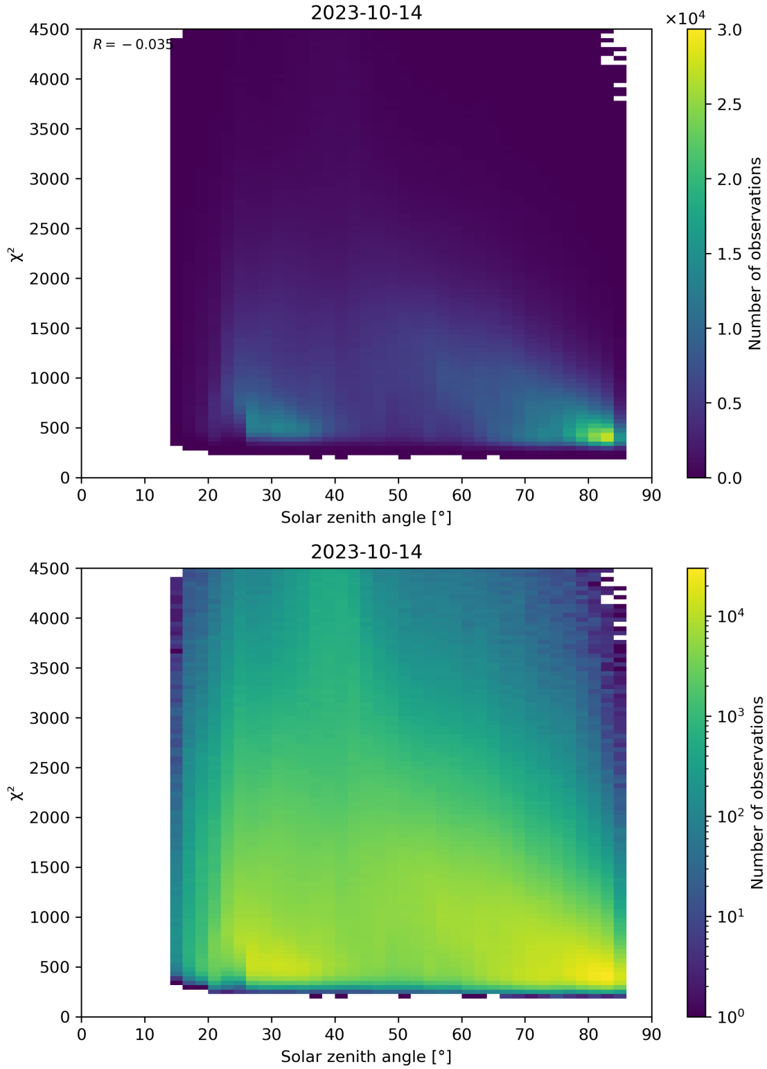
Figure 64: Scatter density plot of “Solar zenith angle” against “ \chi^2 ” for 2023-10-13 to 2023-10-15.
