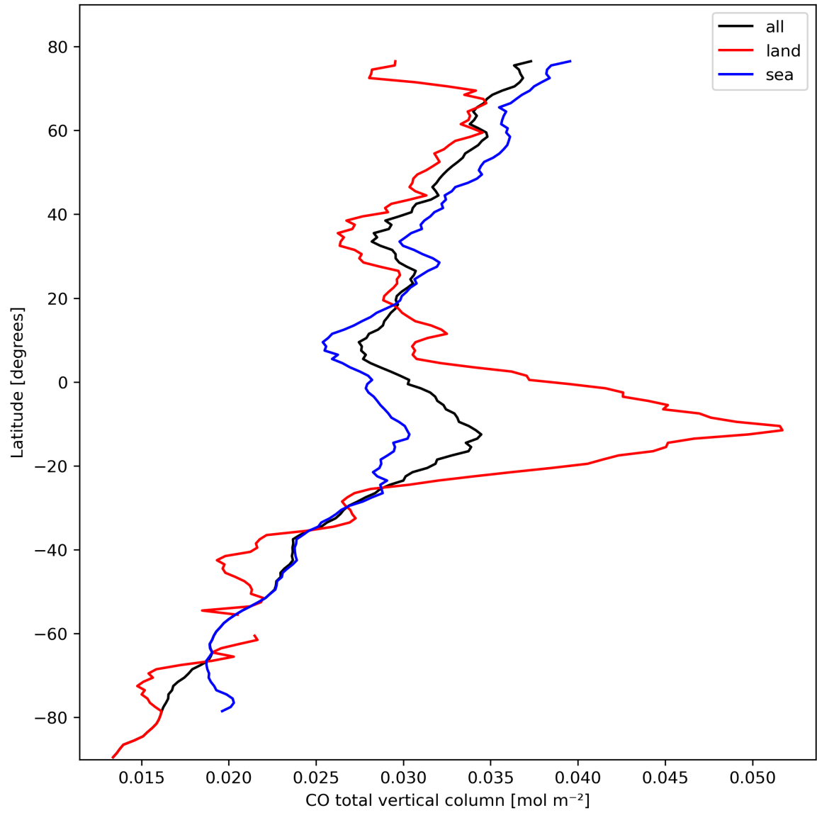
Figure 10: Zonal average of “CO total vertical column” for 2023-10-13 to 2023-10-15.
