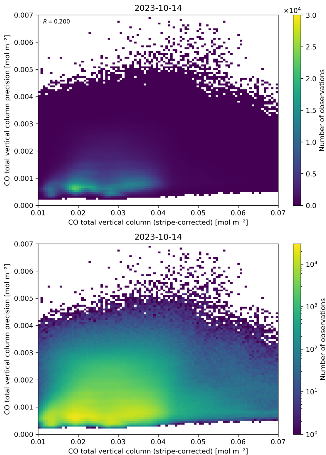
Figure 36: Scatter density plot of “CO total vertical column (stripe-corrected)” against “CO total vertical column precision” for 2023-10-13 to 2023-10-15.
