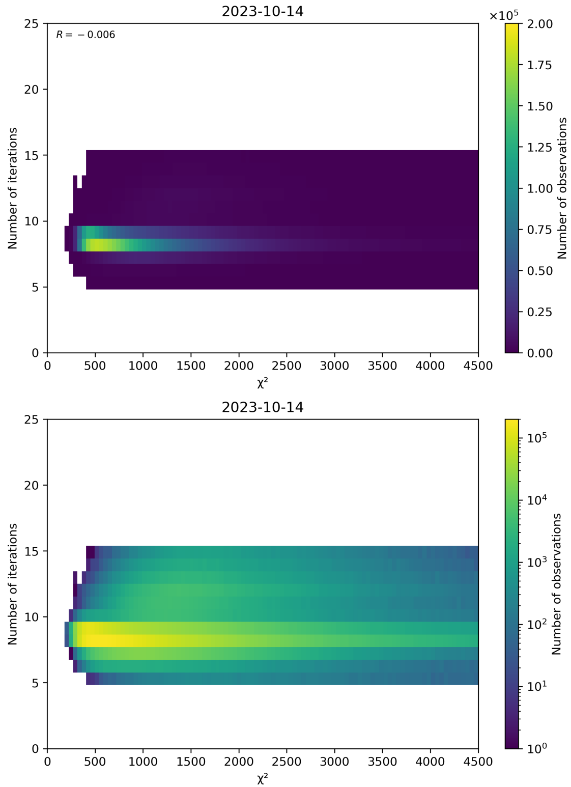
Figure 49: Scatter density plot of “ \chi^2 ” against “Number of iterations” for 2023-10-13 to 2023-10-15.
