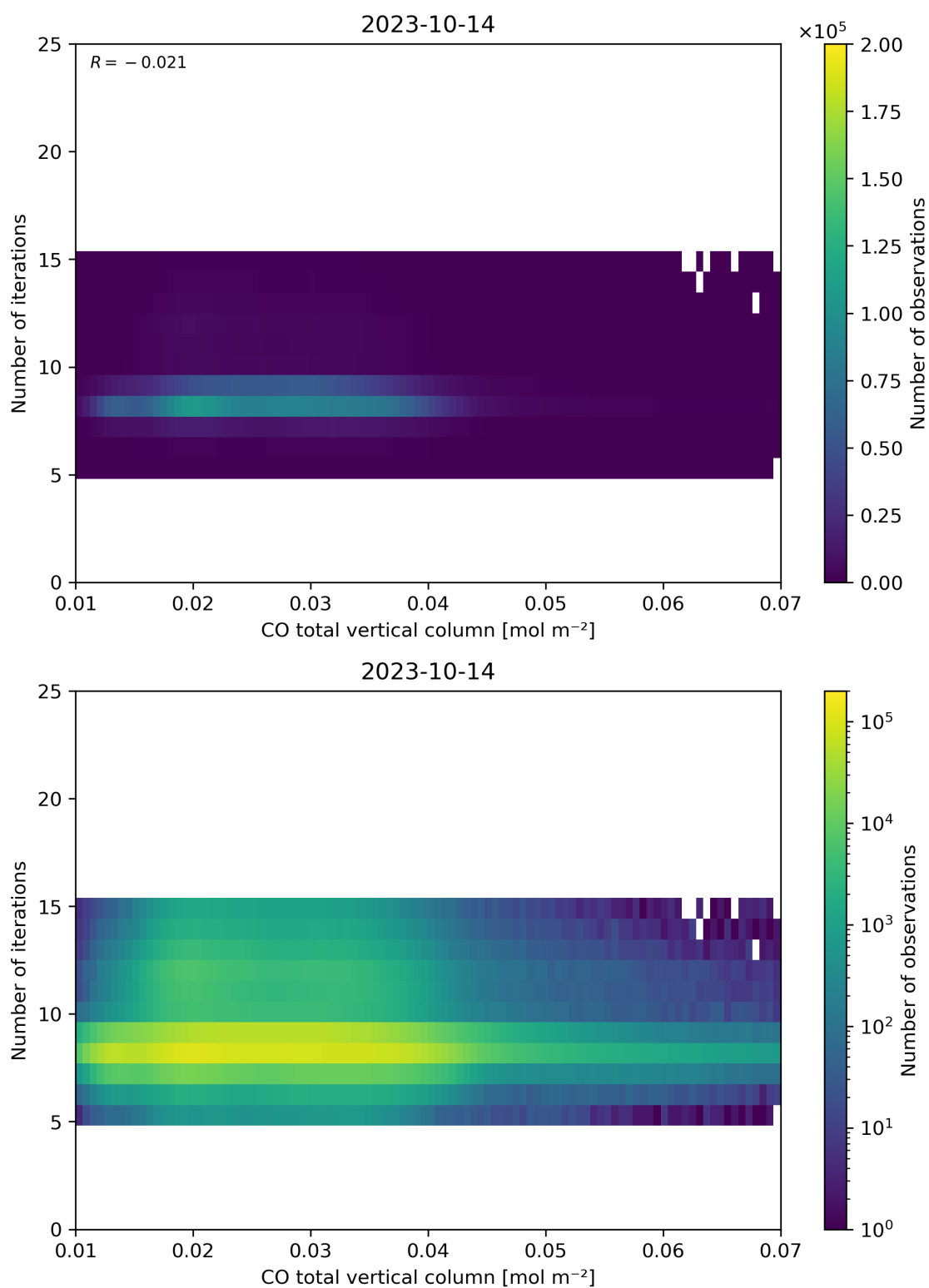
Figure 42: Scatter density plot of “CO total vertical column” against “Number of iterations” for 2023-10-13 to 2023-10-15.
