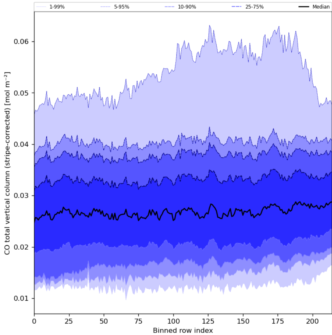
Figure 27: Along track statistics of “CO total vertical column (stripe-corrected)” for 2023-10-13 to 2023-10-15
