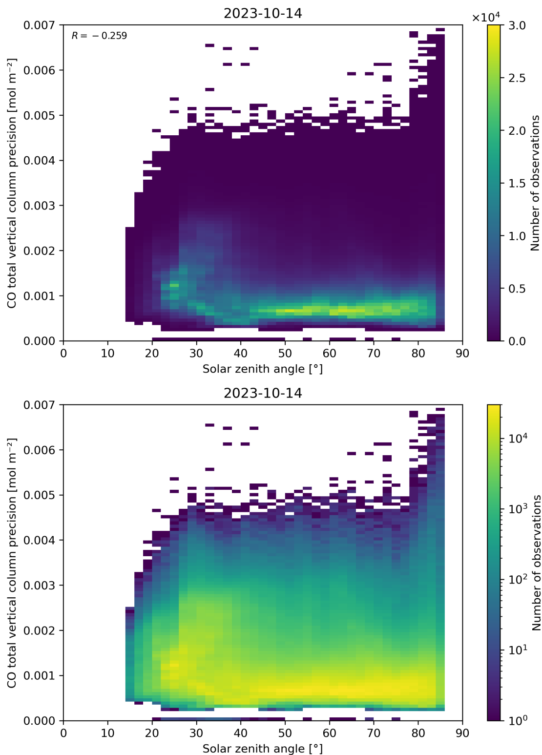
Figure 63: Scatter density plot of “Solar zenith angle” against “CO total vertical column precision” for 2023-10-13 to 2023-10-15.
