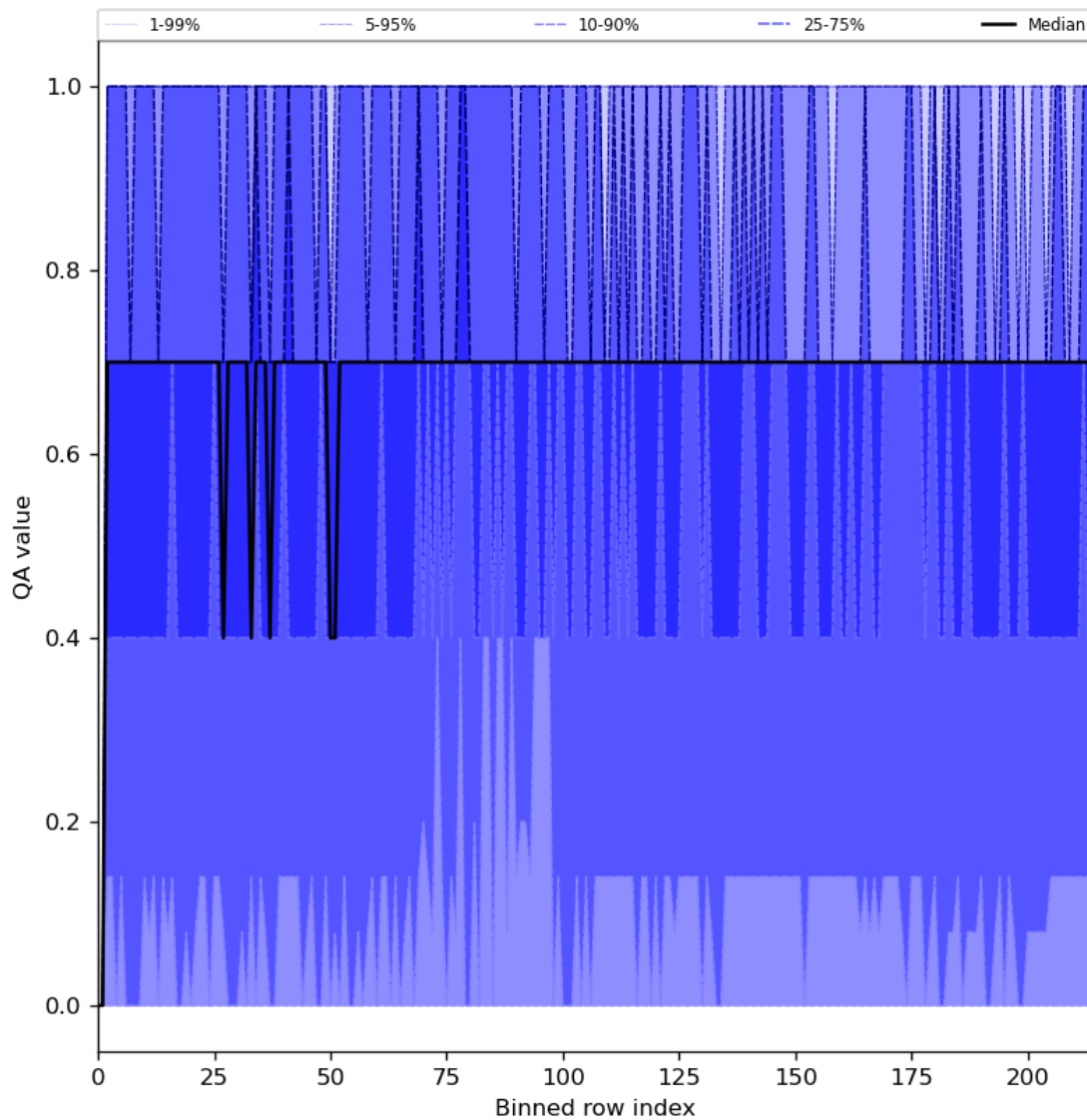
Figure 25: Along track statistics of “QA value” for 2023-10-13 to 2023-10-15
