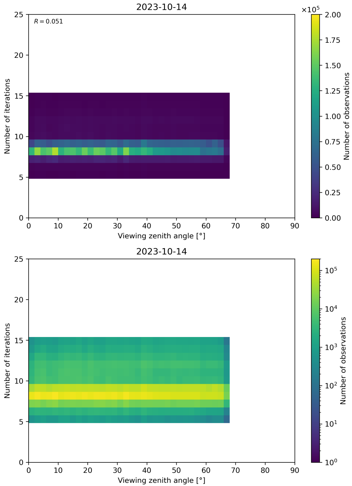
Figure 75: Scatter density plot of “Viewing zenith angle” against “Number of iterations” for 2023-10-13 to 2023-10-15.
