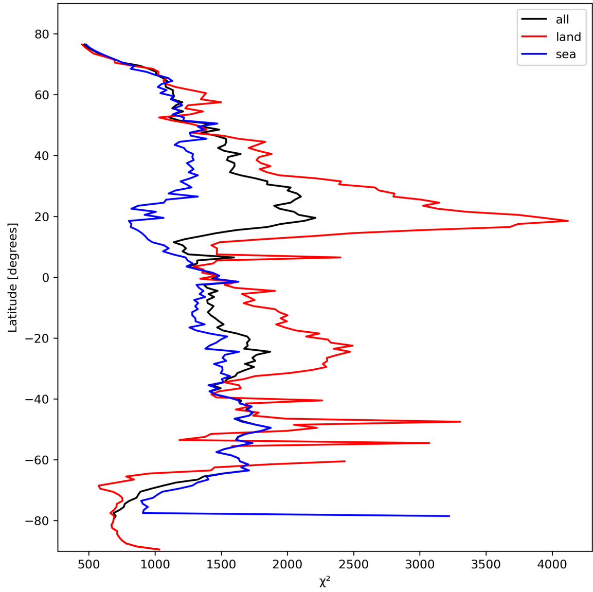
Figure 14: Zonal average of “ \chi^2 ” for 2023-10-13 to 2023-10-15.
