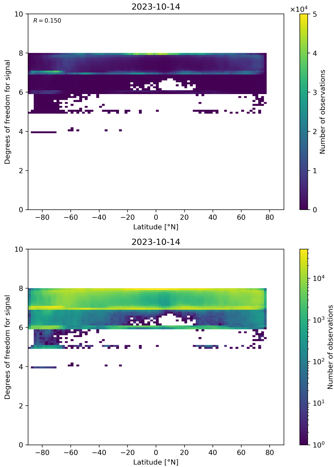
Figure 55: Scatter density plot of “Latitude” against “Degrees of freedom for signal” for 2023-10-13 to 2023-10-15.
