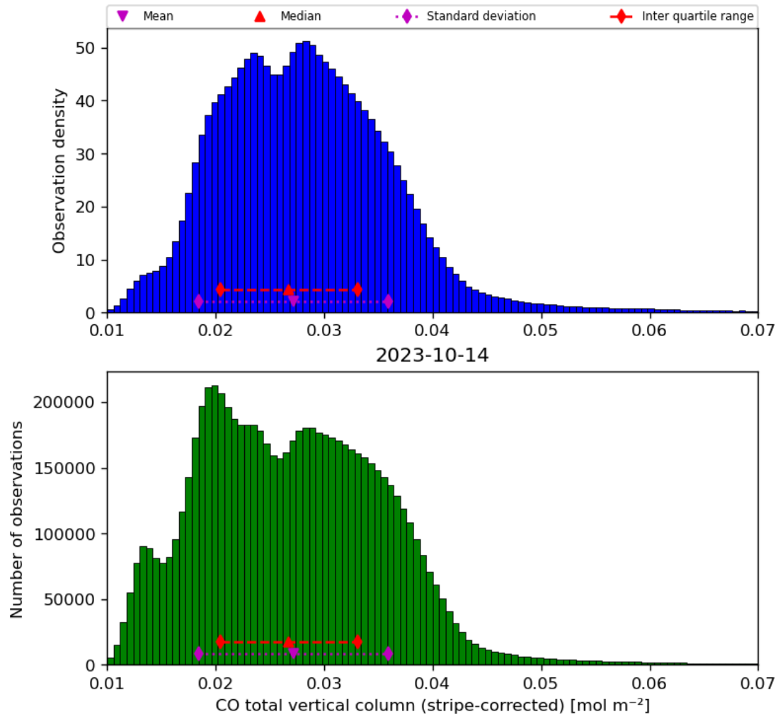
Figure 19: Histogram of “CO total vertical column (stripe-corrected)” for 2023-10-13 to 2023-10-15
