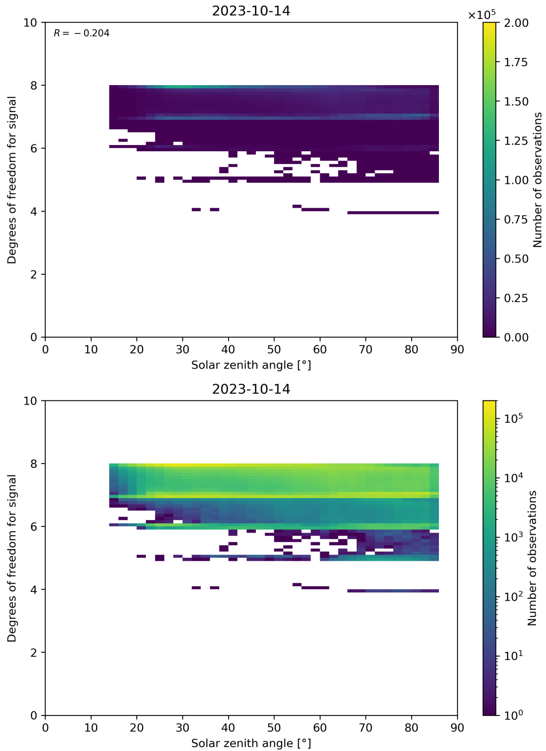
Figure 65: Scatter density plot of “Solar zenith angle” against “Degrees of freedom for signal” for 2023-10-13 to 2023-10-15.
