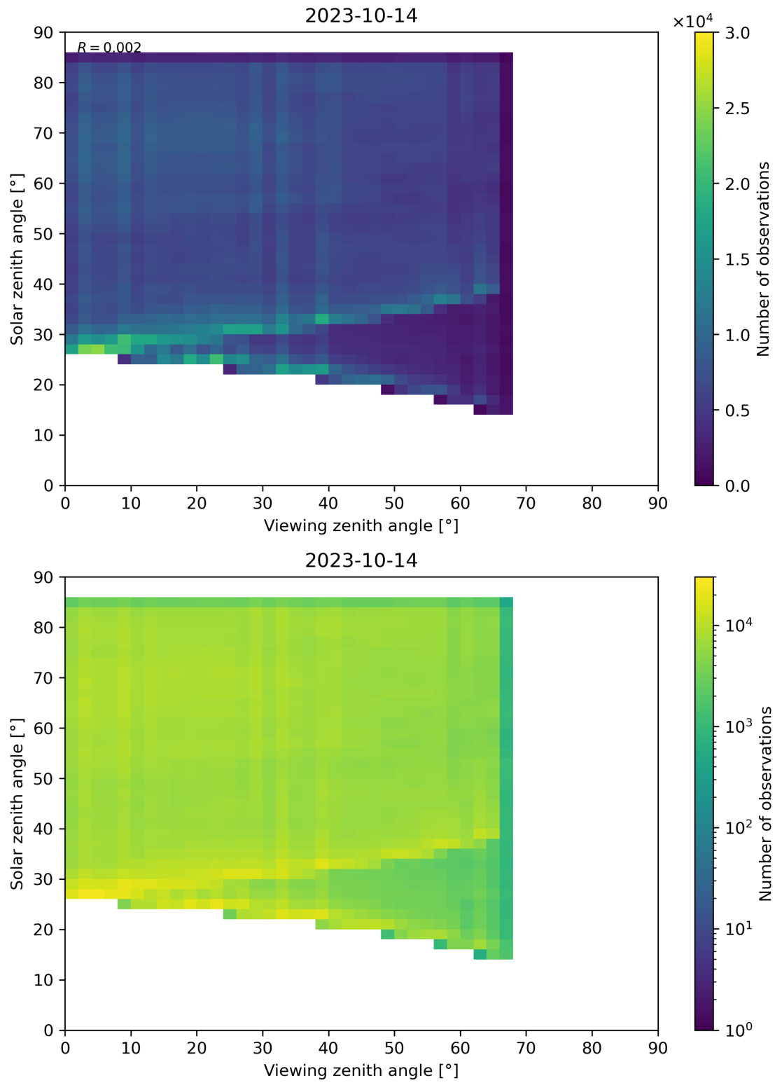
Figure 77: Scatter density plot of “Viewing zenith angle” against “Solar zenith angle” for 2023-10-13 to 2023-10-15.
