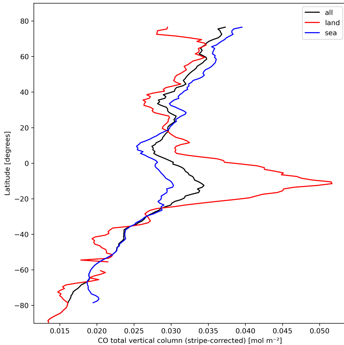
Figure 11: Zonal average of “CO total vertical column (stripe-corrected)” for 2023-10-13 to 2023-10-15.
