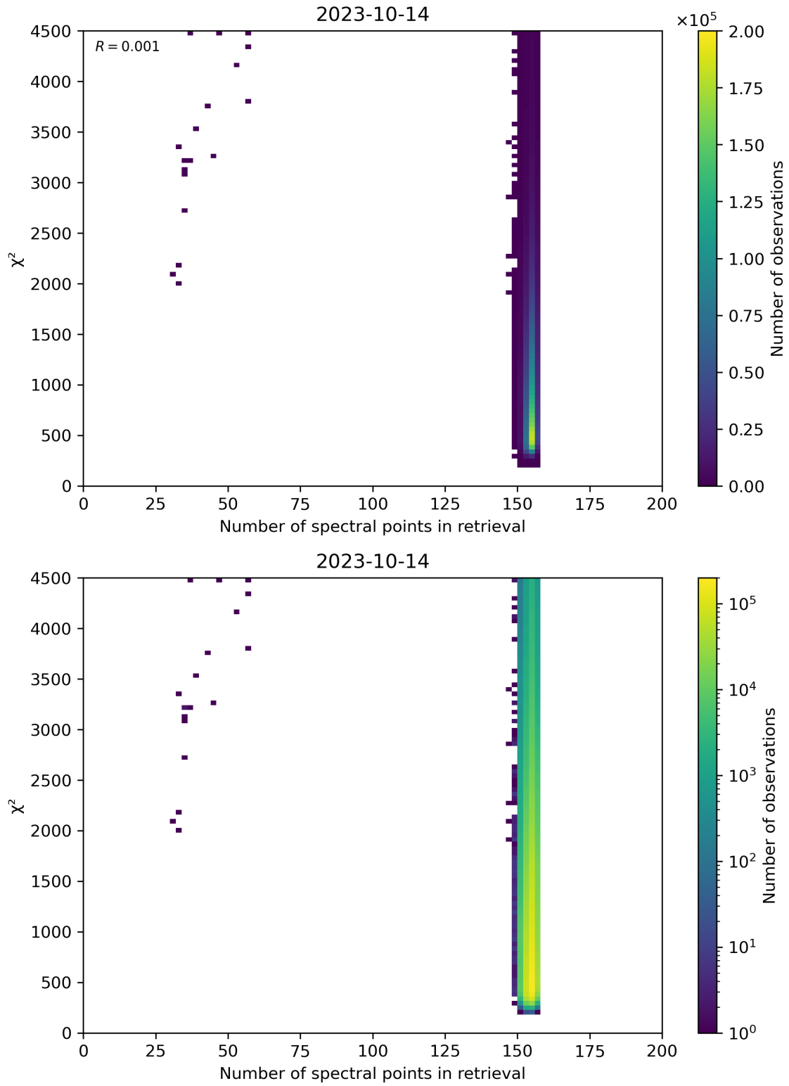
Figure 58: Scatter density plot of “Number of spectral points in retrieval” against “ \chi^2 ” for 2023-10-13 to 2023-10-15.
