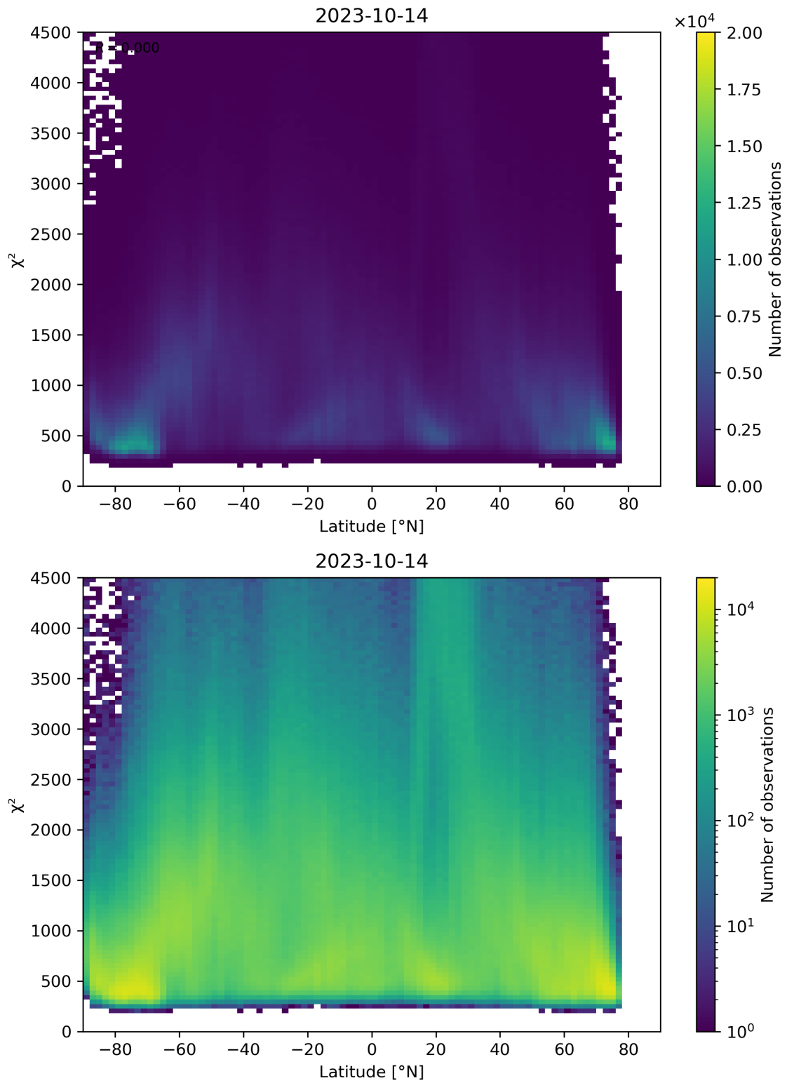
Figure 54: Scatter density plot of “Latitude” against “ \chi^2 ” for 2023-10-13 to 2023-10-15.
