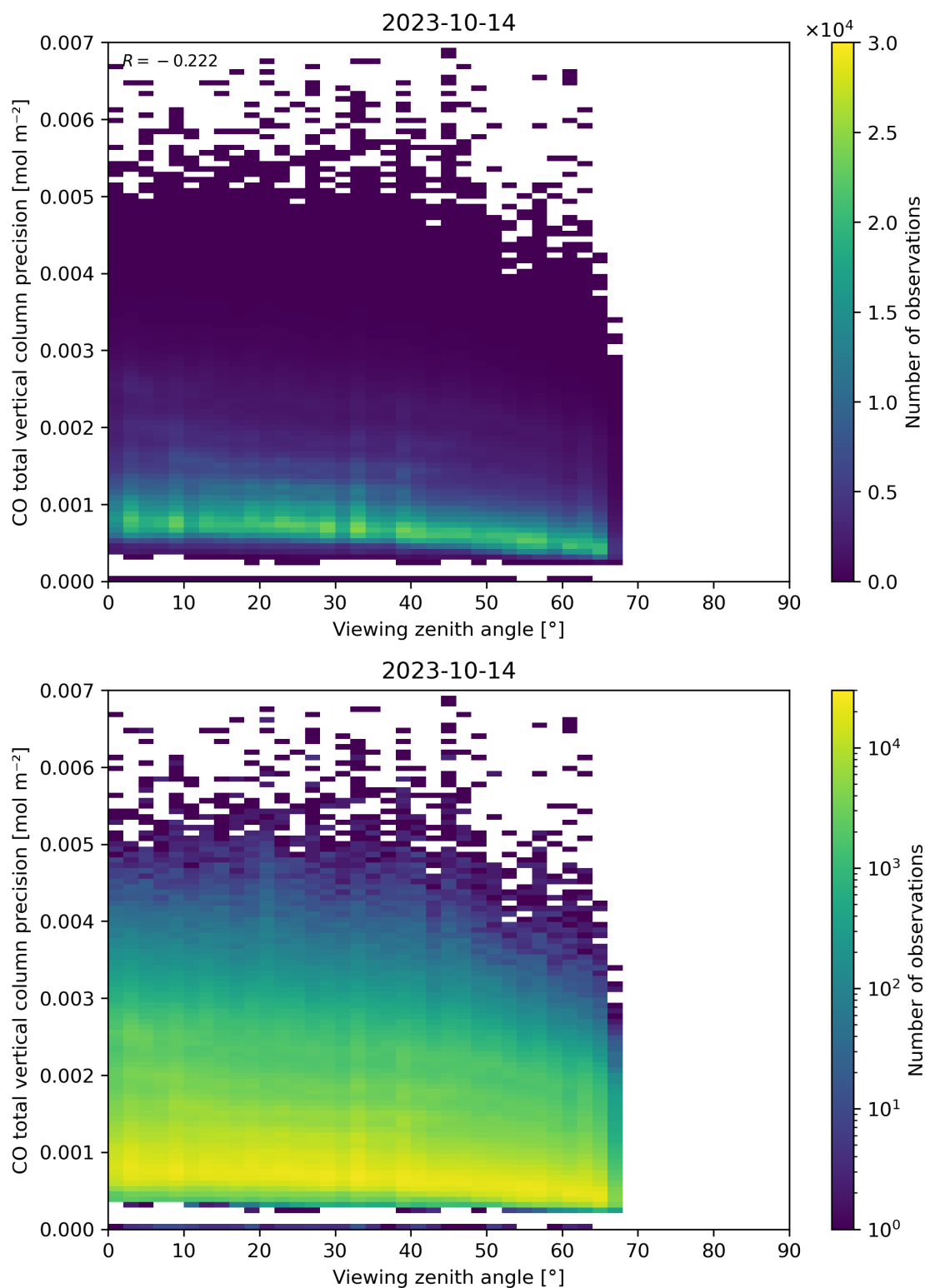
Figure 71: Scatter density plot of “Viewing zenith angle” against “CO total vertical column precision” for 2023-10-13 to 2023-10-15.
