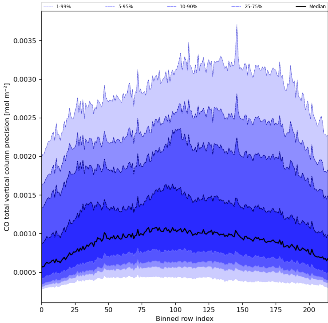
Figure 28: Along track statistics of “CO total vertical column precision” for 2023-10-13 to 2023-10-15
