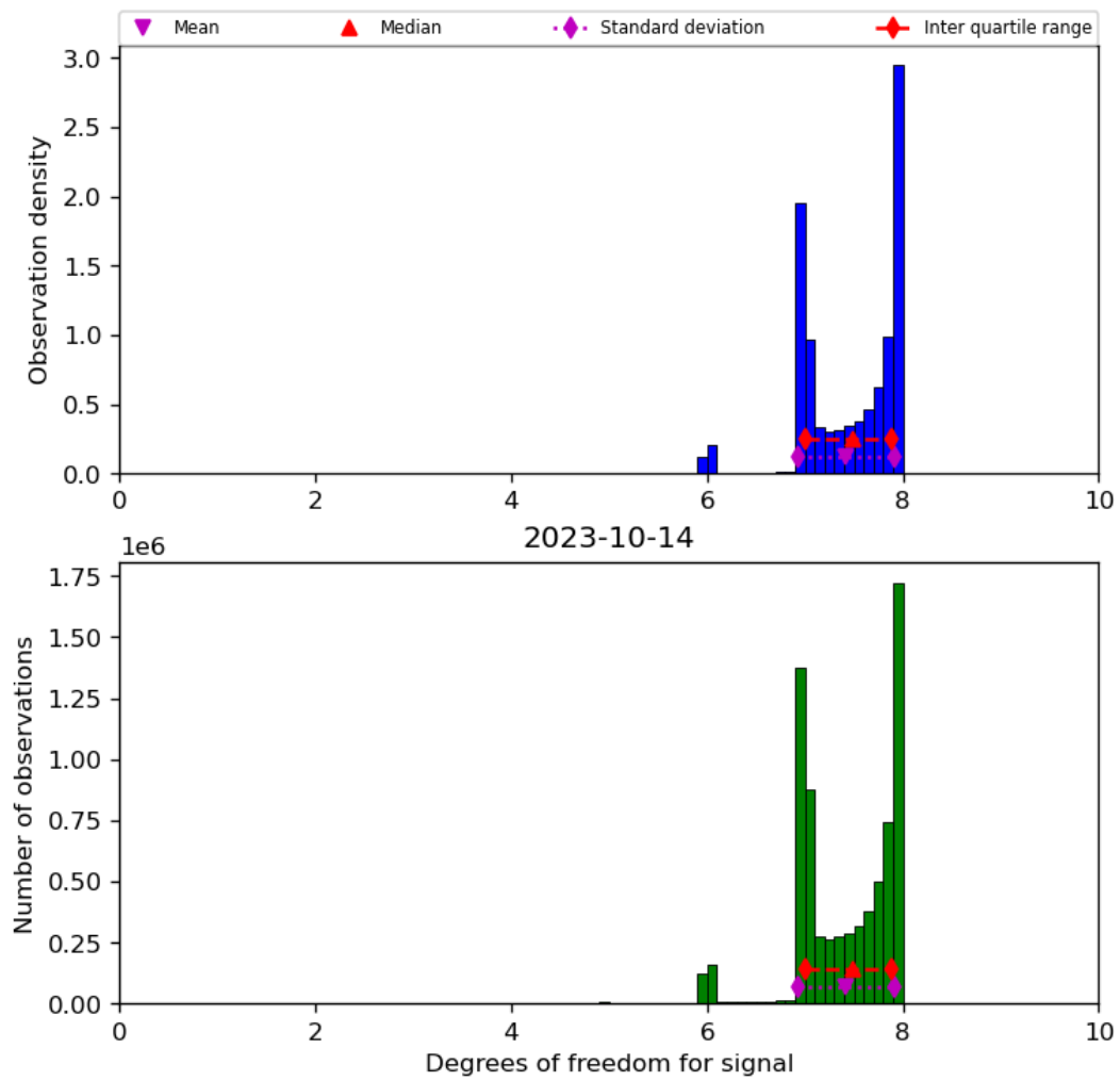
Figure 23: Histogram of “Degrees of freedom for signal” for 2023-10-13 to 2023-10-15
