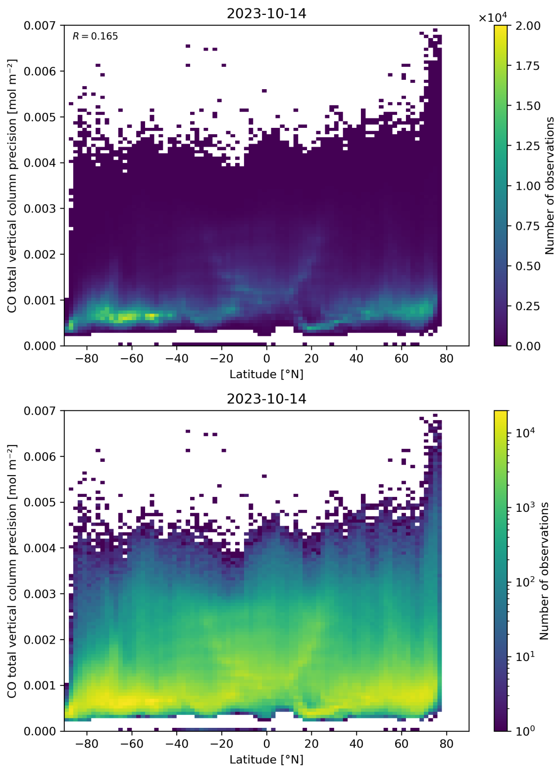
Figure 53: Scatter density plot of “Latitude” against “CO total vertical column precision” for 2023-10-13 to 2023-10-15.
