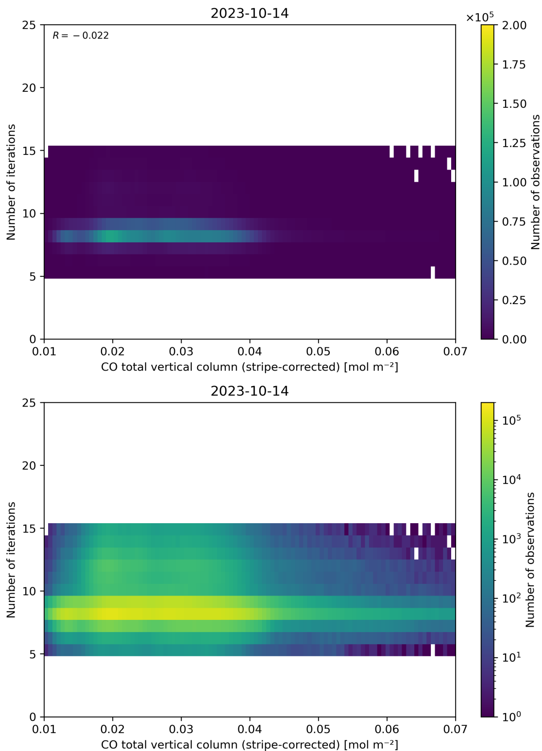
Figure 39: Scatter density plot of “CO total vertical column (stripe-corrected)” against “Number of iterations” for 2023-10-13 to 2023-10-15.
