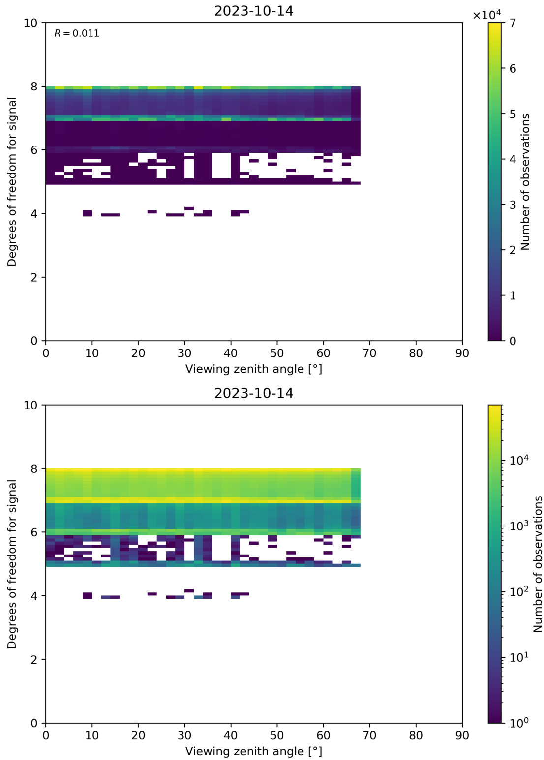
Figure 73: Scatter density plot of “Viewing zenith angle” against “Degrees of freedom for signal” for 2023-10-13 to 2023-10-15.
