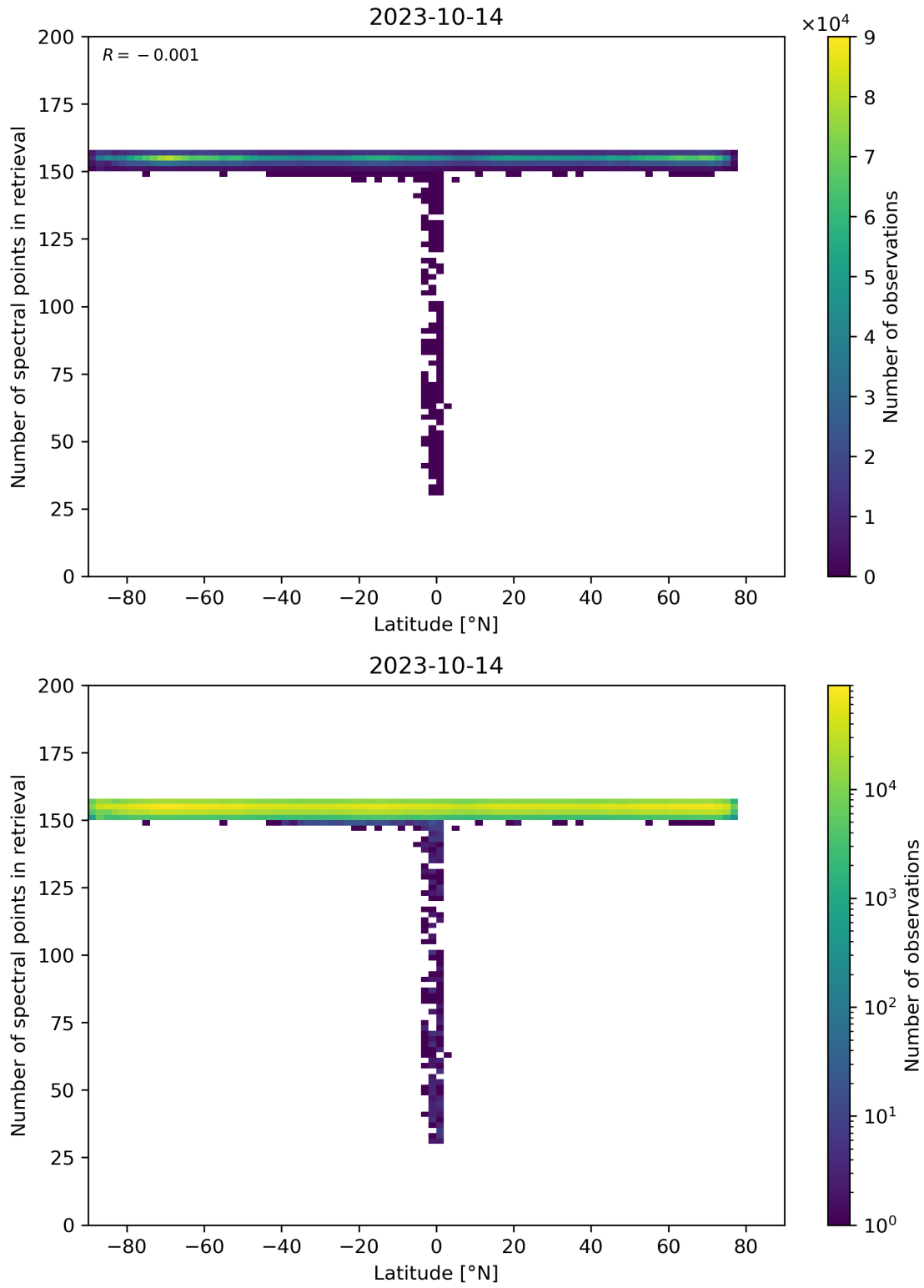
Figure 57: Scatter density plot of “Latitude” against “Number of spectral points in retrieval” for 2023-10-13 to 2023-10-15.
