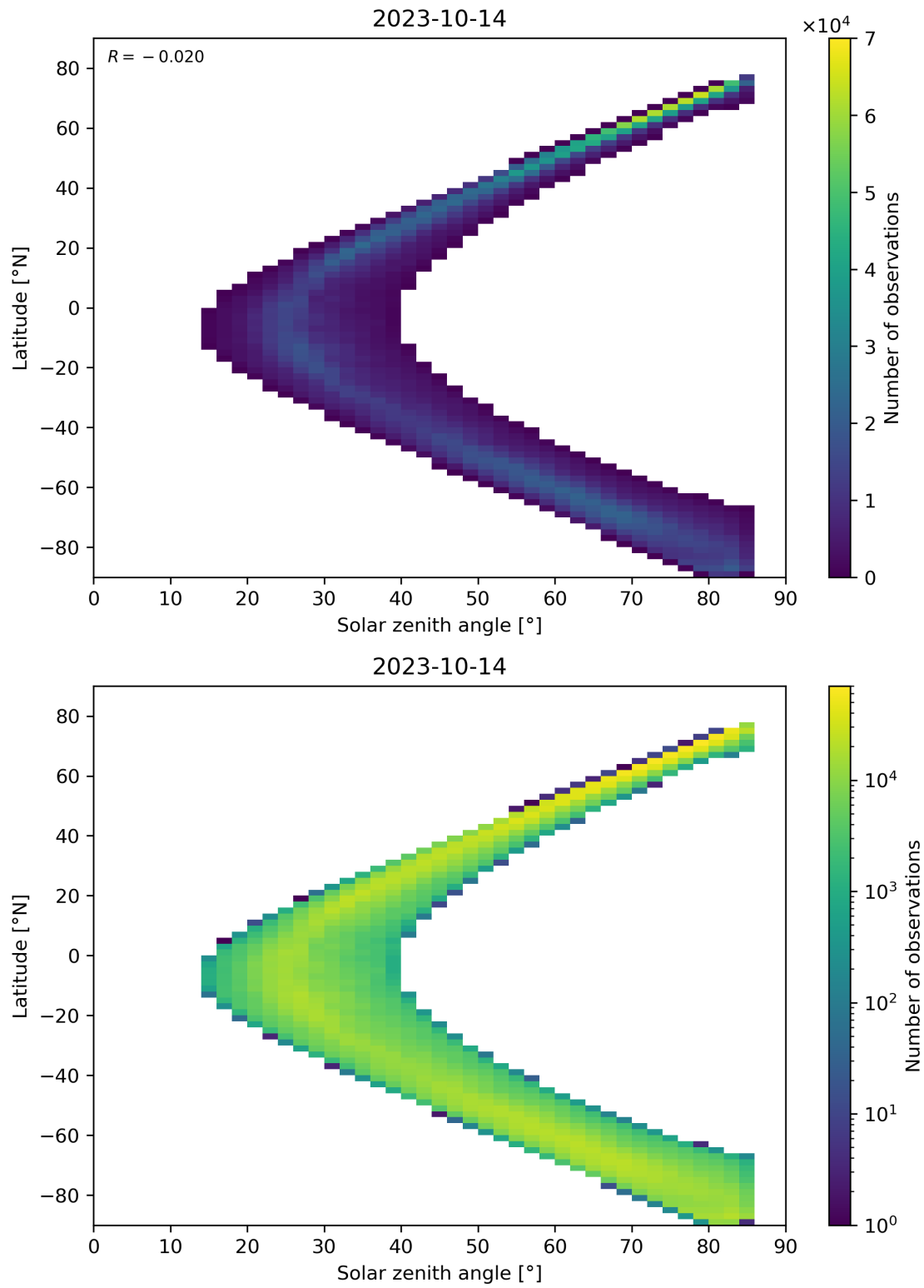
Figure 66: Scatter density plot of “Solar zenith angle” against “Latitude” for 2023-10-13 to 2023-10-15.
