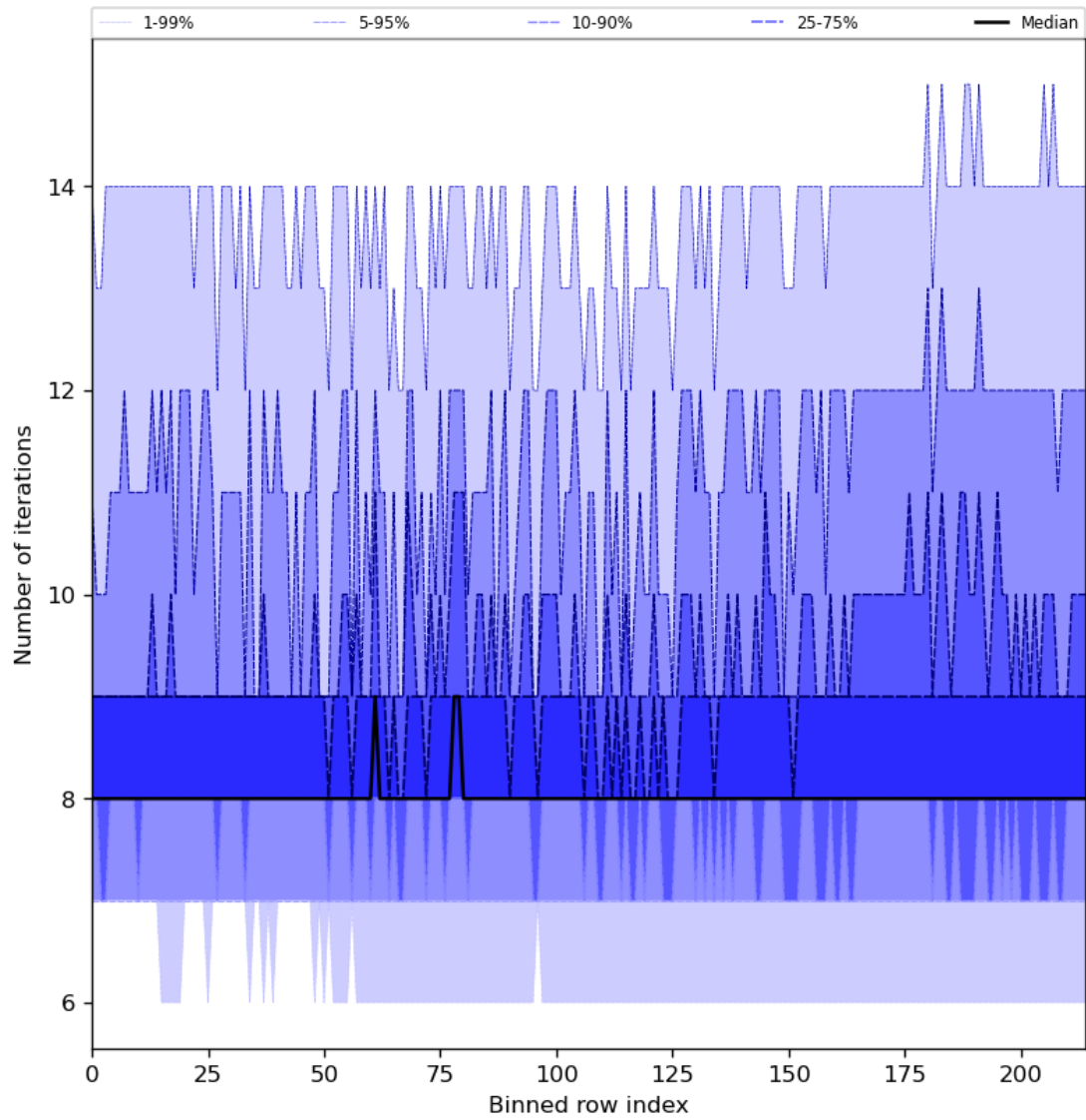
Figure 32: Along track statistics of “Number of iterations” for 2023-10-13 to 2023-10-15
