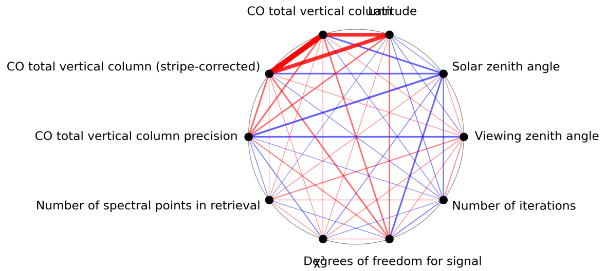
Figure 1: Map of correlation graph for 2023-10-13 to 2023-10-15.
