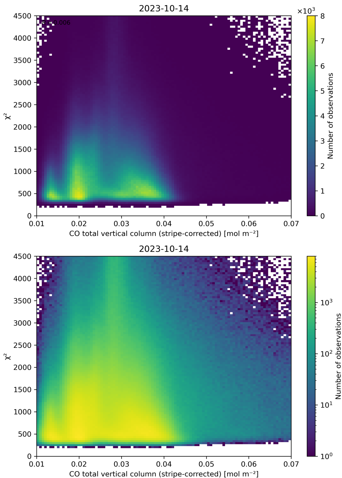
Figure 37: Scatter density plot of “CO total vertical column (stripe-corrected)” against “ \chi^2 ” for 2023-10-13 to 2023-10-15.
