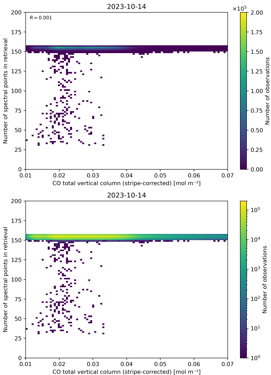
Figure 40: Scatter density plot of “CO total vertical column (stripe-corrected)” against “Number of spectral points in retrieval” for 2023-10-13 to 2023-10-15.
