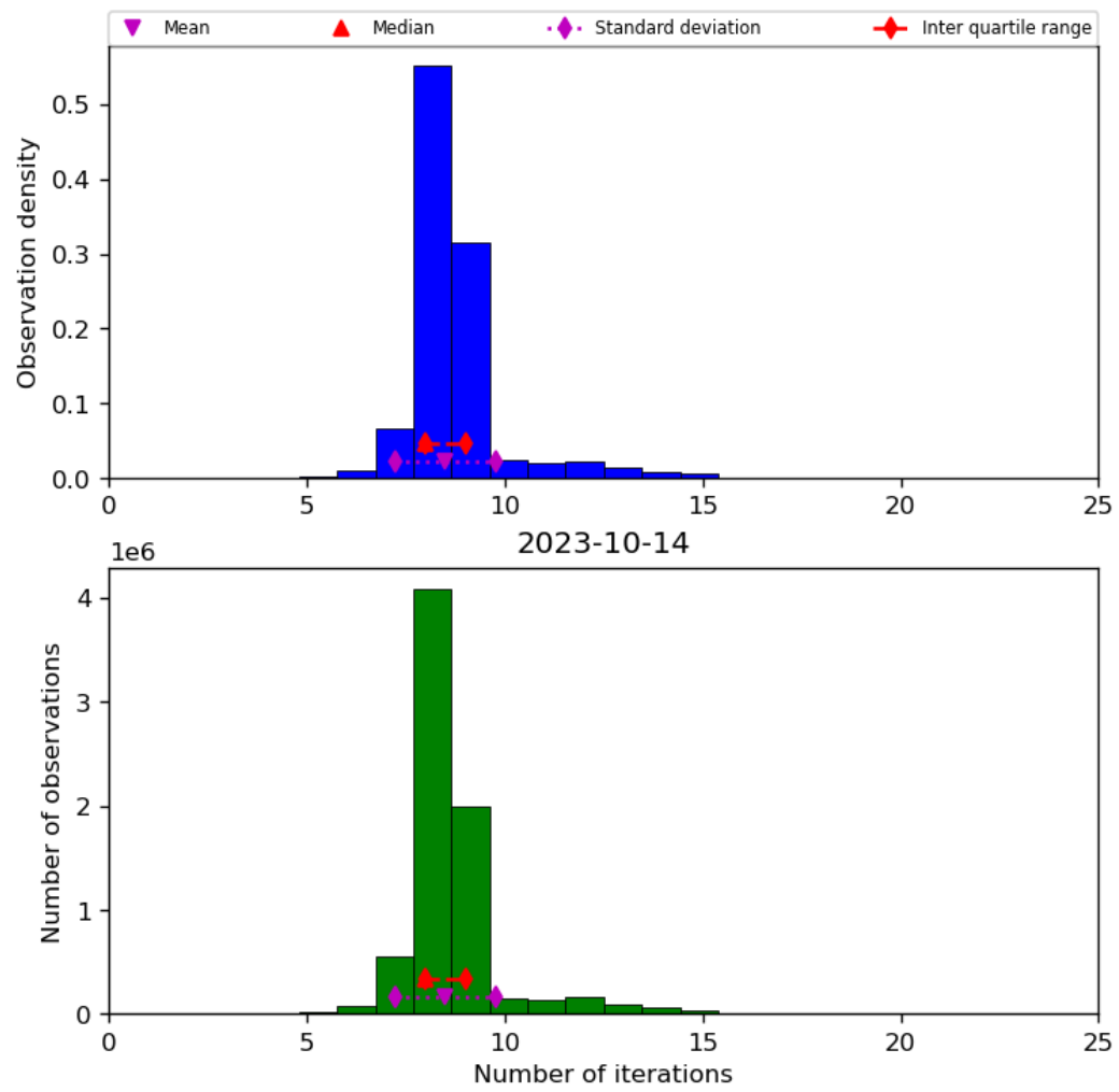
Figure 24: Histogram of “Number of iterations” for 2023-10-13 to 2023-10-15
