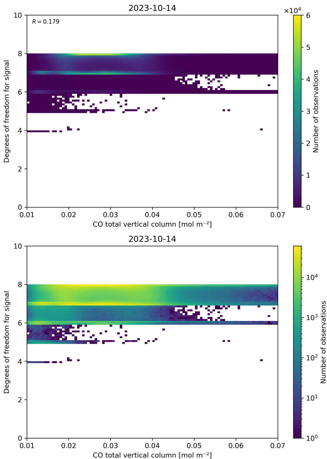
Figure 41: Scatter density plot of “CO total vertical column” against “Degrees of freedom for signal” for 2023-10-13 to 2023-10-15.
