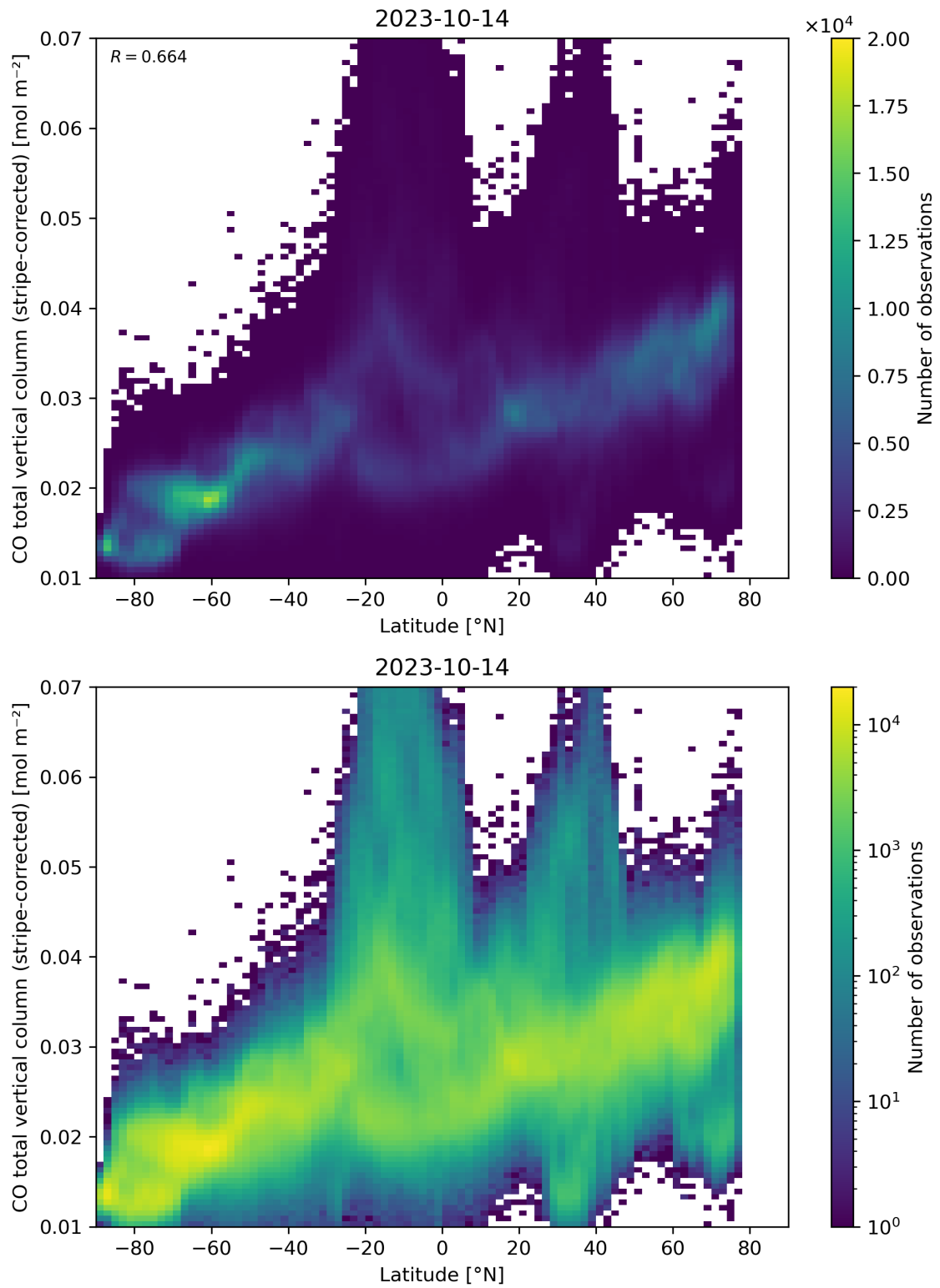
Figure 52: Scatter density plot of “Latitude” against “CO total vertical column (stripe-corrected)” for 2023-10-13 to 2023-10-15.
