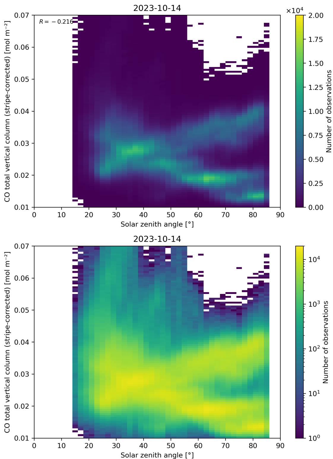
Figure 62: Scatter density plot of “Solar zenith angle” against “CO total vertical column (stripe-corrected)” for 2023-10-13 to 2023-10-15.
