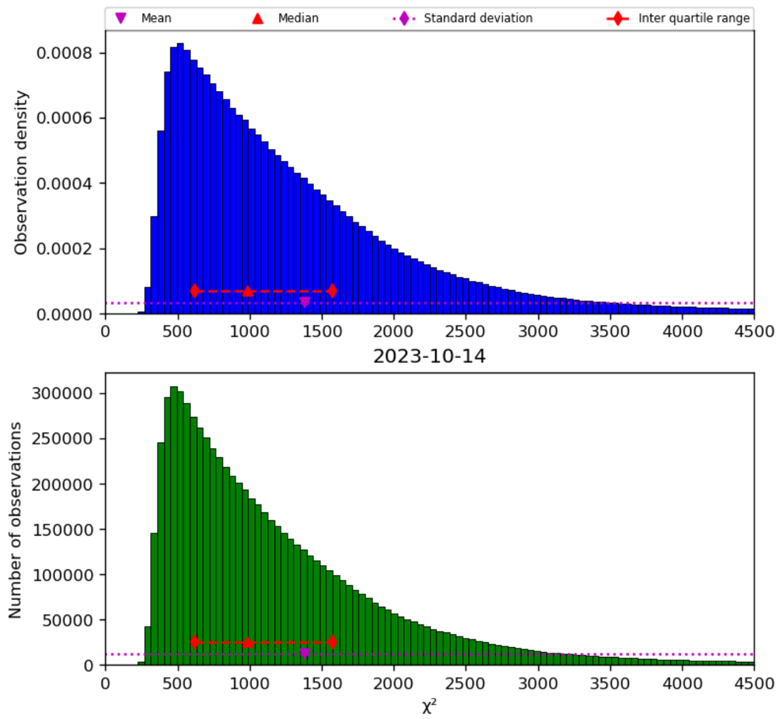
Figure 22: Histogram of “ \chi^2 ” for 2023-10-13 to 2023-10-15
