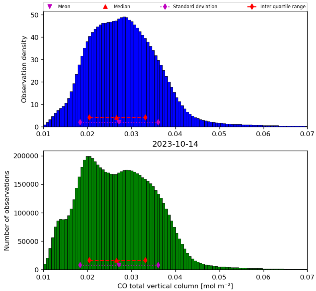
Figure 18: Histogram of “CO total vertical column” for 2023-10-13 to 2023-10-15
