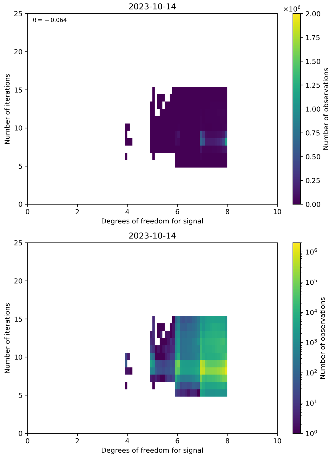
Figure 50: Scatter density plot of “Degrees of freedom for signal” against “Number of iterations” for 2023-10-13 to 2023-10-15.
