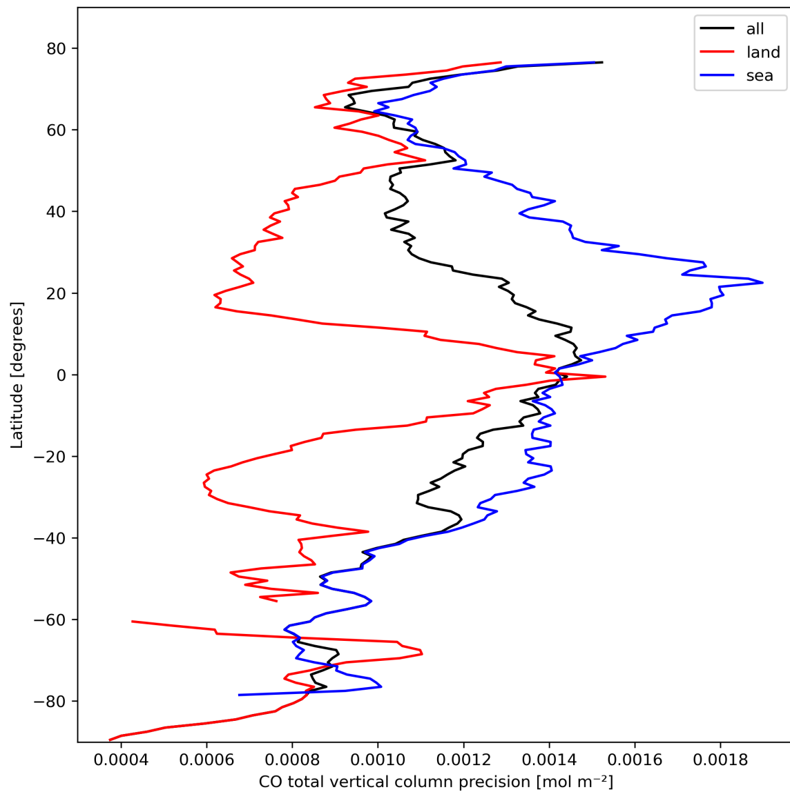
Figure 12: Zonal average of “CO total vertical column precision” for 2023-10-13 to 2023-10-15.
