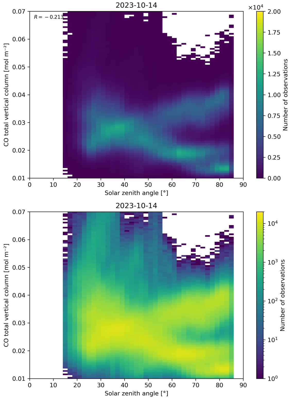
Figure 61: Scatter density plot of “Solar zenith angle” against “CO total vertical column” for 2023-10-13 to 2023-10-15.
