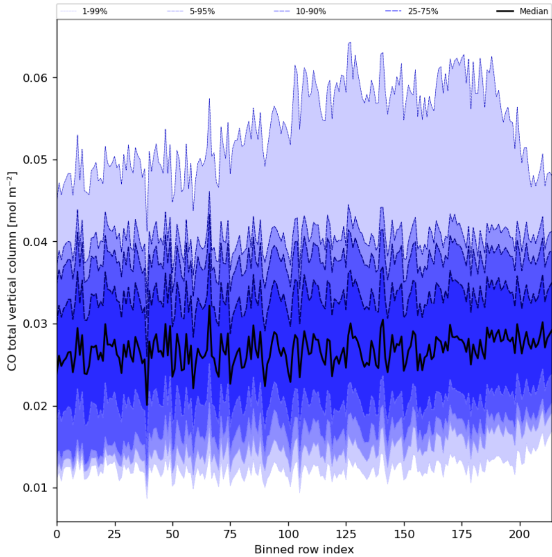
Figure 26: Along track statistics of “CO total vertical column” for 2023-10-13 to 2023-10-15
