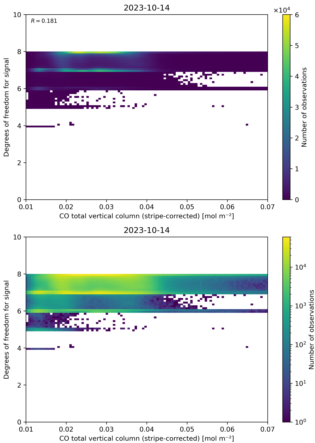
Figure 38: Scatter density plot of “CO total vertical column (stripe-corrected)” against “Degrees of freedom for signal” for 2023-10-13 to 2023-10-15.
