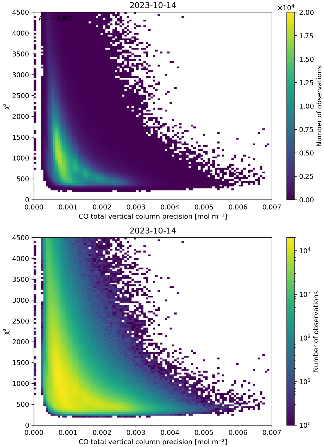
Figure 44: Scatter density plot of “CO total vertical column precision” against “ \chi^2 ” for 2023-10-13 to 2023-10-15.
