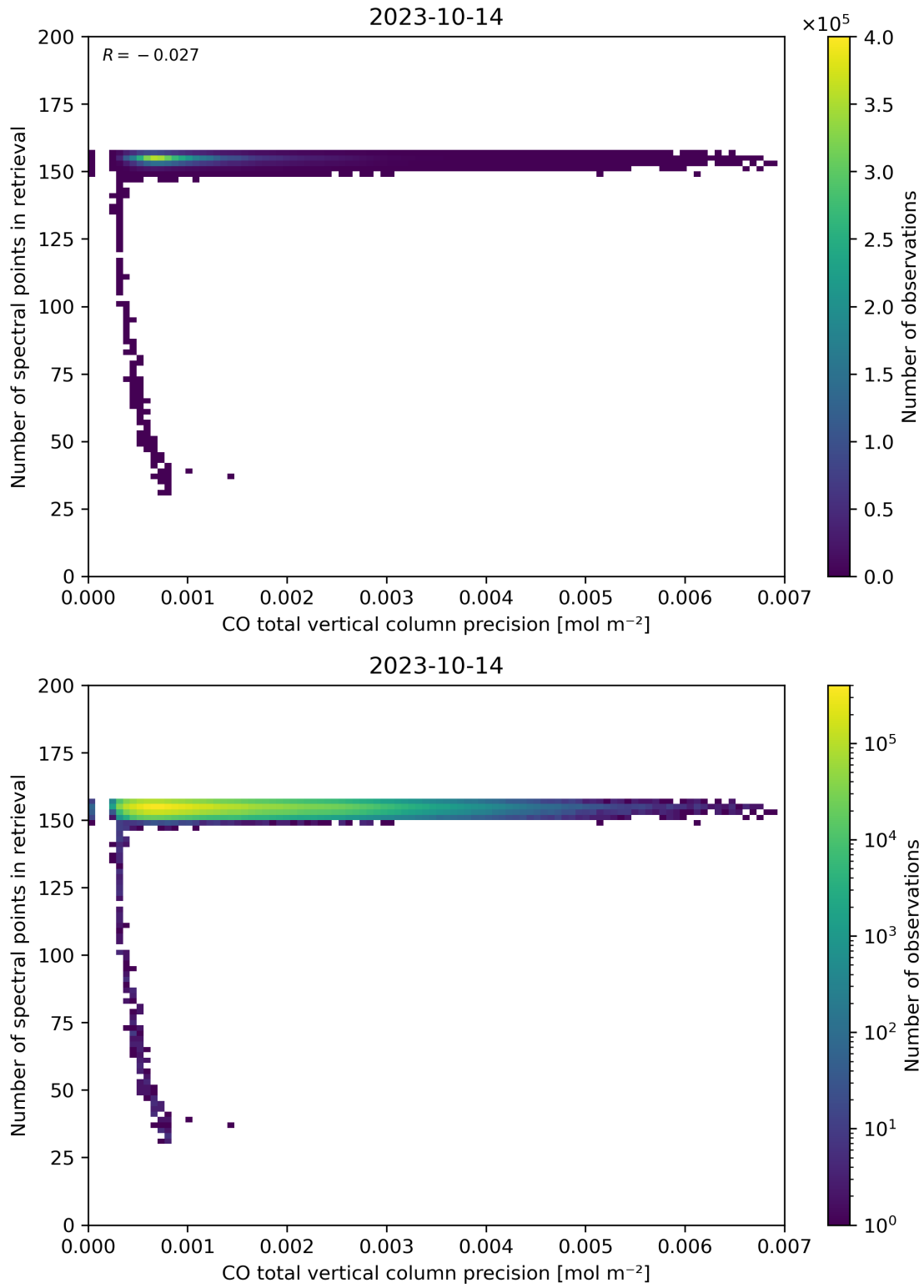
Figure 47: Scatter density plot of “CO total vertical column precision” against “Number of spectral points in retrieval” for 2023-10-13 to 2023-10-15.
