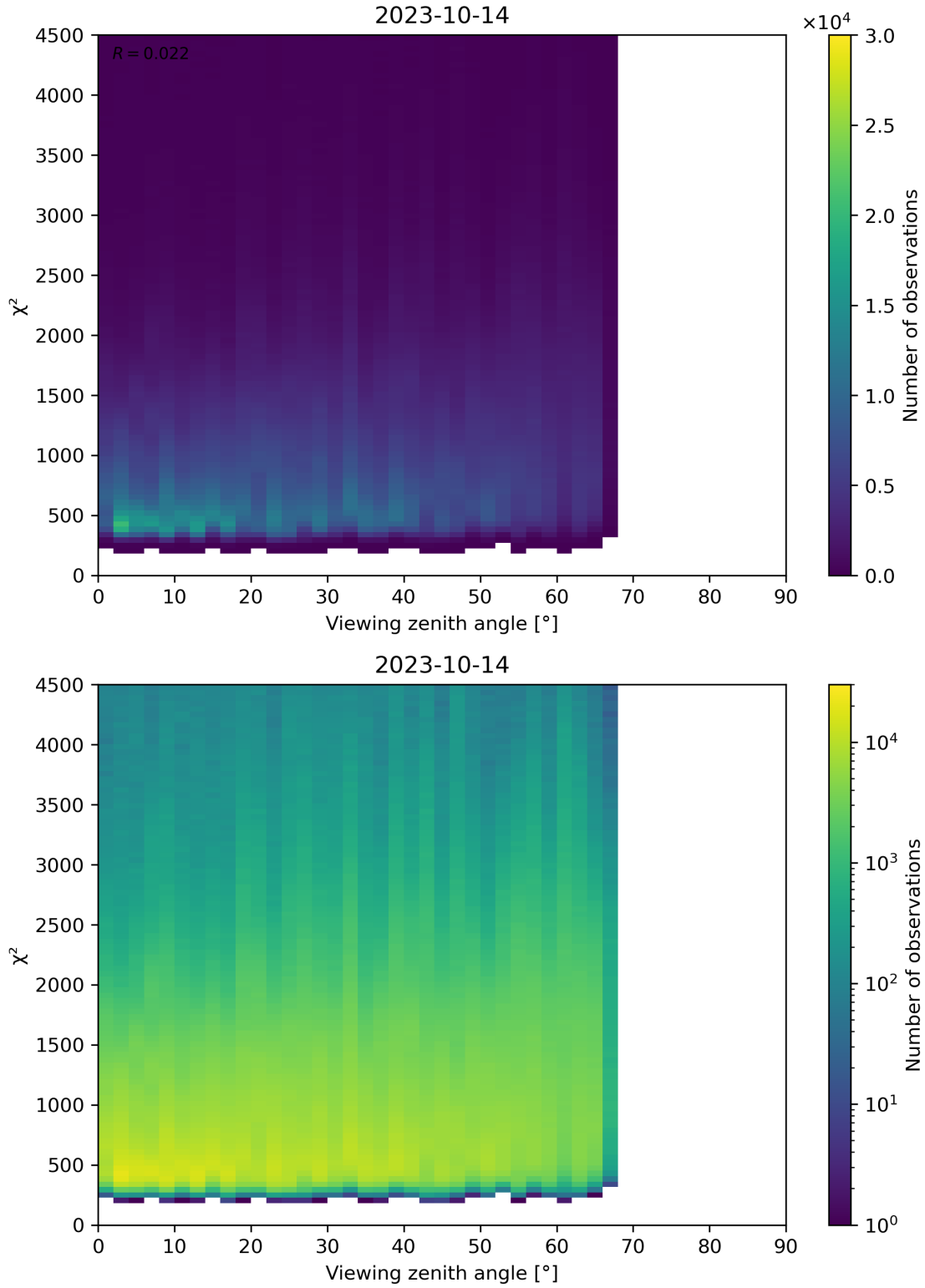
Figure 72: Scatter density plot of “Viewing zenith angle” against “ \chi^2 ” for 2023-10-13 to 2023-10-15.
