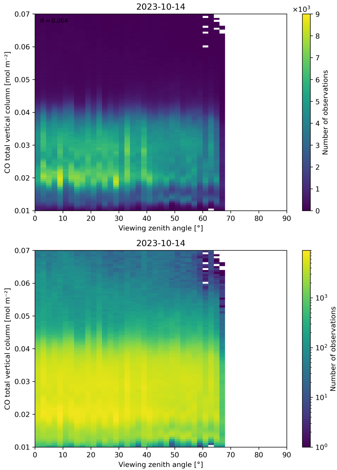
Figure 69: Scatter density plot of “Viewing zenith angle” against “CO total vertical column” for 2023-10-13 to 2023-10-15.
