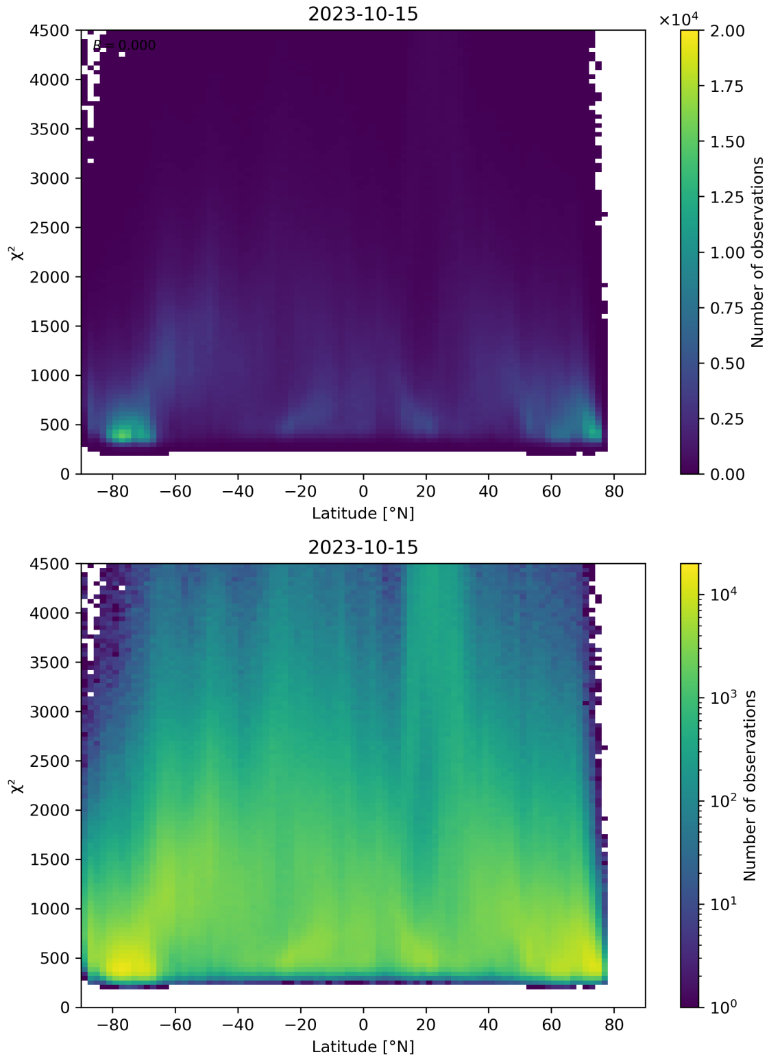
Figure 54: Scatter density plot of “Latitude” against “ \chi^2 ” for 2023-10-14 to 2023-10-16.
