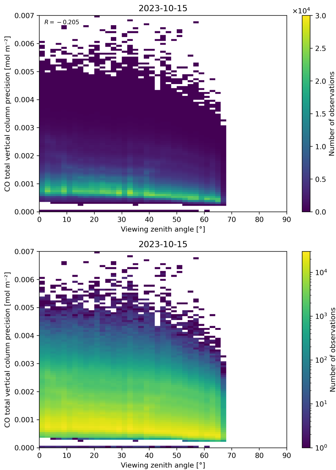
Figure 71: Scatter density plot of “Viewing zenith angle” against “CO total vertical column precision” for 2023-10-14 to 2023-10-16.
