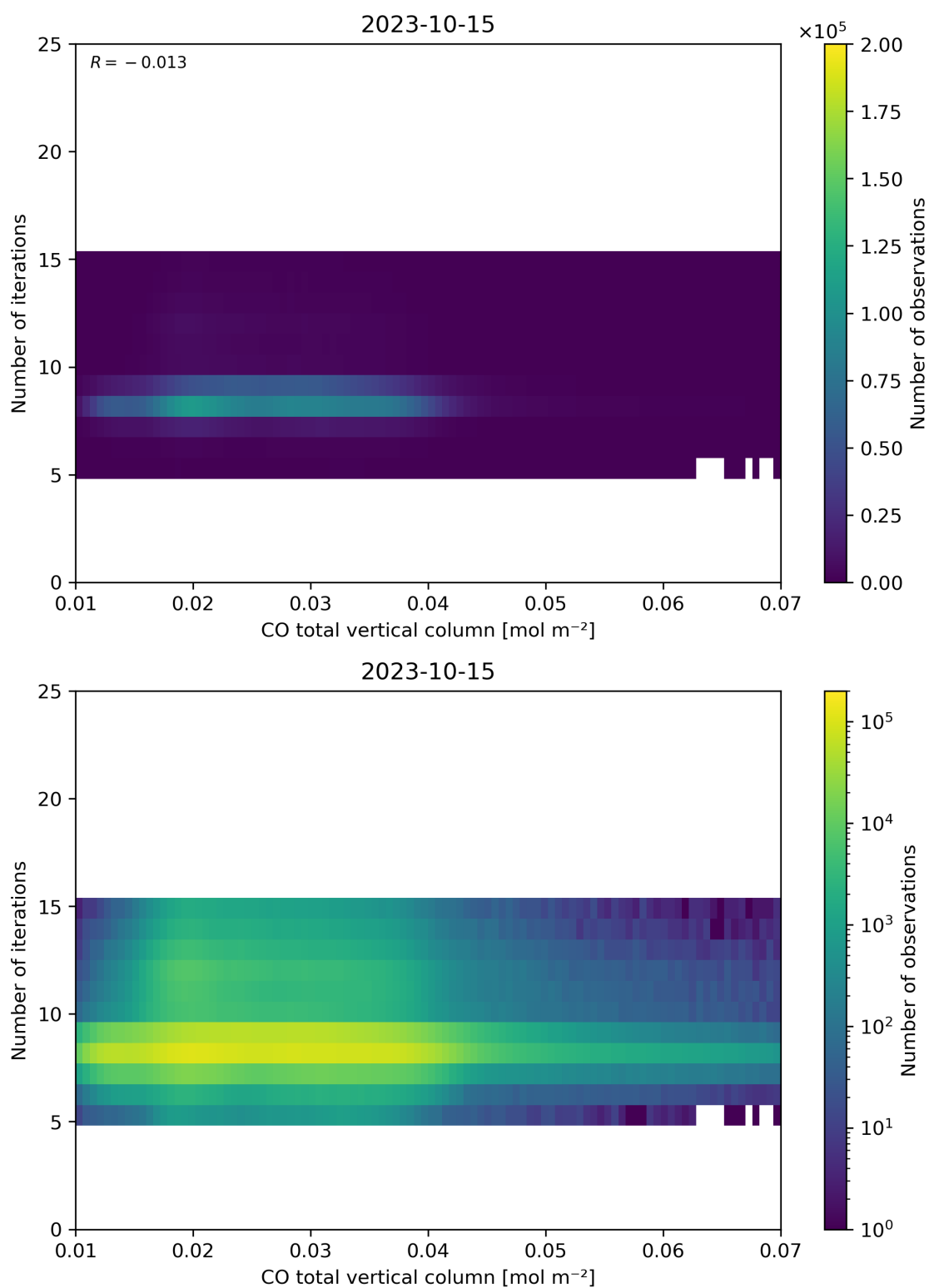
Figure 42: Scatter density plot of “CO total vertical column” against “Number of iterations” for 2023-10-14 to 2023-10-16.
