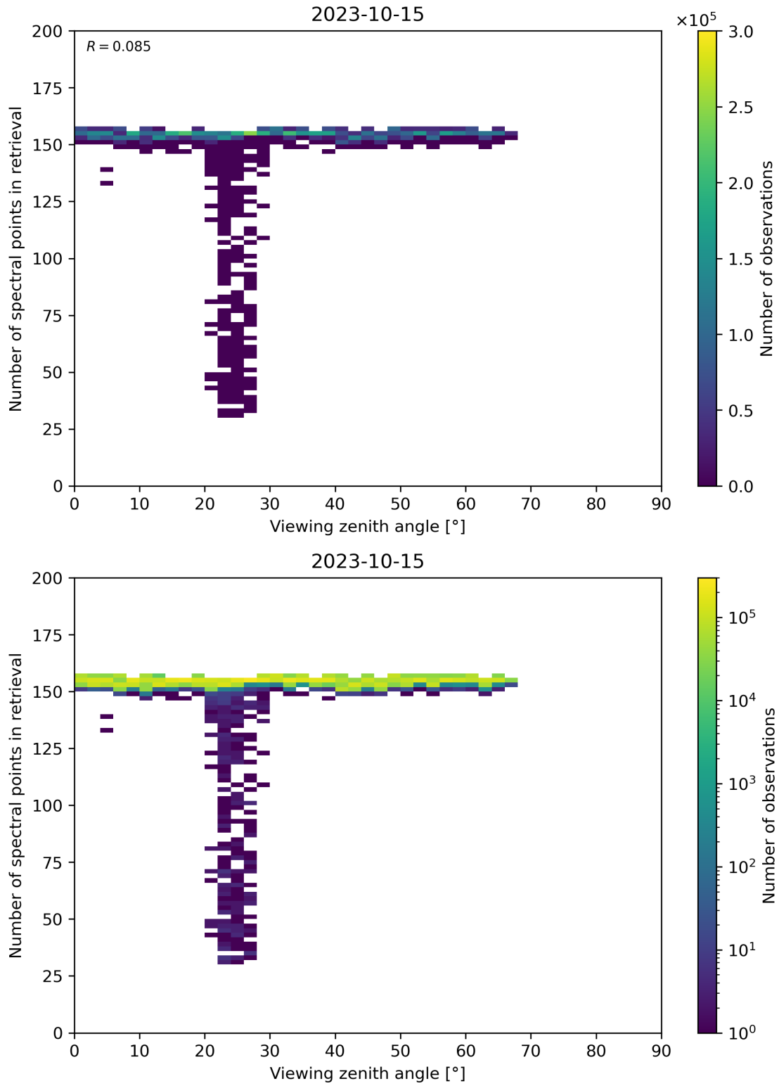
Figure 76: Scatter density plot of “Viewing zenith angle” against “Number of spectral points in retrieval” for 2023-10-14 to 2023-10-16.
