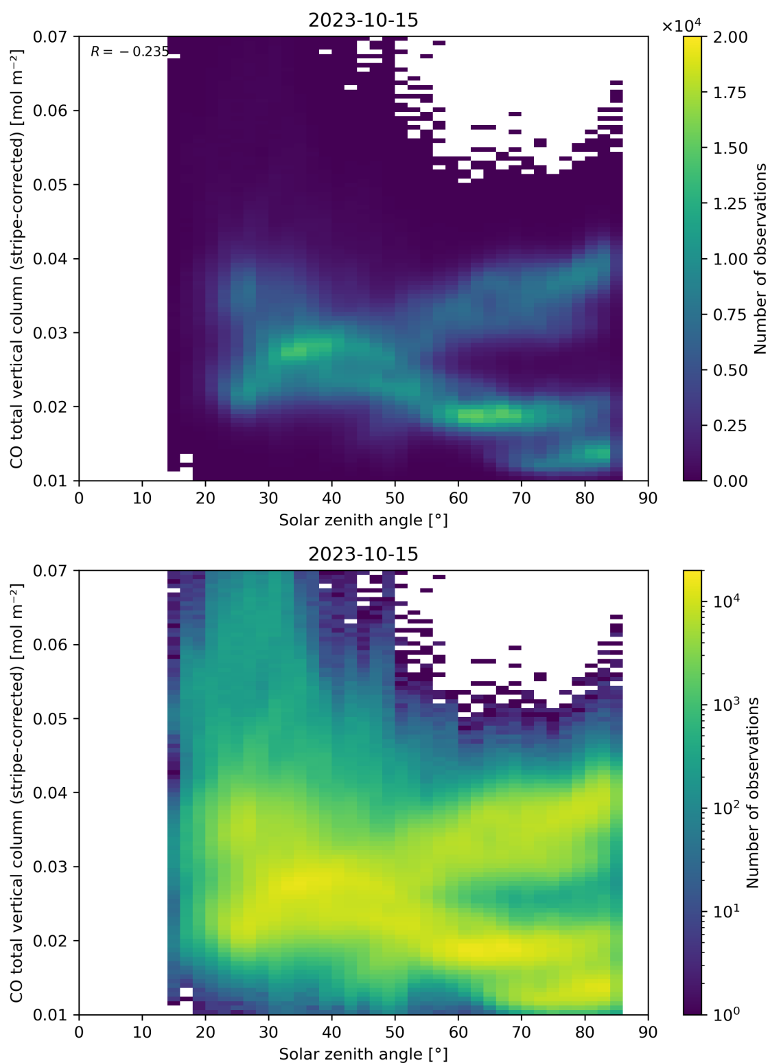
Figure 62: Scatter density plot of “Solar zenith angle” against “CO total vertical column (stripe-corrected)” for 2023-10-14 to 2023-10-16.
