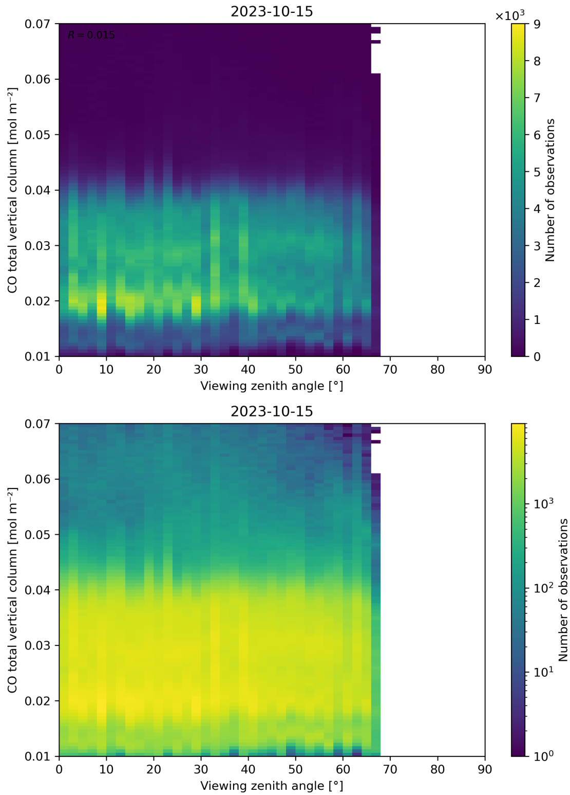
Figure 69: Scatter density plot of “Viewing zenith angle” against “CO total vertical column” for 2023-10-14 to 2023-10-16.
