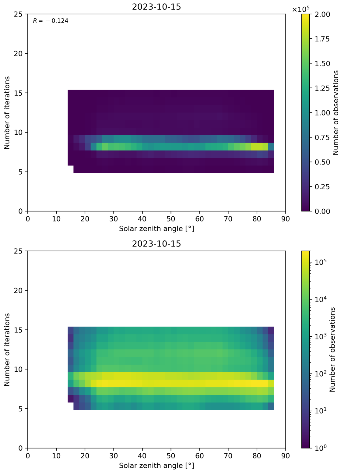
Figure 67: Scatter density plot of “Solar zenith angle” against “Number of iterations” for 2023-10-14 to 2023-10-16.
