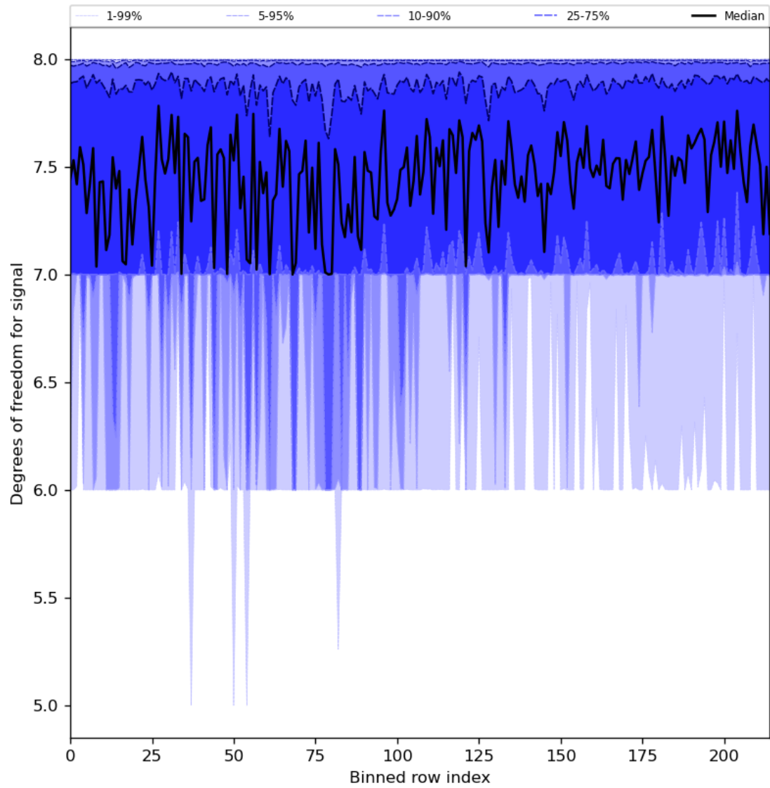
Figure 31: Along track statistics of “Degrees of freedom for signal” for 2023-10-14 to 2023-10-16
