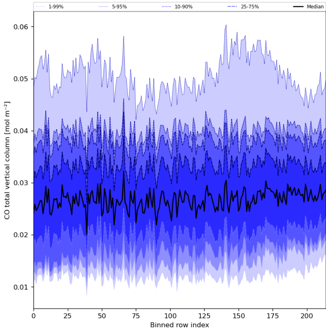
Figure 26: Along track statistics of “CO total vertical column” for 2023-10-14 to 2023-10-16
