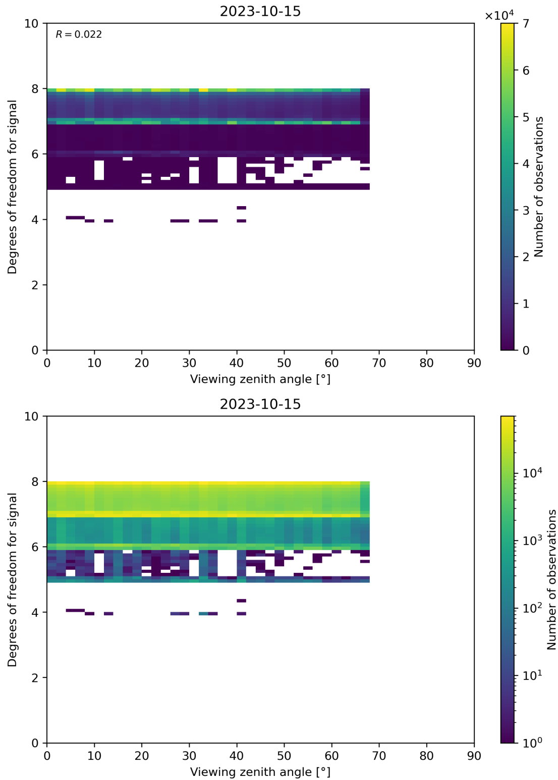
Figure 73: Scatter density plot of “Viewing zenith angle” against “Degrees of freedom for signal” for 2023-10-14 to 2023-10-16.
