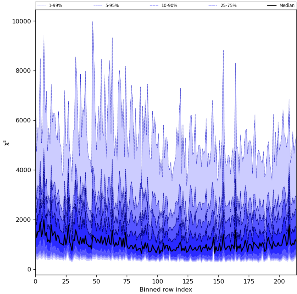
Figure 30: Along track statistics of “ \chi^2 ” for 2023-10-14 to 2023-10-16
