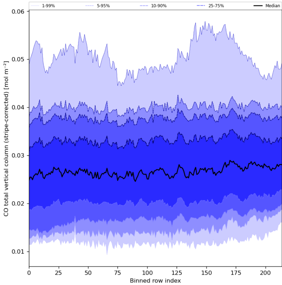
Figure 27: Along track statistics of “CO total vertical column (stripe-corrected)” for 2023-10-14 to 2023-10-16
