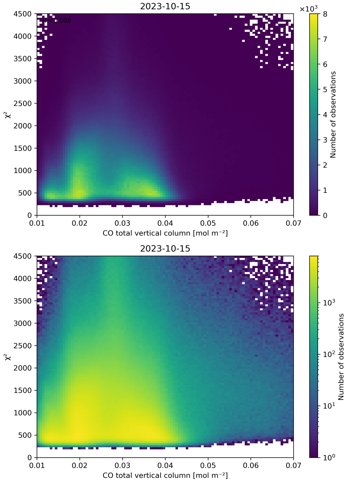
Figure 35: Scatter density plot of “CO total vertical column” against “ \chi^2 ” for 2023-10-14 to 2023-10-16.
