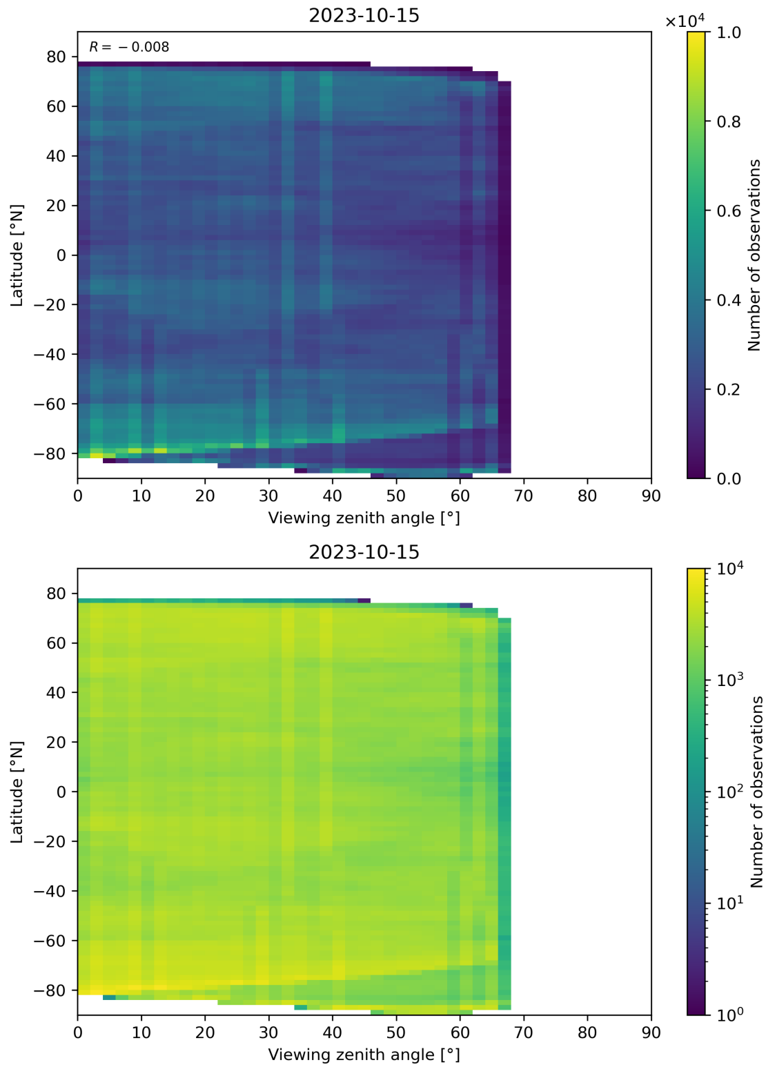
Figure 74: Scatter density plot of “Viewing zenith angle” against “Latitude” for 2023-10-14 to 2023-10-16.
