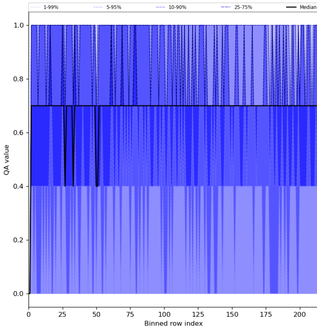
Figure 25: Along track statistics of “QA value” for 2023-10-14 to 2023-10-16
