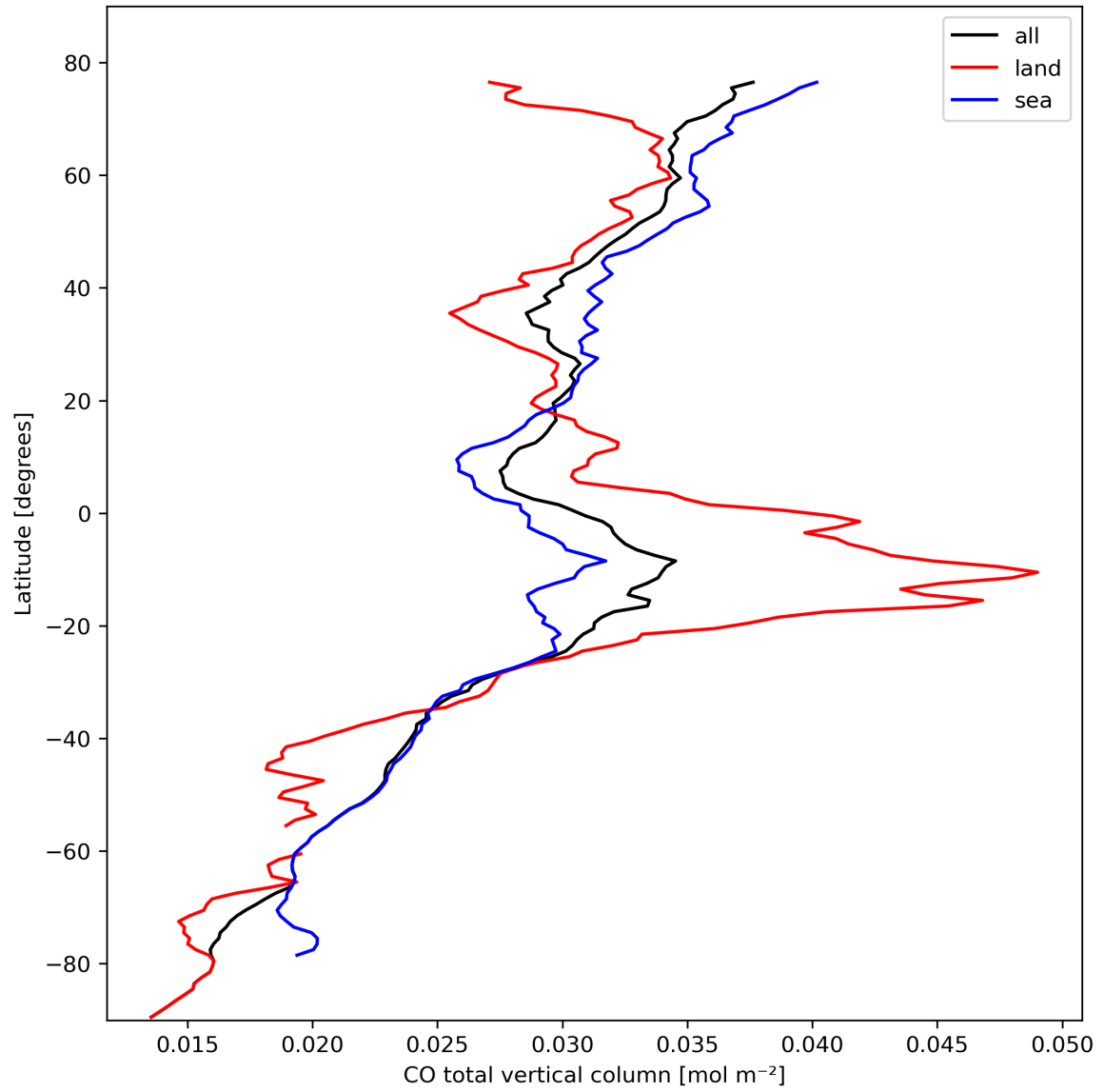
Figure 10: Zonal average of “CO total vertical column” for 2023-10-14 to 2023-10-16.
