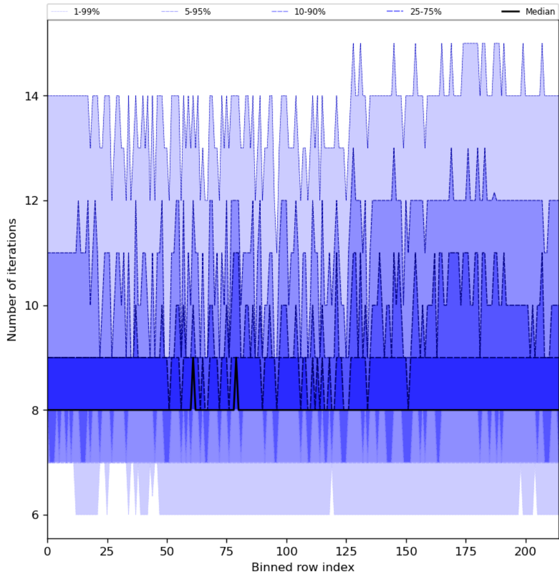
Figure 32: Along track statistics of “Number of iterations” for 2023-10-14 to 2023-10-16
