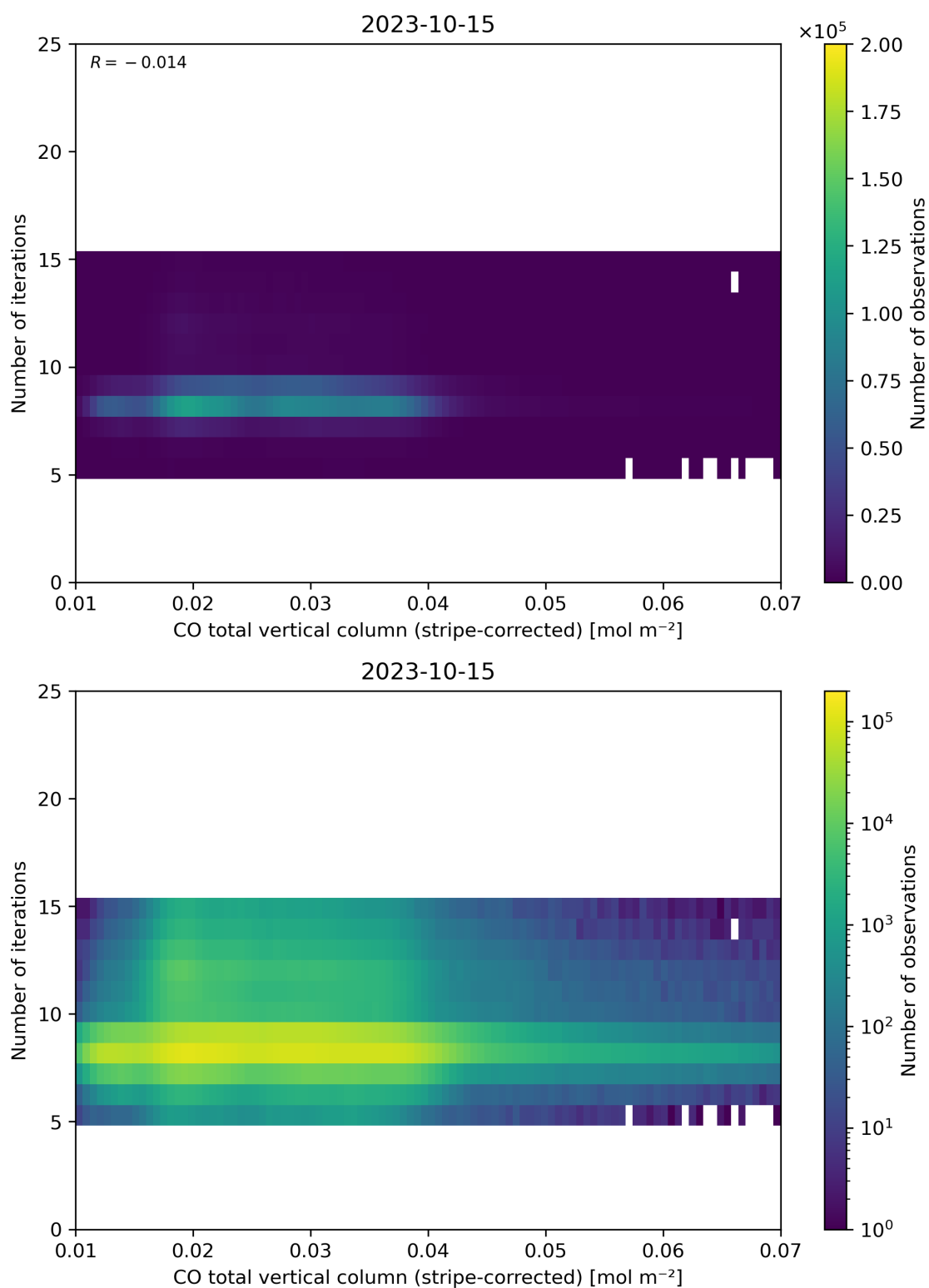
Figure 39: Scatter density plot of “CO total vertical column (stripe-corrected)” against “Number of iterations” for 2023-10-14 to 2023-10-16.
