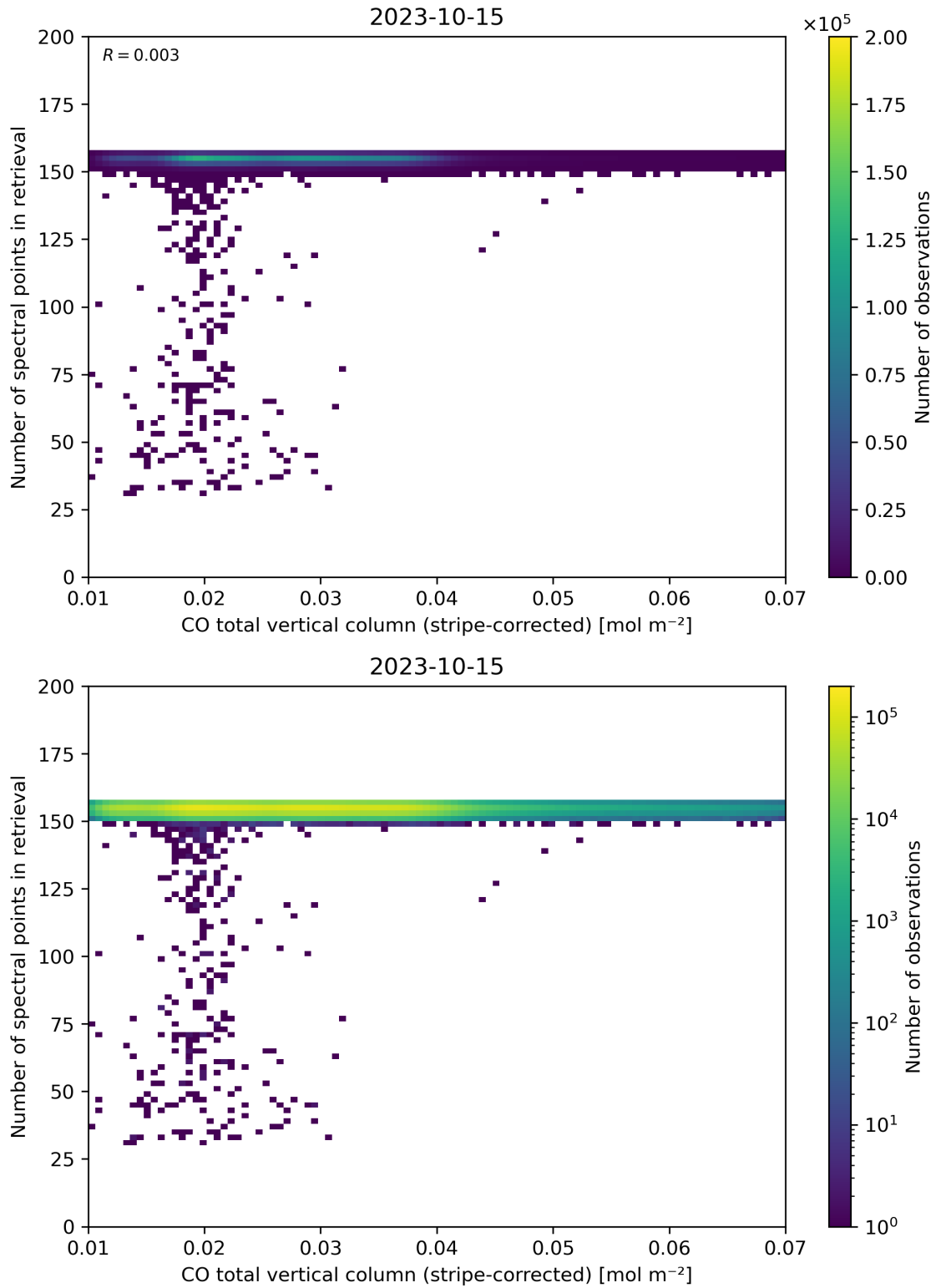
Figure 40: Scatter density plot of “CO total vertical column (stripe-corrected)” against “Number of spectral points in retrieval” for 2023-10-14 to 2023-10-16.
