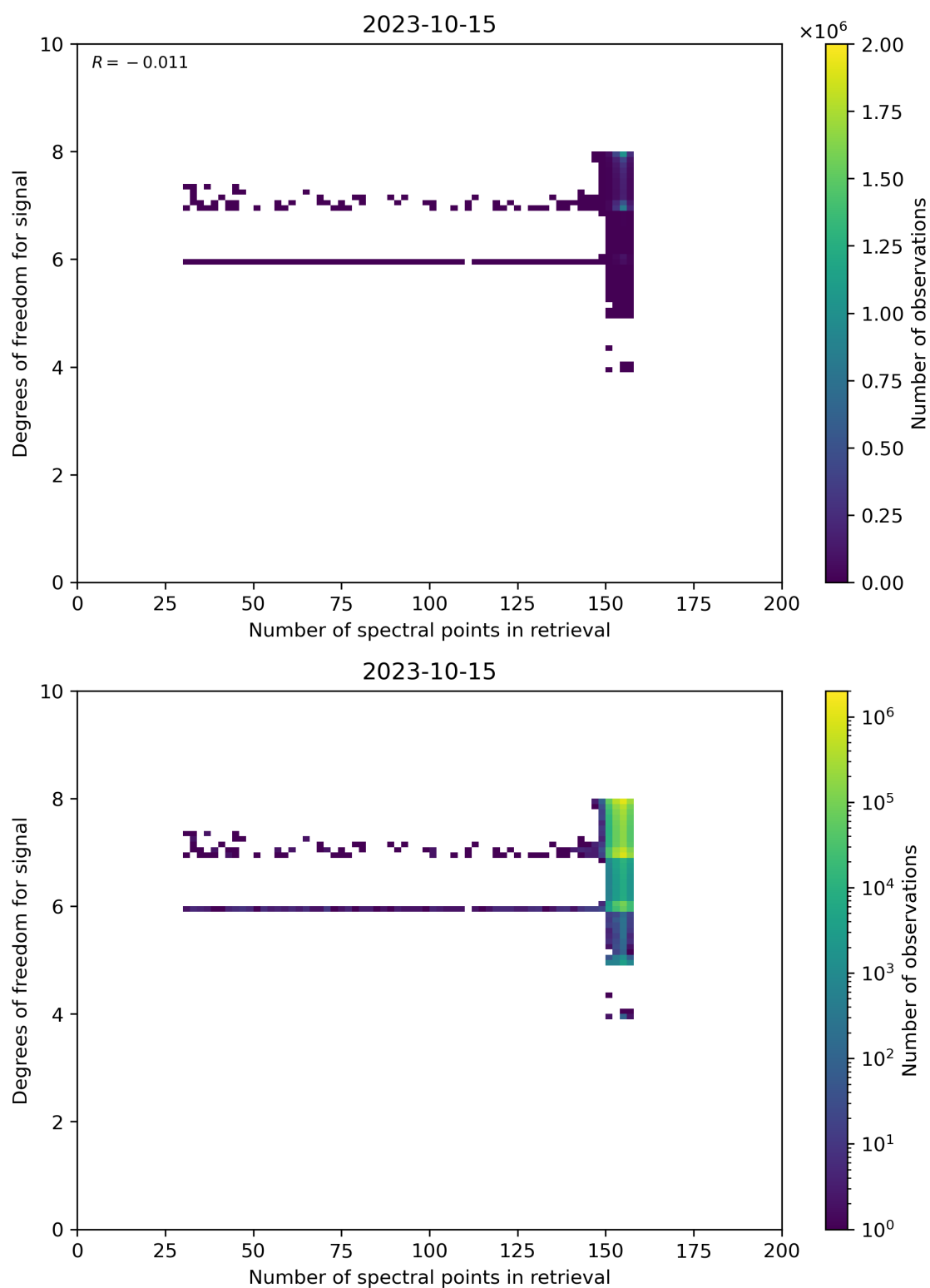
Figure 59: Scatter density plot of “Number of spectral points in retrieval” against “Degrees of freedom for signal” for 2023-10-14 to 2023-10-16.
