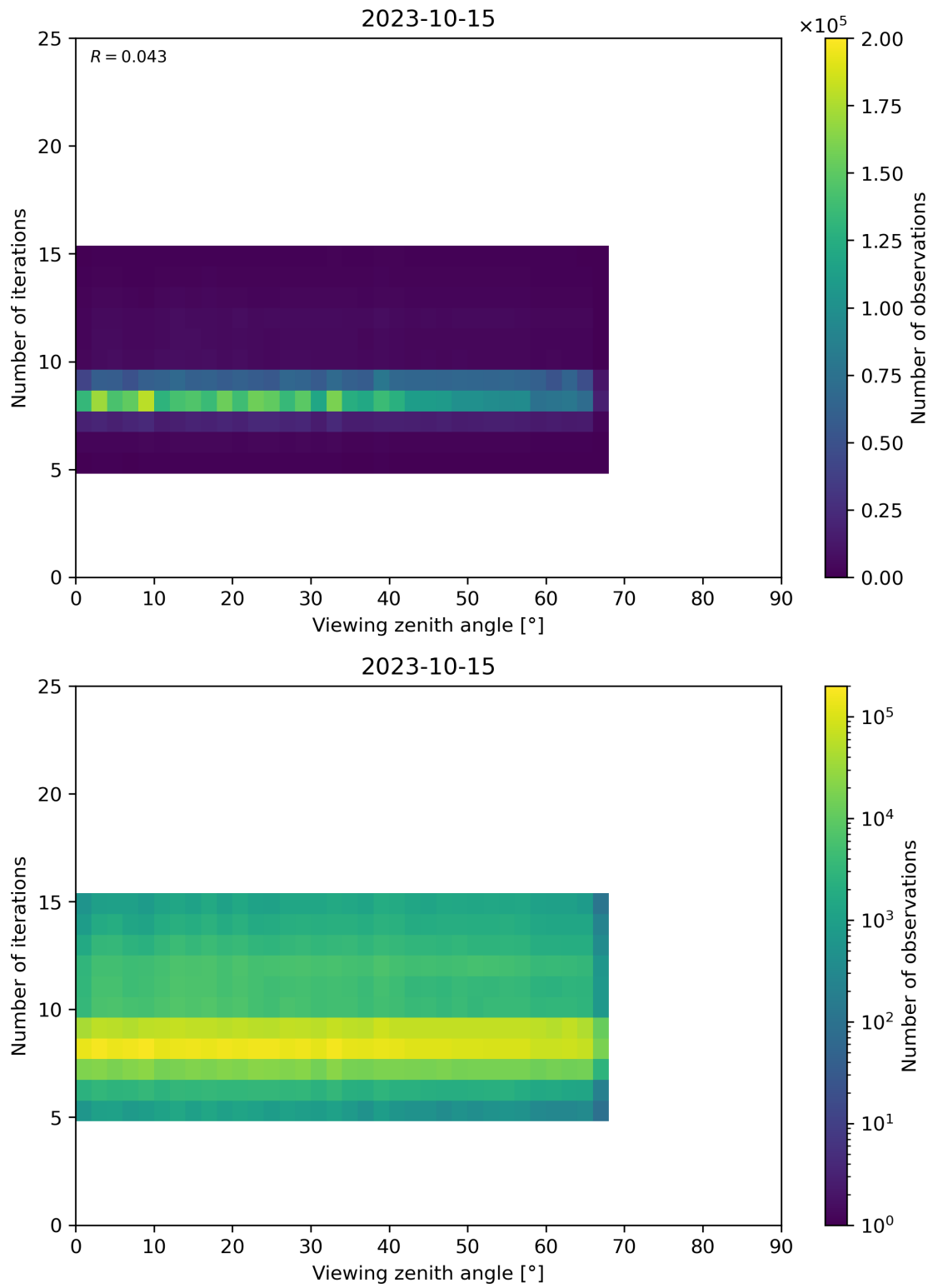
Figure 75: Scatter density plot of “Viewing zenith angle” against “Number of iterations” for 2023-10-14 to 2023-10-16.
