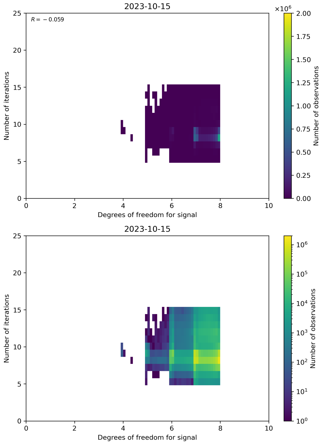
Figure 50: Scatter density plot of “Degrees of freedom for signal” against “Number of iterations” for 2023-10-14 to 2023-10-16.
