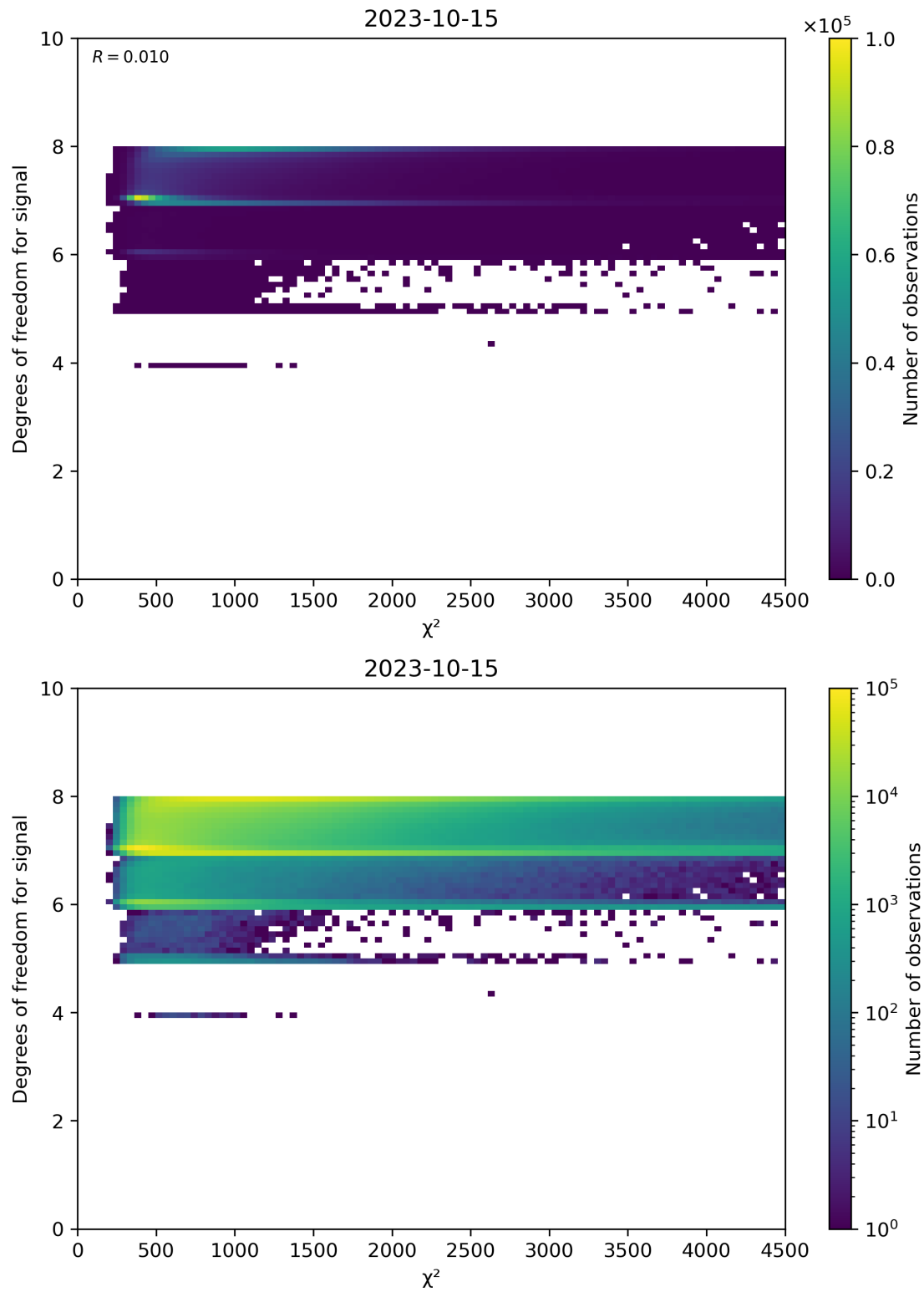
Figure 48: Scatter density plot of “ \chi^2 ” against “Degrees of freedom for signal” for 2023-10-14 to 2023-10-16.
