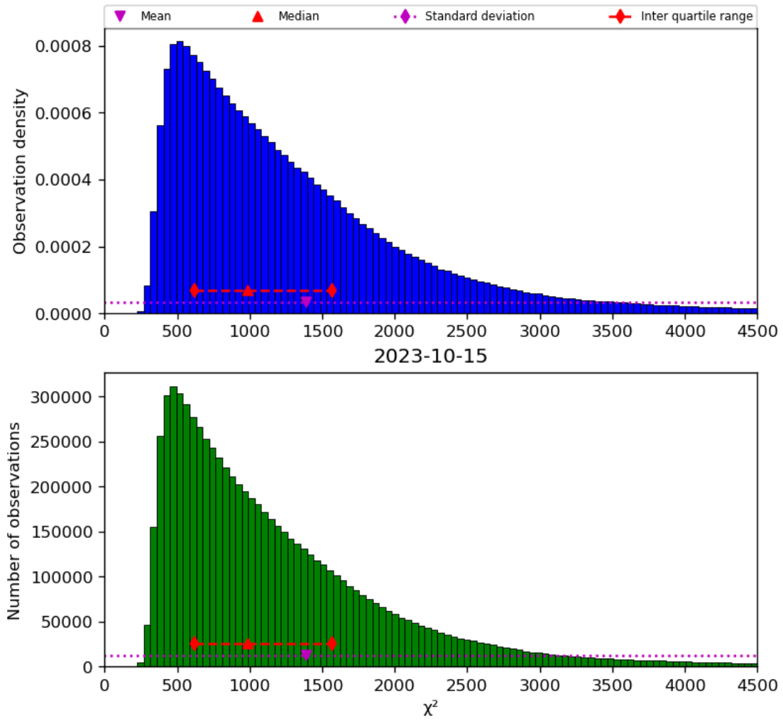
Figure 22: Histogram of “ \chi^2 ” for 2023-10-14 to 2023-10-16
