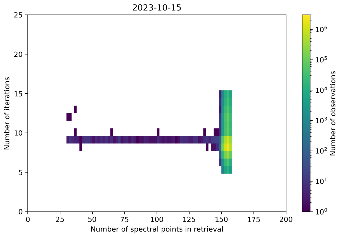
Figure 60: Scatter density plot of “Number of spectral points in retrieval” against “Number of iterations” for 2023-10-14 to 2023-10-16.
