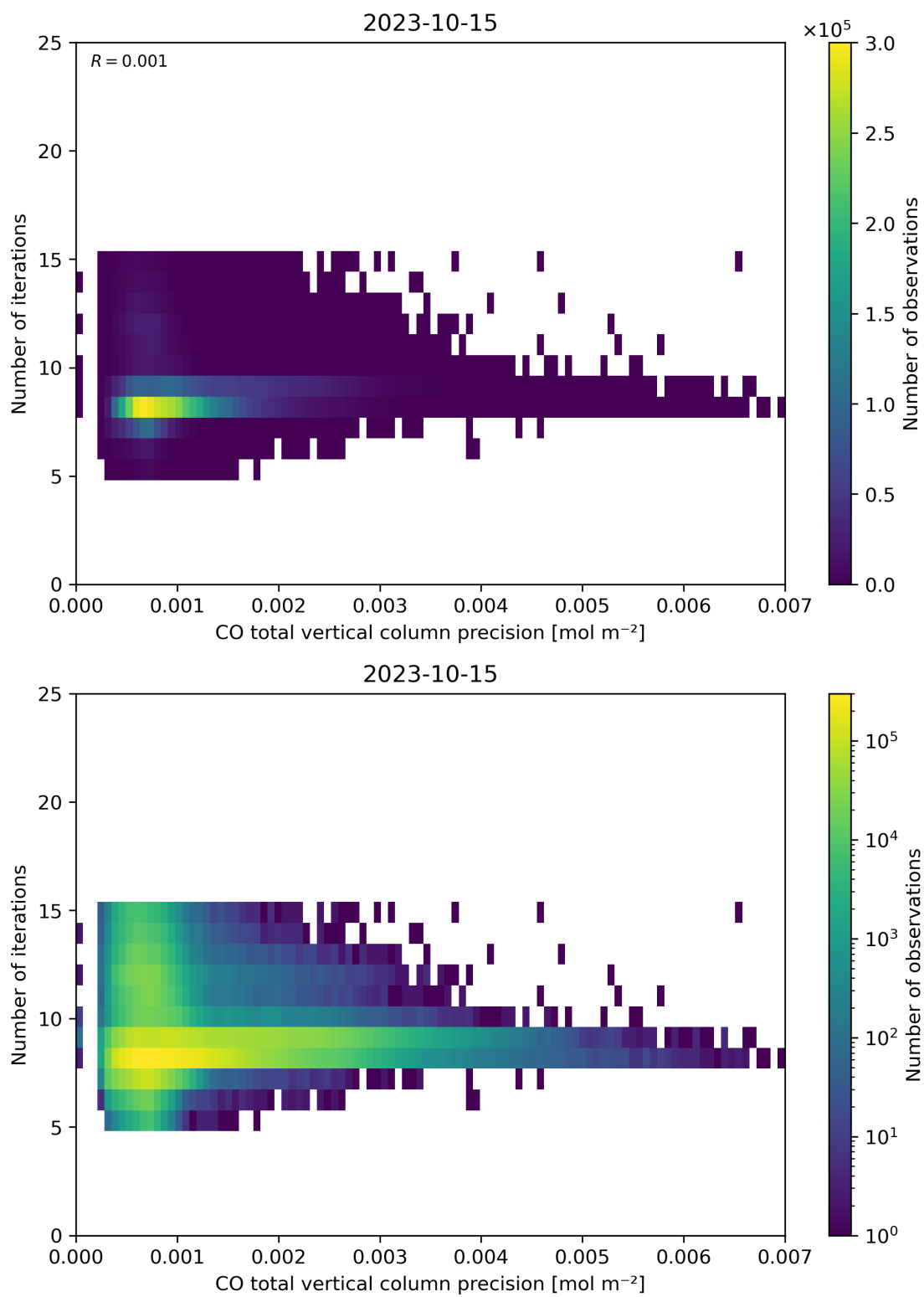
Figure 46: Scatter density plot of “CO total vertical column precision” against “Number of iterations” for 2023-10-14 to 2023-10-16.
