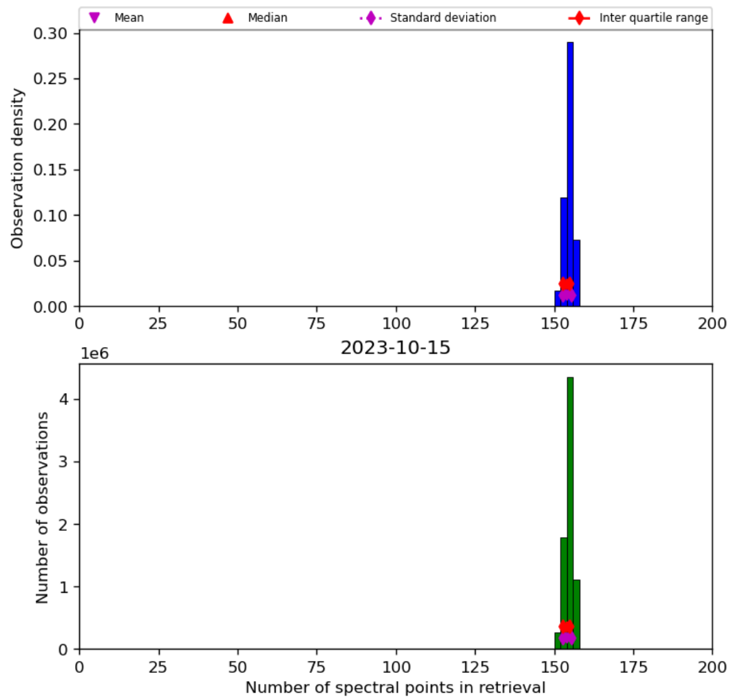
Figure 21: Histogram of “Number of spectral points in retrieval” for 2023-10-14 to 2023-10-16
