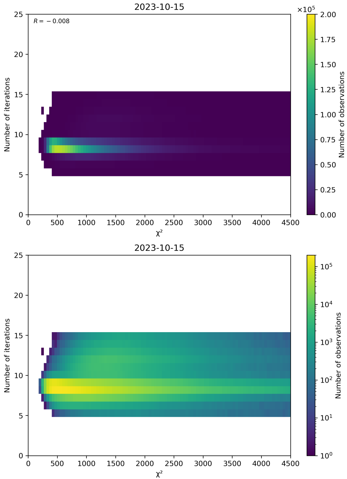
Figure 49: Scatter density plot of “ \chi^2 ” against “Number of iterations” for 2023-10-14 to 2023-10-16.
