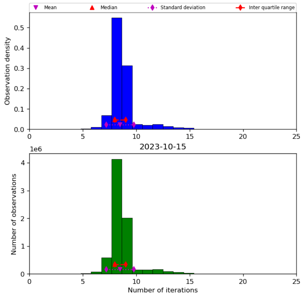
Figure 24: Histogram of “Number of iterations” for 2023-10-14 to 2023-10-16
