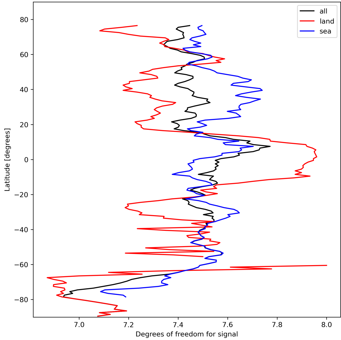
Figure 15: Zonal average of “Degrees of freedom for signal” for 2023-10-14 to 2023-10-16.
