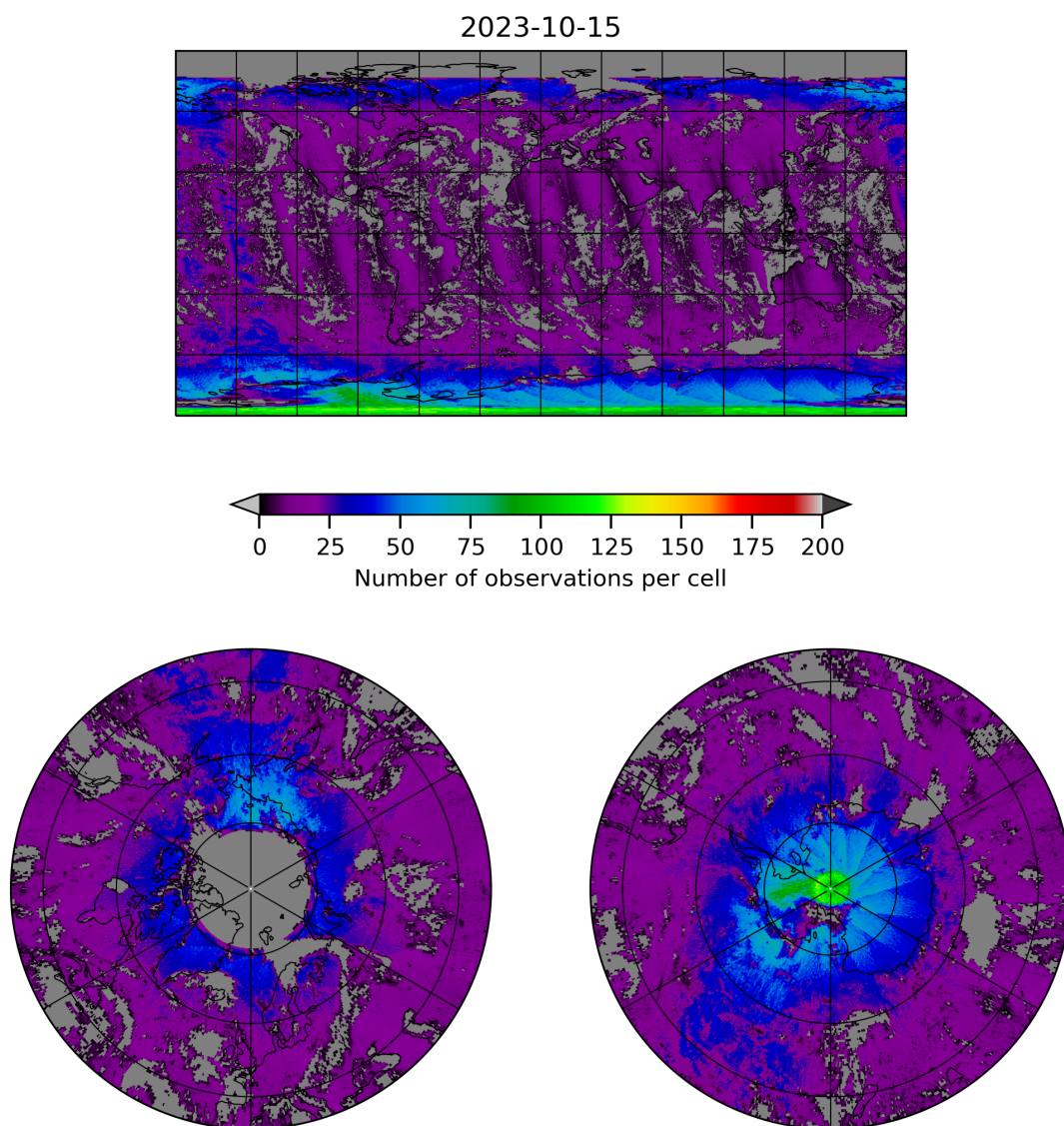
Figure 8: Map of the number of observations for 2023-10-14 to 2023-10-16
