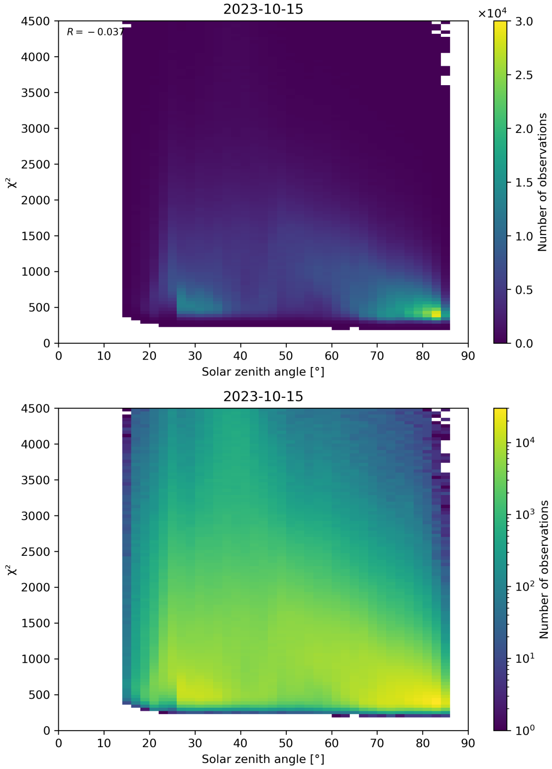
Figure 64: Scatter density plot of “Solar zenith angle” against “ \chi^2 ” for 2023-10-14 to 2023-10-16.
