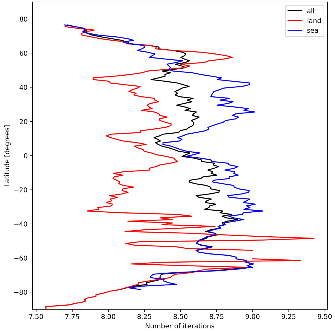
Figure 16: Zonal average of “Number of iterations” for 2023-10-14 to 2023-10-16.
