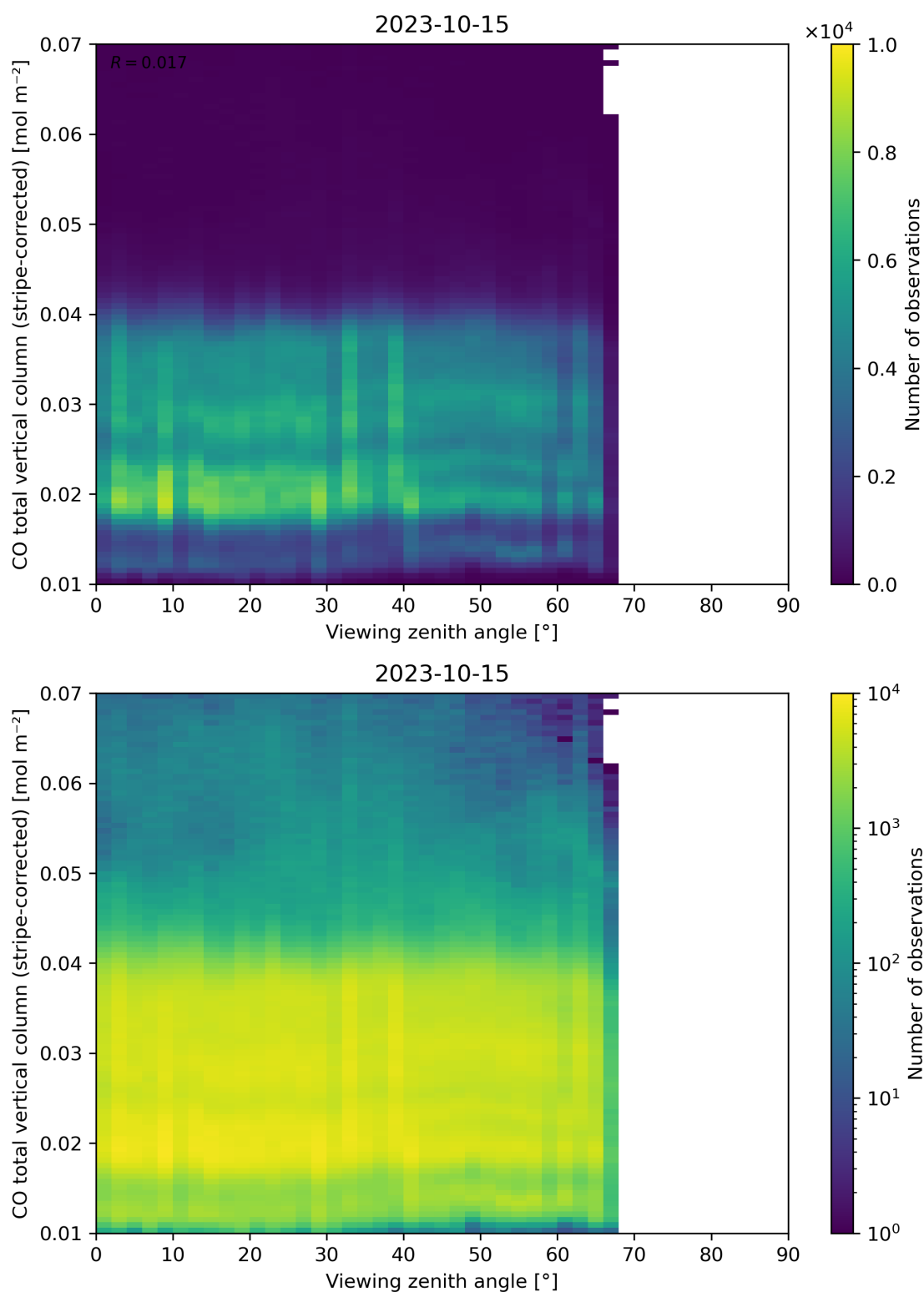
Figure 70: Scatter density plot of “Viewing zenith angle” against “CO total vertical column (stripe-corrected)” for 2023-10-14 to 2023-10-16.
