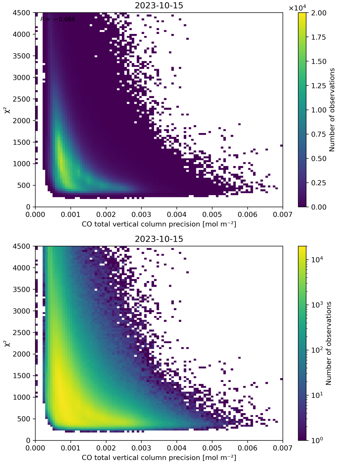
Figure 44: Scatter density plot of “CO total vertical column precision” against “ \chi^2 ” for 2023-10-14 to 2023-10-16.
