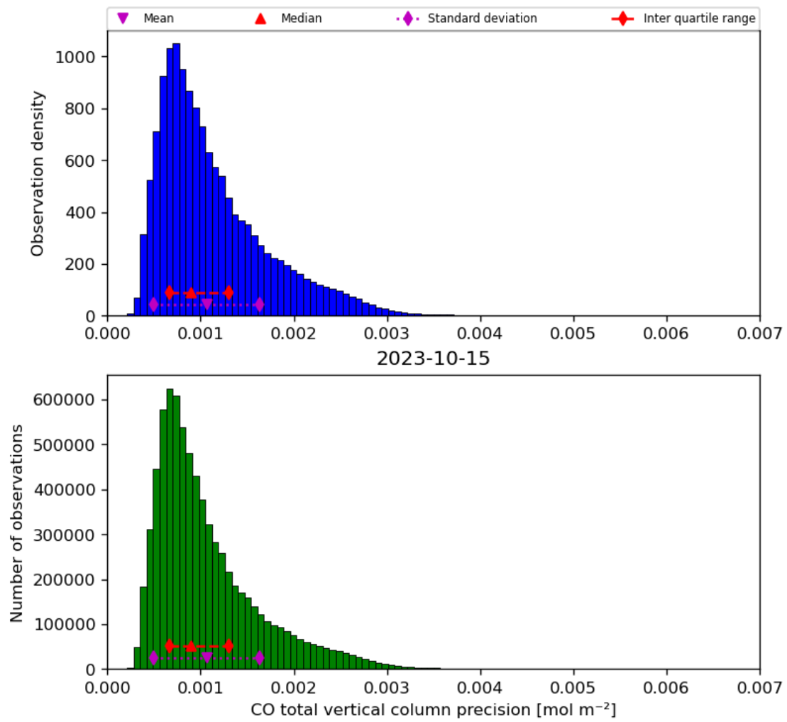
Figure 20: Histogram of “CO total vertical column precision” for 2023-10-14 to 2023-10-16
