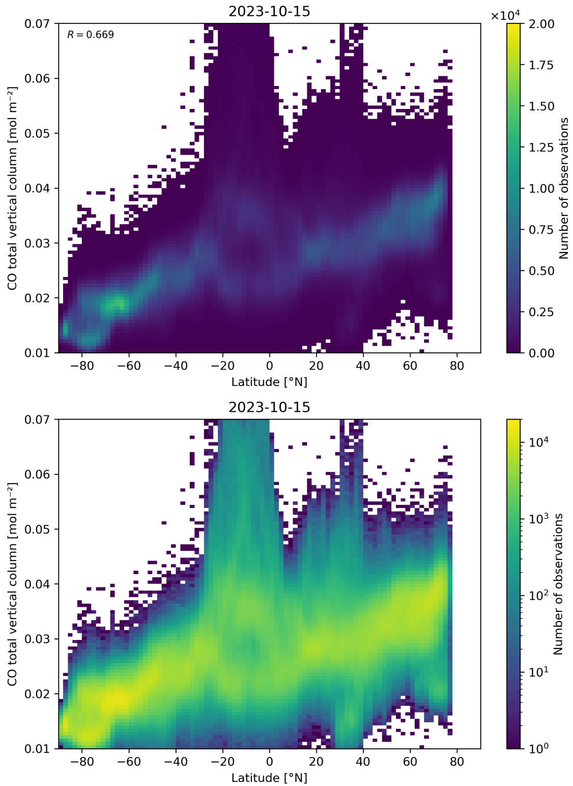
Figure 51: Scatter density plot of “Latitude” against “CO total vertical column” for 2023-10-14 to 2023-10-16.
