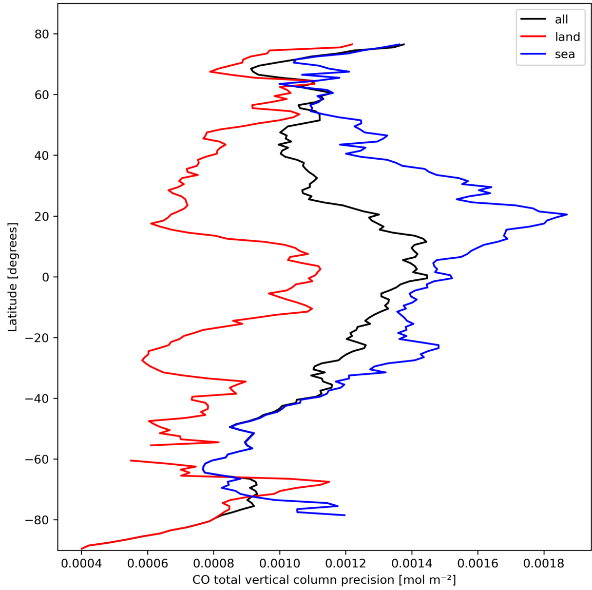
Figure 12: Zonal average of “CO total vertical column precision” for 2023-10-14 to 2023-10-16.
