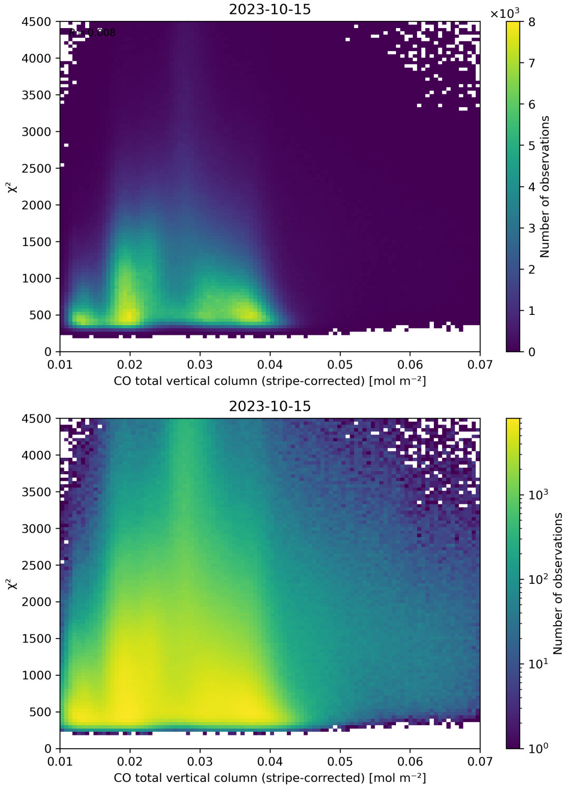
Figure 37: Scatter density plot of “CO total vertical column (stripe-corrected)” against “ \chi^2 ” for 2023-10-14 to 2023-10-16.
