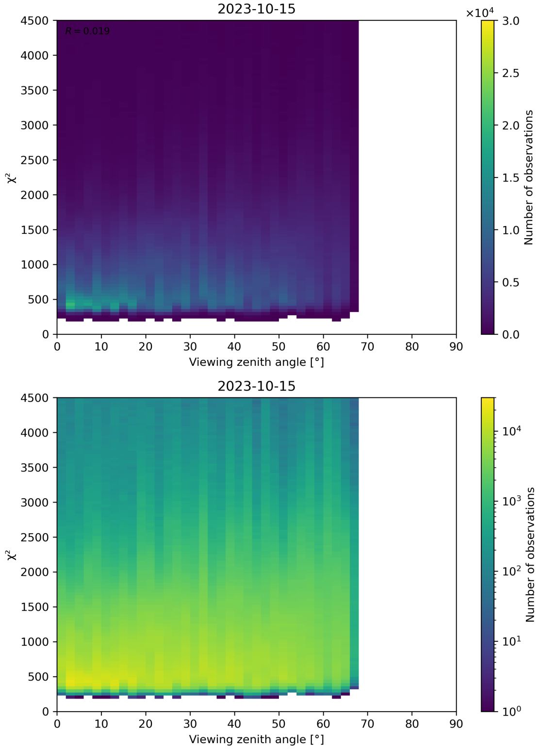
Figure 72: Scatter density plot of “Viewing zenith angle” against “ \chi^2 ” for 2023-10-14 to 2023-10-16.
