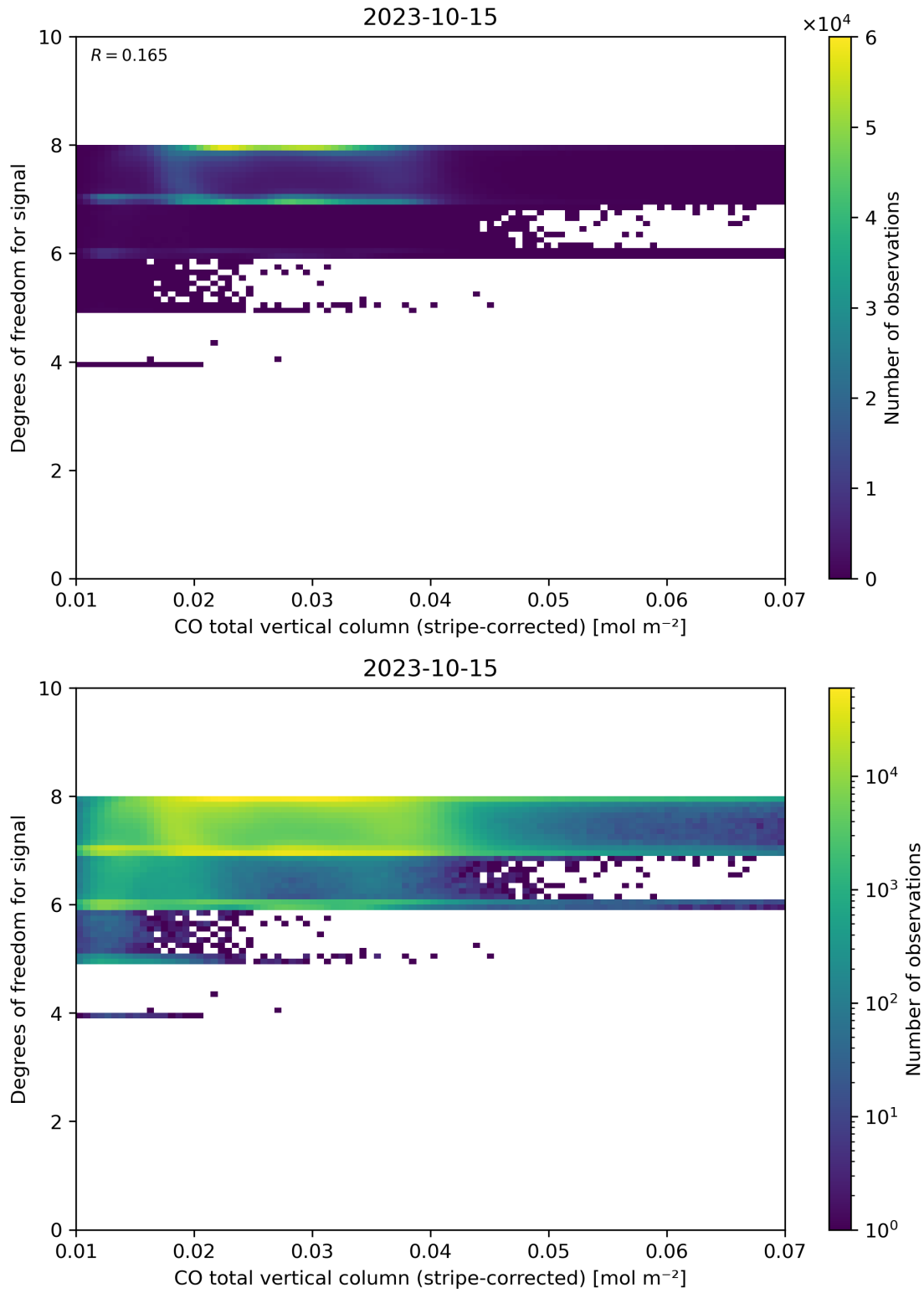
Figure 38: Scatter density plot of “CO total vertical column (stripe-corrected)” against “Degrees of freedom for signal” for 2023-10-14 to 2023-10-16.
