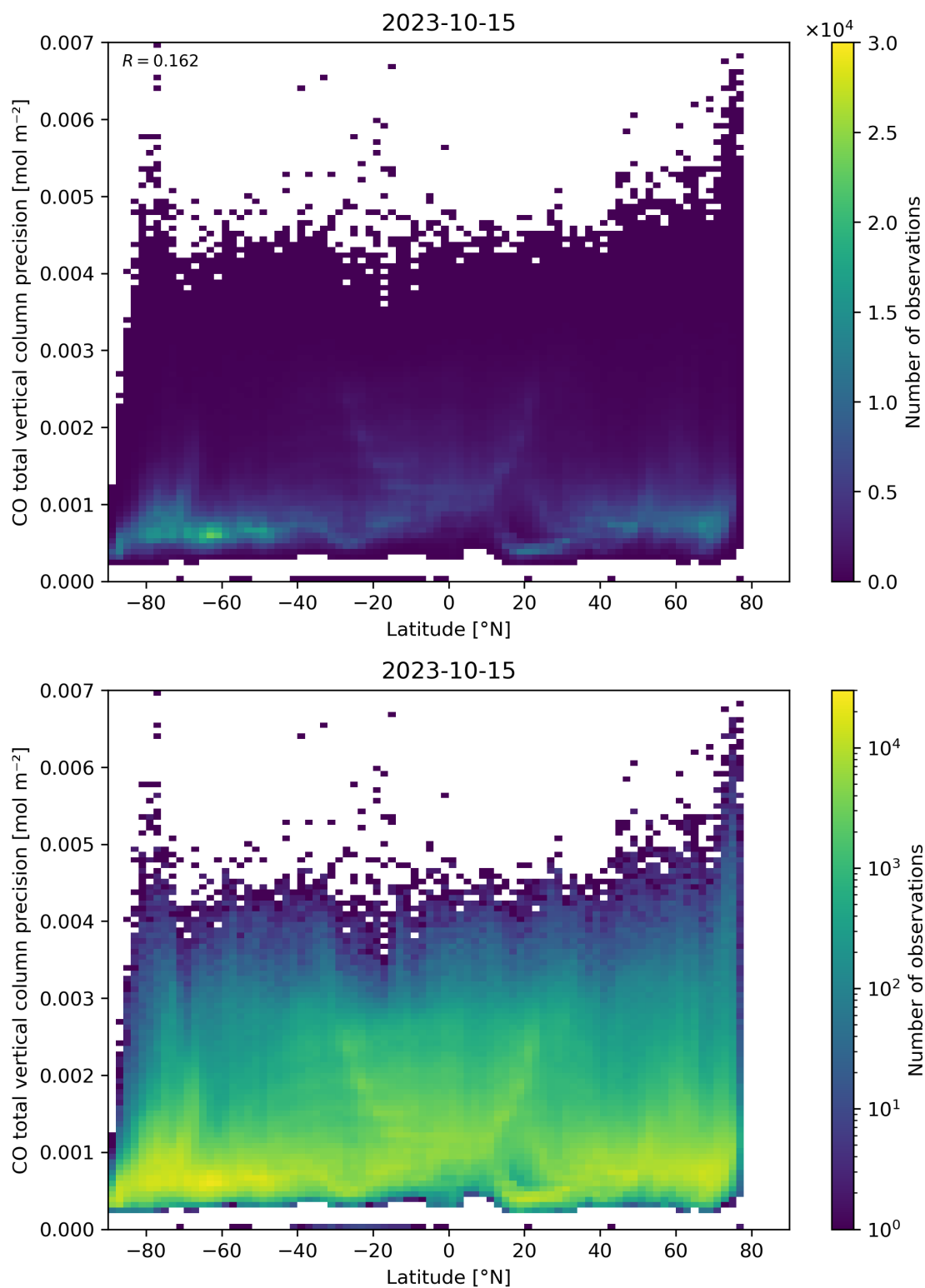
Figure 53: Scatter density plot of “Latitude” against “CO total vertical column precision” for 2023-10-14 to 2023-10-16.
