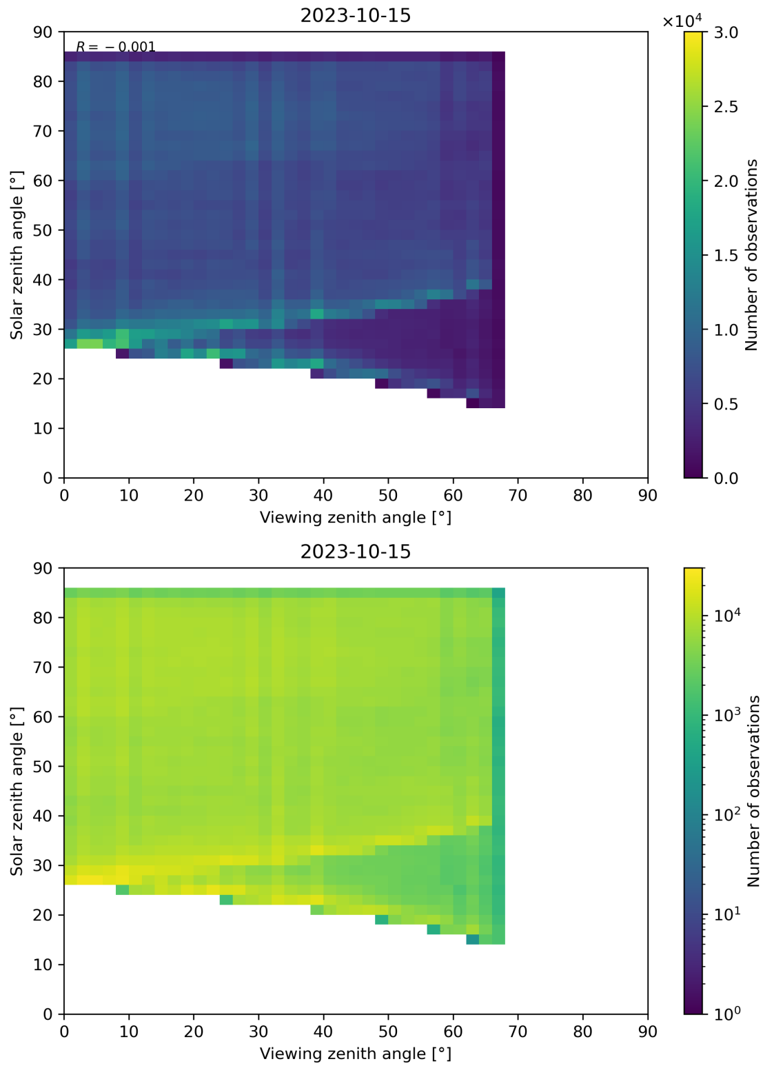
Figure 77: Scatter density plot of “Viewing zenith angle” against “Solar zenith angle” for 2023-10-14 to 2023-10-16.
