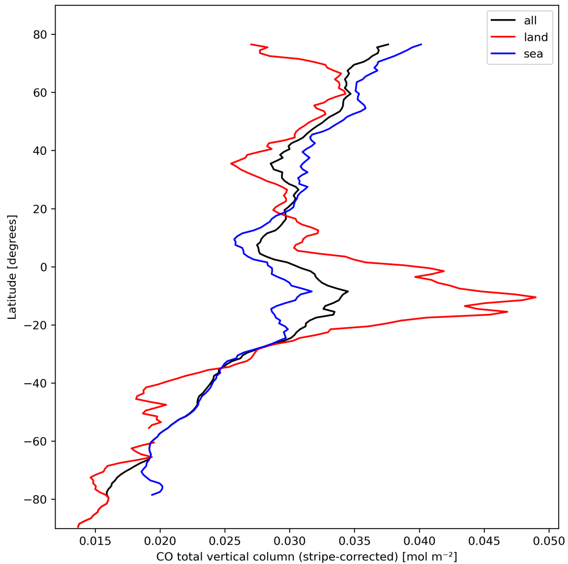
Figure 11: Zonal average of “CO total vertical column (stripe-corrected)” for 2023-10-14 to 2023-10-16.
