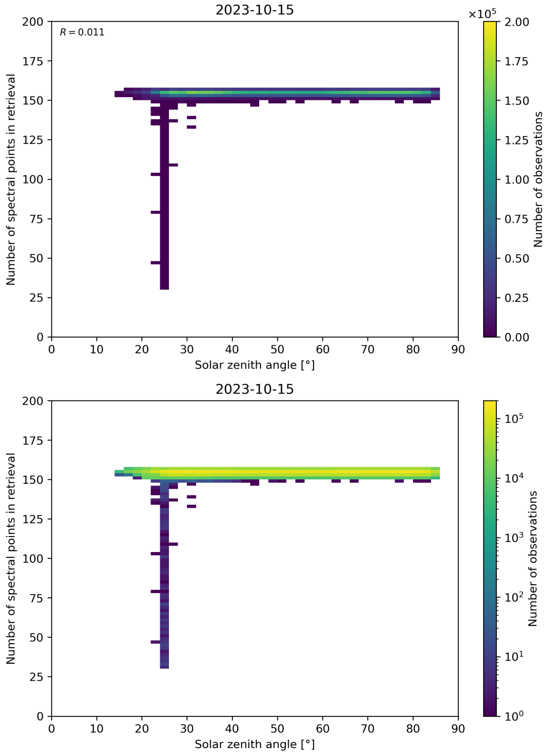
Figure 68: Scatter density plot of “Solar zenith angle” against “Number of spectral points in retrieval” for 2023-10-14 to 2023-10-16.
