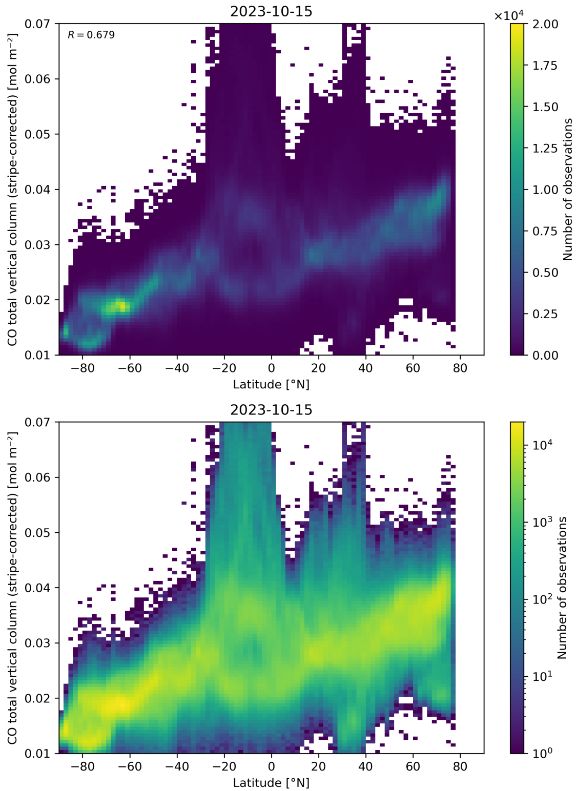
Figure 52: Scatter density plot of “Latitude” against “CO total vertical column (stripe-corrected)” for 2023-10-14 to 2023-10-16.
