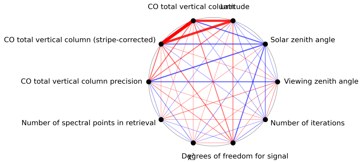
Figure 1: Map of correlation graph for 2023-10-14 to 2023-10-16.
