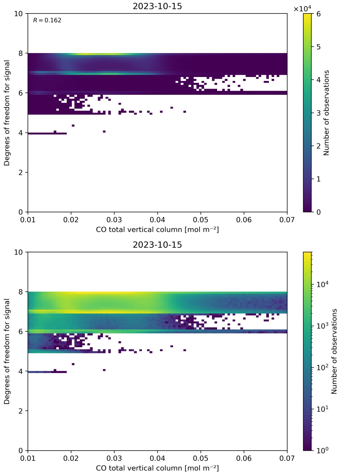
Figure 41: Scatter density plot of “CO total vertical column” against “Degrees of freedom for signal” for 2023-10-14 to 2023-10-16.
