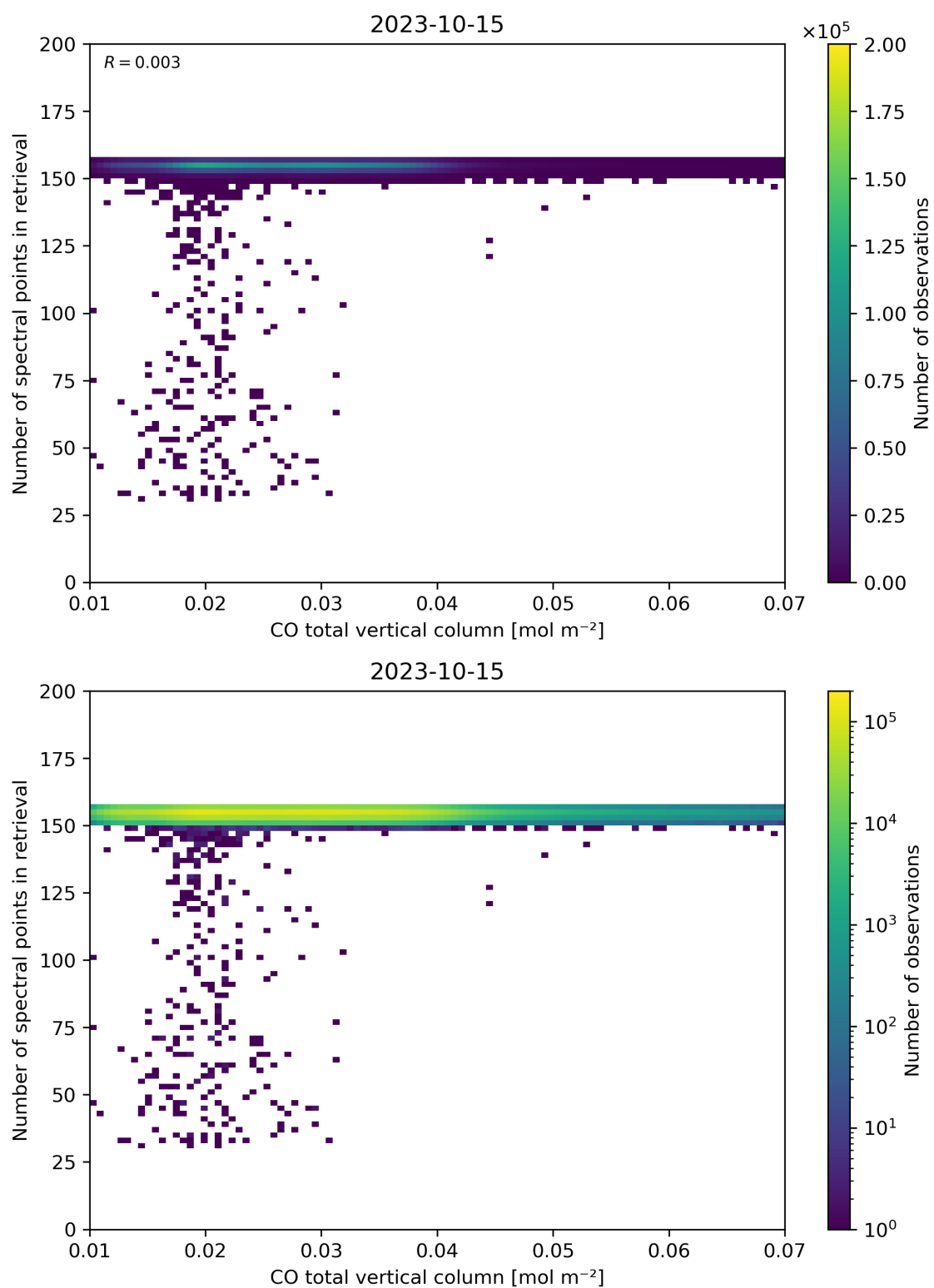
Figure 43: Scatter density plot of “CO total vertical column” against “Number of spectral points in retrieval” for 2023-10-14 to 2023-10-16.
