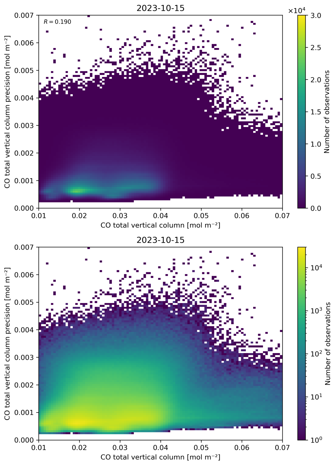
Figure 34: Scatter density plot of “CO total vertical column” against “CO total vertical column precision” for 2023-10-14 to 2023-10-16.
