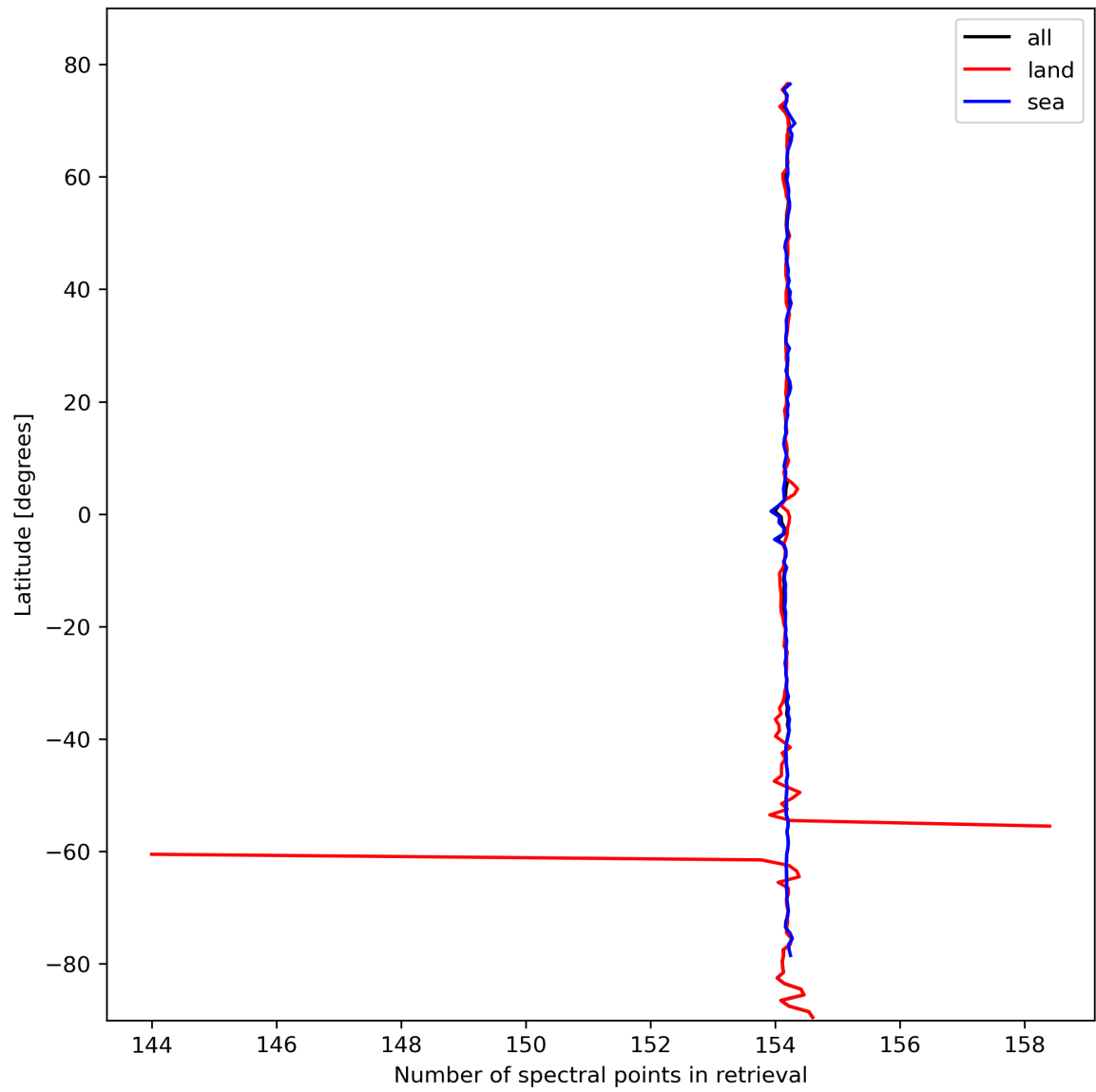
Figure 13: Zonal average of “Number of spectral points in retrieval” for 2023-10-14 to 2023-10-16.
