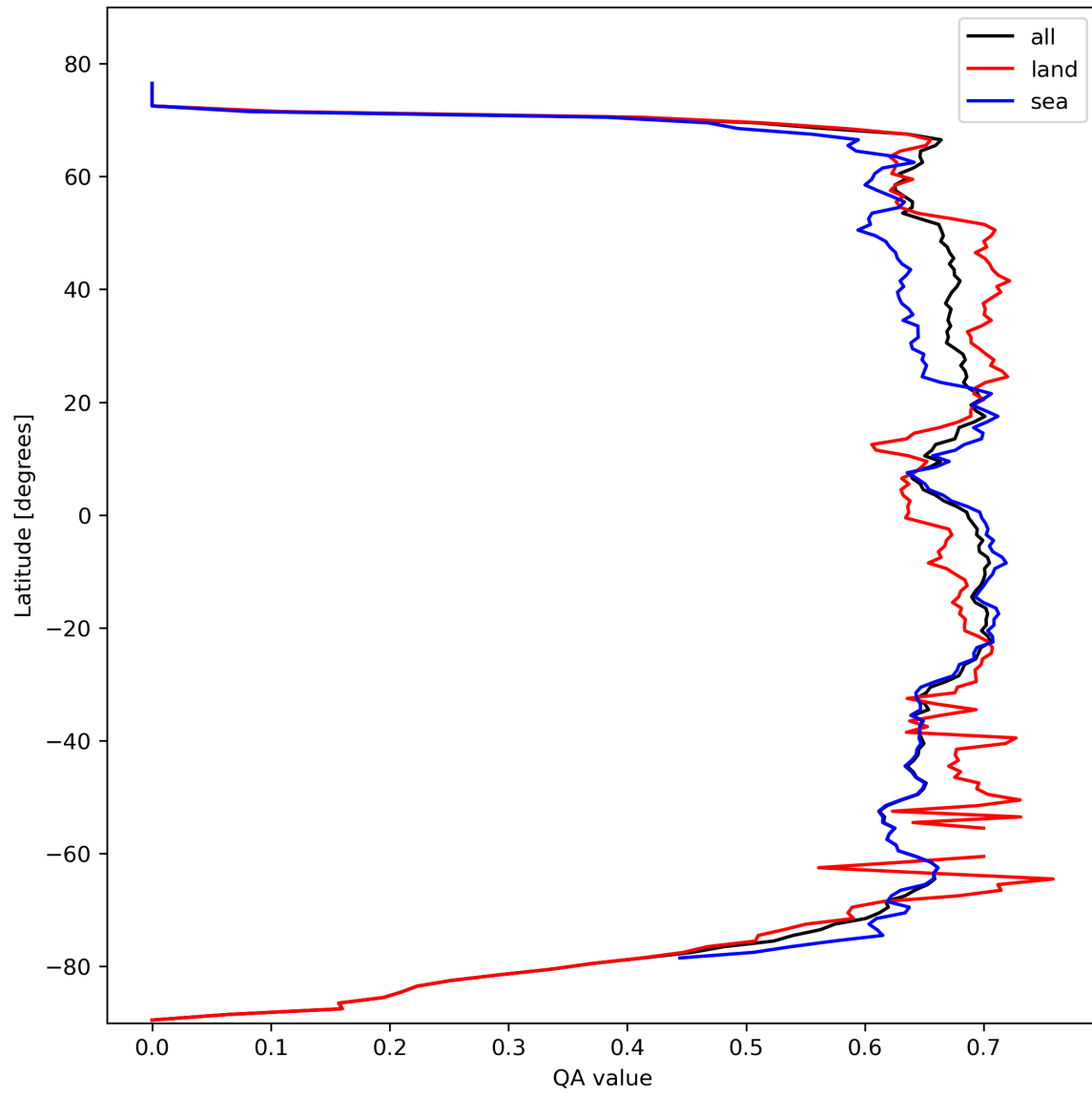
Figure 9: Zonal average of “QA value” for 2023-10-14 to 2023-10-16.
