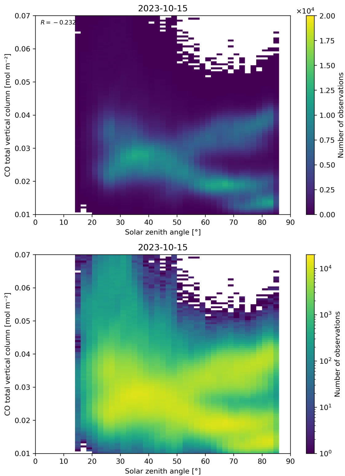
Figure 61: Scatter density plot of “Solar zenith angle” against “CO total vertical column” for 2023-10-14 to 2023-10-16.
