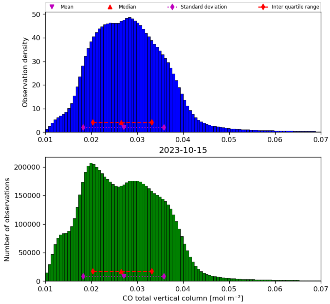
Figure 18: Histogram of “CO total vertical column” for 2023-10-14 to 2023-10-16
