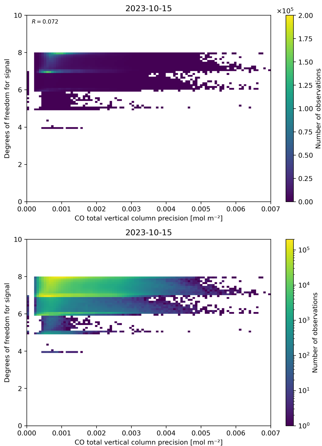
Figure 45: Scatter density plot of “CO total vertical column precision” against “Degrees of freedom for signal” for 2023-10-14 to 2023-10-16.
