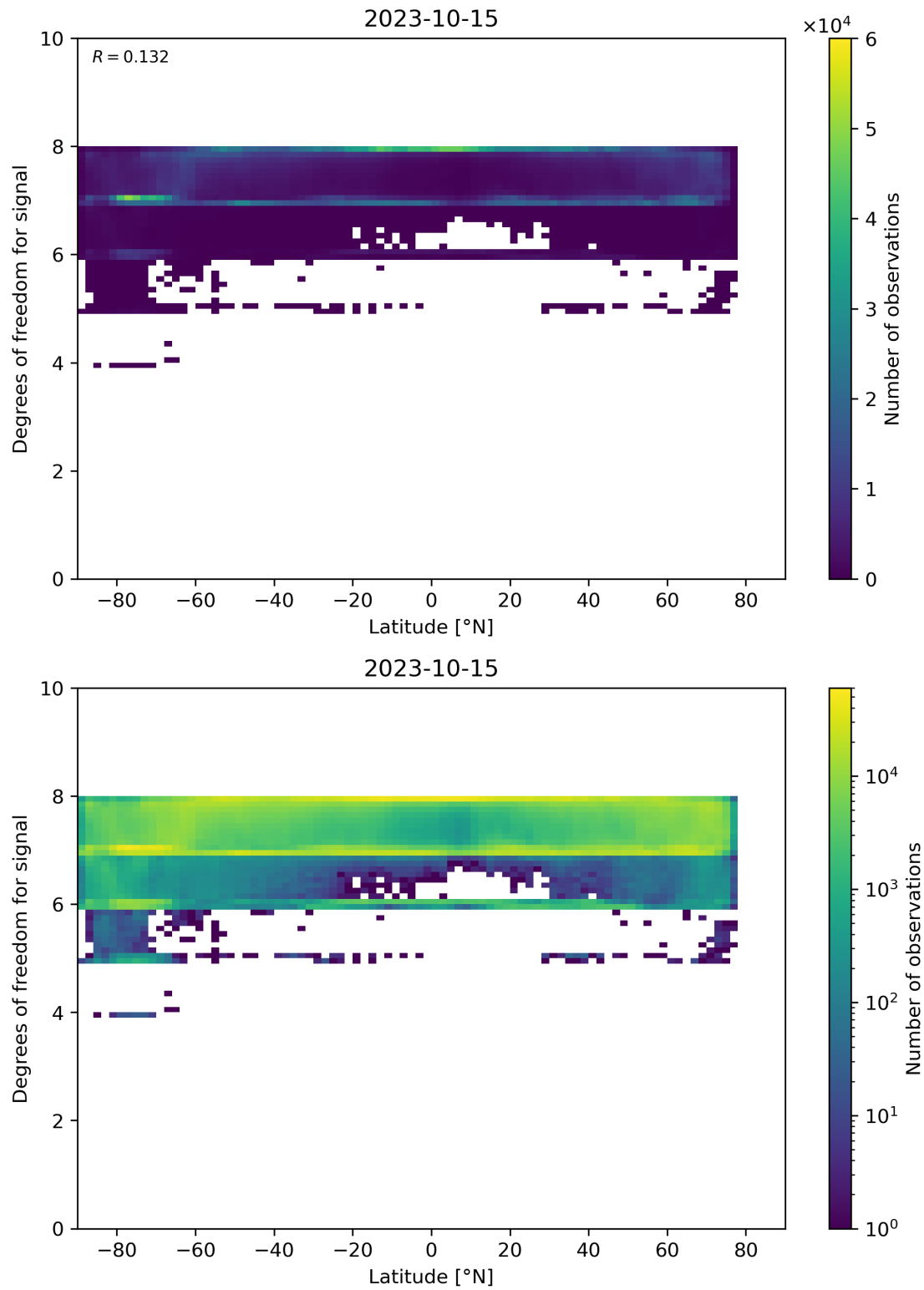
Figure 55: Scatter density plot of “Latitude” against “Degrees of freedom for signal” for 2023-10-14 to 2023-10-16.
