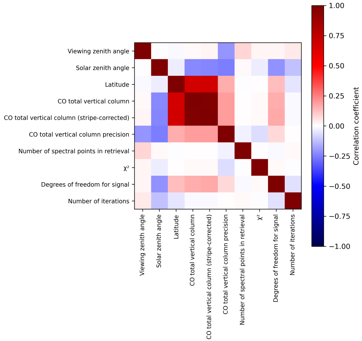
Figure 2: Map of correlation matrix for 2023-10-14 to 2023-10-16.
