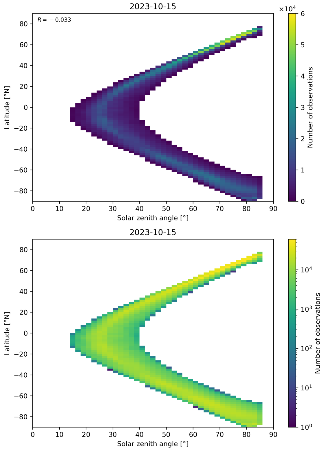
Figure 66: Scatter density plot of “Solar zenith angle” against “Latitude” for 2023-10-14 to 2023-10-16.
