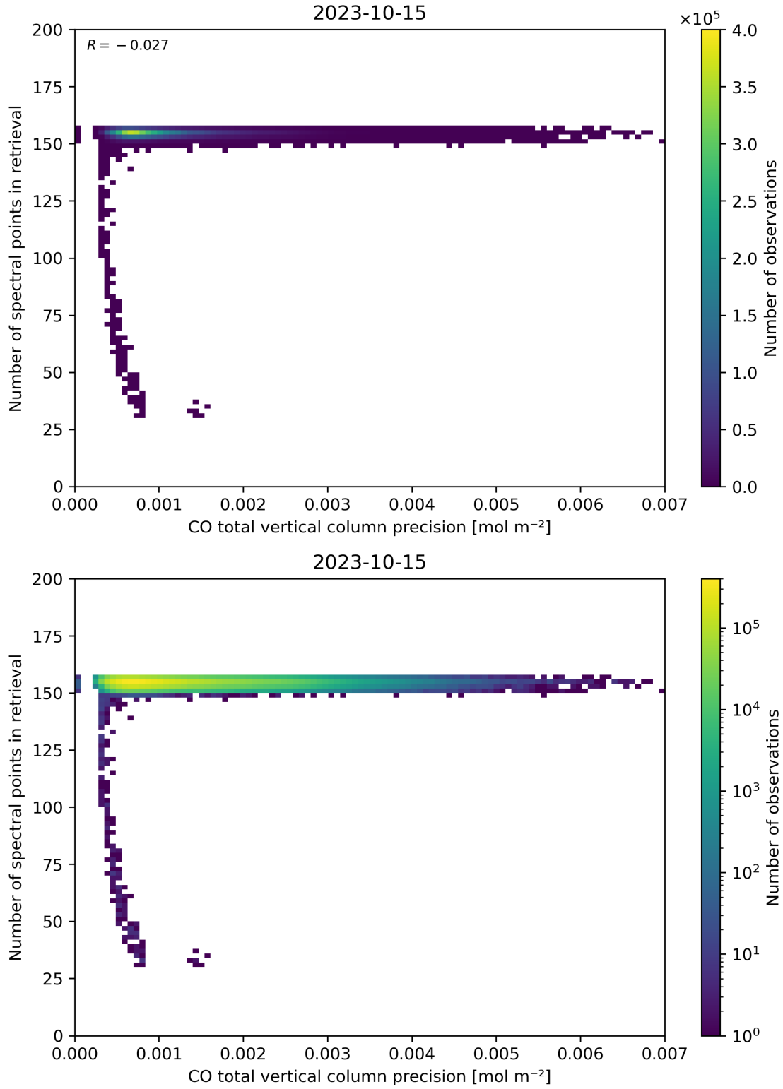
Figure 47: Scatter density plot of “CO total vertical column precision” against “Number of spectral points in retrieval” for 2023-10-14 to 2023-10-16.
