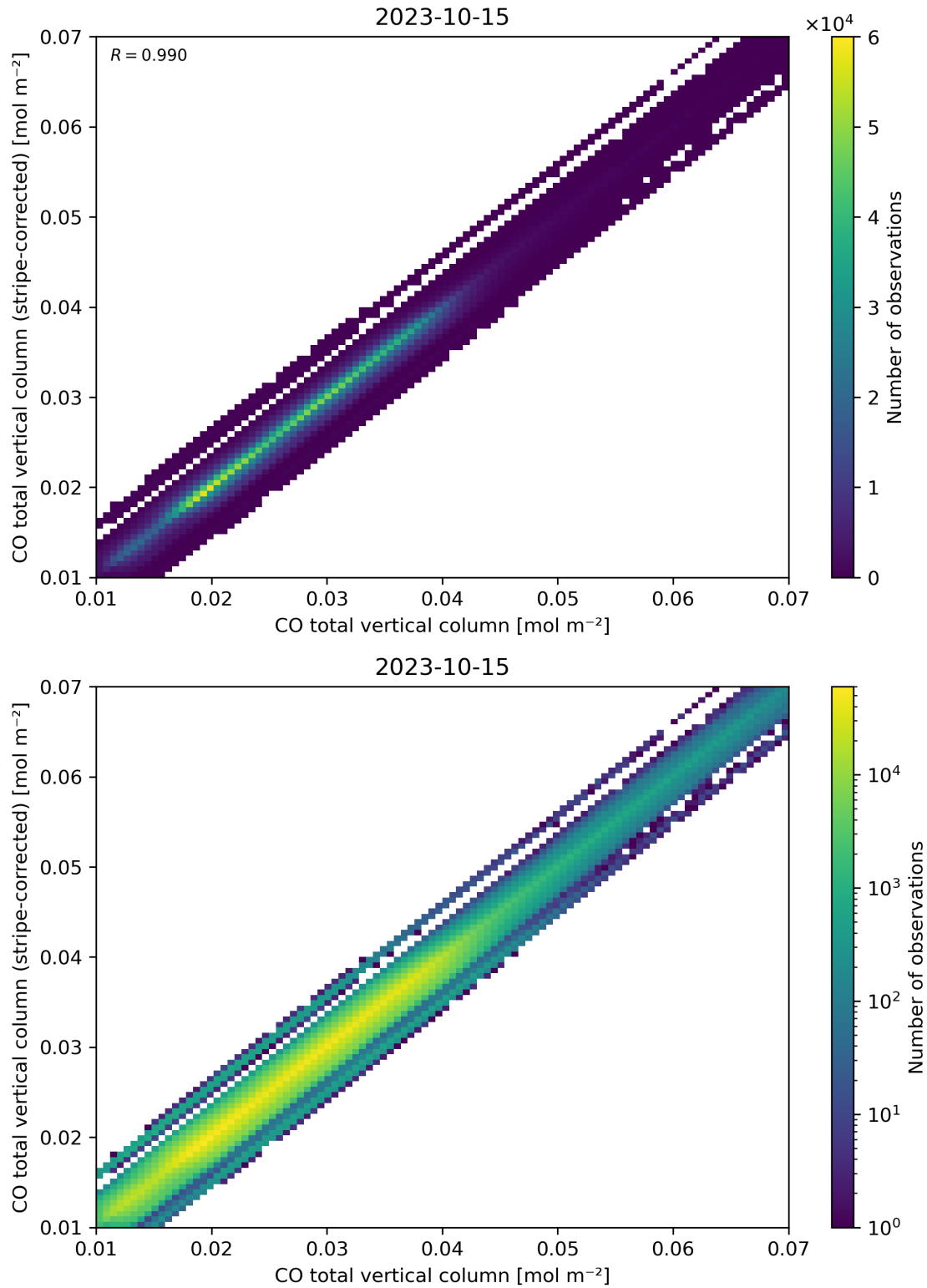
Figure 33: Scatter density plot of “CO total vertical column” against “CO total vertical column (stripe-corrected)” for 2023-10-14 to 2023-10-16.
