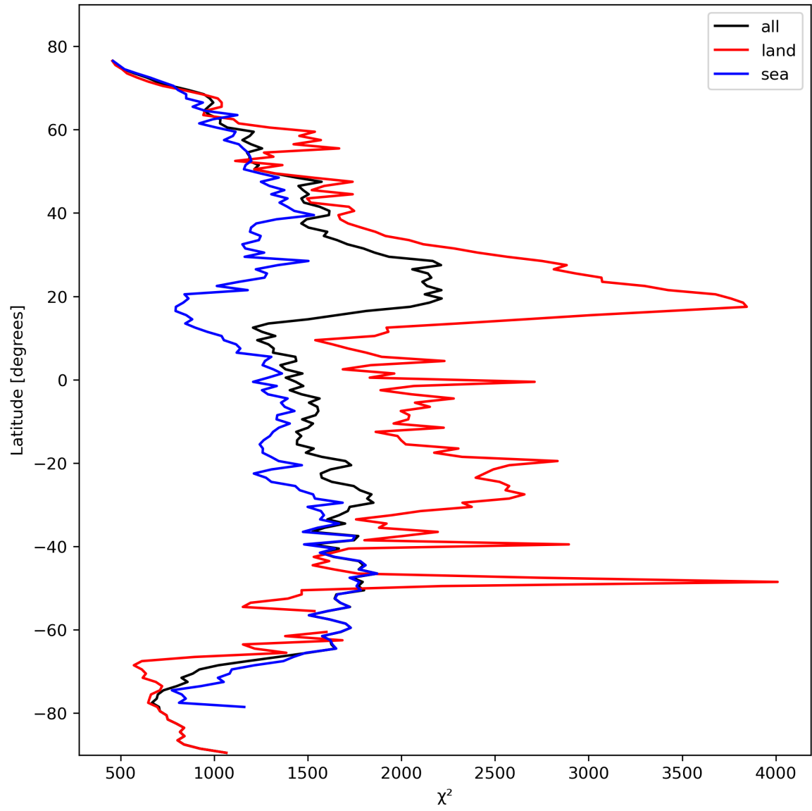
Figure 14: Zonal average of “ \chi^2 ” for 2023-10-14 to 2023-10-16.
