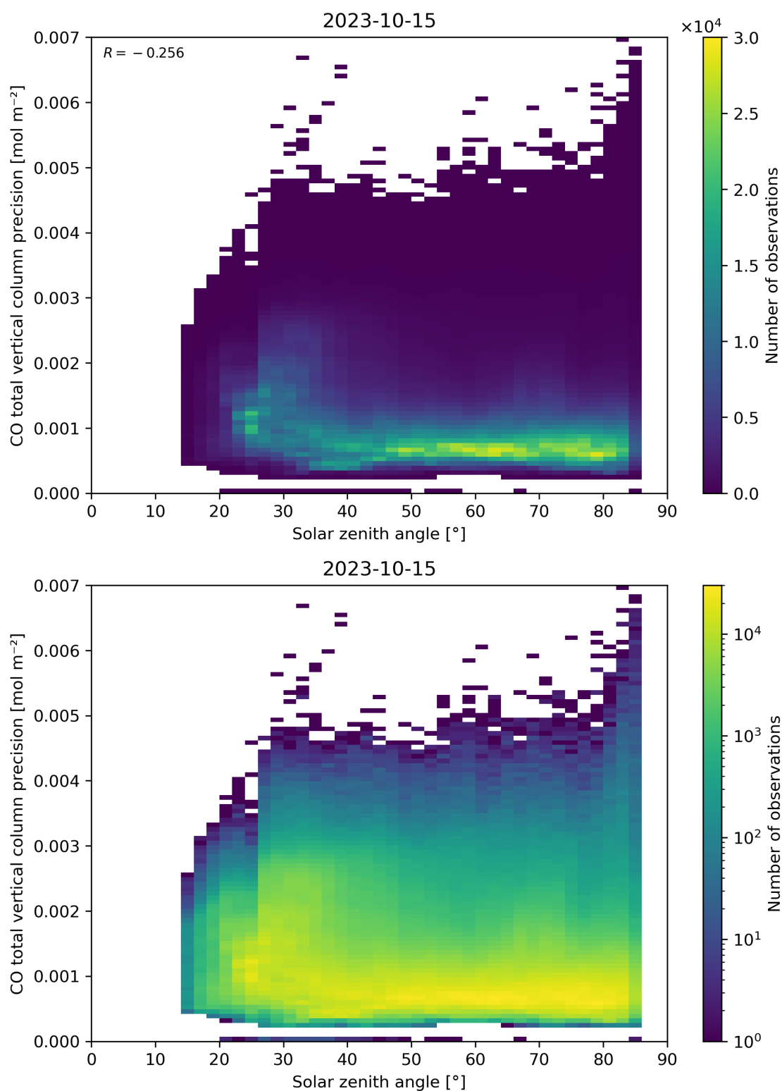
Figure 63: Scatter density plot of “Solar zenith angle” against “CO total vertical column precision” for 2023-10-14 to 2023-10-16.
