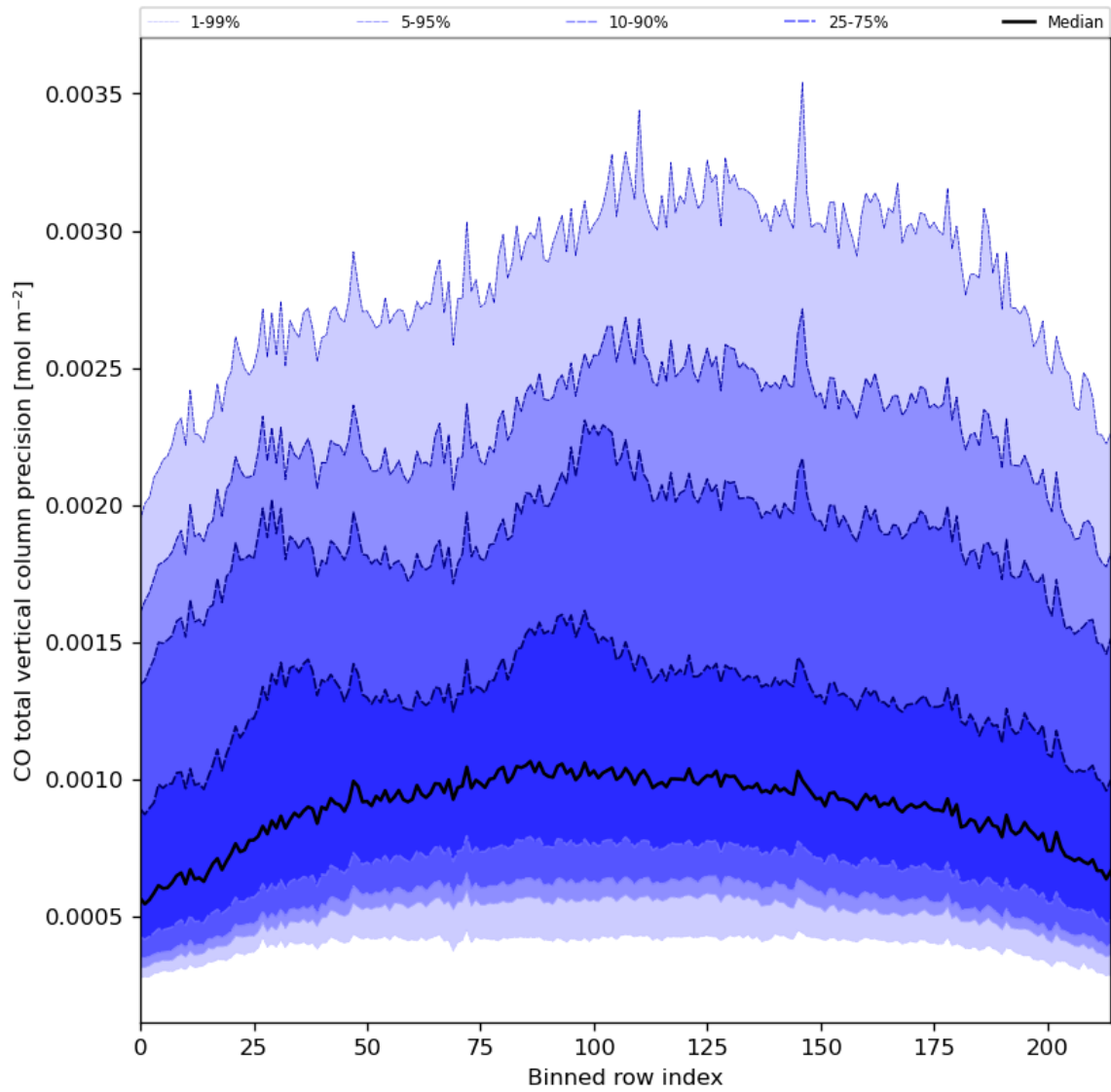
Figure 28: Along track statistics of “CO total vertical column precision” for 2023-10-14 to 2023-10-16
