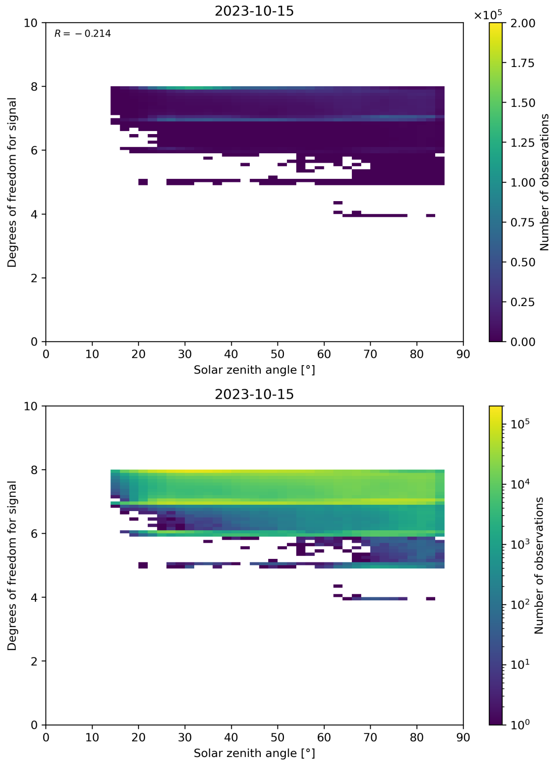
Figure 65: Scatter density plot of “Solar zenith angle” against “Degrees of freedom for signal” for 2023-10-14 to 2023-10-16.
