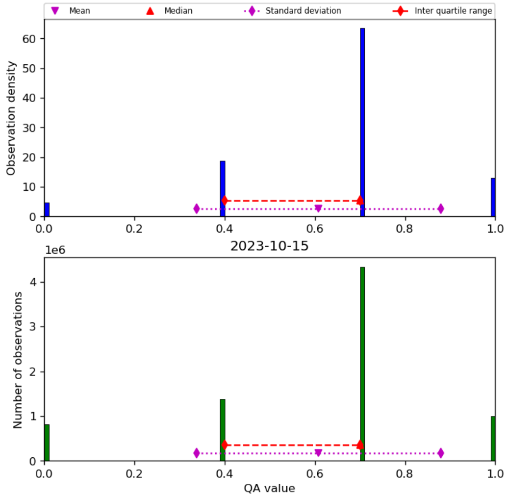
Figure 17: Histogram of “QA value” for 2023-10-14 to 2023-10-16
