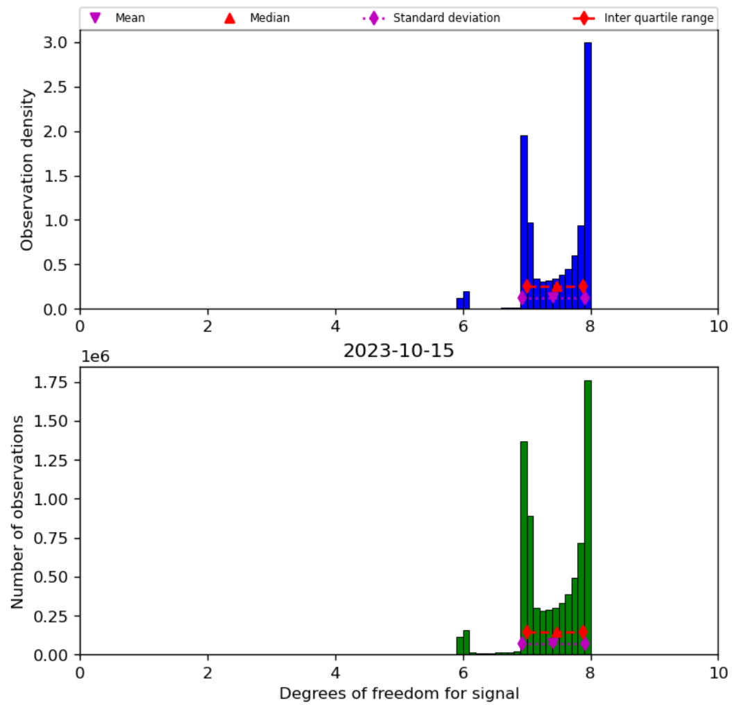
Figure 23: Histogram of “Degrees of freedom for signal” for 2023-10-14 to 2023-10-16
