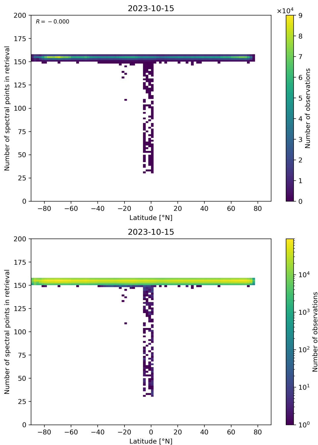
Figure 57: Scatter density plot of “Latitude” against “Number of spectral points in retrieval” for 2023-10-14 to 2023-10-16.
