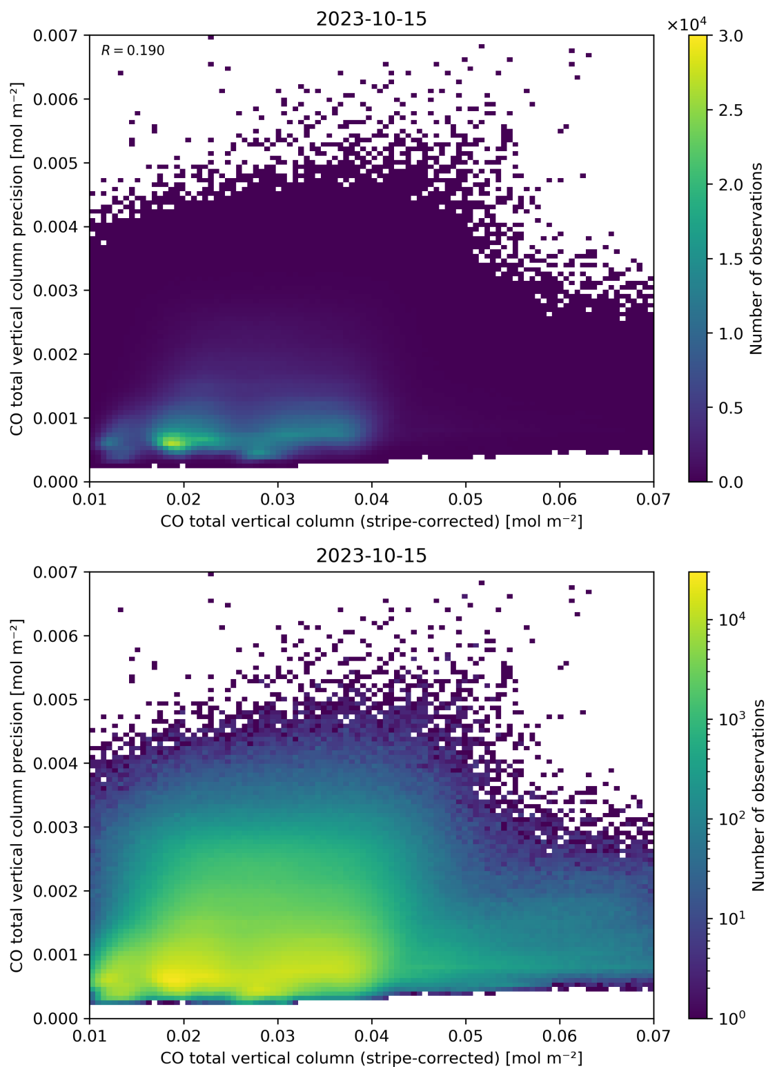
Figure 36: Scatter density plot of “CO total vertical column (stripe-corrected)” against “CO total vertical column precision” for 2023-10-14 to 2023-10-16.
