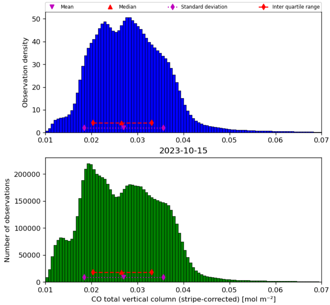
Figure 19: Histogram of “CO total vertical column (stripe-corrected)” for 2023-10-14 to 2023-10-16
