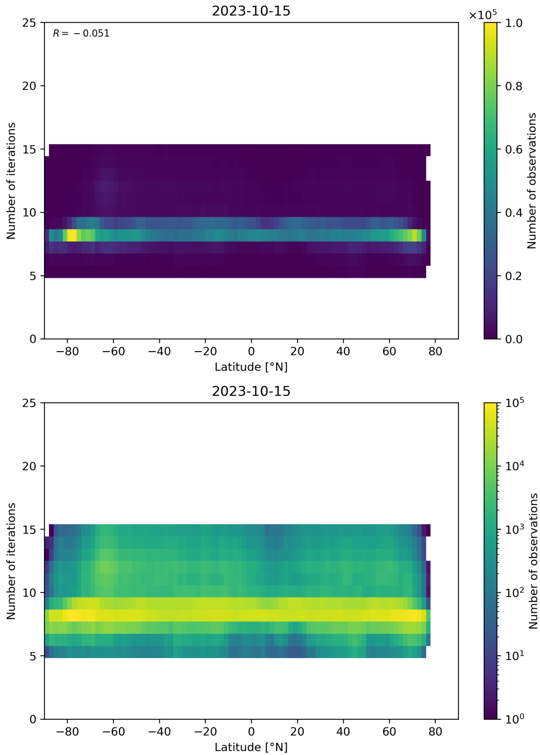
Figure 56: Scatter density plot of “Latitude” against “Number of iterations” for 2023-10-14 to 2023-10-16.
