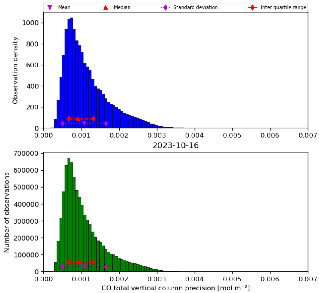
Figure 20: Histogram of “CO total vertical column precision” for 2023-10-15 to 2023-10-17
