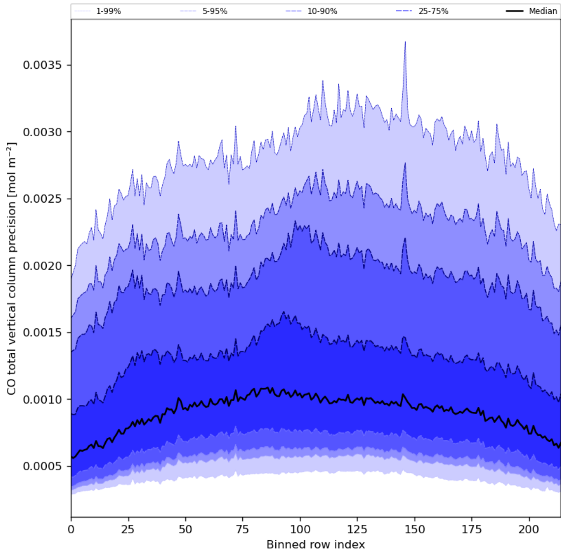
Figure 28: Along track statistics of “CO total vertical column precision” for 2023-10-15 to 2023-10-17
