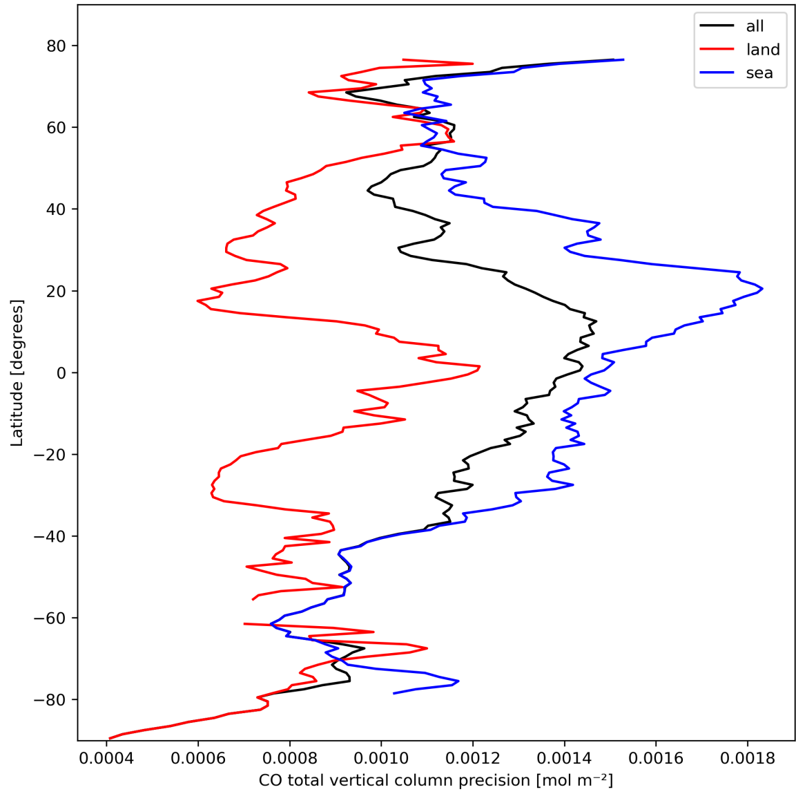
Figure 12: Zonal average of “CO total vertical column precision” for 2023-10-15 to 2023-10-17.
