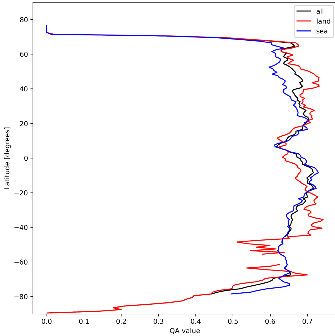
Figure 9: Zonal average of “QA value” for 2023-10-15 to 2023-10-17.
