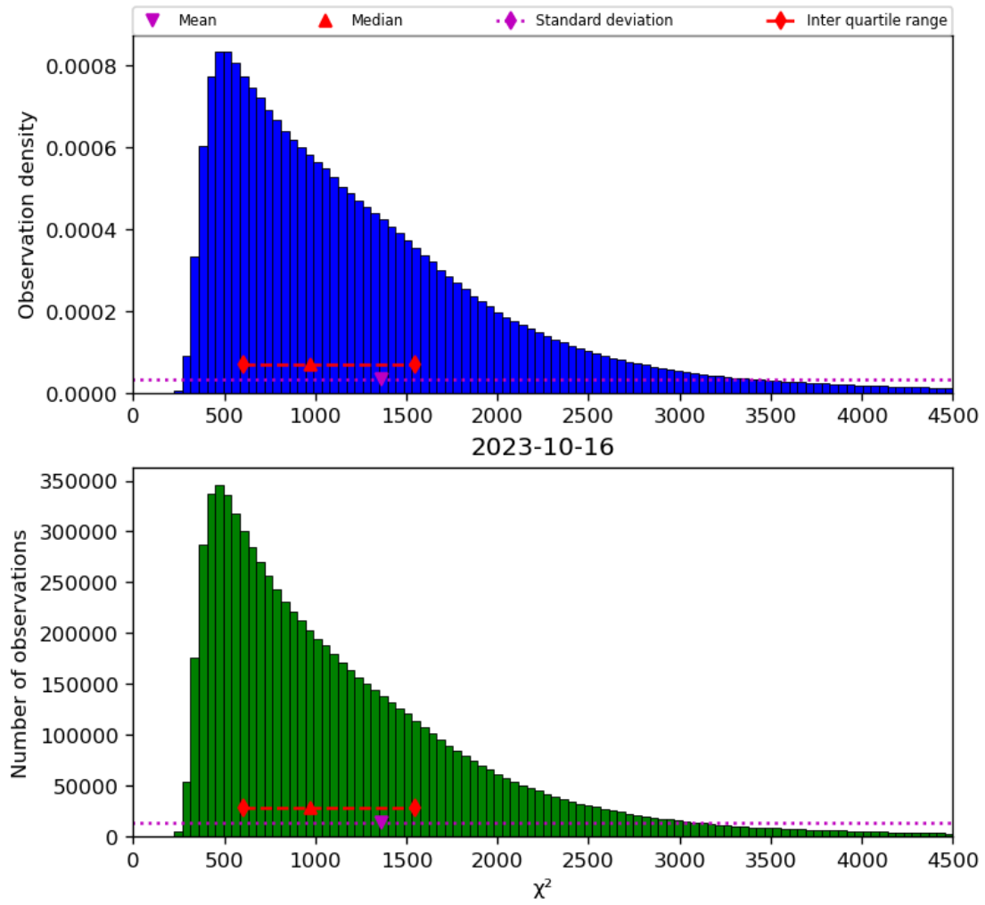
Figure 22: Histogram of “ \chi^2 ” for 2023-10-15 to 2023-10-17
