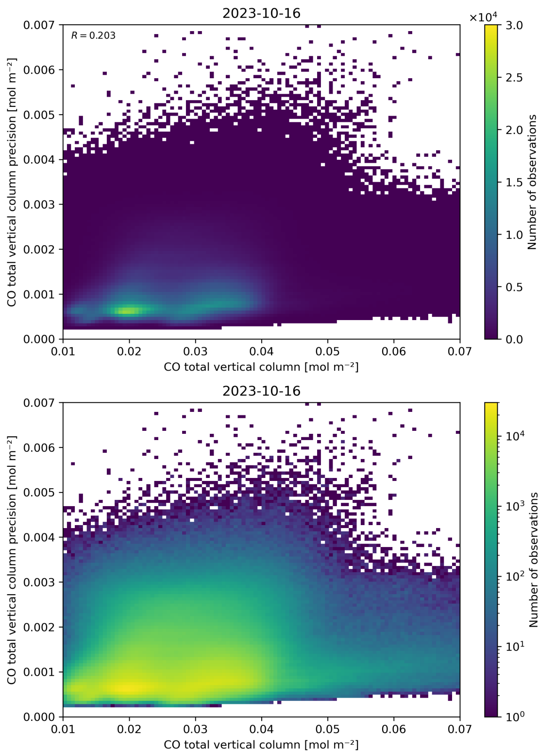
Figure 34: Scatter density plot of “CO total vertical column” against “CO total vertical column precision” for 2023-10-15 to 2023-10-17.
