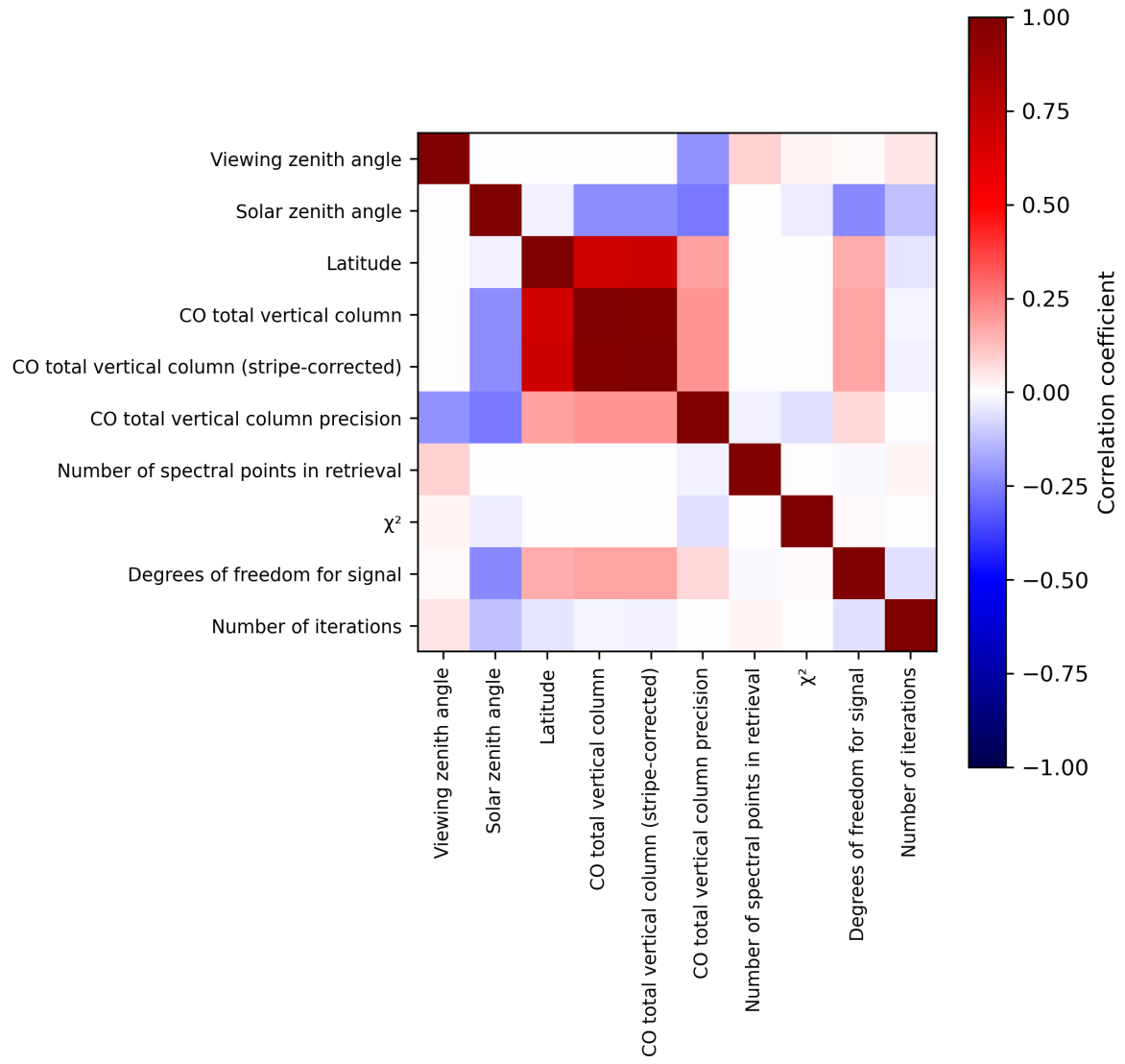
Figure 2: Map of correlation matrix for 2023-10-15 to 2023-10-17.
