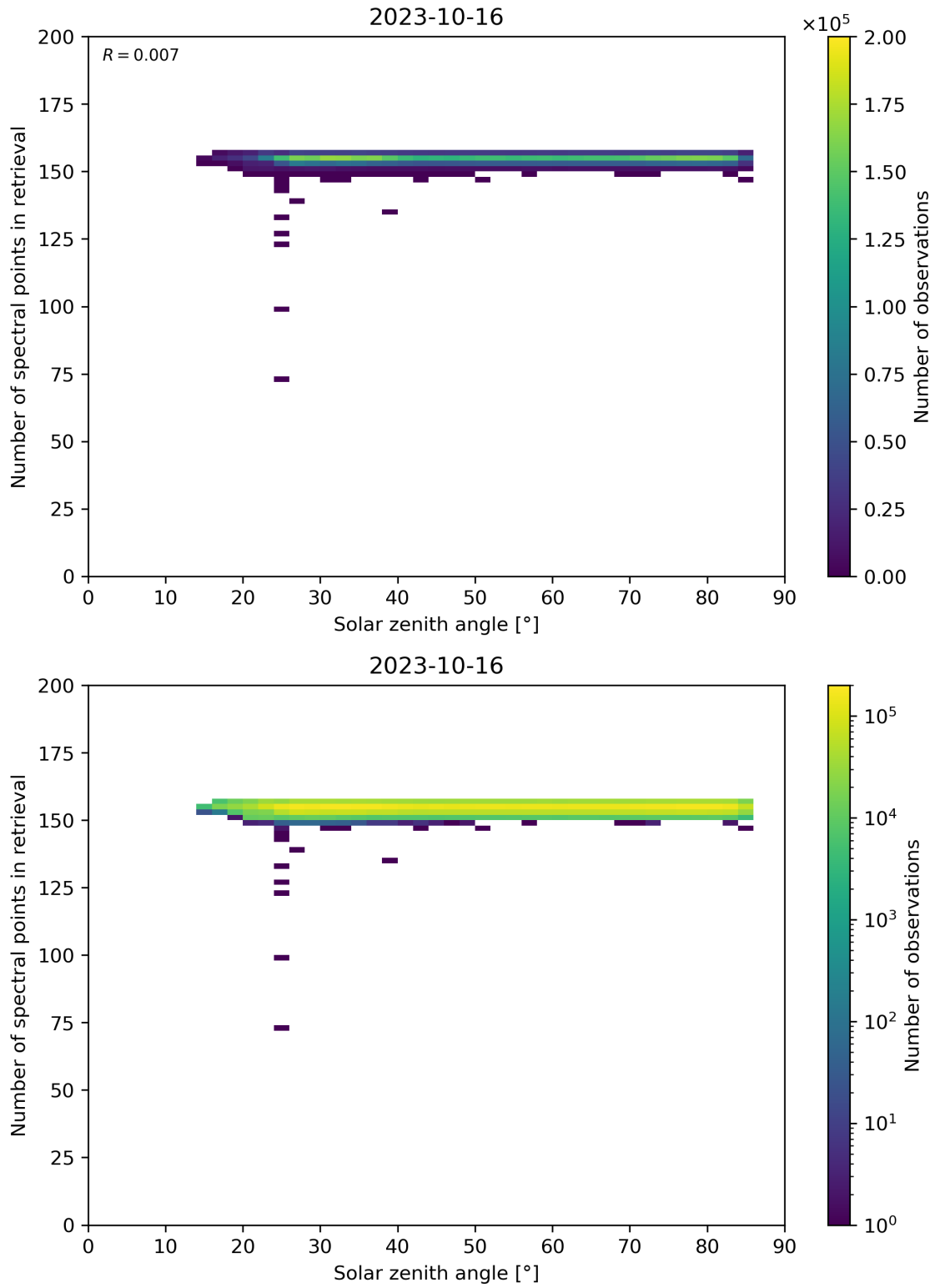
Figure 68: Scatter density plot of “Solar zenith angle” against “Number of spectral points in retrieval” for 2023-10-15 to 2023-10-17.
