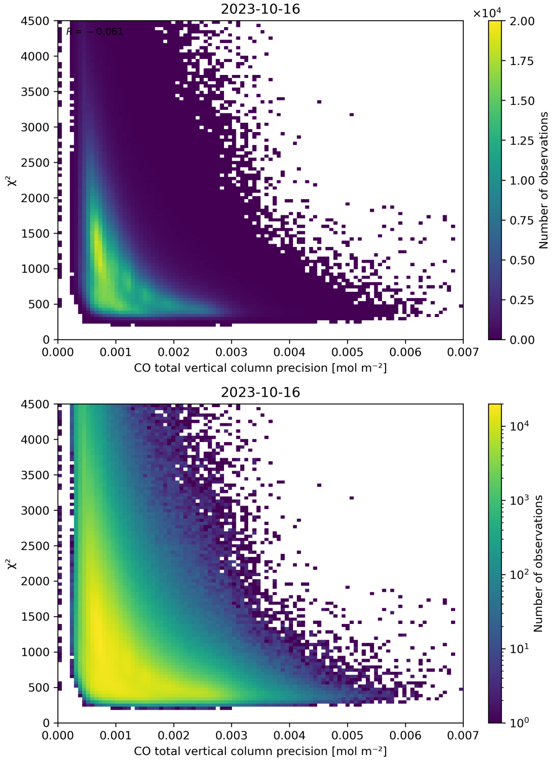
Figure 44: Scatter density plot of “CO total vertical column precision” against “ \chi^2 ” for 2023-10-15 to 2023-10-17.
