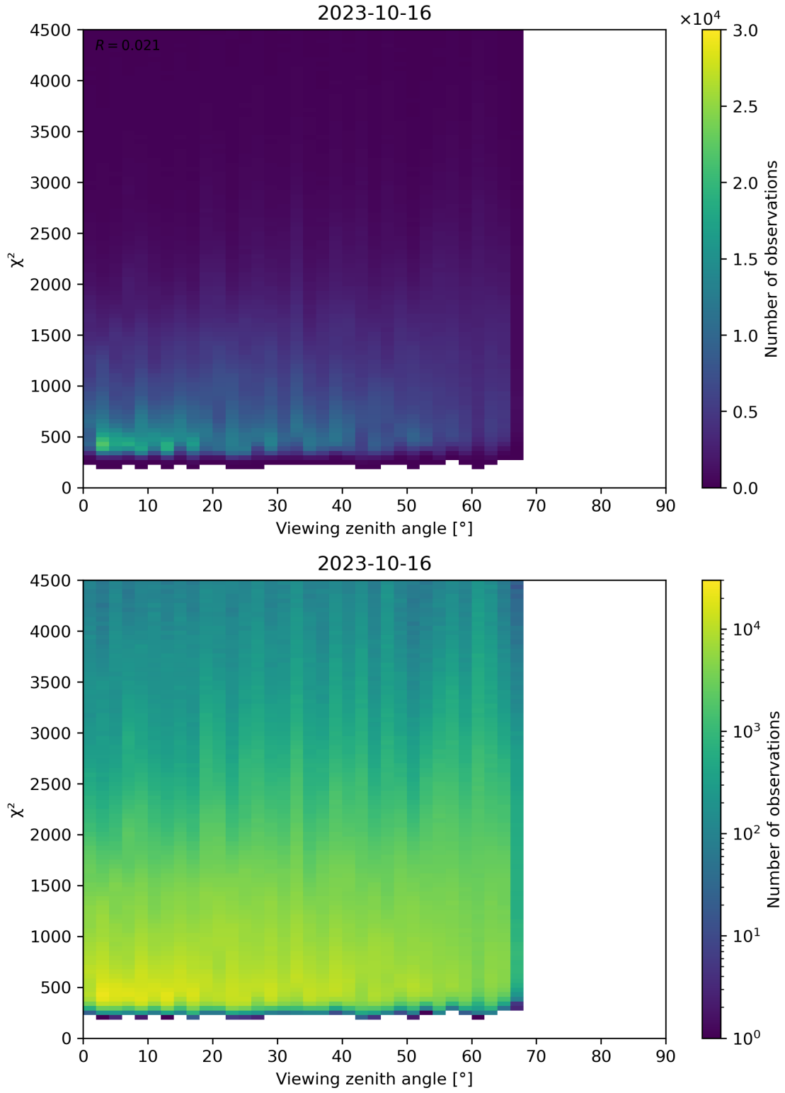
Figure 72: Scatter density plot of “Viewing zenith angle” against “ \chi^2 ” for 2023-10-15 to 2023-10-17.
