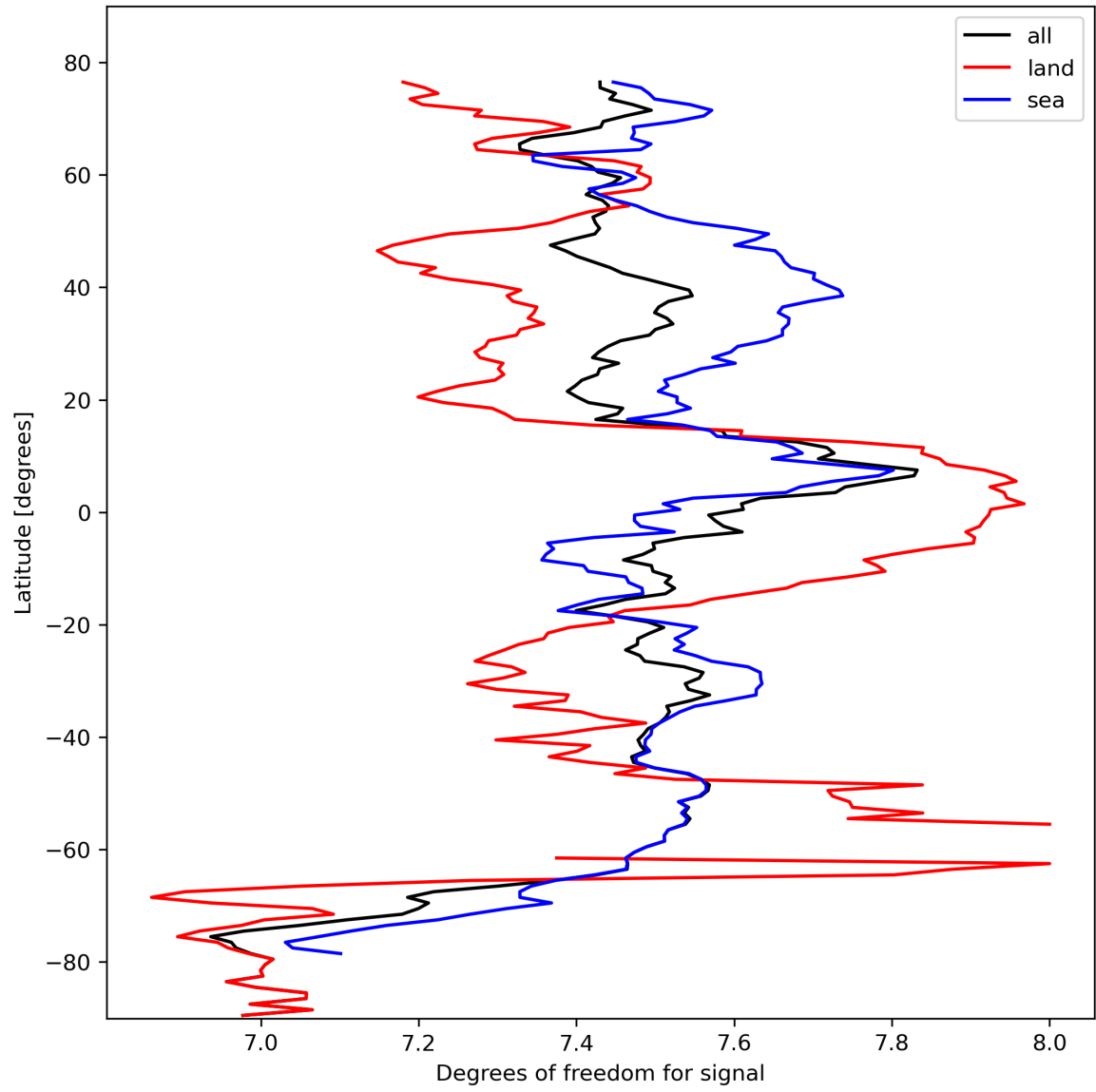
Figure 15: Zonal average of “Degrees of freedom for signal” for 2023-10-15 to 2023-10-17.
