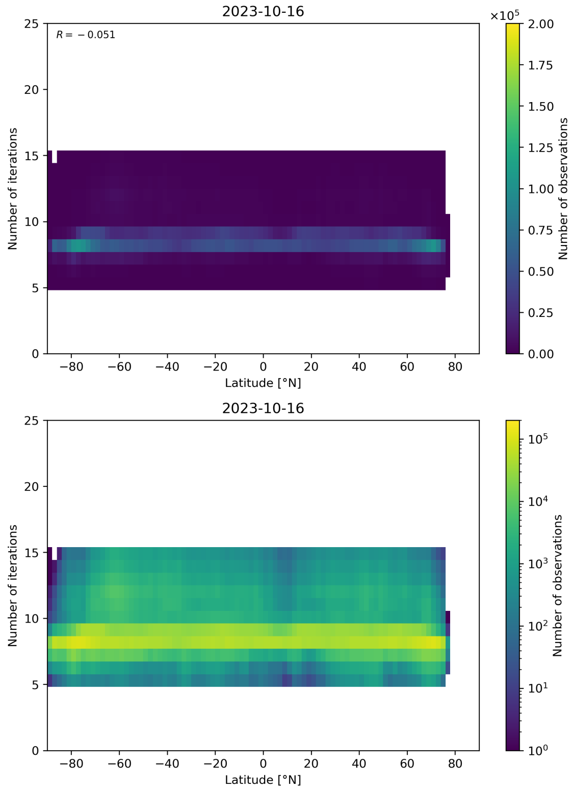
Figure 56: Scatter density plot of “Latitude” against “Number of iterations” for 2023-10-15 to 2023-10-17.
