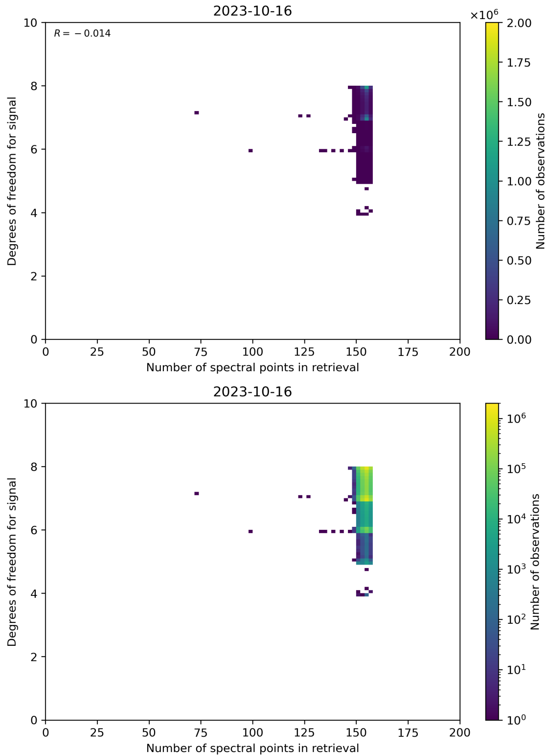
Figure 59: Scatter density plot of “Number of spectral points in retrieval” against “Degrees of freedom for signal” for 2023-10-15 to 2023-10-17.
