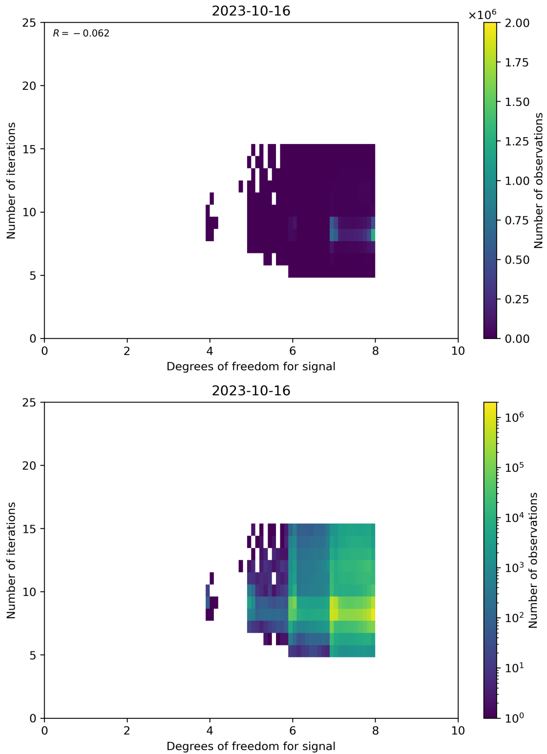
Figure 50: Scatter density plot of “Degrees of freedom for signal” against “Number of iterations” for 2023-10-15 to 2023-10-17.
