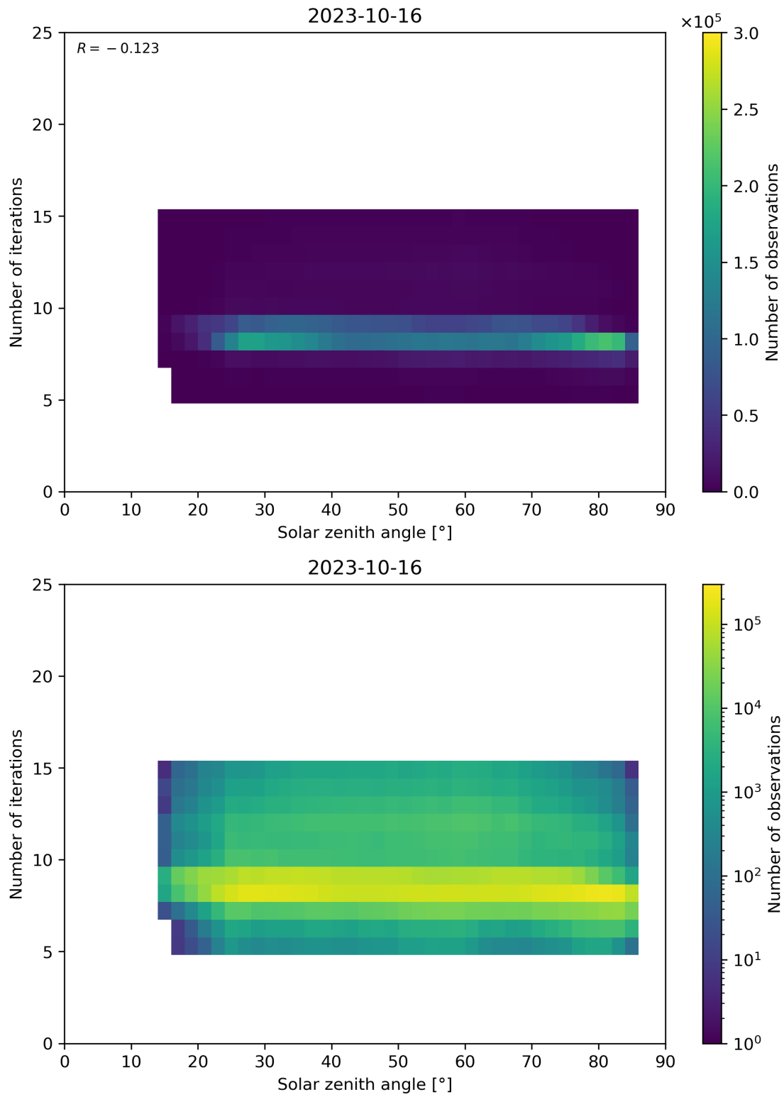
Figure 67: Scatter density plot of “Solar zenith angle” against “Number of iterations” for 2023-10-15 to 2023-10-17.
