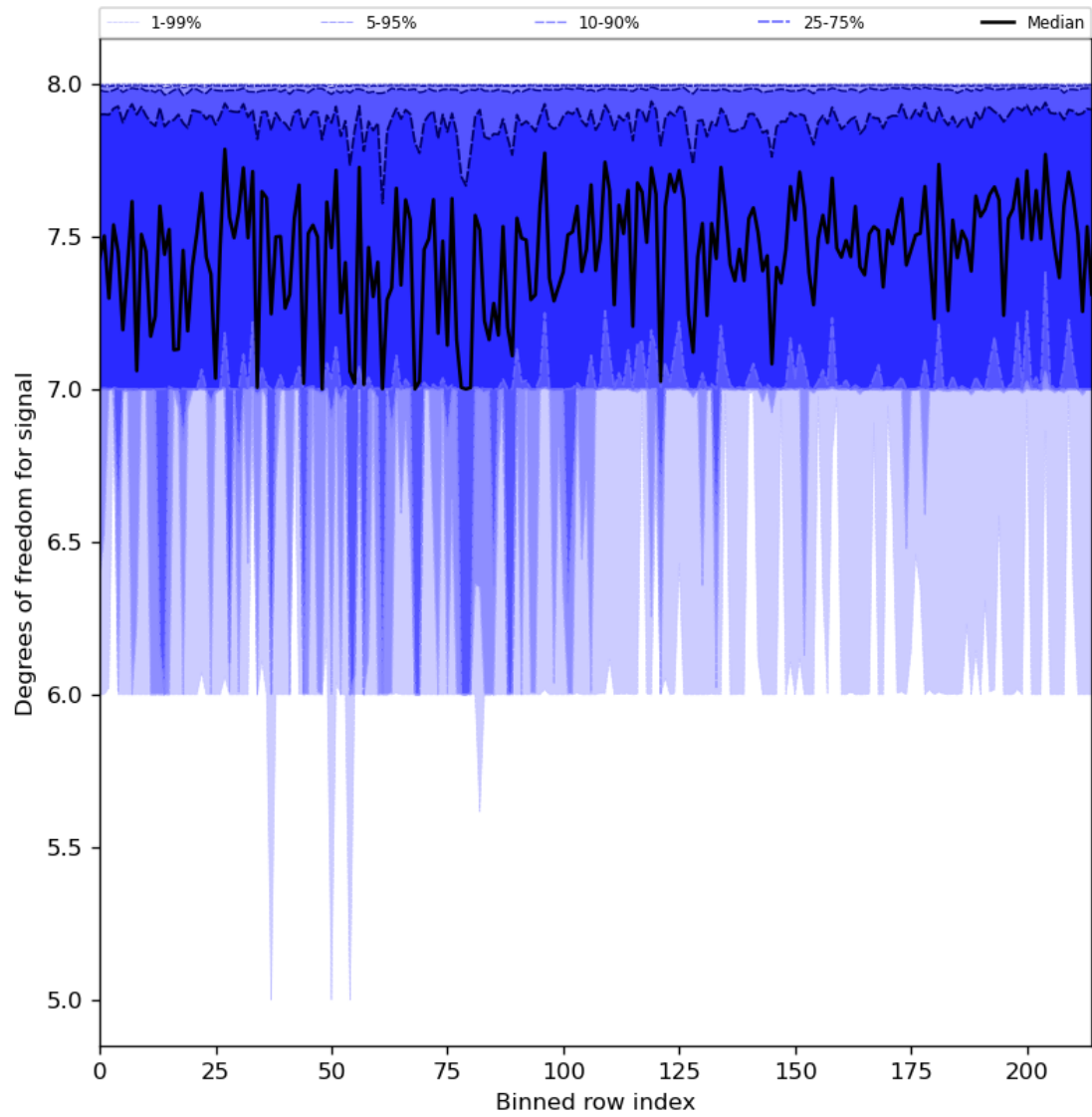
Figure 31: Along track statistics of “Degrees of freedom for signal” for 2023-10-15 to 2023-10-17
