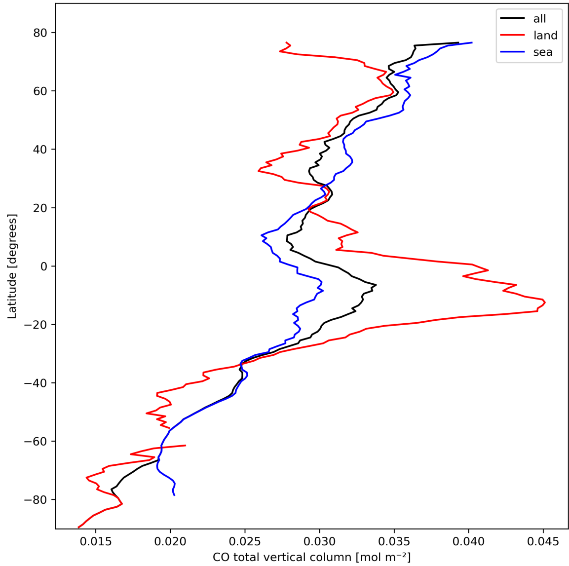
Figure 10: Zonal average of “CO total vertical column” for 2023-10-15 to 2023-10-17.
