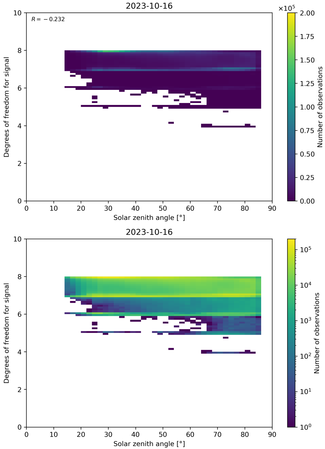
Figure 65: Scatter density plot of “Solar zenith angle” against “Degrees of freedom for signal” for 2023-10-15 to 2023-10-17.
