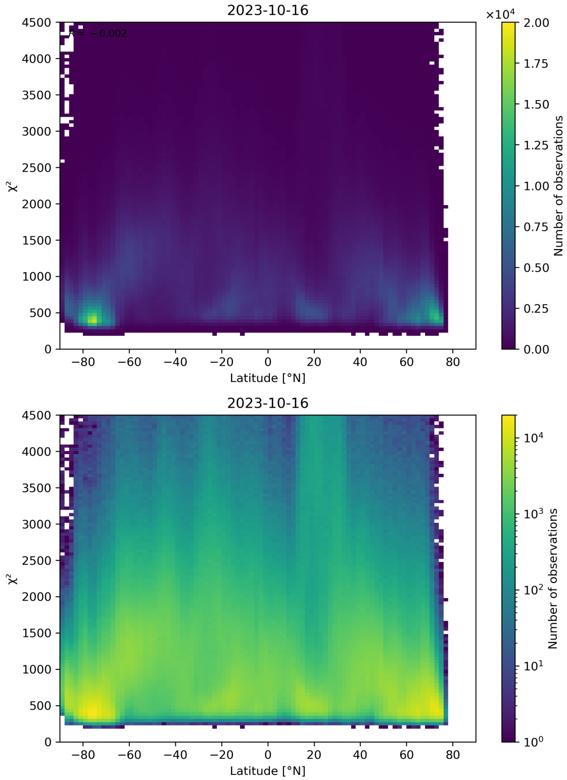
Figure 54: Scatter density plot of “Latitude” against “ \chi^2 ” for 2023-10-15 to 2023-10-17.
