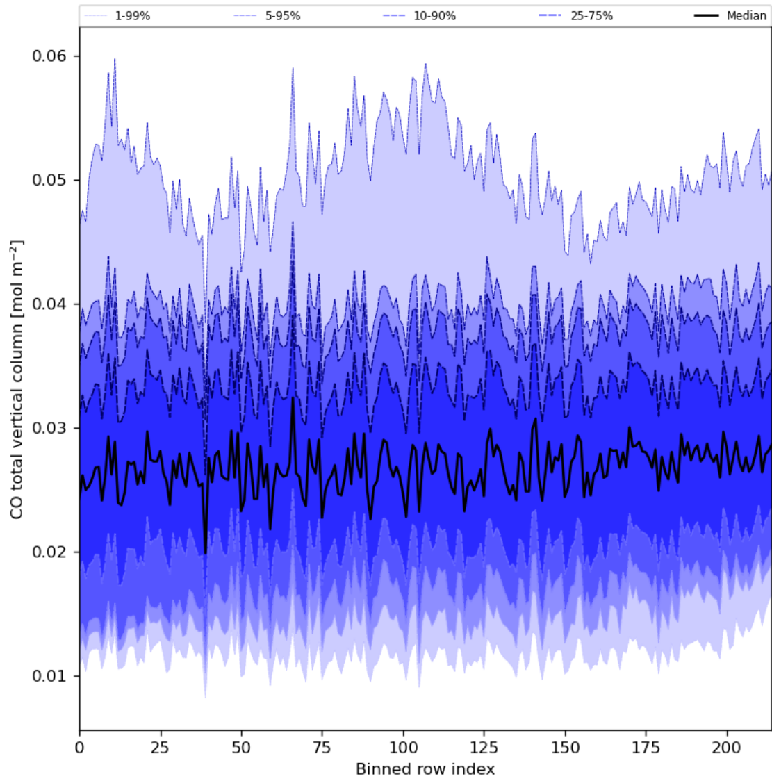
Figure 26: Along track statistics of “CO total vertical column” for 2023-10-15 to 2023-10-17
