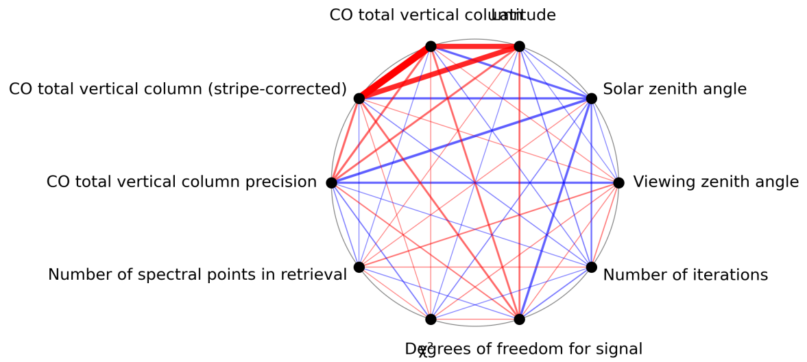
Figure 1: Map of correlation graph for 2023-10-15 to 2023-10-17.
