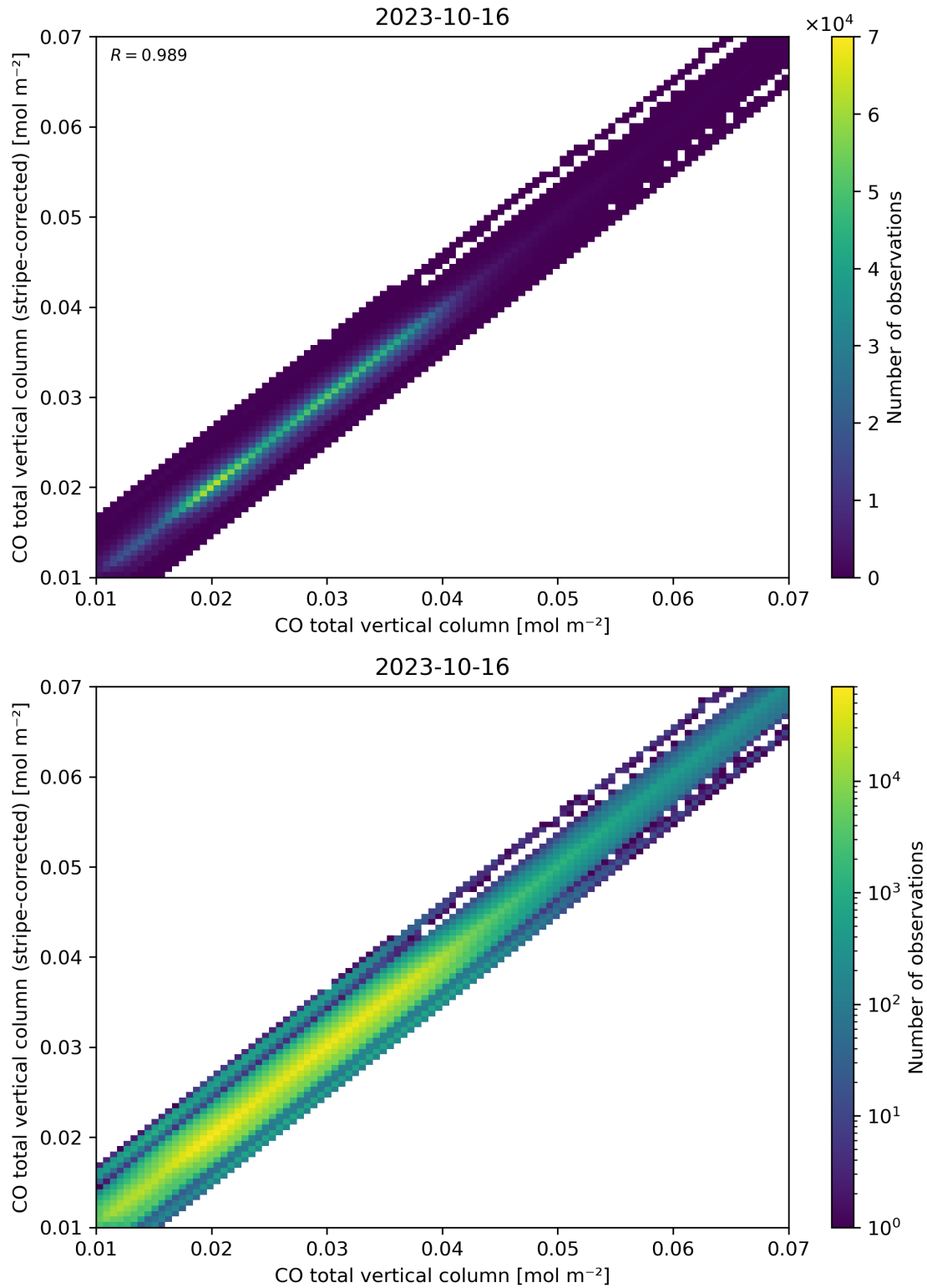
Figure 33: Scatter density plot of “CO total vertical column” against “CO total vertical column (stripe-corrected)” for 2023-10-15 to 2023-10-17.
