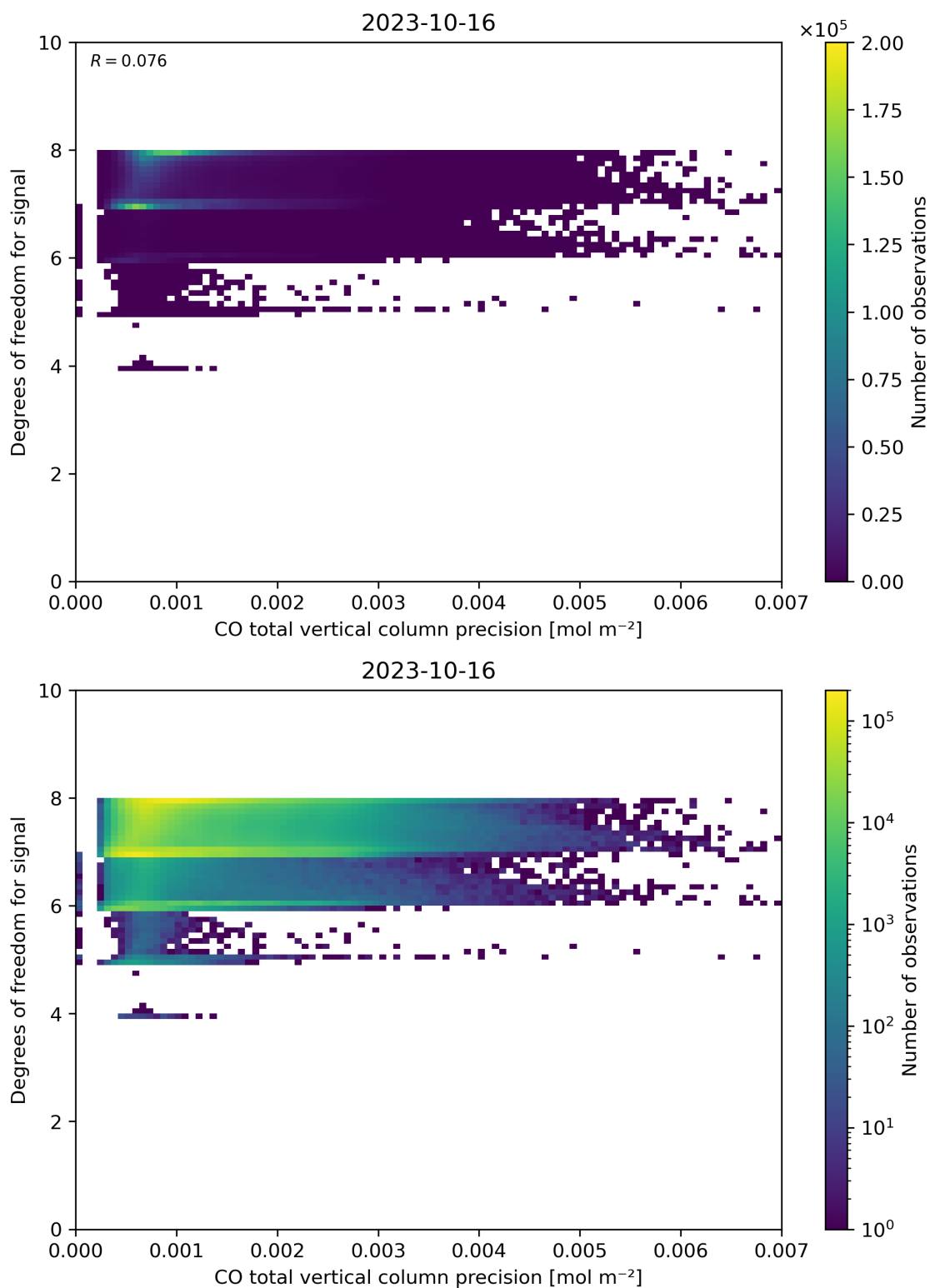
Figure 45: Scatter density plot of “CO total vertical column precision” against “Degrees of freedom for signal” for 2023-10-15 to 2023-10-17.
