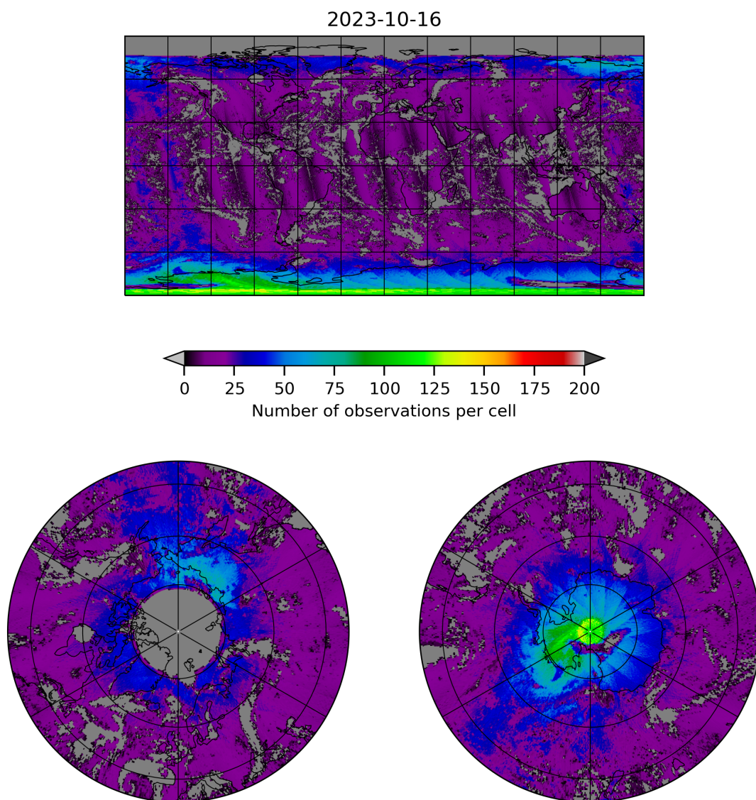
Figure 8: Map of the number of observations for 2023-10-15 to 2023-10-17
