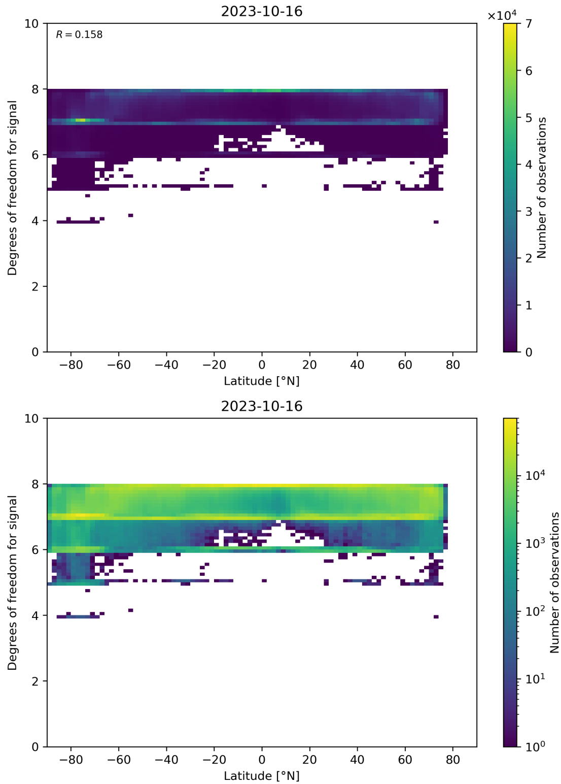
Figure 55: Scatter density plot of “Latitude” against “Degrees of freedom for signal” for 2023-10-15 to 2023-10-17.
