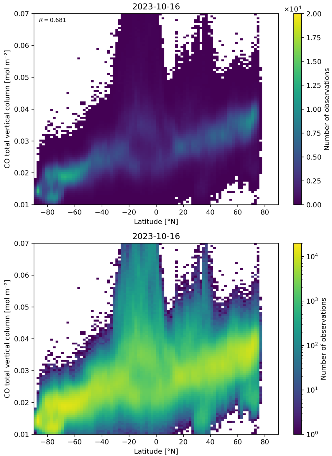
Figure 51: Scatter density plot of “Latitude” against “CO total vertical column” for 2023-10-15 to 2023-10-17.
