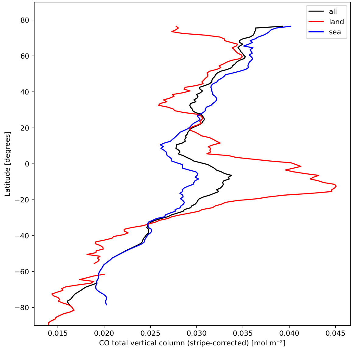
Figure 11: Zonal average of “CO total vertical column (stripe-corrected)” for 2023-10-15 to 2023-10-17.
