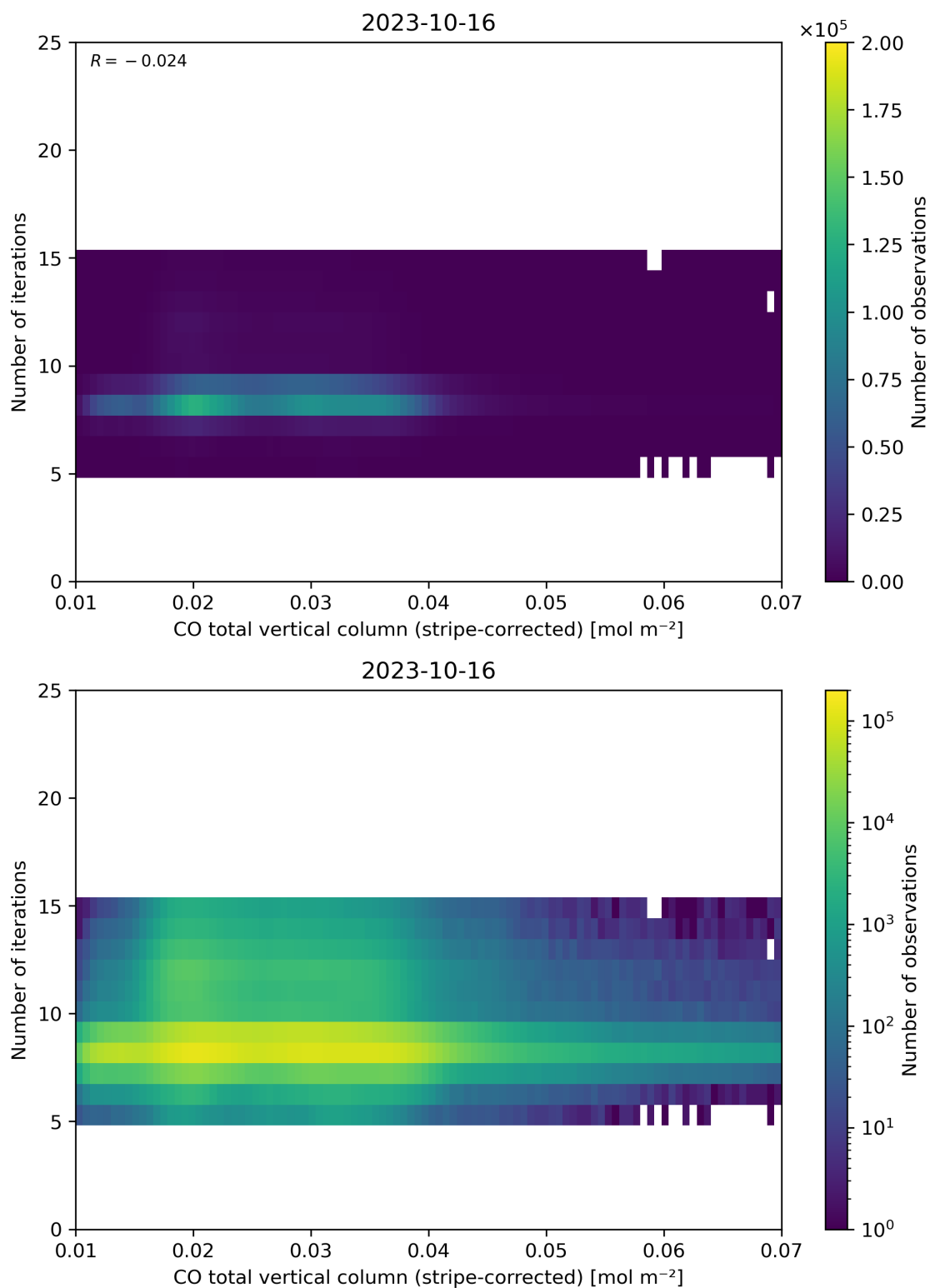
Figure 39: Scatter density plot of “CO total vertical column (stripe-corrected)” against “Number of iterations” for 2023-10-15 to 2023-10-17.
