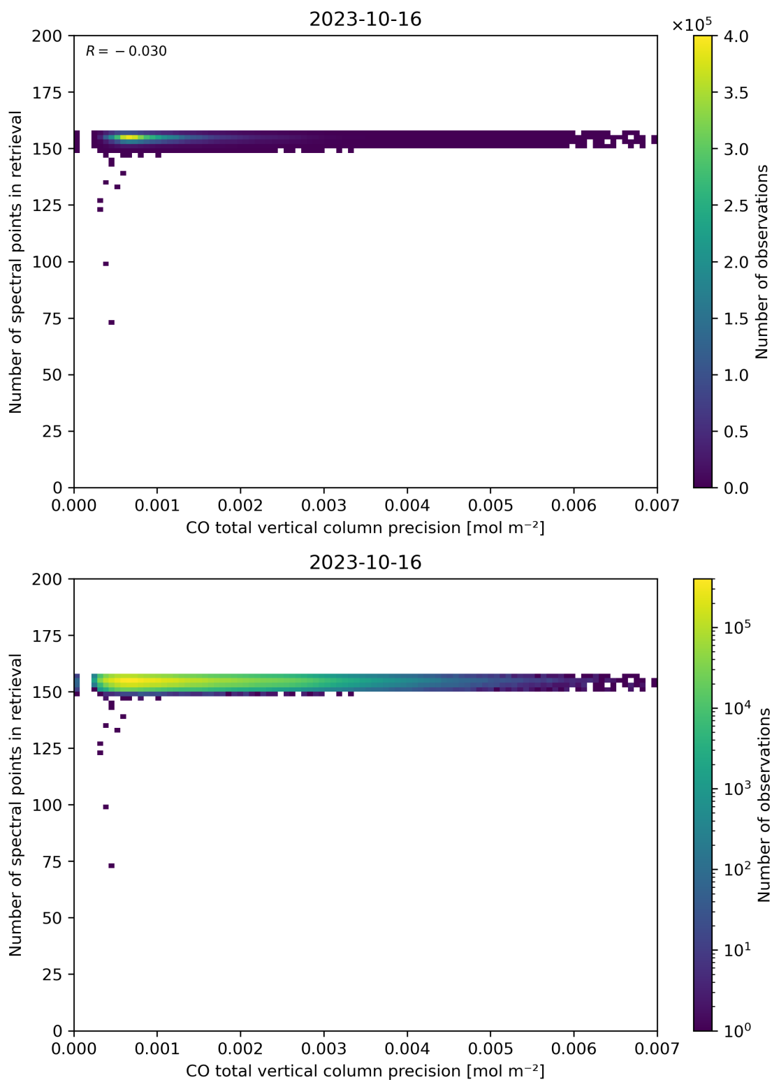
Figure 47: Scatter density plot of “CO total vertical column precision” against “Number of spectral points in retrieval” for 2023-10-15 to 2023-10-17.
