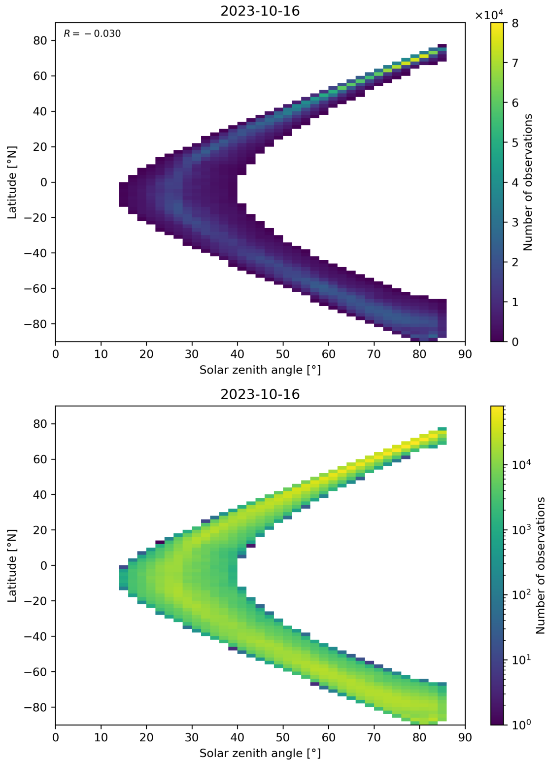
Figure 66: Scatter density plot of “Solar zenith angle” against “Latitude” for 2023-10-15 to 2023-10-17.
