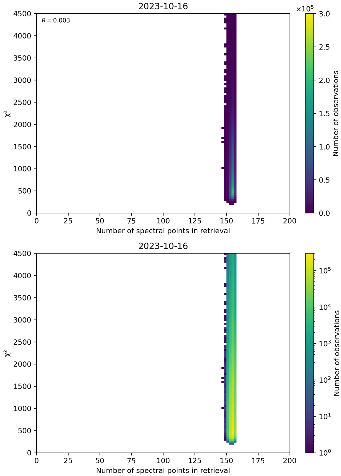
Figure 58: Scatter density plot of “Number of spectral points in retrieval” against “ \chi^2 ” for 2023-10-15 to 2023-10-17.
