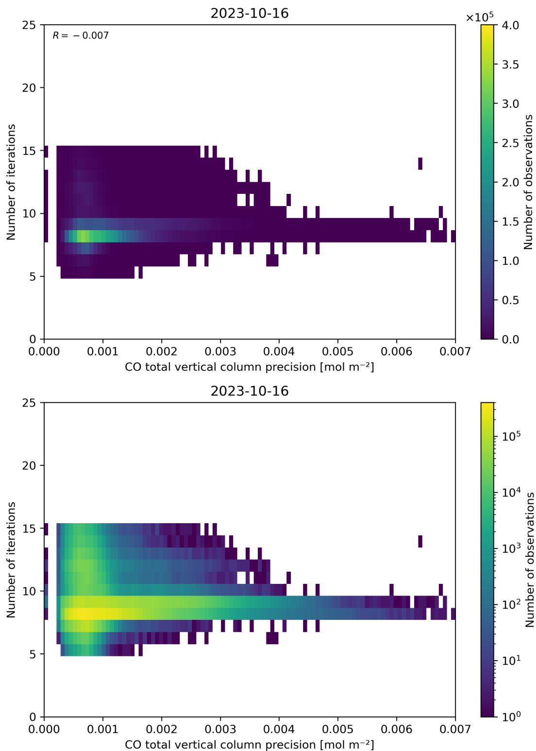
Figure 46: Scatter density plot of “CO total vertical column precision” against “Number of iterations” for 2023-10-15 to 2023-10-17.
