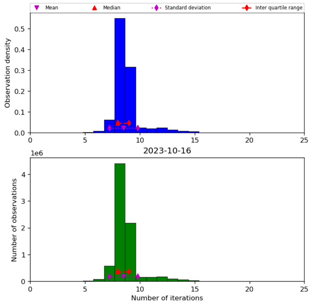
Figure 24: Histogram of “Number of iterations” for 2023-10-15 to 2023-10-17
