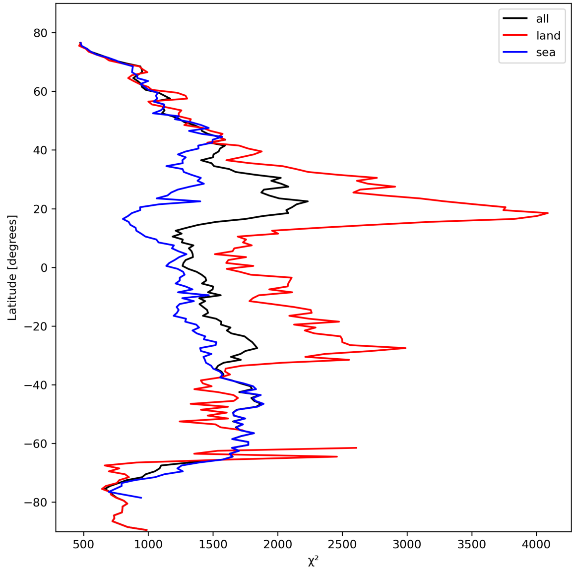
Figure 14: Zonal average of “ \chi^2 ” for 2023-10-15 to 2023-10-17.
