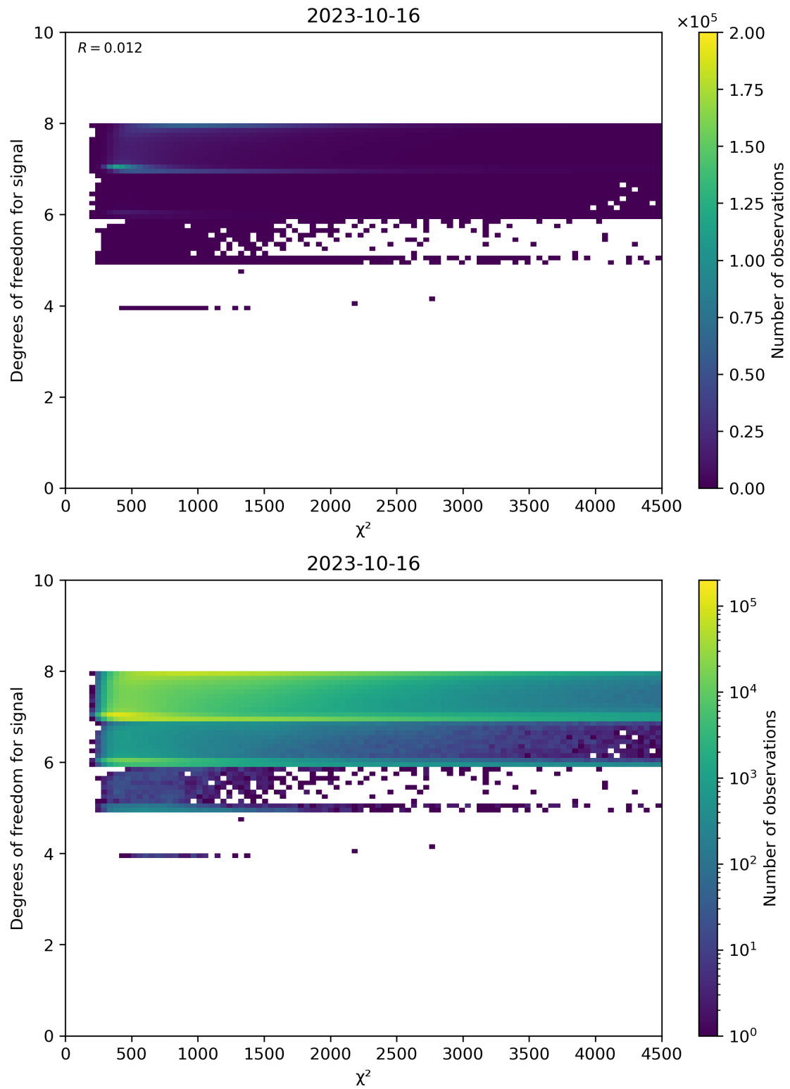
Figure 48: Scatter density plot of “ \chi^2 ” against “Degrees of freedom for signal” for 2023-10-15 to 2023-10-17.
