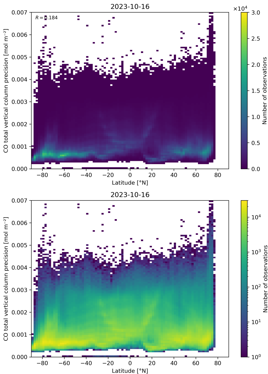
Figure 53: Scatter density plot of “Latitude” against “CO total vertical column precision” for 2023-10-15 to 2023-10-17.
