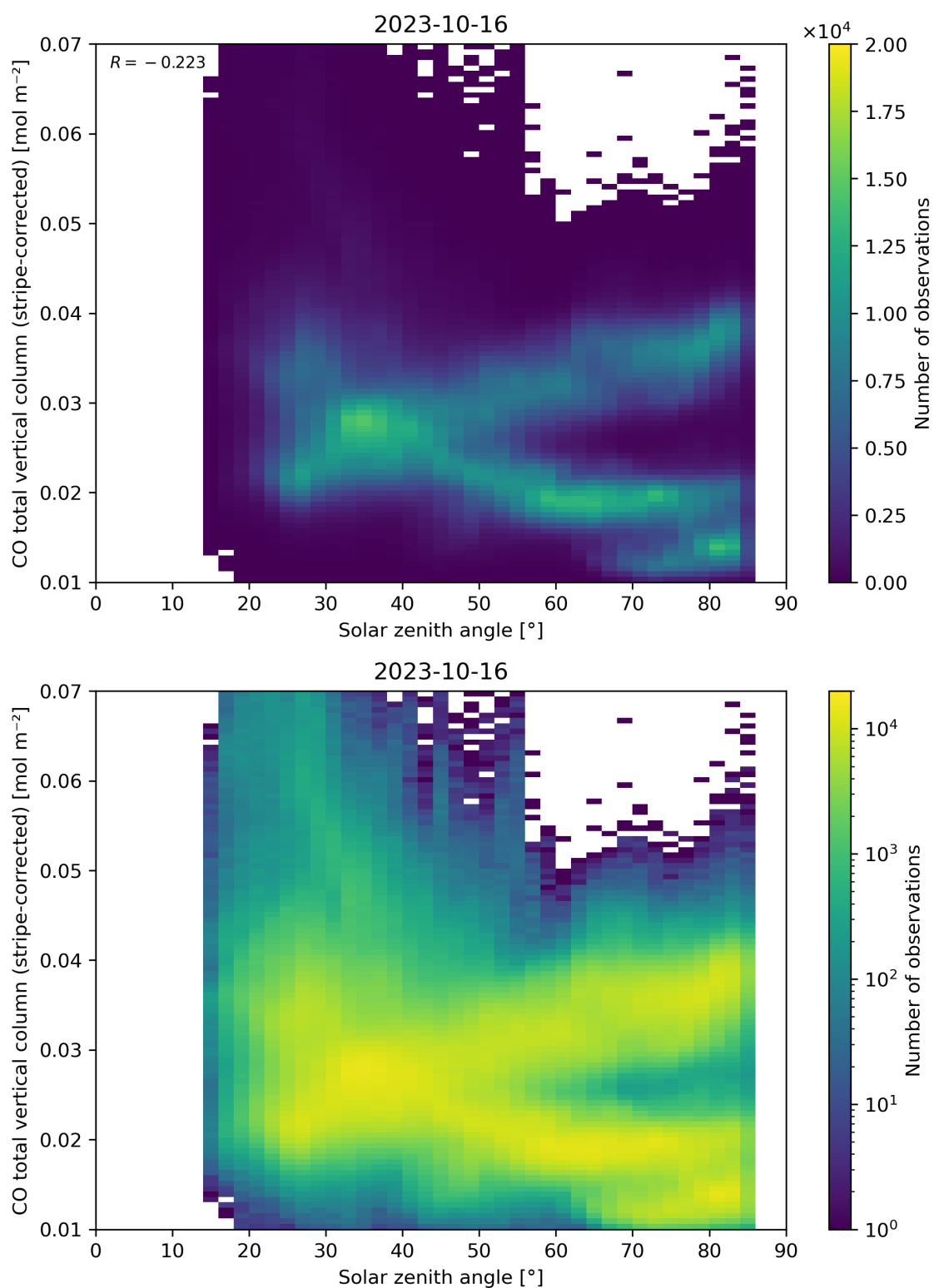
Figure 62: Scatter density plot of “Solar zenith angle” against “CO total vertical column (stripe-corrected)” for 2023-10-15 to 2023-10-17.
