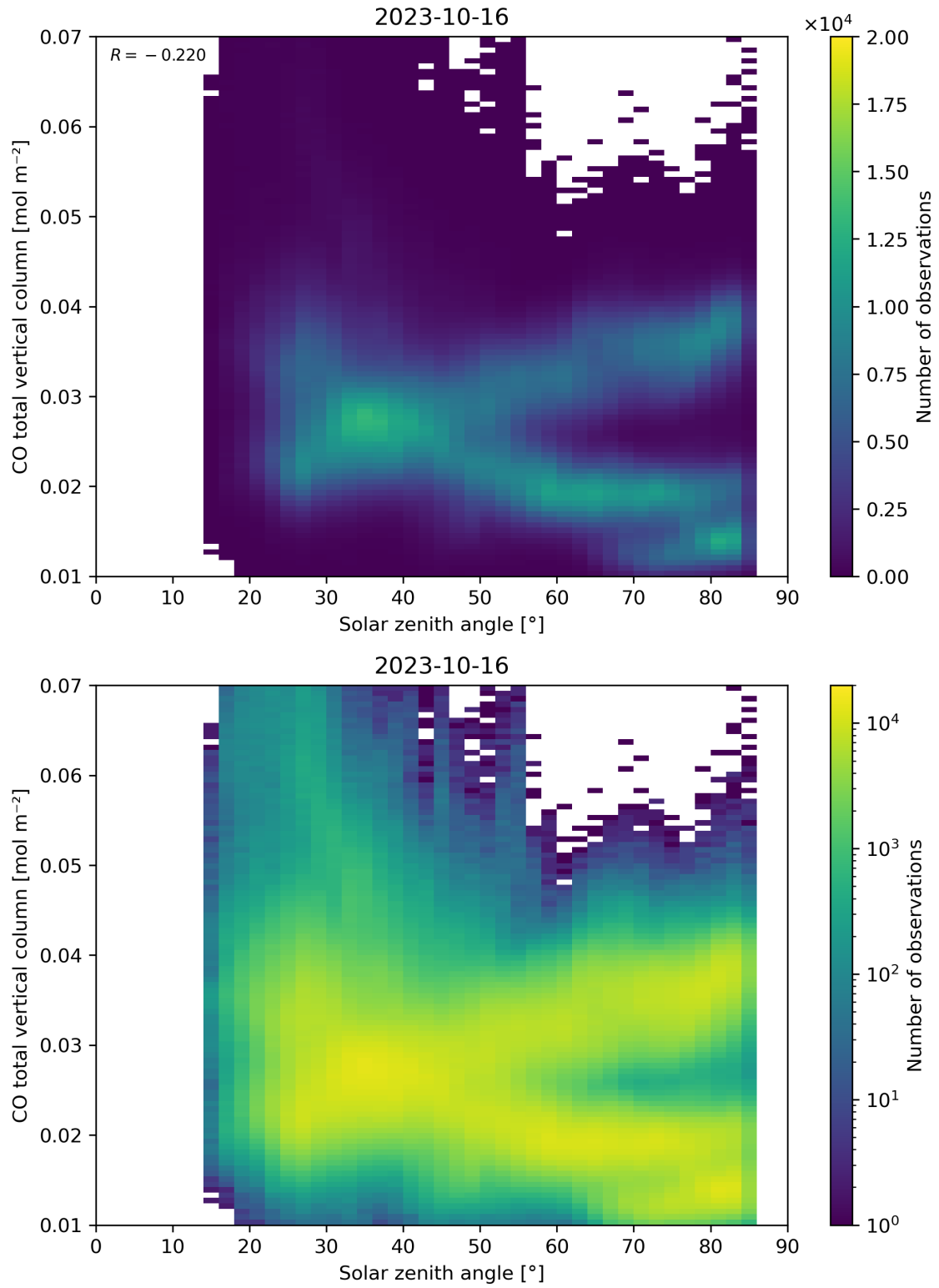
Figure 61: Scatter density plot of “Solar zenith angle” against “CO total vertical column” for 2023-10-15 to 2023-10-17.
