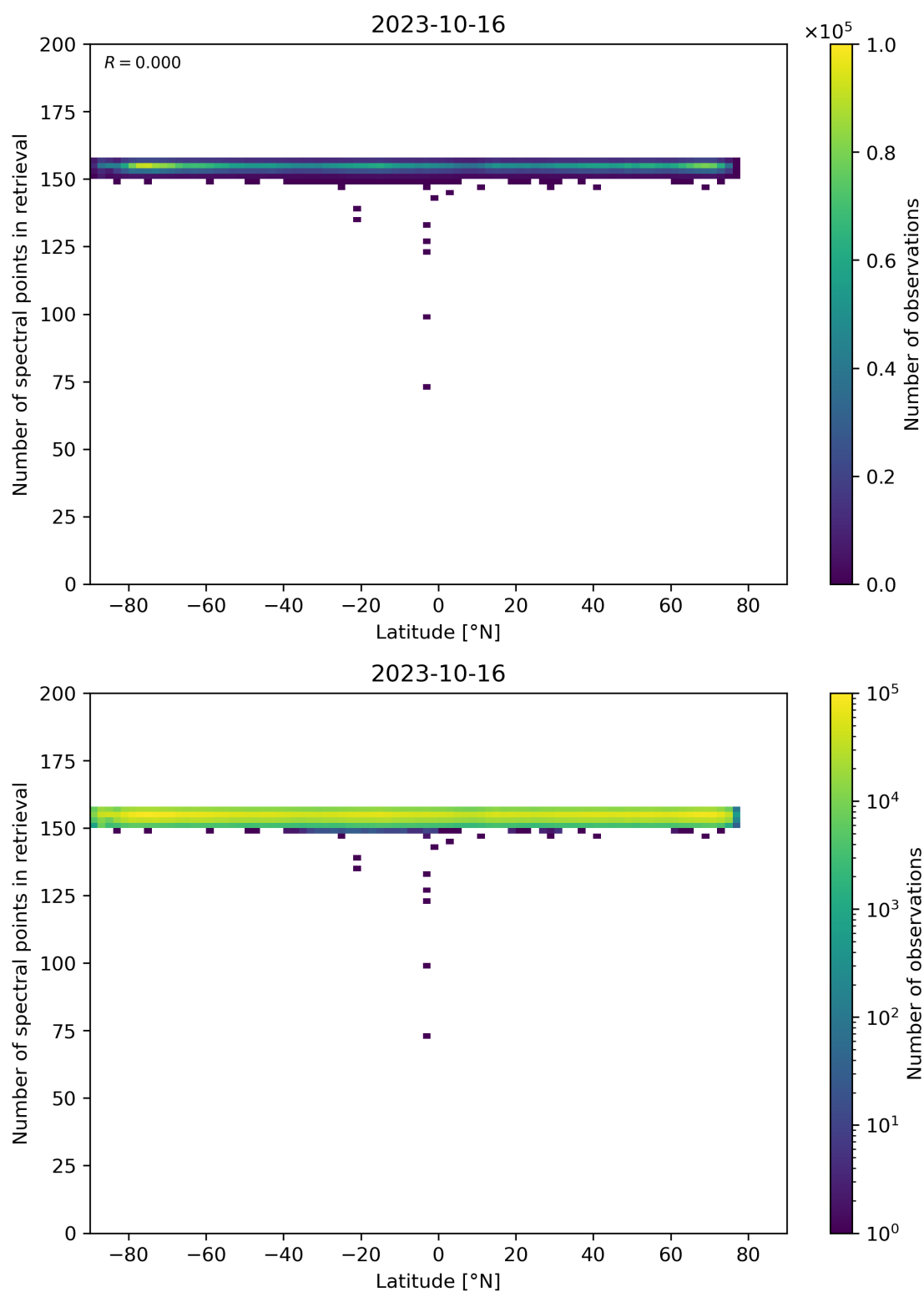
Figure 57: Scatter density plot of “Latitude” against “Number of spectral points in retrieval” for 2023-10-15 to 2023-10-17.
