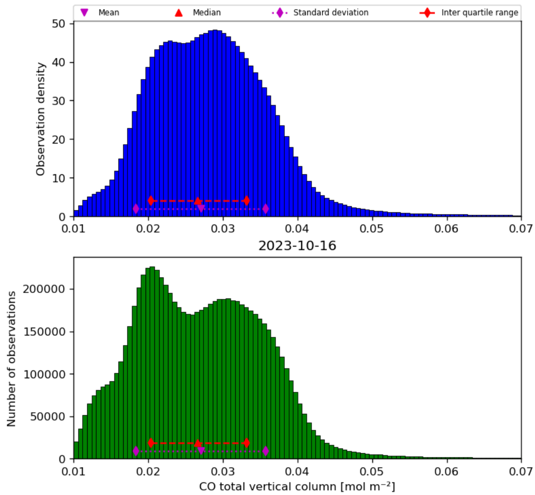
Figure 18: Histogram of “CO total vertical column” for 2023-10-15 to 2023-10-17
