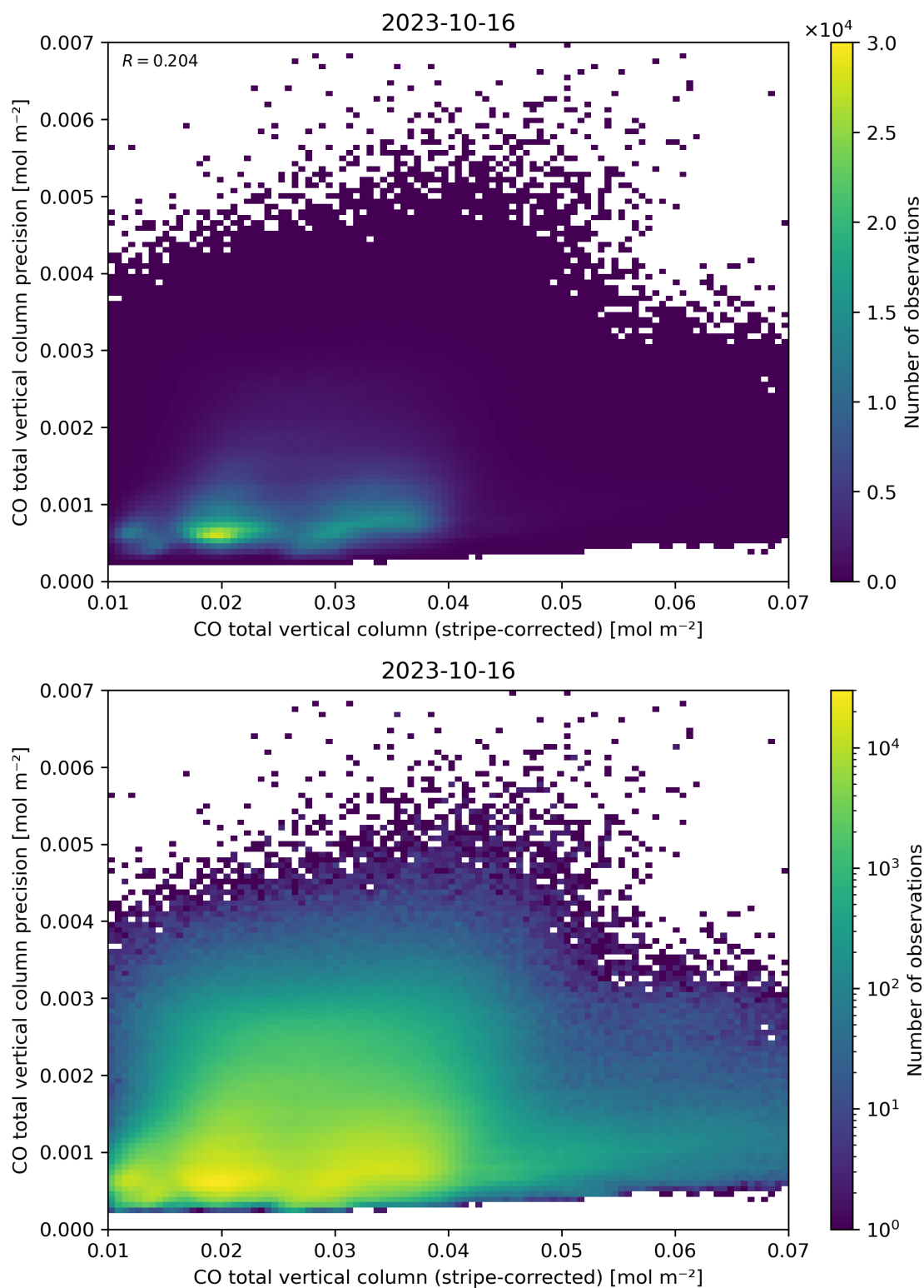
Figure 36: Scatter density plot of “CO total vertical column (stripe-corrected)” against “CO total vertical column precision” for 2023-10-15 to 2023-10-17.
