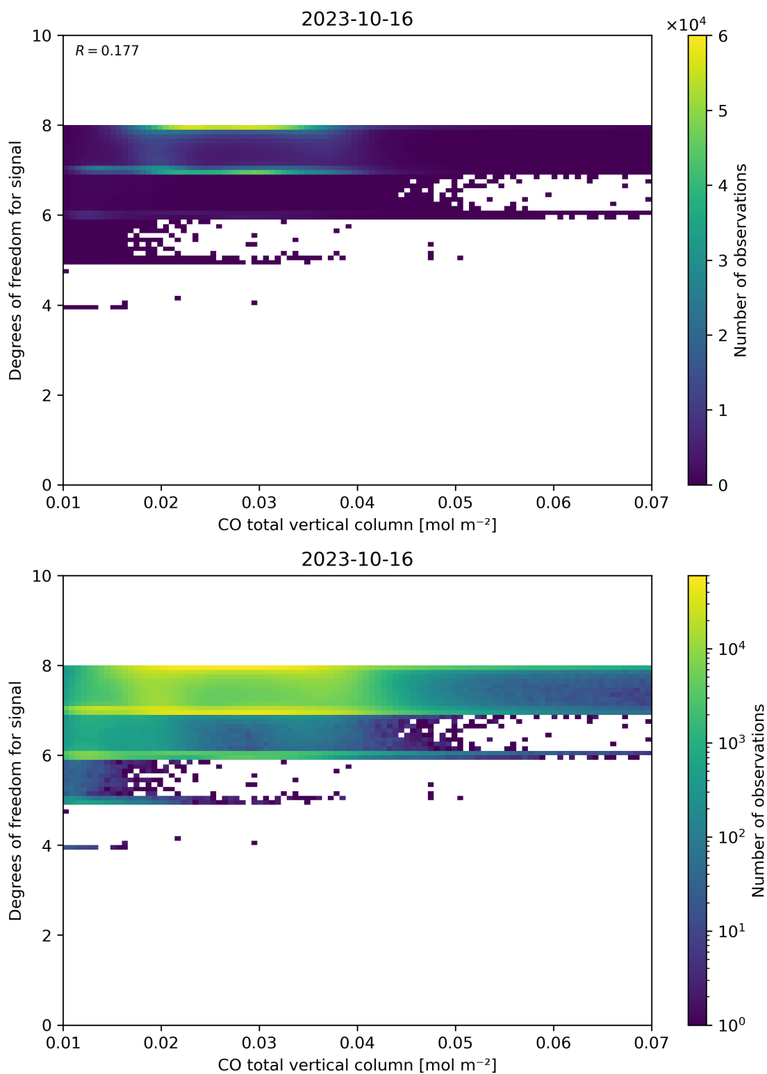
Figure 41: Scatter density plot of “CO total vertical column” against “Degrees of freedom for signal” for 2023-10-15 to 2023-10-17.
