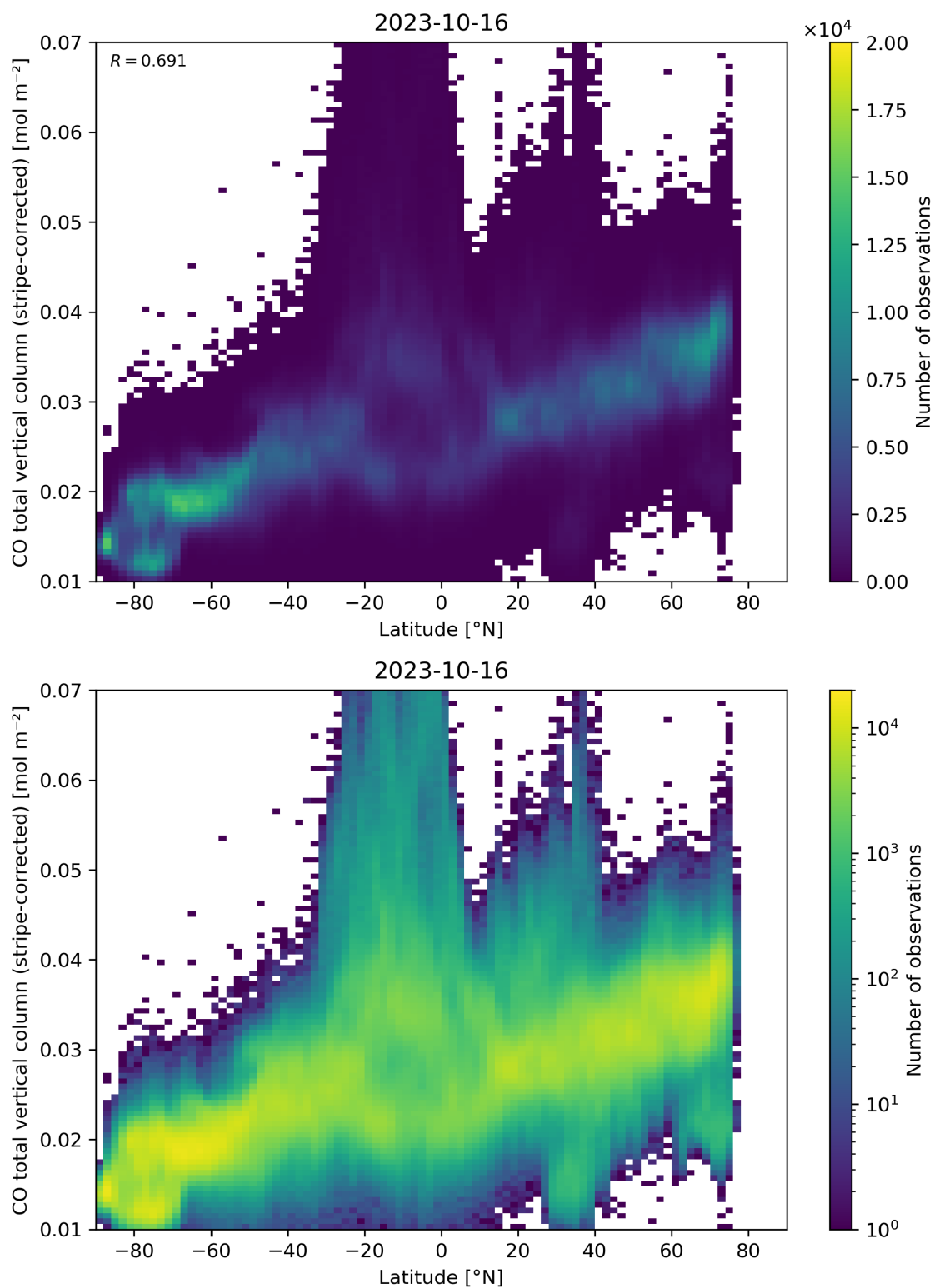
Figure 52: Scatter density plot of “Latitude” against “CO total vertical column (stripe-corrected)” for 2023-10-15 to 2023-10-17.
