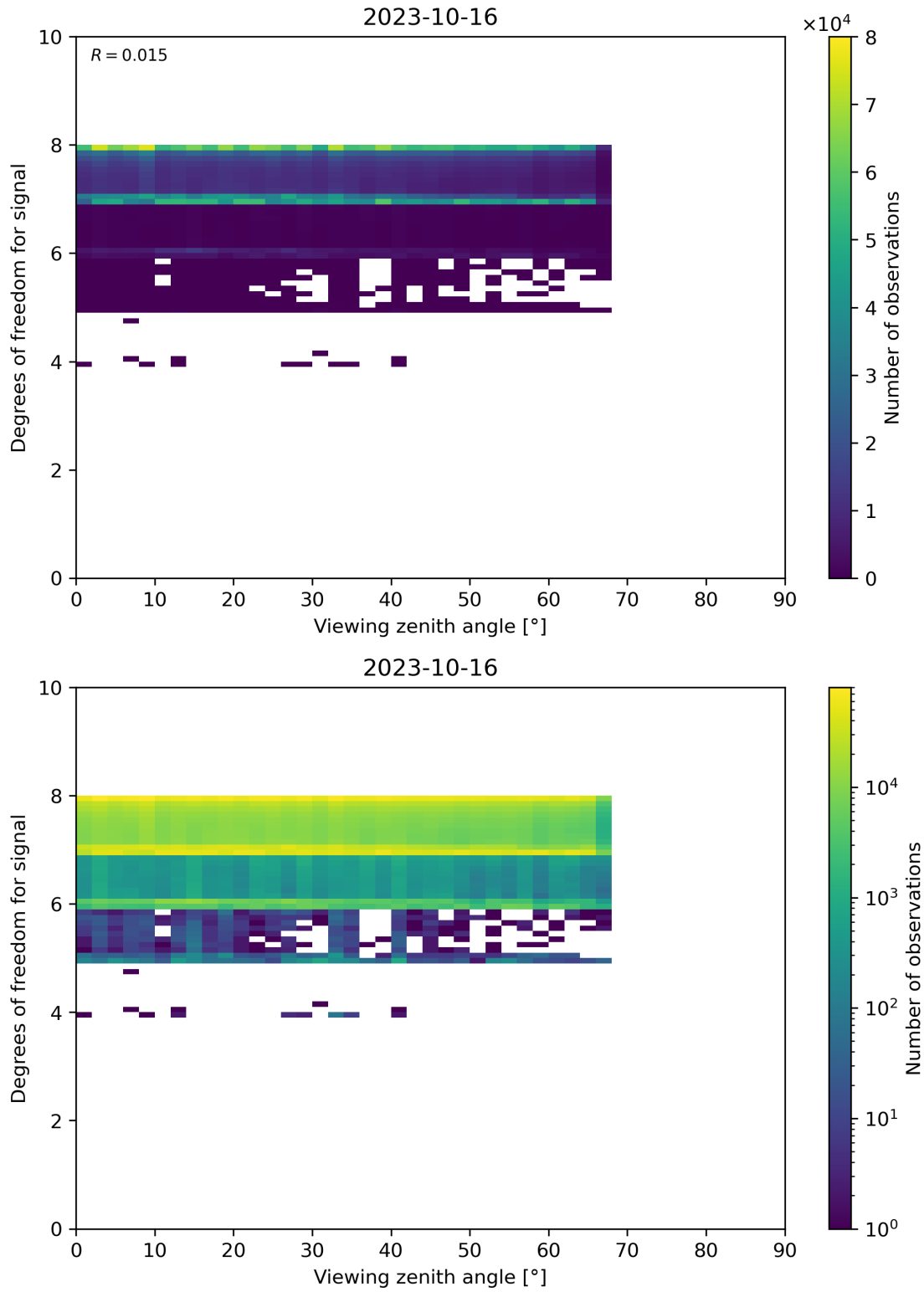
Figure 73: Scatter density plot of “Viewing zenith angle” against “Degrees of freedom for signal” for 2023-10-15 to 2023-10-17.
