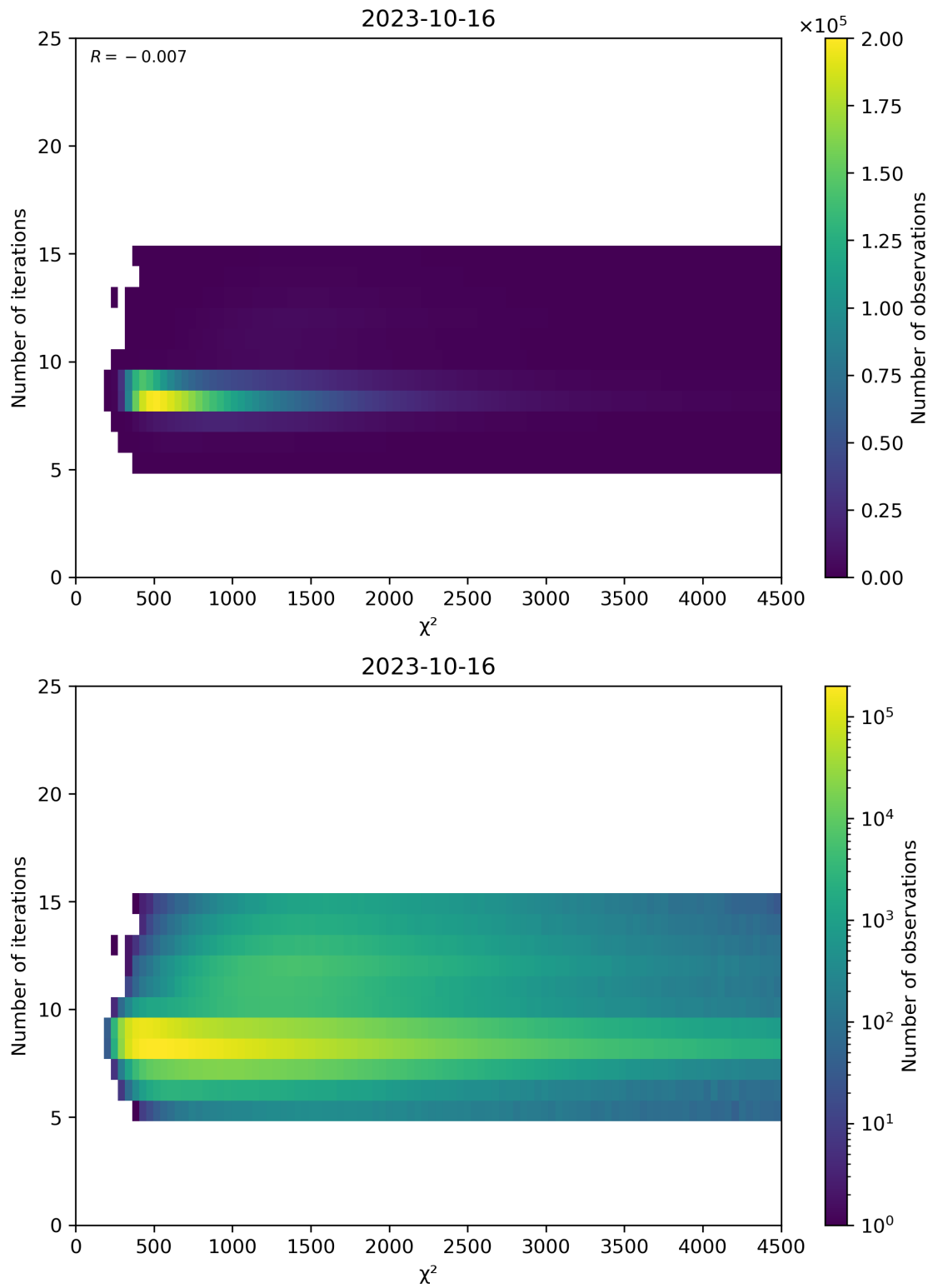
Figure 49: Scatter density plot of “ \chi^2 ” against “Number of iterations” for 2023-10-15 to 2023-10-17.
