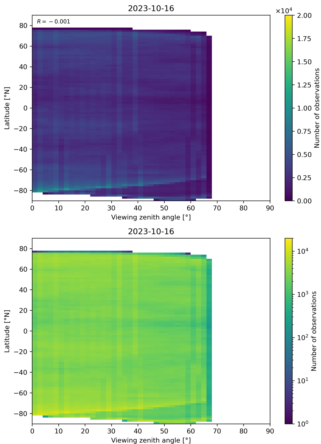
Figure 74: Scatter density plot of “Viewing zenith angle” against “Latitude” for 2023-10-15 to 2023-10-17.
