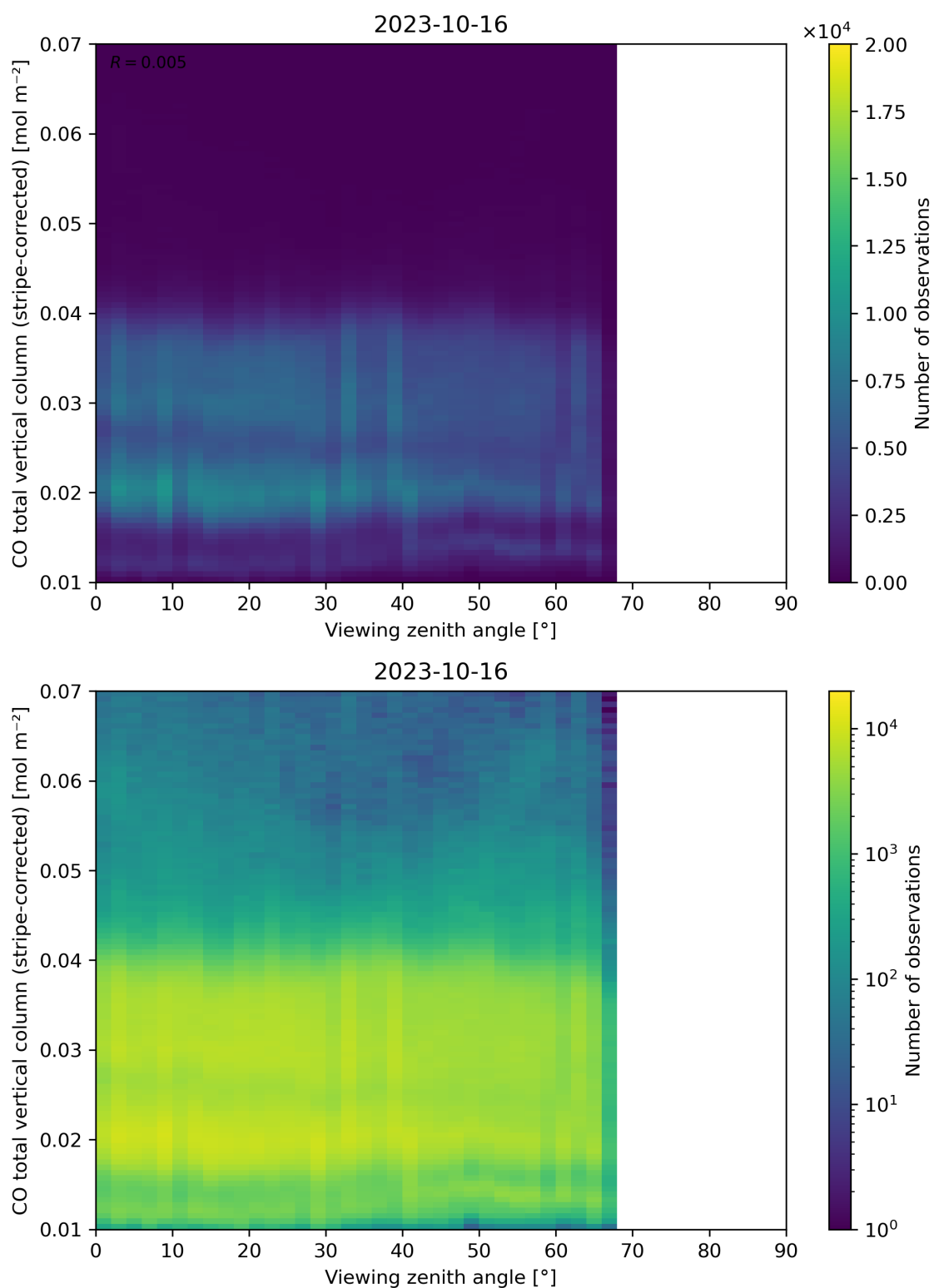
Figure 70: Scatter density plot of “Viewing zenith angle” against “CO total vertical column (stripe-corrected)” for 2023-10-15 to 2023-10-17.
