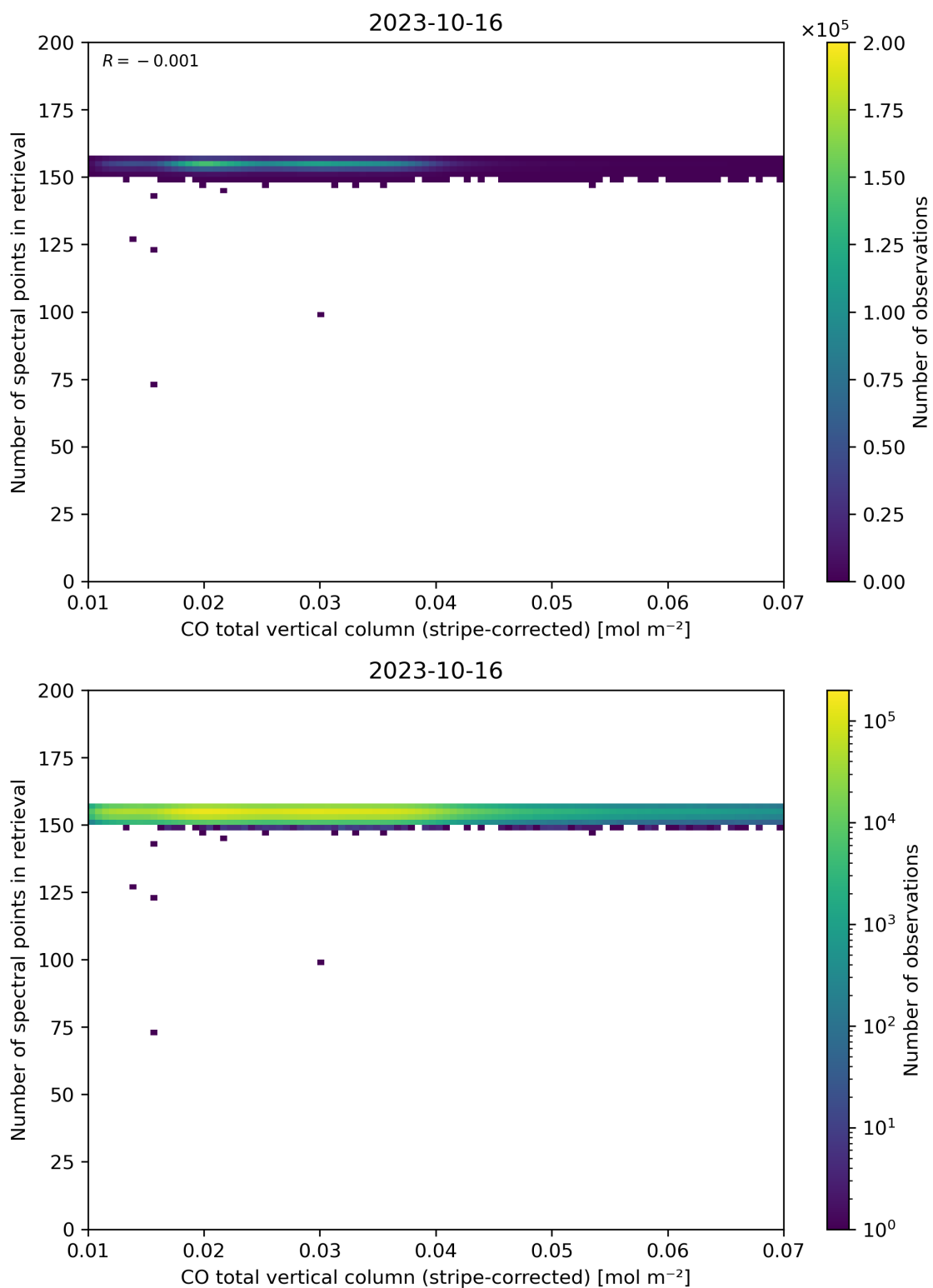
Figure 40: Scatter density plot of “CO total vertical column (stripe-corrected)” against “Number of spectral points in retrieval” for 2023-10-15 to 2023-10-17.
