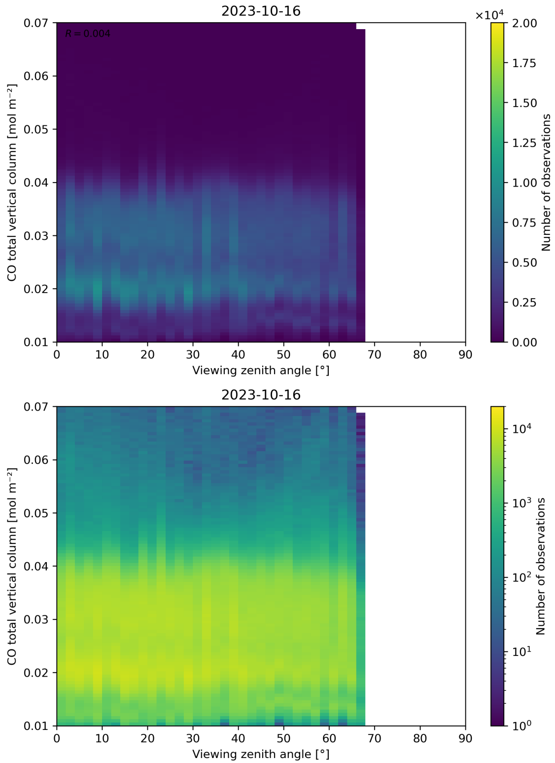
Figure 69: Scatter density plot of “Viewing zenith angle” against “CO total vertical column” for 2023-10-15 to 2023-10-17.
