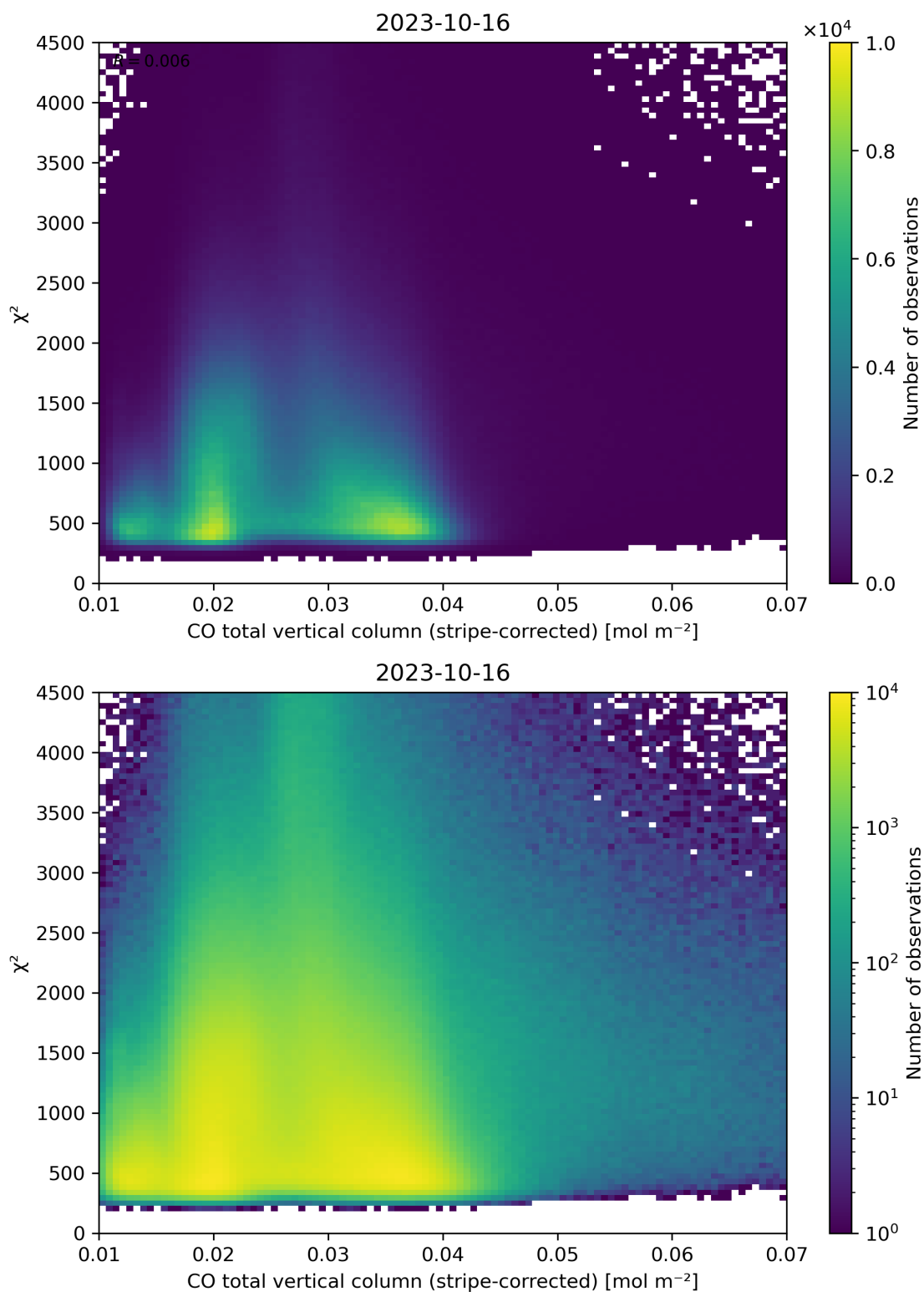
Figure 37: Scatter density plot of “CO total vertical column (stripe-corrected)” against “ \chi^2 ” for 2023-10-15 to 2023-10-17.
