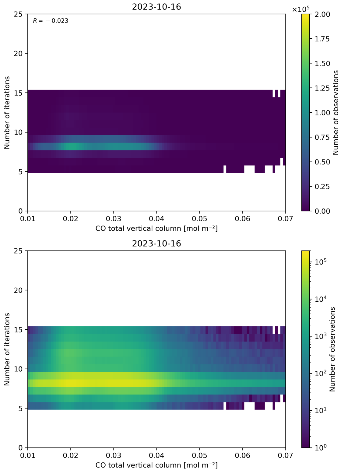
Figure 42: Scatter density plot of “CO total vertical column” against “Number of iterations” for 2023-10-15 to 2023-10-17.
