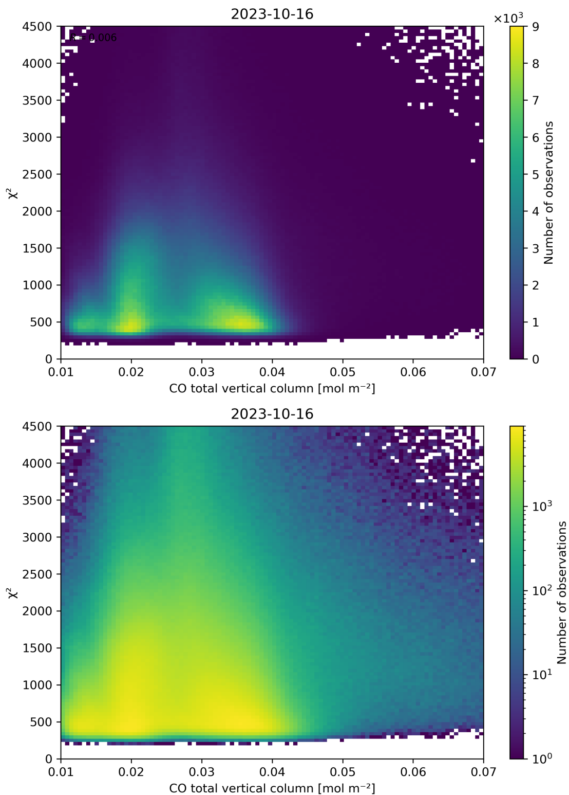
Figure 35: Scatter density plot of “CO total vertical column” against “ \chi^2 ” for 2023-10-15 to 2023-10-17.
