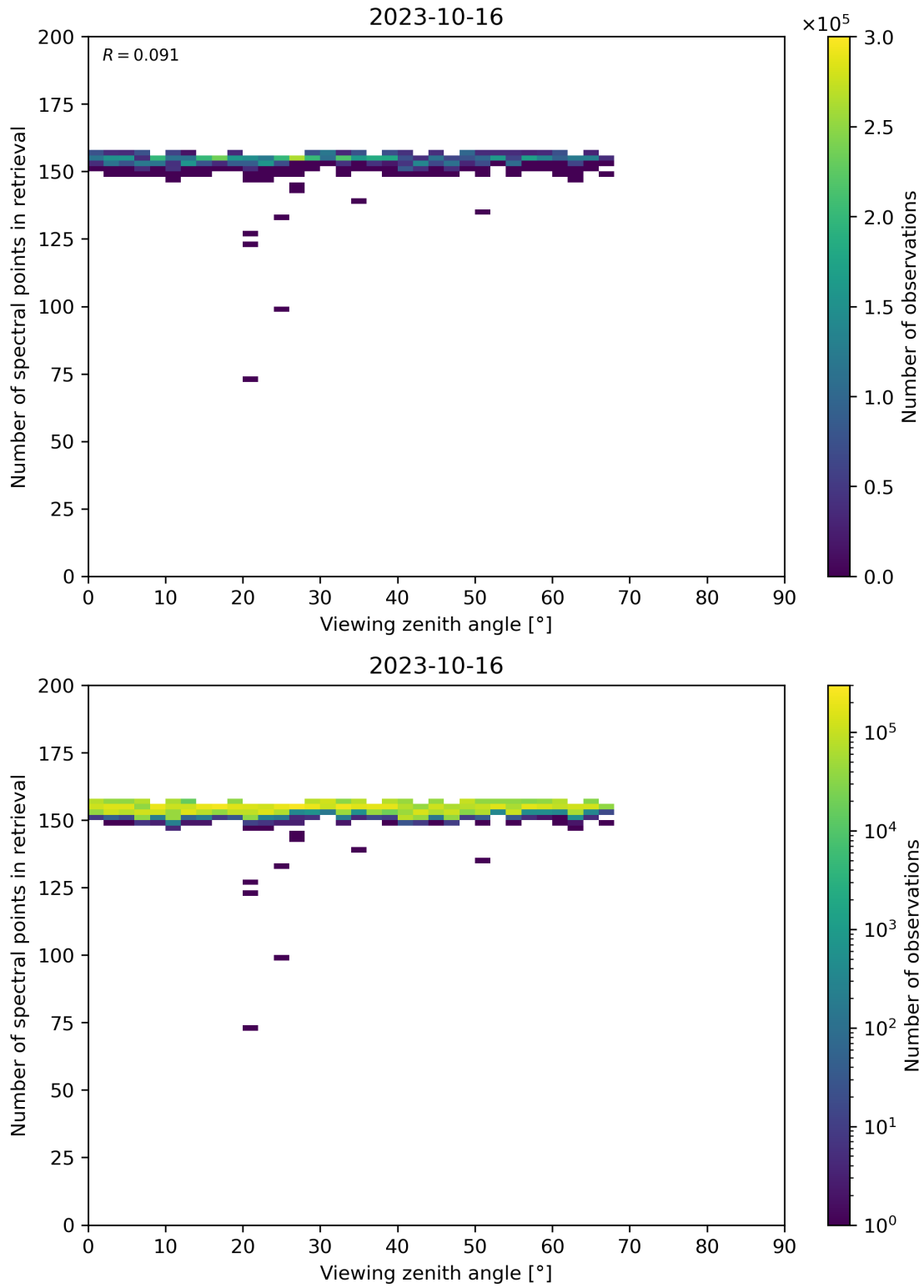
Figure 76: Scatter density plot of “Viewing zenith angle” against “Number of spectral points in retrieval” for 2023-10-15 to 2023-10-17.
