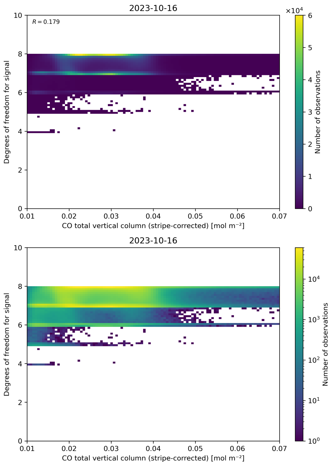
Figure 38: Scatter density plot of “CO total vertical column (stripe-corrected)” against “Degrees of freedom for signal” for 2023-10-15 to 2023-10-17.
