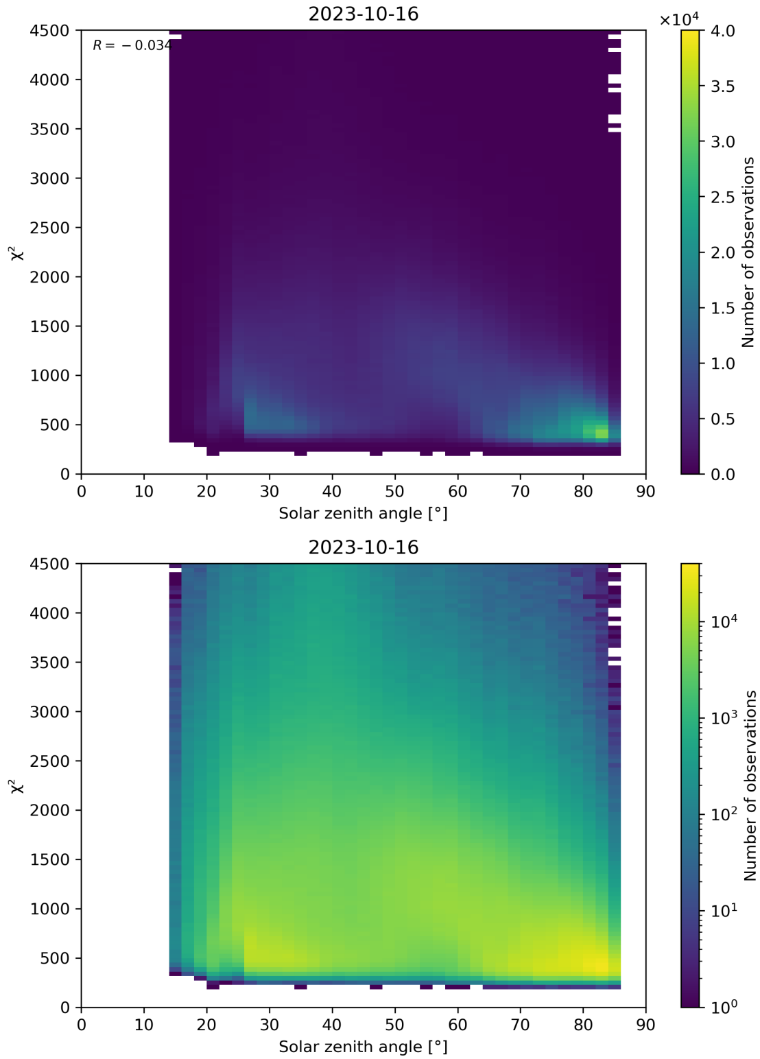
Figure 64: Scatter density plot of “Solar zenith angle” against “ \chi^2 ” for 2023-10-15 to 2023-10-17.
