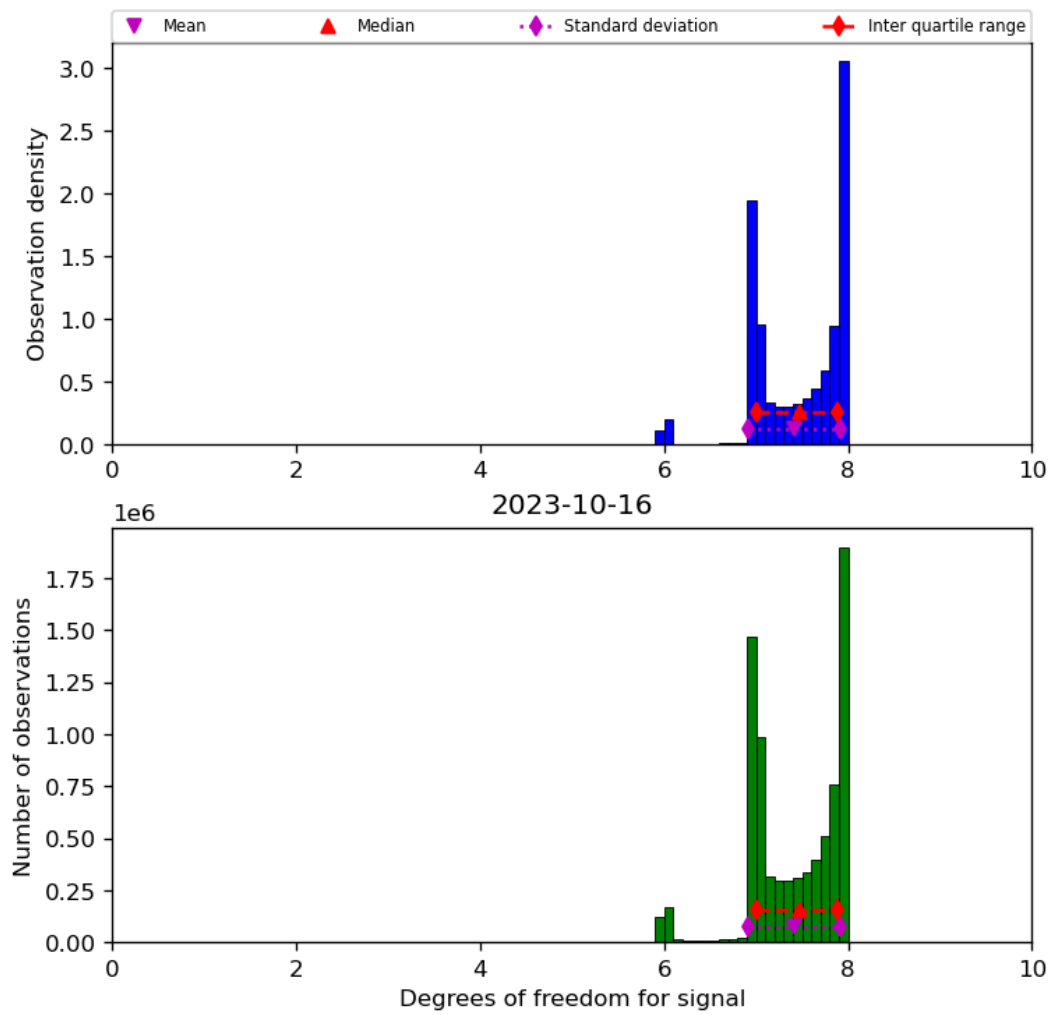
Figure 23: Histogram of “Degrees of freedom for signal” for 2023-10-15 to 2023-10-17
