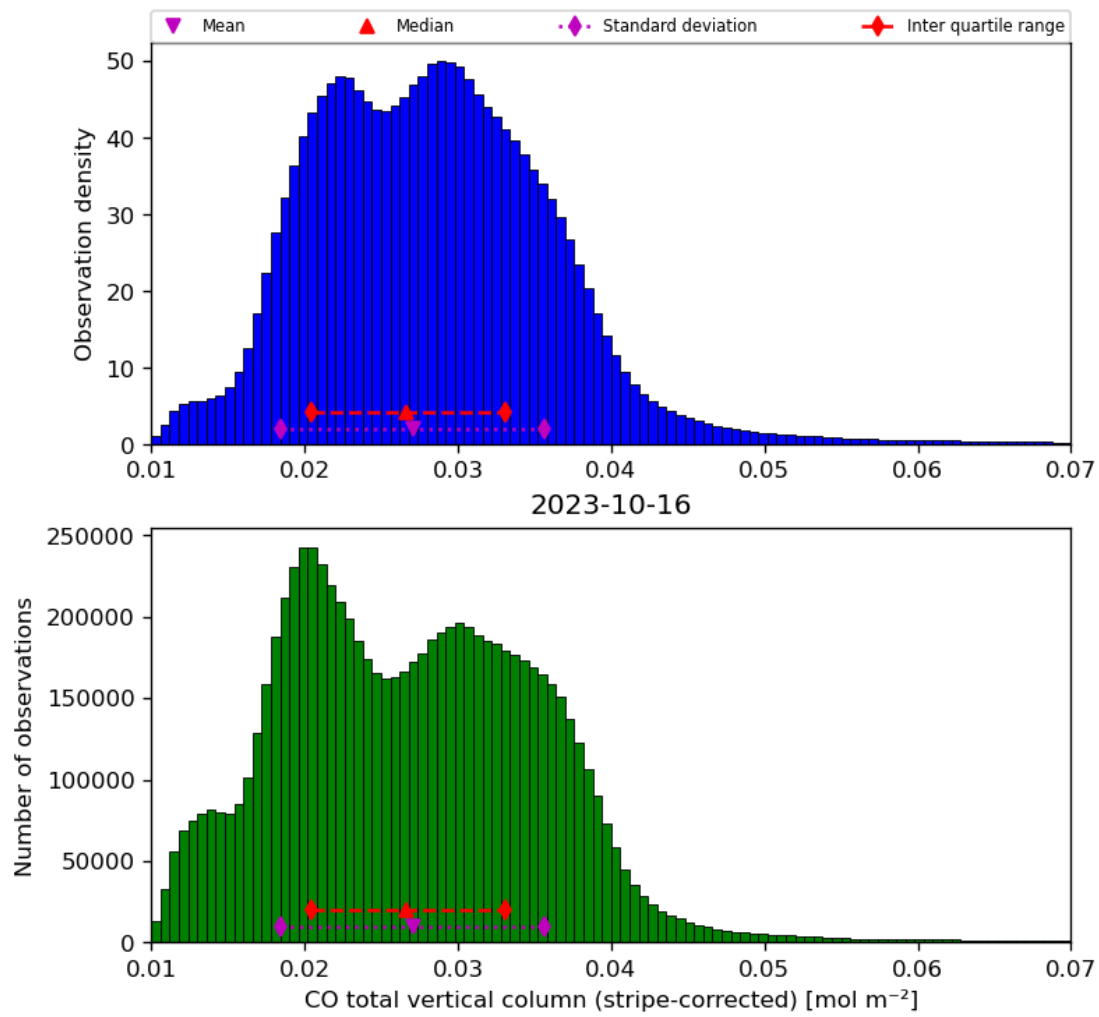
Figure 19: Histogram of “CO total vertical column (stripe-corrected)” for 2023-10-15 to 2023-10-17
