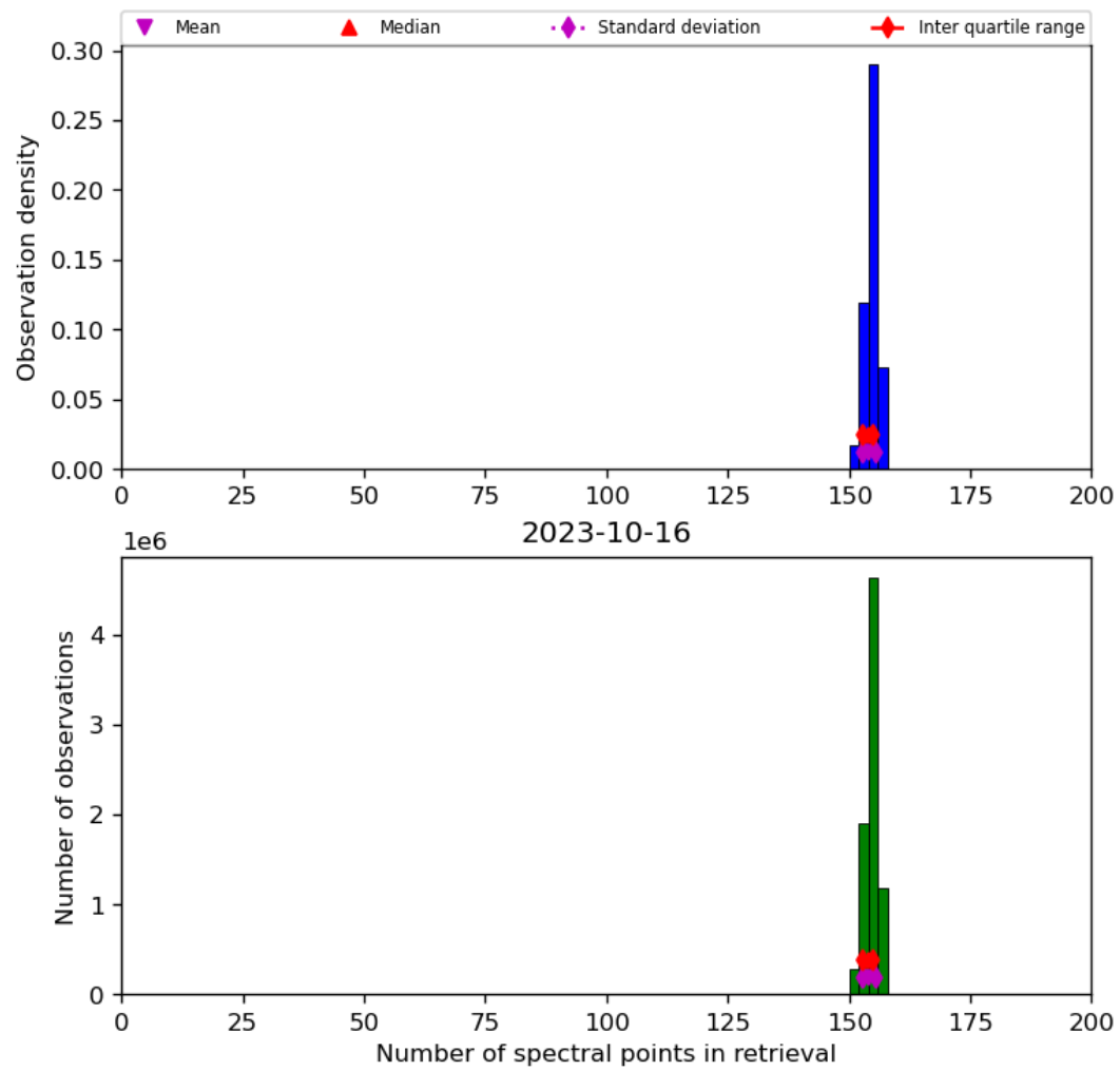
Figure 21: Histogram of “Number of spectral points in retrieval” for 2023-10-15 to 2023-10-17
