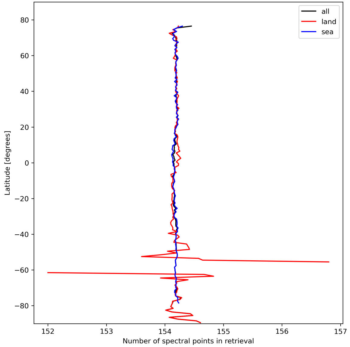
Figure 13: Zonal average of “Number of spectral points in retrieval” for 2023-10-15 to 2023-10-17.
