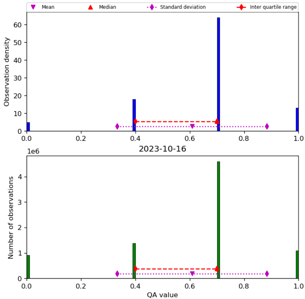
Figure 17: Histogram of “QA value” for 2023-10-15 to 2023-10-17
