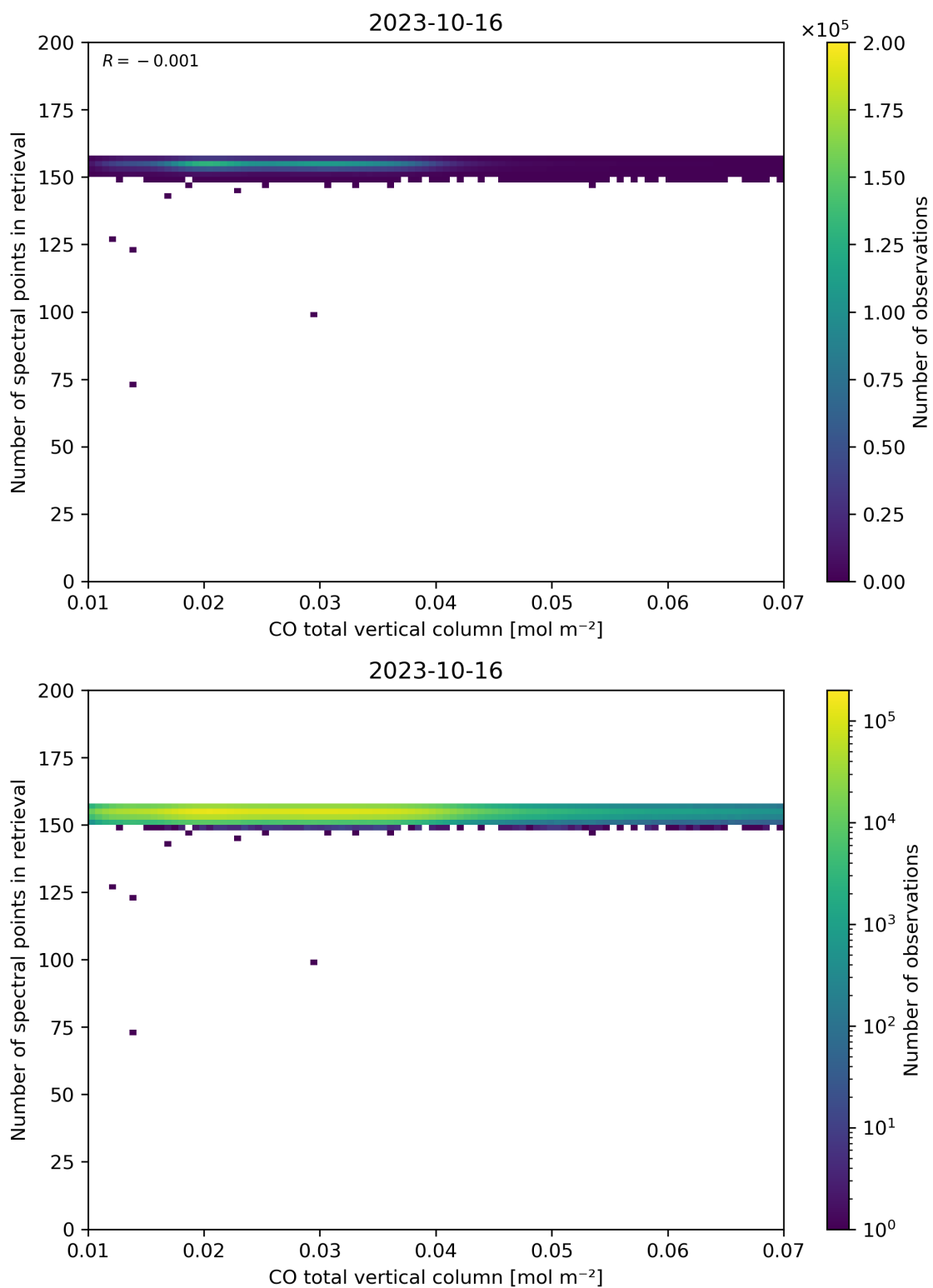
Figure 43: Scatter density plot of “CO total vertical column” against “Number of spectral points in retrieval” for 2023-10-15 to 2023-10-17.
