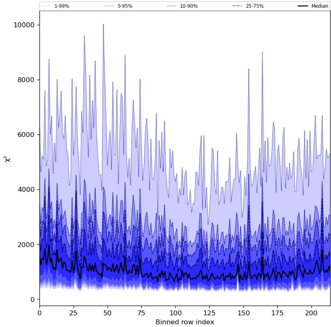
Figure 30: Along track statistics of “ \chi^2 ” for 2023-10-15 to 2023-10-17
