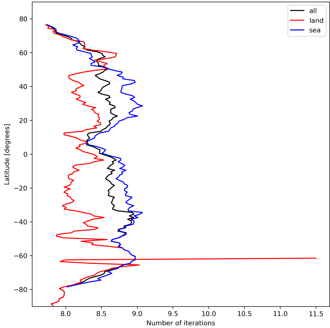
Figure 16: Zonal average of “Number of iterations” for 2023-10-15 to 2023-10-17.
