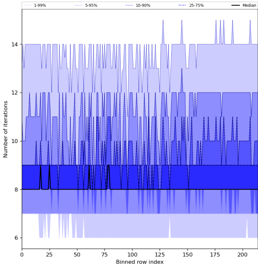
Figure 32: Along track statistics of “Number of iterations” for 2023-10-15 to 2023-10-17
