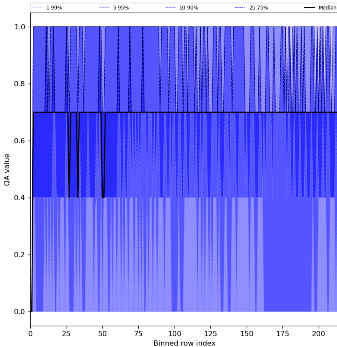
Figure 25: Along track statistics of “QA value” for 2023-10-15 to 2023-10-17
