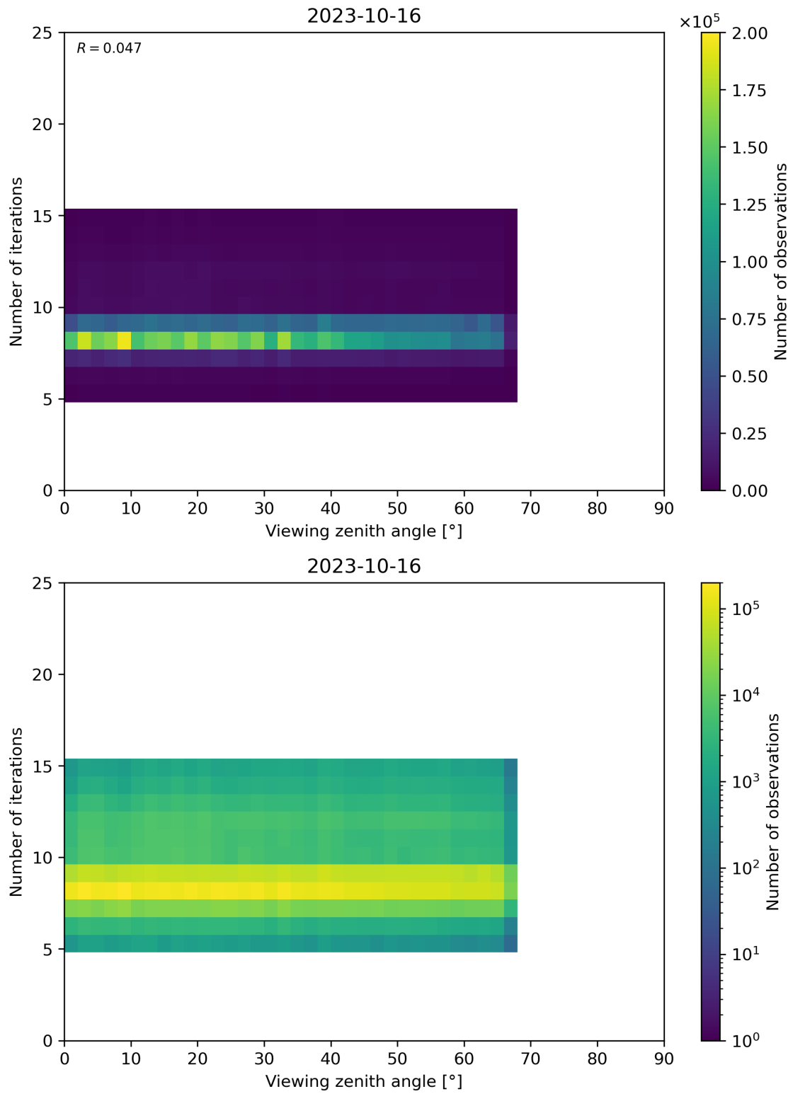
Figure 75: Scatter density plot of “Viewing zenith angle” against “Number of iterations” for 2023-10-15 to 2023-10-17.
