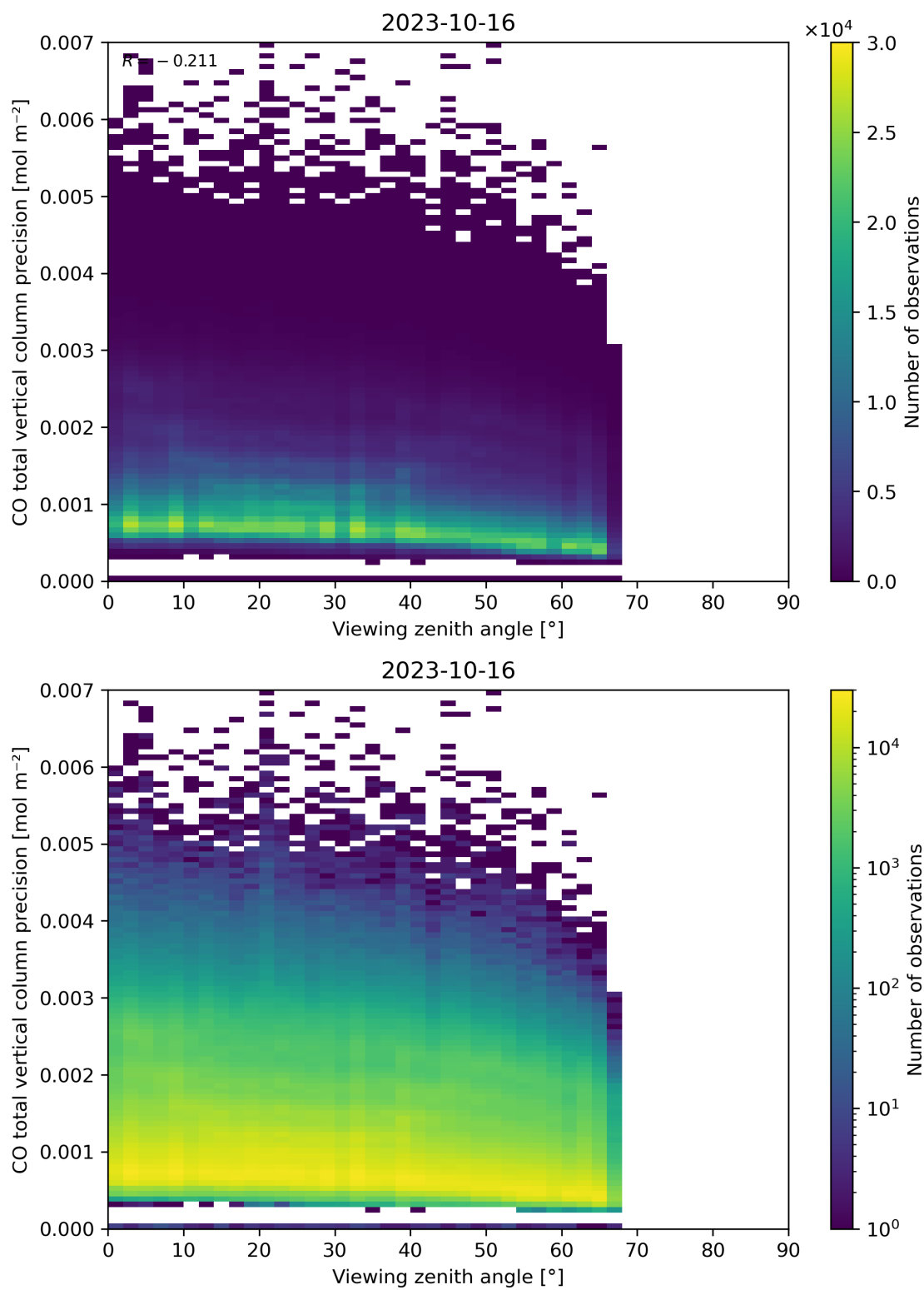
Figure 71: Scatter density plot of “Viewing zenith angle” against “CO total vertical column precision” for 2023-10-15 to 2023-10-17.
