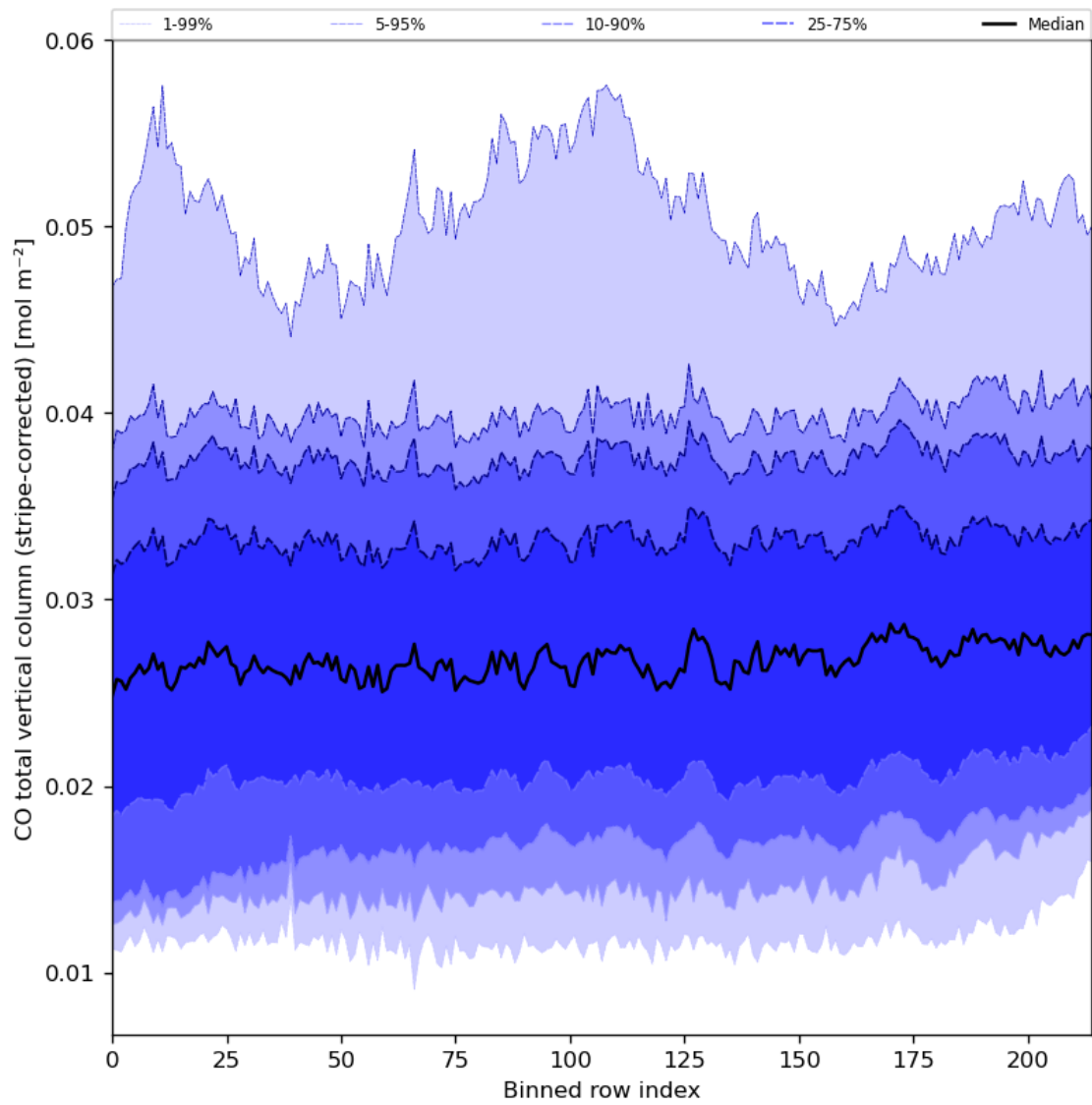
Figure 27: Along track statistics of “CO total vertical column (stripe-corrected)” for 2023-10-15 to 2023-10-17
