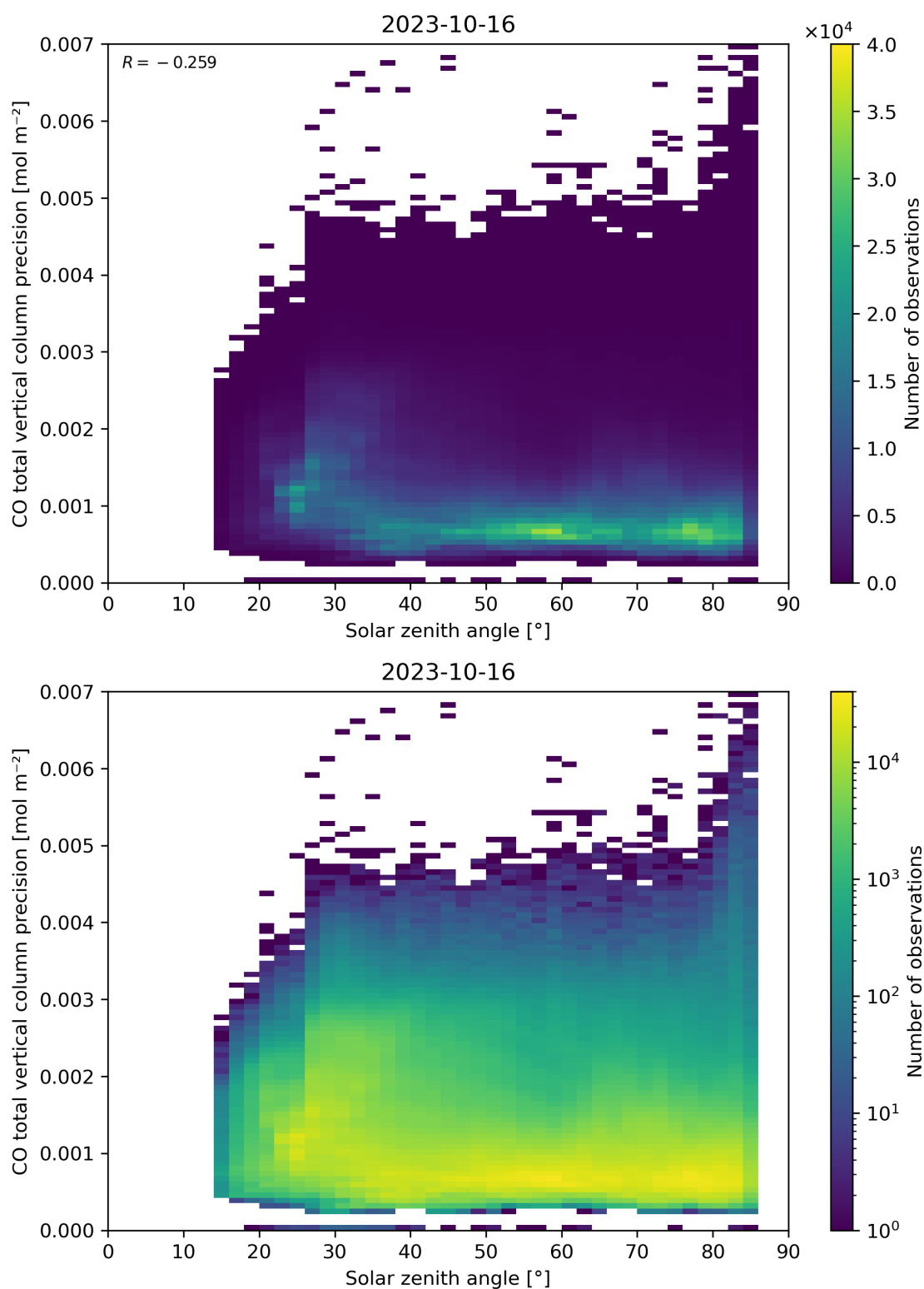
Figure 63: Scatter density plot of “Solar zenith angle” against “CO total vertical column precision” for 2023-10-15 to 2023-10-17.
