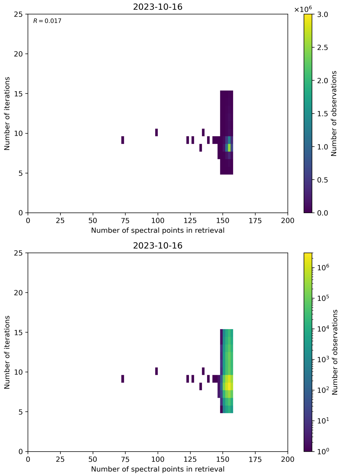
Figure 60: Scatter density plot of “Number of spectral points in retrieval” against “Number of iterations” for 2023-10-15 to 2023-10-17.
