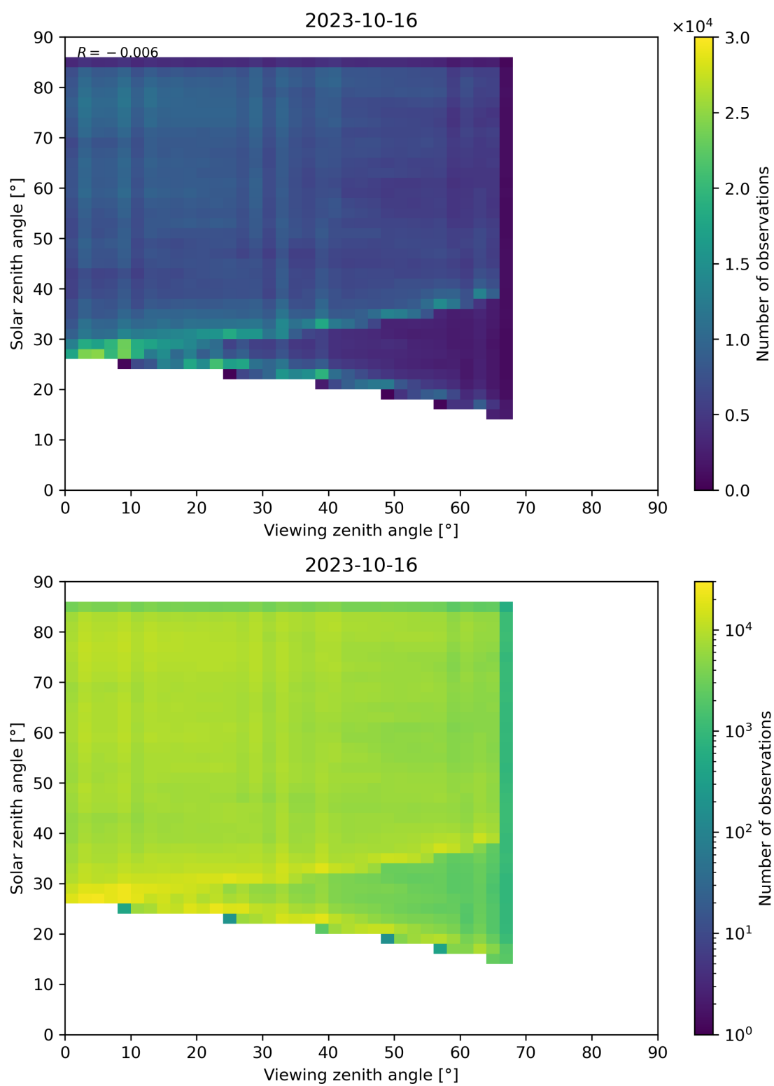
Figure 77: Scatter density plot of “Viewing zenith angle” against “Solar zenith angle” for 2023-10-15 to 2023-10-17.
