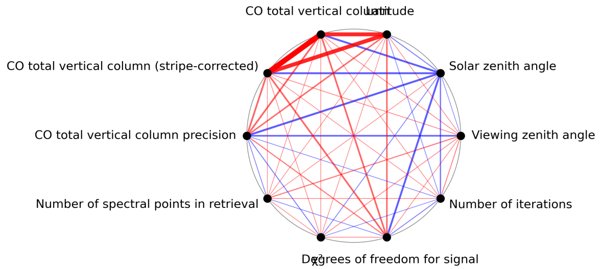
Figure 1: Map of correlation graph for 2023-10-17 to 2023-10-18.
