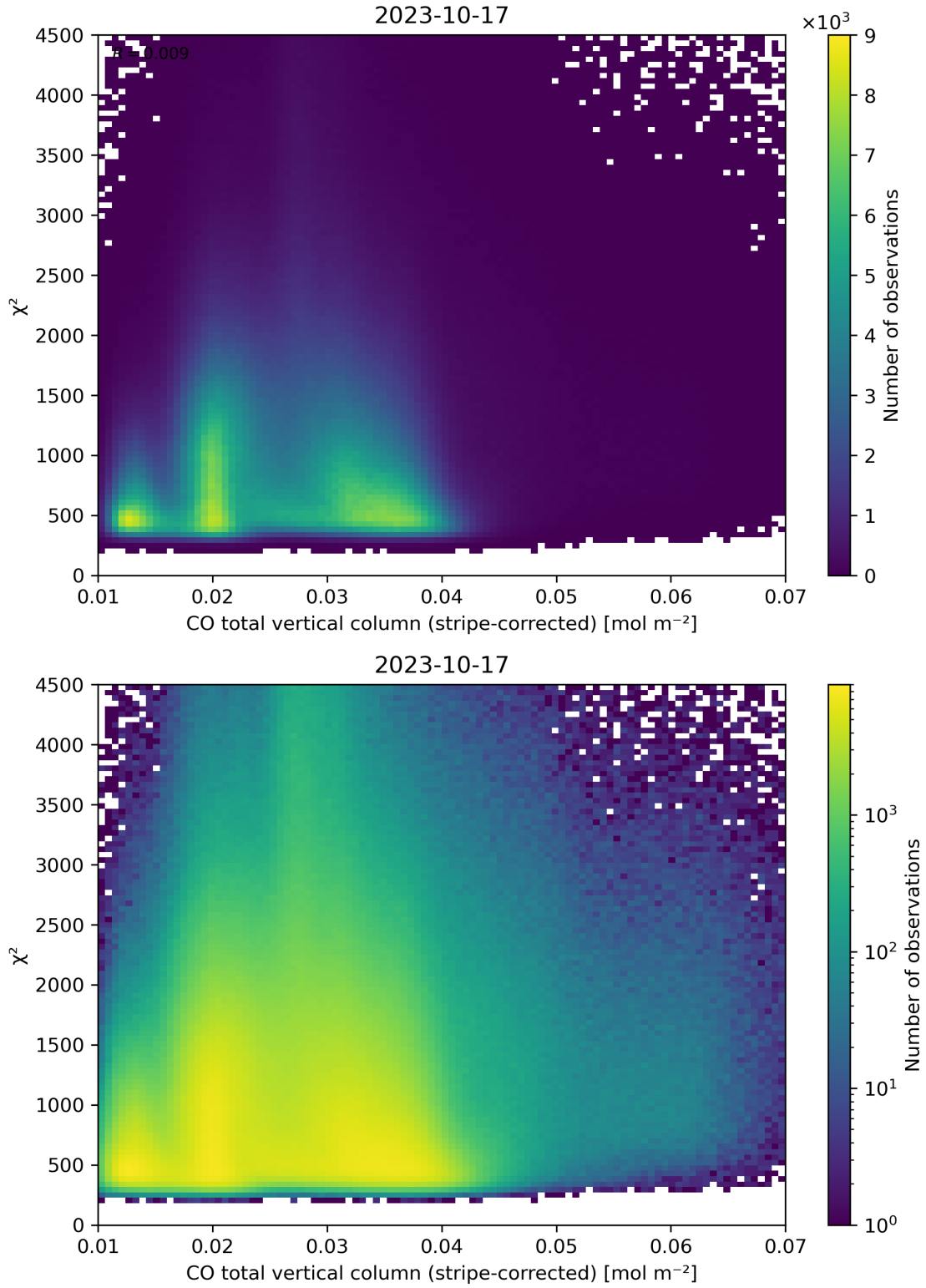
Figure 37: Scatter density plot of “CO total vertical column (stripe-corrected)” against “ \chi^2 ” for 2023-10-17 to 2023-10-18.
