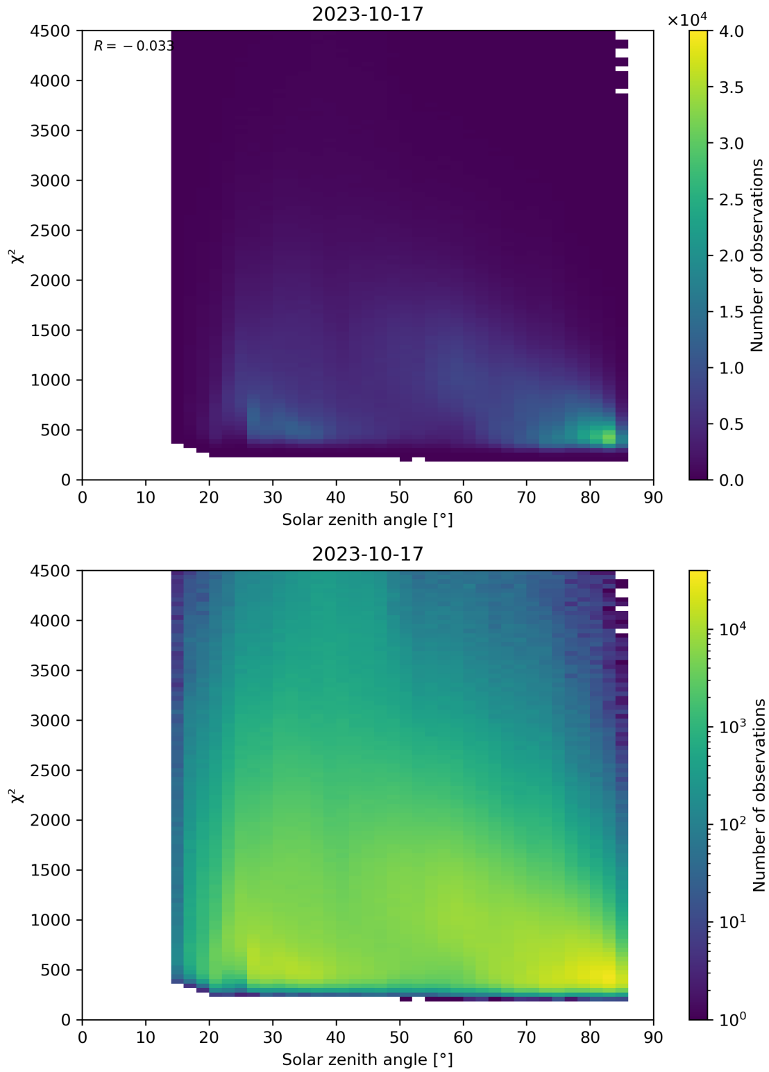
Figure 64: Scatter density plot of “Solar zenith angle” against “ \chi^2 ” for 2023-10-17 to 2023-10-18.
