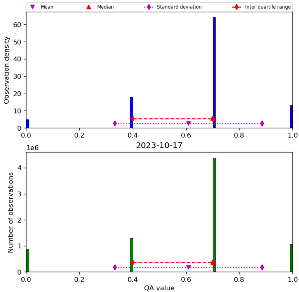
Figure 17: Histogram of “QA value” for 2023-10-17 to 2023-10-18
