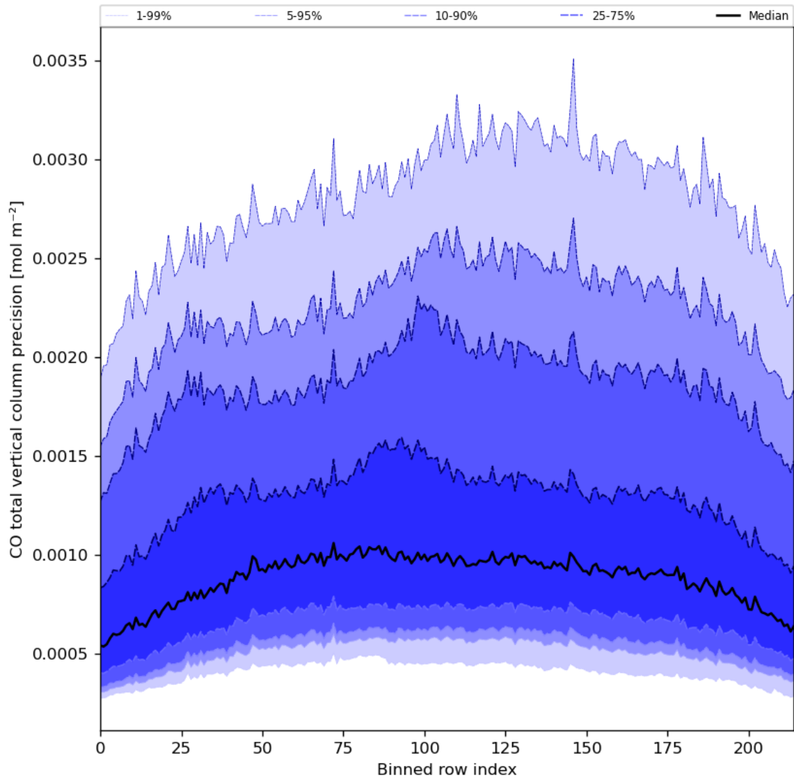
Figure 28: Along track statistics of “CO total vertical column precision” for 2023-10-17 to 2023-10-18
