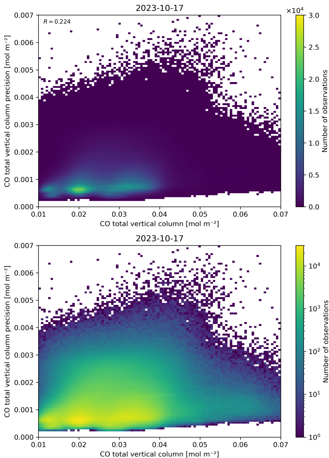
Figure 34: Scatter density plot of “CO total vertical column” against “CO total vertical column precision” for 2023-10-17 to 2023-10-18.
