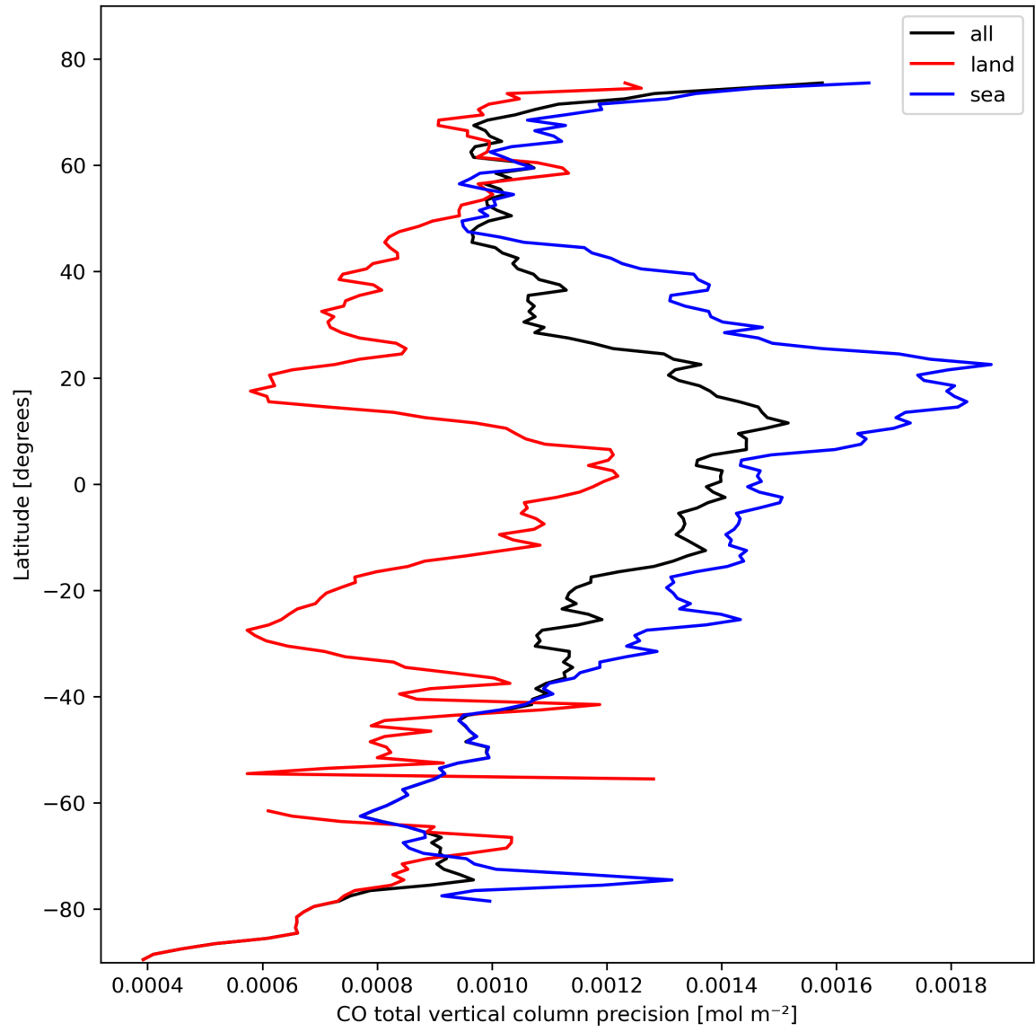
Figure 12: Zonal average of “CO total vertical column precision” for 2023-10-17 to 2023-10-18.
