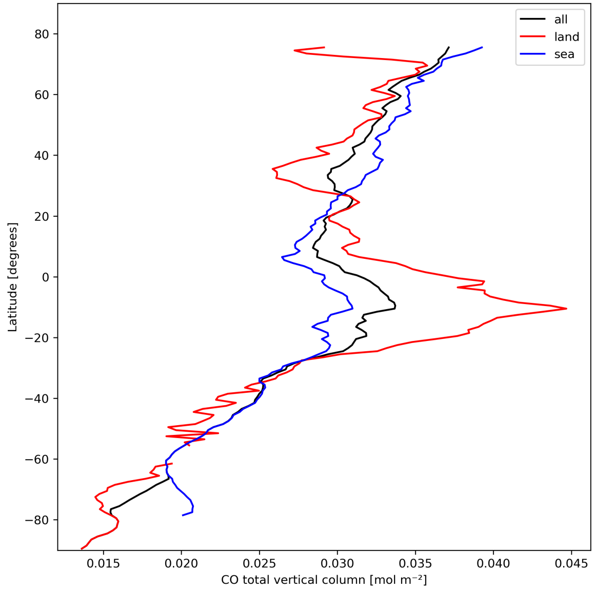
Figure 10: Zonal average of “CO total vertical column” for 2023-10-17 to 2023-10-18.
