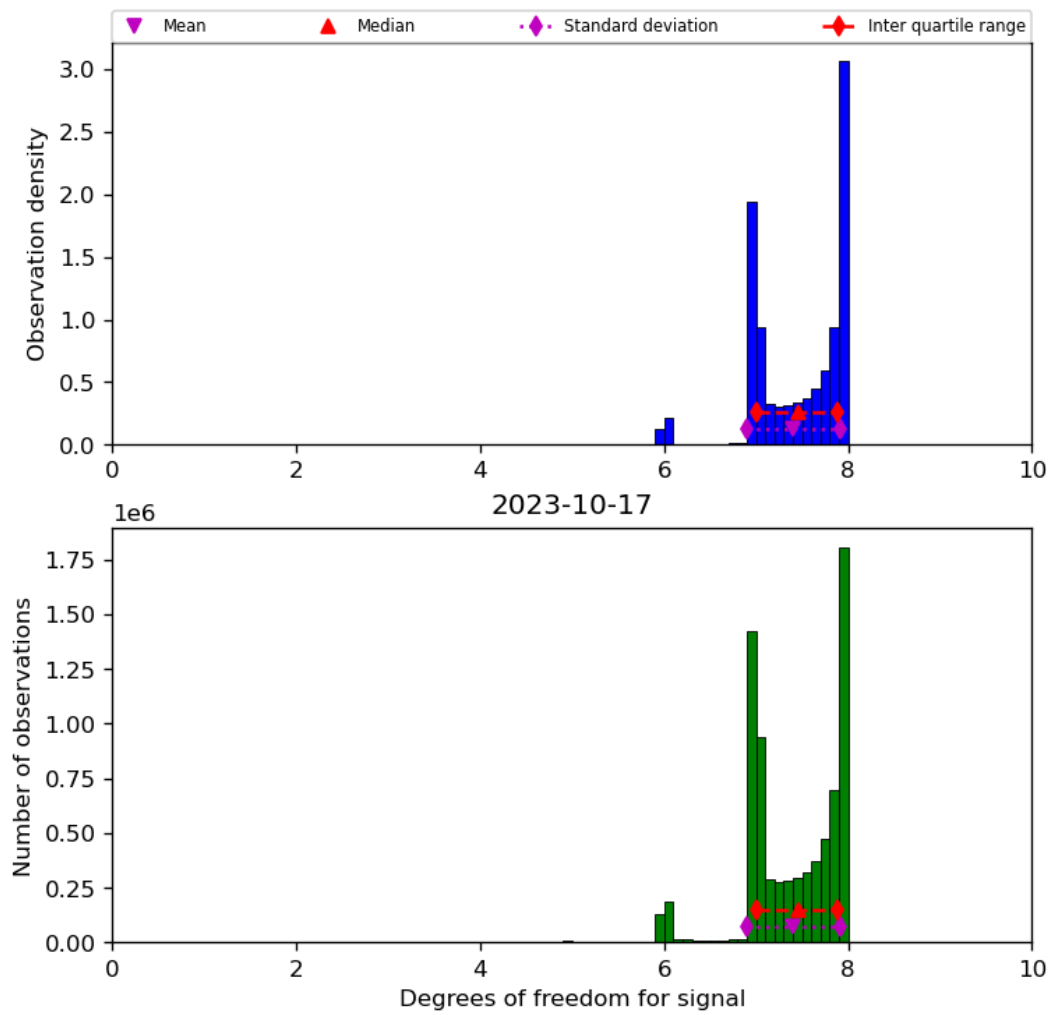
Figure 23: Histogram of “Degrees of freedom for signal” for 2023-10-17 to 2023-10-18
