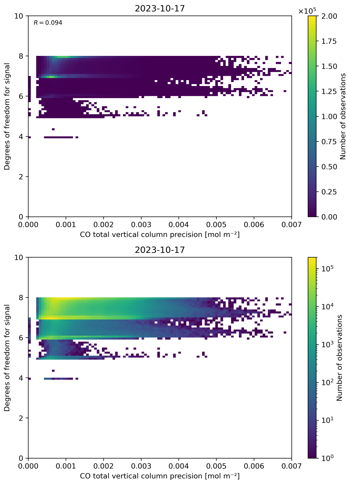
Figure 45: Scatter density plot of “CO total vertical column precision” against “Degrees of freedom for signal” for 2023-10-17 to 2023-10-18.
