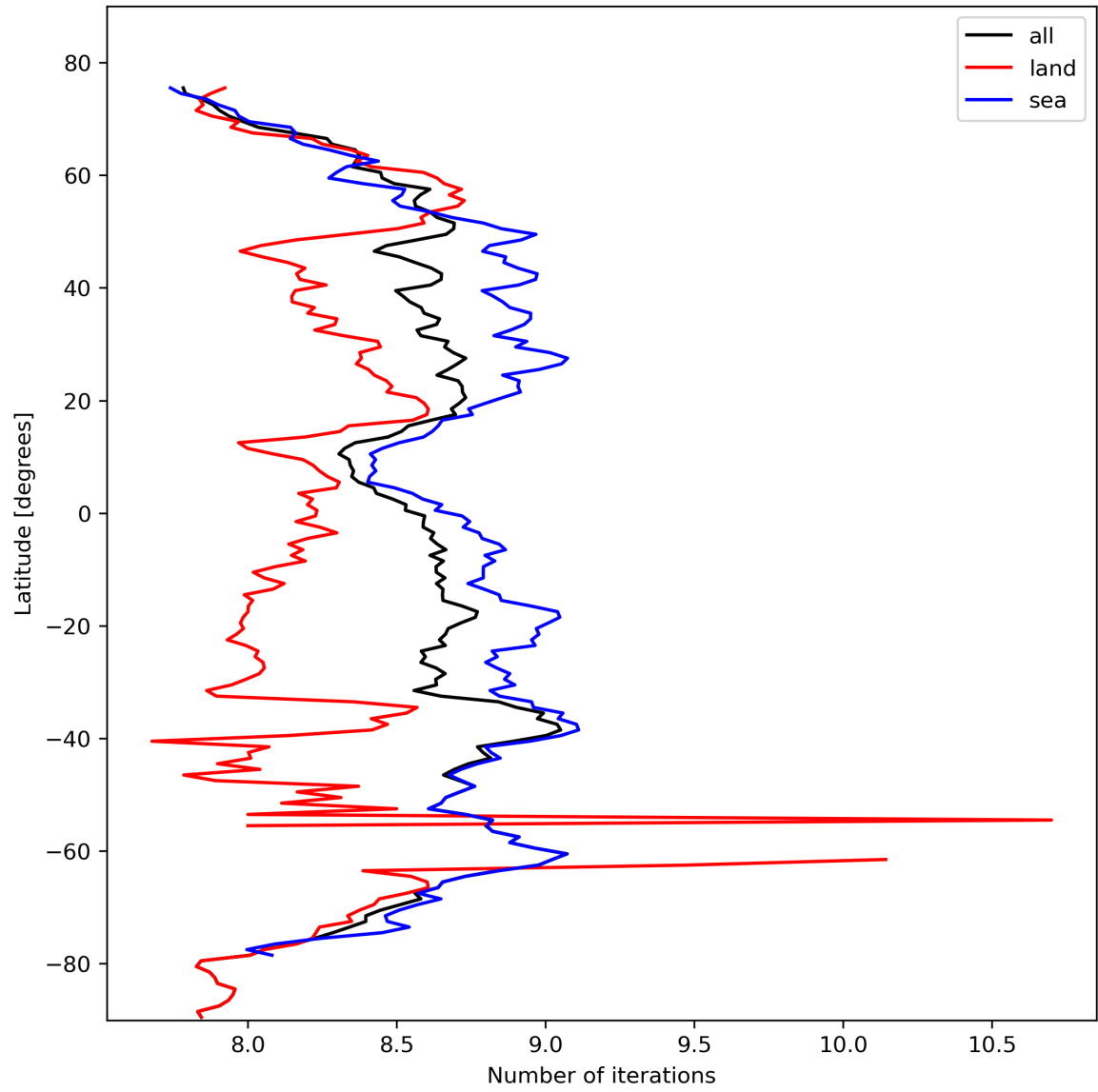
Figure 16: Zonal average of “Number of iterations” for 2023-10-17 to 2023-10-18.
