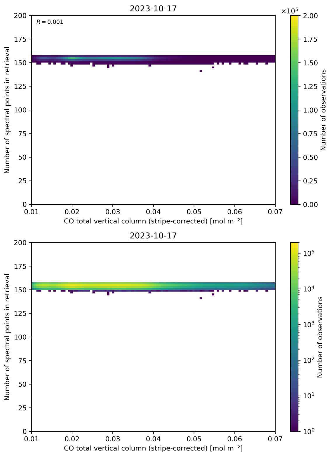
Figure 40: Scatter density plot of “CO total vertical column (stripe-corrected)” against “Number of spectral points in retrieval” for 2023-10-17 to 2023-10-18.
