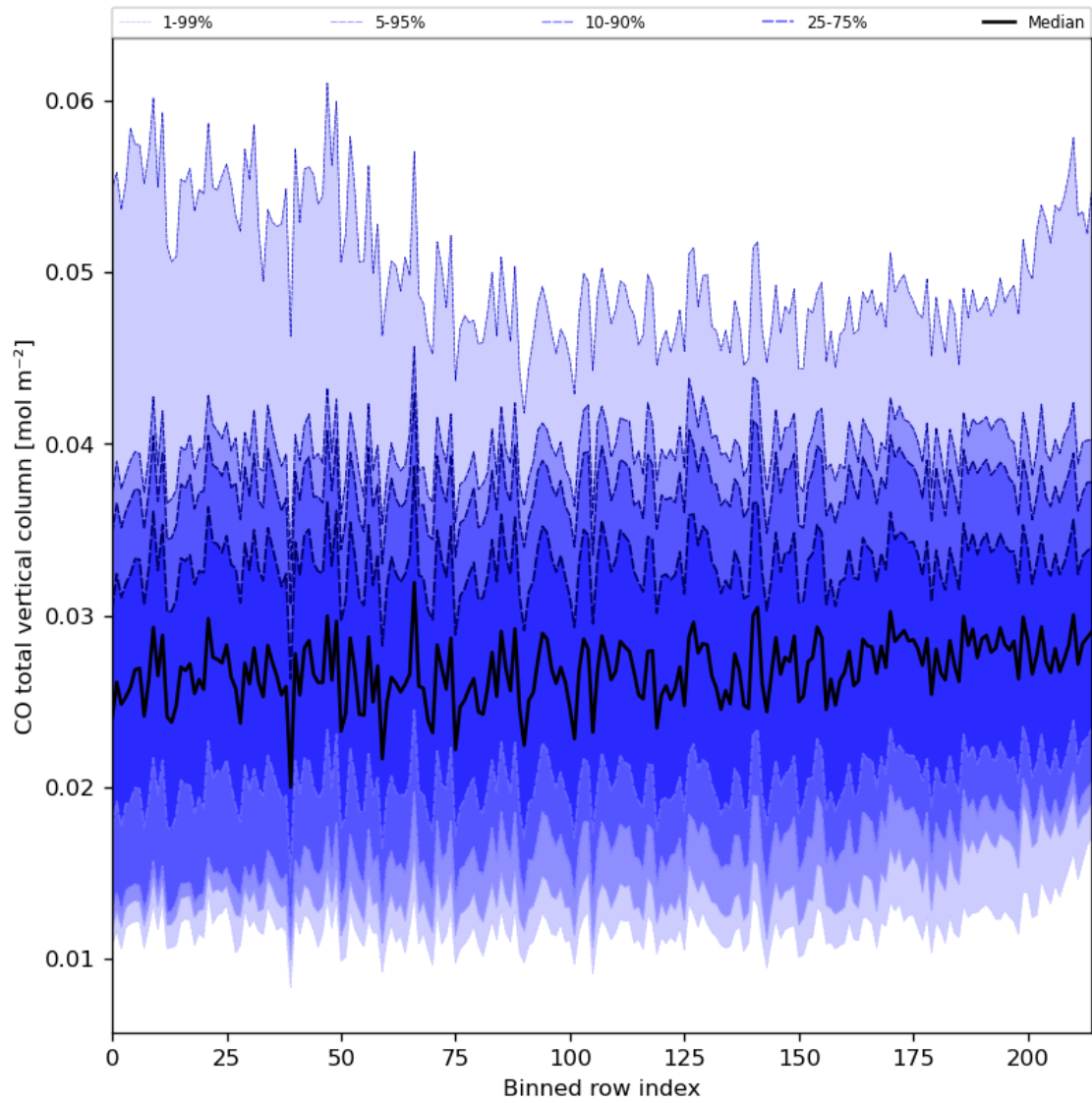
Figure 26: Along track statistics of “CO total vertical column” for 2023-10-17 to 2023-10-18
