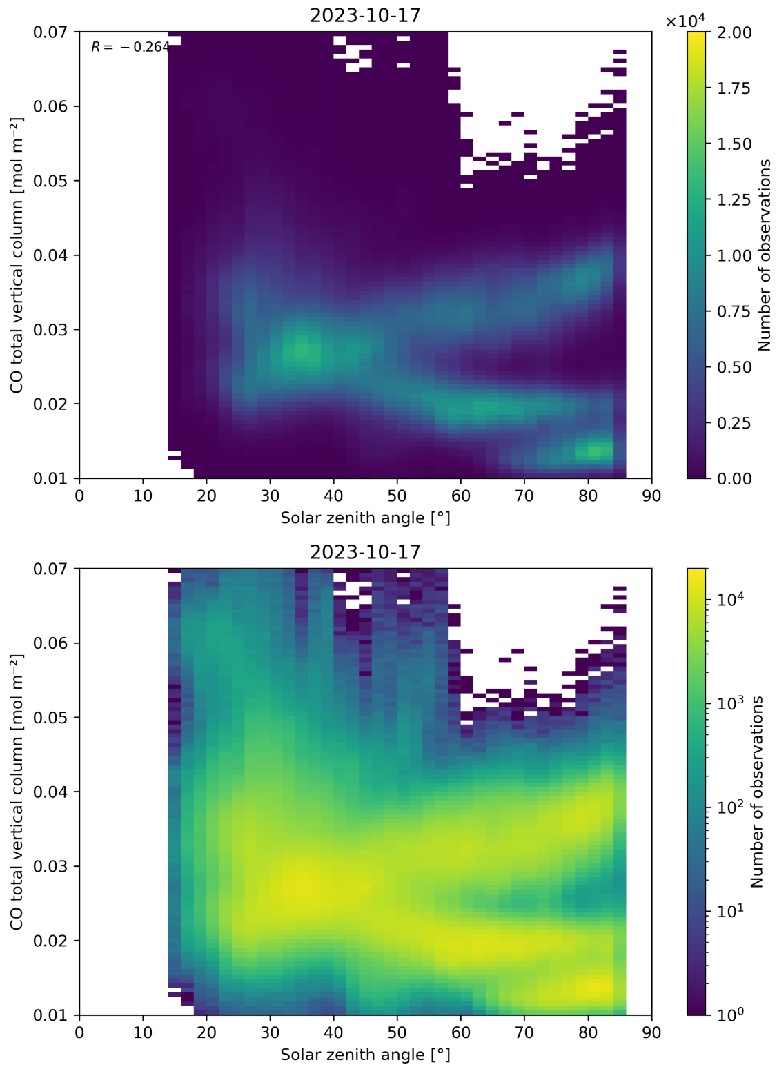
Figure 61: Scatter density plot of “Solar zenith angle” against “CO total vertical column” for 2023-10-17 to 2023-10-18.
