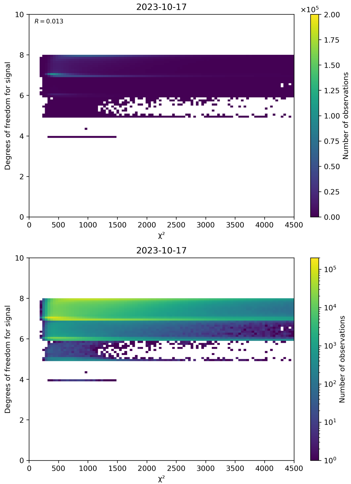
Figure 48: Scatter density plot of “ \chi^2 ” against “Degrees of freedom for signal” for 2023-10-17 to 2023-10-18.
