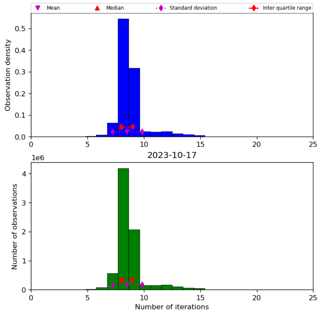
Figure 24: Histogram of “Number of iterations” for 2023-10-17 to 2023-10-18
