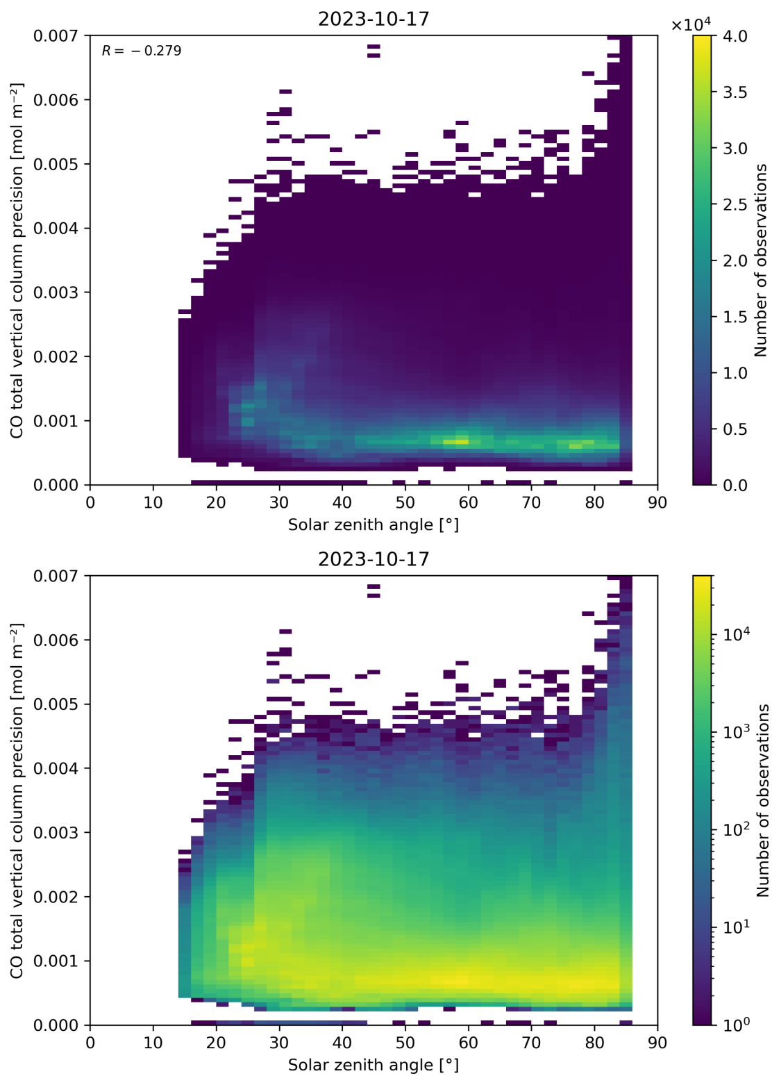
Figure 63: Scatter density plot of “Solar zenith angle” against “CO total vertical column precision” for 2023-10-17 to 2023-10-18.
