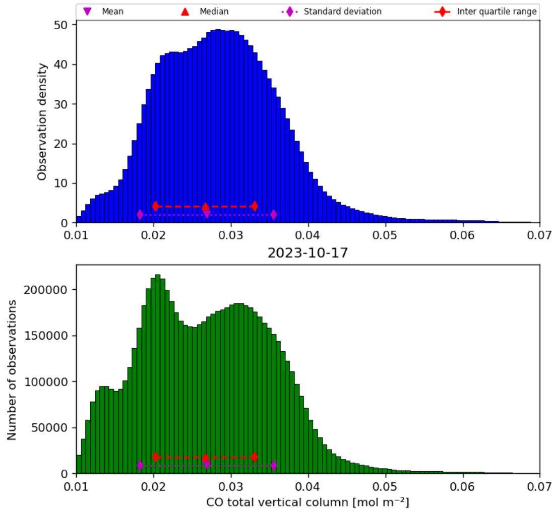
Figure 18: Histogram of “CO total vertical column” for 2023-10-17 to 2023-10-18
