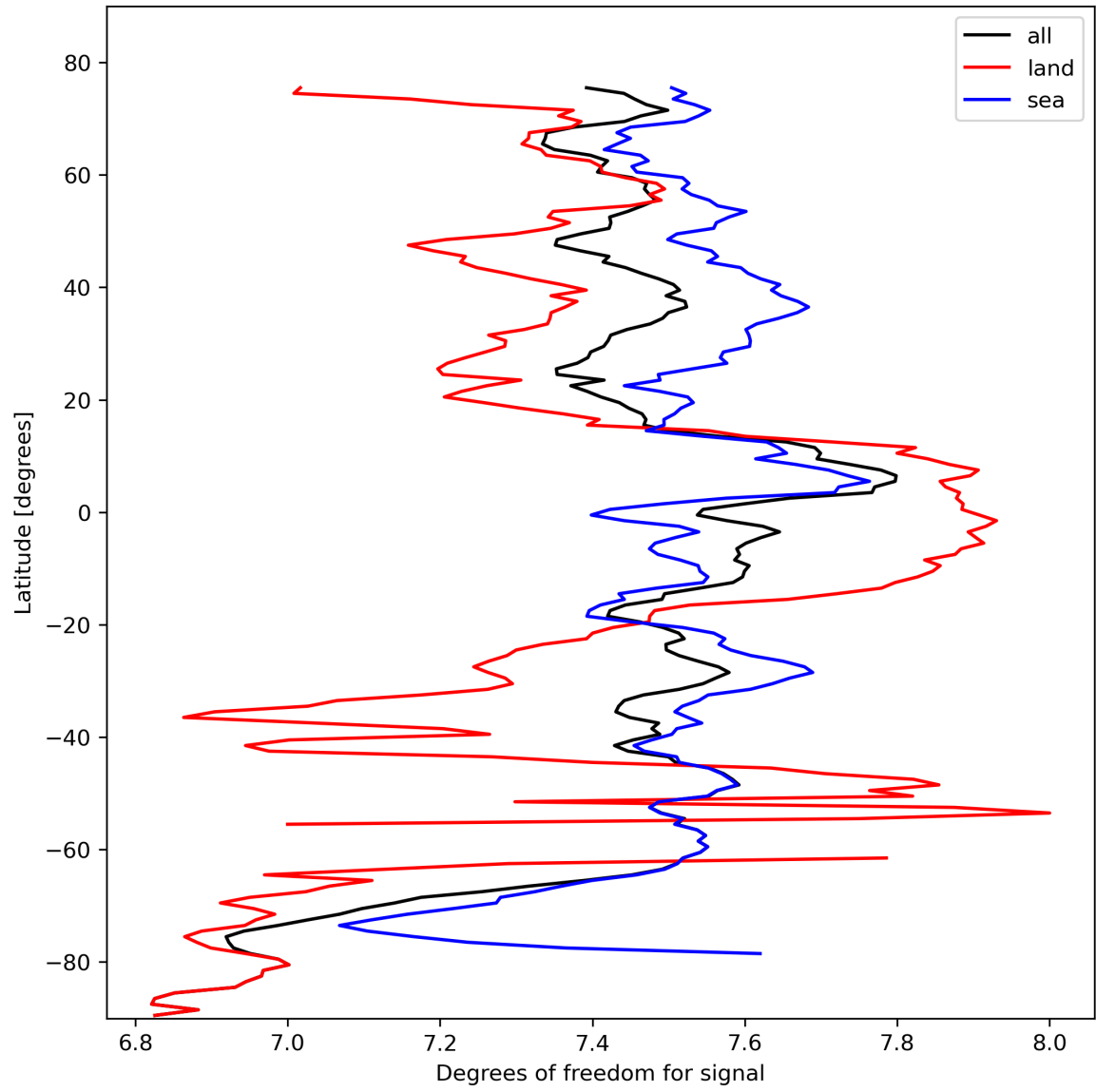
Figure 15: Zonal average of “Degrees of freedom for signal” for 2023-10-17 to 2023-10-18.
