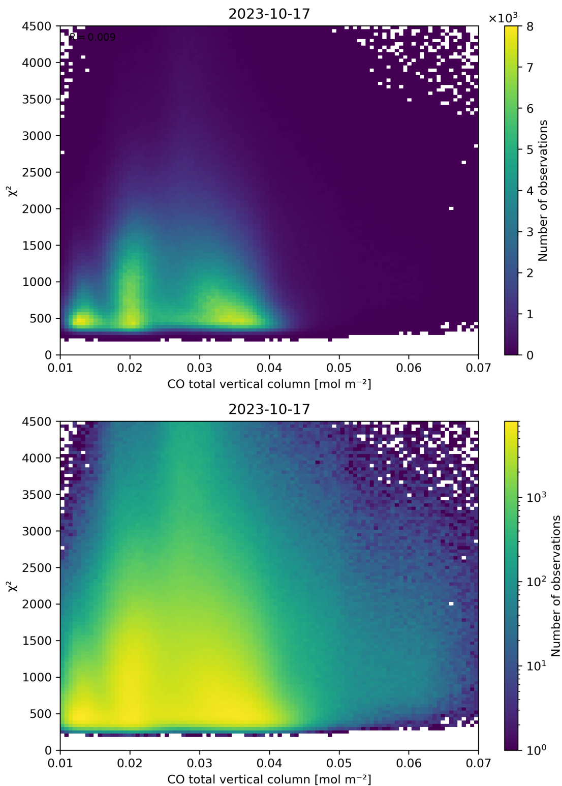
Figure 35: Scatter density plot of “CO total vertical column” against “ \chi^2 ” for 2023-10-17 to 2023-10-18.
