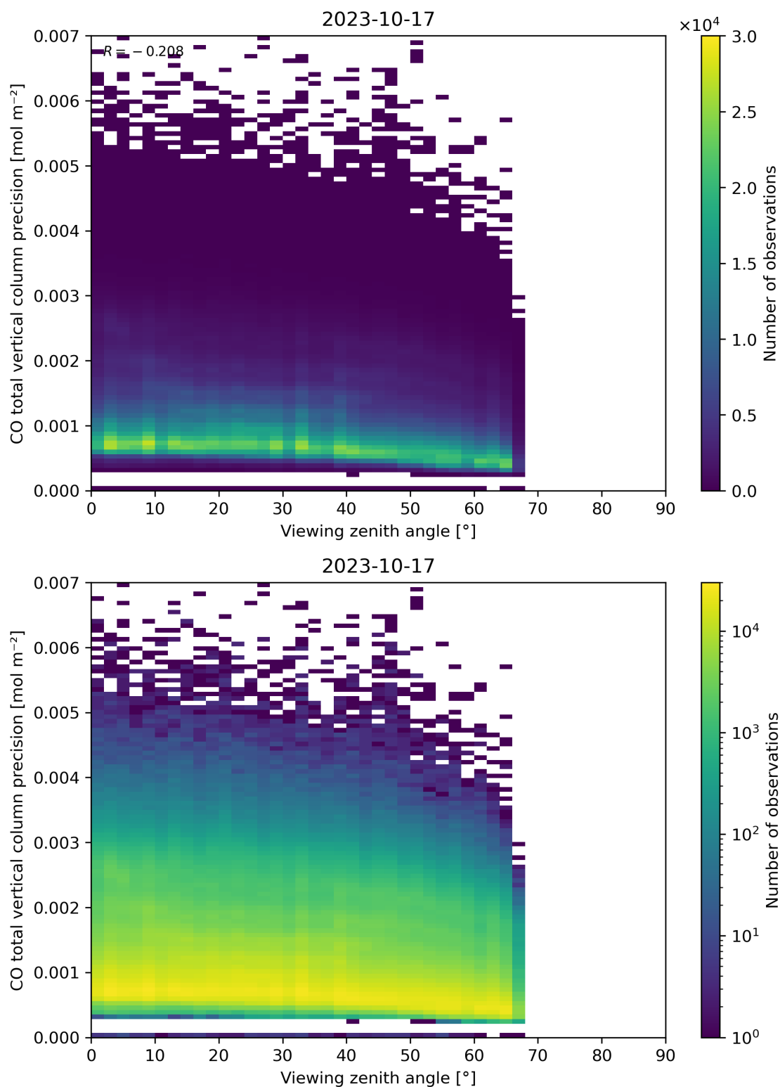
Figure 71: Scatter density plot of “Viewing zenith angle” against “CO total vertical column precision” for 2023-10-17 to 2023-10-18.
