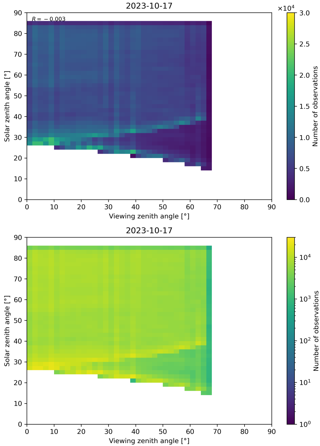
Figure 77: Scatter density plot of “Viewing zenith angle” against “Solar zenith angle” for 2023-10-17 to 2023-10-18.
