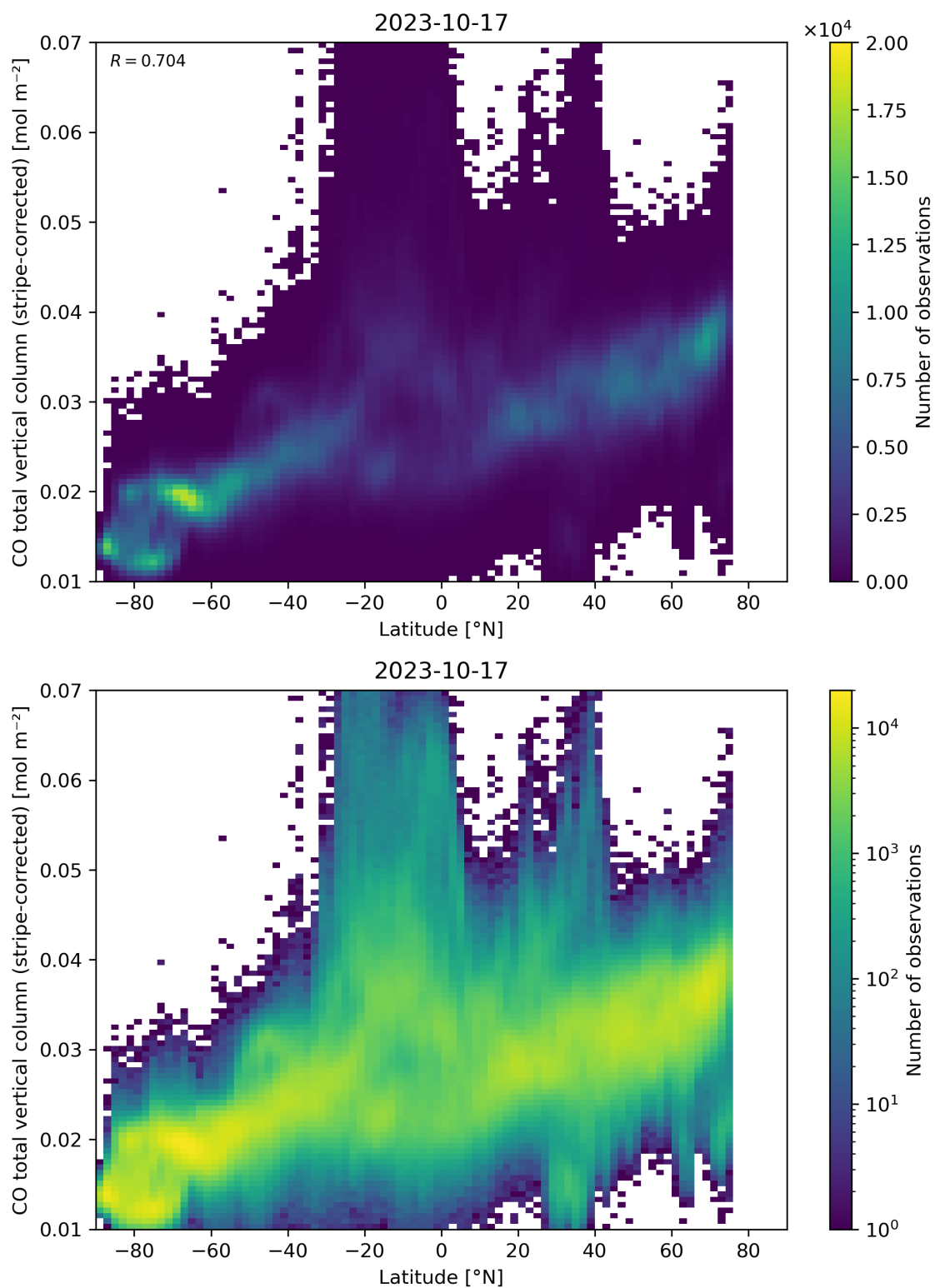
Figure 52: Scatter density plot of “Latitude” against “CO total vertical column (stripe-corrected)” for 2023-10-17 to 2023-10-18.
