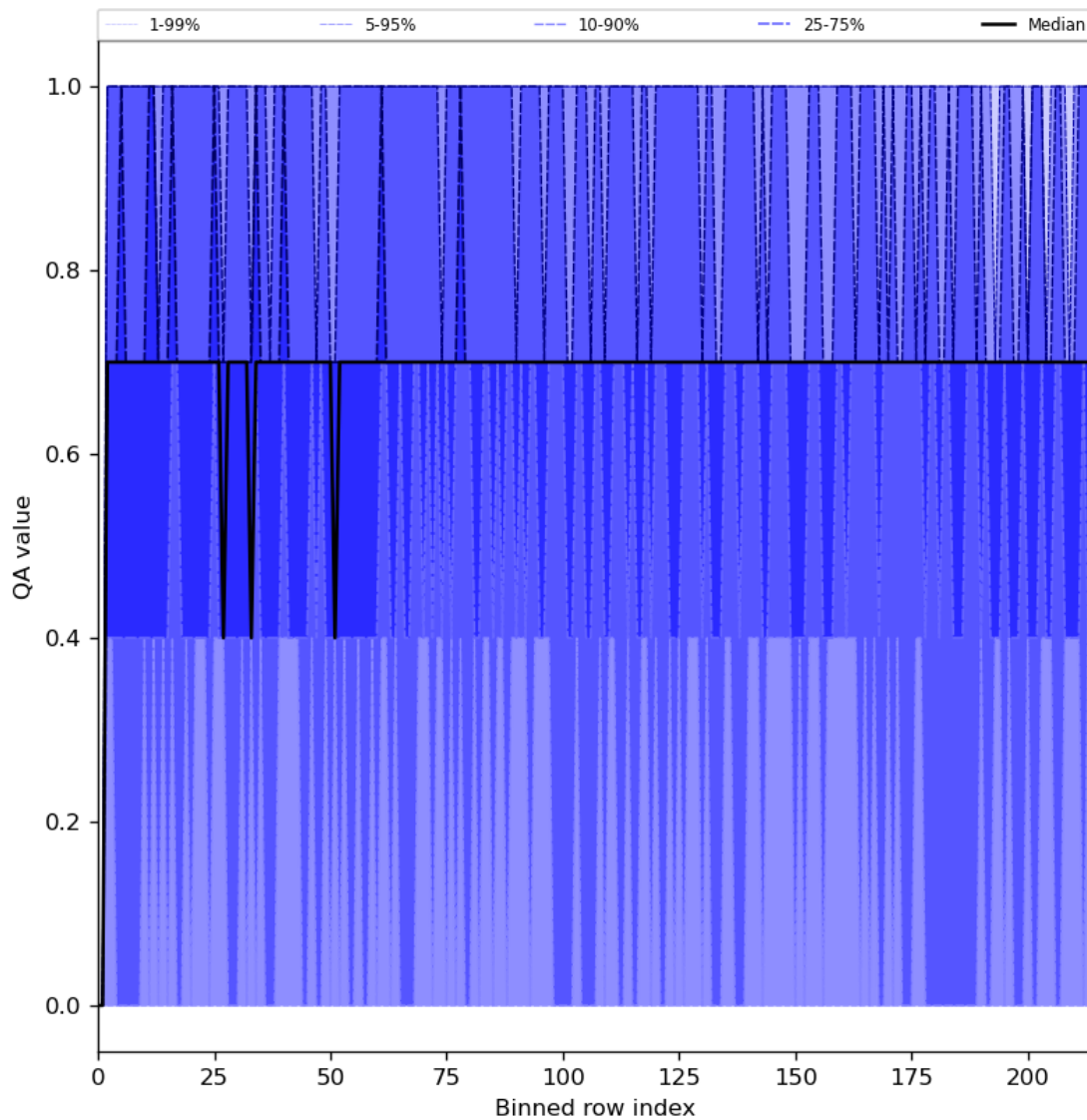
Figure 25: Along track statistics of “QA value” for 2023-10-17 to 2023-10-18
