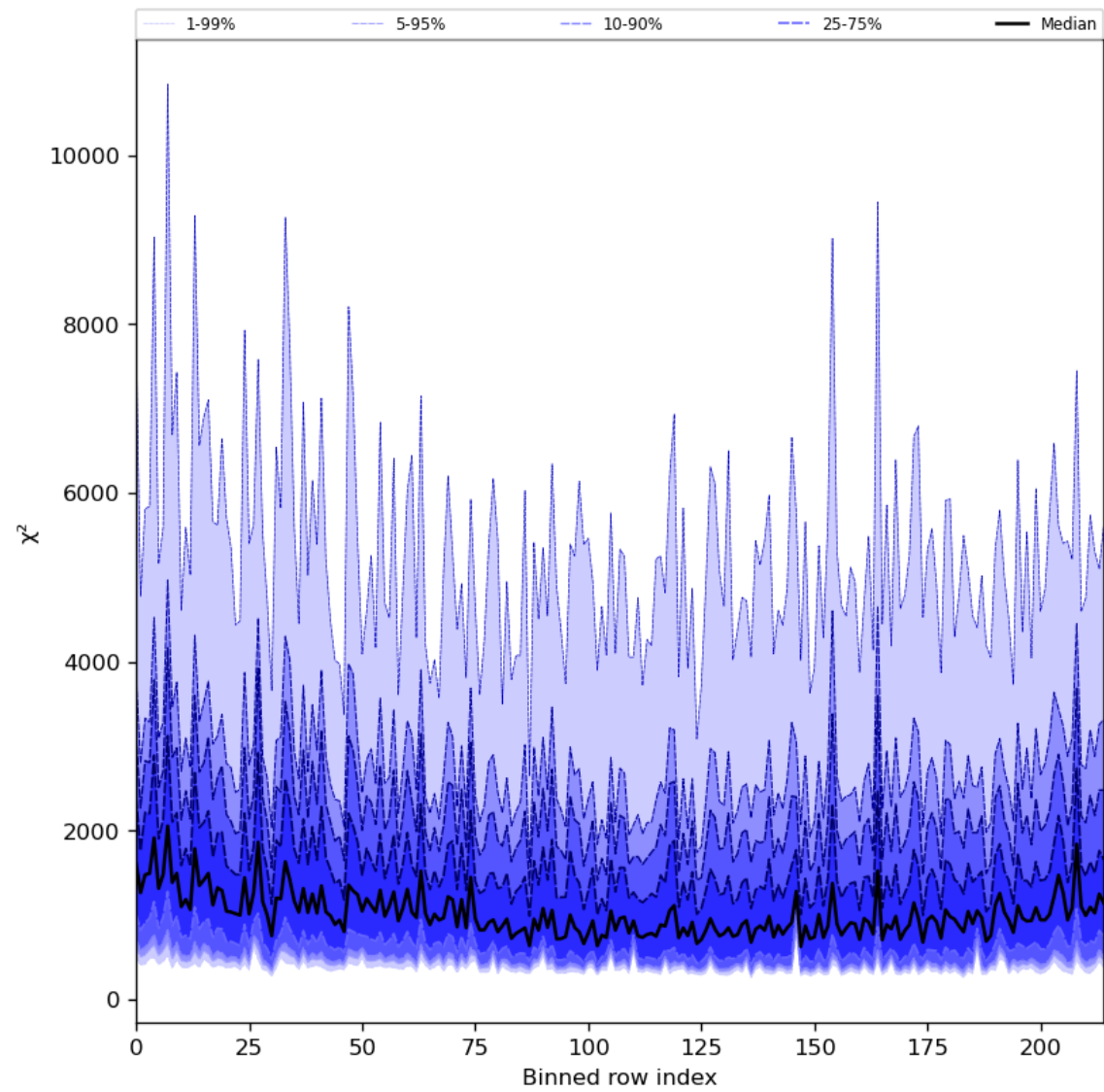
Figure 30: Along track statistics of “ \chi^2 ” for 2023-10-17 to 2023-10-18
