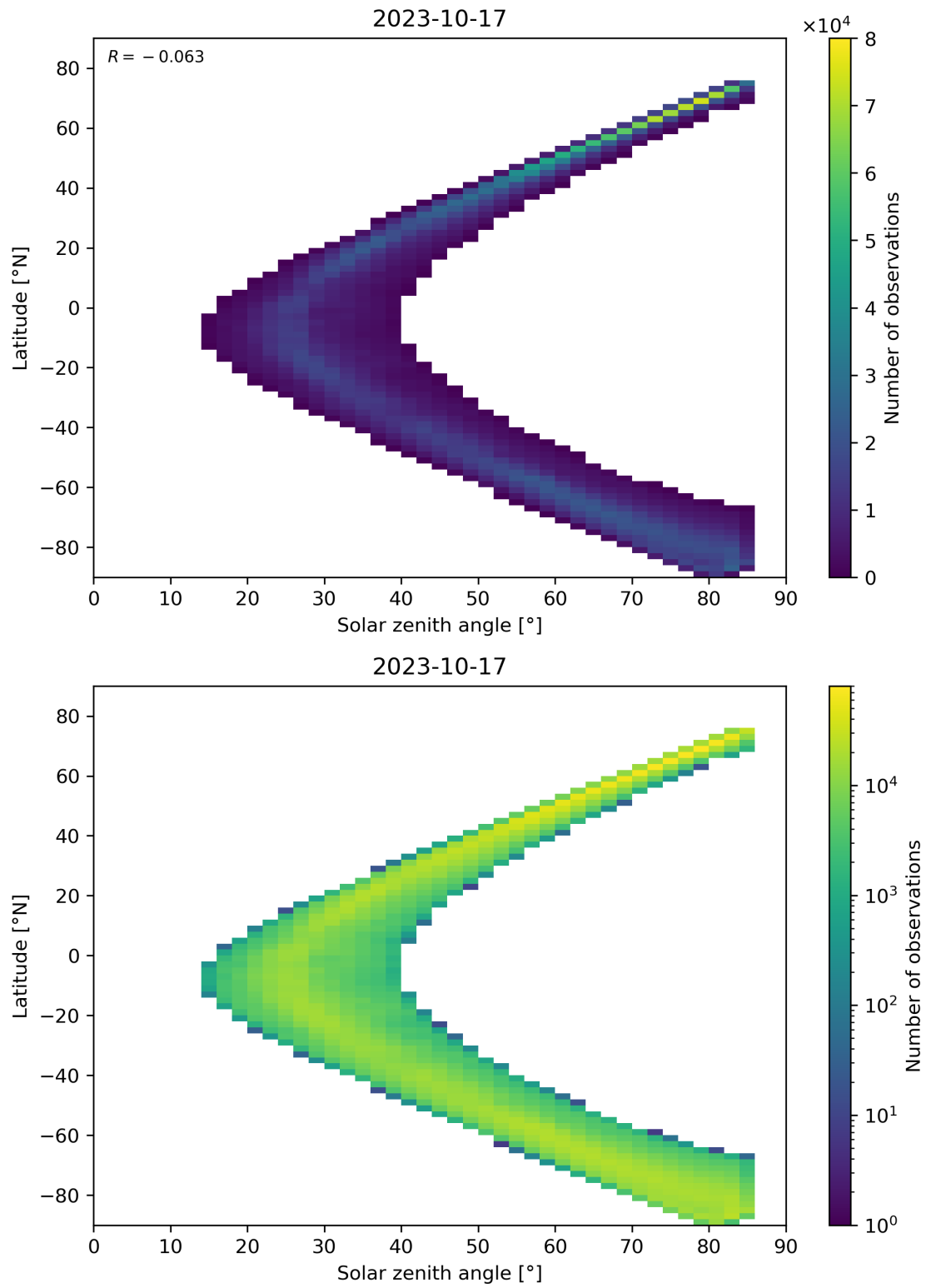
Figure 66: Scatter density plot of “Solar zenith angle” against “Latitude” for 2023-10-17 to 2023-10-18.
