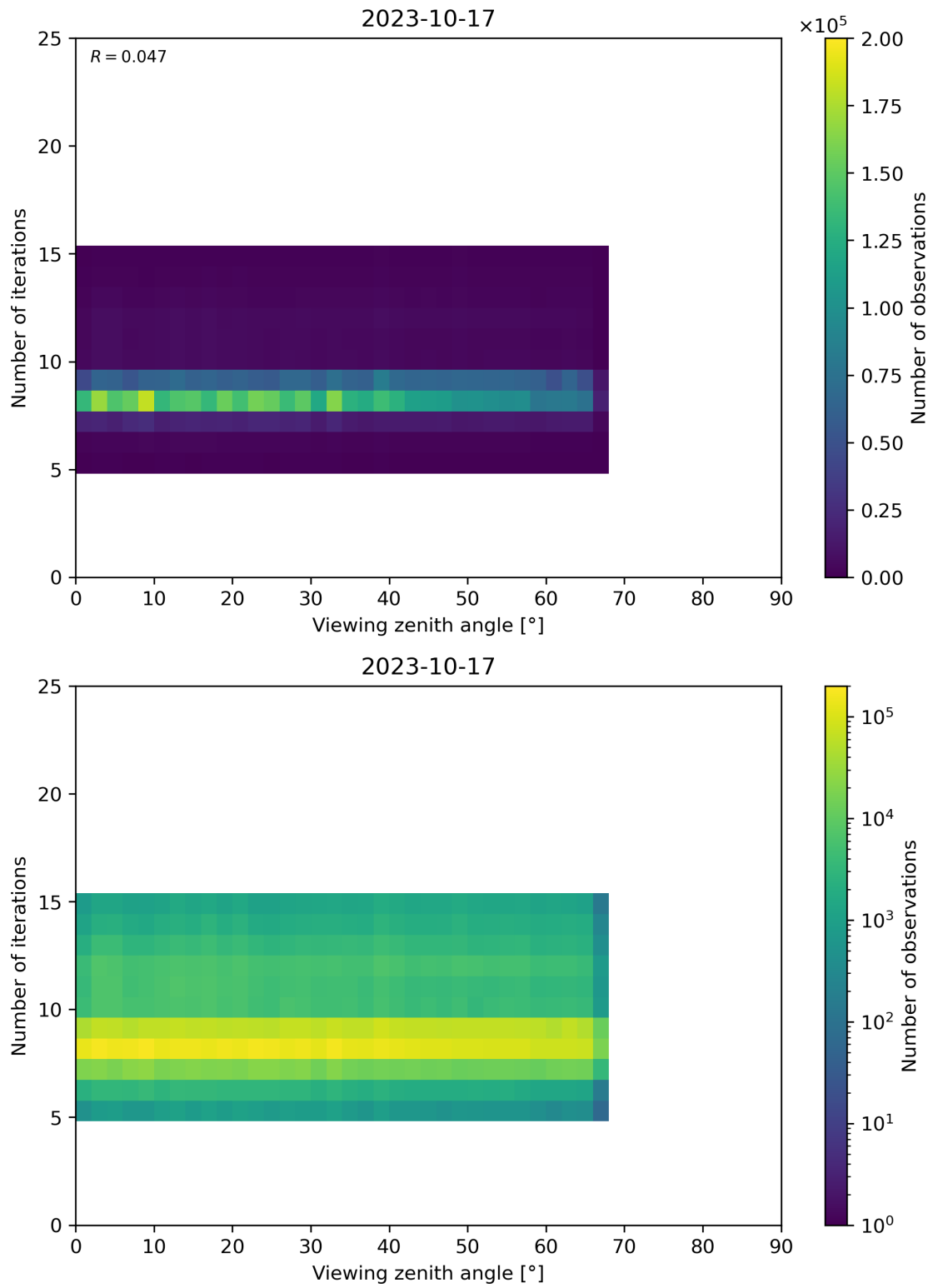
Figure 75: Scatter density plot of “Viewing zenith angle” against “Number of iterations” for 2023-10-17 to 2023-10-18.
