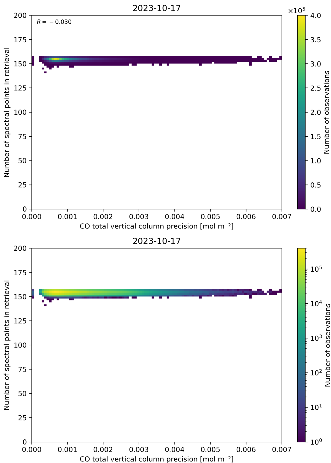
Figure 47: Scatter density plot of “CO total vertical column precision” against “Number of spectral points in retrieval” for 2023-10-17 to 2023-10-18.
