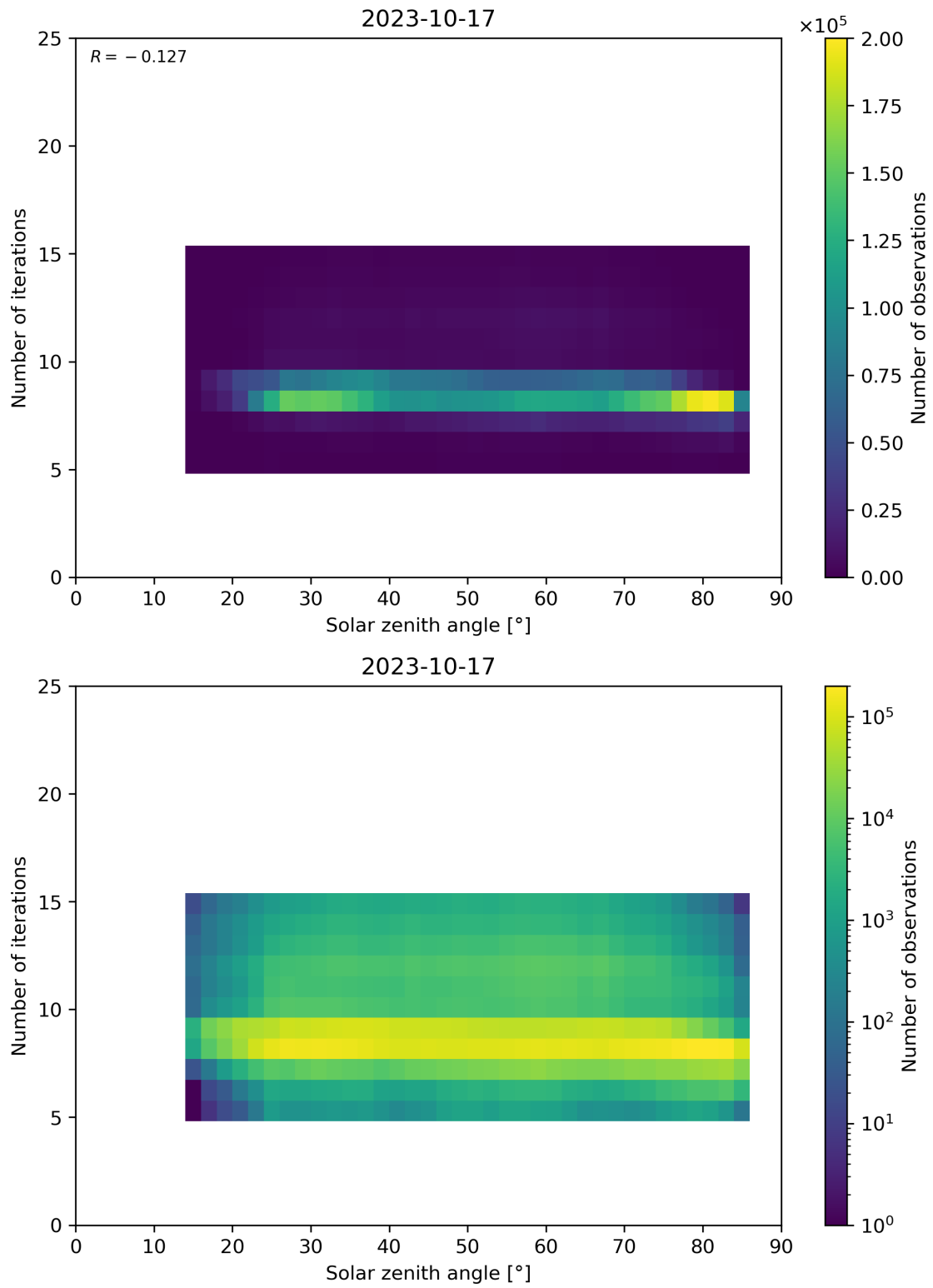
Figure 67: Scatter density plot of “Solar zenith angle” against “Number of iterations” for 2023-10-17 to 2023-10-18.
