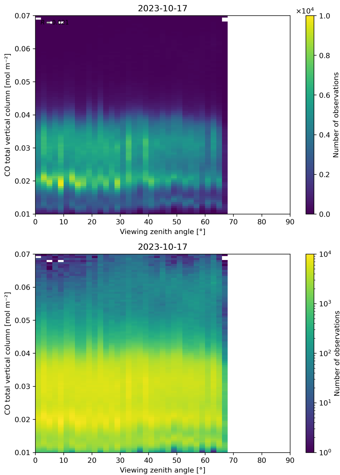
Figure 69: Scatter density plot of “Viewing zenith angle” against “CO total vertical column” for 2023-10-17 to 2023-10-18.
