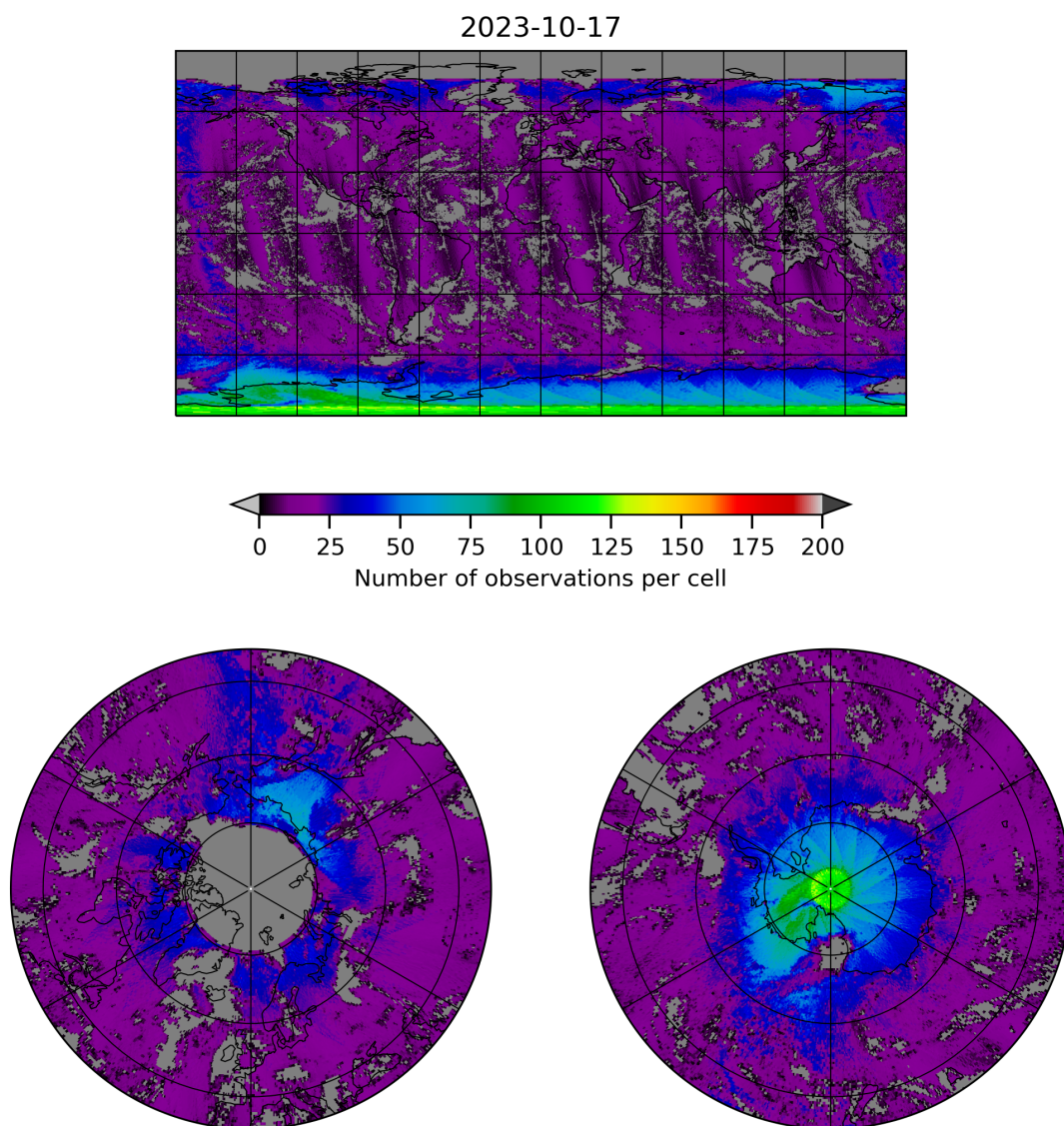
Figure 8: Map of the number of observations for 2023-10-17 to 2023-10-18
