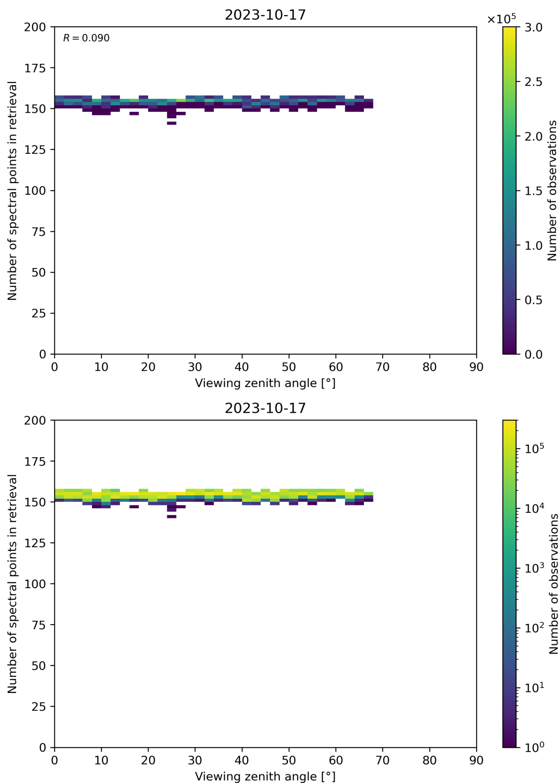
Figure 76: Scatter density plot of “Viewing zenith angle” against “Number of spectral points in retrieval” for 2023-10-17 to 2023-10-18.
