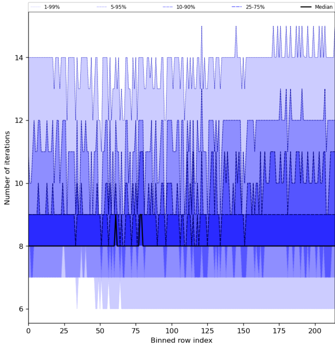
Figure 32: Along track statistics of “Number of iterations” for 2023-10-17 to 2023-10-18
