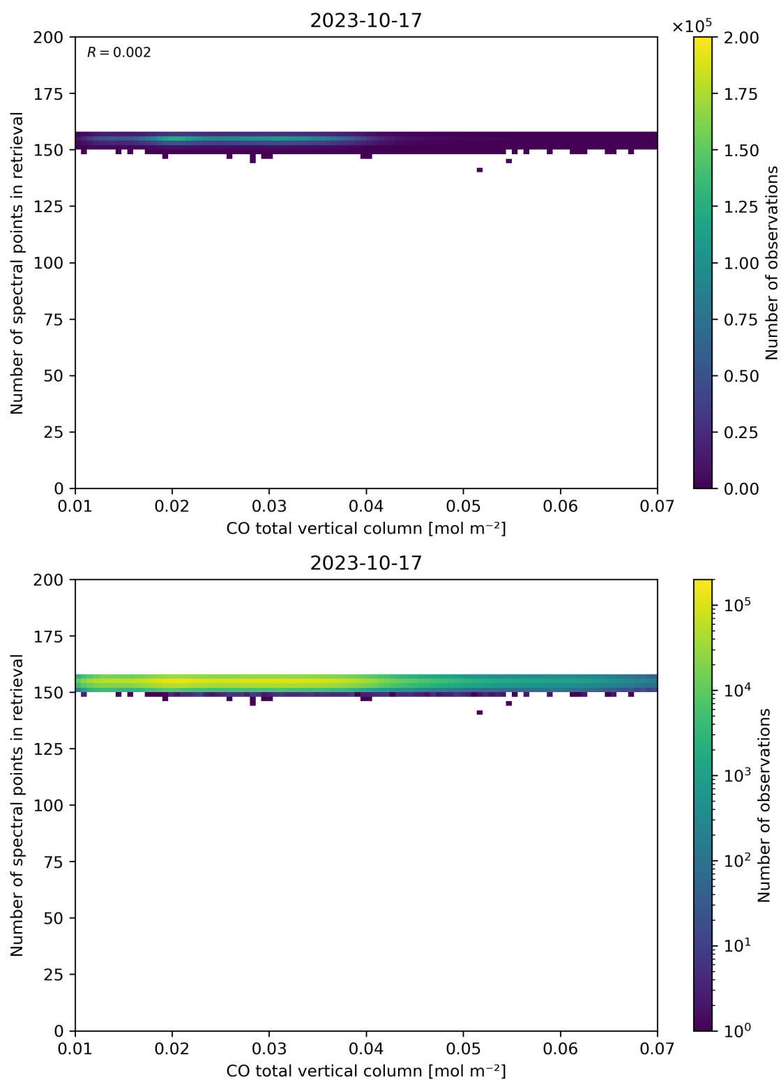
Figure 43: Scatter density plot of “CO total vertical column” against “Number of spectral points in retrieval” for 2023-10-17 to 2023-10-18.
