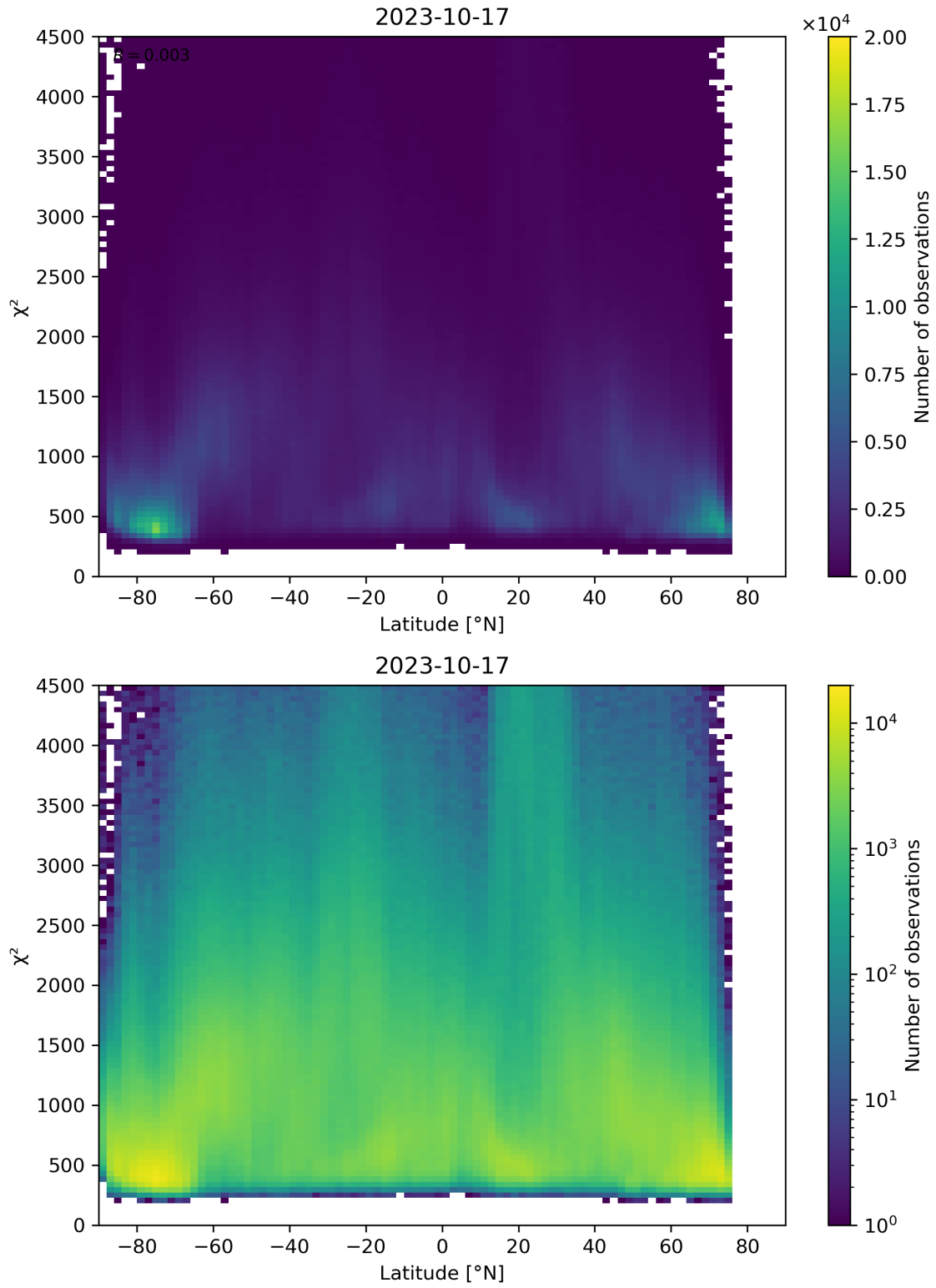
Figure 54: Scatter density plot of “Latitude” against “ \chi^2 ” for 2023-10-17 to 2023-10-18.
