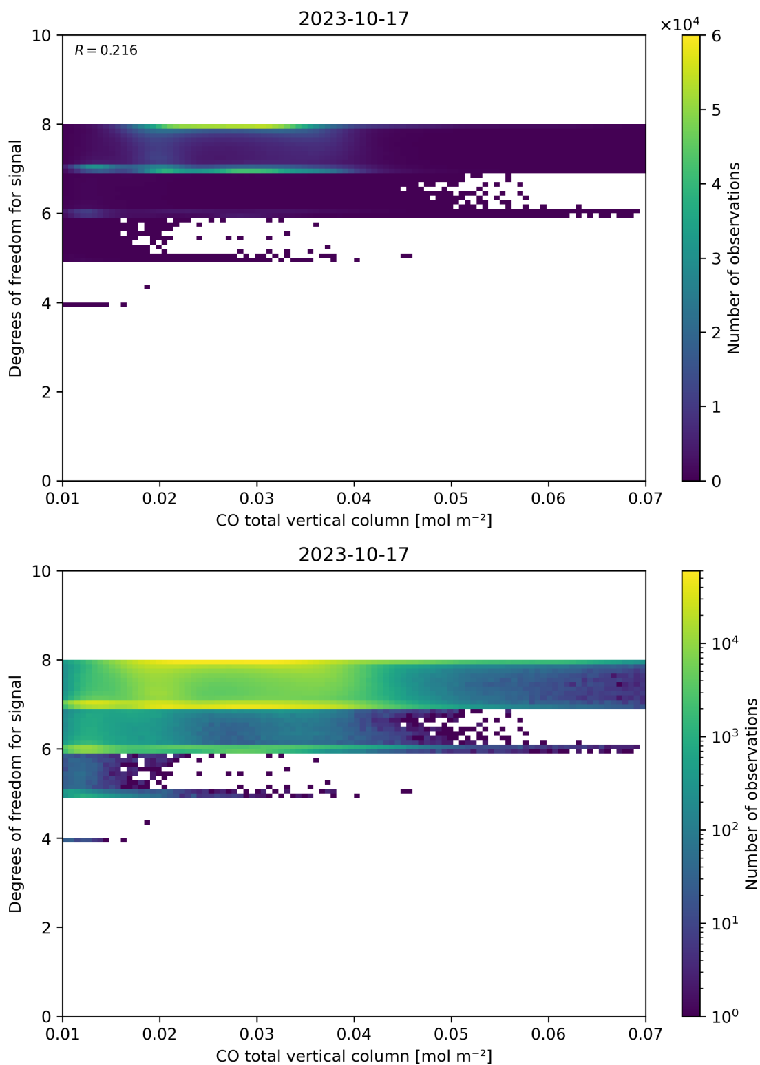
Figure 41: Scatter density plot of “CO total vertical column” against “Degrees of freedom for signal” for 2023-10-17 to 2023-10-18.
