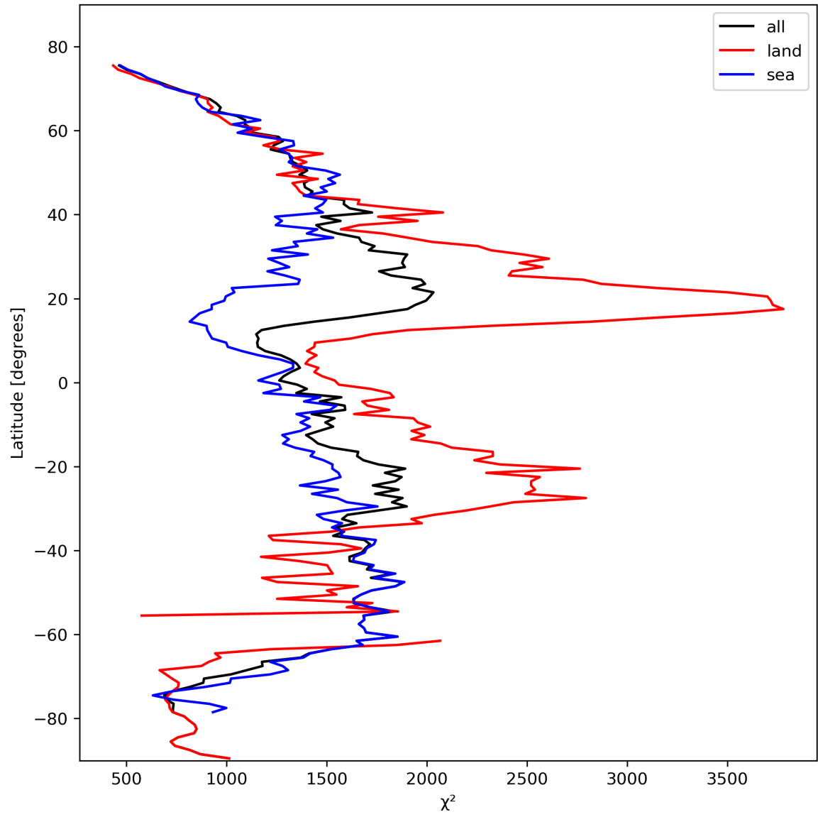
Figure 14: Zonal average of “ \chi^2 ” for 2023-10-17 to 2023-10-18.
