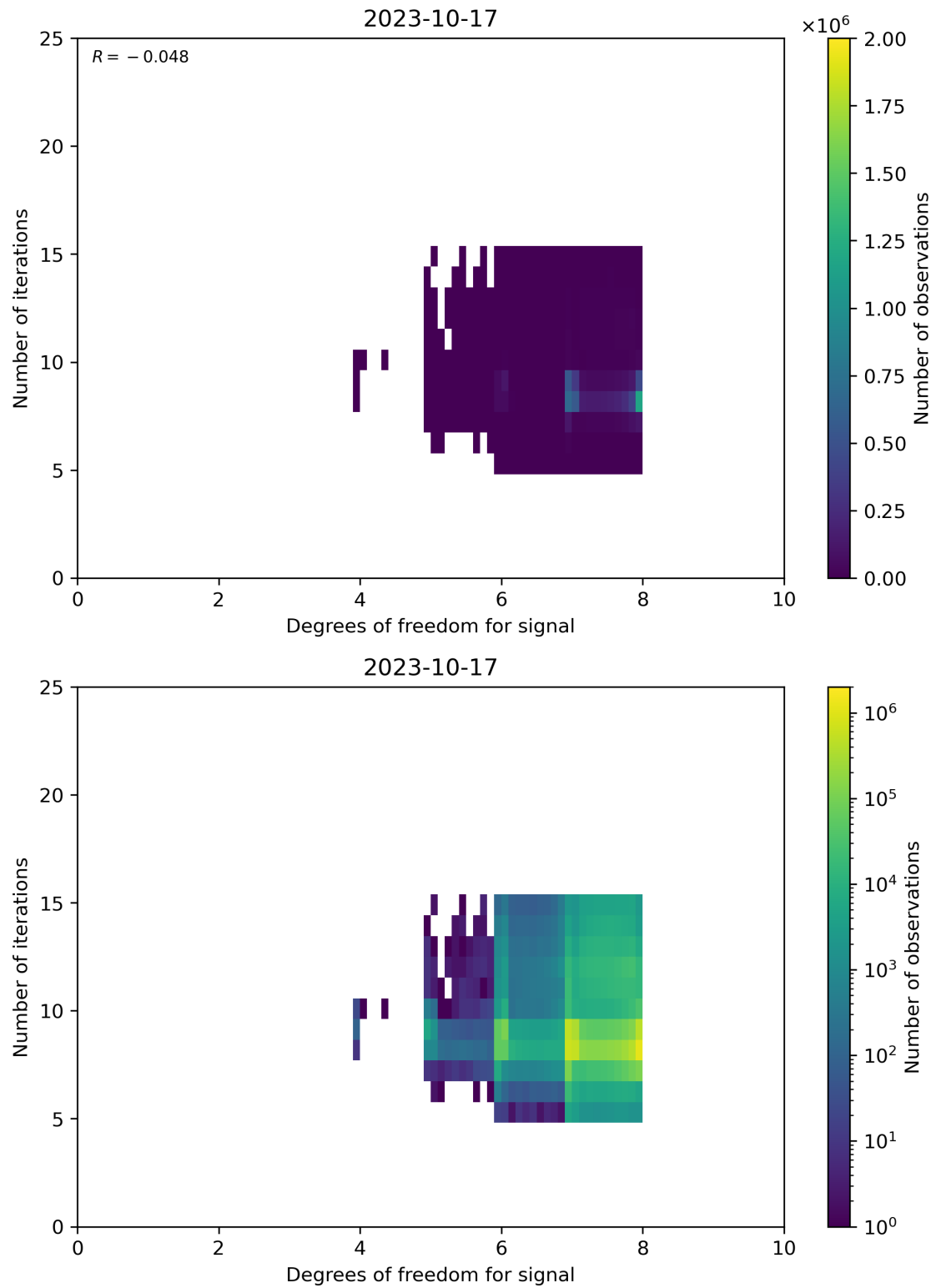
Figure 50: Scatter density plot of “Degrees of freedom for signal” against “Number of iterations” for 2023-10-17 to 2023-10-18.
