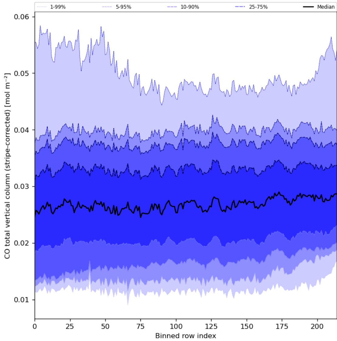
Figure 27: Along track statistics of “CO total vertical column (stripe-corrected)” for 2023-10-17 to 2023-10-18
