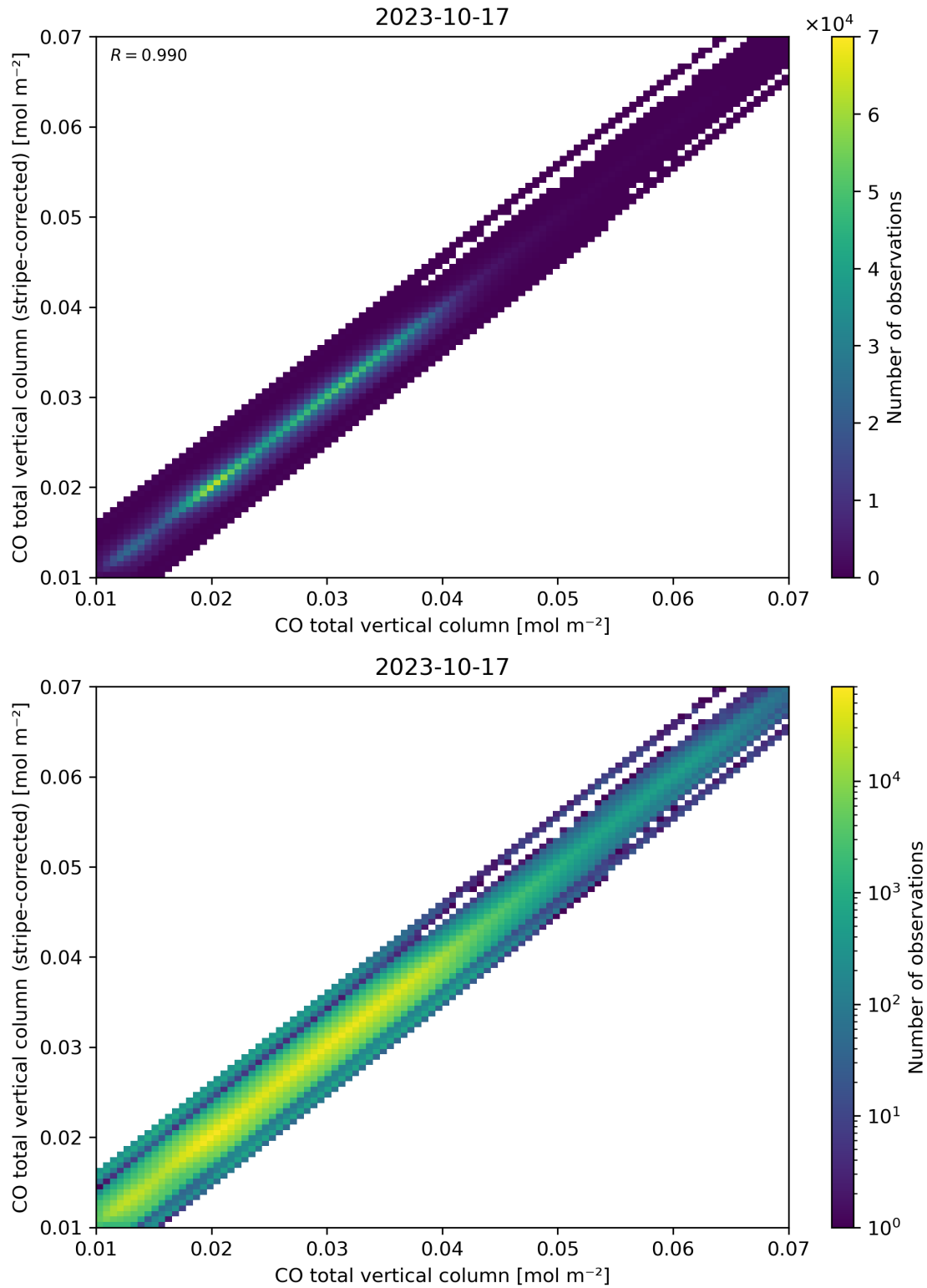
Figure 33: Scatter density plot of “CO total vertical column” against “CO total vertical column (stripe-corrected)” for 2023-10-17 to 2023-10-18.
