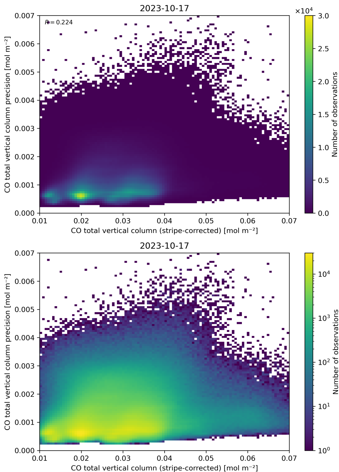
Figure 36: Scatter density plot of “CO total vertical column (stripe-corrected)” against “CO total vertical column precision” for 2023-10-17 to 2023-10-18.
