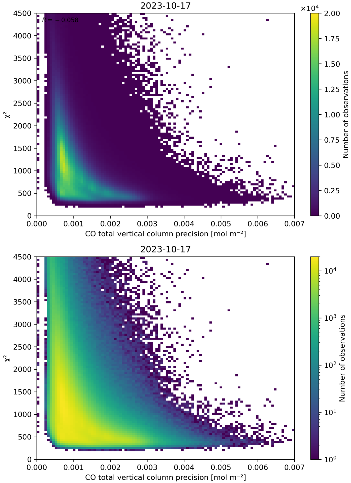
Figure 44: Scatter density plot of “CO total vertical column precision” against “ \chi^2 ” for 2023-10-17 to 2023-10-18.
