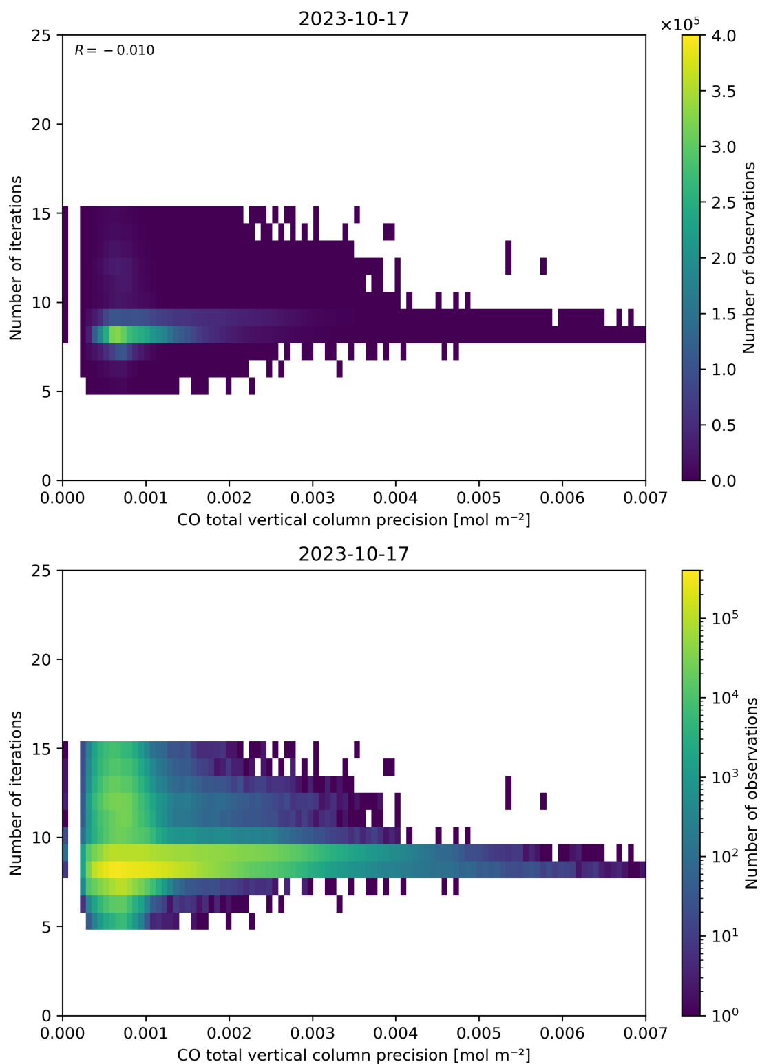
Figure 46: Scatter density plot of “CO total vertical column precision” against “Number of iterations” for 2023-10-17 to 2023-10-18.
