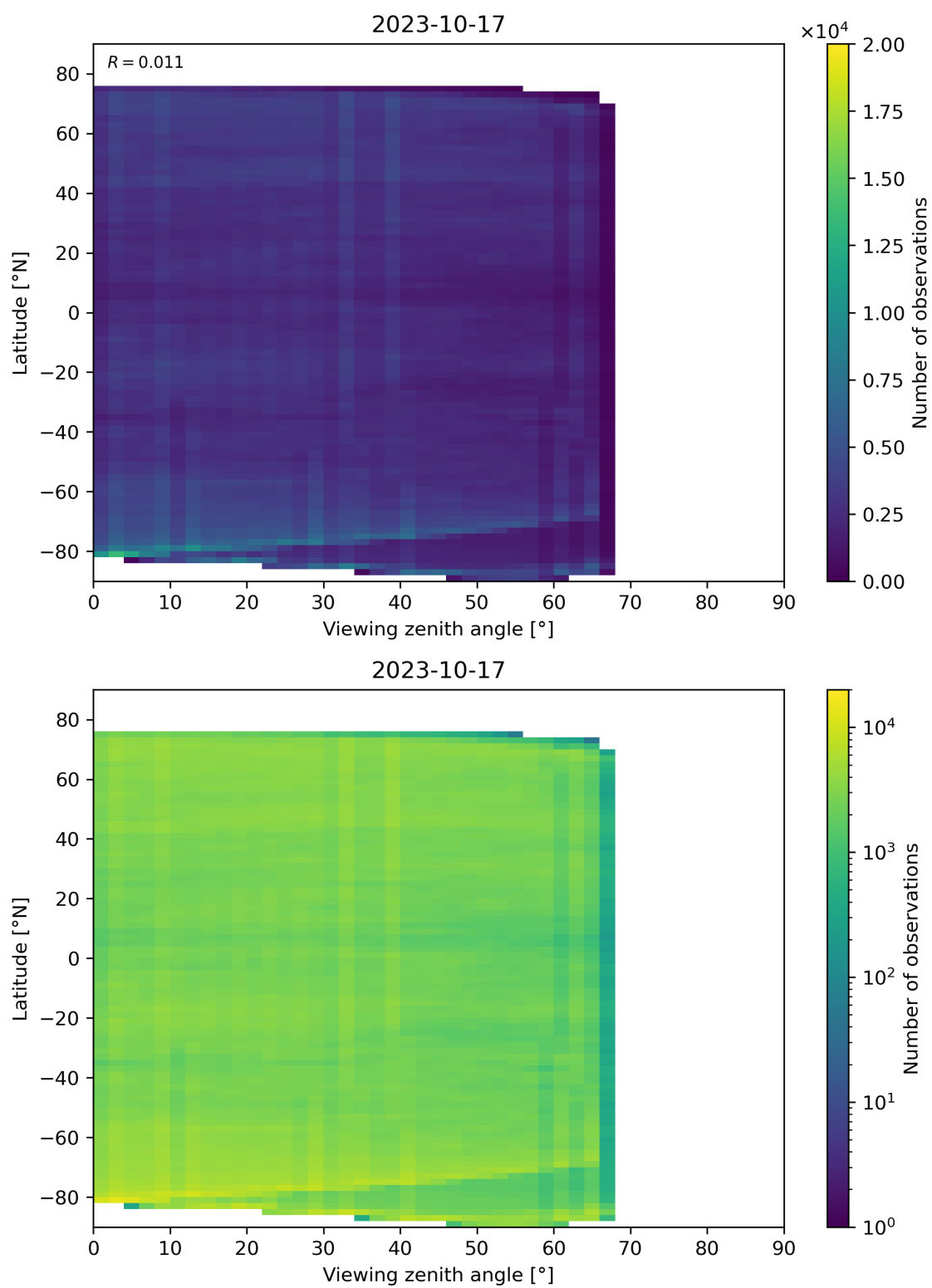
Figure 74: Scatter density plot of “Viewing zenith angle” against “Latitude” for 2023-10-17 to 2023-10-18.
