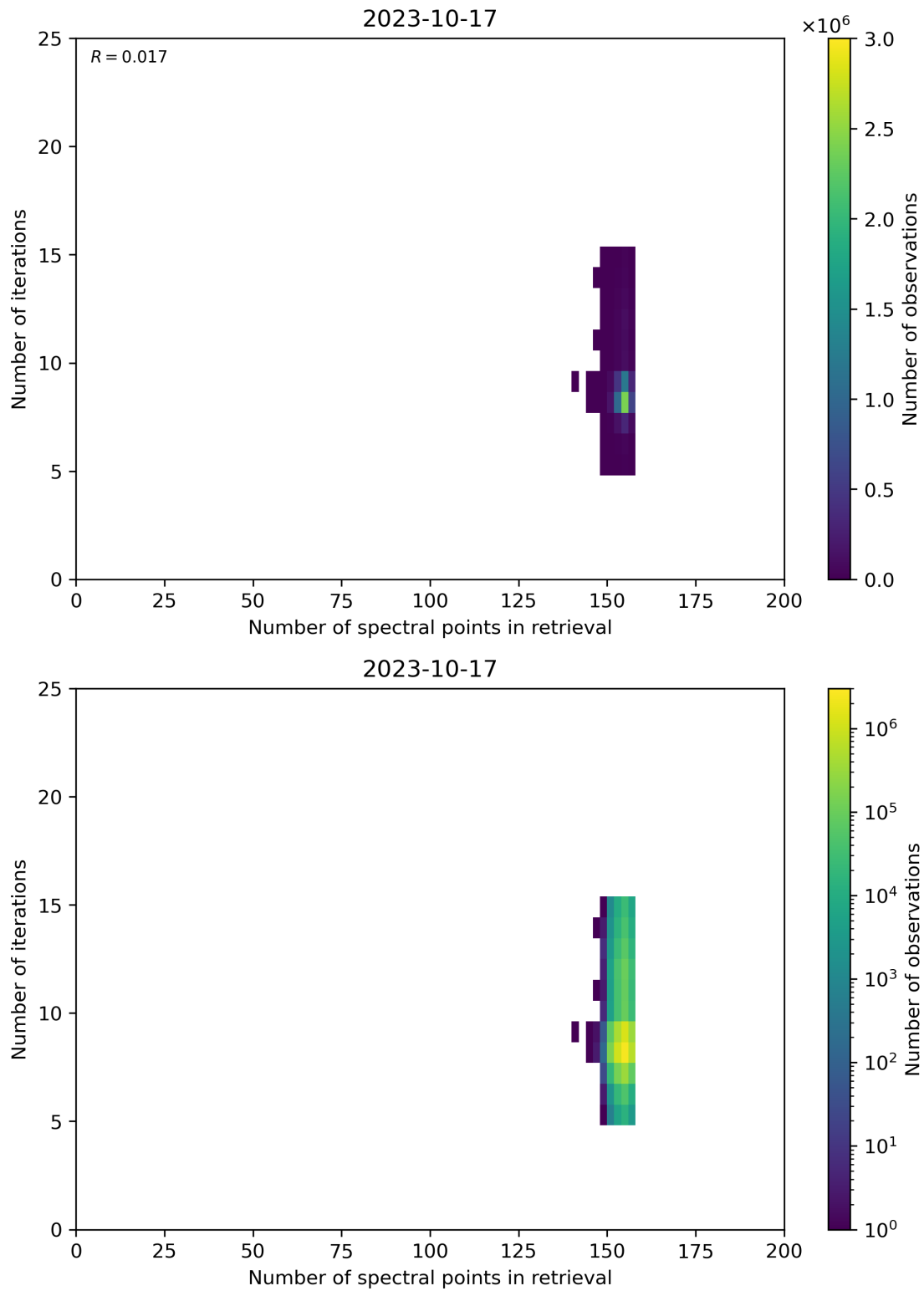
Figure 60: Scatter density plot of “Number of spectral points in retrieval” against “Number of iterations” for 2023-10-17 to 2023-10-18.
