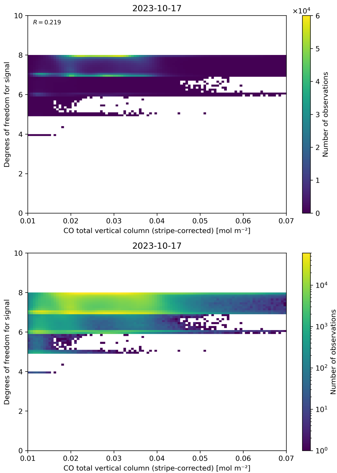
Figure 38: Scatter density plot of “CO total vertical column (stripe-corrected)” against “Degrees of freedom for signal” for 2023-10-17 to 2023-10-18.
