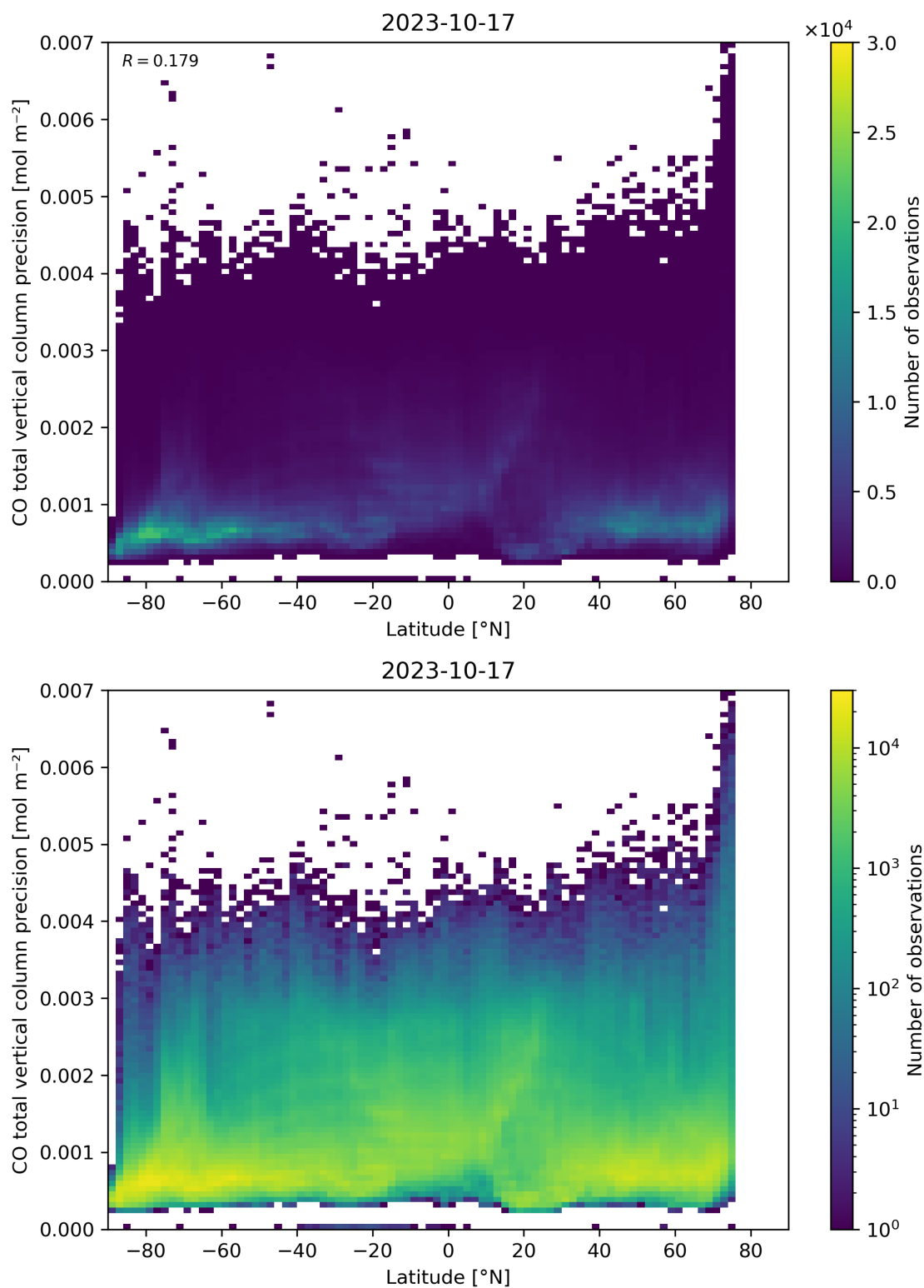
Figure 53: Scatter density plot of “Latitude” against “CO total vertical column precision” for 2023-10-17 to 2023-10-18.
