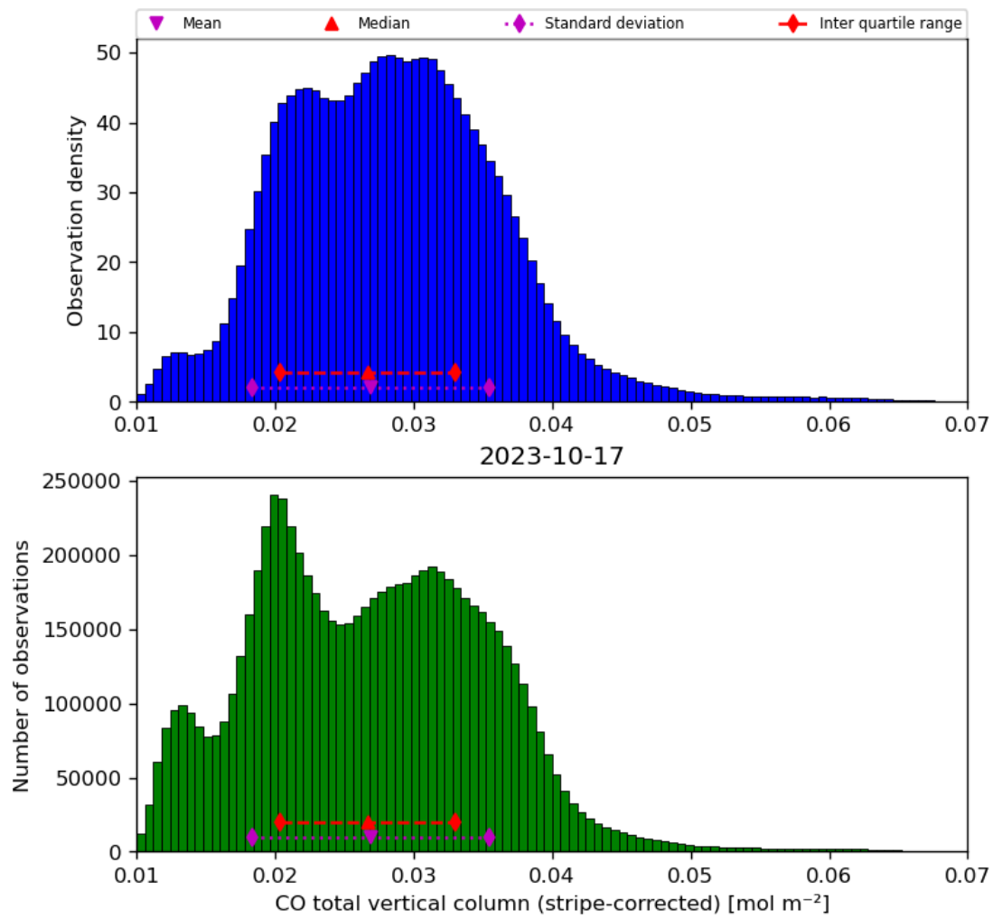
Figure 19: Histogram of “CO total vertical column (stripe-corrected)” for 2023-10-17 to 2023-10-18
