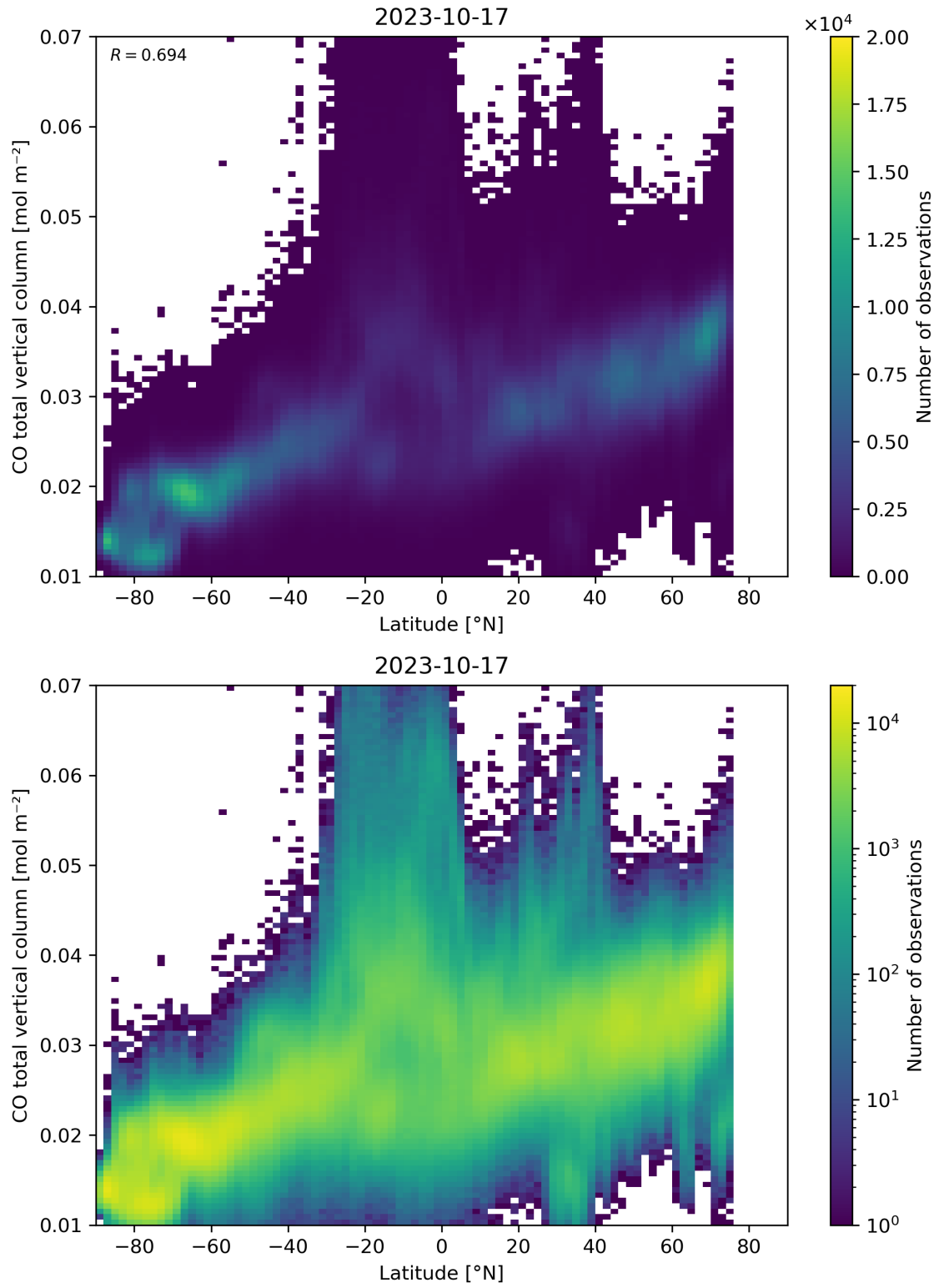
Figure 51: Scatter density plot of “Latitude” against “CO total vertical column” for 2023-10-17 to 2023-10-18.
