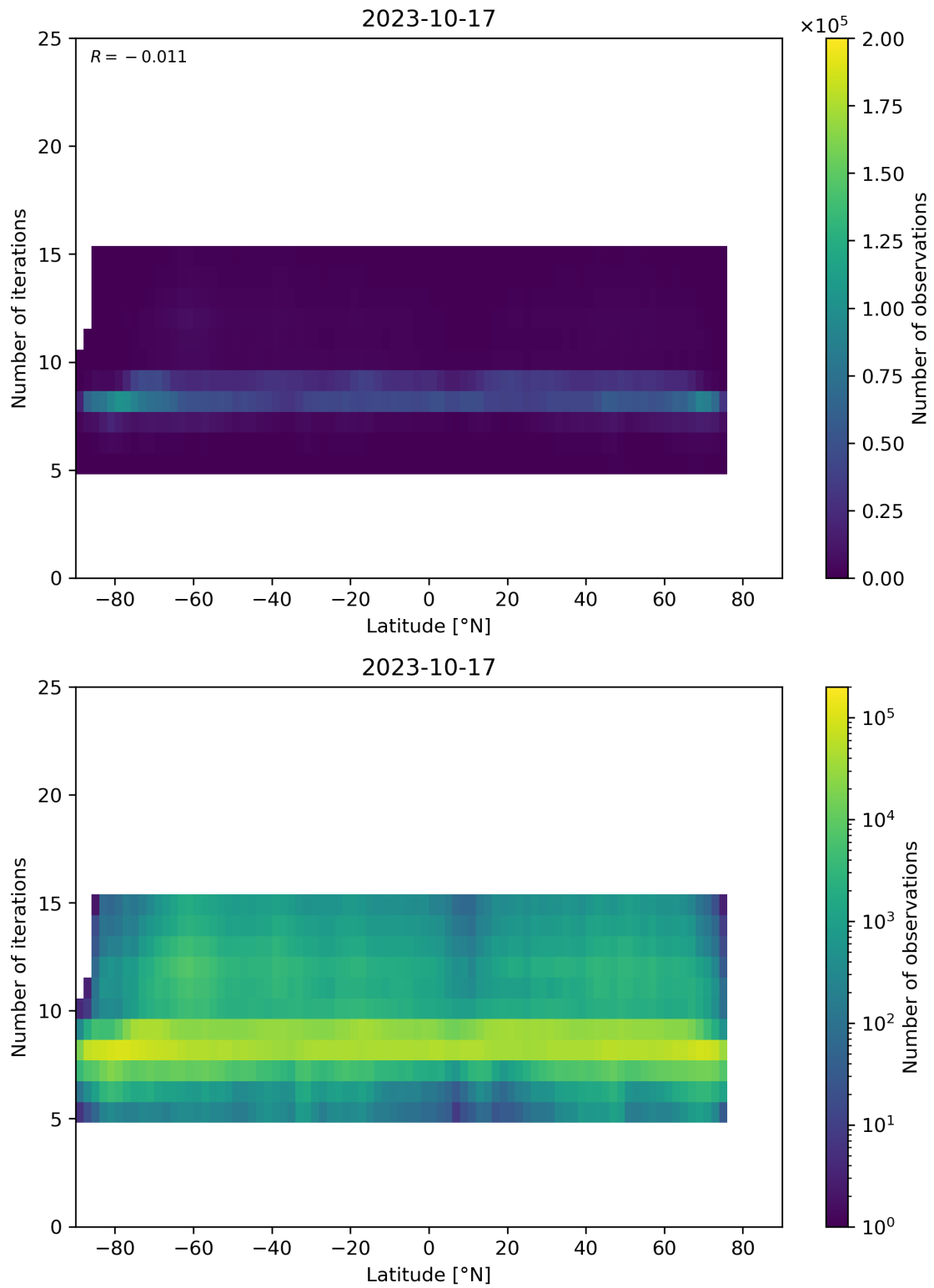
Figure 56: Scatter density plot of “Latitude” against “Number of iterations” for 2023-10-17 to 2023-10-18.
