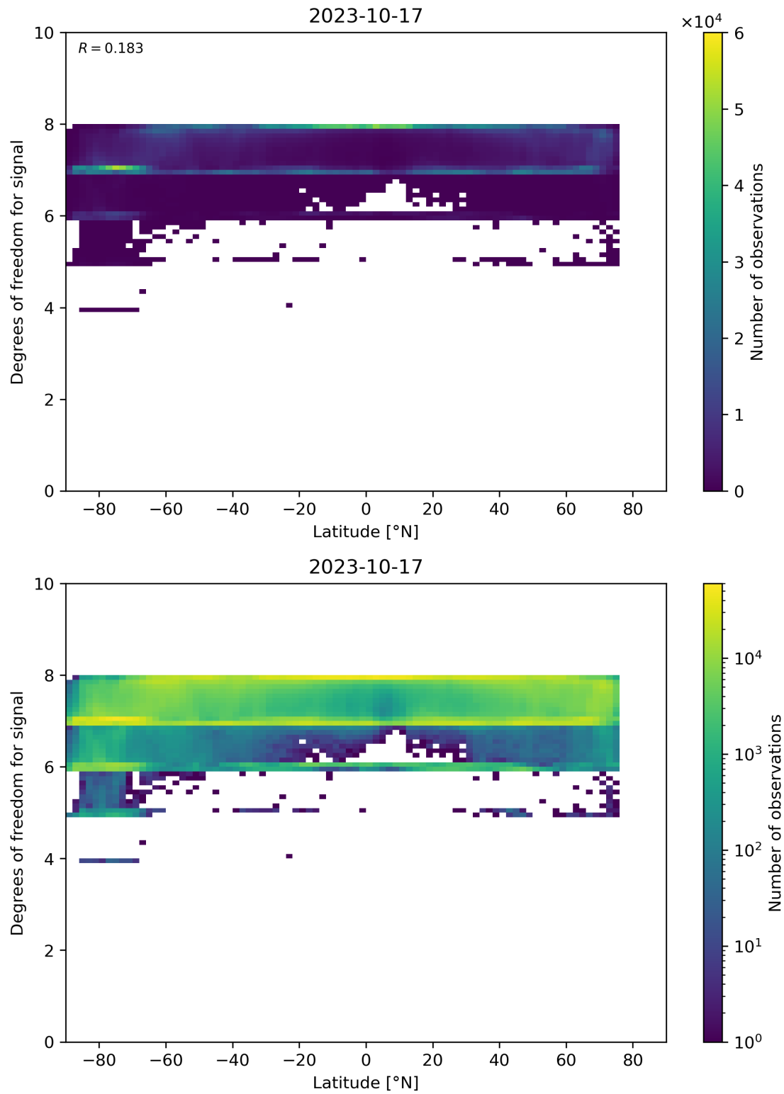
Figure 55: Scatter density plot of “Latitude” against “Degrees of freedom for signal” for 2023-10-17 to 2023-10-18.
