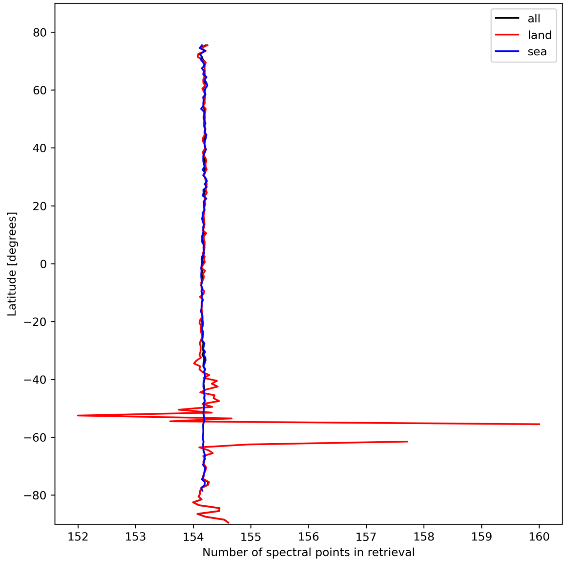
Figure 13: Zonal average of “Number of spectral points in retrieval” for 2023-10-17 to 2023-10-18.
