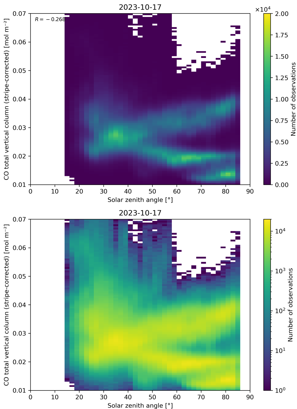
Figure 62: Scatter density plot of “Solar zenith angle” against “CO total vertical column (stripe-corrected)” for 2023-10-17 to 2023-10-18.
