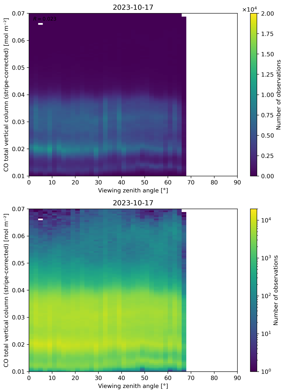
Figure 70: Scatter density plot of “Viewing zenith angle” against “CO total vertical column (stripe-corrected)” for 2023-10-17 to 2023-10-18.
