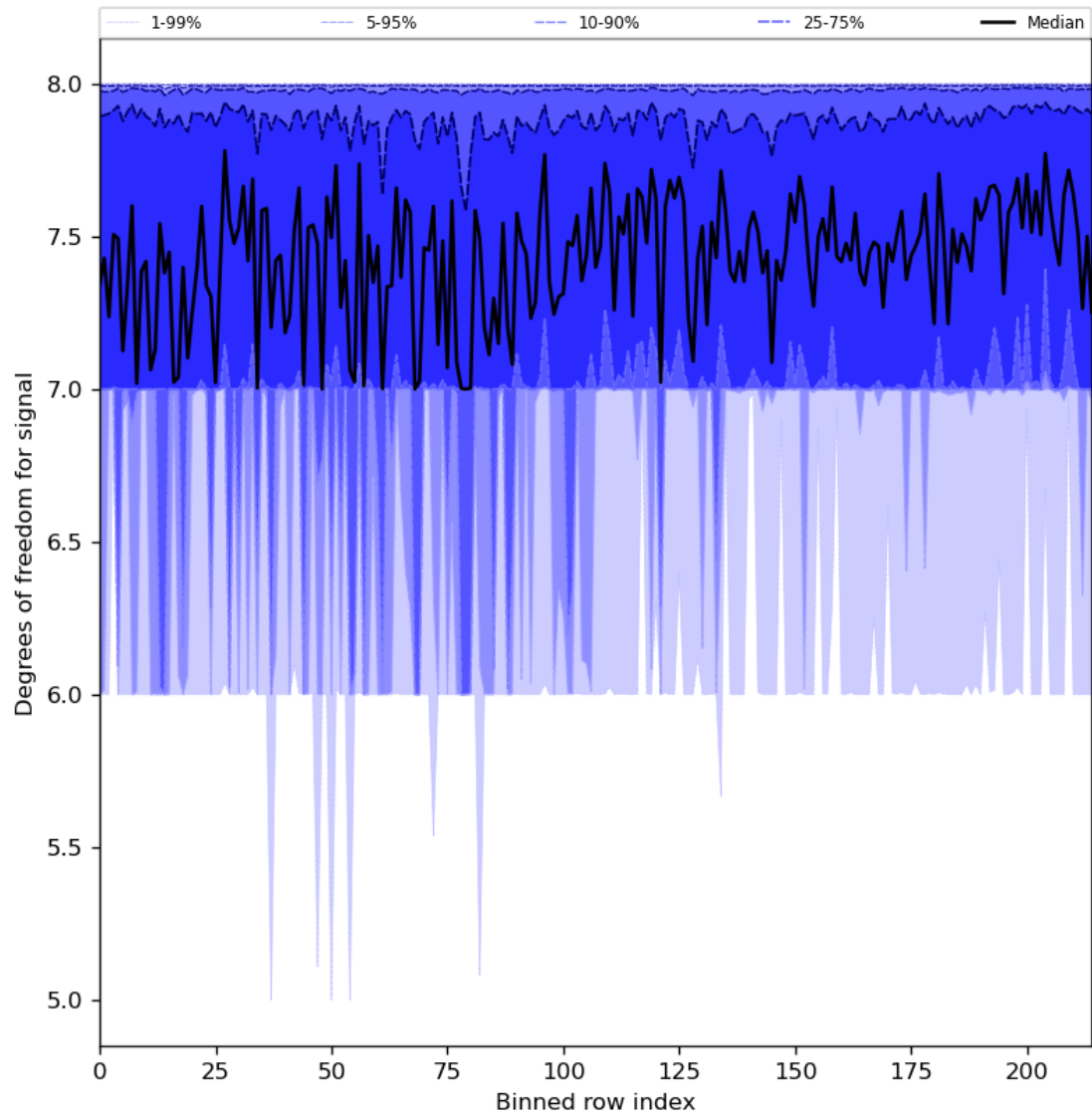
Figure 31: Along track statistics of “Degrees of freedom for signal” for 2023-10-17 to 2023-10-18
