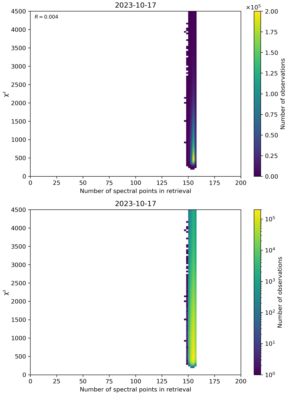
Figure 58: Scatter density plot of “Number of spectral points in retrieval” against “ \chi^2 ” for 2023-10-17 to 2023-10-18.
