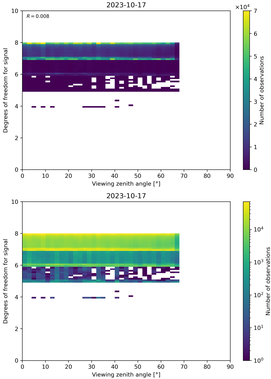
Figure 73: Scatter density plot of “Viewing zenith angle” against “Degrees of freedom for signal” for 2023-10-17 to 2023-10-18.
