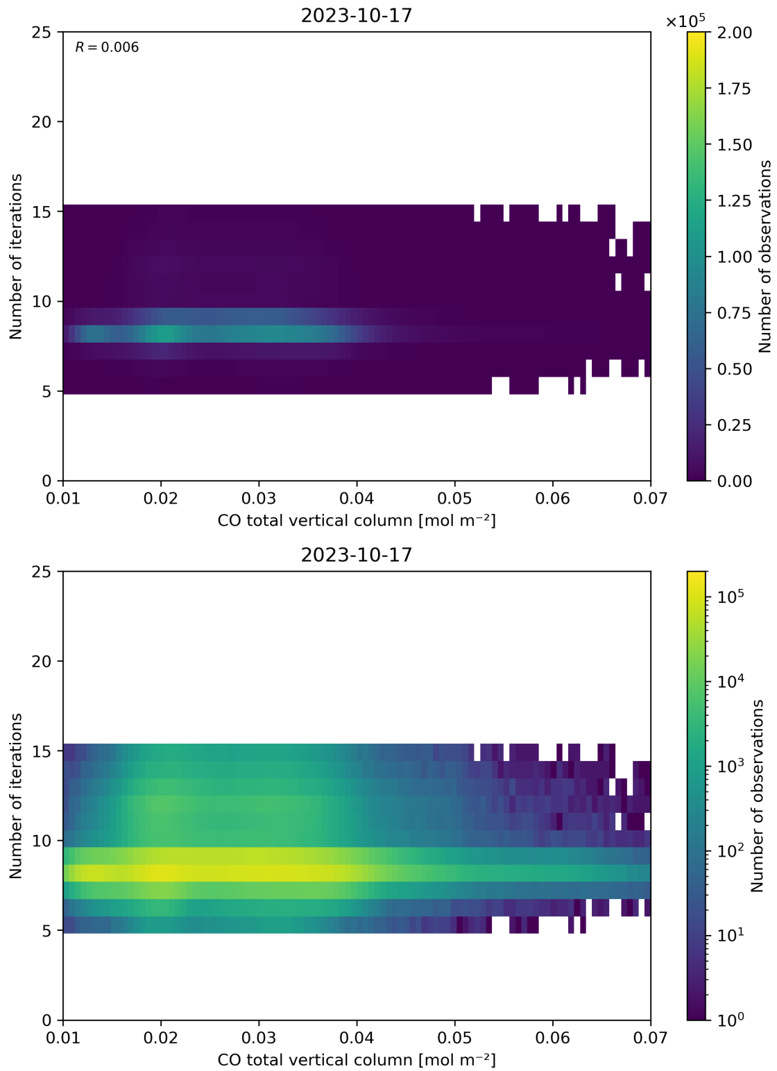
Figure 42: Scatter density plot of “CO total vertical column” against “Number of iterations” for 2023-10-17 to 2023-10-18.
