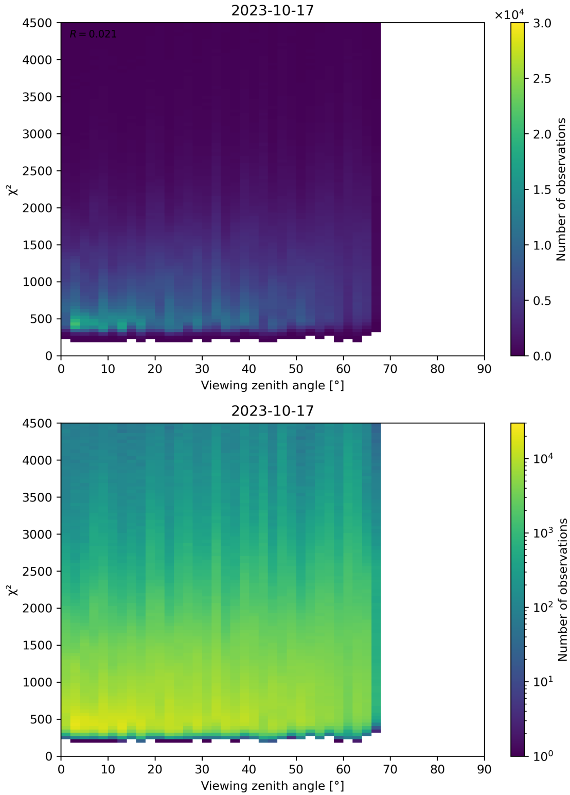
Figure 72: Scatter density plot of “Viewing zenith angle” against “ \chi^2 ” for 2023-10-17 to 2023-10-18.
