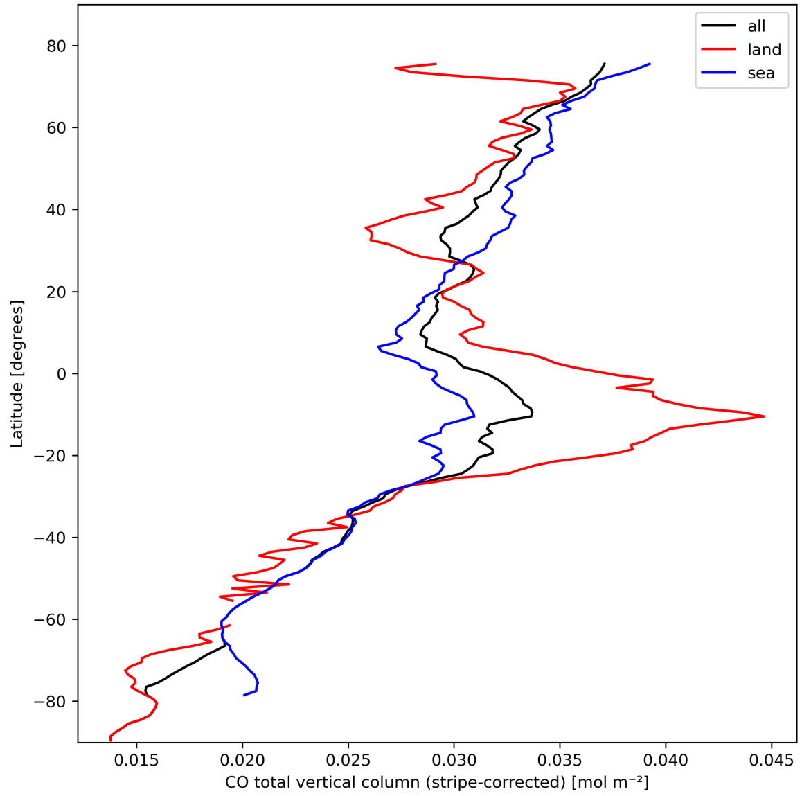
Figure 11: Zonal average of “CO total vertical column (stripe-corrected)” for 2023-10-17 to 2023-10-18.
