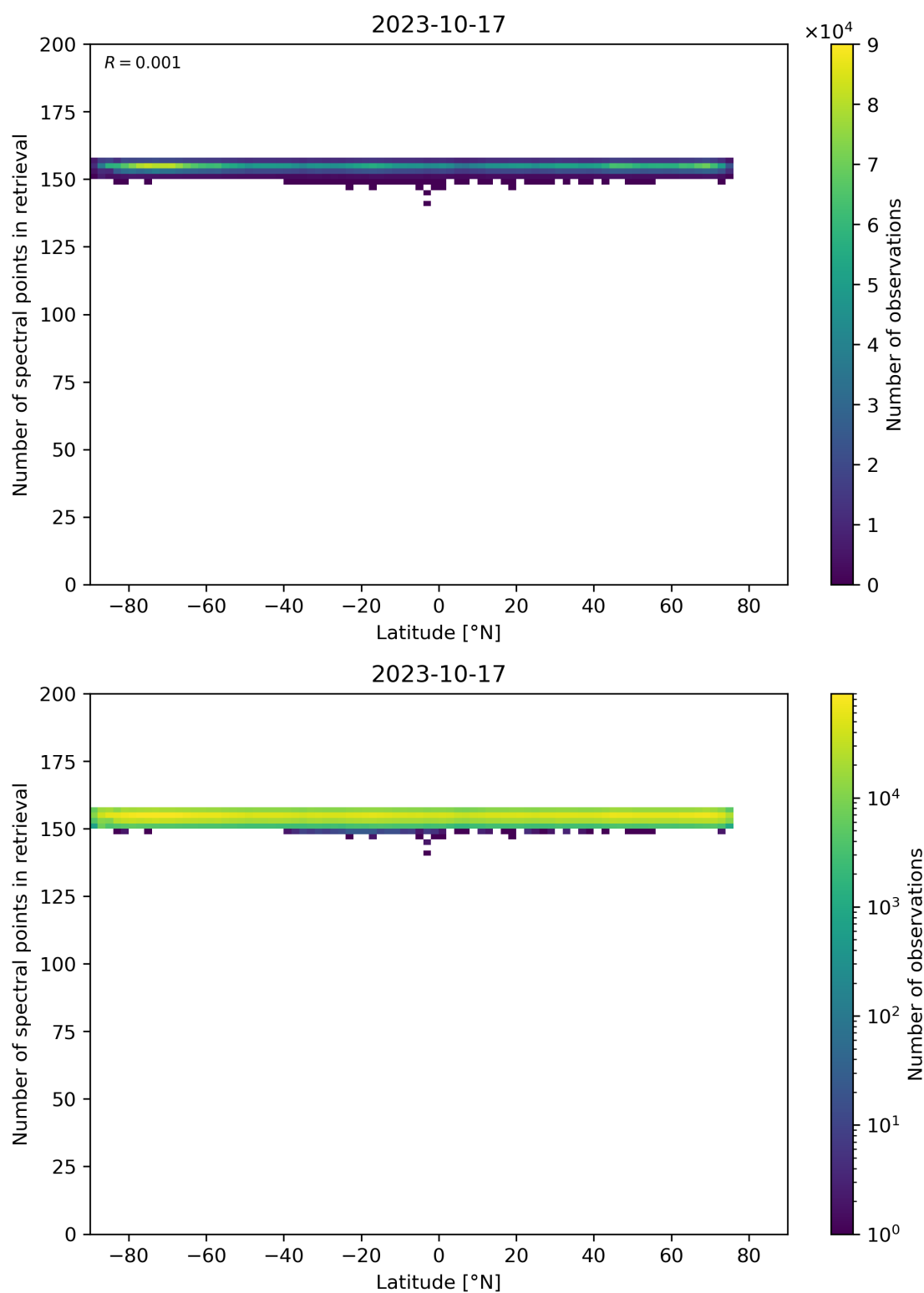
Figure 57: Scatter density plot of “Latitude” against “Number of spectral points in retrieval” for 2023-10-17 to 2023-10-18.
