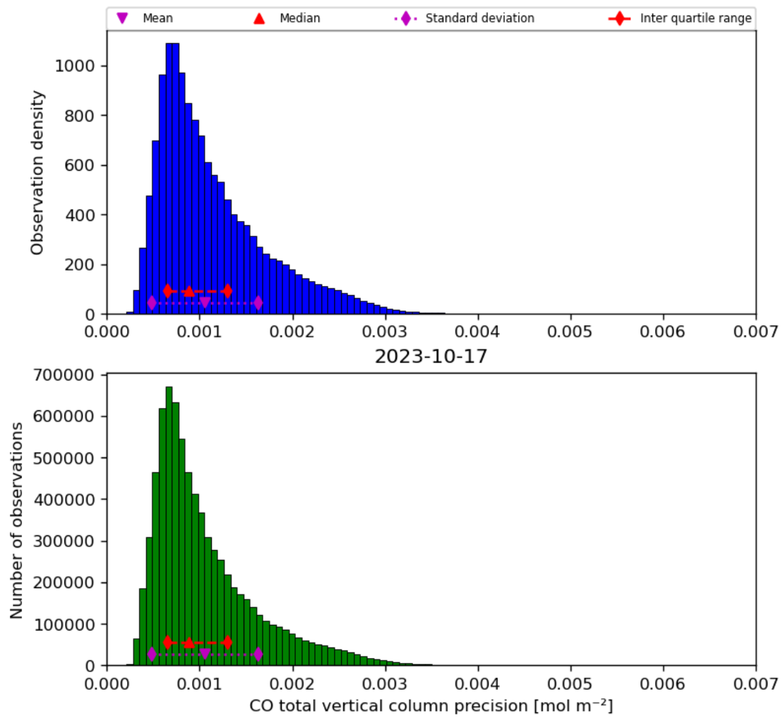
Figure 20: Histogram of “CO total vertical column precision” for 2023-10-17 to 2023-10-18
