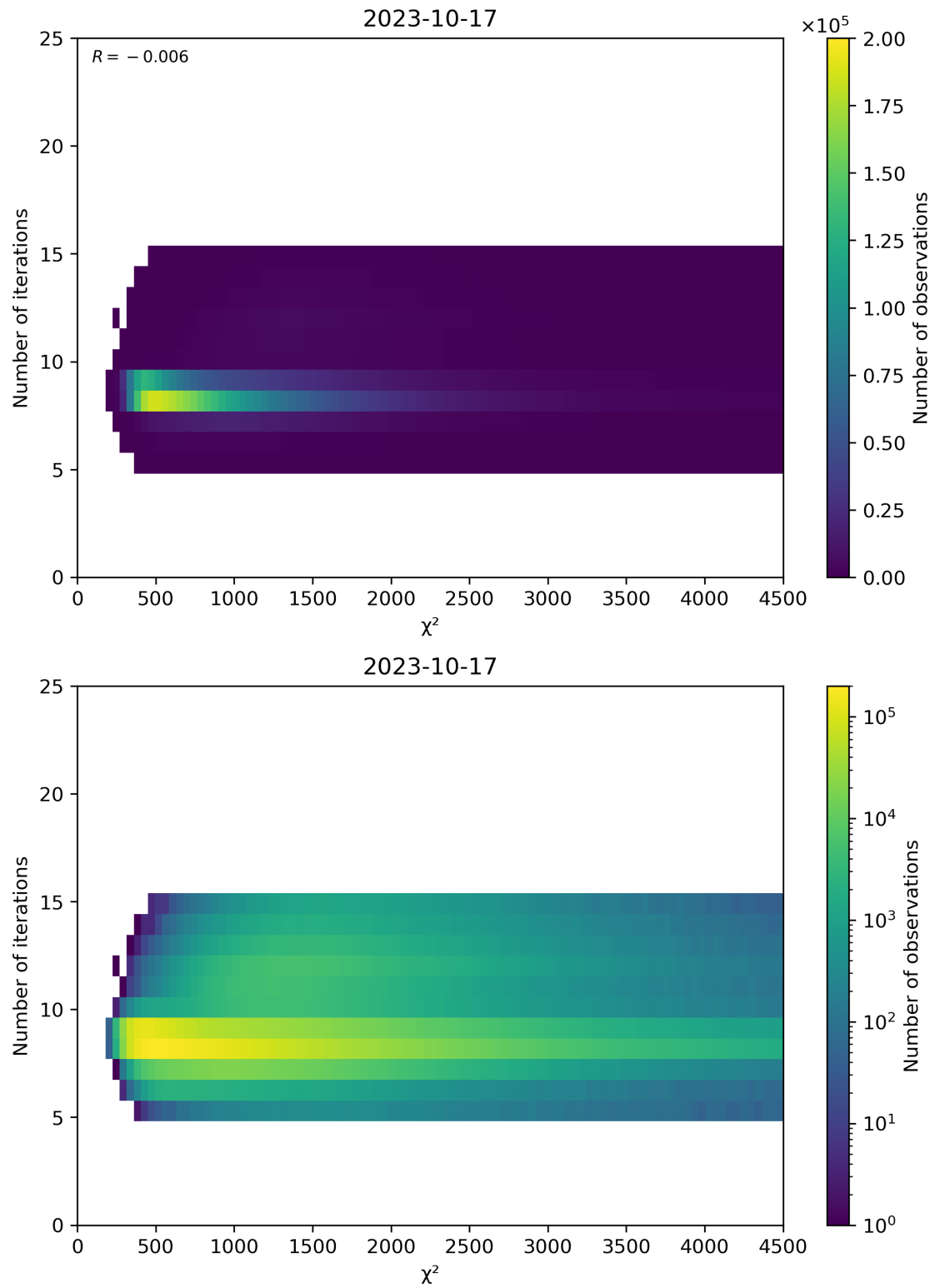
Figure 49: Scatter density plot of “ \chi^2 ” against “Number of iterations” for 2023-10-17 to 2023-10-18.
