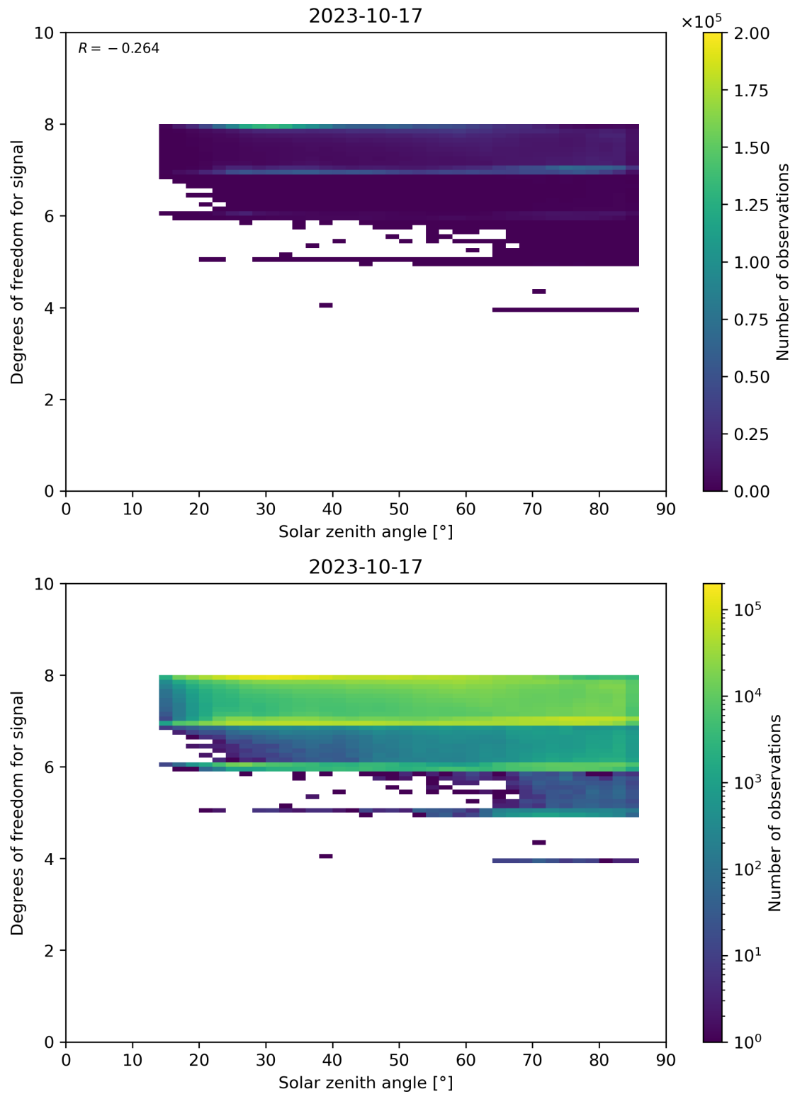
Figure 65: Scatter density plot of “Solar zenith angle” against “Degrees of freedom for signal” for 2023-10-17 to 2023-10-18.
