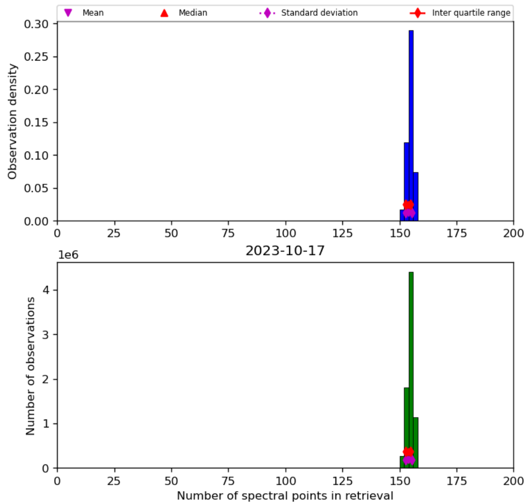
Figure 21: Histogram of “Number of spectral points in retrieval” for 2023-10-17 to 2023-10-18
