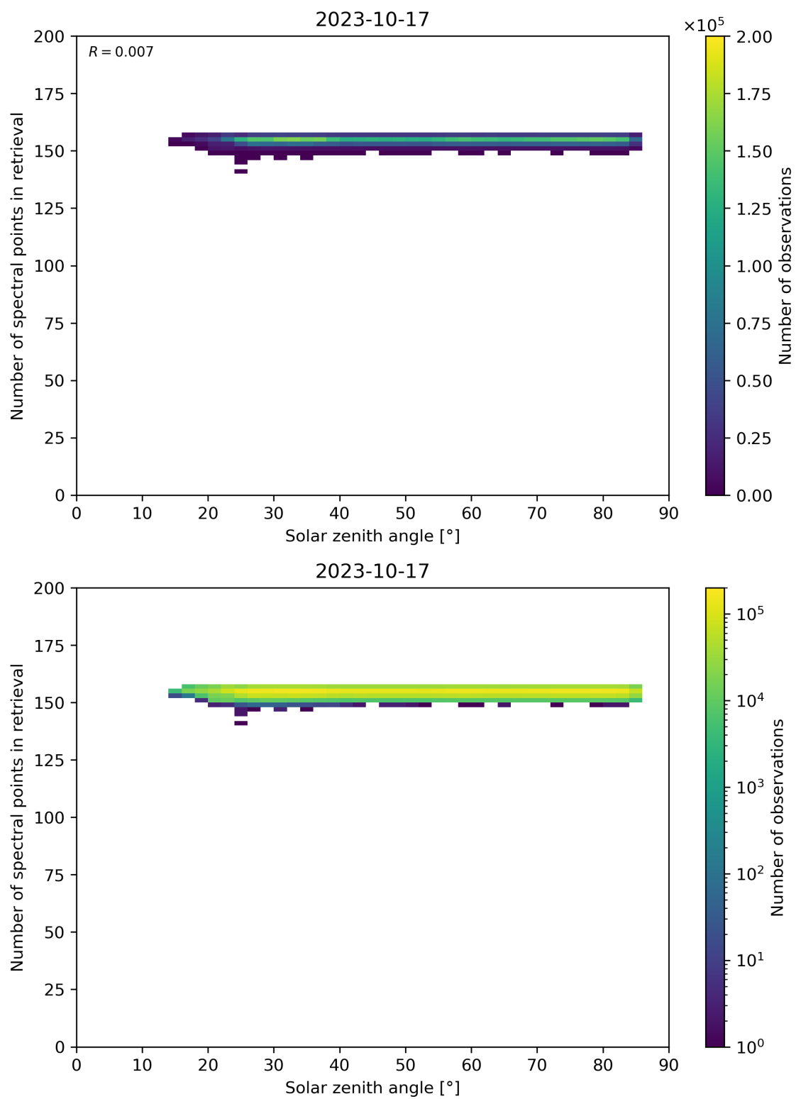
Figure 68: Scatter density plot of “Solar zenith angle” against “Number of spectral points in retrieval” for 2023-10-17 to 2023-10-18.
