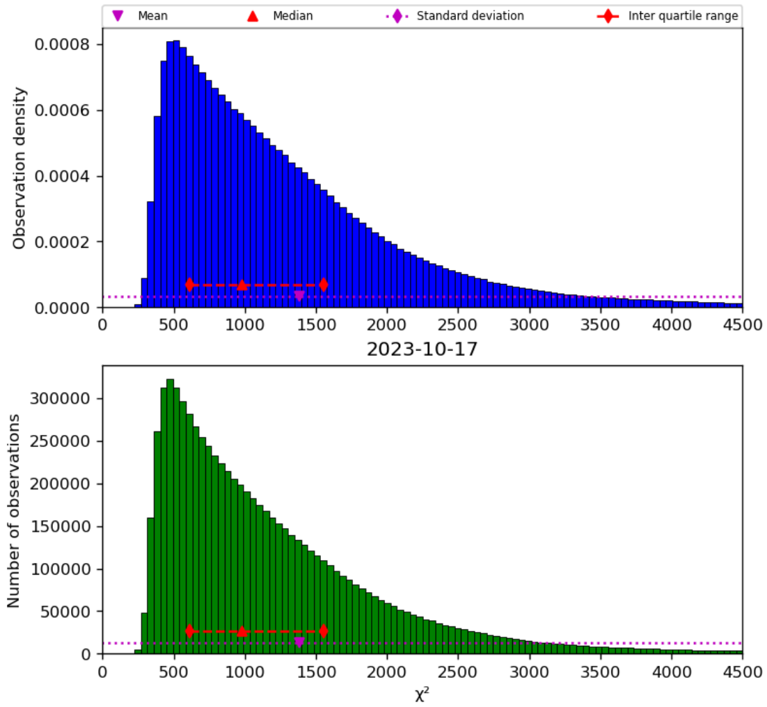
Figure 22: Histogram of “ \chi^2 ” for 2023-10-17 to 2023-10-18
