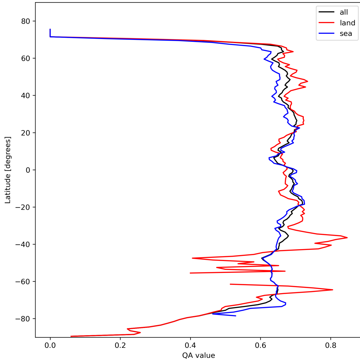
Figure 9: Zonal average of “QA value” for 2023-10-17 to 2023-10-18.
