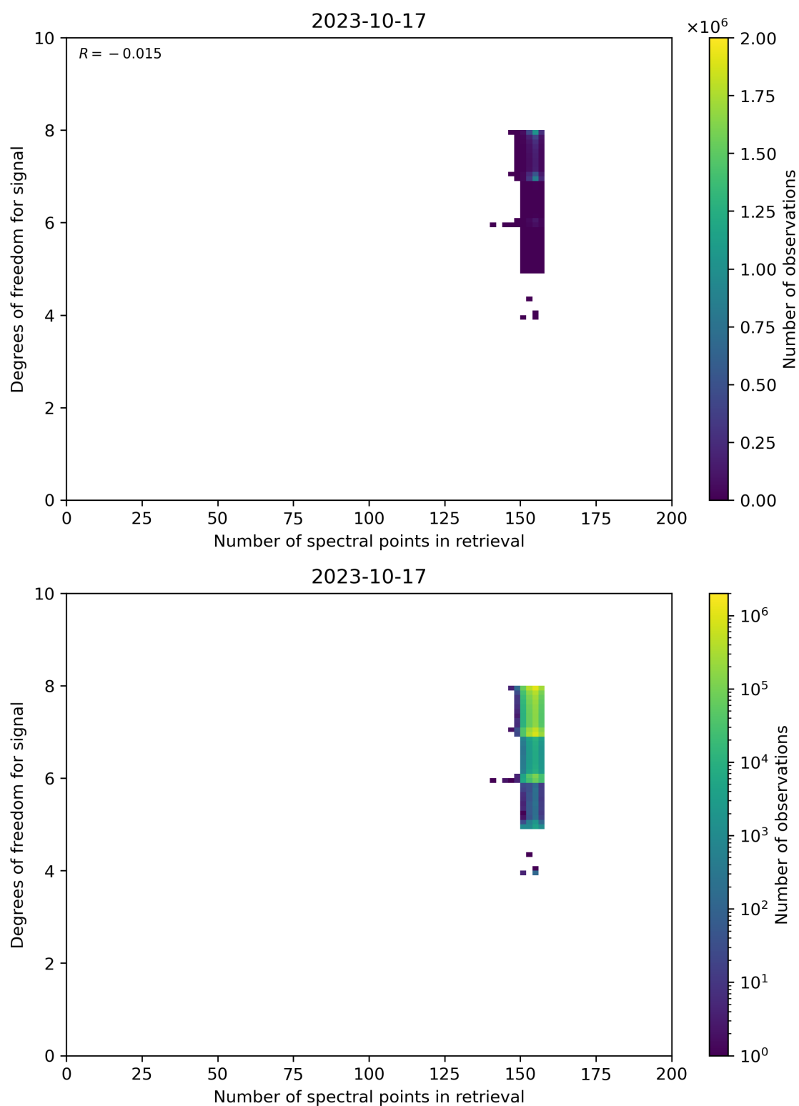
Figure 59: Scatter density plot of “Number of spectral points in retrieval” against “Degrees of freedom for signal” for 2023-10-17 to 2023-10-18.
