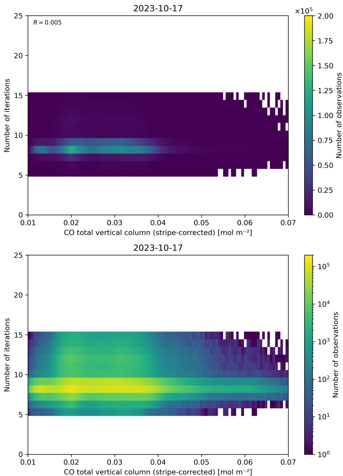
Figure 39: Scatter density plot of “CO total vertical column (stripe-corrected)” against “Number of iterations” for 2023-10-17 to 2023-10-18.
