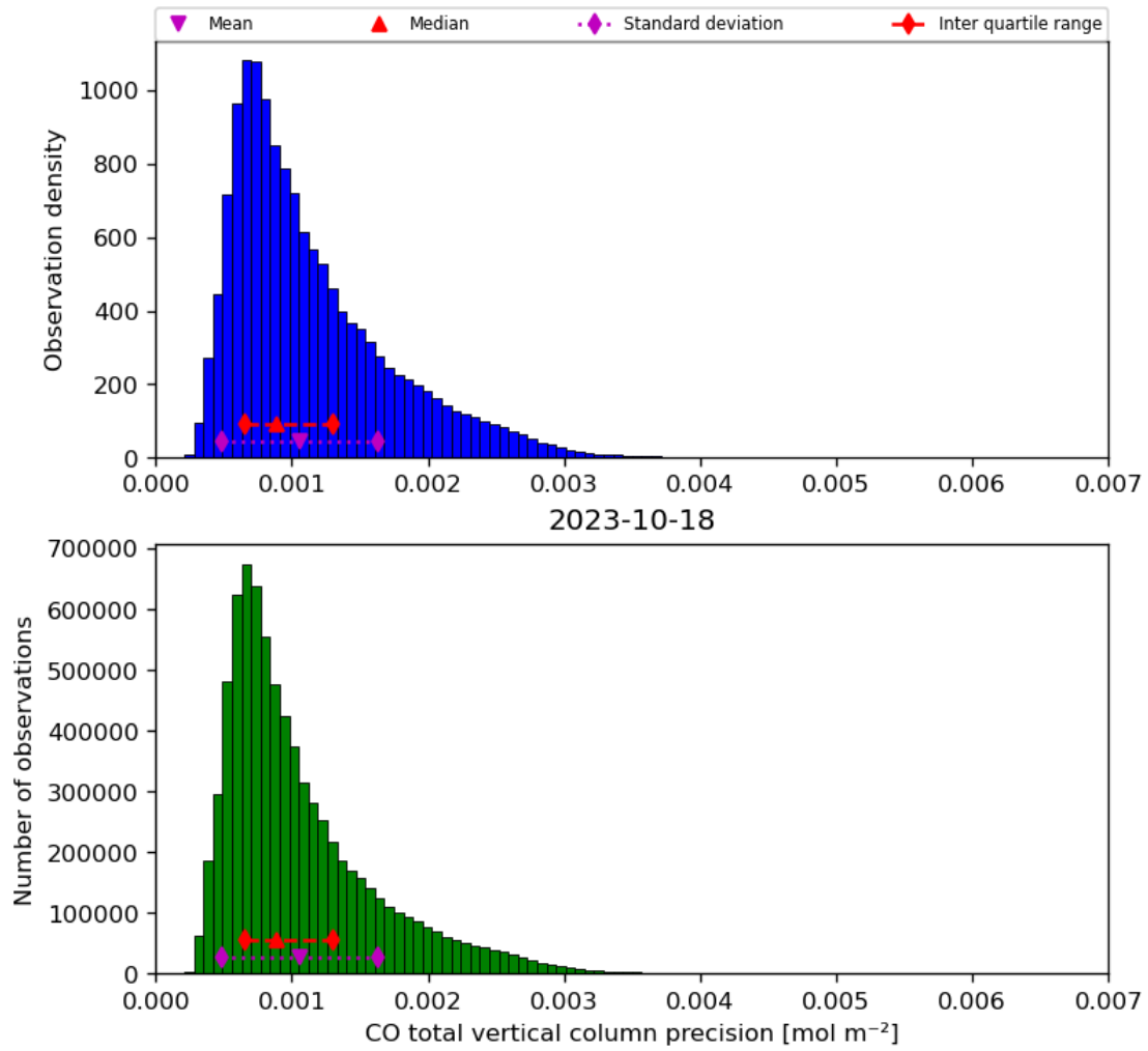
Figure 20: Histogram of “CO total vertical column precision” for 2023-10-17 to 2023-10-19
