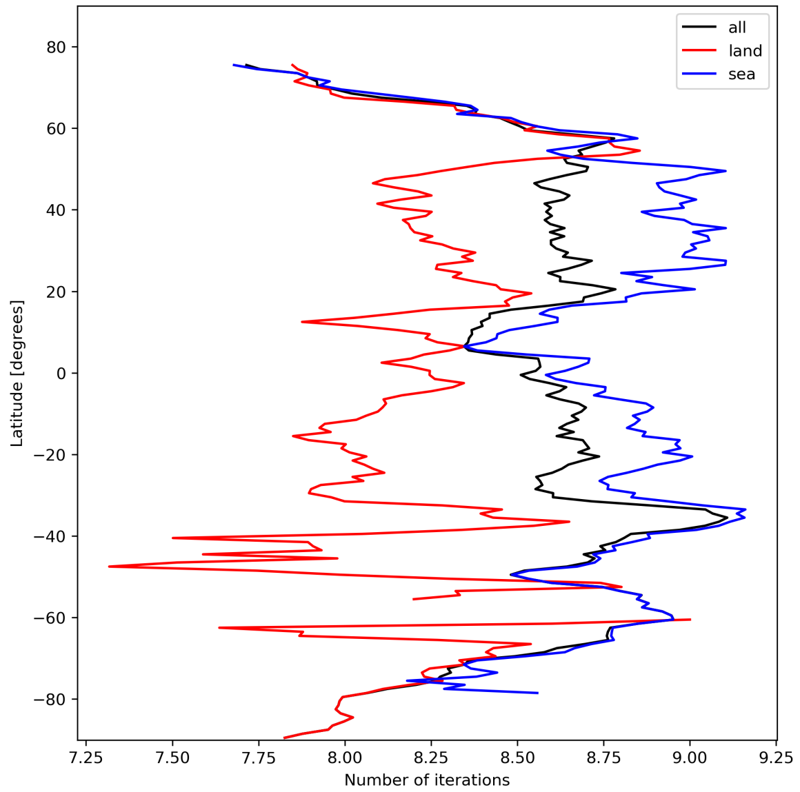
Figure 16: Zonal average of “Number of iterations” for 2023-10-17 to 2023-10-19.
