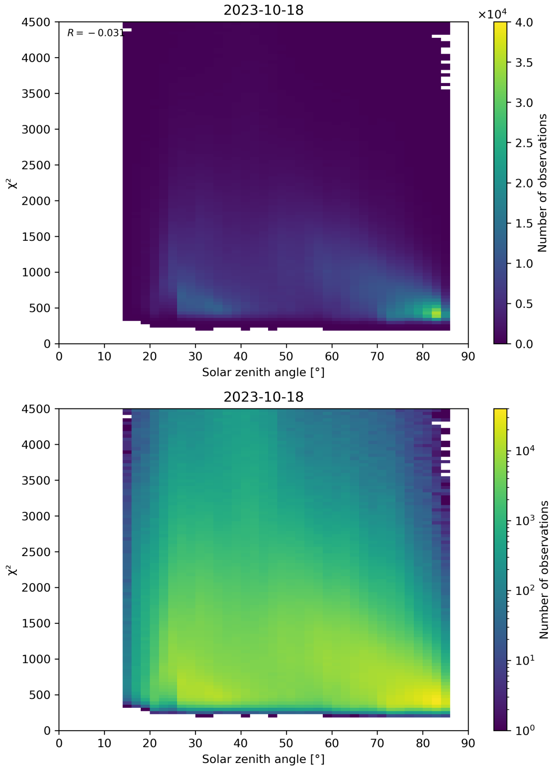
Figure 64: Scatter density plot of “Solar zenith angle” against “ \chi^2 ” for 2023-10-17 to 2023-10-19.
