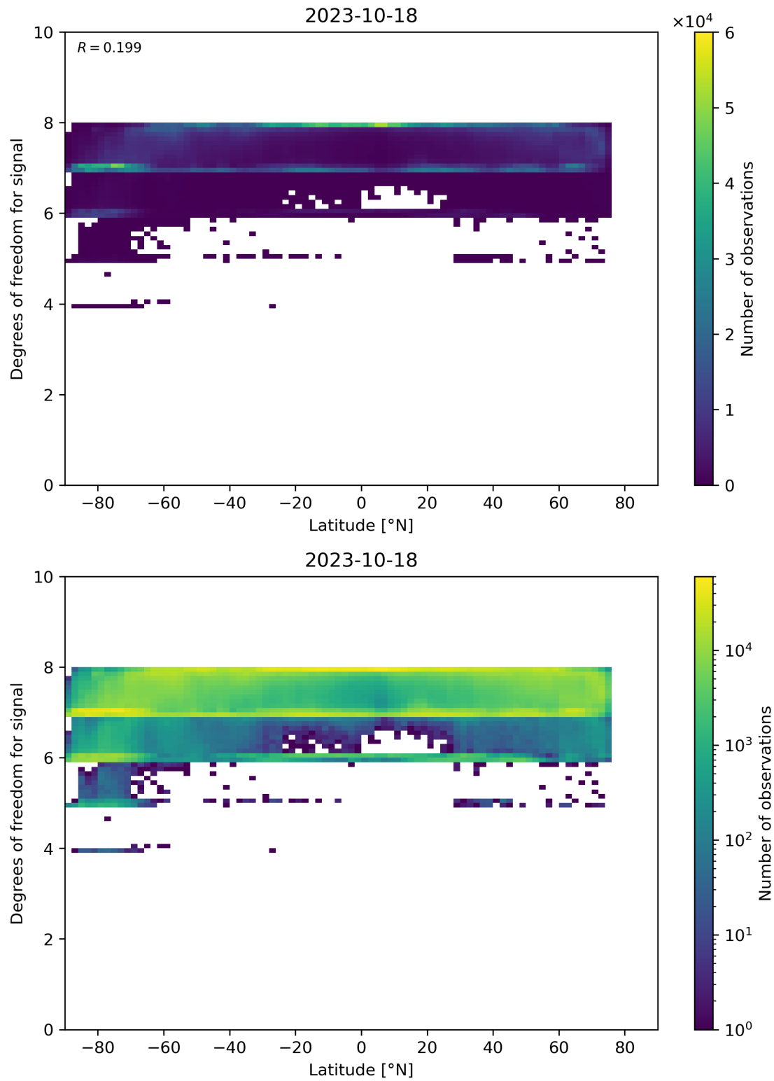
Figure 55: Scatter density plot of “Latitude” against “Degrees of freedom for signal” for 2023-10-17 to 2023-10-19.
