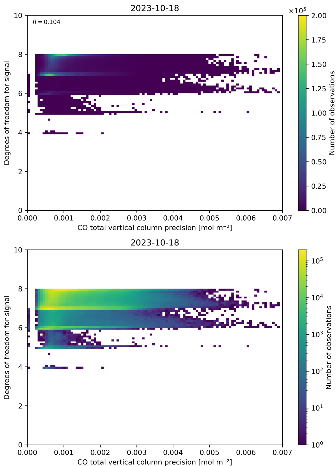
Figure 45: Scatter density plot of “CO total vertical column precision” against “Degrees of freedom for signal” for 2023-10-17 to 2023-10-19.
