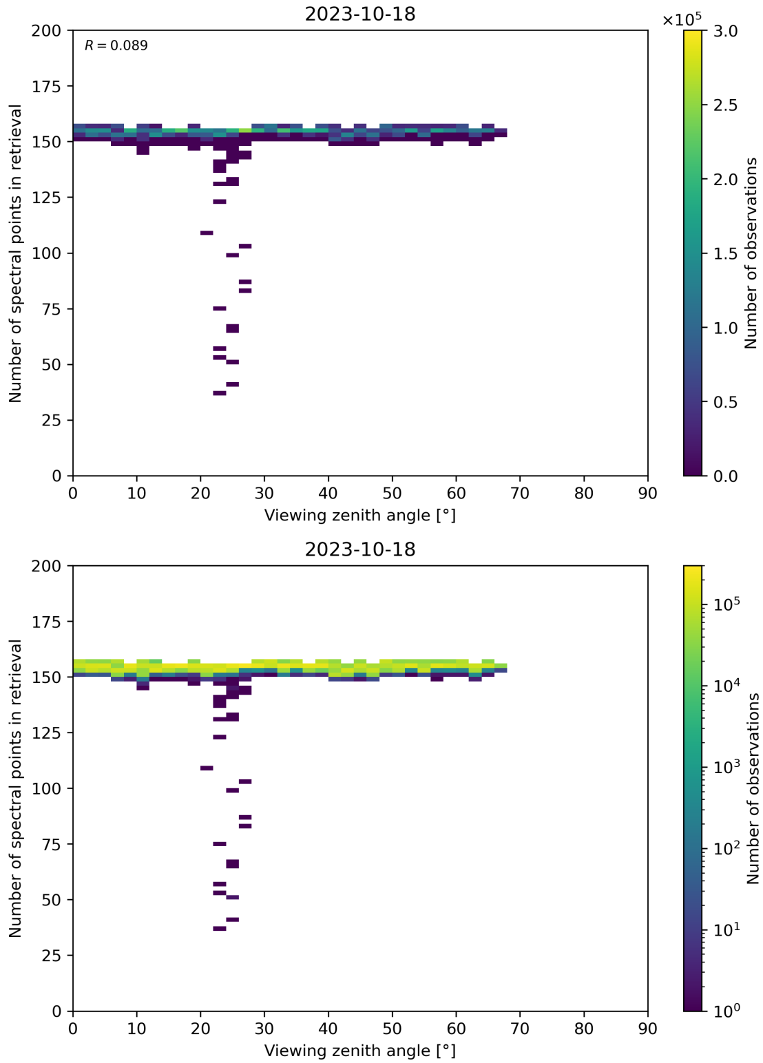
Figure 76: Scatter density plot of “Viewing zenith angle” against “Number of spectral points in retrieval” for 2023-10-17 to 2023-10-19.
