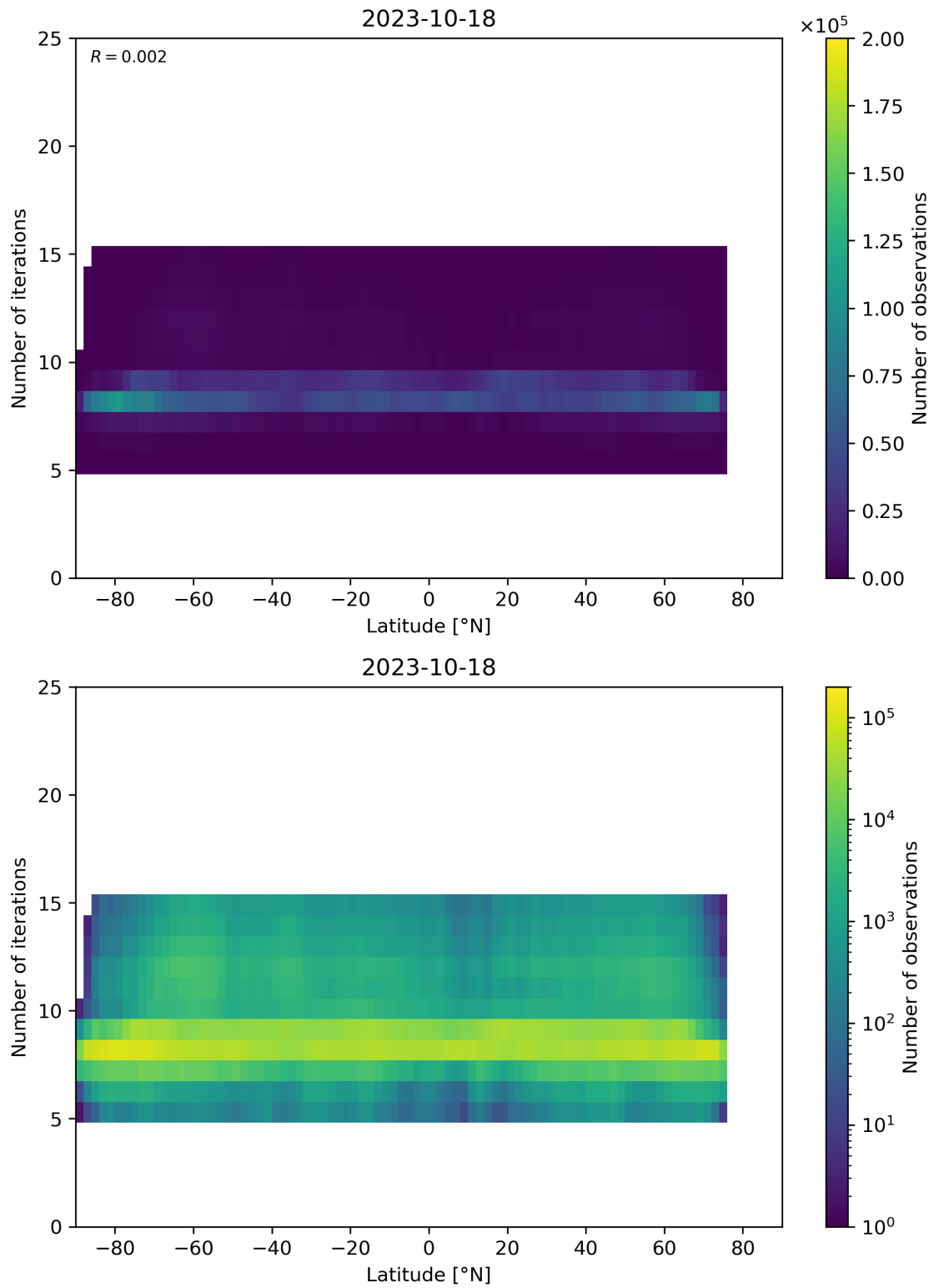
Figure 56: Scatter density plot of “Latitude” against “Number of iterations” for 2023-10-17 to 2023-10-19.
