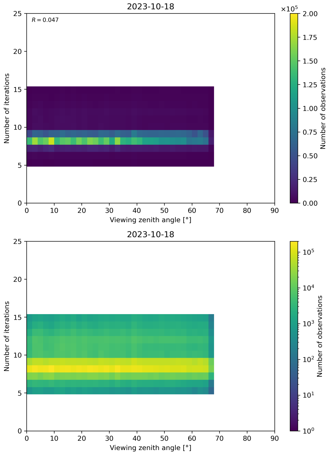
Figure 75: Scatter density plot of “Viewing zenith angle” against “Number of iterations” for 2023-10-17 to 2023-10-19.
