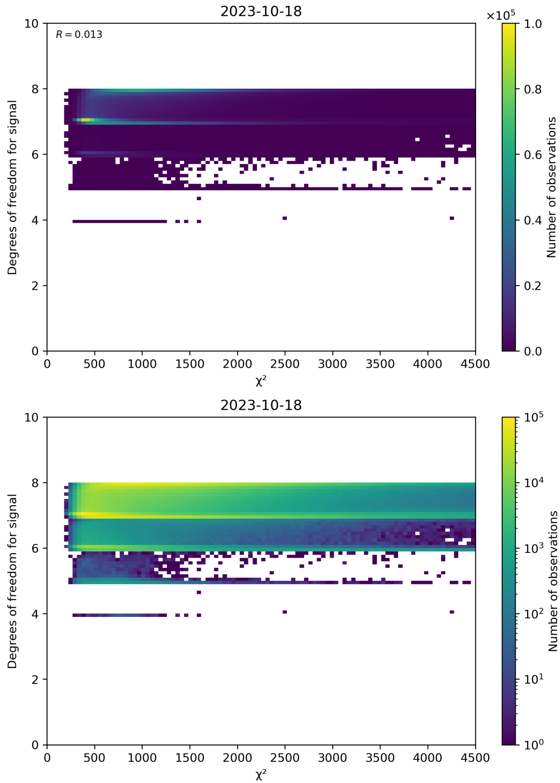
Figure 48: Scatter density plot of “ \chi^2 ” against “Degrees of freedom for signal” for 2023-10-17 to 2023-10-19.
