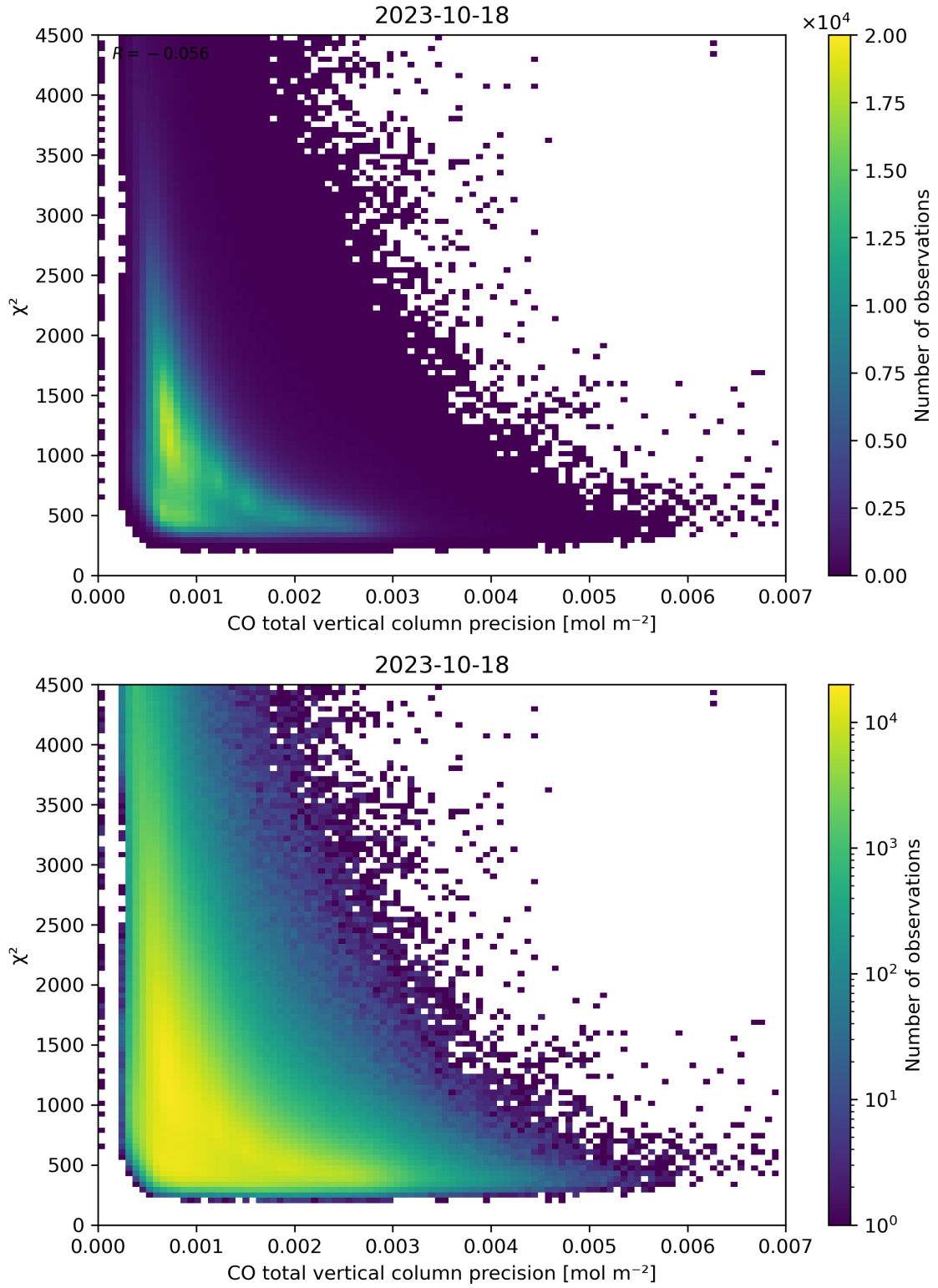
Figure 44: Scatter density plot of “CO total vertical column precision” against “ \chi^2 ” for 2023-10-17 to 2023-10-19.
