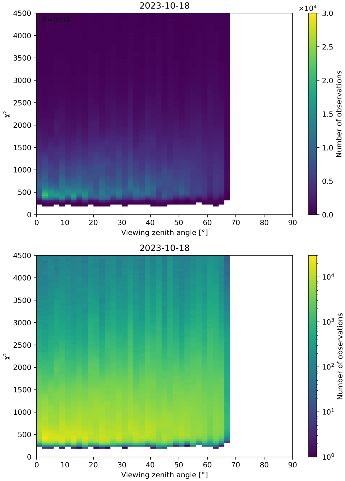
Figure 72: Scatter density plot of “Viewing zenith angle” against “ \chi^2 ” for 2023-10-17 to 2023-10-19.
