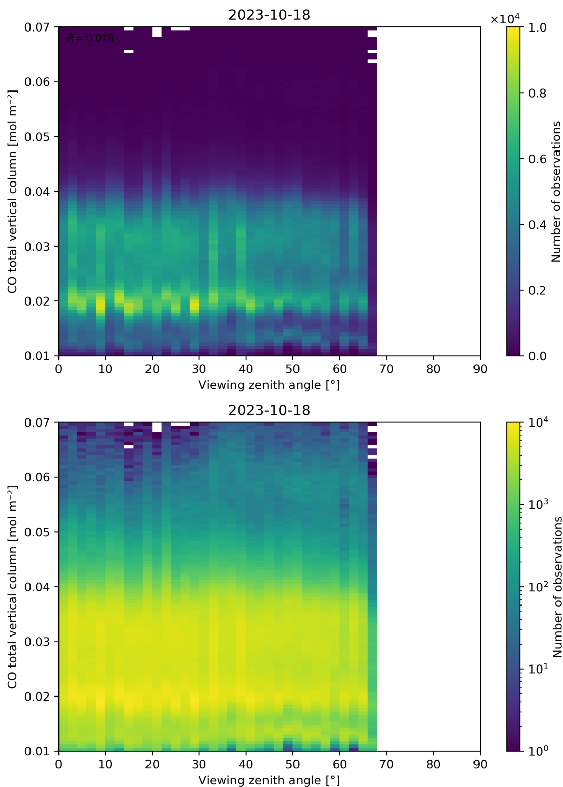
Figure 69: Scatter density plot of “Viewing zenith angle” against “CO total vertical column” for 2023-10-17 to 2023-10-19.
