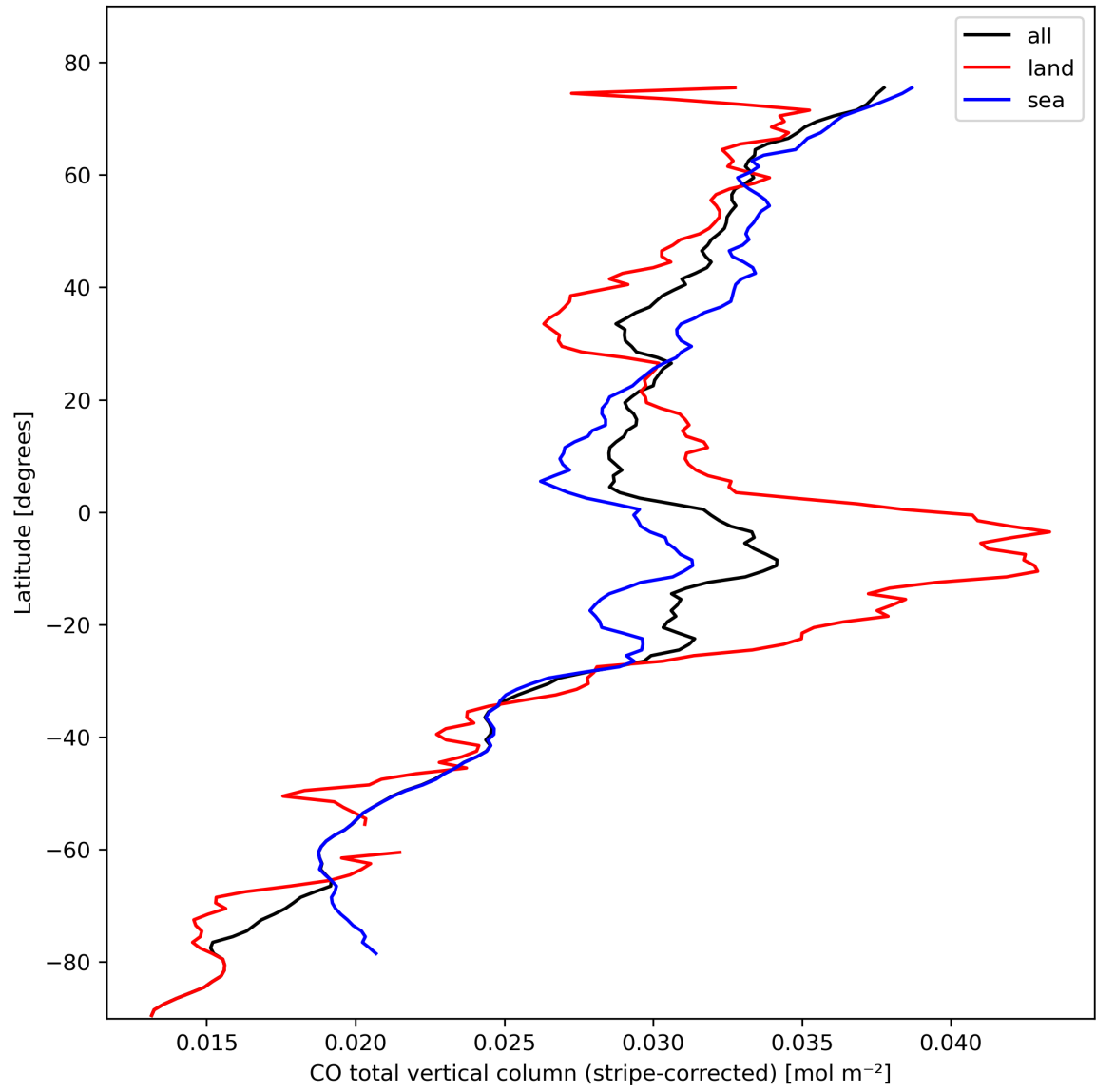
Figure 11: Zonal average of “CO total vertical column (stripe-corrected)” for 2023-10-17 to 2023-10-19.
