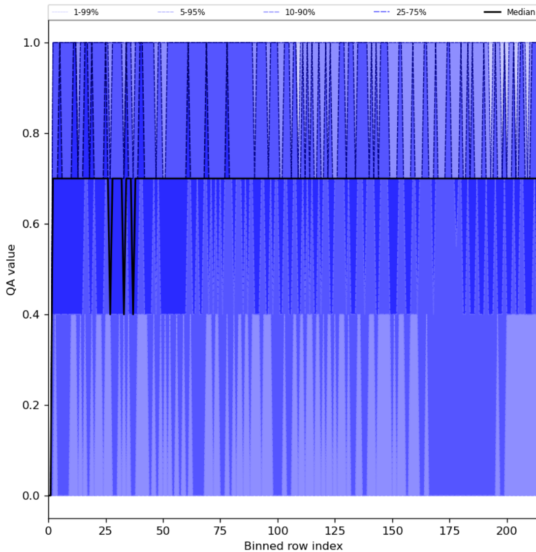
Figure 25: Along track statistics of “QA value” for 2023-10-17 to 2023-10-19
