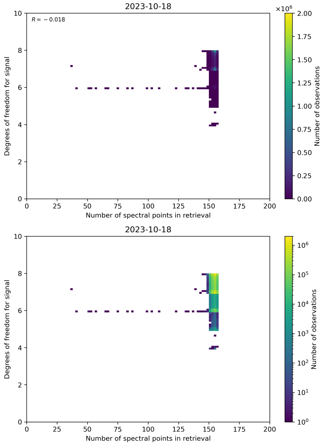
Figure 59: Scatter density plot of “Number of spectral points in retrieval” against “Degrees of freedom for signal” for 2023-10-17 to 2023-10-19.
