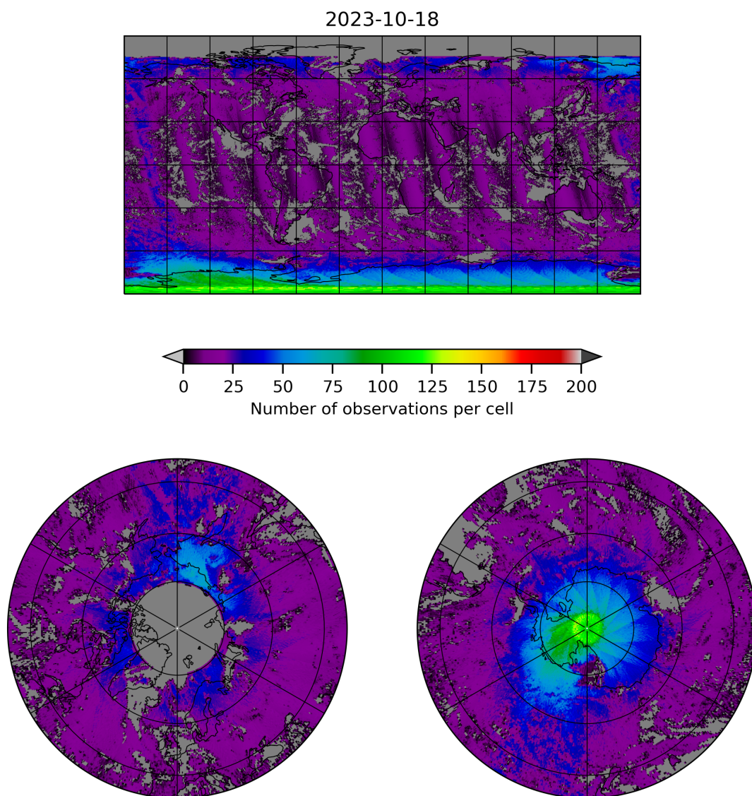
Figure 8: Map of the number of observations for 2023-10-17 to 2023-10-19
