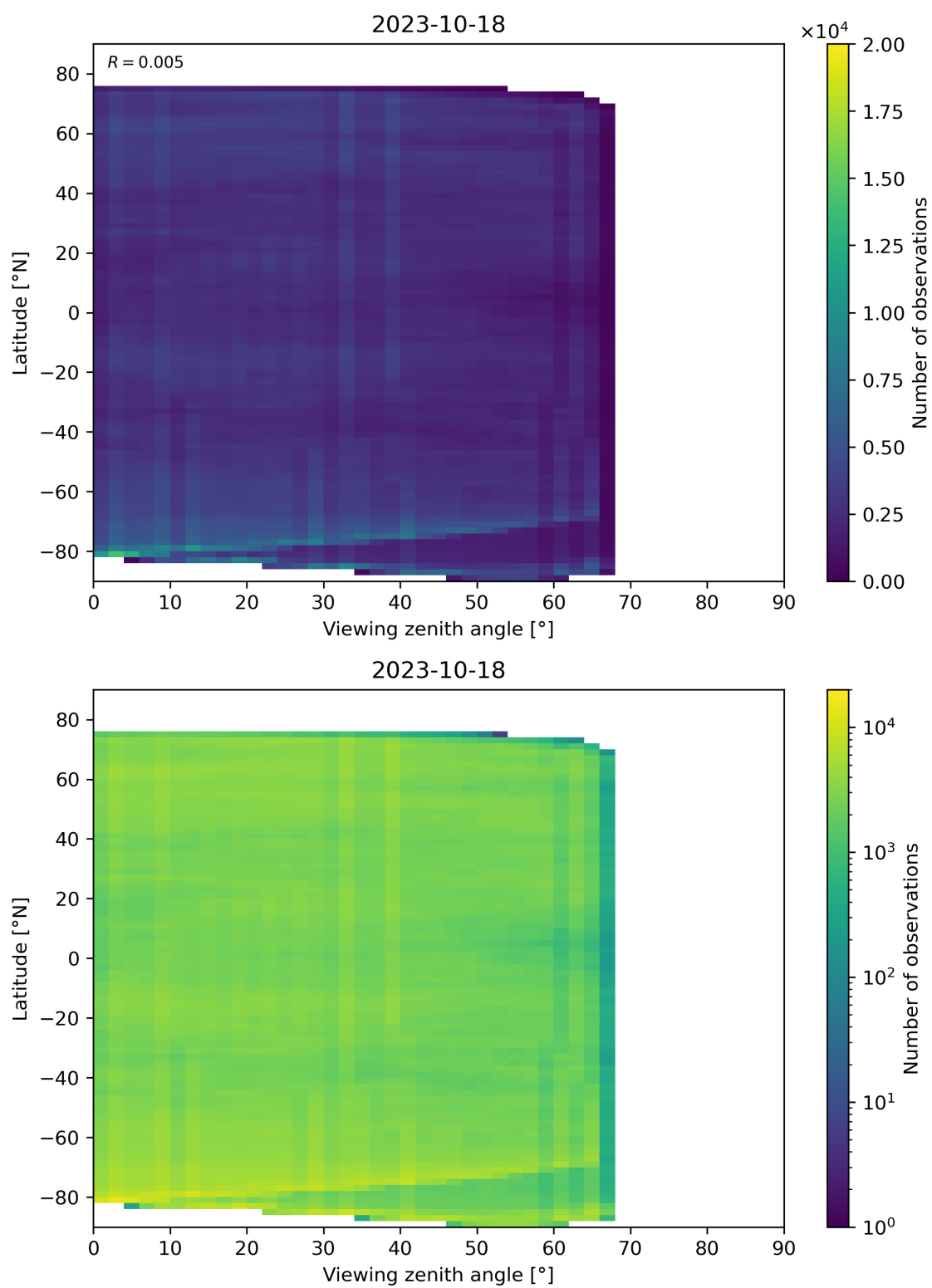
Figure 74: Scatter density plot of “Viewing zenith angle” against “Latitude” for 2023-10-17 to 2023-10-19.
