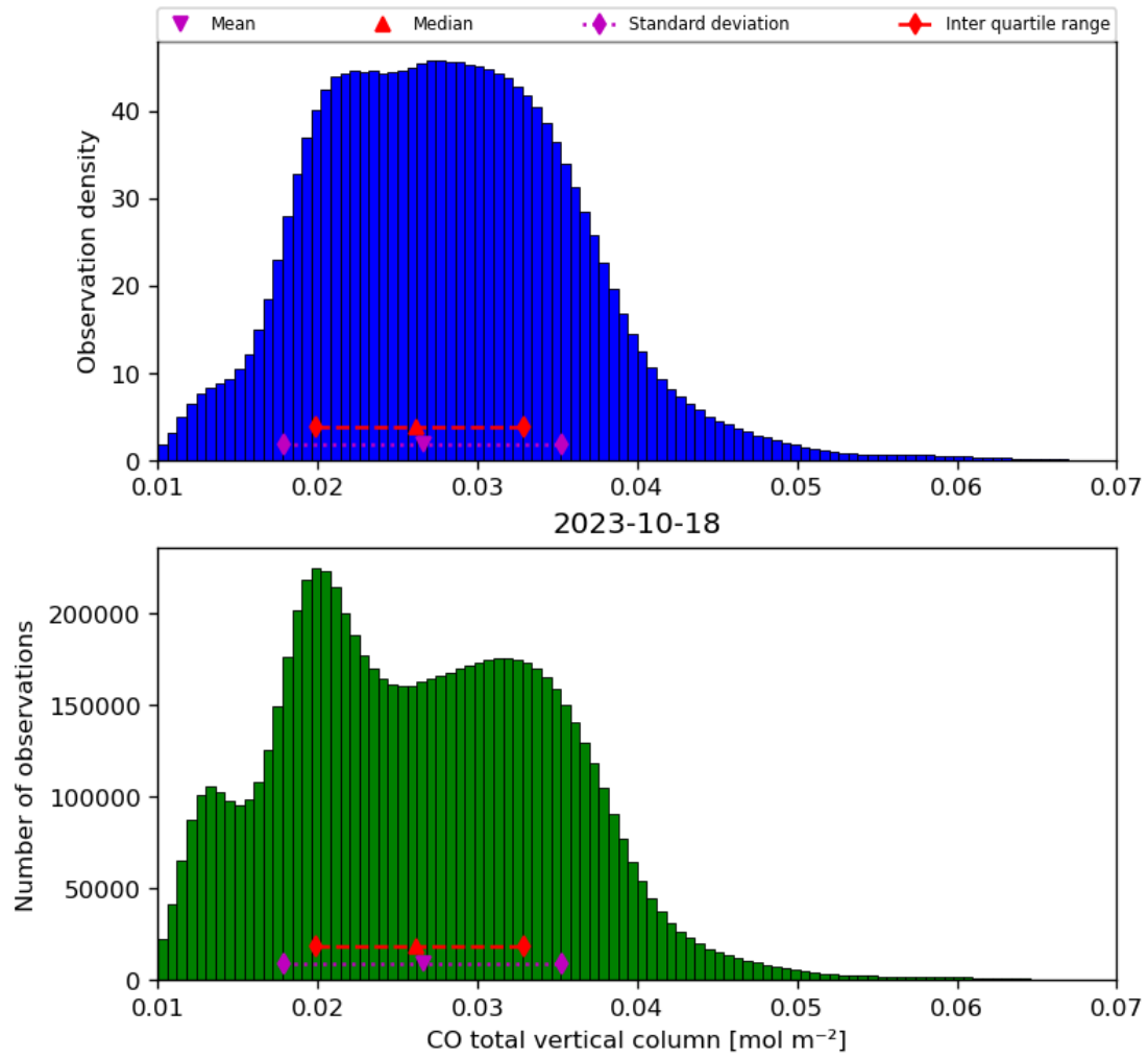
Figure 18: Histogram of “CO total vertical column” for 2023-10-17 to 2023-10-19
