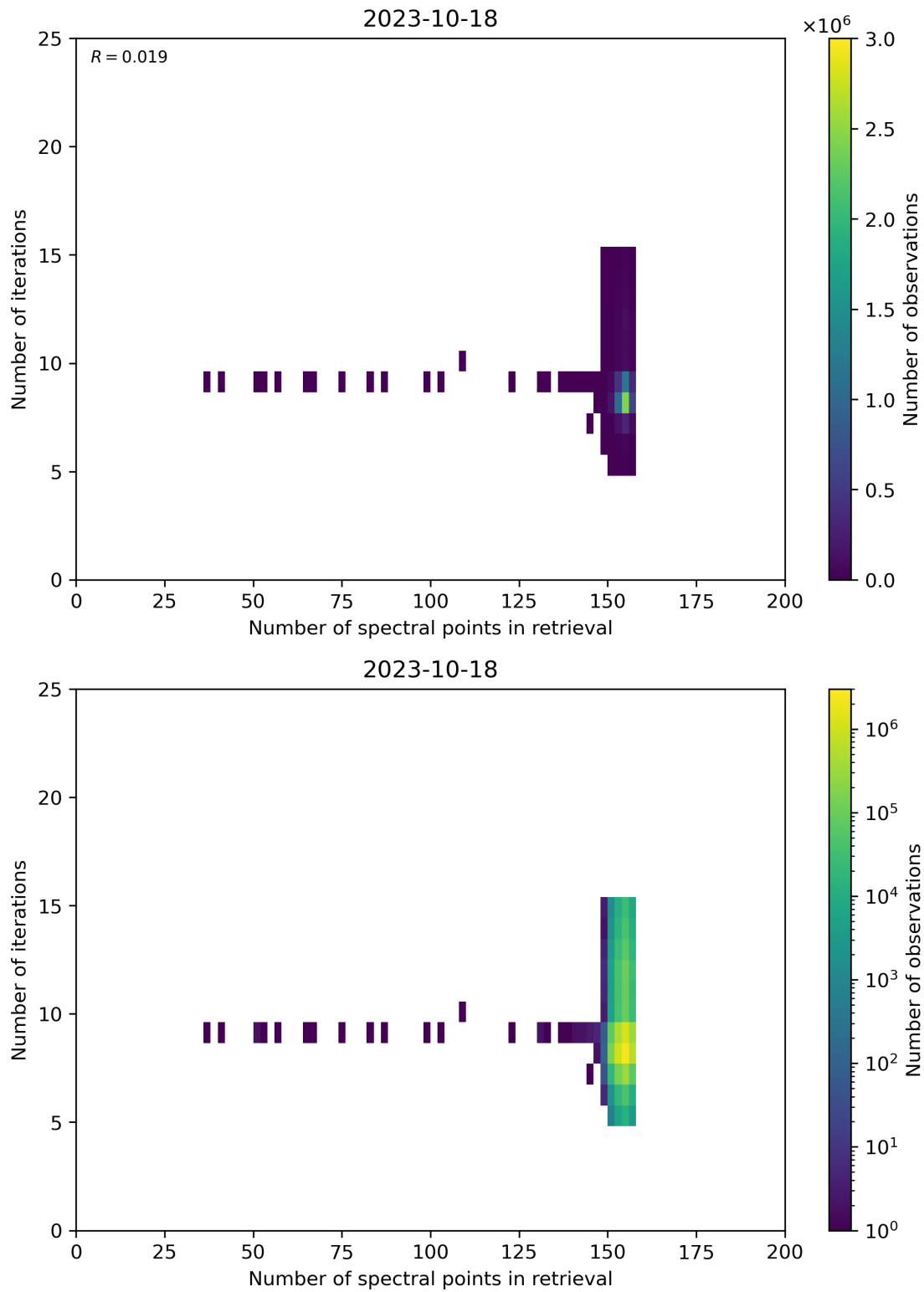
Figure 60: Scatter density plot of “Number of spectral points in retrieval” against “Number of iterations” for 2023-10-17 to 2023-10-19.
