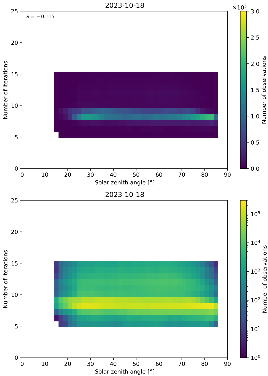
Figure 67: Scatter density plot of “Solar zenith angle” against “Number of iterations” for 2023-10-17 to 2023-10-19.
