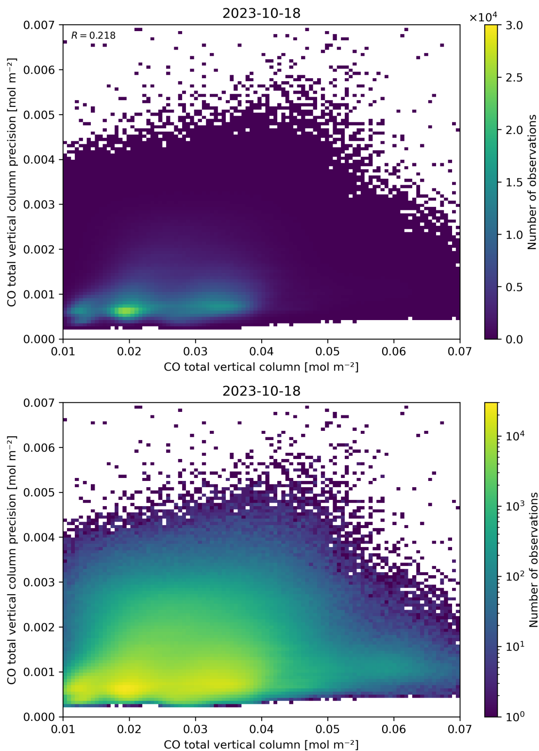
Figure 34: Scatter density plot of “CO total vertical column” against “CO total vertical column precision” for 2023-10-17 to 2023-10-19.
