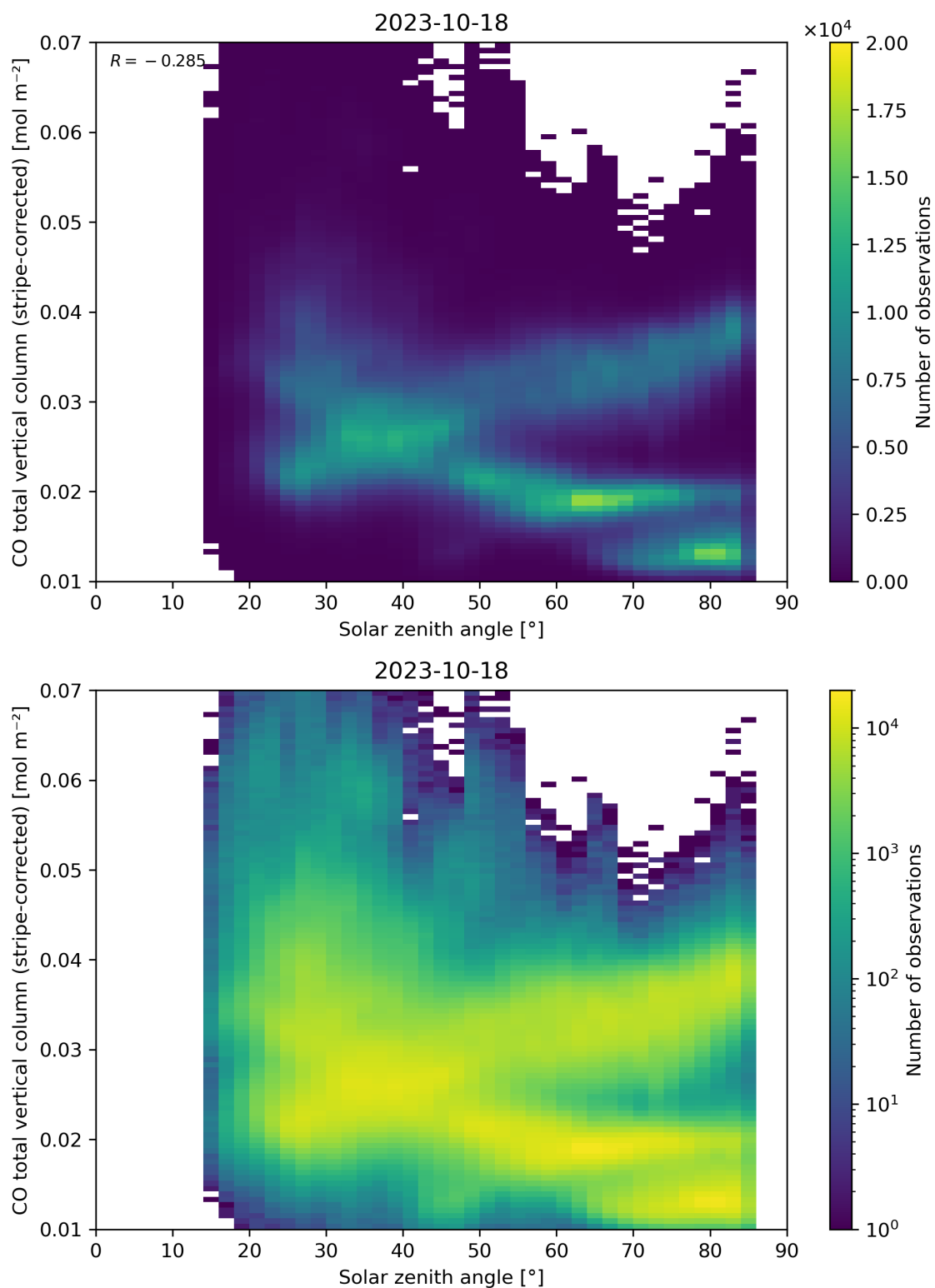
Figure 62: Scatter density plot of “Solar zenith angle” against “CO total vertical column (stripe-corrected)” for 2023-10-17 to 2023-10-19.
