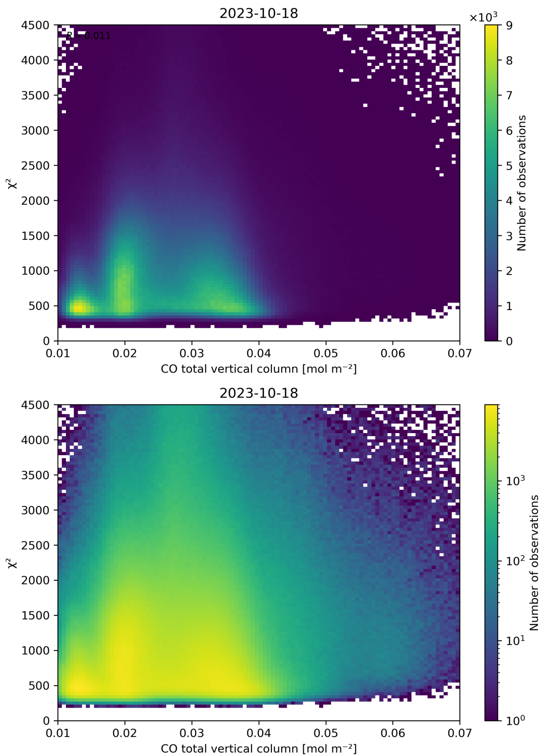
Figure 35: Scatter density plot of “CO total vertical column” against “ \chi^2 ” for 2023-10-17 to 2023-10-19.
