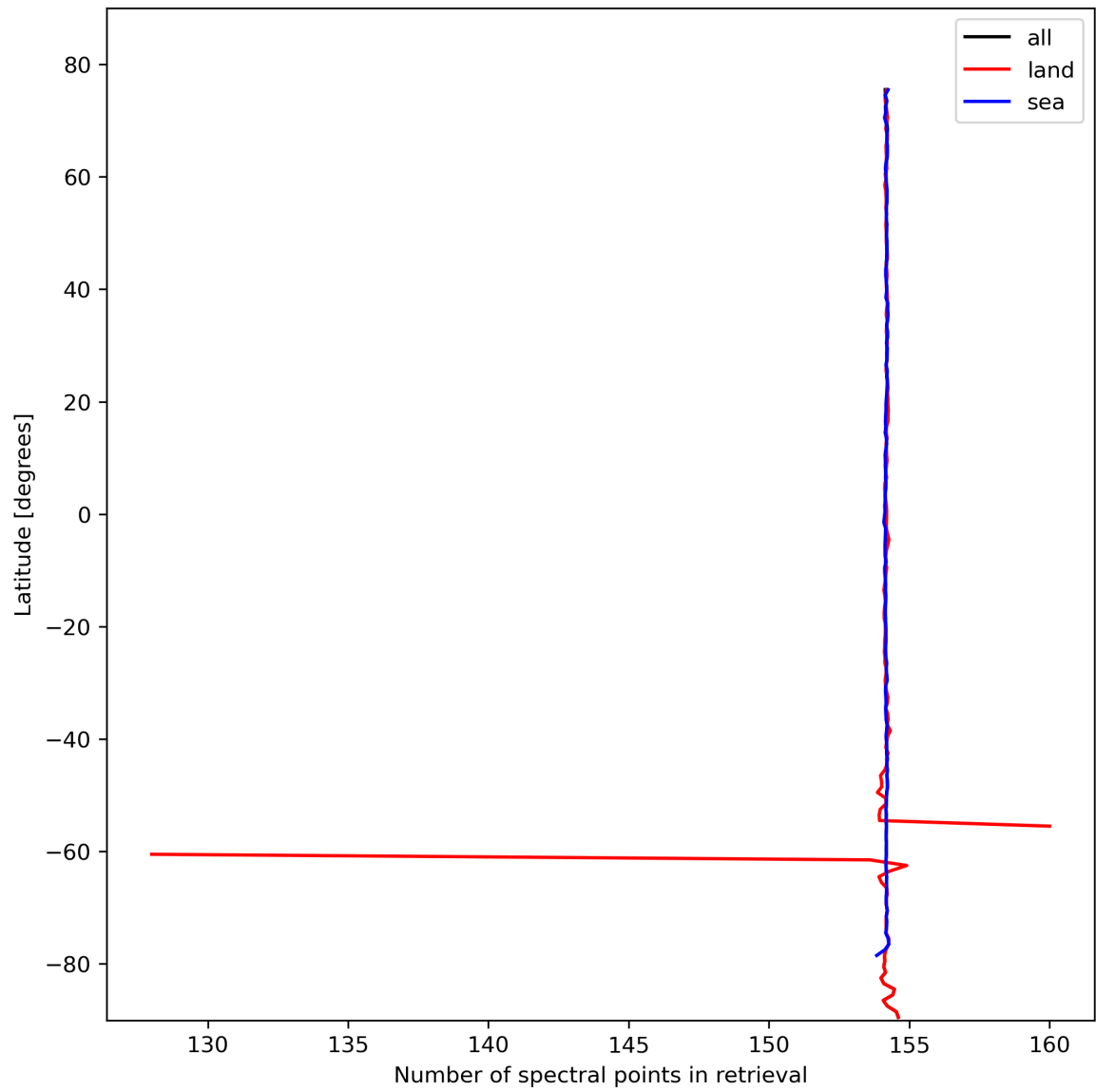
Figure 13: Zonal average of “Number of spectral points in retrieval” for 2023-10-17 to 2023-10-19.
