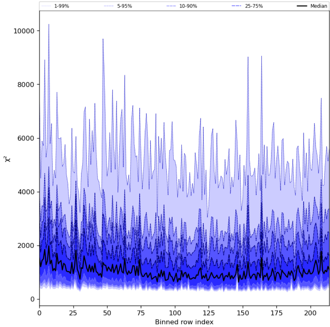
Figure 30: Along track statistics of “ \chi^2 ” for 2023-10-17 to 2023-10-19
