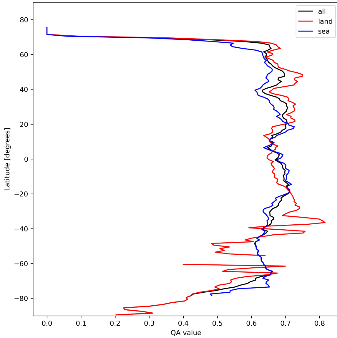
Figure 9: Zonal average of “QA value” for 2023-10-17 to 2023-10-19.
