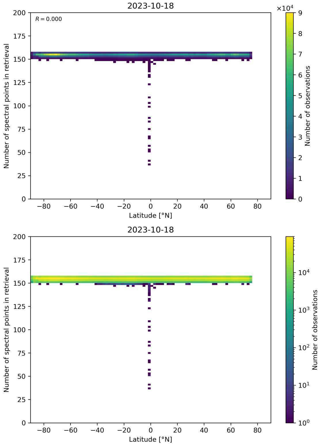
Figure 57: Scatter density plot of “Latitude” against “Number of spectral points in retrieval” for 2023-10-17 to 2023-10-19.
