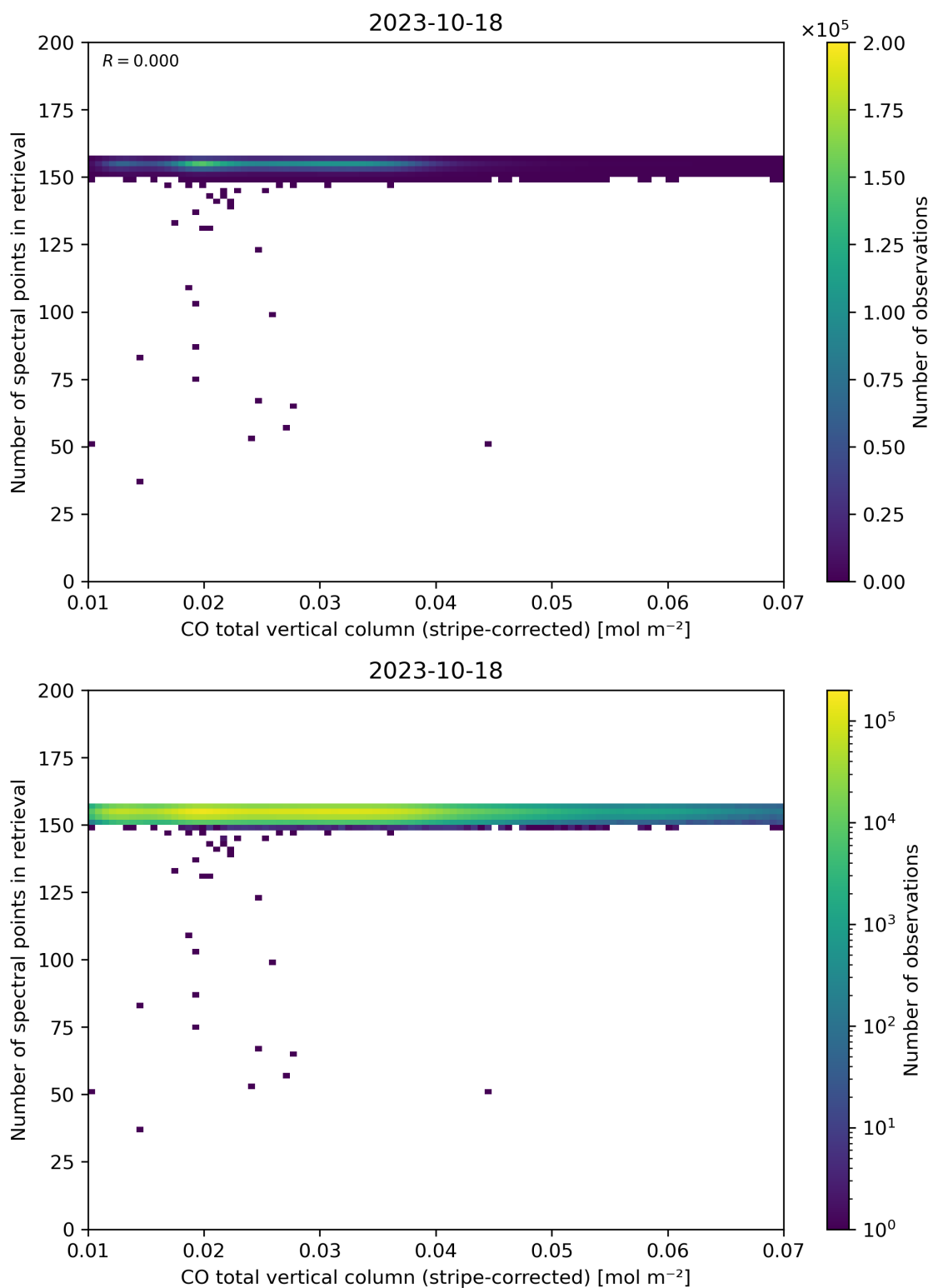
Figure 40: Scatter density plot of “CO total vertical column (stripe-corrected)” against “Number of spectral points in retrieval” for 2023-10-17 to 2023-10-19.
