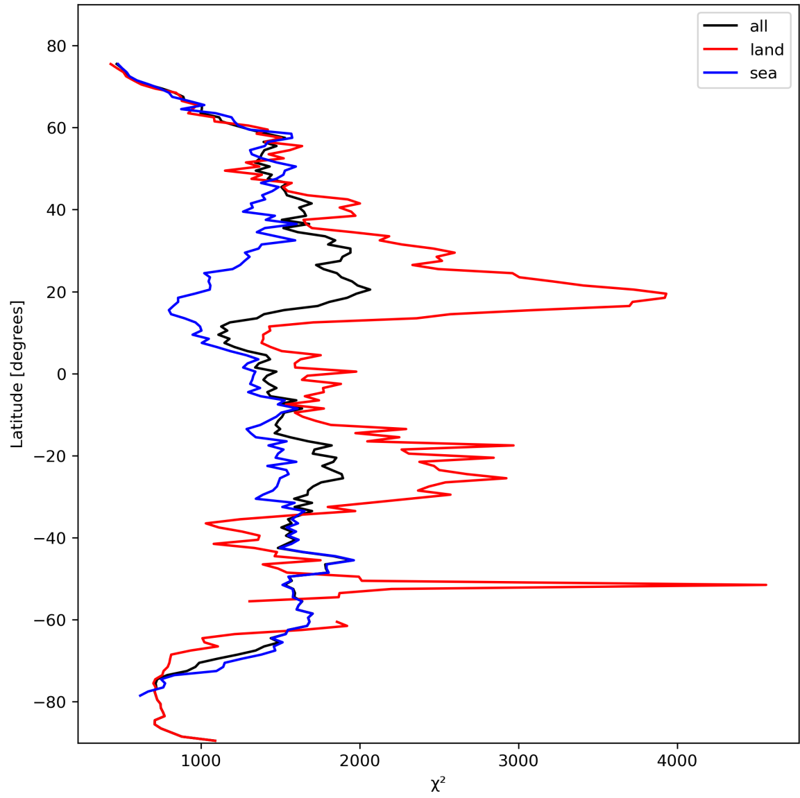
Figure 14: Zonal average of “ \chi^2 ” for 2023-10-17 to 2023-10-19.
