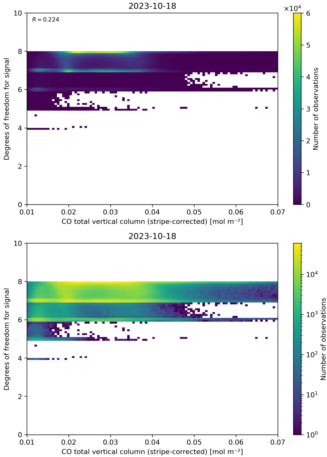
Figure 38: Scatter density plot of “CO total vertical column (stripe-corrected)” against “Degrees of freedom for signal” for 2023-10-17 to 2023-10-19.
