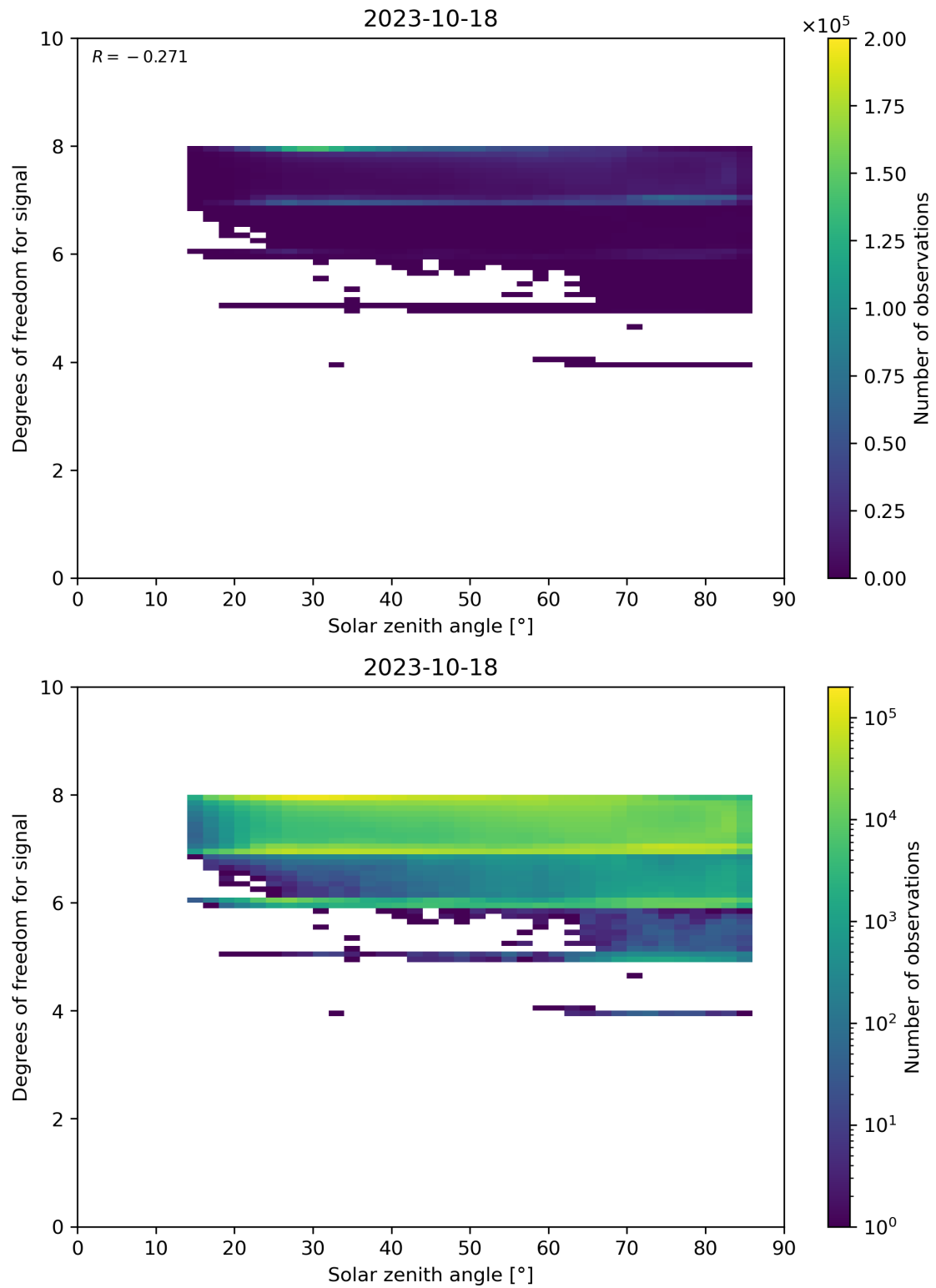
Figure 65: Scatter density plot of “Solar zenith angle” against “Degrees of freedom for signal” for 2023-10-17 to 2023-10-19.
