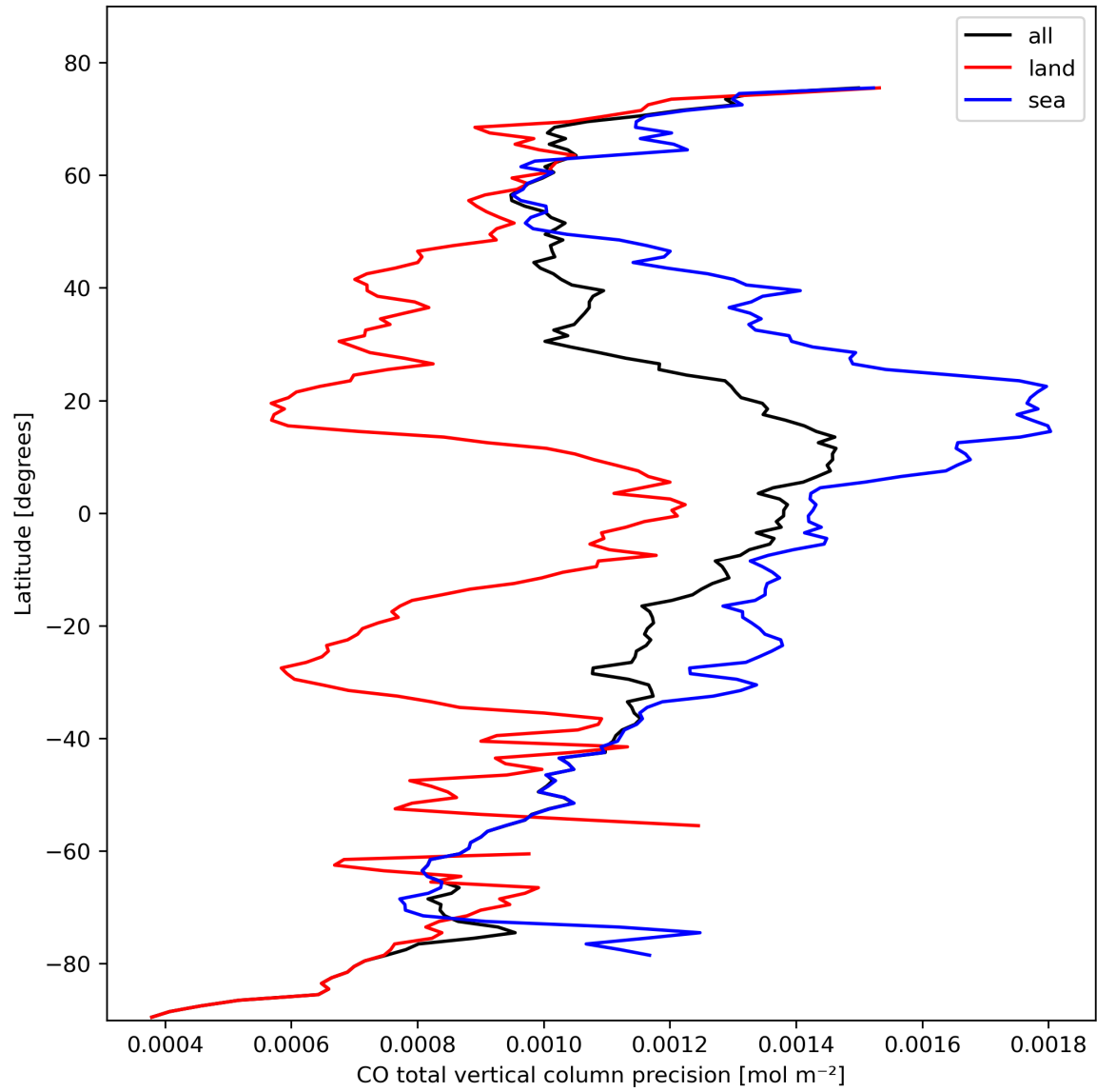
Figure 12: Zonal average of “CO total vertical column precision” for 2023-10-17 to 2023-10-19.
