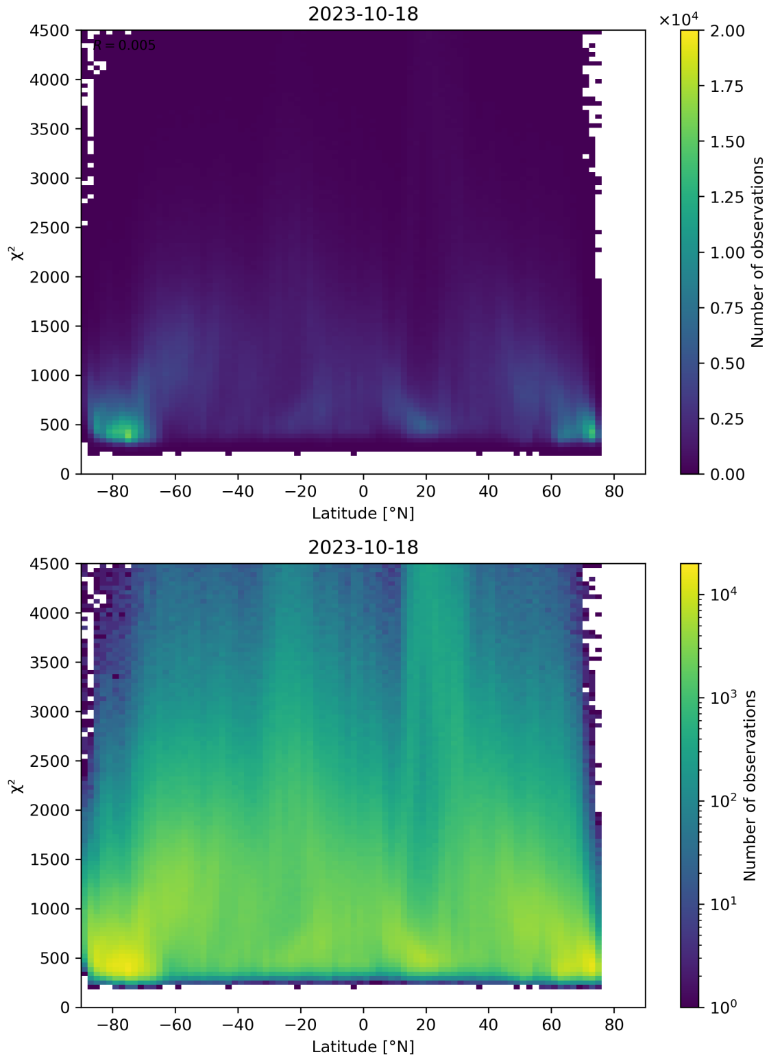
Figure 54: Scatter density plot of “Latitude” against “ \chi^2 ” for 2023-10-17 to 2023-10-19.
