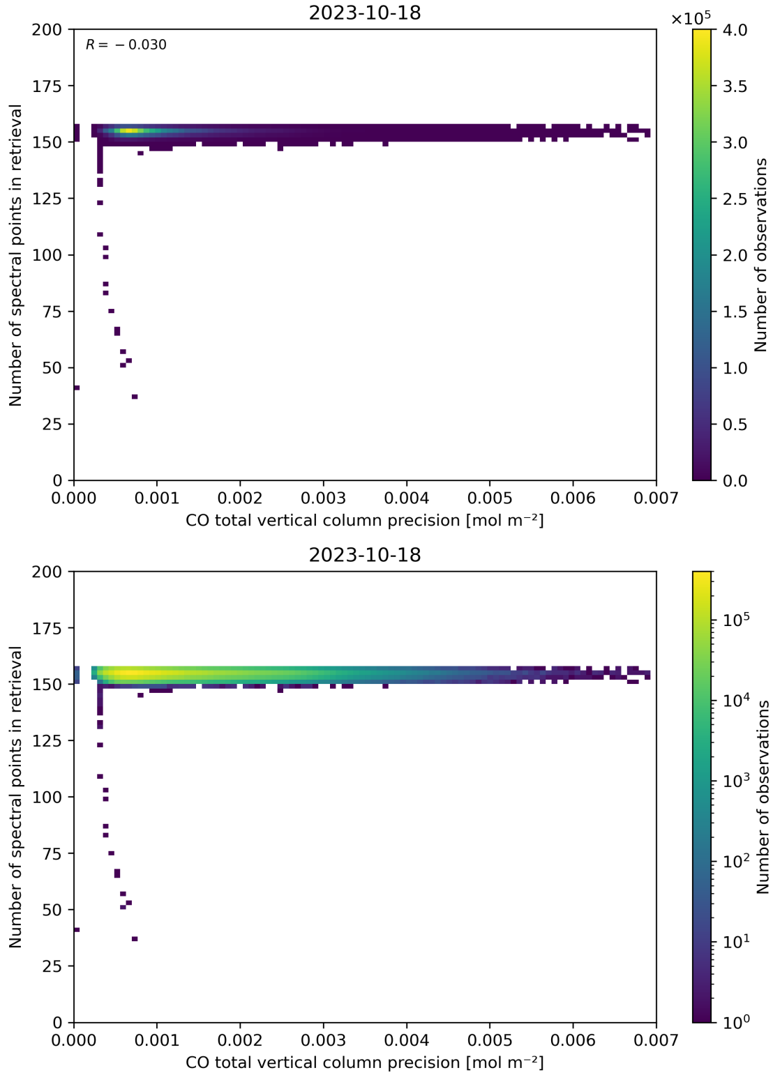
Figure 47: Scatter density plot of “CO total vertical column precision” against “Number of spectral points in retrieval” for 2023-10-17 to 2023-10-19.
