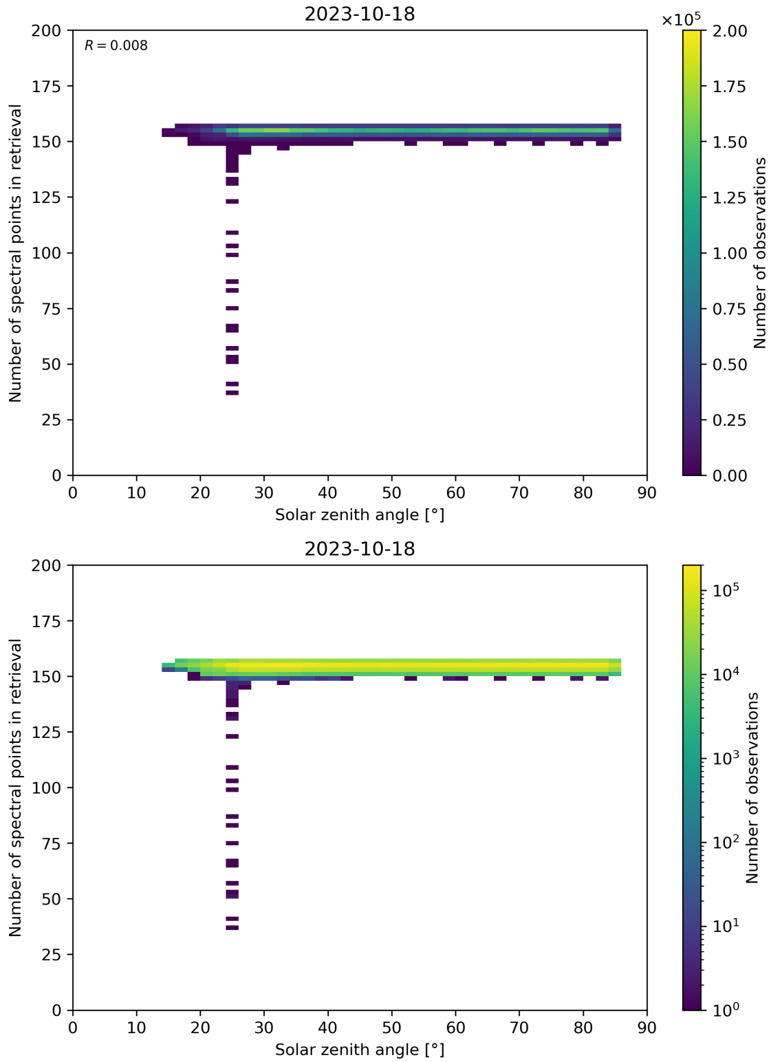
Figure 68: Scatter density plot of “Solar zenith angle” against “Number of spectral points in retrieval” for 2023-10-17 to 2023-10-19.
