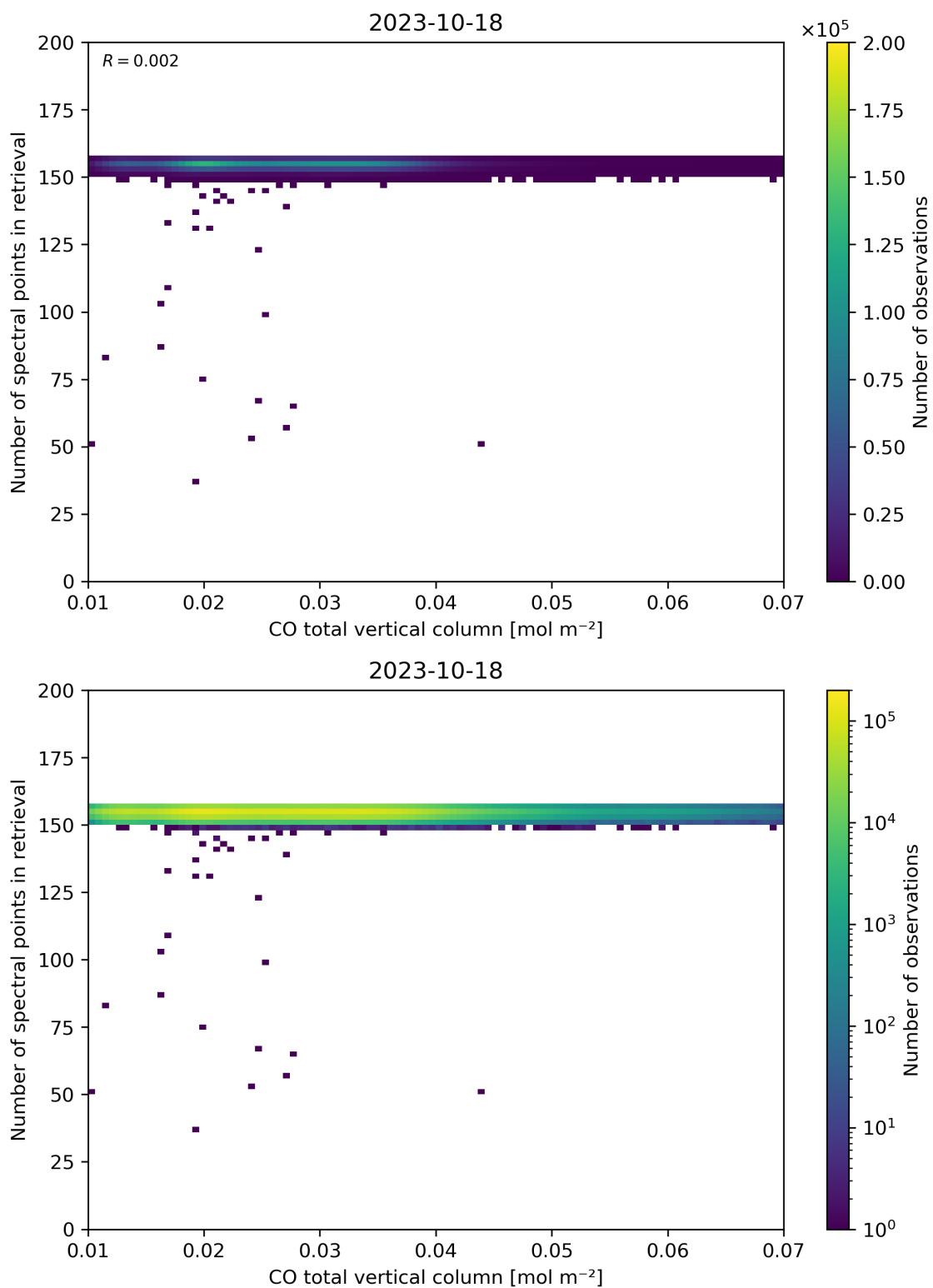
Figure 43: Scatter density plot of “CO total vertical column” against “Number of spectral points in retrieval” for 2023-10-17 to 2023-10-19.
