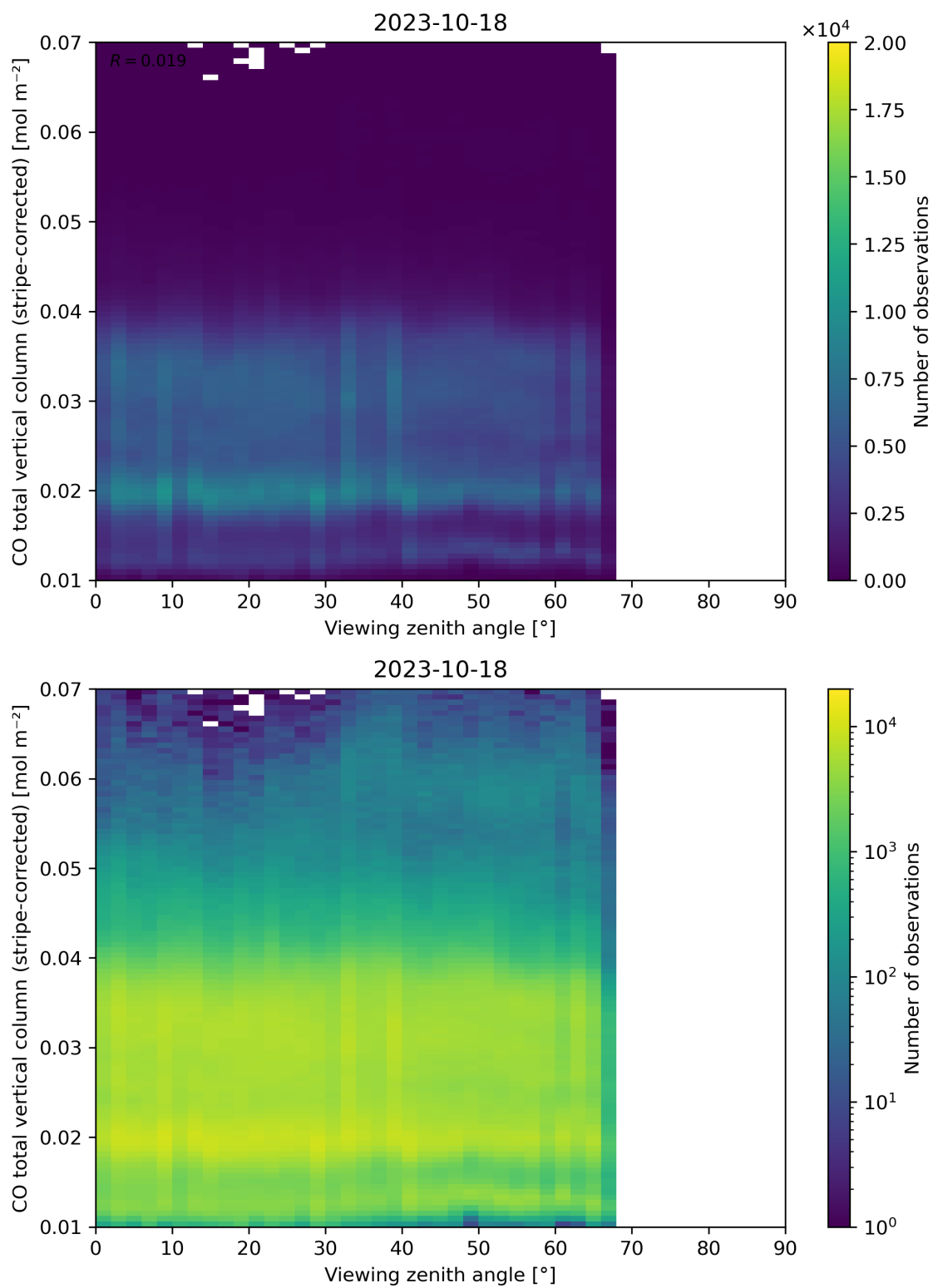
Figure 70: Scatter density plot of “Viewing zenith angle” against “CO total vertical column (stripe-corrected)” for 2023-10-17 to 2023-10-19.
