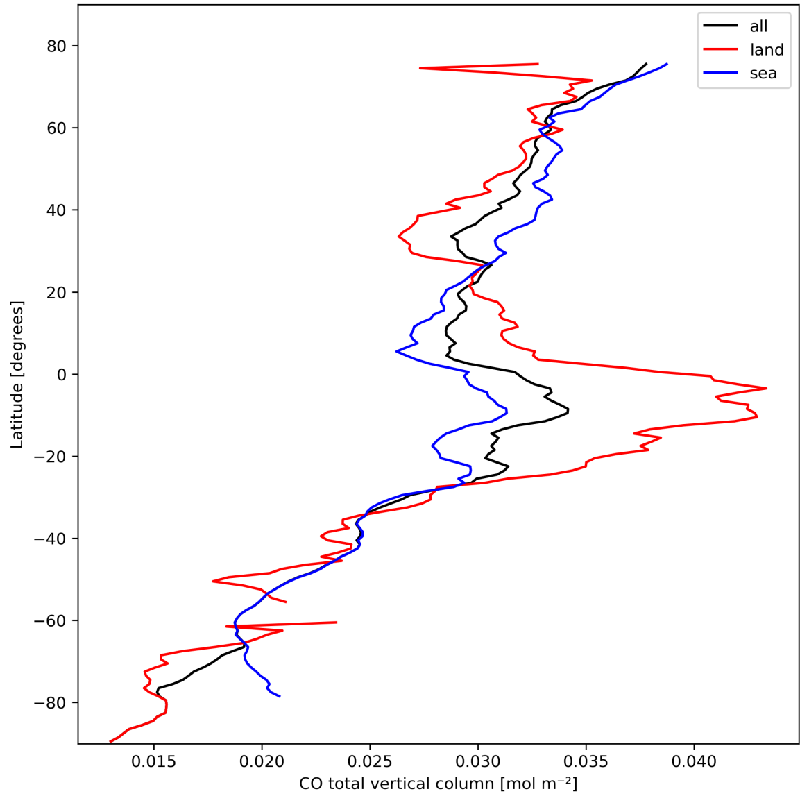
Figure 10: Zonal average of “CO total vertical column” for 2023-10-17 to 2023-10-19.
