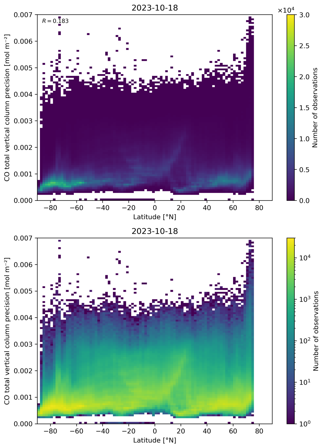
Figure 53: Scatter density plot of “Latitude” against “CO total vertical column precision” for 2023-10-17 to 2023-10-19.
