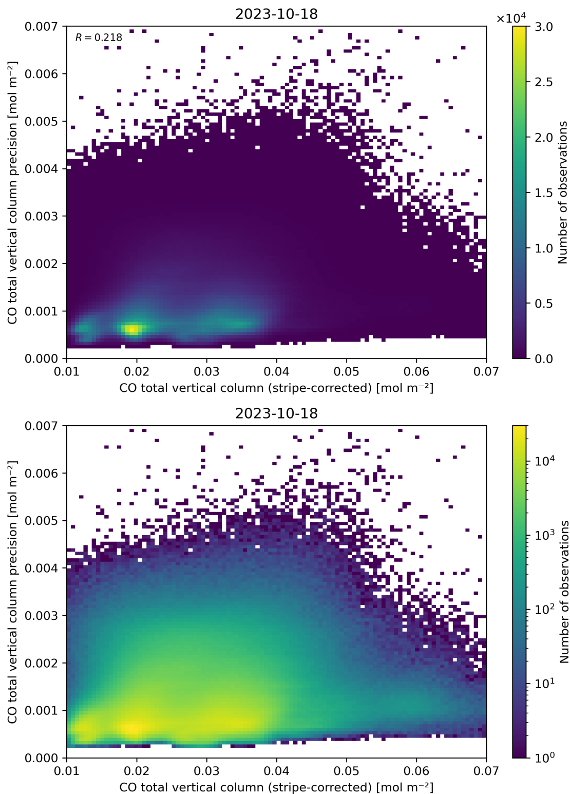
Figure 36: Scatter density plot of “CO total vertical column (stripe-corrected)” against “CO total vertical column precision” for 2023-10-17 to 2023-10-19.
