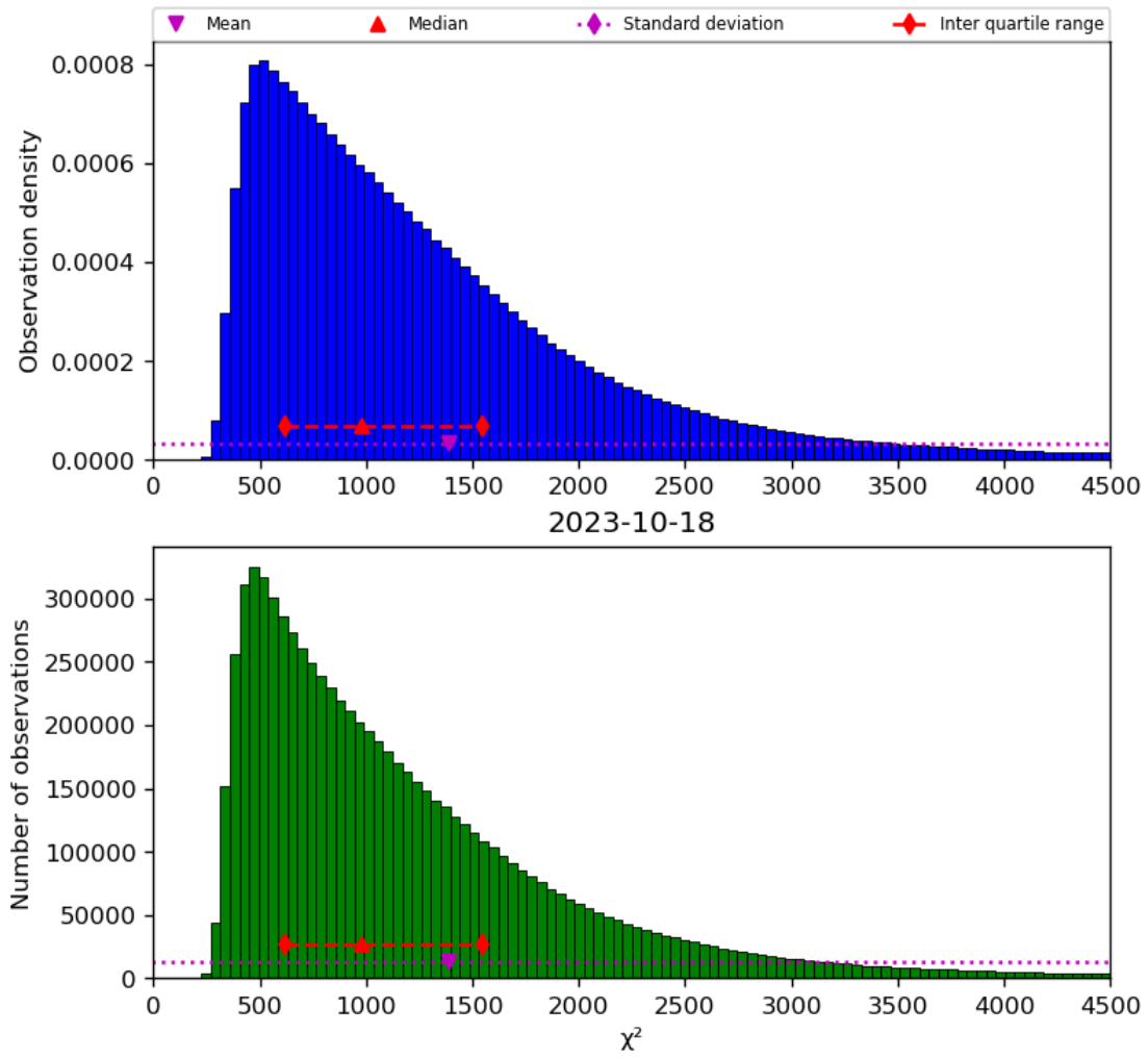
Figure 22: Histogram of “ \chi^2 ” for 2023-10-17 to 2023-10-19
