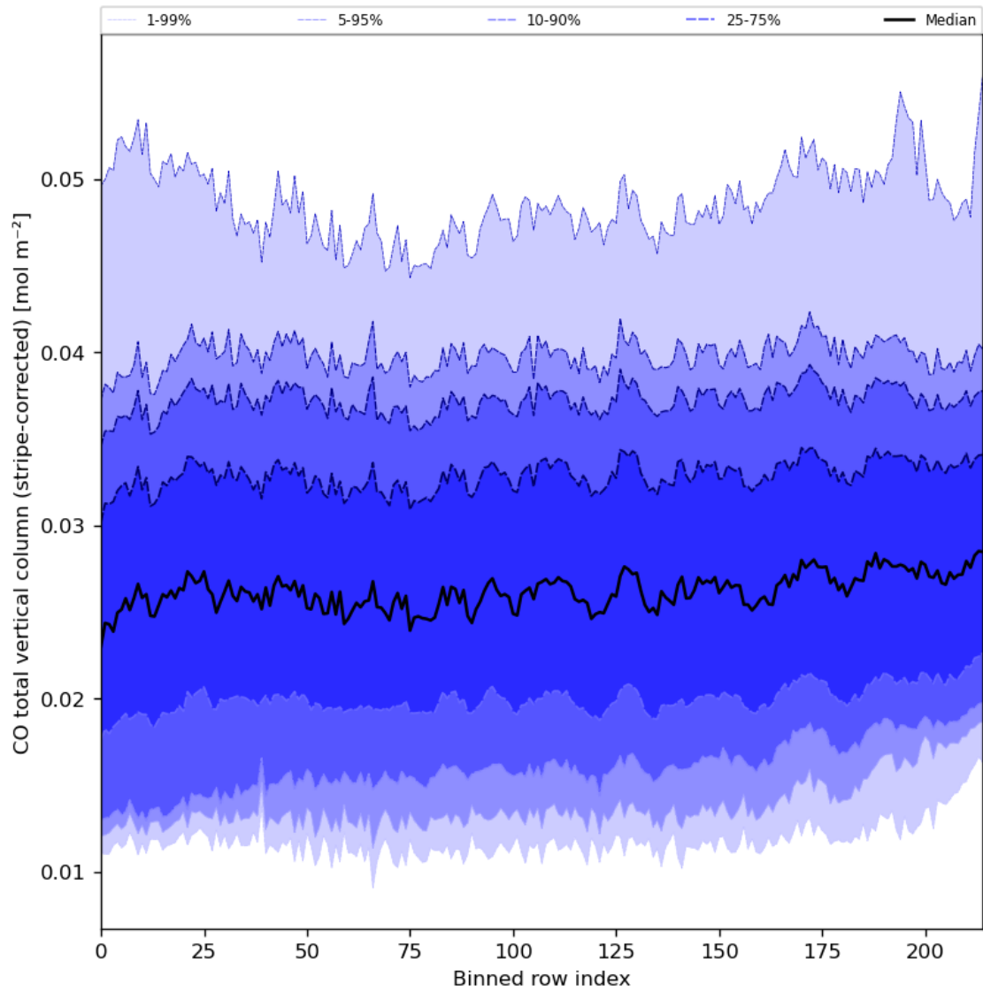
Figure 27: Along track statistics of “CO total vertical column (stripe-corrected)” for 2023-10-17 to 2023-10-19
