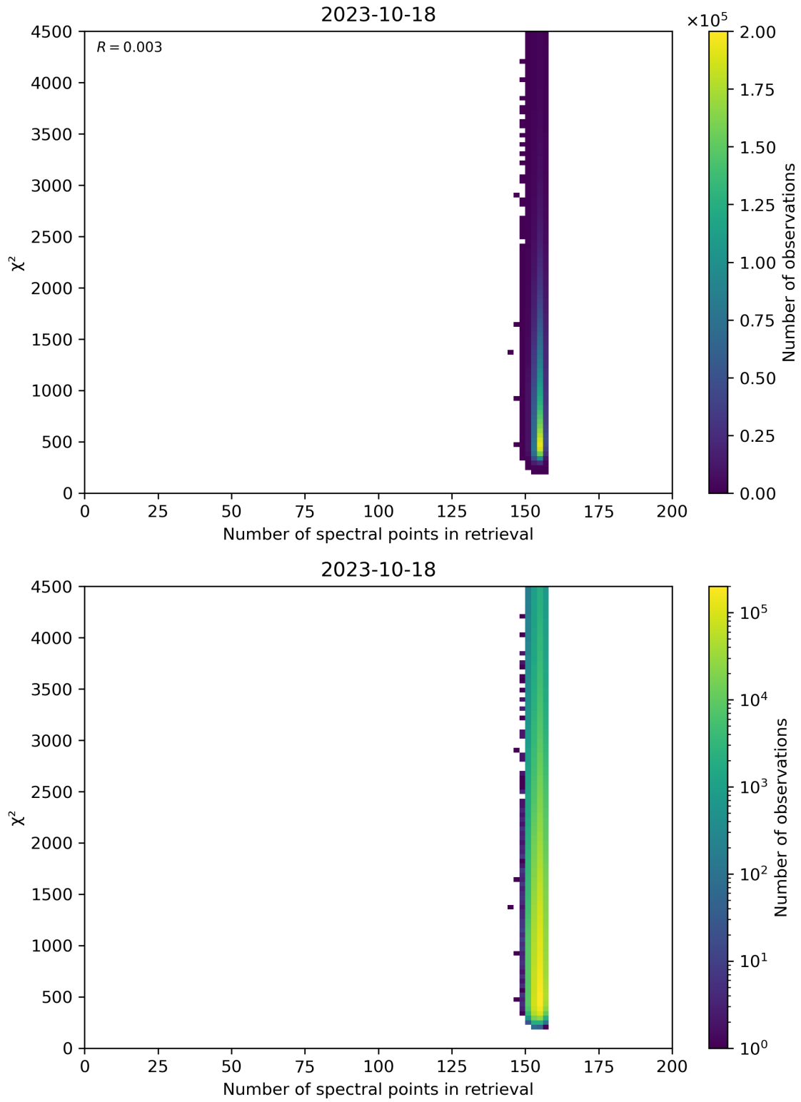
Figure 58: Scatter density plot of “Number of spectral points in retrieval” against “ \chi^2 ” for 2023-10-17 to 2023-10-19.
