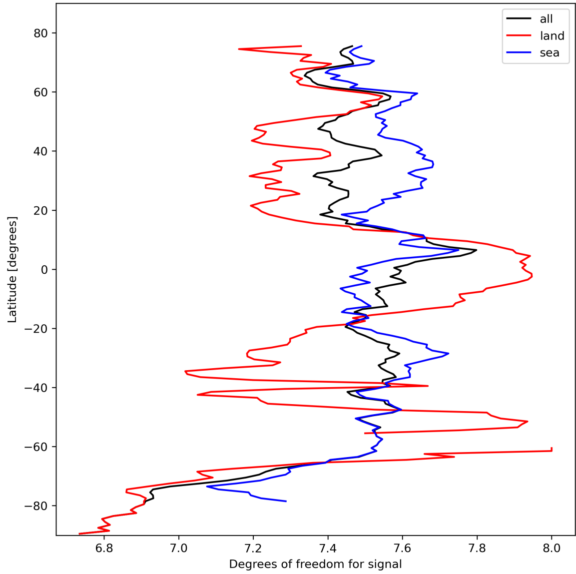
Figure 15: Zonal average of “Degrees of freedom for signal” for 2023-10-17 to 2023-10-19.
