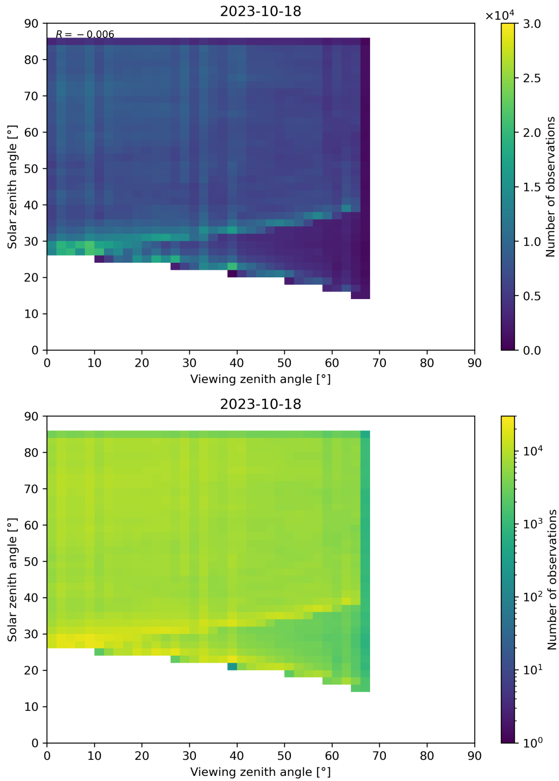
Figure 77: Scatter density plot of “Viewing zenith angle” against “Solar zenith angle” for 2023-10-17 to 2023-10-19.
