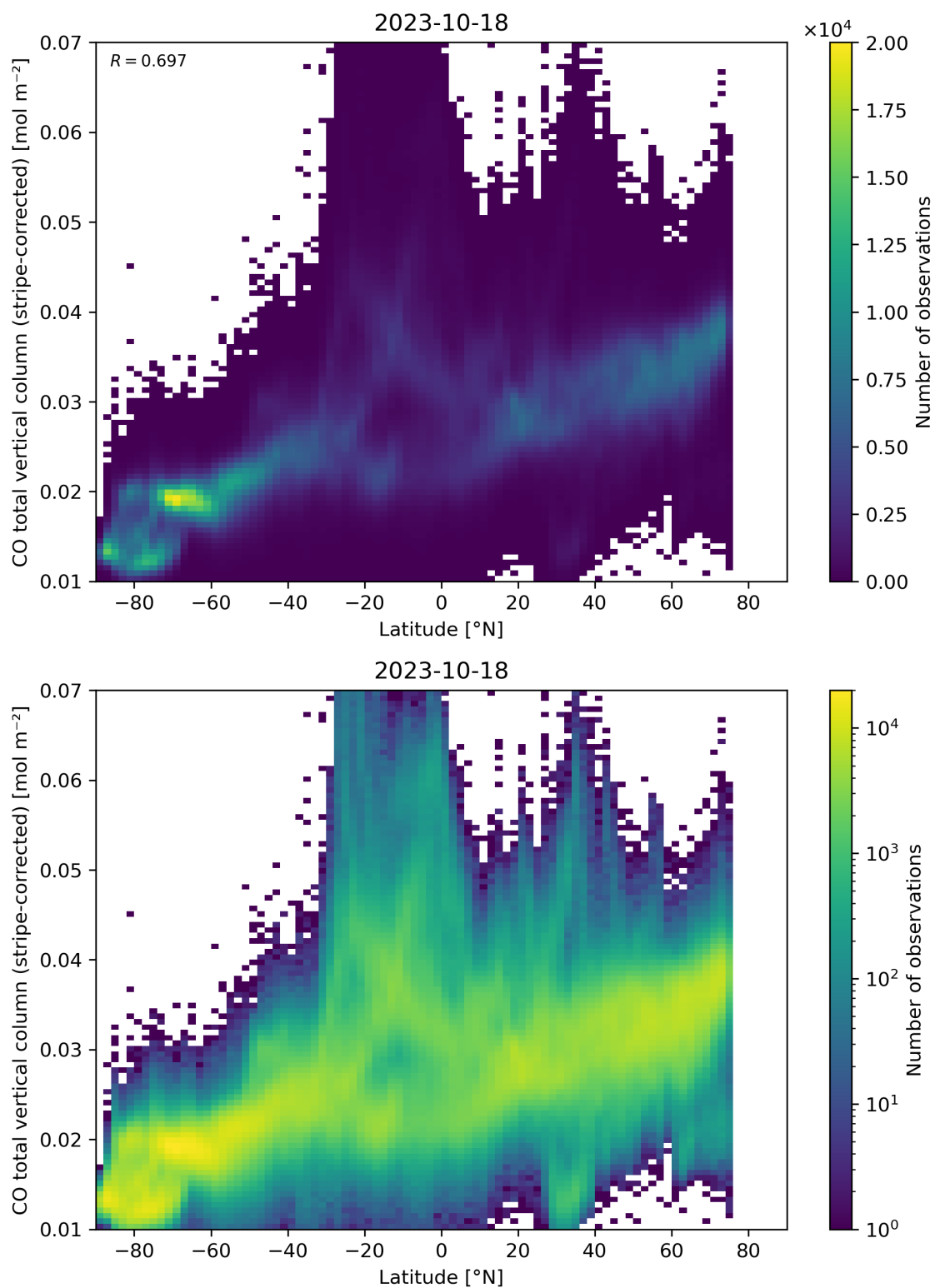
Figure 52: Scatter density plot of “Latitude” against “CO total vertical column (stripe-corrected)” for 2023-10-17 to 2023-10-19.
