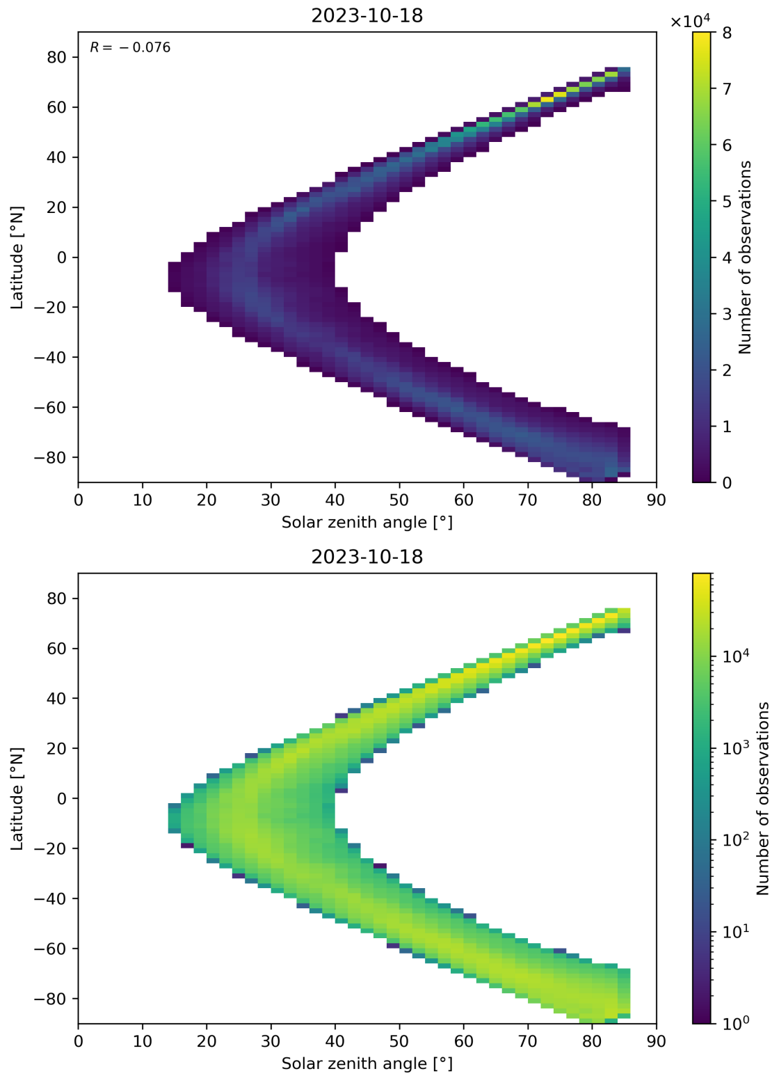
Figure 66: Scatter density plot of “Solar zenith angle” against “Latitude” for 2023-10-17 to 2023-10-19.
