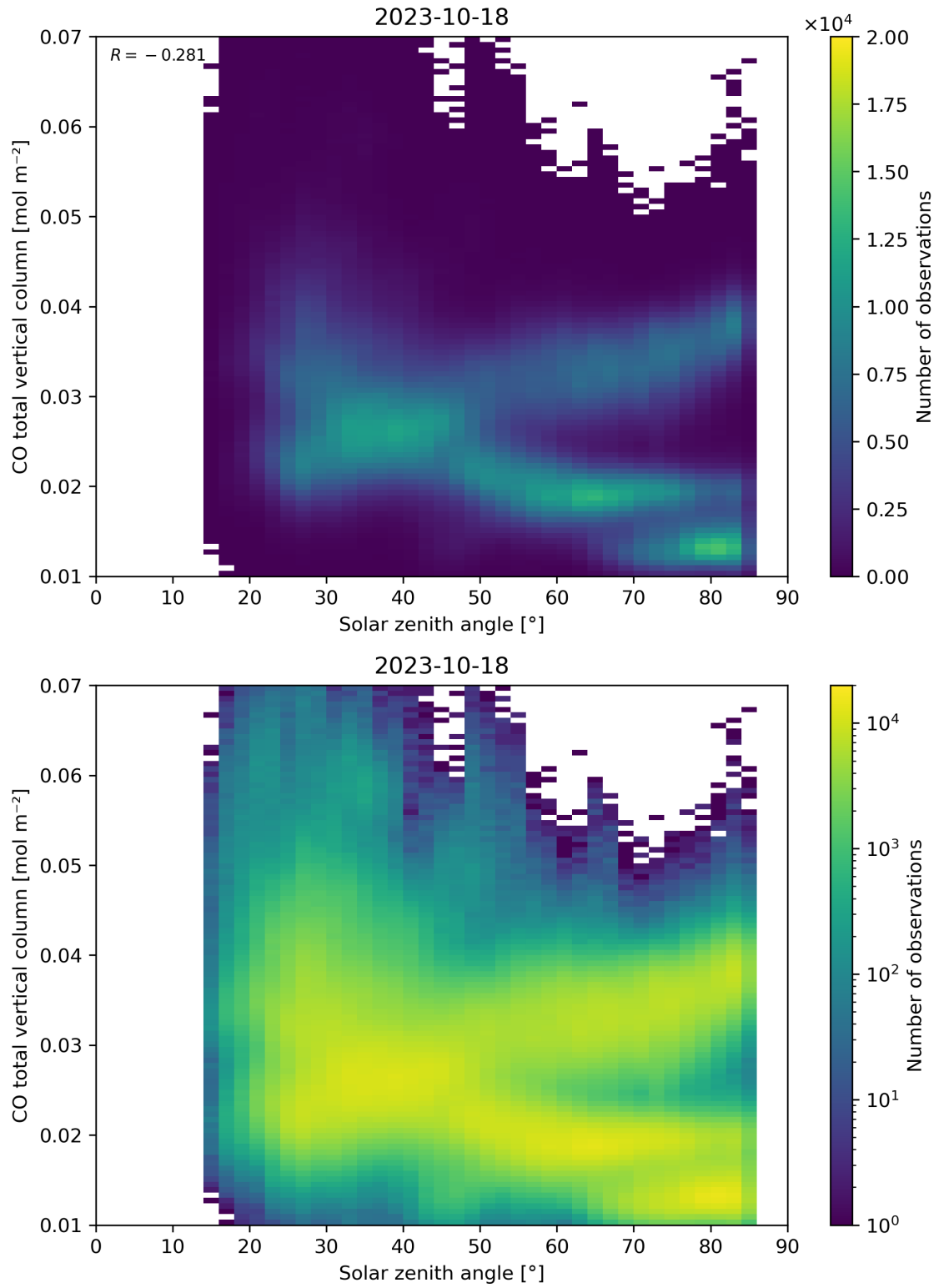
Figure 61: Scatter density plot of “Solar zenith angle” against “CO total vertical column” for 2023-10-17 to 2023-10-19.
