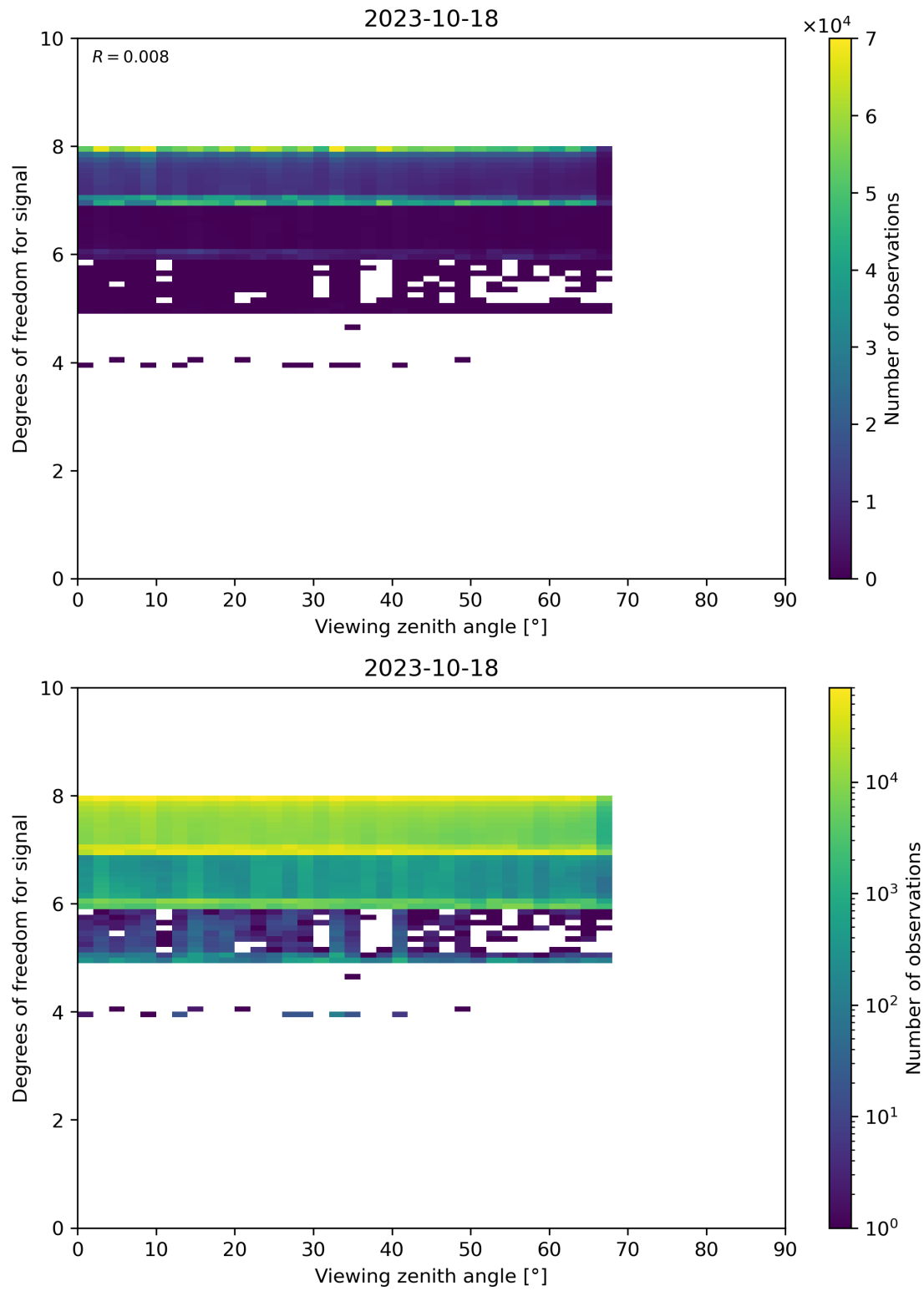
Figure 73: Scatter density plot of “Viewing zenith angle” against “Degrees of freedom for signal” for 2023-10-17 to 2023-10-19.
