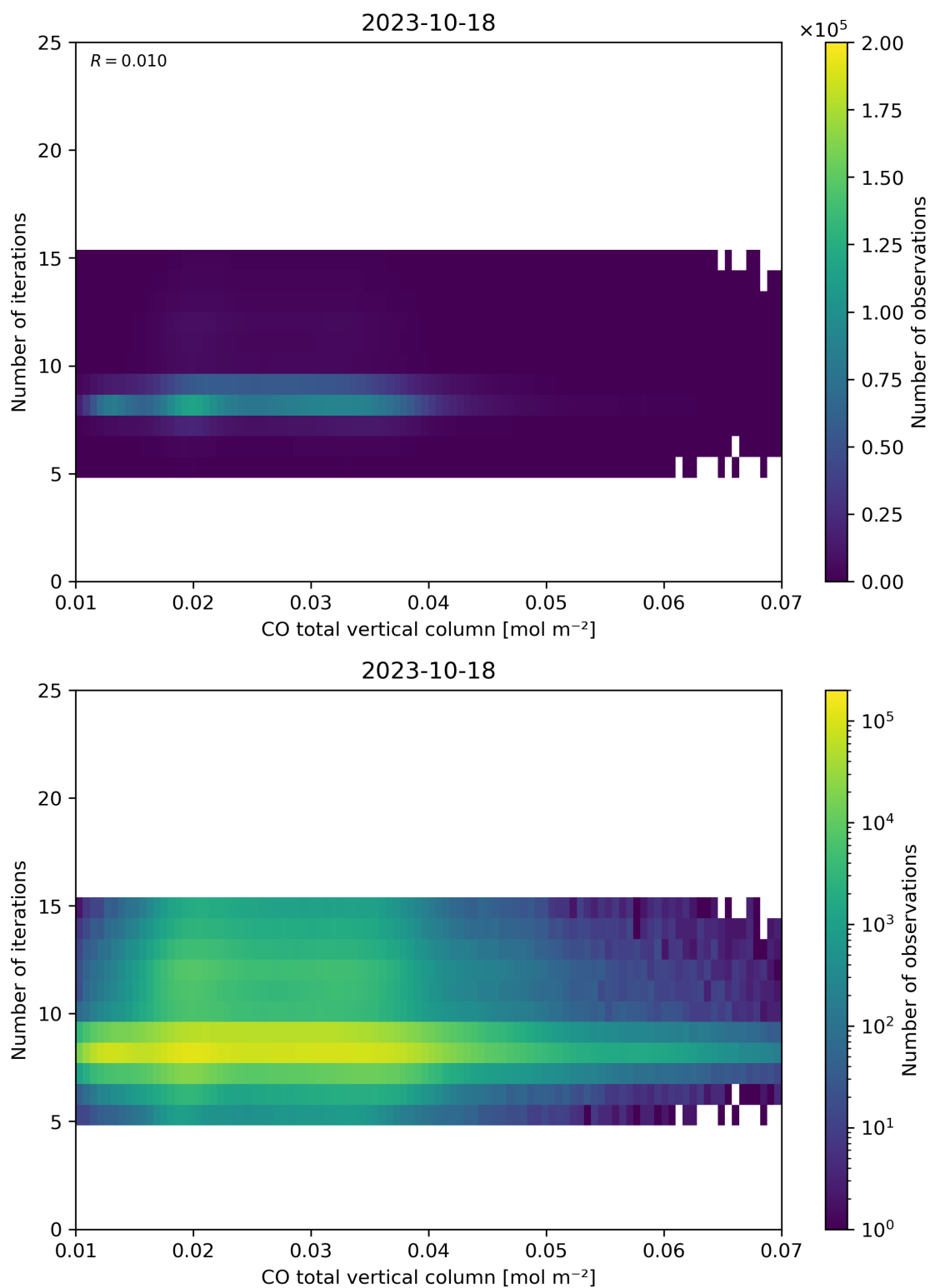
Figure 42: Scatter density plot of “CO total vertical column” against “Number of iterations” for 2023-10-17 to 2023-10-19.
