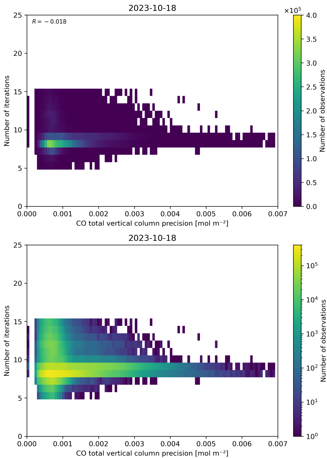
Figure 46: Scatter density plot of “CO total vertical column precision” against “Number of iterations” for 2023-10-17 to 2023-10-19.
