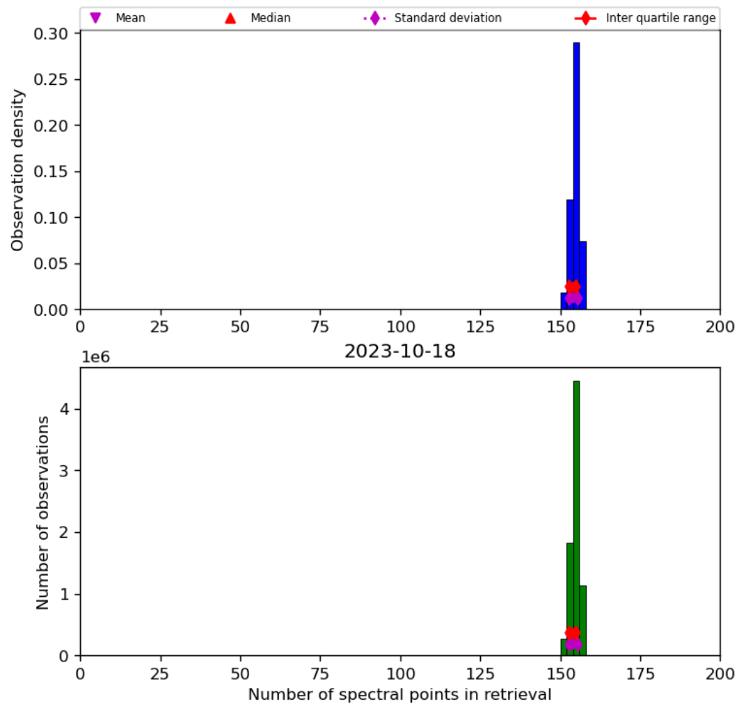
Figure 21: Histogram of “Number of spectral points in retrieval” for 2023-10-17 to 2023-10-19
