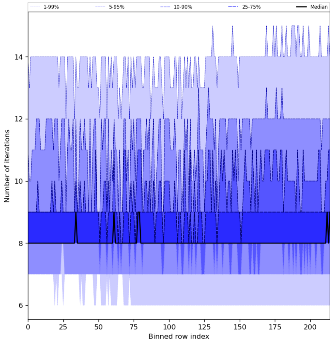
Figure 32: Along track statistics of “Number of iterations” for 2023-10-17 to 2023-10-19
