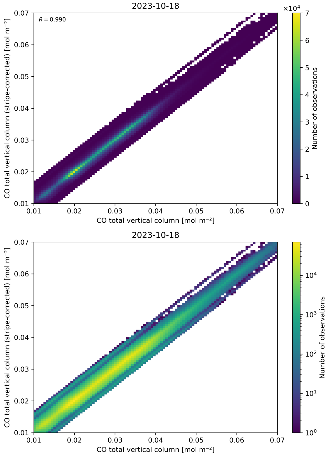
Figure 33: Scatter density plot of “CO total vertical column” against “CO total vertical column (stripe-corrected)” for 2023-10-17 to 2023-10-19.
