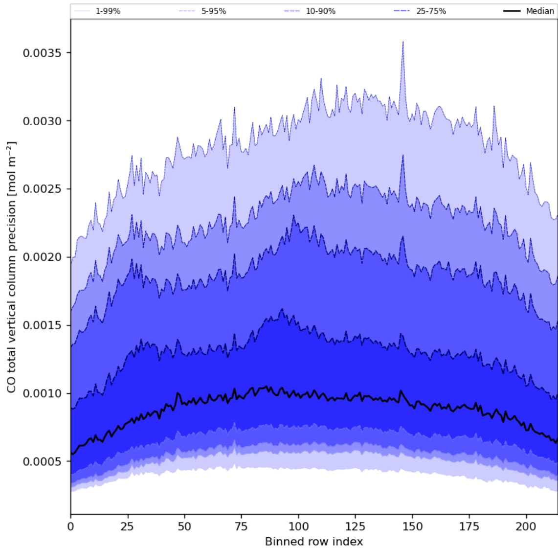
Figure 28: Along track statistics of “CO total vertical column precision” for 2023-10-17 to 2023-10-19
