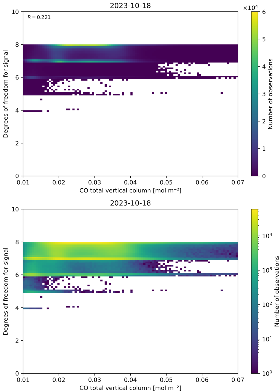
Figure 41: Scatter density plot of “CO total vertical column” against “Degrees of freedom for signal” for 2023-10-17 to 2023-10-19.
