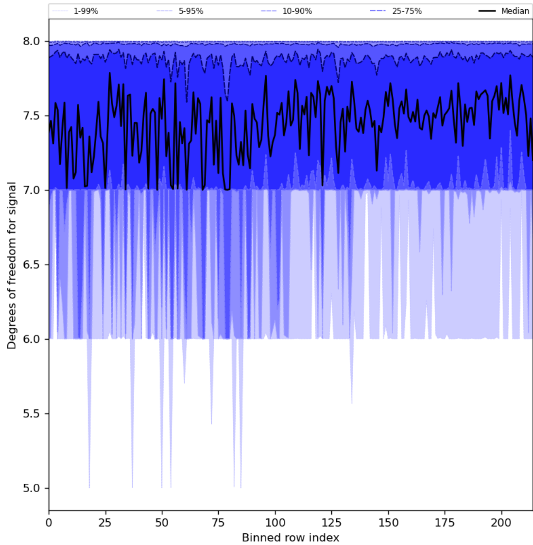
Figure 31: Along track statistics of “Degrees of freedom for signal” for 2023-10-17 to 2023-10-19
