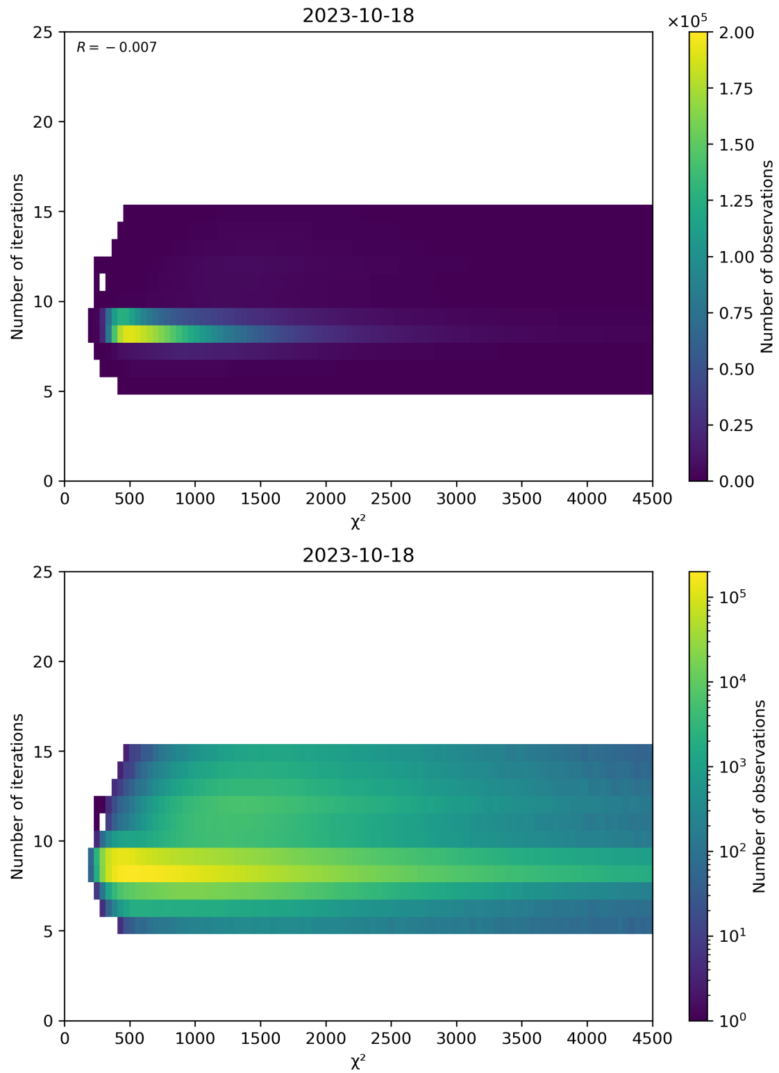
Figure 49: Scatter density plot of “ \chi^2 ” against “Number of iterations” for 2023-10-17 to 2023-10-19.
