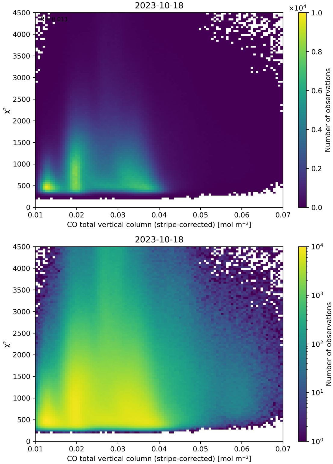
Figure 37: Scatter density plot of “CO total vertical column (stripe-corrected)” against “ \chi^2 ” for 2023-10-17 to 2023-10-19.
