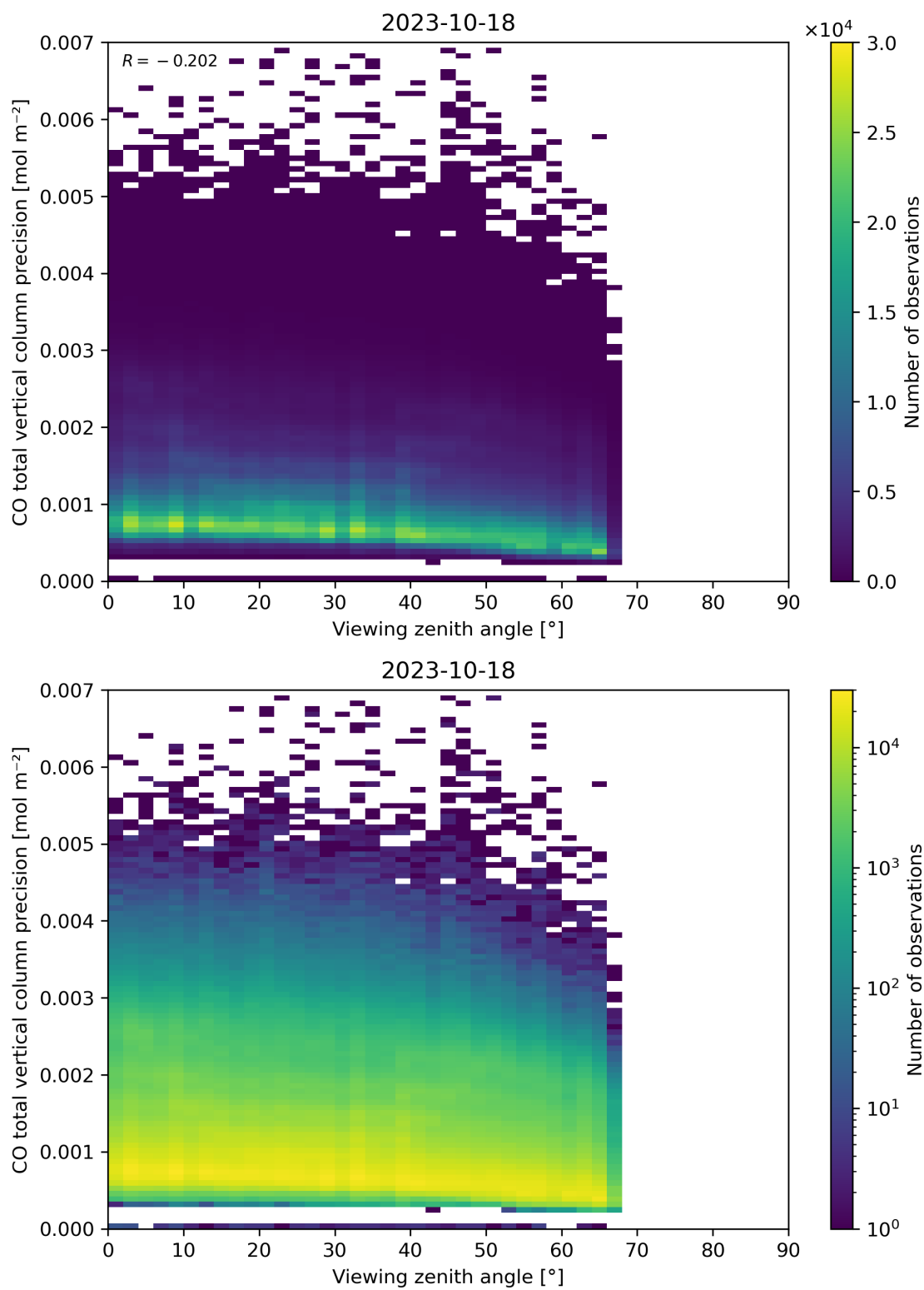
Figure 71: Scatter density plot of “Viewing zenith angle” against “CO total vertical column precision” for 2023-10-17 to 2023-10-19.
