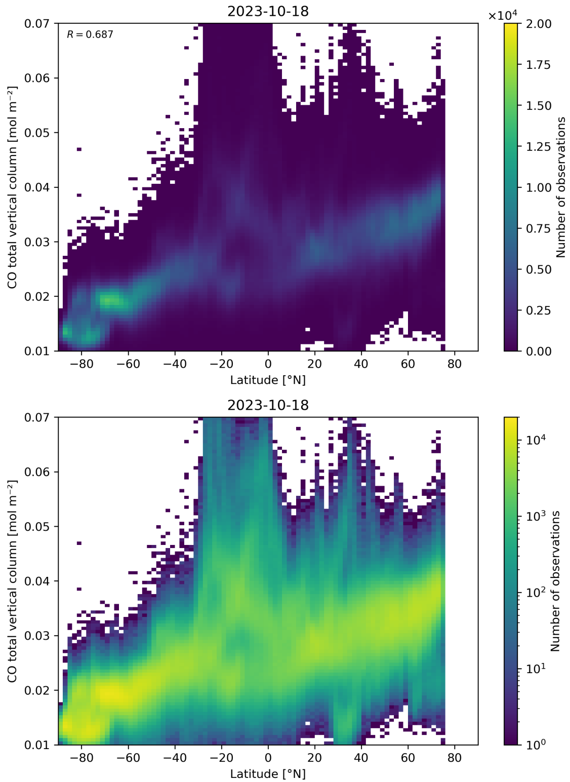
Figure 51: Scatter density plot of “Latitude” against “CO total vertical column” for 2023-10-17 to 2023-10-19.
