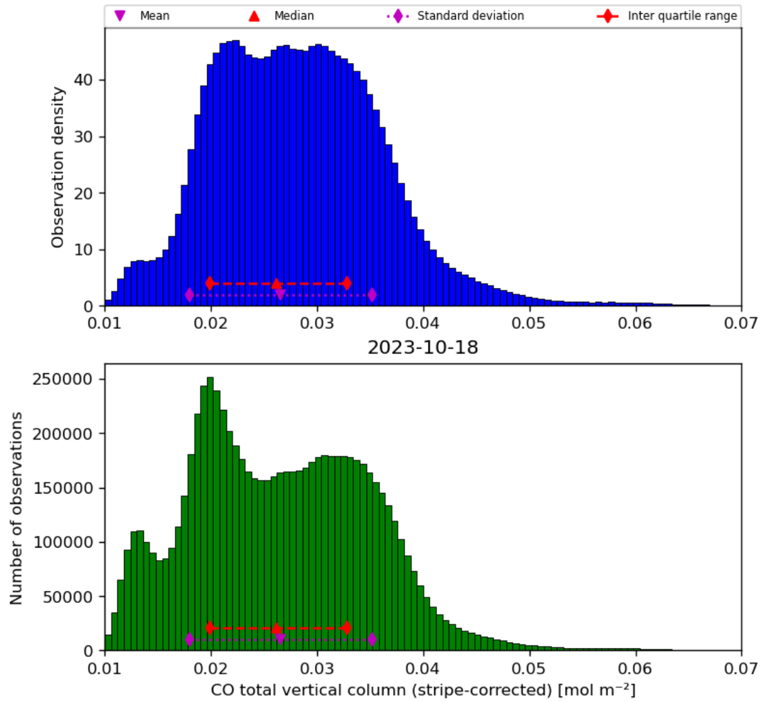
Figure 19: Histogram of “CO total vertical column (stripe-corrected)” for 2023-10-17 to 2023-10-19
