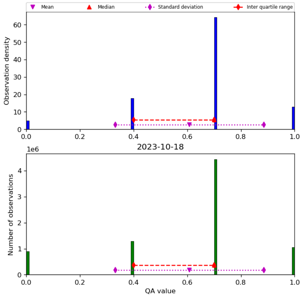
Figure 17: Histogram of “QA value” for 2023-10-17 to 2023-10-19
