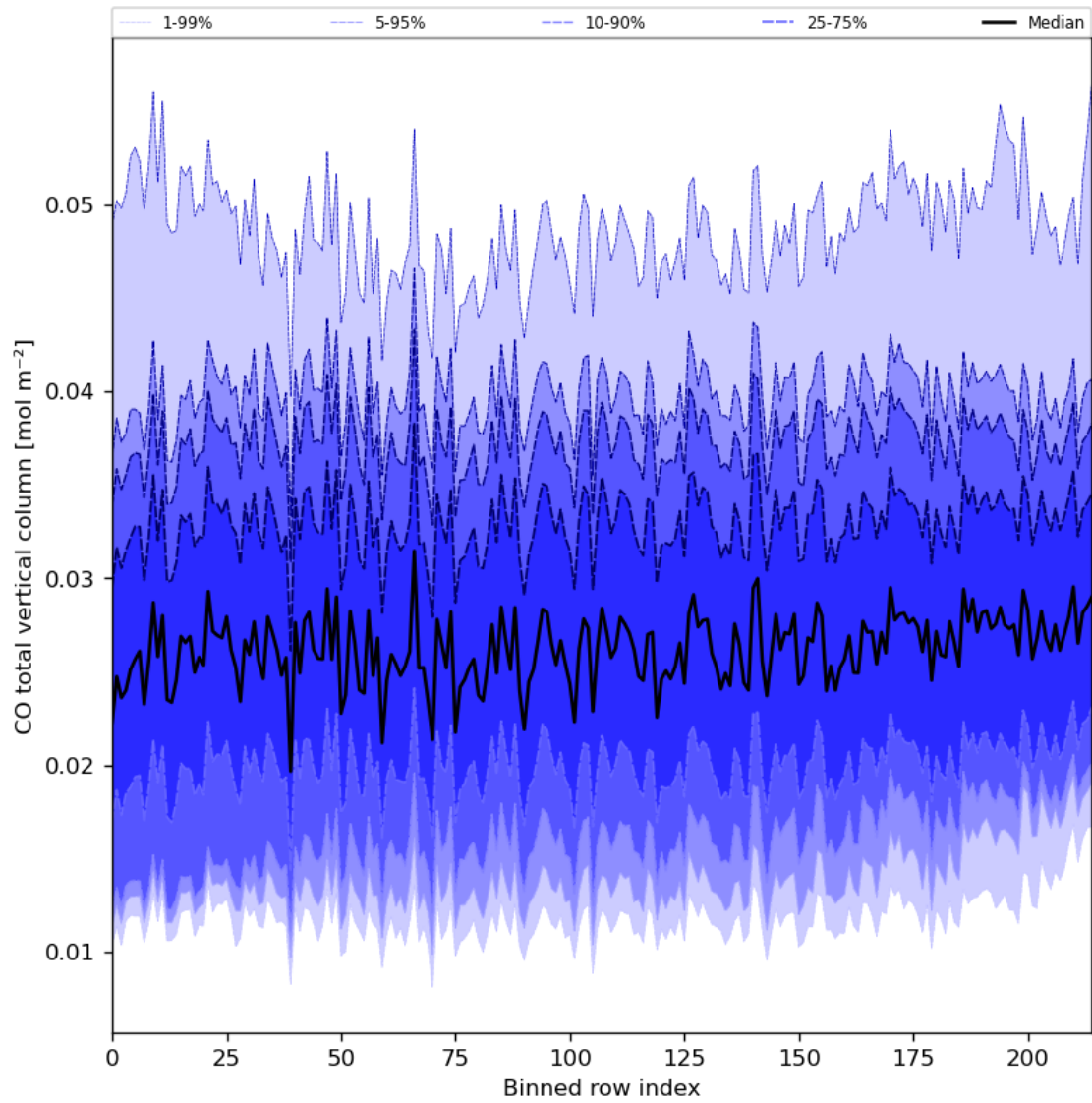
Figure 26: Along track statistics of "CO total vertical column" for 2023-10-17 to 2023-10-19
