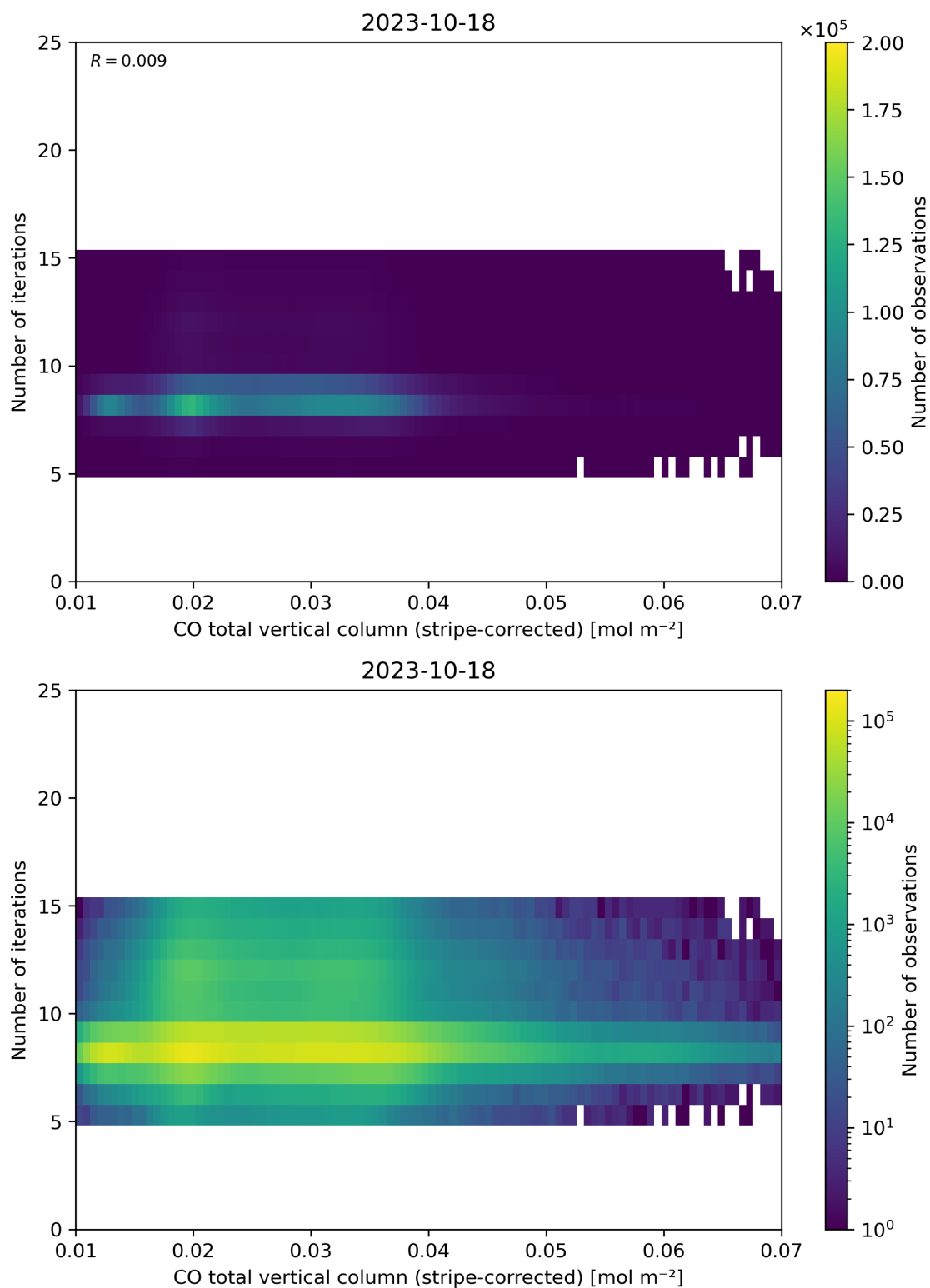
Figure 39: Scatter density plot of “CO total vertical column (stripe-corrected)” against “Number of iterations” for 2023-10-17 to 2023-10-19.
