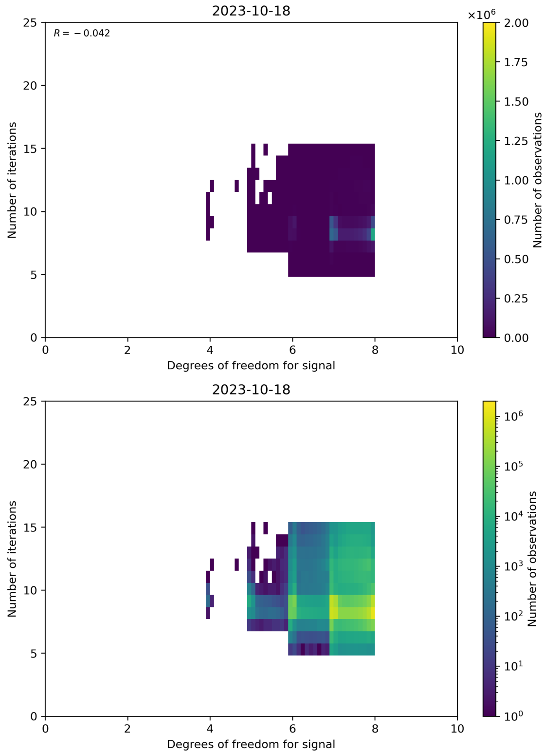
Figure 50: Scatter density plot of “Degrees of freedom for signal” against “Number of iterations” for 2023-10-17 to 2023-10-19.
