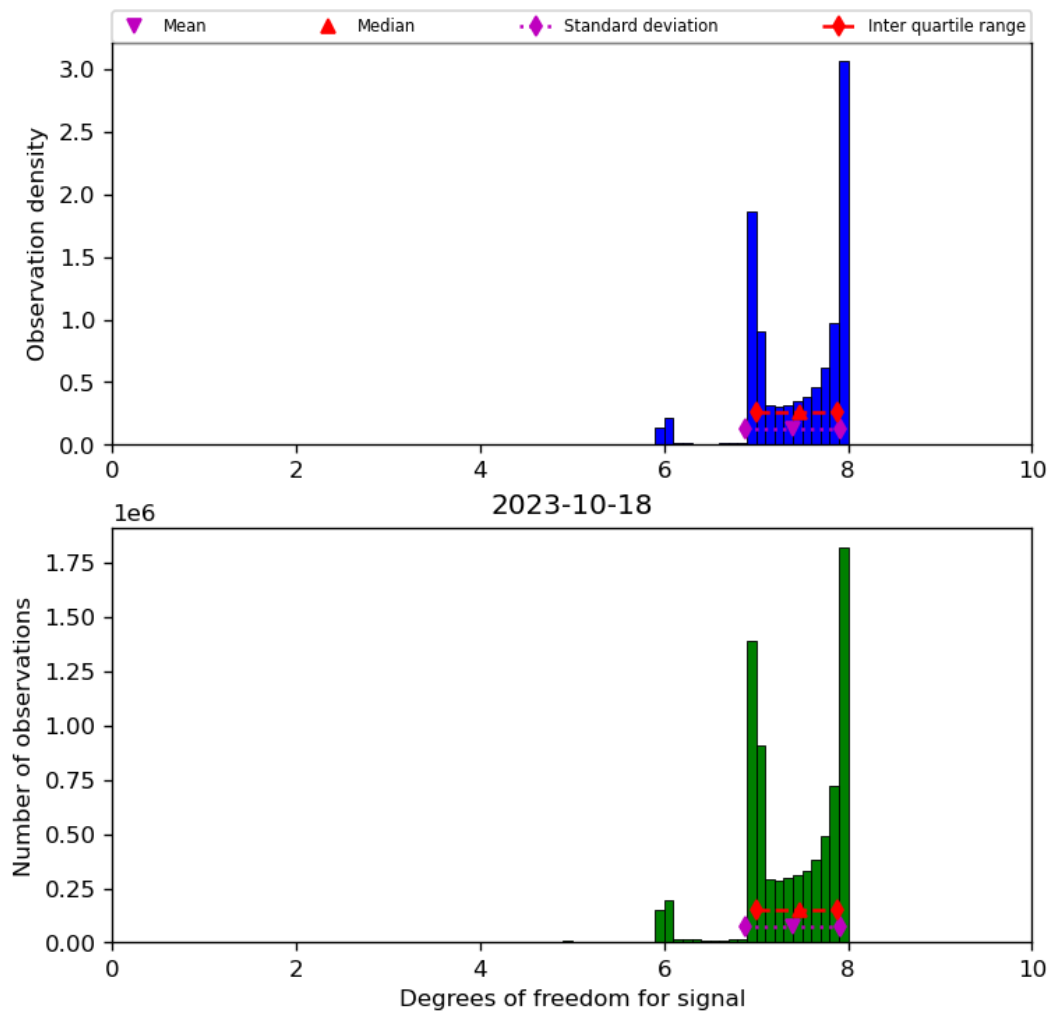
Figure 23: Histogram of “Degrees of freedom for signal” for 2023-10-17 to 2023-10-19
