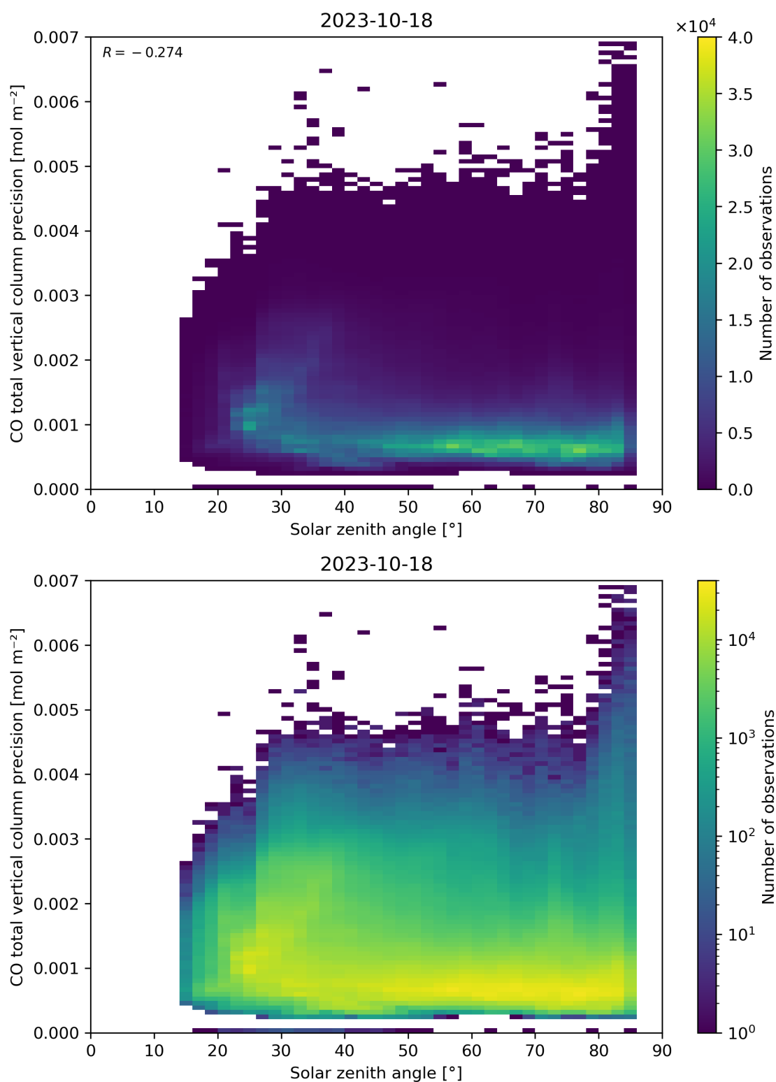
Figure 63: Scatter density plot of “Solar zenith angle” against “CO total vertical column precision” for 2023-10-17 to 2023-10-19.
