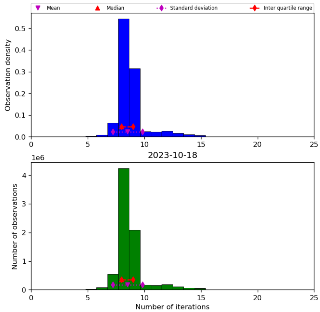
Figure 24: Histogram of “Number of iterations” for 2023-10-17 to 2023-10-19
