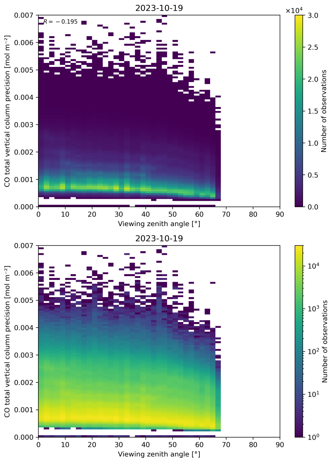
Figure 71: Scatter density plot of “Viewing zenith angle” against “CO total vertical column precision” for 2023-10-18 to 2023-10-20.
