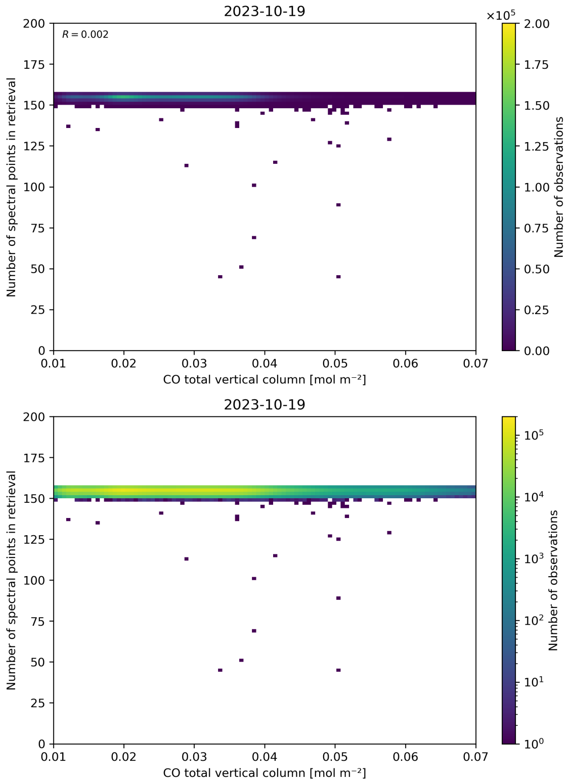
Figure 43: Scatter density plot of “CO total vertical column” against “Number of spectral points in retrieval” for 2023-10-18 to 2023-10-20.
