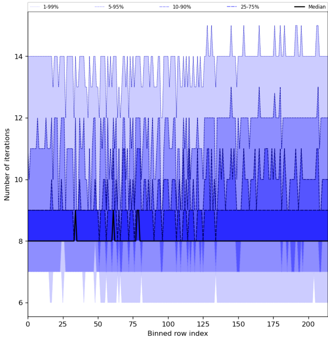
Figure 32: Along track statistics of “Number of iterations” for 2023-10-18 to 2023-10-20
