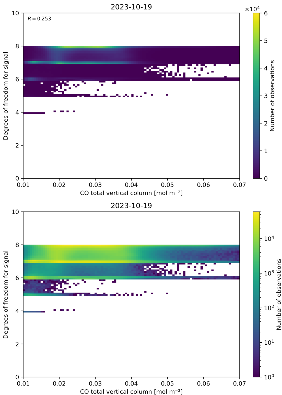
Figure 41: Scatter density plot of “CO total vertical column” against “Degrees of freedom for signal” for 2023-10-18 to 2023-10-20.
