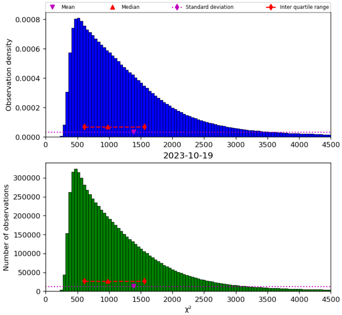
Figure 22: Histogram of “ \chi^2 ” for 2023-10-18 to 2023-10-20
