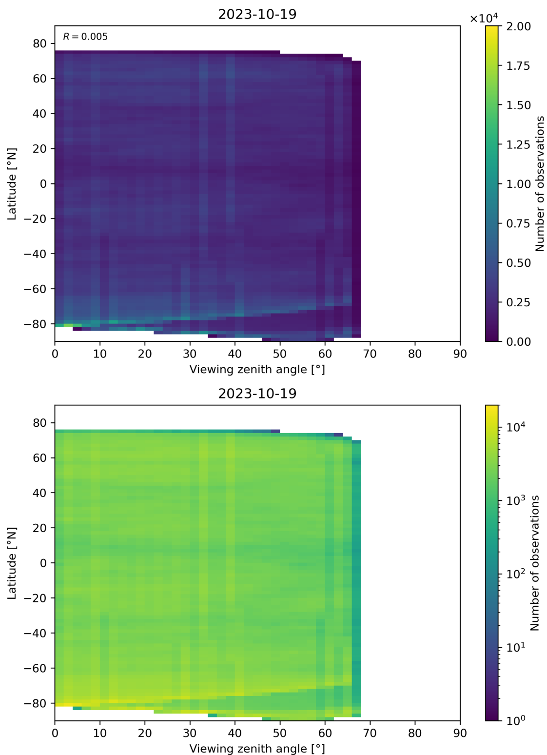
Figure 74: Scatter density plot of “Viewing zenith angle” against “Latitude” for 2023-10-18 to 2023-10-20.
