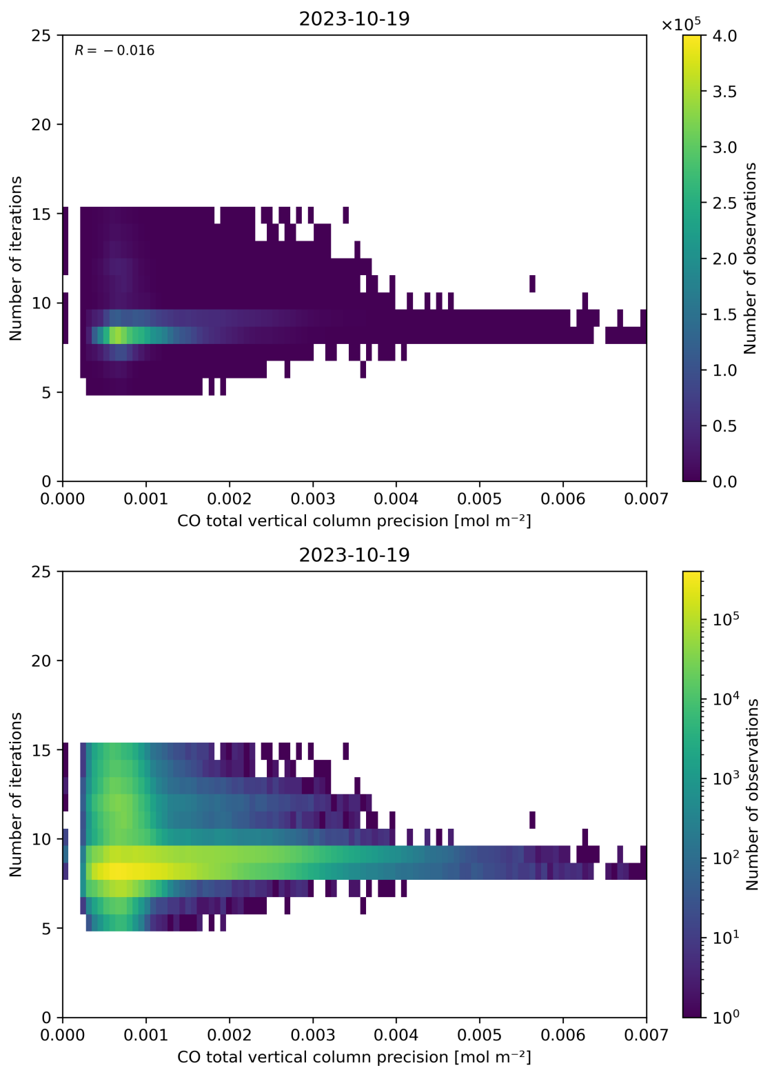
Figure 46: Scatter density plot of “CO total vertical column precision” against “Number of iterations” for 2023-10-18 to 2023-10-20.
