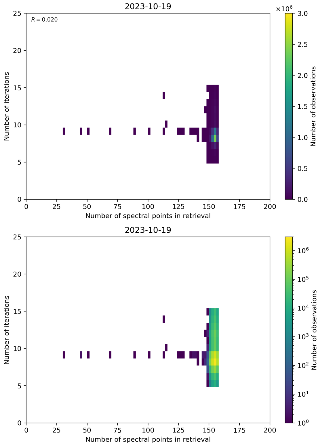
Figure 60: Scatter density plot of “Number of spectral points in retrieval” against “Number of iterations” for 2023-10-18 to 2023-10-20.
