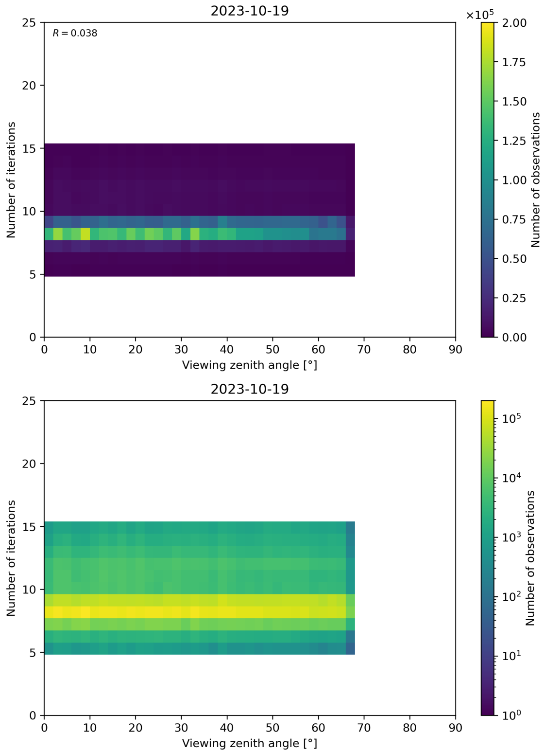
Figure 75: Scatter density plot of “Viewing zenith angle” against “Number of iterations” for 2023-10-18 to 2023-10-20.
