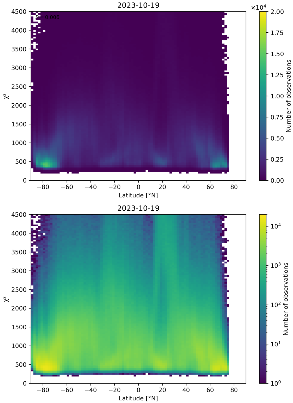
Figure 54: Scatter density plot of “Latitude” against “ \chi^2 ” for 2023-10-18 to 2023-10-20.
