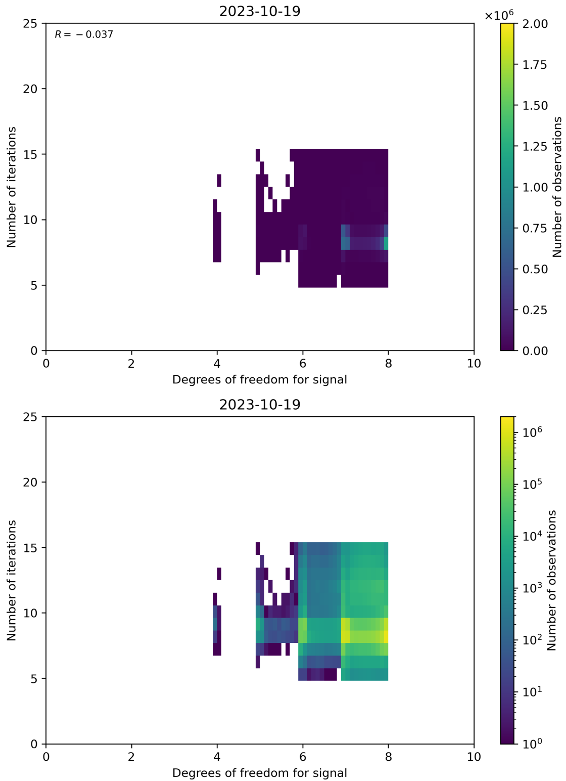
Figure 50: Scatter density plot of “Degrees of freedom for signal” against “Number of iterations” for 2023-10-18 to 2023-10-20.
