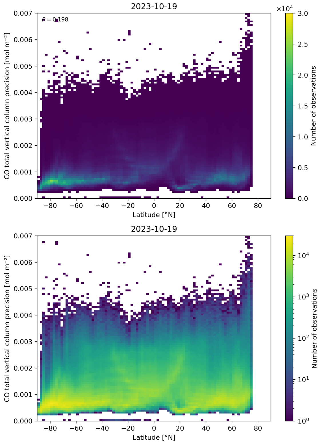
Figure 53: Scatter density plot of “Latitude” against “CO total vertical column precision” for 2023-10-18 to 2023-10-20.
