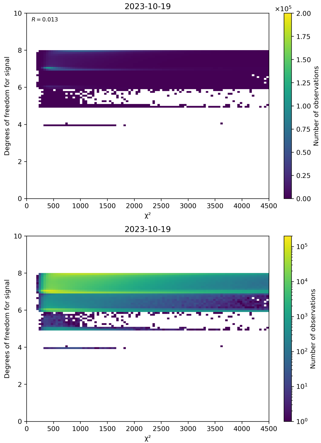
Figure 48: Scatter density plot of “ \chi^2 ” against “Degrees of freedom for signal” for 2023-10-18 to 2023-10-20.
