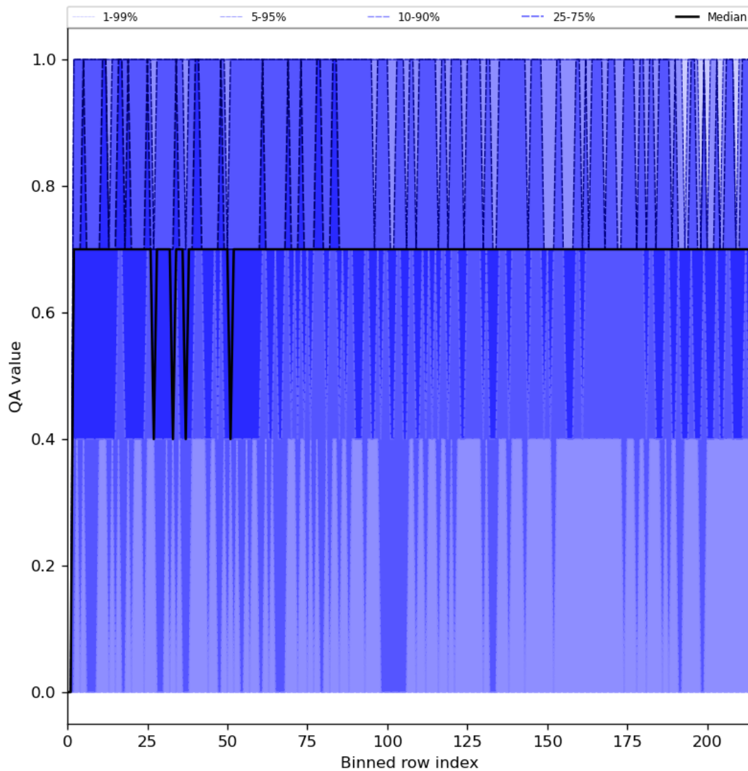
Figure 25: Along track statistics of “QA value” for 2023-10-18 to 2023-10-20
