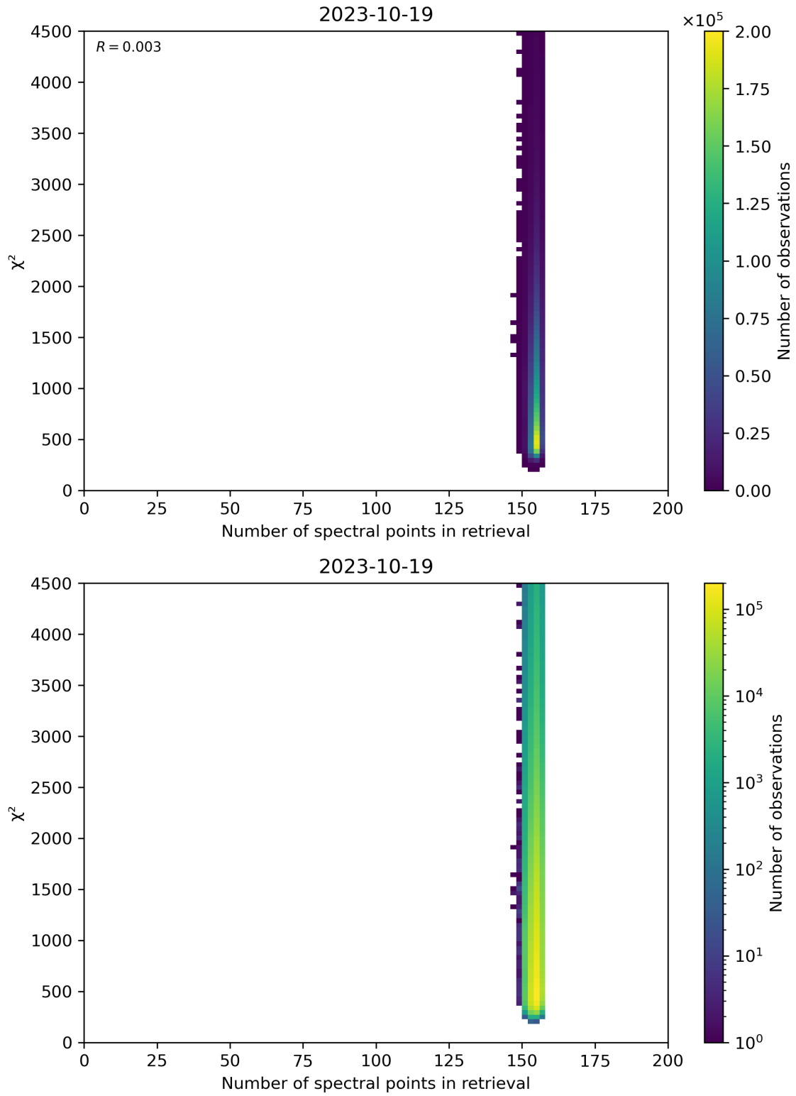
Figure 58: Scatter density plot of “Number of spectral points in retrieval” against “ \chi^2 ” for 2023-10-18 to 2023-10-20.
