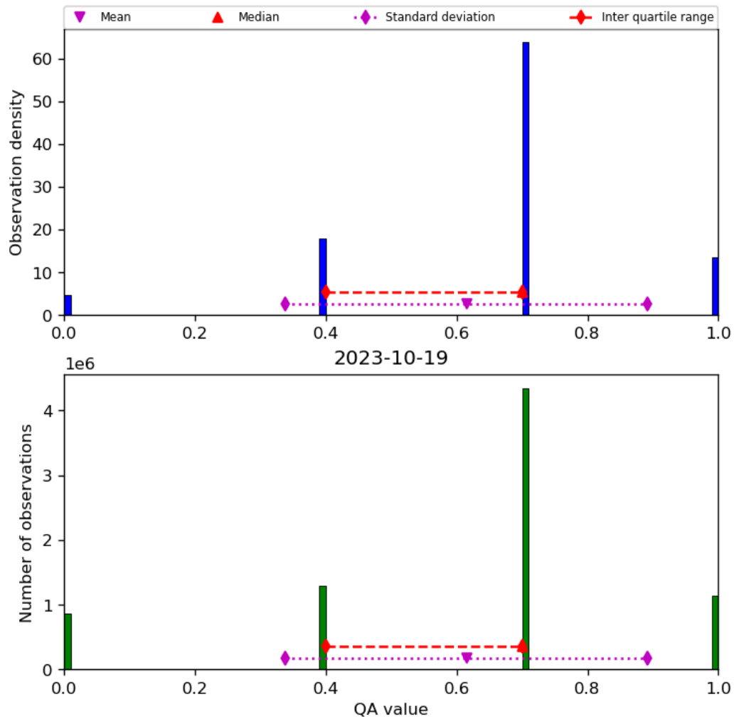
Figure 17: Histogram of "QA value" for 2023-10-18 to 2023-10-20
