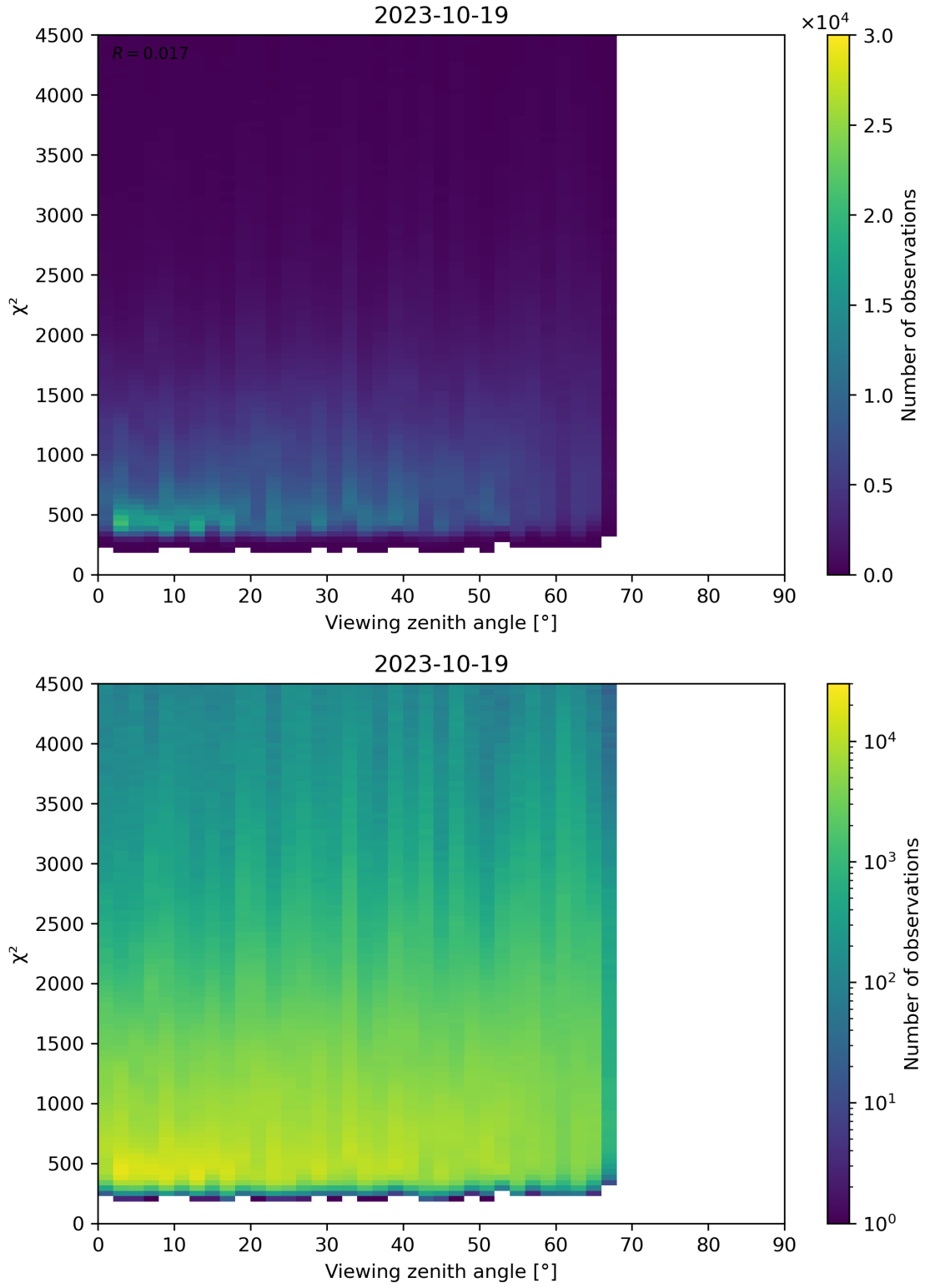
Figure 72: Scatter density plot of “Viewing zenith angle” against “ \chi^2 ” for 2023-10-18 to 2023-10-20.
