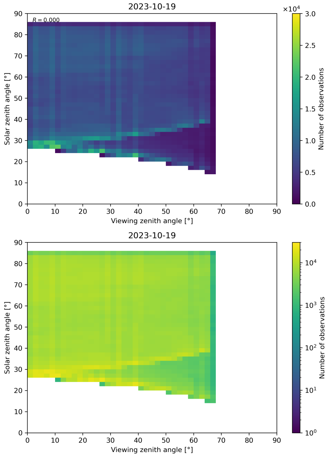
Figure 77: Scatter density plot of “Viewing zenith angle” against “Solar zenith angle” for 2023-10-18 to 2023-10-20.
