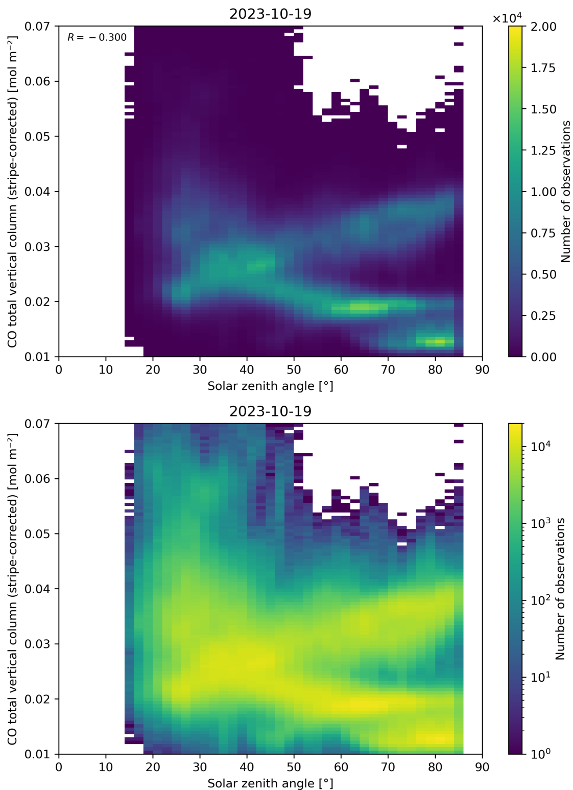
Figure 62: Scatter density plot of “Solar zenith angle” against “CO total vertical column (stripe-corrected)” for 2023-10-18 to 2023-10-20.
