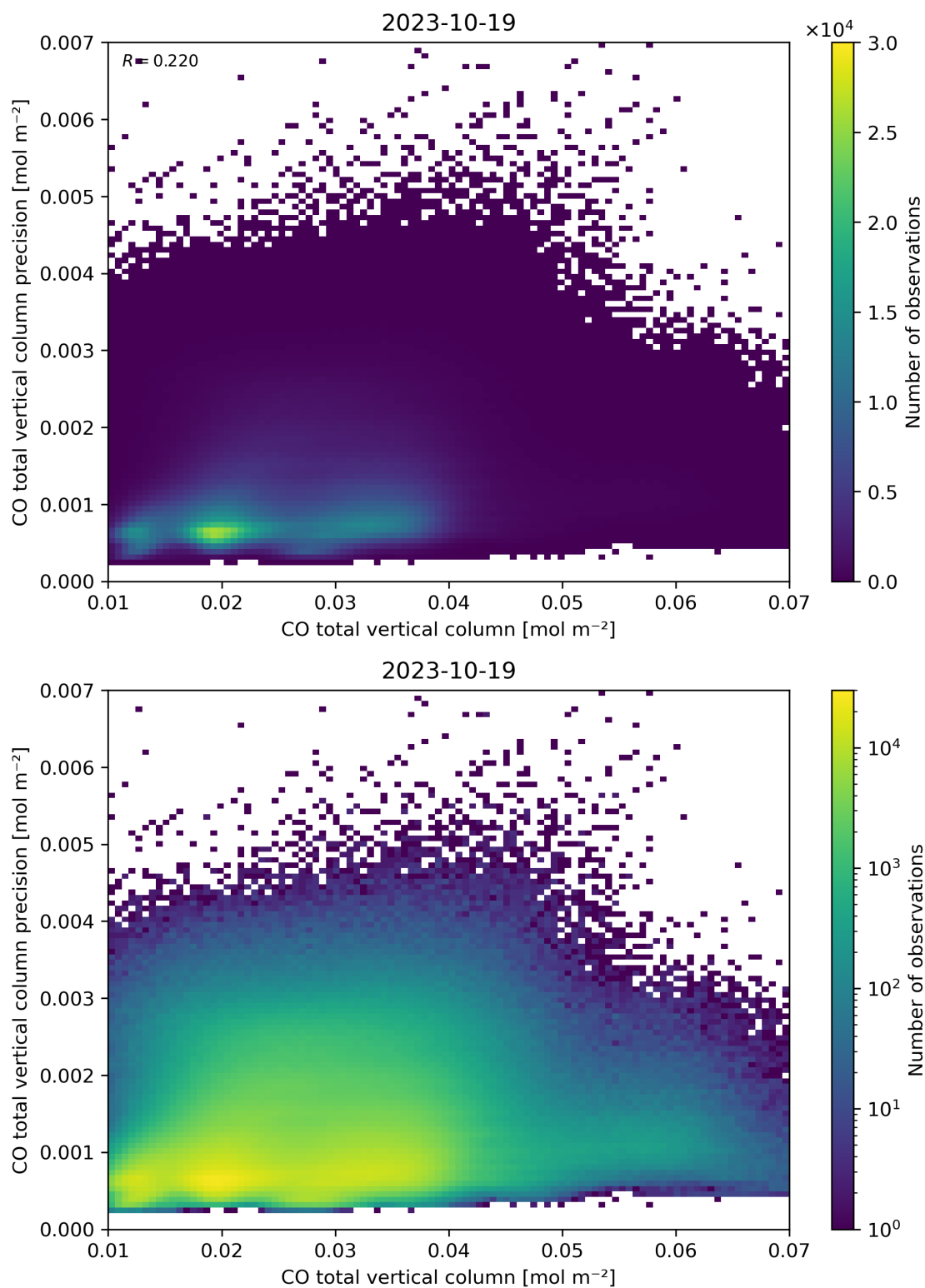
Figure 34: Scatter density plot of “CO total vertical column” against “CO total vertical column precision” for 2023-10-18 to 2023-10-20.
