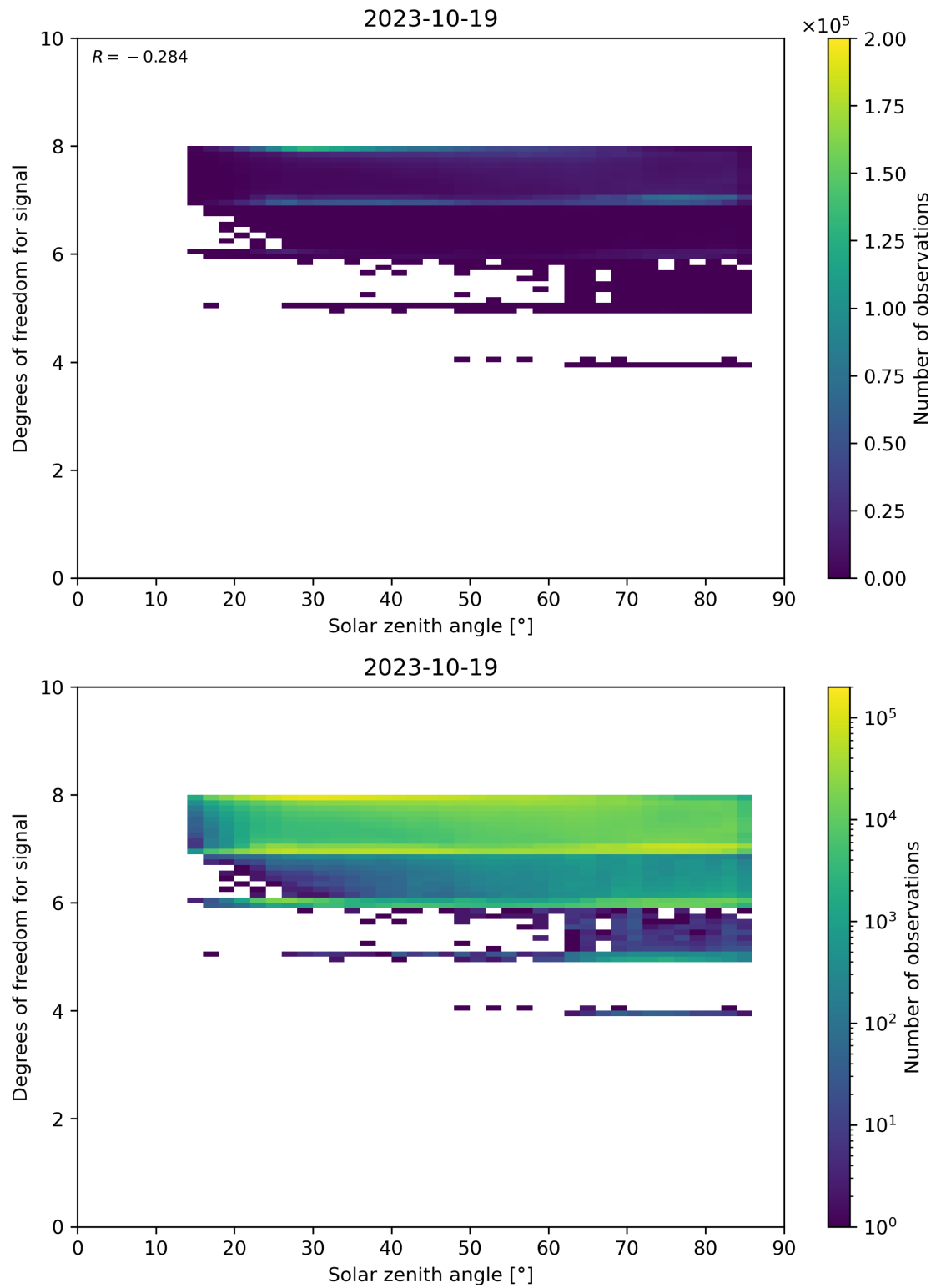
Figure 65: Scatter density plot of “Solar zenith angle” against “Degrees of freedom for signal” for 2023-10-18 to 2023-10-20.
