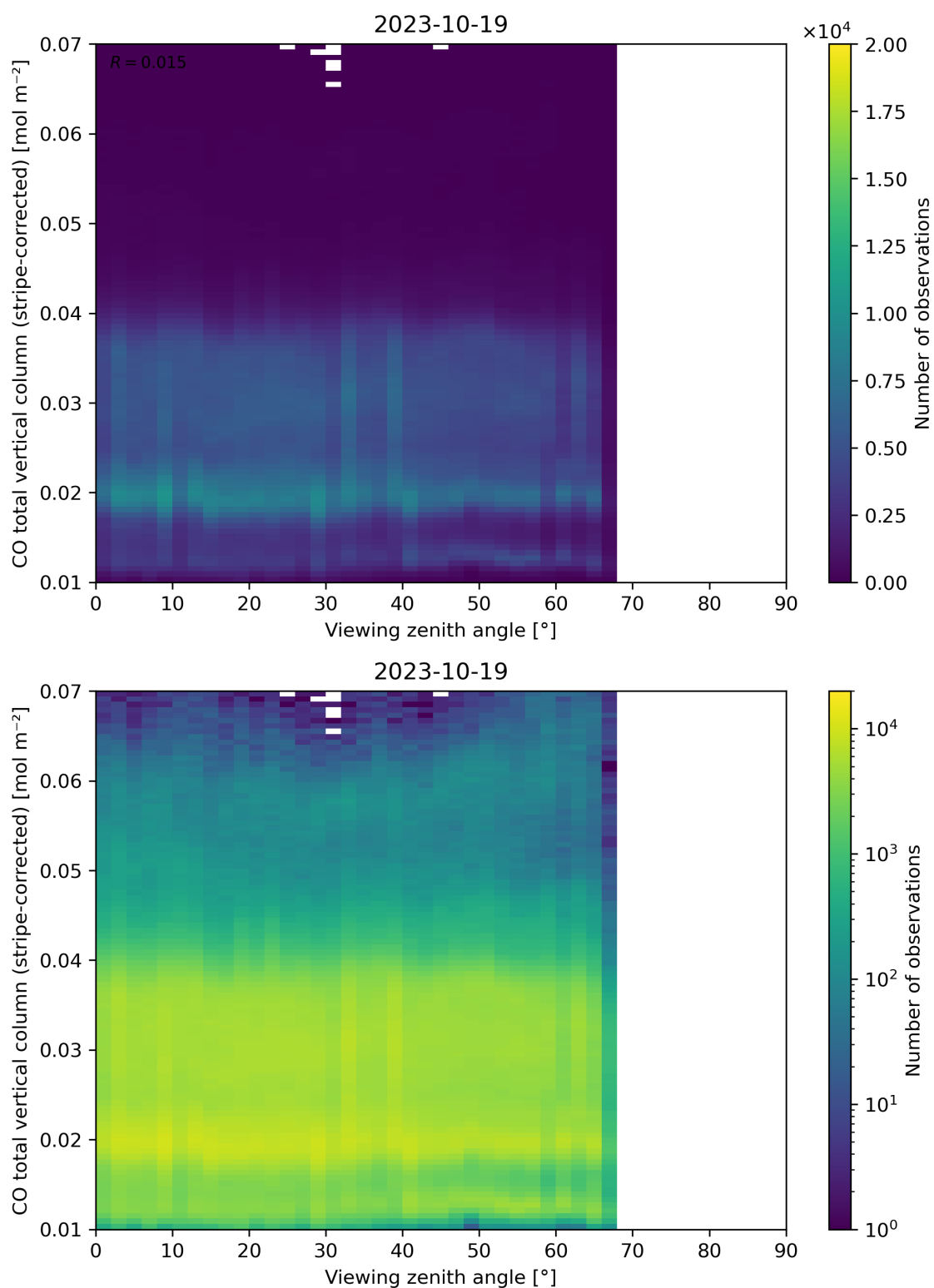
Figure 70: Scatter density plot of “Viewing zenith angle” against “CO total vertical column (stripe-corrected)” for 2023-10-18 to 2023-10-20.
