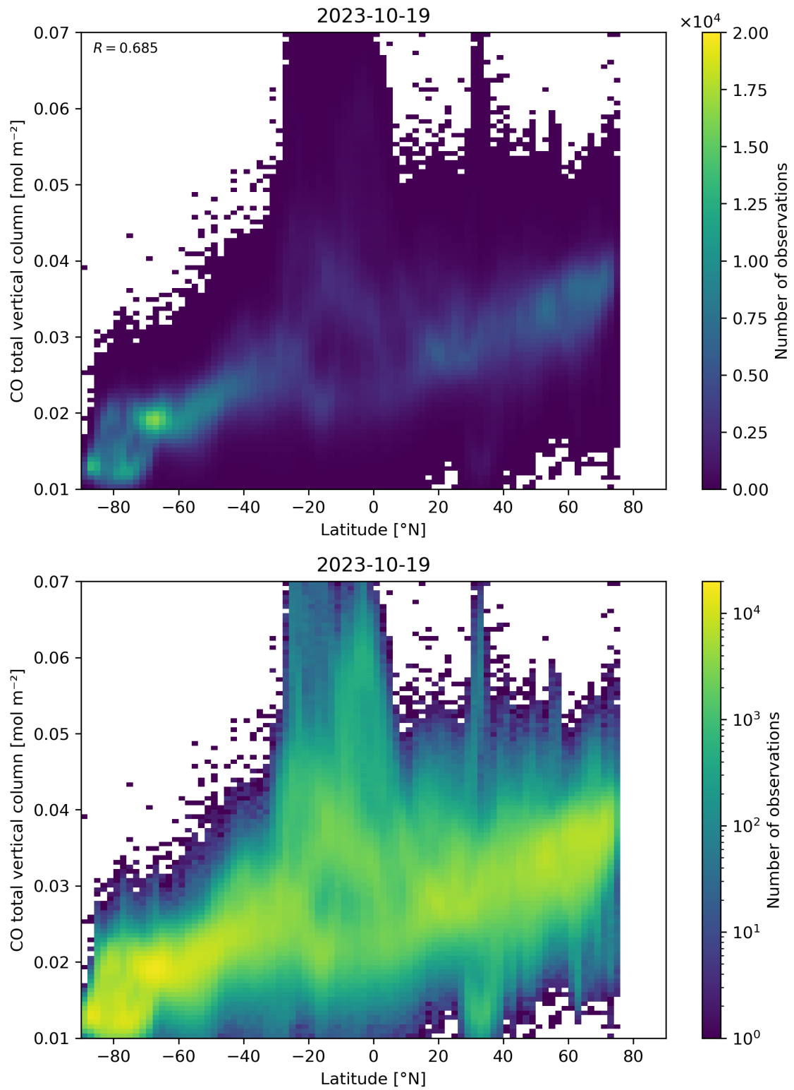
Figure 51: Scatter density plot of “Latitude” against “CO total vertical column” for 2023-10-18 to 2023-10-20.
