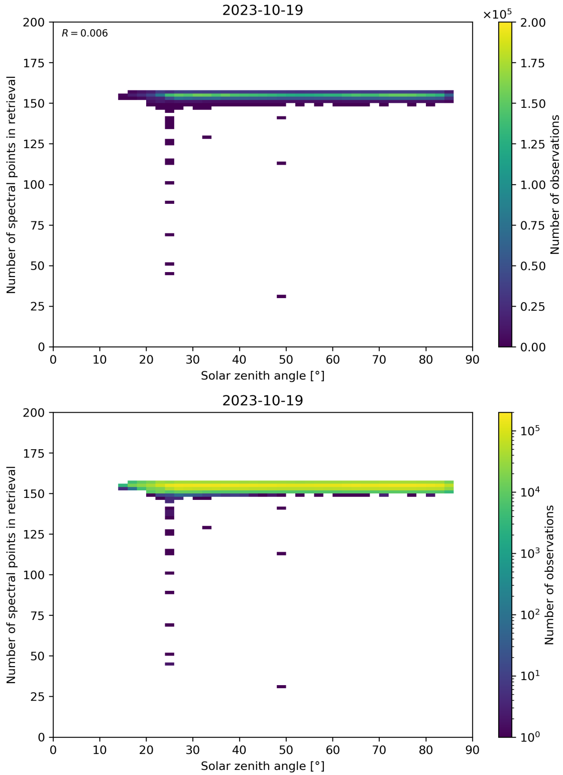
Figure 68: Scatter density plot of “Solar zenith angle” against “Number of spectral points in retrieval” for 2023-10-18 to 2023-10-20.
