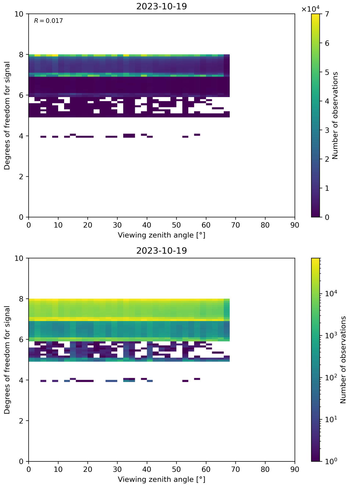
Figure 73: Scatter density plot of “Viewing zenith angle” against “Degrees of freedom for signal” for 2023-10-18 to 2023-10-20.
