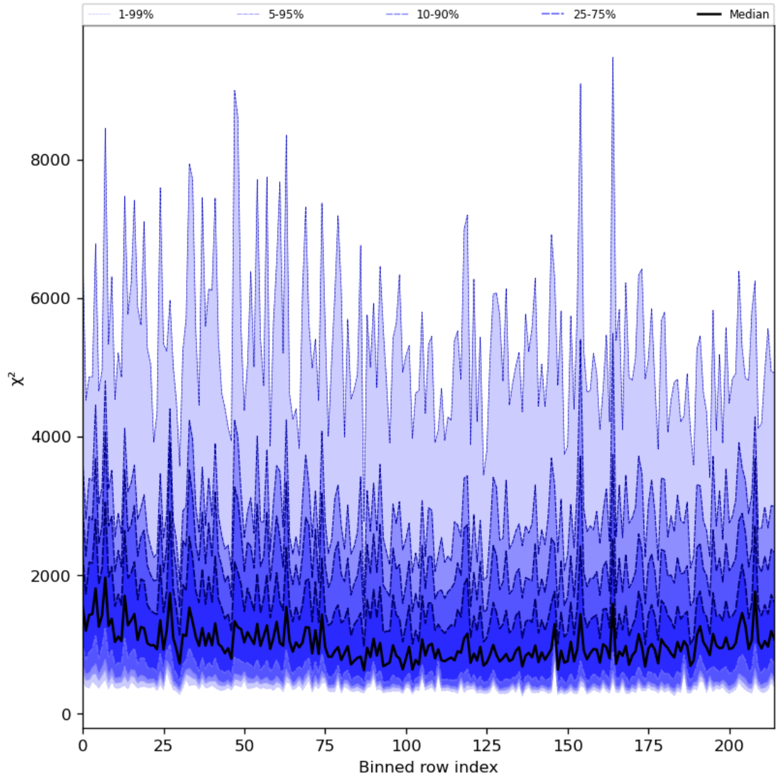
Figure 30: Along track statistics of “ \chi^2 ” for 2023-10-18 to 2023-10-20
