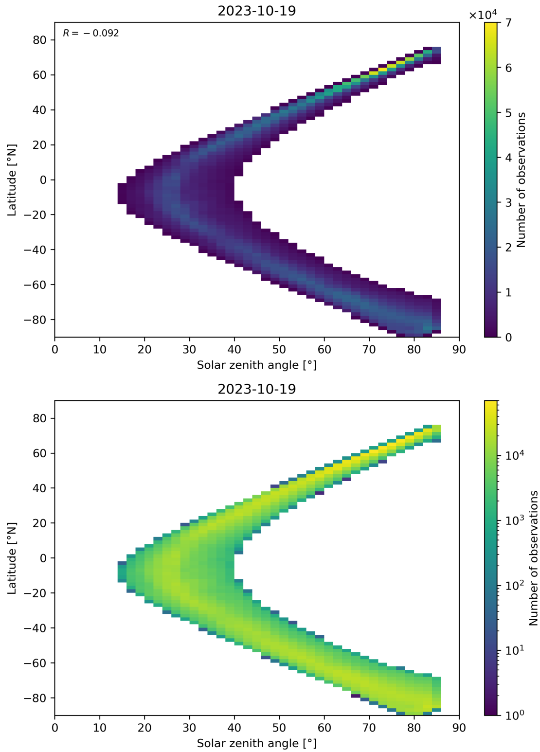
Figure 66: Scatter density plot of “Solar zenith angle” against “Latitude” for 2023-10-18 to 2023-10-20.
