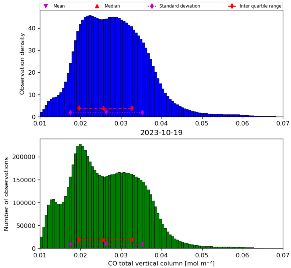
Figure 18: Histogram of “CO total vertical column” for 2023-10-18 to 2023-10-20
