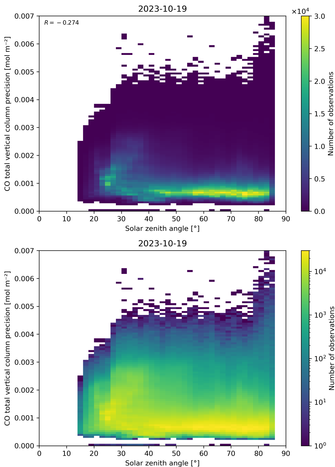
Figure 63: Scatter density plot of “Solar zenith angle” against “CO total vertical column precision” for 2023-10-18 to 2023-10-20.
