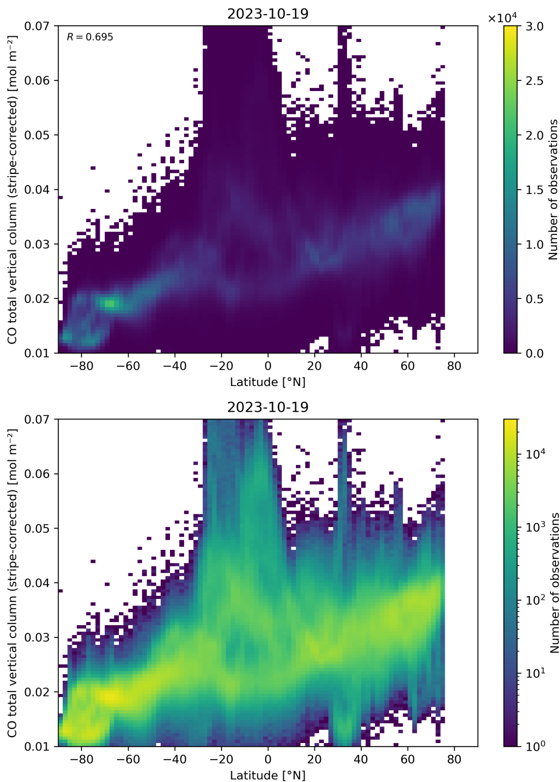
Figure 52: Scatter density plot of “Latitude” against “CO total vertical column (stripe-corrected)” for 2023-10-18 to 2023-10-20.
