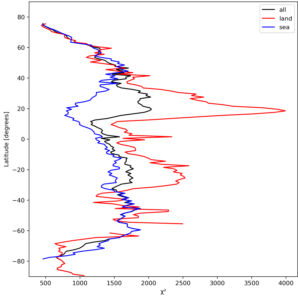
Figure 14: Zonal average of “ \chi^2 ” for 2023-10-18 to 2023-10-20.
