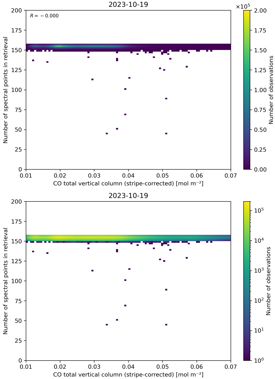
Figure 40: Scatter density plot of “CO total vertical column (stripe-corrected)” against “Number of spectral points in retrieval” for 2023-10-18 to 2023-10-20.
