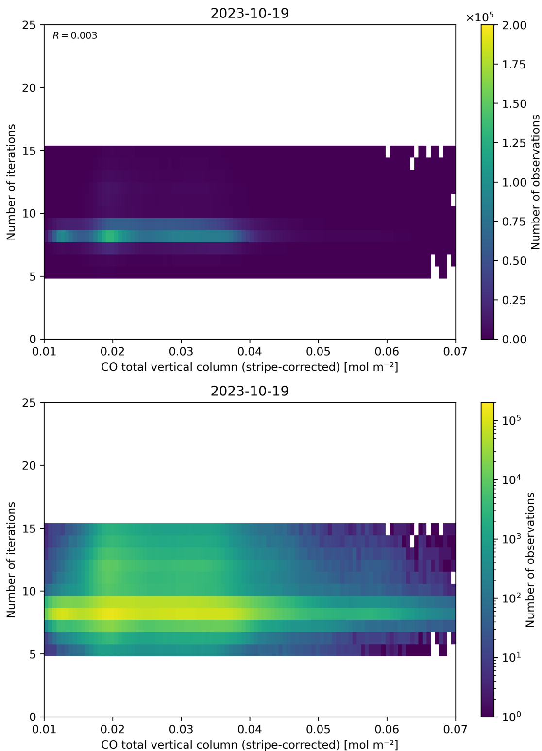
Figure 39: Scatter density plot of “CO total vertical column (stripe-corrected)” against “Number of iterations” for 2023-10-18 to 2023-10-20.
