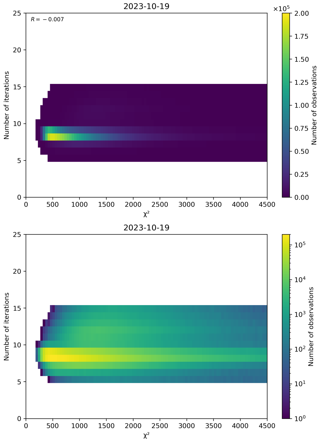
Figure 49: Scatter density plot of “ \chi^2 ” against “Number of iterations” for 2023-10-18 to 2023-10-20.
