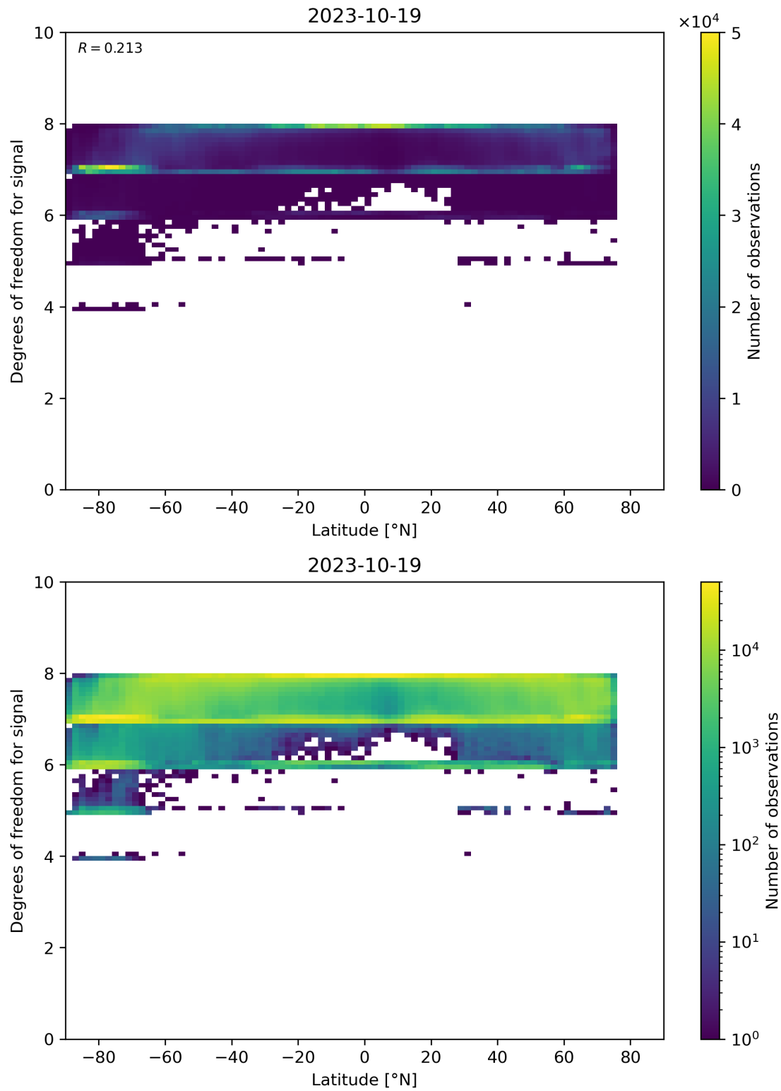
Figure 55: Scatter density plot of “Latitude” against “Degrees of freedom for signal” for 2023-10-18 to 2023-10-20.
