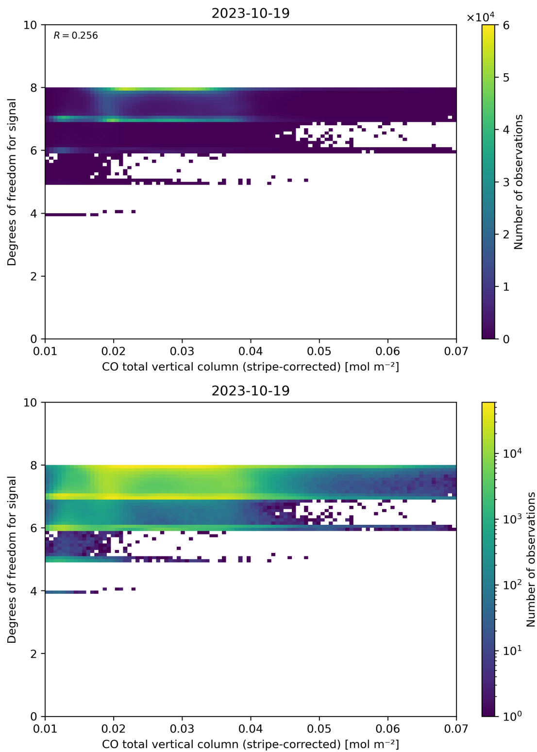
Figure 38: Scatter density plot of “CO total vertical column (stripe-corrected)” against “Degrees of freedom for signal” for 2023-10-18 to 2023-10-20.
