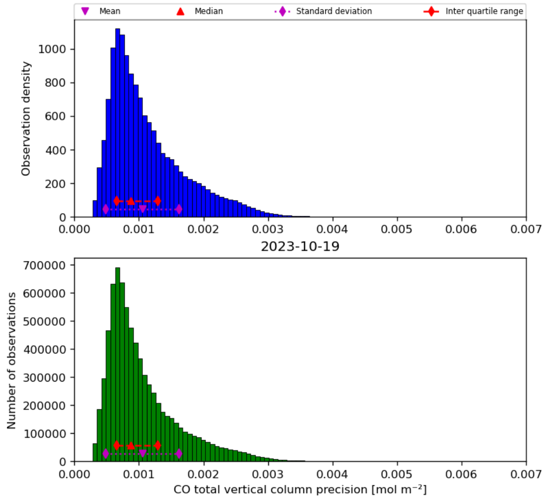
Figure 20: Histogram of “CO total vertical column precision” for 2023-10-18 to 2023-10-20
