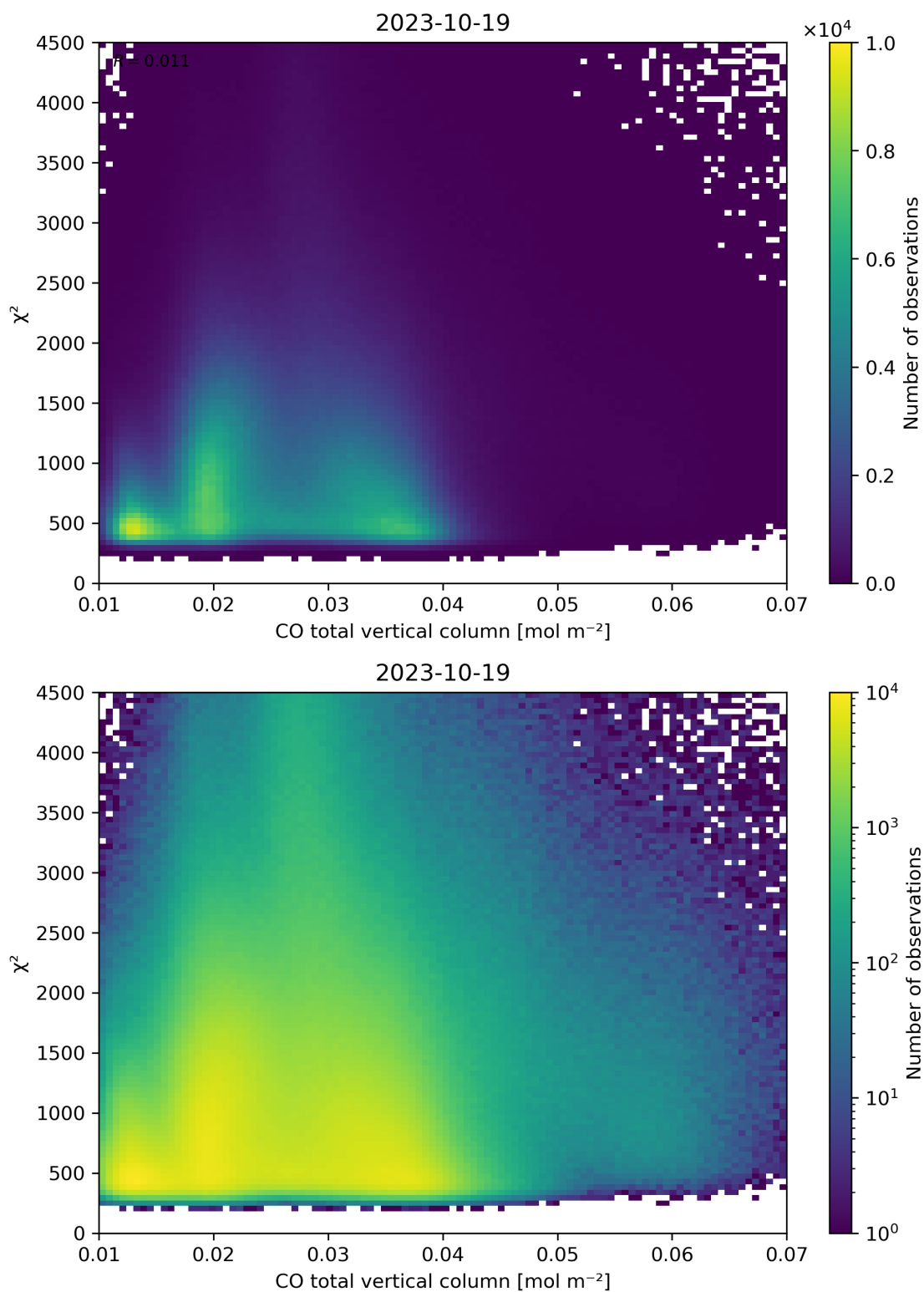
Figure 35: Scatter density plot of “CO total vertical column” against “ \chi^2 ” for 2023-10-18 to 2023-10-20.
