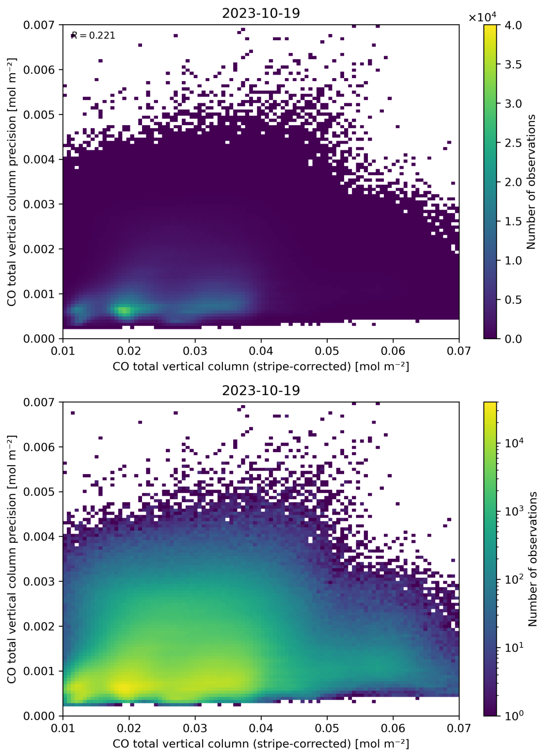
Figure 36: Scatter density plot of “CO total vertical column (stripe-corrected)” against “CO total vertical column precision” for 2023-10-18 to 2023-10-20.
