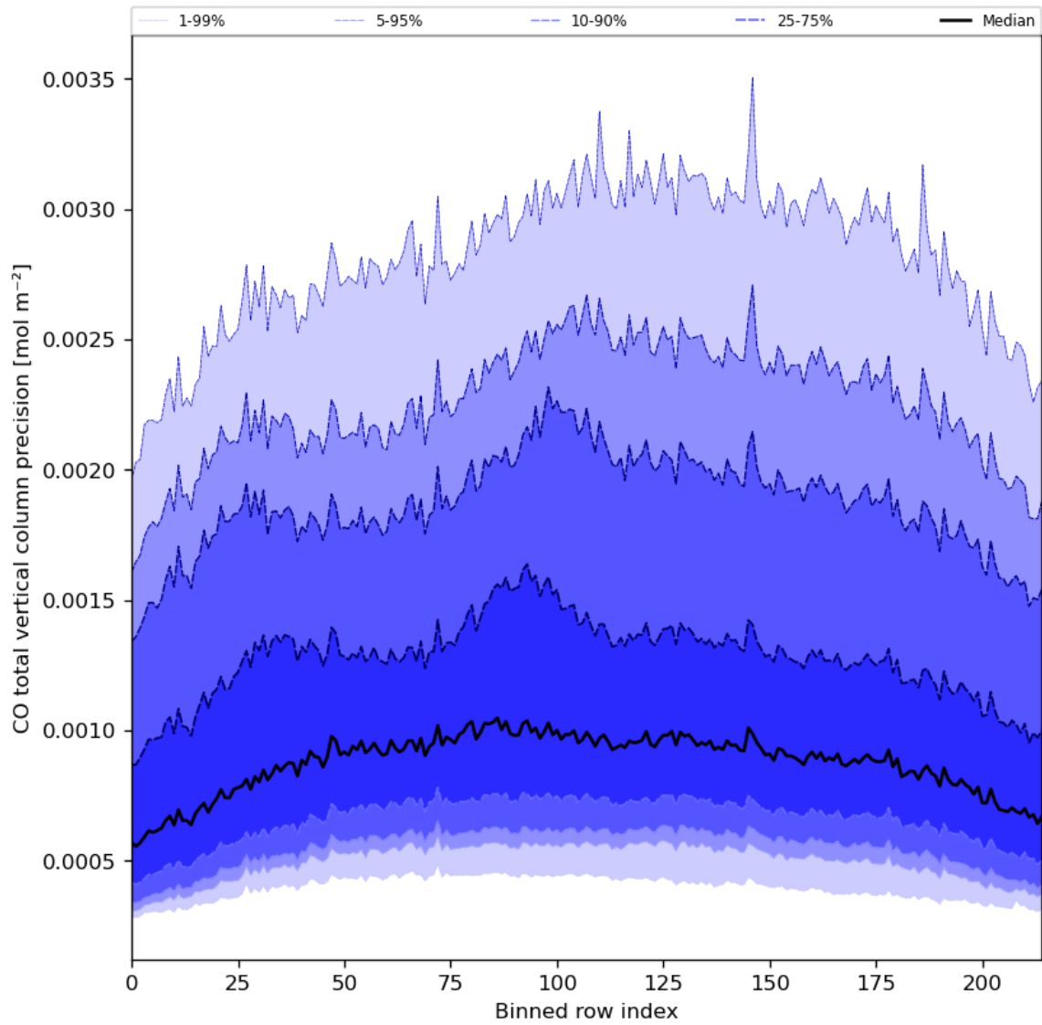
Figure 28: Along track statistics of “CO total vertical column precision” for 2023-10-18 to 2023-10-20
