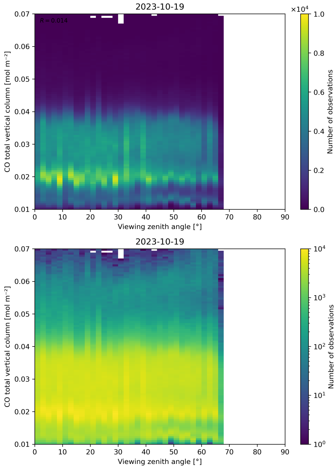
Figure 69: Scatter density plot of “Viewing zenith angle” against “CO total vertical column” for 2023-10-18 to 2023-10-20.
