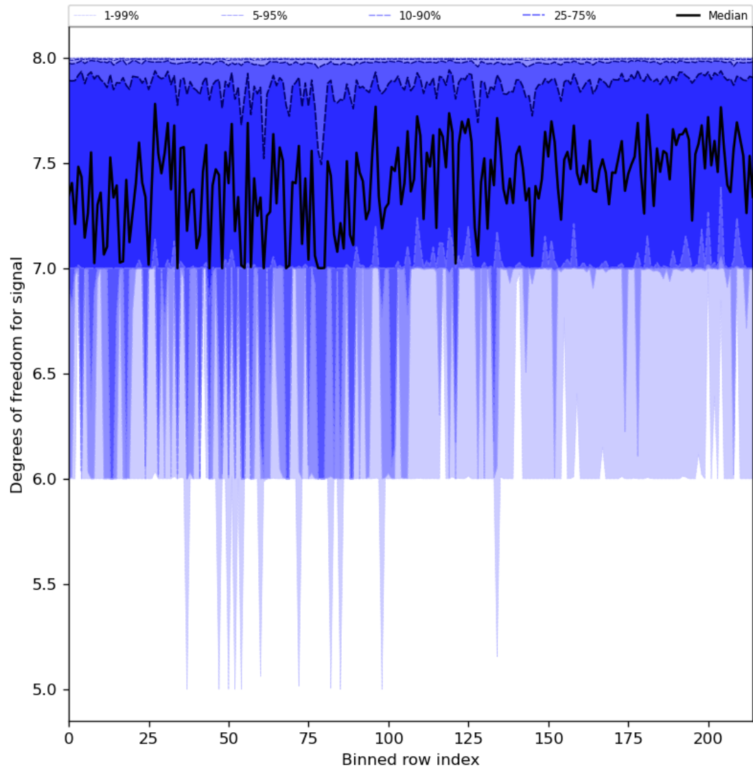
Figure 31: Along track statistics of “Degrees of freedom for signal” for 2023-10-18 to 2023-10-20
