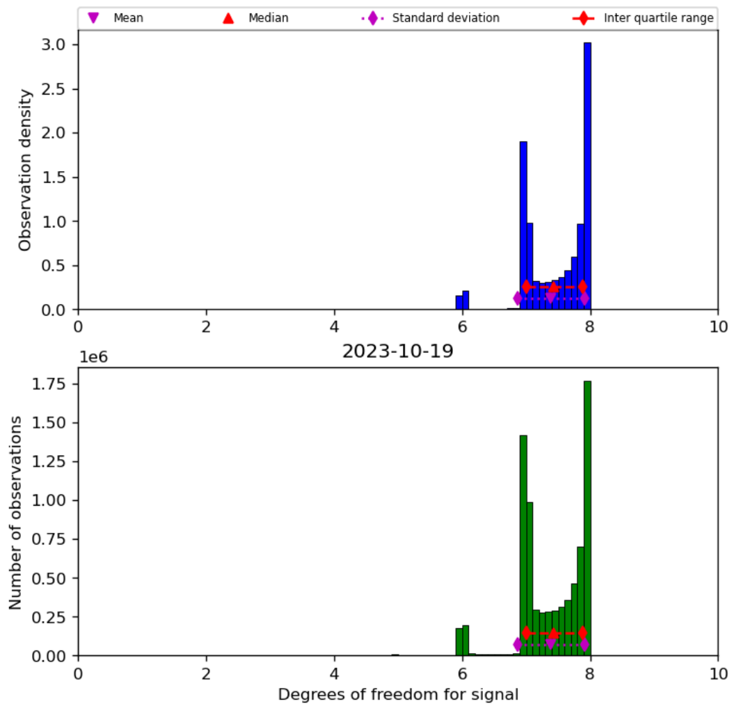
Figure 23: Histogram of “Degrees of freedom for signal” for 2023-10-18 to 2023-10-20
