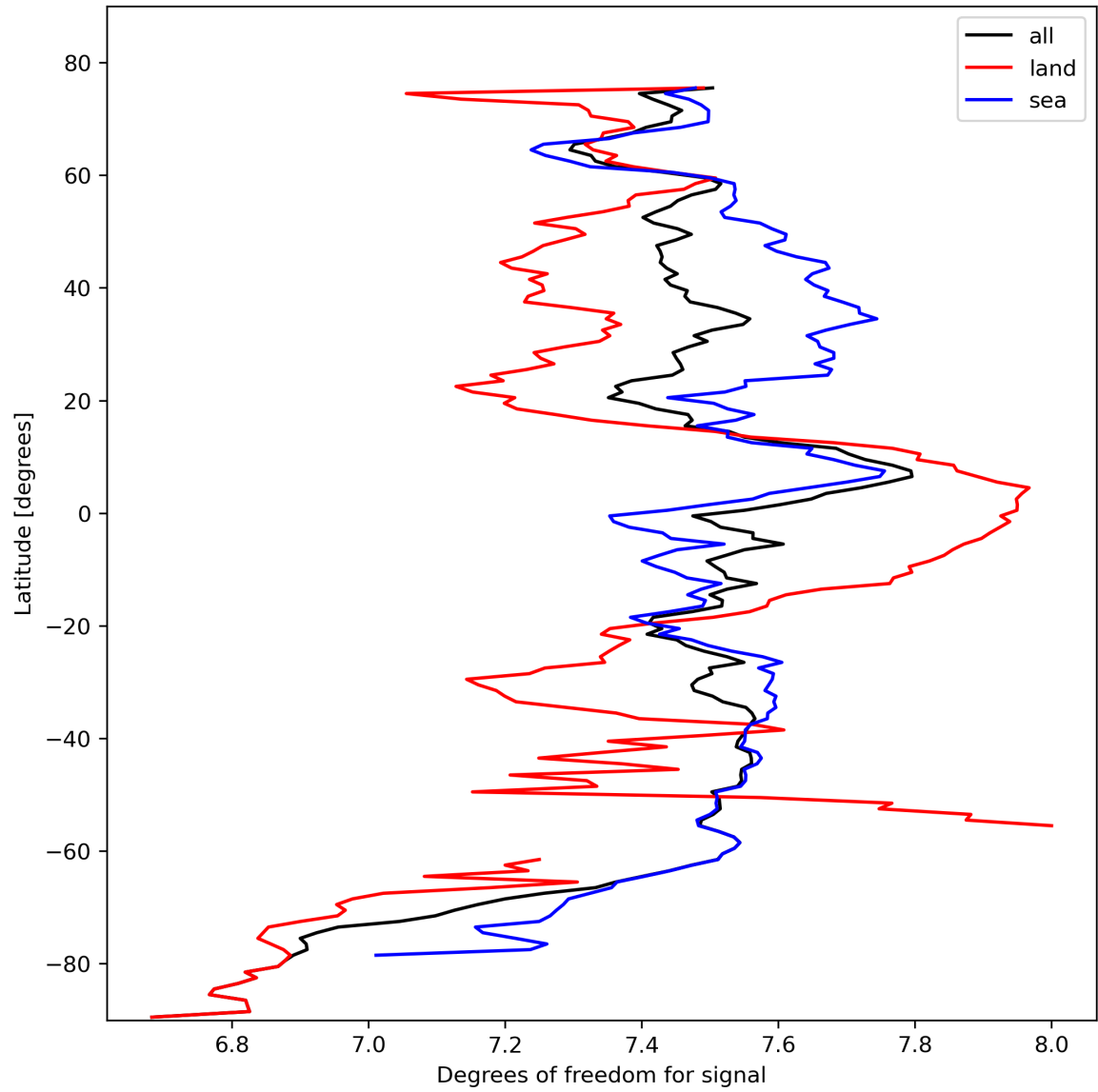
Figure 15: Zonal average of “Degrees of freedom for signal” for 2023-10-18 to 2023-10-20.
