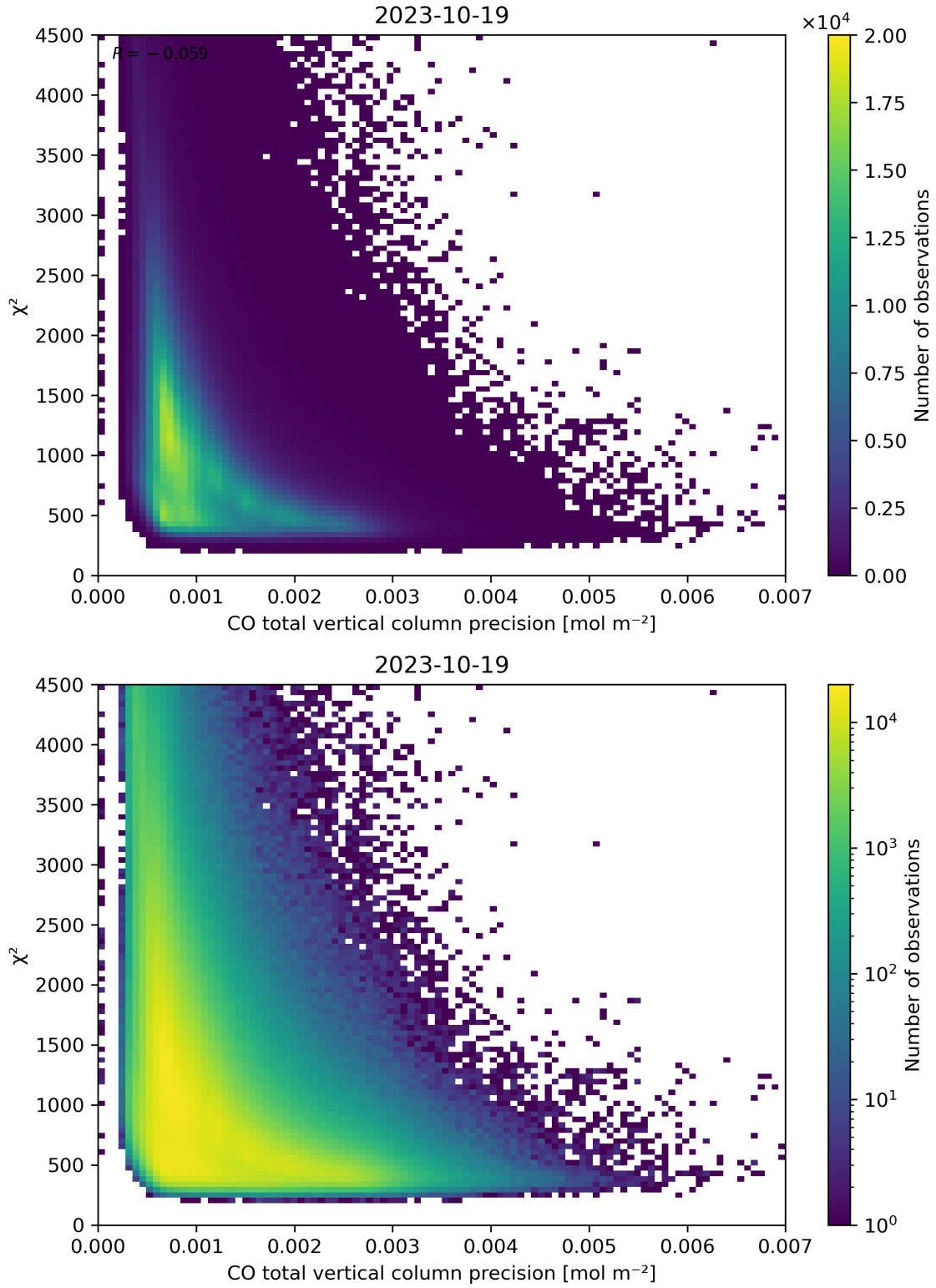
Figure 44: Scatter density plot of “CO total vertical column precision” against “ \chi^2 ” for 2023-10-18 to 2023-10-20.
