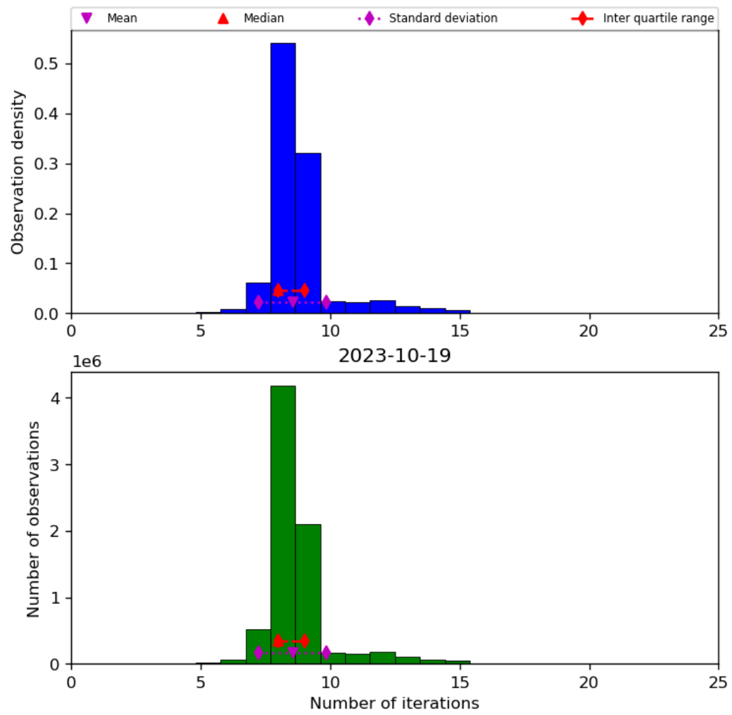
Figure 24: Histogram of “Number of iterations” for 2023-10-18 to 2023-10-20
