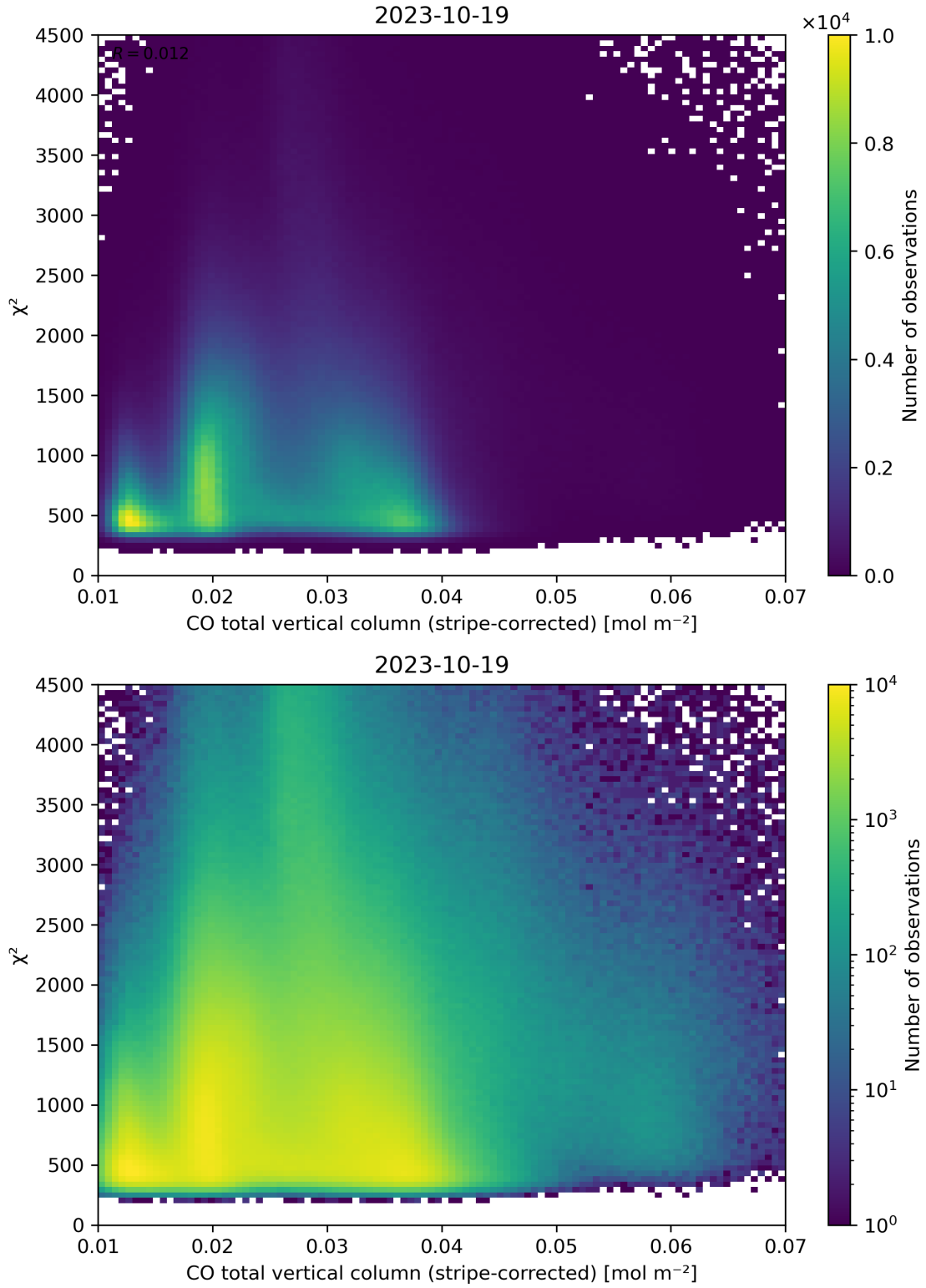
Figure 37: Scatter density plot of “CO total vertical column (stripe-corrected)” against “ \chi^2 ” for 2023-10-18 to 2023-10-20.
