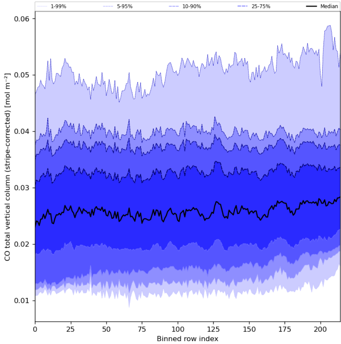
Figure 27: Along track statistics of “CO total vertical column (stripe-corrected)” for 2023-10-18 to 2023-10-20
