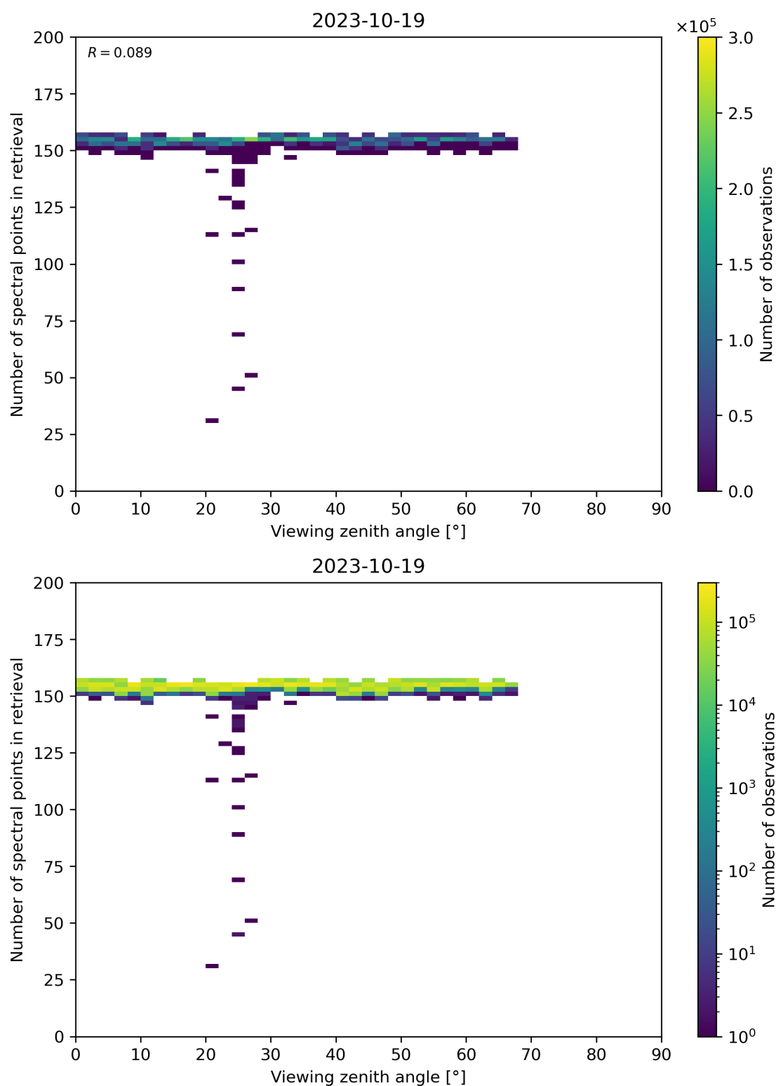
Figure 76: Scatter density plot of “Viewing zenith angle” against “Number of spectral points in retrieval” for 2023-10-18 to 2023-10-20.
