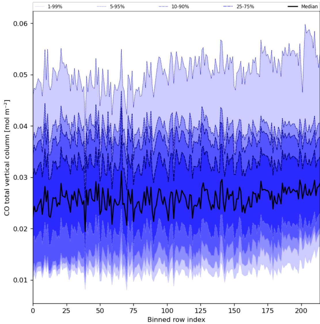
Figure 26: Along track statistics of “CO total vertical column” for 2023-10-18 to 2023-10-20
