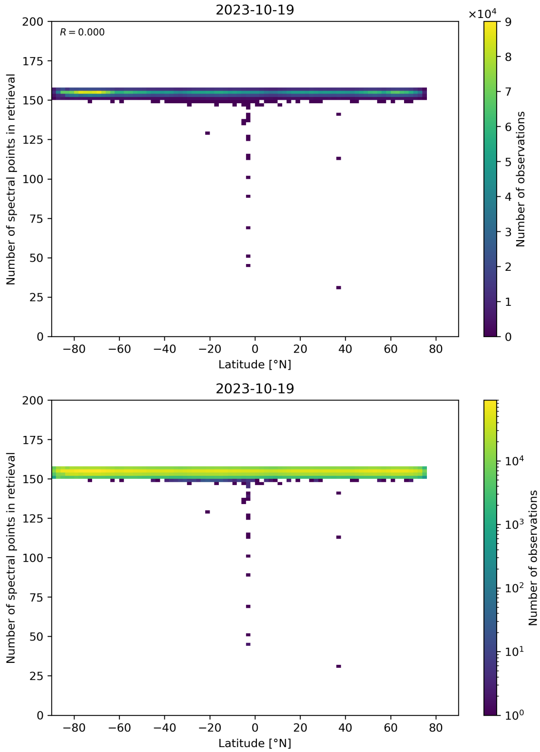
Figure 57: Scatter density plot of “Latitude” against “Number of spectral points in retrieval” for 2023-10-18 to 2023-10-20.
