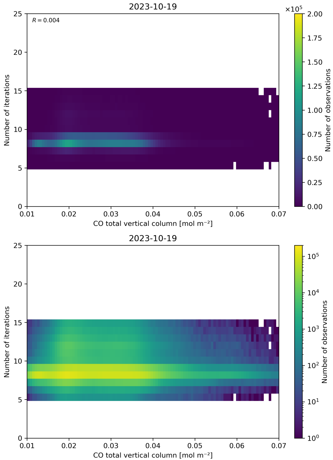
Figure 42: Scatter density plot of “CO total vertical column” against “Number of iterations” for 2023-10-18 to 2023-10-20.
