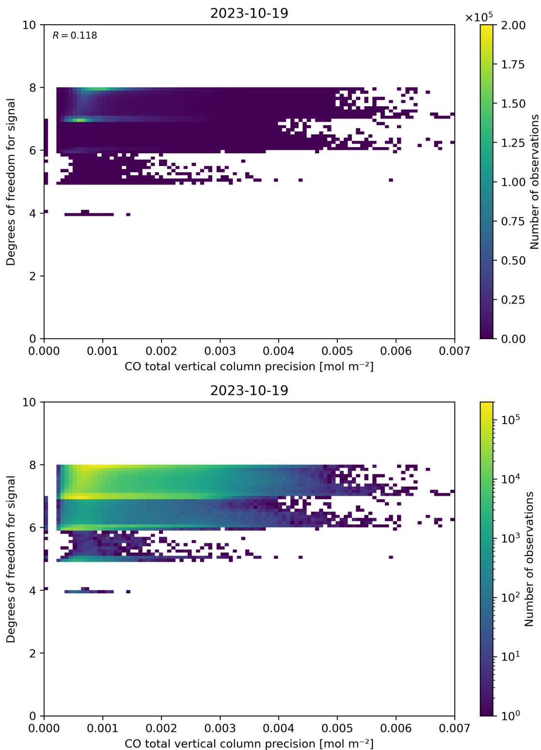
Figure 45: Scatter density plot of “CO total vertical column precision” against “Degrees of freedom for signal” for 2023-10-18 to 2023-10-20.
