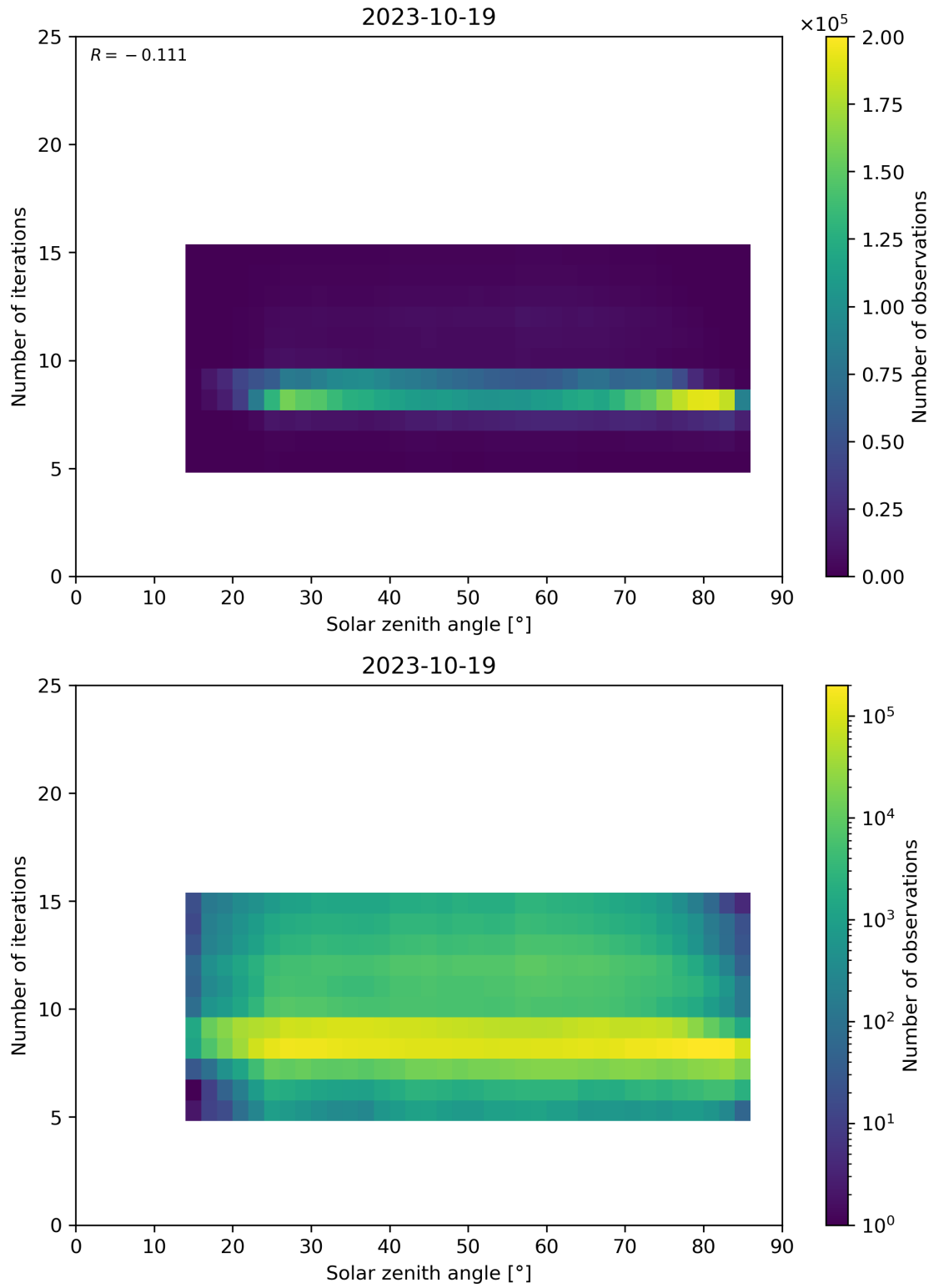
Figure 67: Scatter density plot of “Solar zenith angle” against “Number of iterations” for 2023-10-18 to 2023-10-20.
