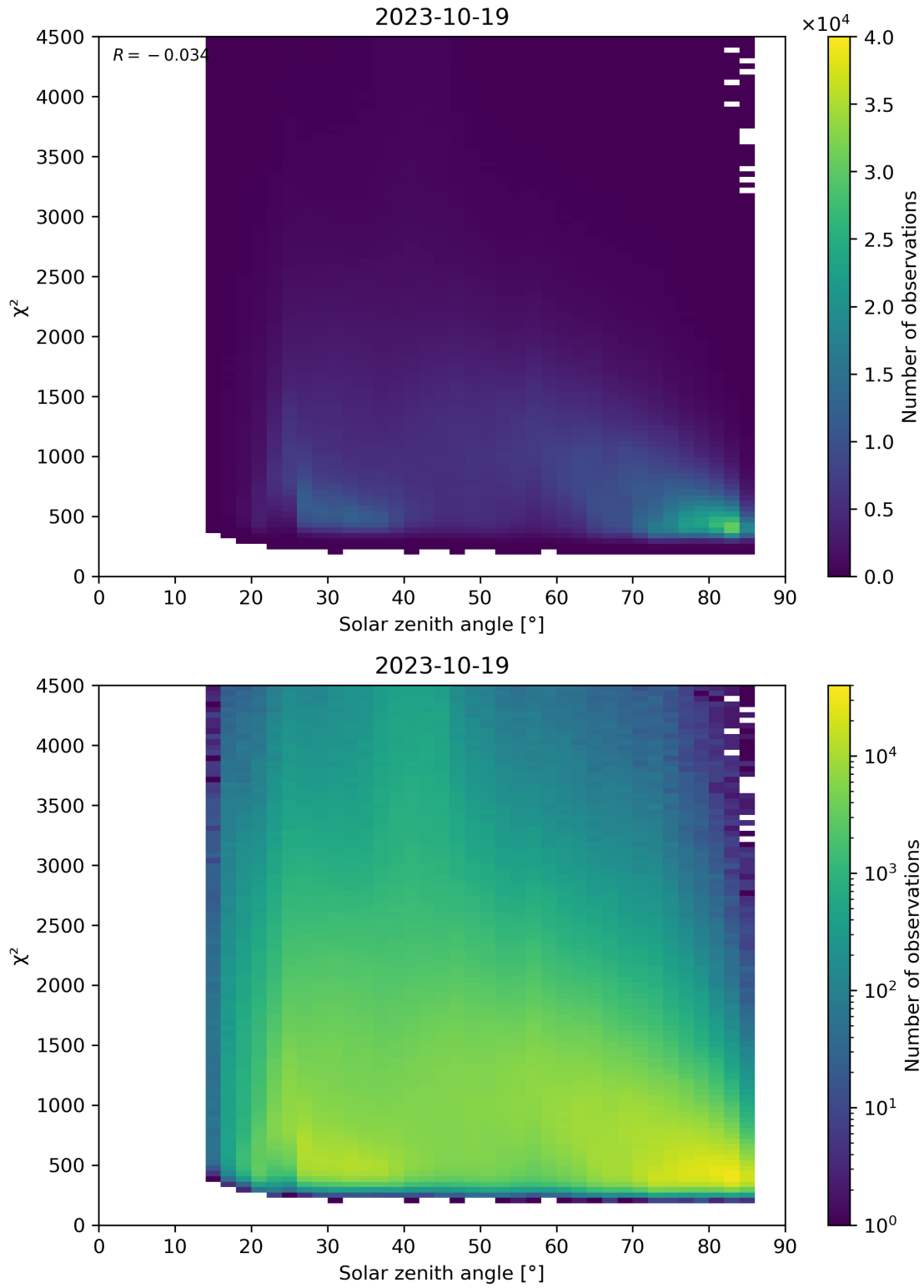
Figure 64: Scatter density plot of “Solar zenith angle” against “ \chi^2 ” for 2023-10-18 to 2023-10-20.
