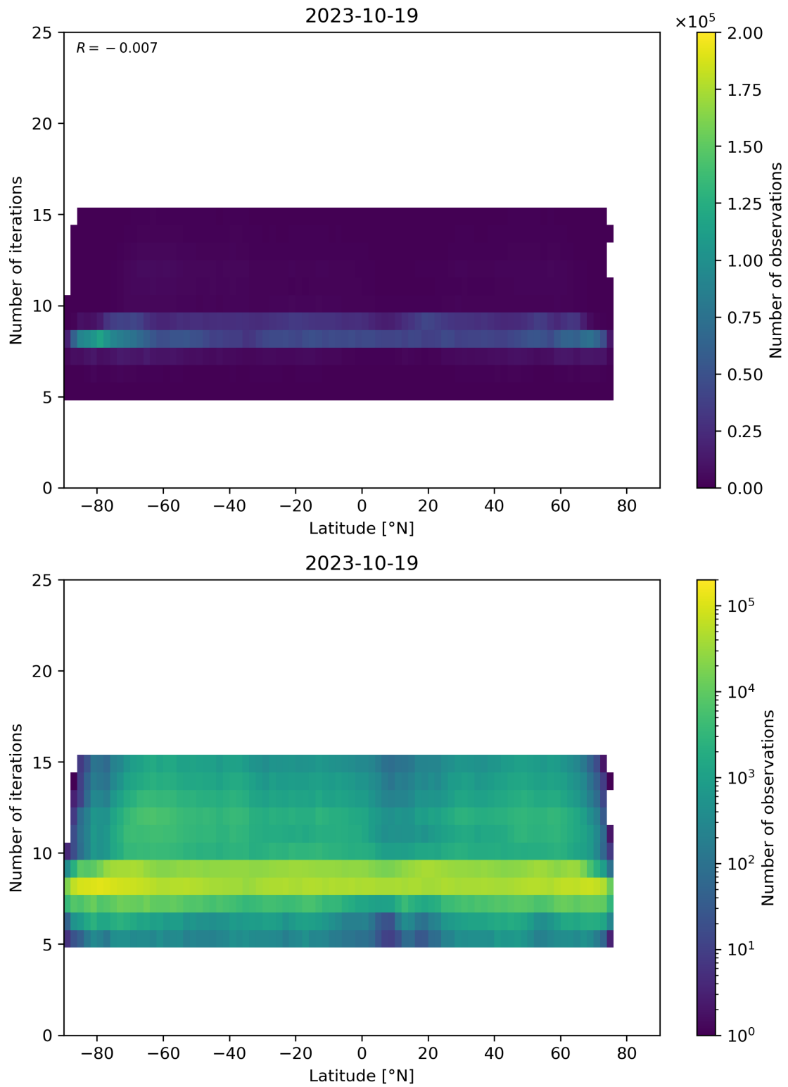
Figure 56: Scatter density plot of “Latitude” against “Number of iterations” for 2023-10-18 to 2023-10-20.
