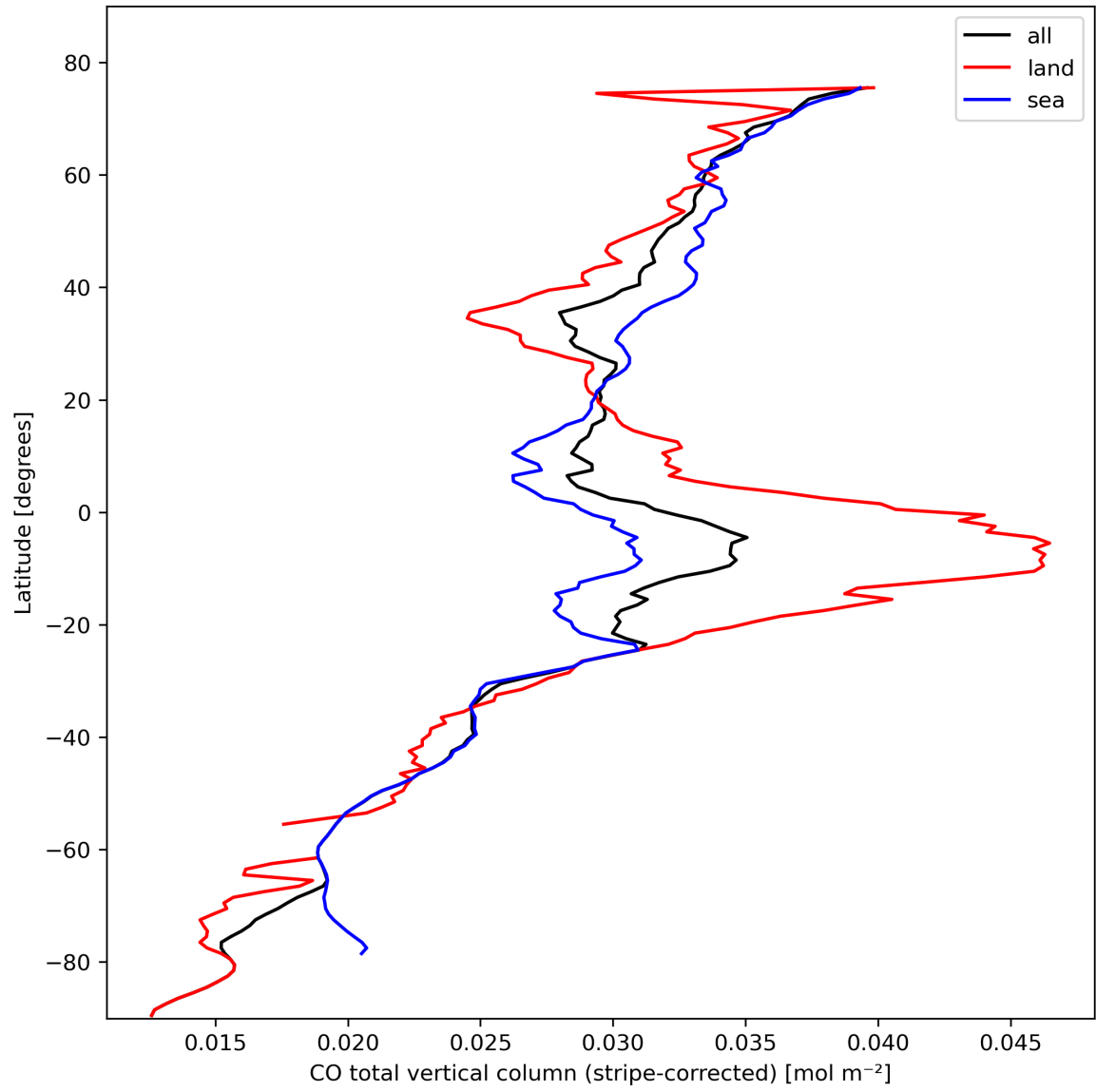
Figure 11: Zonal average of “CO total vertical column (stripe-corrected)” for 2023-10-18 to 2023-10-20.
