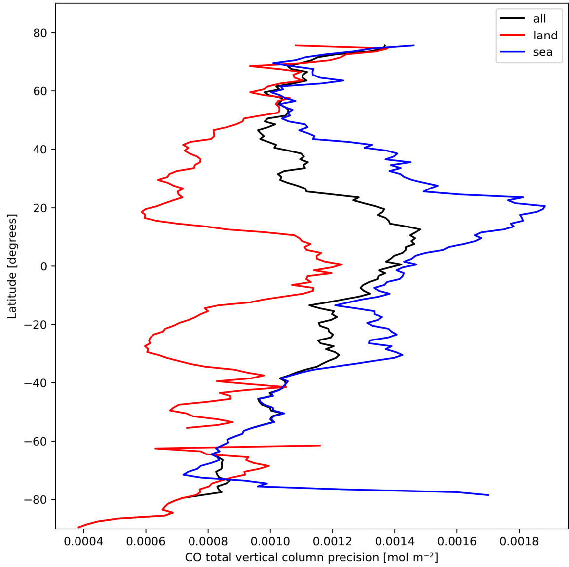
Figure 12: Zonal average of “CO total vertical column precision” for 2023-10-18 to 2023-10-20.
