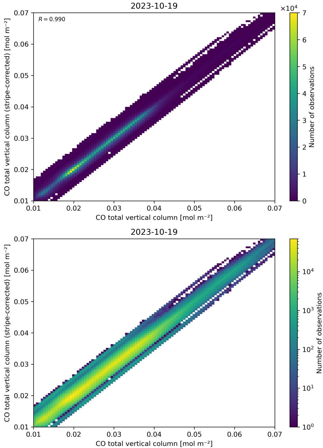
Figure 33: Scatter density plot of “CO total vertical column” against “CO total vertical column (stripe-corrected)” for 2023-10-18 to 2023-10-20.
