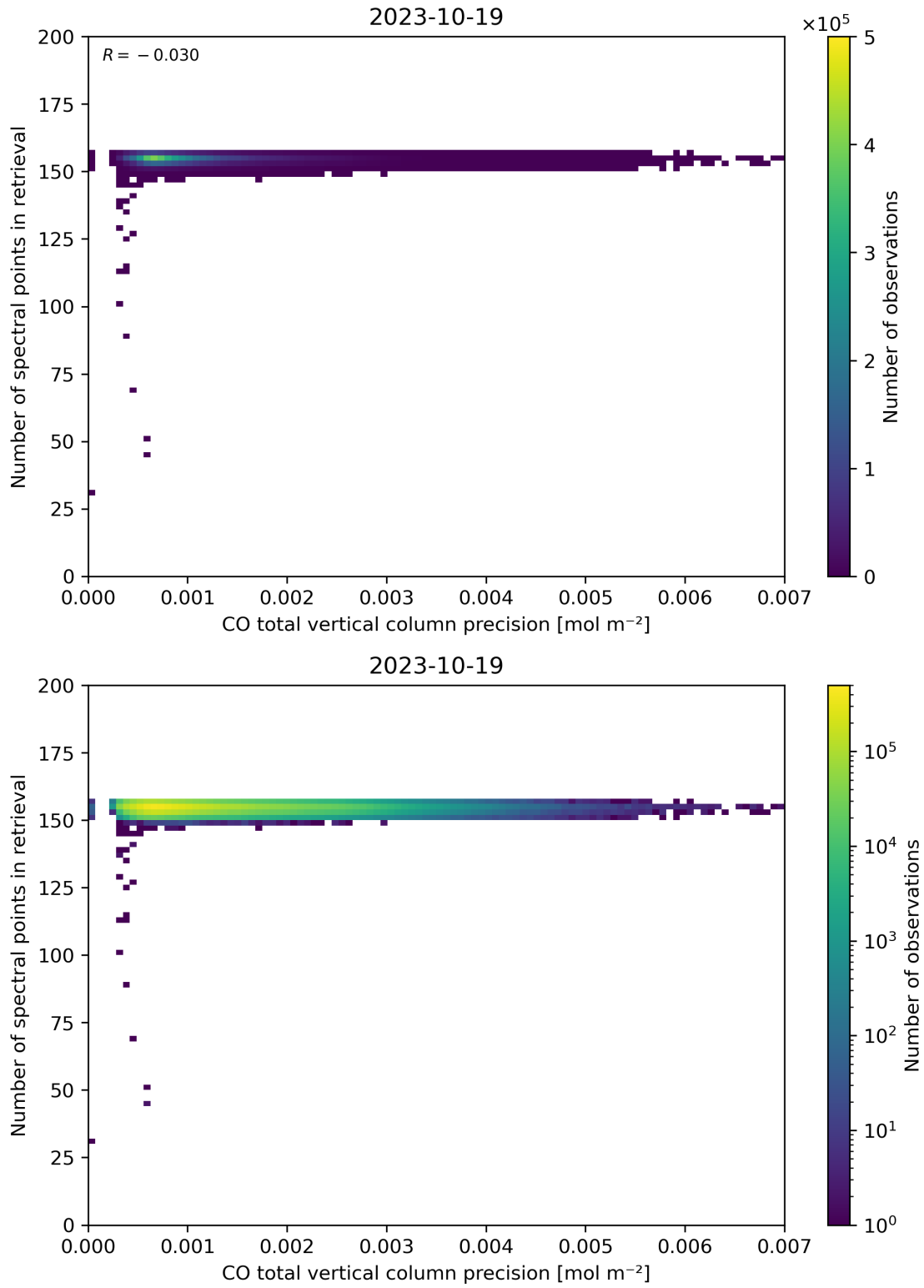
Figure 47: Scatter density plot of “CO total vertical column precision” against “Number of spectral points in retrieval” for 2023-10-18 to 2023-10-20.
