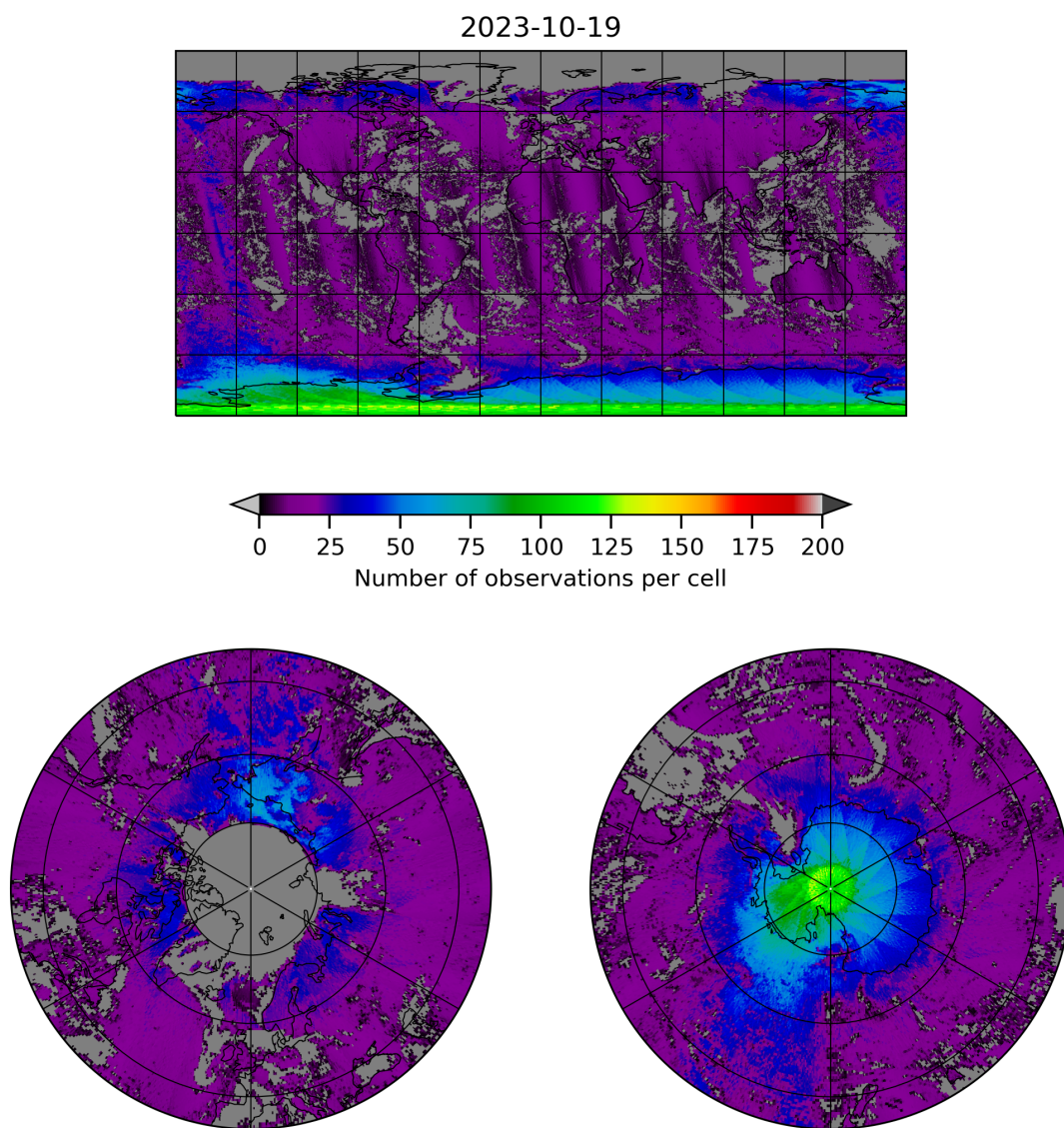
Figure 8: Map of the number of observations for 2023-10-18 to 2023-10-20
