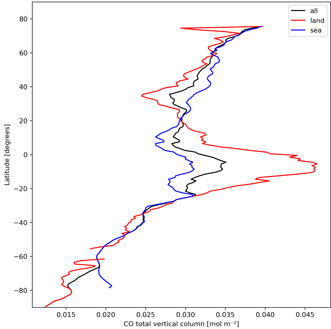
Figure 10: Zonal average of “CO total vertical column” for 2023-10-18 to 2023-10-20.
