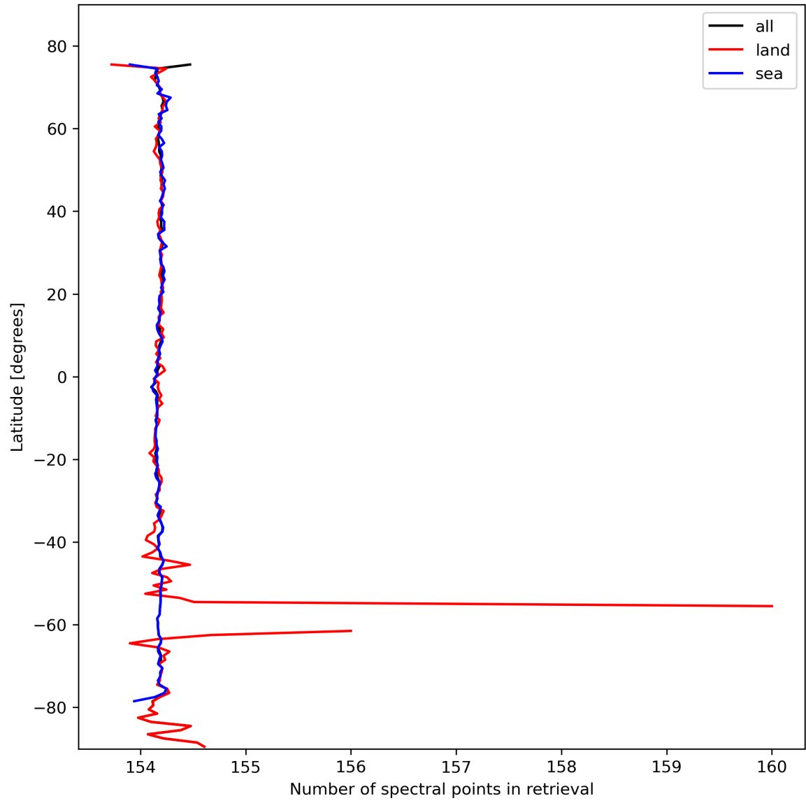
Figure 13: Zonal average of “Number of spectral points in retrieval” for 2023-10-18 to 2023-10-20.
