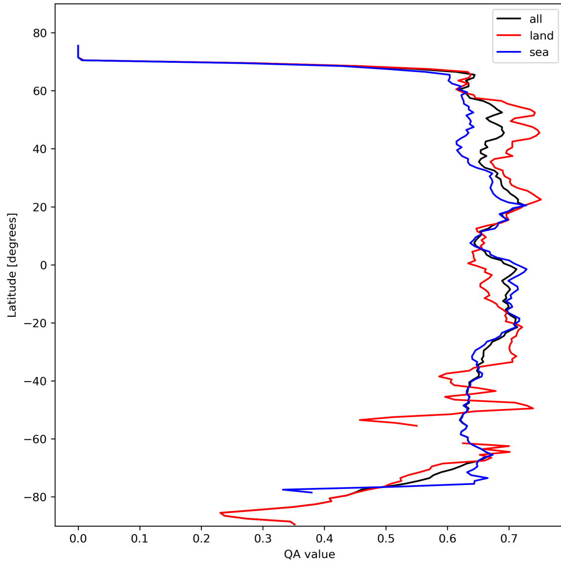
Figure 9: Zonal average of “QA value” for 2023-10-18 to 2023-10-20.
