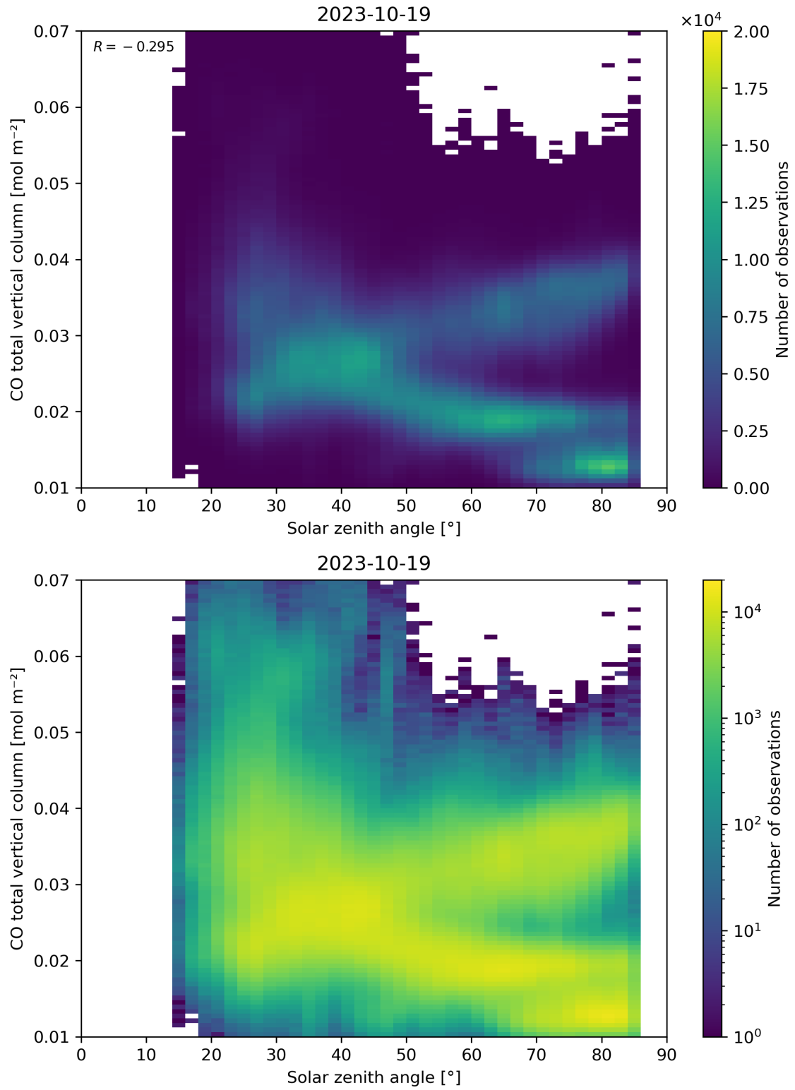
Figure 61: Scatter density plot of “Solar zenith angle” against “CO total vertical column” for 2023-10-18 to 2023-10-20.
