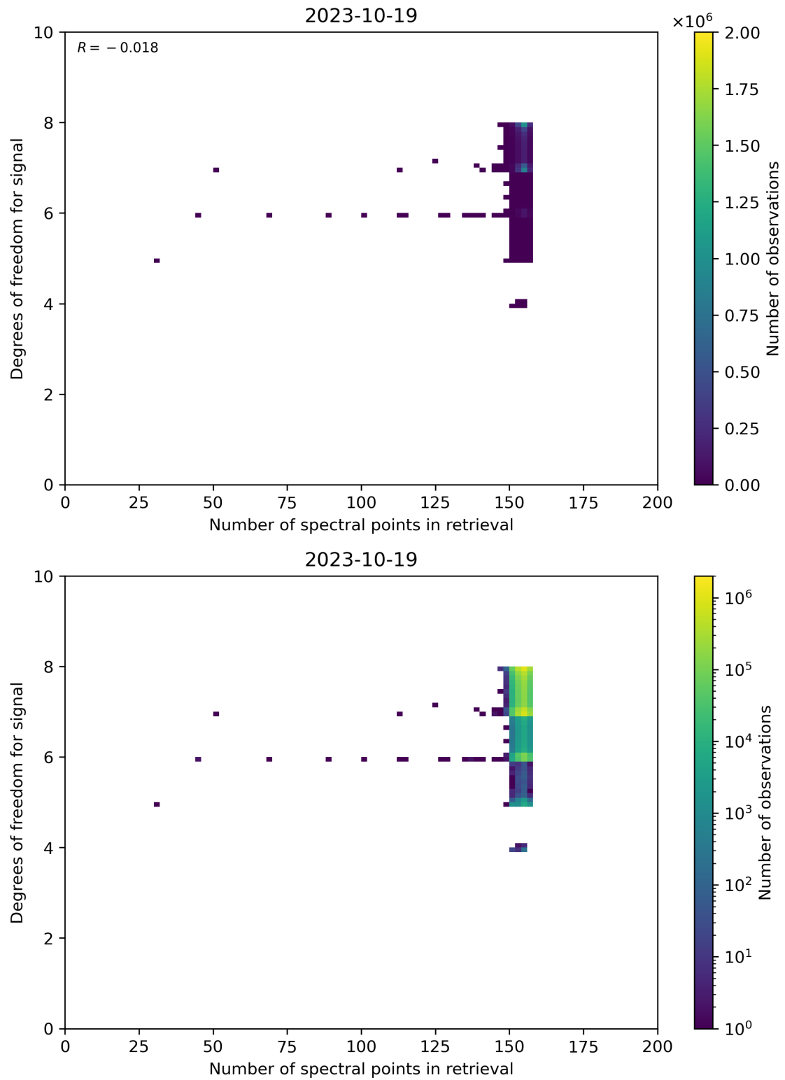
Figure 59: Scatter density plot of “Number of spectral points in retrieval” against “Degrees of freedom for signal” for 2023-10-18 to 2023-10-20.
