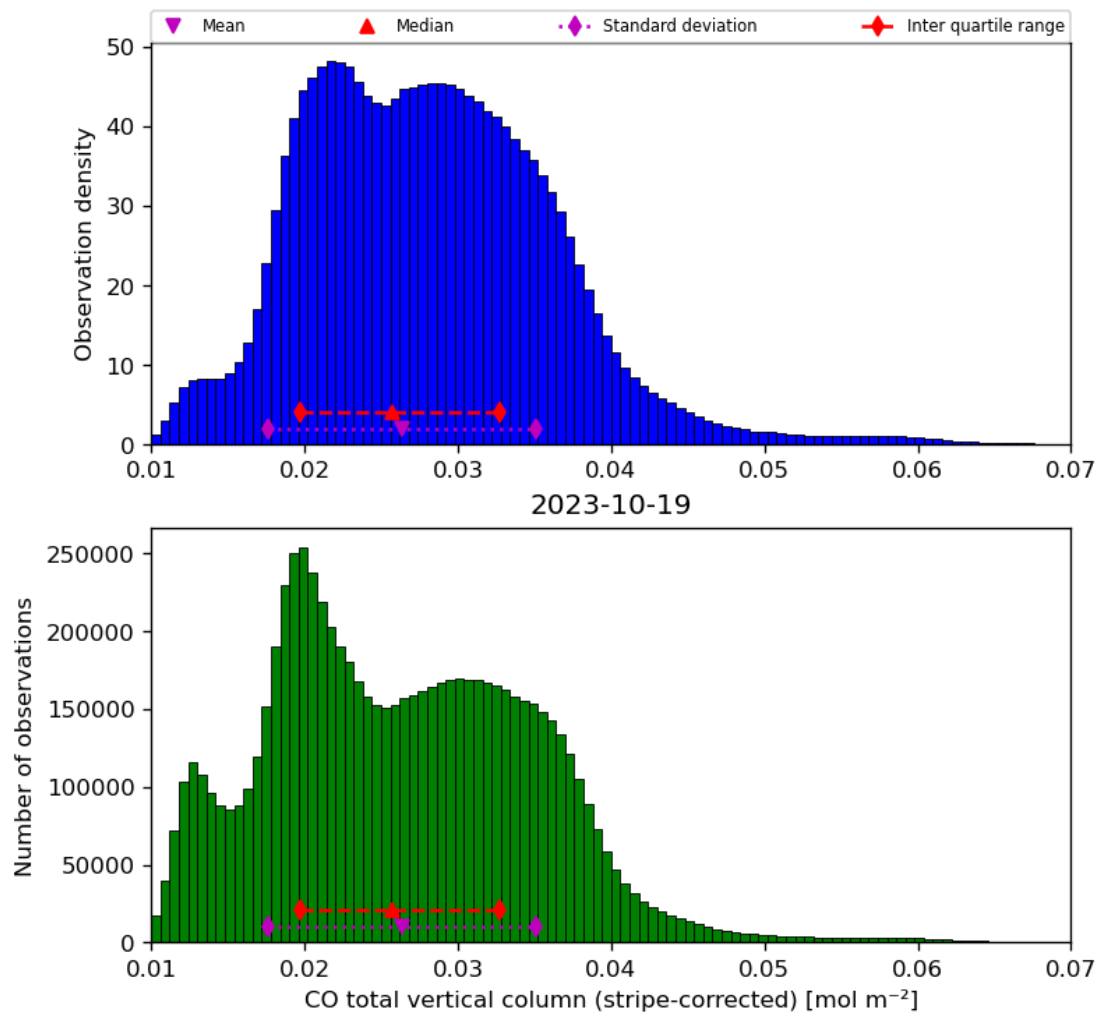
Figure 19: Histogram of “CO total vertical column (stripe-corrected)” for 2023-10-18 to 2023-10-20
