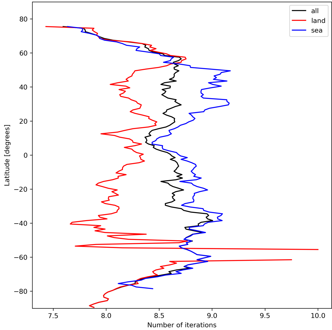
Figure 16: Zonal average of “Number of iterations” for 2023-10-18 to 2023-10-20.
