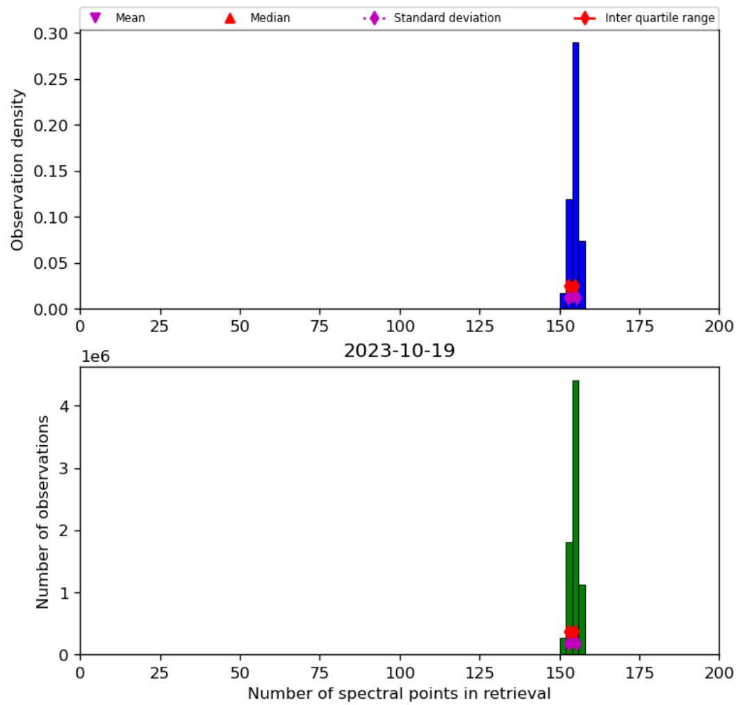
Figure 21: Histogram of “Number of spectral points in retrieval” for 2023-10-18 to 2023-10-20
