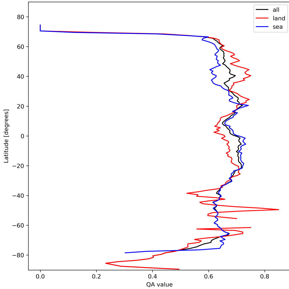
Figure 9: Zonal average of “QA value” for 2023-10-19 to 2023-10-21.
