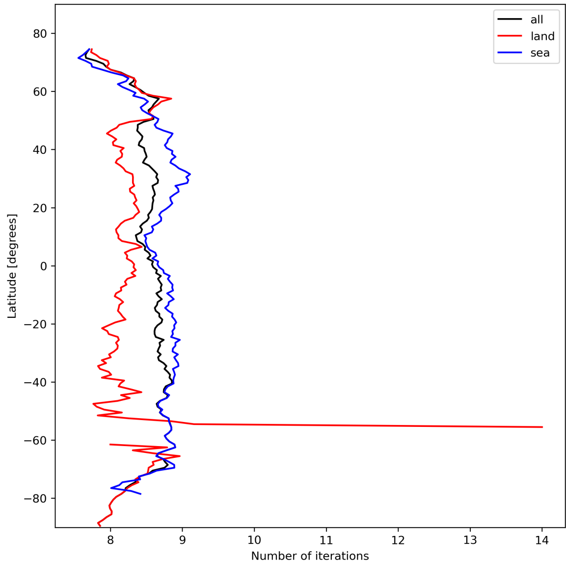
Figure 16: Zonal average of “Number of iterations” for 2023-10-19 to 2023-10-21.
