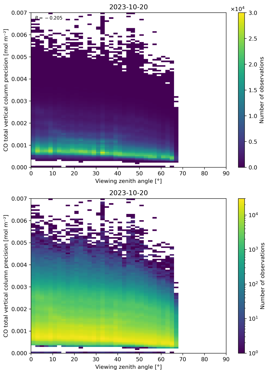
Figure 71: Scatter density plot of “Viewing zenith angle” against “CO total vertical column precision” for 2023-10-19 to 2023-10-21.
