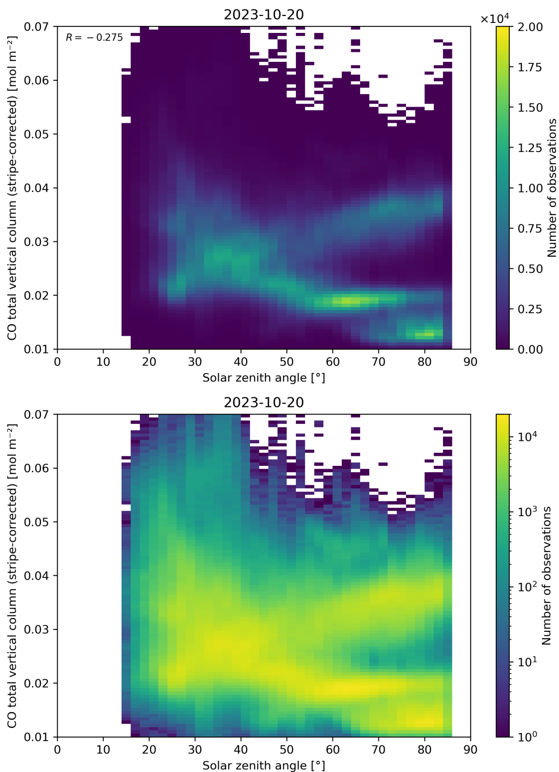
Figure 62: Scatter density plot of “Solar zenith angle” against “CO total vertical column (stripe-corrected)” for 2023-10-19 to 2023-10-21.
