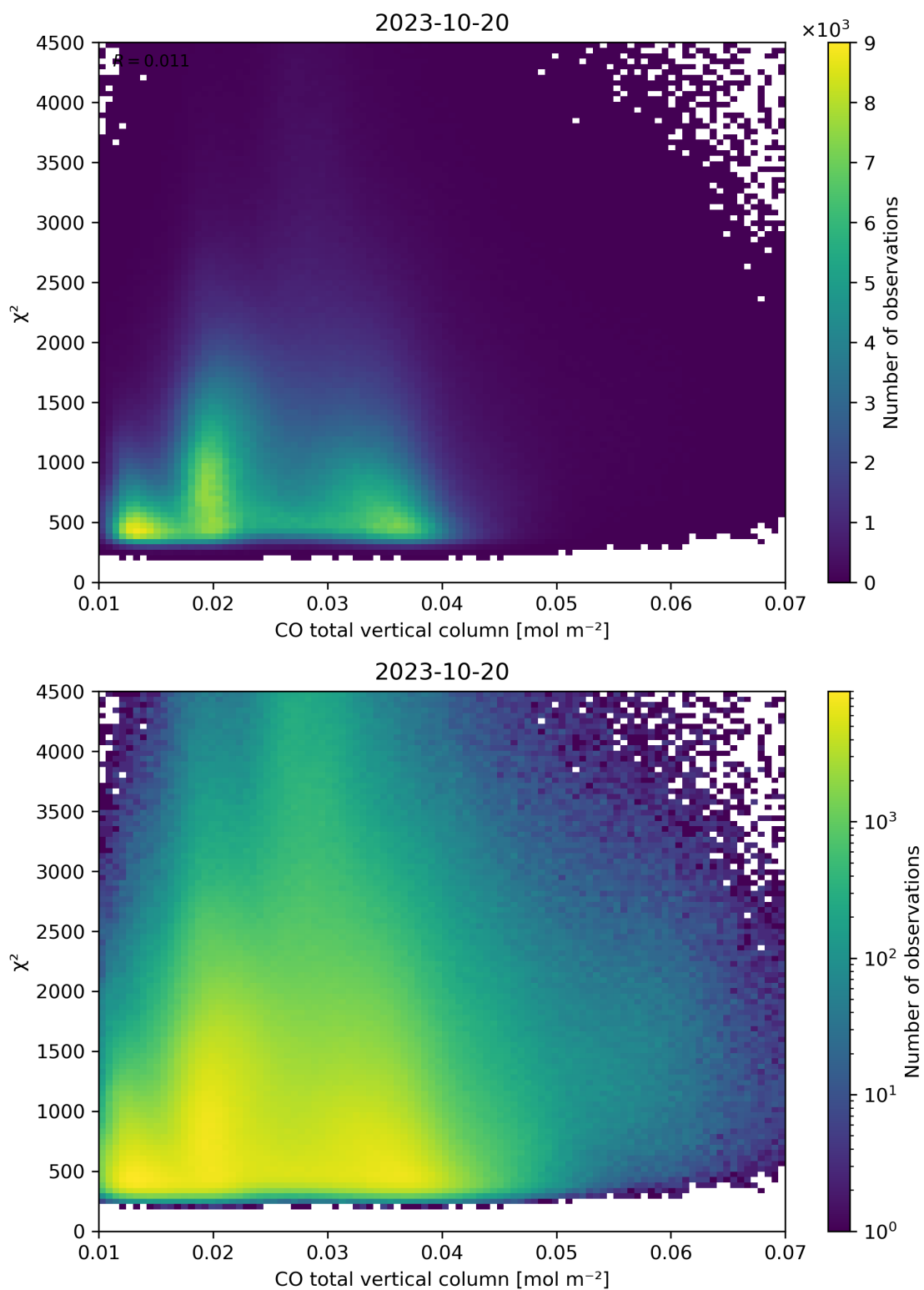
Figure 35: Scatter density plot of “CO total vertical column” against “ \chi^2 ” for 2023-10-19 to 2023-10-21.
