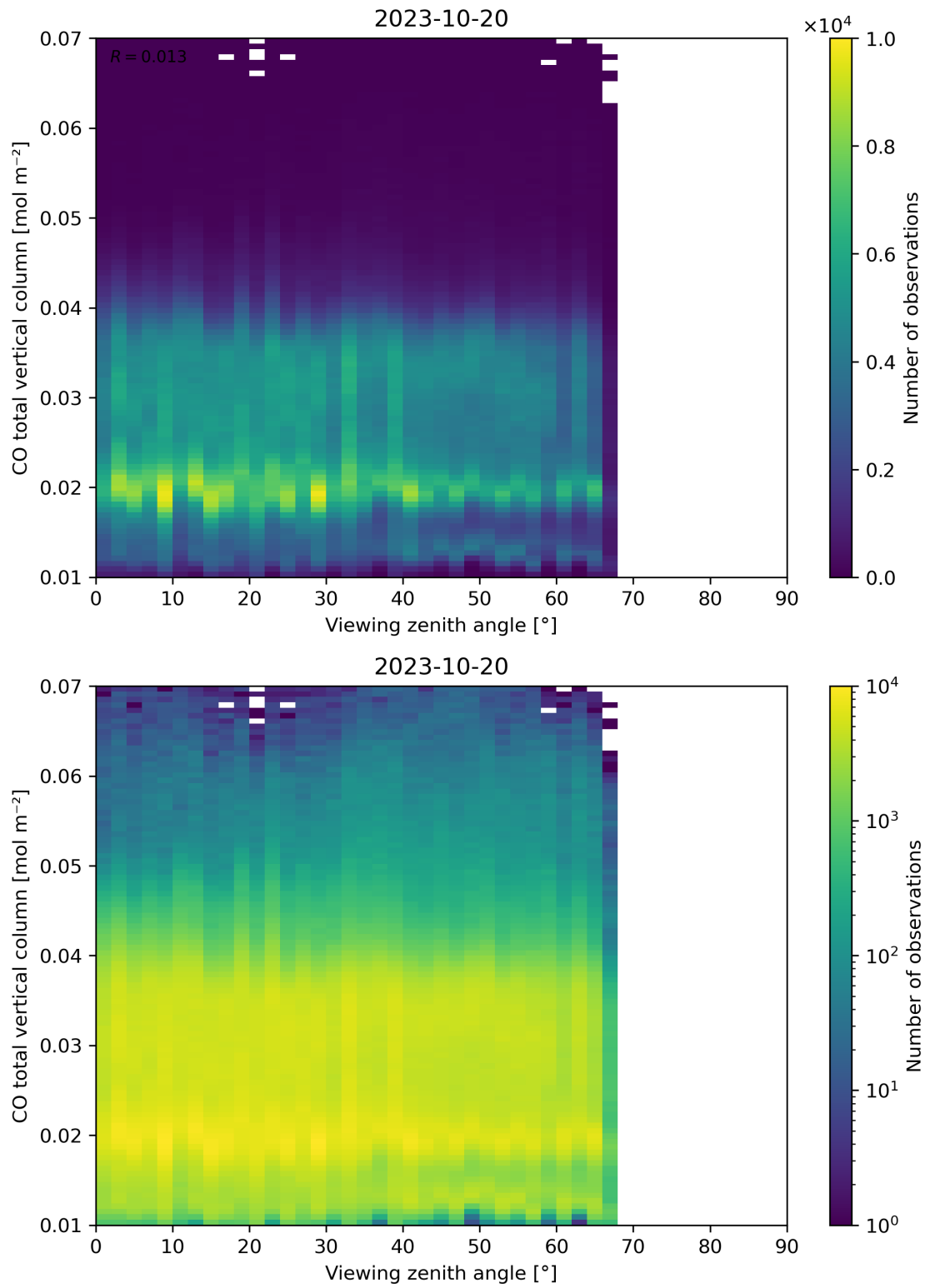
Figure 69: Scatter density plot of “Viewing zenith angle” against “CO total vertical column” for 2023-10-19 to 2023-10-21.
