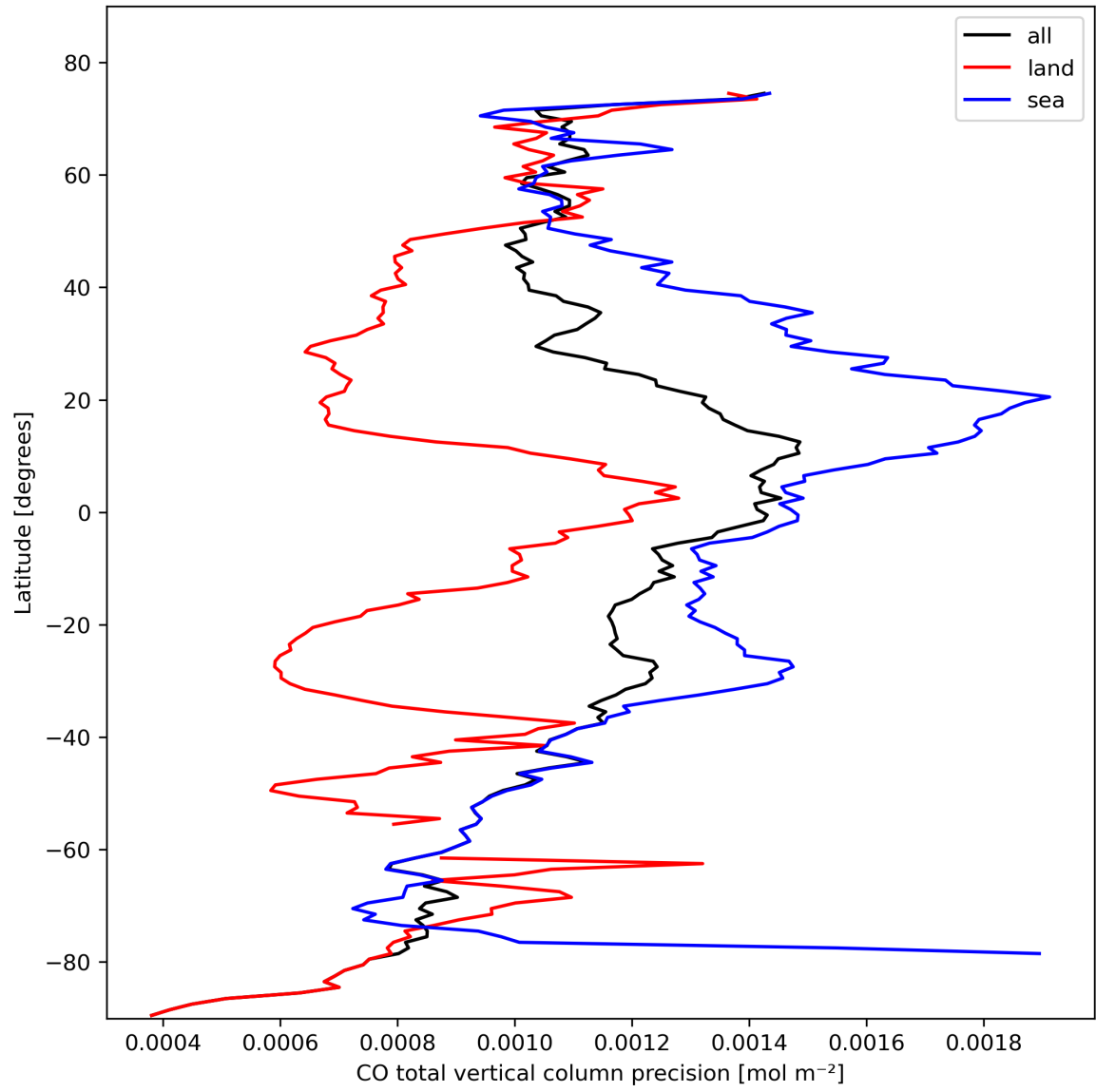
Figure 12: Zonal average of “CO total vertical column precision” for 2023-10-19 to 2023-10-21.
