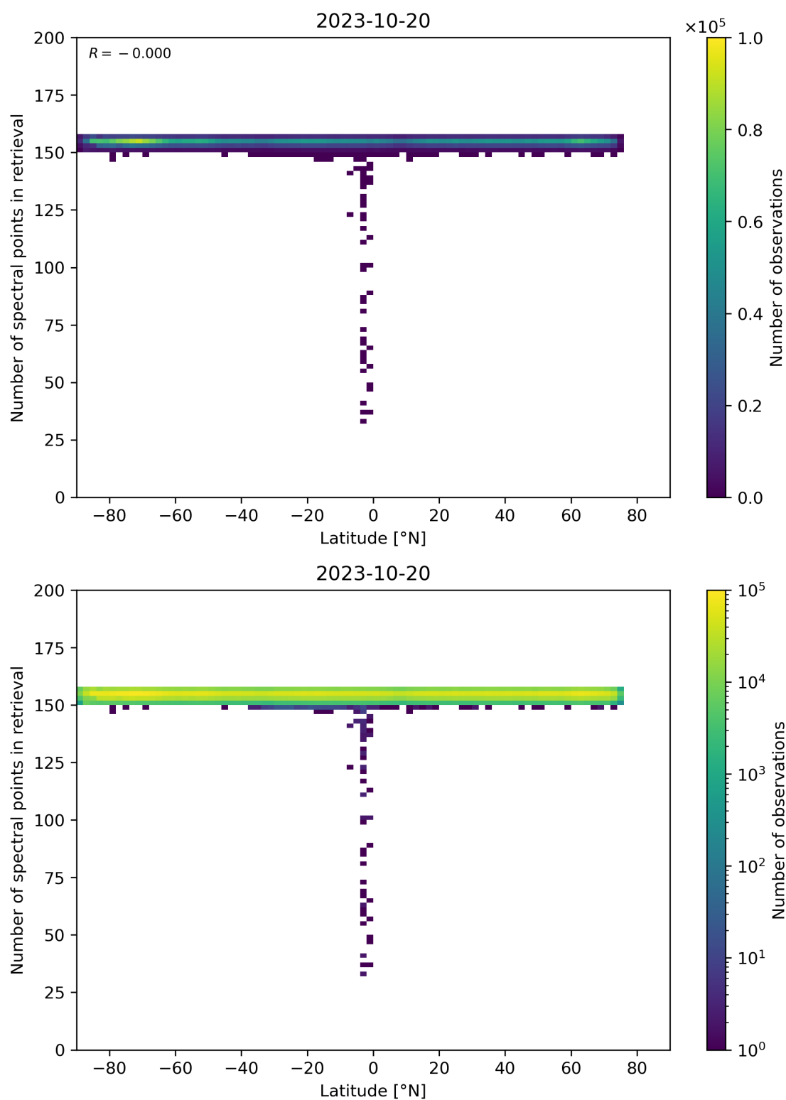
Figure 57: Scatter density plot of “Latitude” against “Number of spectral points in retrieval” for 2023-10-19 to 2023-10-21.
