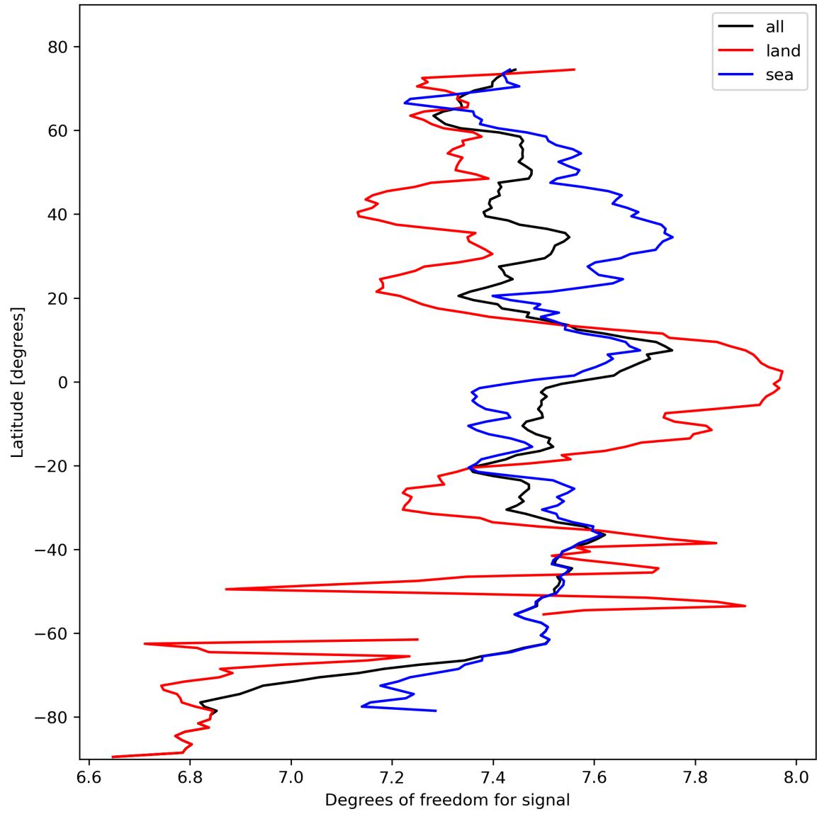
Figure 15: Zonal average of “Degrees of freedom for signal” for 2023-10-19 to 2023-10-21.
