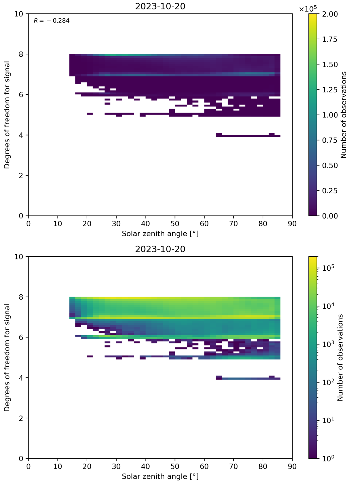
Figure 65: Scatter density plot of “Solar zenith angle” against “Degrees of freedom for signal” for 2023-10-19 to 2023-10-21.
