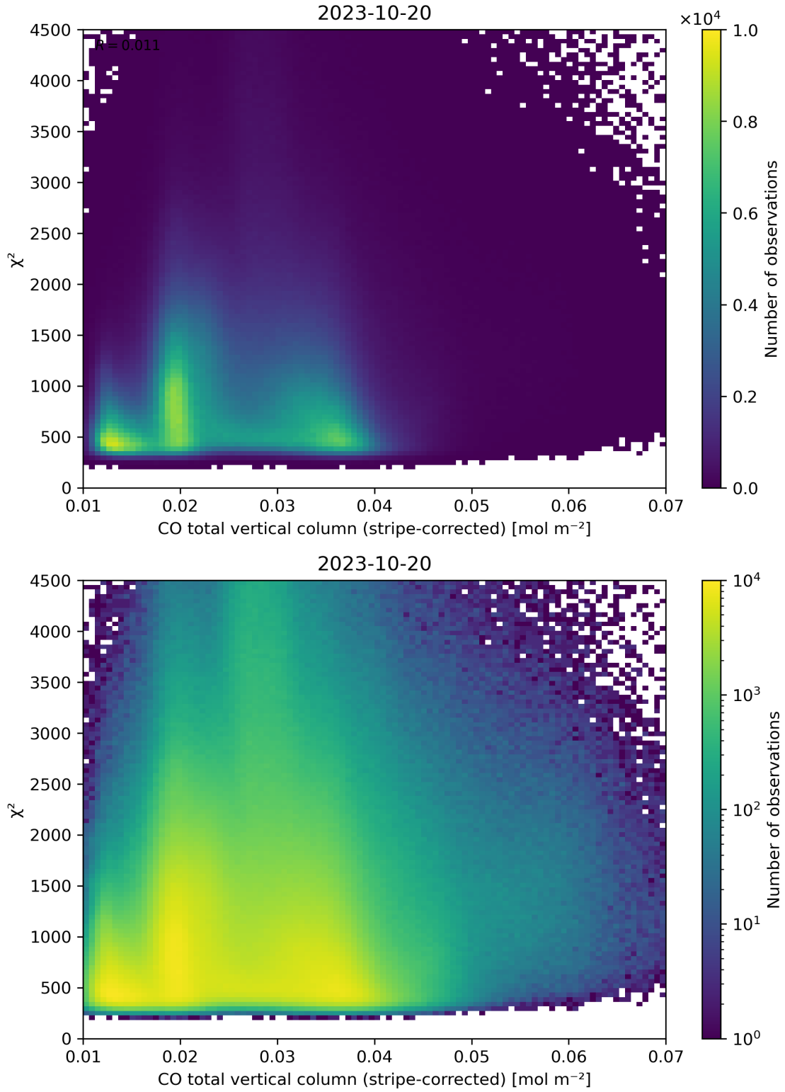
Figure 37: Scatter density plot of “CO total vertical column (stripe-corrected)” against “ \chi^2 ” for 2023-10-19 to 2023-10-21.
