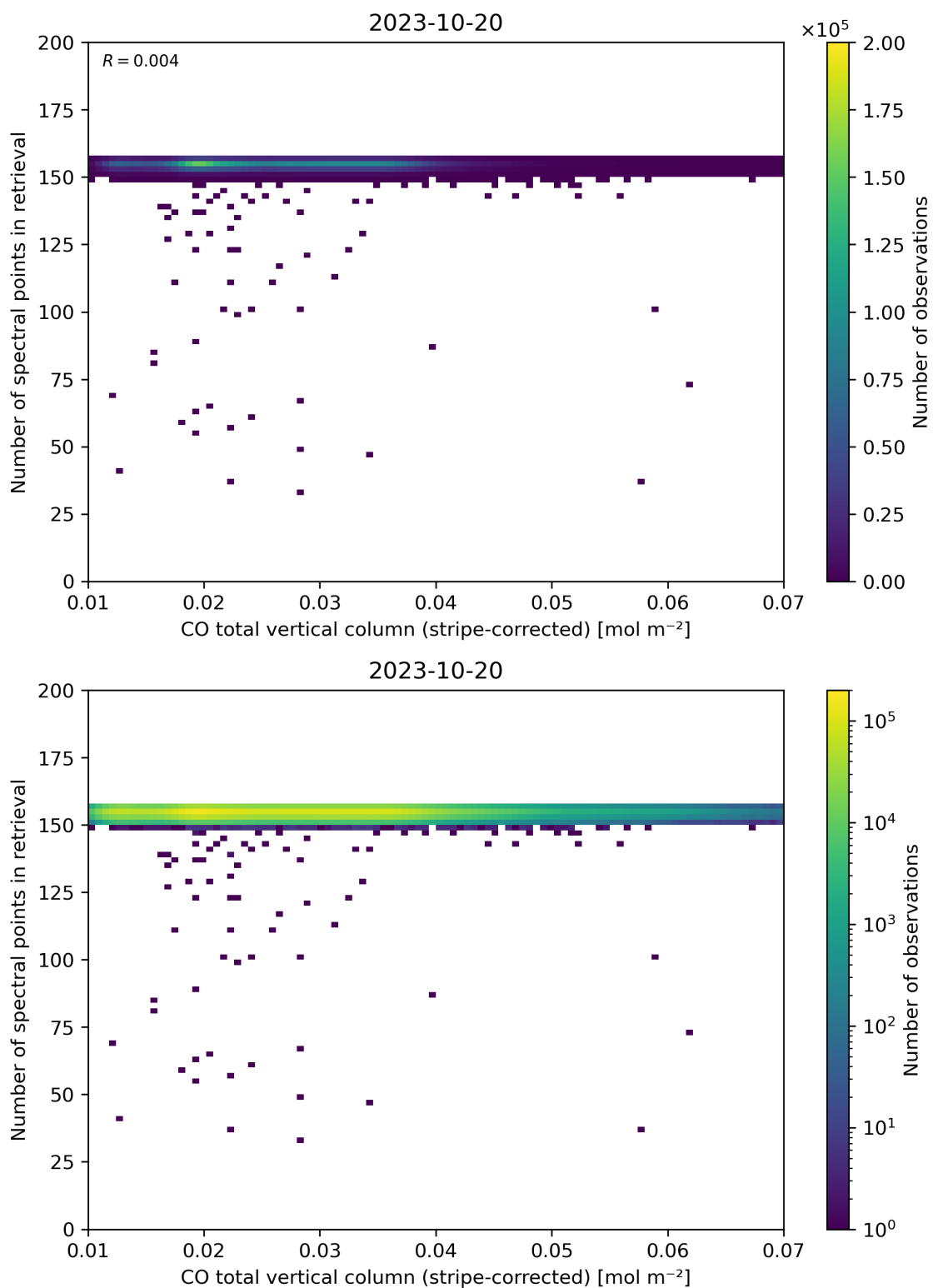
Figure 40: Scatter density plot of “CO total vertical column (stripe-corrected)” against “Number of spectral points in retrieval” for 2023-10-19 to 2023-10-21.
