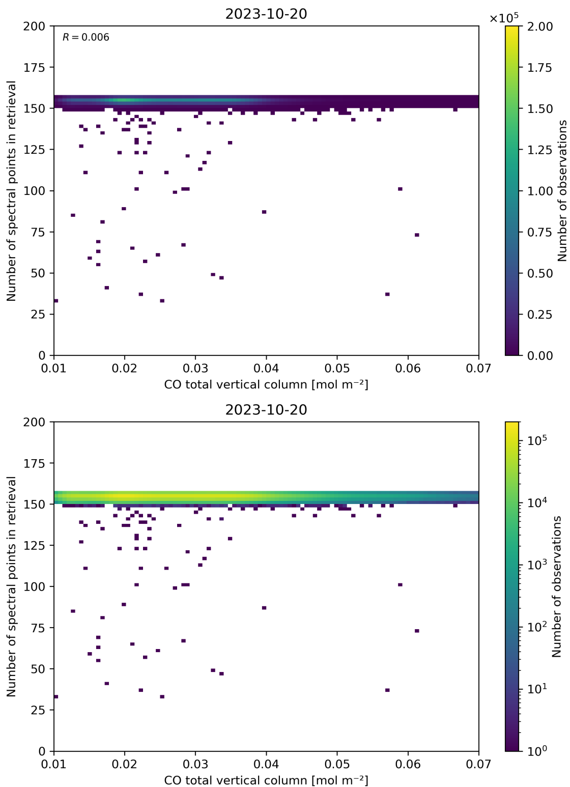
Figure 43: Scatter density plot of “CO total vertical column” against “Number of spectral points in retrieval” for 2023-10-19 to 2023-10-21.
