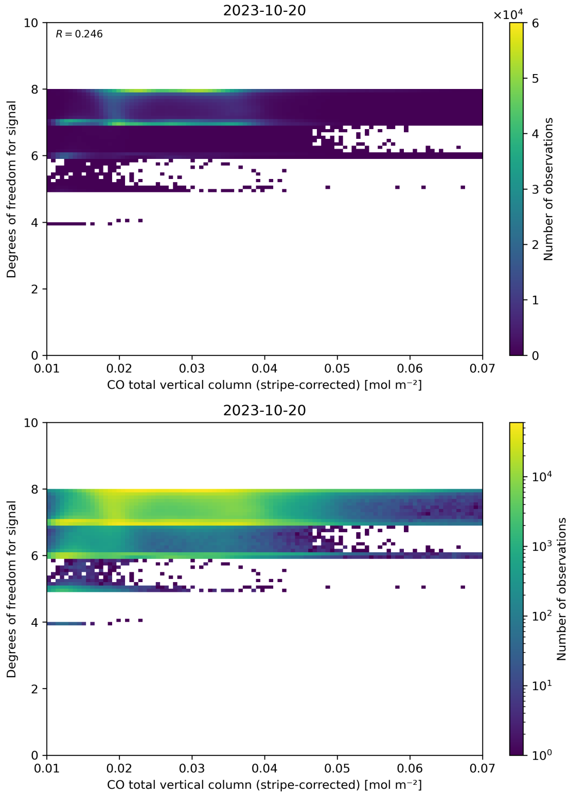
Figure 38: Scatter density plot of “CO total vertical column (stripe-corrected)” against “Degrees of freedom for signal” for 2023-10-19 to 2023-10-21.
