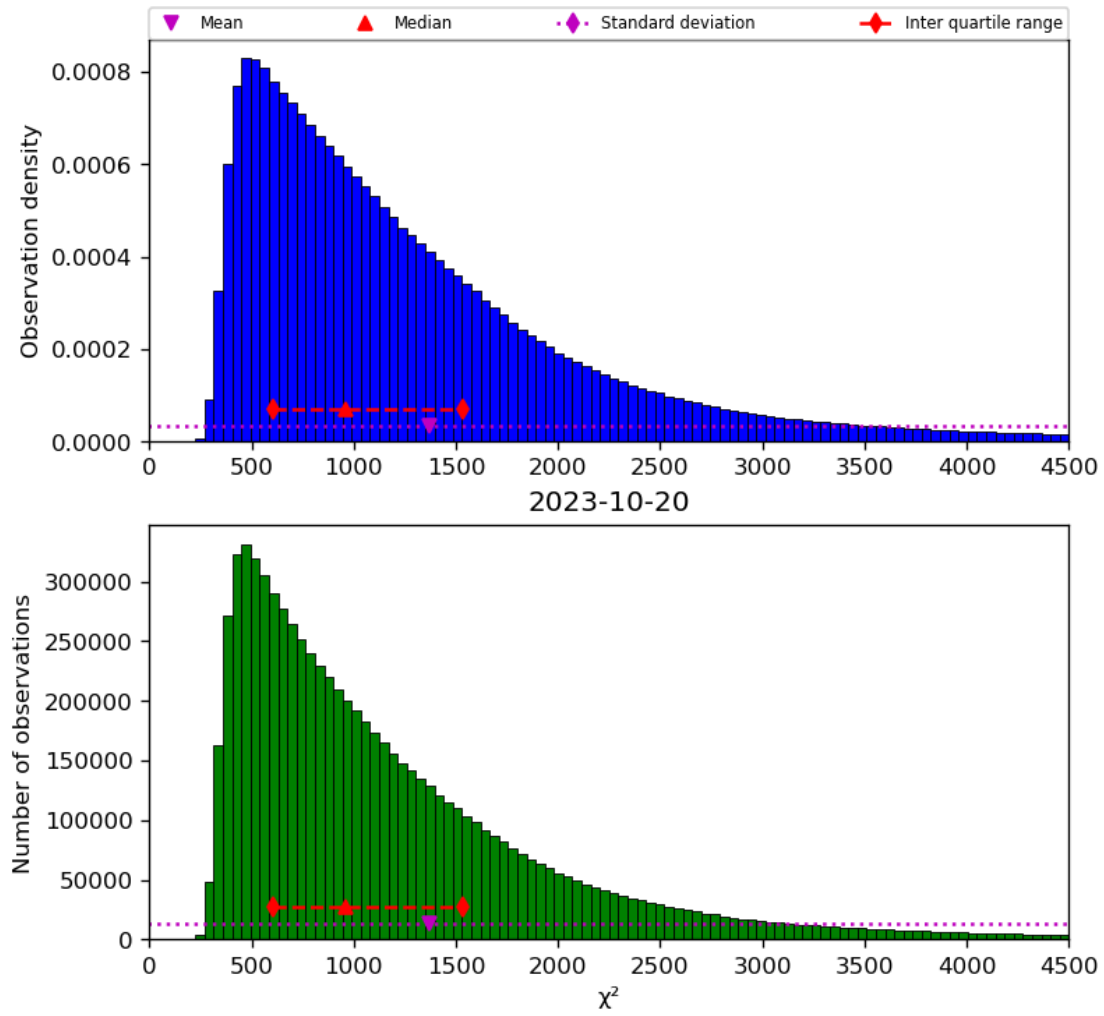
Figure 22: Histogram of “ \chi^2 ” for 2023-10-19 to 2023-10-21
