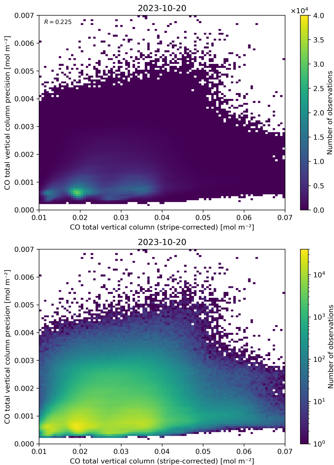
Figure 36: Scatter density plot of “CO total vertical column (stripe-corrected)” against “CO total vertical column precision” for 2023-10-19 to 2023-10-21.
