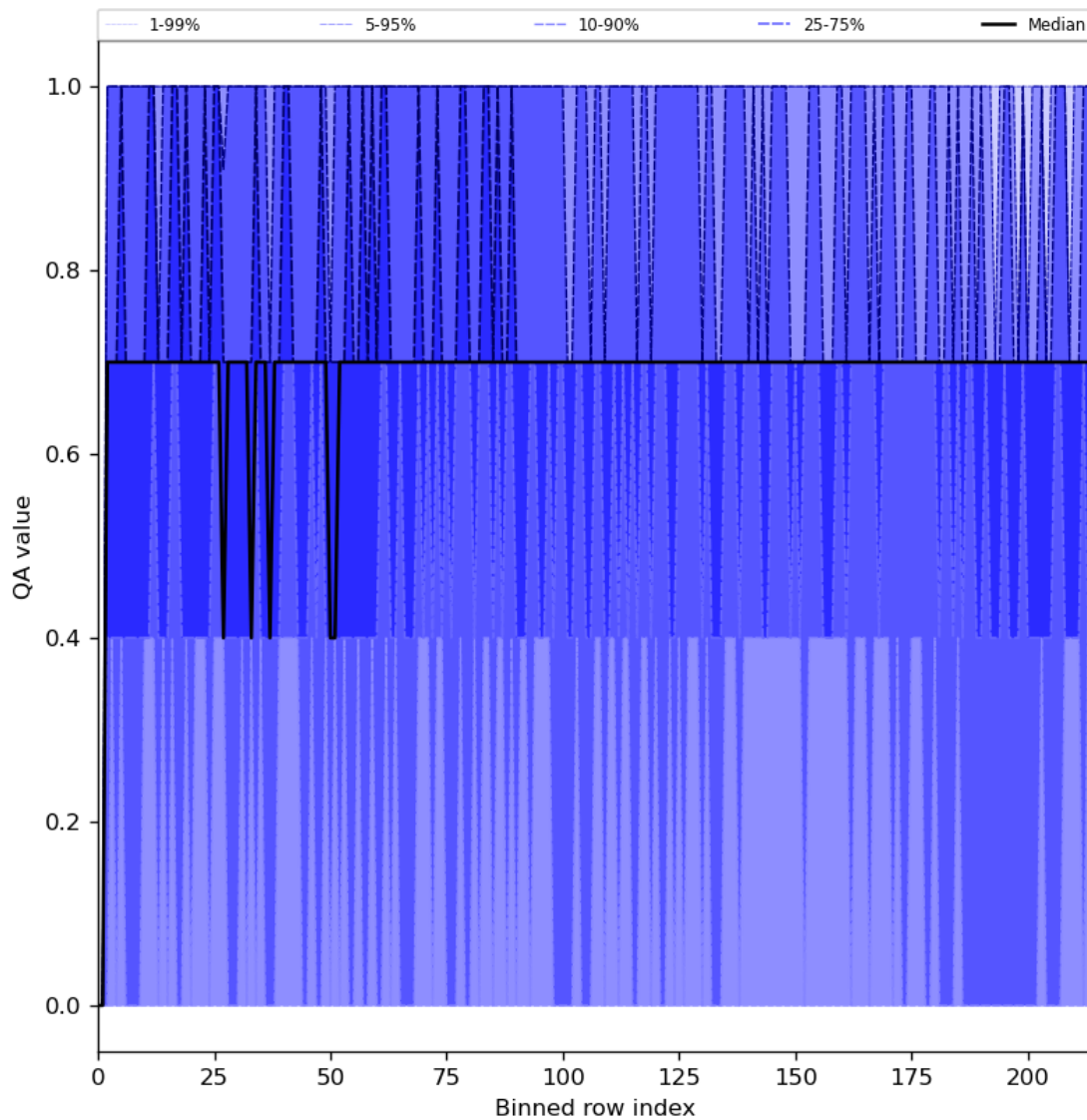
Figure 25: Along track statistics of “QA value” for 2023-10-19 to 2023-10-21
