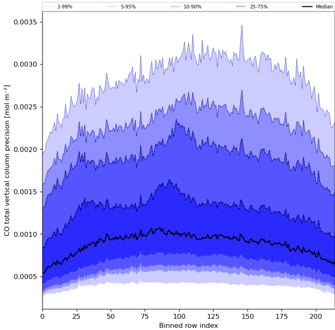
Figure 28: Along track statistics of “CO total vertical column precision” for 2023-10-19 to 2023-10-21
