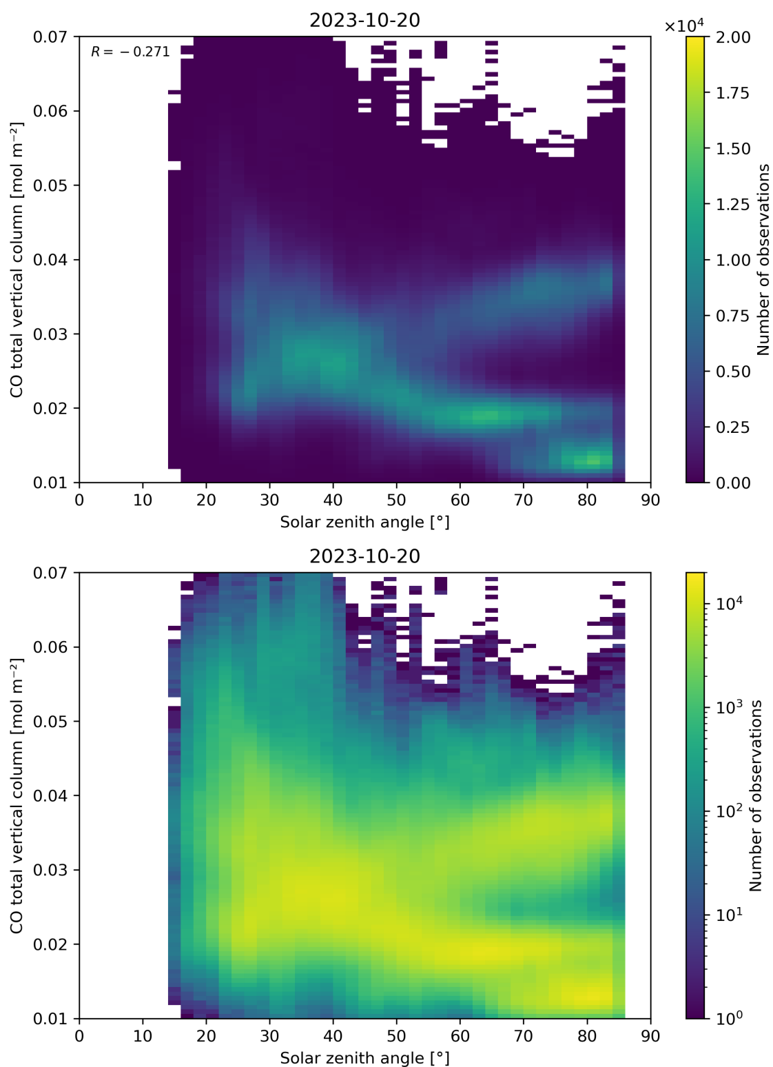
Figure 61: Scatter density plot of “Solar zenith angle” against “CO total vertical column” for 2023-10-19 to 2023-10-21.
