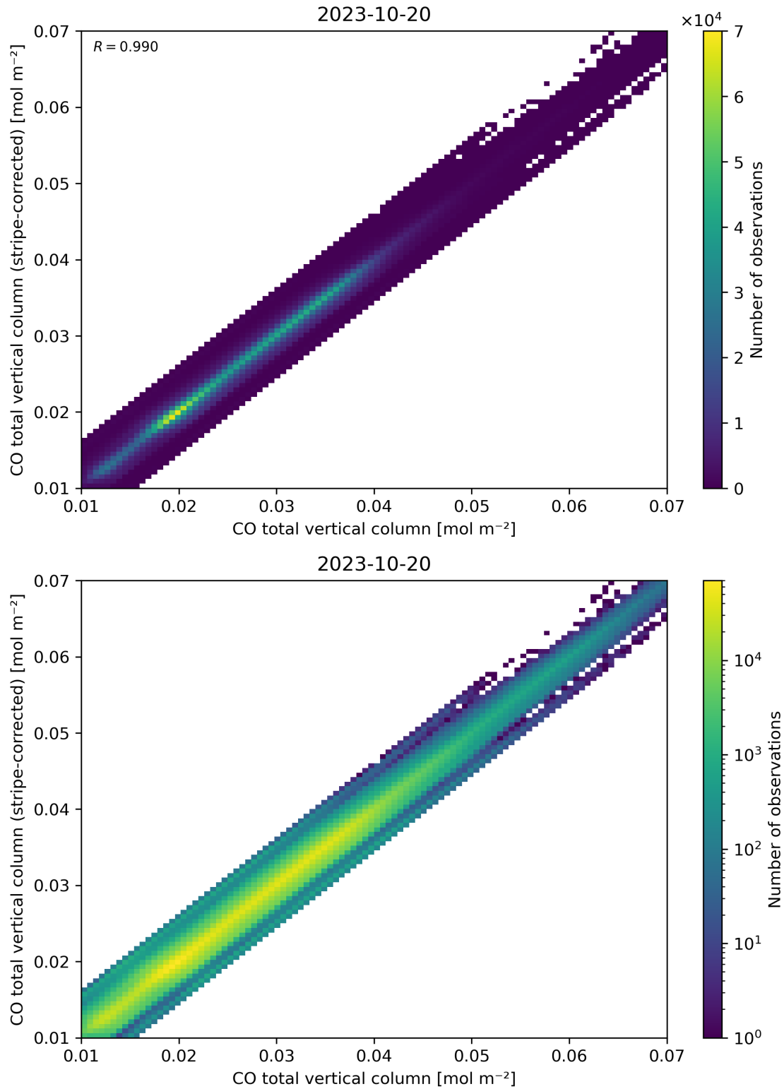
Figure 33: Scatter density plot of “CO total vertical column” against “CO total vertical column (stripe-corrected)” for 2023-10-19 to 2023-10-21.
