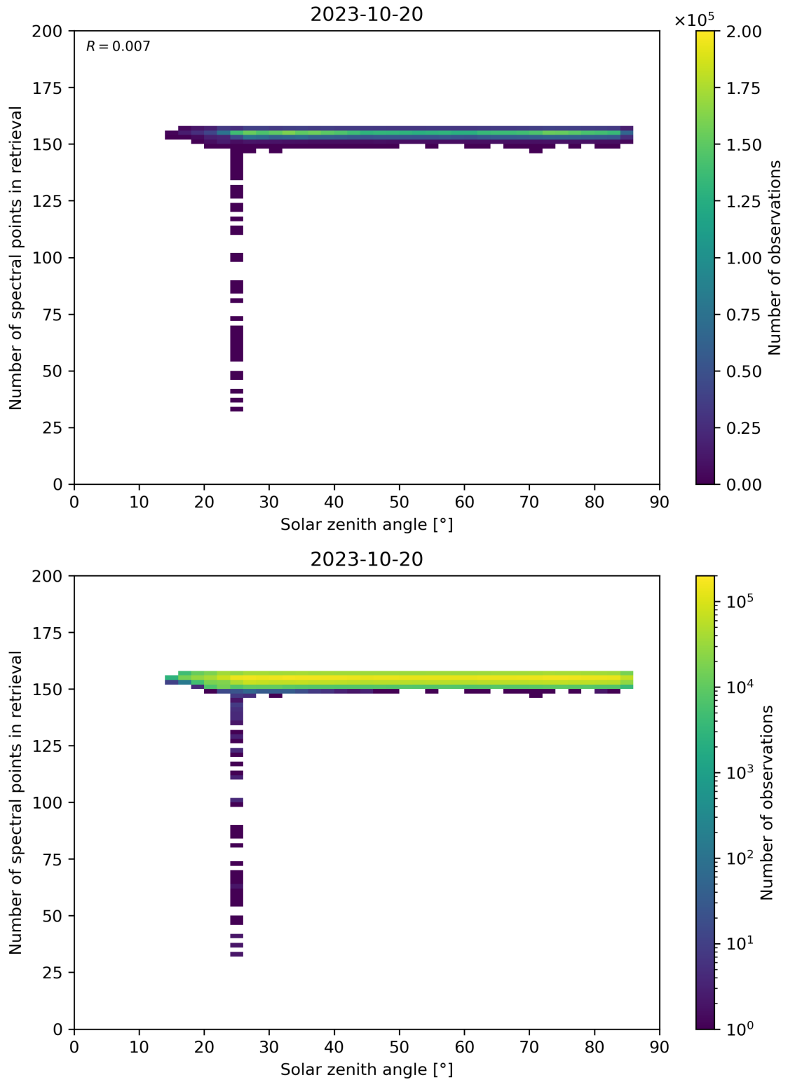
Figure 68: Scatter density plot of “Solar zenith angle” against “Number of spectral points in retrieval” for 2023-10-19 to 2023-10-21.
