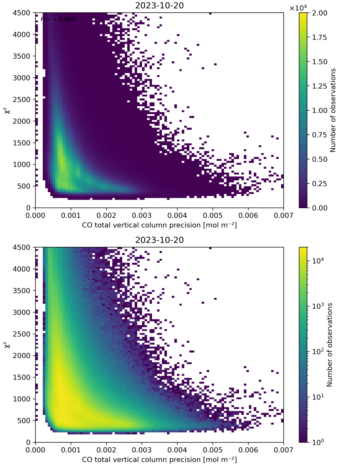
Figure 44: Scatter density plot of “CO total vertical column precision” against “ \chi^2 ” for 2023-10-19 to 2023-10-21.
