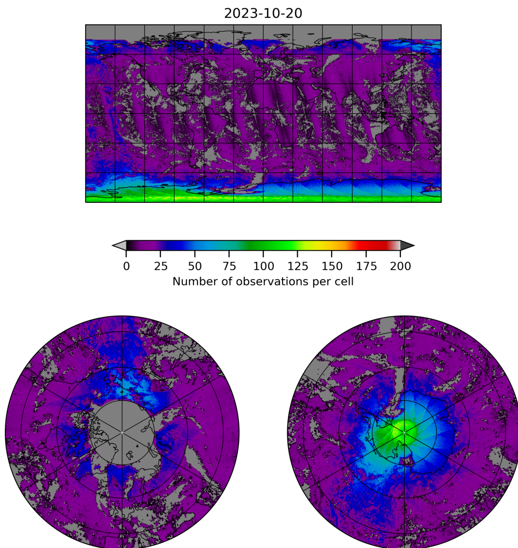
Figure 8: Map of the number of observations for 2023-10-19 to 2023-10-21
