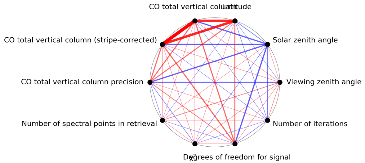
Figure 1: Map of correlation graph for 2023-10-19 to 2023-10-21.
