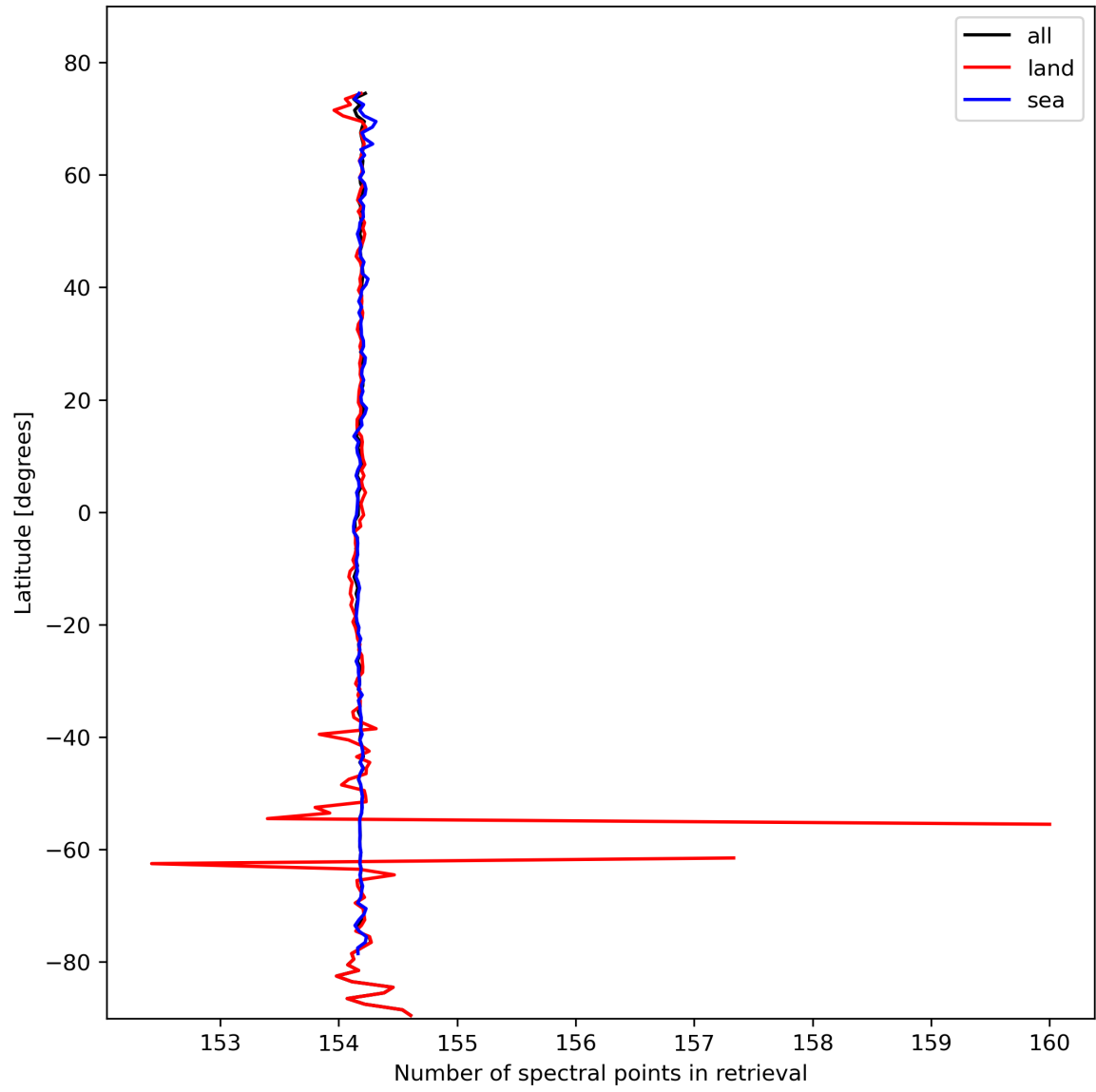
Figure 13: Zonal average of “Number of spectral points in retrieval” for 2023-10-19 to 2023-10-21.
