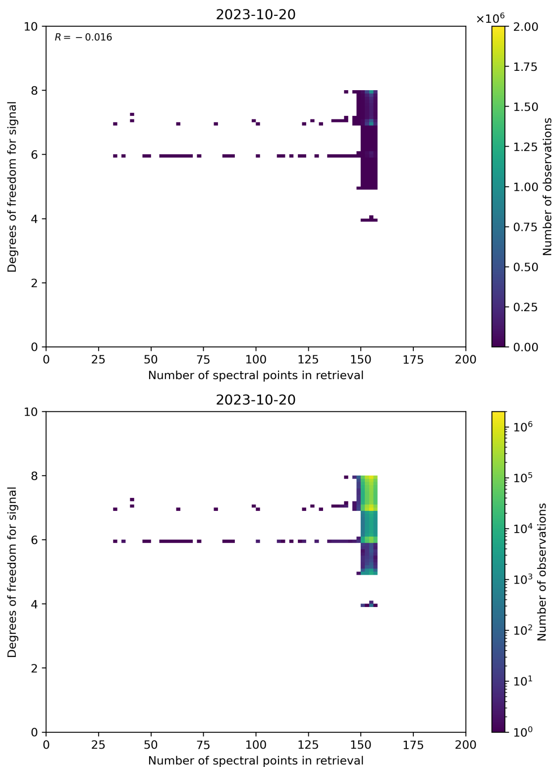
Figure 59: Scatter density plot of “Number of spectral points in retrieval” against “Degrees of freedom for signal” for 2023-10-19 to 2023-10-21.
