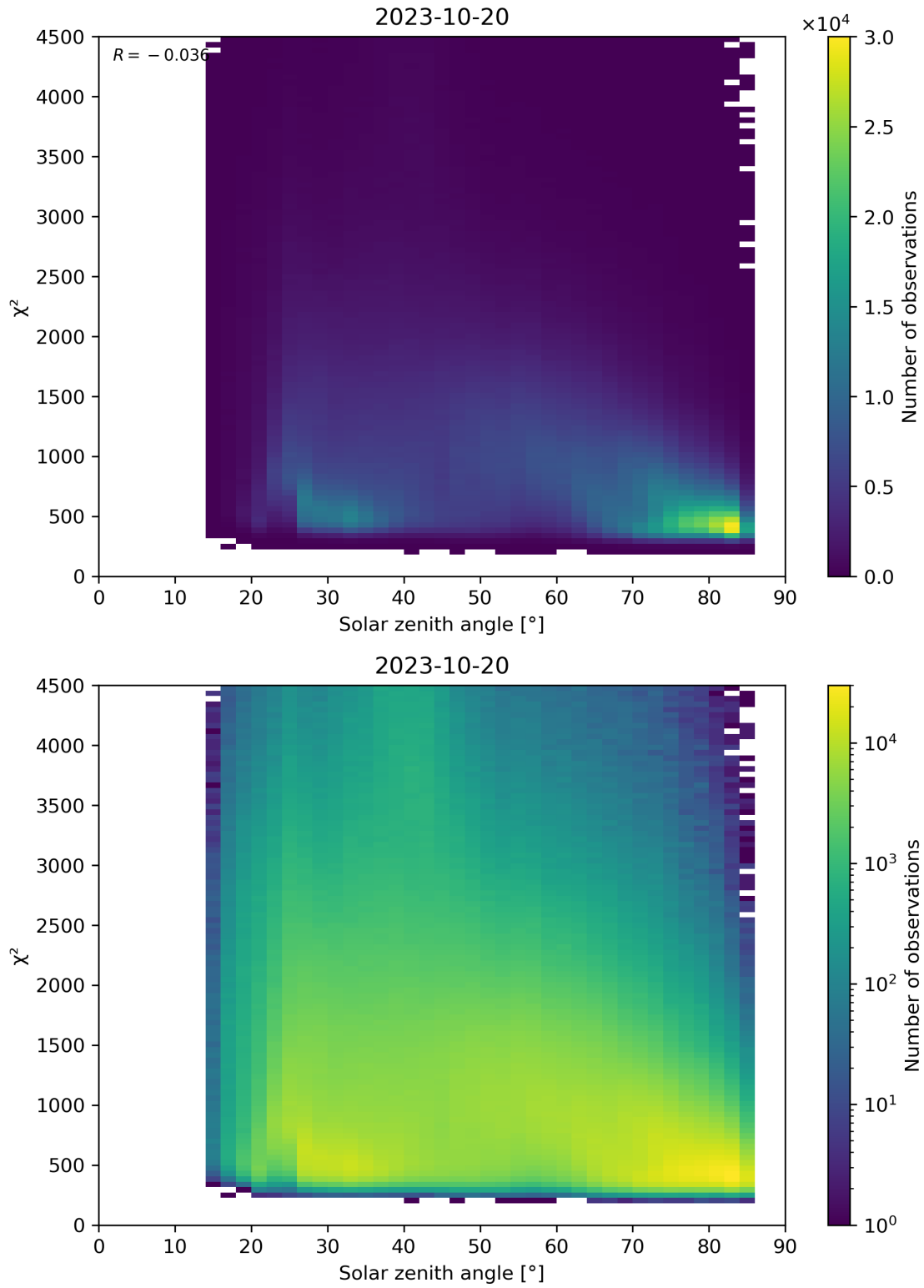
Figure 64: Scatter density plot of “Solar zenith angle” against “ \chi^2 ” for 2023-10-19 to 2023-10-21.
