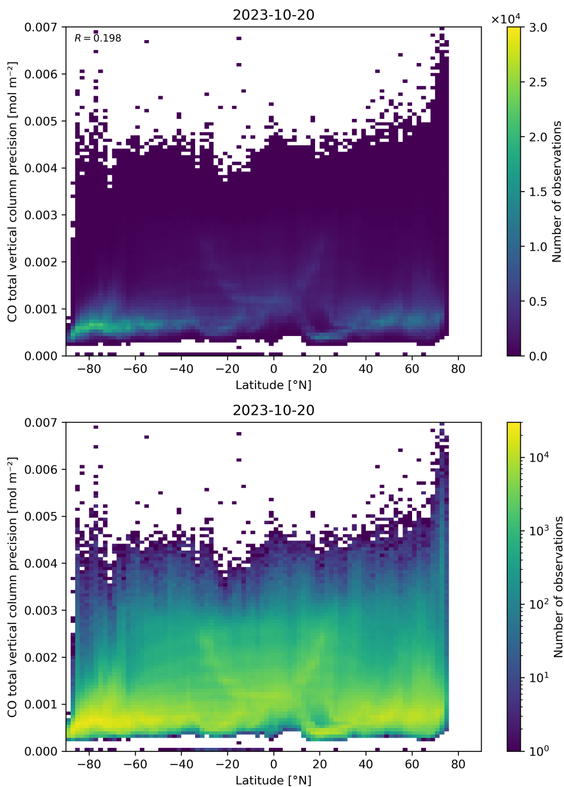
Figure 53: Scatter density plot of “Latitude” against “CO total vertical column precision” for 2023-10-19 to 2023-10-21.
