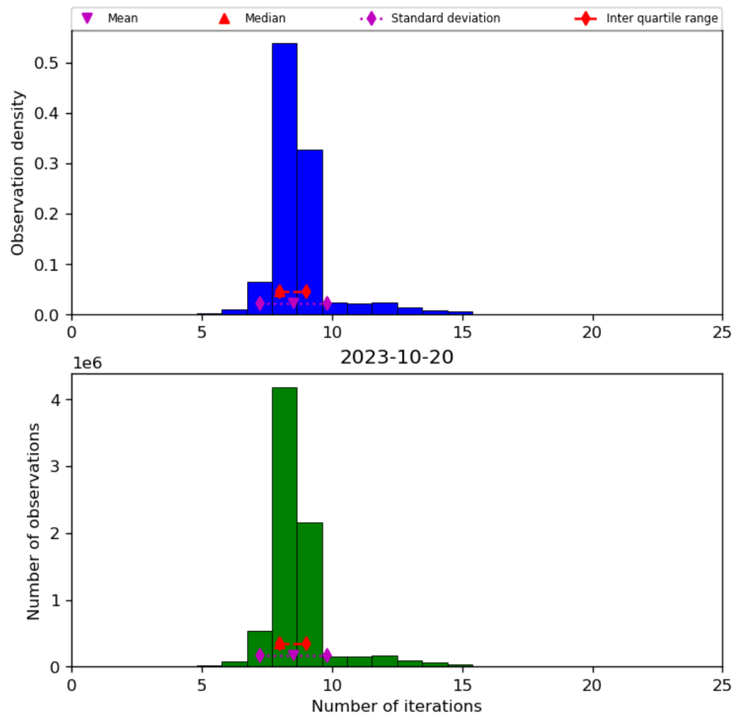
Figure 24: Histogram of “Number of iterations” for 2023-10-19 to 2023-10-21
