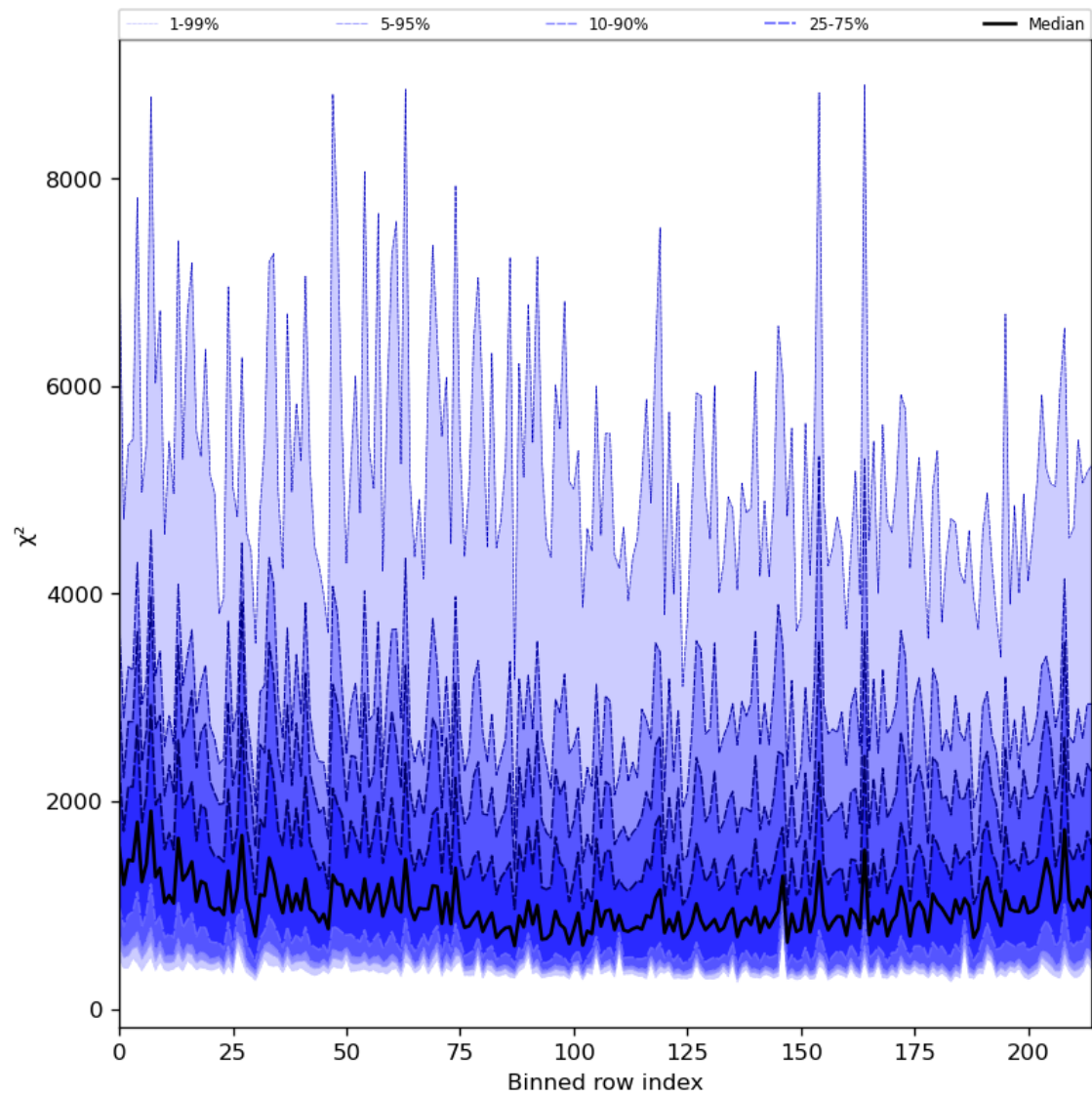
Figure 30: Along track statistics of “ \chi^2 ” for 2023-10-19 to 2023-10-21
