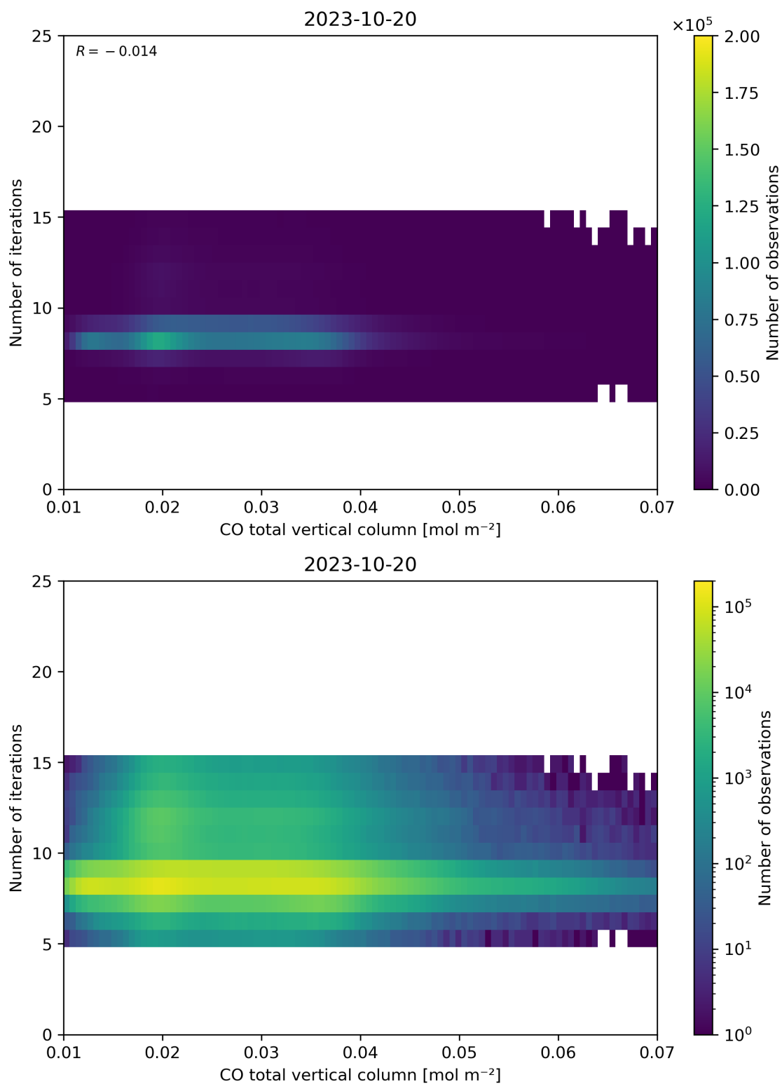
Figure 42: Scatter density plot of “CO total vertical column” against “Number of iterations” for 2023-10-19 to 2023-10-21.
