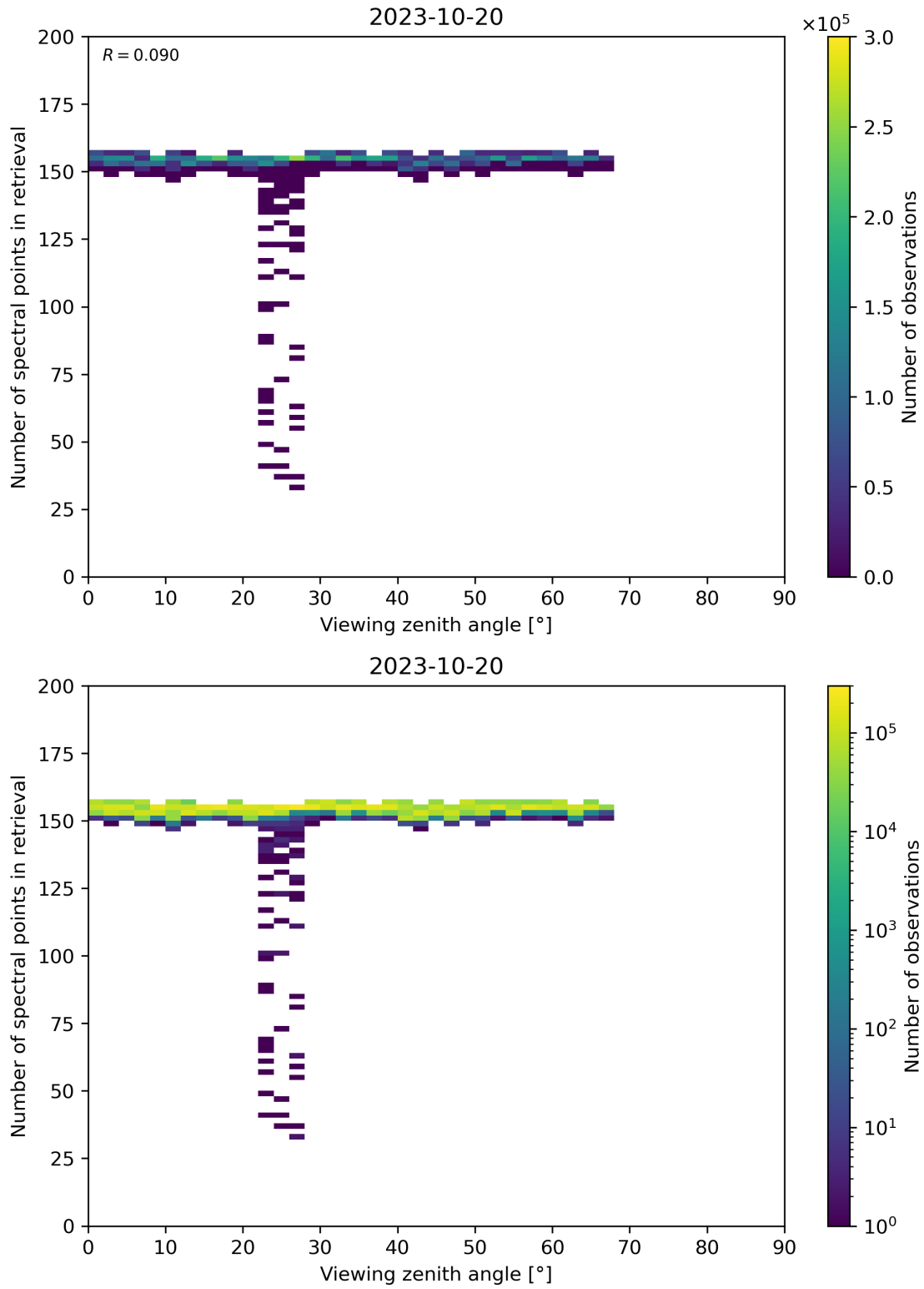
Figure 76: Scatter density plot of “Viewing zenith angle” against “Number of spectral points in retrieval” for 2023-10-19 to 2023-10-21.
