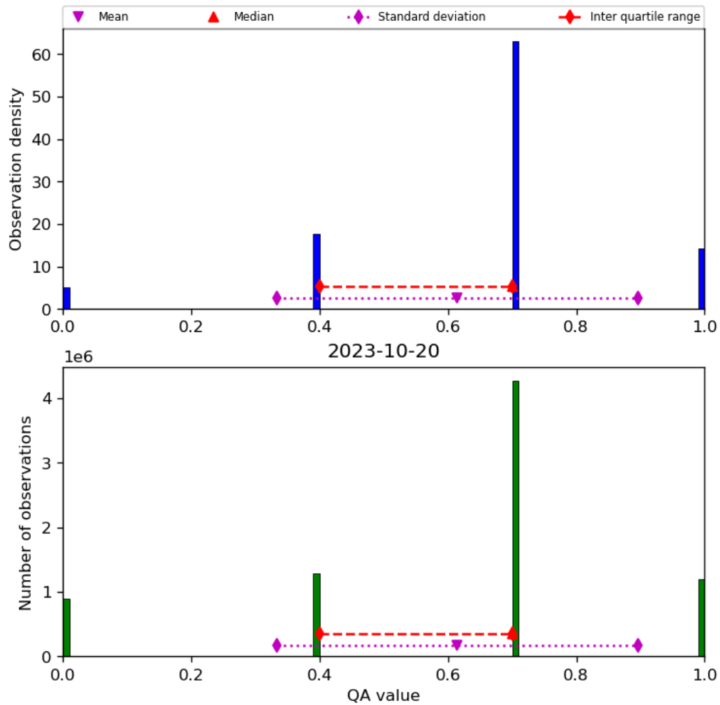
Figure 17: Histogram of “QA value” for 2023-10-19 to 2023-10-21
