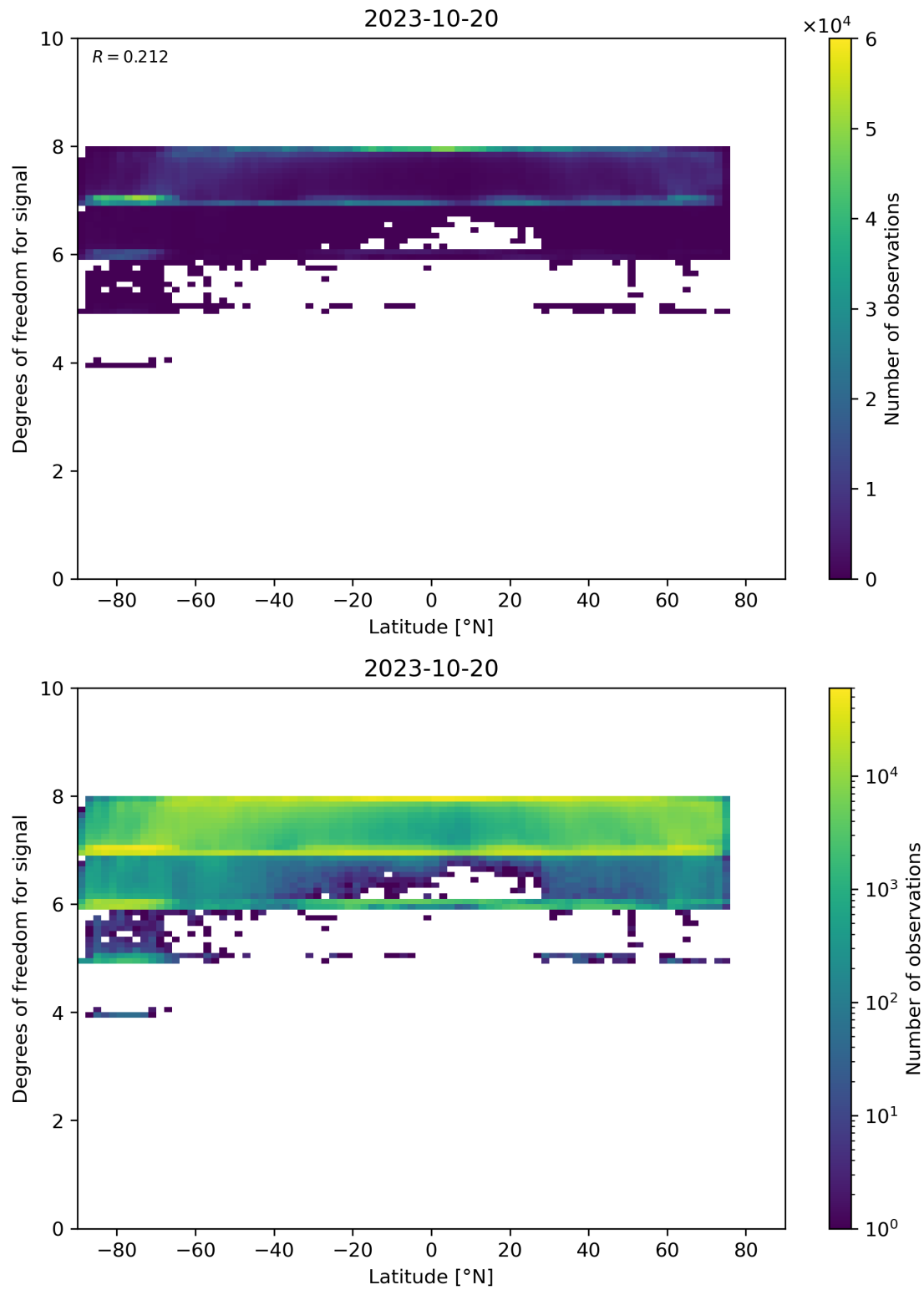
Figure 55: Scatter density plot of “Latitude” against “Degrees of freedom for signal” for 2023-10-19 to 2023-10-21.
