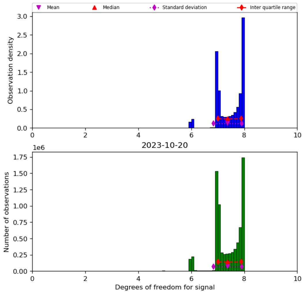
Figure 23: Histogram of “Degrees of freedom for signal” for 2023-10-19 to 2023-10-21
