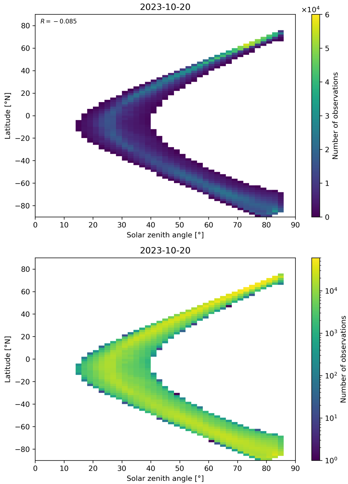
Figure 66: Scatter density plot of “Solar zenith angle” against “Latitude” for 2023-10-19 to 2023-10-21.
