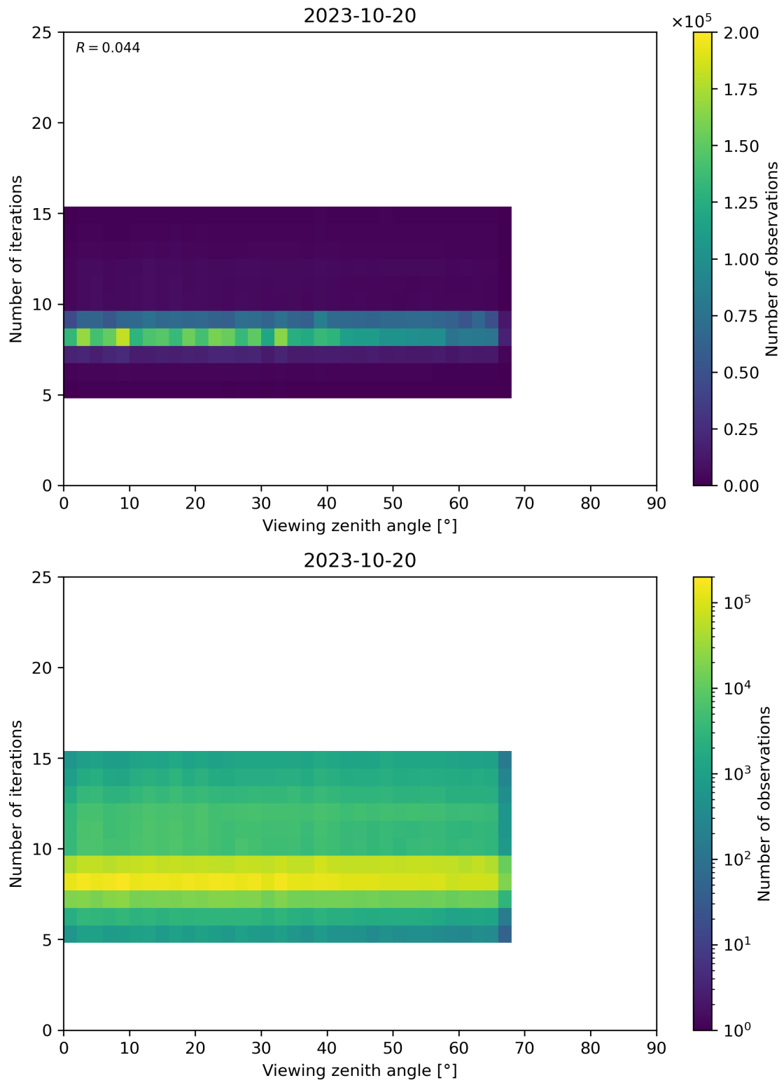
Figure 75: Scatter density plot of “Viewing zenith angle” against “Number of iterations” for 2023-10-19 to 2023-10-21.
