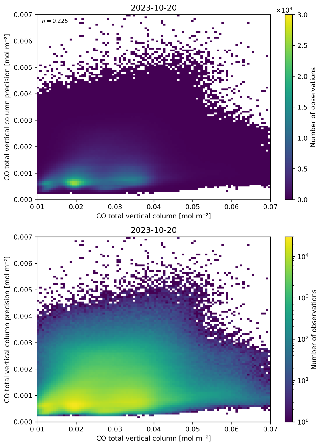
Figure 34: Scatter density plot of “CO total vertical column” against “CO total vertical column precision” for 2023-10-19 to 2023-10-21.
