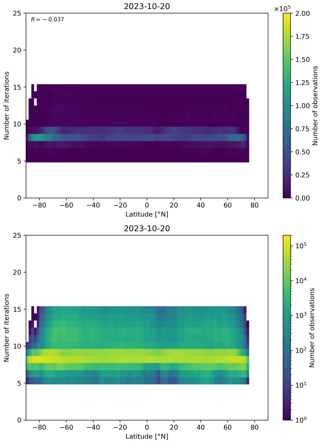
Figure 56: Scatter density plot of “Latitude” against “Number of iterations” for 2023-10-19 to 2023-10-21.
