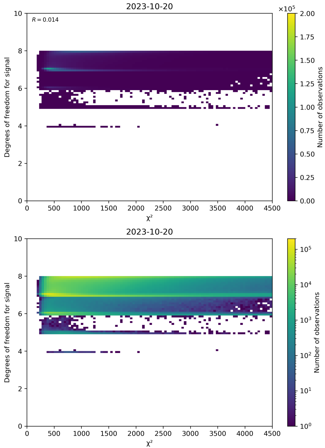
Figure 48: Scatter density plot of “ \chi^2 ” against “Degrees of freedom for signal” for 2023-10-19 to 2023-10-21.
