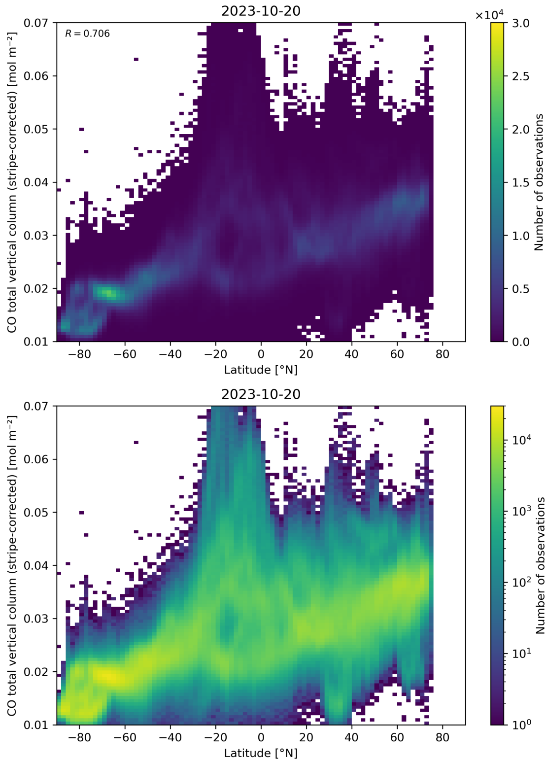
Figure 52: Scatter density plot of “Latitude” against “CO total vertical column (stripe-corrected)” for 2023-10-19 to 2023-10-21.
