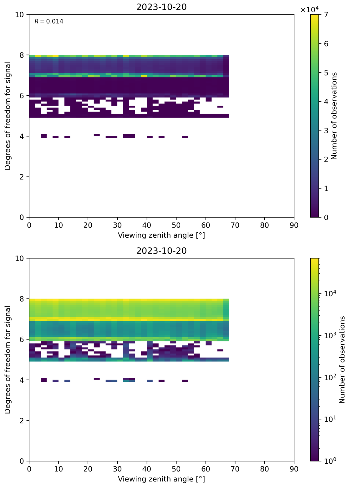
Figure 73: Scatter density plot of “Viewing zenith angle” against “Degrees of freedom for signal” for 2023-10-19 to 2023-10-21.
