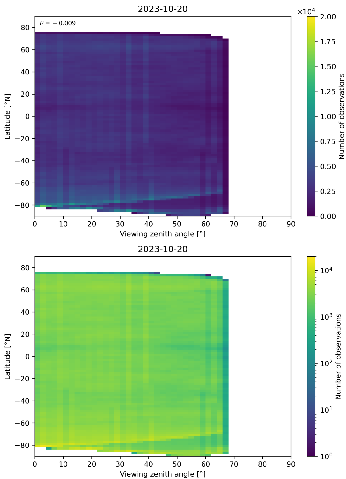
Figure 74: Scatter density plot of “Viewing zenith angle” against “Latitude” for 2023-10-19 to 2023-10-21.
