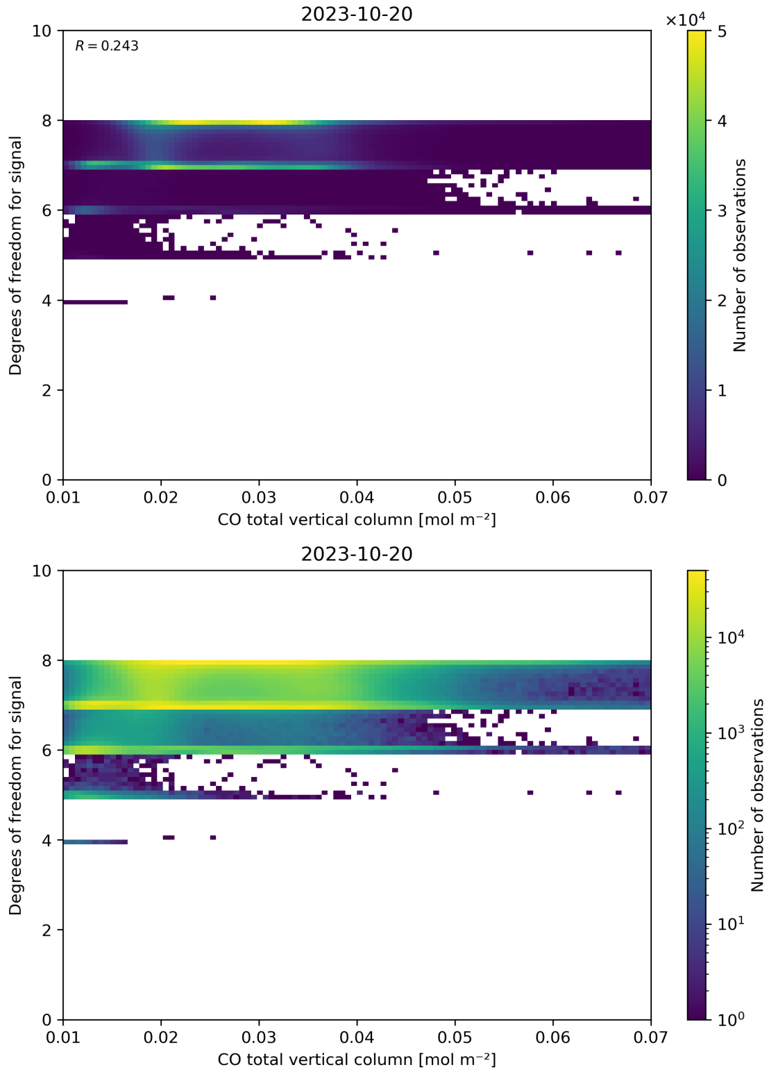
Figure 41: Scatter density plot of “CO total vertical column” against “Degrees of freedom for signal” for 2023-10-19 to 2023-10-21.
