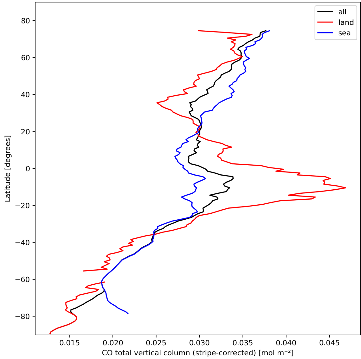
Figure 11: Zonal average of “CO total vertical column (stripe-corrected)” for 2023-10-19 to 2023-10-21.
