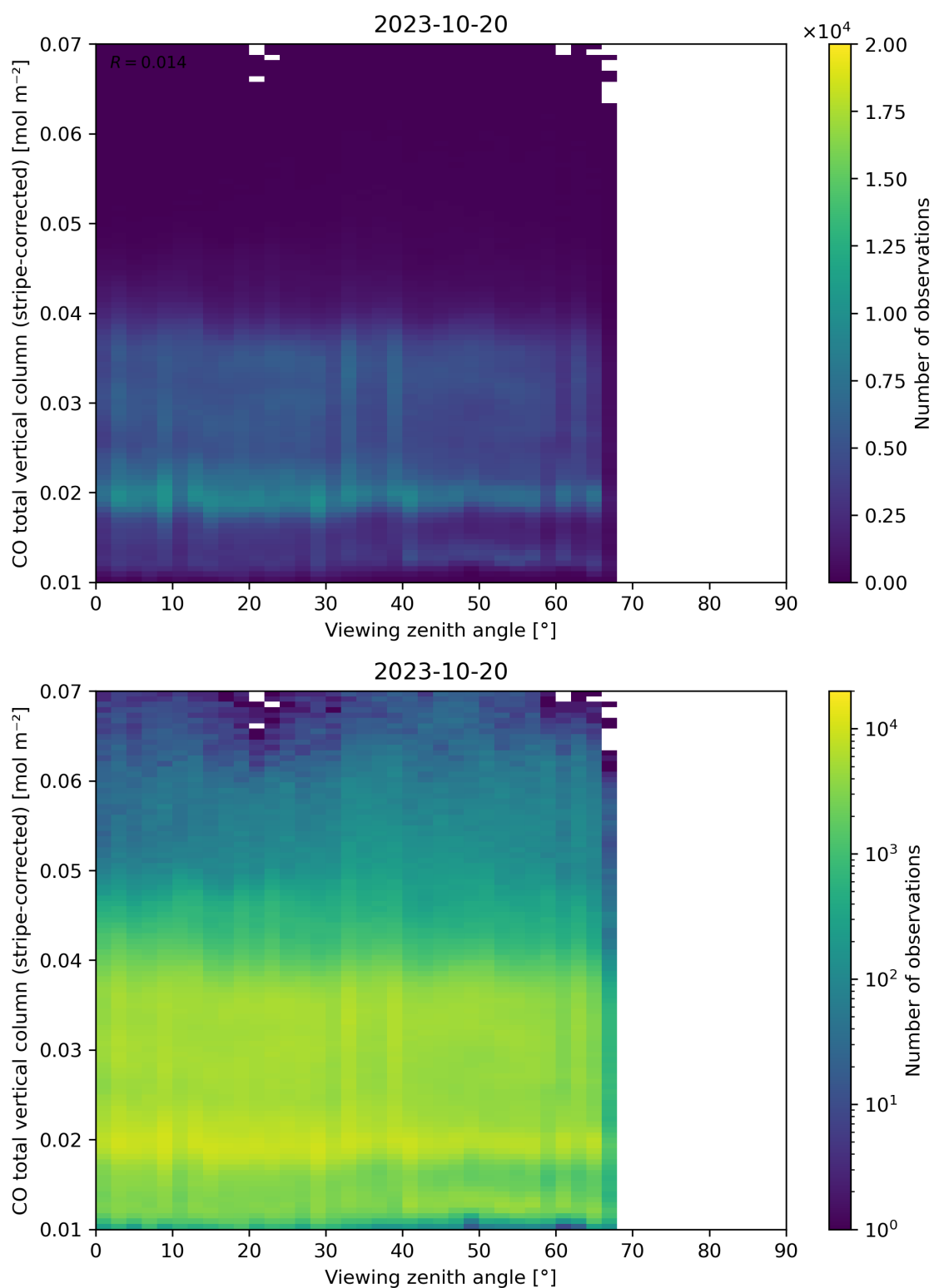
Figure 70: Scatter density plot of “Viewing zenith angle” against “CO total vertical column (stripe-corrected)” for 2023-10-19 to 2023-10-21.
