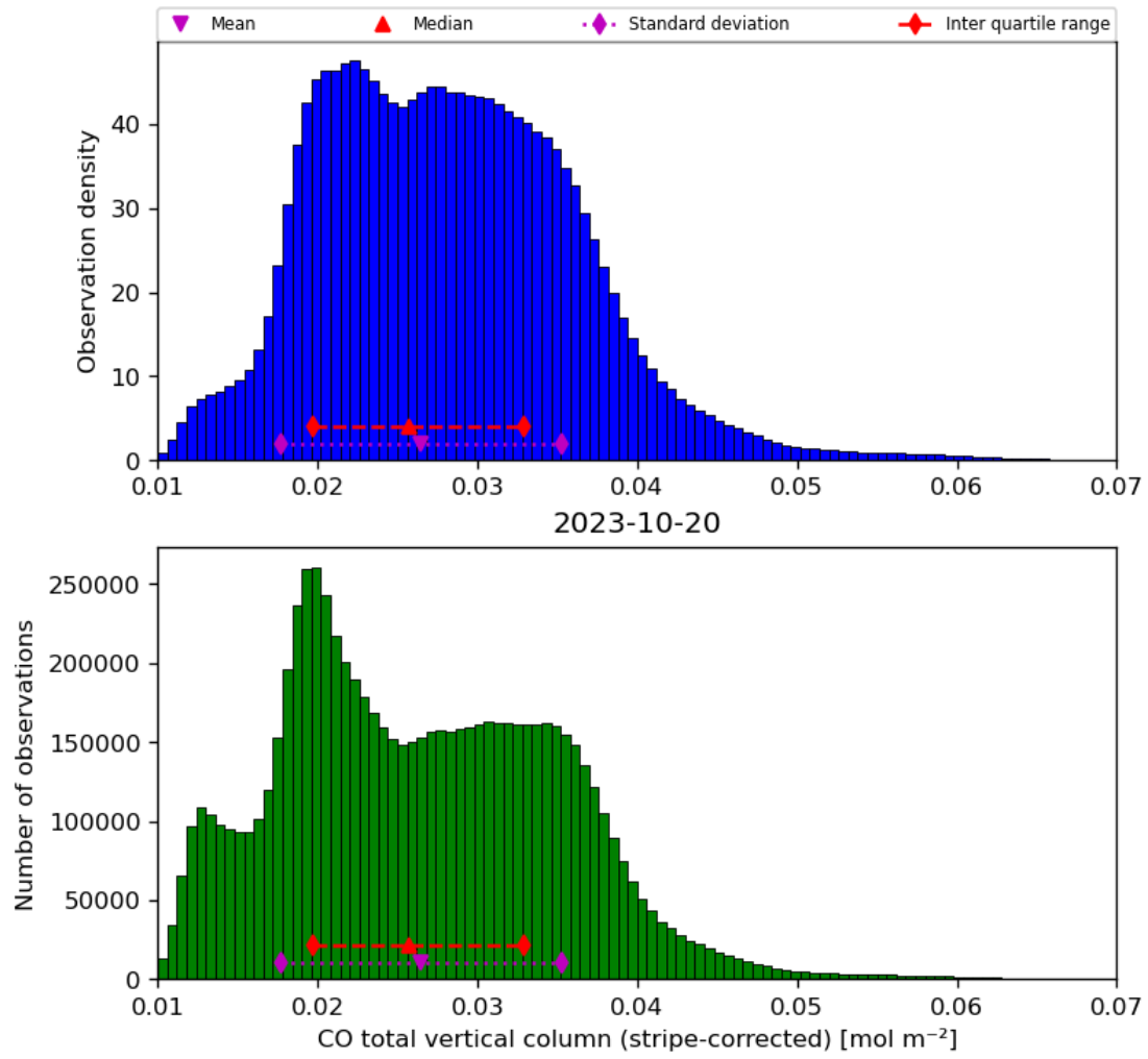
Figure 19: Histogram of “CO total vertical column (stripe-corrected)” for 2023-10-19 to 2023-10-21
