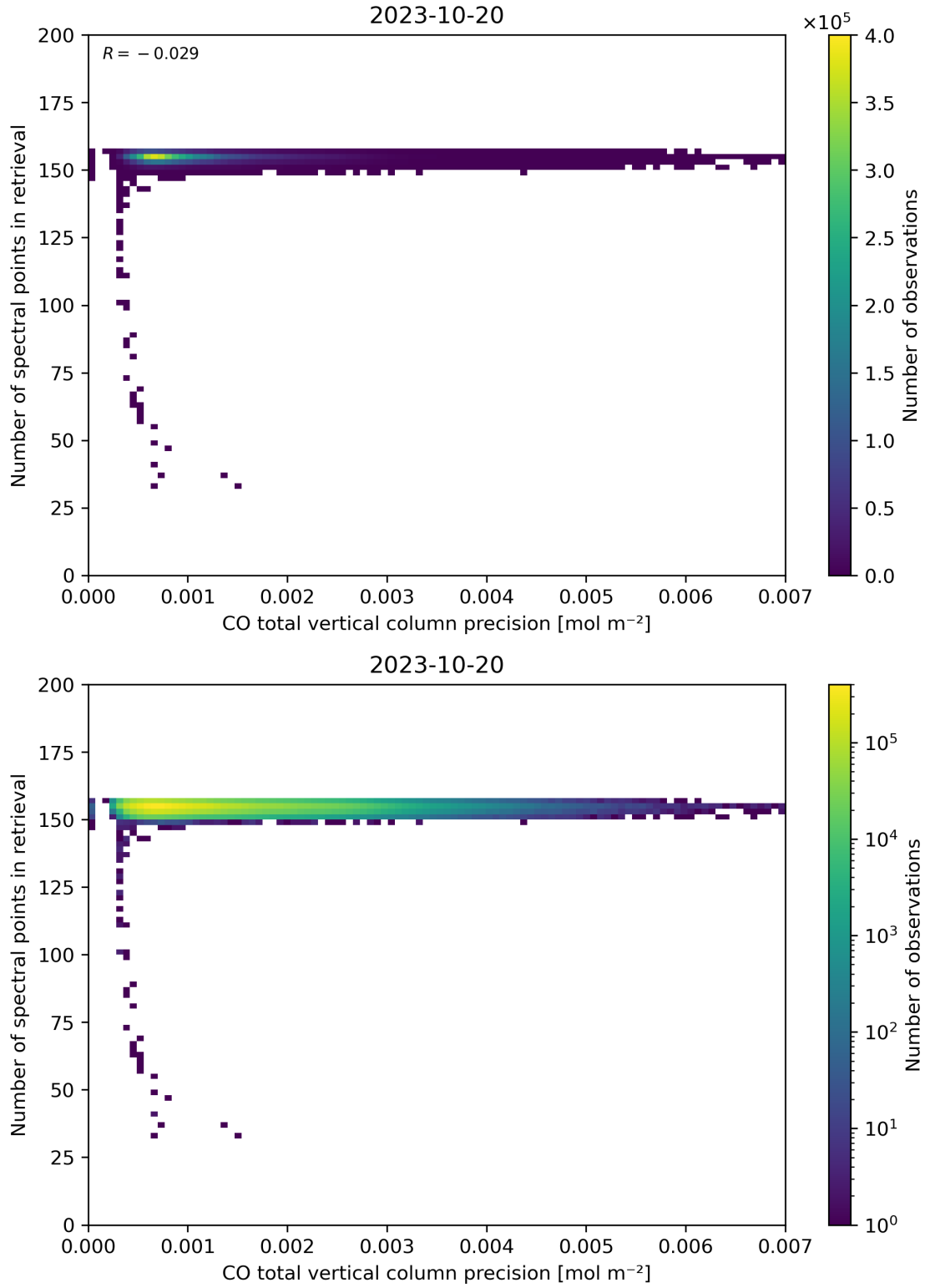
Figure 47: Scatter density plot of “CO total vertical column precision” against “Number of spectral points in retrieval” for 2023-10-19 to 2023-10-21.
