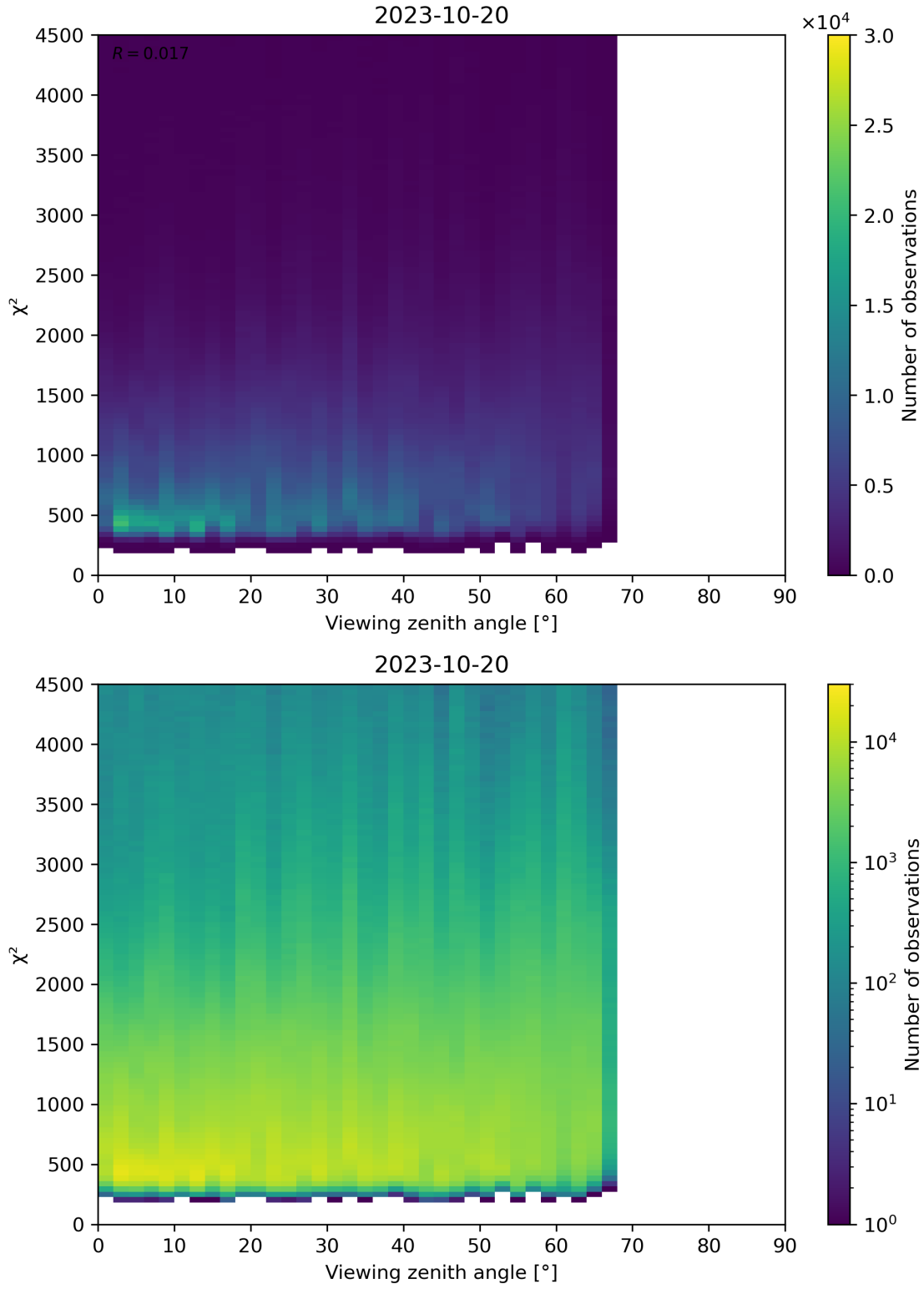
Figure 72: Scatter density plot of “Viewing zenith angle” against “ \chi^2 ” for 2023-10-19 to 2023-10-21.
