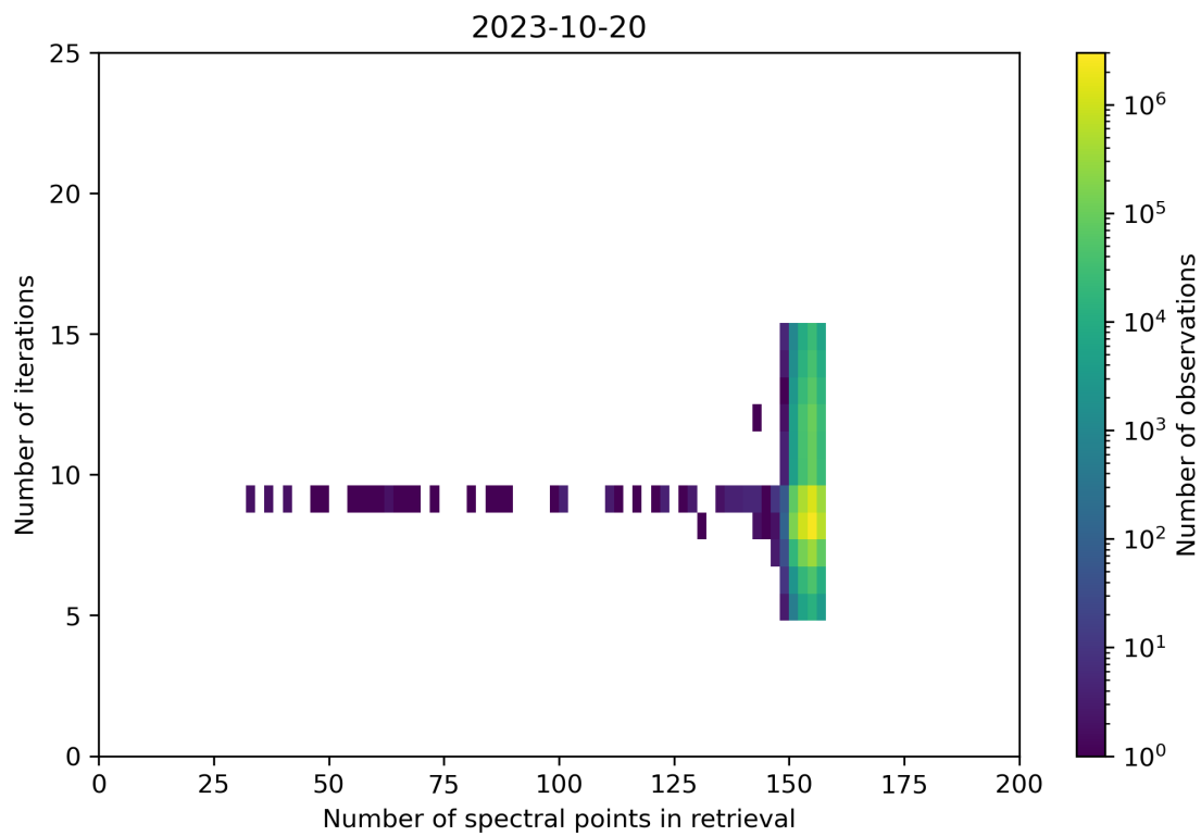
Figure 60: Scatter density plot of “Number of spectral points in retrieval” against “Number of iterations” for 2023-10-19 to 2023-10-21.
