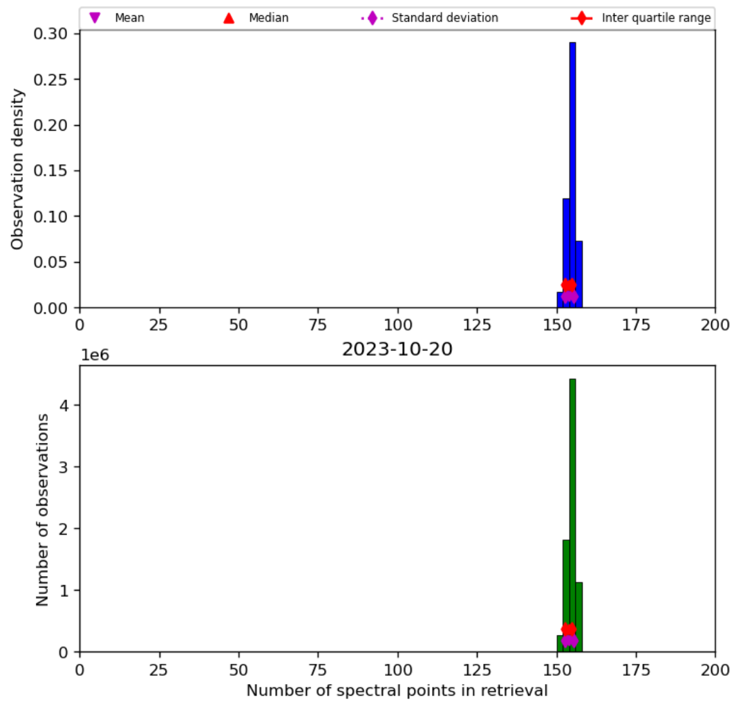
Figure 21: Histogram of “Number of spectral points in retrieval” for 2023-10-19 to 2023-10-21
