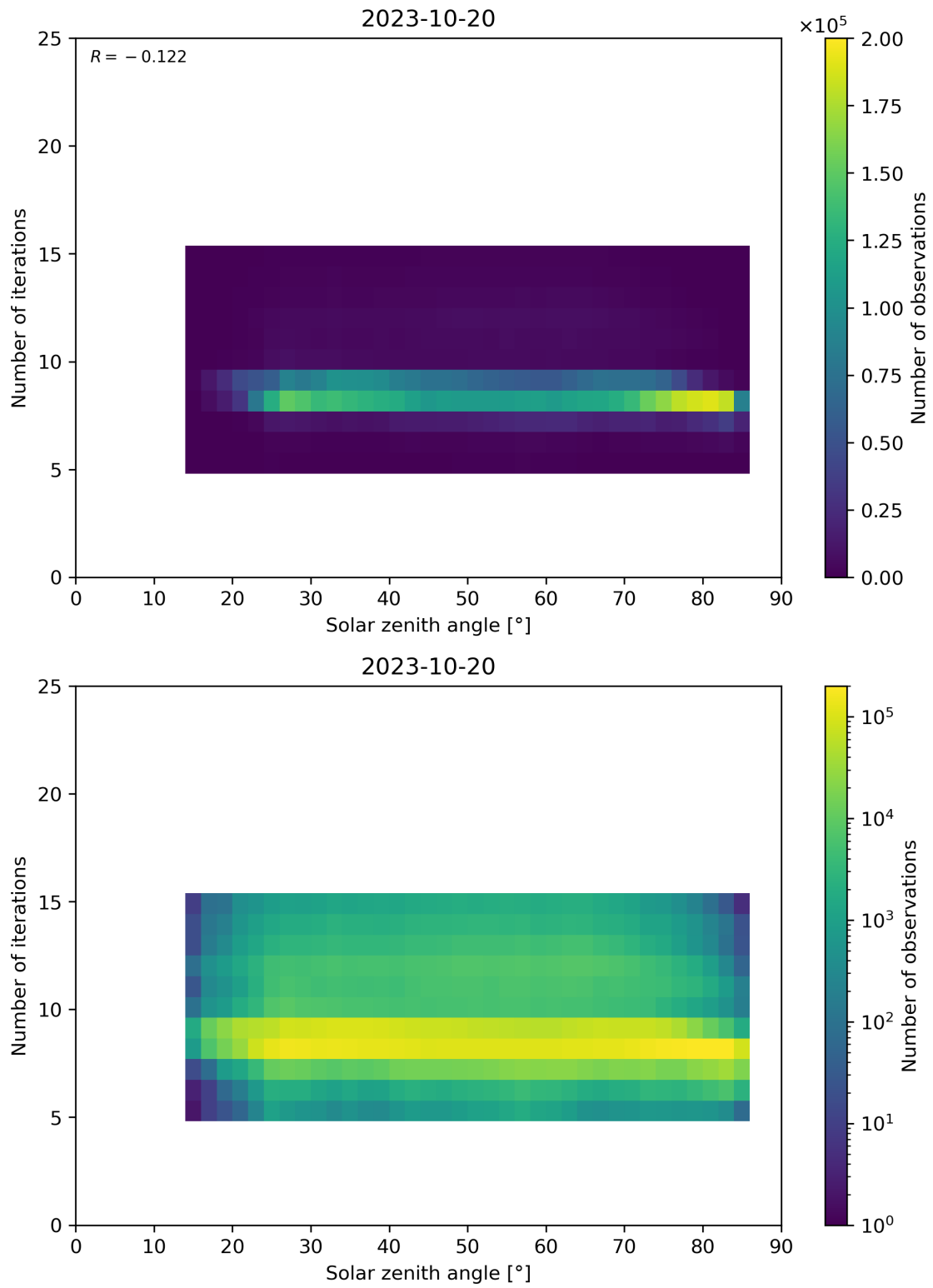
Figure 67: Scatter density plot of “Solar zenith angle” against “Number of iterations” for 2023-10-19 to 2023-10-21.
