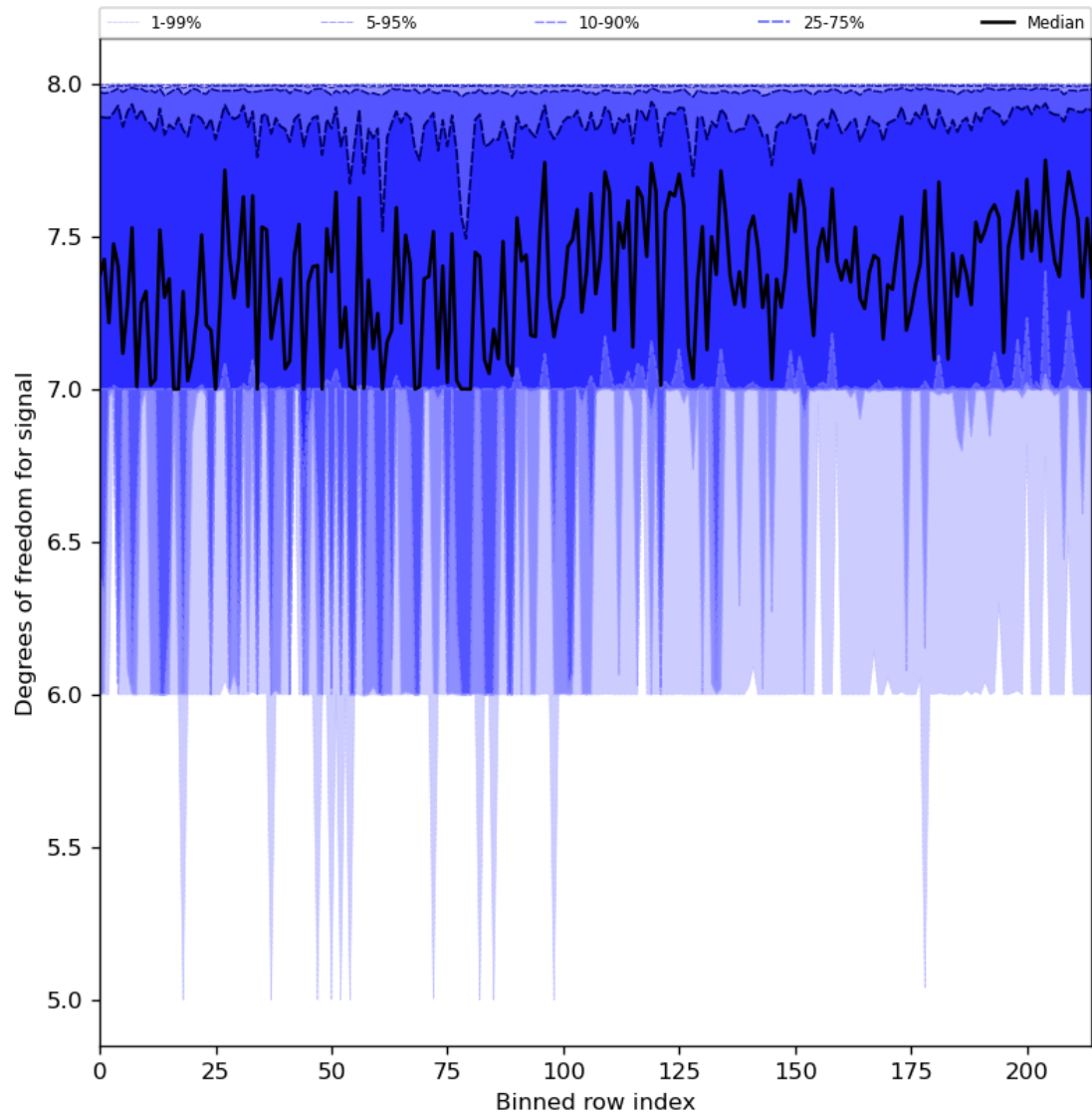
Figure 31: Along track statistics of “Degrees of freedom for signal” for 2023-10-19 to 2023-10-21
