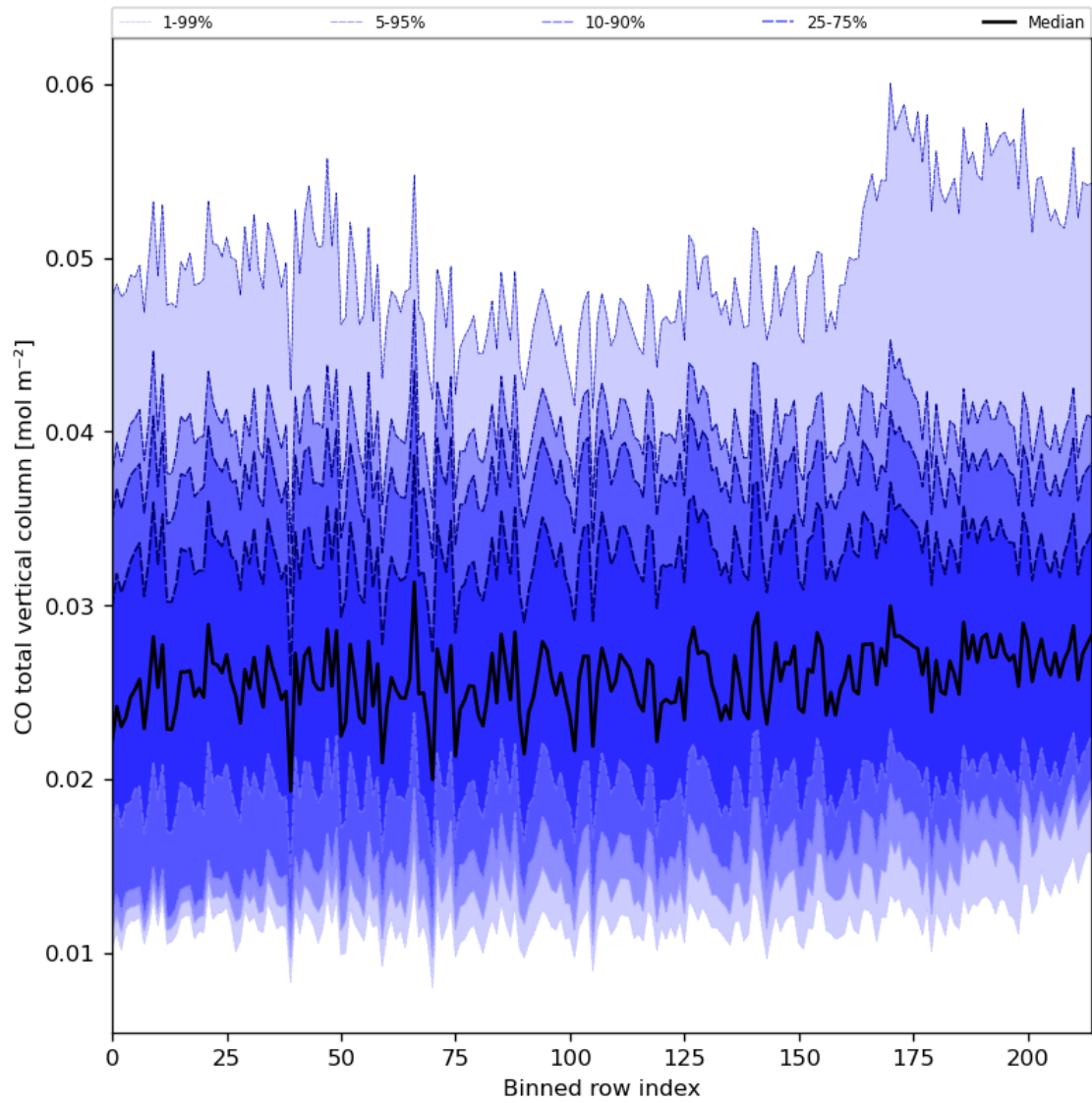
Figure 26: Along track statistics of “CO total vertical column” for 2023-10-19 to 2023-10-21
