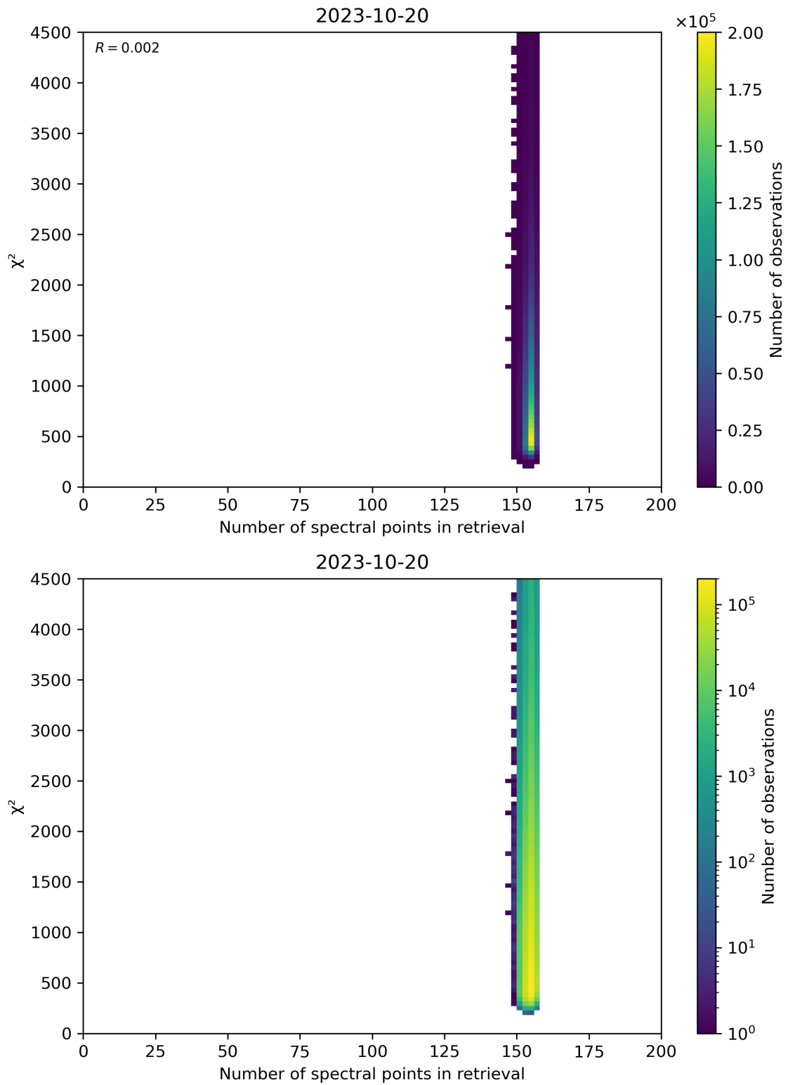
Figure 58: Scatter density plot of “Number of spectral points in retrieval” against “ \chi^2 ” for 2023-10-19 to 2023-10-21.
