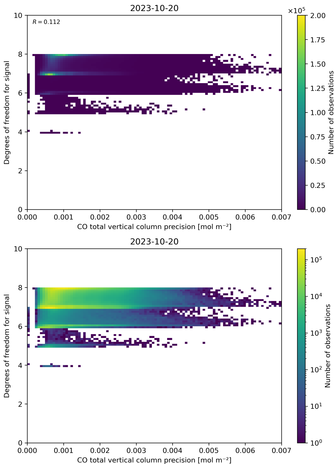
Figure 45: Scatter density plot of “CO total vertical column precision” against “Degrees of freedom for signal” for 2023-10-19 to 2023-10-21.
