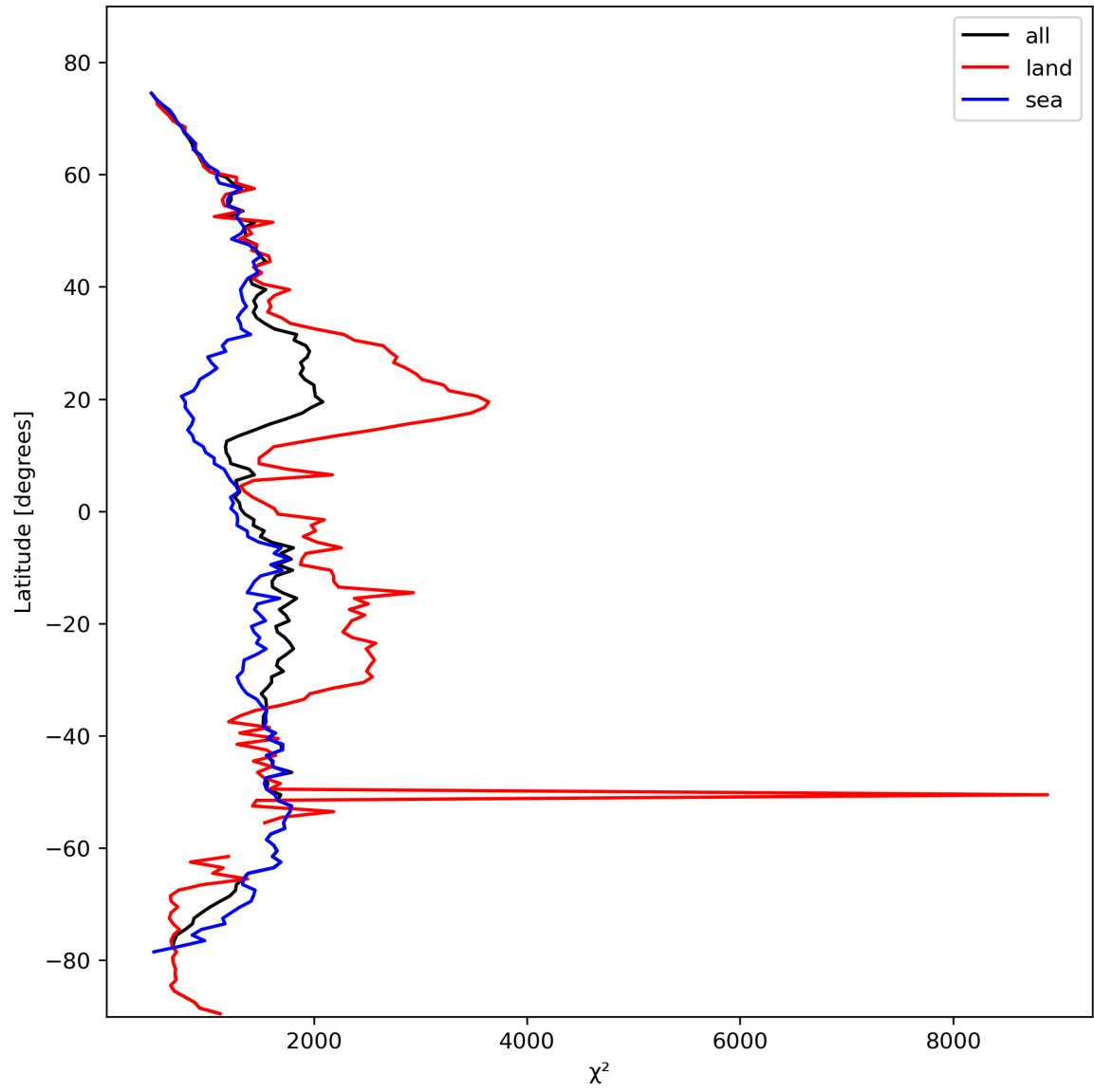
Figure 14: Zonal average of “ \chi^2 ” for 2023-10-19 to 2023-10-21.
