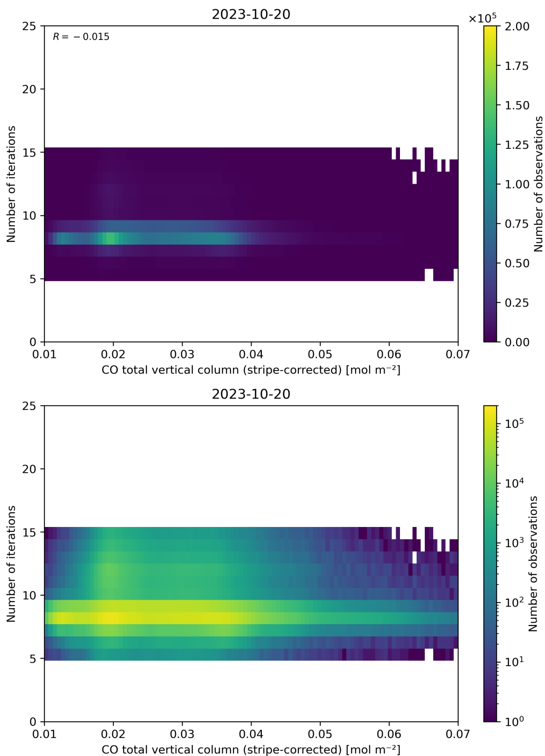
Figure 39: Scatter density plot of “CO total vertical column (stripe-corrected)” against “Number of iterations” for 2023-10-19 to 2023-10-21.
