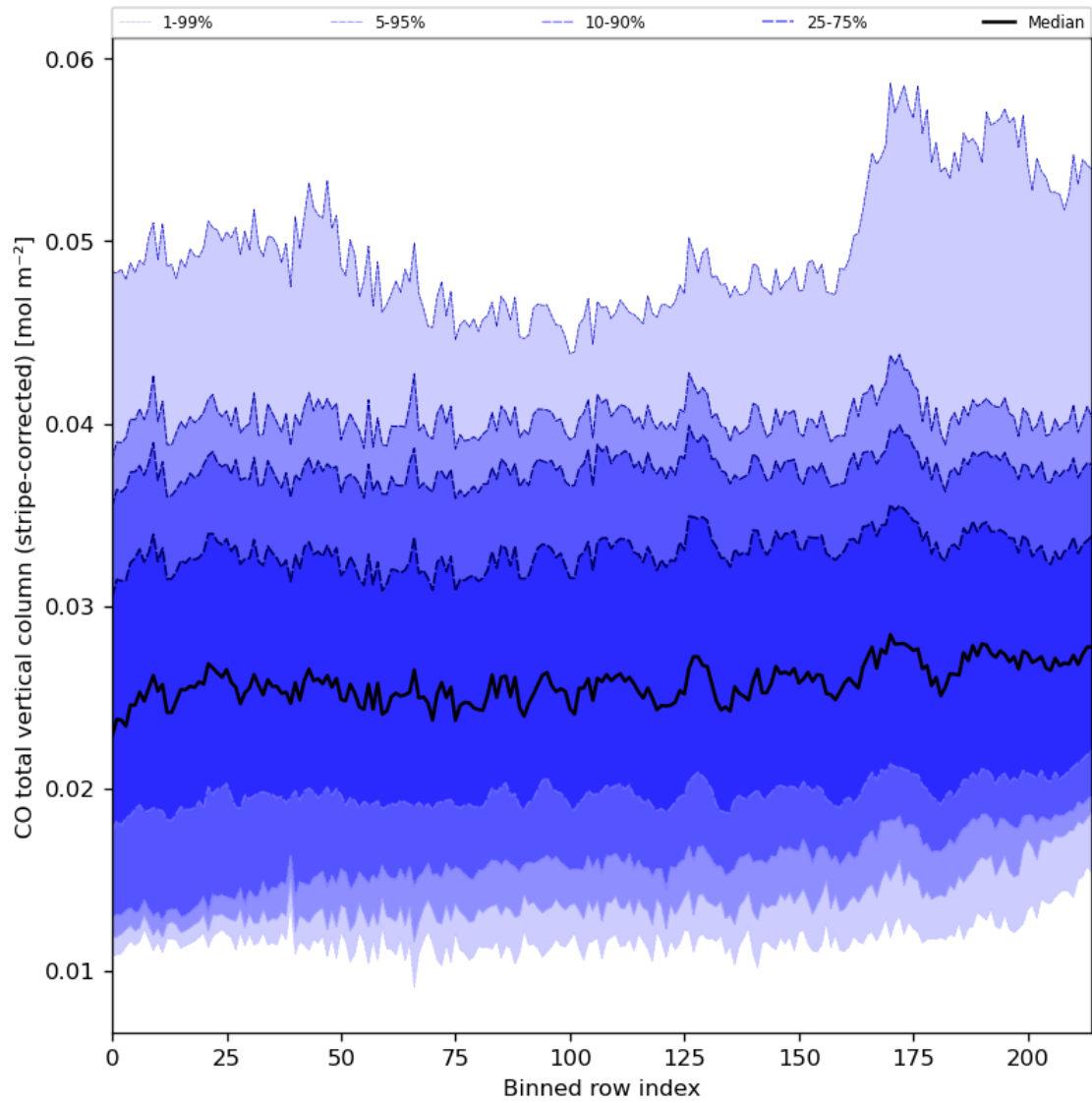
Figure 27: Along track statistics of “CO total vertical column (stripe-corrected)” for 2023-10-19 to 2023-10-21
