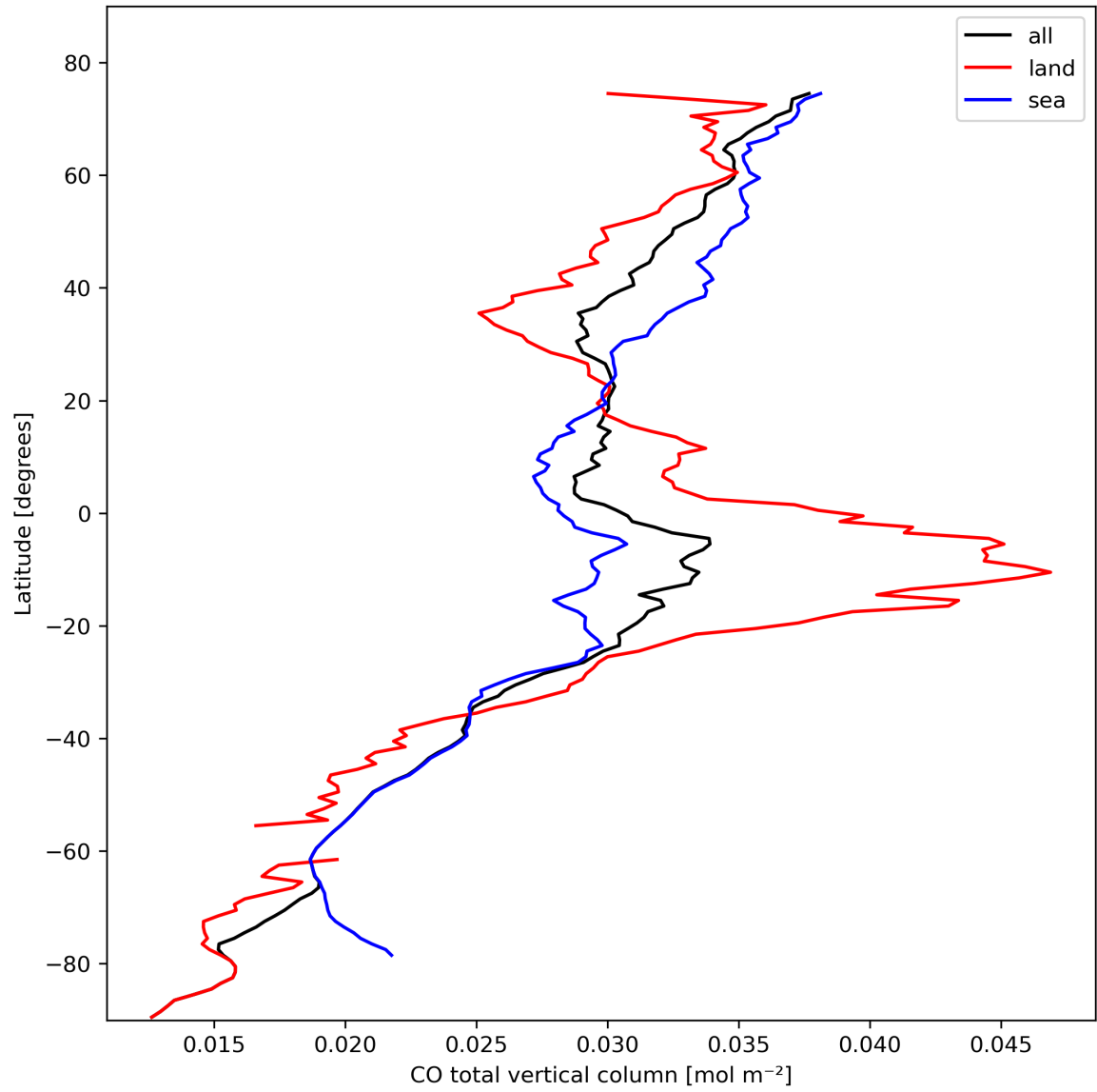
Figure 10: Zonal average of “CO total vertical column” for 2023-10-19 to 2023-10-21.
