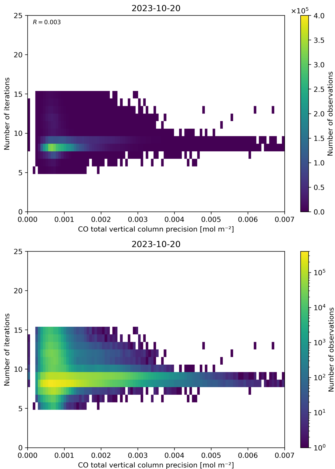
Figure 46: Scatter density plot of “CO total vertical column precision” against “Number of iterations” for 2023-10-19 to 2023-10-21.
