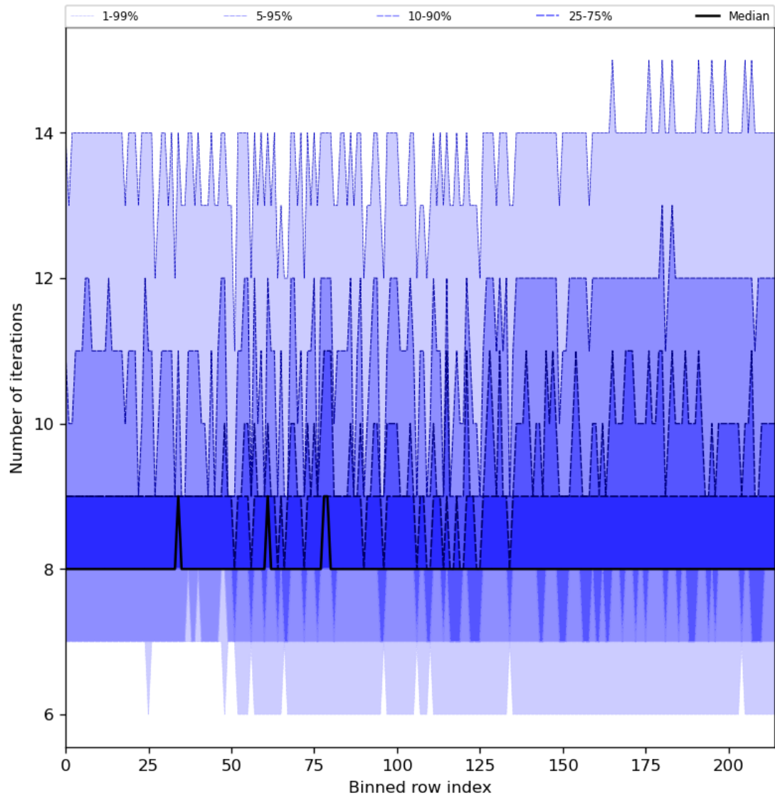
Figure 32: Along track statistics of “Number of iterations” for 2023-10-19 to 2023-10-21
