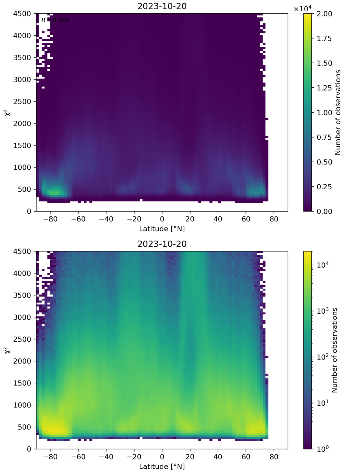
Figure 54: Scatter density plot of “Latitude” against “ \chi^2 ” for 2023-10-19 to 2023-10-21.
