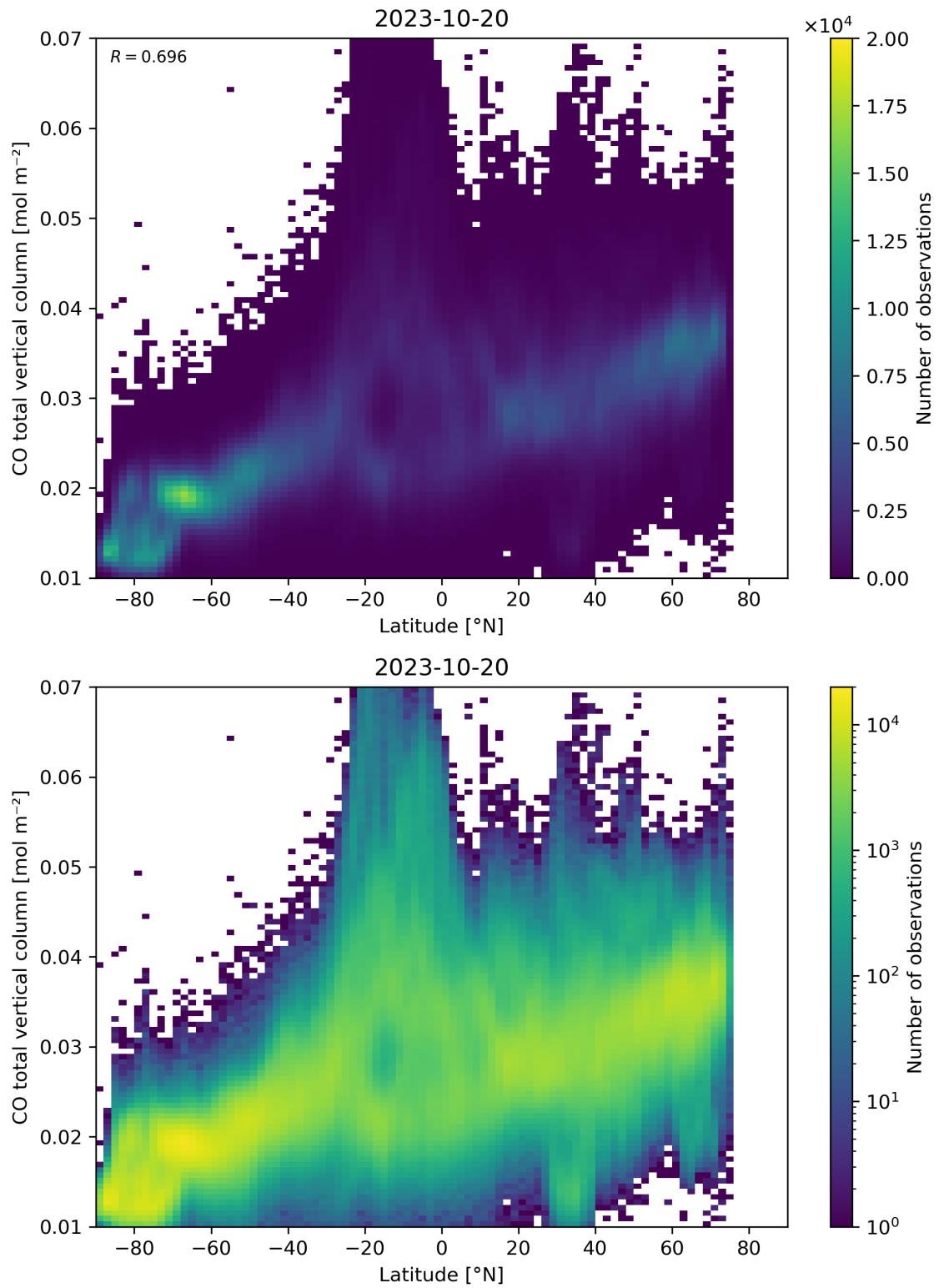
Figure 51: Scatter density plot of “Latitude” against “CO total vertical column” for 2023-10-19 to 2023-10-21.
