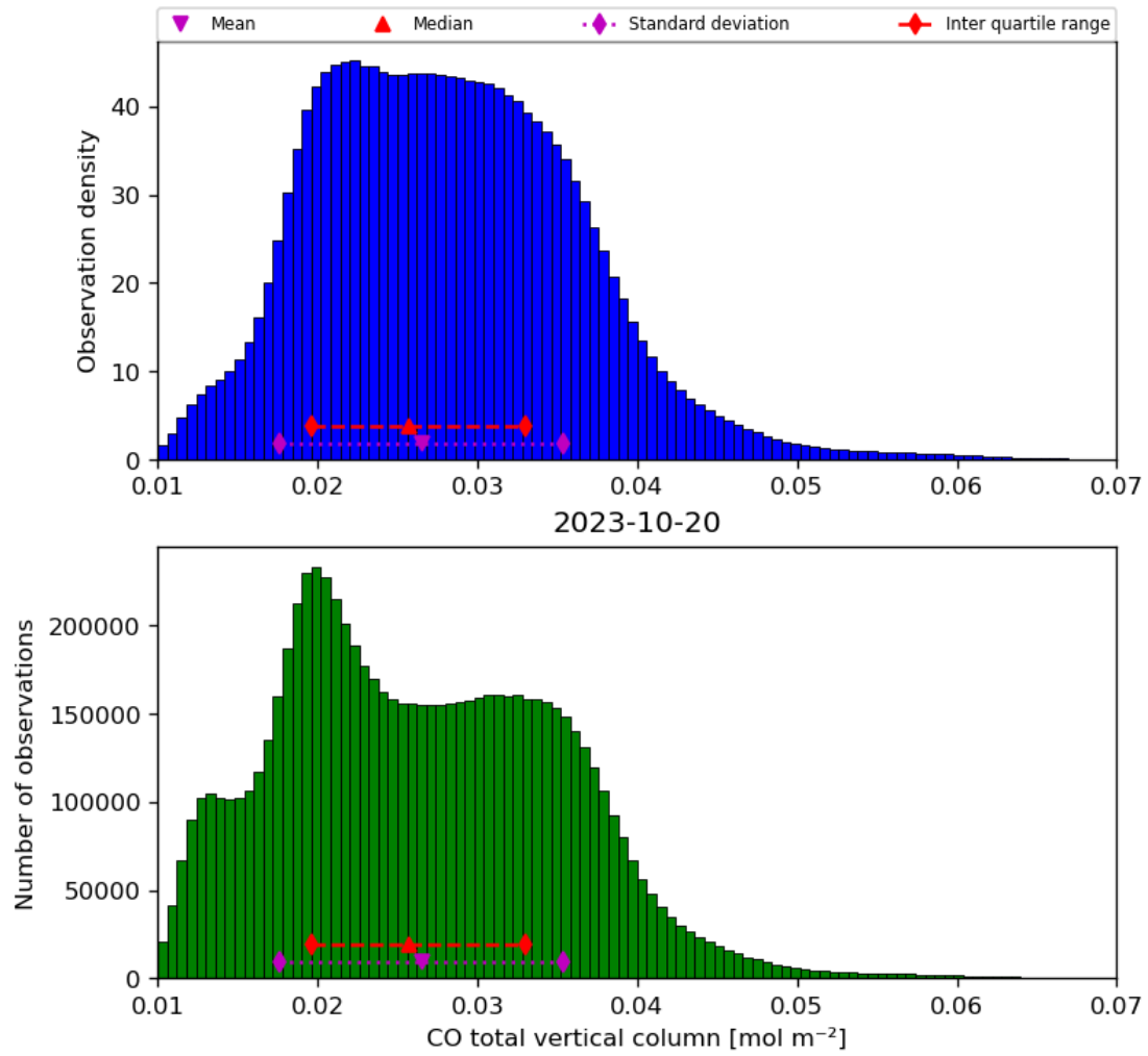
Figure 18: Histogram of “CO total vertical column” for 2023-10-19 to 2023-10-21
