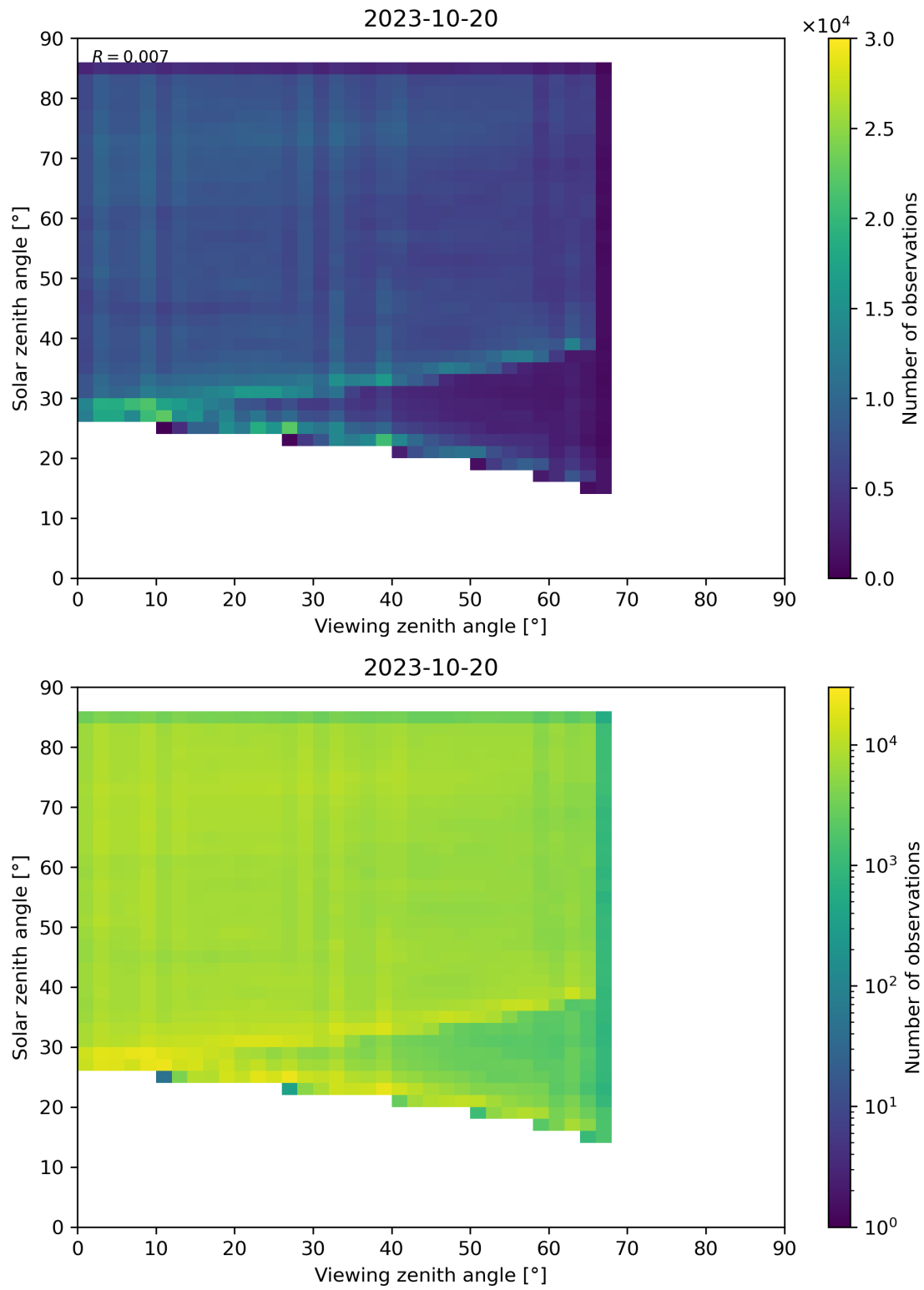
Figure 77: Scatter density plot of “Viewing zenith angle” against “Solar zenith angle” for 2023-10-19 to 2023-10-21.
