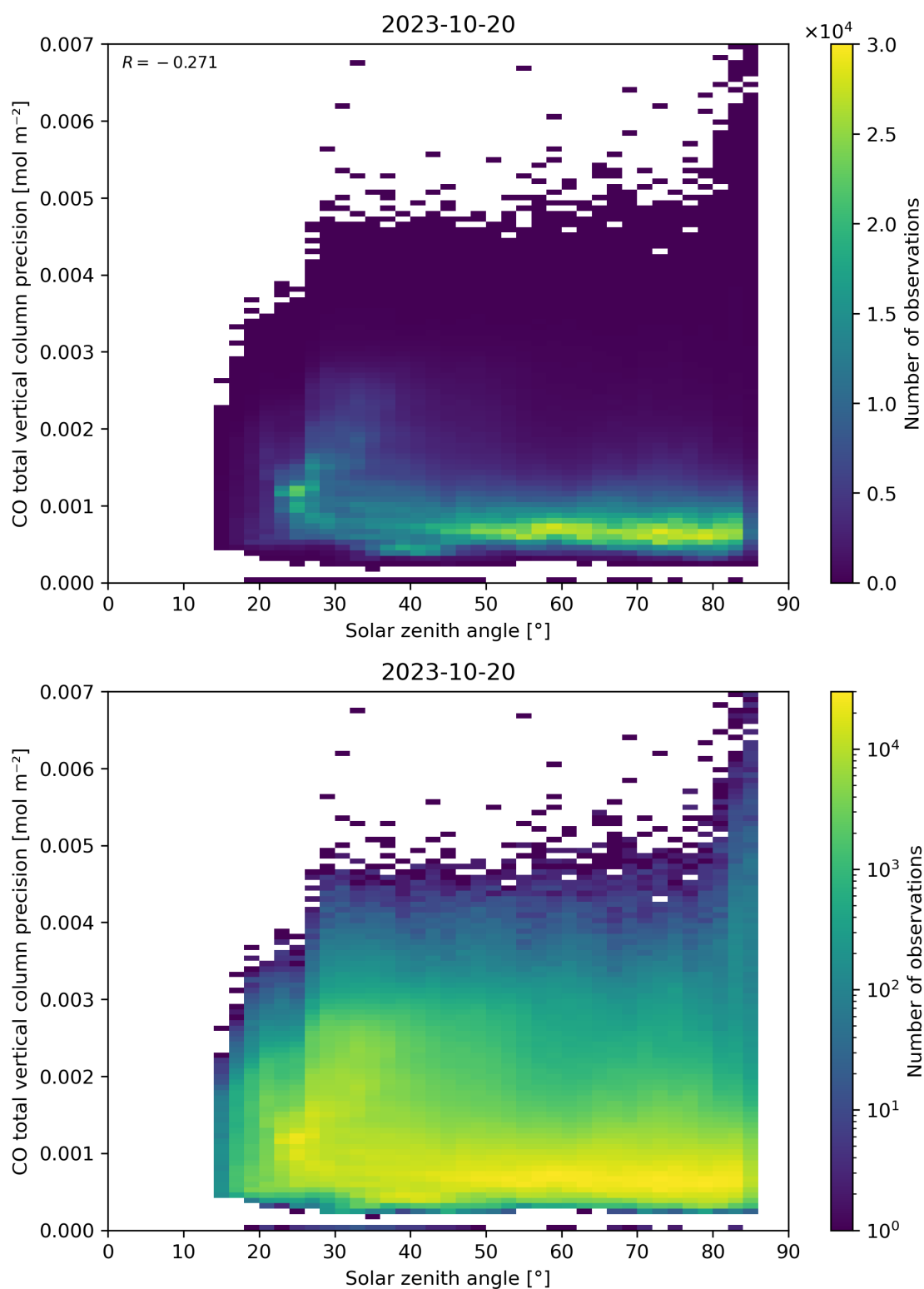
Figure 63: Scatter density plot of “Solar zenith angle” against “CO total vertical column precision” for 2023-10-19 to 2023-10-21.
