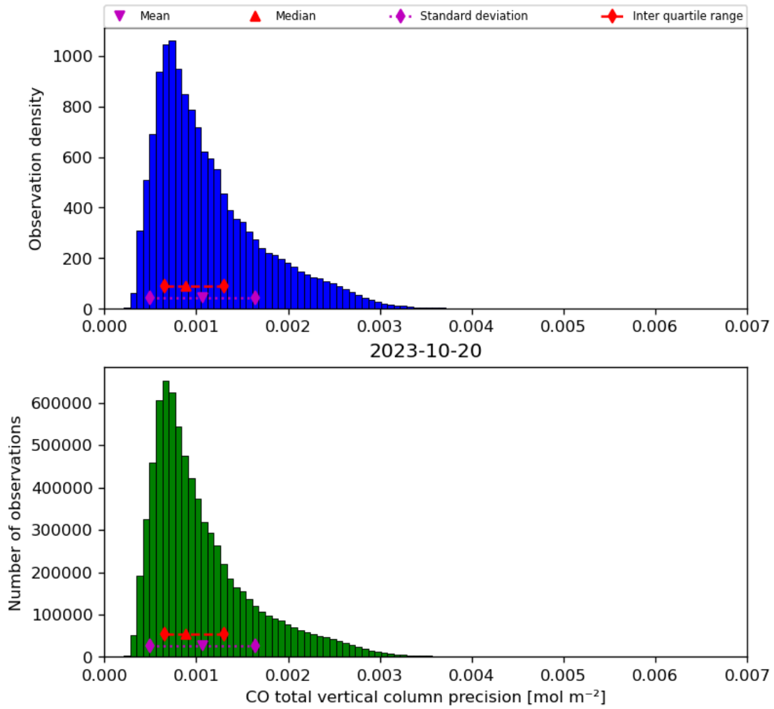
Figure 20: Histogram of “CO total vertical column precision” for 2023-10-19 to 2023-10-21
