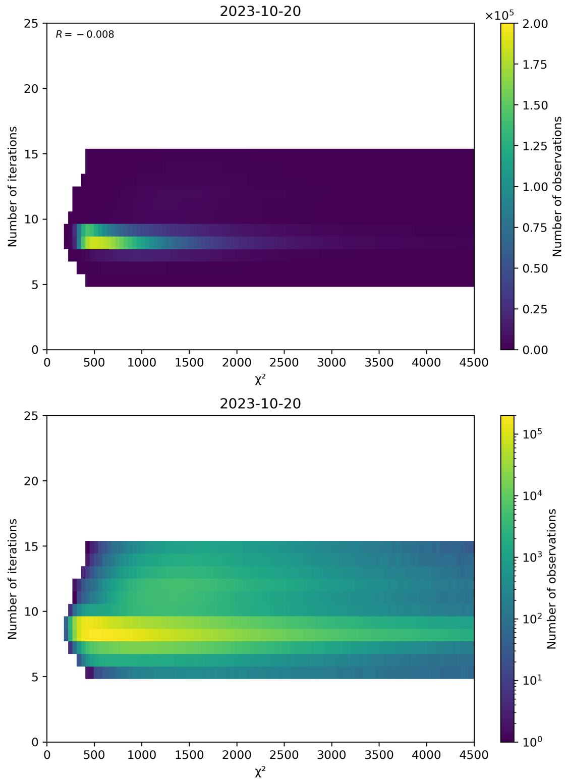
Figure 49: Scatter density plot of “ \chi^2 ” against “Number of iterations” for 2023-10-19 to 2023-10-21.
