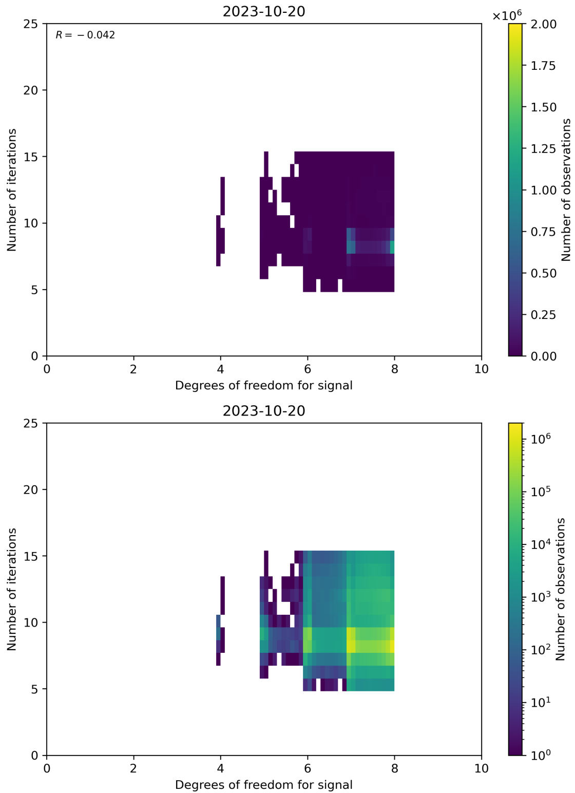
Figure 50: Scatter density plot of “Degrees of freedom for signal” against “Number of iterations” for 2023-10-19 to 2023-10-21.
