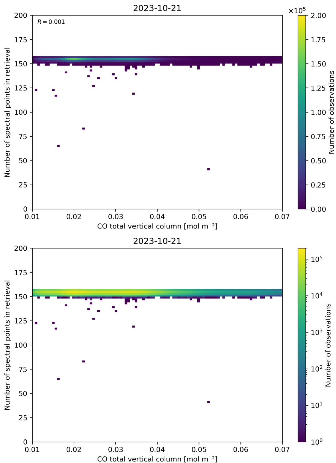
Figure 43: Scatter density plot of “CO total vertical column” against “Number of spectral points in retrieval” for 2023-10-20 to 2023-10-22.
