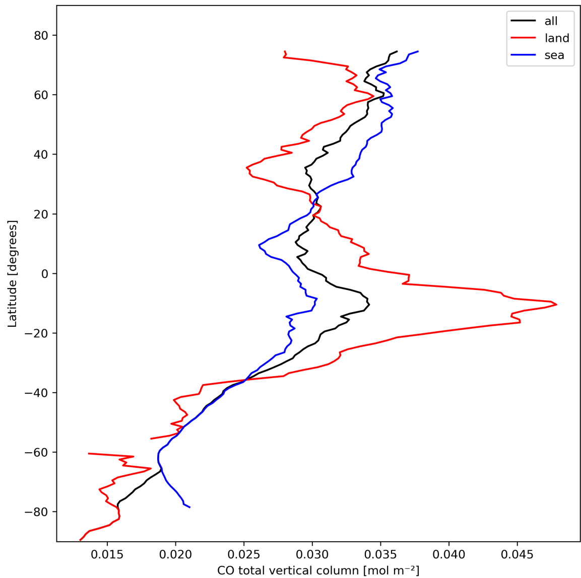
Figure 10: Zonal average of “CO total vertical column” for 2023-10-20 to 2023-10-22.
