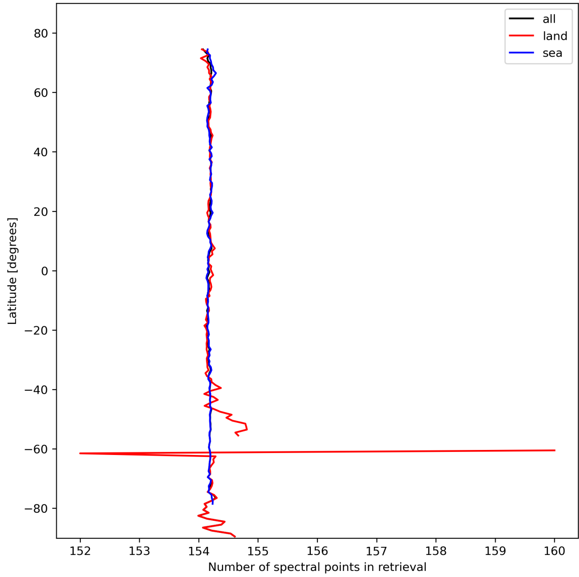
Figure 13: Zonal average of “Number of spectral points in retrieval” for 2023-10-20 to 2023-10-22.
