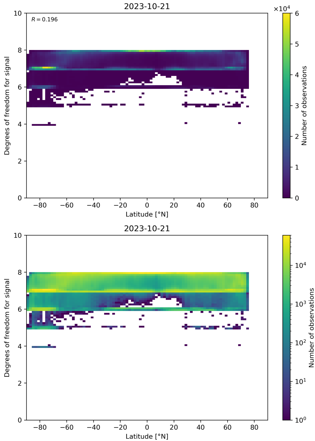
Figure 55: Scatter density plot of “Latitude” against “Degrees of freedom for signal” for 2023-10-20 to 2023-10-22.
