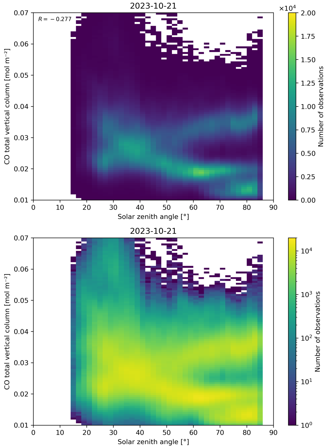
Figure 61: Scatter density plot of “Solar zenith angle” against “CO total vertical column” for 2023-10-20 to 2023-10-22.
