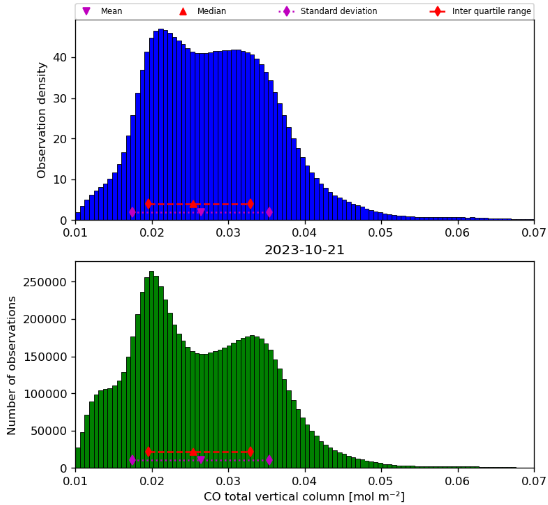
Figure 18: Histogram of “CO total vertical column” for 2023-10-20 to 2023-10-22
