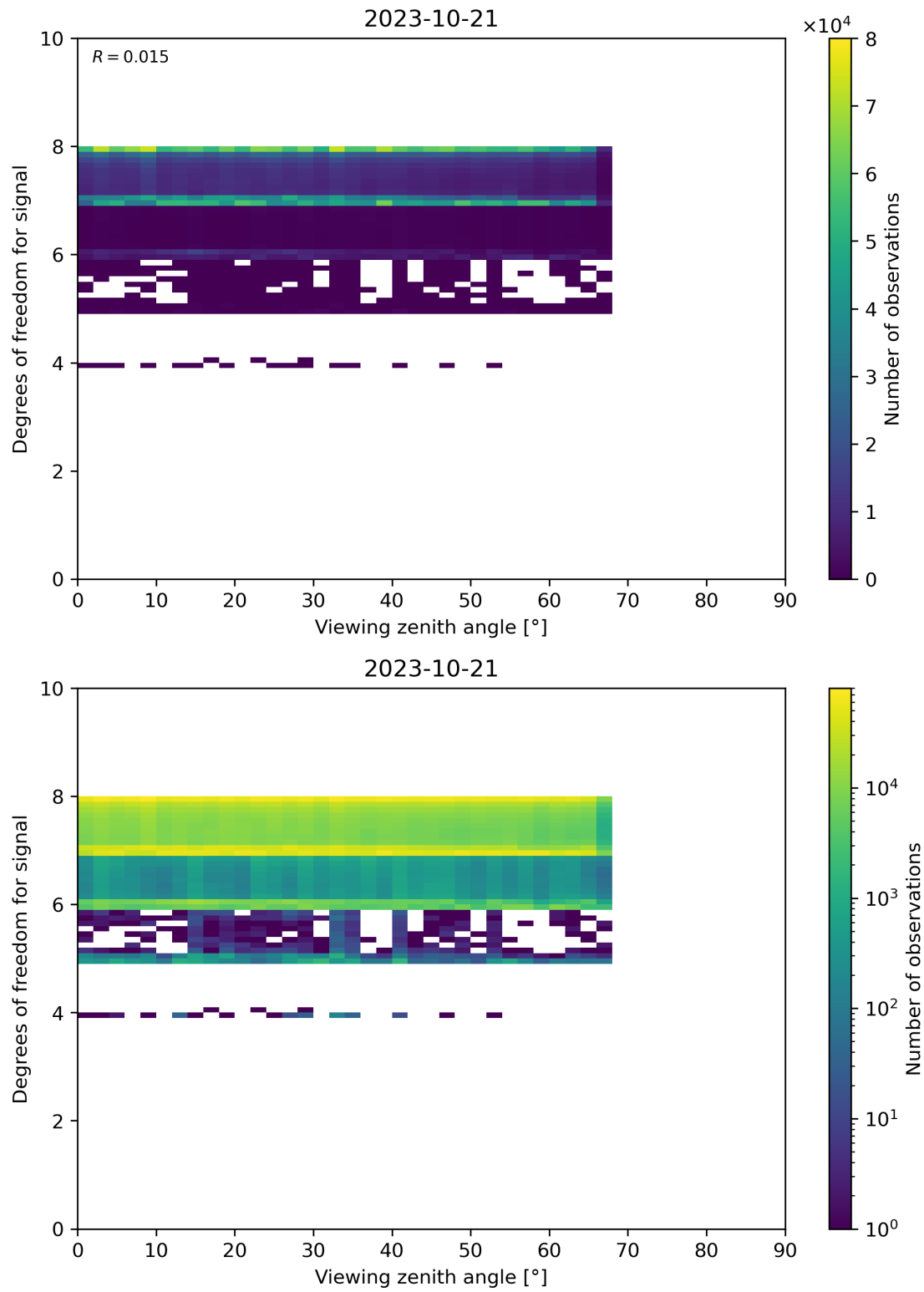
Figure 73: Scatter density plot of “Viewing zenith angle” against “Degrees of freedom for signal” for 2023-10-20 to 2023-10-22.
