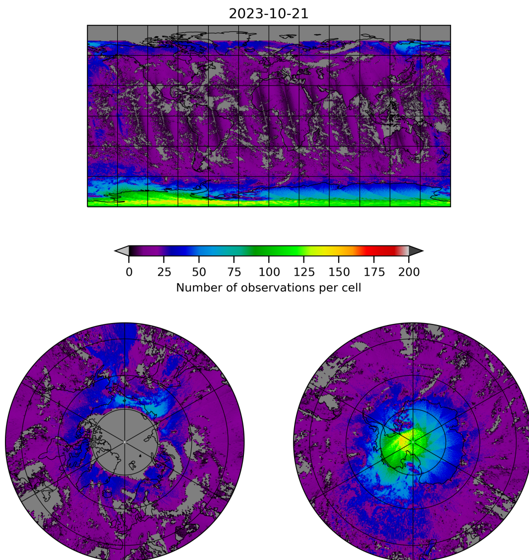
Figure 8: Map of the number of observations for 2023-10-20 to 2023-10-22
