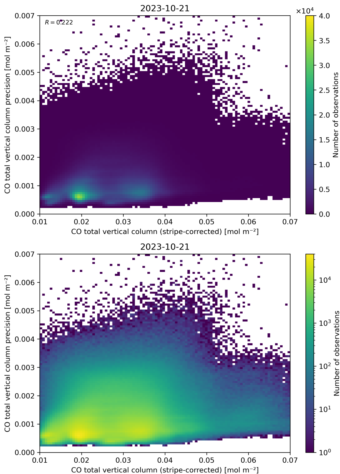
Figure 36: Scatter density plot of “CO total vertical column (stripe-corrected)” against “CO total vertical column precision” for 2023-10-20 to 2023-10-22.
