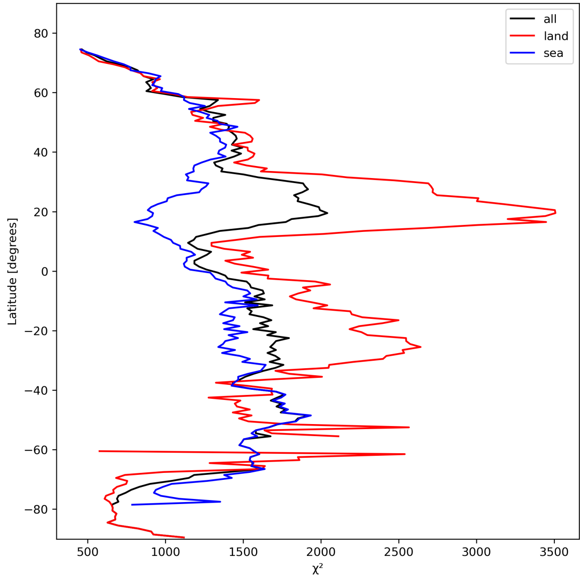
Figure 14: Zonal average of “ \chi^2 ” for 2023-10-20 to 2023-10-22.
