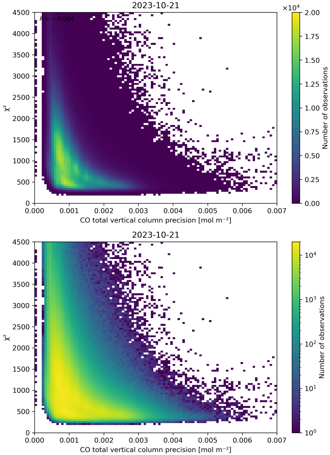
Figure 44: Scatter density plot of “CO total vertical column precision” against “ \chi^2 ” for 2023-10-20 to 2023-10-22.
