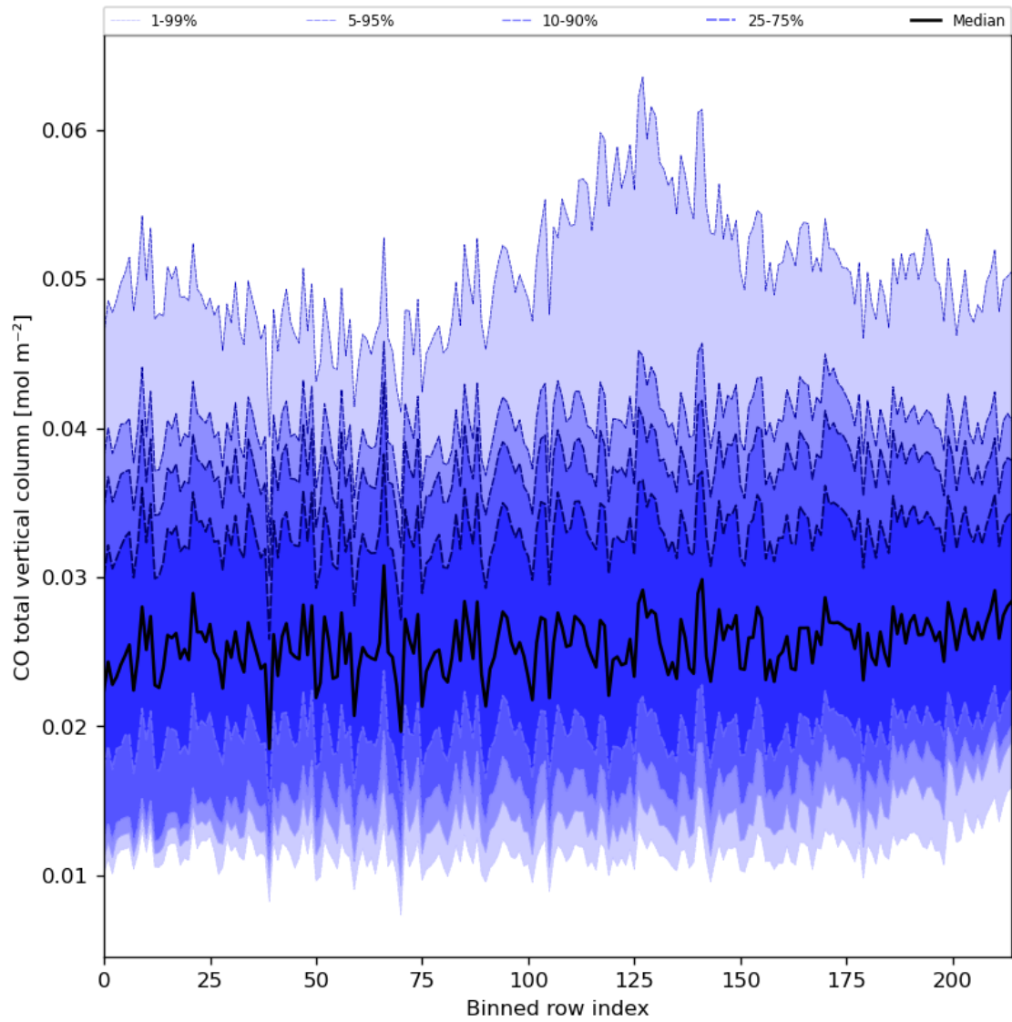
Figure 26: Along track statistics of “CO total vertical column” for 2023-10-20 to 2023-10-22
