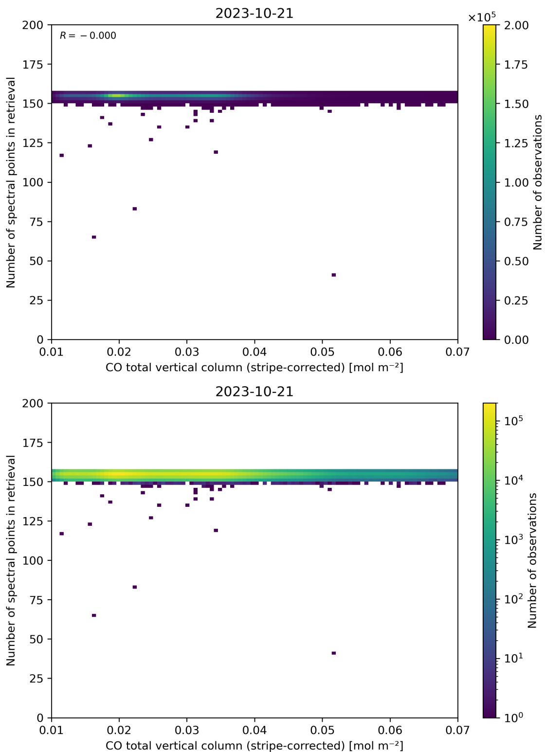
Figure 40: Scatter density plot of “CO total vertical column (stripe-corrected)” against “Number of spectral points in retrieval” for 2023-10-20 to 2023-10-22.
