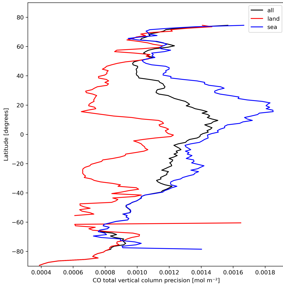
Figure 12: Zonal average of “CO total vertical column precision” for 2023-10-20 to 2023-10-22.
