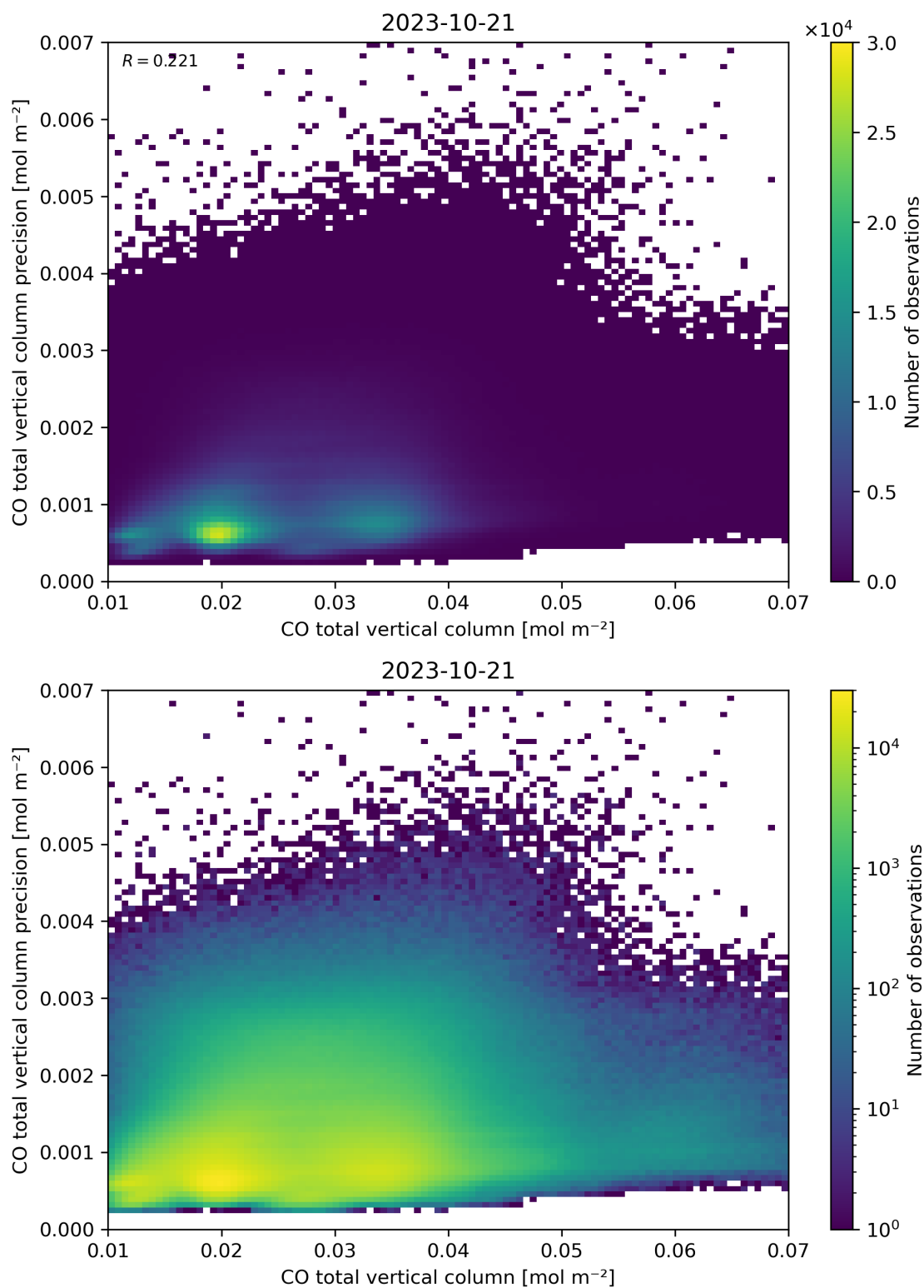
Figure 34: Scatter density plot of “CO total vertical column” against “CO total vertical column precision” for 2023-10-20 to 2023-10-22.
