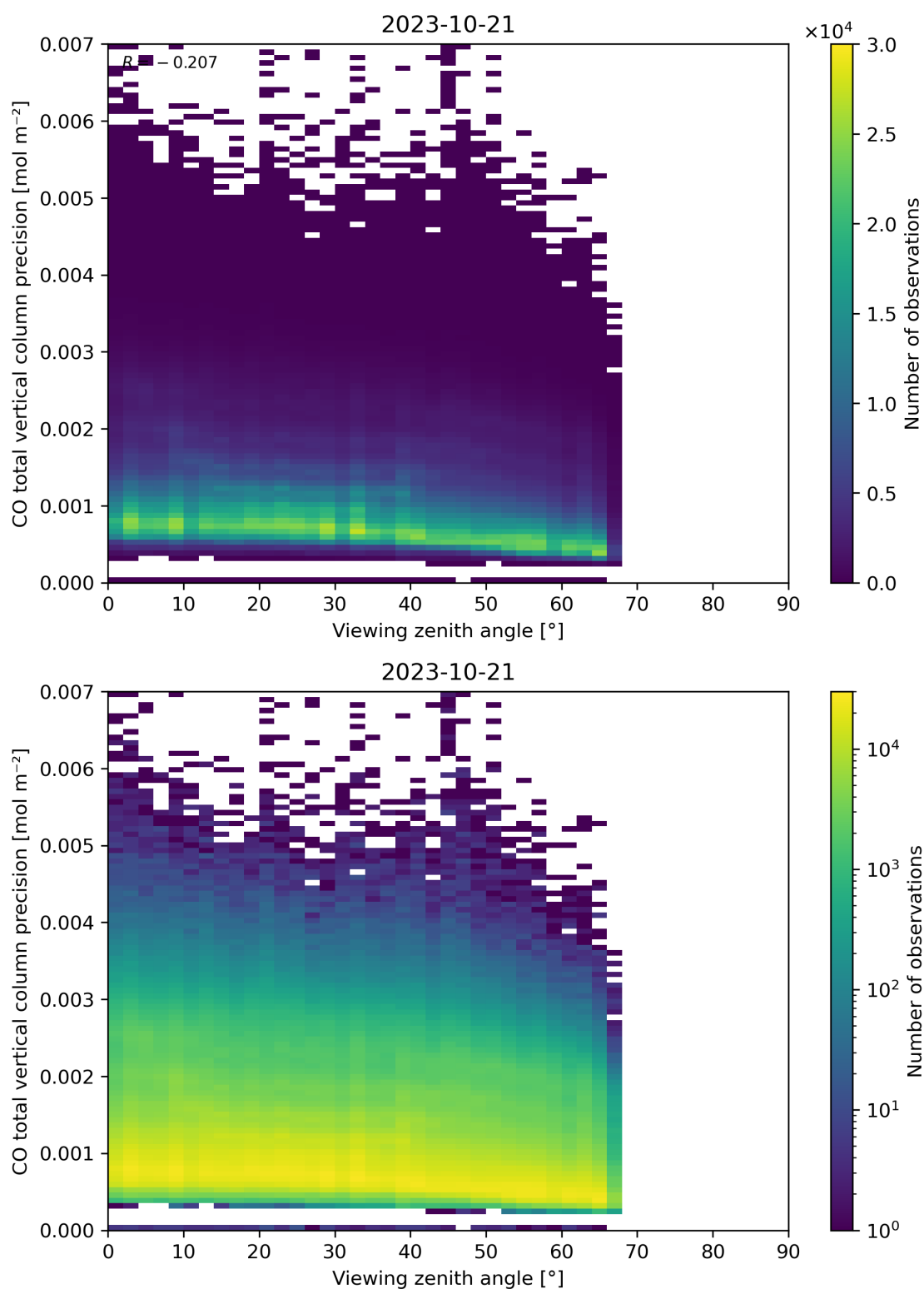
Figure 71: Scatter density plot of “Viewing zenith angle” against “CO total vertical column precision” for 2023-10-20 to 2023-10-22.
