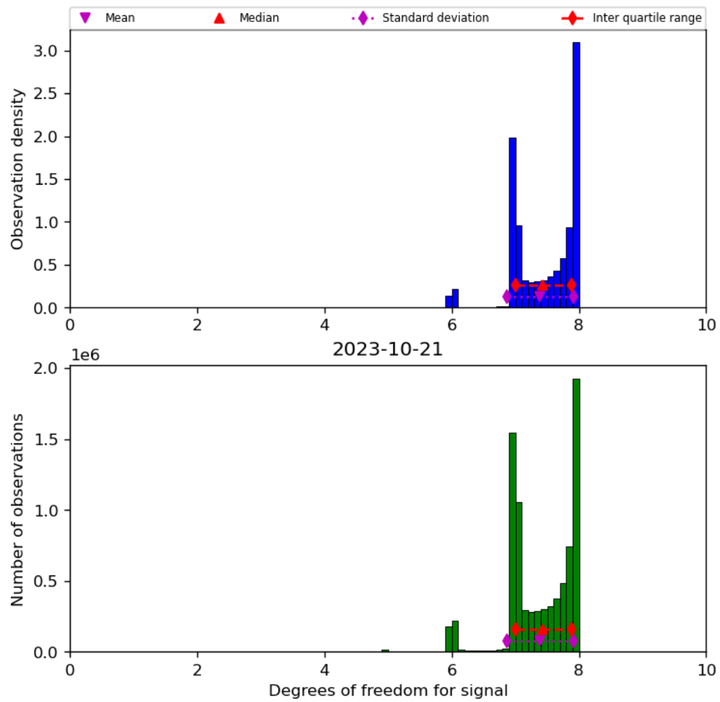
Figure 23: Histogram of “Degrees of freedom for signal” for 2023-10-20 to 2023-10-22
