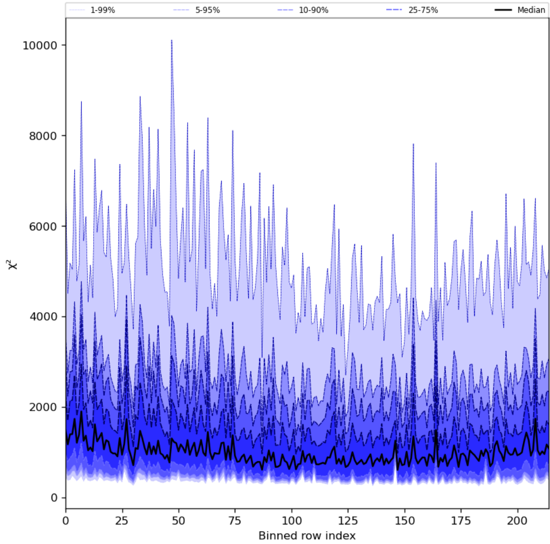
Figure 30: Along track statistics of “ \chi^2 ” for 2023-10-20 to 2023-10-22
