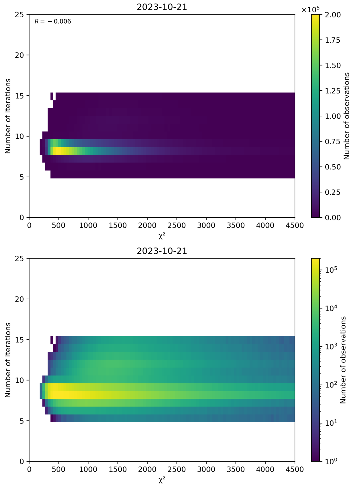
Figure 49: Scatter density plot of “ \chi^2 ” against “Number of iterations” for 2023-10-20 to 2023-10-22.
