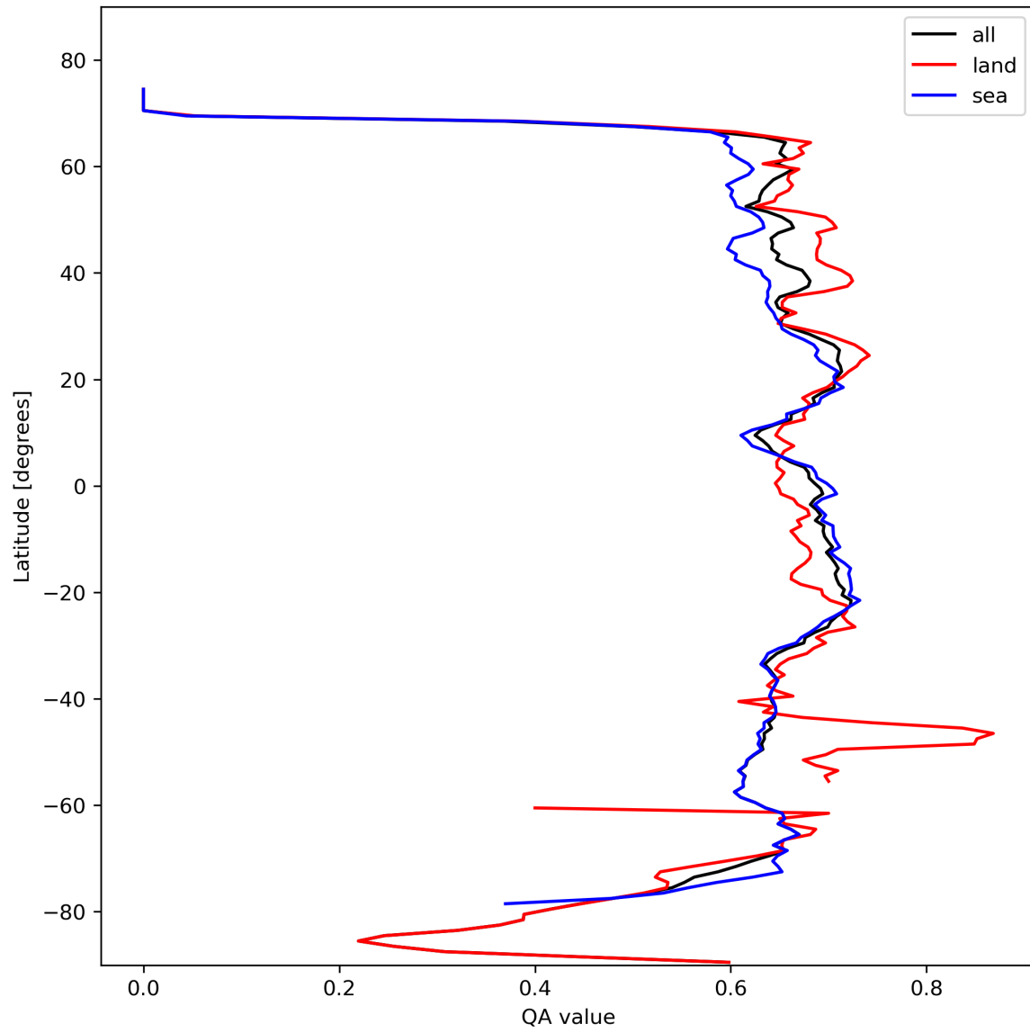
Figure 9: Zonal average of “QA value” for 2023-10-20 to 2023-10-22.
