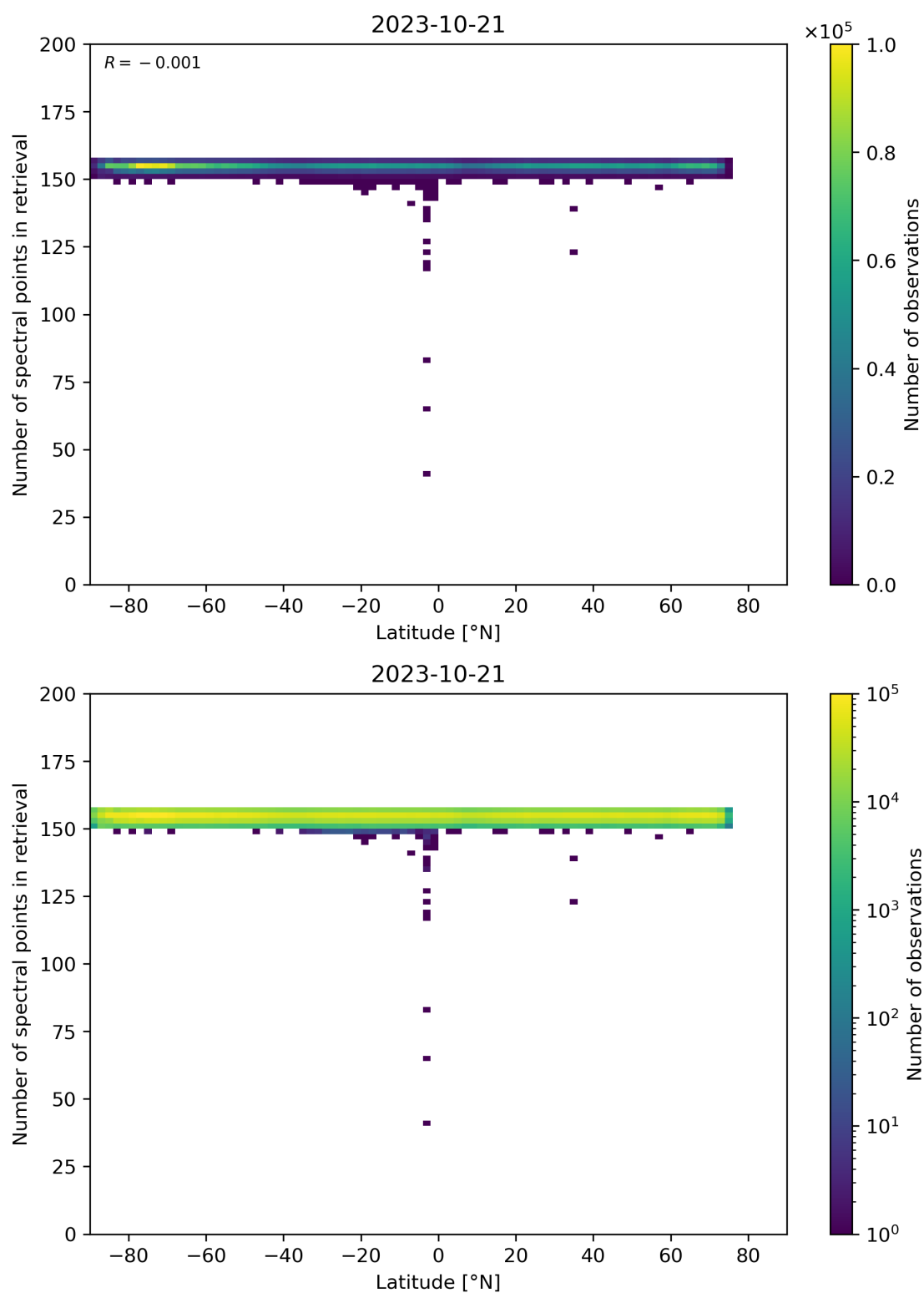
Figure 57: Scatter density plot of “Latitude” against “Number of spectral points in retrieval” for 2023-10-20 to 2023-10-22.
