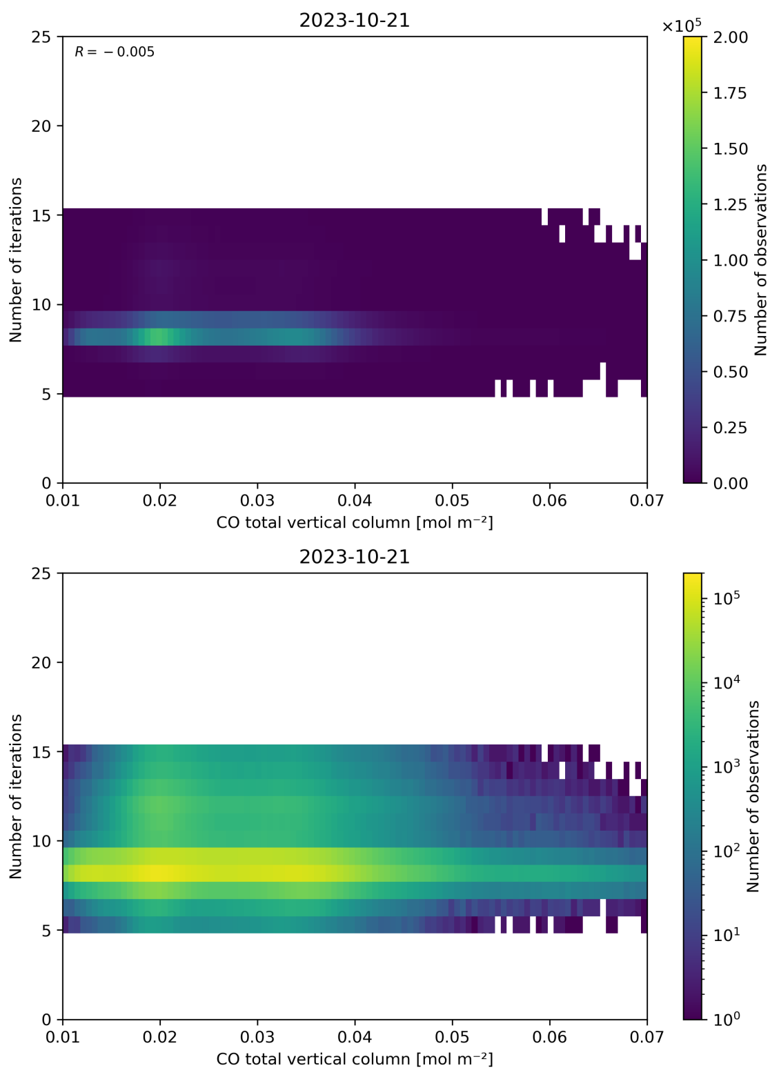
Figure 42: Scatter density plot of “CO total vertical column” against “Number of iterations” for 2023-10-20 to 2023-10-22.
