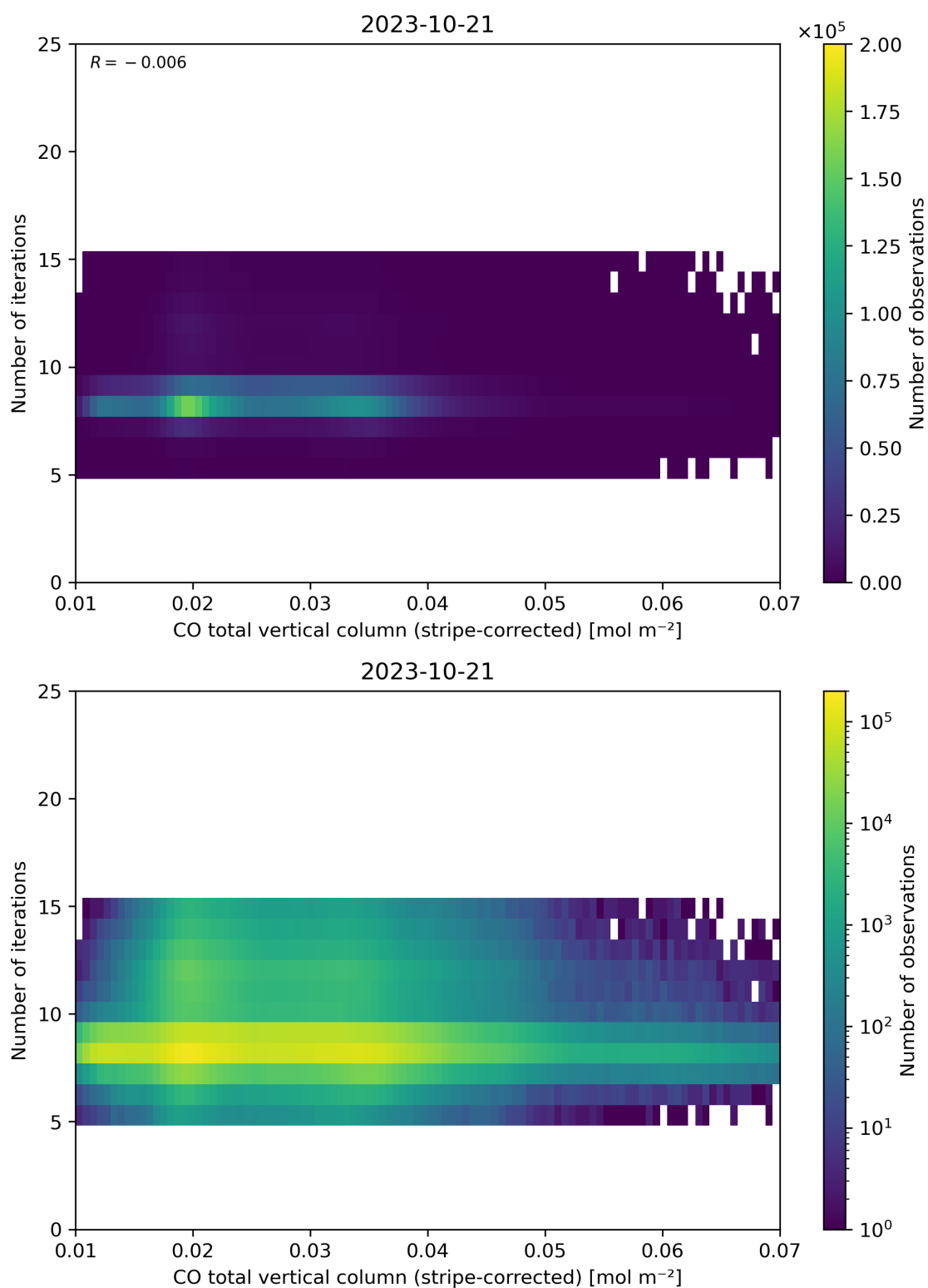
Figure 39: Scatter density plot of “CO total vertical column (stripe-corrected)” against “Number of iterations” for 2023-10-20 to 2023-10-22.
