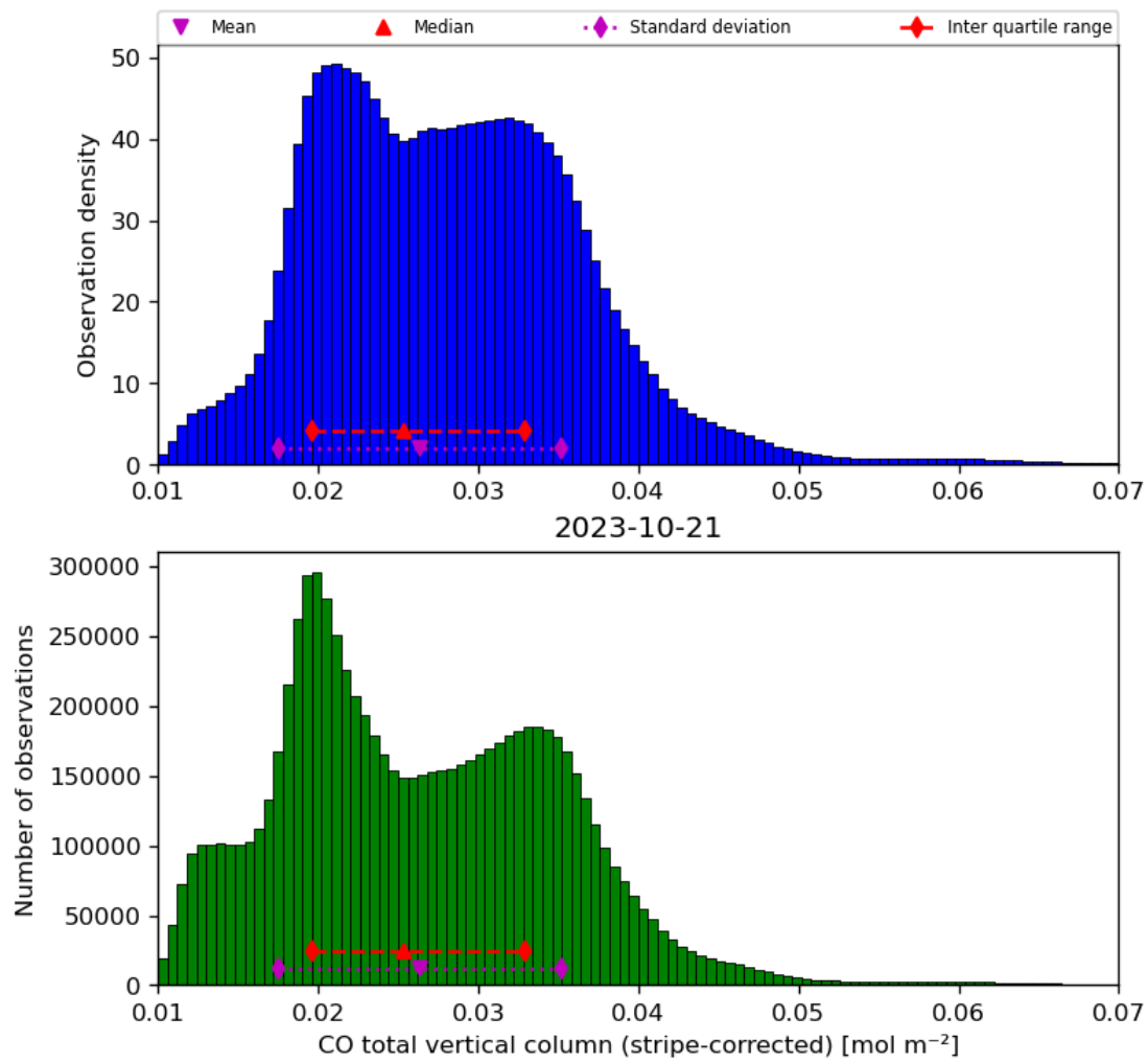
Figure 19: Histogram of “CO total vertical column (stripe-corrected)” for 2023-10-20 to 2023-10-22
