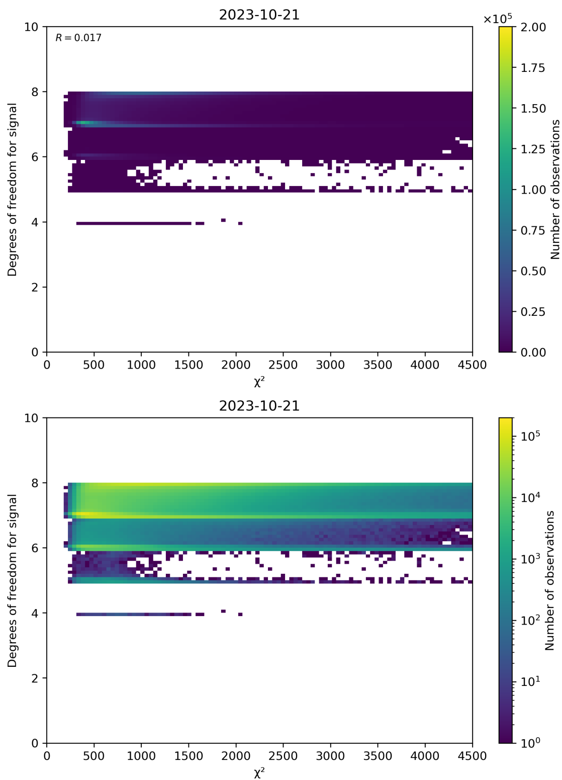
Figure 48: Scatter density plot of “ \chi^2 ” against “Degrees of freedom for signal” for 2023-10-20 to 2023-10-22.
