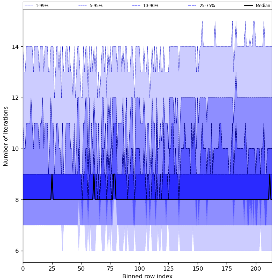
Figure 32: Along track statistics of “Number of iterations” for 2023-10-20 to 2023-10-22
