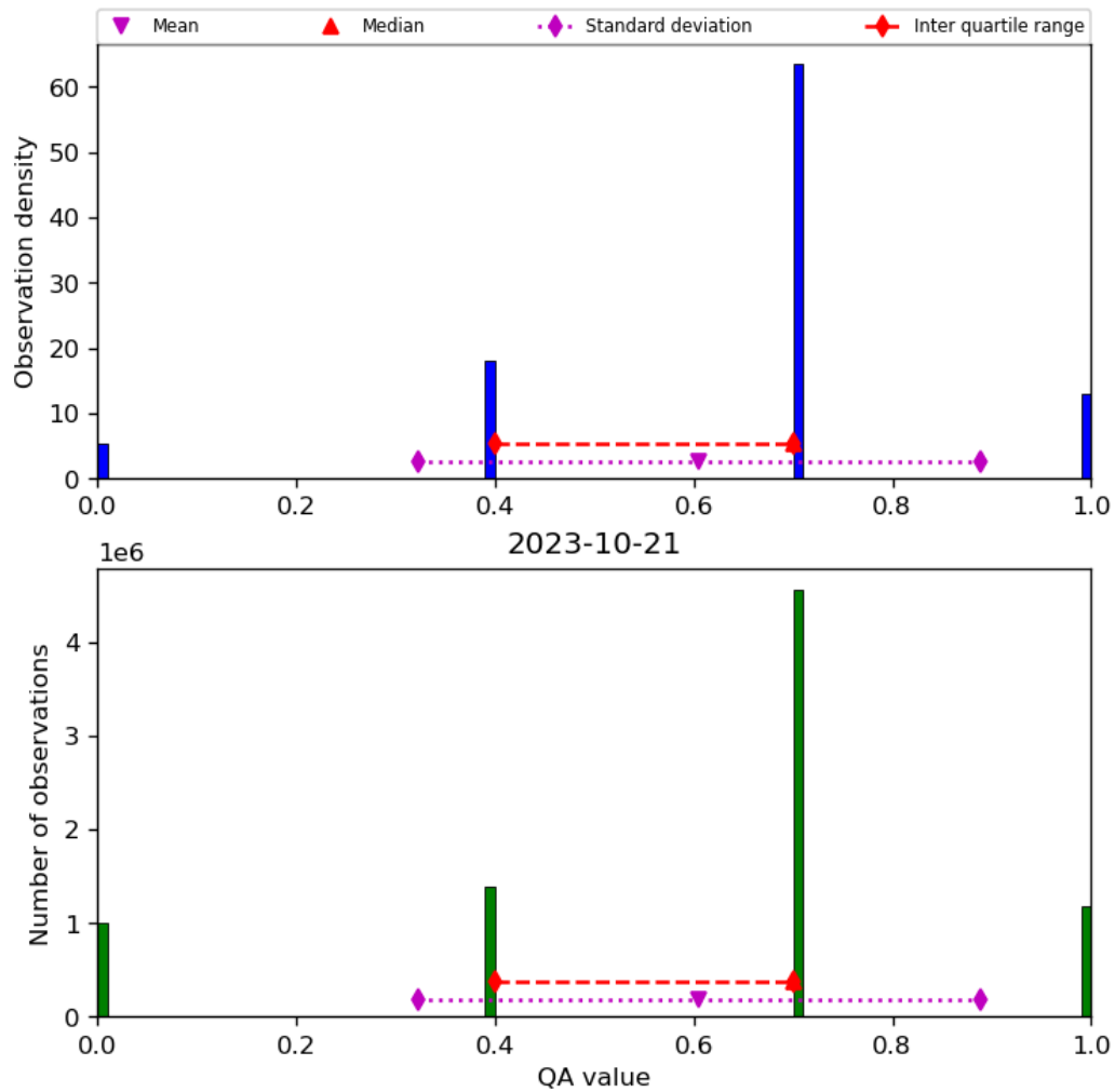
Figure 17: Histogram of “QA value” for 2023-10-20 to 2023-10-22
