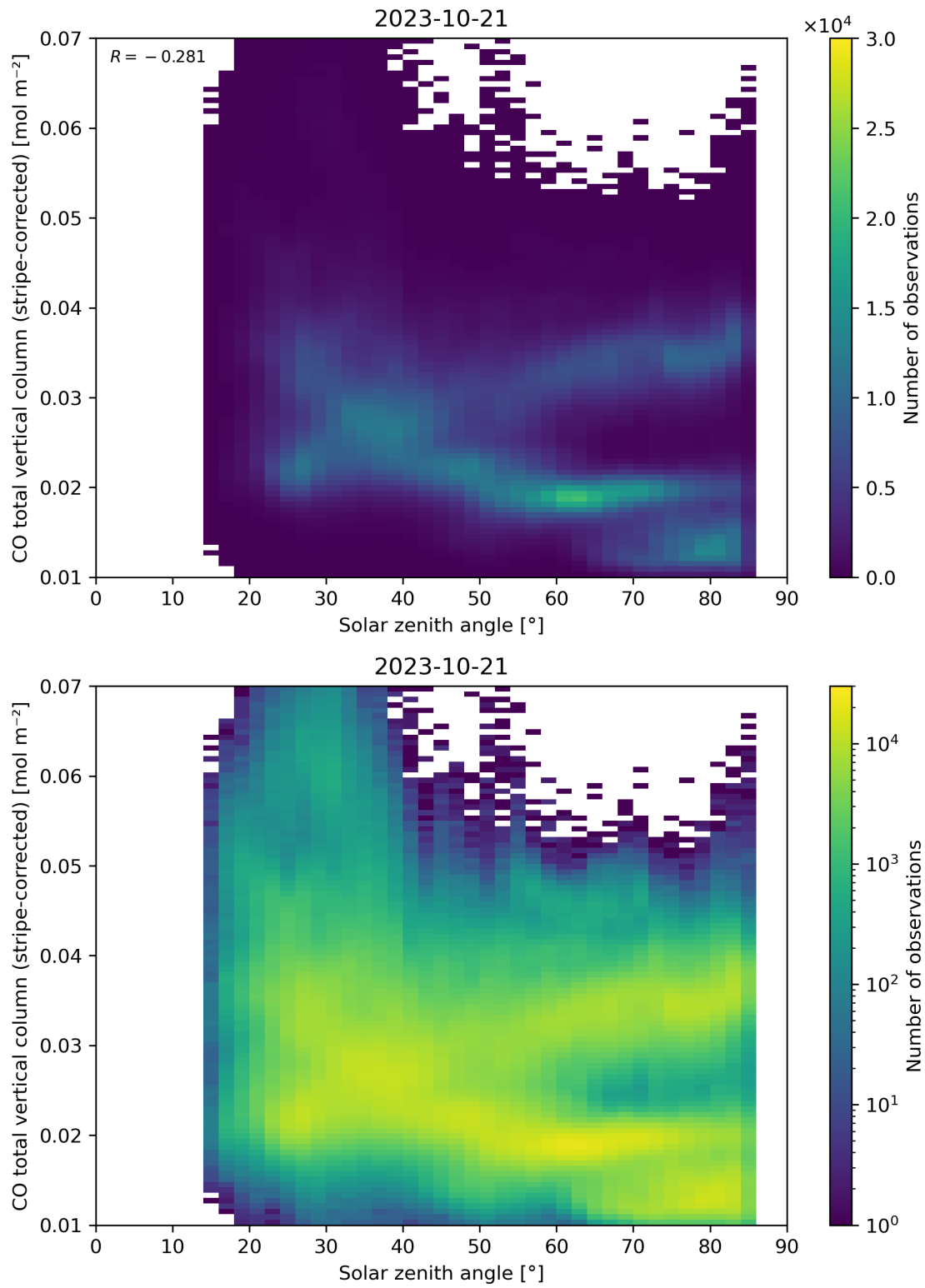
Figure 62: Scatter density plot of “Solar zenith angle” against “CO total vertical column (stripe-corrected)” for 2023-10-20 to 2023-10-22.
