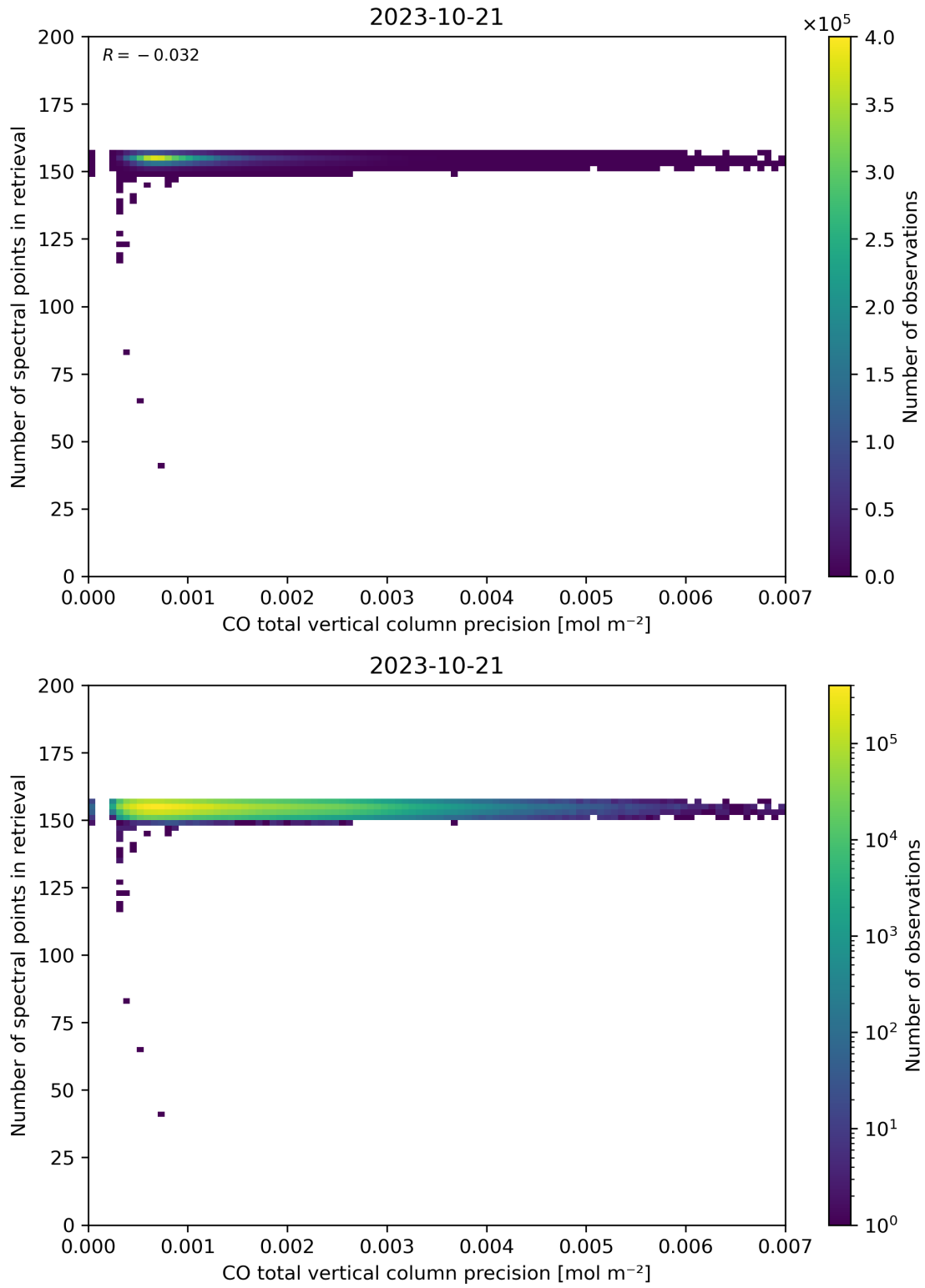
Figure 47: Scatter density plot of “CO total vertical column precision” against “Number of spectral points in retrieval” for 2023-10-20 to 2023-10-22.
