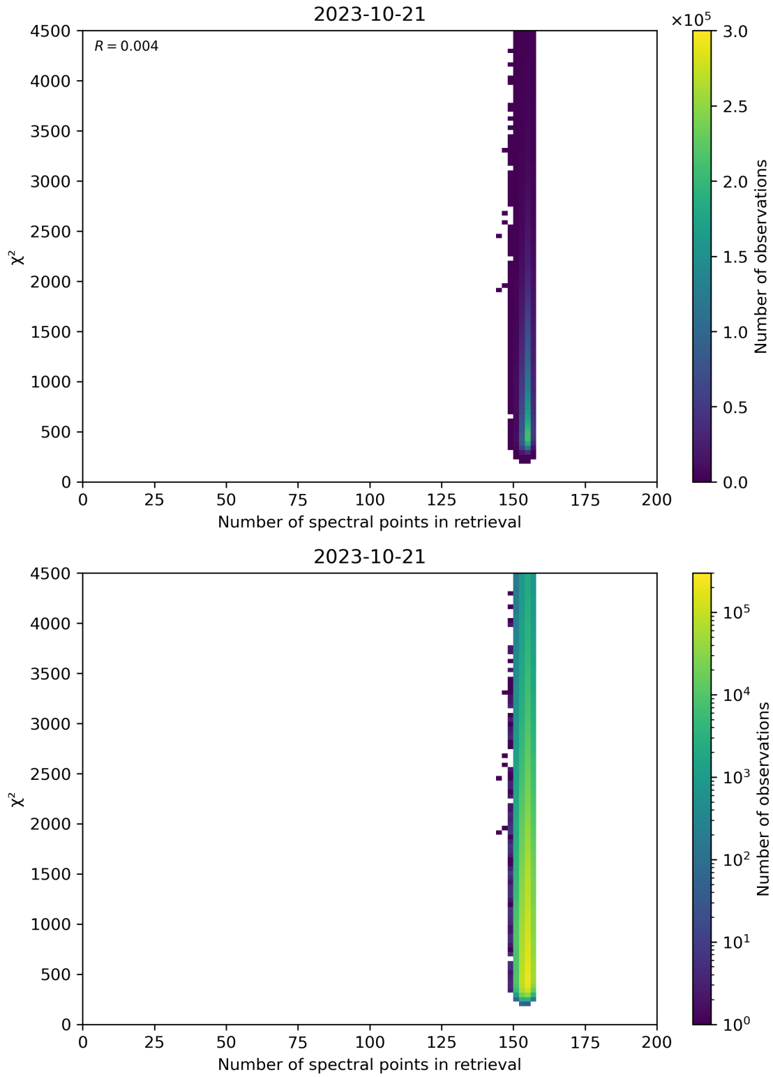
Figure 58: Scatter density plot of “Number of spectral points in retrieval” against “ \chi^2 ” for 2023-10-20 to 2023-10-22.
