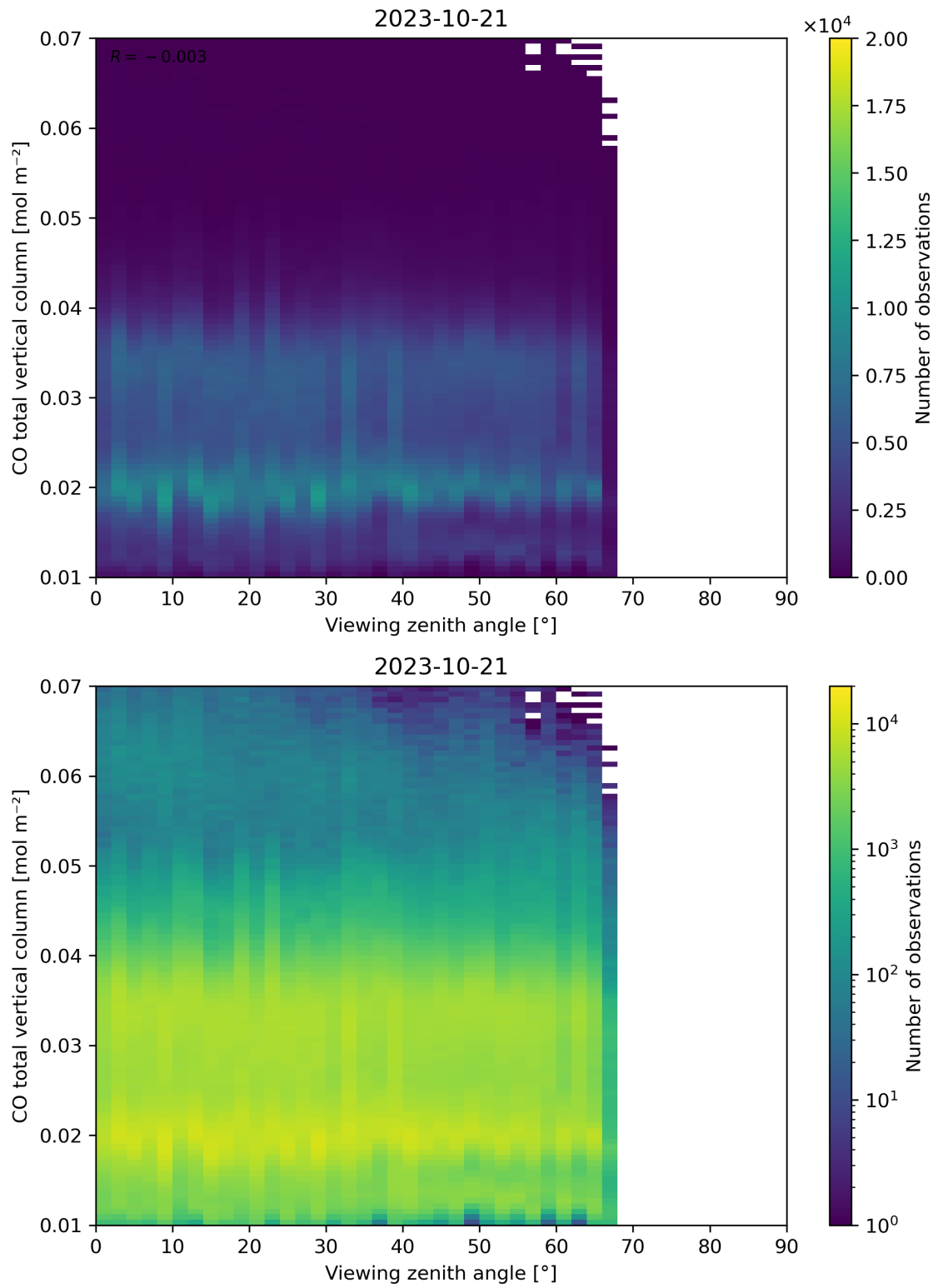
Figure 69: Scatter density plot of “Viewing zenith angle” against “CO total vertical column” for 2023-10-20 to 2023-10-22.
