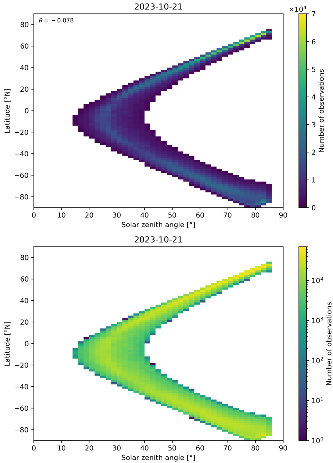
Figure 66: Scatter density plot of “Solar zenith angle” against “Latitude” for 2023-10-20 to 2023-10-22.
