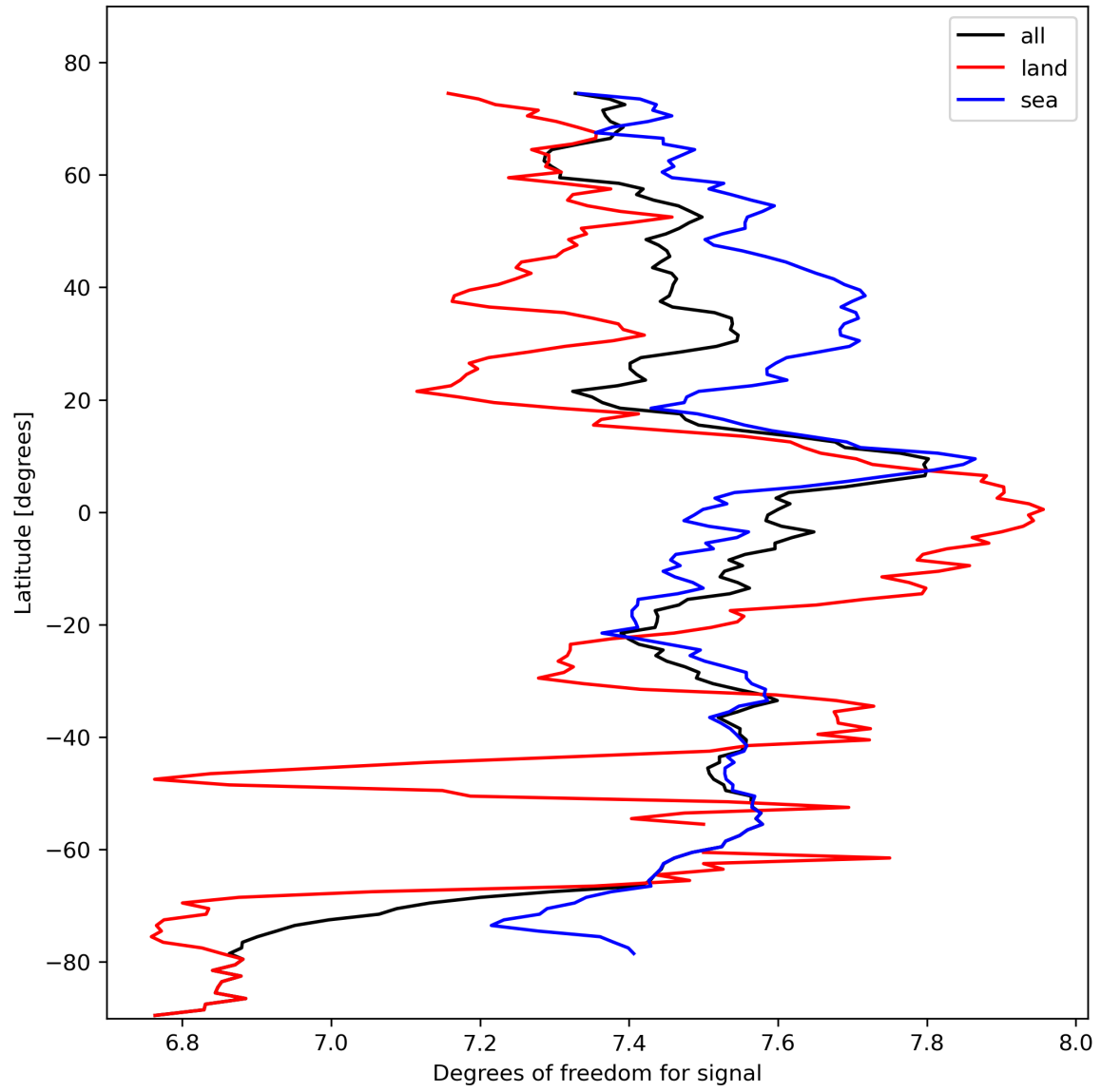
Figure 15: Zonal average of “Degrees of freedom for signal” for 2023-10-20 to 2023-10-22.
