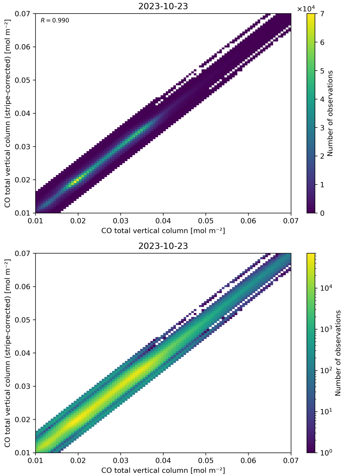
Figure 33: Scatter density plot of “CO total vertical column” against “CO total vertical column (stripe-corrected)” for 2023-10-22 to 2023-10-24.
