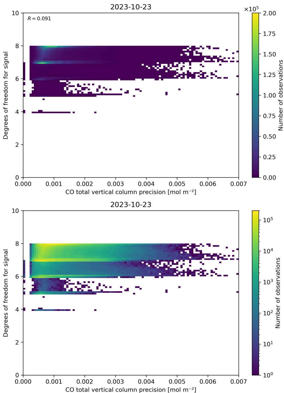
Figure 45: Scatter density plot of “CO total vertical column precision” against “Degrees of freedom for signal” for 2023-10-22 to 2023-10-24.
