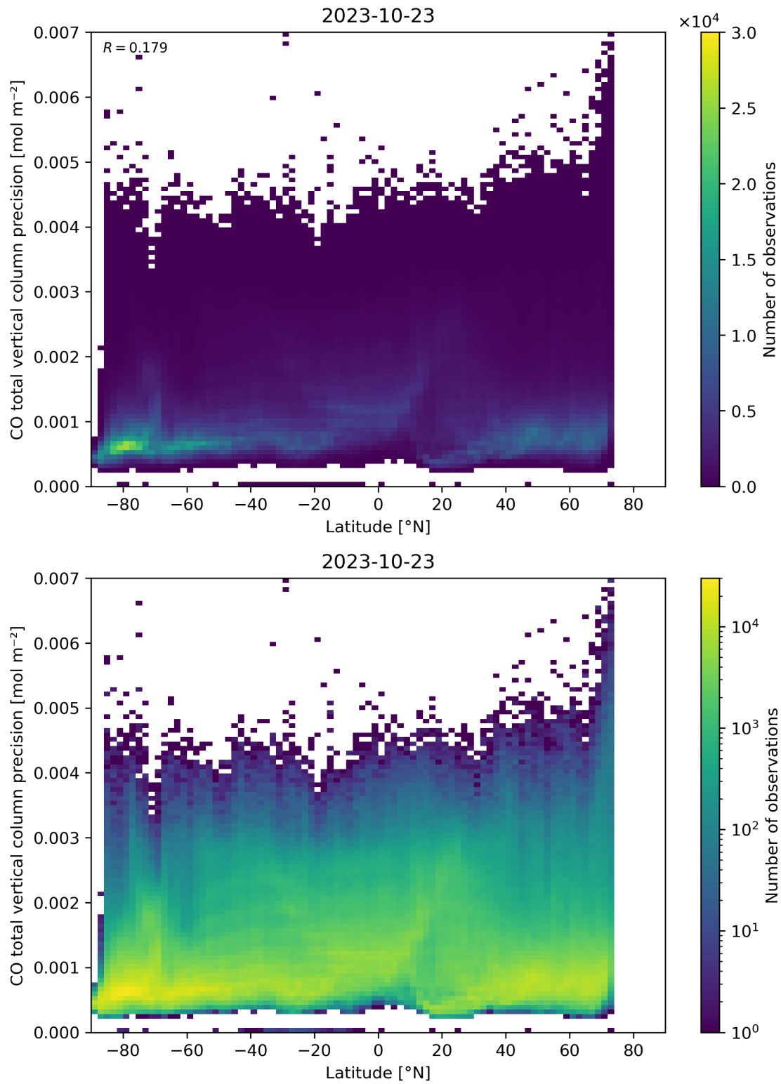
Figure 53: Scatter density plot of “Latitude” against “CO total vertical column precision” for 2023-10-22 to 2023-10-24.
