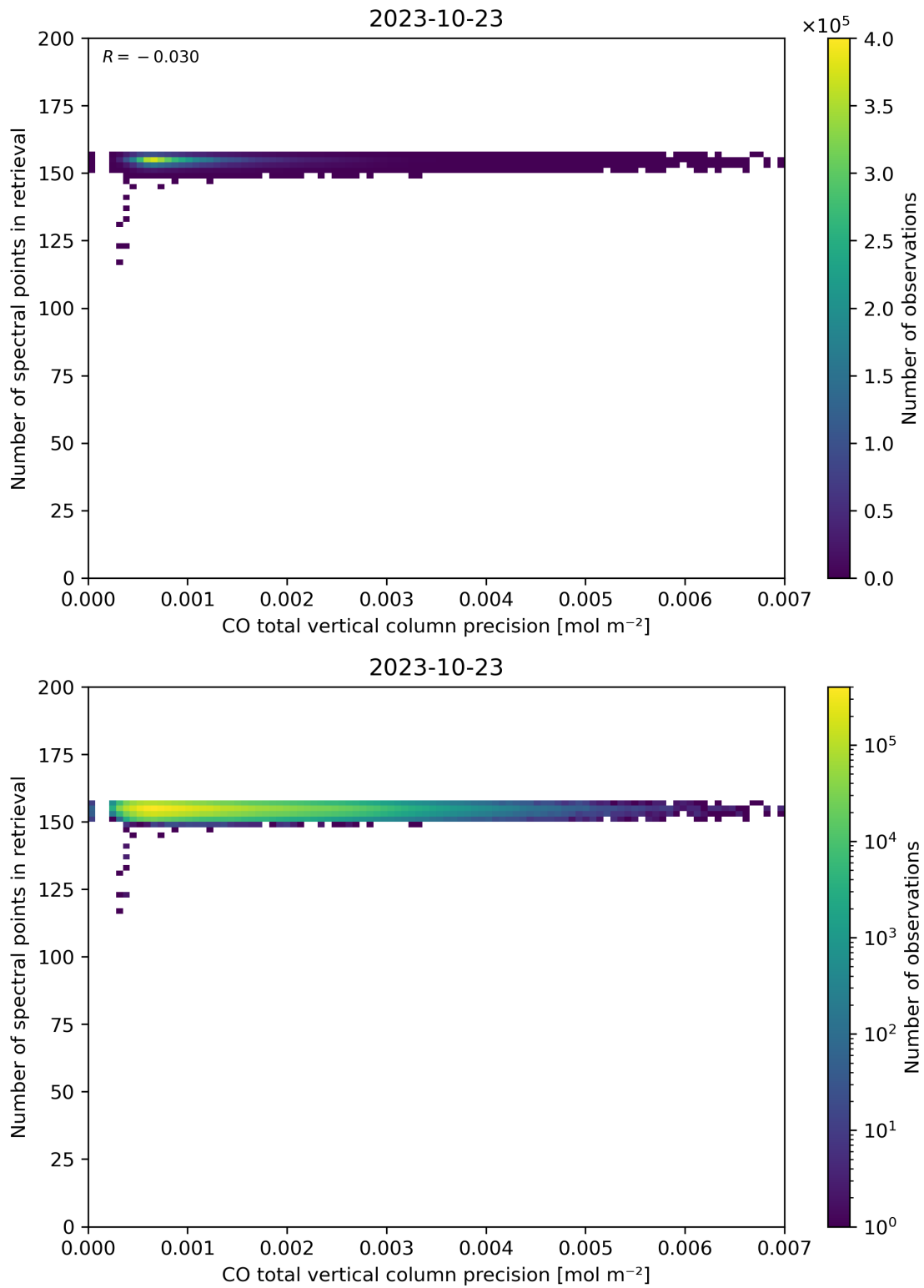
Figure 47: Scatter density plot of “CO total vertical column precision” against “Number of spectral points in retrieval” for 2023-10-22 to 2023-10-24.
