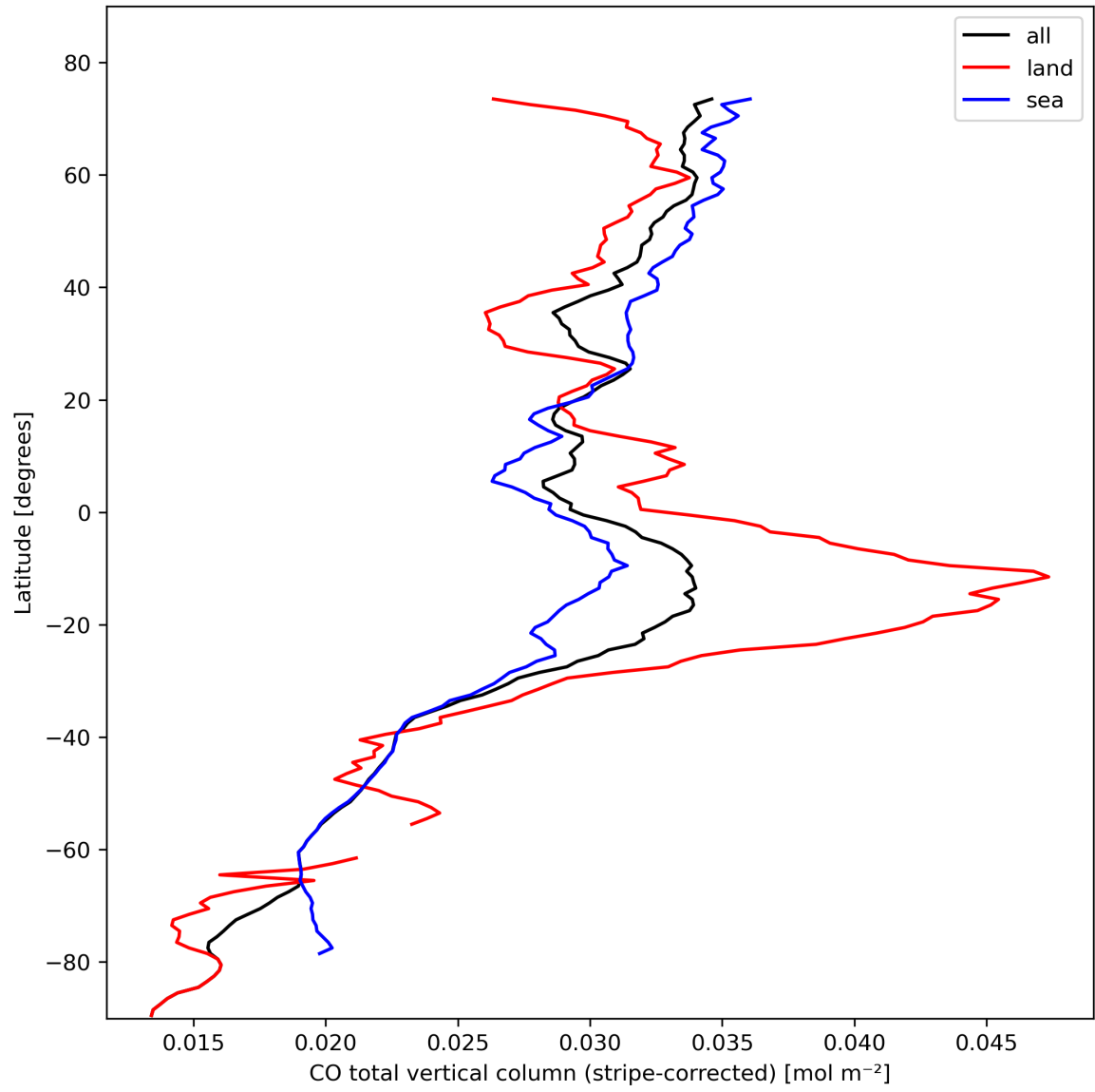
Figure 11: Zonal average of “CO total vertical column (stripe-corrected)” for 2023-10-22 to 2023-10-24.
