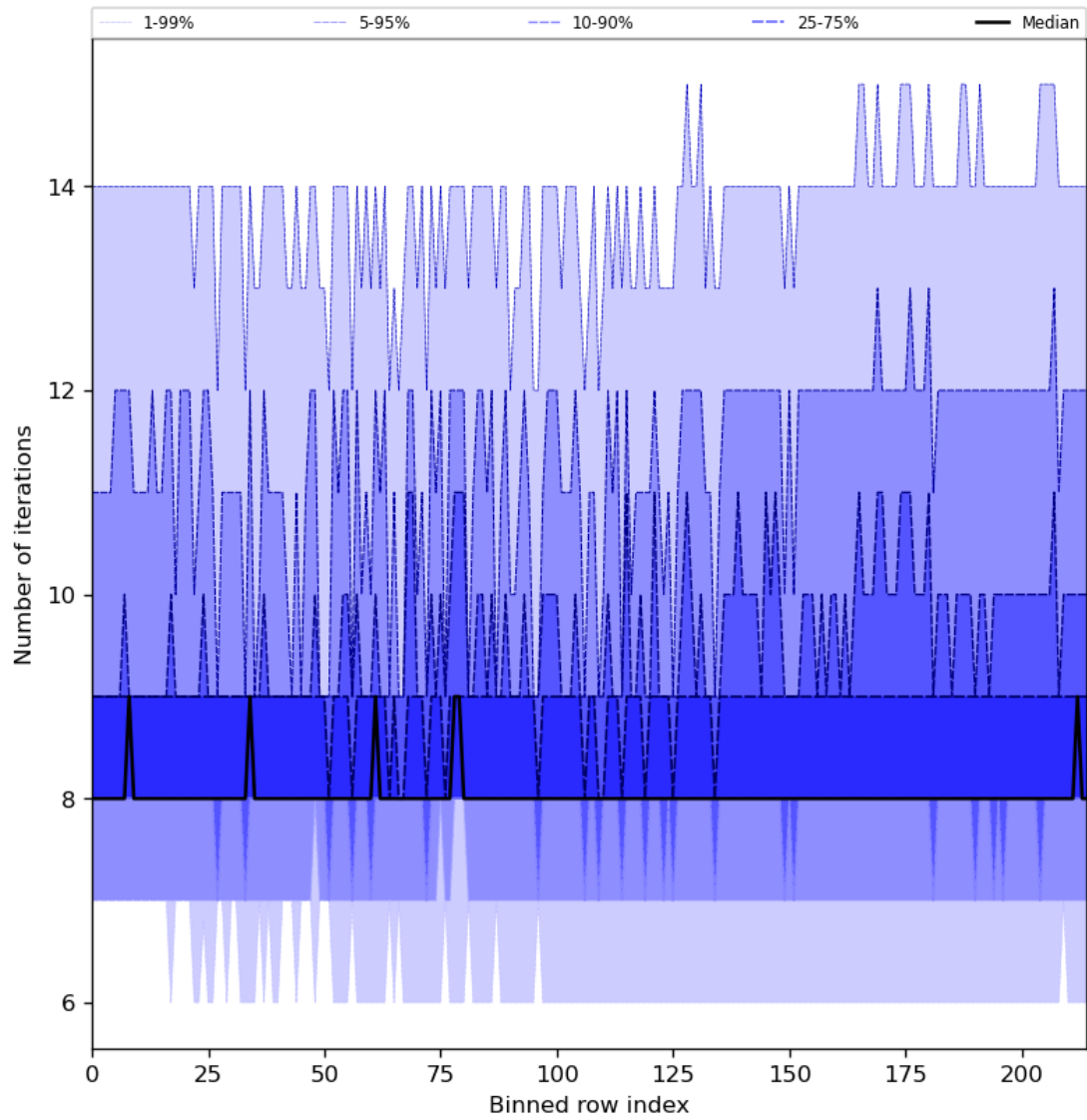
Figure 32: Along track statistics of “Number of iterations” for 2023-10-22 to 2023-10-24
