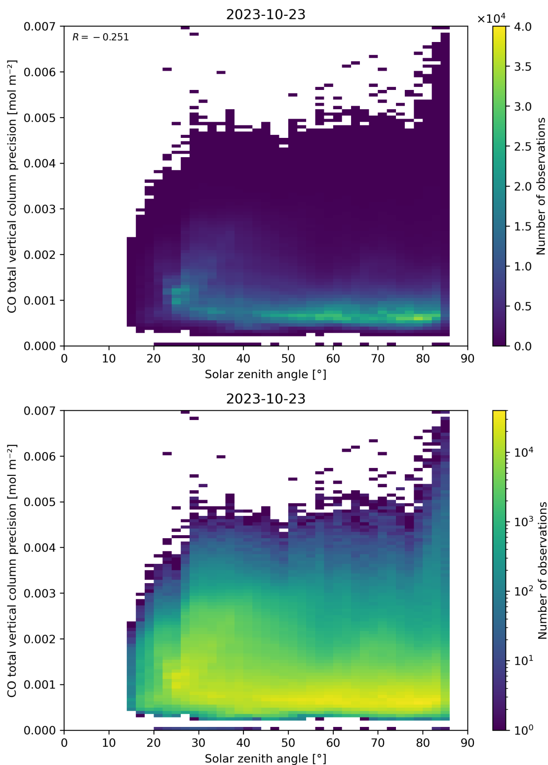
Figure 63: Scatter density plot of “Solar zenith angle” against “CO total vertical column precision” for 2023-10-22 to 2023-10-24.
