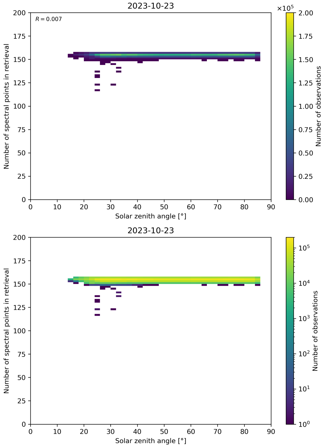
Figure 68: Scatter density plot of “Solar zenith angle” against “Number of spectral points in retrieval” for 2023-10-22 to 2023-10-24.
