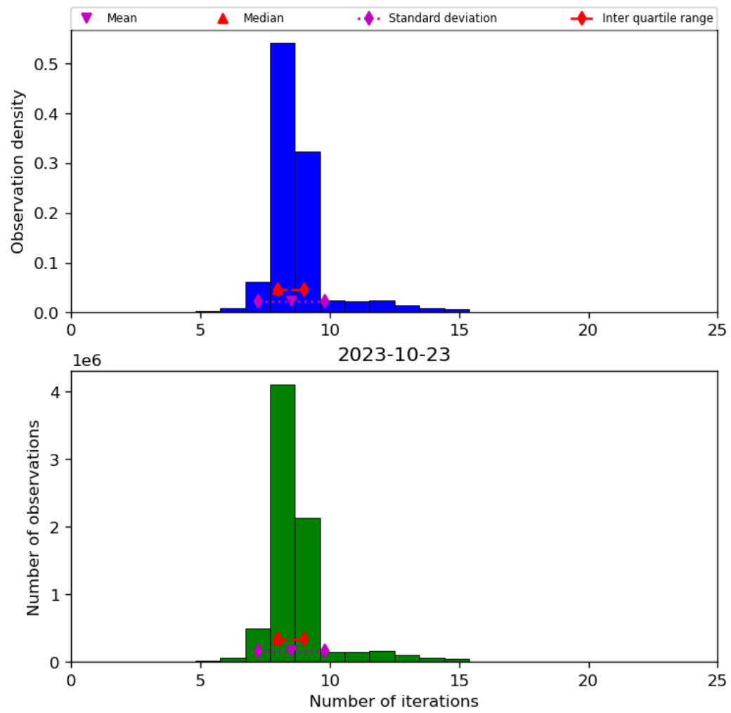
Figure 24: Histogram of “Number of iterations” for 2023-10-22 to 2023-10-24
