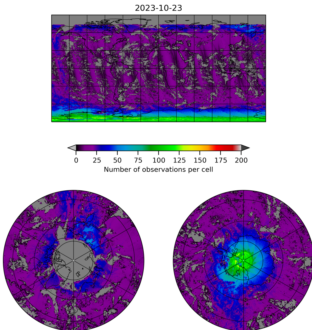
Figure 8: Map of the number of observations for 2023-10-22 to 2023-10-24
