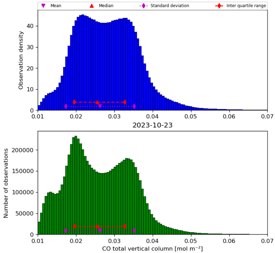
Figure 18: Histogram of “CO total vertical column” for 2023-10-22 to 2023-10-24
