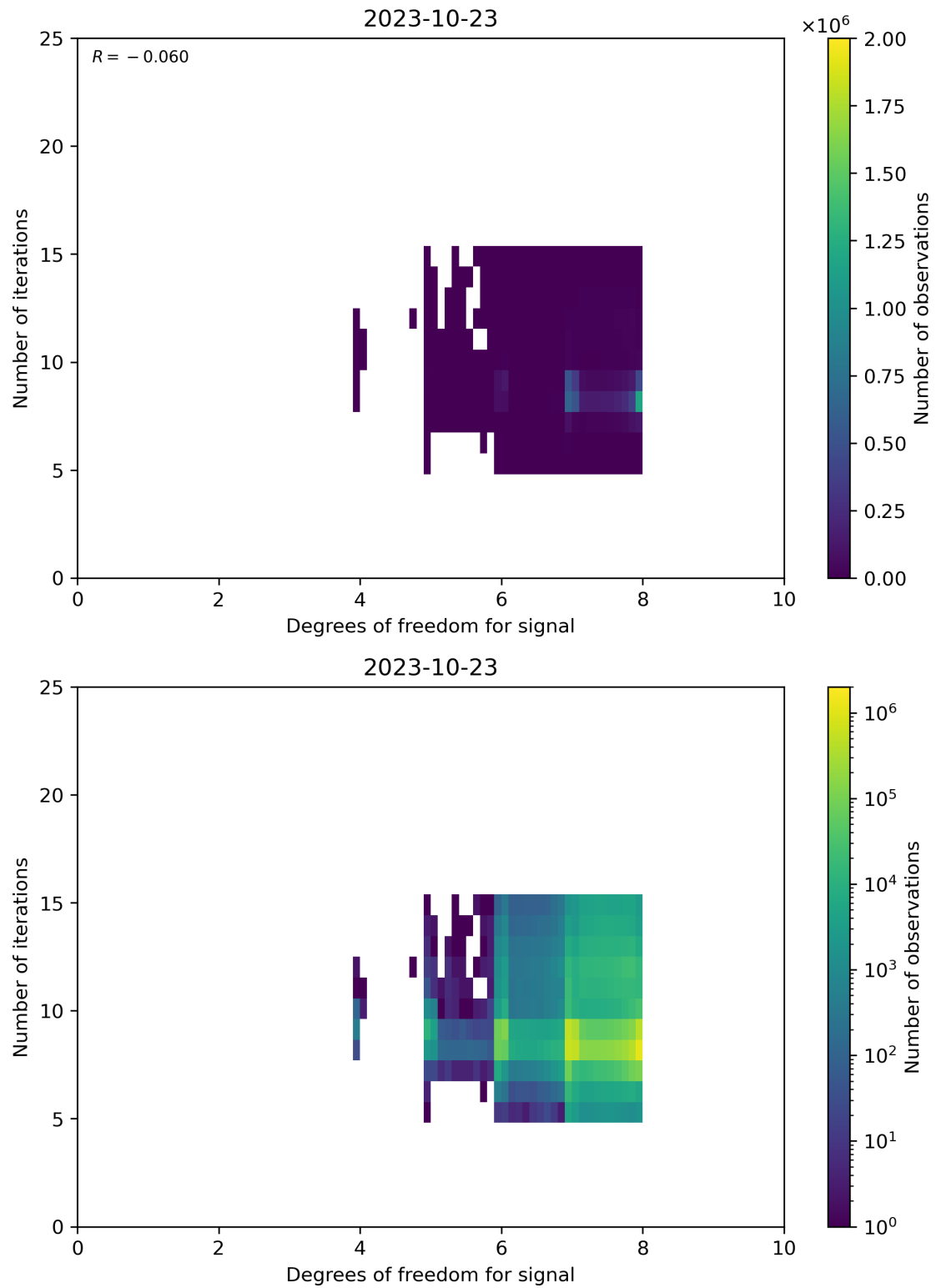
Figure 50: Scatter density plot of “Degrees of freedom for signal” against “Number of iterations” for 2023-10-22 to 2023-10-24.
