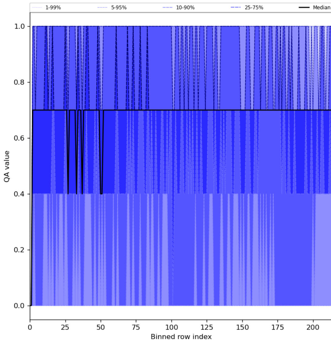
Figure 25: Along track statistics of “QA value” for 2023-10-22 to 2023-10-24
