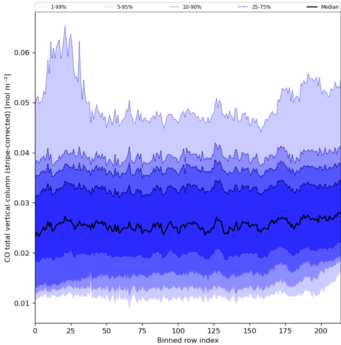
Figure 27: Along track statistics of “CO total vertical column (stripe-corrected)” for 2023-10-22 to 2023-10-24
