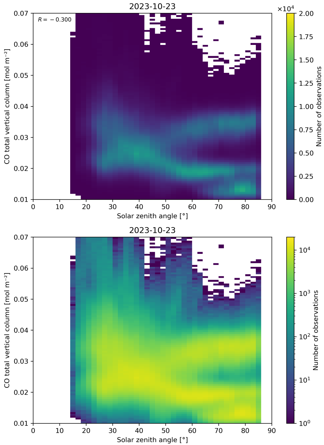
Figure 61: Scatter density plot of “Solar zenith angle” against “CO total vertical column” for 2023-10-22 to 2023-10-24.
