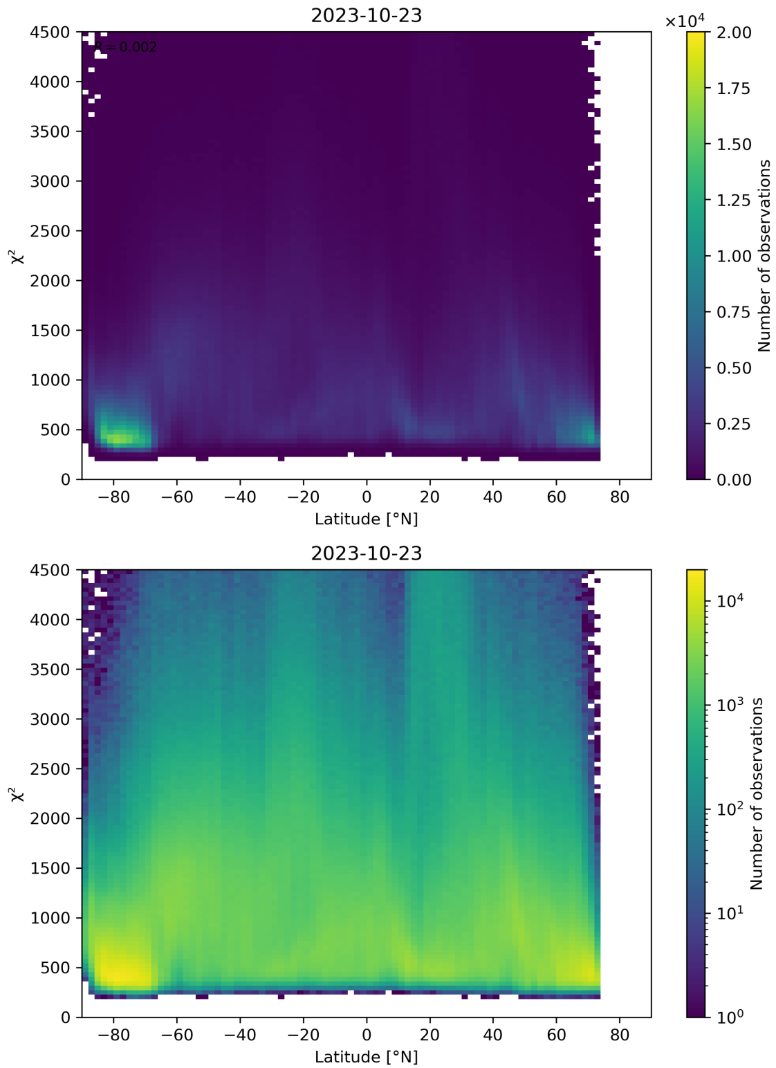
Figure 54: Scatter density plot of “Latitude” against “ \chi^2 ” for 2023-10-22 to 2023-10-24.
