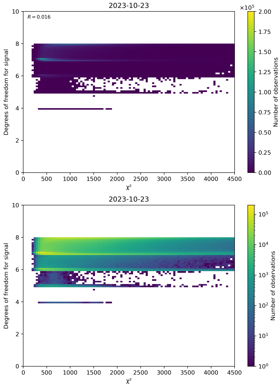
Figure 48: Scatter density plot of “ \chi^2 ” against “Degrees of freedom for signal” for 2023-10-22 to 2023-10-24.
