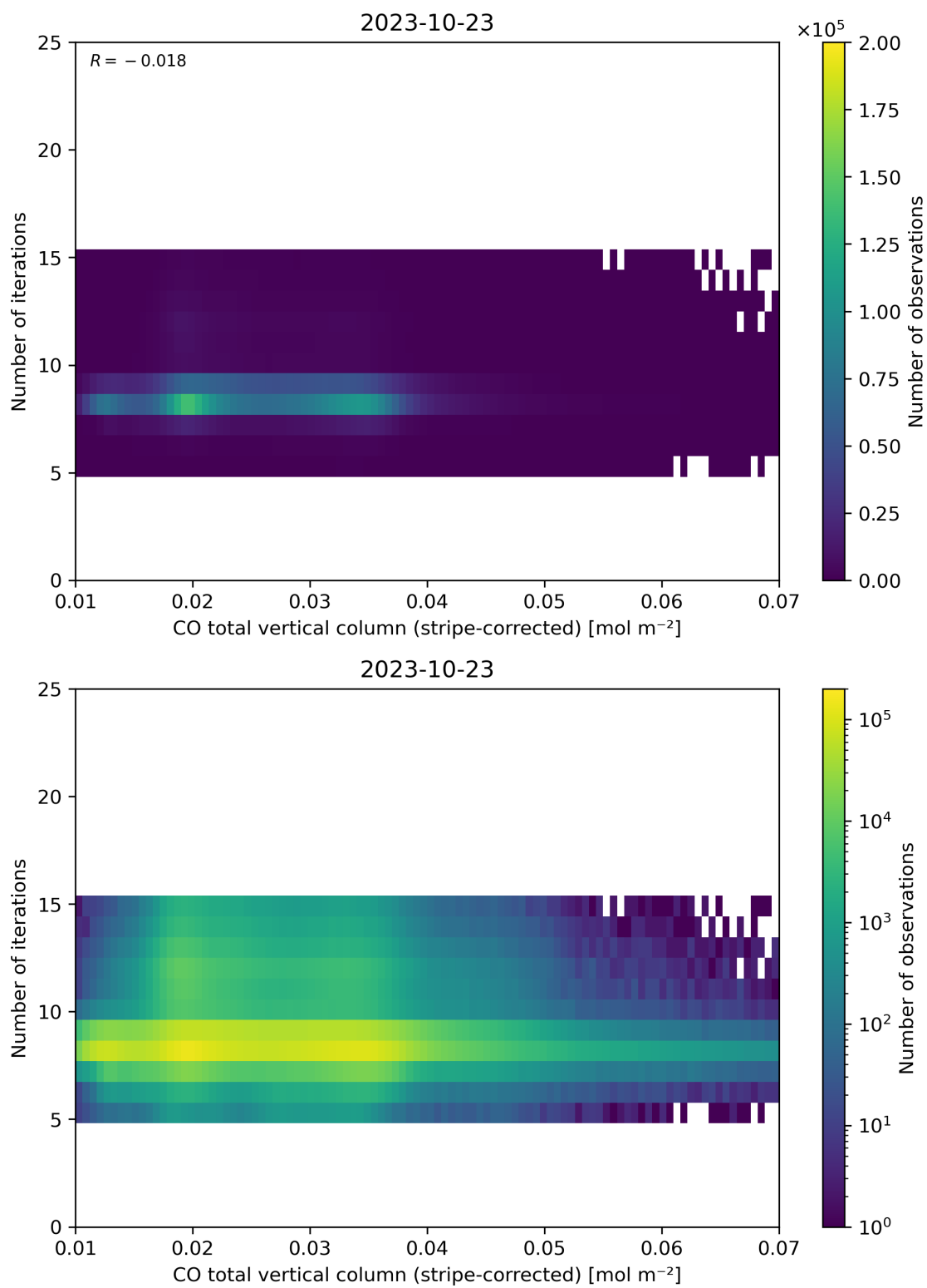
Figure 39: Scatter density plot of “CO total vertical column (stripe-corrected)” against “Number of iterations” for 2023-10-22 to 2023-10-24.
