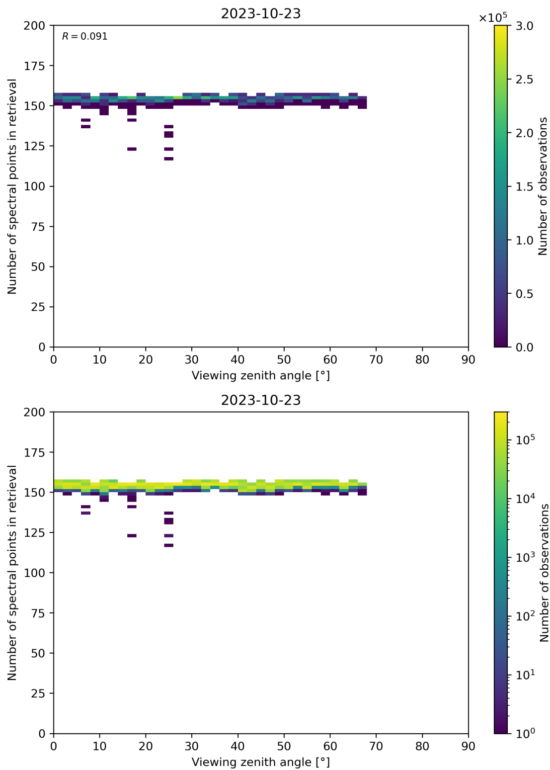
Figure 76: Scatter density plot of “Viewing zenith angle” against “Number of spectral points in retrieval” for 2023-10-22 to 2023-10-24.
