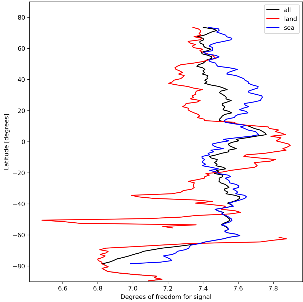
Figure 15: Zonal average of “Degrees of freedom for signal” for 2023-10-22 to 2023-10-24.
