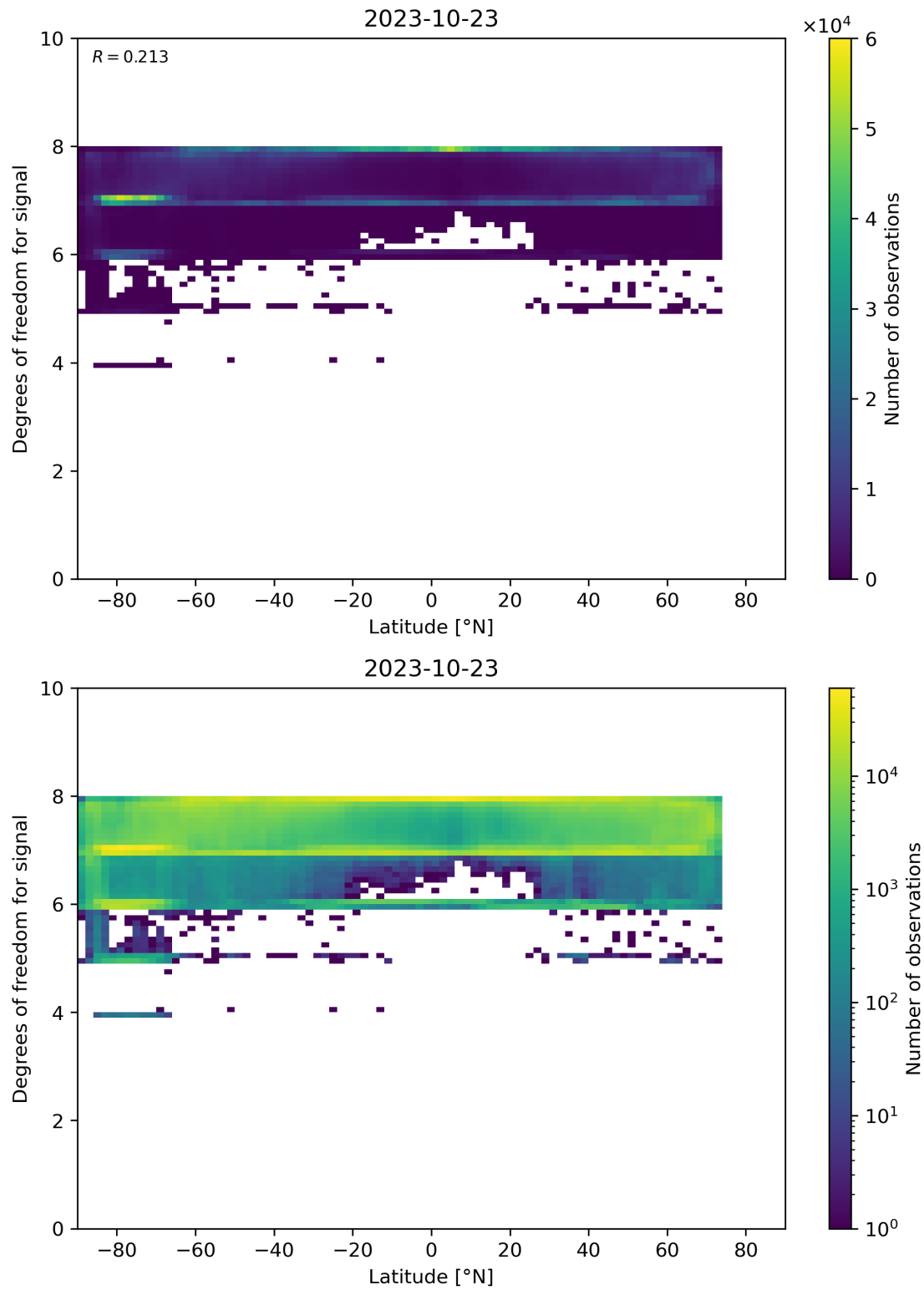
Figure 55: Scatter density plot of “Latitude” against “Degrees of freedom for signal” for 2023-10-22 to 2023-10-24.
