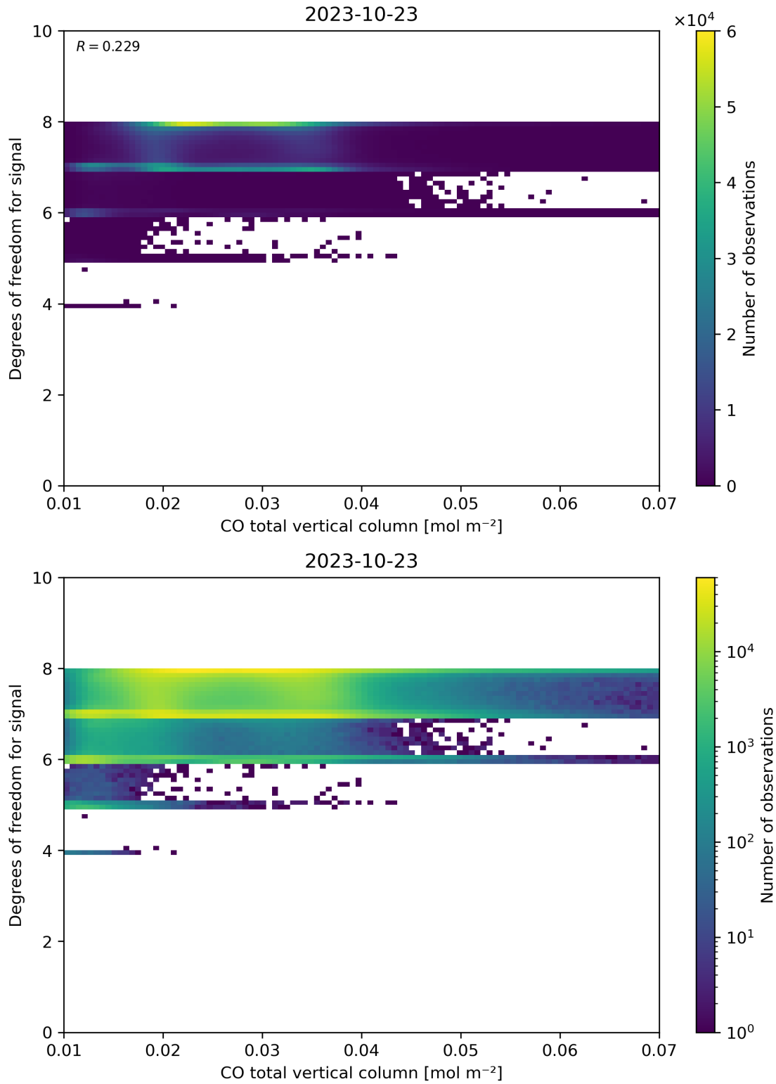
Figure 41: Scatter density plot of “CO total vertical column” against “Degrees of freedom for signal” for 2023-10-22 to 2023-10-24.
