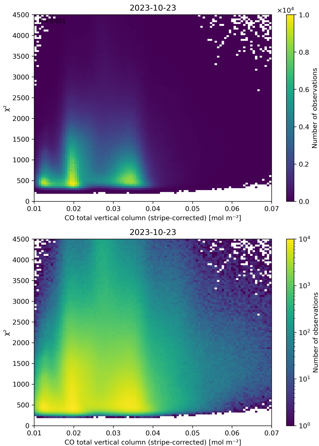
Figure 37: Scatter density plot of “CO total vertical column (stripe-corrected)” against “ \chi^2 ” for 2023-10-22 to 2023-10-24.
