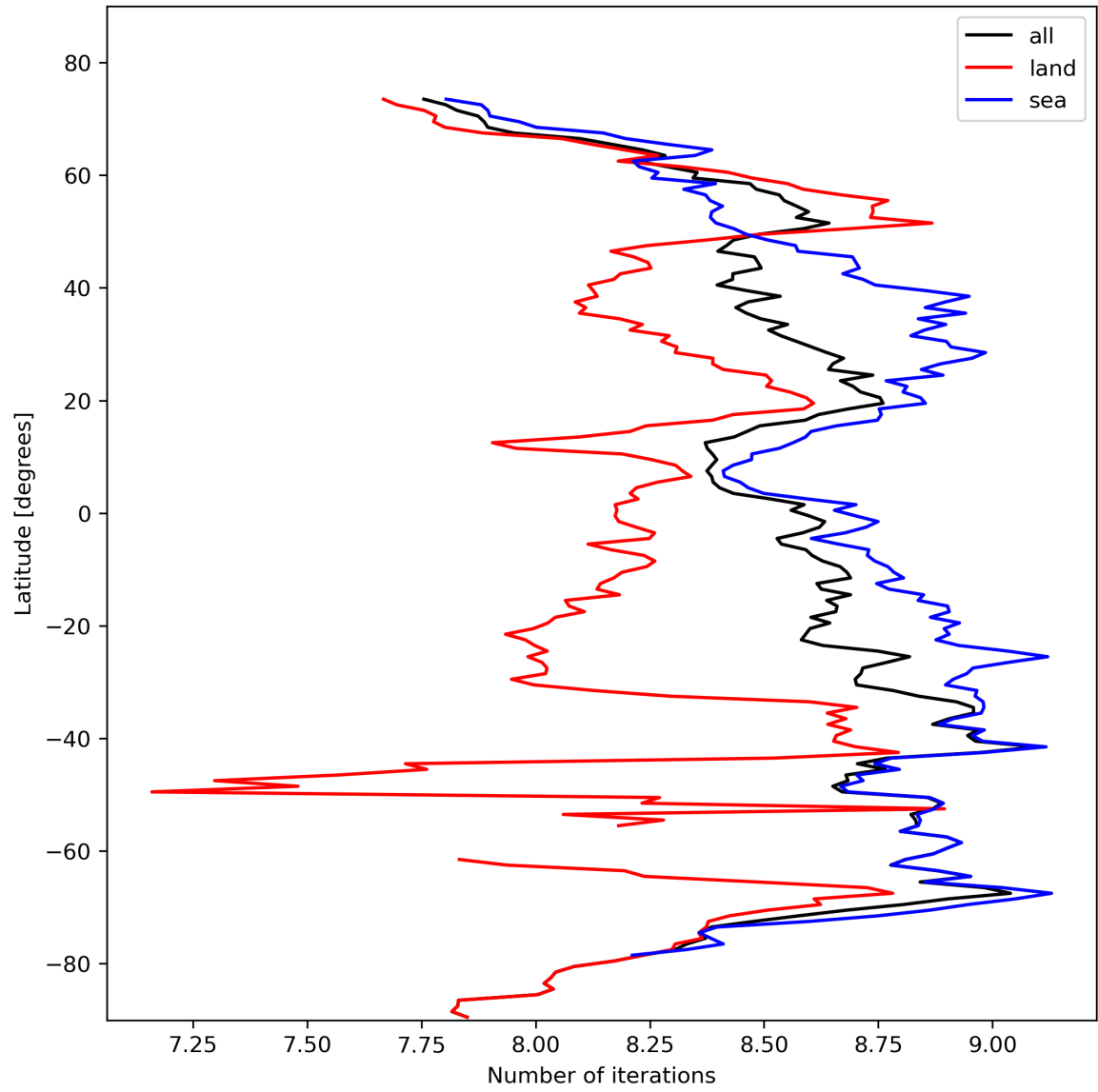
Figure 16: Zonal average of “Number of iterations” for 2023-10-22 to 2023-10-24.
