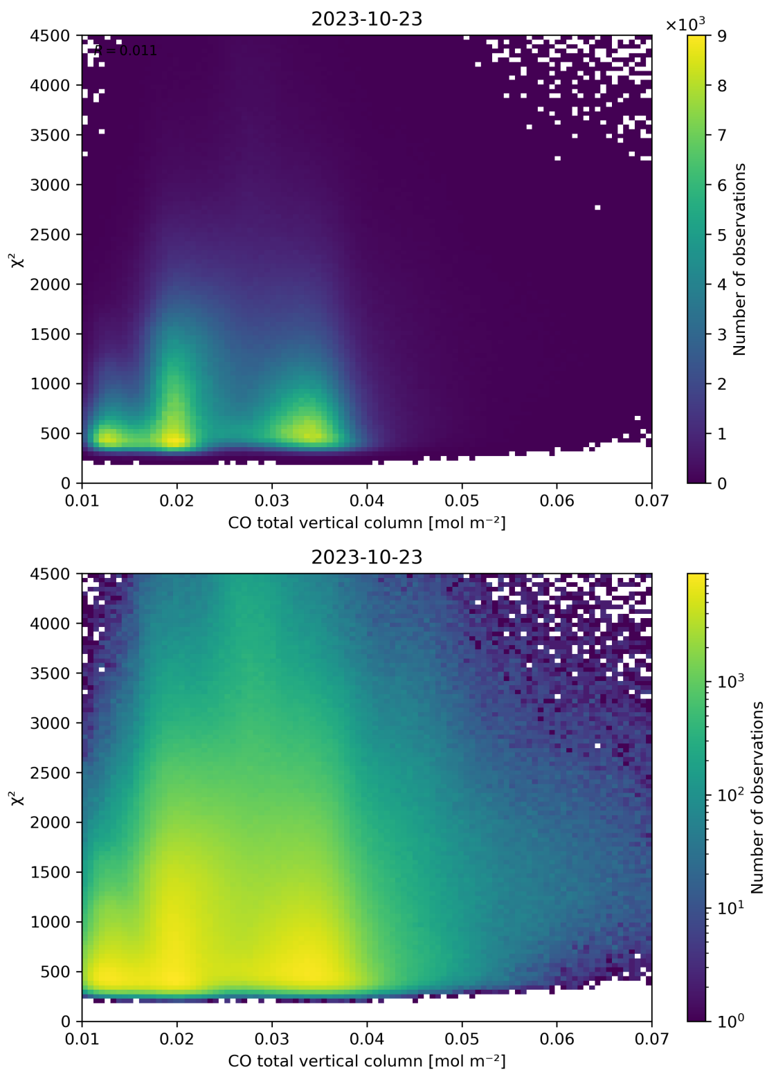
Figure 35: Scatter density plot of “CO total vertical column” against “ \chi^2 ” for 2023-10-22 to 2023-10-24.
