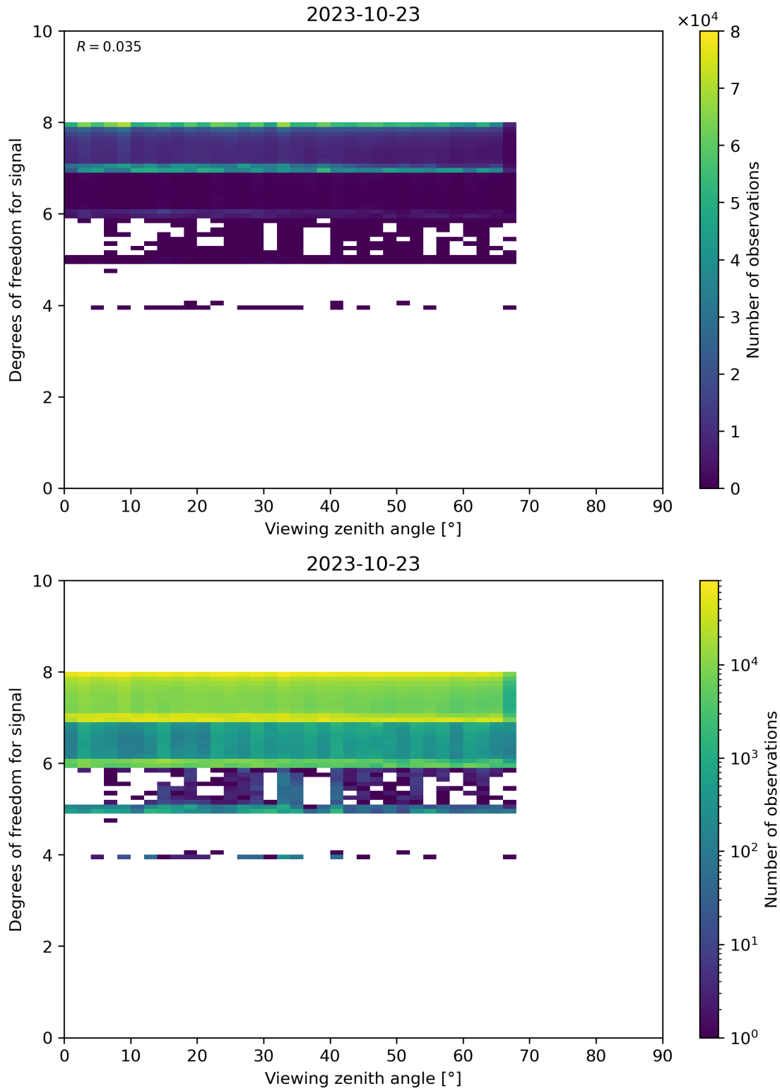
Figure 73: Scatter density plot of “Viewing zenith angle” against “Degrees of freedom for signal” for 2023-10-22 to 2023-10-24.
