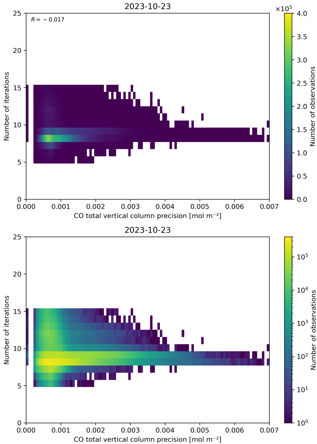
Figure 46: Scatter density plot of “CO total vertical column precision” against “Number of iterations” for 2023-10-22 to 2023-10-24.
