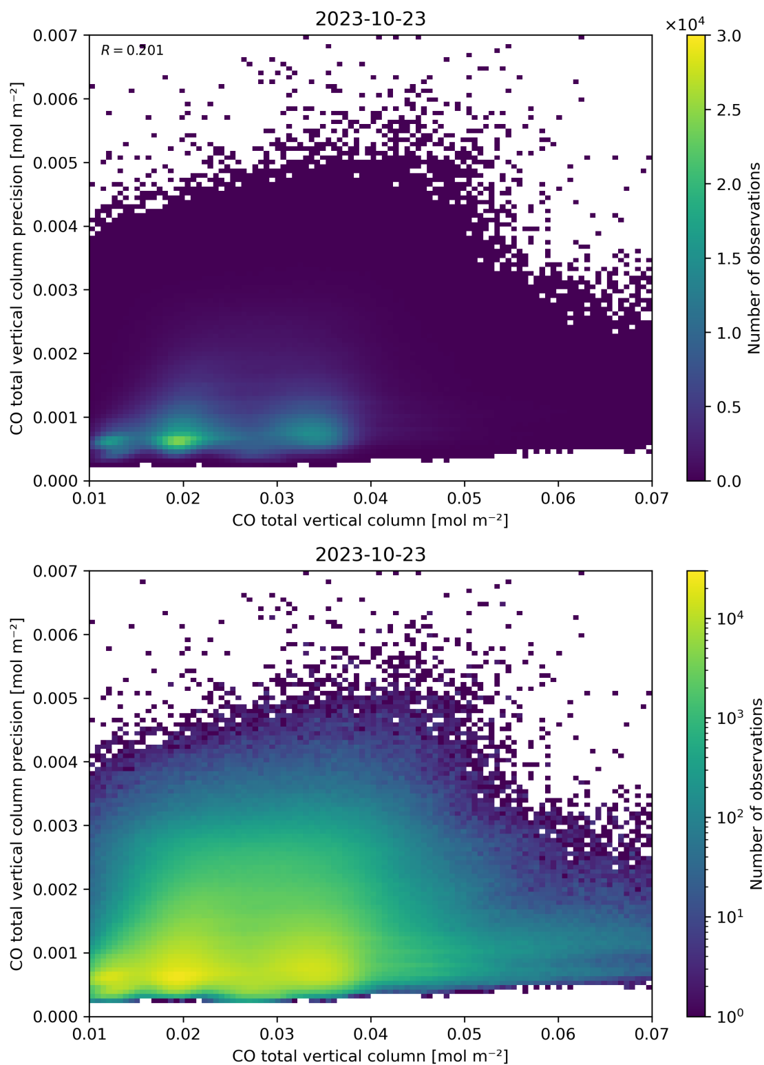
Figure 34: Scatter density plot of “CO total vertical column” against “CO total vertical column precision” for 2023-10-22 to 2023-10-24.
