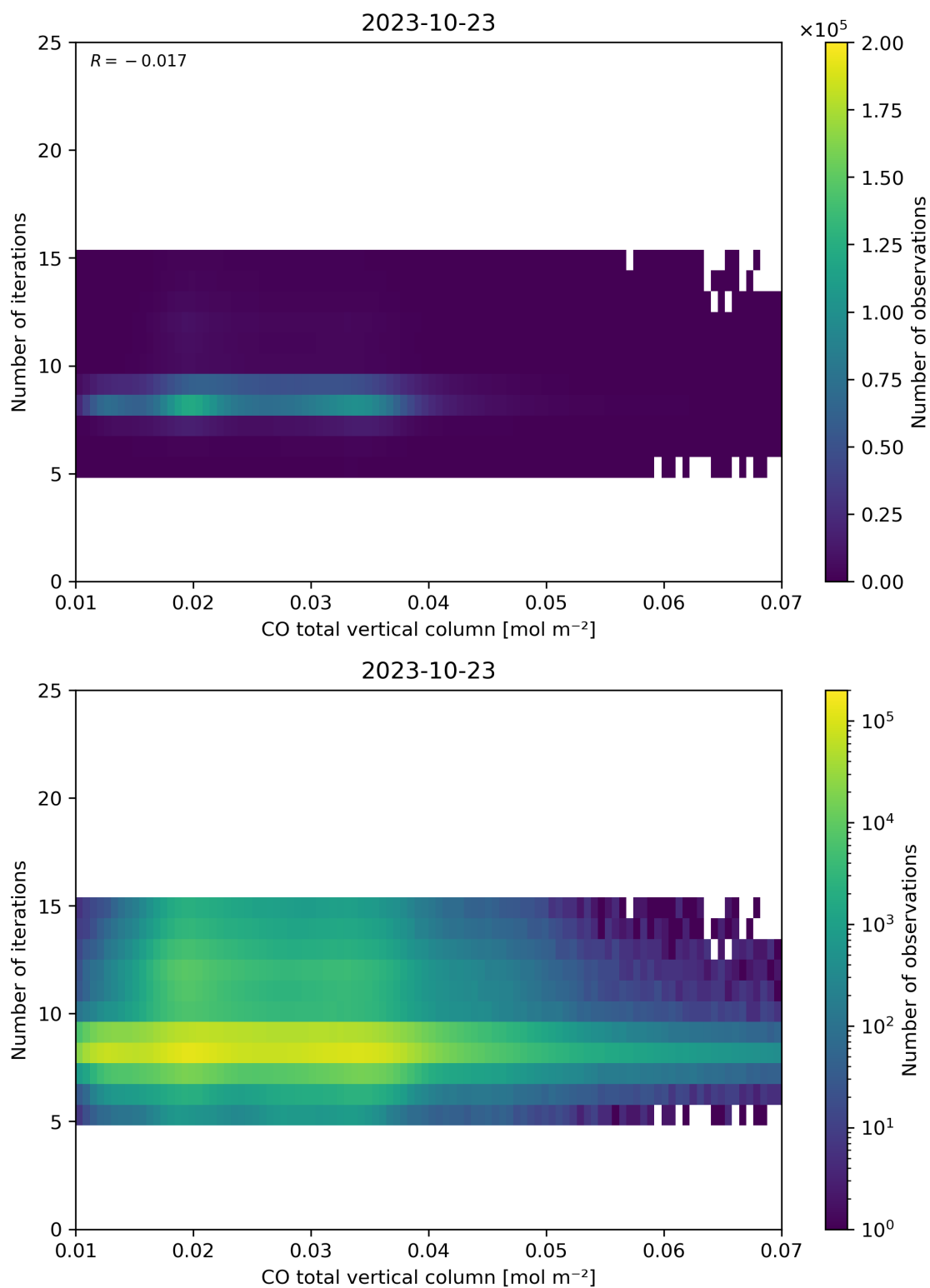
Figure 42: Scatter density plot of “CO total vertical column” against “Number of iterations” for 2023-10-22 to 2023-10-24.
