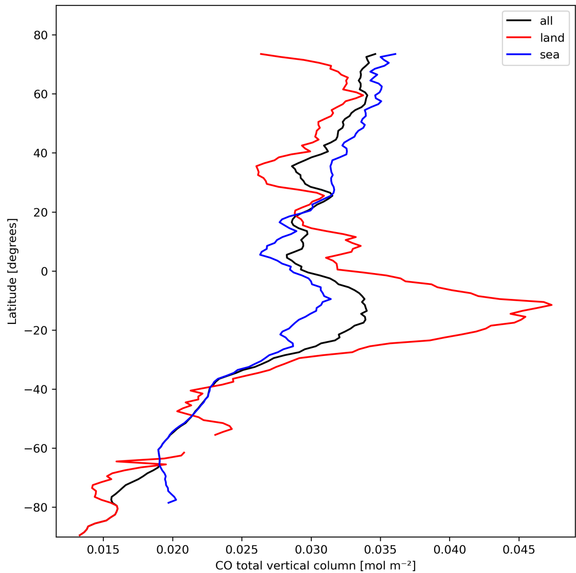
Figure 10: Zonal average of “CO total vertical column” for 2023-10-22 to 2023-10-24.
