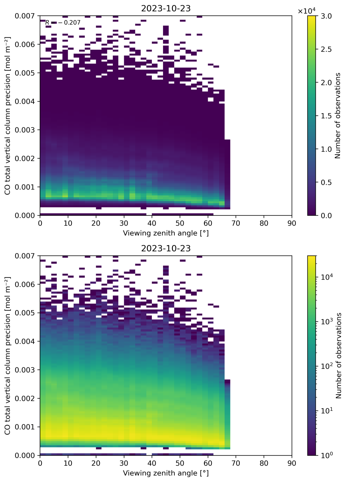
Figure 71: Scatter density plot of “Viewing zenith angle” against “CO total vertical column precision” for 2023-10-22 to 2023-10-24.
