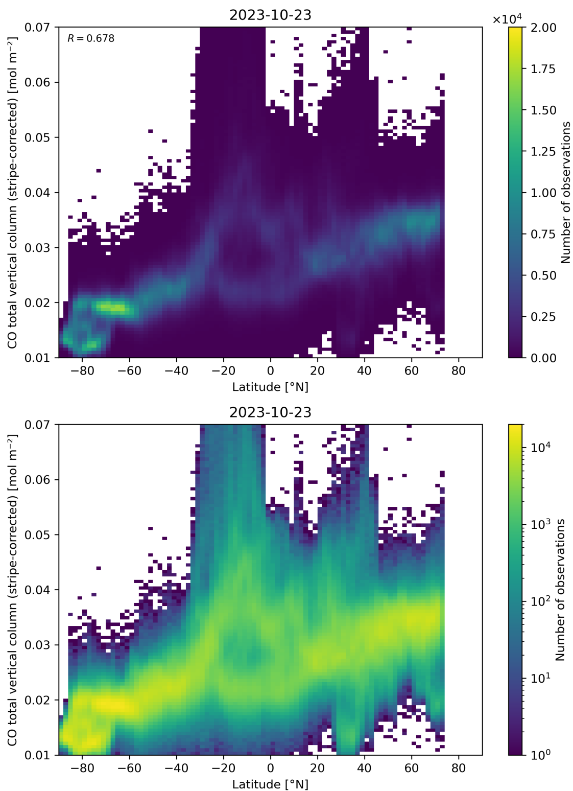
Figure 52: Scatter density plot of “Latitude” against “CO total vertical column (stripe-corrected)” for 2023-10-22 to 2023-10-24.
