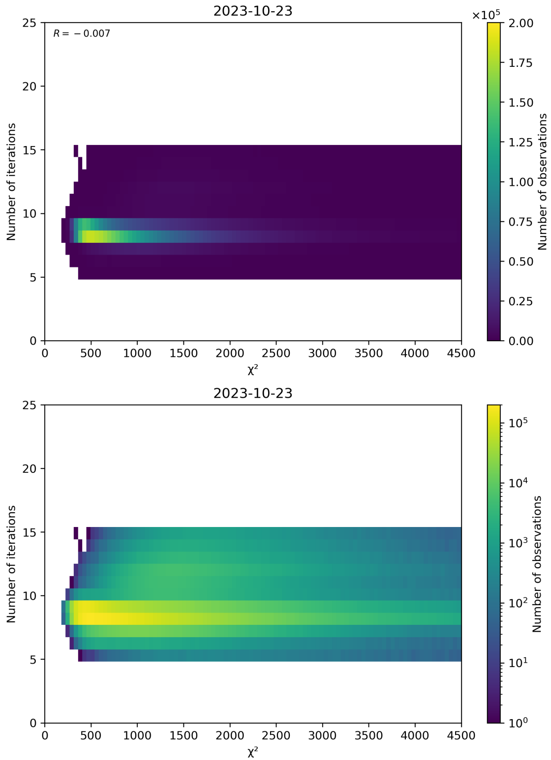
Figure 49: Scatter density plot of " \chi^2 " against "Number of iterations" for 2023-10-22 to 2023-10-24.
