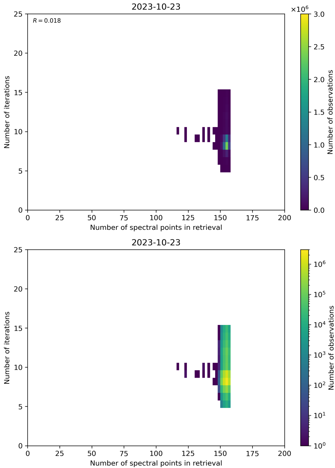
Figure 60: Scatter density plot of “Number of spectral points in retrieval” against “Number of iterations” for 2023-10-22 to 2023-10-24.
