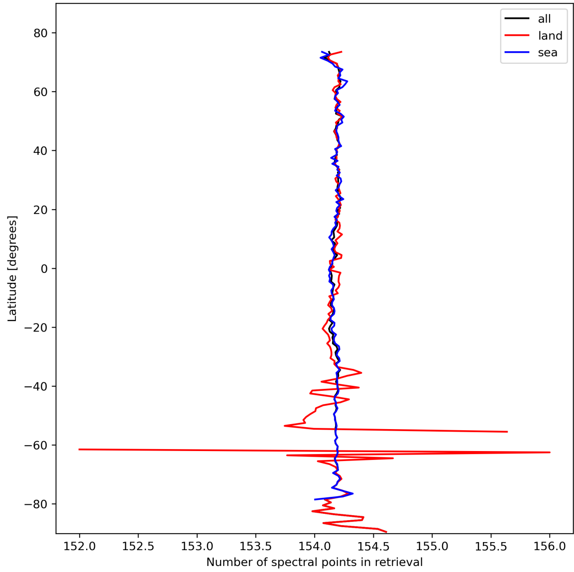
Figure 13: Zonal average of “Number of spectral points in retrieval” for 2023-10-22 to 2023-10-24.
