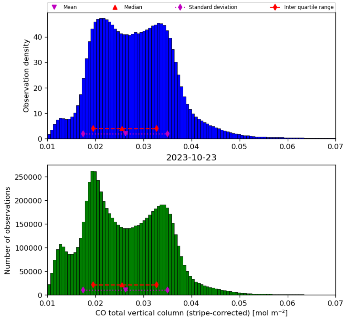
Figure 19: Histogram of “CO total vertical column (stripe-corrected)” for 2023-10-22 to 2023-10-24
