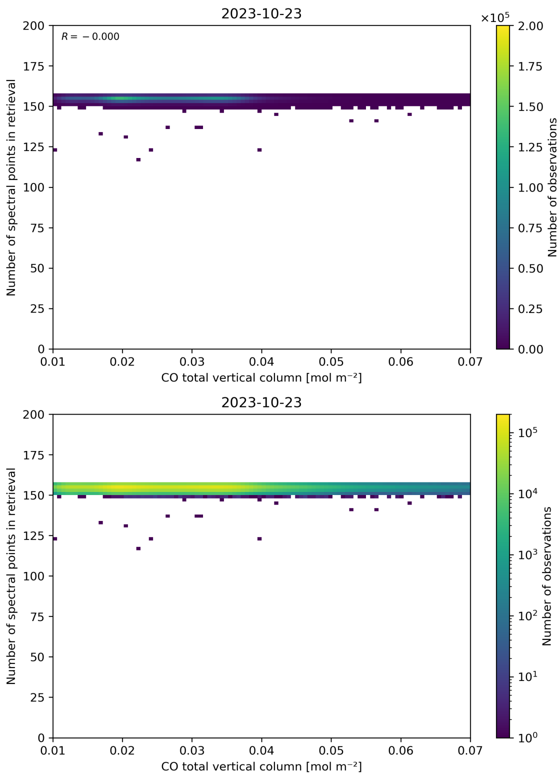
Figure 43: Scatter density plot of “CO total vertical column” against “Number of spectral points in retrieval” for 2023-10-22 to 2023-10-24.
