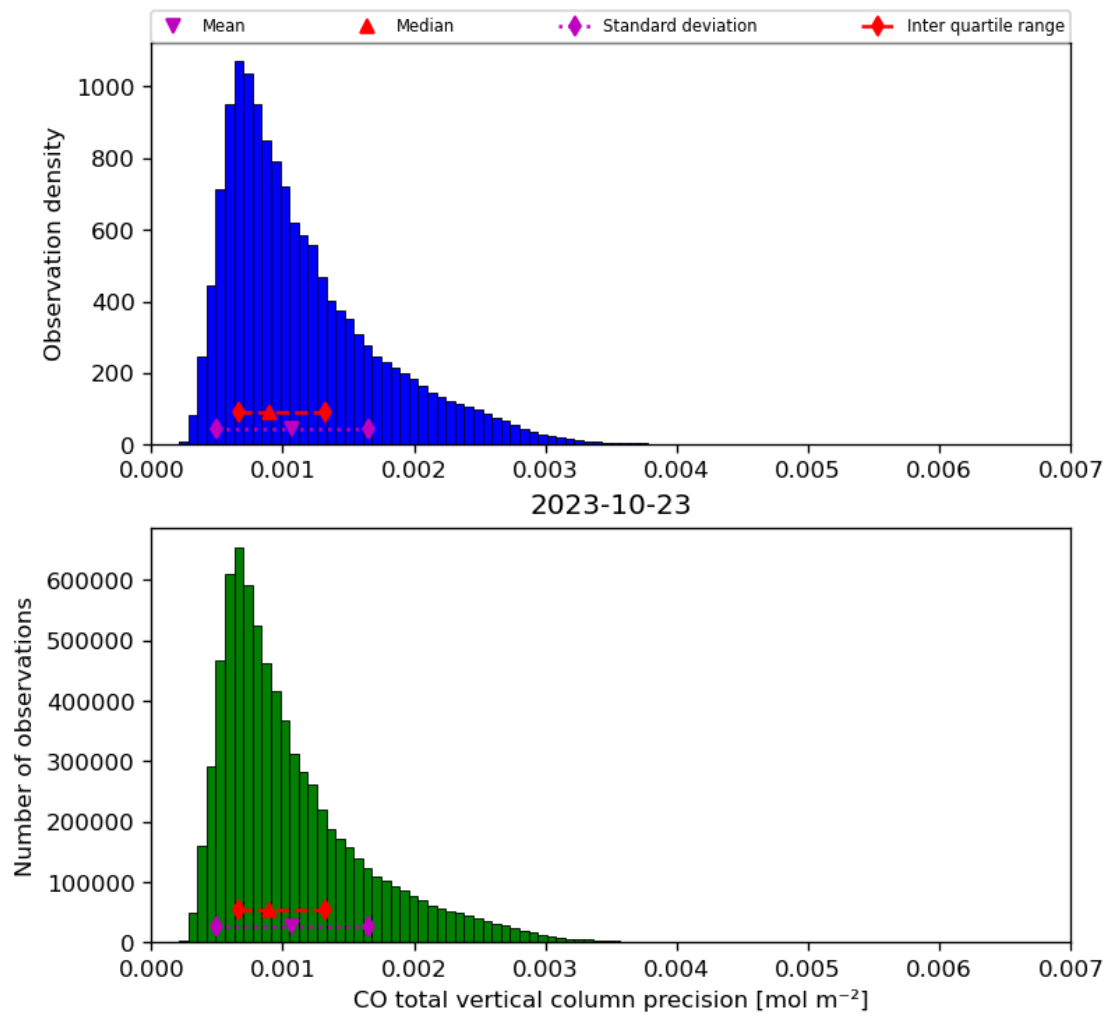
Figure 20: Histogram of “CO total vertical column precision” for 2023-10-22 to 2023-10-24
