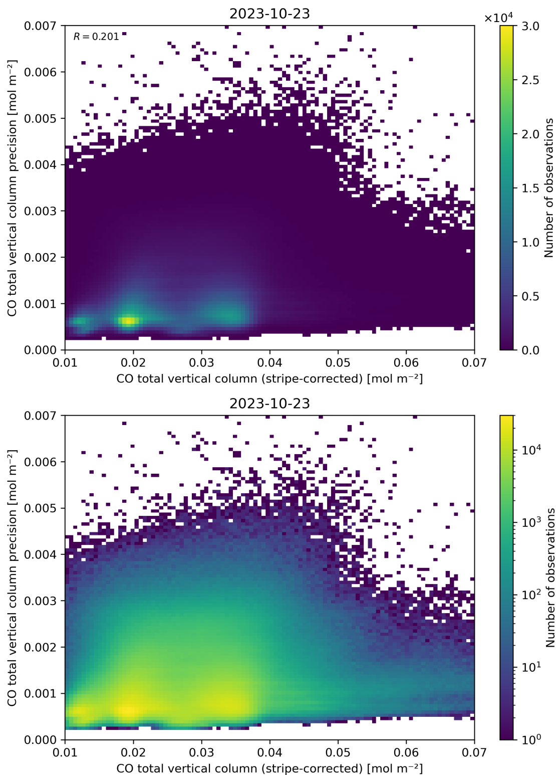
Figure 36: Scatter density plot of “CO total vertical column (stripe-corrected)” against “CO total vertical column precision” for 2023-10-22 to 2023-10-24.
