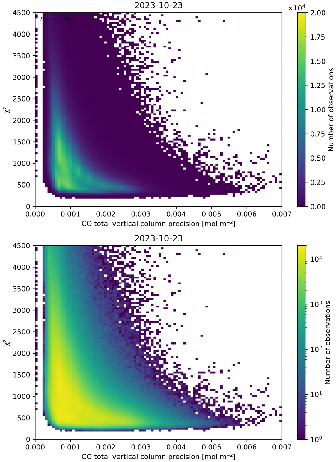
Figure 44: Scatter density plot of “CO total vertical column precision” against “ \chi^2 ” for 2023-10-22 to 2023-10-24.
