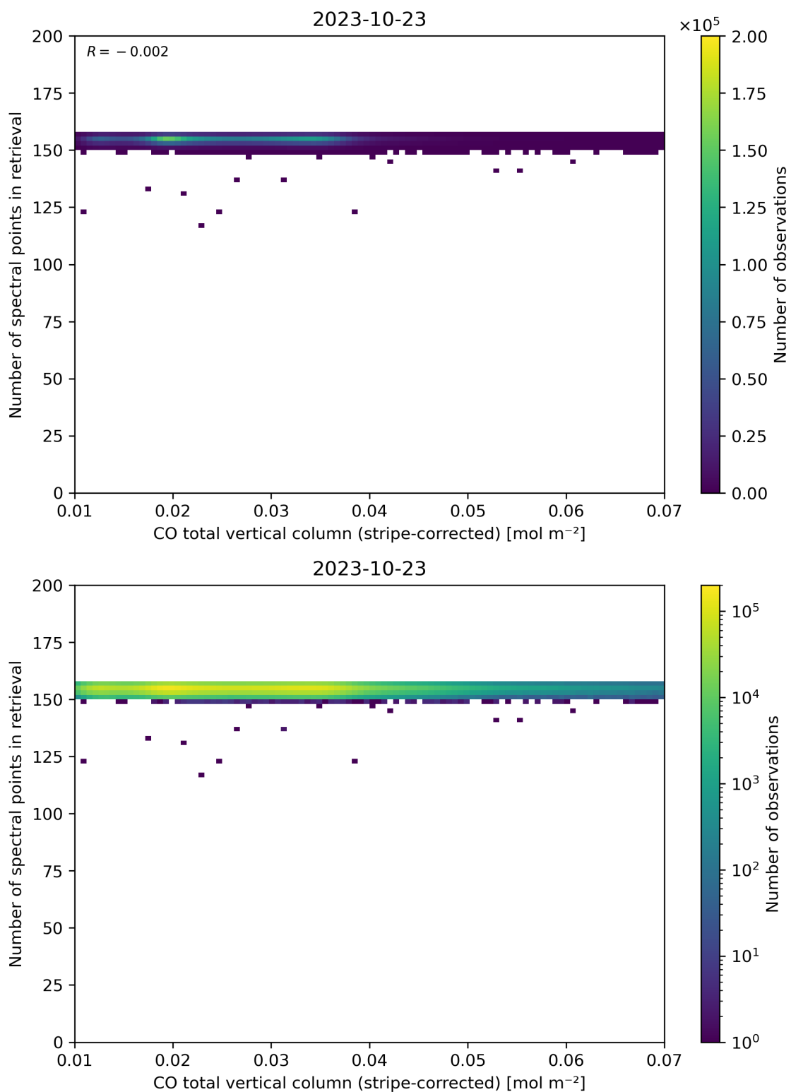
Figure 40: Scatter density plot of “CO total vertical column (stripe-corrected)” against “Number of spectral points in retrieval” for 2023-10-22 to 2023-10-24.
