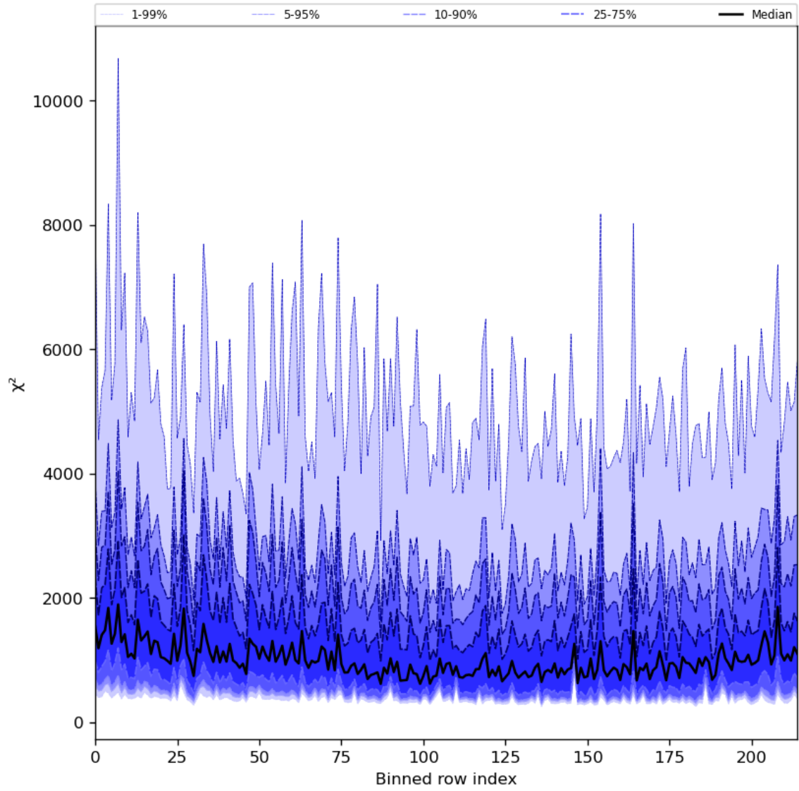
Figure 30: Along track statistics of “ \chi^2 ” for 2023-10-22 to 2023-10-24
