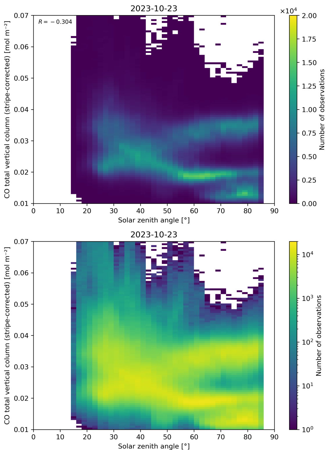
Figure 62: Scatter density plot of “Solar zenith angle” against “CO total vertical column (stripe-corrected)” for 2023-10-22 to 2023-10-24.
