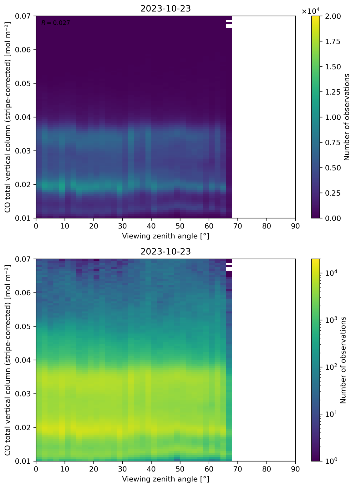
Figure 70: Scatter density plot of “Viewing zenith angle” against “CO total vertical column (stripe-corrected)” for 2023-10-22 to 2023-10-24.
