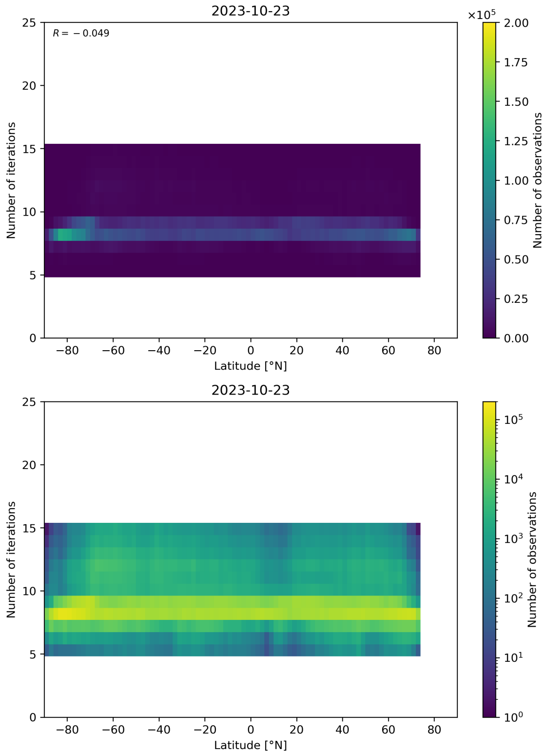
Figure 56: Scatter density plot of “Latitude” against “Number of iterations” for 2023-10-22 to 2023-10-24.
