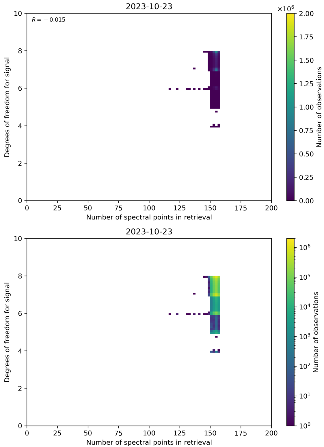
Figure 59: Scatter density plot of “Number of spectral points in retrieval” against “Degrees of freedom for signal” for 2023-10-22 to 2023-10-24.
