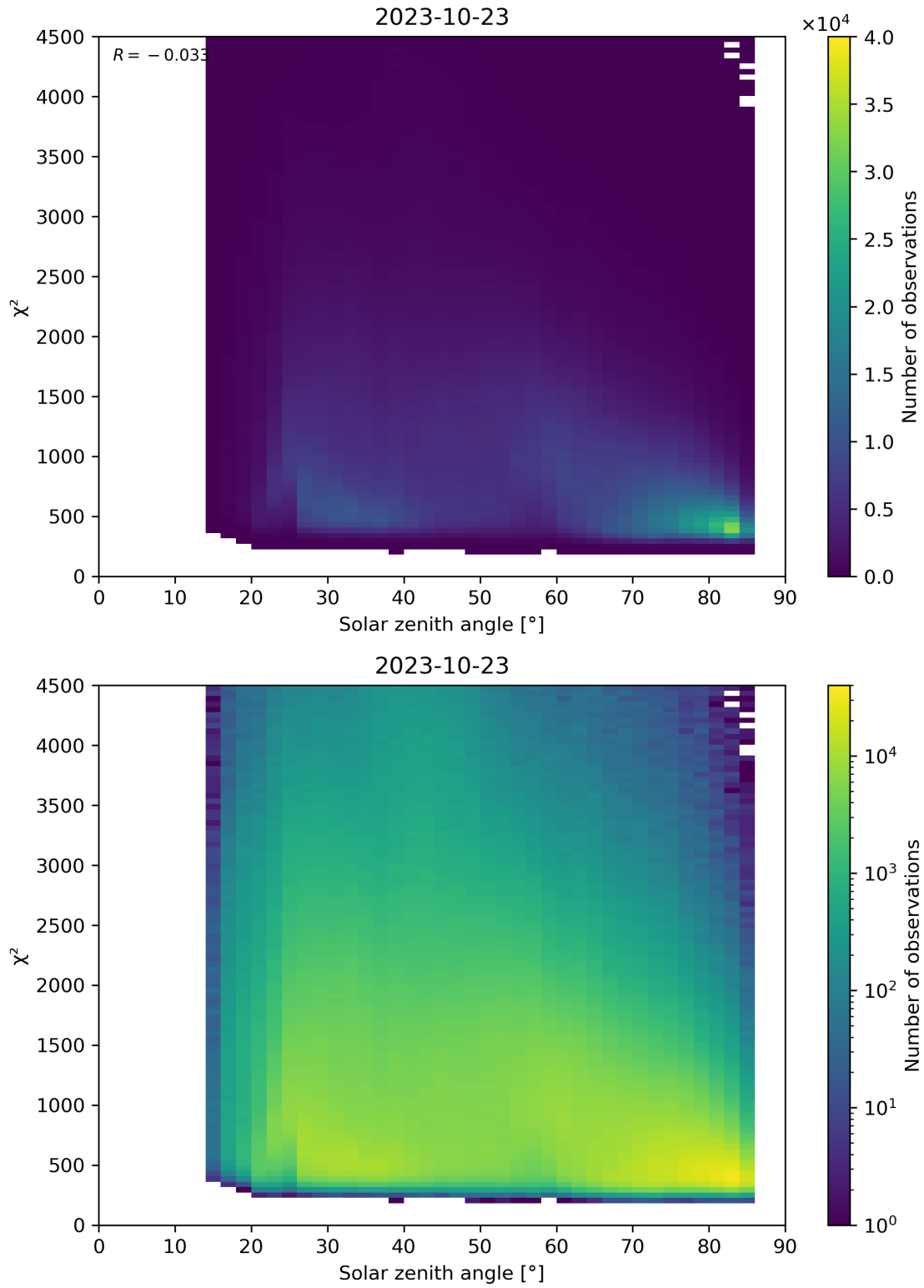
Figure 64: Scatter density plot of “Solar zenith angle” against “ \chi^2 ” for 2023-10-22 to 2023-10-24.
