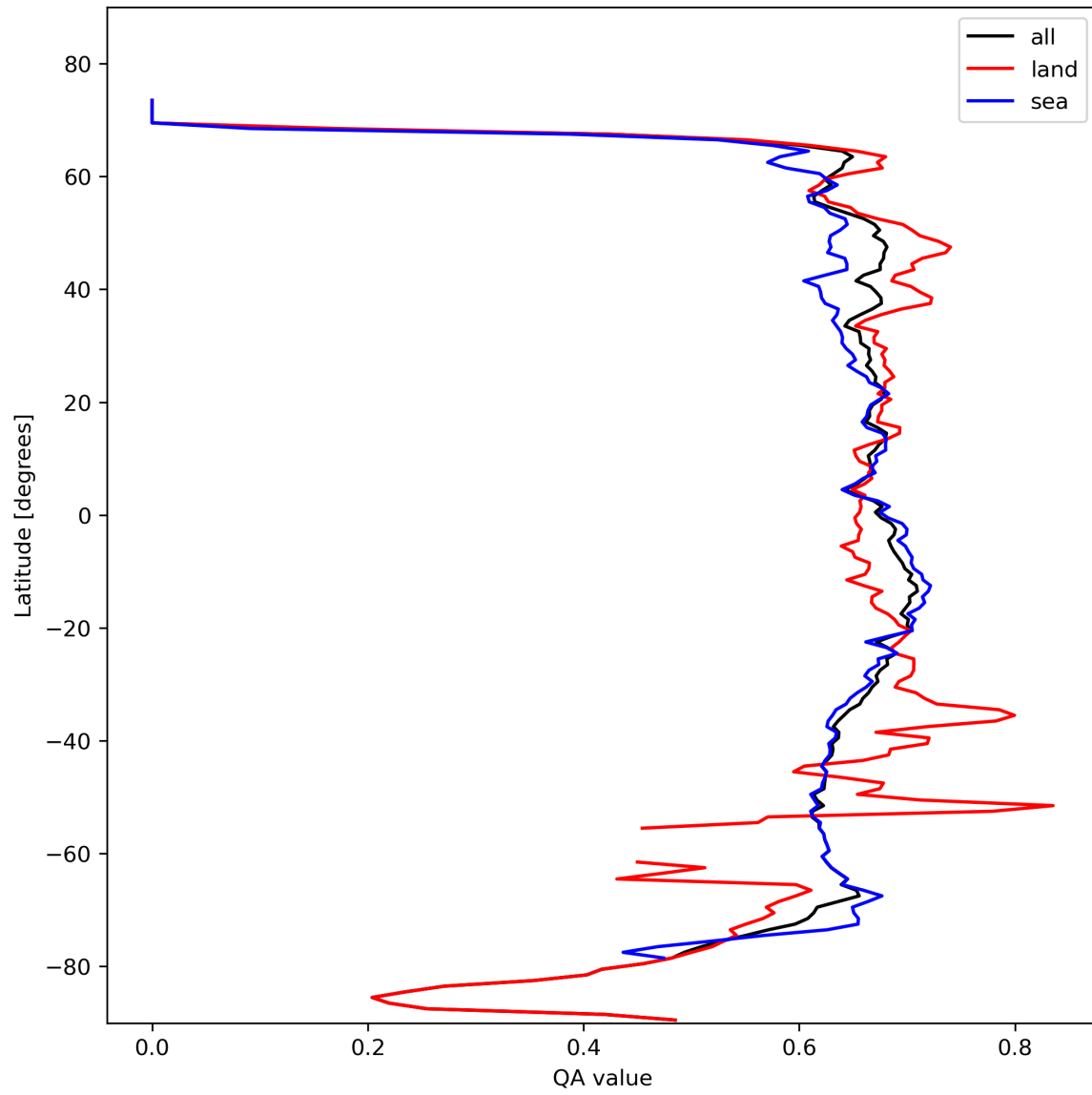
Figure 9: Zonal average of “QA value” for 2023-10-22 to 2023-10-24.
