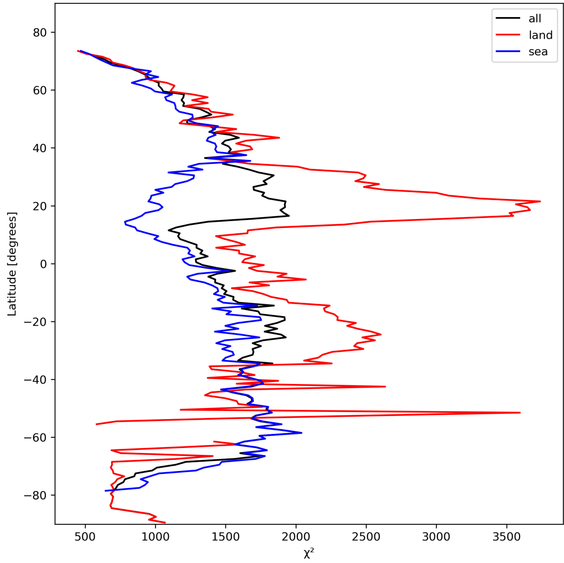
Figure 14: Zonal average of “ \chi^2 ” for 2023-10-22 to 2023-10-24.
