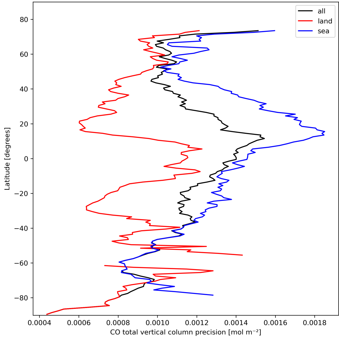
Figure 12: Zonal average of “CO total vertical column precision” for 2023-10-22 to 2023-10-24.
