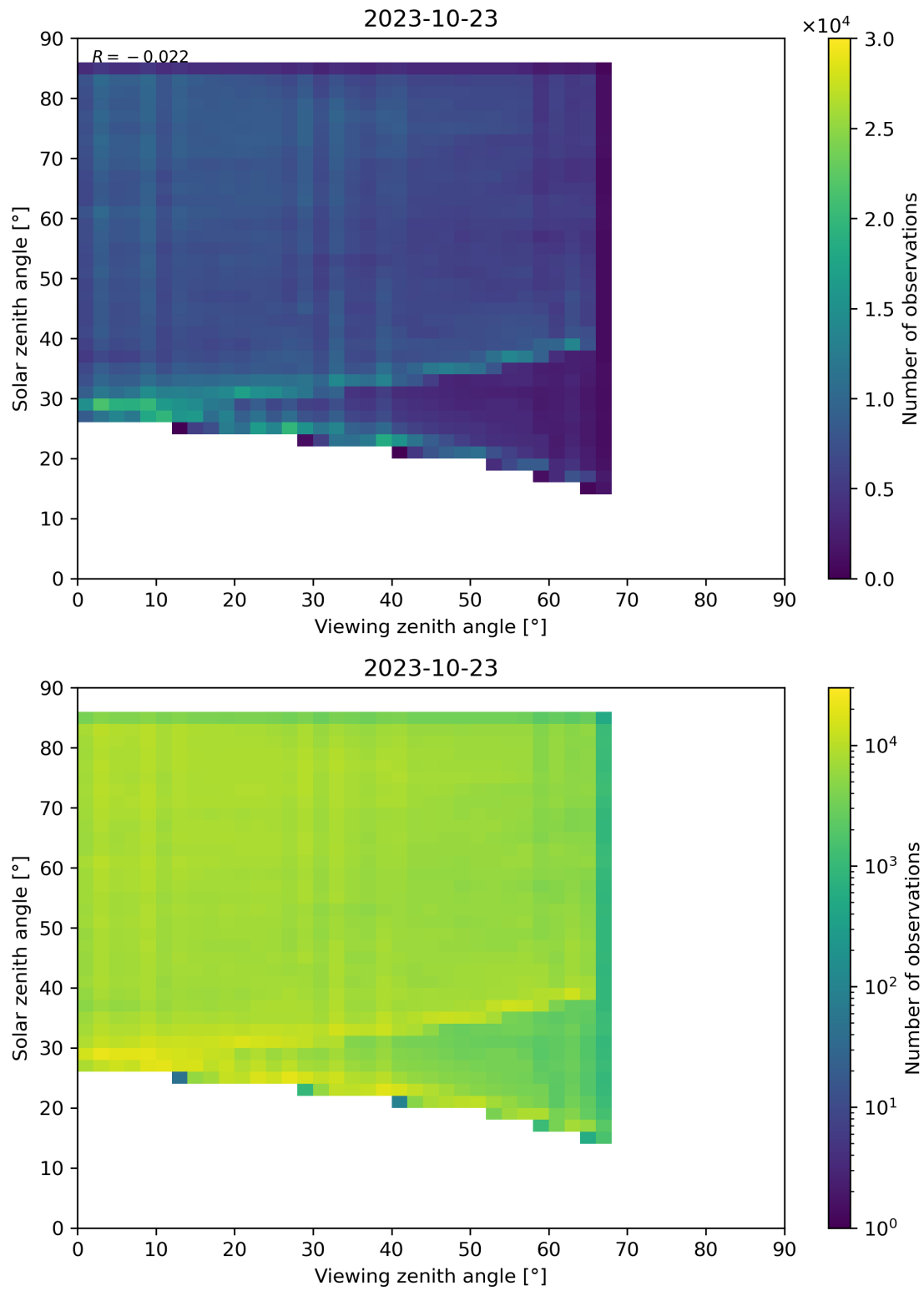
Figure 77: Scatter density plot of “Viewing zenith angle” against “Solar zenith angle” for 2023-10-22 to 2023-10-24.
