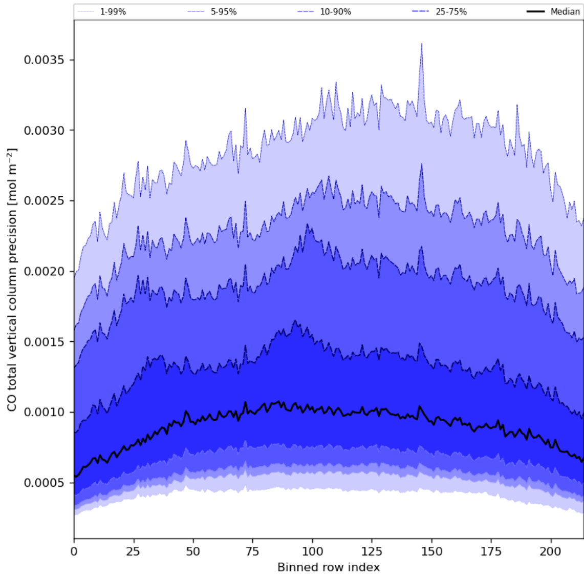
Figure 28: Along track statistics of “CO total vertical column precision” for 2023-10-22 to 2023-10-24
