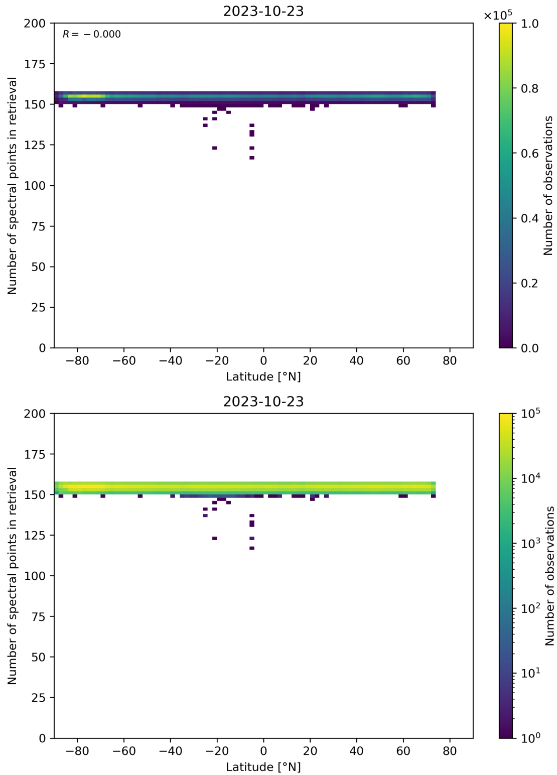
Figure 57: Scatter density plot of “Latitude” against “Number of spectral points in retrieval” for 2023-10-22 to 2023-10-24.
