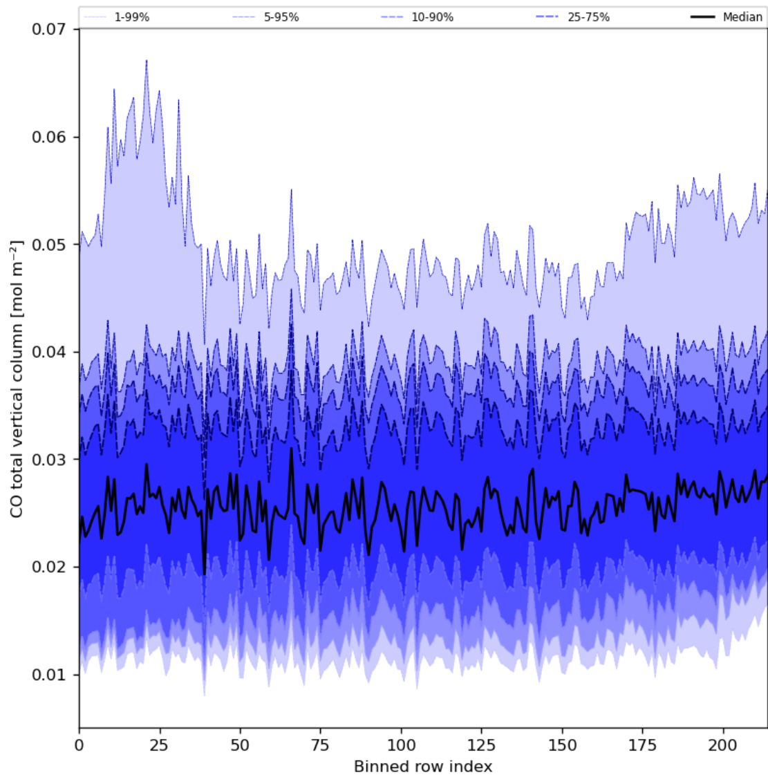
Figure 26: Along track statistics of “CO total vertical column” for 2023-10-22 to 2023-10-24
