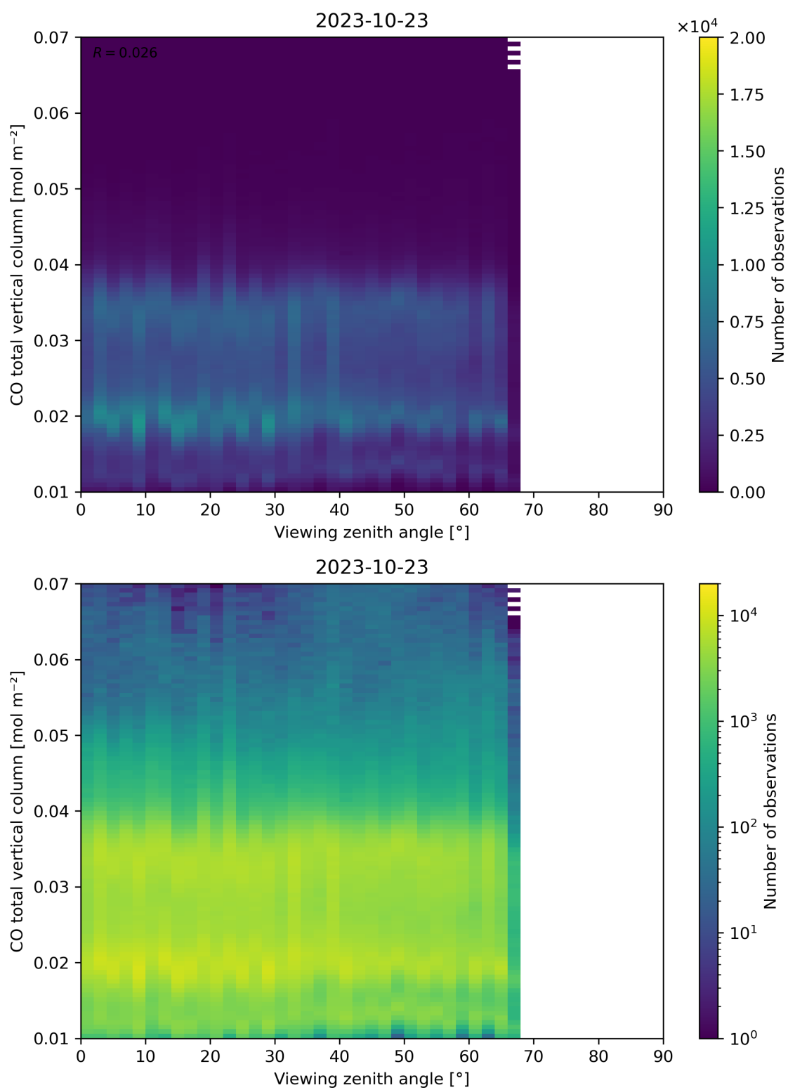
Figure 69: Scatter density plot of “Viewing zenith angle” against “CO total vertical column” for 2023-10-22 to 2023-10-24.
