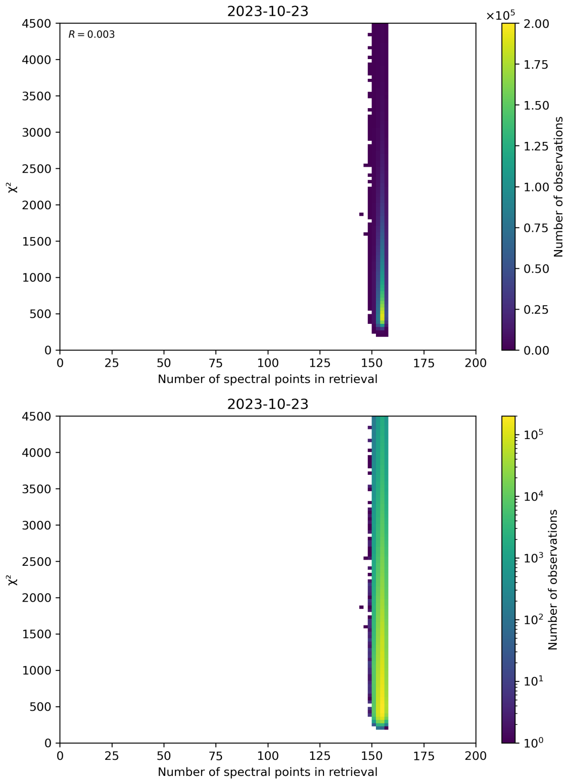
Figure 58: Scatter density plot of “Number of spectral points in retrieval” against “ \chi^2 ” for 2023-10-22 to 2023-10-24.
