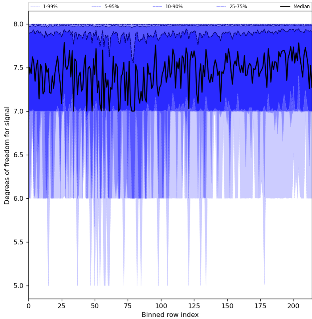
Figure 31: Along track statistics of “Degrees of freedom for signal” for 2023-10-22 to 2023-10-24
