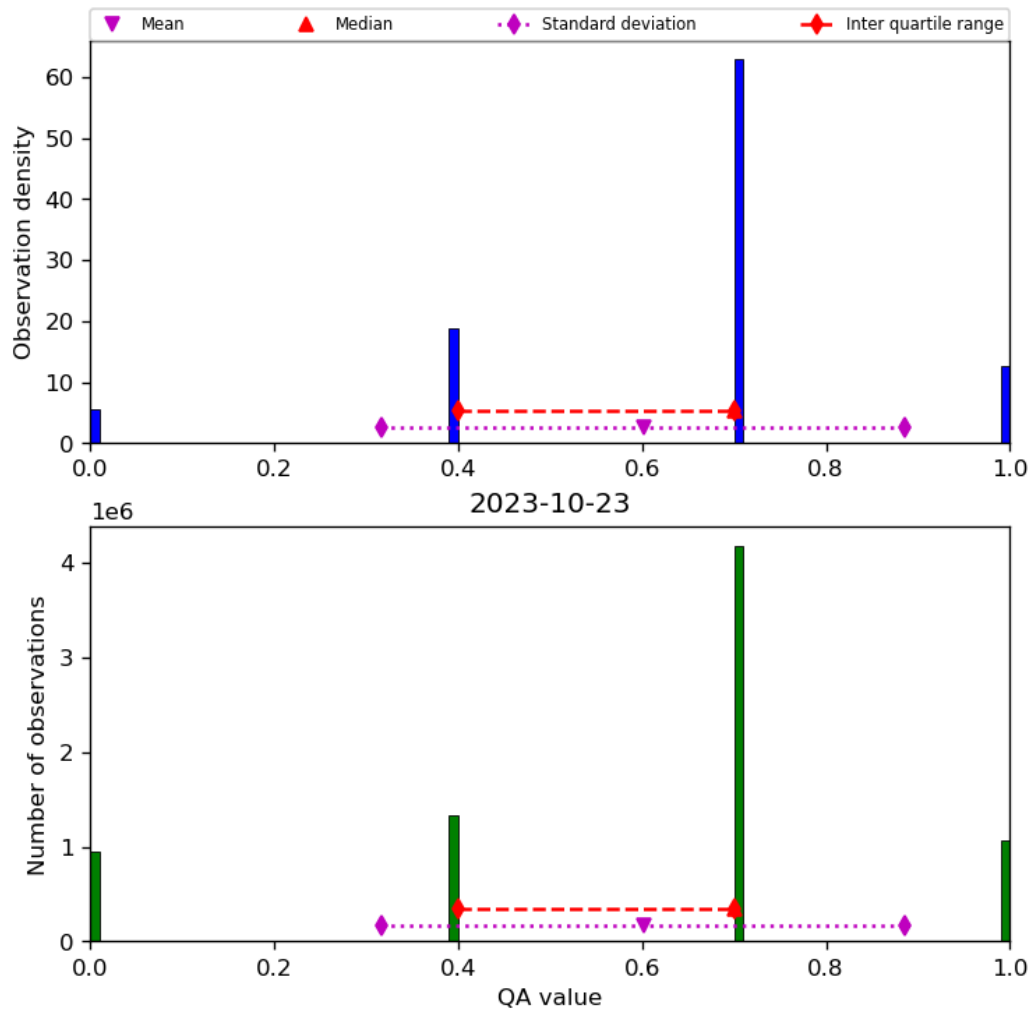
Figure 17: Histogram of “QA value” for 2023-10-22 to 2023-10-24
