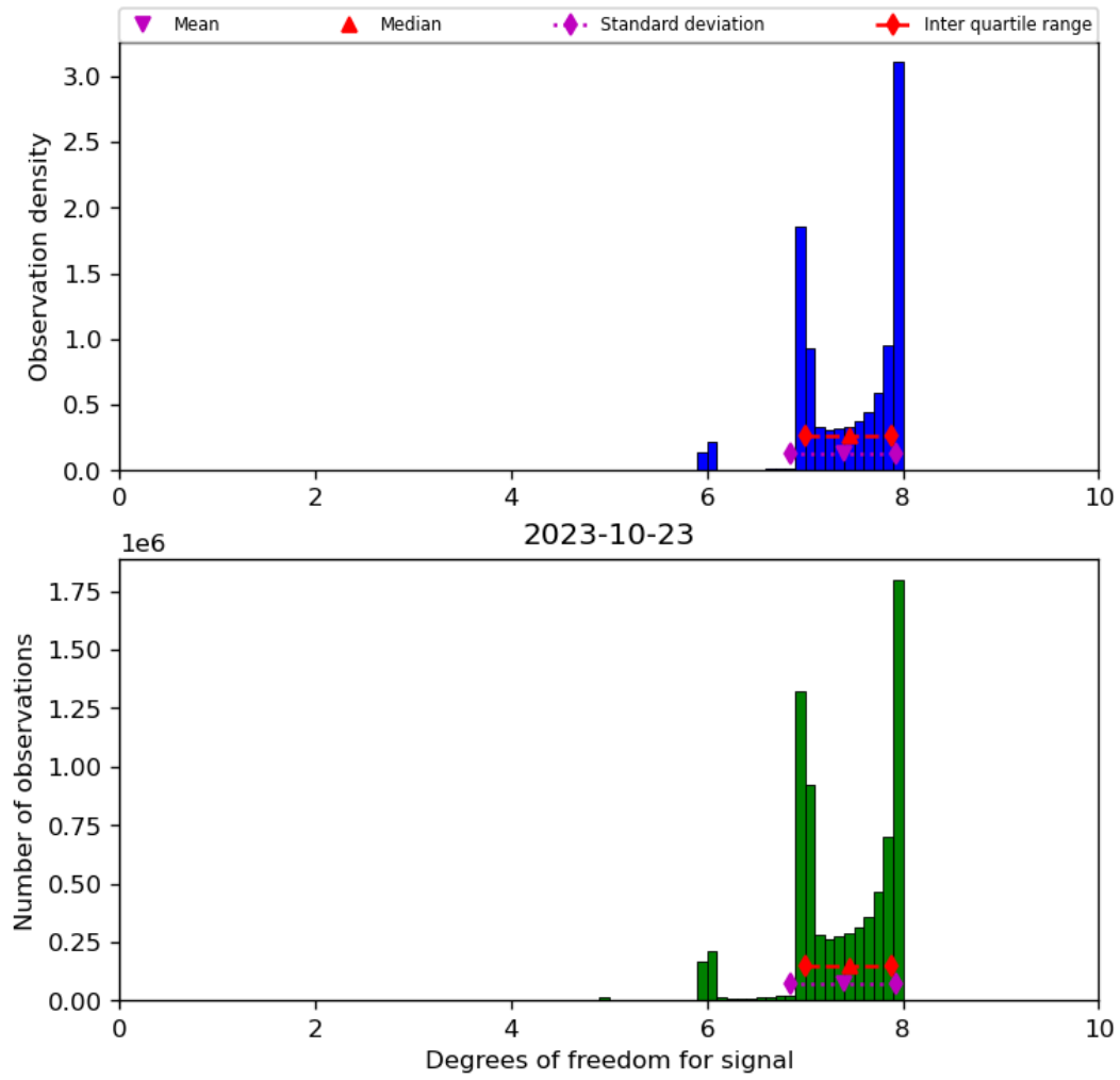
Figure 23: Histogram of “Degrees of freedom for signal” for 2023-10-22 to 2023-10-24
