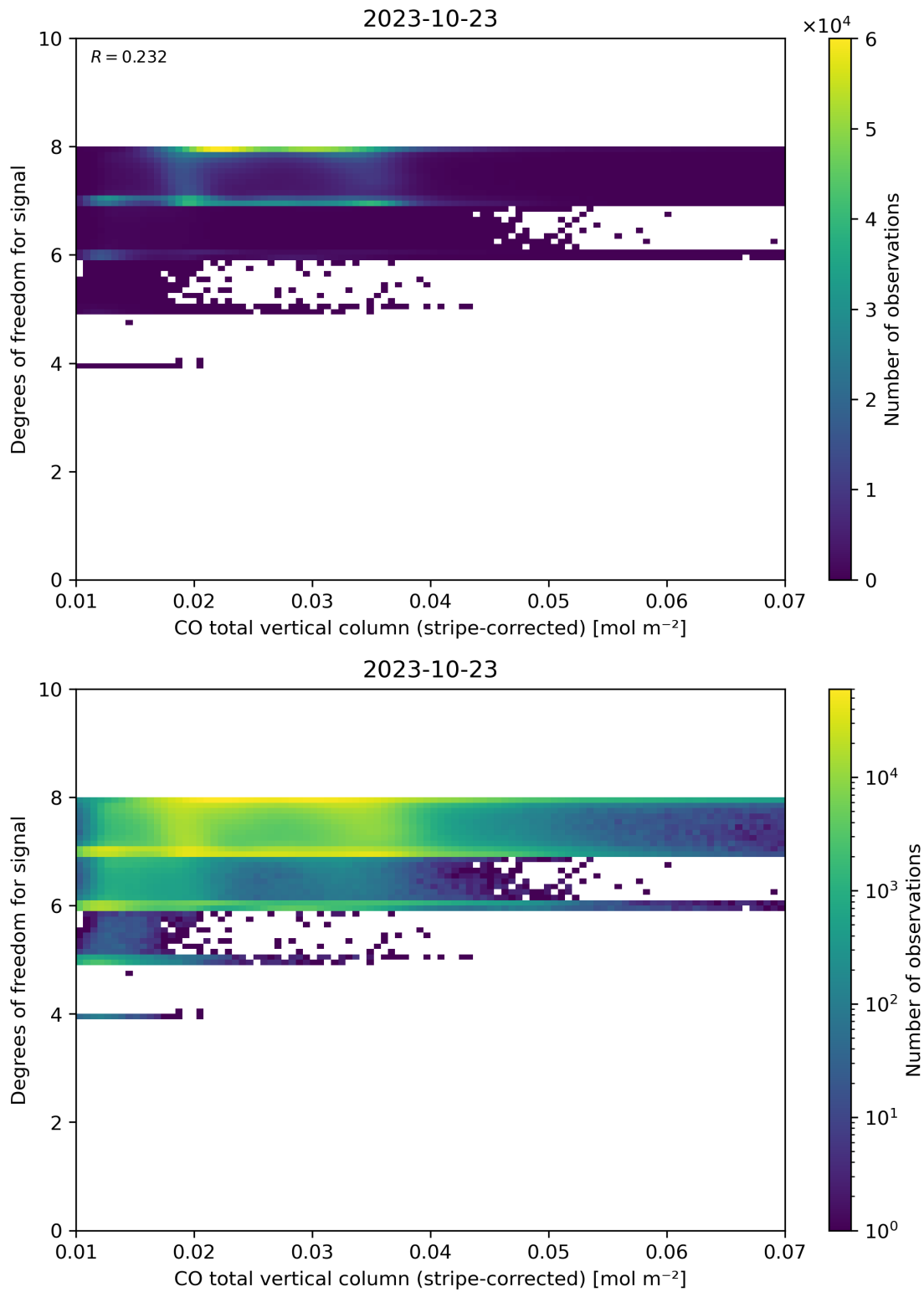
Figure 38: Scatter density plot of “CO total vertical column (stripe-corrected)” against “Degrees of freedom for signal” for 2023-10-22 to 2023-10-24.
