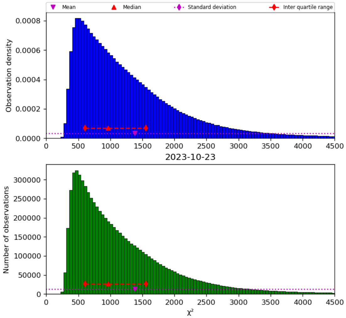
Figure 22: Histogram of “ \chi^2 ” for 2023-10-22 to 2023-10-24
