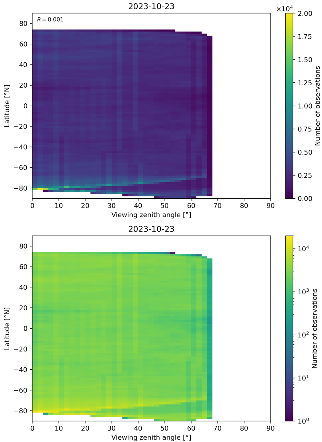
Figure 74: Scatter density plot of “Viewing zenith angle” against “Latitude” for 2023-10-22 to 2023-10-24.
