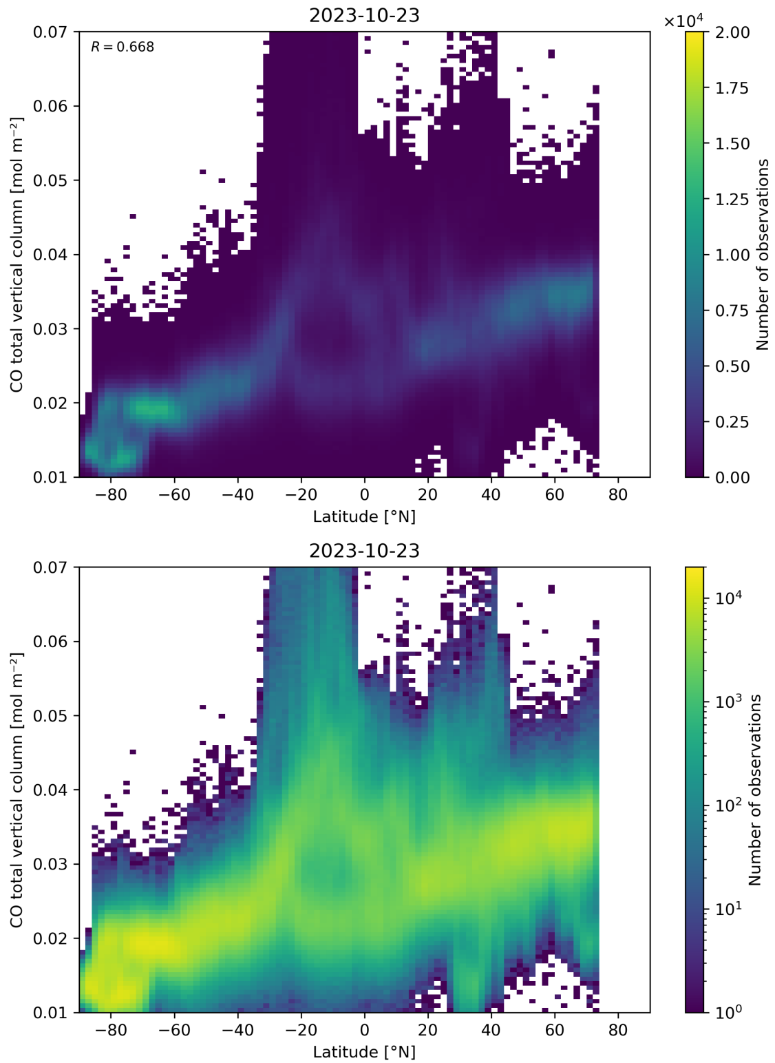
Figure 51: Scatter density plot of “Latitude” against “CO total vertical column” for 2023-10-22 to 2023-10-24.
