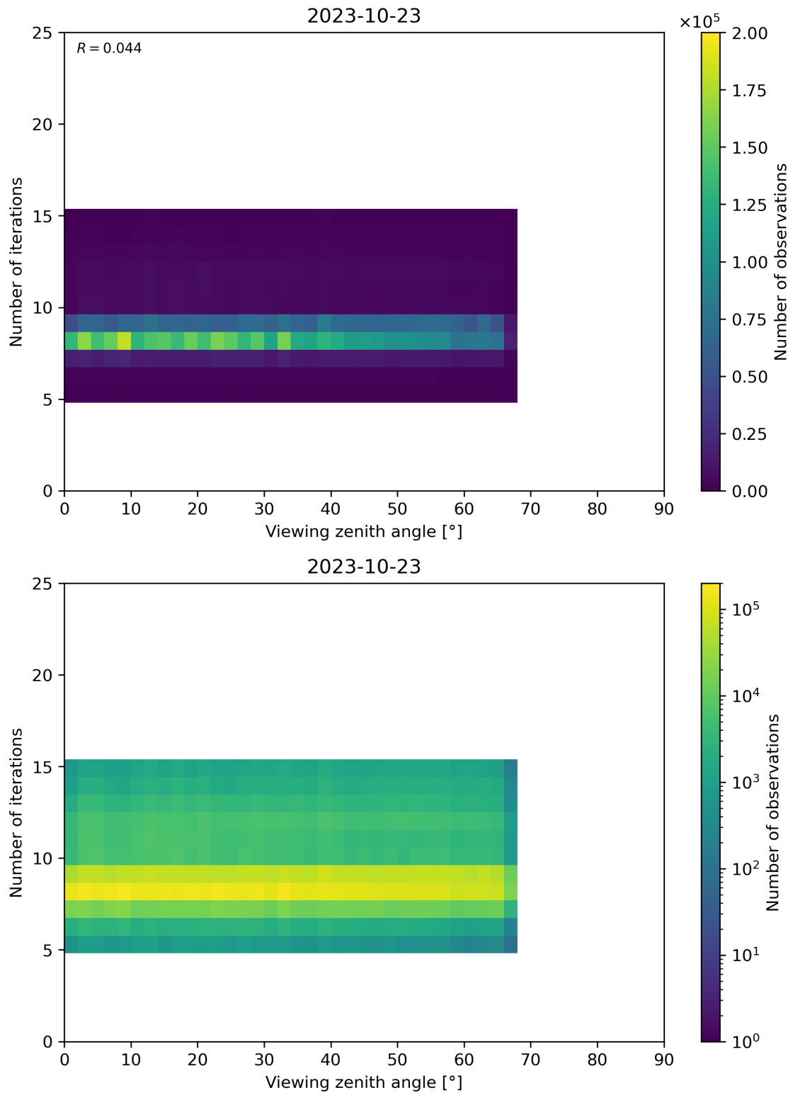
Figure 75: Scatter density plot of “Viewing zenith angle” against “Number of iterations” for 2023-10-22 to 2023-10-24.
