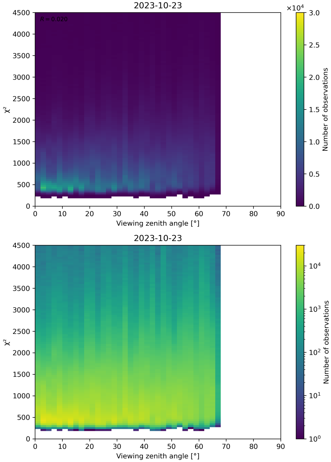
Figure 72: Scatter density plot of “Viewing zenith angle” against “ \chi^2 ” for 2023-10-22 to 2023-10-24.
