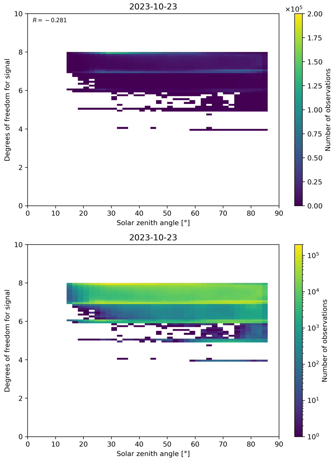
Figure 65: Scatter density plot of “Solar zenith angle” against “Degrees of freedom for signal” for 2023-10-22 to 2023-10-24.
