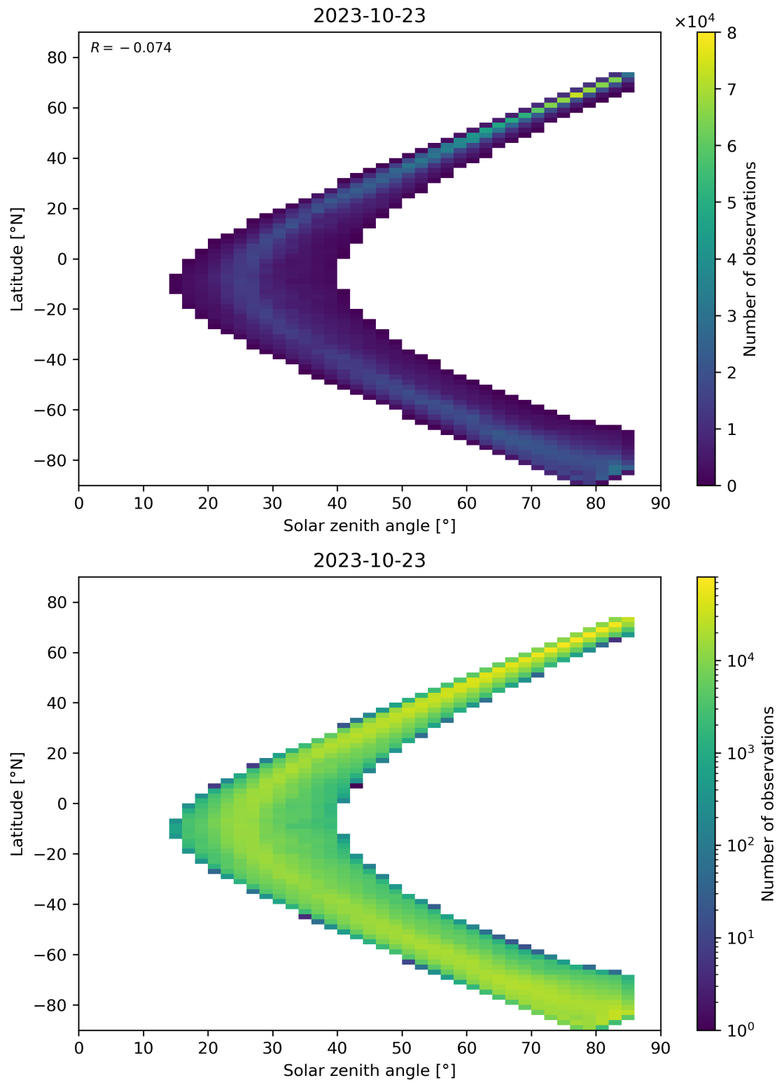
Figure 66: Scatter density plot of “Solar zenith angle” against “Latitude” for 2023-10-22 to 2023-10-24.
