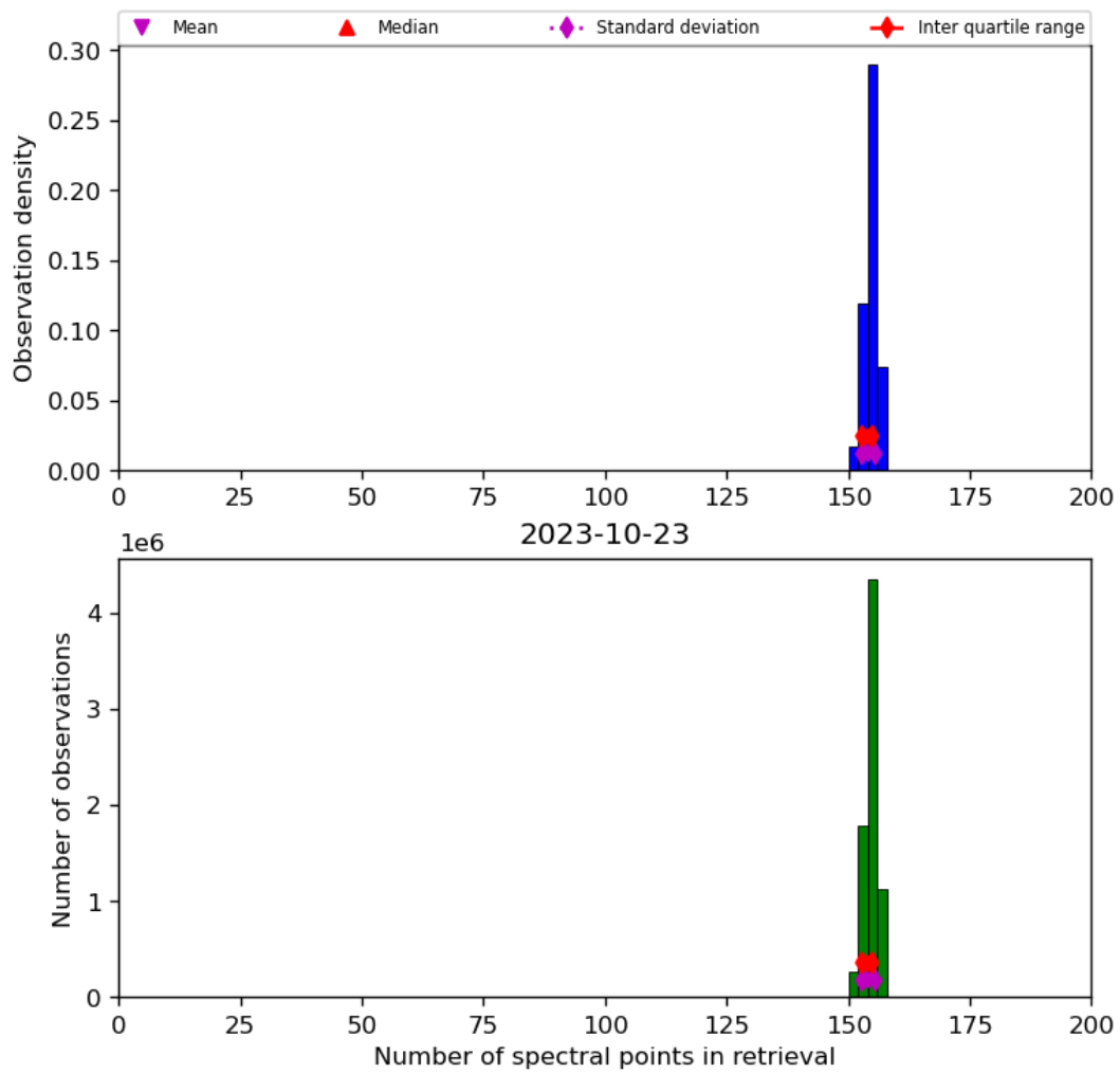
Figure 21: Histogram of “Number of spectral points in retrieval” for 2023-10-22 to 2023-10-24
