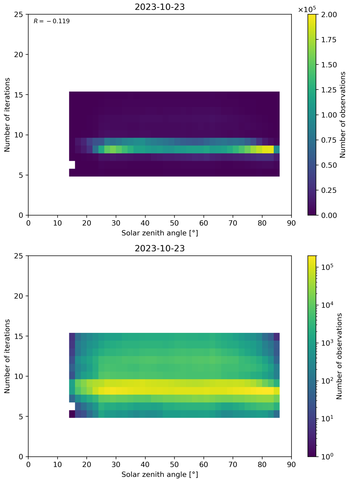
Figure 67: Scatter density plot of “Solar zenith angle” against “Number of iterations” for 2023-10-22 to 2023-10-24.
