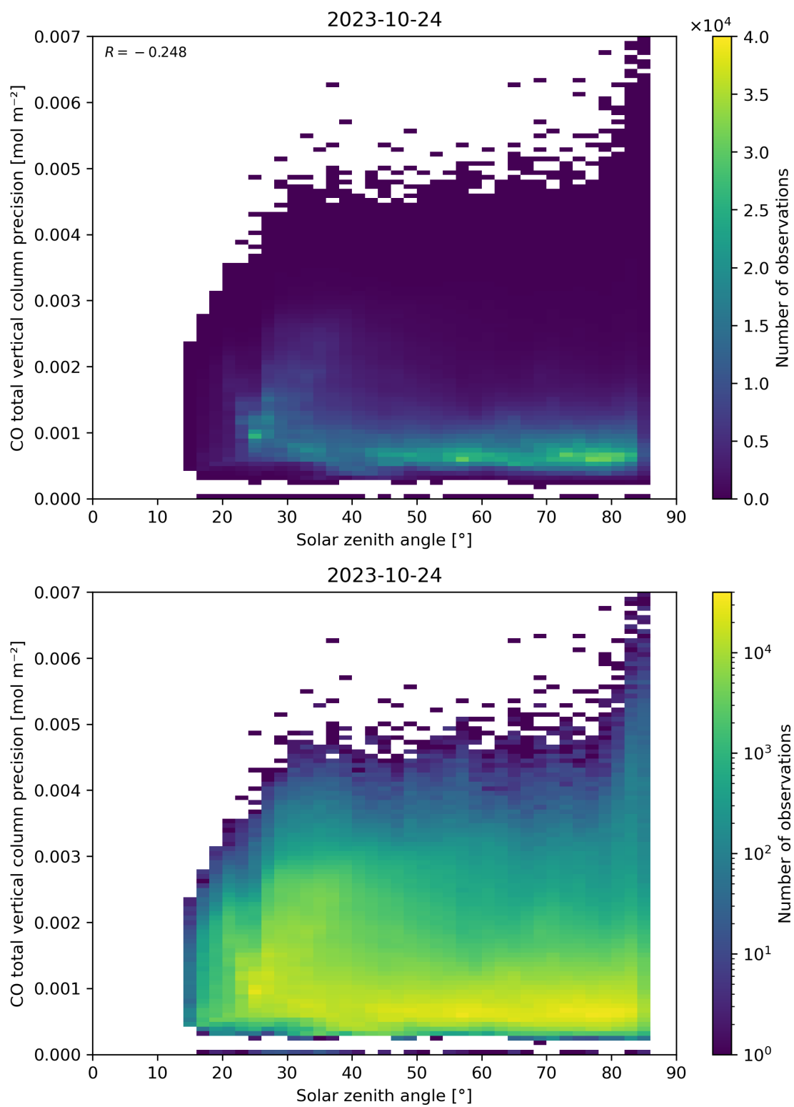
Figure 63: Scatter density plot of “Solar zenith angle” against “CO total vertical column precision” for 2023-10-23 to 2023-10-25.
