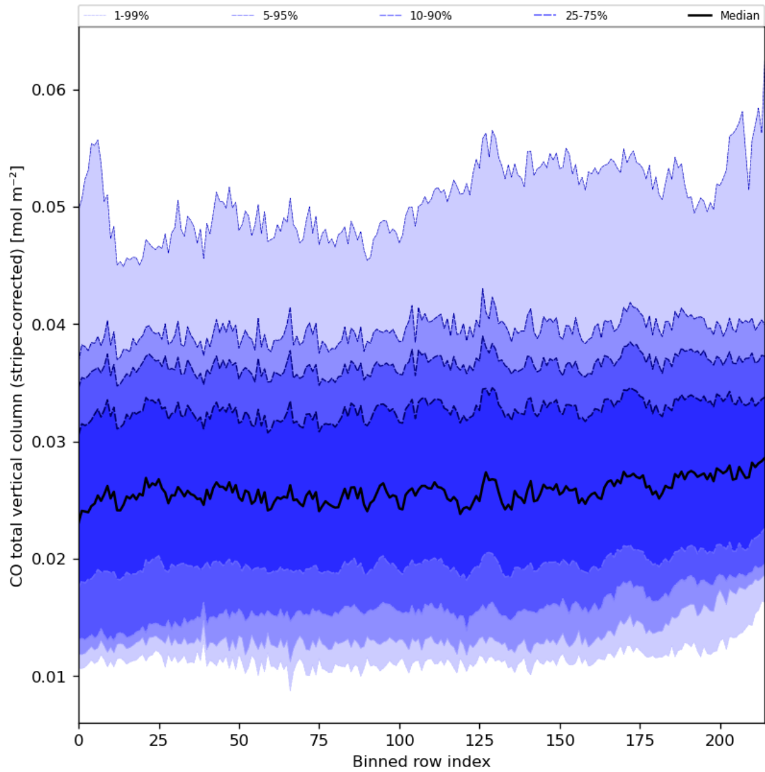
Figure 27: Along track statistics of “CO total vertical column (stripe-corrected)” for 2023-10-23 to 2023-10-25
