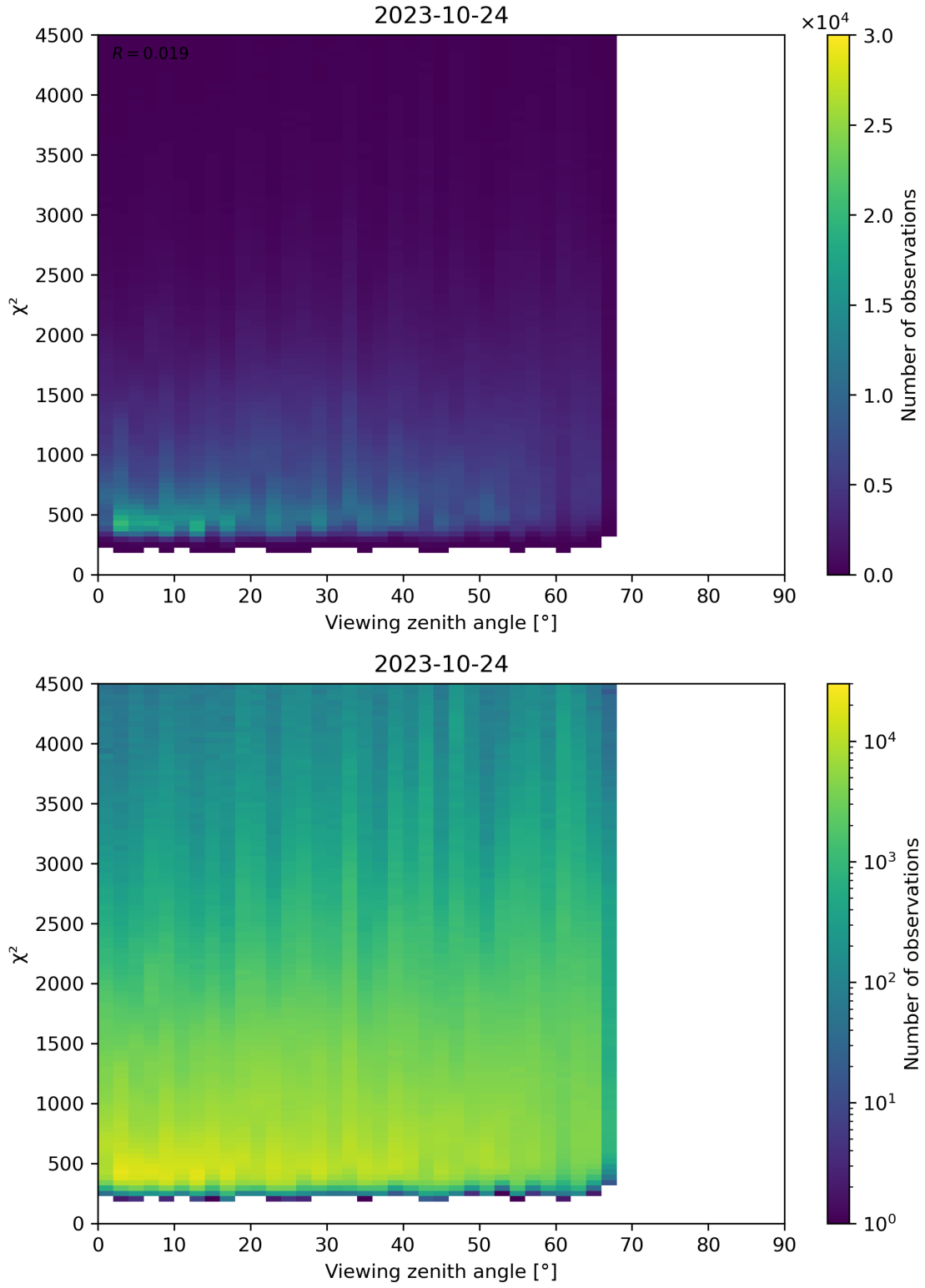
Figure 72: Scatter density plot of “Viewing zenith angle” against “ \chi^2 ” for 2023-10-23 to 2023-10-25.
