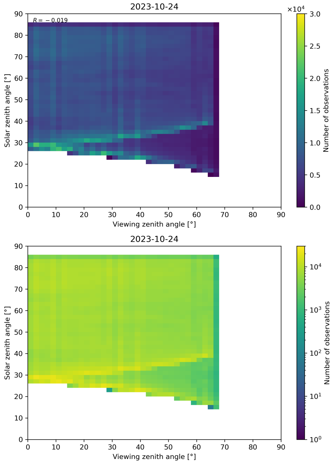
Figure 77: Scatter density plot of “Viewing zenith angle” against “Solar zenith angle” for 2023-10-23 to 2023-10-25.
