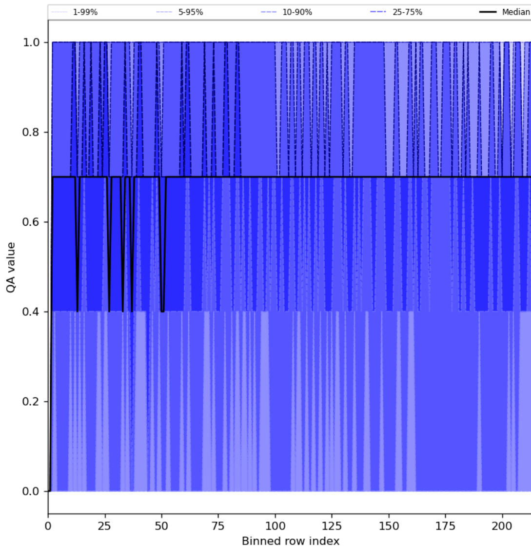
Figure 25: Along track statistics of “QA value” for 2023-10-23 to 2023-10-25
