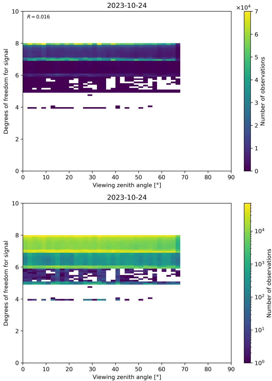
Figure 73: Scatter density plot of “Viewing zenith angle” against “Degrees of freedom for signal” for 2023-10-23 to 2023-10-25.
