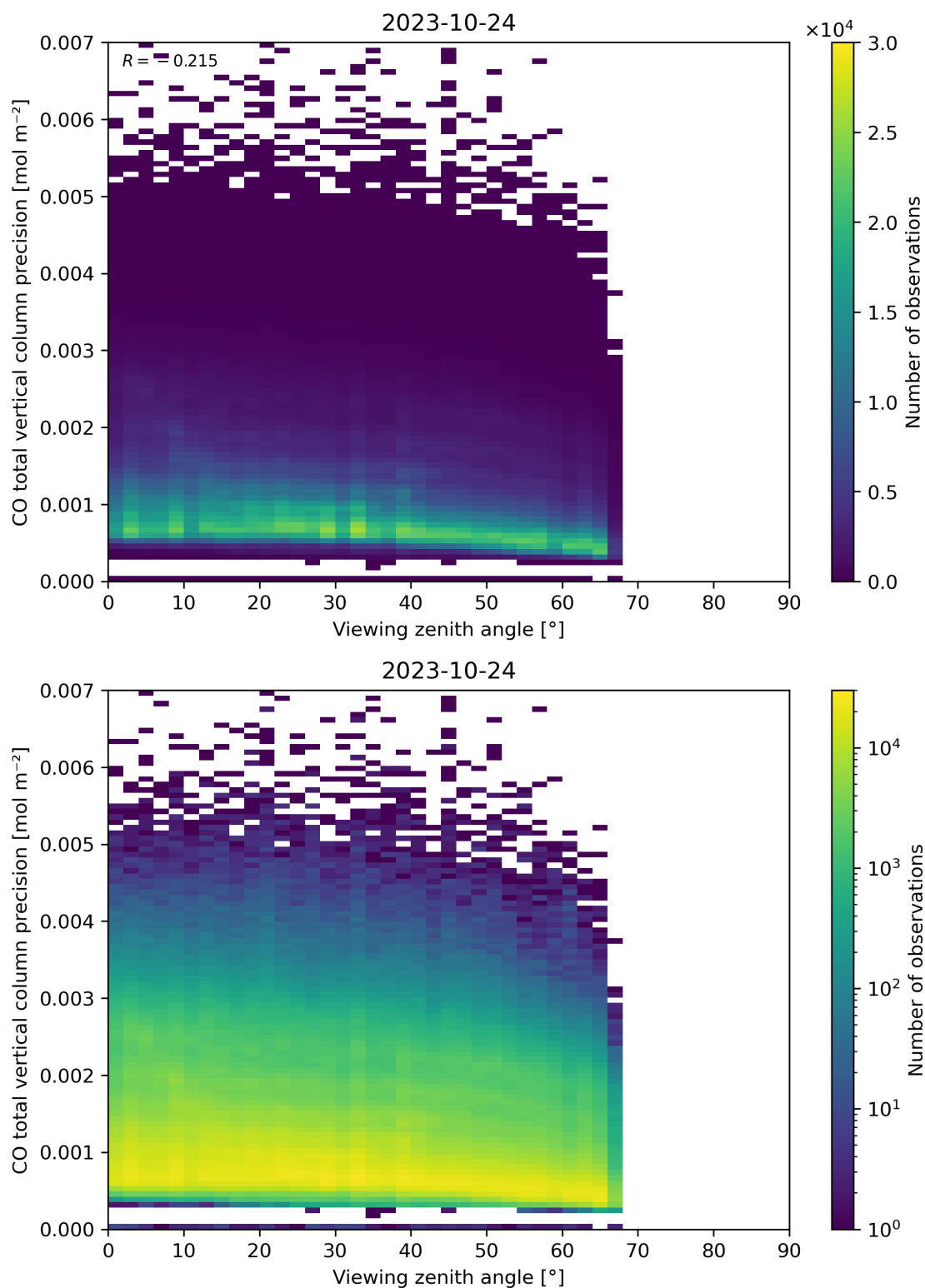
Figure 71: Scatter density plot of “Viewing zenith angle” against “CO total vertical column precision” for 2023-10-23 to 2023-10-25.
