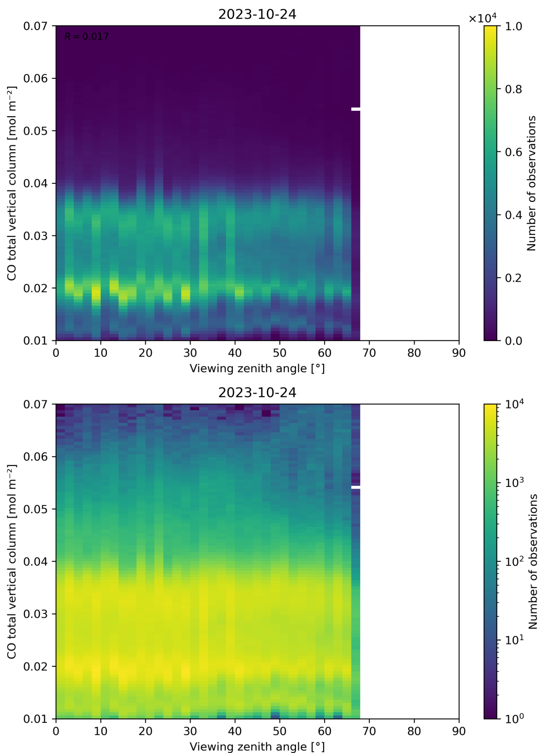
Figure 69: Scatter density plot of “Viewing zenith angle” against “CO total vertical column” for 2023-10-23 to 2023-10-25.
