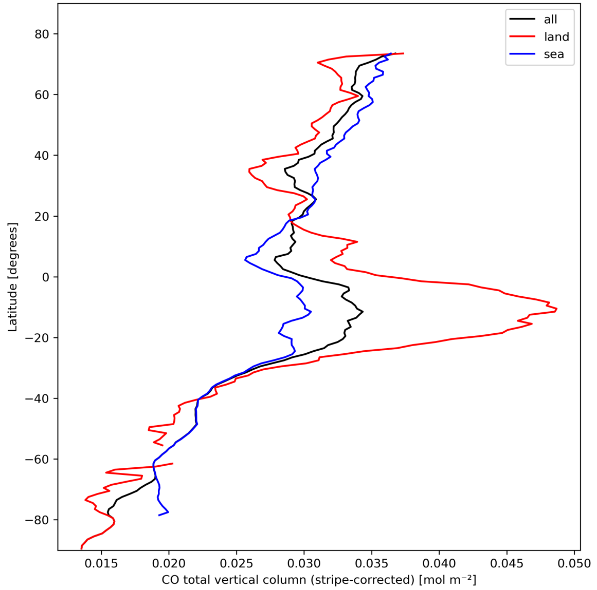
Figure 11: Zonal average of “CO total vertical column (stripe-corrected)” for 2023-10-23 to 2023-10-25.
