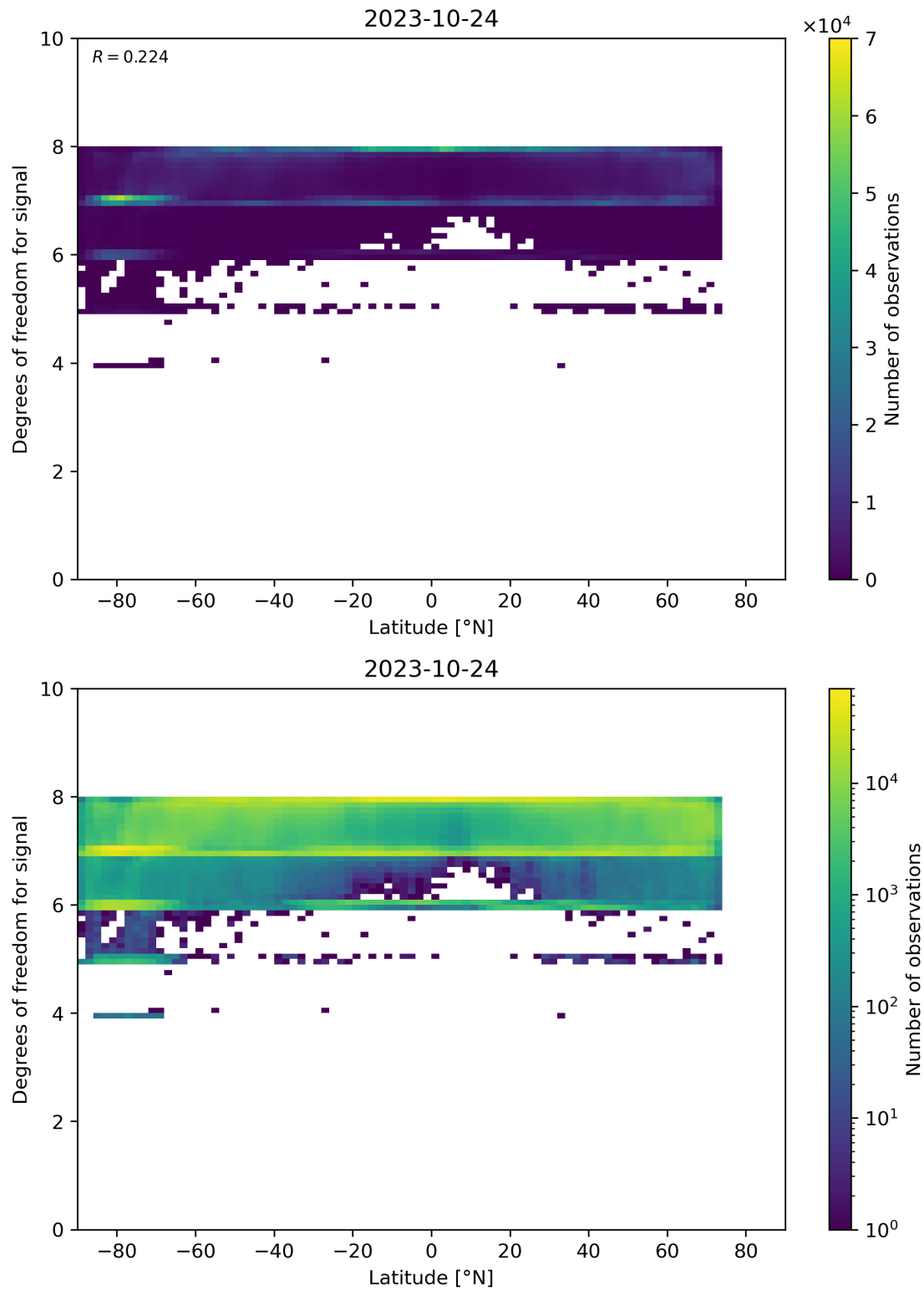
Figure 55: Scatter density plot of “Latitude” against “Degrees of freedom for signal” for 2023-10-23 to 2023-10-25.
