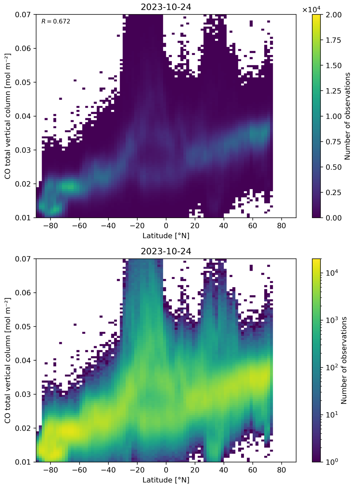
Figure 51: Scatter density plot of “Latitude” against “CO total vertical column” for 2023-10-23 to 2023-10-25.
