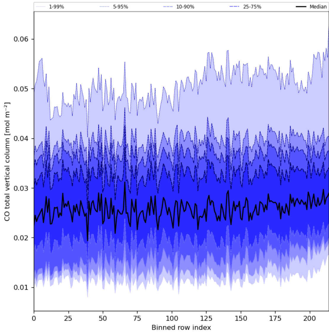
Figure 26: Along track statistics of “CO total vertical column” for 2023-10-23 to 2023-10-25
