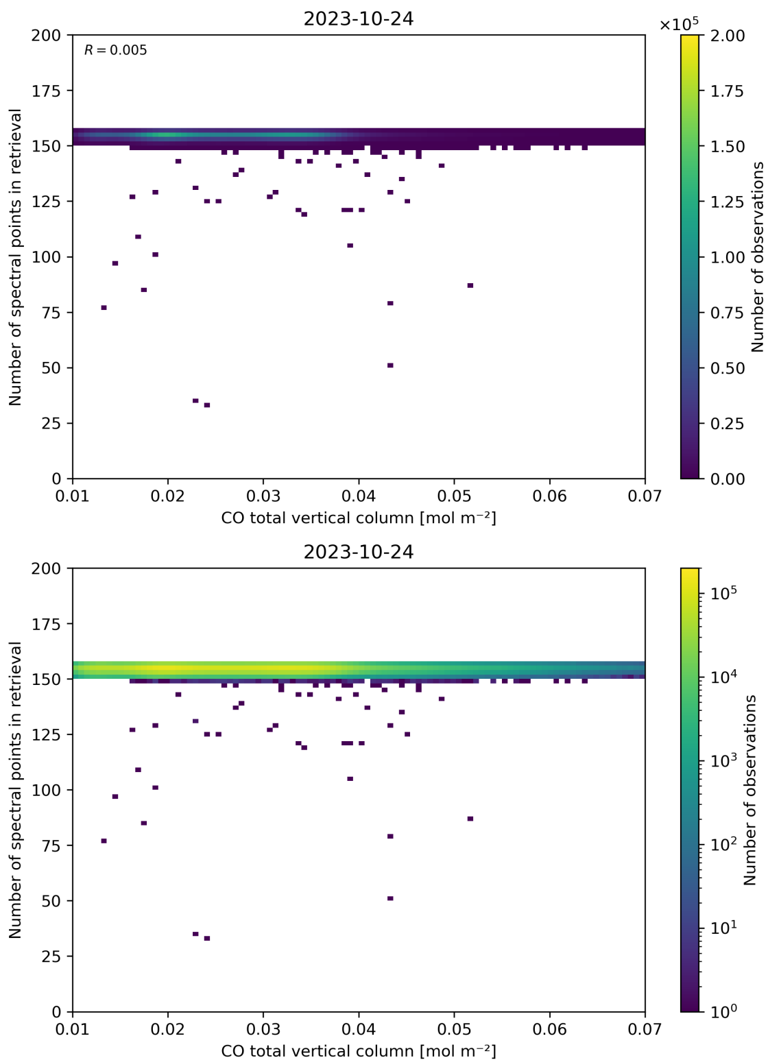
Figure 43: Scatter density plot of “CO total vertical column” against “Number of spectral points in retrieval” for 2023-10-23 to 2023-10-25.
