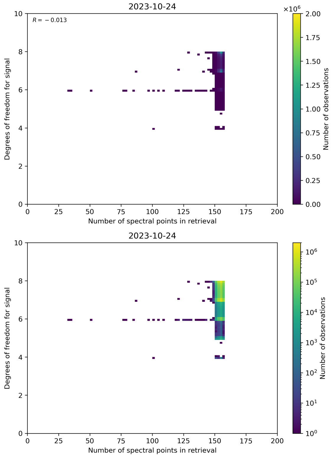
Figure 59: Scatter density plot of “Number of spectral points in retrieval” against “Degrees of freedom for signal” for 2023-10-23 to 2023-10-25.
