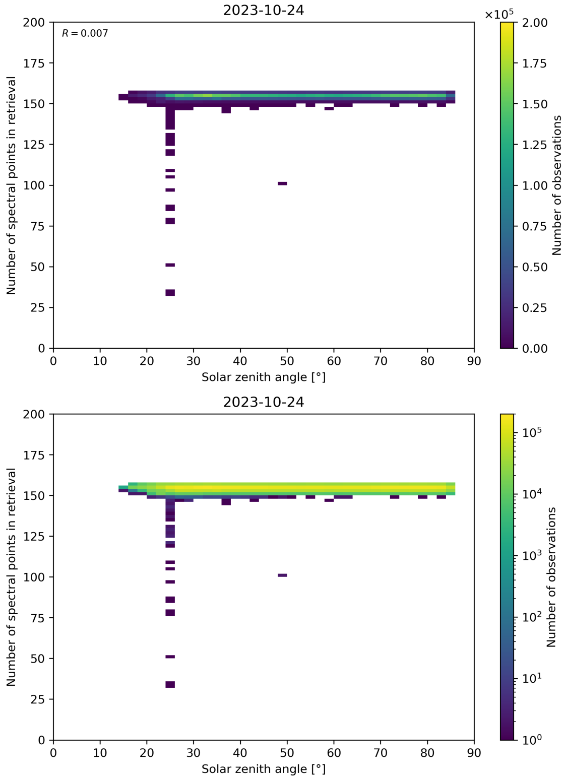
Figure 68: Scatter density plot of “Solar zenith angle” against “Number of spectral points in retrieval” for 2023-10-23 to 2023-10-25.
