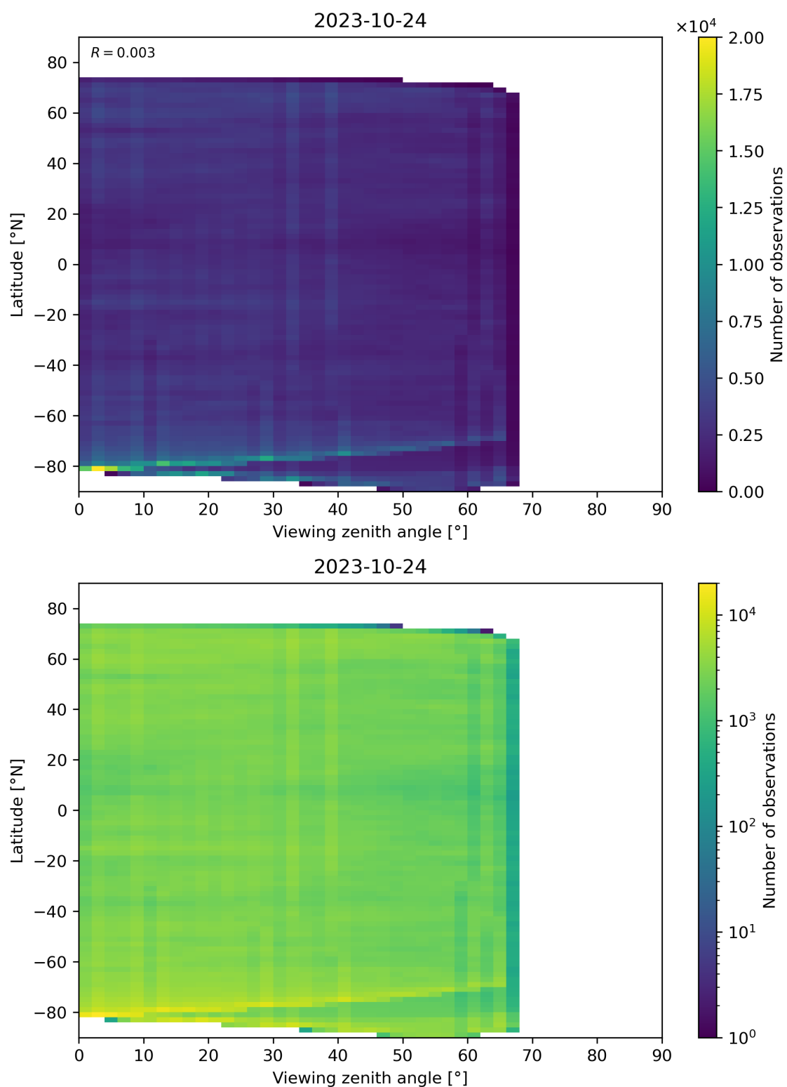
Figure 74: Scatter density plot of “Viewing zenith angle” against “Latitude” for 2023-10-23 to 2023-10-25.
