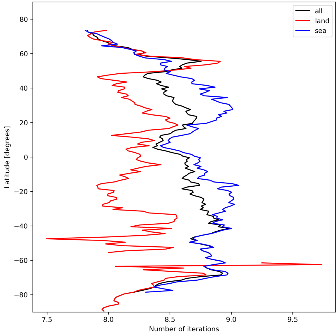
Figure 16: Zonal average of “Number of iterations” for 2023-10-23 to 2023-10-25.
