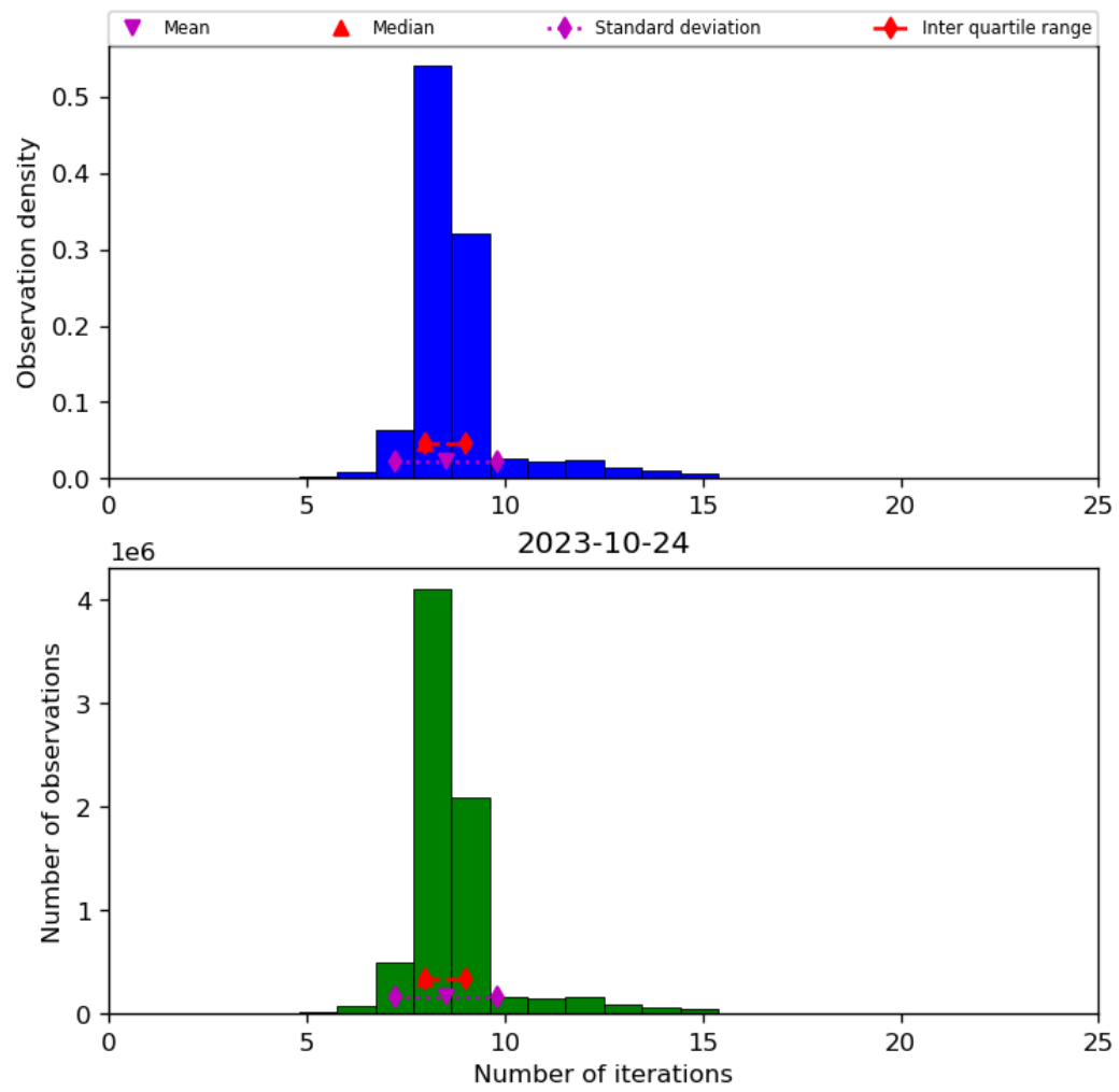
Figure 24: Histogram of “Number of iterations” for 2023-10-23 to 2023-10-25
