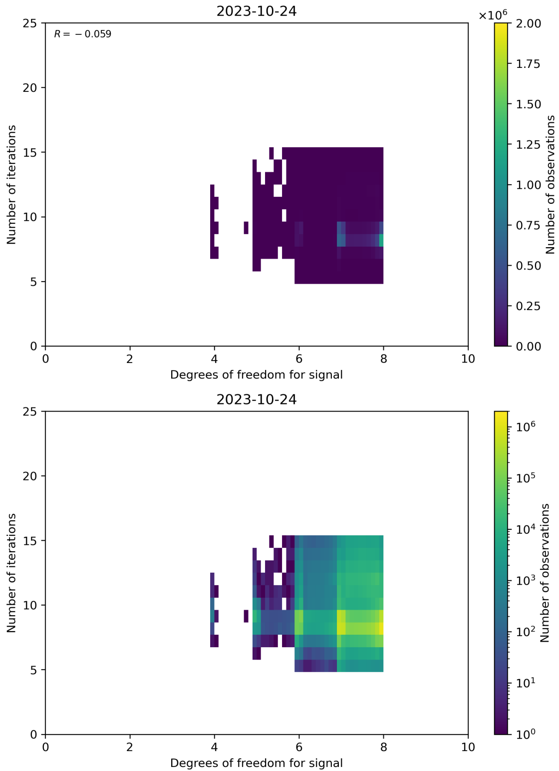
Figure 50: Scatter density plot of “Degrees of freedom for signal” against “Number of iterations” for 2023-10-23 to 2023-10-25.
