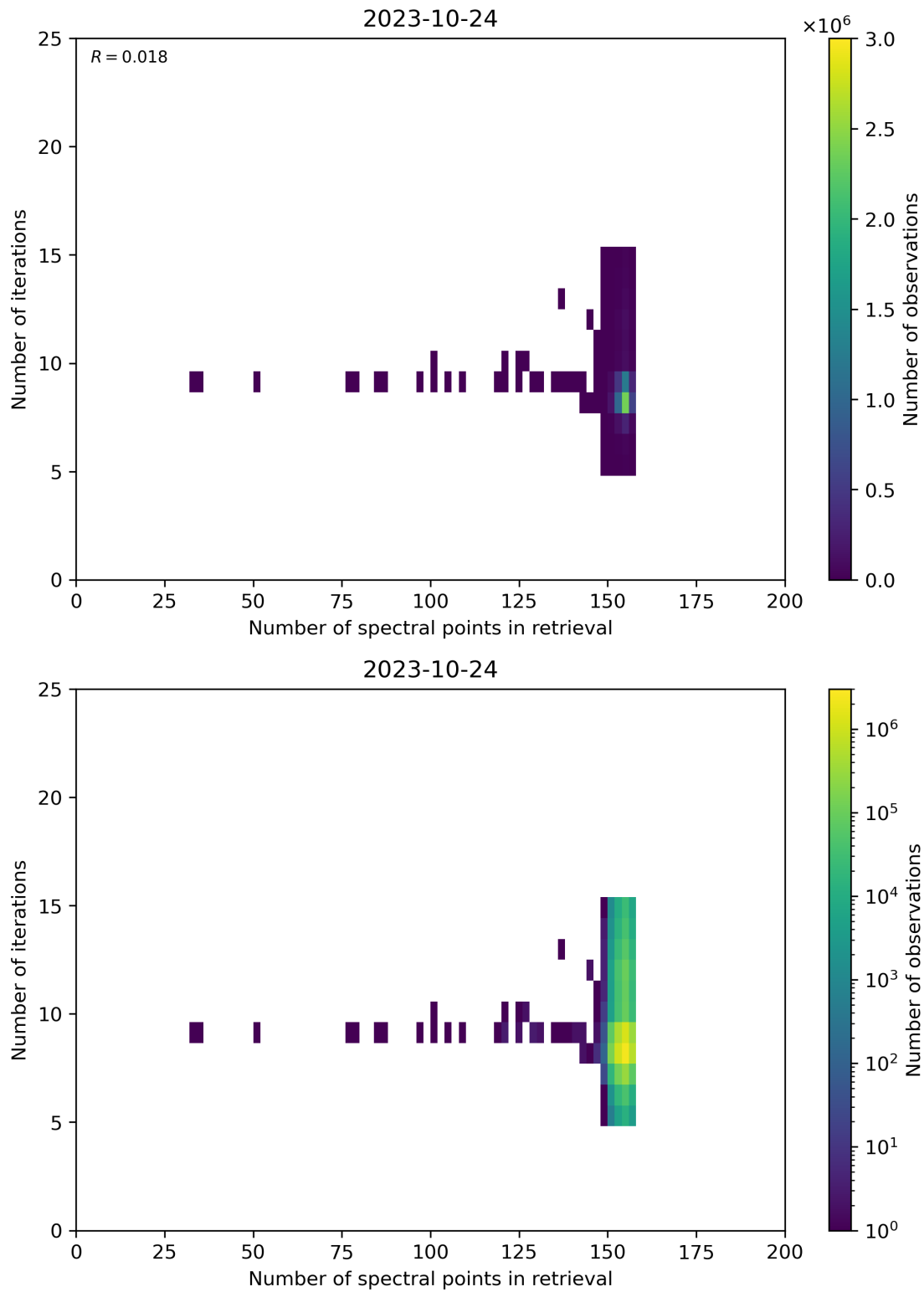
Figure 60: Scatter density plot of “Number of spectral points in retrieval” against “Number of iterations” for 2023-10-23 to 2023-10-25.
