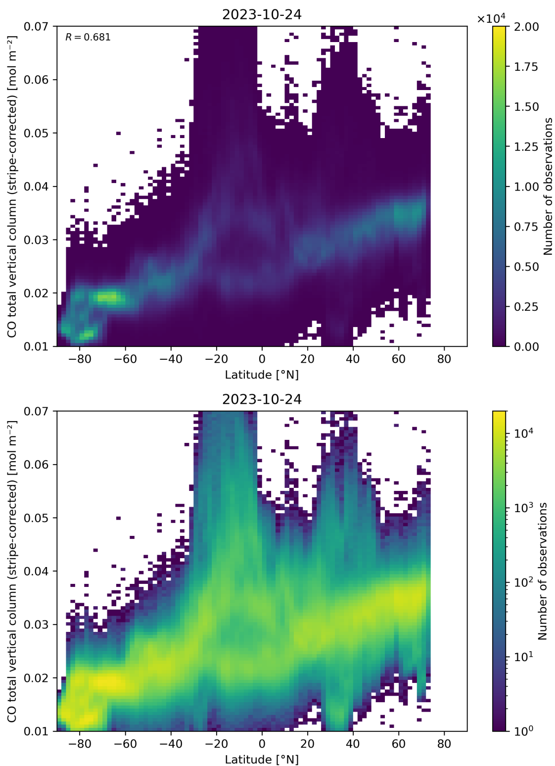
Figure 52: Scatter density plot of “Latitude” against “CO total vertical column (stripe-corrected)” for 2023-10-23 to 2023-10-25.
