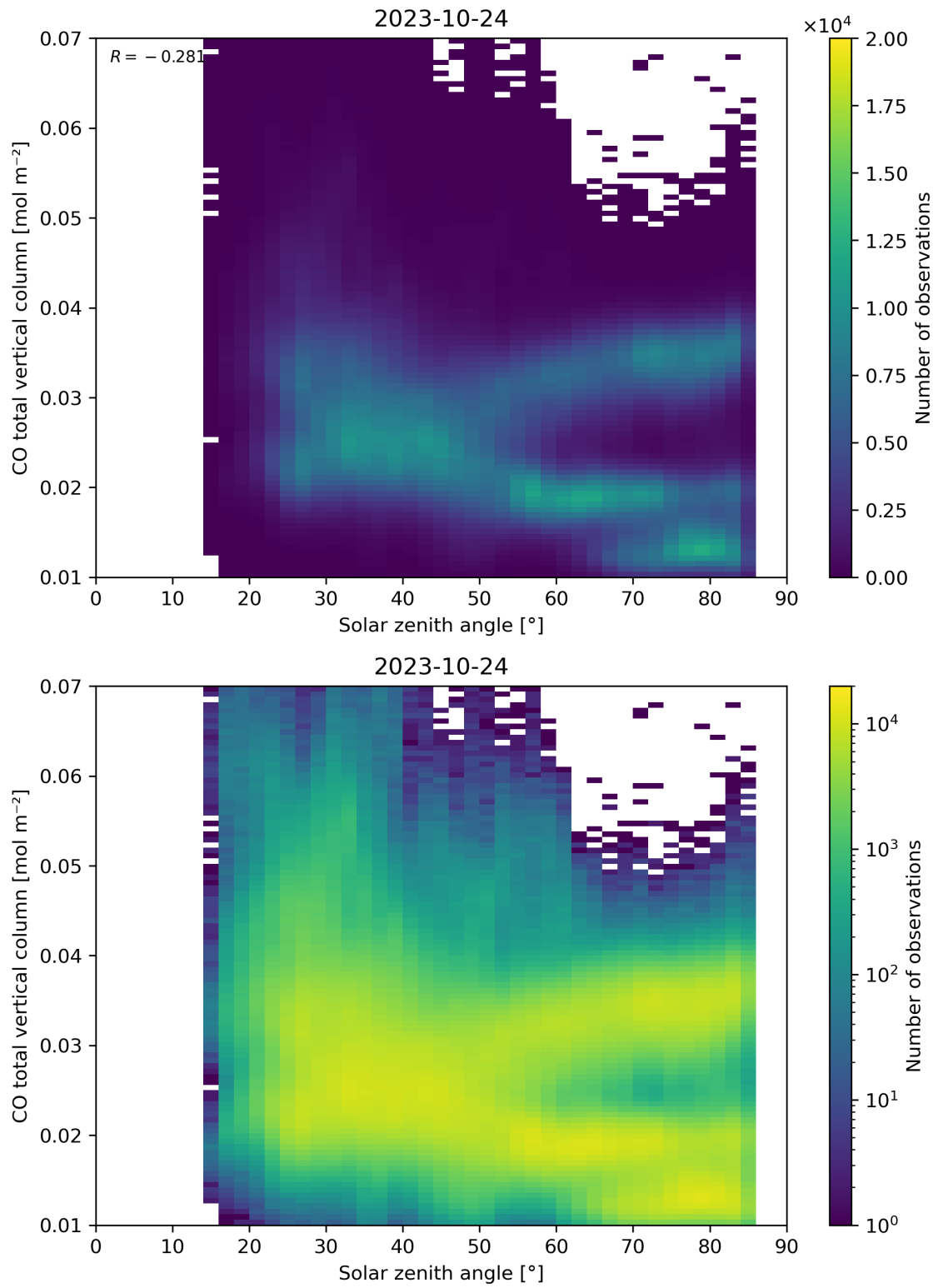
Figure 61: Scatter density plot of “Solar zenith angle” against “CO total vertical column” for 2023-10-23 to 2023-10-25.
