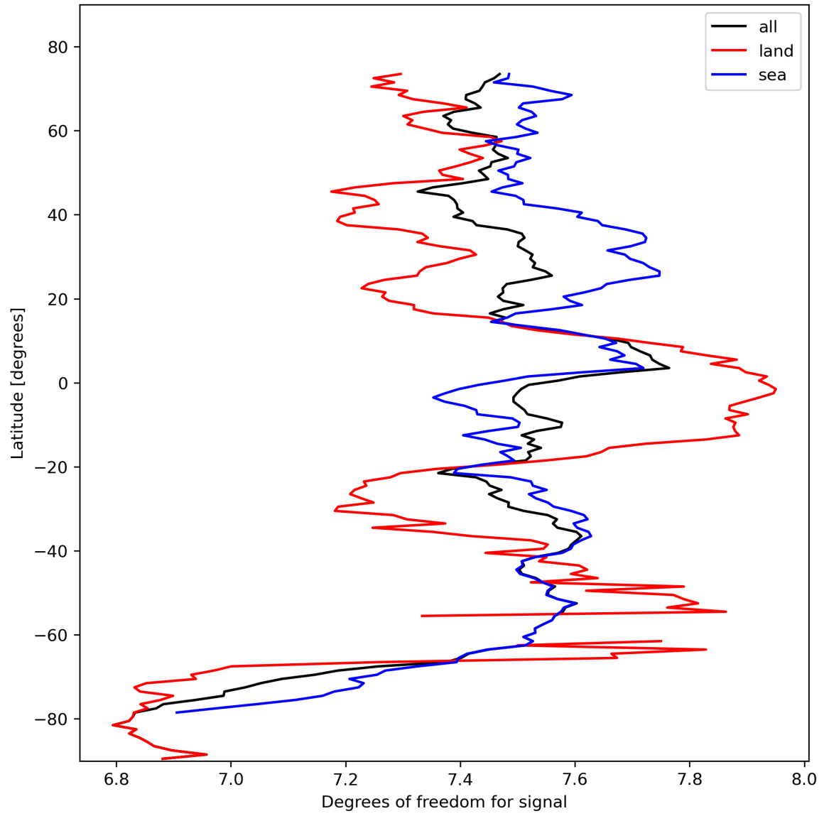
Figure 15: Zonal average of “Degrees of freedom for signal” for 2023-10-23 to 2023-10-25.
