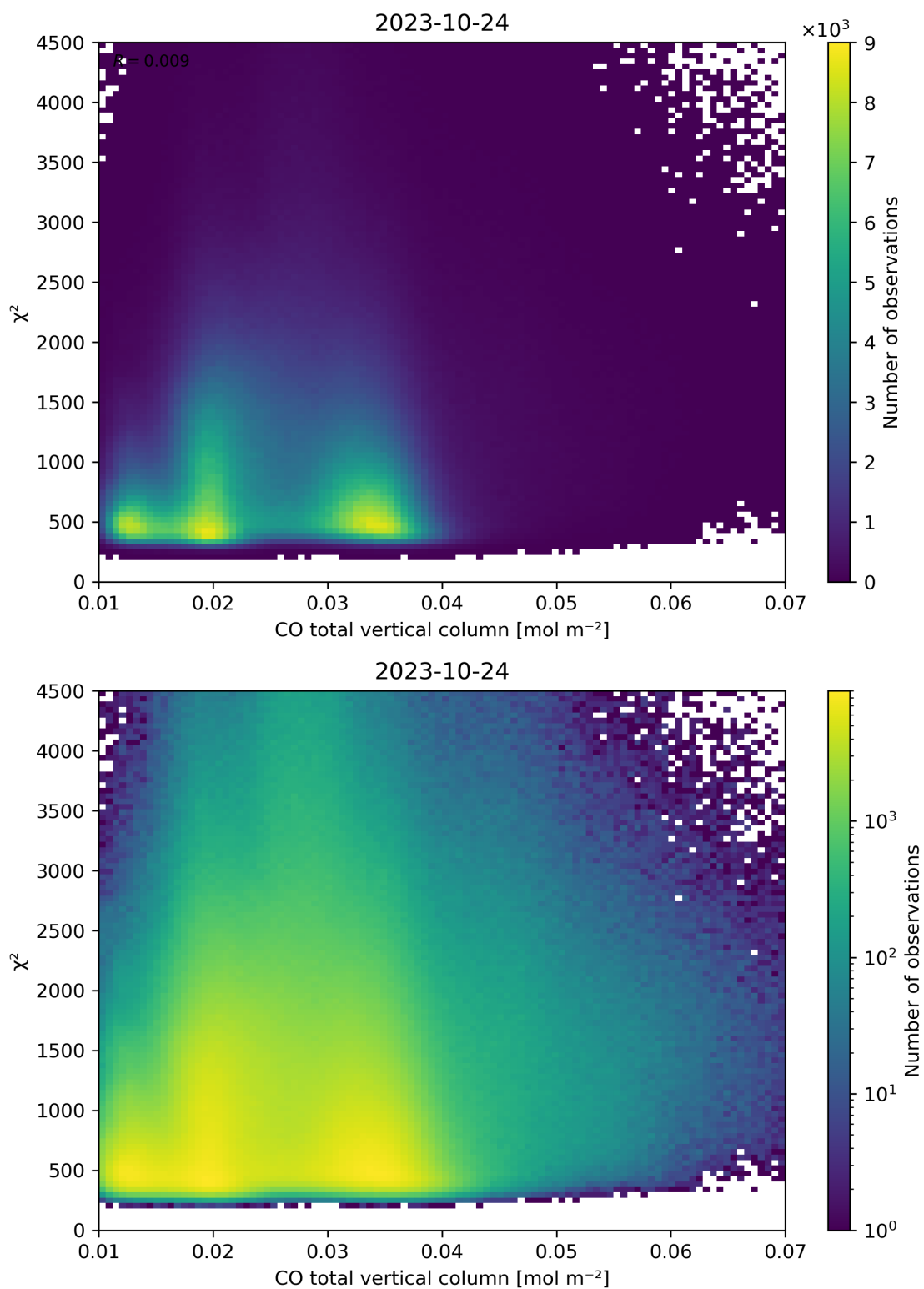
Figure 35: Scatter density plot of “CO total vertical column” against “ \chi^2 ” for 2023-10-23 to 2023-10-25.
