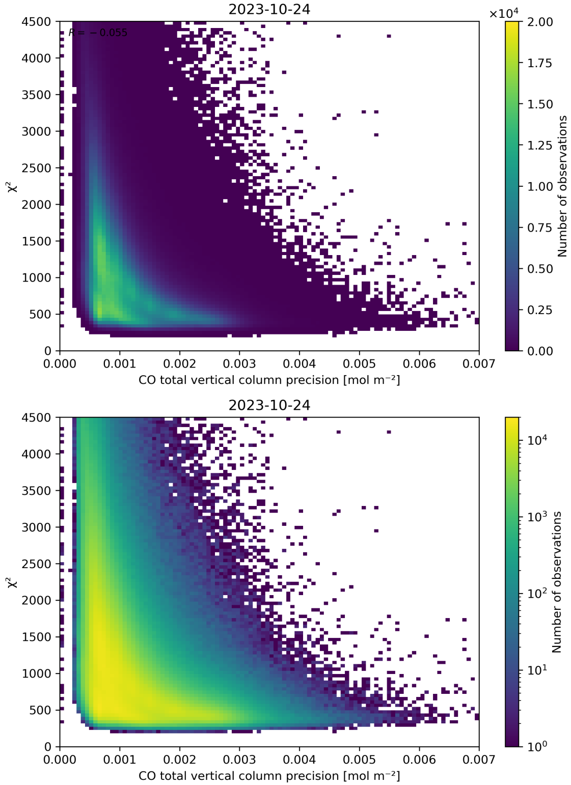
Figure 44: Scatter density plot of “CO total vertical column precision” against “ \chi^2 ” for 2023-10-23 to 2023-10-25.
