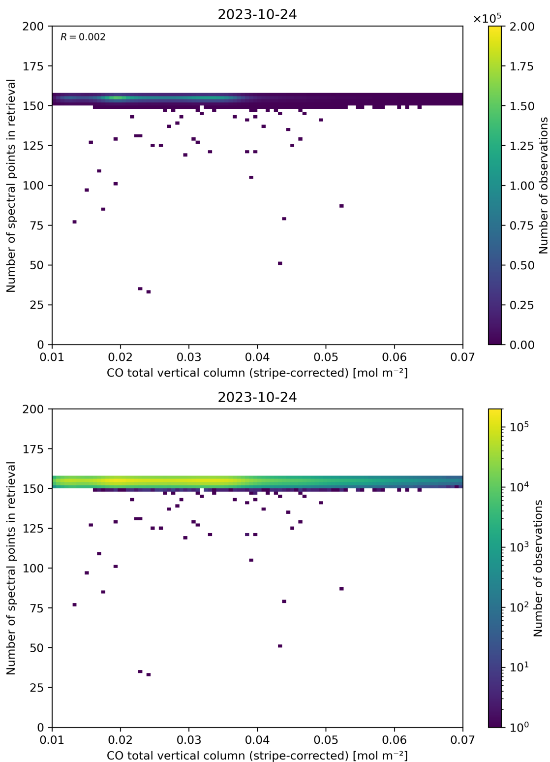
Figure 40: Scatter density plot of “CO total vertical column (stripe-corrected)” against “Number of spectral points in retrieval” for 2023-10-23 to 2023-10-25.
