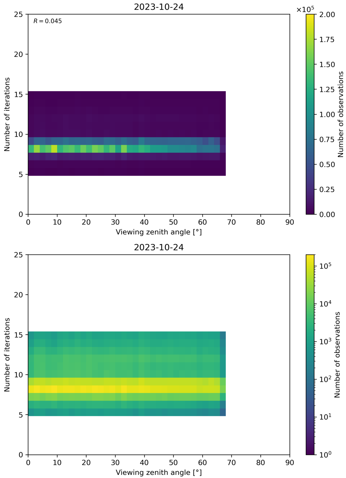
Figure 75: Scatter density plot of “Viewing zenith angle” against “Number of iterations” for 2023-10-23 to 2023-10-25.
