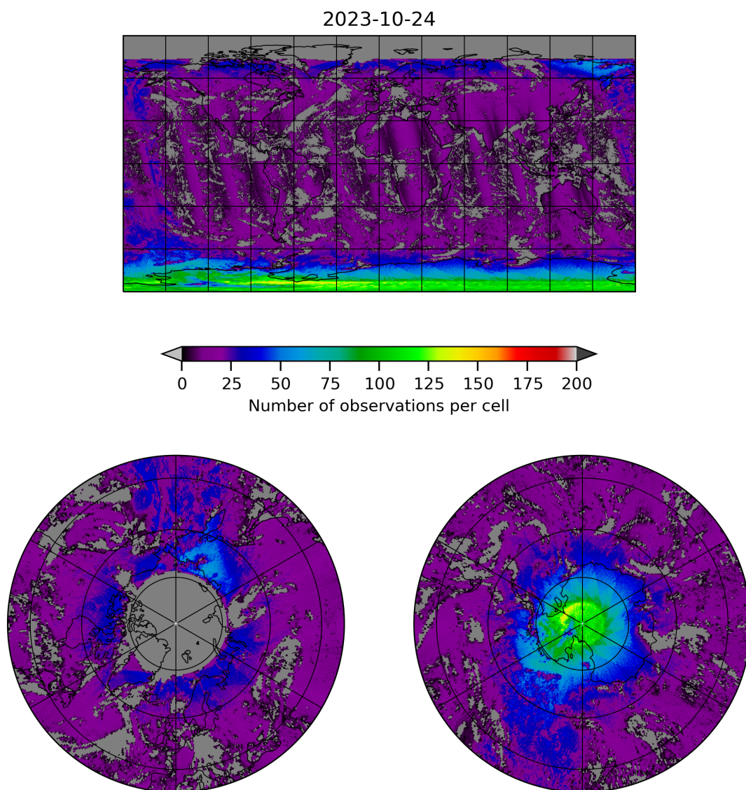
Figure 8: Map of the number of observations for 2023-10-23 to 2023-10-25
