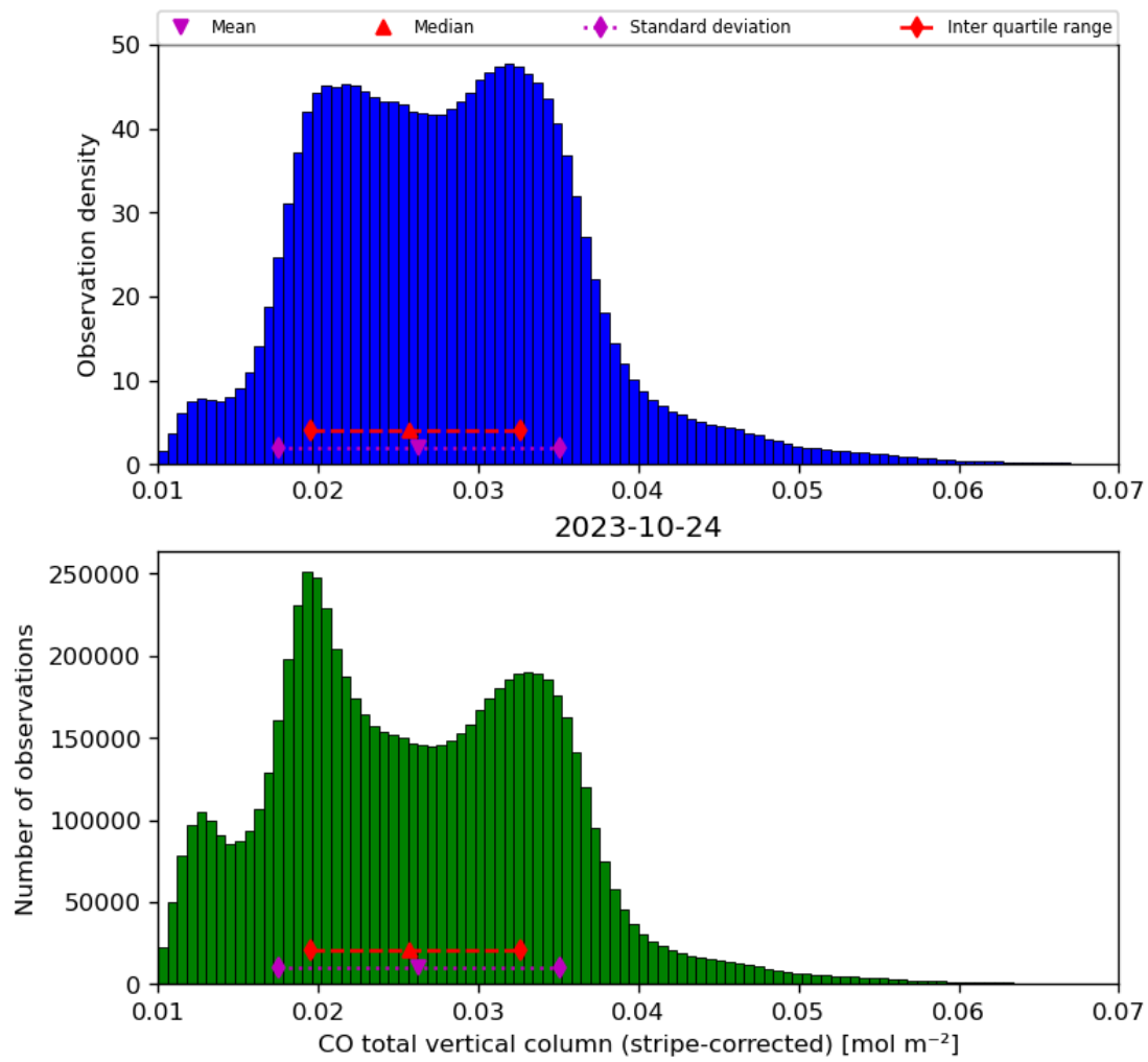
Figure 19: Histogram of “CO total vertical column (stripe-corrected)” for 2023-10-23 to 2023-10-25
