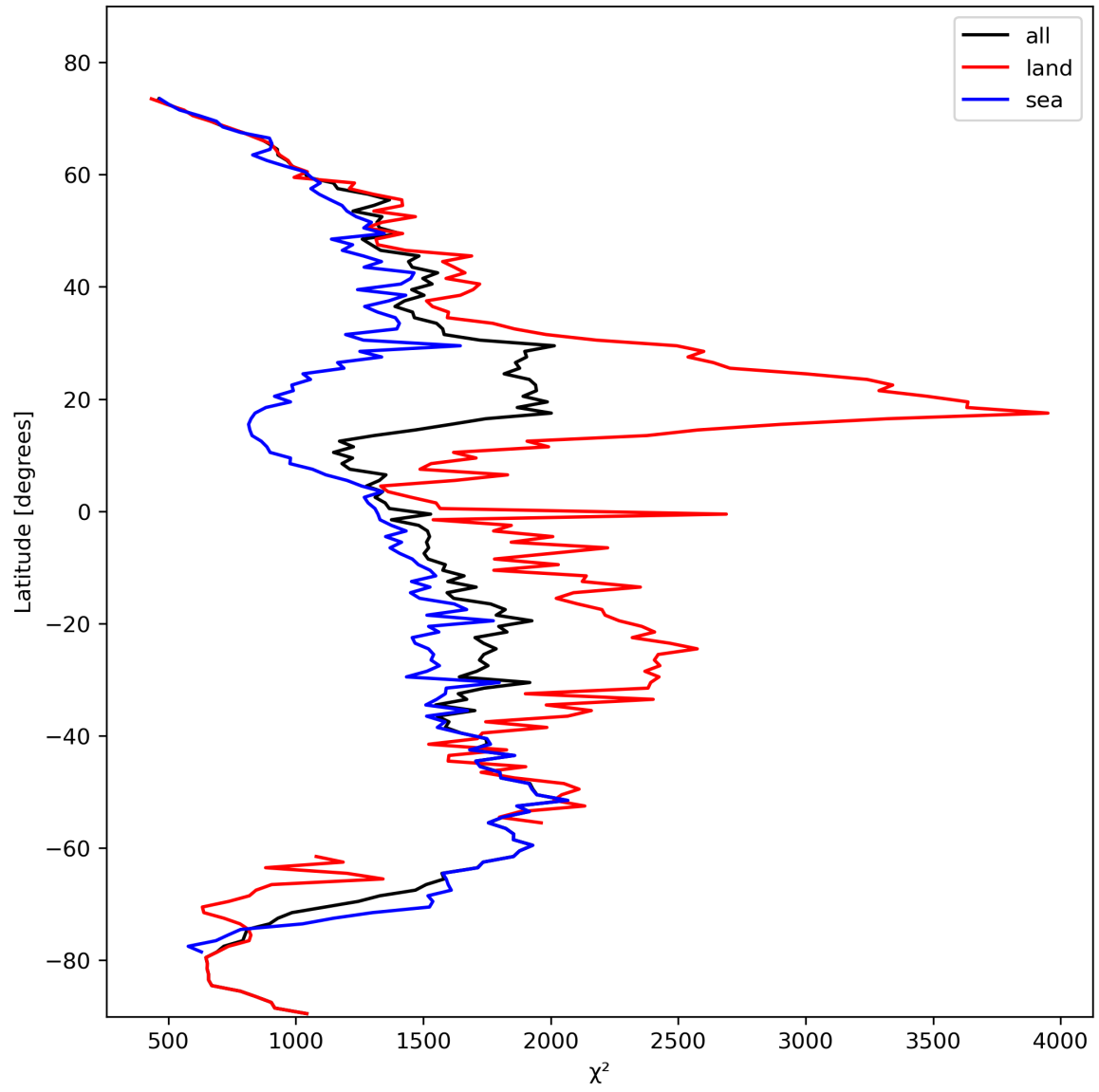
Figure 14: Zonal average of “ \chi^2 ” for 2023-10-23 to 2023-10-25.
