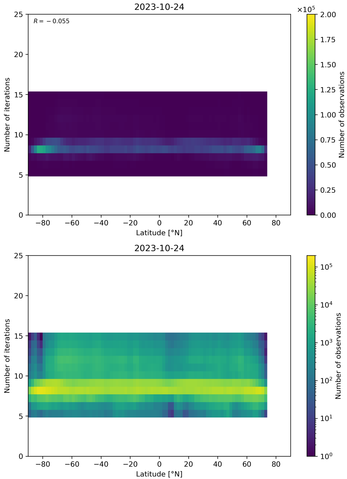
Figure 56: Scatter density plot of “Latitude” against “Number of iterations” for 2023-10-23 to 2023-10-25.
