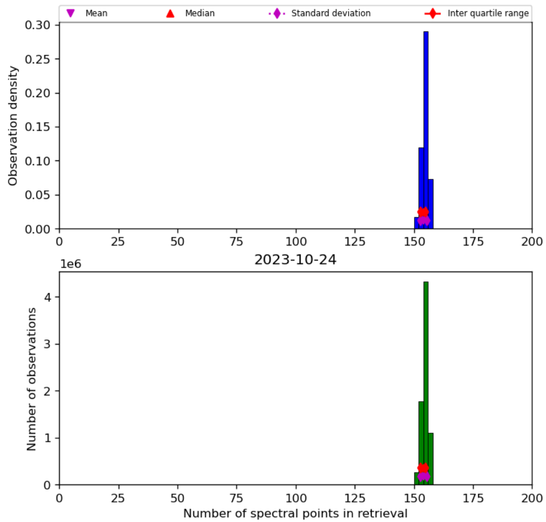
Figure 21: Histogram of “Number of spectral points in retrieval” for 2023-10-23 to 2023-10-25
