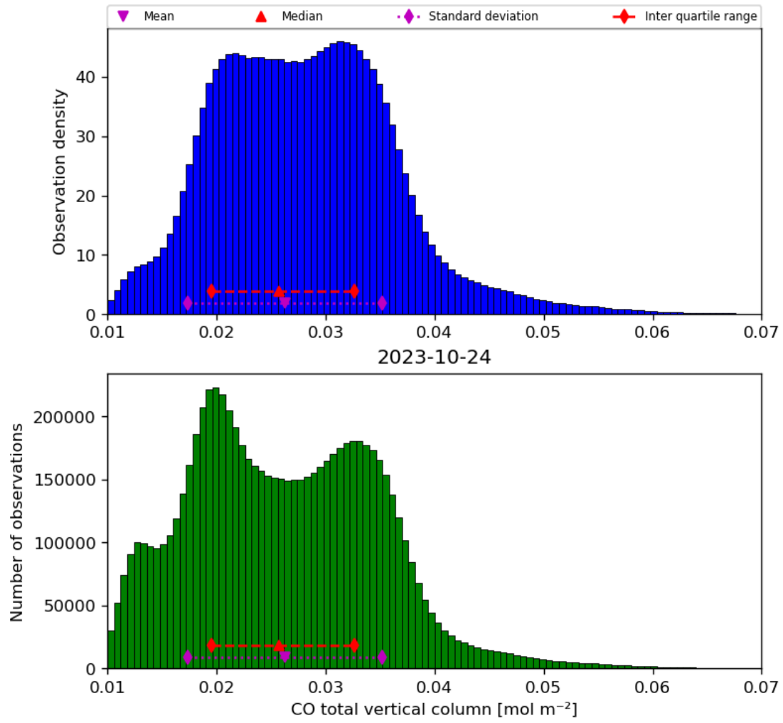
Figure 18: Histogram of “CO total vertical column” for 2023-10-23 to 2023-10-25
