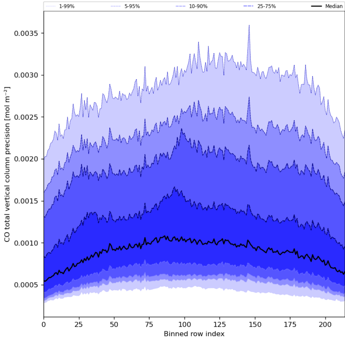
Figure 28: Along track statistics of “CO total vertical column precision” for 2023-10-23 to 2023-10-25
