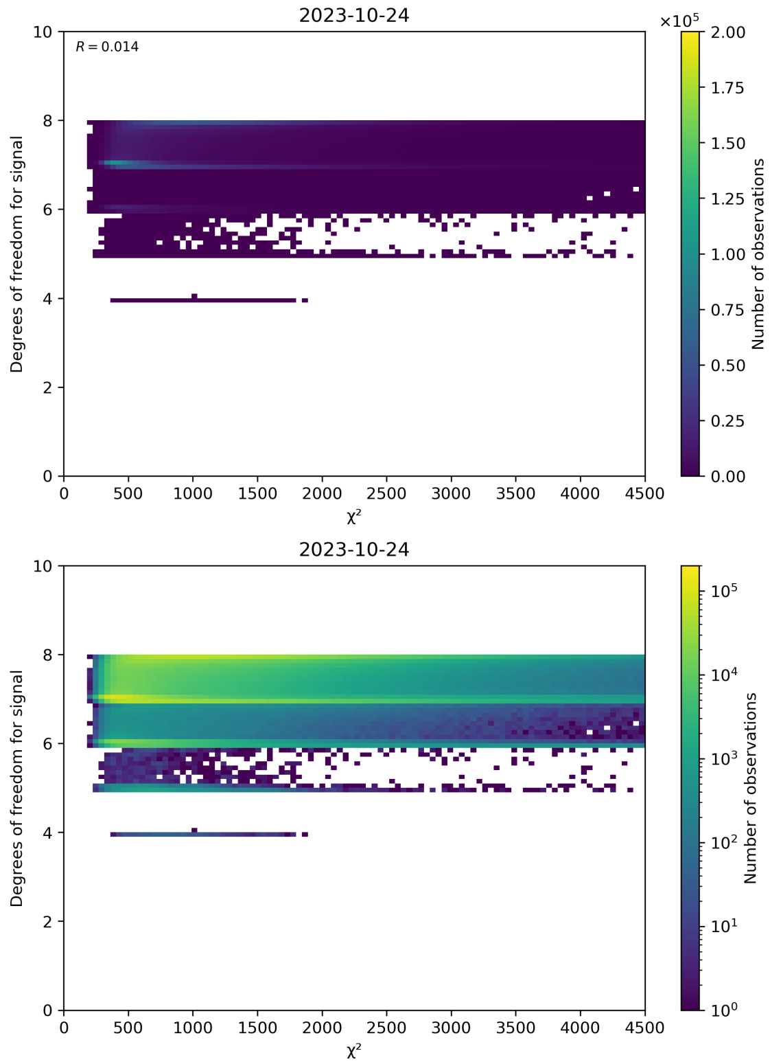
Figure 48: Scatter density plot of “ \chi^2 ” against “Degrees of freedom for signal” for 2023-10-23 to 2023-10-25.
