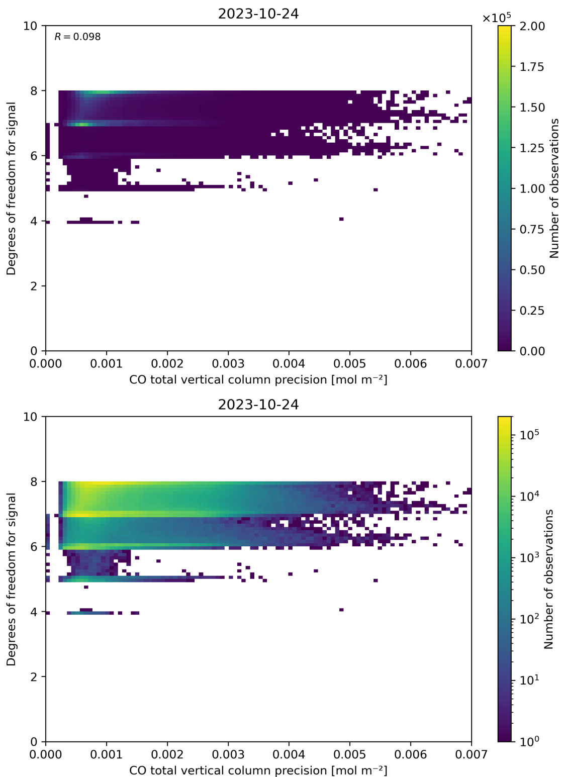
Figure 45: Scatter density plot of “CO total vertical column precision” against “Degrees of freedom for signal” for 2023-10-23 to 2023-10-25.
