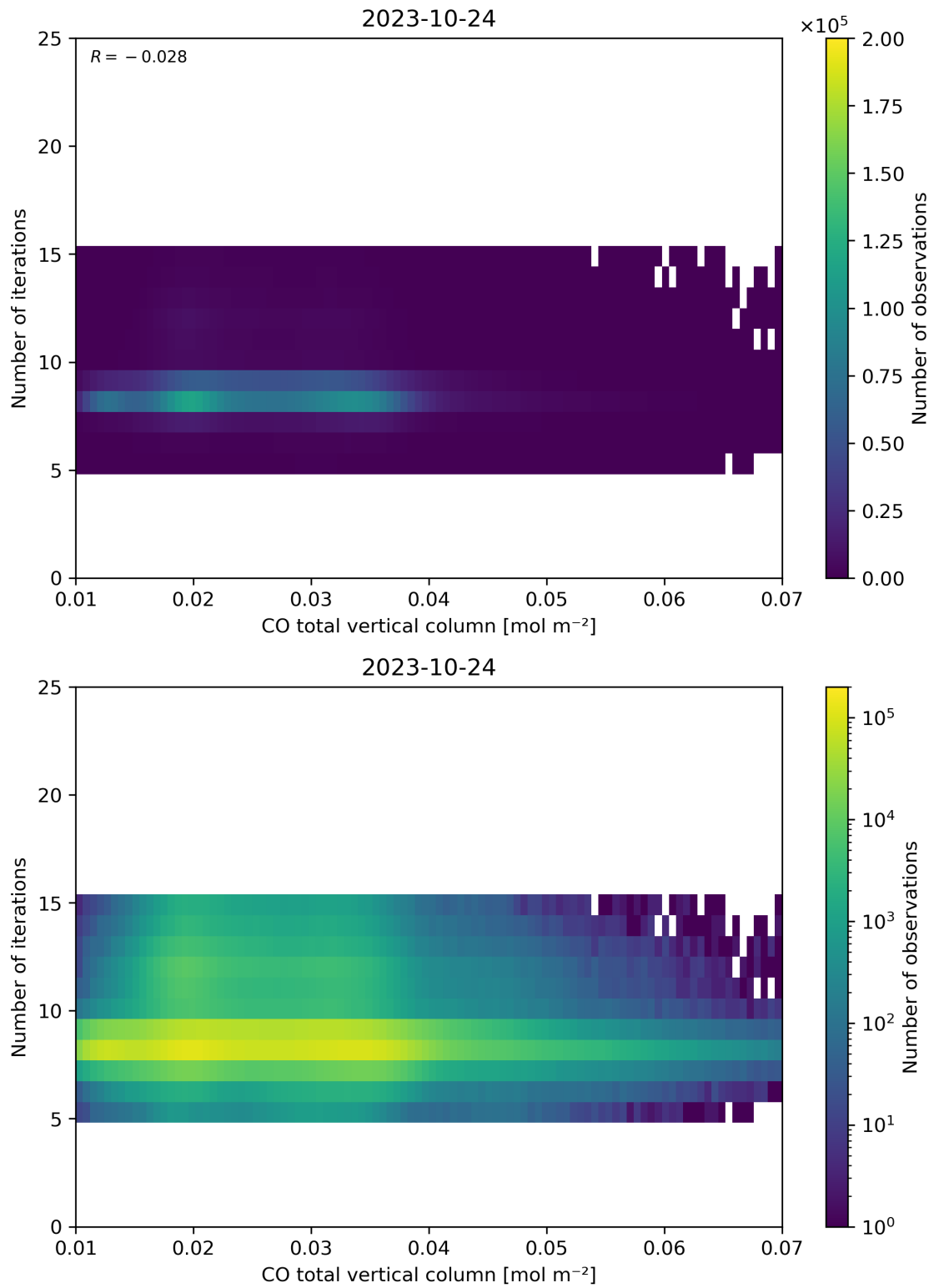
Figure 42: Scatter density plot of “CO total vertical column” against “Number of iterations” for 2023-10-23 to 2023-10-25.
