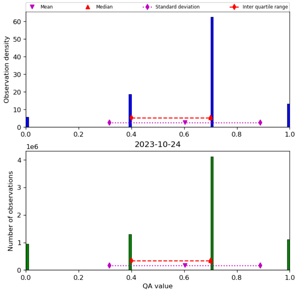
Figure 17: Histogram of “QA value” for 2023-10-23 to 2023-10-25
