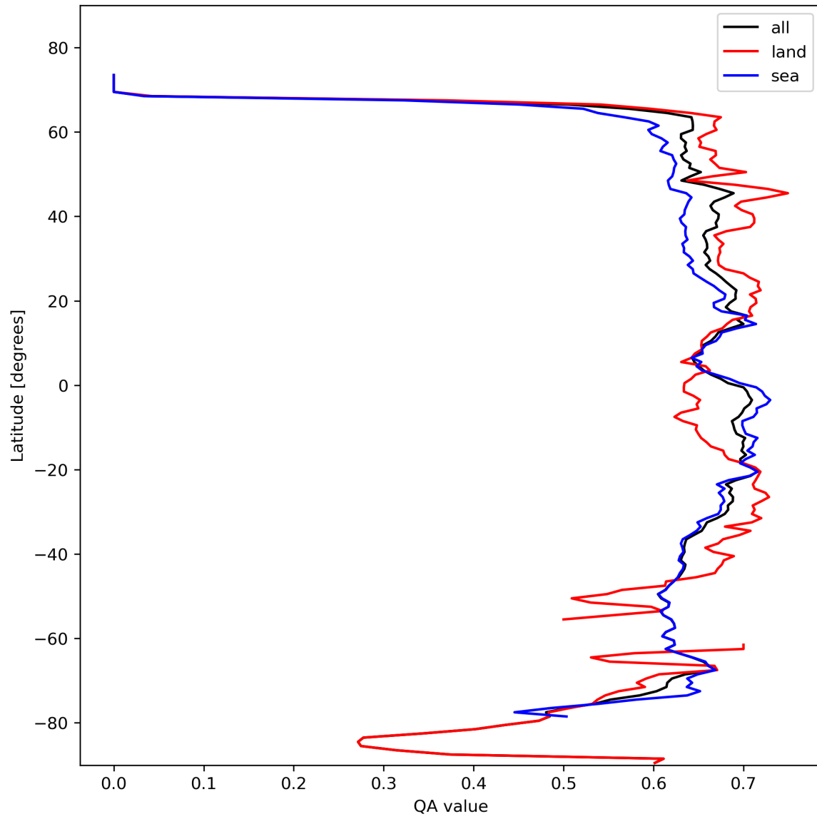
Figure 9: Zonal average of “QA value” for 2023-10-23 to 2023-10-25.
