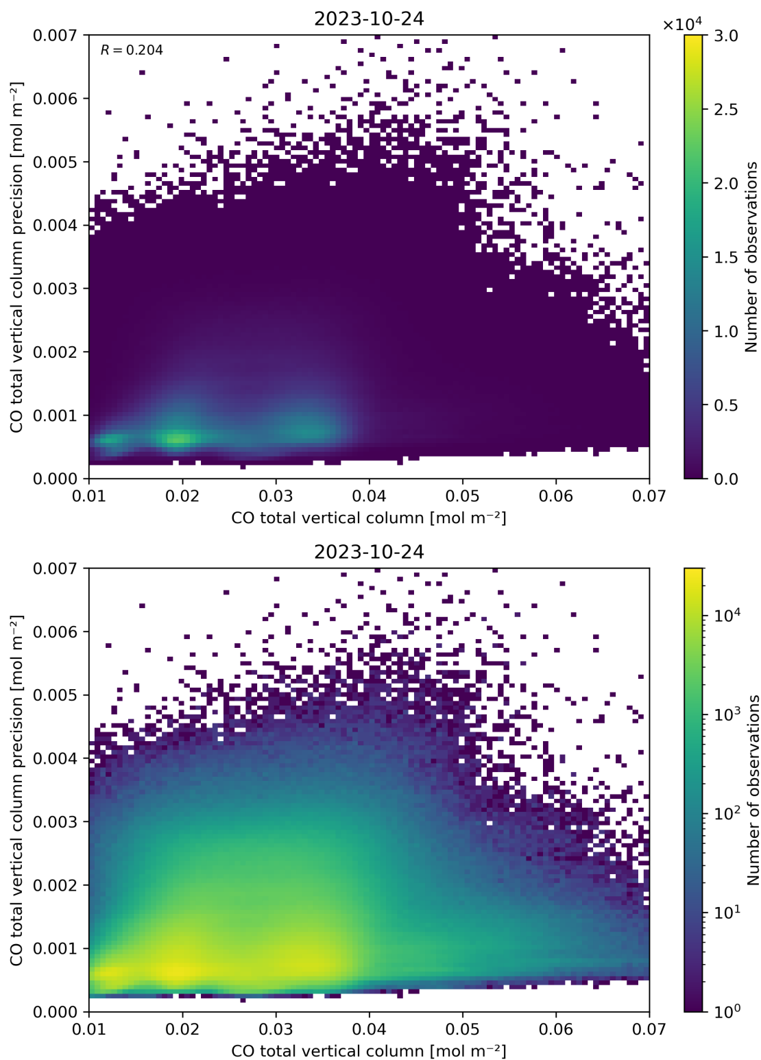
Figure 34: Scatter density plot of “CO total vertical column” against “CO total vertical column precision” for 2023-10-23 to 2023-10-25.
