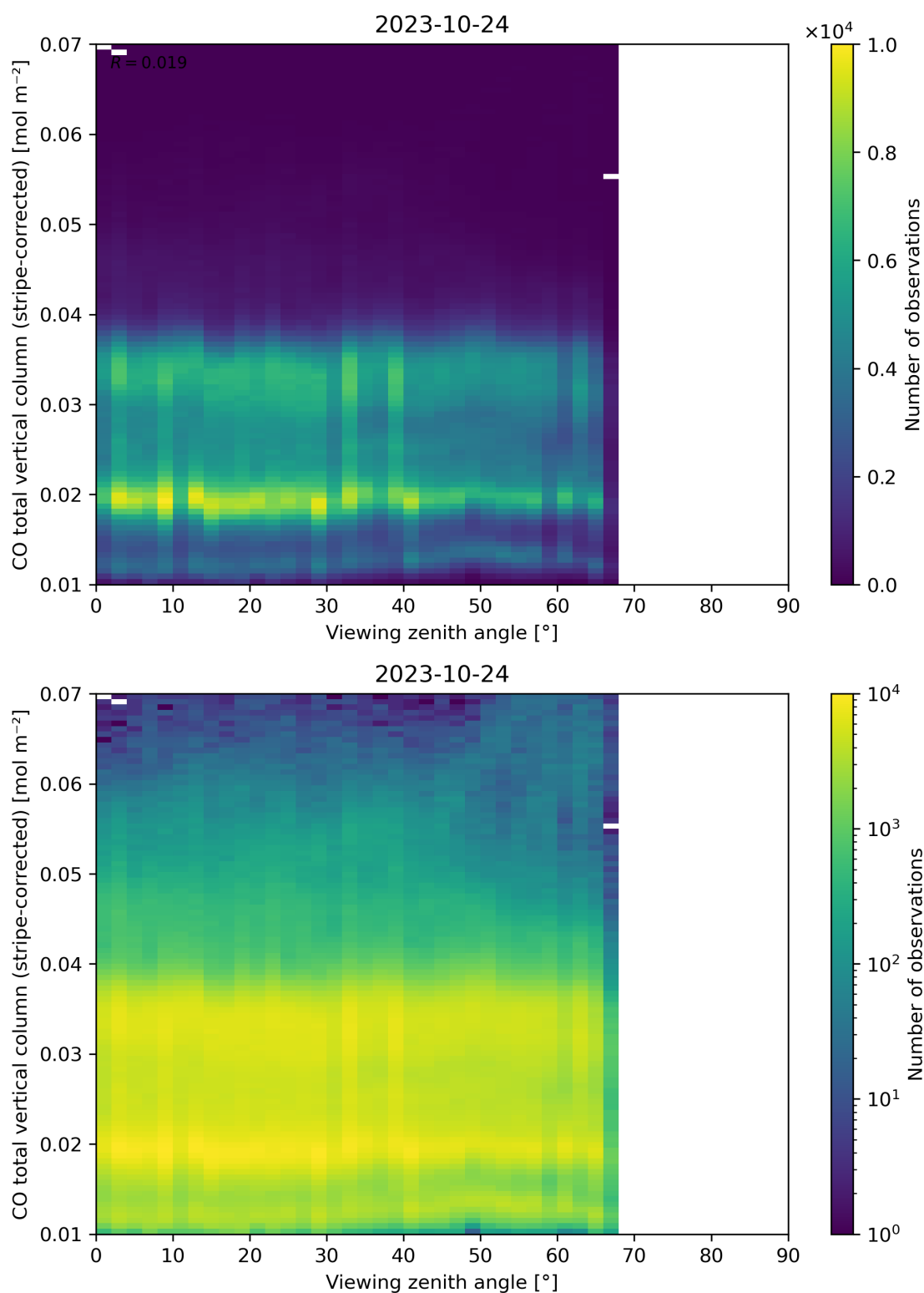
Figure 70: Scatter density plot of “Viewing zenith angle” against “CO total vertical column (stripe-corrected)” for 2023-10-23 to 2023-10-25.
