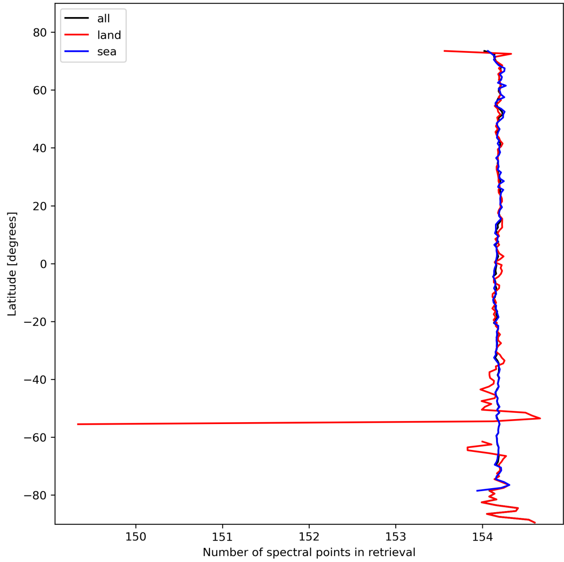
Figure 13: Zonal average of “Number of spectral points in retrieval” for 2023-10-23 to 2023-10-25.
