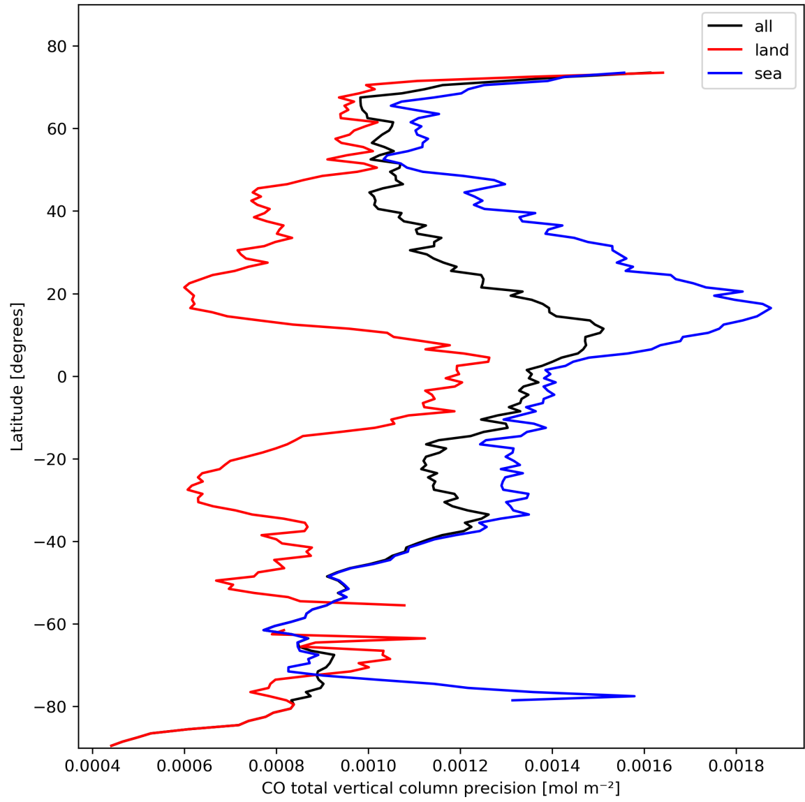
Figure 12: Zonal average of “CO total vertical column precision” for 2023-10-23 to 2023-10-25.
