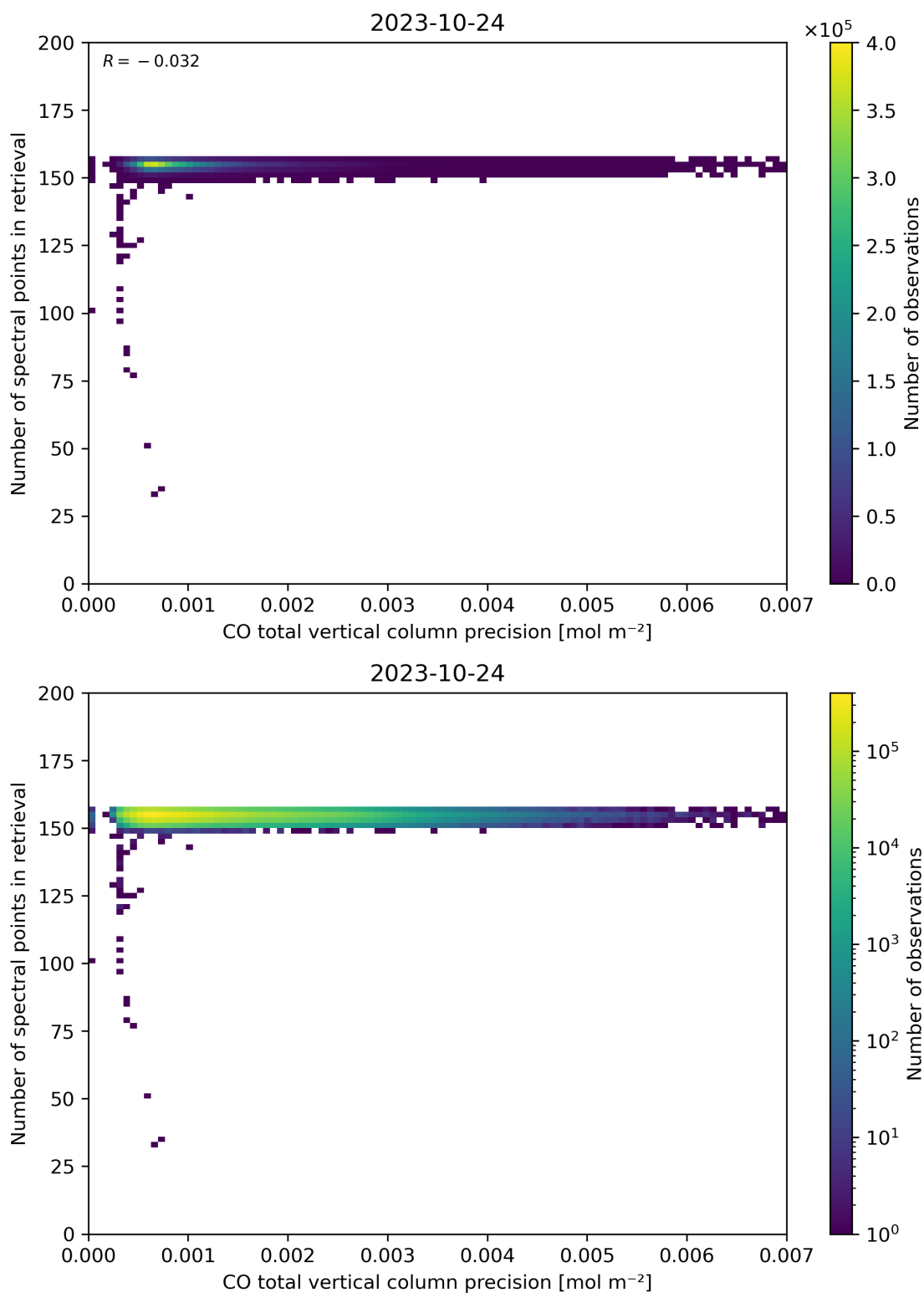
Figure 47: Scatter density plot of “CO total vertical column precision” against “Number of spectral points in retrieval” for 2023-10-23 to 2023-10-25.
