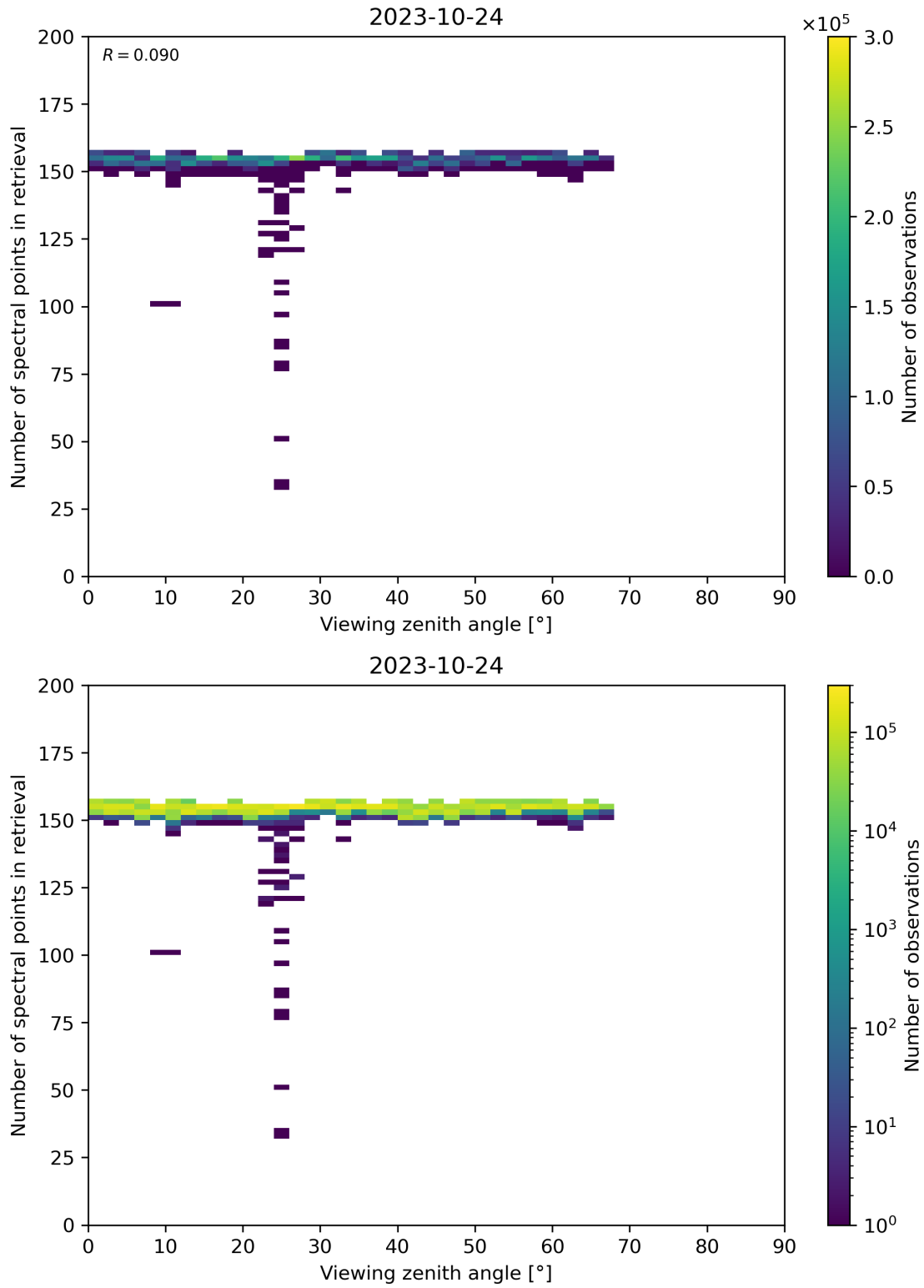
Figure 76: Scatter density plot of “Viewing zenith angle” against “Number of spectral points in retrieval” for 2023-10-23 to 2023-10-25.
