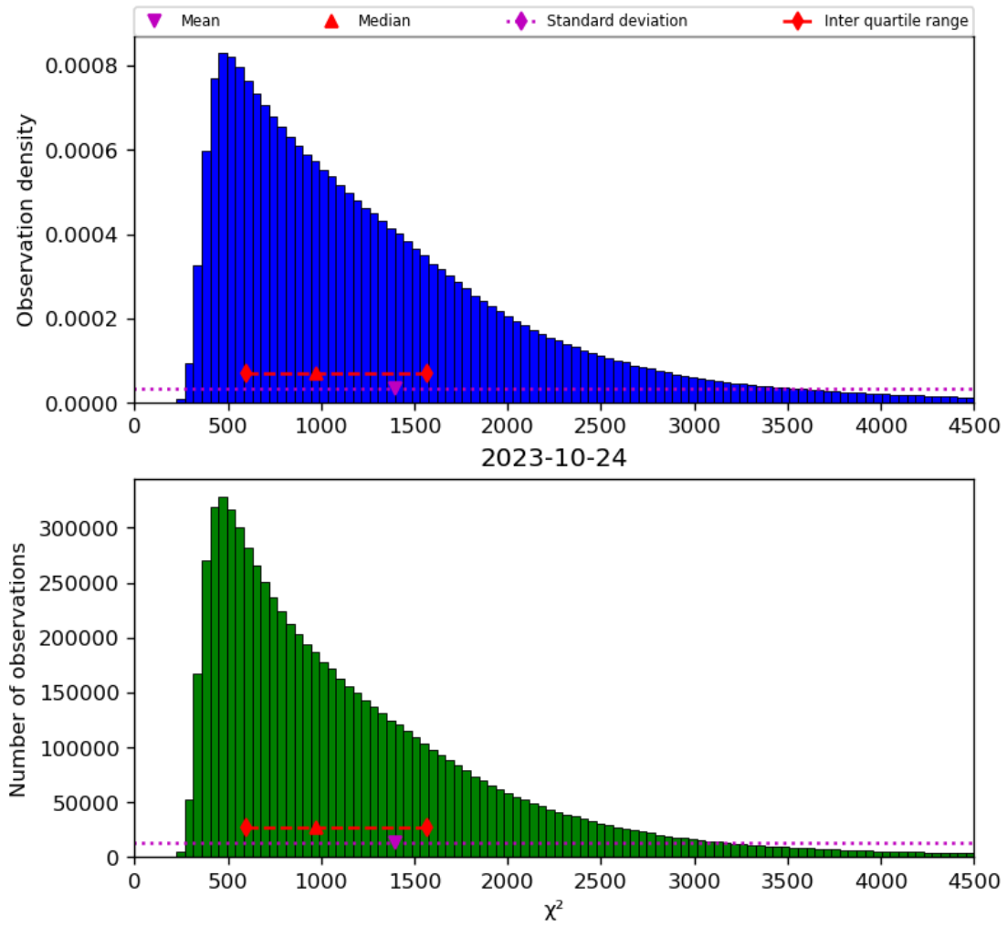
Figure 22: Histogram of “ \chi^2 ” for 2023-10-23 to 2023-10-25
