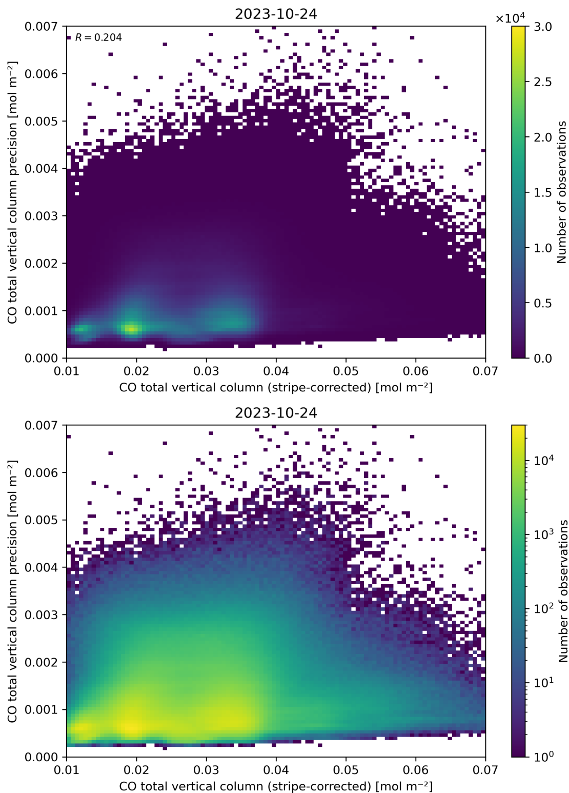
Figure 36: Scatter density plot of “CO total vertical column (stripe-corrected)” against “CO total vertical column precision” for 2023-10-23 to 2023-10-25.
