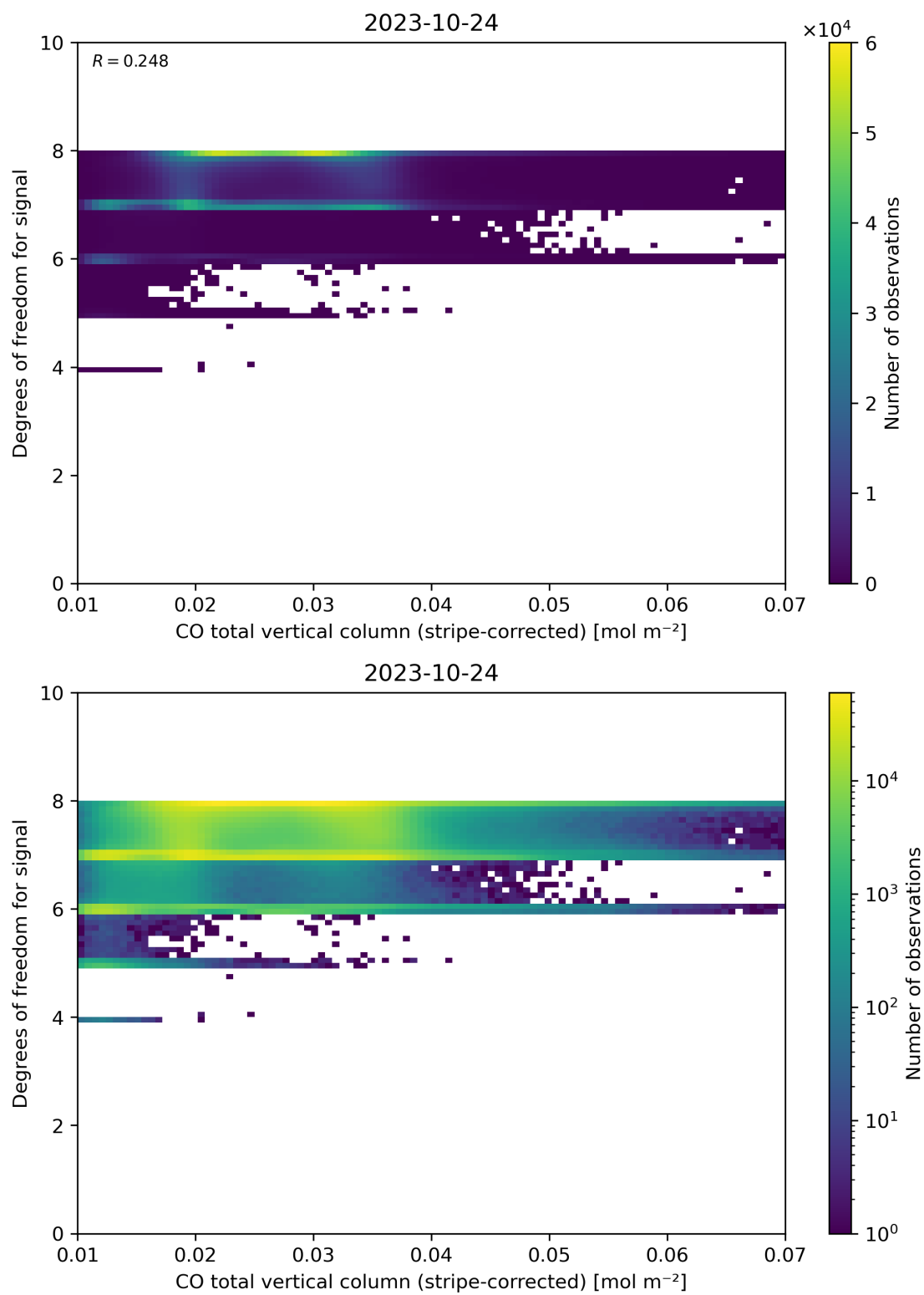
Figure 38: Scatter density plot of “CO total vertical column (stripe-corrected)” against “Degrees of freedom for signal” for 2023-10-23 to 2023-10-25.
