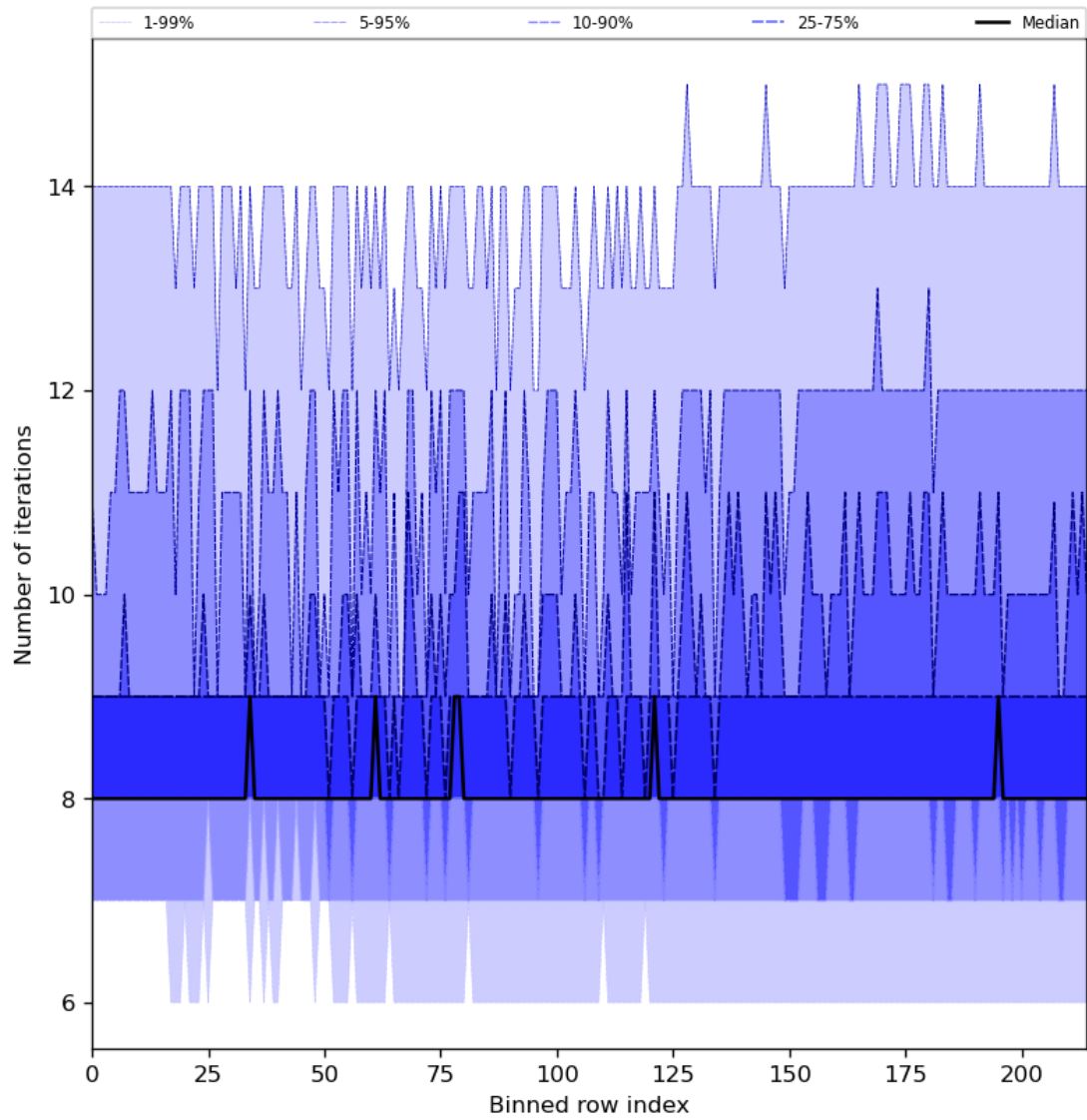
Figure 32: Along track statistics of “Number of iterations” for 2023-10-23 to 2023-10-25
