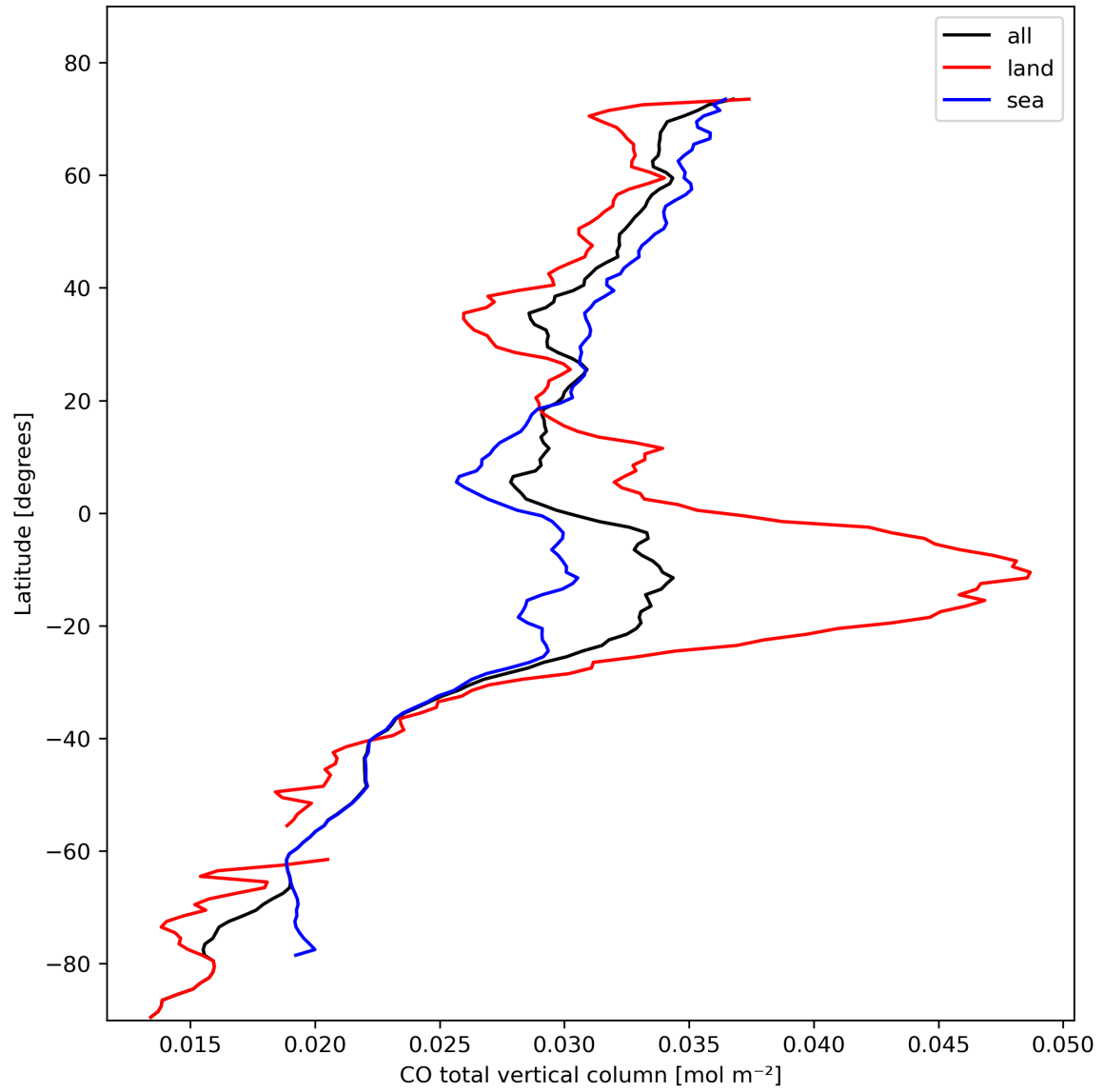
Figure 10: Zonal average of “CO total vertical column” for 2023-10-23 to 2023-10-25.
