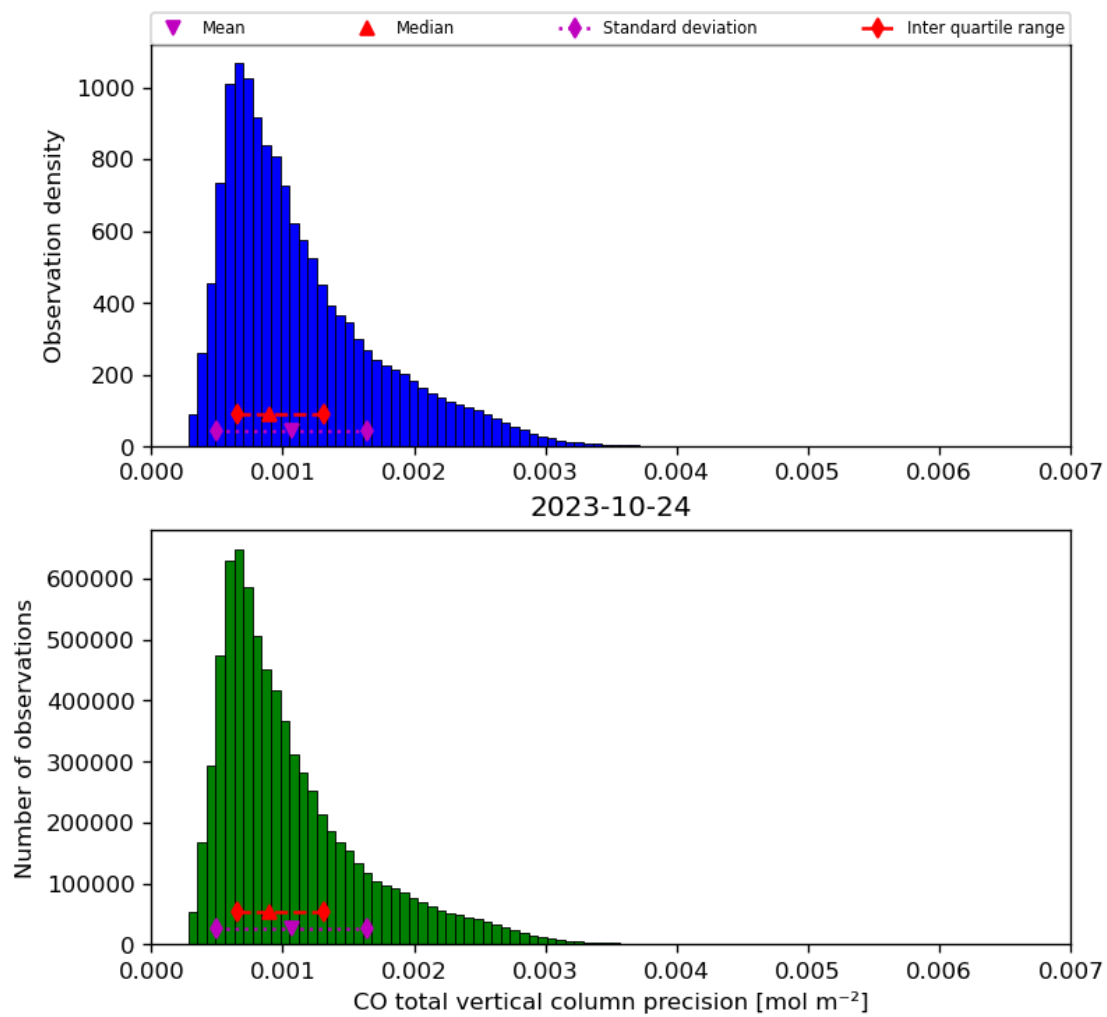
Figure 20: Histogram of “CO total vertical column precision” for 2023-10-23 to 2023-10-25
