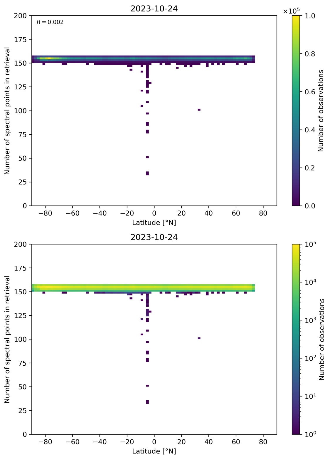
Figure 57: Scatter density plot of “Latitude” against “Number of spectral points in retrieval” for 2023-10-23 to 2023-10-25.
