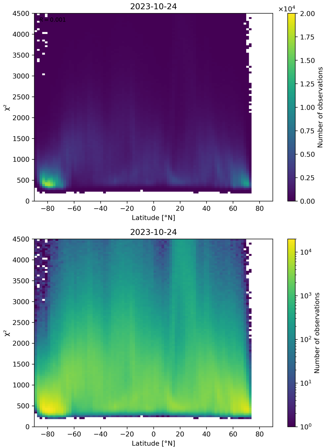
Figure 54: Scatter density plot of “Latitude” against “ \chi^2 ” for 2023-10-23 to 2023-10-25.
