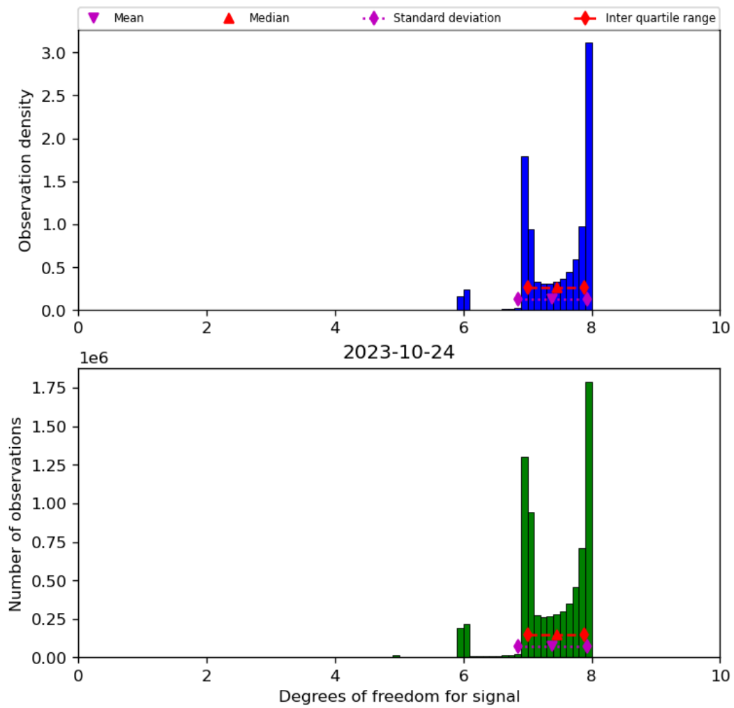
Figure 23: Histogram of “Degrees of freedom for signal” for 2023-10-23 to 2023-10-25
