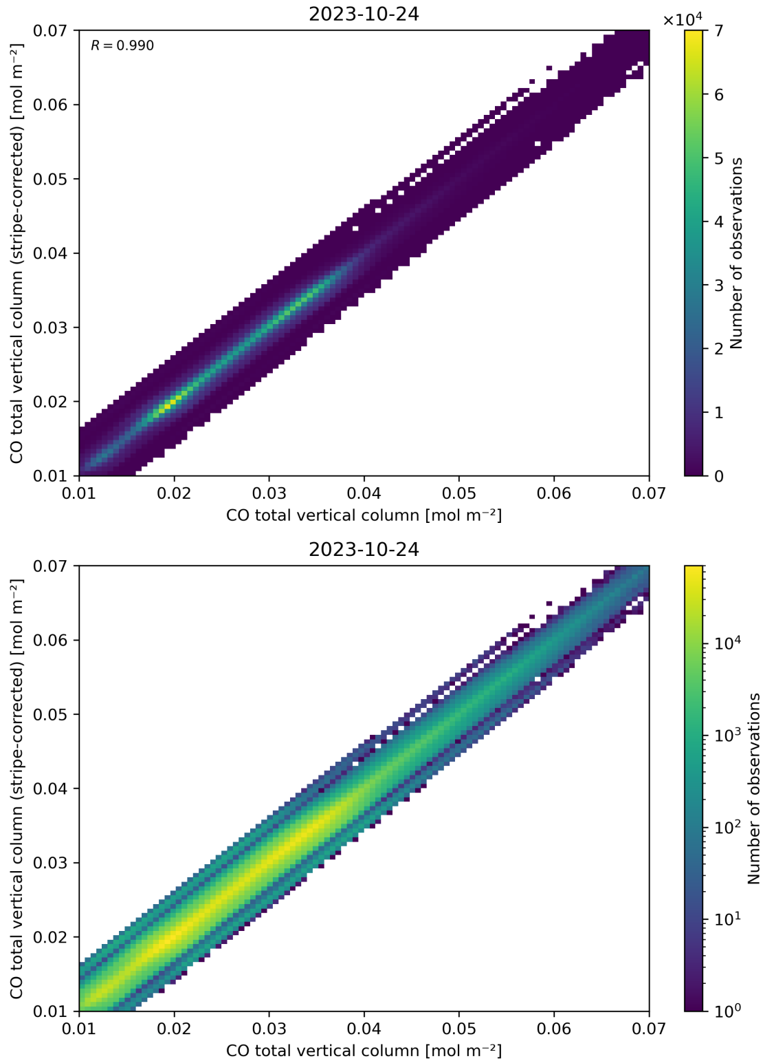
Figure 33: Scatter density plot of “CO total vertical column” against “CO total vertical column (stripe-corrected)” for 2023-10-23 to 2023-10-25.
