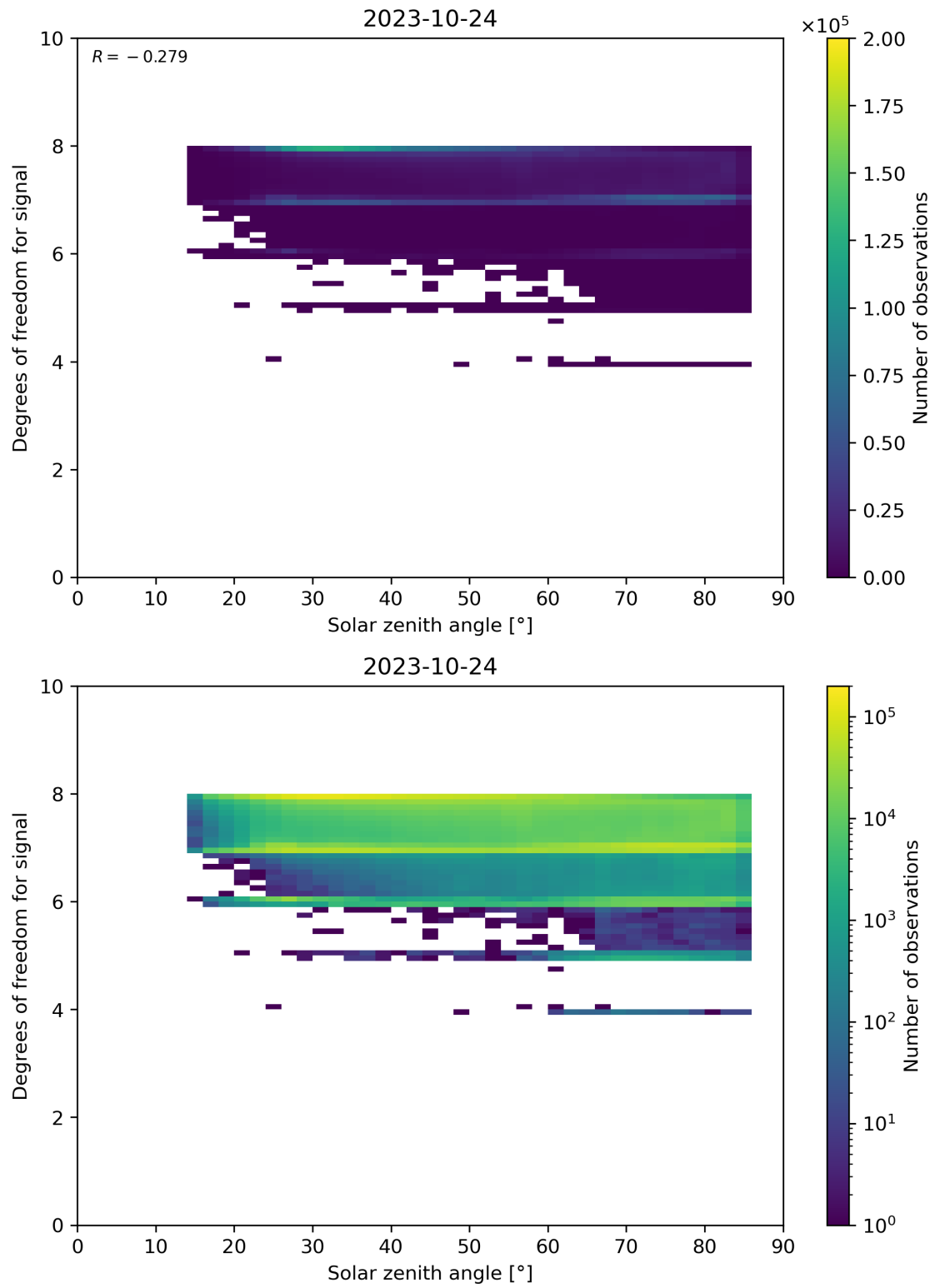
Figure 65: Scatter density plot of “Solar zenith angle” against “Degrees of freedom for signal” for 2023-10-23 to 2023-10-25.
