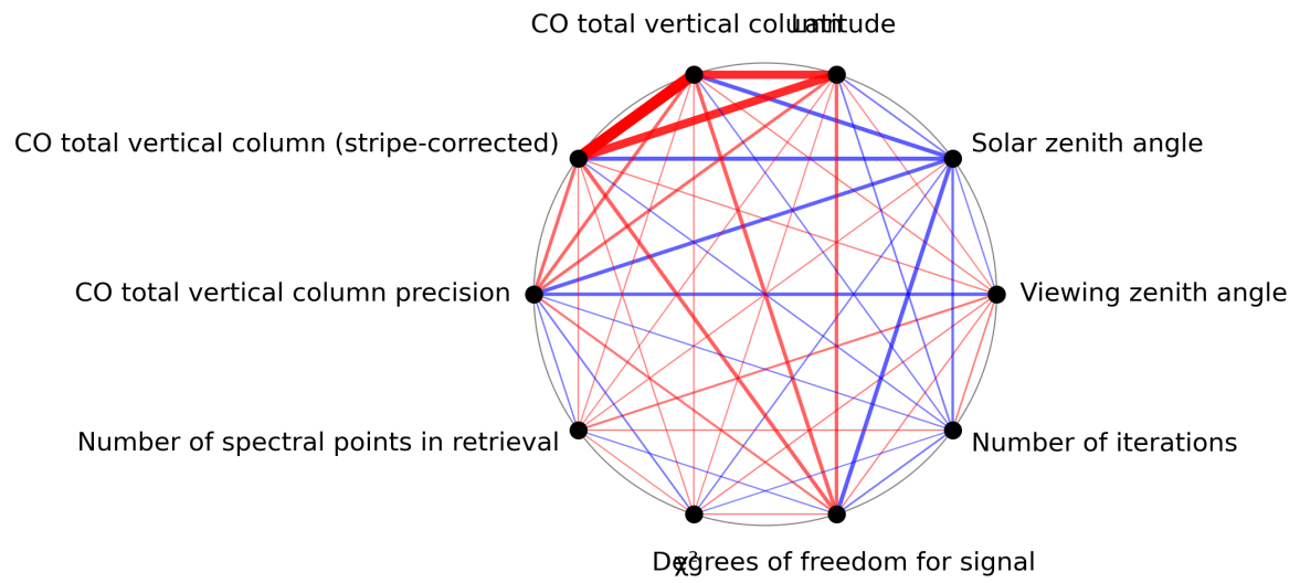
Figure 1: Map of correlation graph for 2023-10-23 to 2023-10-25.
