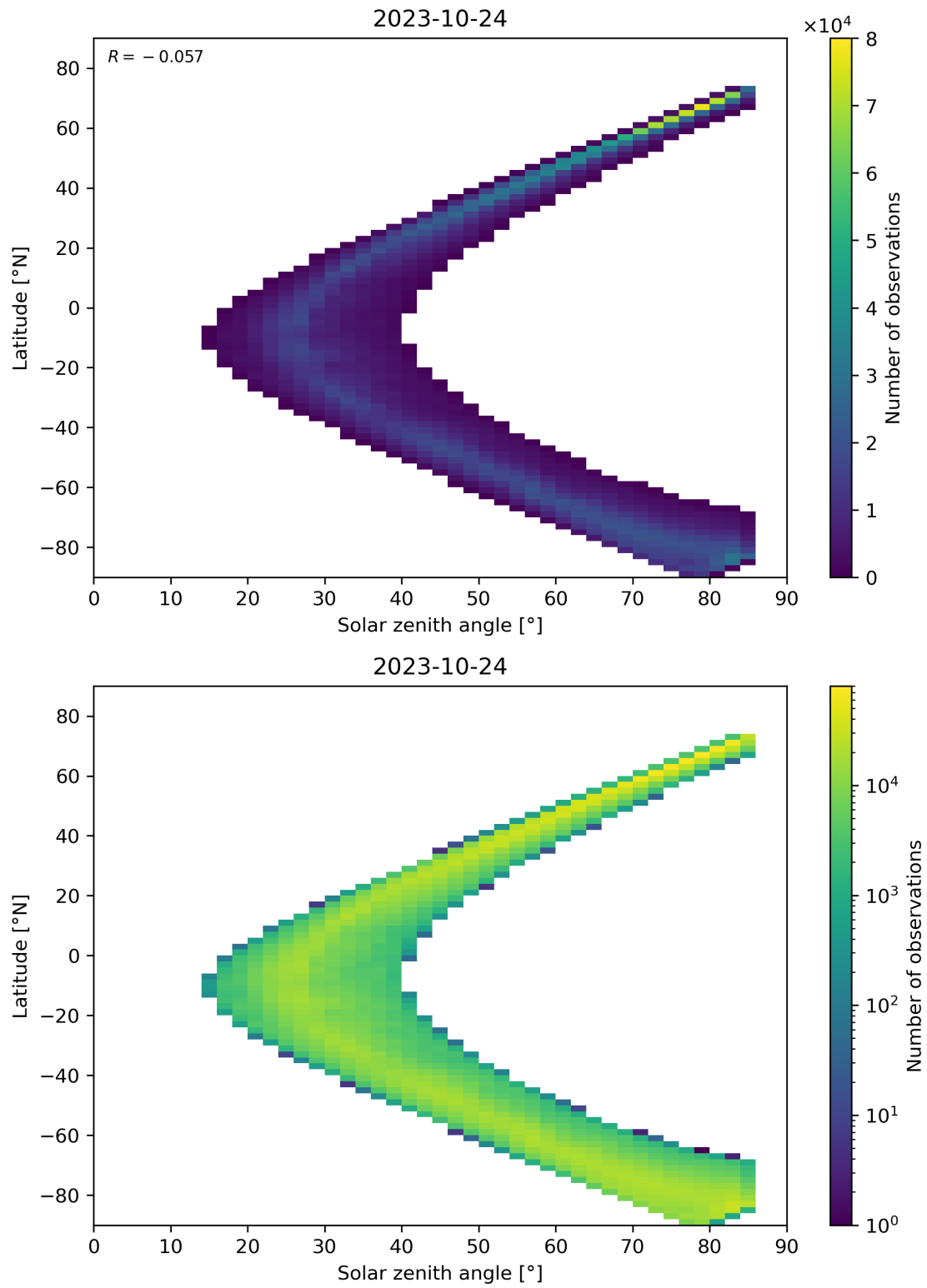
Figure 66: Scatter density plot of “Solar zenith angle” against “Latitude” for 2023-10-23 to 2023-10-25.
