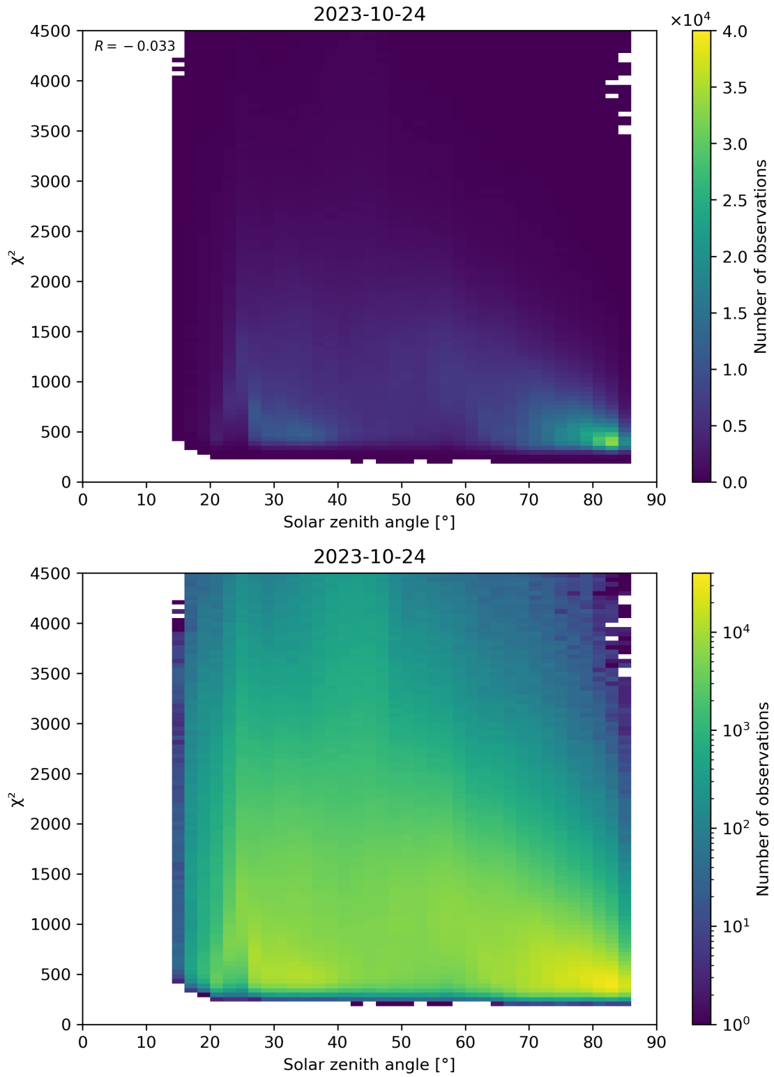
Figure 64: Scatter density plot of “Solar zenith angle” against “ \chi^2 ” for 2023-10-23 to 2023-10-25.
