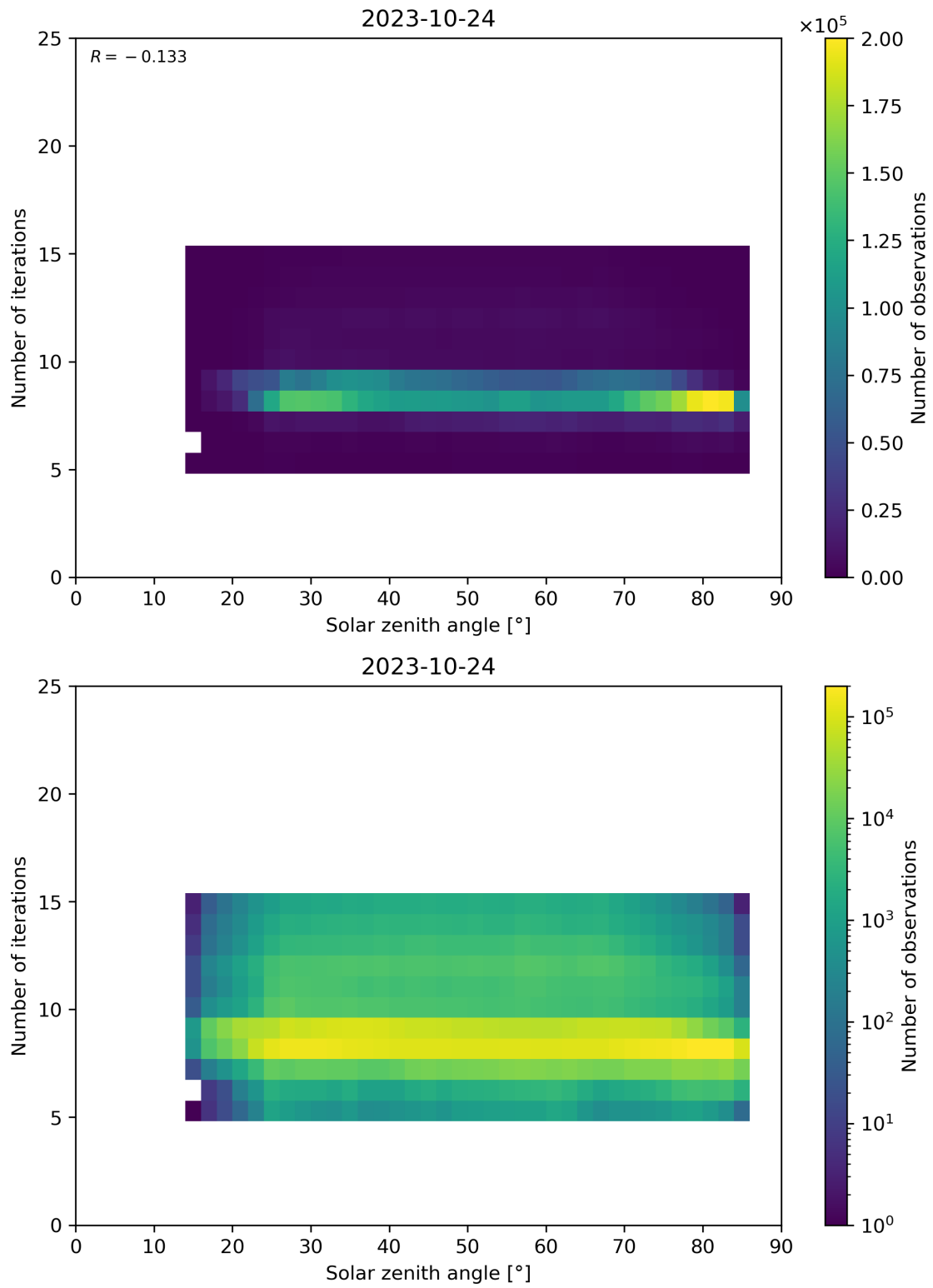
Figure 67: Scatter density plot of “Solar zenith angle” against “Number of iterations” for 2023-10-23 to 2023-10-25.
