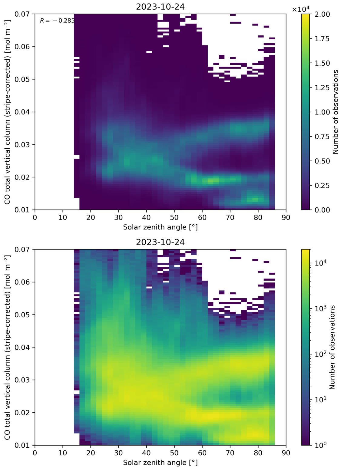
Figure 62: Scatter density plot of “Solar zenith angle” against “CO total vertical column (stripe-corrected)” for 2023-10-23 to 2023-10-25.
