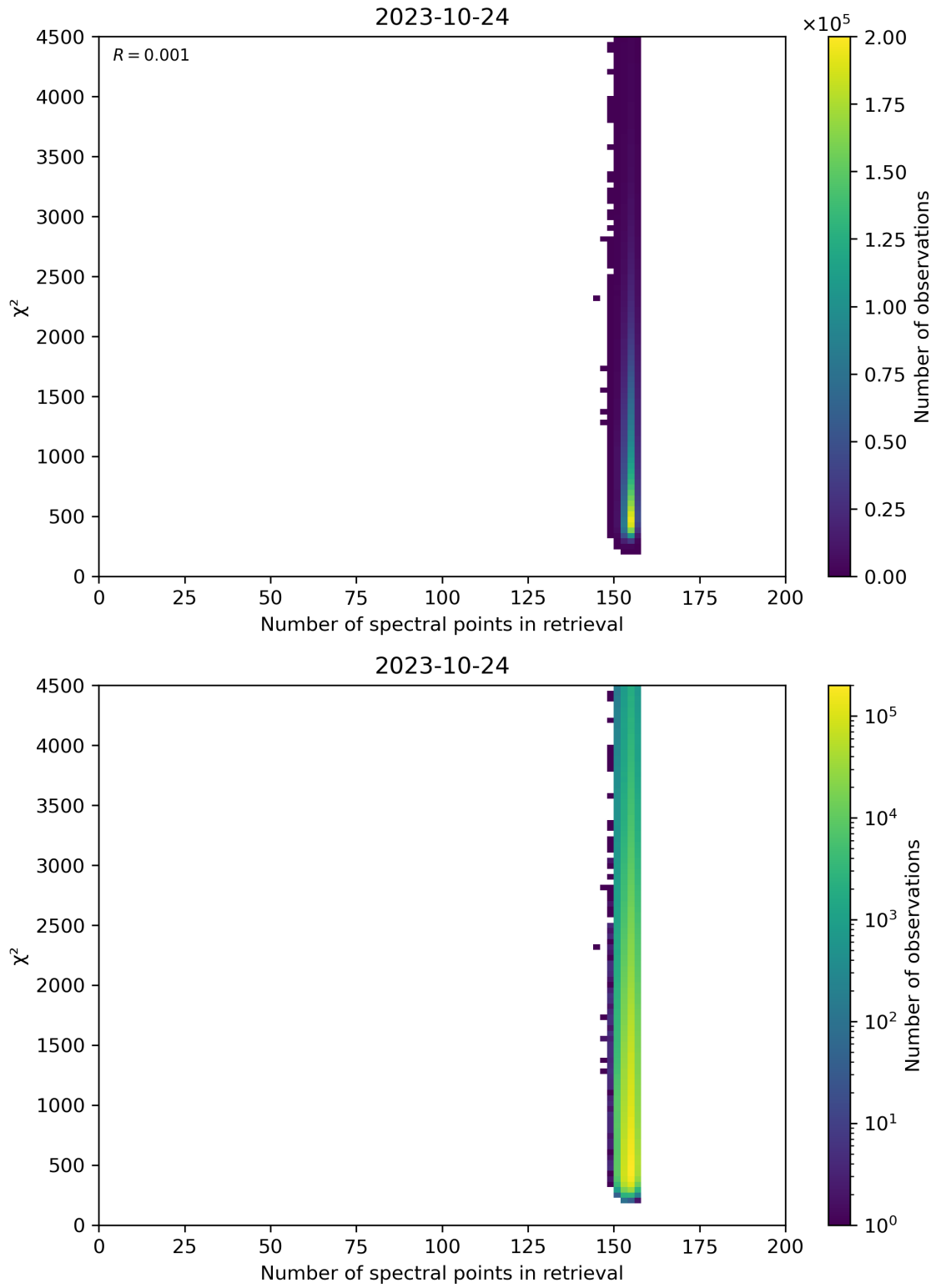
Figure 58: Scatter density plot of “Number of spectral points in retrieval” against “ \chi^2 ” for 2023-10-23 to 2023-10-25.
