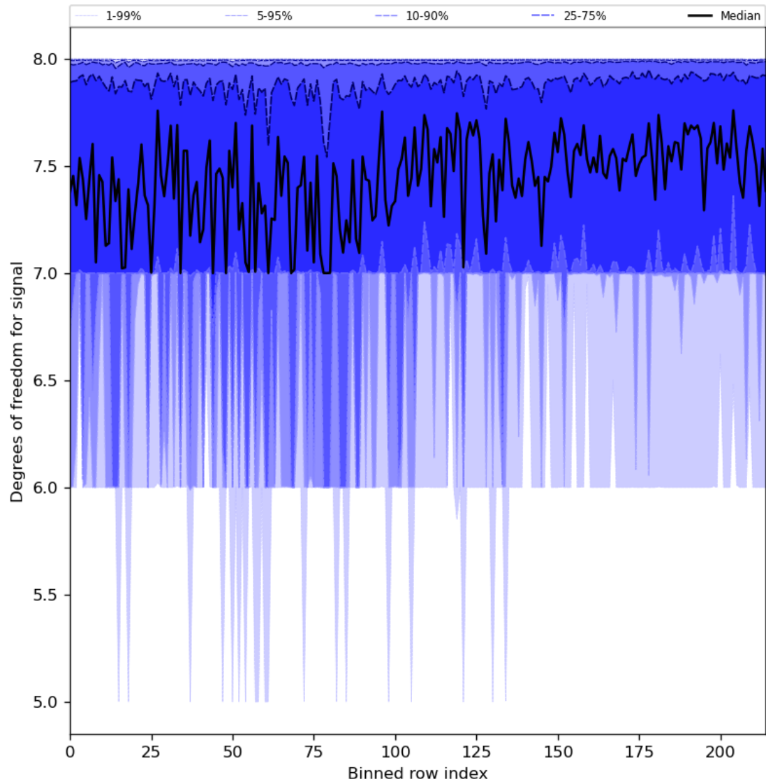
Figure 31: Along track statistics of “Degrees of freedom for signal” for 2023-10-23 to 2023-10-25
