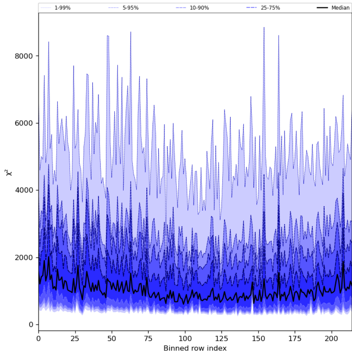
Figure 30: Along track statistics of “ \chi^2 ” for 2023-10-23 to 2023-10-25
