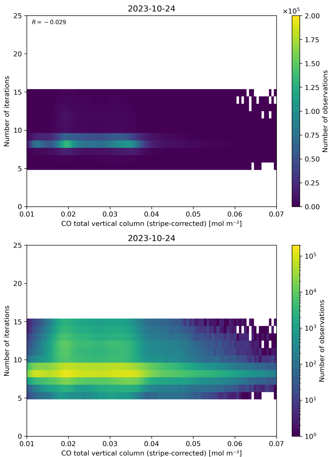
Figure 39: Scatter density plot of “CO total vertical column (stripe-corrected)” against “Number of iterations” for 2023-10-23 to 2023-10-25.
