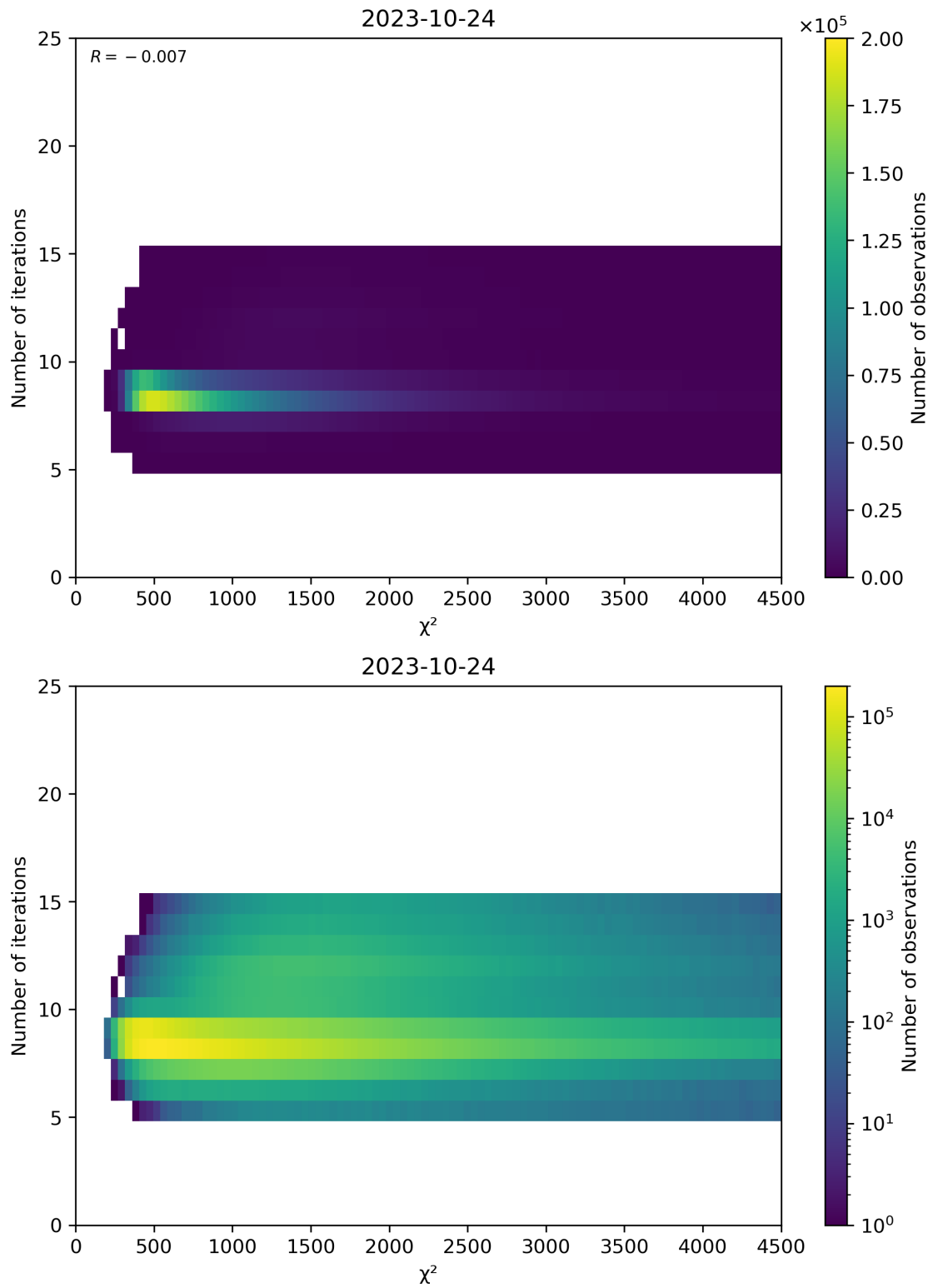
Figure 49: Scatter density plot of “ \chi^2 ” against “Number of iterations” for 2023-10-23 to 2023-10-25.
