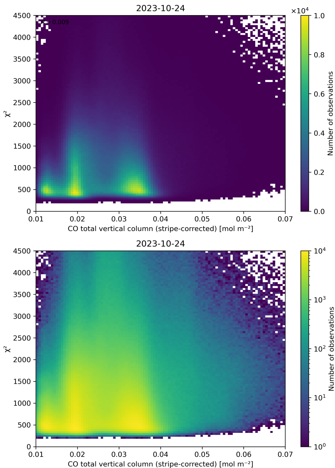
Figure 37: Scatter density plot of “CO total vertical column (stripe-corrected)” against “ \chi^2 ” for 2023-10-23 to 2023-10-25.
