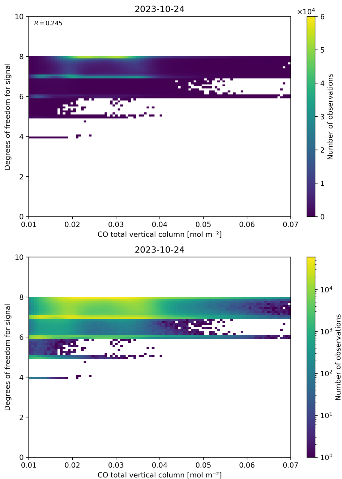
Figure 41: Scatter density plot of “CO total vertical column” against “Degrees of freedom for signal” for 2023-10-23 to 2023-10-25.
