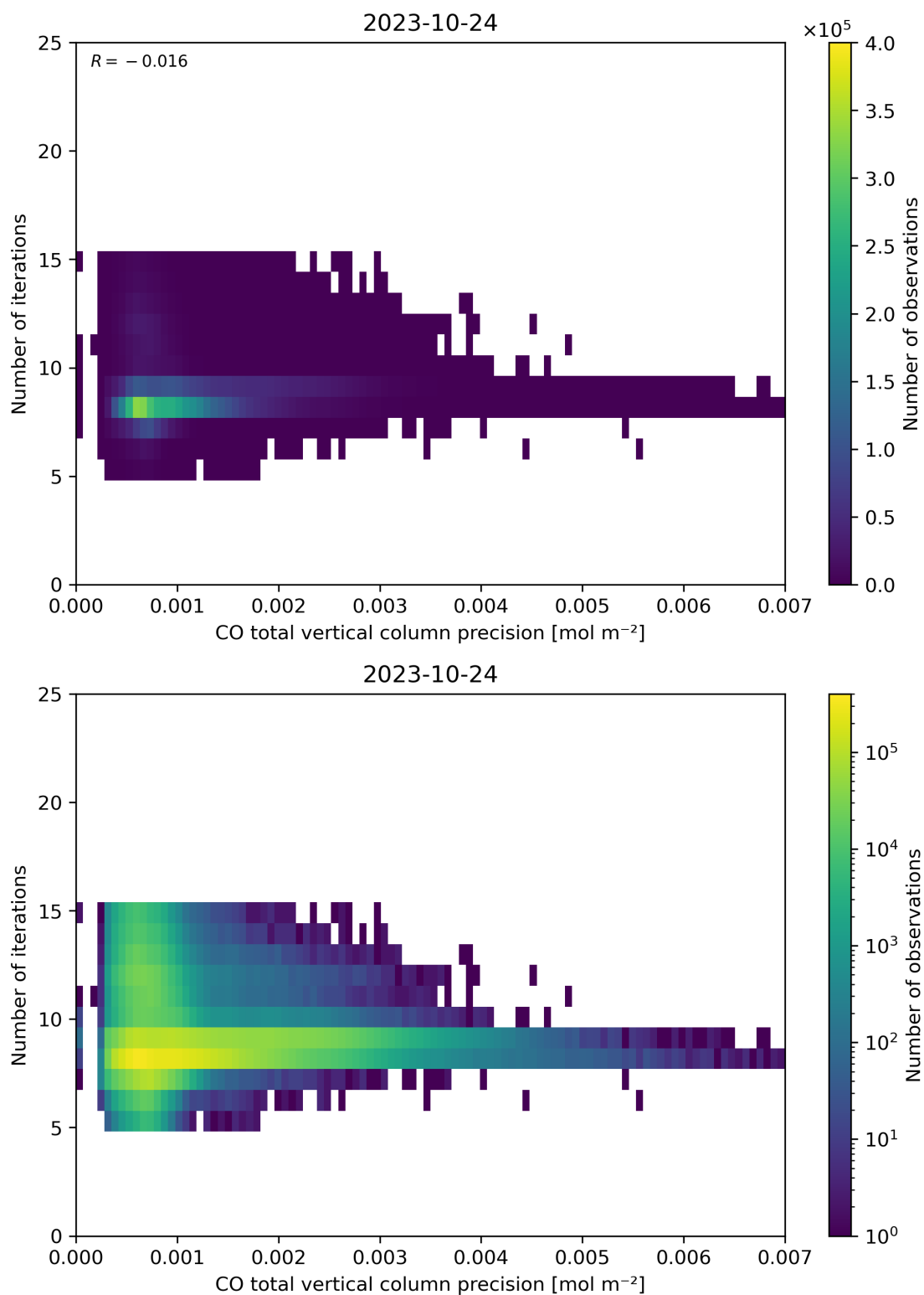
Figure 46: Scatter density plot of “CO total vertical column precision” against “Number of iterations” for 2023-10-23 to 2023-10-25.
