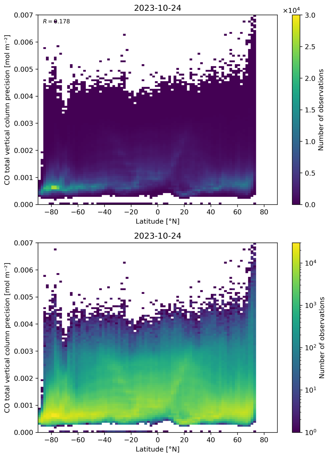
Figure 53: Scatter density plot of “Latitude” against “CO total vertical column precision” for 2023-10-23 to 2023-10-25.
