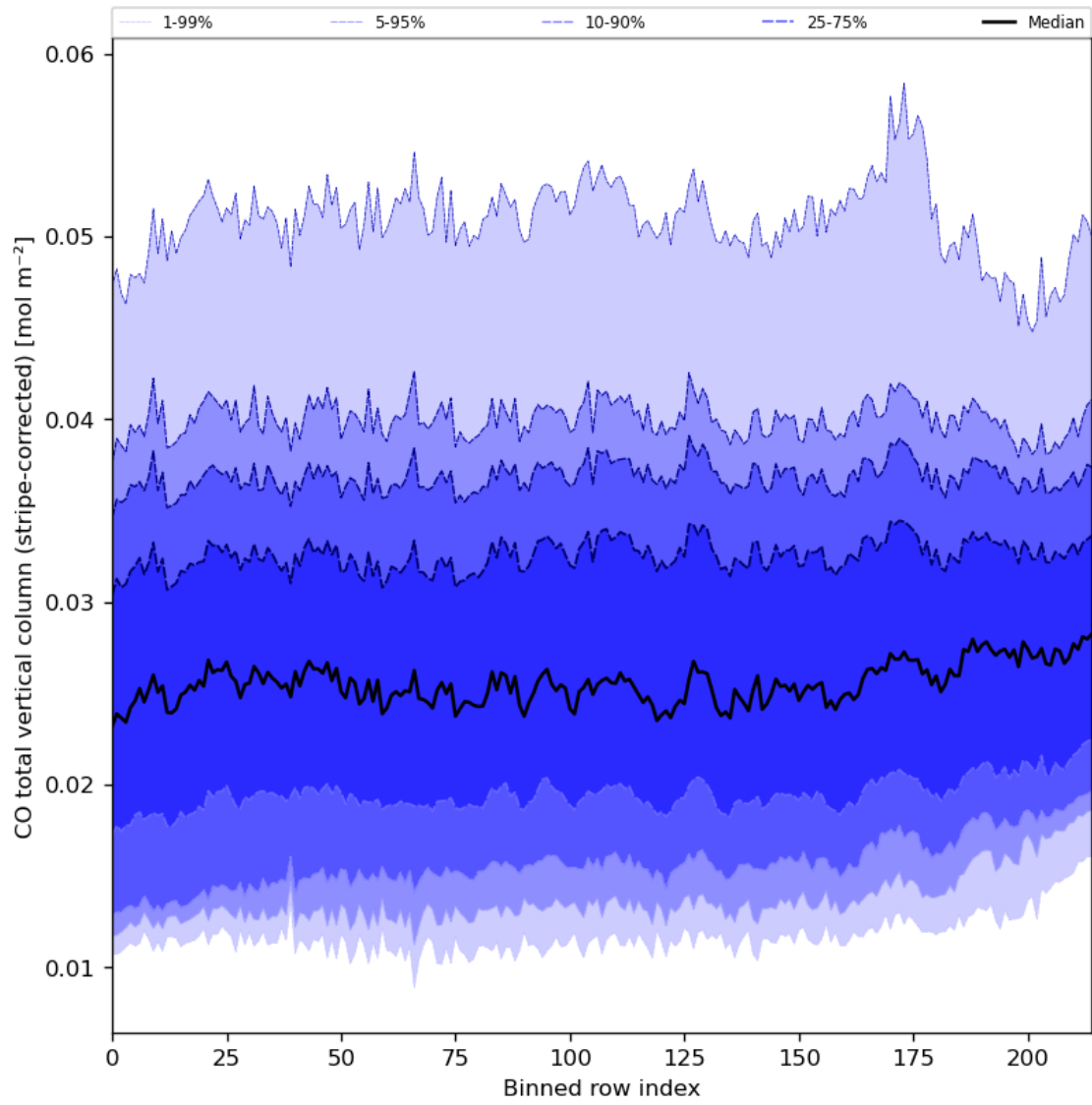
Figure 27: Along track statistics of “CO total vertical column (stripe-corrected)” for 2023-10-24 to 2023-10-26
