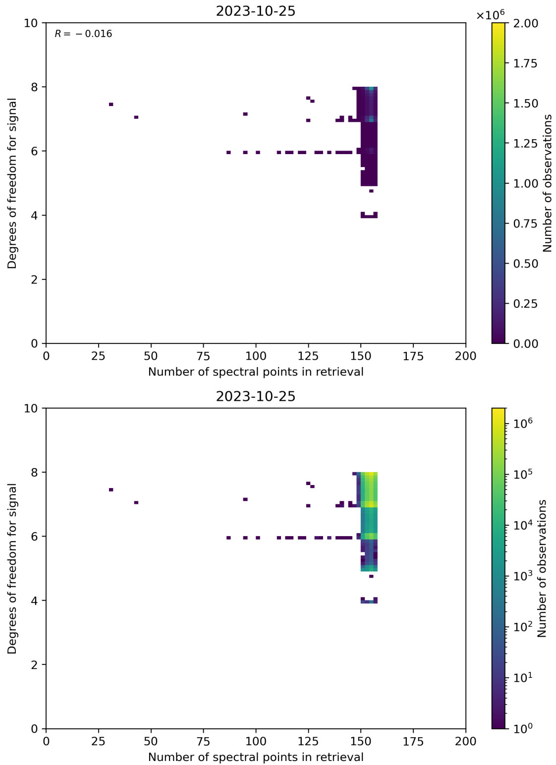
Figure 59: Scatter density plot of “Number of spectral points in retrieval” against “Degrees of freedom for signal” for 2023-10-24 to 2023-10-26.
