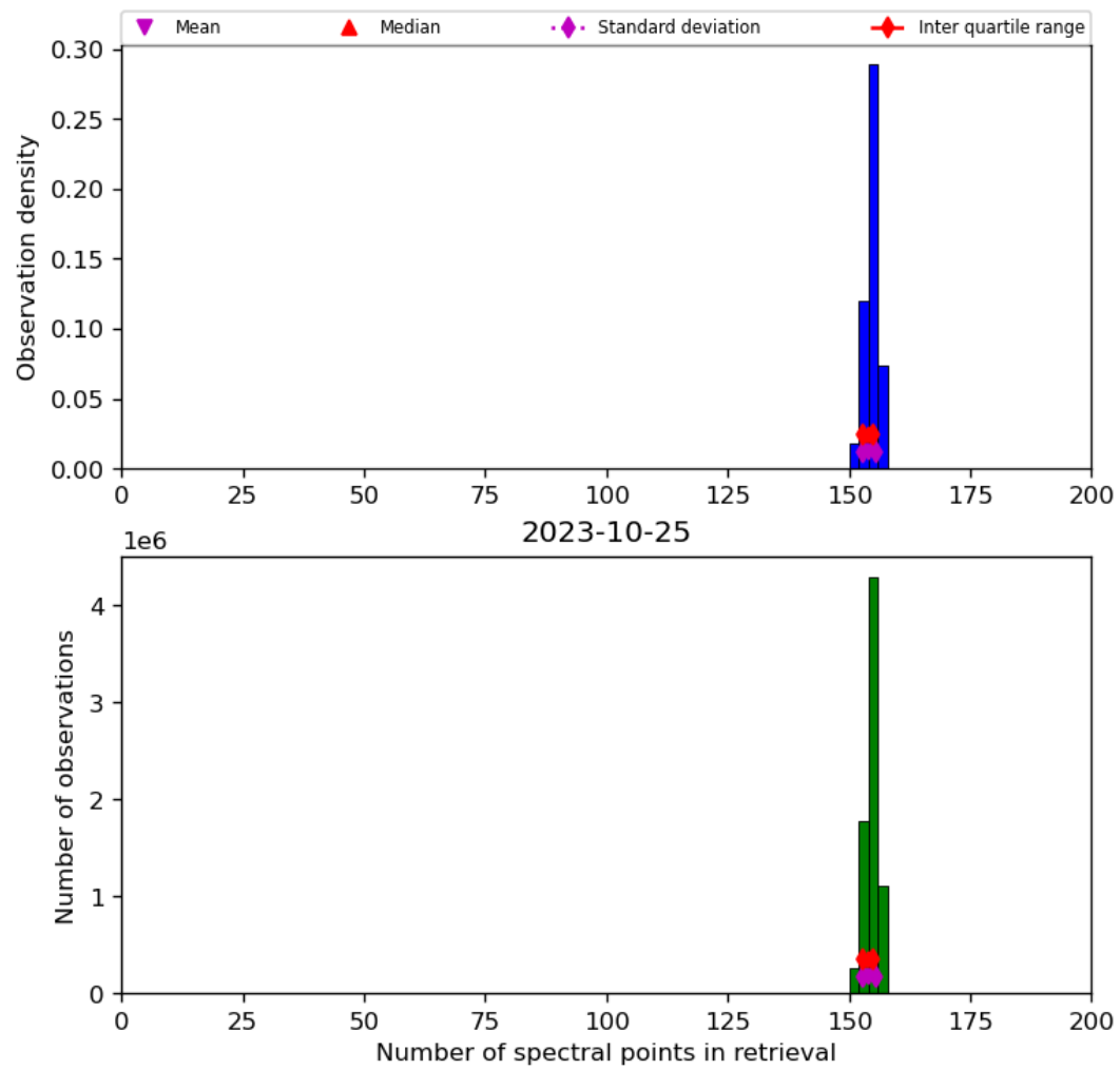
Figure 21: Histogram of “Number of spectral points in retrieval” for 2023-10-24 to 2023-10-26
