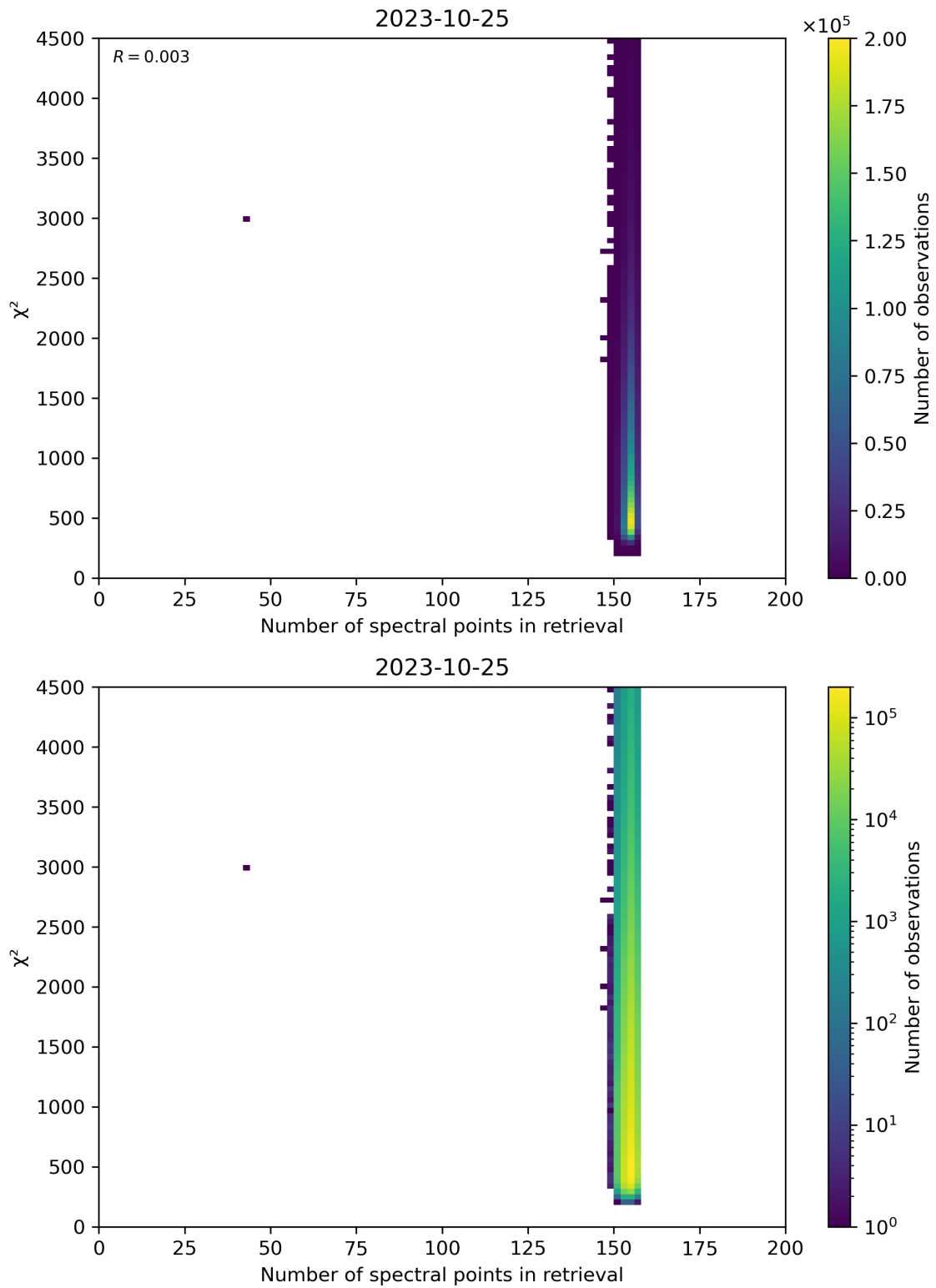
Figure 58: Scatter density plot of “Number of spectral points in retrieval” against “ \chi^2 ” for 2023-10-24 to 2023-10-26.
