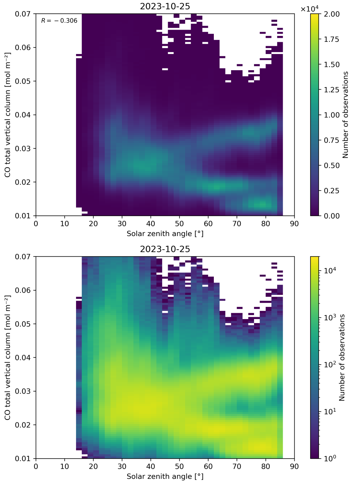
Figure 61: Scatter density plot of “Solar zenith angle” against “CO total vertical column” for 2023-10-24 to 2023-10-26.
