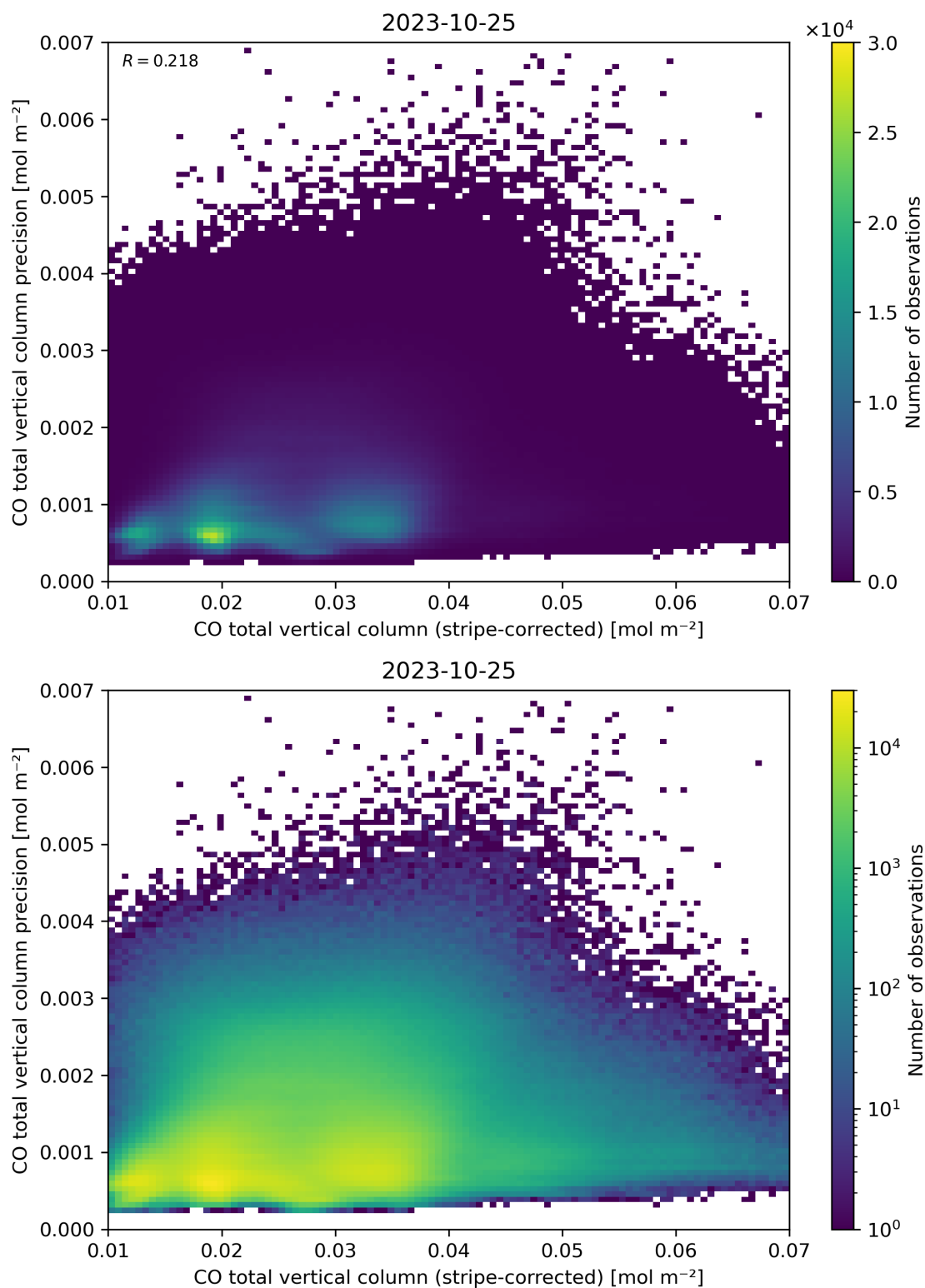
Figure 36: Scatter density plot of “CO total vertical column (stripe-corrected)” against “CO total vertical column precision” for 2023-10-24 to 2023-10-26.
