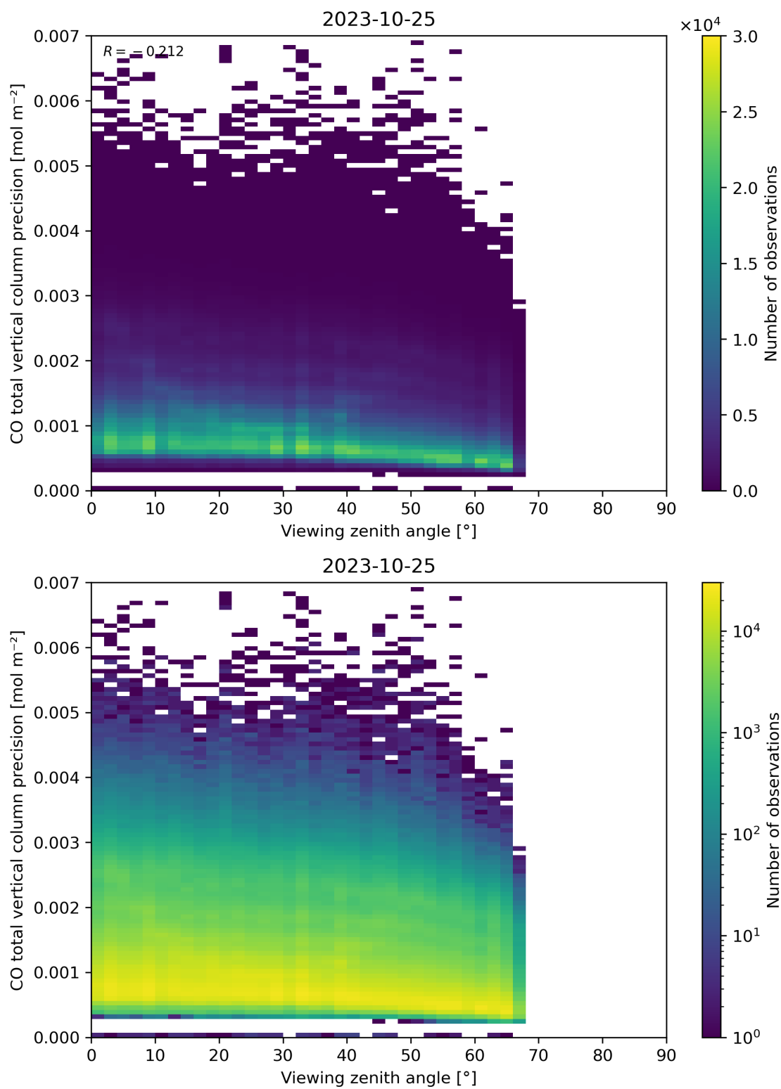
Figure 71: Scatter density plot of “Viewing zenith angle” against “CO total vertical column precision” for 2023-10-24 to 2023-10-26.
