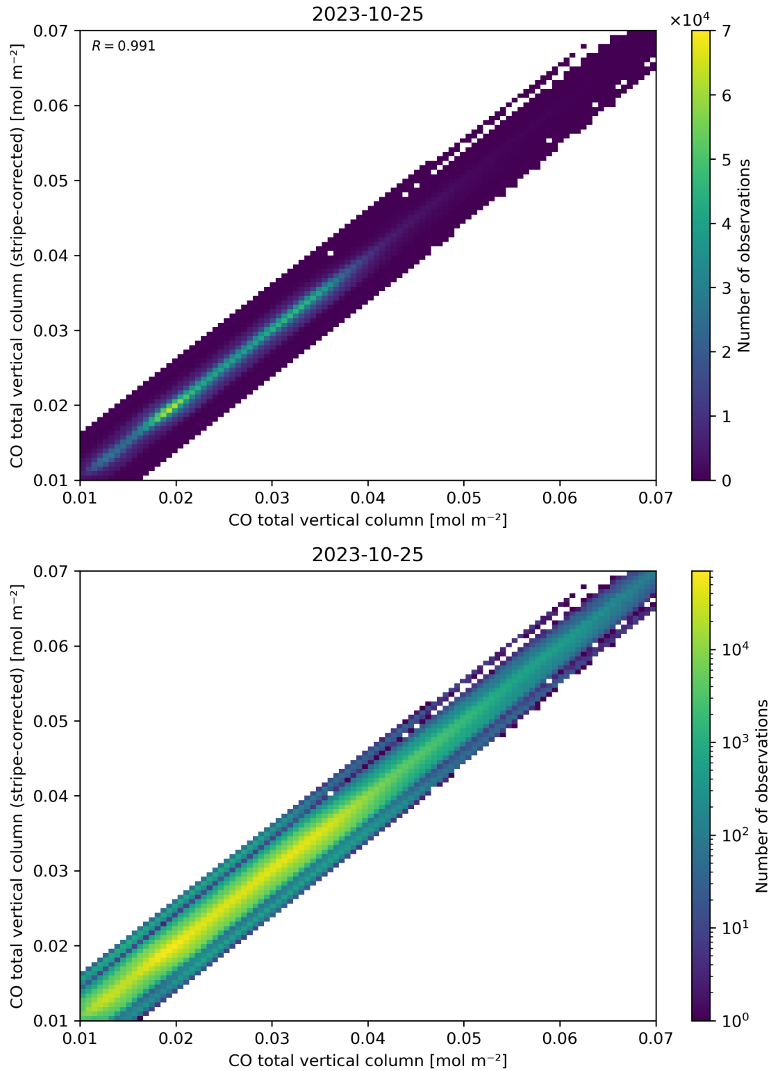
Figure 33: Scatter density plot of “CO total vertical column” against “CO total vertical column (stripe-corrected)” for 2023-10-24 to 2023-10-26.
