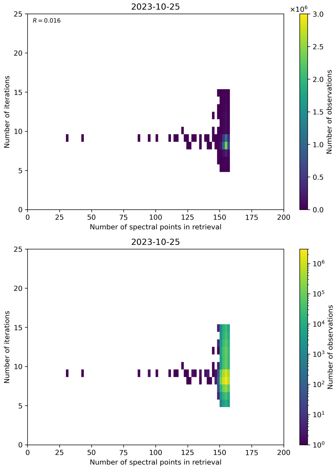
Figure 60: Scatter density plot of “Number of spectral points in retrieval” against “Number of iterations” for 2023-10-24 to 2023-10-26.
