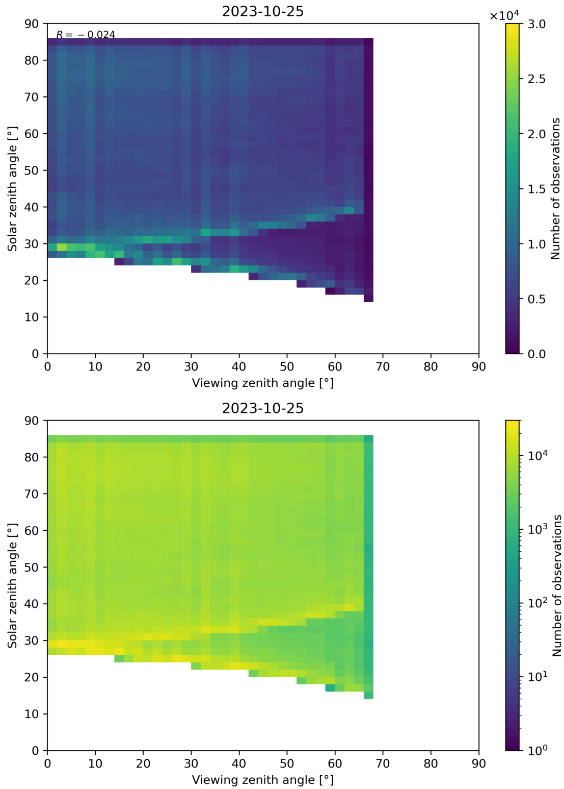
Figure 77: Scatter density plot of “Viewing zenith angle” against “Solar zenith angle” for 2023-10-24 to 2023-10-26.
