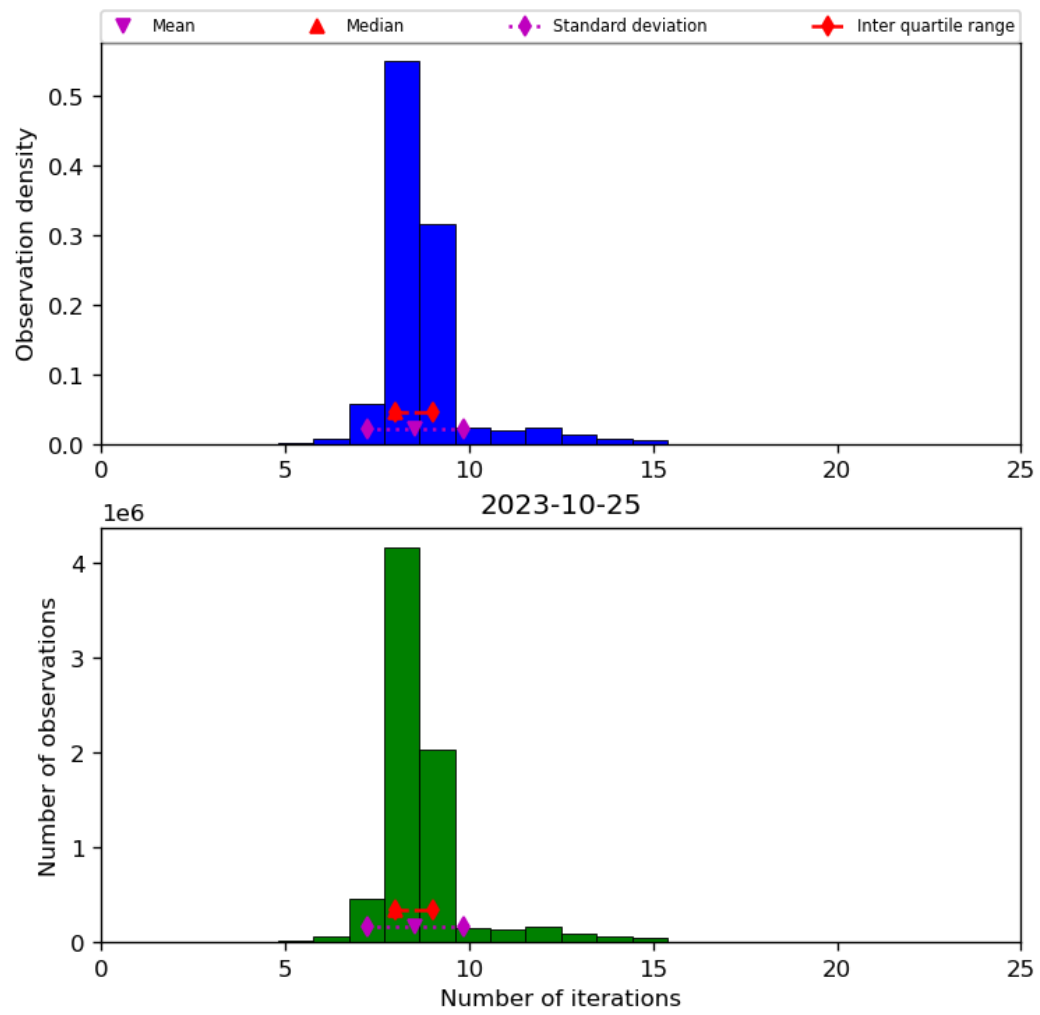
Figure 24: Histogram of “Number of iterations” for 2023-10-24 to 2023-10-26
