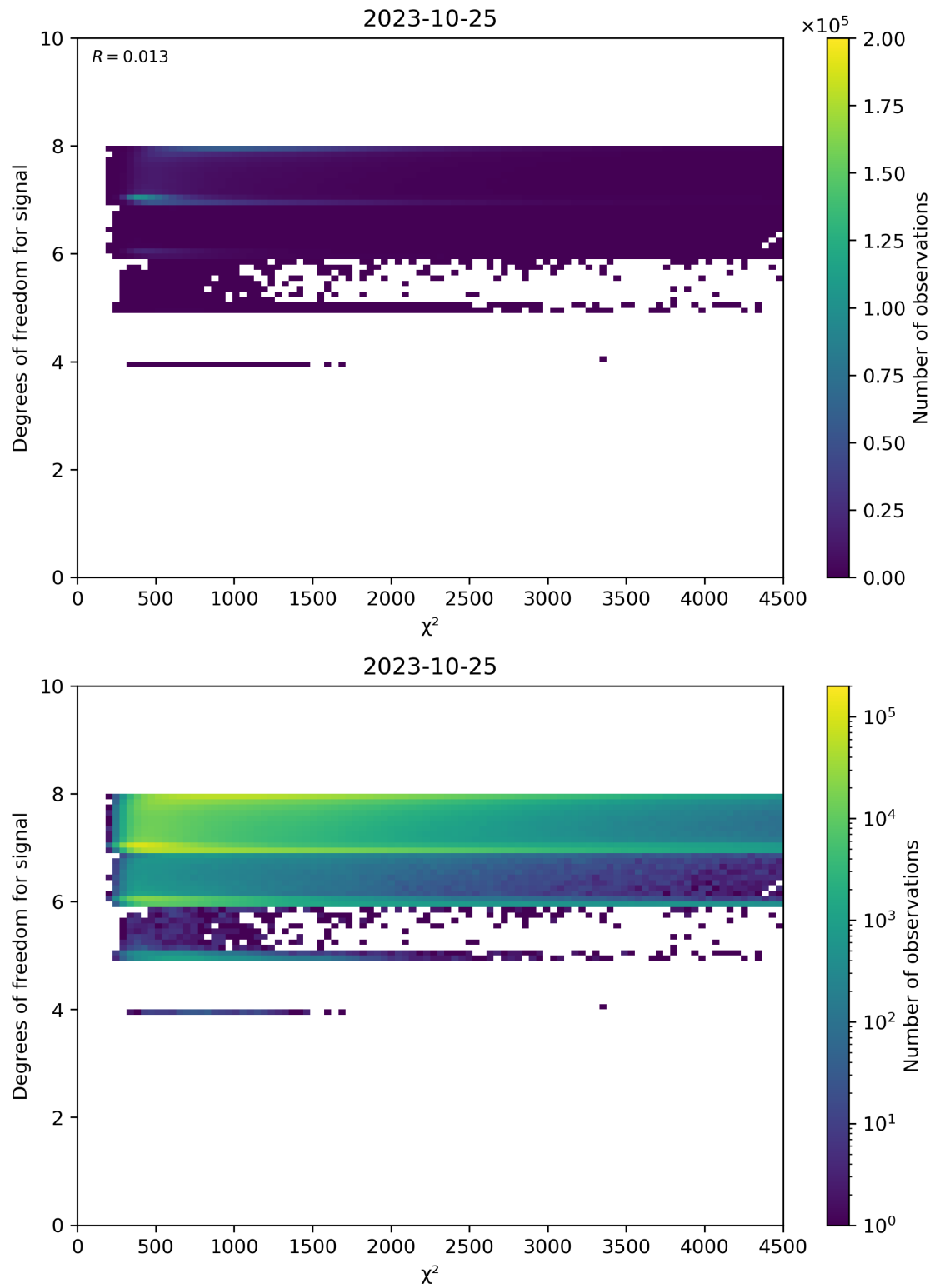
Figure 48: Scatter density plot of “ \chi^2 ” against “Degrees of freedom for signal” for 2023-10-24 to 2023-10-26.
