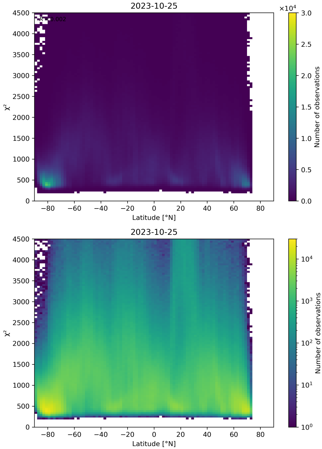
Figure 54: Scatter density plot of “Latitude” against “ \chi^2 ” for 2023-10-24 to 2023-10-26.
