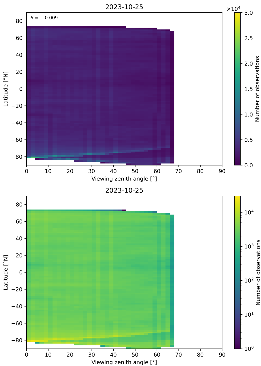
Figure 74: Scatter density plot of “Viewing zenith angle” against “Latitude” for 2023-10-24 to 2023-10-26.
