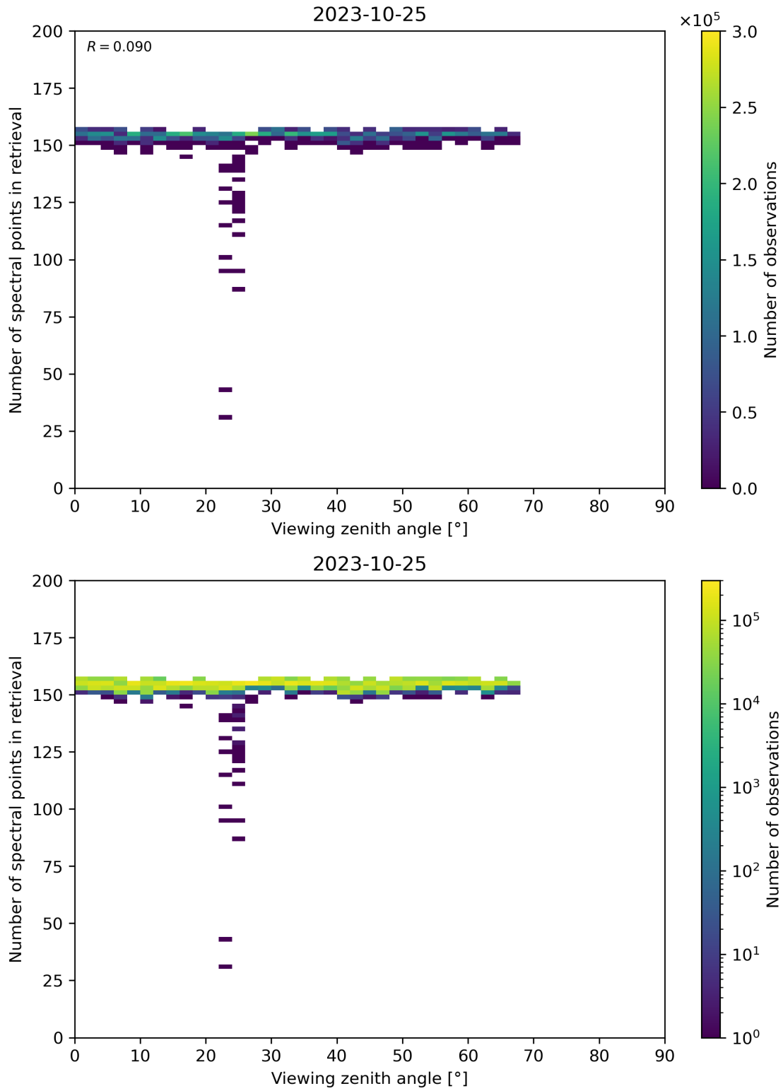
Figure 76: Scatter density plot of “Viewing zenith angle” against “Number of spectral points in retrieval” for 2023-10-24 to 2023-10-26.
