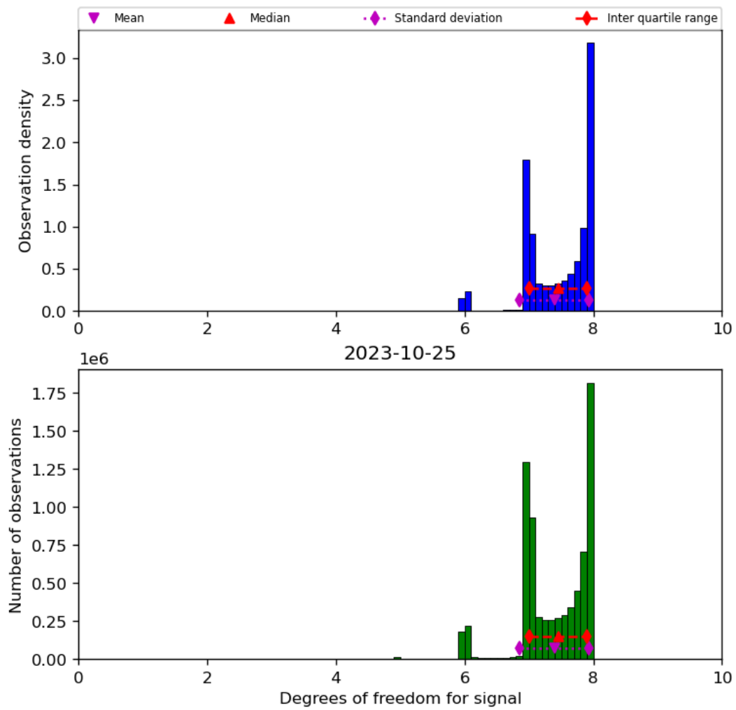
Figure 23: Histogram of “Degrees of freedom for signal” for 2023-10-24 to 2023-10-26
