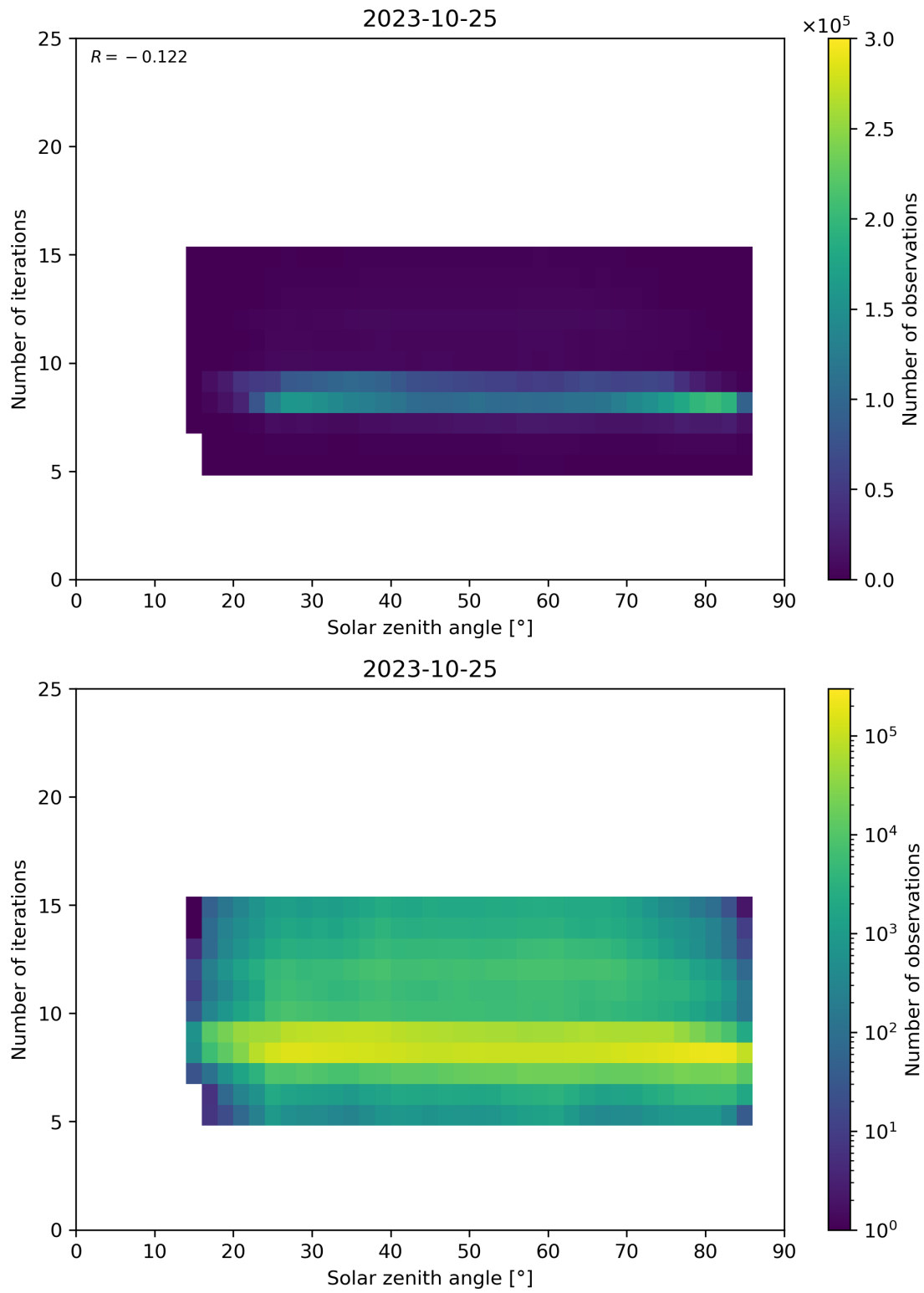
Figure 67: Scatter density plot of “Solar zenith angle” against “Number of iterations” for 2023-10-24 to 2023-10-26.
