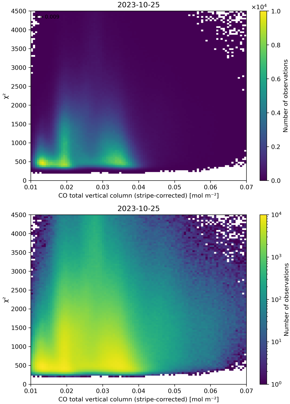
Figure 37: Scatter density plot of “CO total vertical column (stripe-corrected)” against “ \chi^2 ” for 2023-10-24 to 2023-10-26.
