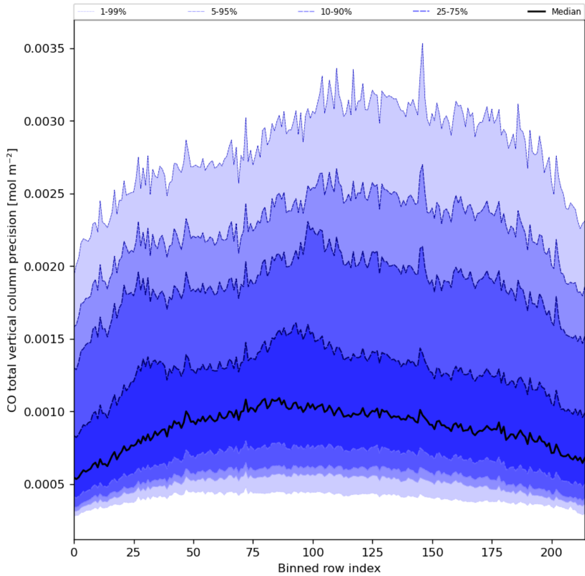
Figure 28: Along track statistics of “CO total vertical column precision” for 2023-10-24 to 2023-10-26
