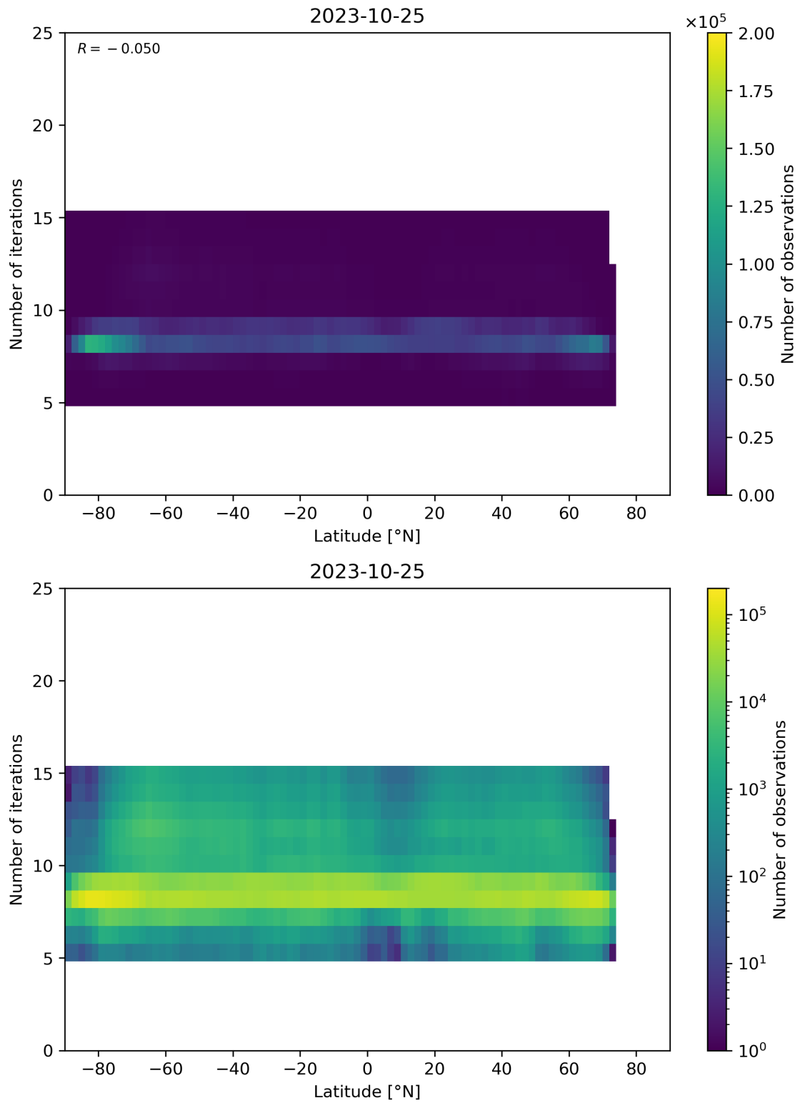
Figure 56: Scatter density plot of “Latitude” against “Number of iterations” for 2023-10-24 to 2023-10-26.
