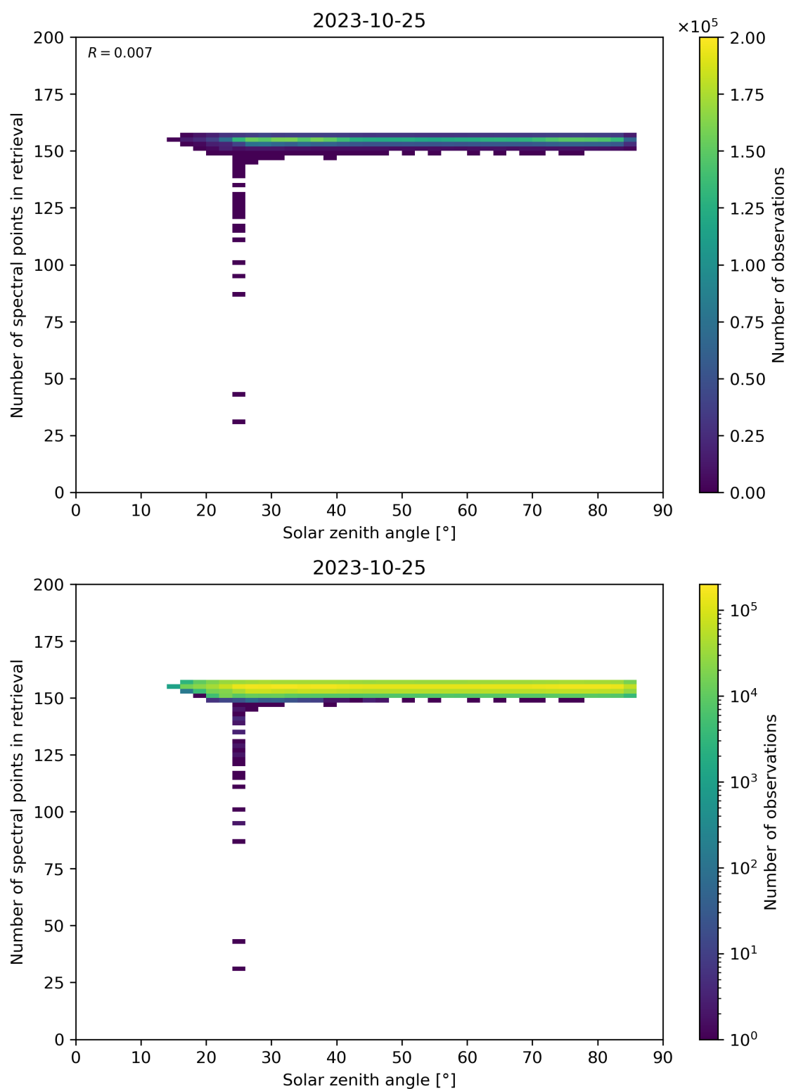
Figure 68: Scatter density plot of “Solar zenith angle” against “Number of spectral points in retrieval” for 2023-10-24 to 2023-10-26.
