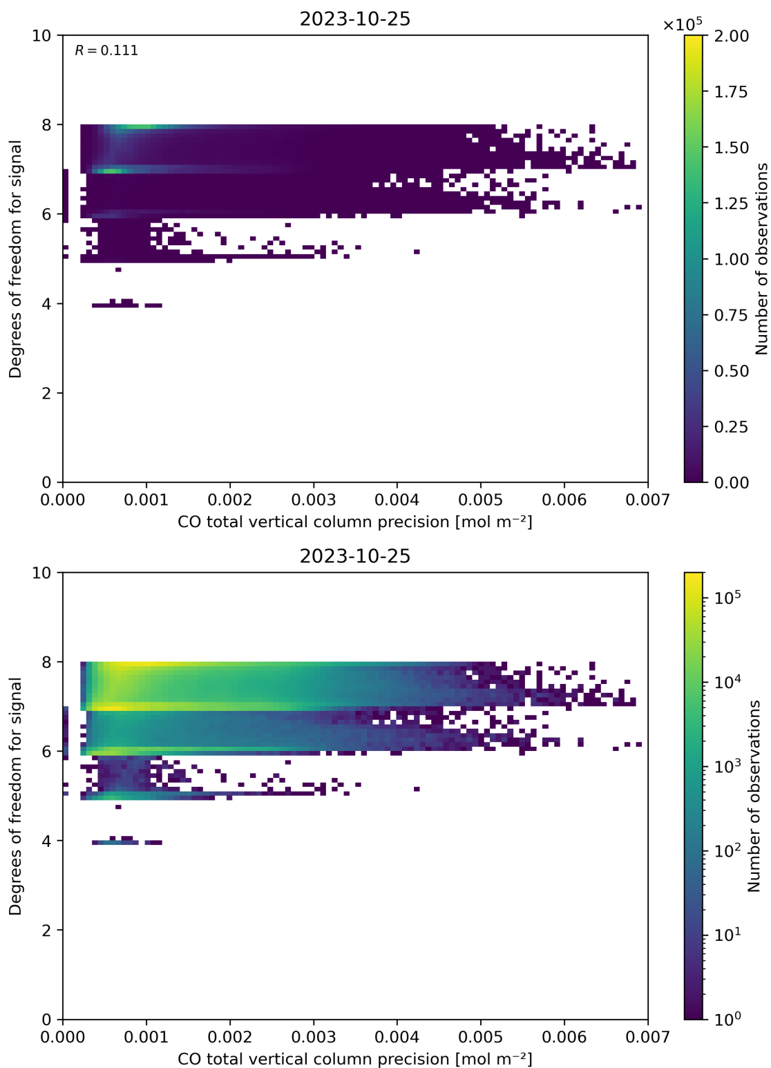
Figure 45: Scatter density plot of “CO total vertical column precision” against “Degrees of freedom for signal” for 2023-10-24 to 2023-10-26.
