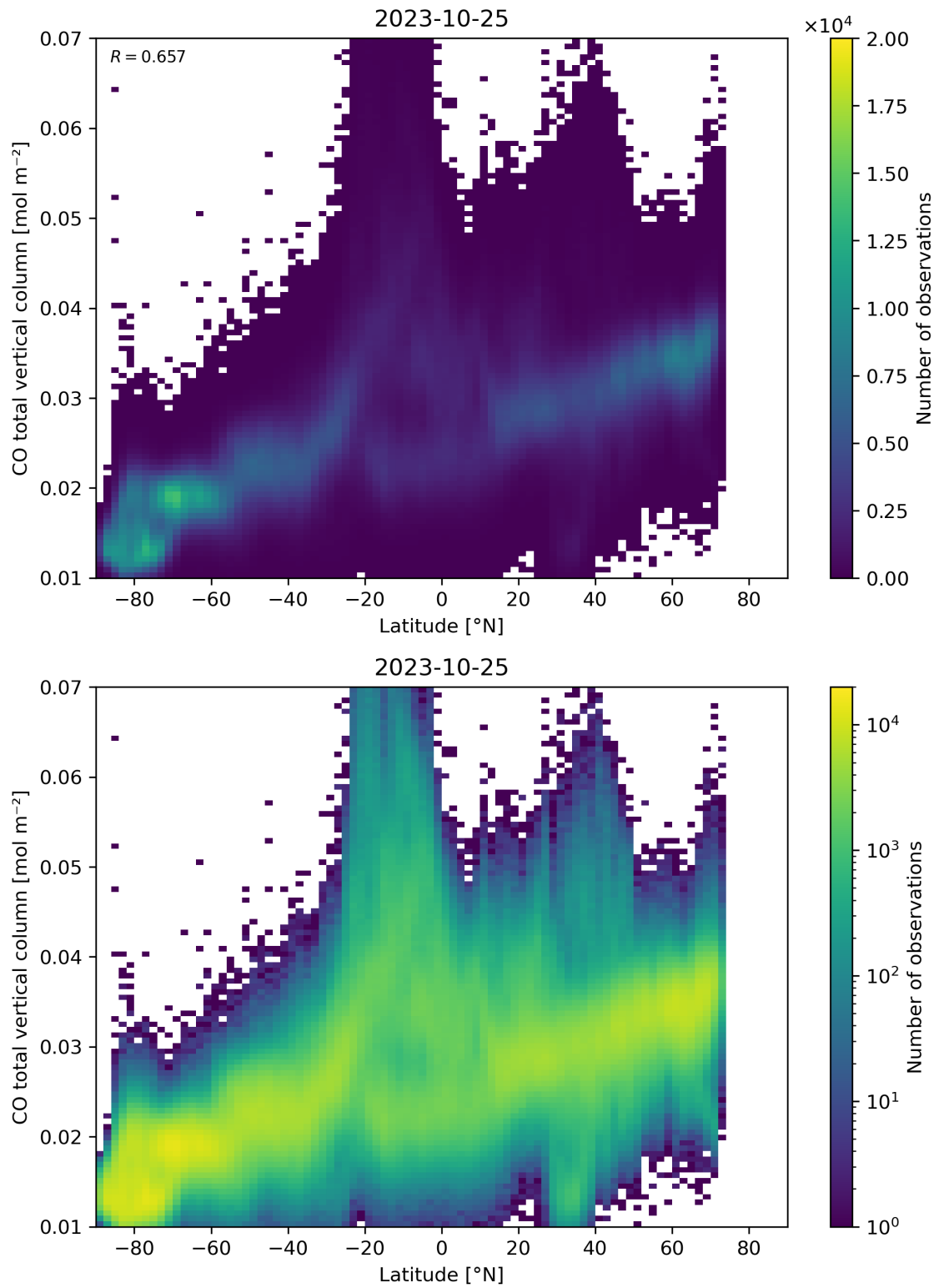
Figure 51: Scatter density plot of “Latitude” against “CO total vertical column” for 2023-10-24 to 2023-10-26.
