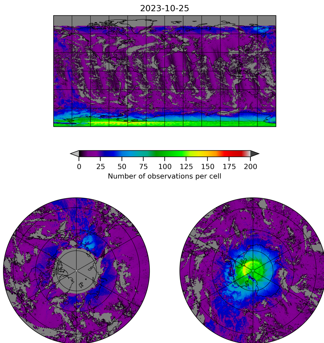
Figure 8: Map of the number of observations for 2023-10-24 to 2023-10-26
