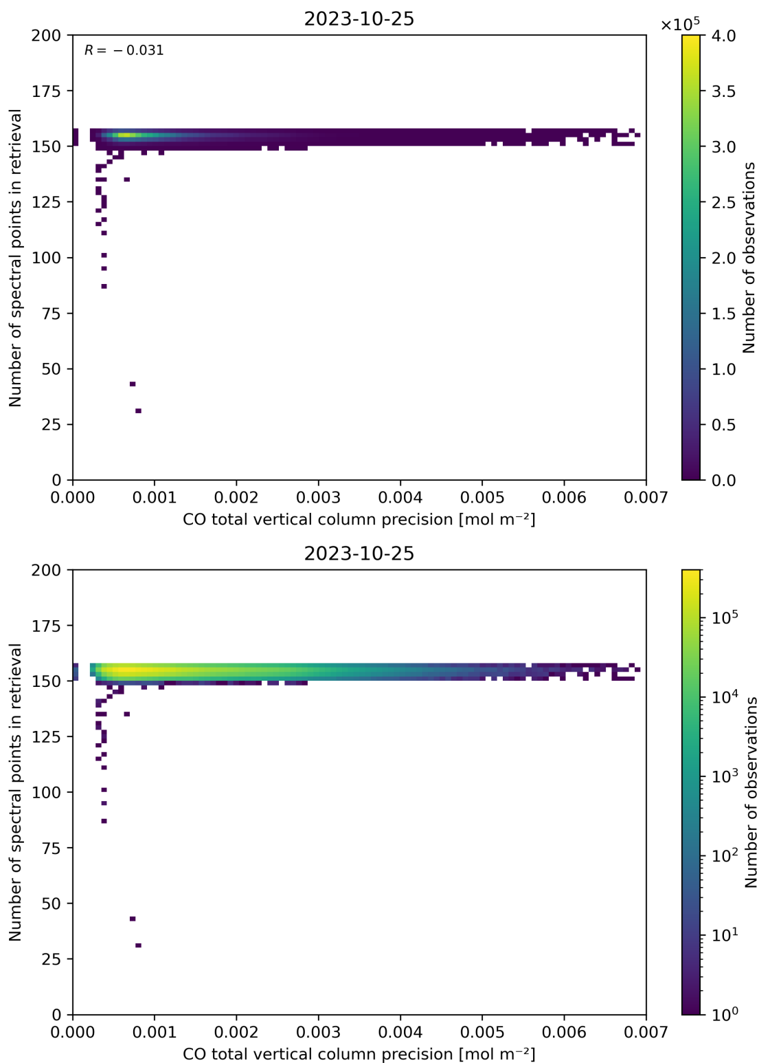
Figure 47: Scatter density plot of “CO total vertical column precision” against “Number of spectral points in retrieval” for 2023-10-24 to 2023-10-26.
