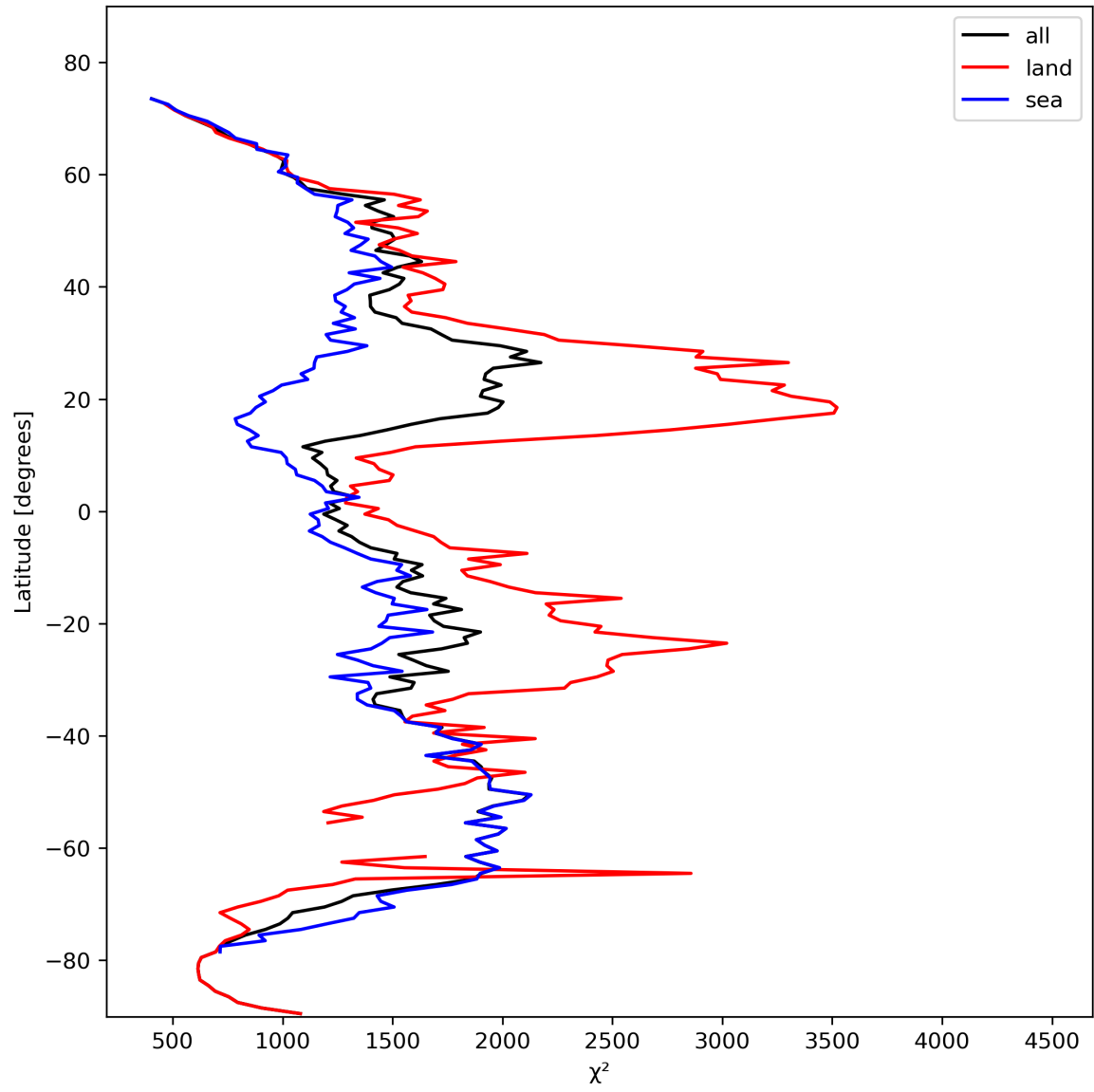
Figure 14: Zonal average of “ \chi^2 ” for 2023-10-24 to 2023-10-26.
