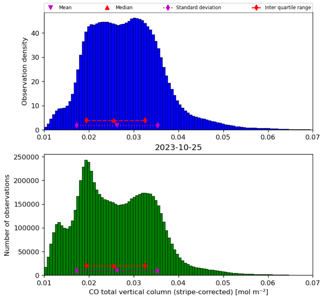
Figure 19: Histogram of “CO total vertical column (stripe-corrected)” for 2023-10-24 to 2023-10-26
