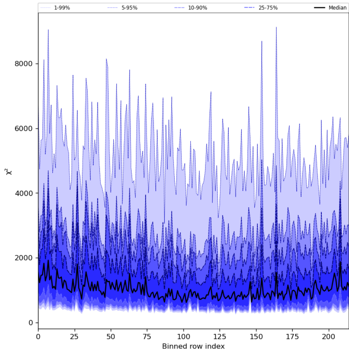
Figure 30: Along track statistics of “ \chi^2 ” for 2023-10-24 to 2023-10-26
