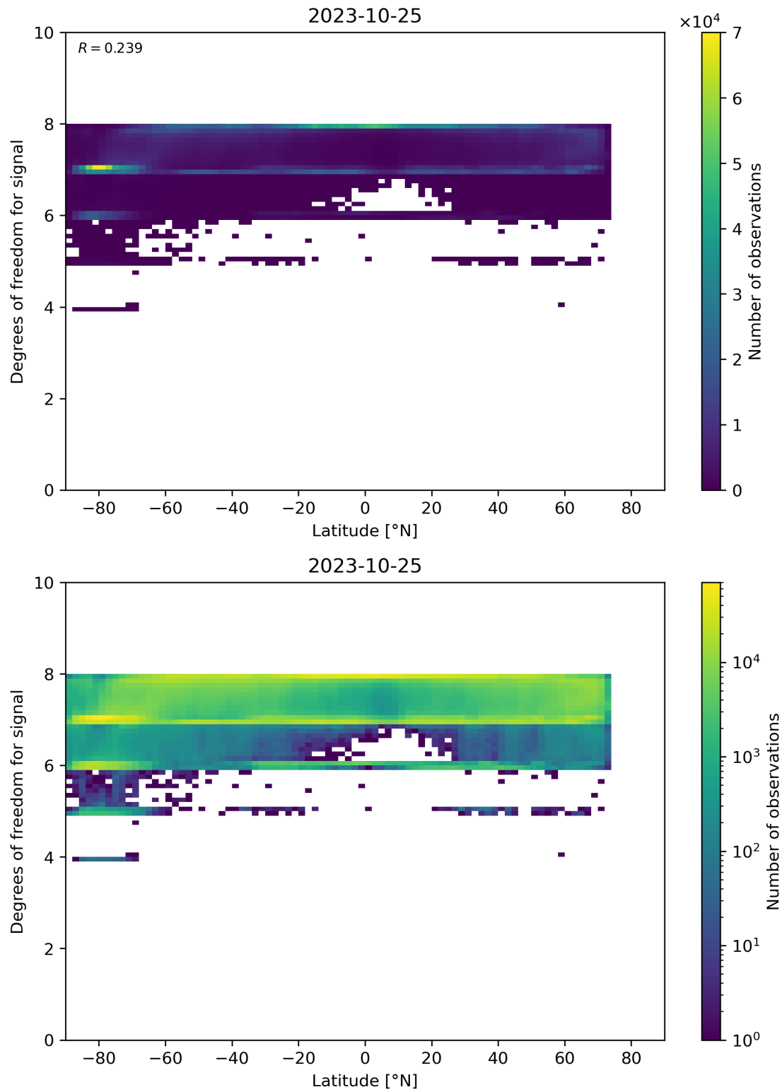
Figure 55: Scatter density plot of “Latitude” against “Degrees of freedom for signal” for 2023-10-24 to 2023-10-26.
