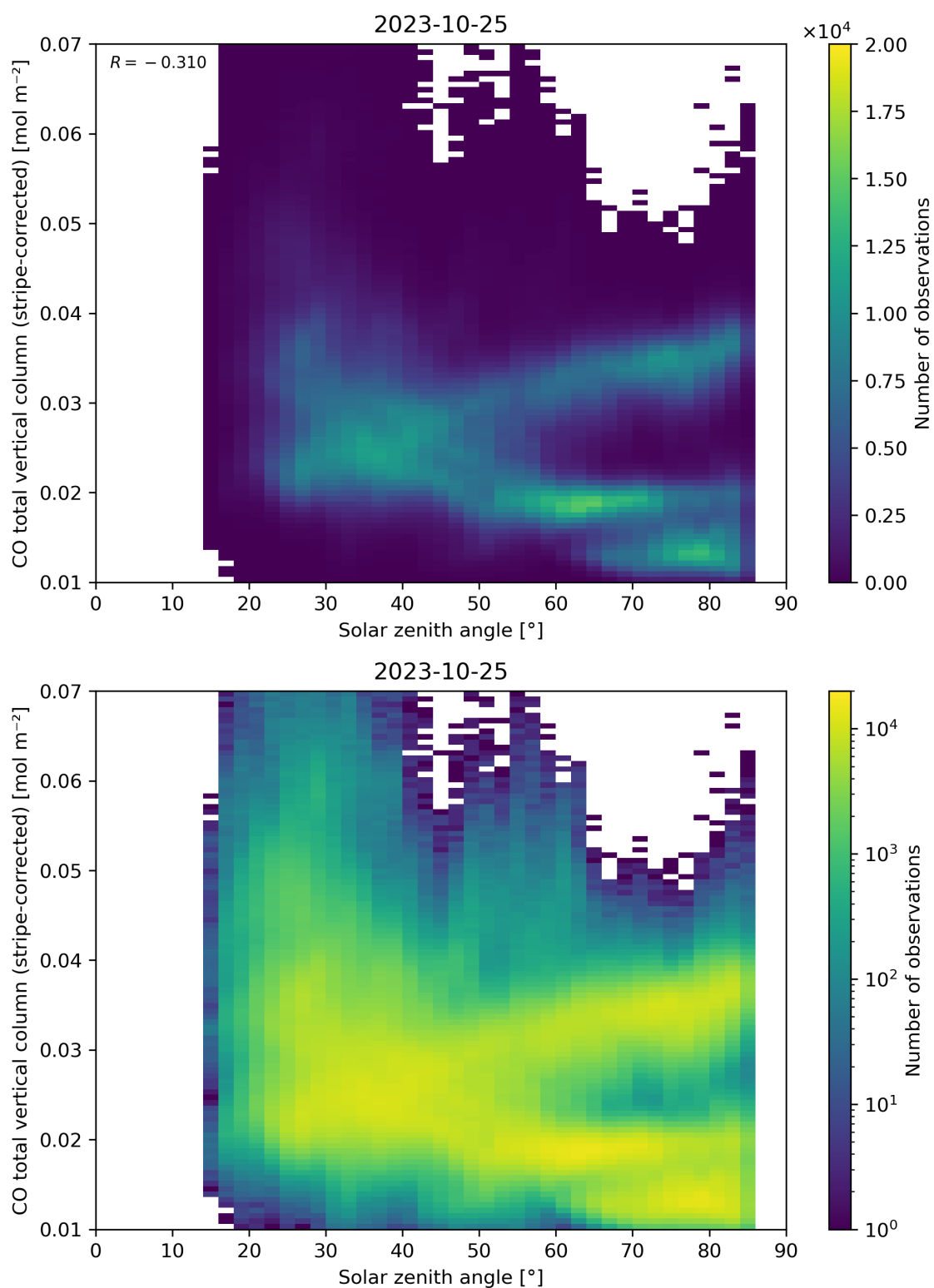
Figure 62: Scatter density plot of “Solar zenith angle” against “CO total vertical column (stripe-corrected)” for 2023-10-24 to 2023-10-26.
