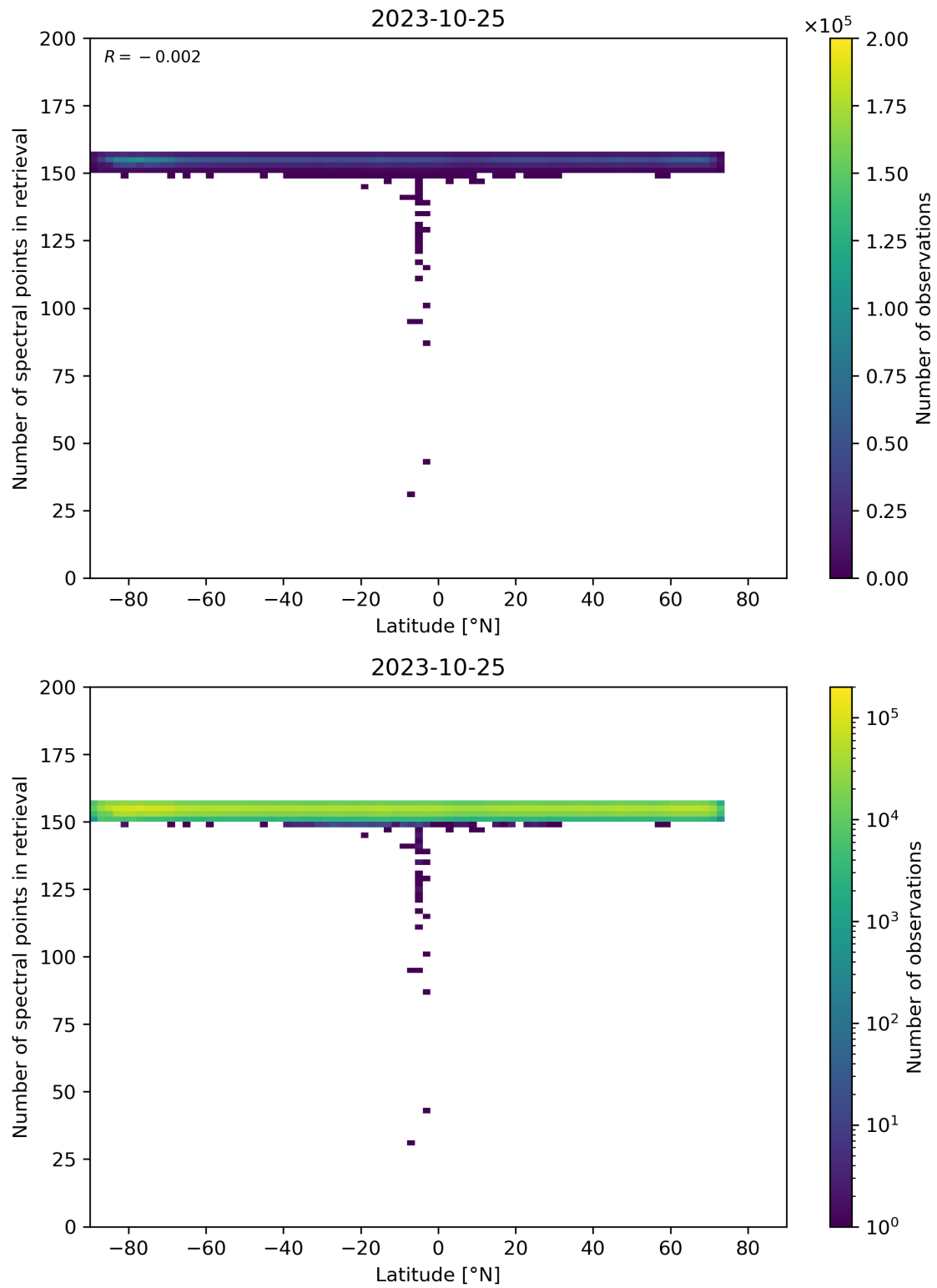
Figure 57: Scatter density plot of “Latitude” against “Number of spectral points in retrieval” for 2023-10-24 to 2023-10-26.
