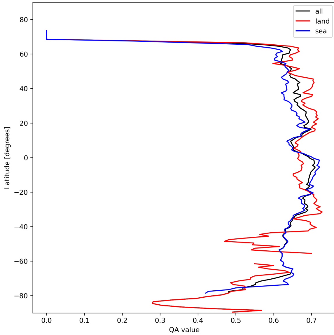
Figure 9: Zonal average of “QA value” for 2023-10-24 to 2023-10-26.
