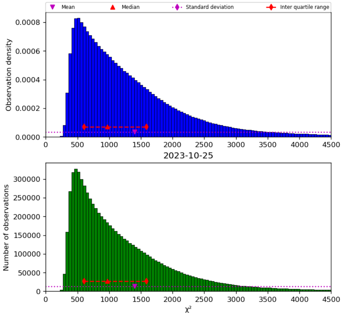
Figure 22: Histogram of “ \chi^2 ” for 2023-10-24 to 2023-10-26
