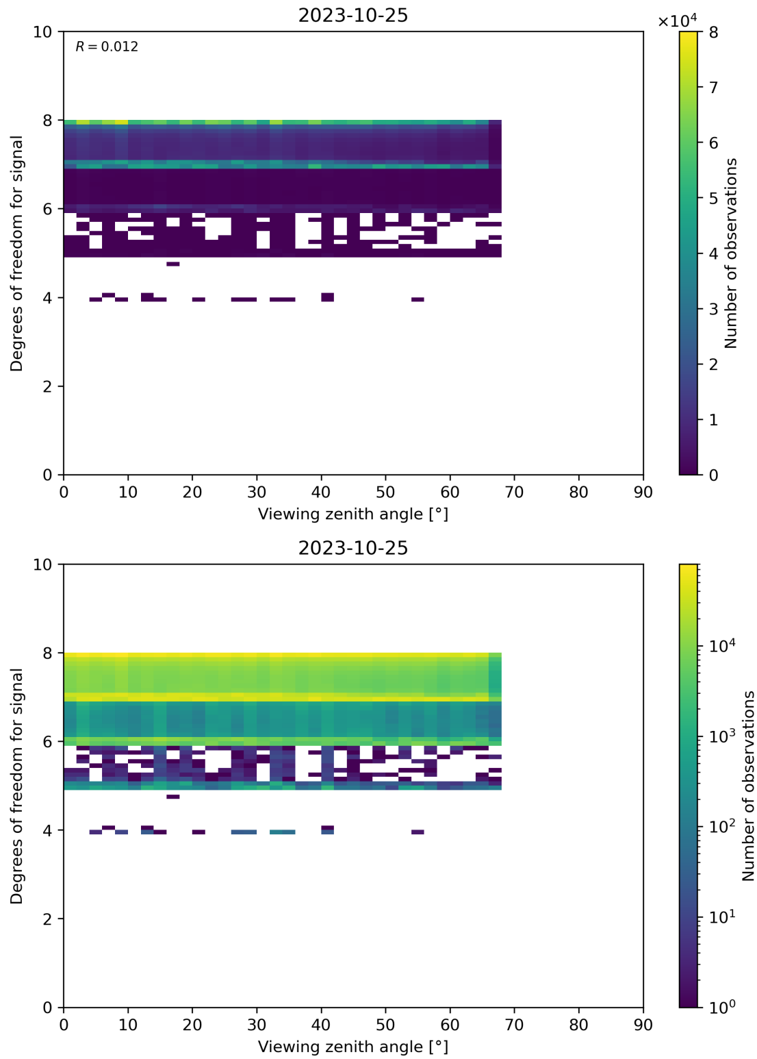
Figure 73: Scatter density plot of “Viewing zenith angle” against “Degrees of freedom for signal” for 2023-10-24 to 2023-10-26.
