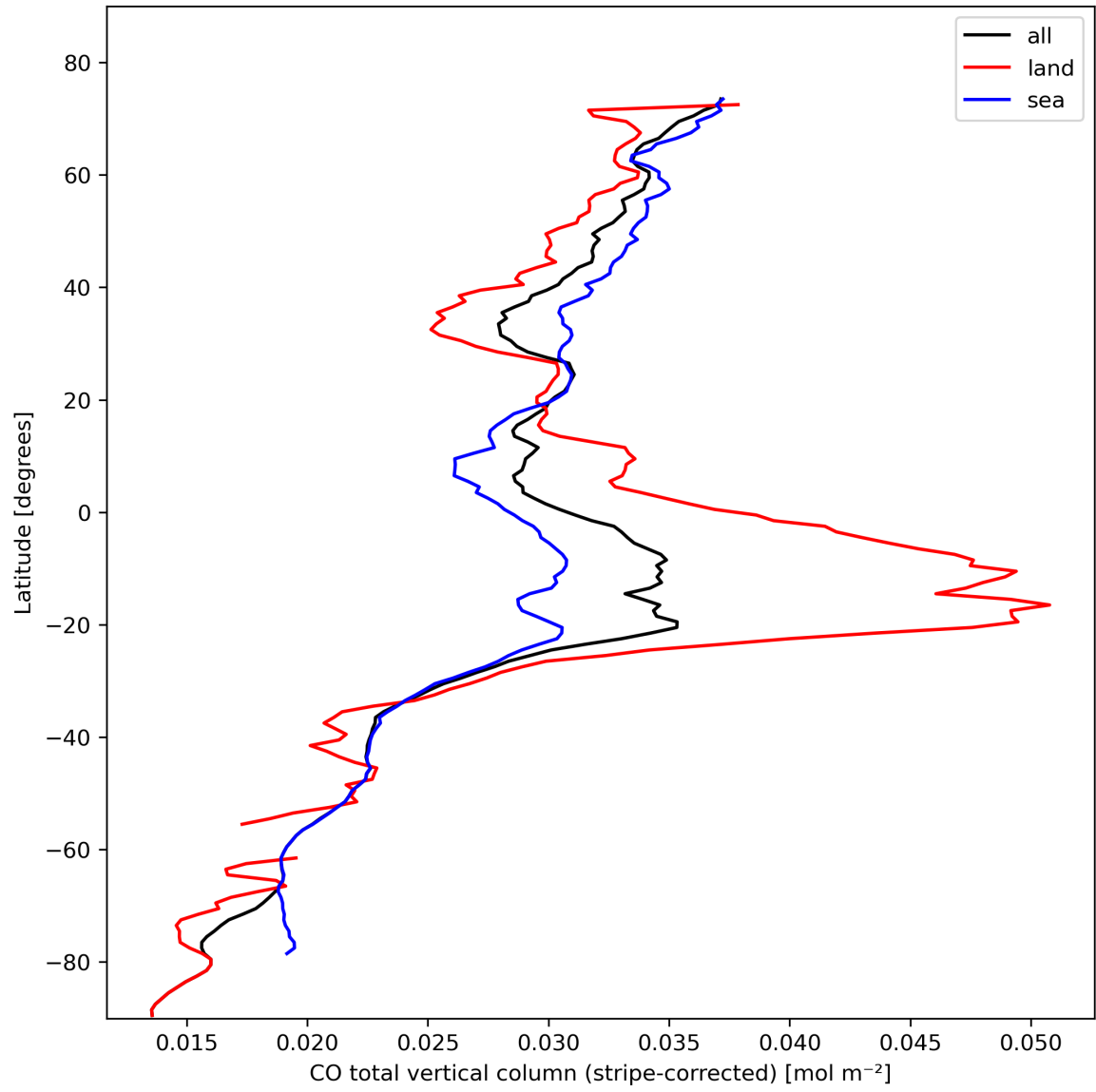
Figure 11: Zonal average of “CO total vertical column (stripe-corrected)” for 2023-10-24 to 2023-10-26.
