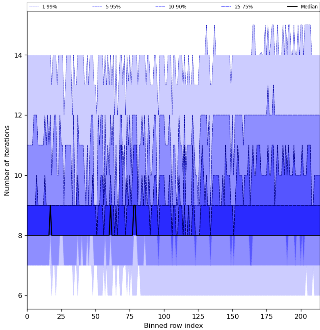
Figure 32: Along track statistics of “Number of iterations” for 2023-10-24 to 2023-10-26
