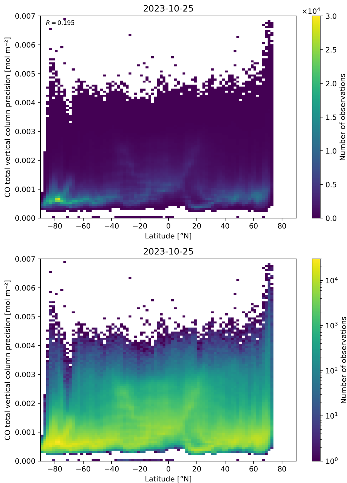
Figure 53: Scatter density plot of “Latitude” against “CO total vertical column precision” for 2023-10-24 to 2023-10-26.
