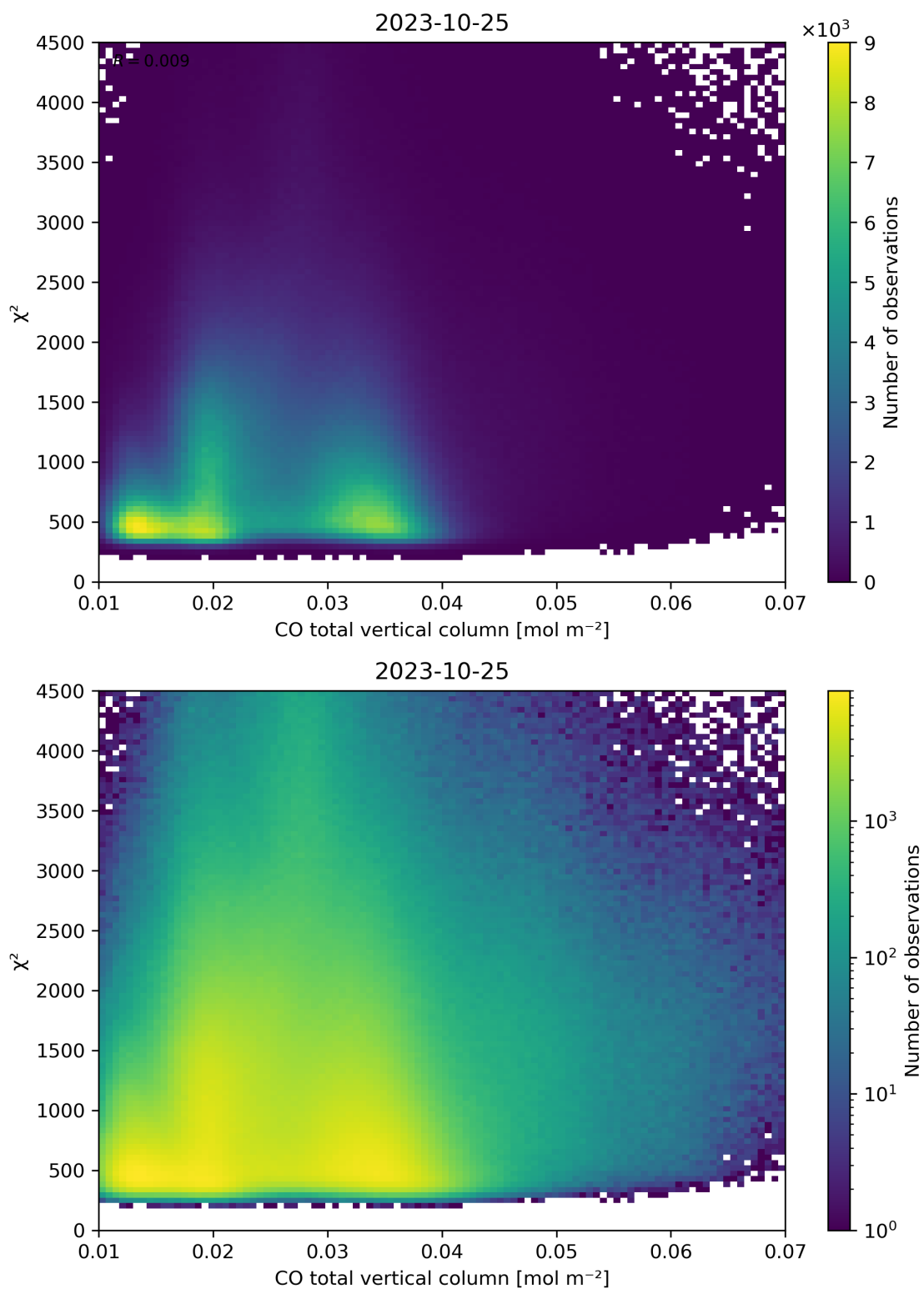
Figure 35: Scatter density plot of “CO total vertical column” against “ \chi^2 ” for 2023-10-24 to 2023-10-26.
