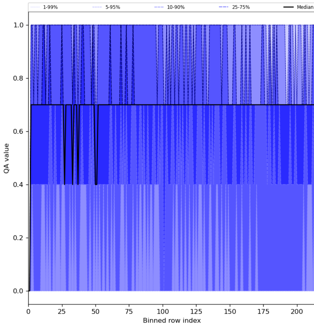
Figure 25: Along track statistics of “QA value” for 2023-10-24 to 2023-10-26
