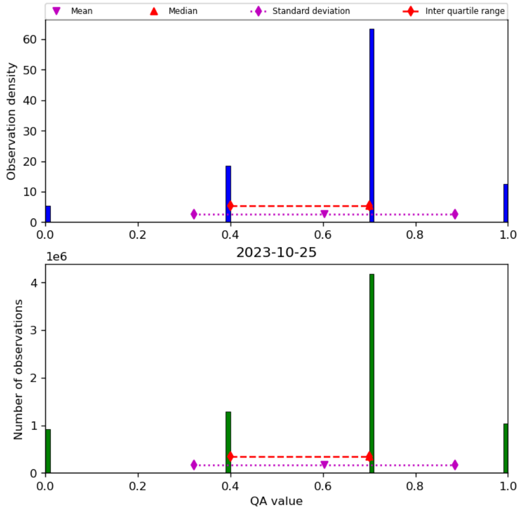
Figure 17: Histogram of “QA value” for 2023-10-24 to 2023-10-26
