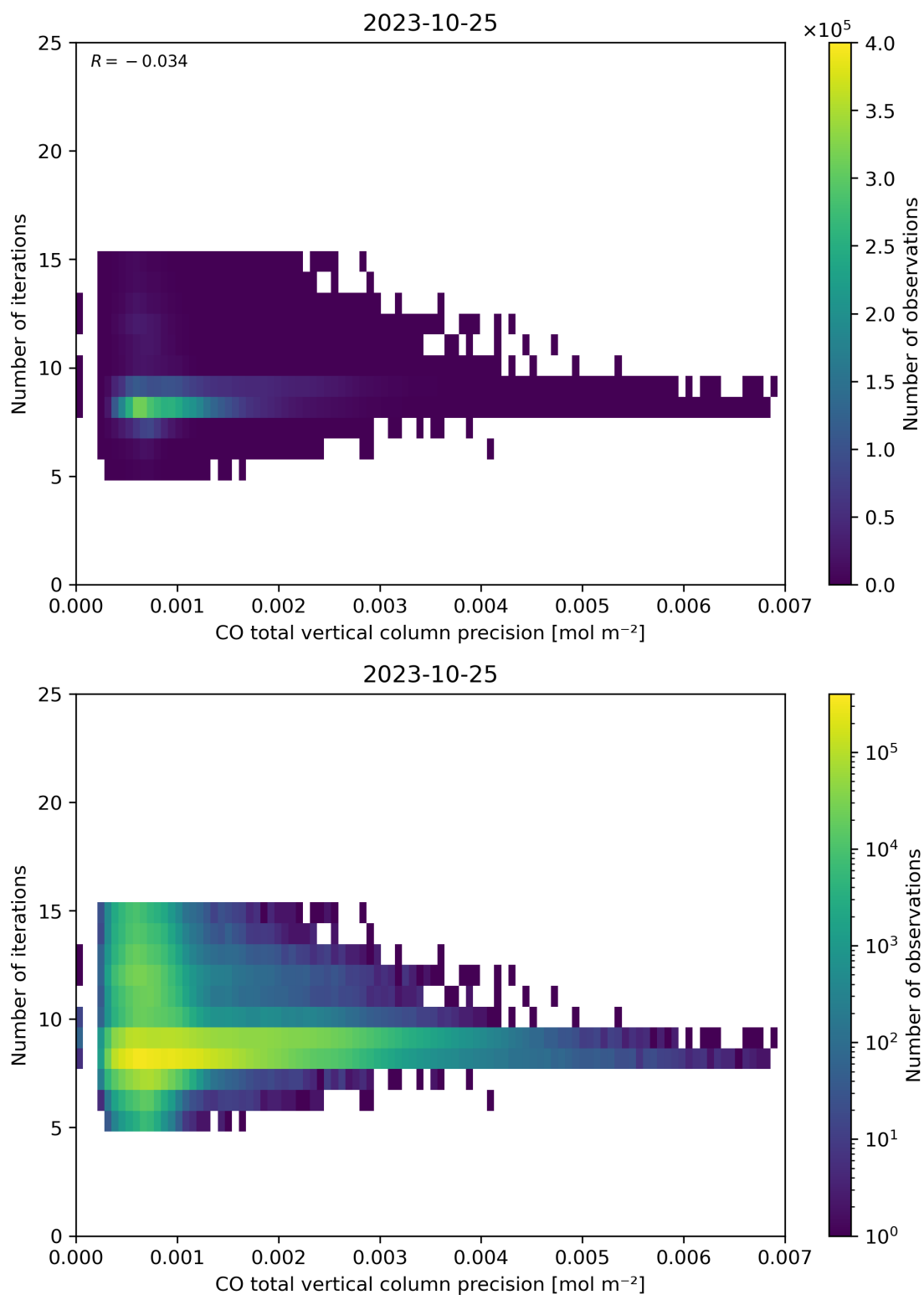
Figure 46: Scatter density plot of “CO total vertical column precision” against “Number of iterations” for 2023-10-24 to 2023-10-26.
