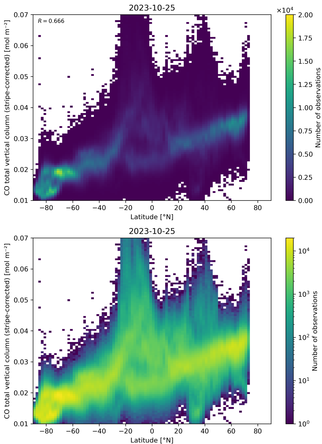
Figure 52: Scatter density plot of “Latitude” against “CO total vertical column (stripe-corrected)” for 2023-10-24 to 2023-10-26.
