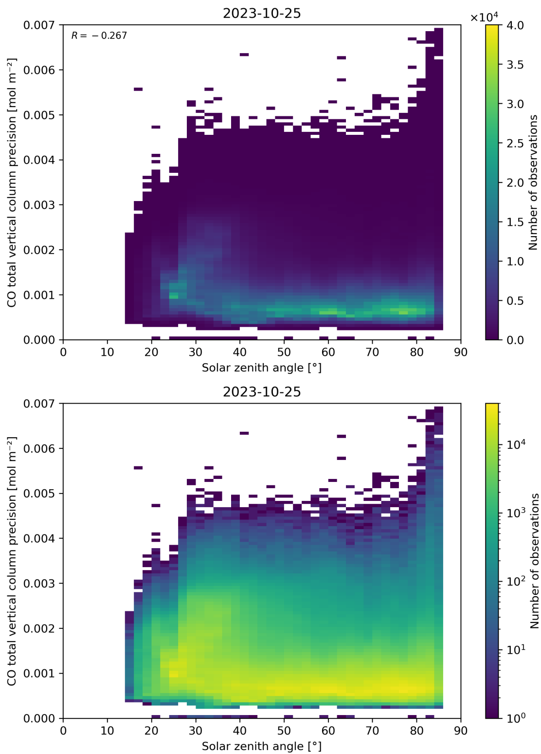
Figure 63: Scatter density plot of “Solar zenith angle” against “CO total vertical column precision” for 2023-10-24 to 2023-10-26.
