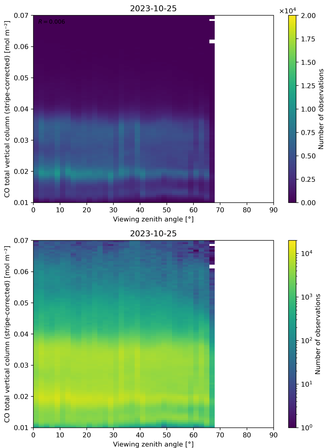
Figure 70: Scatter density plot of “Viewing zenith angle” against “CO total vertical column (stripe-corrected)” for 2023-10-24 to 2023-10-26.
