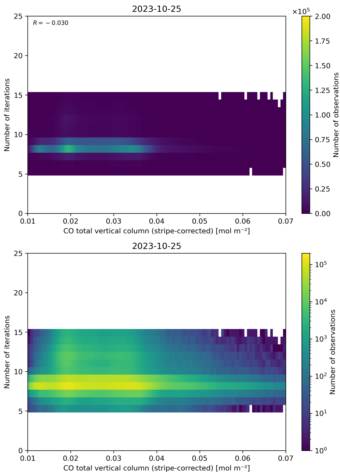
Figure 39: Scatter density plot of “CO total vertical column (stripe-corrected)” against “Number of iterations” for 2023-10-24 to 2023-10-26.
