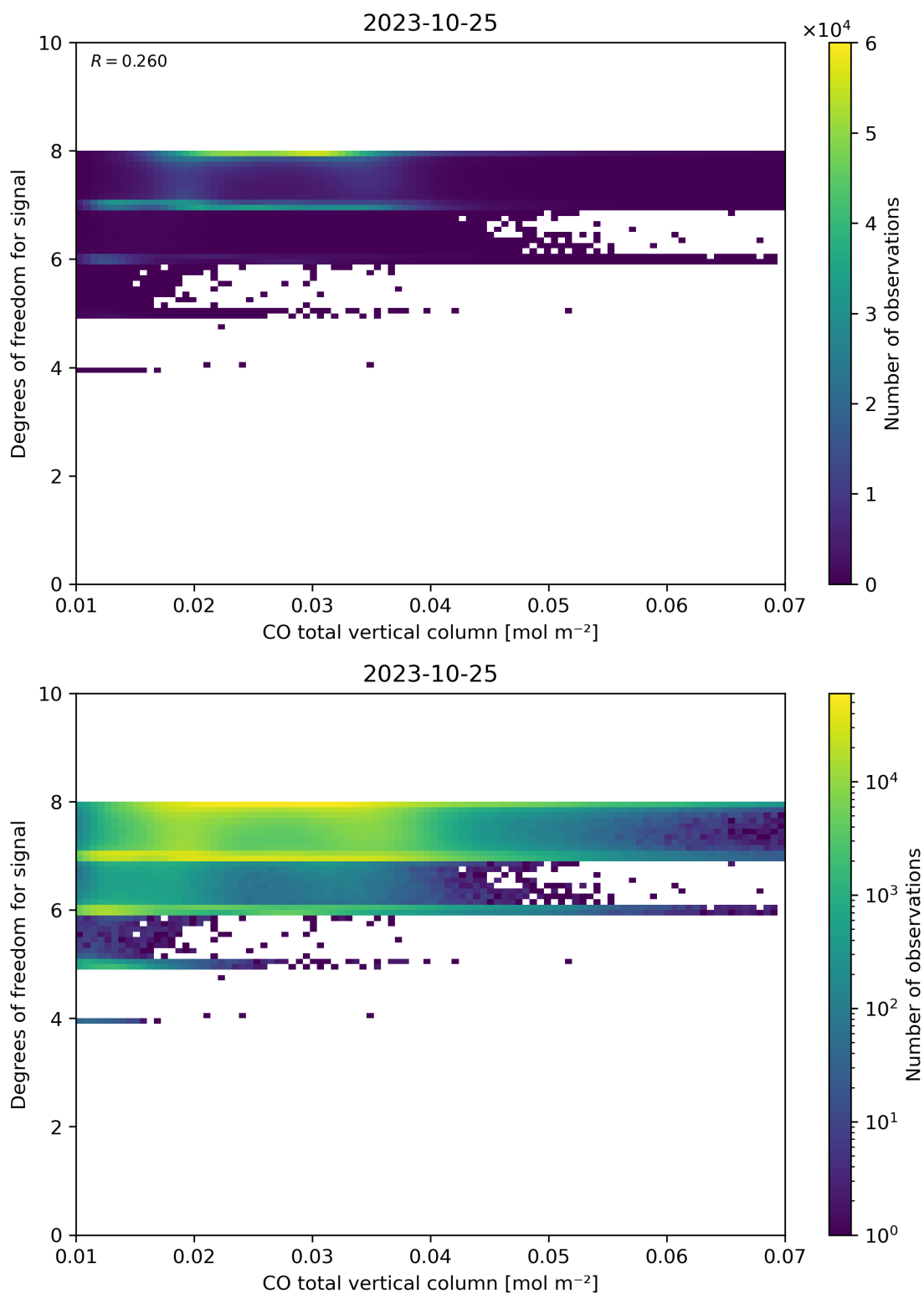
Figure 41: Scatter density plot of “CO total vertical column” against “Degrees of freedom for signal” for 2023-10-24 to 2023-10-26.
