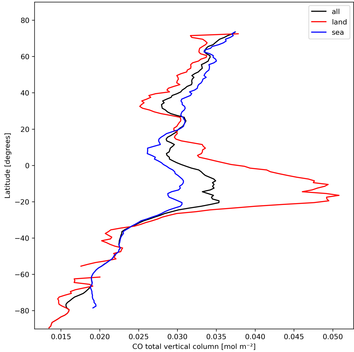
Figure 10: Zonal average of “CO total vertical column” for 2023-10-24 to 2023-10-26.
