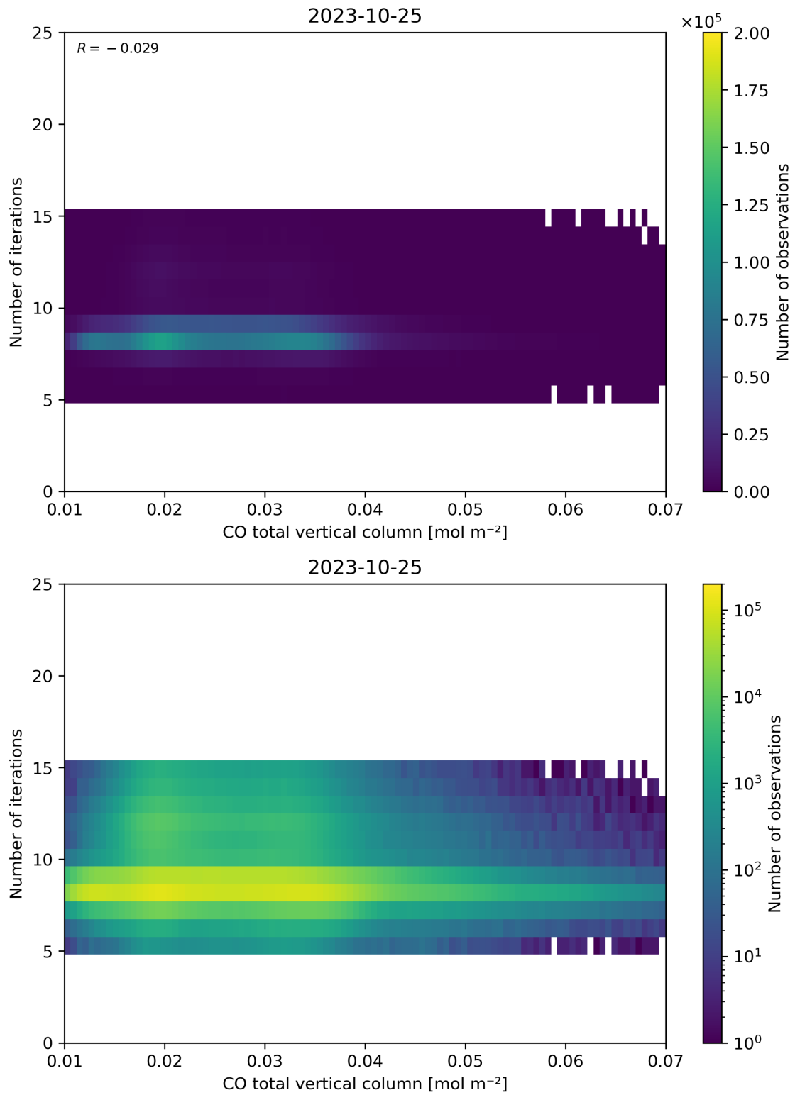
Figure 42: Scatter density plot of “CO total vertical column” against “Number of iterations” for 2023-10-24 to 2023-10-26.
