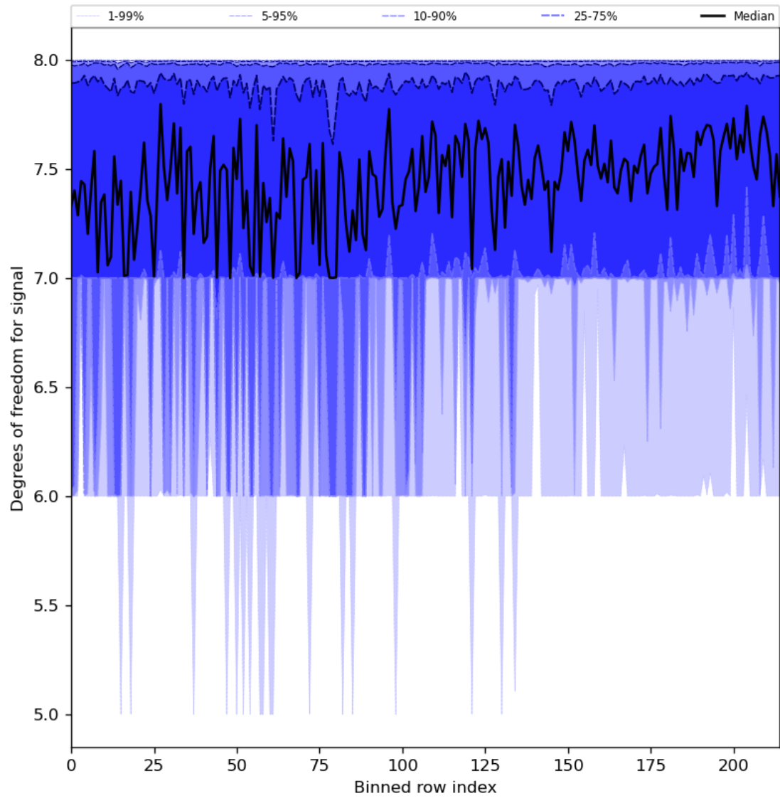
Figure 31: Along track statistics of “Degrees of freedom for signal” for 2023-10-24 to 2023-10-26
