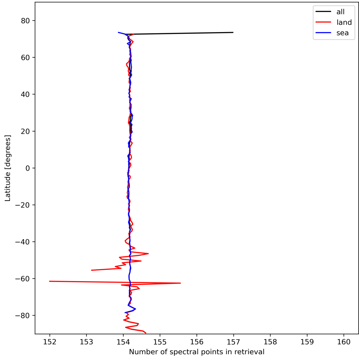
Figure 13: Zonal average of “Number of spectral points in retrieval” for 2023-10-24 to 2023-10-26.
