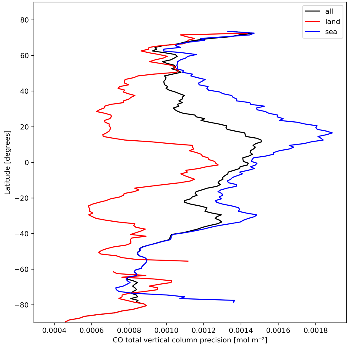
Figure 12: Zonal average of “CO total vertical column precision” for 2023-10-24 to 2023-10-26.
