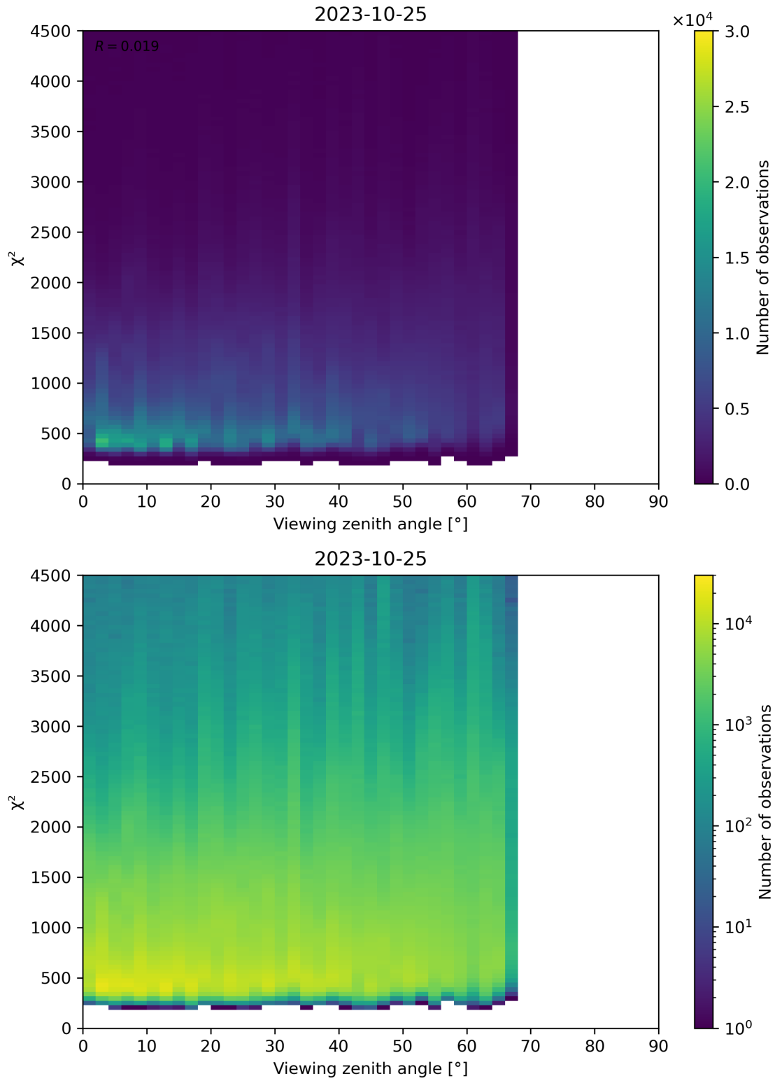
Figure 72: Scatter density plot of “Viewing zenith angle” against “ \chi^2 ” for 2023-10-24 to 2023-10-26.
