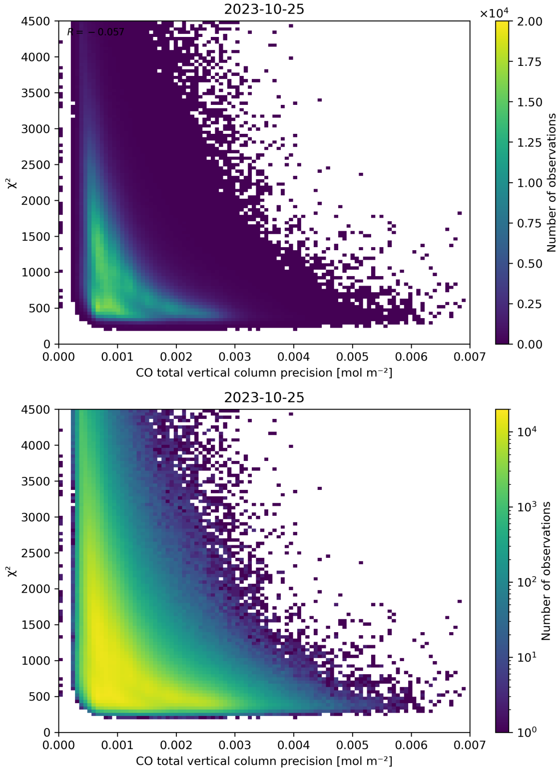
Figure 44: Scatter density plot of “CO total vertical column precision” against “ \chi^2 ” for 2023-10-24 to 2023-10-26.
