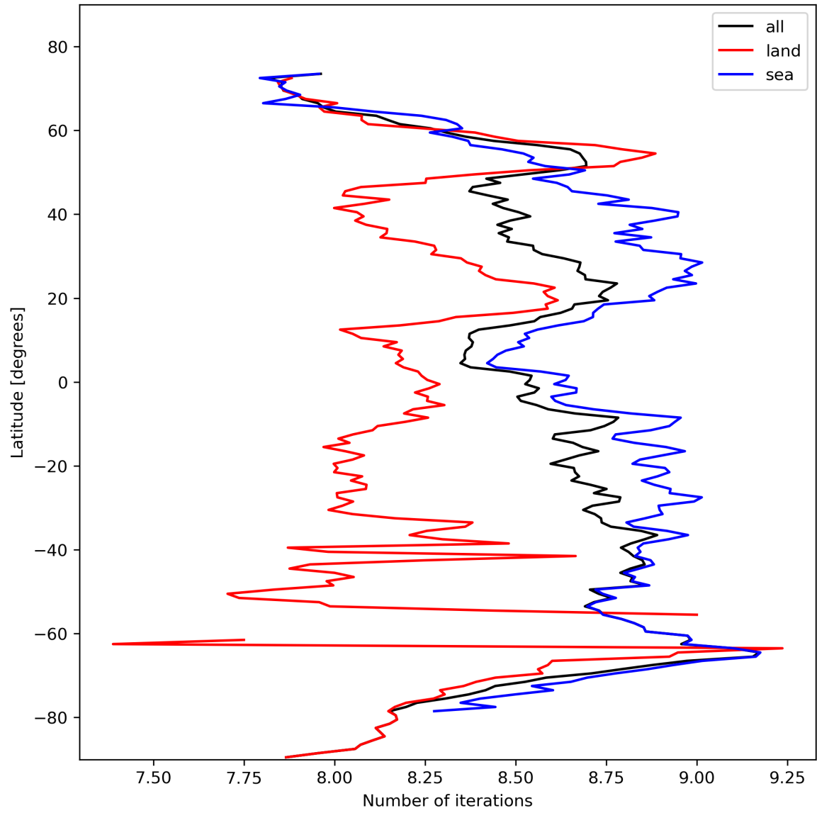
Figure 16: Zonal average of “Number of iterations” for 2023-10-24 to 2023-10-26.
