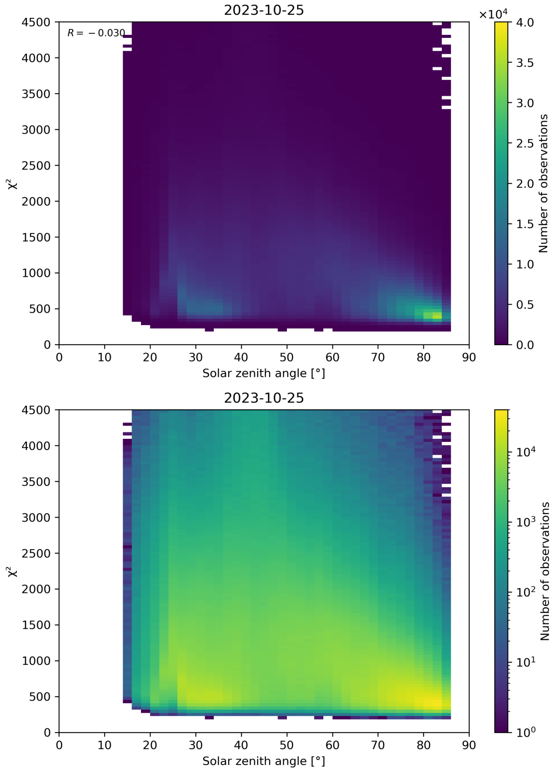
Figure 64: Scatter density plot of “Solar zenith angle” against “ \chi^2 ” for 2023-10-24 to 2023-10-26.
