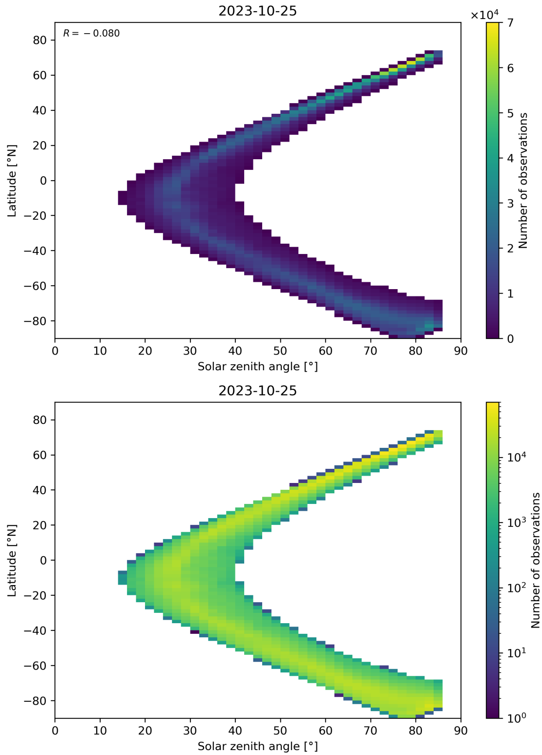
Figure 66: Scatter density plot of “Solar zenith angle” against “Latitude” for 2023-10-24 to 2023-10-26.
