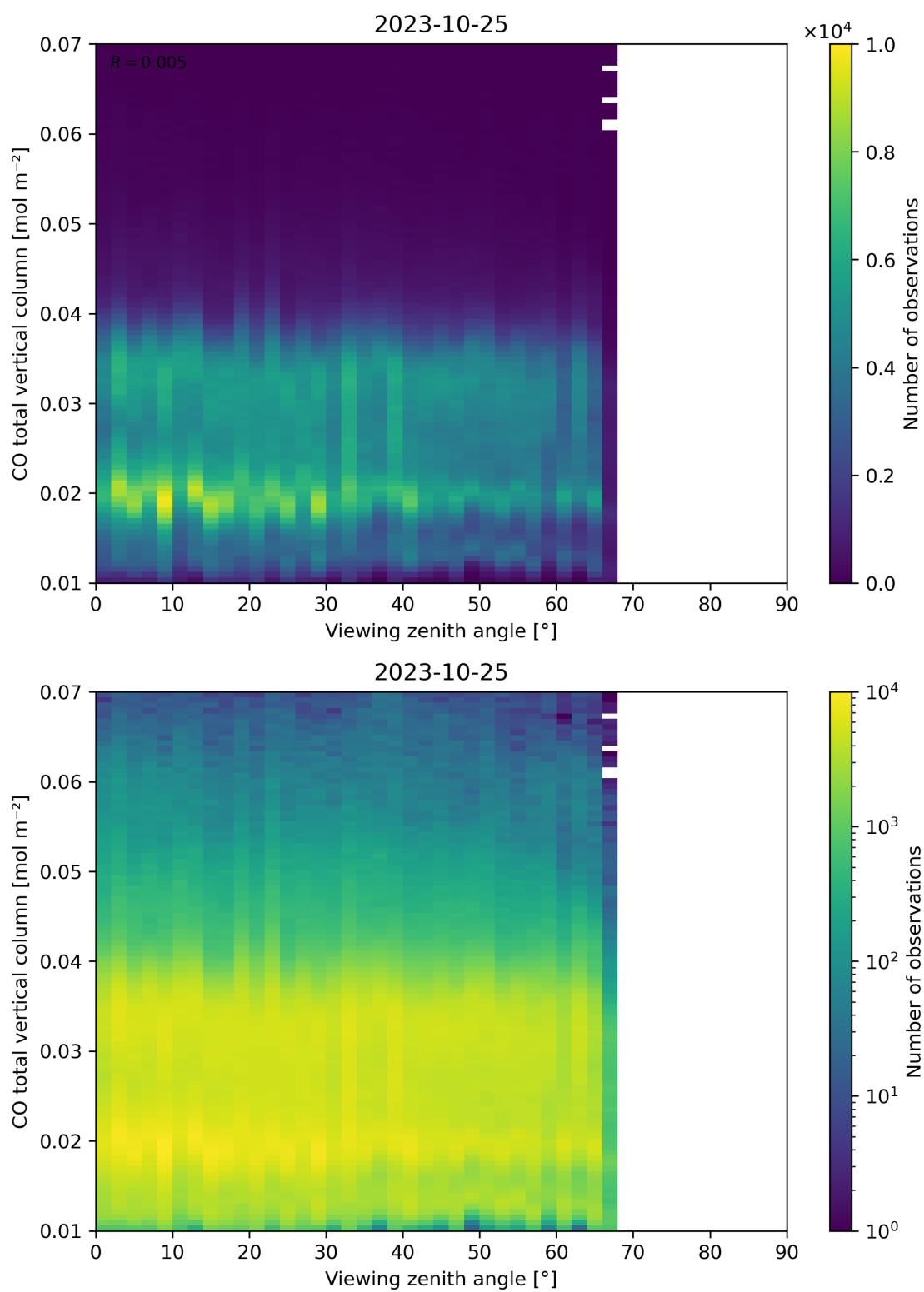
Figure 69: Scatter density plot of “Viewing zenith angle” against “CO total vertical column” for 2023-10-24 to 2023-10-26.
