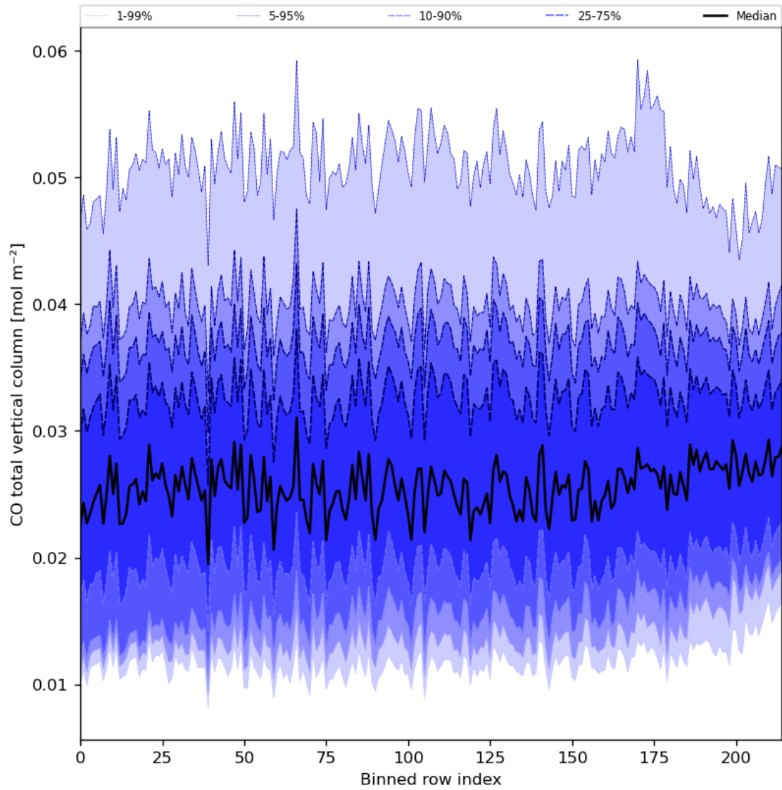
Figure 26: Along track statistics of “CO total vertical column” for 2023-10-24 to 2023-10-26
