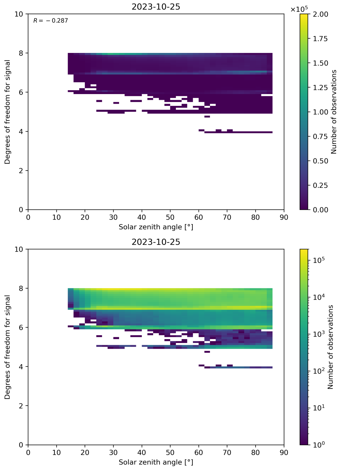
Figure 65: Scatter density plot of “Solar zenith angle” against “Degrees of freedom for signal” for 2023-10-24 to 2023-10-26.
