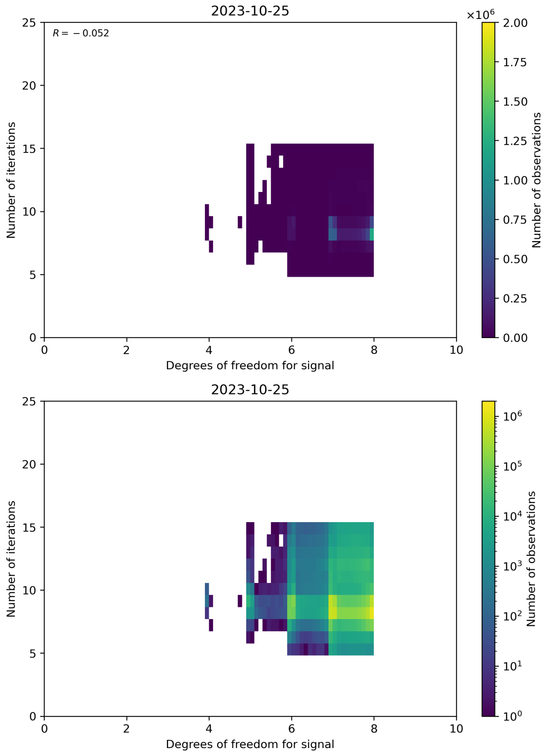
Figure 50: Scatter density plot of “Degrees of freedom for signal” against “Number of iterations” for 2023-10-24 to 2023-10-26.
