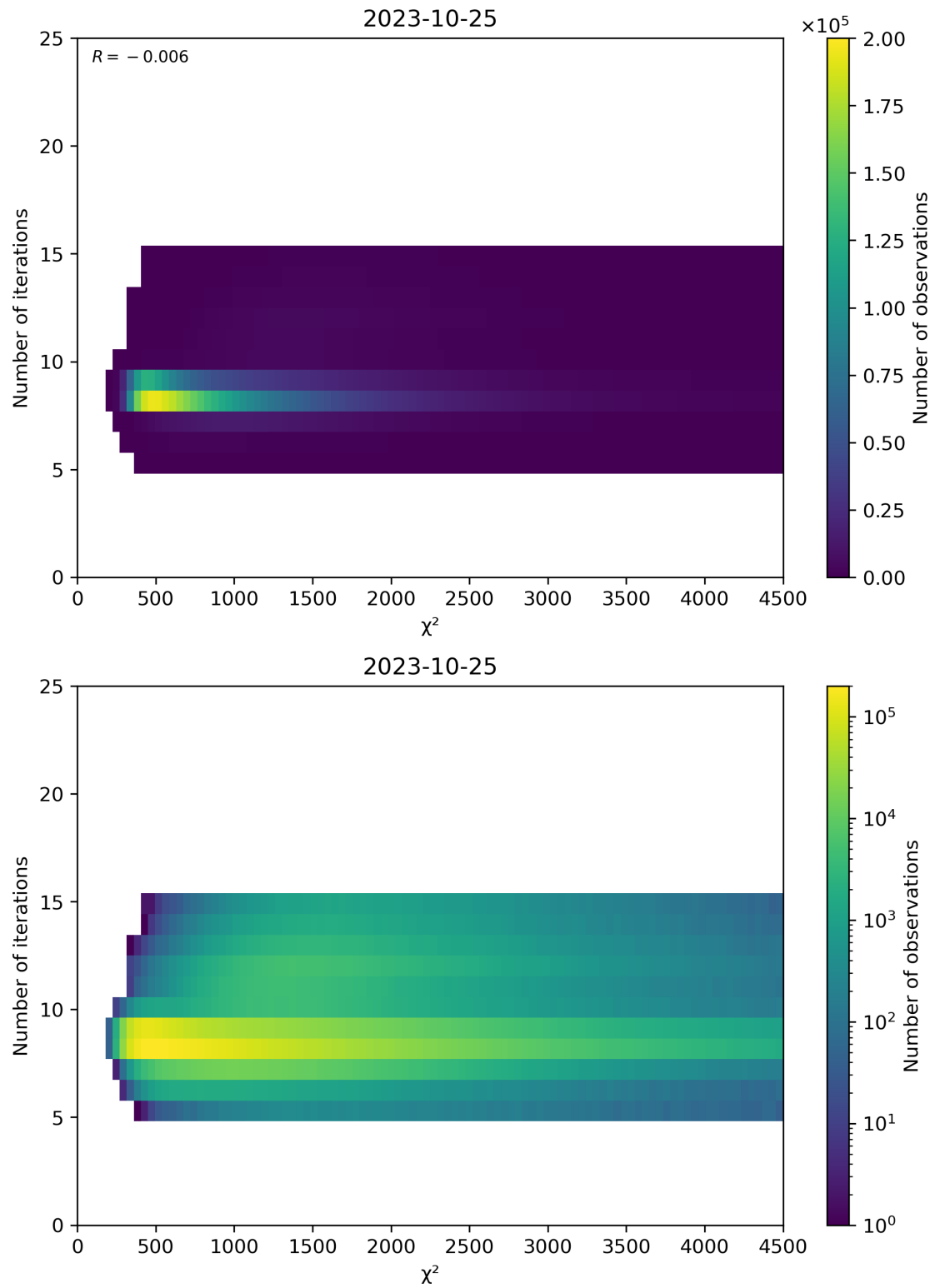
Figure 49: Scatter density plot of “ \chi^2 ” against “Number of iterations” for 2023-10-24 to 2023-10-26.
