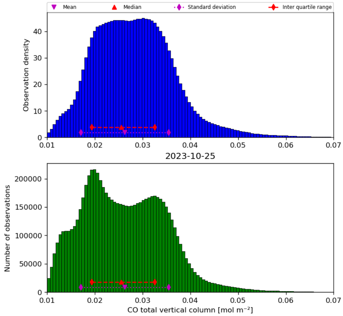
Figure 18: Histogram of “CO total vertical column” for 2023-10-24 to 2023-10-26
