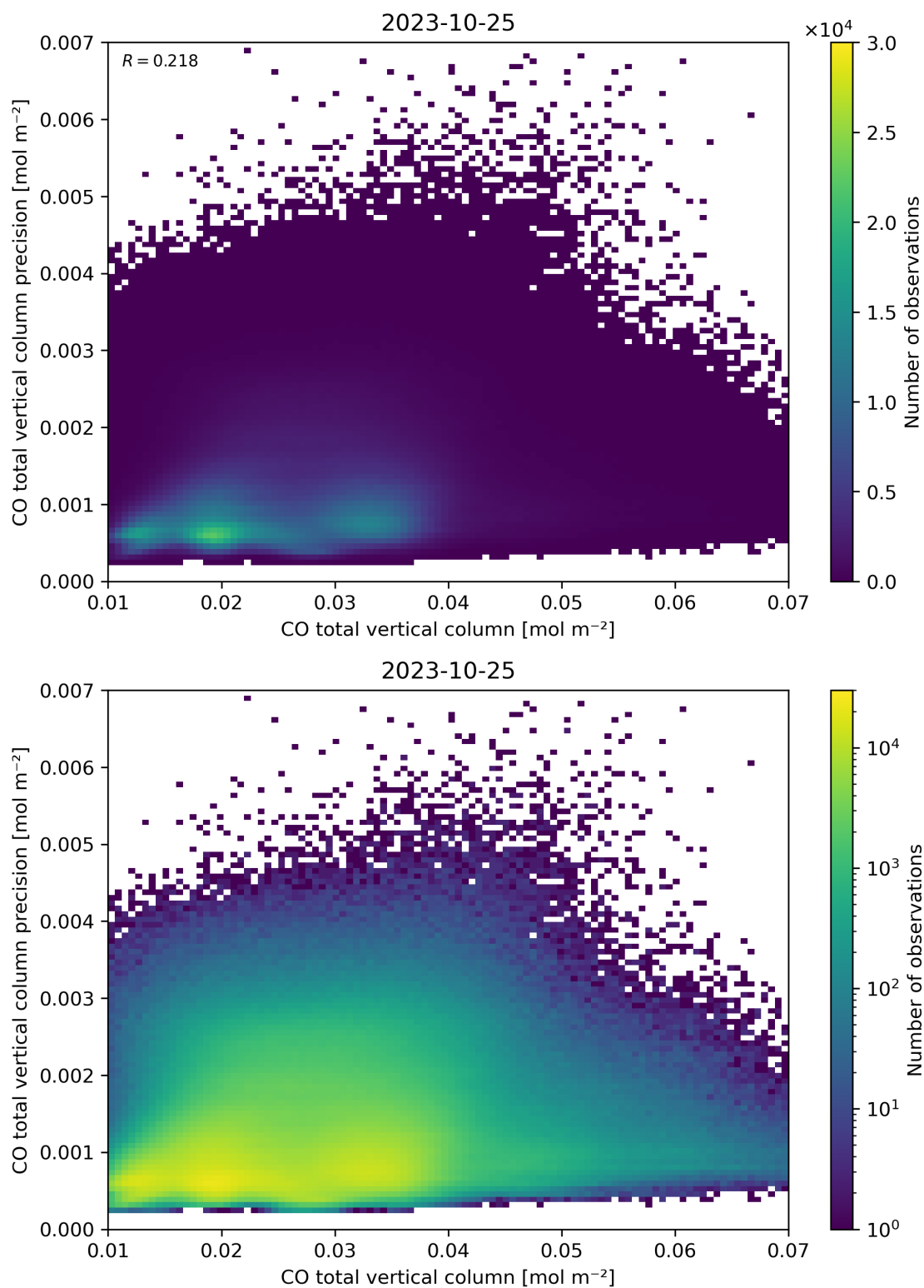
Figure 34: Scatter density plot of “CO total vertical column” against “CO total vertical column precision” for 2023-10-24 to 2023-10-26.
