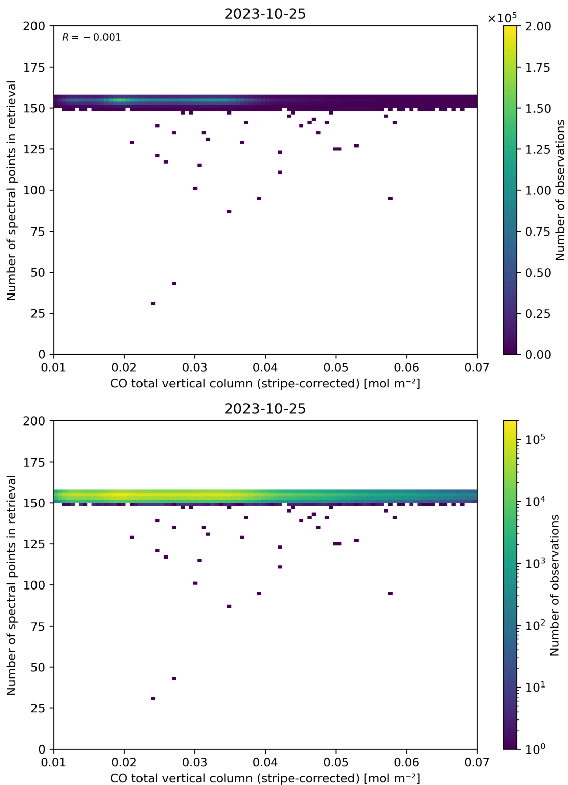
Figure 40: Scatter density plot of “CO total vertical column (stripe-corrected)” against “Number of spectral points in retrieval” for 2023-10-24 to 2023-10-26.
