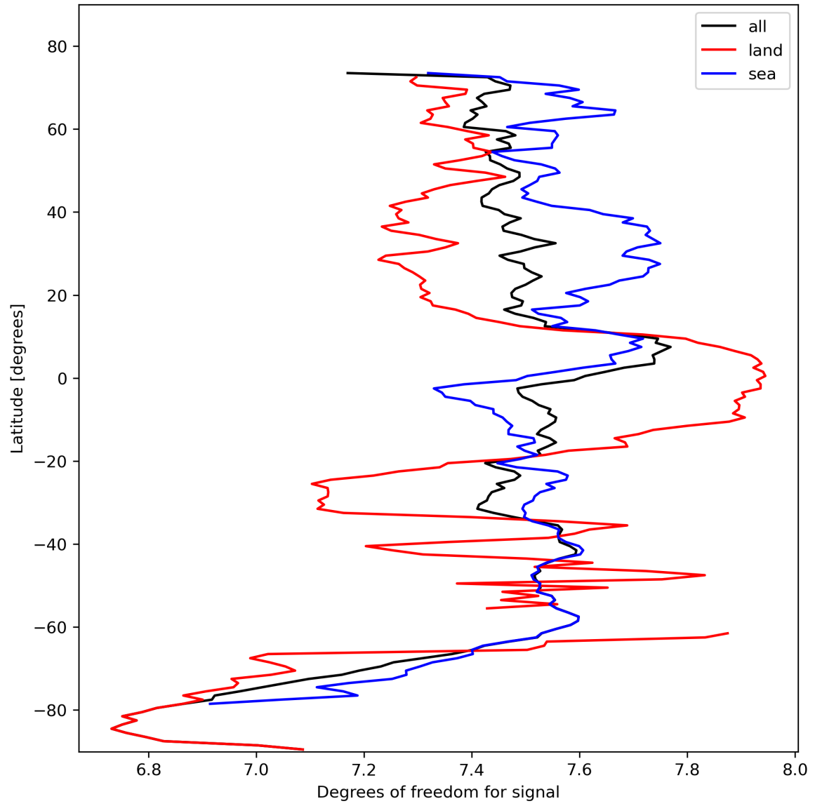
Figure 15: Zonal average of “Degrees of freedom for signal” for 2023-10-24 to 2023-10-26.
