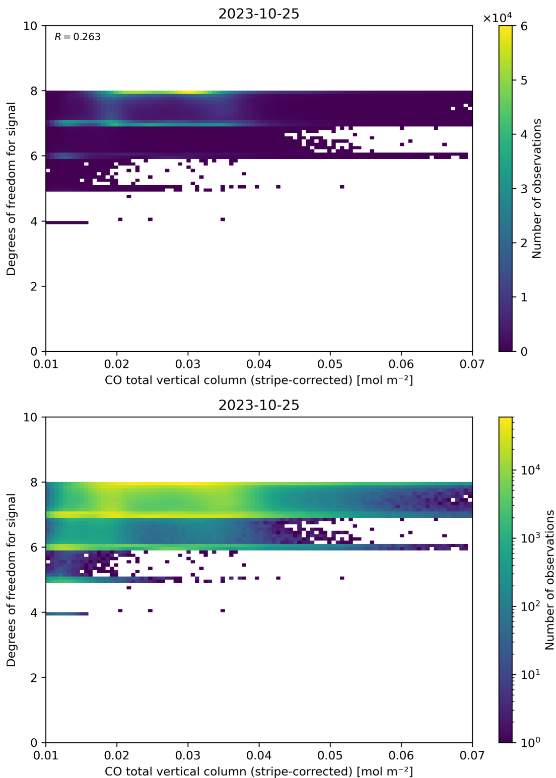
Figure 38: Scatter density plot of “CO total vertical column (stripe-corrected)” against “Degrees of freedom for signal” for 2023-10-24 to 2023-10-26.
