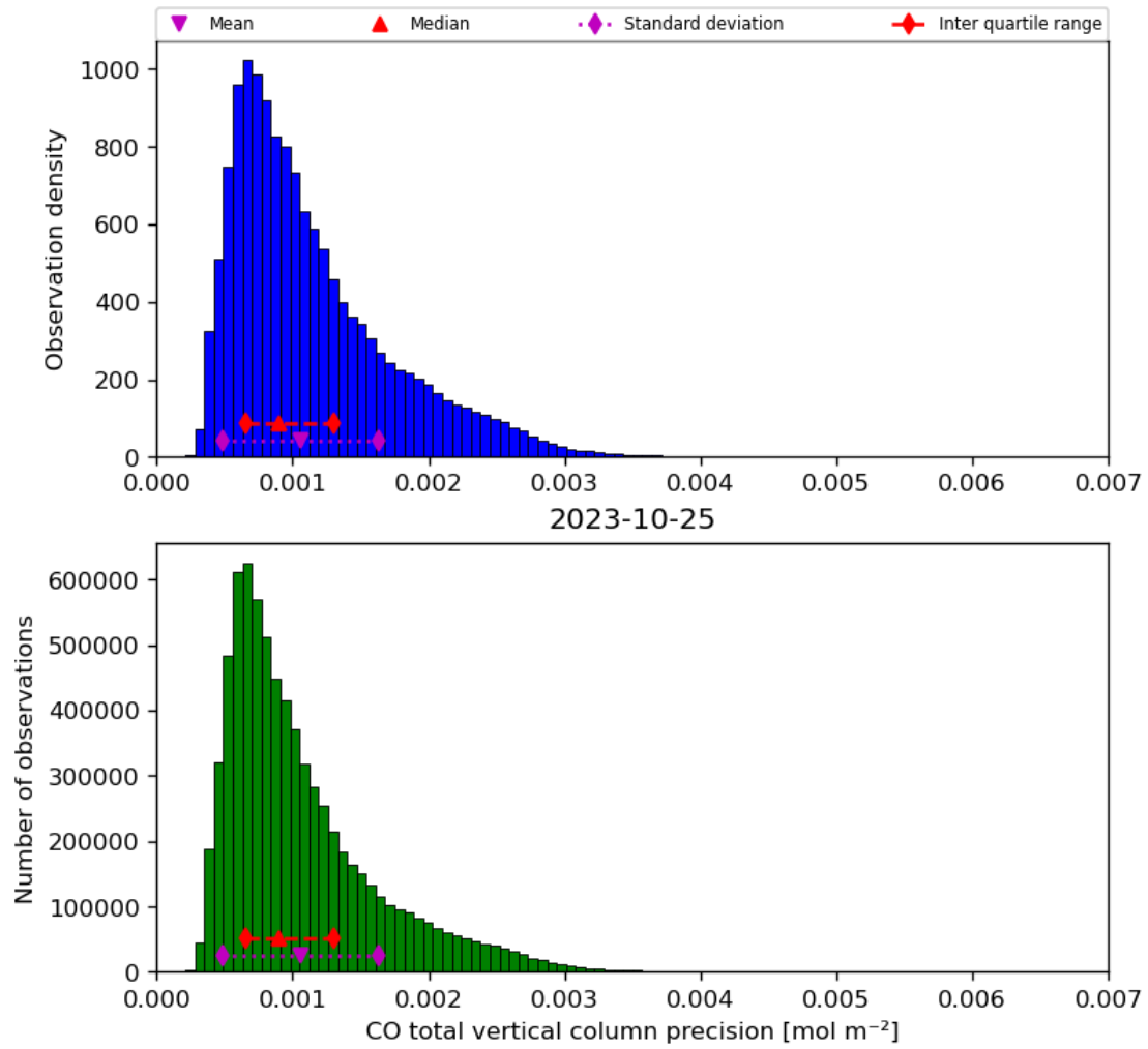
Figure 20: Histogram of “CO total vertical column precision” for 2023-10-24 to 2023-10-26
