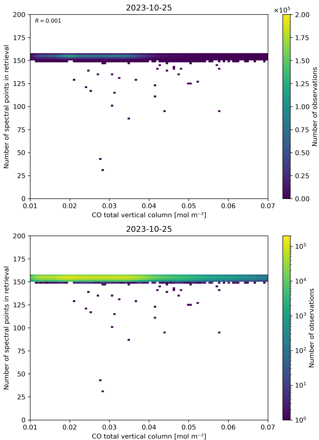
Figure 43: Scatter density plot of “CO total vertical column” against “Number of spectral points in retrieval” for 2023-10-24 to 2023-10-26.
