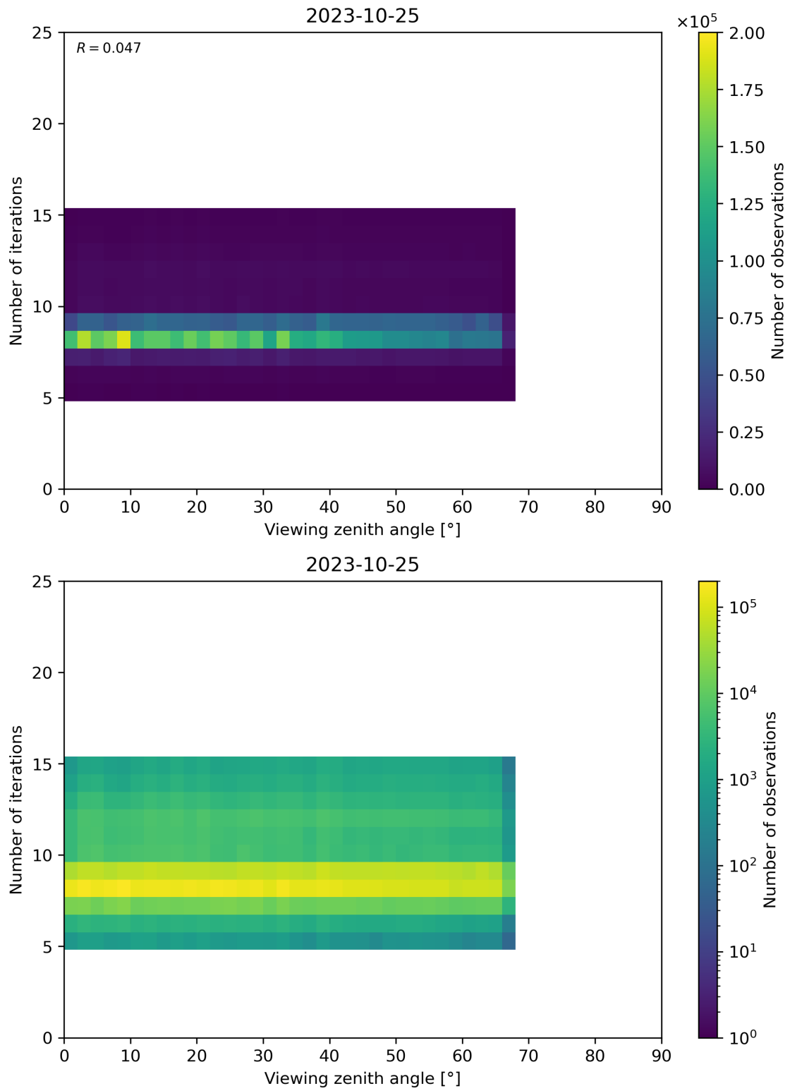
Figure 75: Scatter density plot of “Viewing zenith angle” against “Number of iterations” for 2023-10-24 to 2023-10-26.
