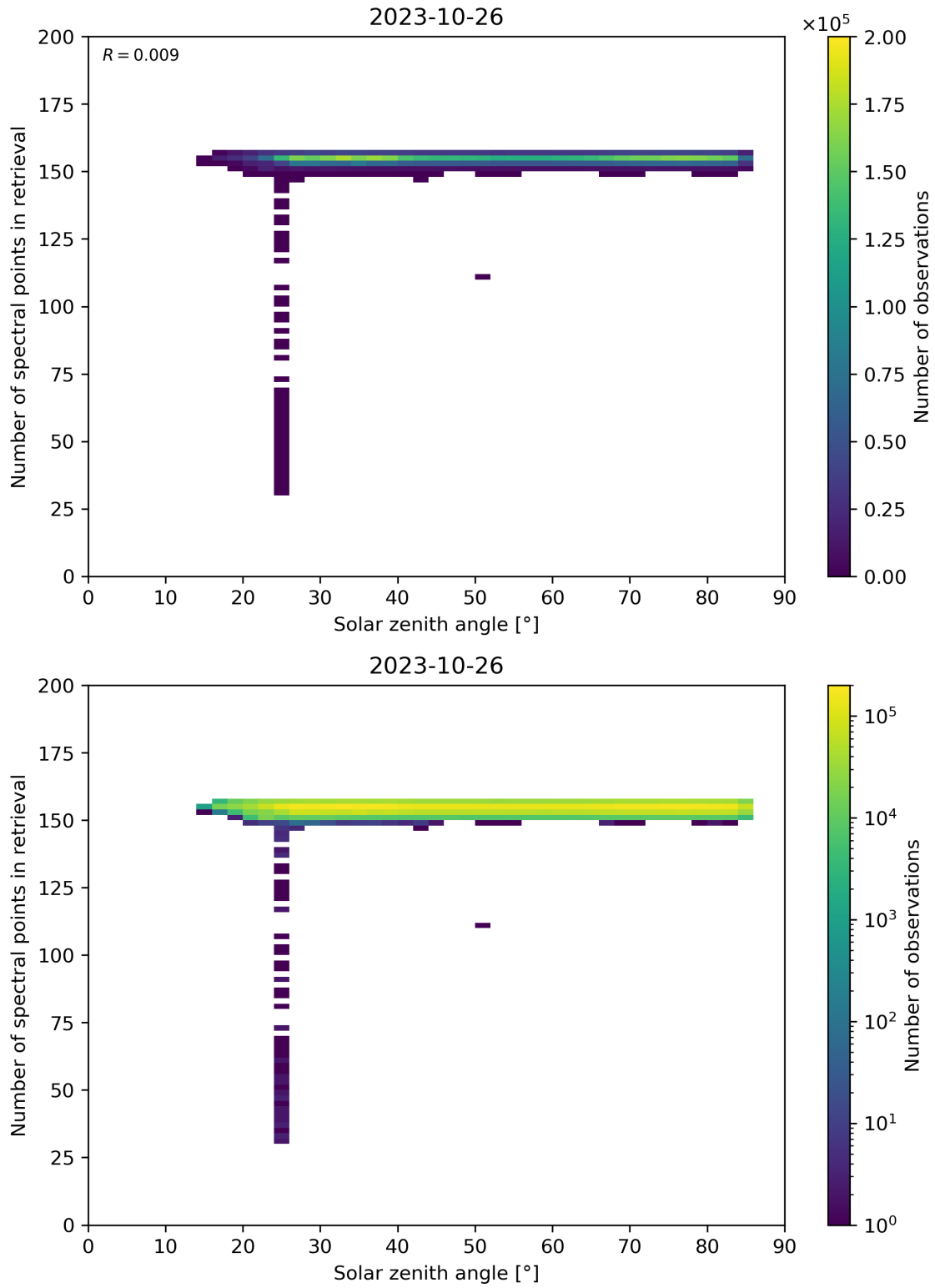
Figure 68: Scatter density plot of “Solar zenith angle” against “Number of spectral points in retrieval” for 2023-10-25 to 2023-10-27.
