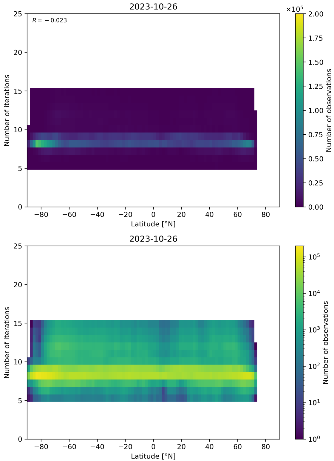
Figure 56: Scatter density plot of “Latitude” against “Number of iterations” for 2023-10-25 to 2023-10-27.
