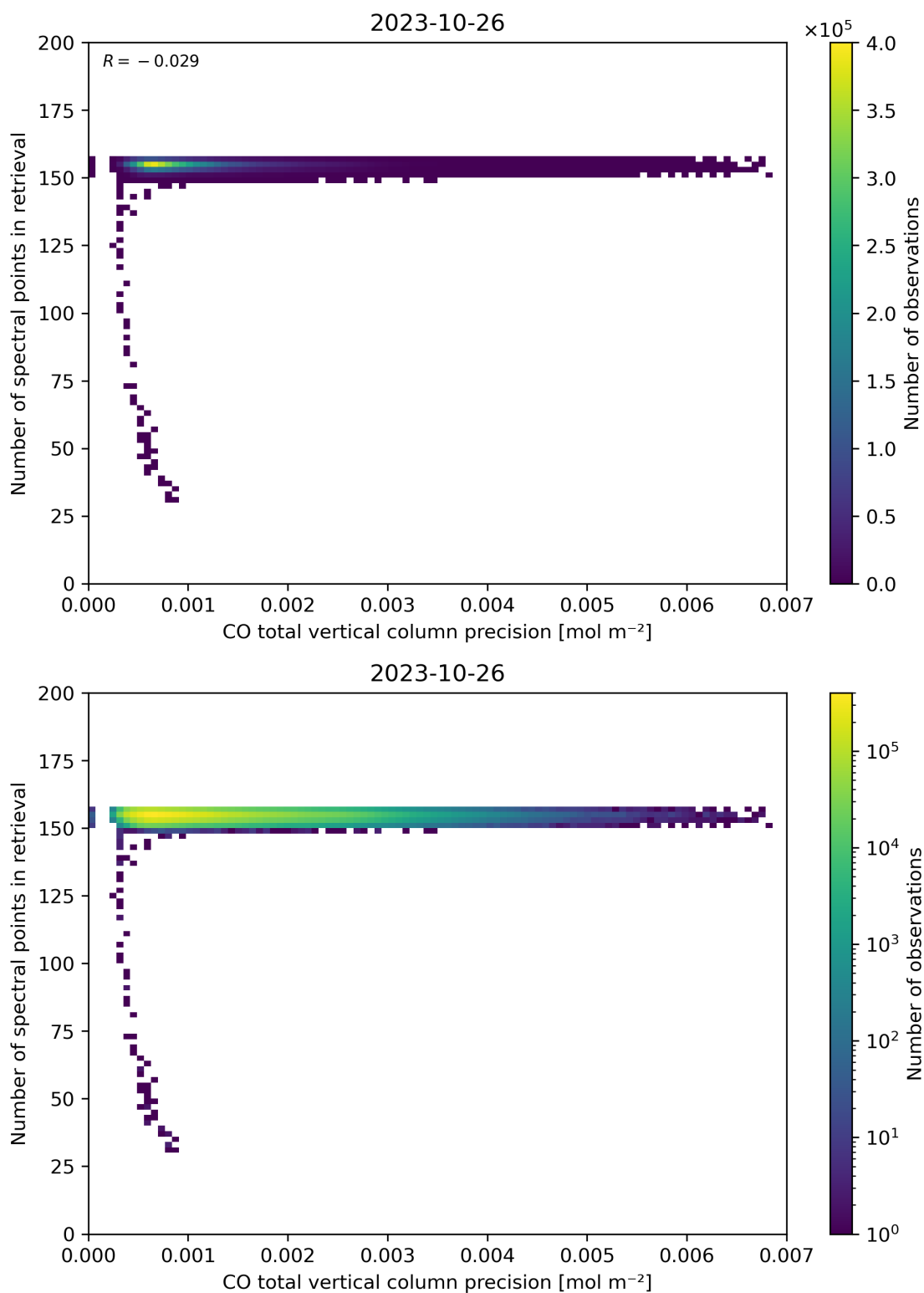
Figure 47: Scatter density plot of “CO total vertical column precision” against “Number of spectral points in retrieval” for 2023-10-25 to 2023-10-27.
