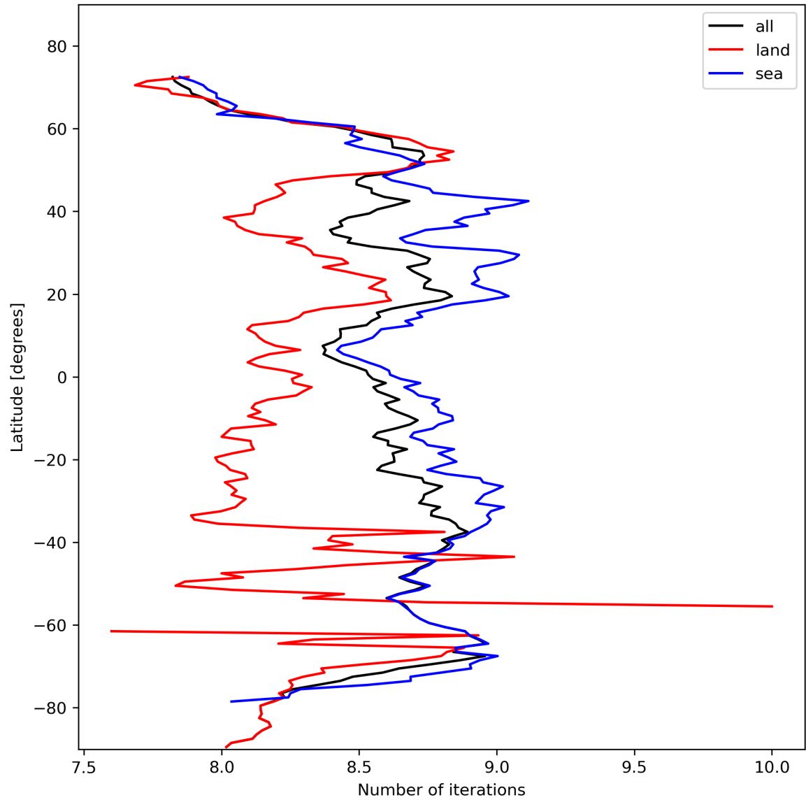
Figure 16: Zonal average of “Number of iterations” for 2023-10-25 to 2023-10-27.
