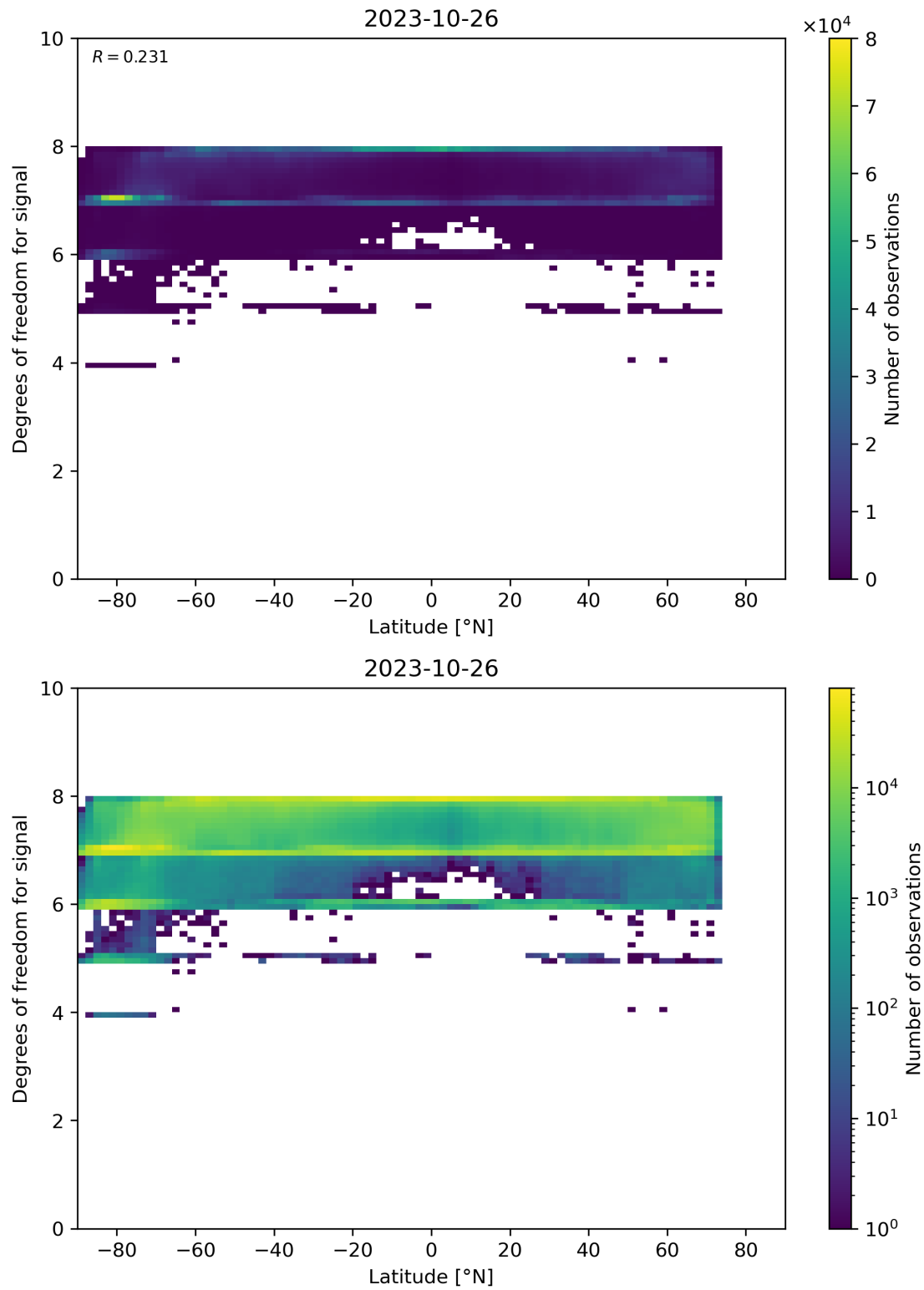
Figure 55: Scatter density plot of “Latitude” against “Degrees of freedom for signal” for 2023-10-25 to 2023-10-27.
