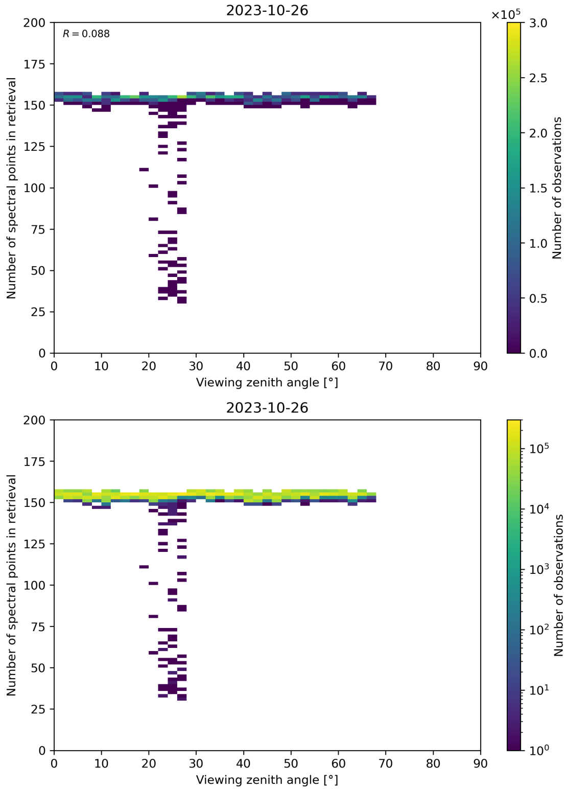
Figure 76: Scatter density plot of “Viewing zenith angle” against “Number of spectral points in retrieval” for 2023-10-25 to 2023-10-27.
