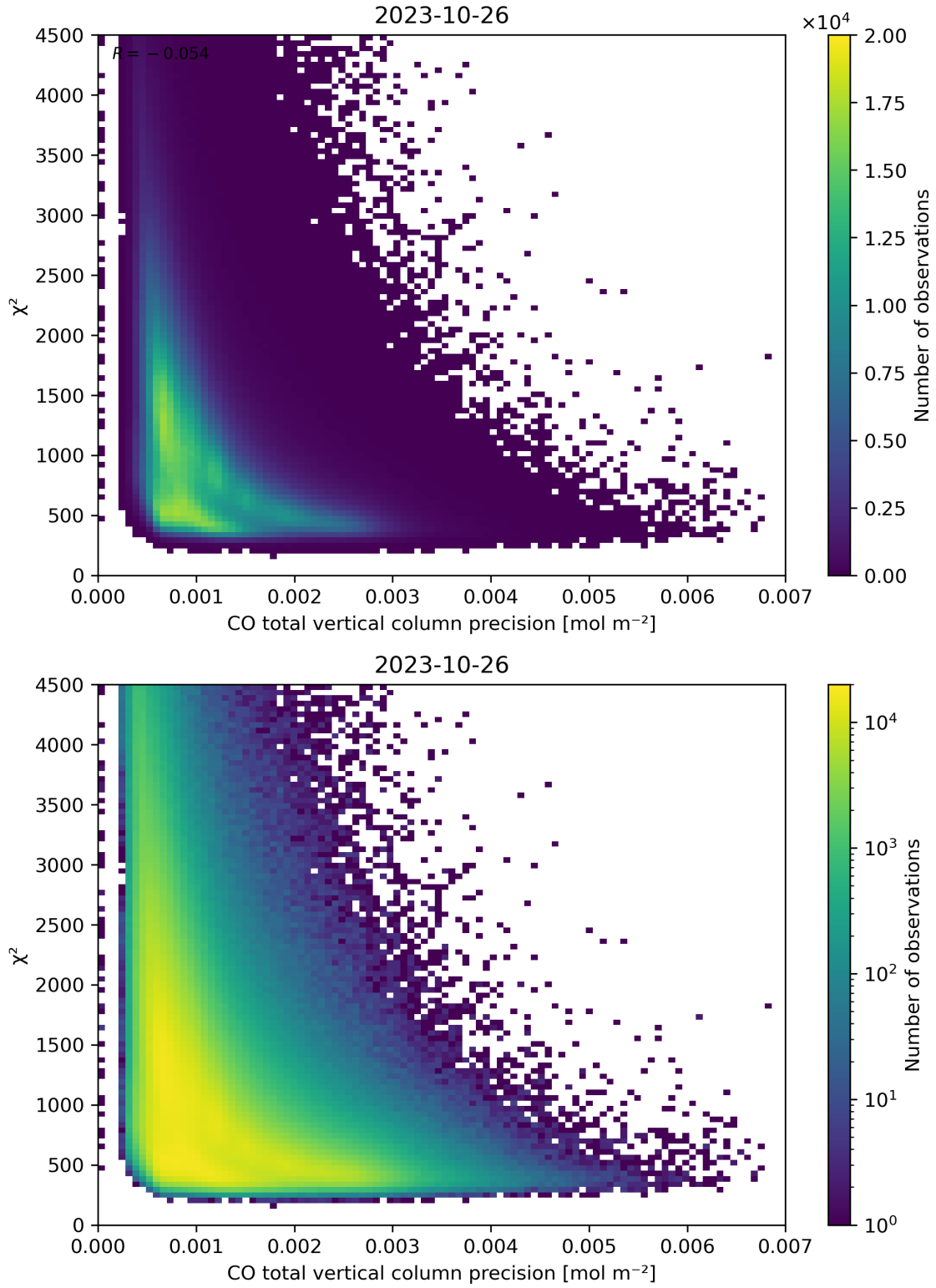
Figure 44: Scatter density plot of “CO total vertical column precision” against “ \chi^2 ” for 2023-10-25 to 2023-10-27.
