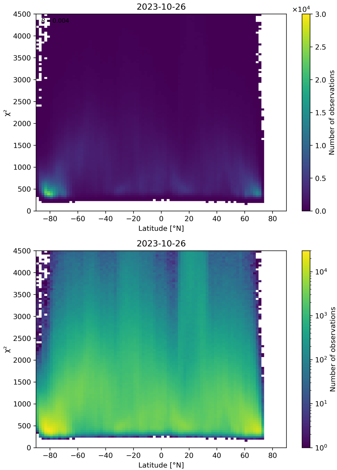
Figure 54: Scatter density plot of “Latitude” against “ \chi^2 ” for 2023-10-25 to 2023-10-27.
