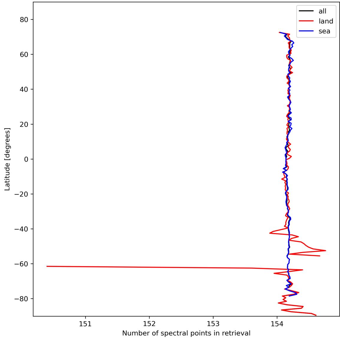
Figure 13: Zonal average of “Number of spectral points in retrieval” for 2023-10-25 to 2023-10-27.
