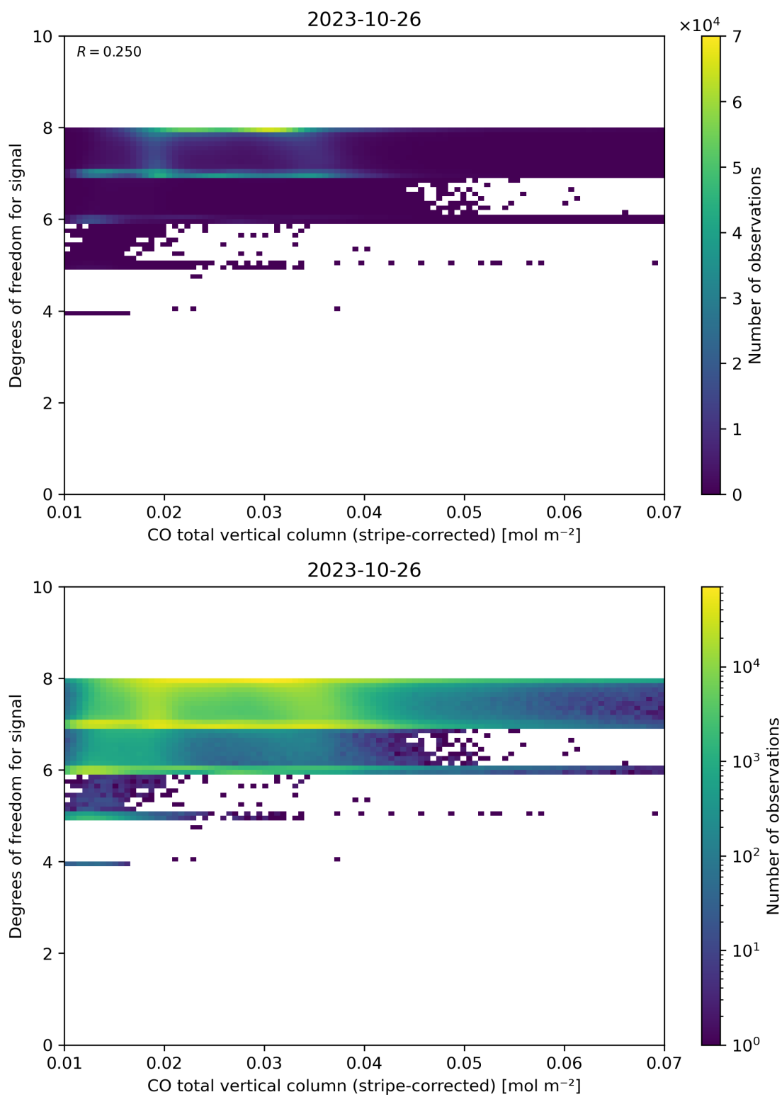
Figure 38: Scatter density plot of “CO total vertical column (stripe-corrected)” against “Degrees of freedom for signal” for 2023-10-25 to 2023-10-27.
