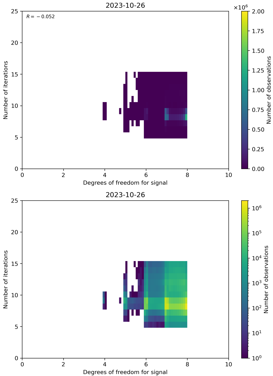
Figure 50: Scatter density plot of “Degrees of freedom for signal” against “Number of iterations” for 2023-10-25 to 2023-10-27.
