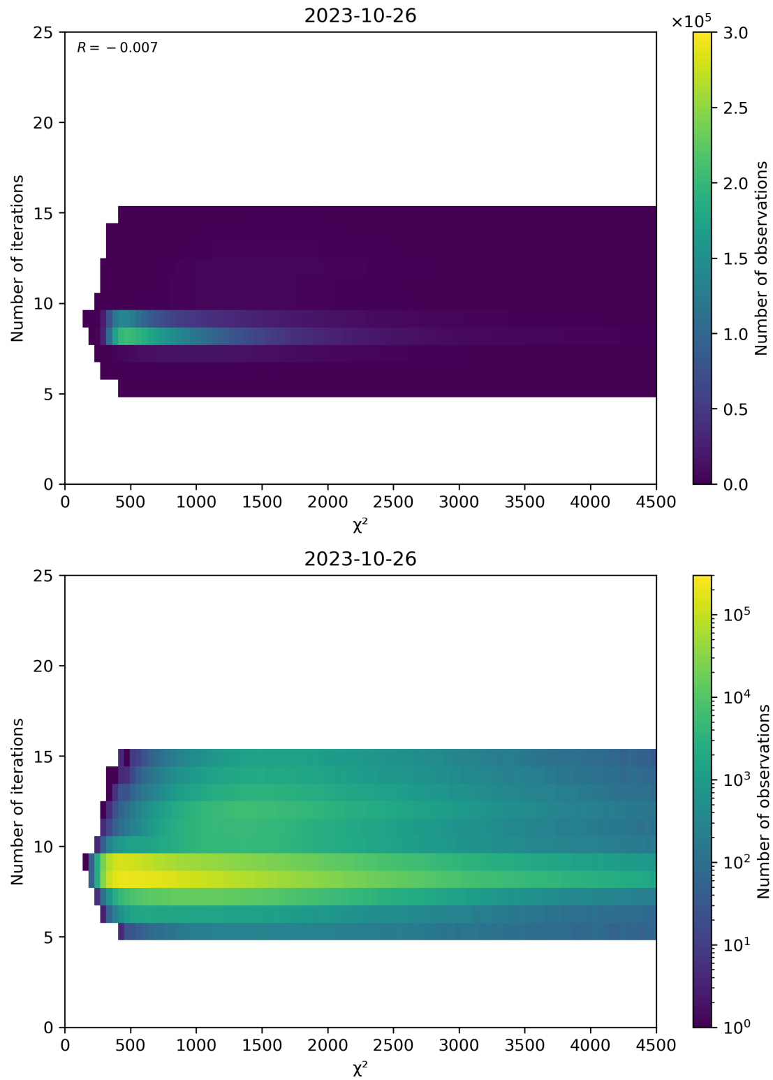
Figure 49: Scatter density plot of “ \chi^2 ” against “Number of iterations” for 2023-10-25 to 2023-10-27.
