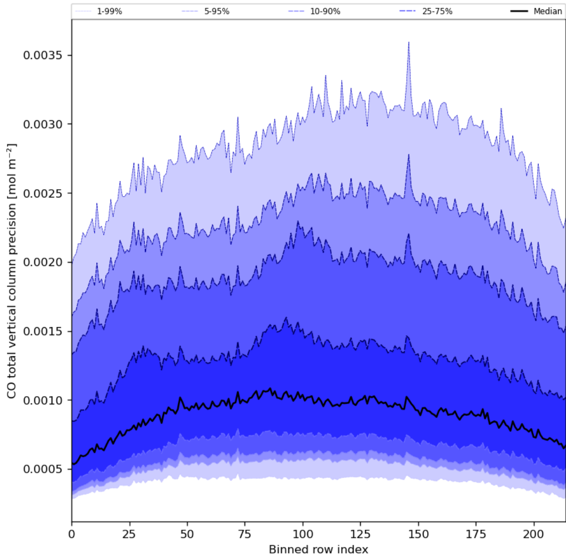
Figure 28: Along track statistics of “CO total vertical column precision” for 2023-10-25 to 2023-10-27
