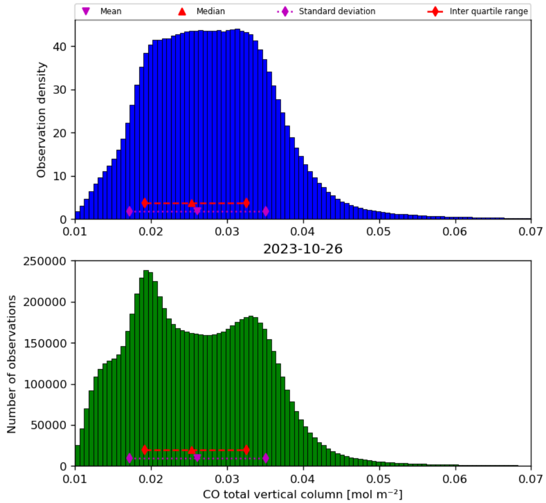
Figure 18: Histogram of “CO total vertical column” for 2023-10-25 to 2023-10-27
