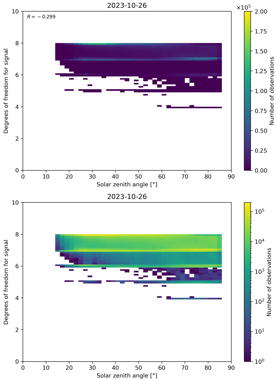
Figure 65: Scatter density plot of “Solar zenith angle” against “Degrees of freedom for signal” for 2023-10-25 to 2023-10-27.
