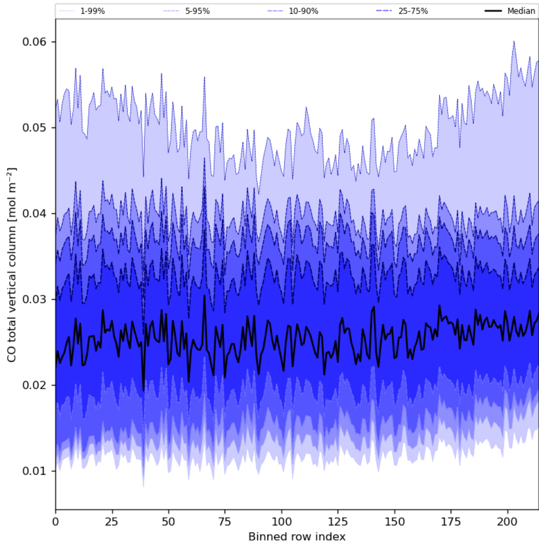
Figure 26: Along track statistics of “CO total vertical column” for 2023-10-25 to 2023-10-27
