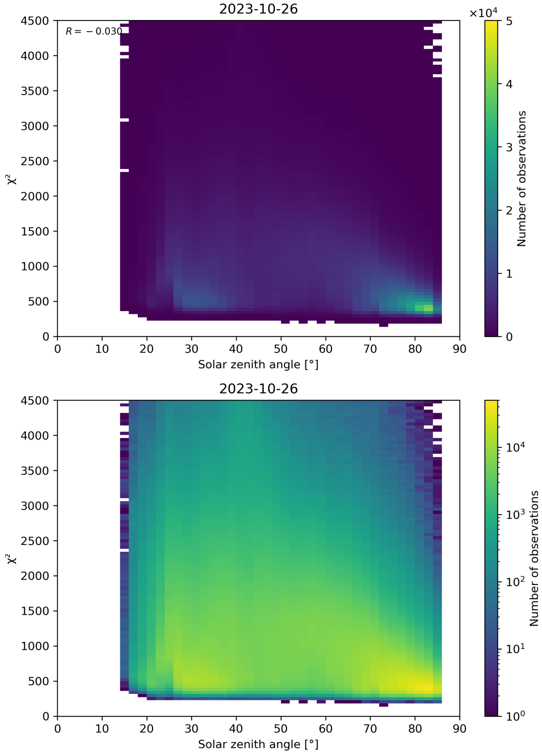
Figure 64: Scatter density plot of “Solar zenith angle” against “ \chi^2 ” for 2023-10-25 to 2023-10-27.
