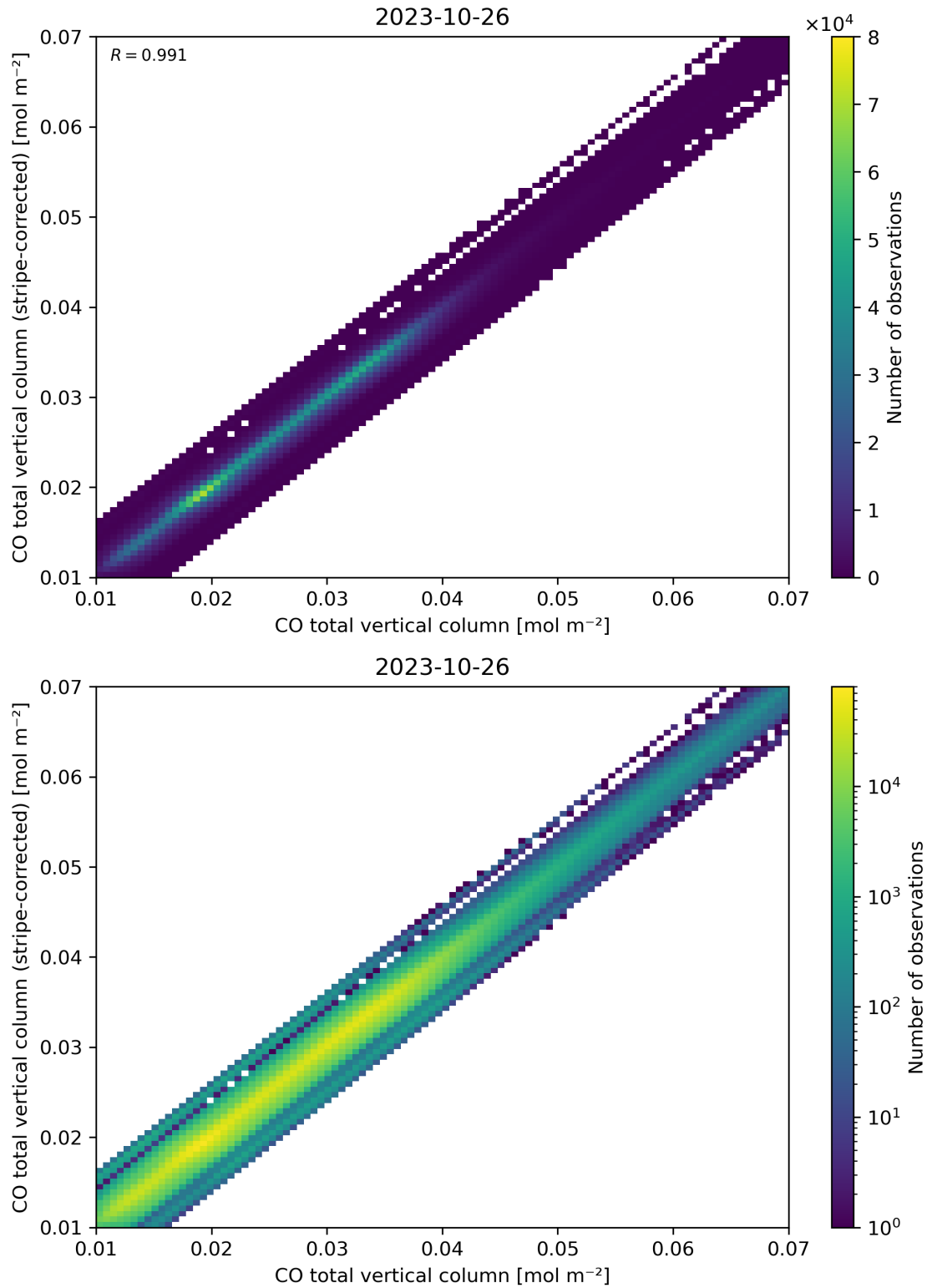
Figure 33: Scatter density plot of “CO total vertical column” against “CO total vertical column (stripe-corrected)” for 2023-10-25 to 2023-10-27.
