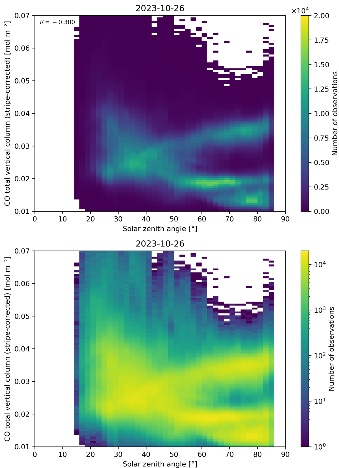
Figure 62: Scatter density plot of “Solar zenith angle” against “CO total vertical column (stripe-corrected)” for 2023-10-25 to 2023-10-27.
