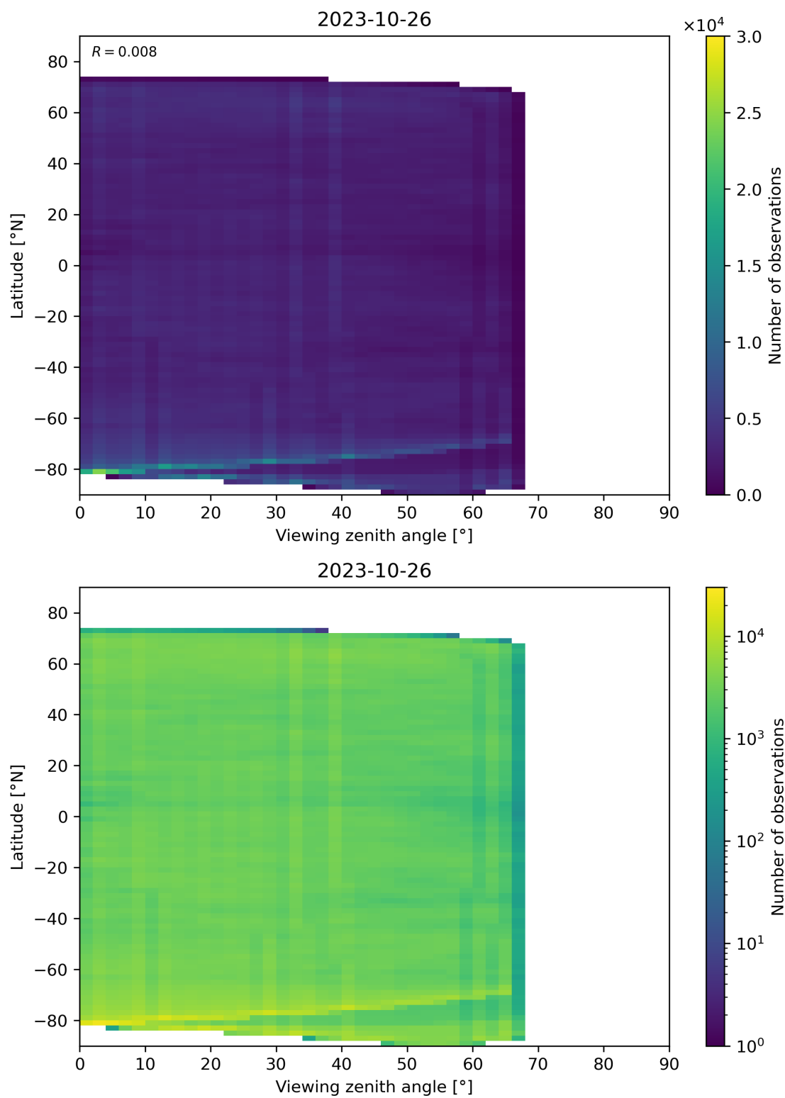
Figure 74: Scatter density plot of “Viewing zenith angle” against “Latitude” for 2023-10-25 to 2023-10-27.
