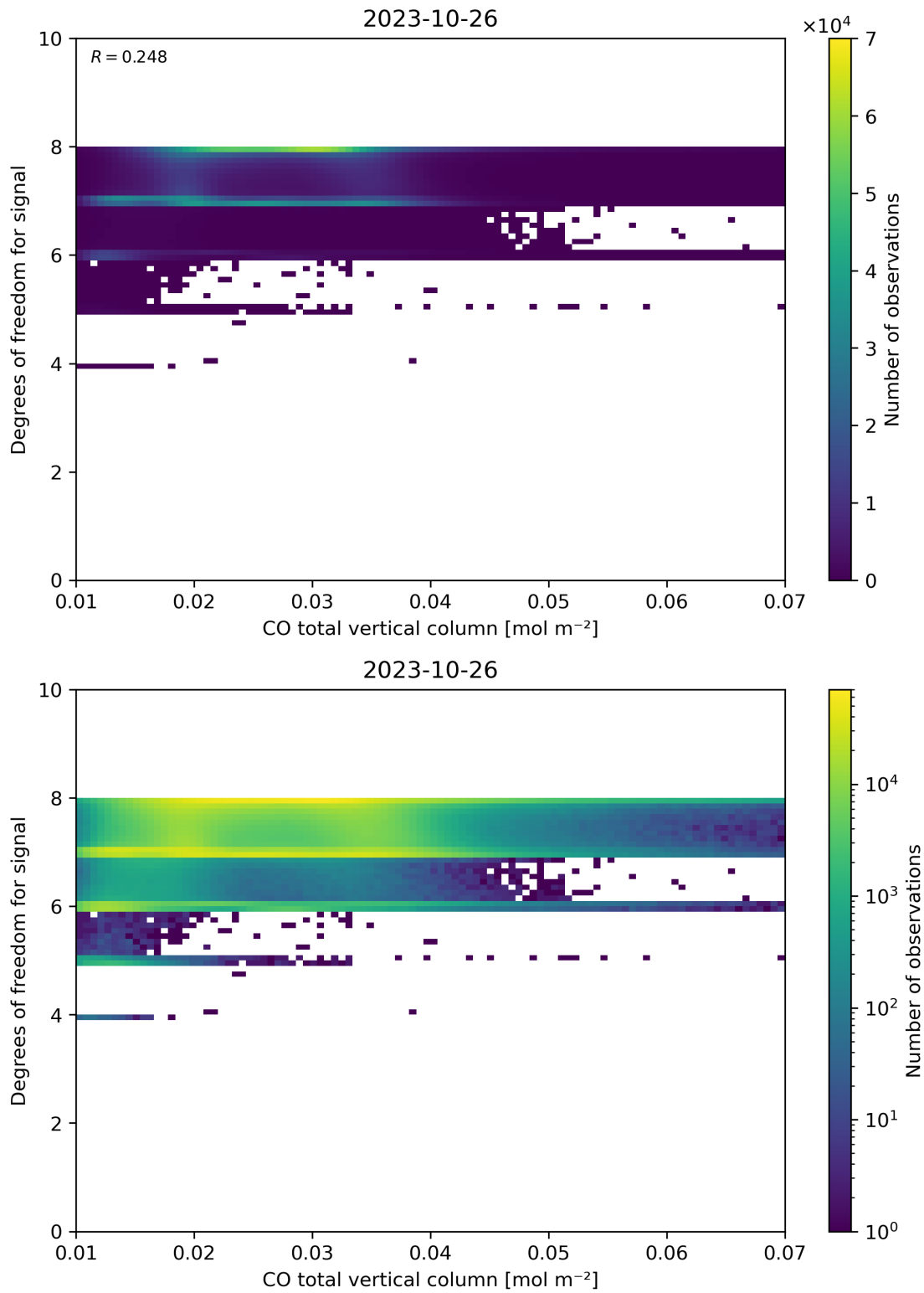
Figure 41: Scatter density plot of “CO total vertical column” against “Degrees of freedom for signal” for 2023-10-25 to 2023-10-27.
