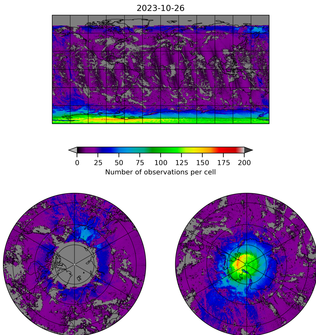
Figure 8: Map of the number of observations for 2023-10-25 to 2023-10-27
