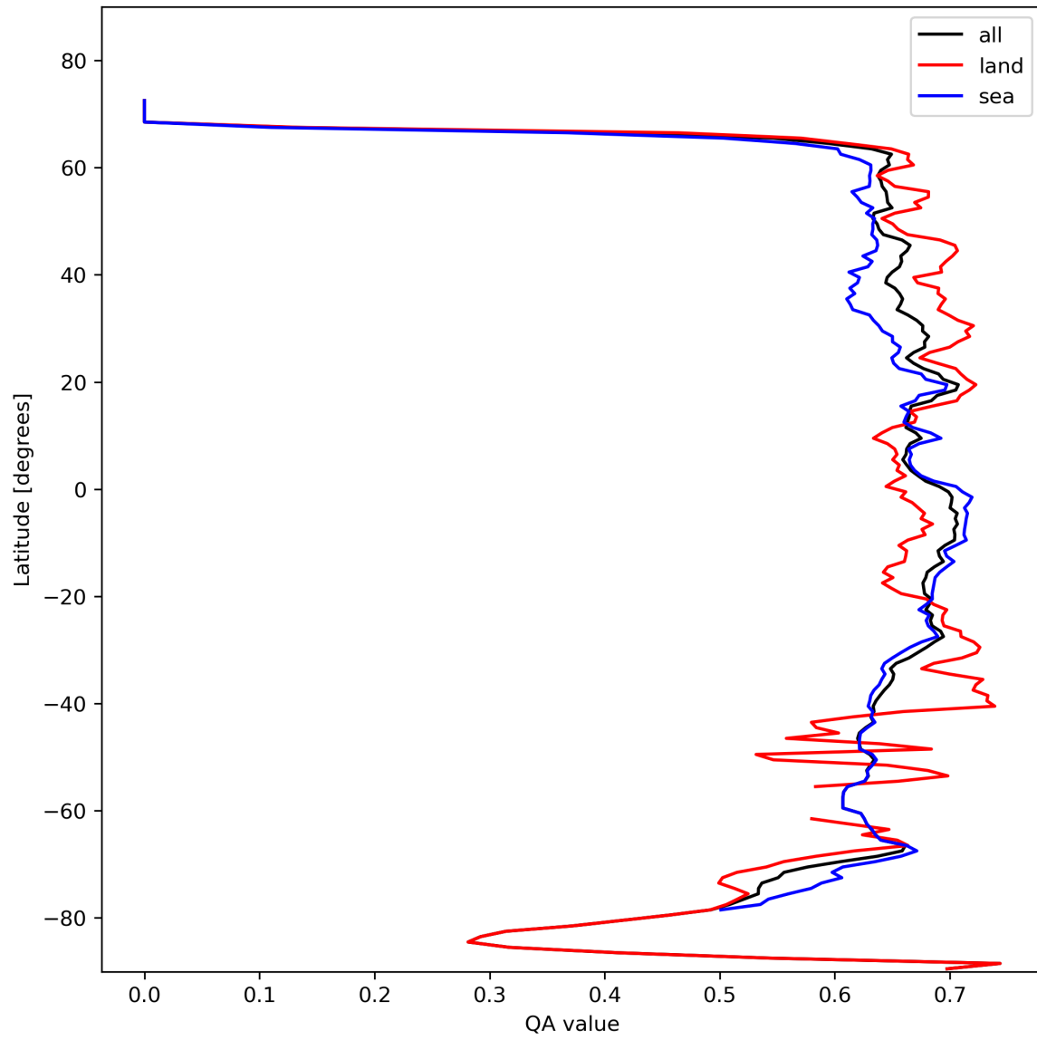
Figure 9: Zonal average of “QA value” for 2023-10-25 to 2023-10-27.
