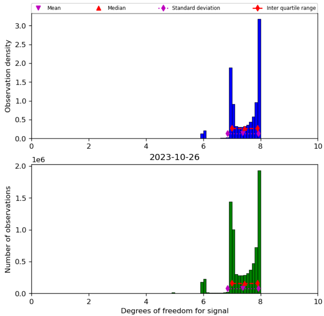
Figure 23: Histogram of “Degrees of freedom for signal” for 2023-10-25 to 2023-10-27
