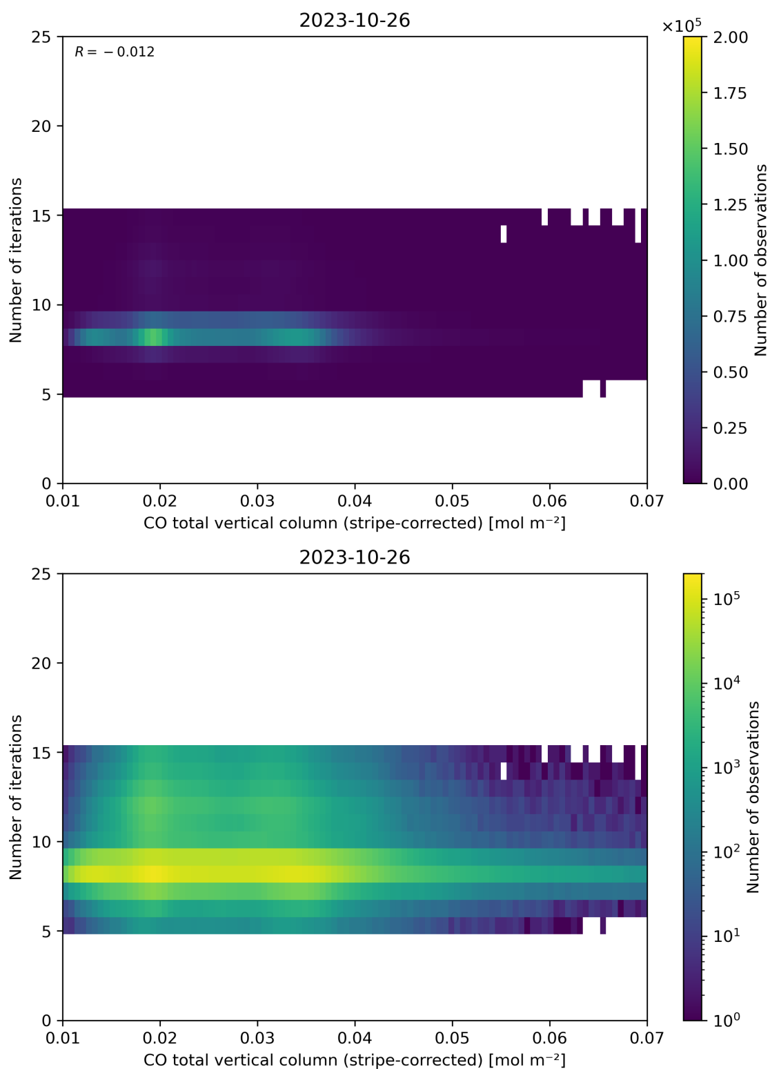
Figure 39: Scatter density plot of “CO total vertical column (stripe-corrected)” against “Number of iterations” for 2023-10-25 to 2023-10-27.
