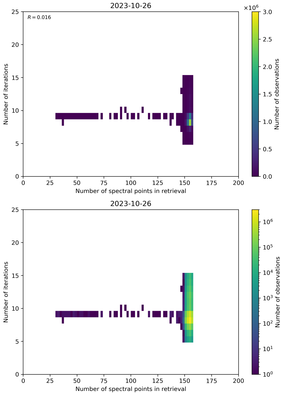
Figure 60: Scatter density plot of “Number of spectral points in retrieval” against “Number of iterations” for 2023-10-25 to 2023-10-27.
