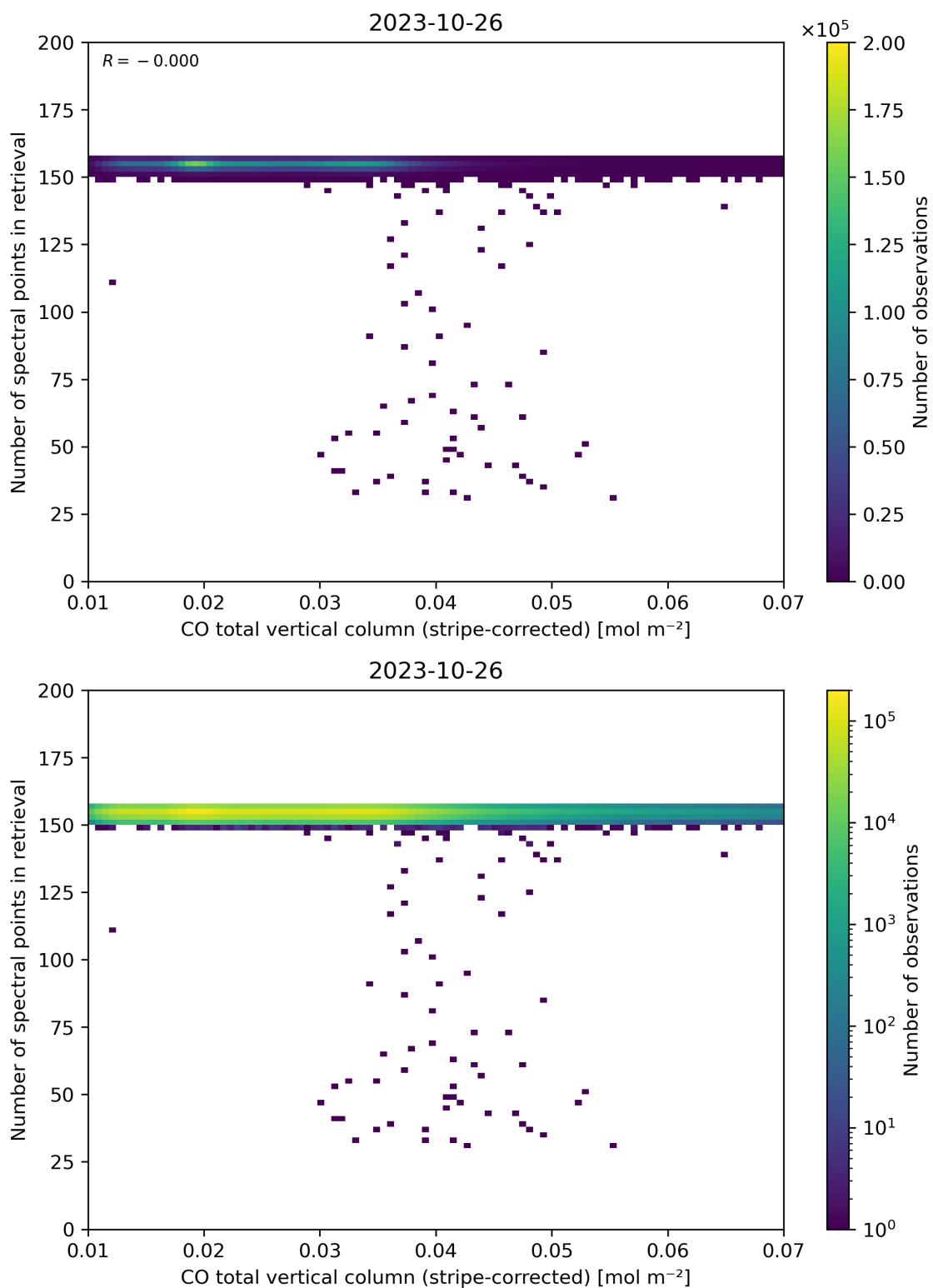
Figure 40: Scatter density plot of “CO total vertical column (stripe-corrected)” against “Number of spectral points in retrieval” for 2023-10-25 to 2023-10-27.
