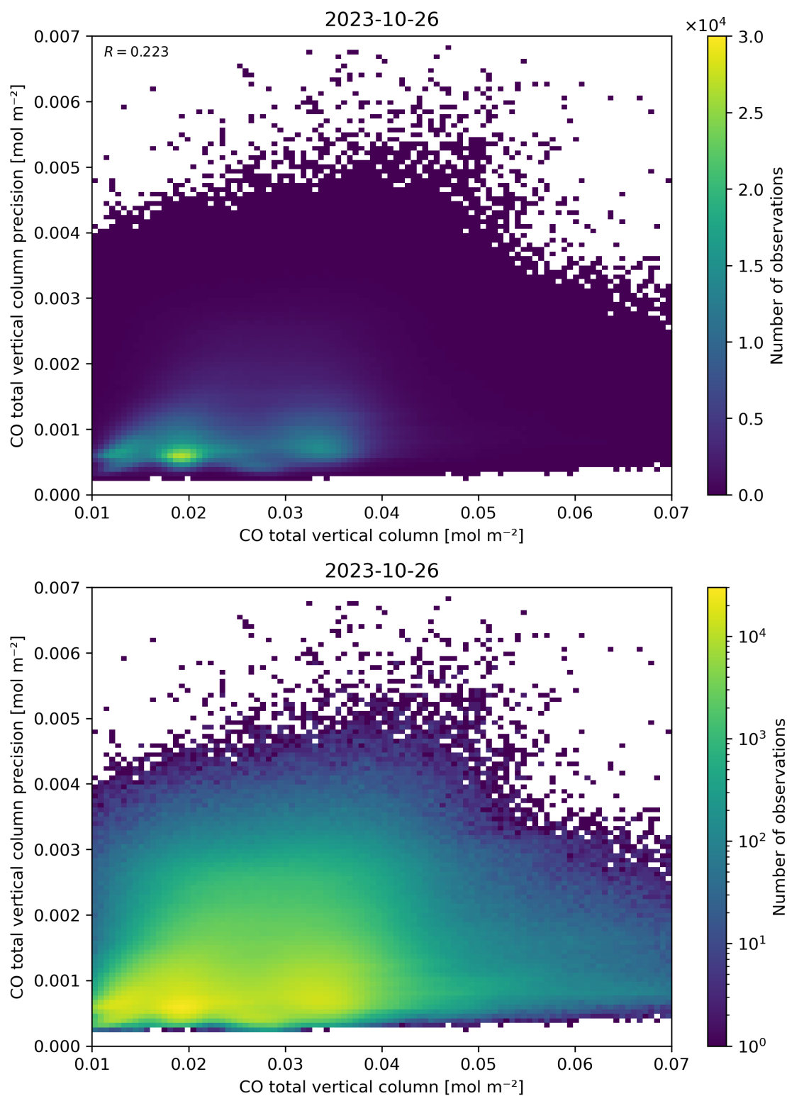
Figure 34: Scatter density plot of “CO total vertical column” against “CO total vertical column precision” for 2023-10-25 to 2023-10-27.
