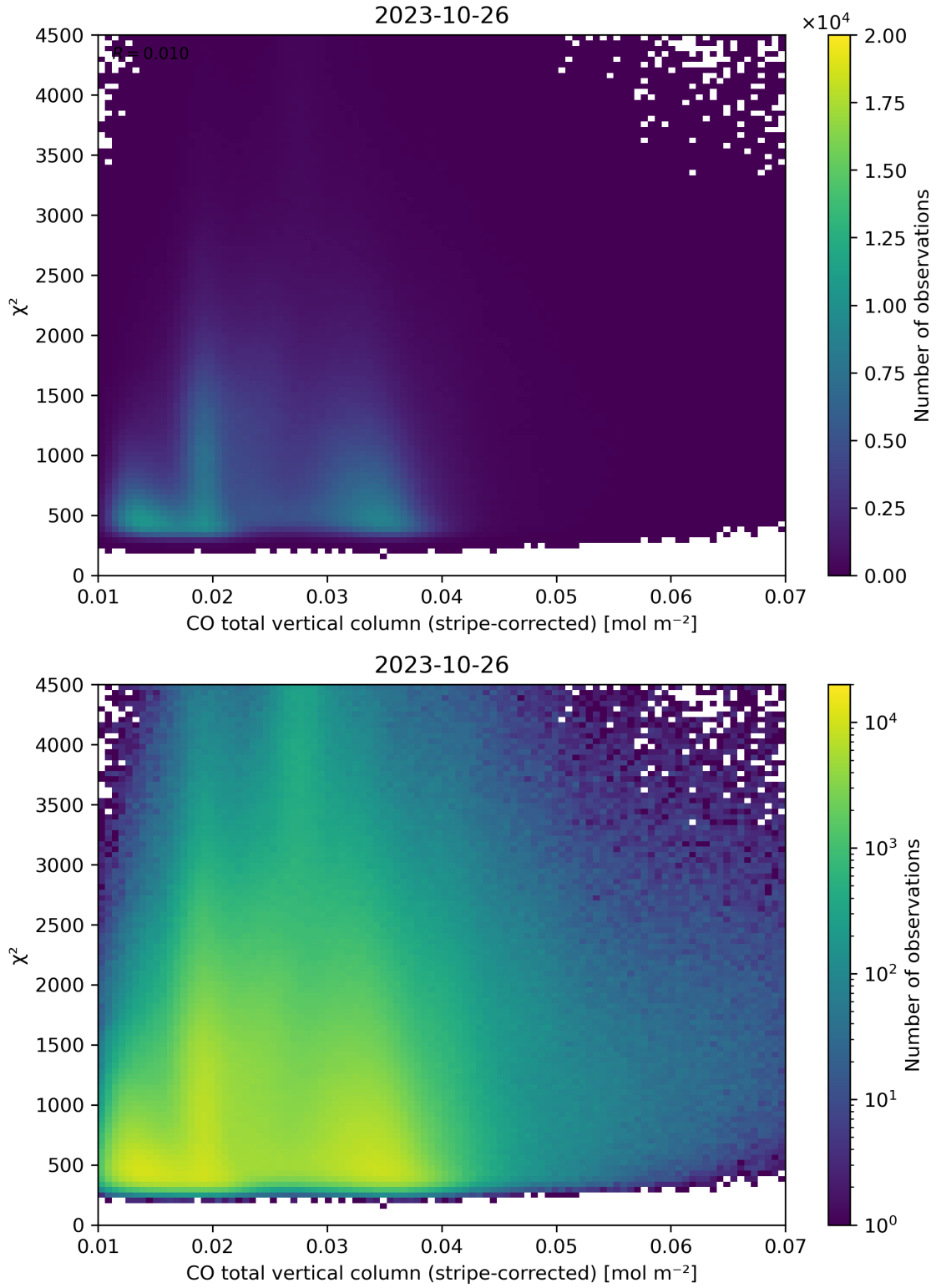
Figure 37: Scatter density plot of “CO total vertical column (stripe-corrected)” against “ \chi^2 ” for 2023-10-25 to 2023-10-27.
