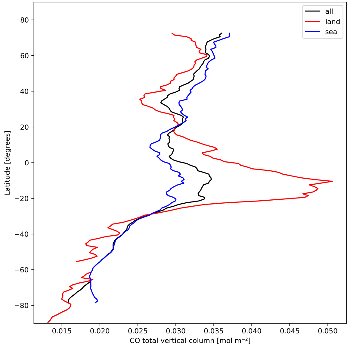
Figure 10: Zonal average of “CO total vertical column” for 2023-10-25 to 2023-10-27.
