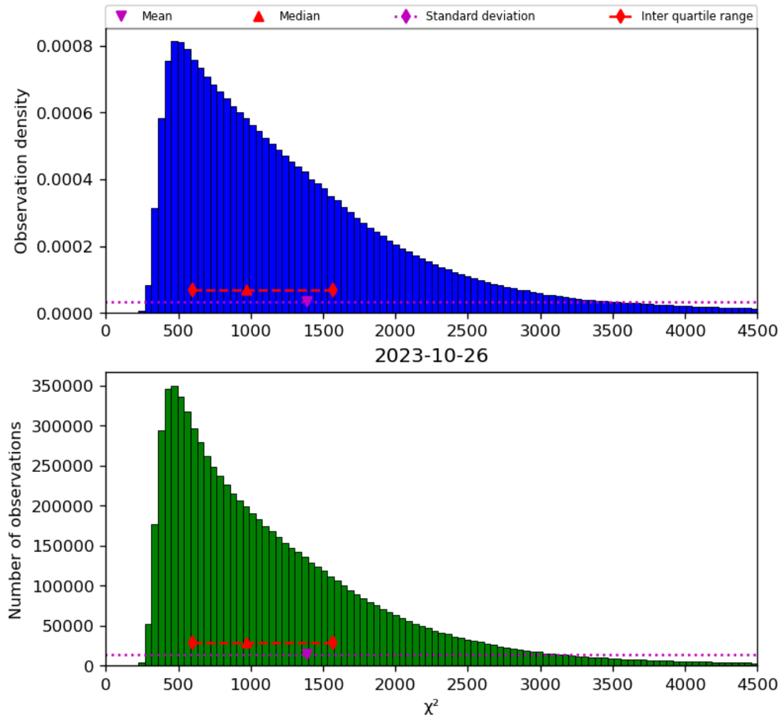
Figure 22: Histogram of “ \chi^2 ” for 2023-10-25 to 2023-10-27
