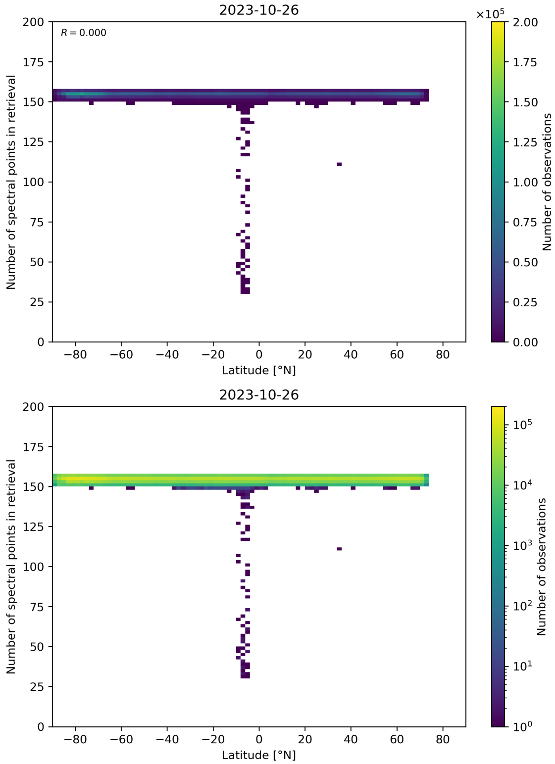
Figure 57: Scatter density plot of “Latitude” against “Number of spectral points in retrieval” for 2023-10-25 to 2023-10-27.
