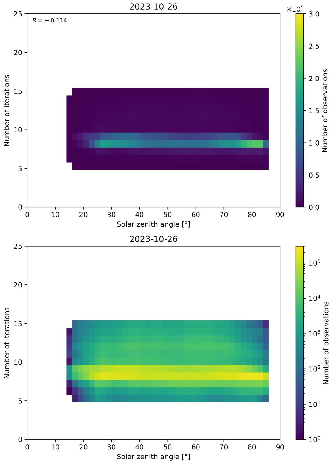
Figure 67: Scatter density plot of “Solar zenith angle” against “Number of iterations” for 2023-10-25 to 2023-10-27.
