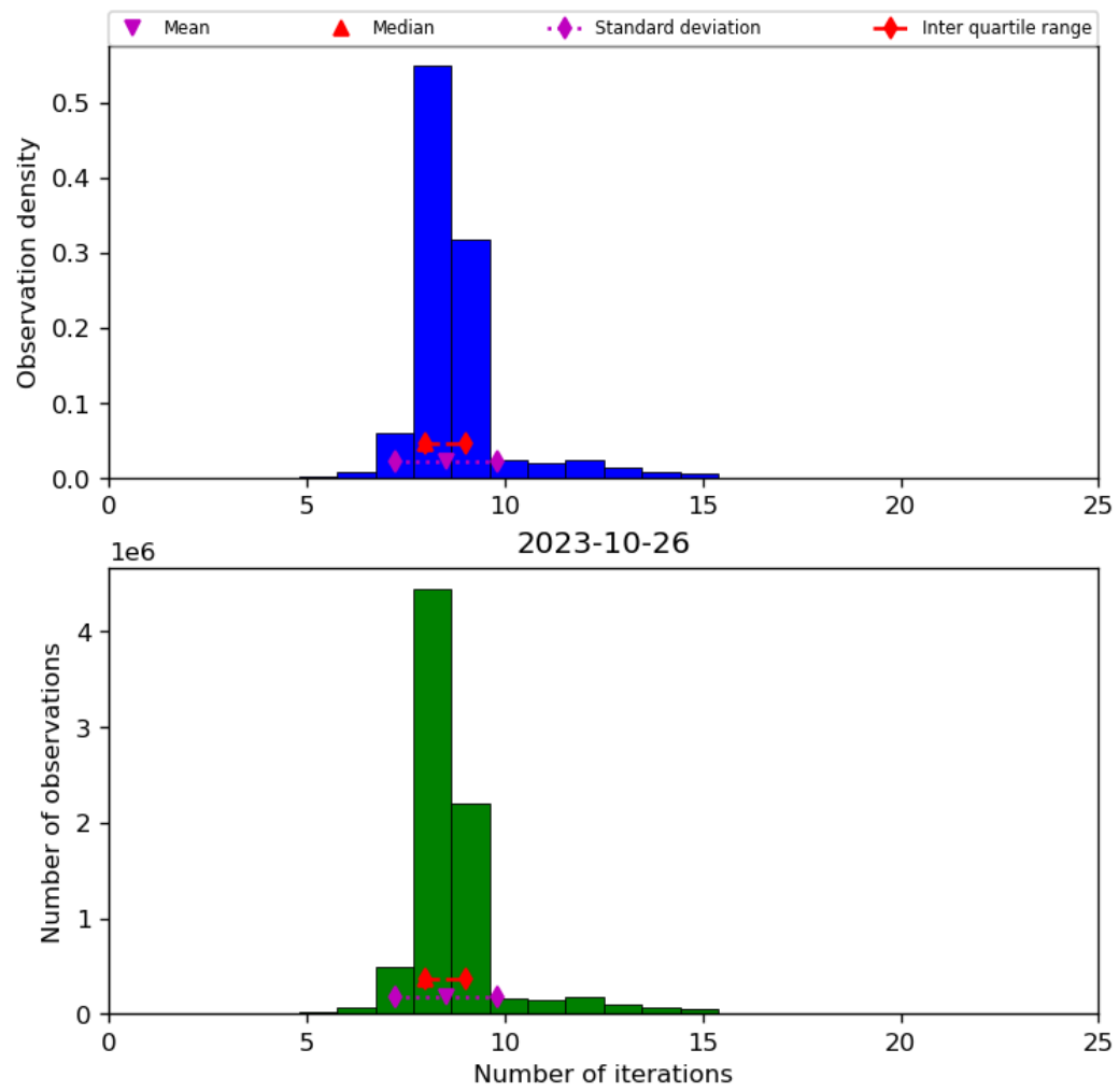
Figure 24: Histogram of “Number of iterations” for 2023-10-25 to 2023-10-27
