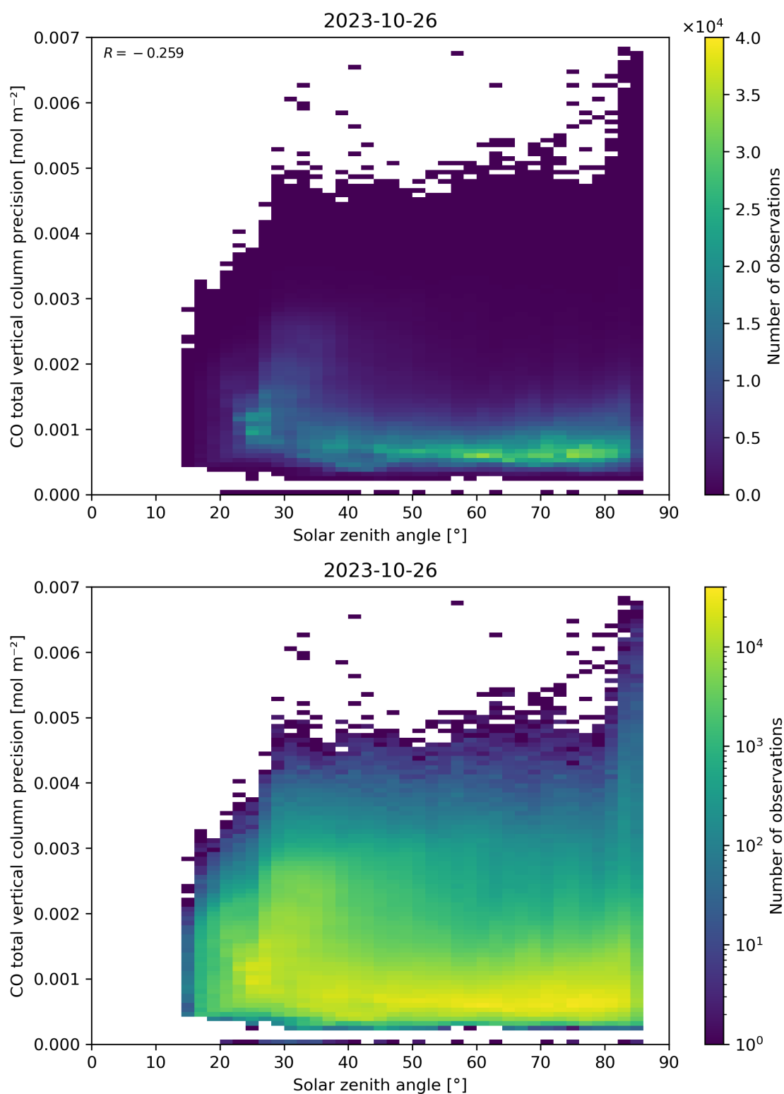
Figure 63: Scatter density plot of “Solar zenith angle” against “CO total vertical column precision” for 2023-10-25 to 2023-10-27.
