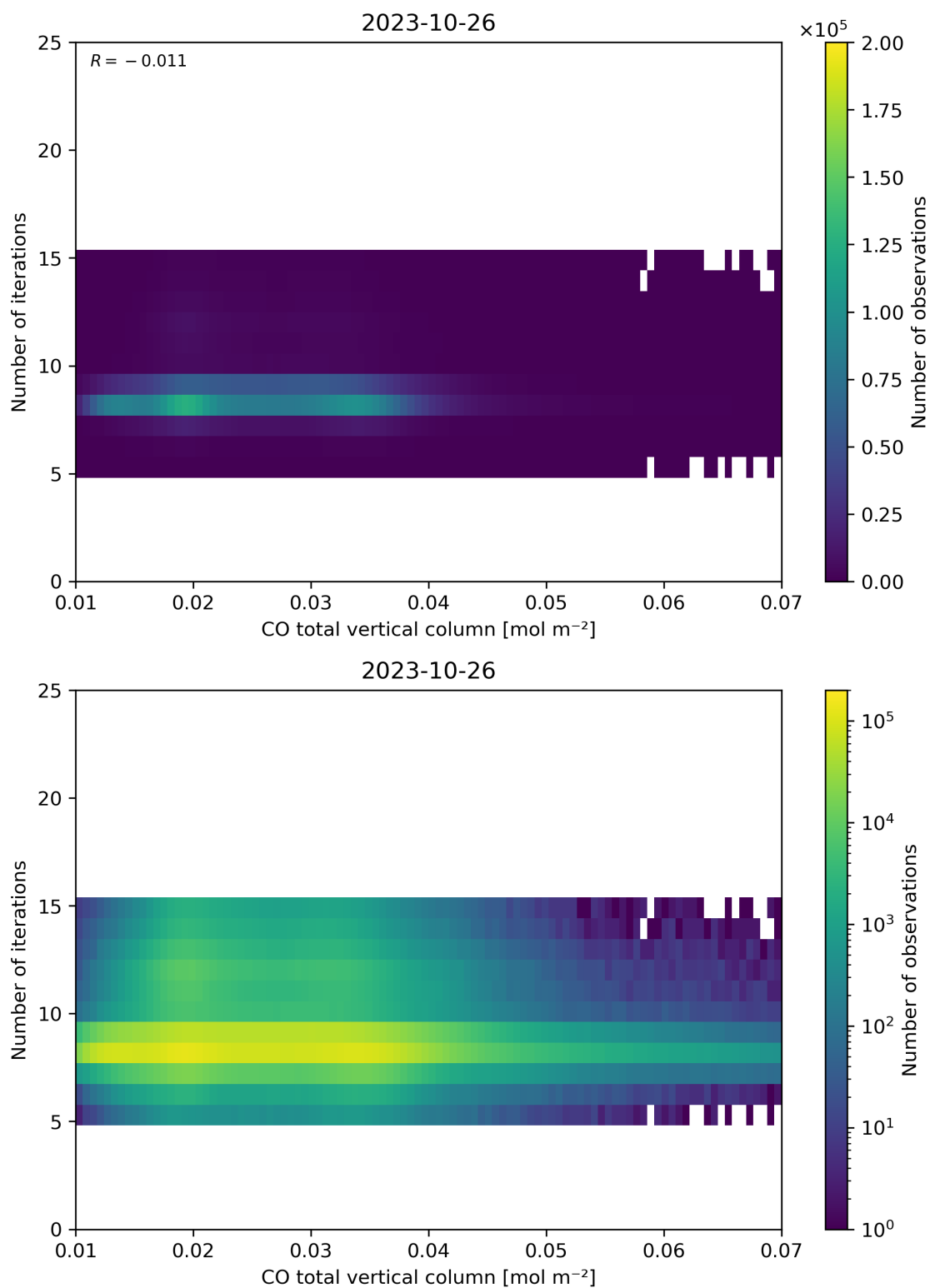
Figure 42: Scatter density plot of “CO total vertical column” against “Number of iterations” for 2023-10-25 to 2023-10-27.
