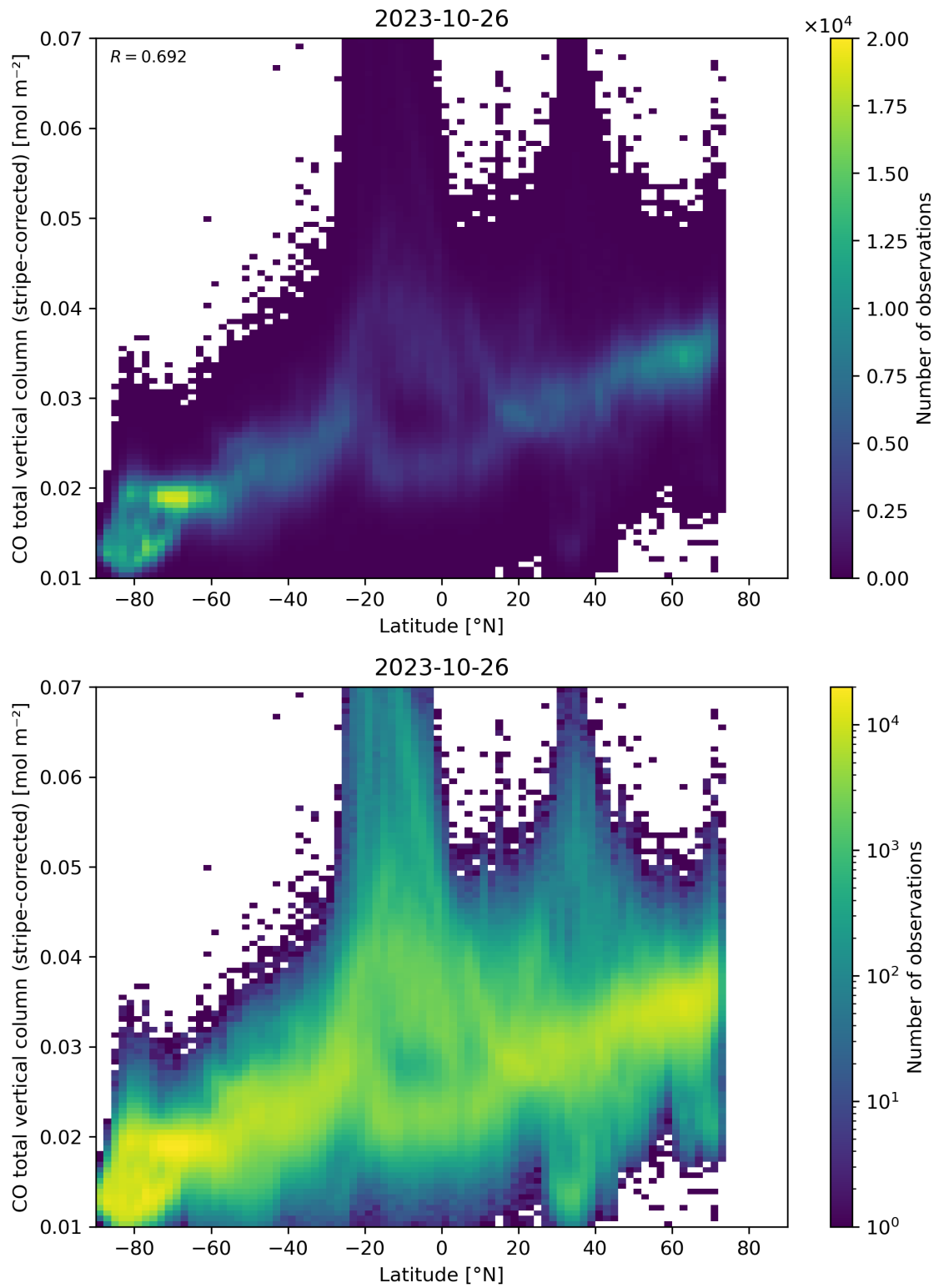
Figure 52: Scatter density plot of “Latitude” against “CO total vertical column (stripe-corrected)” for 2023-10-25 to 2023-10-27.
