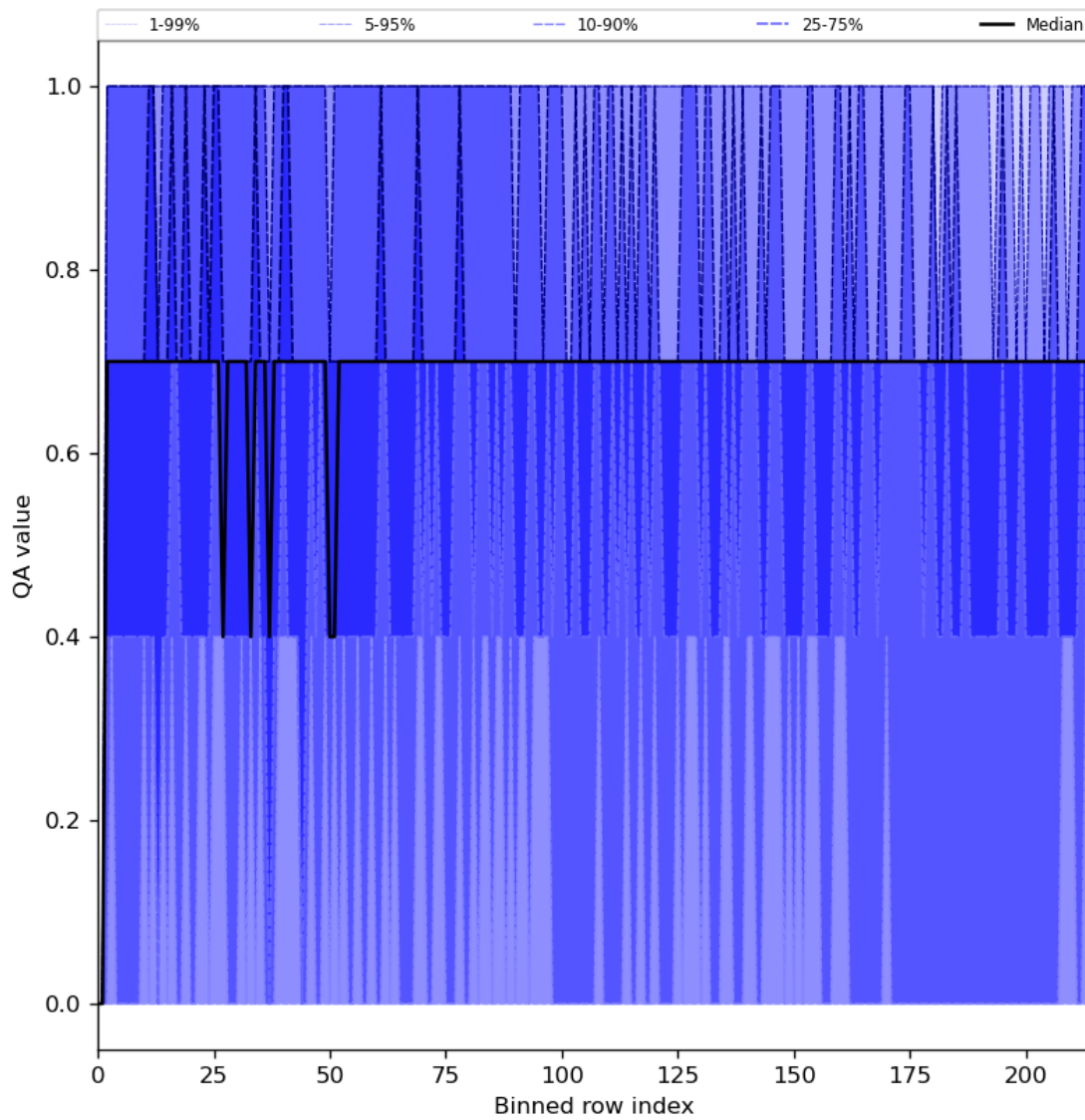
Figure 25: Along track statistics of “QA value” for 2023-10-25 to 2023-10-27
