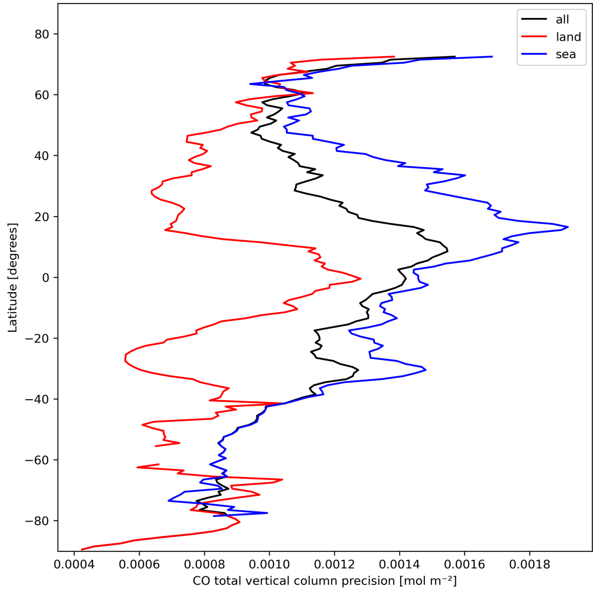
Figure 12: Zonal average of “CO total vertical column precision” for 2023-10-25 to 2023-10-27.
