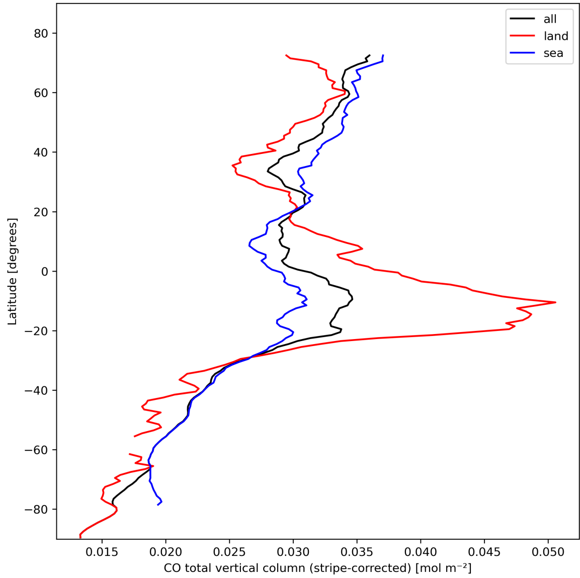
Figure 11: Zonal average of “CO total vertical column (stripe-corrected)” for 2023-10-25 to 2023-10-27.
