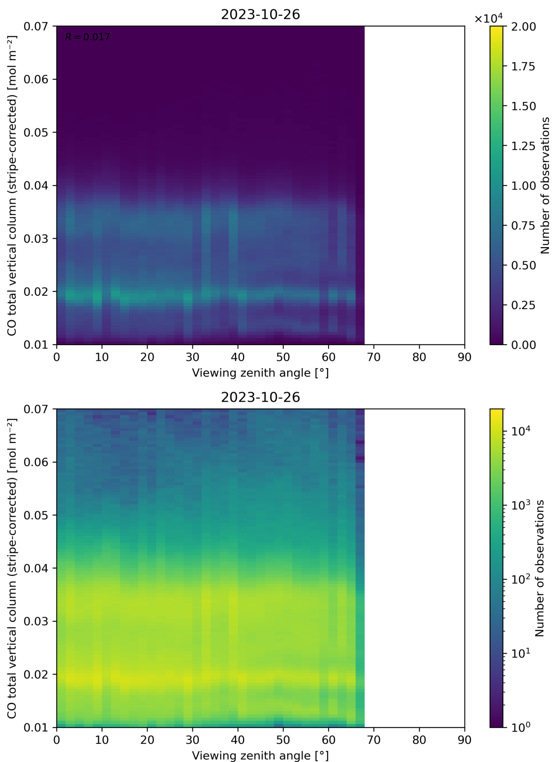
Figure 70: Scatter density plot of “Viewing zenith angle” against “CO total vertical column (stripe-corrected)” for 2023-10-25 to 2023-10-27.
