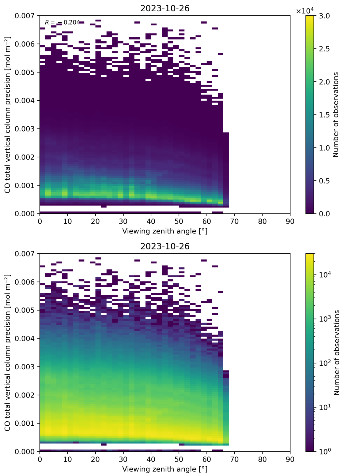
Figure 71: Scatter density plot of “Viewing zenith angle” against “CO total vertical column precision” for 2023-10-25 to 2023-10-27.
