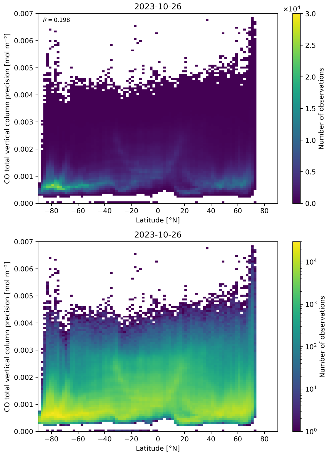
Figure 53: Scatter density plot of “Latitude” against “CO total vertical column precision” for 2023-10-25 to 2023-10-27.
