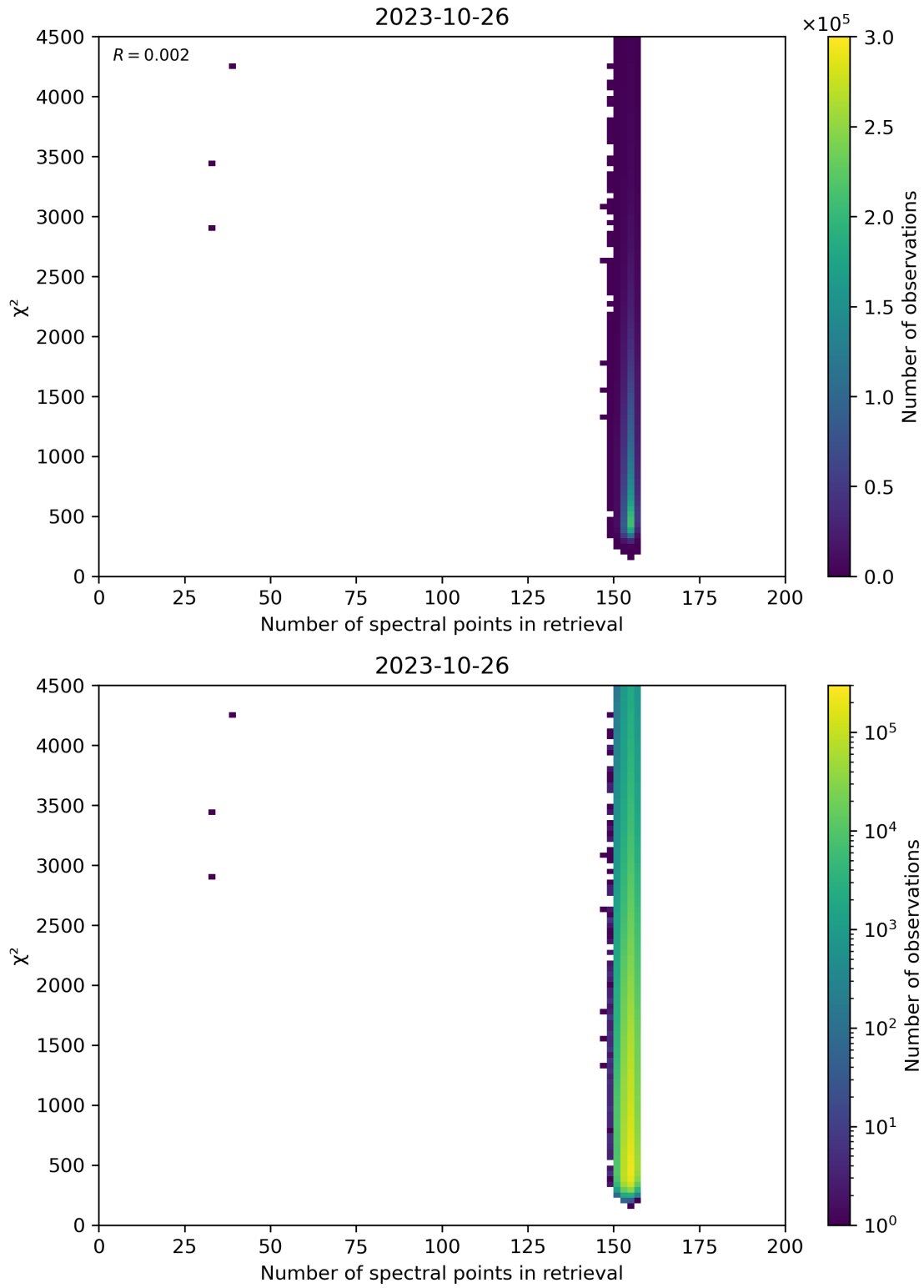
Figure 58: Scatter density plot of “Number of spectral points in retrieval” against “ \chi^2 ” for 2023-10-25 to 2023-10-27.
