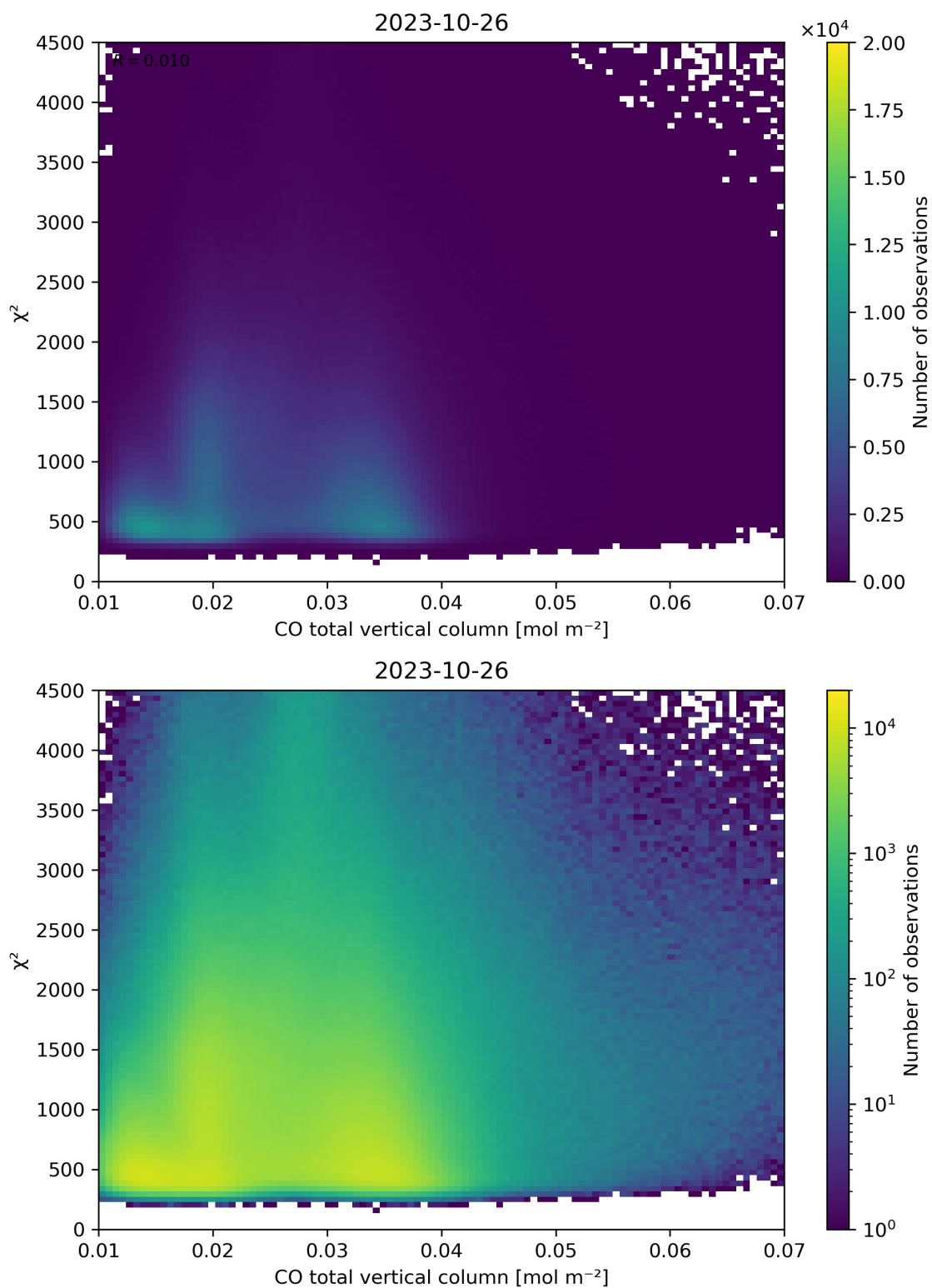
Figure 35: Scatter density plot of “CO total vertical column” against “ \chi^2 ” for 2023-10-25 to 2023-10-27.
