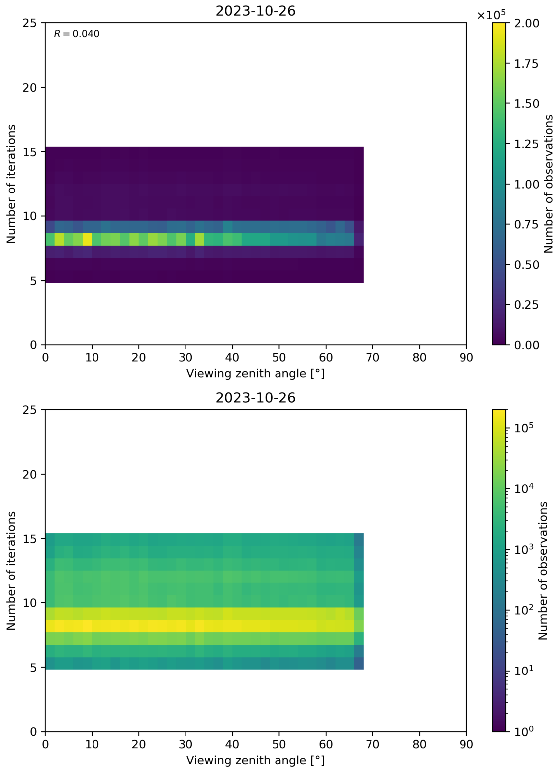
Figure 75: Scatter density plot of “Viewing zenith angle” against “Number of iterations” for 2023-10-25 to 2023-10-27.
