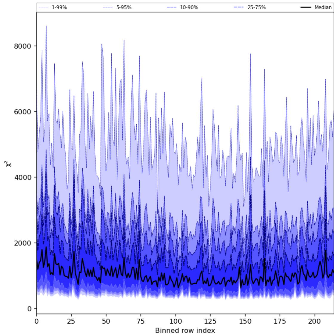
Figure 30: Along track statistics of “ \chi^2 ” for 2023-10-25 to 2023-10-27
