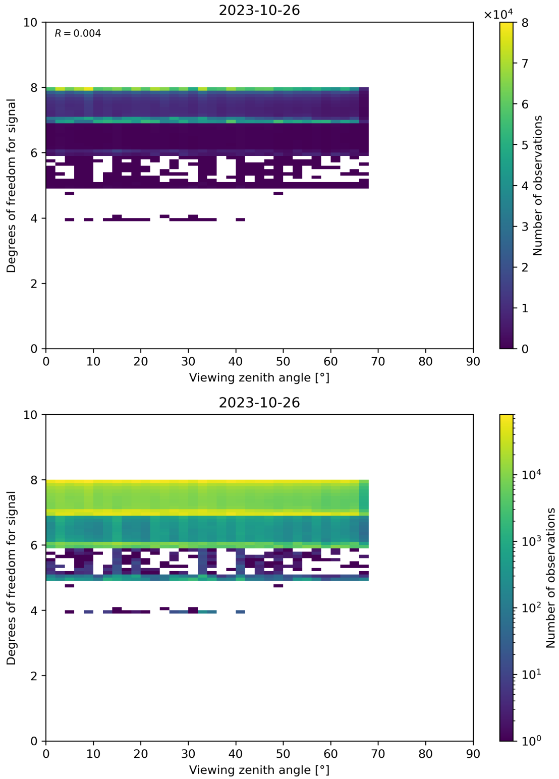
Figure 73: Scatter density plot of “Viewing zenith angle” against “Degrees of freedom for signal” for 2023-10-25 to 2023-10-27.
