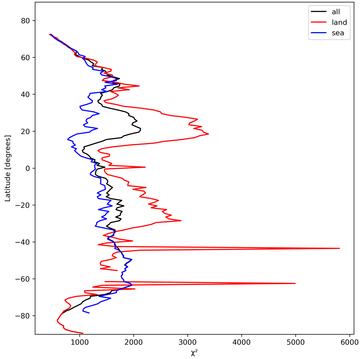
Figure 14: Zonal average of “ \chi^2 ” for 2023-10-25 to 2023-10-27.
