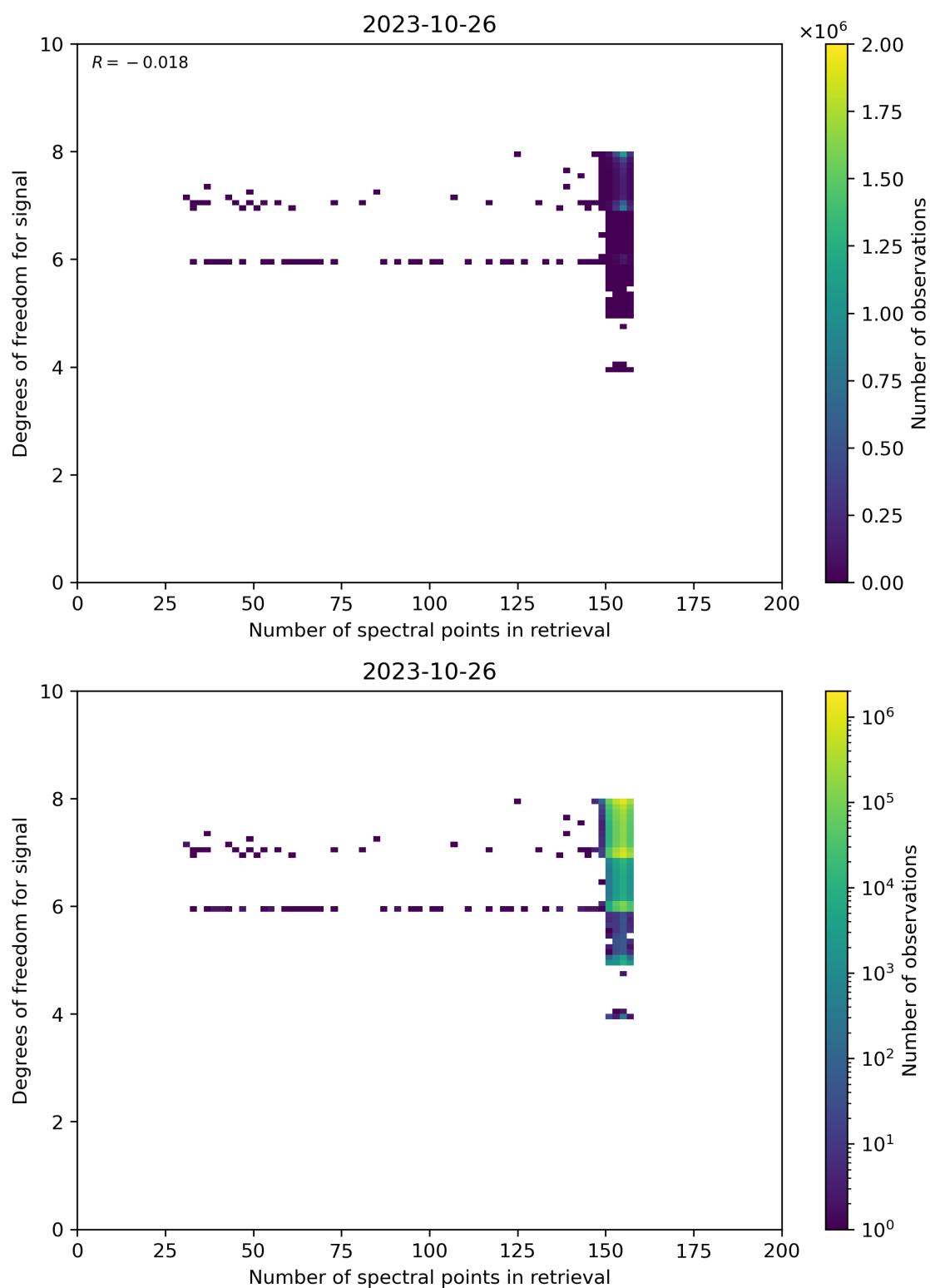
Figure 59: Scatter density plot of “Number of spectral points in retrieval” against “Degrees of freedom for signal” for 2023-10-25 to 2023-10-27.
