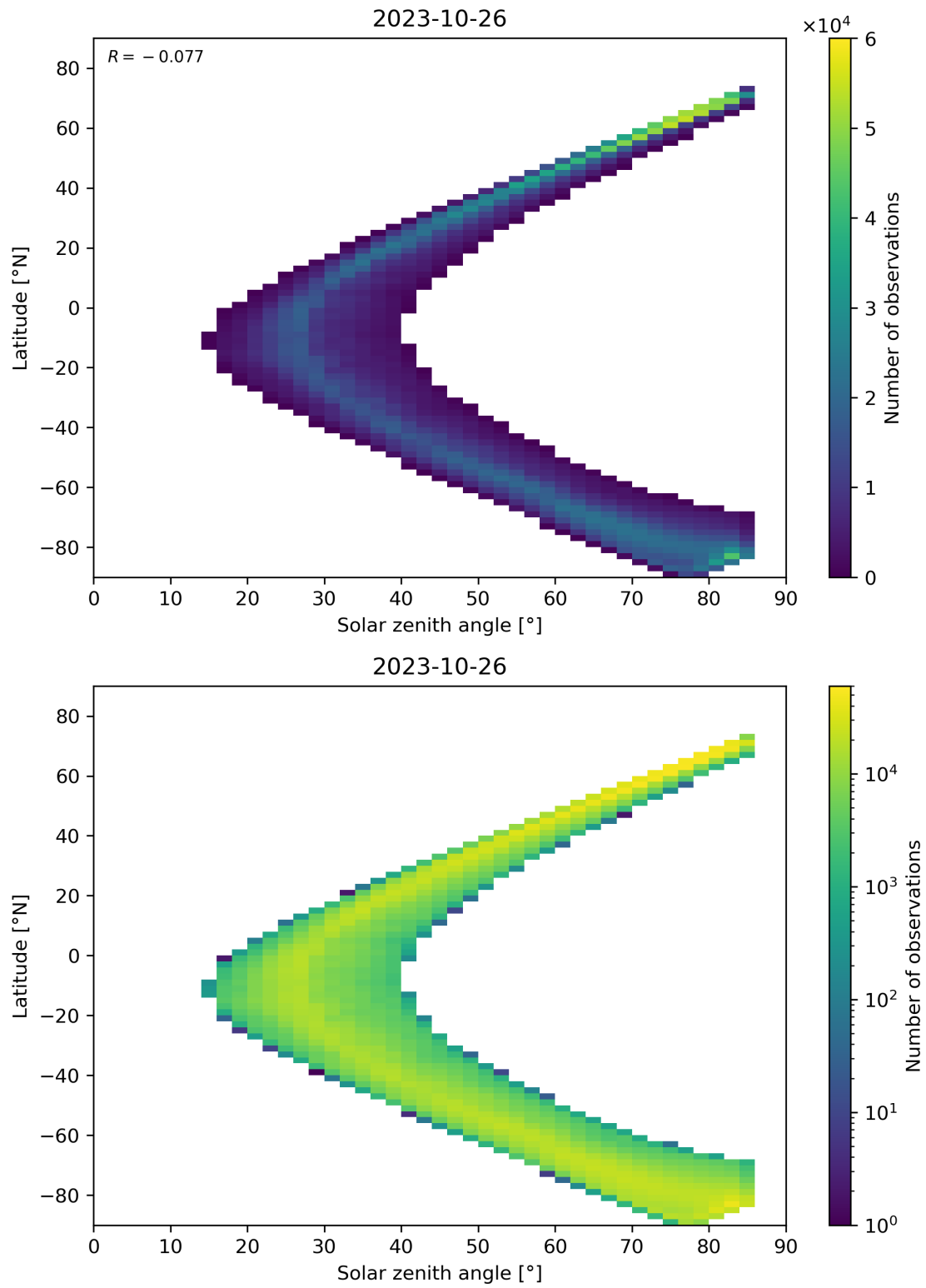
Figure 66: Scatter density plot of “Solar zenith angle” against “Latitude” for 2023-10-25 to 2023-10-27.
