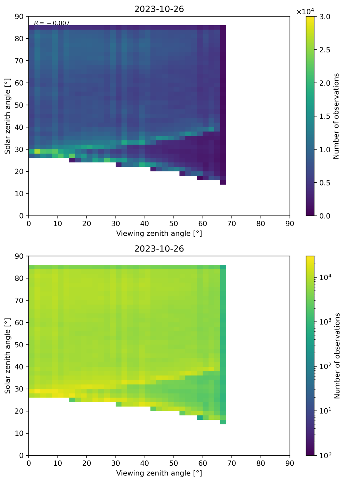
Figure 77: Scatter density plot of “Viewing zenith angle” against “Solar zenith angle” for 2023-10-25 to 2023-10-27.
