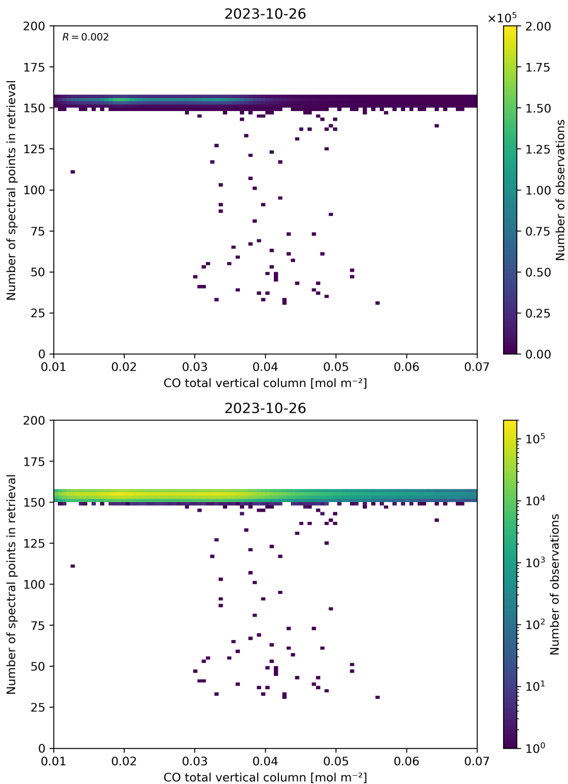
Figure 43: Scatter density plot of “CO total vertical column” against “Number of spectral points in retrieval” for 2023-10-25 to 2023-10-27.
