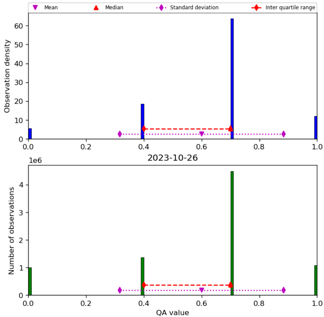
Figure 17: Histogram of “QA value” for 2023-10-25 to 2023-10-27
