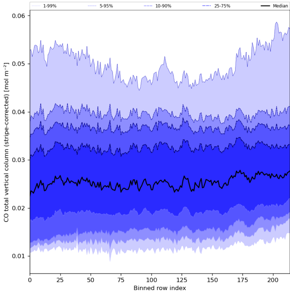
Figure 27: Along track statistics of “CO total vertical column (stripe-corrected)” for 2023-10-25 to 2023-10-27
