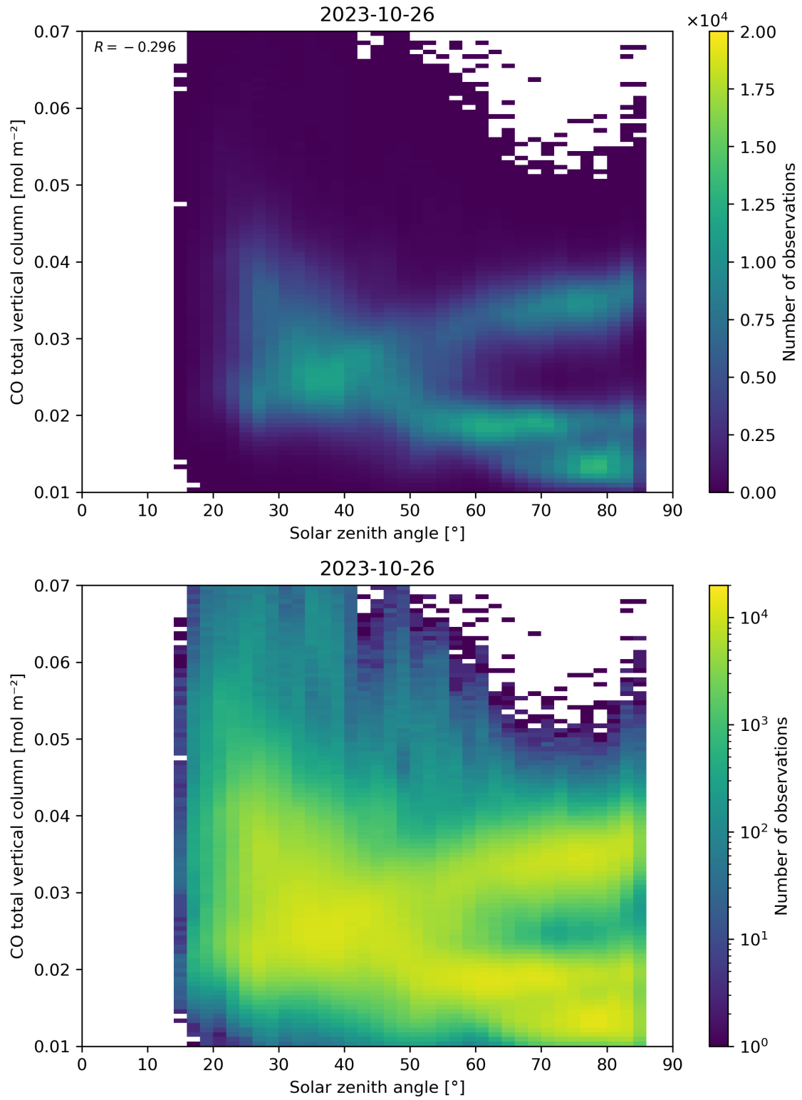
Figure 61: Scatter density plot of “Solar zenith angle” against “CO total vertical column” for 2023-10-25 to 2023-10-27.
