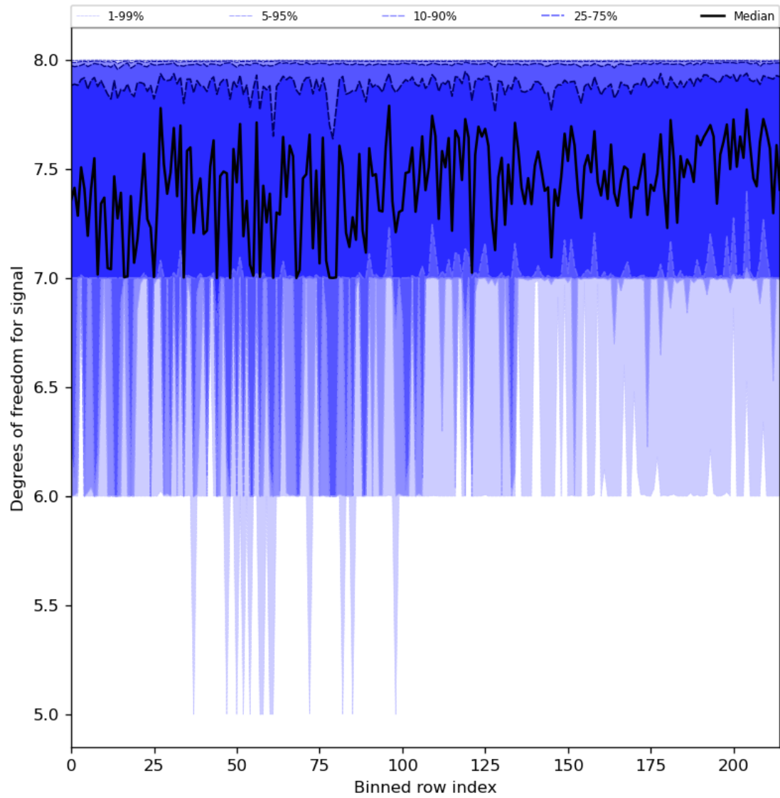
Figure 31: Along track statistics of “Degrees of freedom for signal” for 2023-10-25 to 2023-10-27
