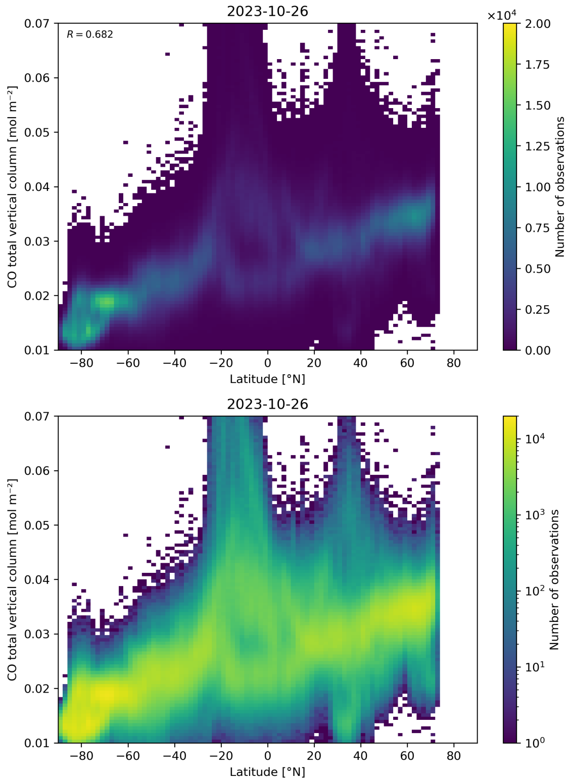
Figure 51: Scatter density plot of “Latitude” against “CO total vertical column” for 2023-10-25 to 2023-10-27.
