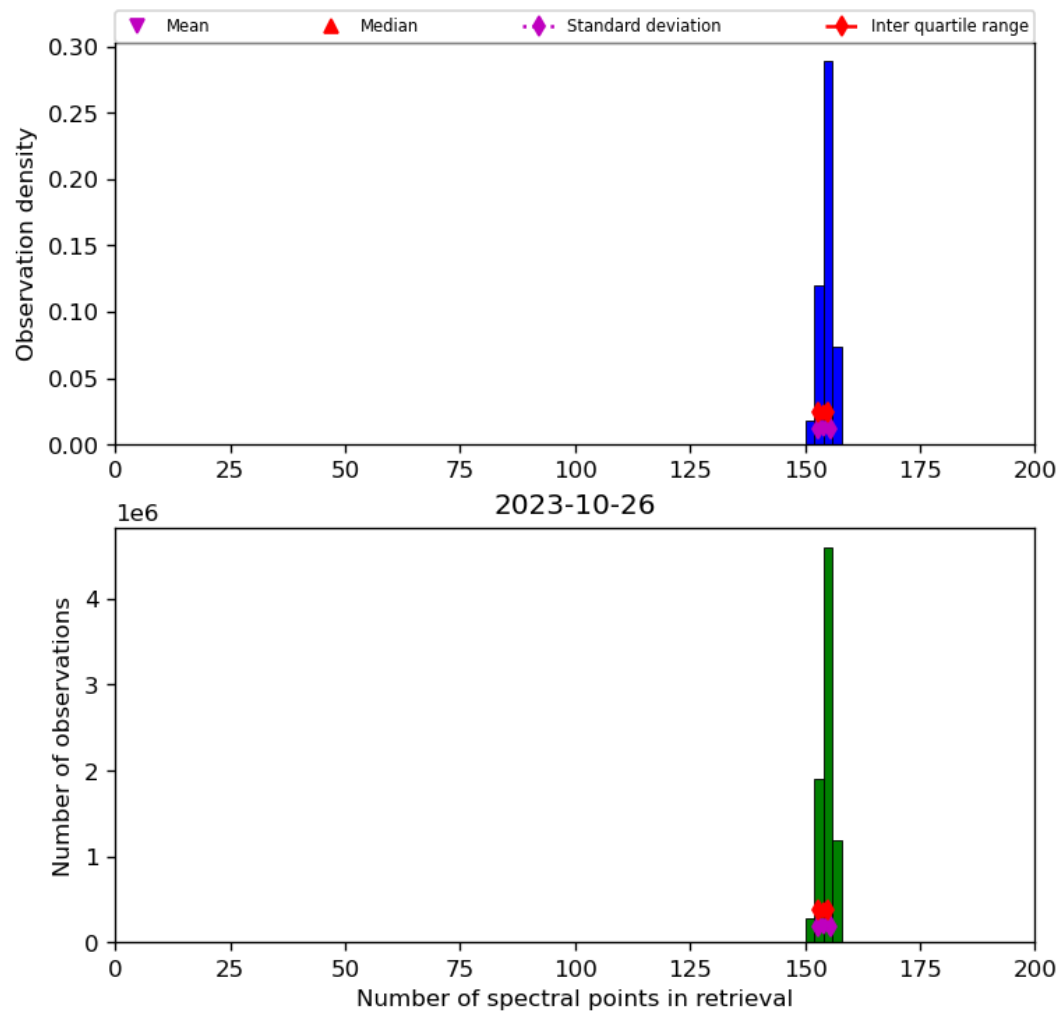
Figure 21: Histogram of “Number of spectral points in retrieval” for 2023-10-25 to 2023-10-27
