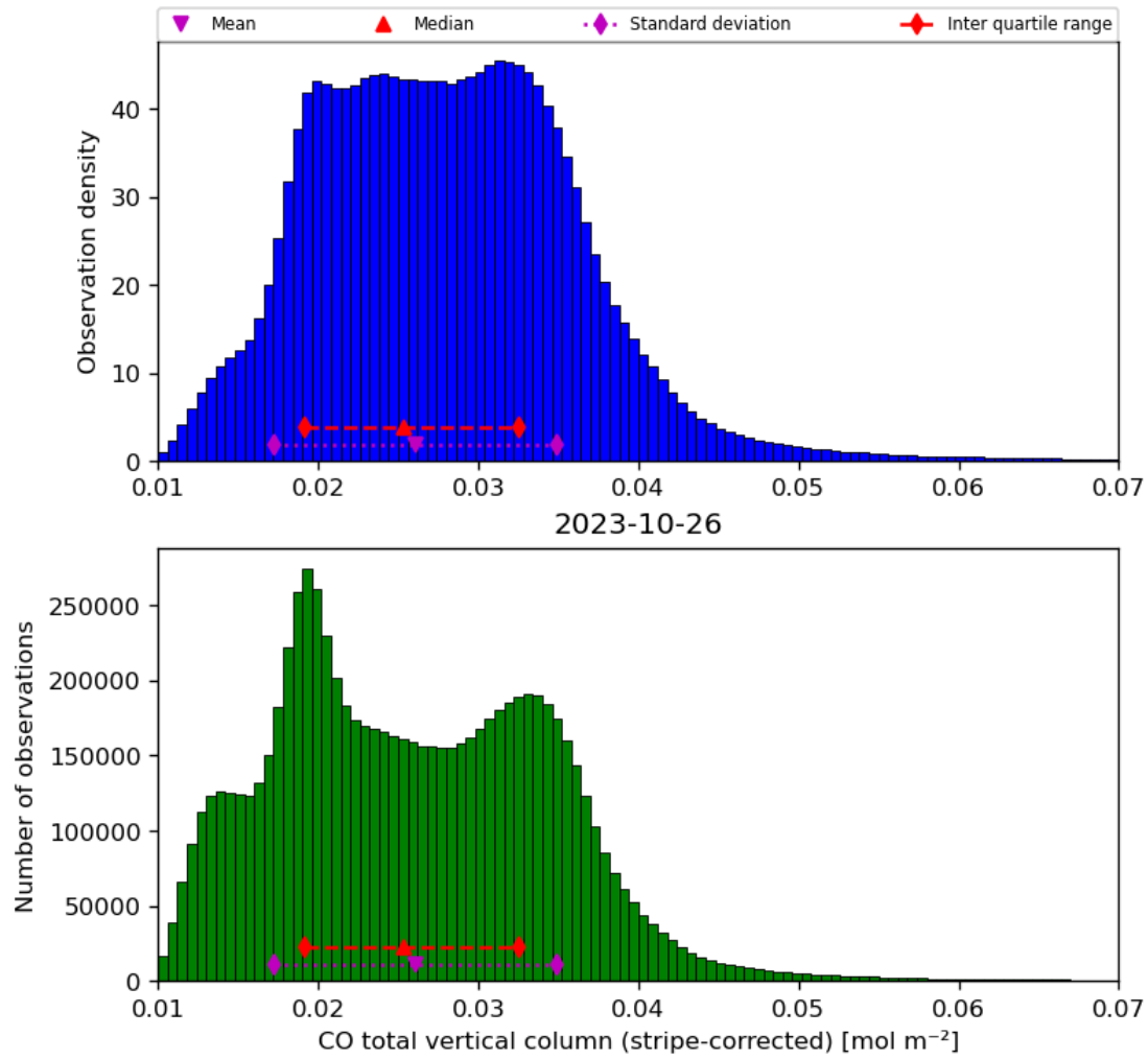
Figure 19: Histogram of “CO total vertical column (stripe-corrected)” for 2023-10-25 to 2023-10-27
