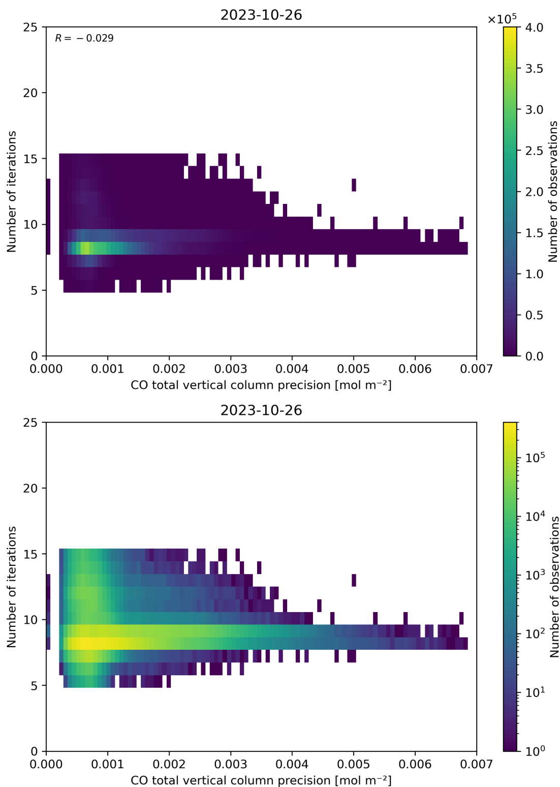
Figure 46: Scatter density plot of “CO total vertical column precision” against “Number of iterations” for 2023-10-25 to 2023-10-27.
