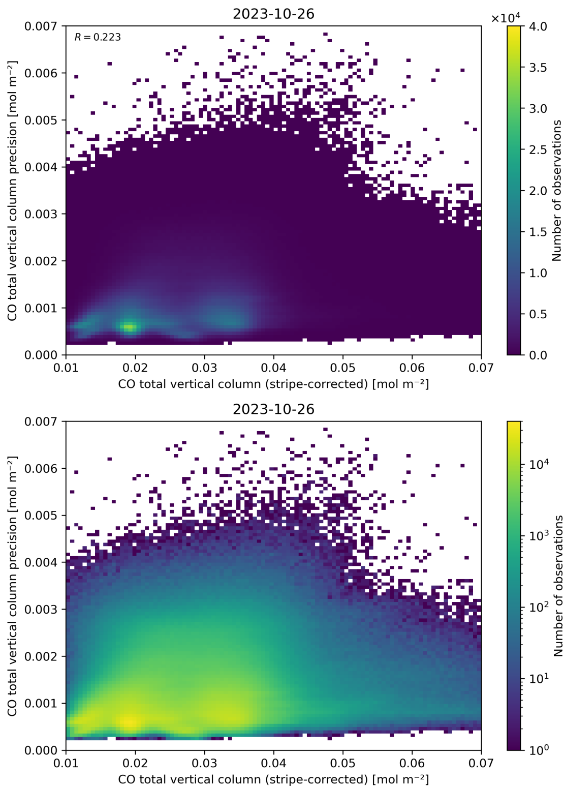
Figure 36: Scatter density plot of “CO total vertical column (stripe-corrected)” against “CO total vertical column precision” for 2023-10-25 to 2023-10-27.
