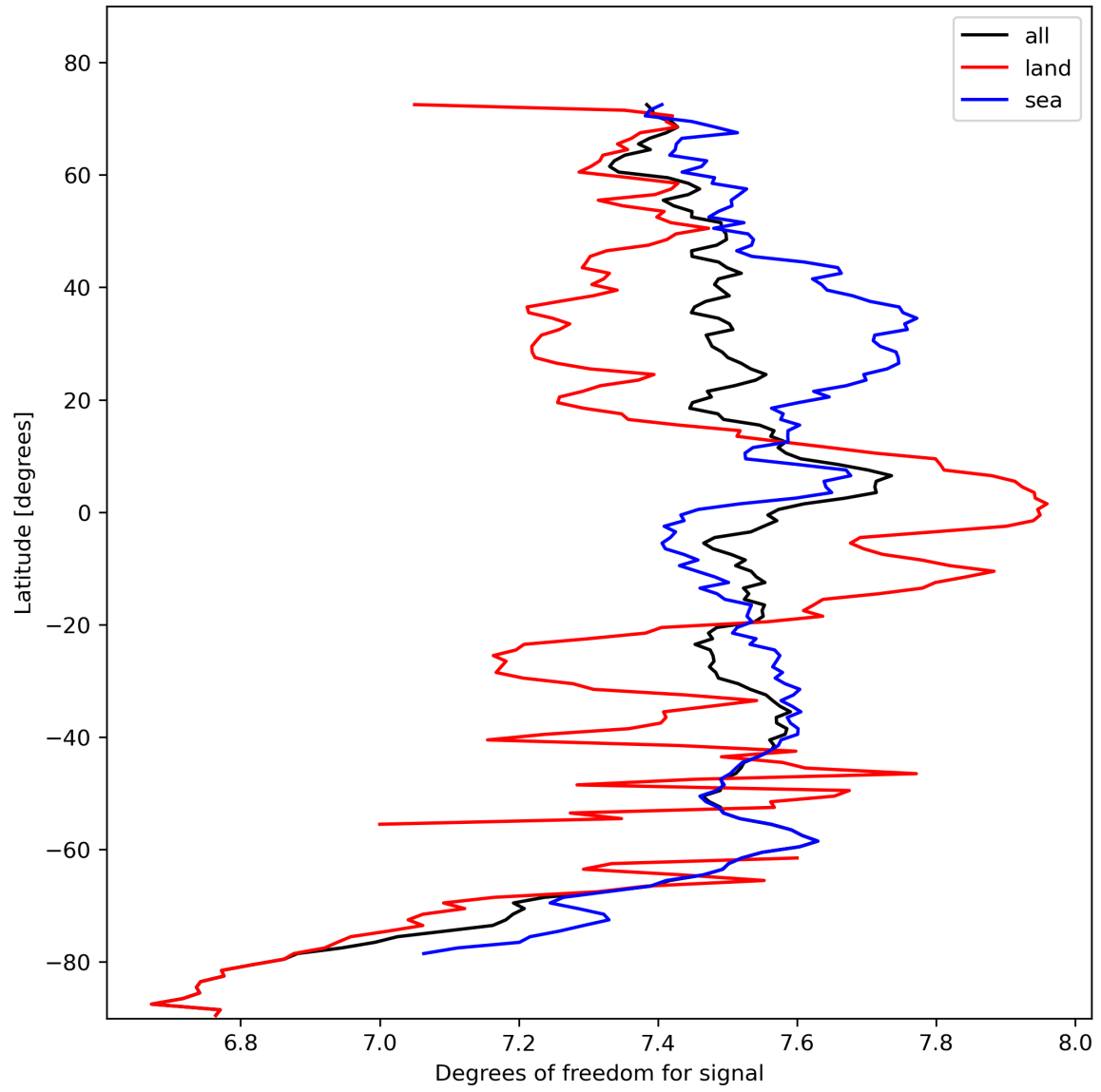
Figure 15: Zonal average of “Degrees of freedom for signal” for 2023-10-25 to 2023-10-27.
