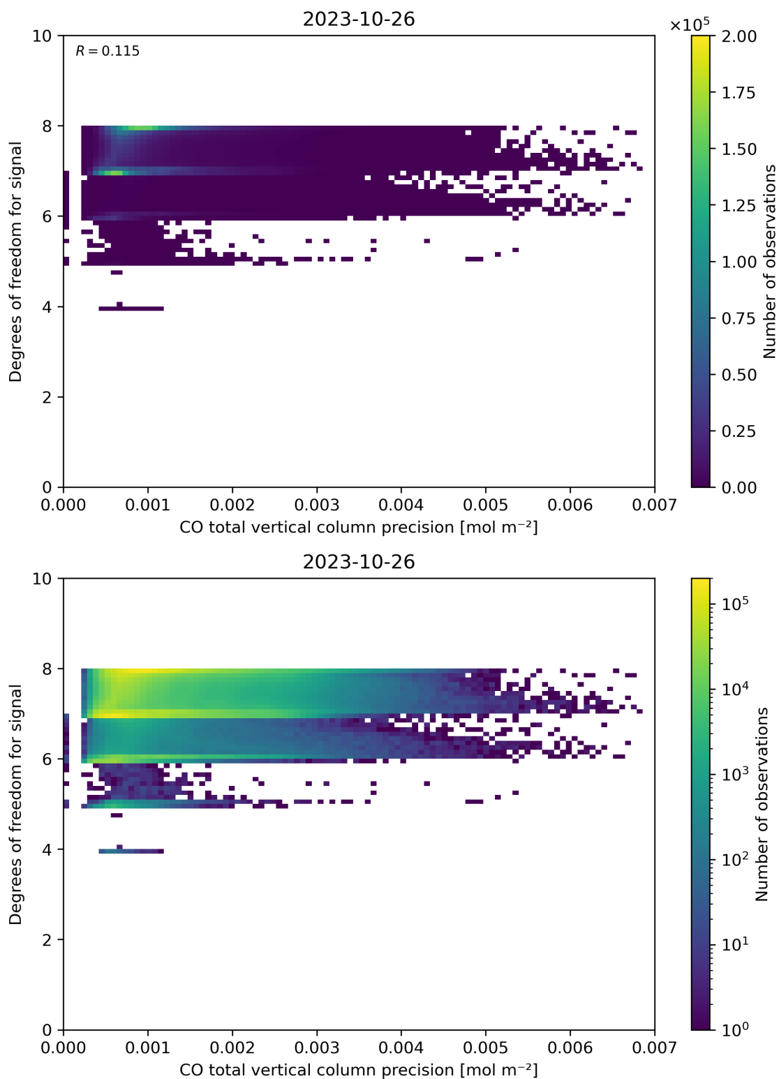
Figure 45: Scatter density plot of “CO total vertical column precision” against “Degrees of freedom for signal” for 2023-10-25 to 2023-10-27.
