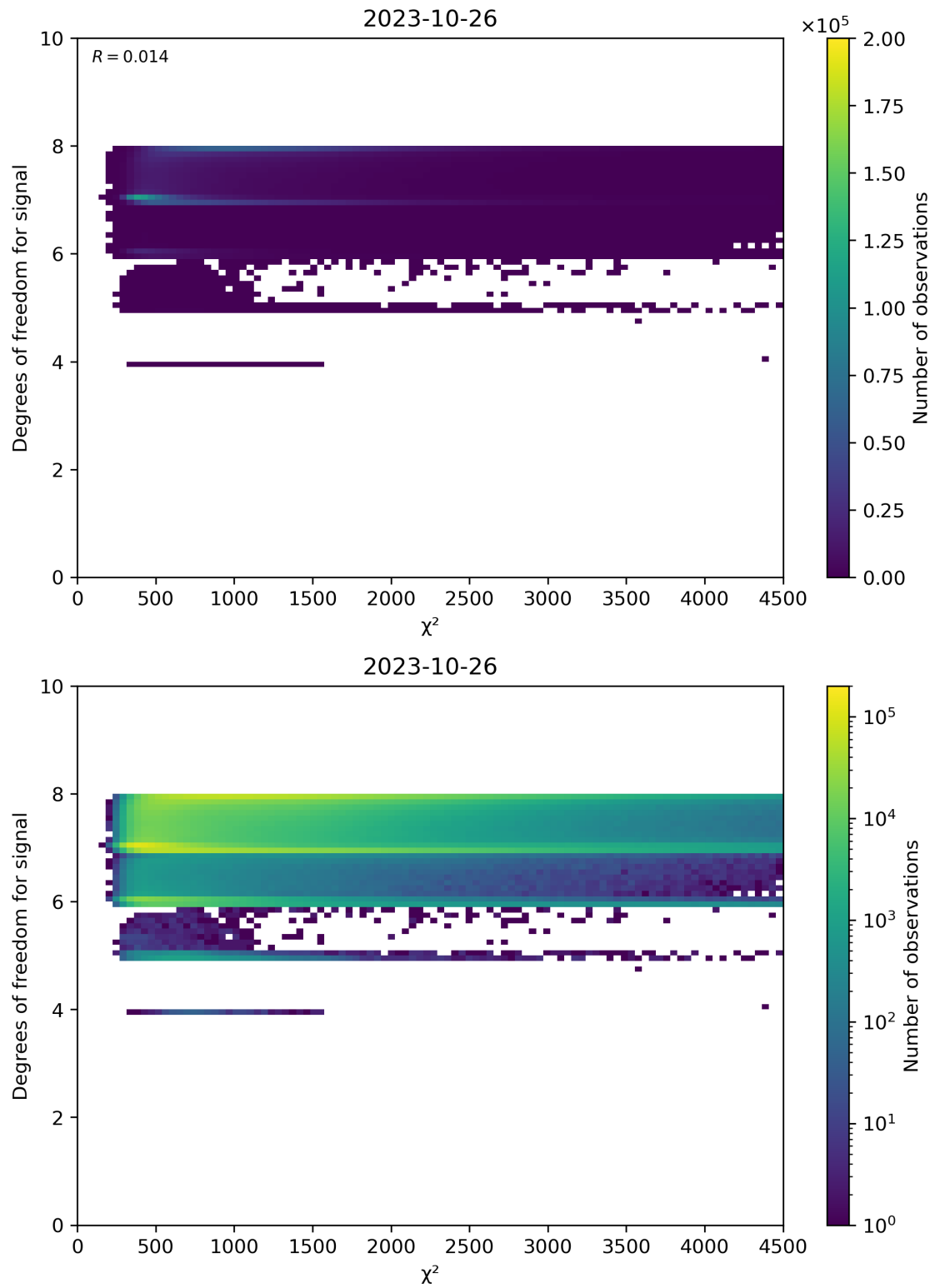
Figure 48: Scatter density plot of “ \chi^2 ” against “Degrees of freedom for signal” for 2023-10-25 to 2023-10-27.
