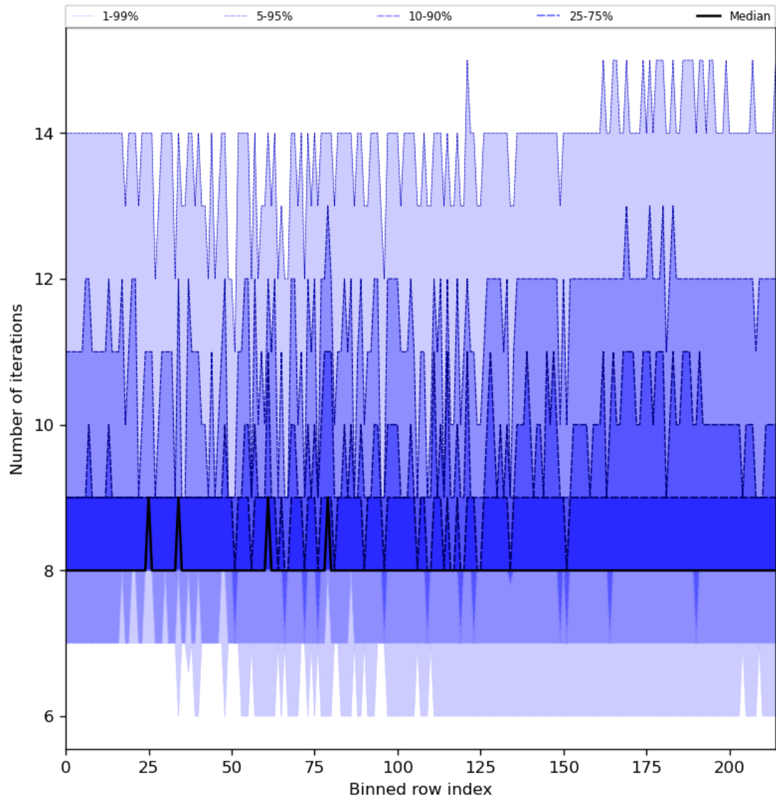
Figure 32: Along track statistics of “Number of iterations” for 2023-10-25 to 2023-10-27
