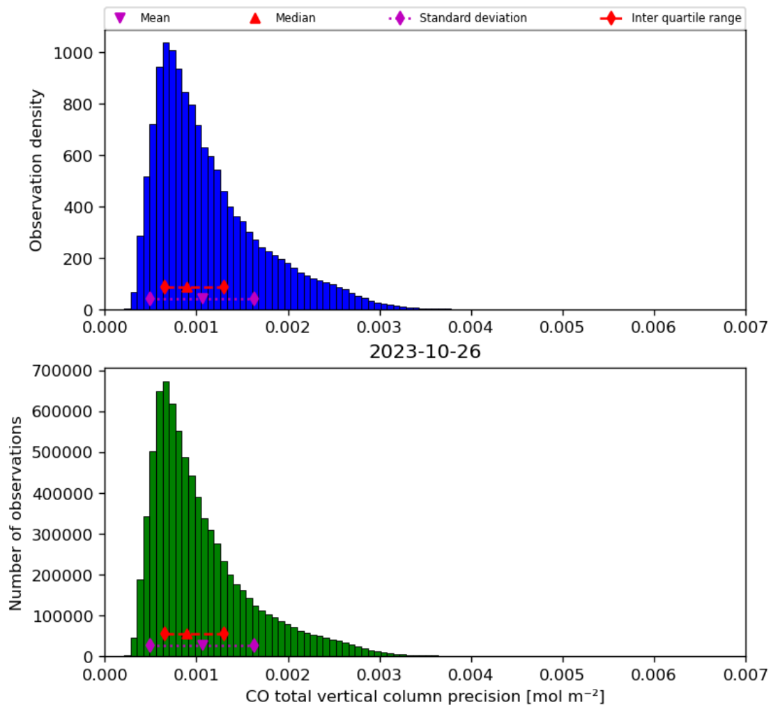
Figure 20: Histogram of “CO total vertical column precision” for 2023-10-25 to 2023-10-27
