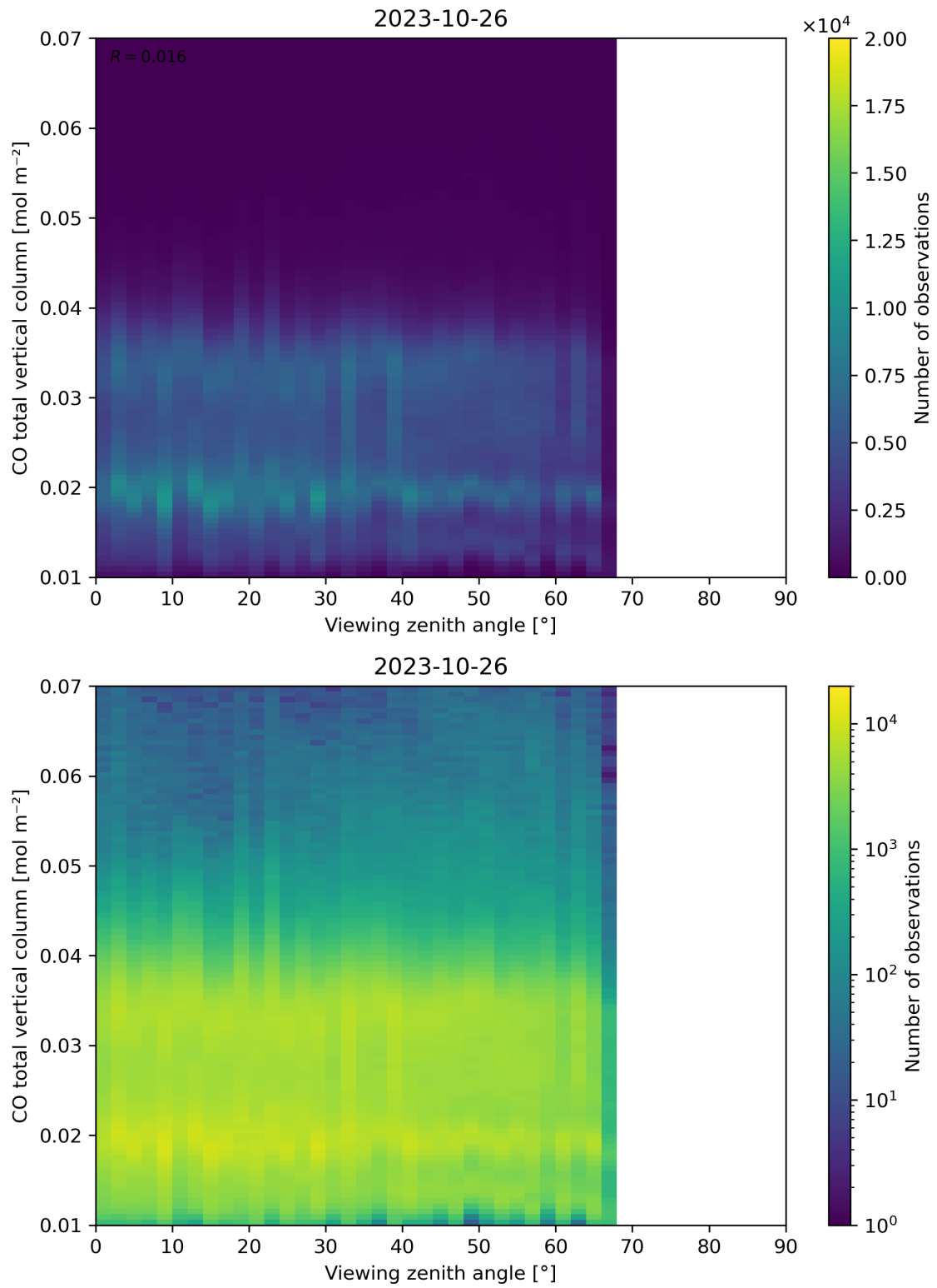
Figure 69: Scatter density plot of “Viewing zenith angle” against “CO total vertical column” for 2023-10-25 to 2023-10-27.
