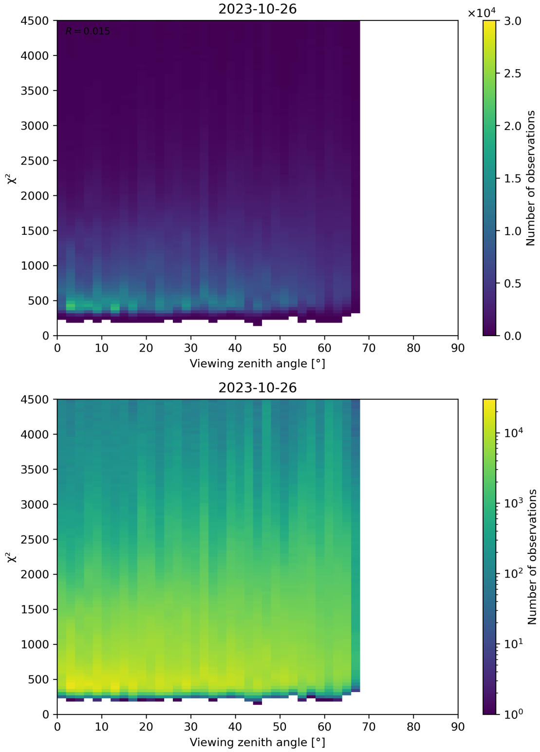
Figure 72: Scatter density plot of “Viewing zenith angle” against “ \chi^2 ” for 2023-10-25 to 2023-10-27.
