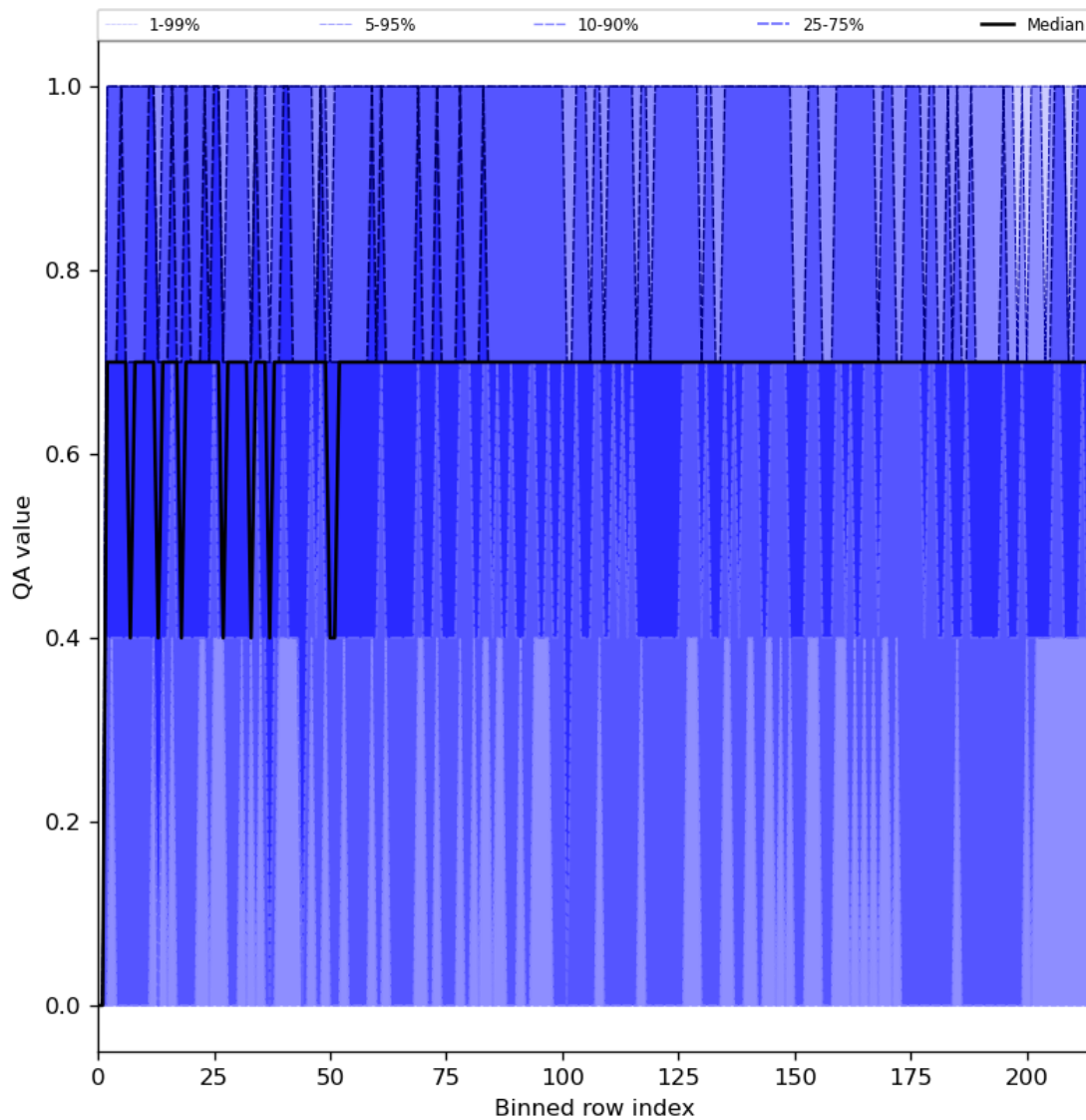
Figure 25: Along track statistics of “QA value” for 2023-10-28 to 2023-10-29
