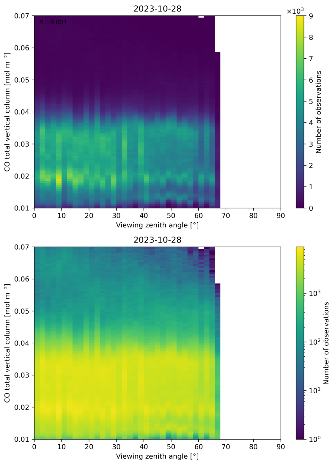
Figure 69: Scatter density plot of “Viewing zenith angle” against “CO total vertical column” for 2023-10-28 to 2023-10-29.
