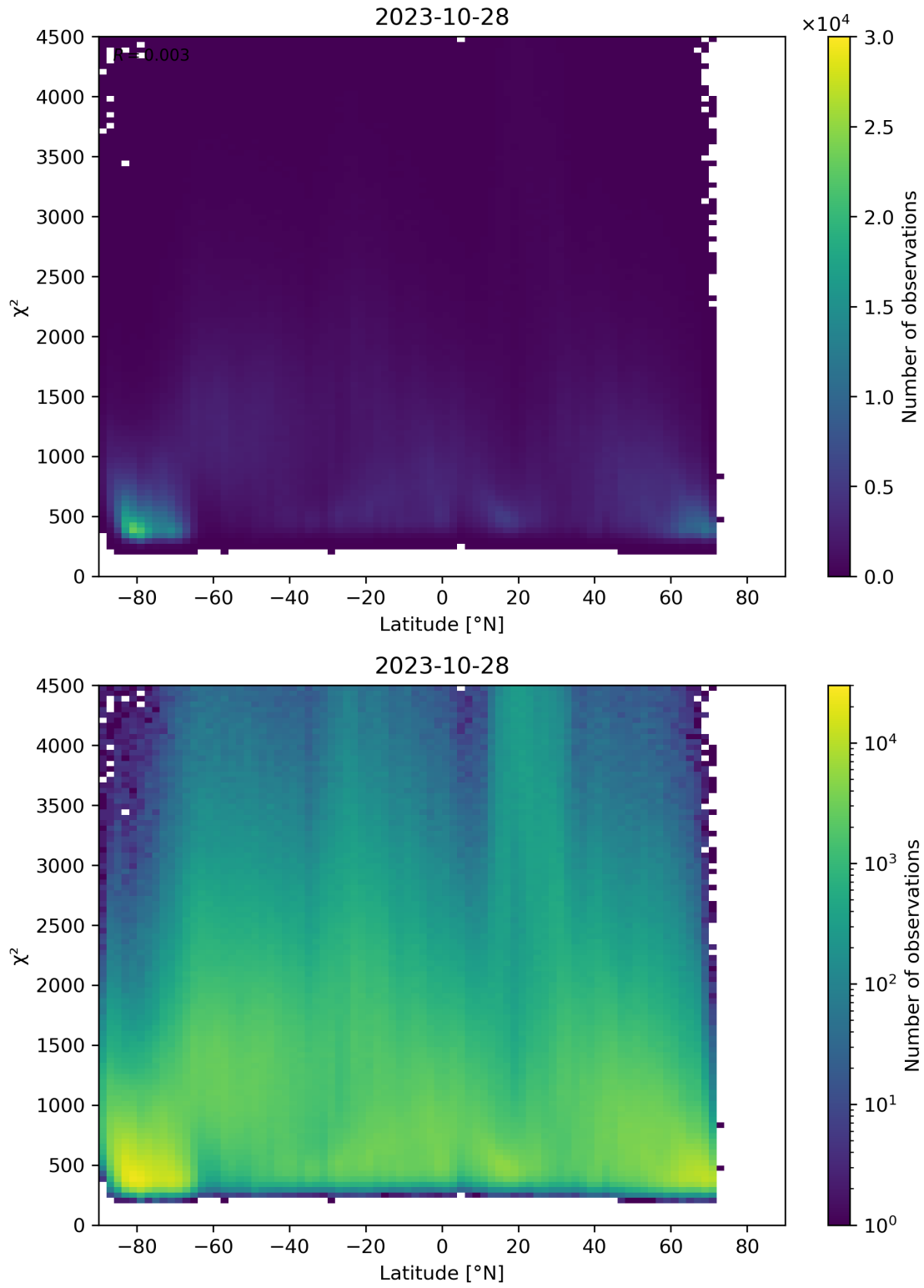
Figure 54: Scatter density plot of “Latitude” against “ \chi^2 ” for 2023-10-28 to 2023-10-29.
