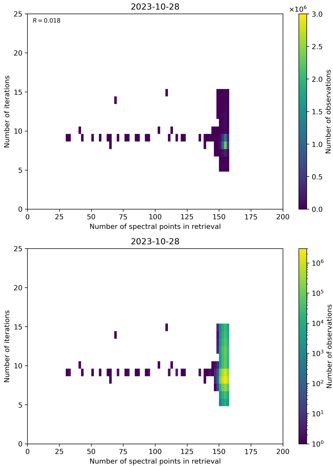
Figure 60: Scatter density plot of “Number of spectral points in retrieval” against “Number of iterations” for 2023-10-28 to 2023-10-29.
