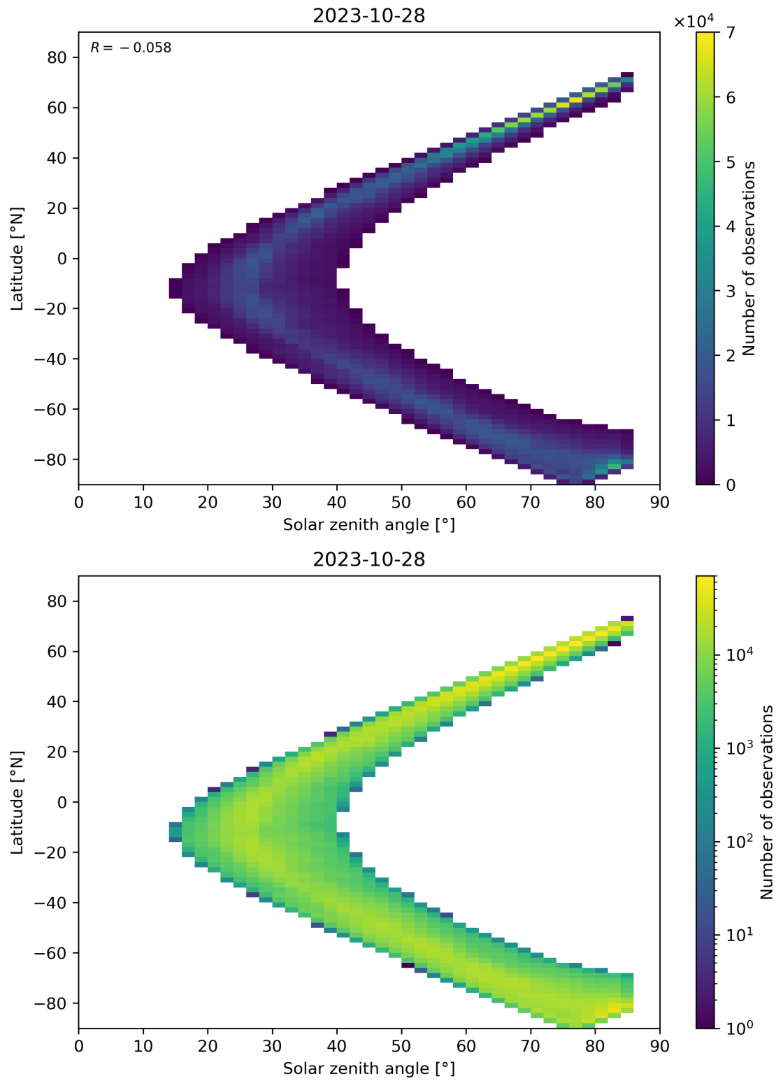
Figure 66: Scatter density plot of “Solar zenith angle” against “Latitude” for 2023-10-28 to 2023-10-29.
