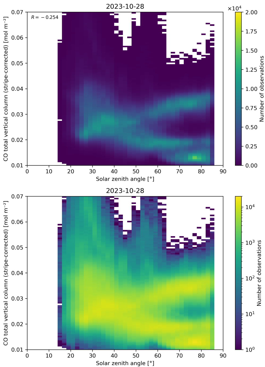
Figure 62: Scatter density plot of “Solar zenith angle” against “CO total vertical column (stripe-corrected)” for 2023-10-28 to 2023-10-29.
