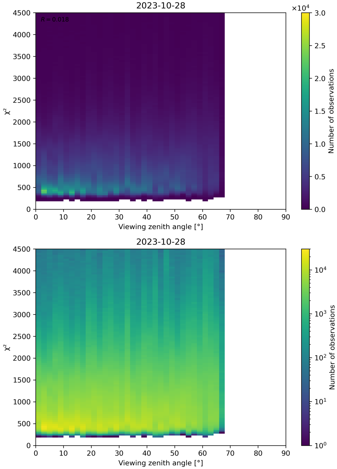
Figure 72: Scatter density plot of “Viewing zenith angle” against “ \chi^2 ” for 2023-10-28 to 2023-10-29.
