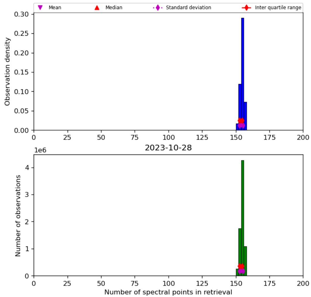
Figure 21: Histogram of “Number of spectral points in retrieval” for 2023-10-28 to 2023-10-29
