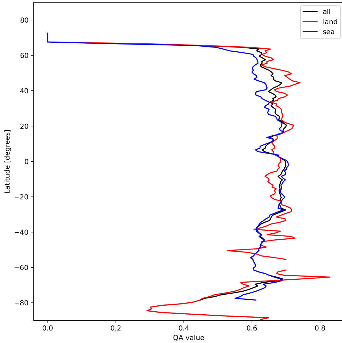
Figure 9: Zonal average of “QA value” for 2023-10-28 to 2023-10-29.
