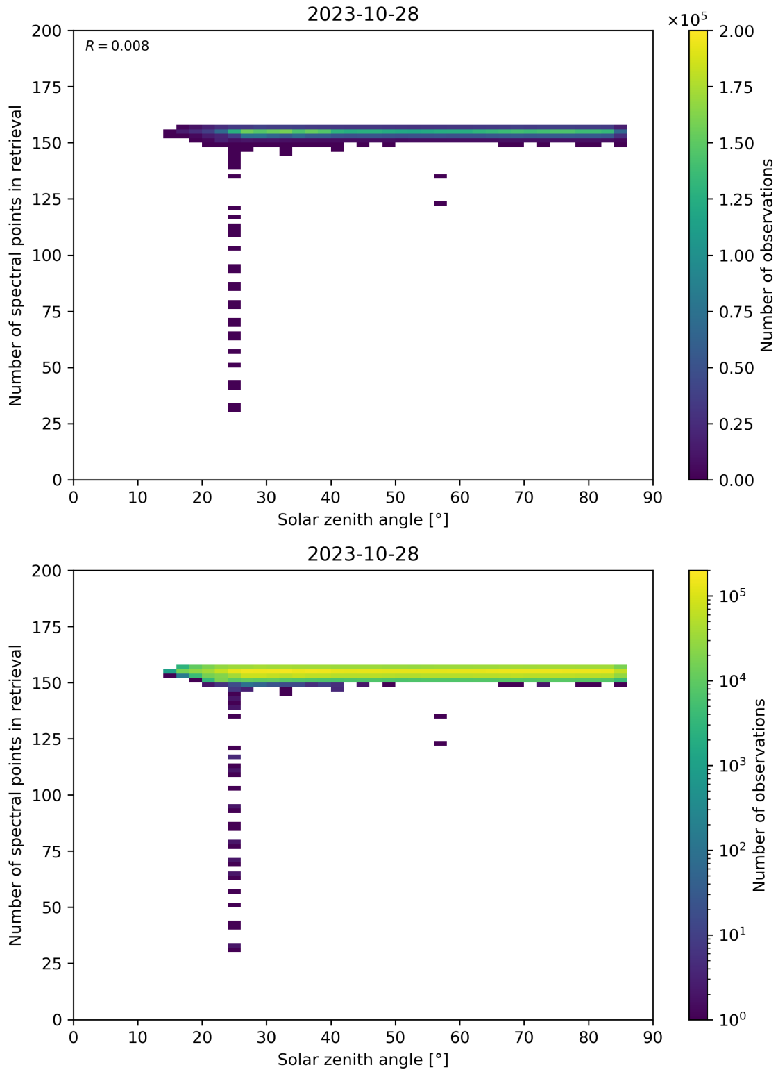
Figure 68: Scatter density plot of “Solar zenith angle” against “Number of spectral points in retrieval” for 2023-10-28 to 2023-10-29.
