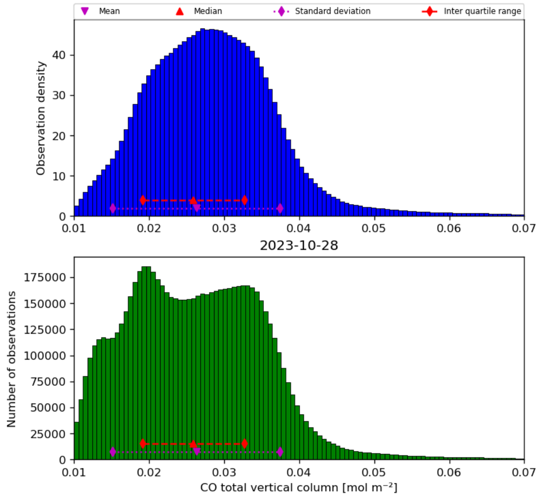
Figure 18: Histogram of “CO total vertical column” for 2023-10-28 to 2023-10-29
