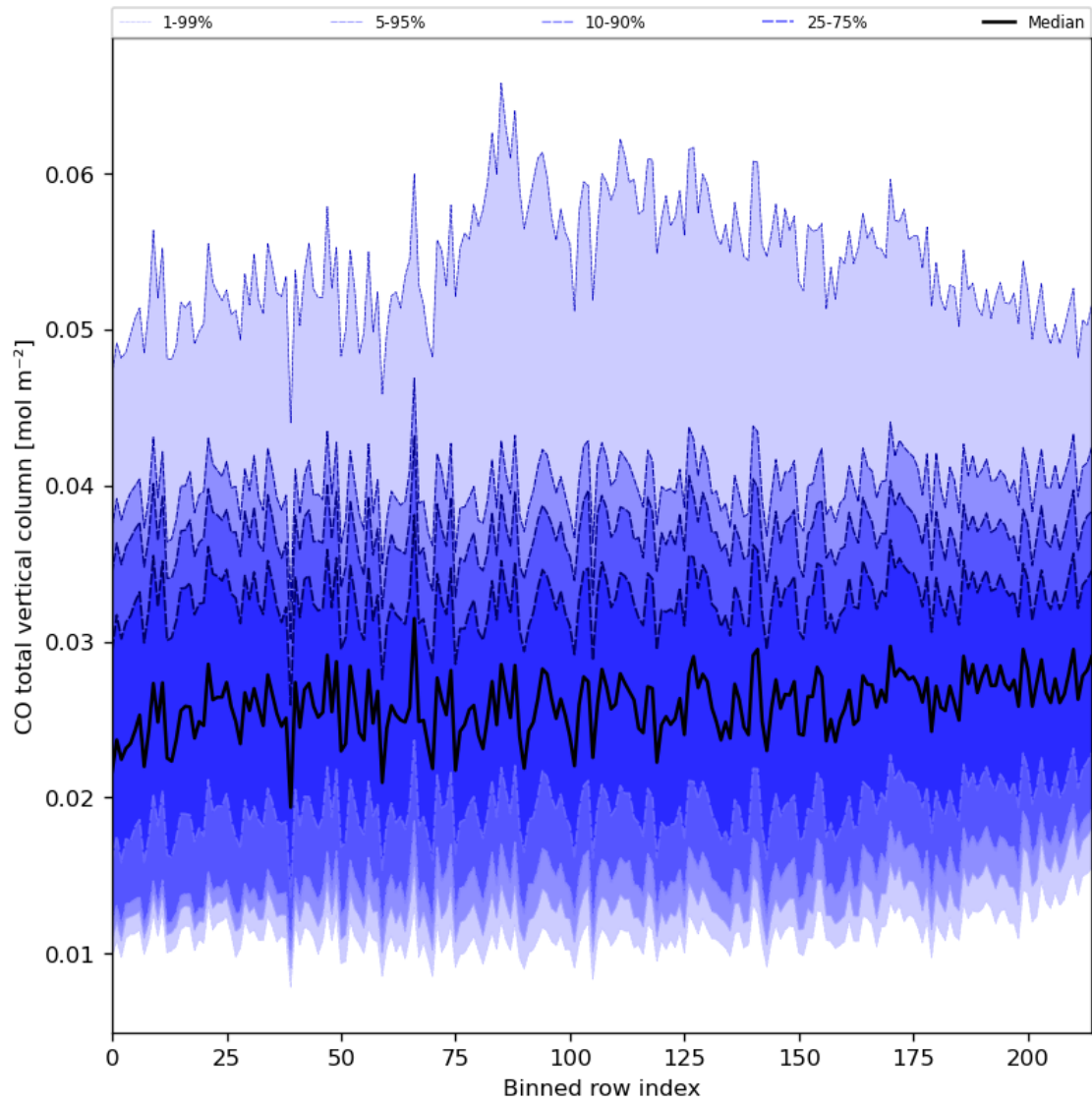
Figure 26: Along track statistics of “CO total vertical column” for 2023-10-28 to 2023-10-29
