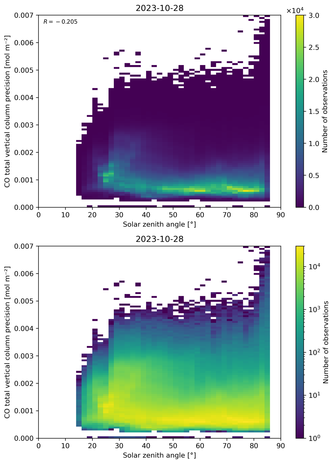
Figure 63: Scatter density plot of “Solar zenith angle” against “CO total vertical column precision” for 2023-10-28 to 2023-10-29.
