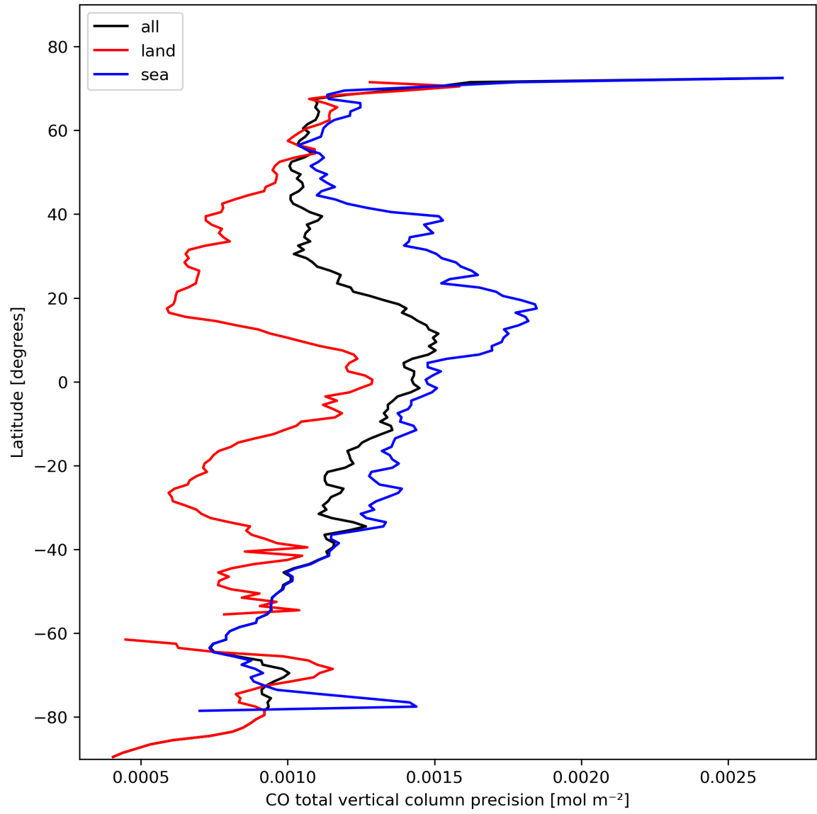
Figure 12: Zonal average of “CO total vertical column precision” for 2023-10-28 to 2023-10-29.
