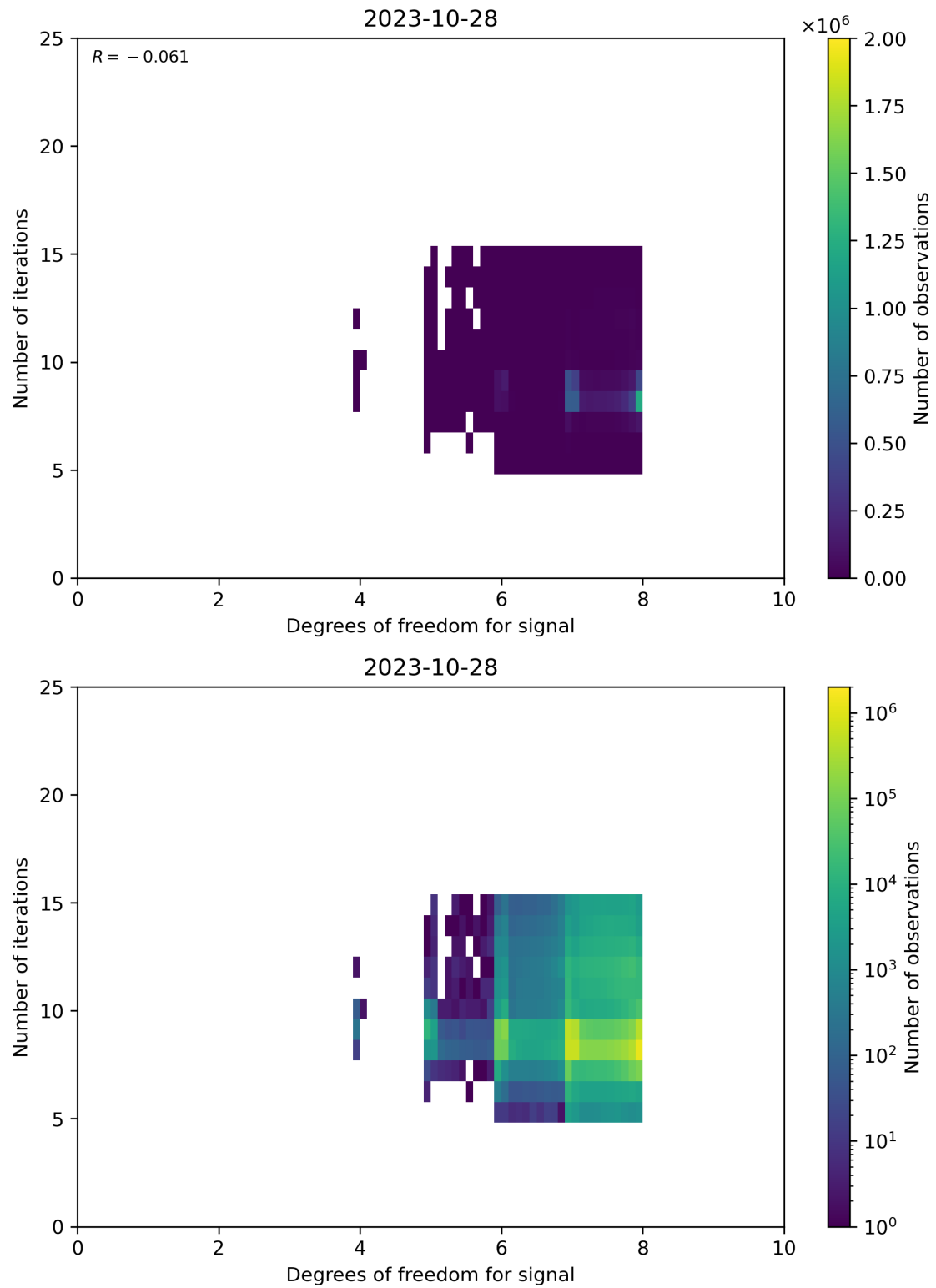
Figure 50: Scatter density plot of “Degrees of freedom for signal” against “Number of iterations” for 2023-10-28 to 2023-10-29.
