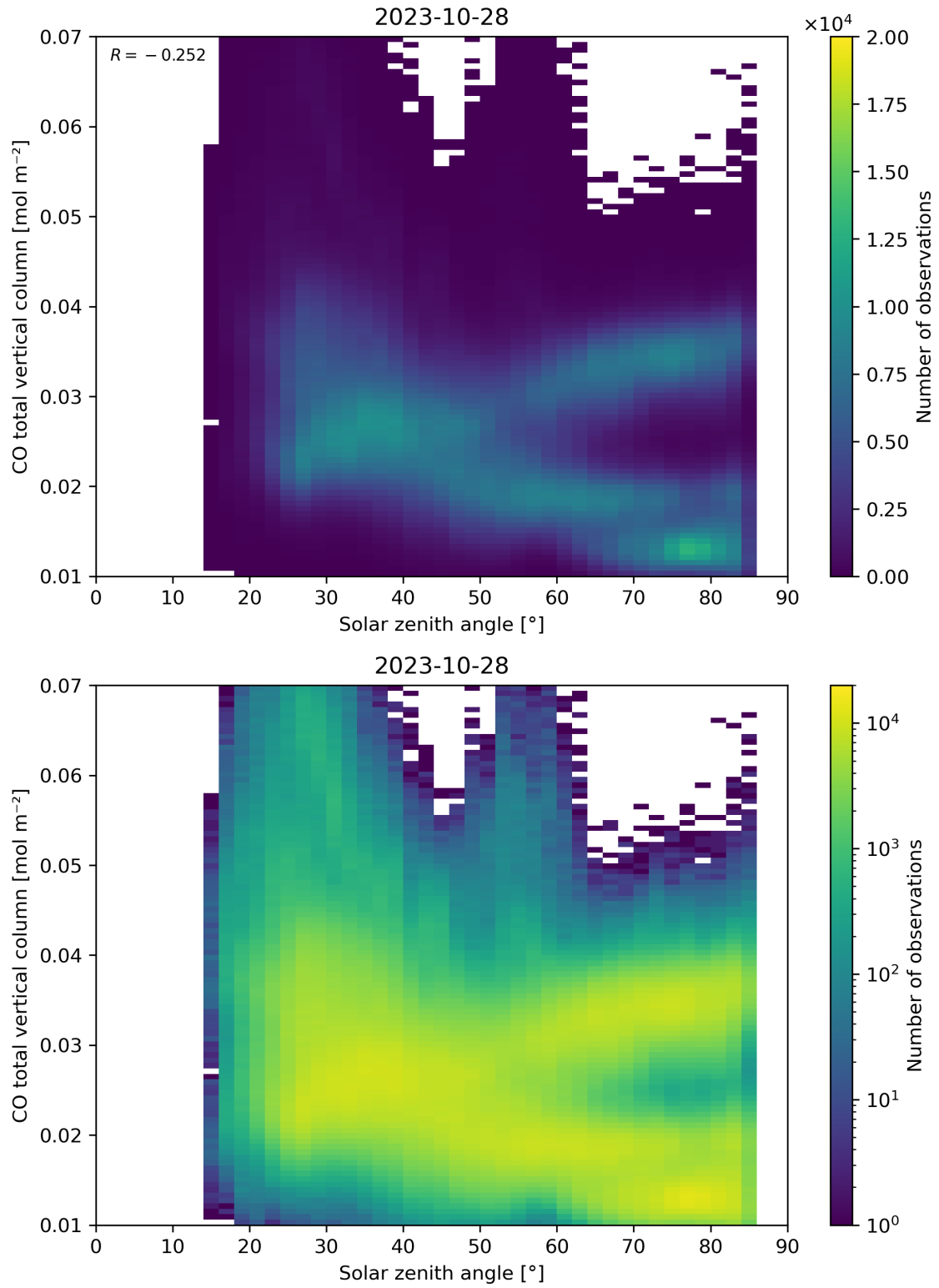
Figure 61: Scatter density plot of “Solar zenith angle” against “CO total vertical column” for 2023-10-28 to 2023-10-29.
