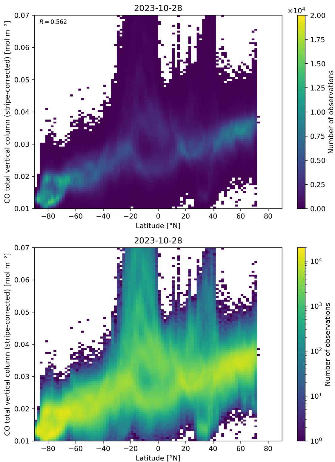
Figure 52: Scatter density plot of “Latitude” against “CO total vertical column (stripe-corrected)” for 2023-10-28 to 2023-10-29.
