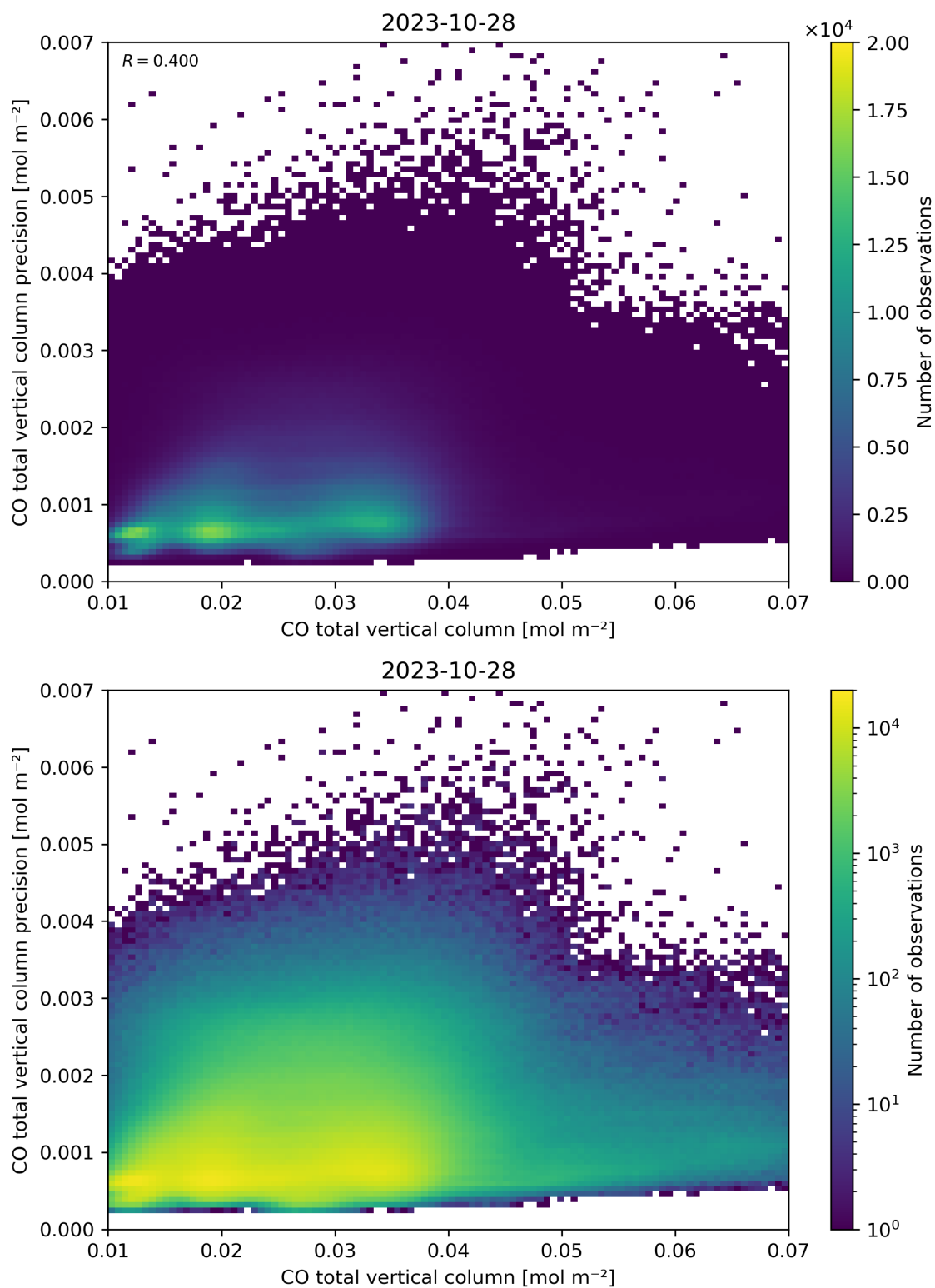
Figure 34: Scatter density plot of “CO total vertical column” against “CO total vertical column precision” for 2023-10-28 to 2023-10-29.
