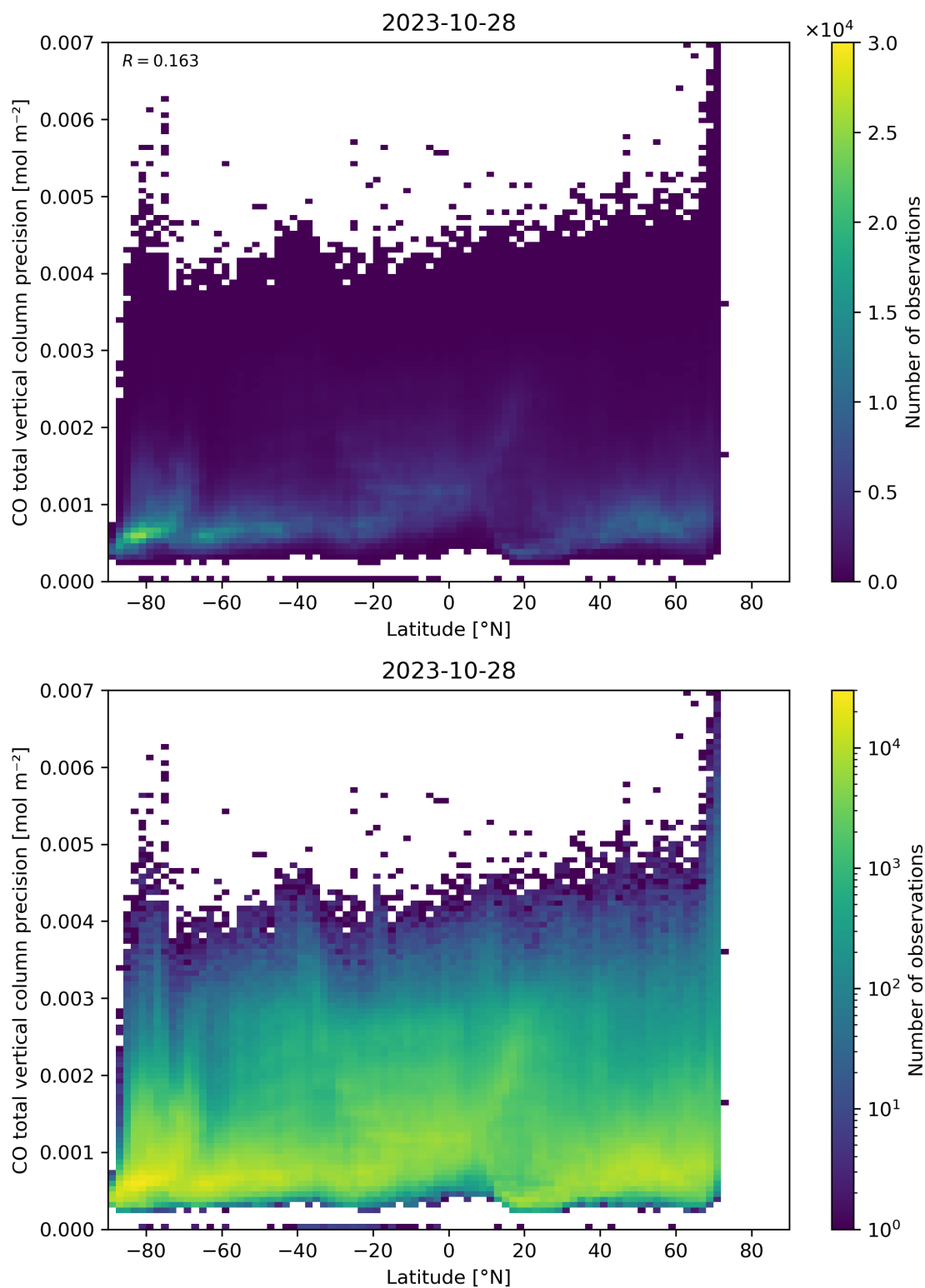
Figure 53: Scatter density plot of “Latitude” against “CO total vertical column precision” for 2023-10-28 to 2023-10-29.
