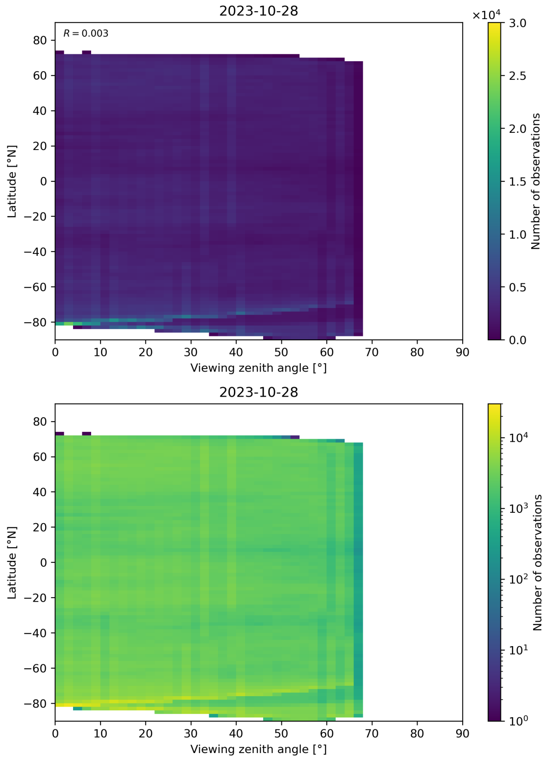
Figure 74: Scatter density plot of “Viewing zenith angle” against “Latitude” for 2023-10-28 to 2023-10-29.
