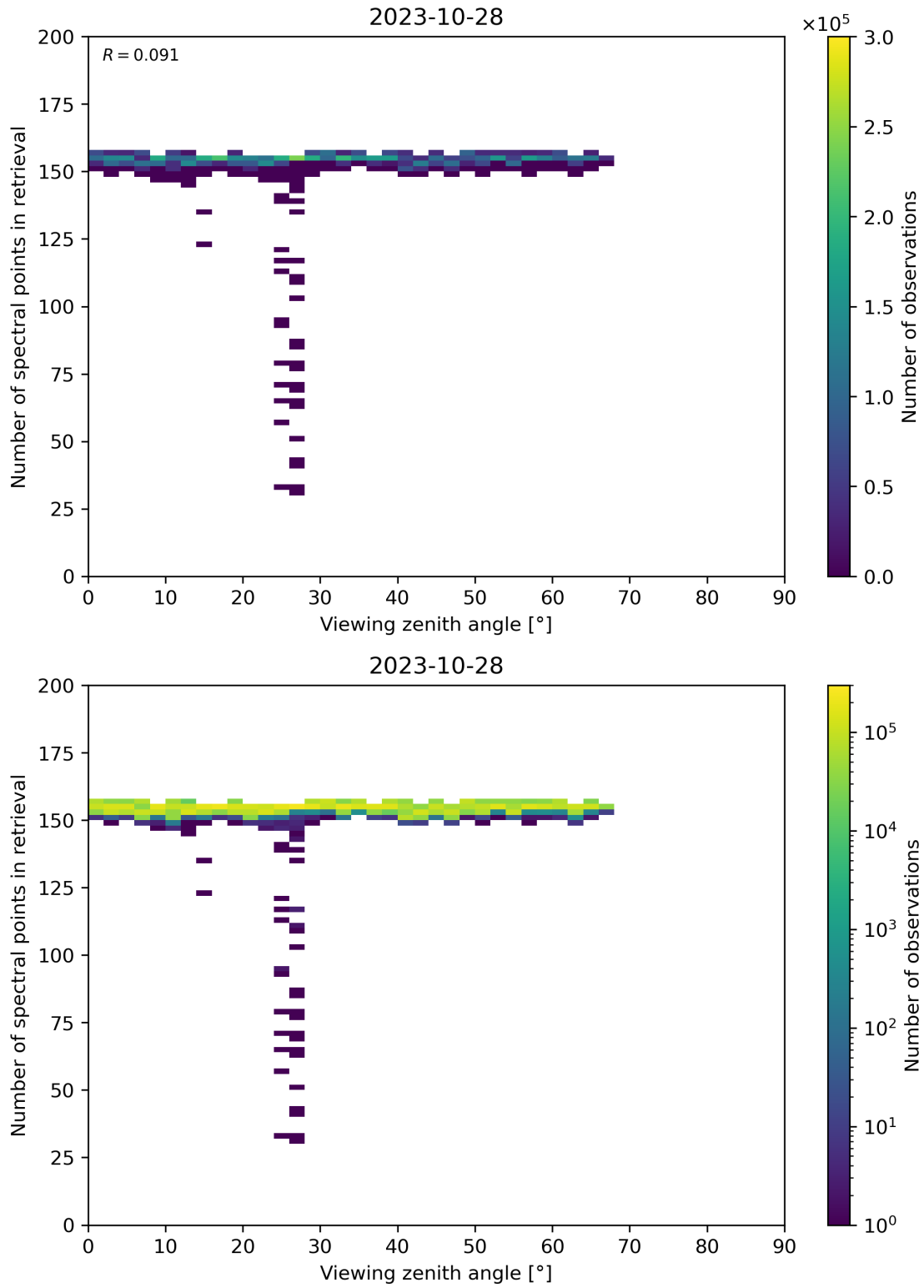
Figure 76: Scatter density plot of “Viewing zenith angle” against “Number of spectral points in retrieval” for 2023-10-28 to 2023-10-29.
