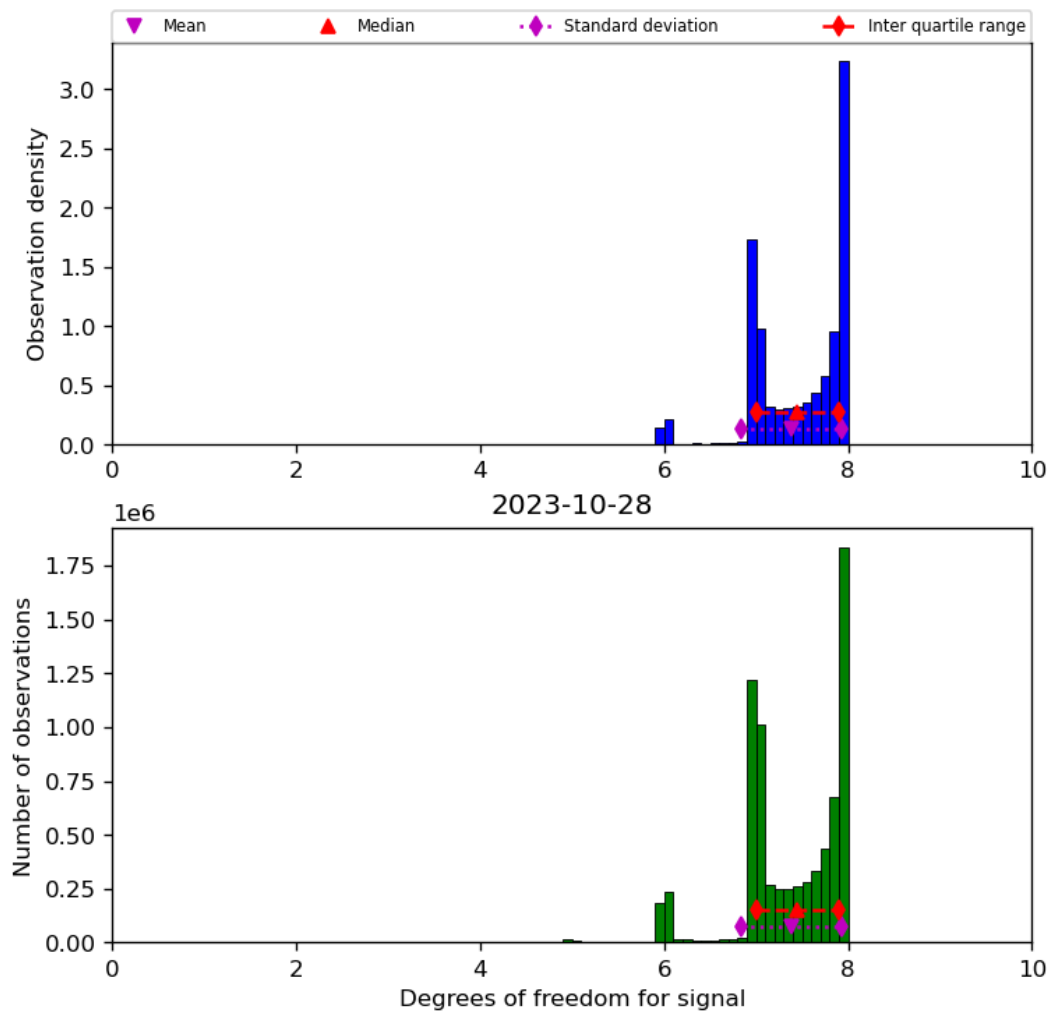
Figure 23: Histogram of “Degrees of freedom for signal” for 2023-10-28 to 2023-10-29
