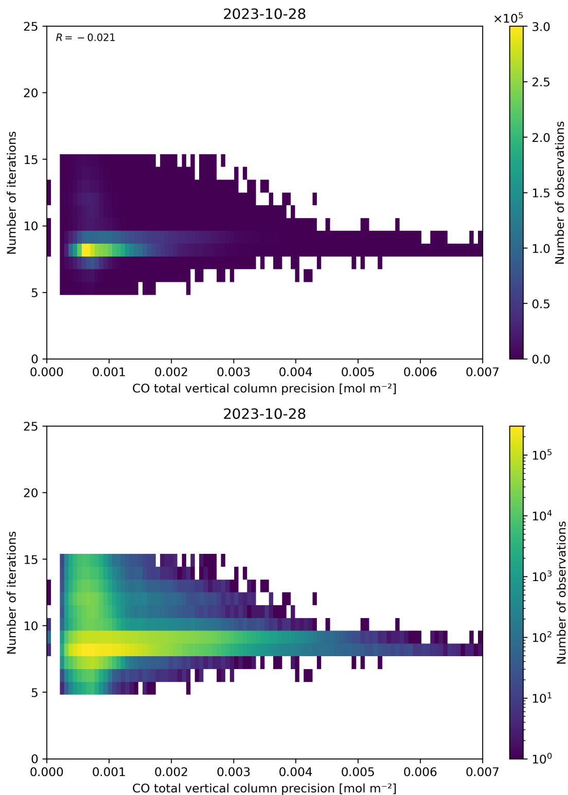
Figure 46: Scatter density plot of “CO total vertical column precision” against “Number of iterations” for 2023-10-28 to 2023-10-29.
