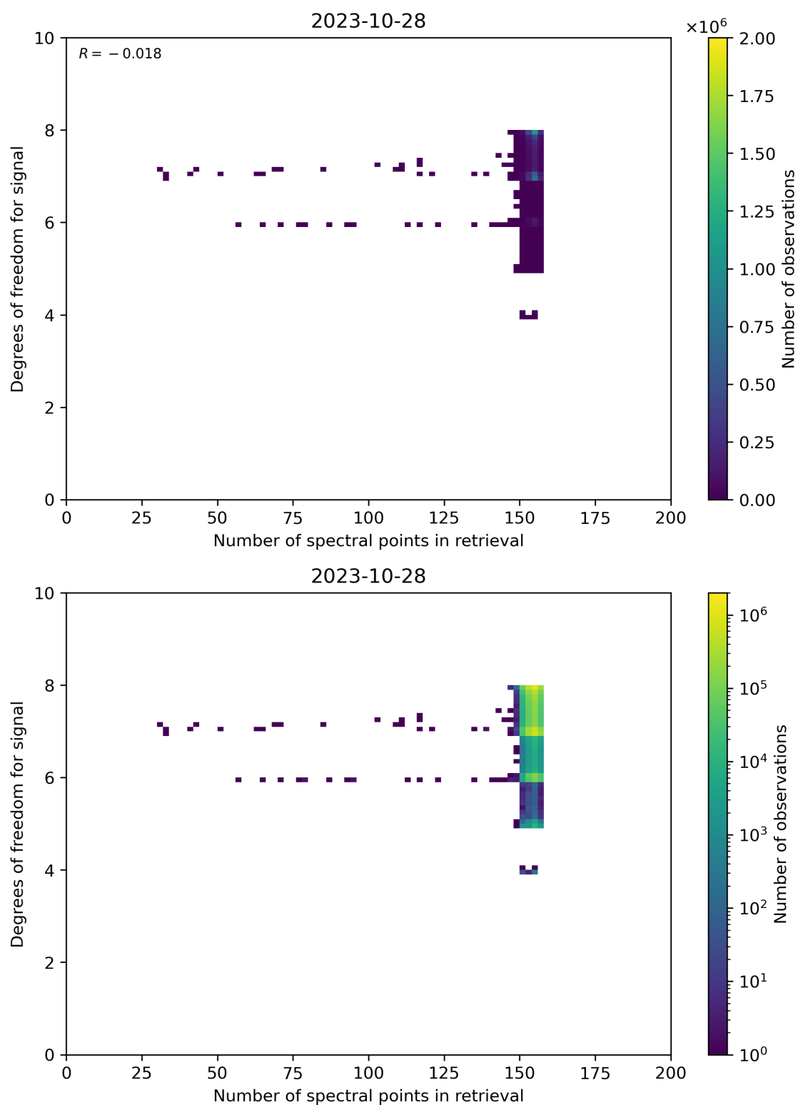
Figure 59: Scatter density plot of “Number of spectral points in retrieval” against “Degrees of freedom for signal” for 2023-10-28 to 2023-10-29.
