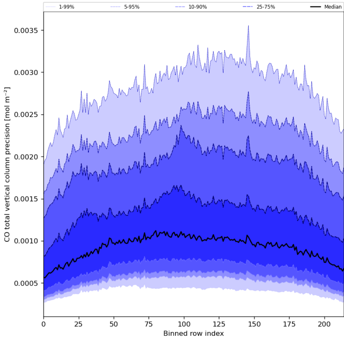
Figure 28: Along track statistics of “CO total vertical column precision” for 2023-10-28 to 2023-10-29
