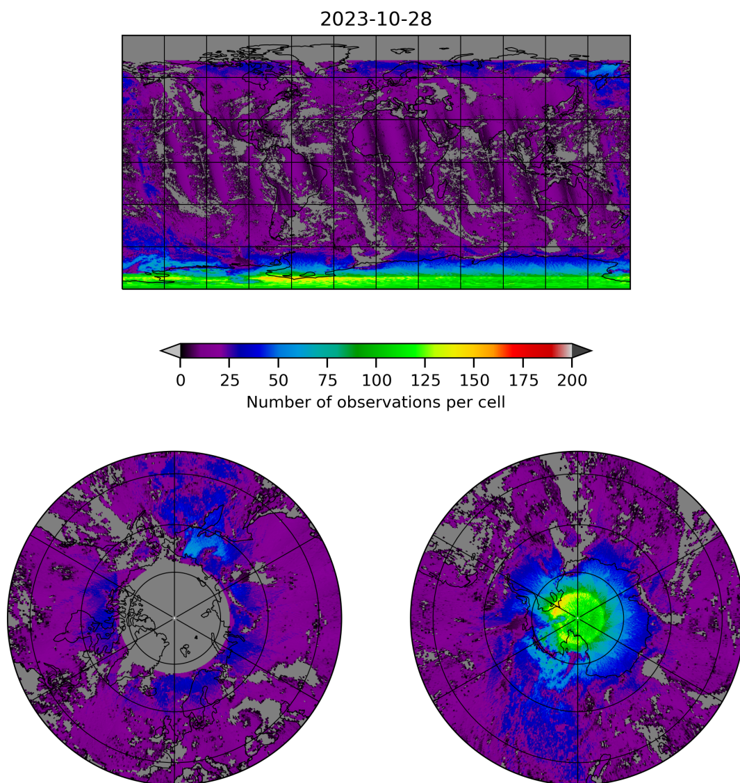
Figure 8: Map of the number of observations for 2023-10-28 to 2023-10-29
