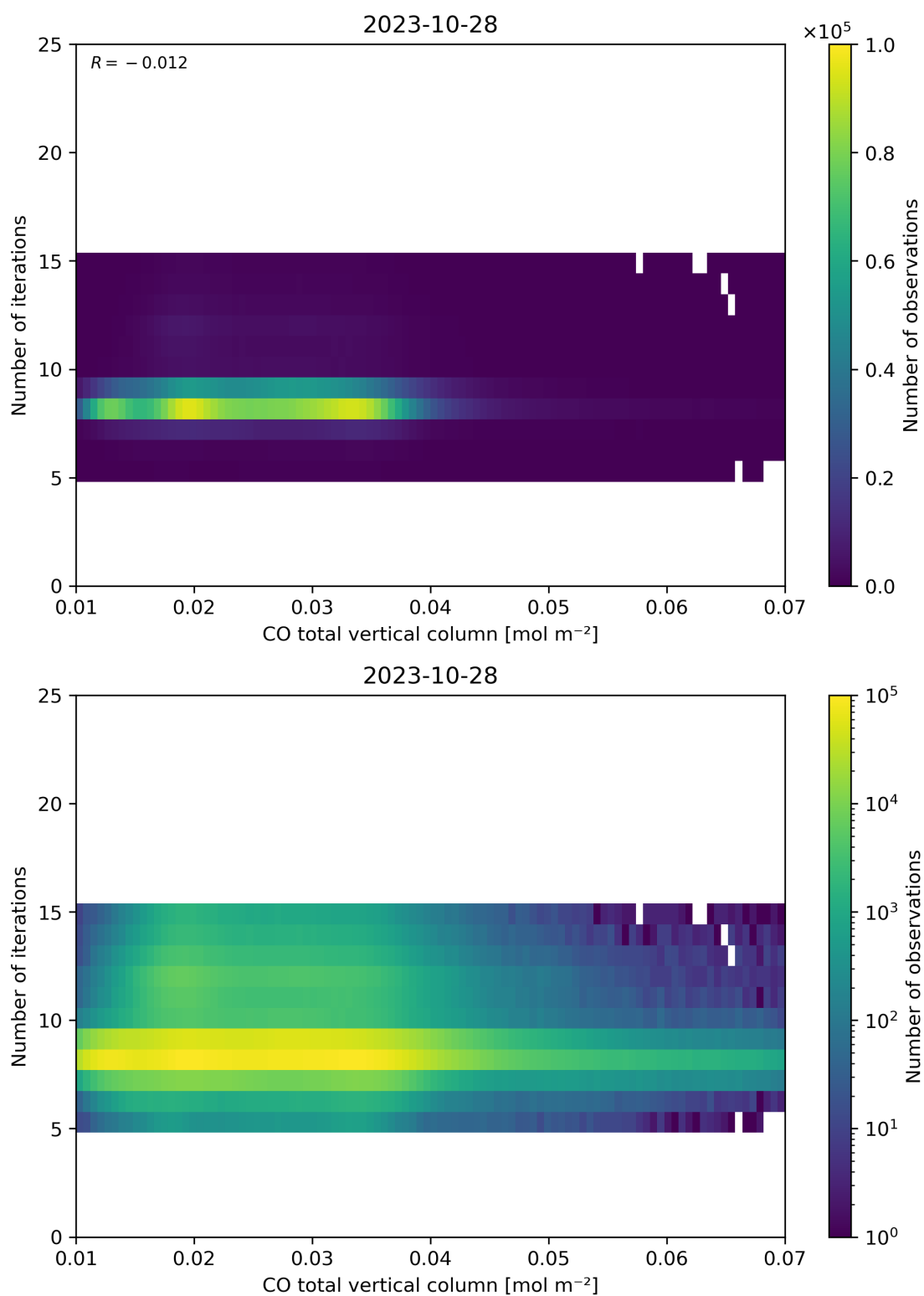
Figure 42: Scatter density plot of “CO total vertical column” against “Number of iterations” for 2023-10-28 to 2023-10-29.
