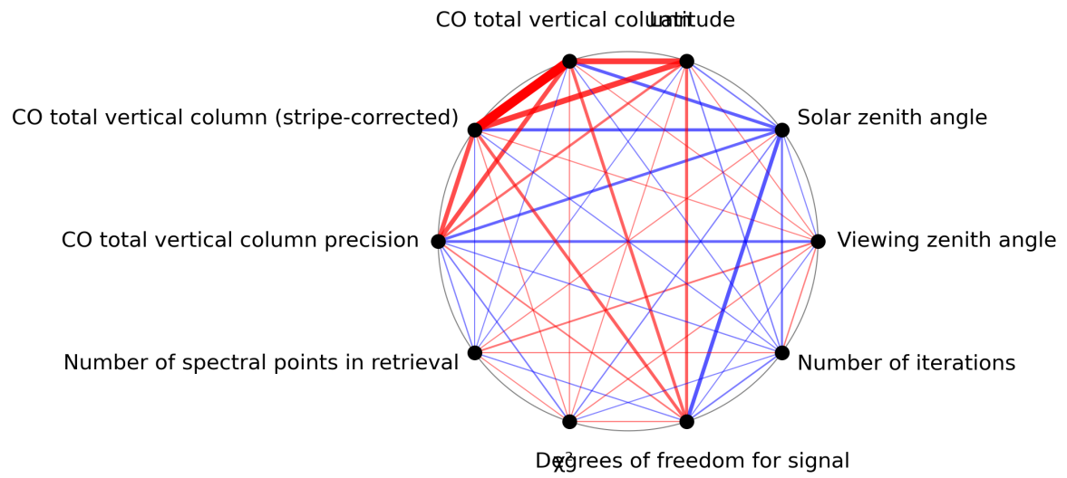
Figure 1: Map of correlation graph for 2023-10-28 to 2023-10-29.
