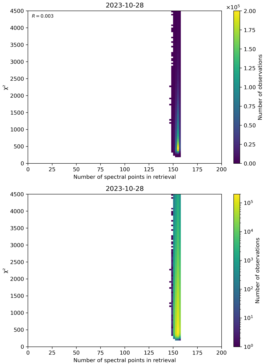
Figure 58: Scatter density plot of “Number of spectral points in retrieval” against “ \chi^2 ” for 2023-10-28 to 2023-10-29.
