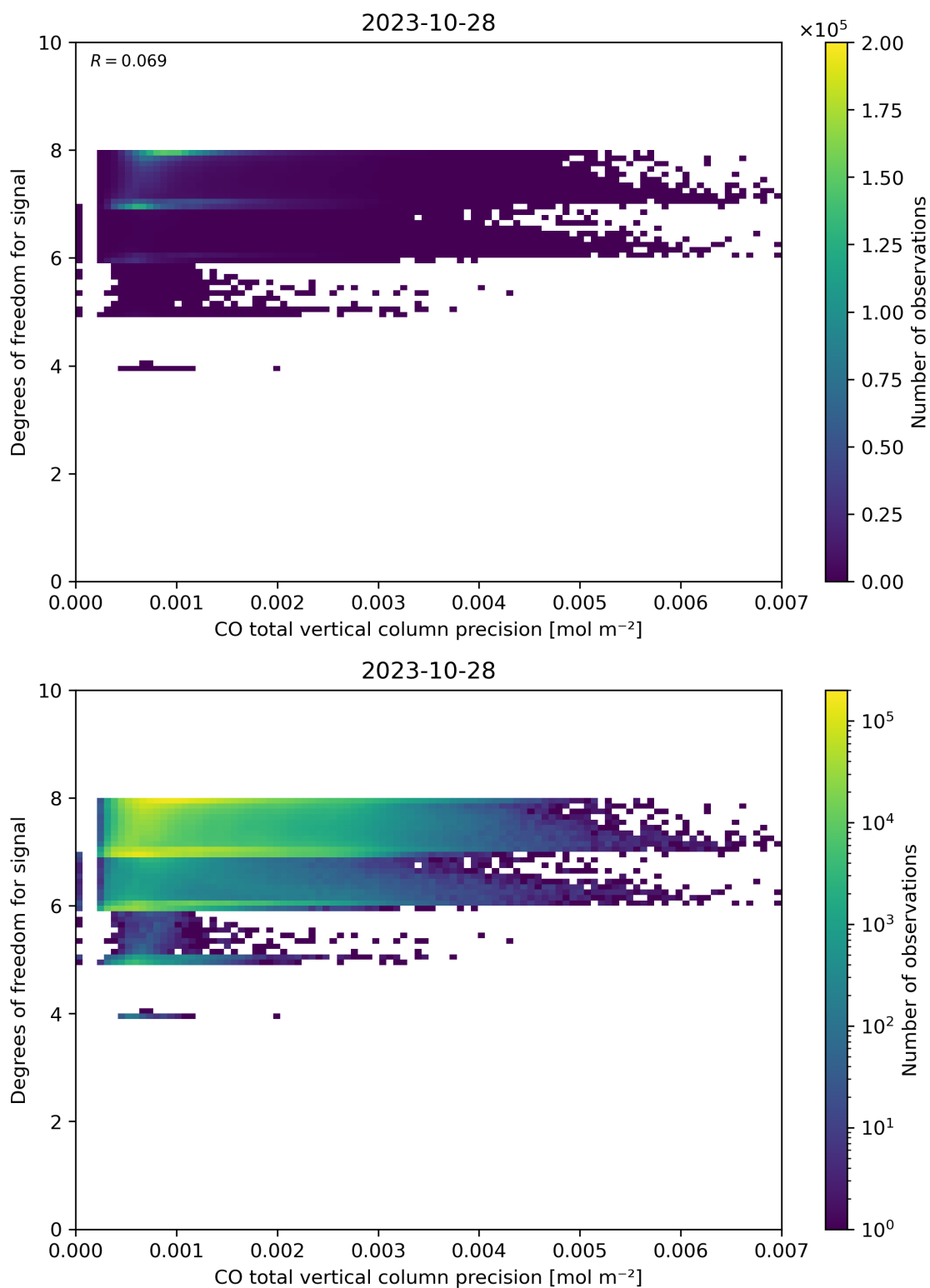
Figure 45: Scatter density plot of “CO total vertical column precision” against “Degrees of freedom for signal” for 2023-10-28 to 2023-10-29.
