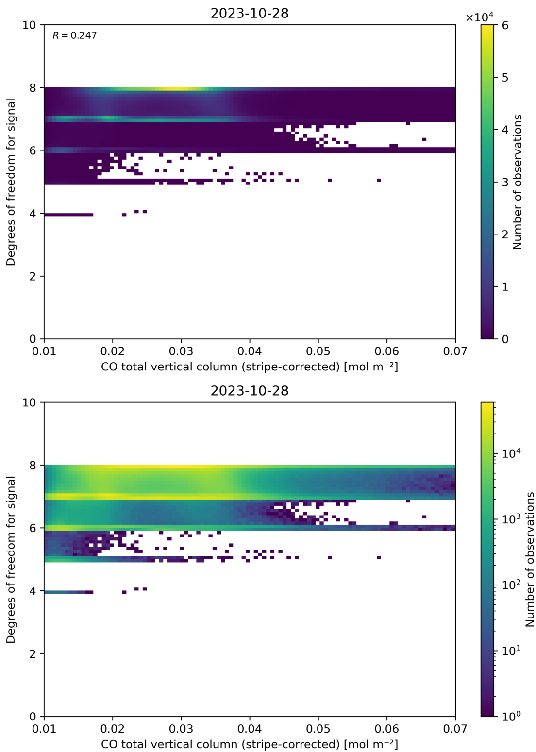
Figure 38: Scatter density plot of “CO total vertical column (stripe-corrected)” against “Degrees of freedom for signal” for 2023-10-28 to 2023-10-29.
