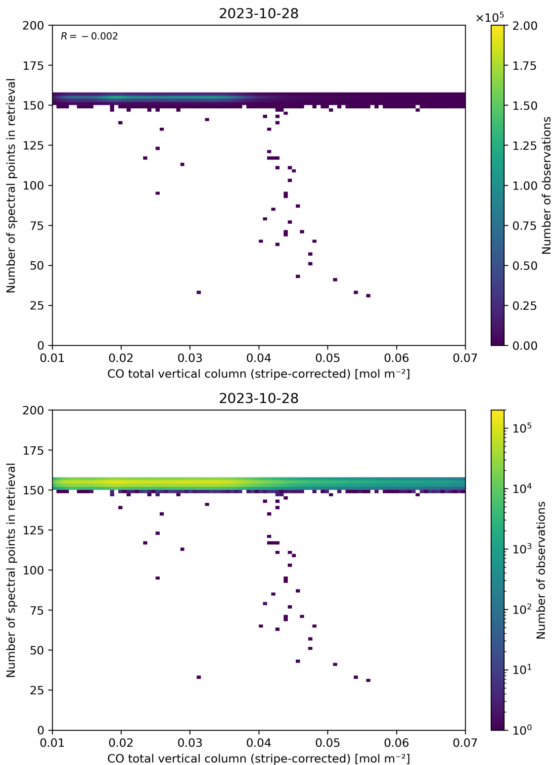
Figure 40: Scatter density plot of “CO total vertical column (stripe-corrected)” against “Number of spectral points in retrieval” for 2023-10-28 to 2023-10-29.
