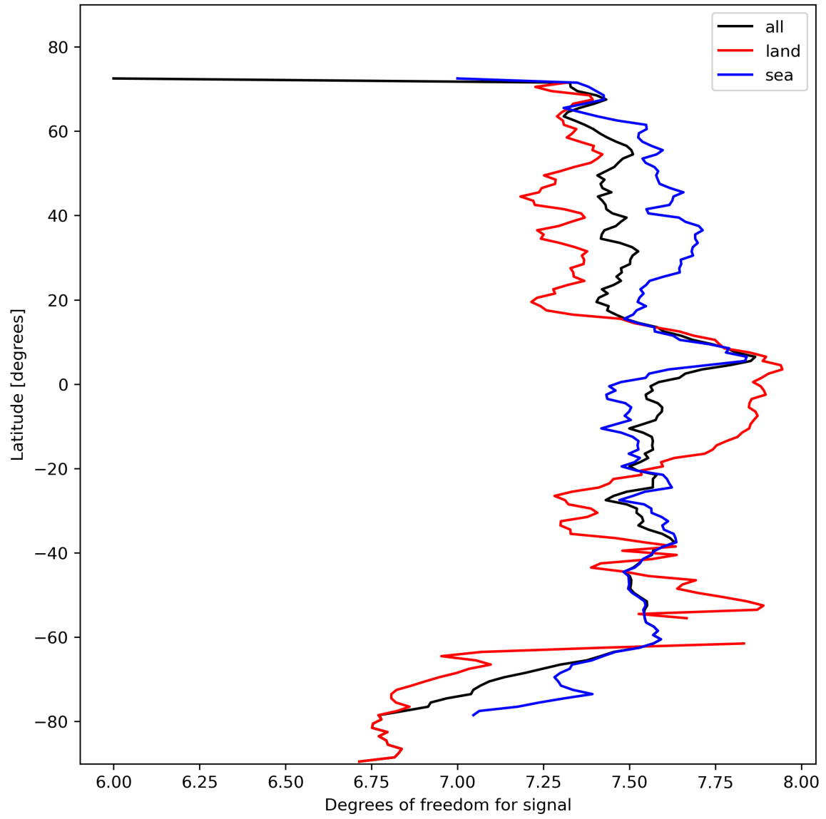
Figure 15: Zonal average of “Degrees of freedom for signal” for 2023-10-28 to 2023-10-29.
