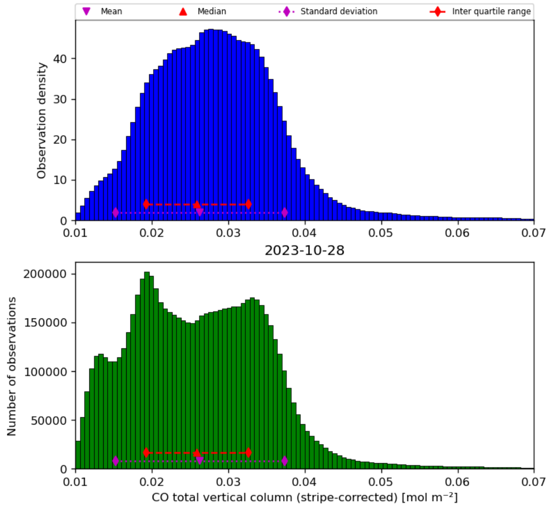
Figure 19: Histogram of “CO total vertical column (stripe-corrected)” for 2023-10-28 to 2023-10-29
