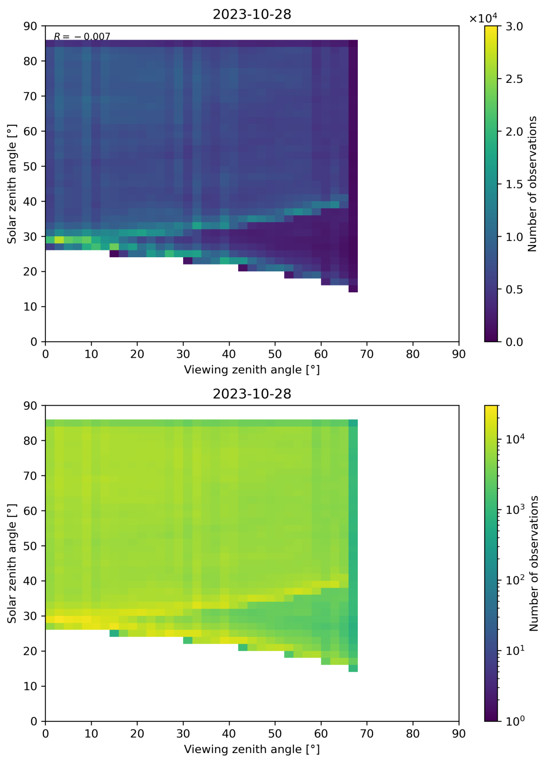
Figure 77: Scatter density plot of “Viewing zenith angle” against “Solar zenith angle” for 2023-10-28 to 2023-10-29.
