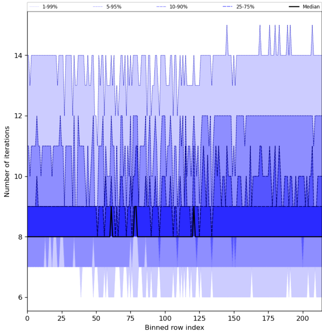
Figure 32: Along track statistics of “Number of iterations” for 2023-10-28 to 2023-10-29
