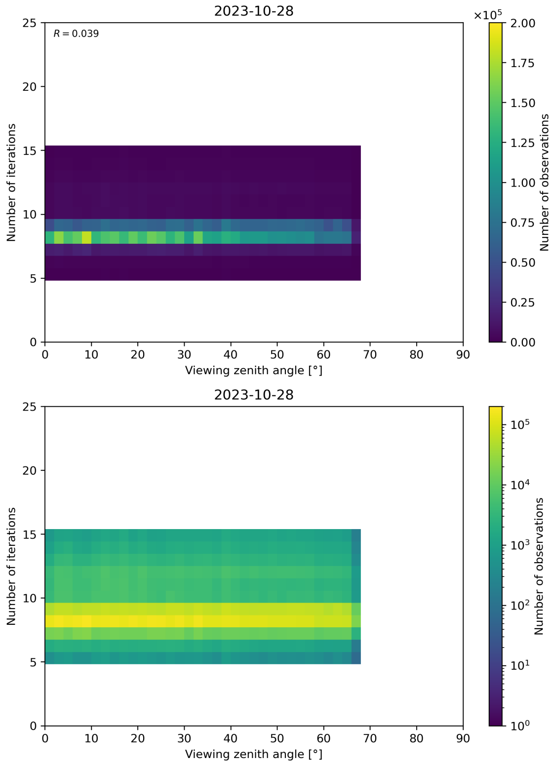
Figure 75: Scatter density plot of “Viewing zenith angle” against “Number of iterations” for 2023-10-28 to 2023-10-29.
