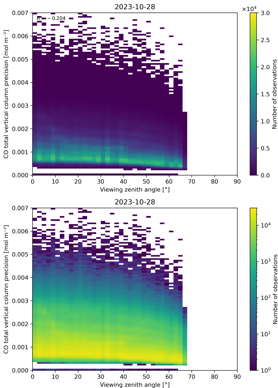
Figure 71: Scatter density plot of “Viewing zenith angle” against “CO total vertical column precision” for 2023-10-28 to 2023-10-29.
