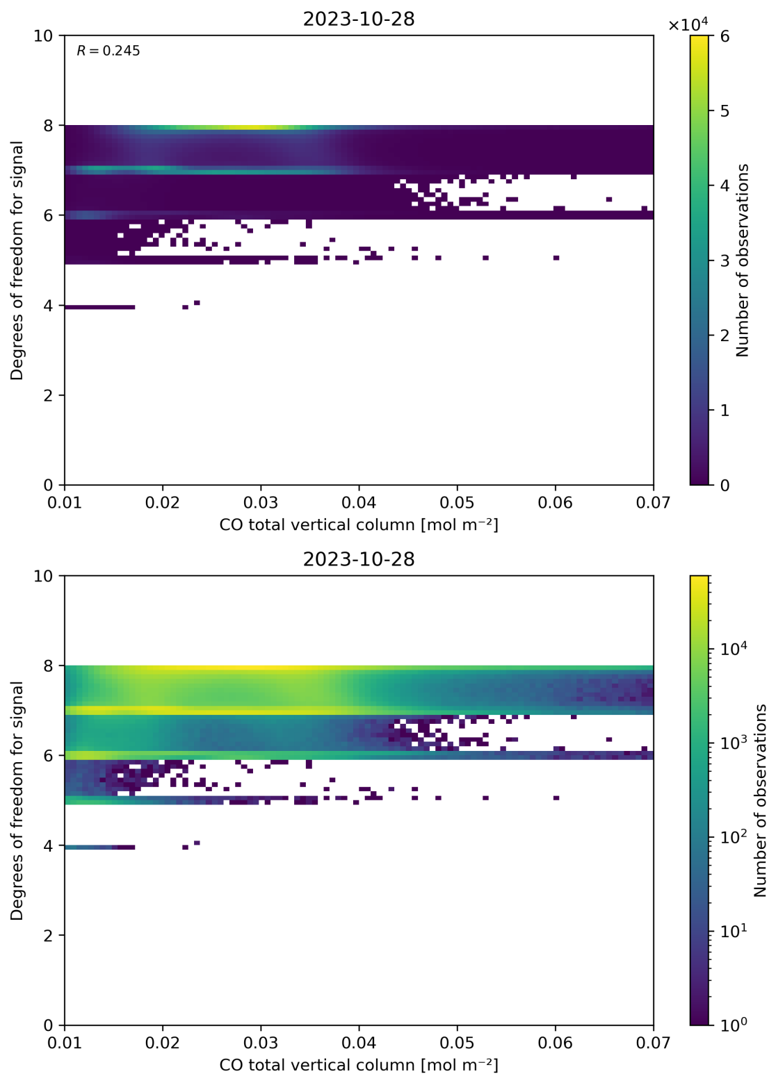
Figure 41: Scatter density plot of “CO total vertical column” against “Degrees of freedom for signal” for 2023-10-28 to 2023-10-29.
