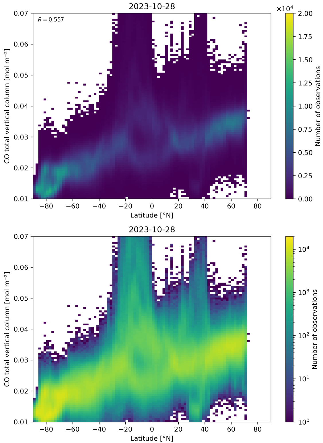
Figure 51: Scatter density plot of “Latitude” against “CO total vertical column” for 2023-10-28 to 2023-10-29.
