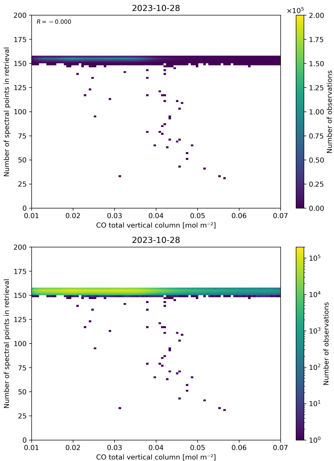
Figure 43: Scatter density plot of “CO total vertical column” against “Number of spectral points in retrieval” for 2023-10-28 to 2023-10-29.
