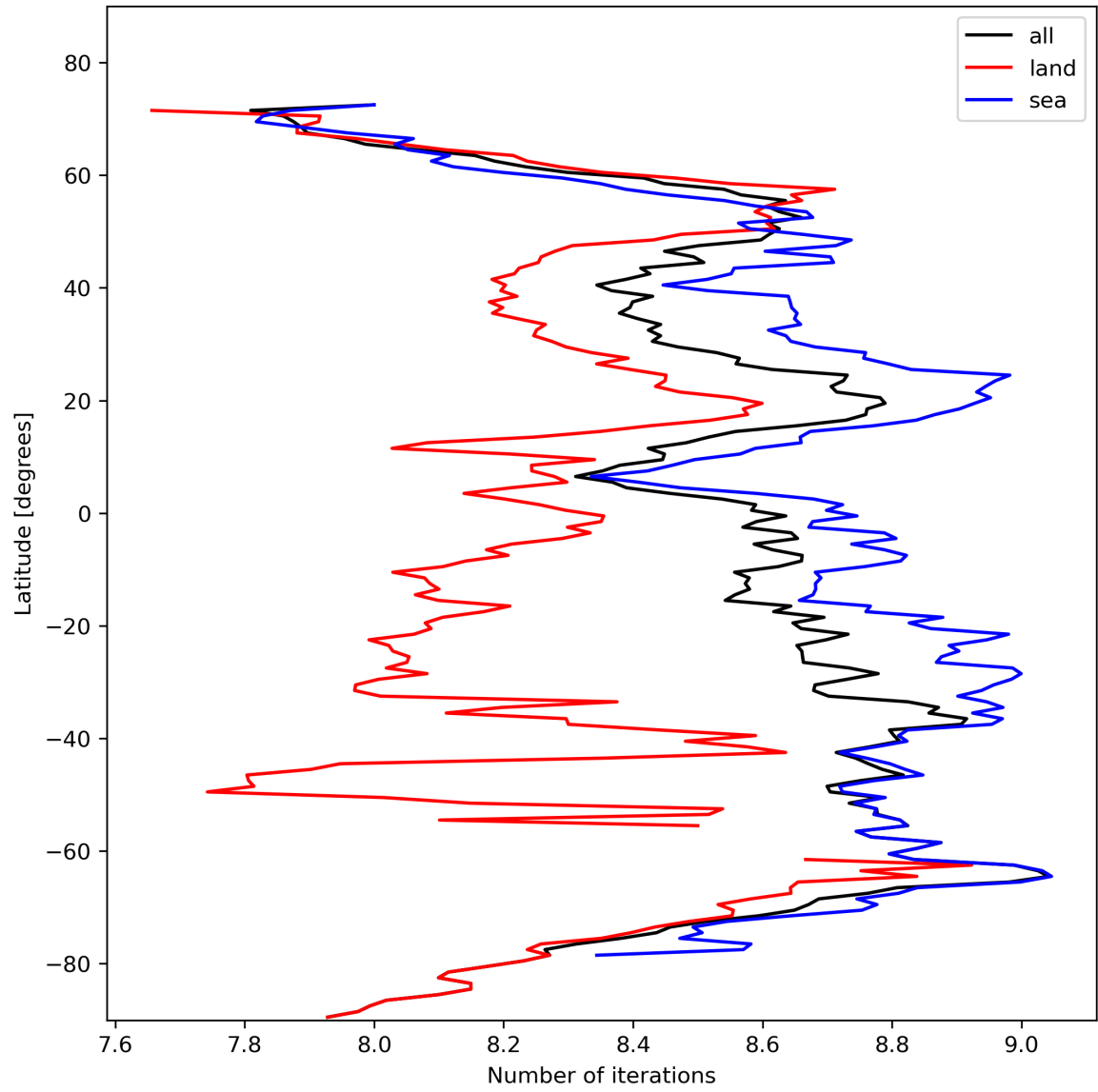
Figure 16: Zonal average of “Number of iterations” for 2023-10-28 to 2023-10-29.
