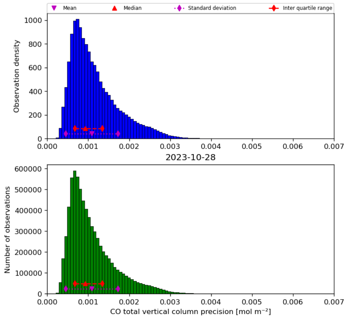
Figure 20: Histogram of “CO total vertical column precision” for 2023-10-28 to 2023-10-29
