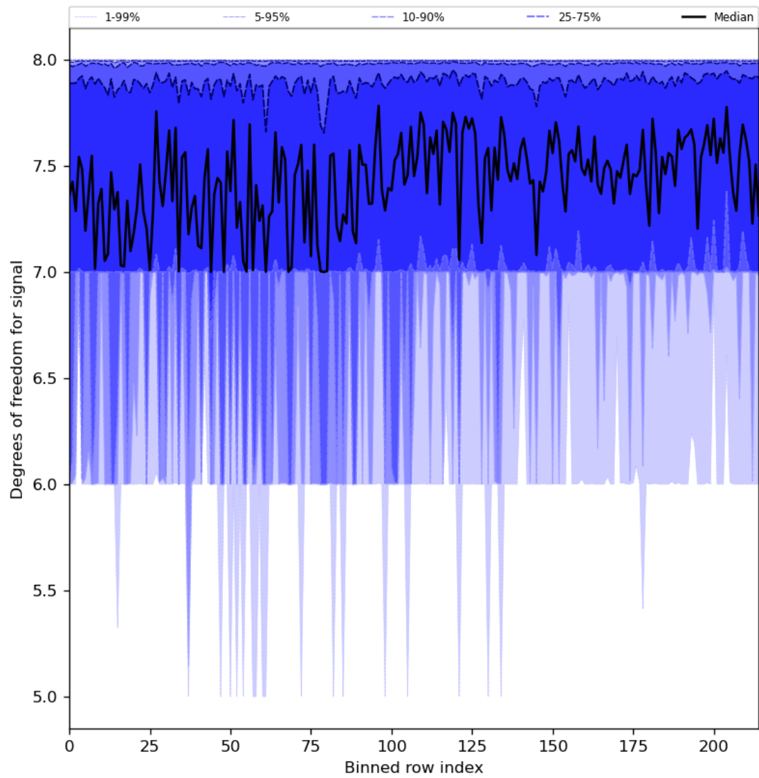
Figure 31: Along track statistics of “Degrees of freedom for signal” for 2023-10-28 to 2023-10-29
