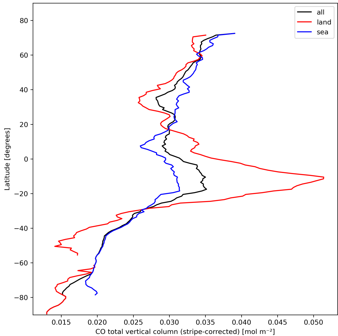
Figure 11: Zonal average of “CO total vertical column (stripe-corrected)” for 2023-10-28 to 2023-10-29.
