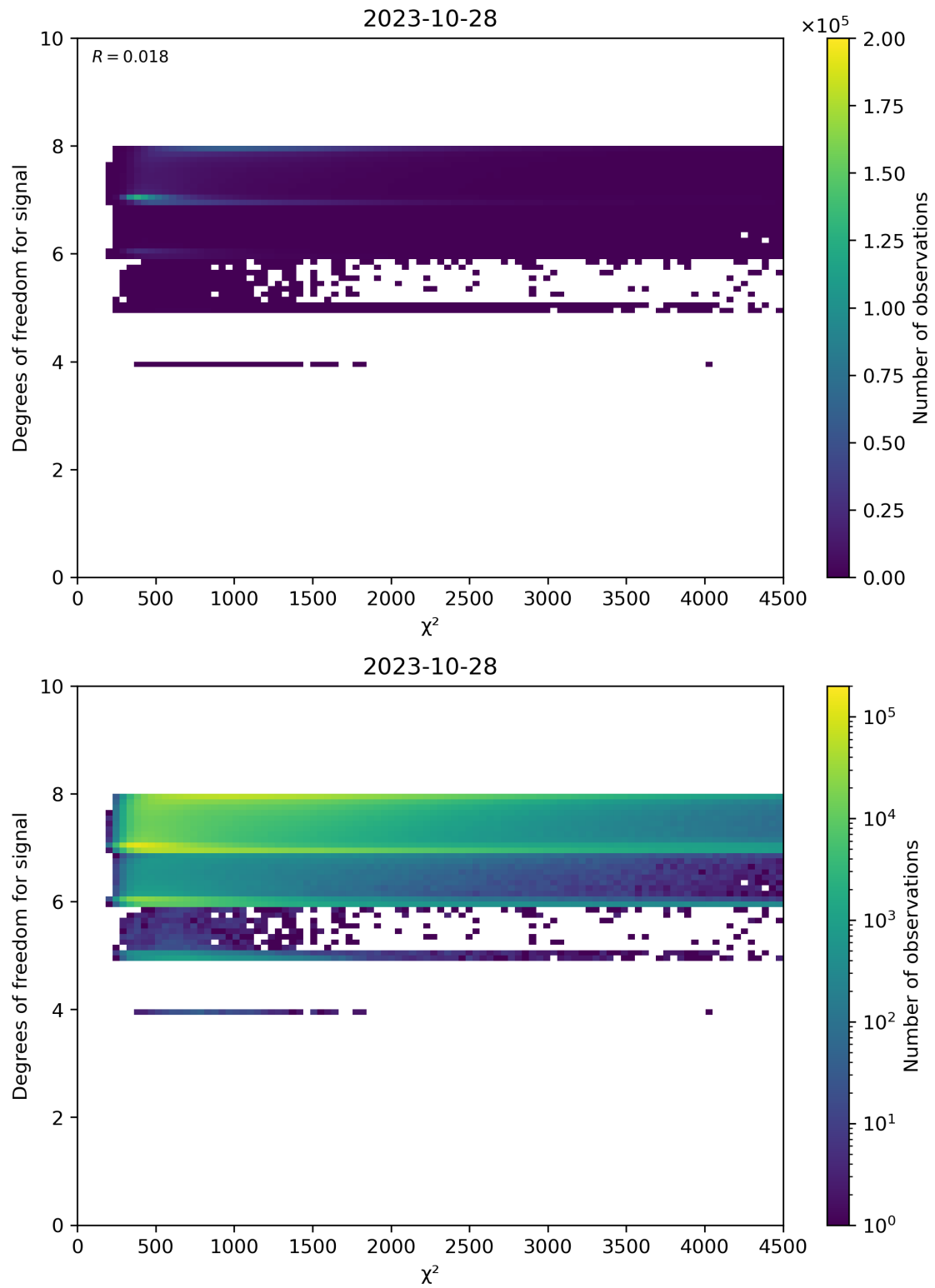
Figure 48: Scatter density plot of “ \chi^2 ” against “Degrees of freedom for signal” for 2023-10-28 to 2023-10-29.
