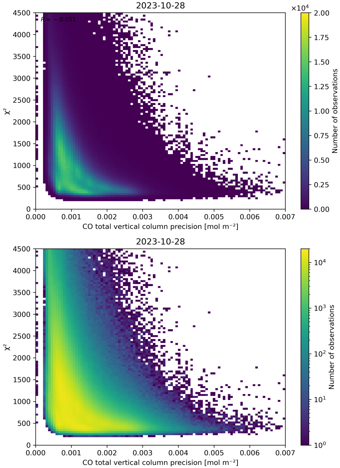
Figure 44: Scatter density plot of “CO total vertical column precision” against “ \chi^2 ” for 2023-10-28 to 2023-10-29.
