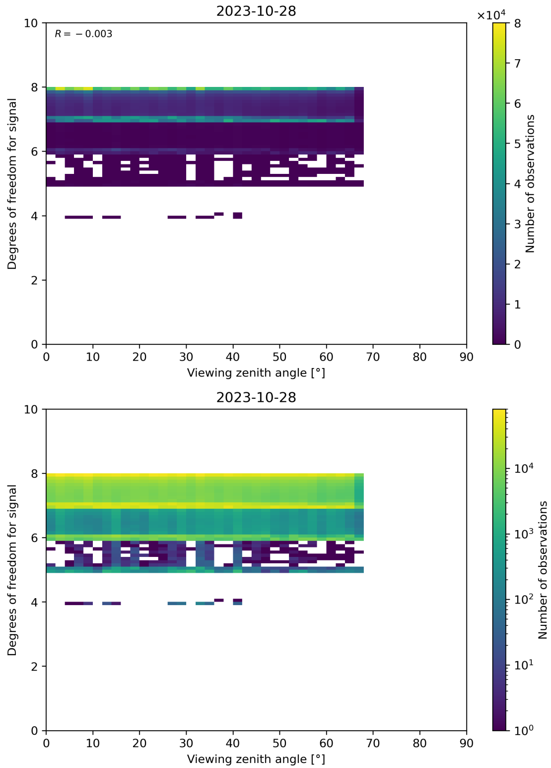
Figure 73: Scatter density plot of “Viewing zenith angle” against “Degrees of freedom for signal” for 2023-10-28 to 2023-10-29.
