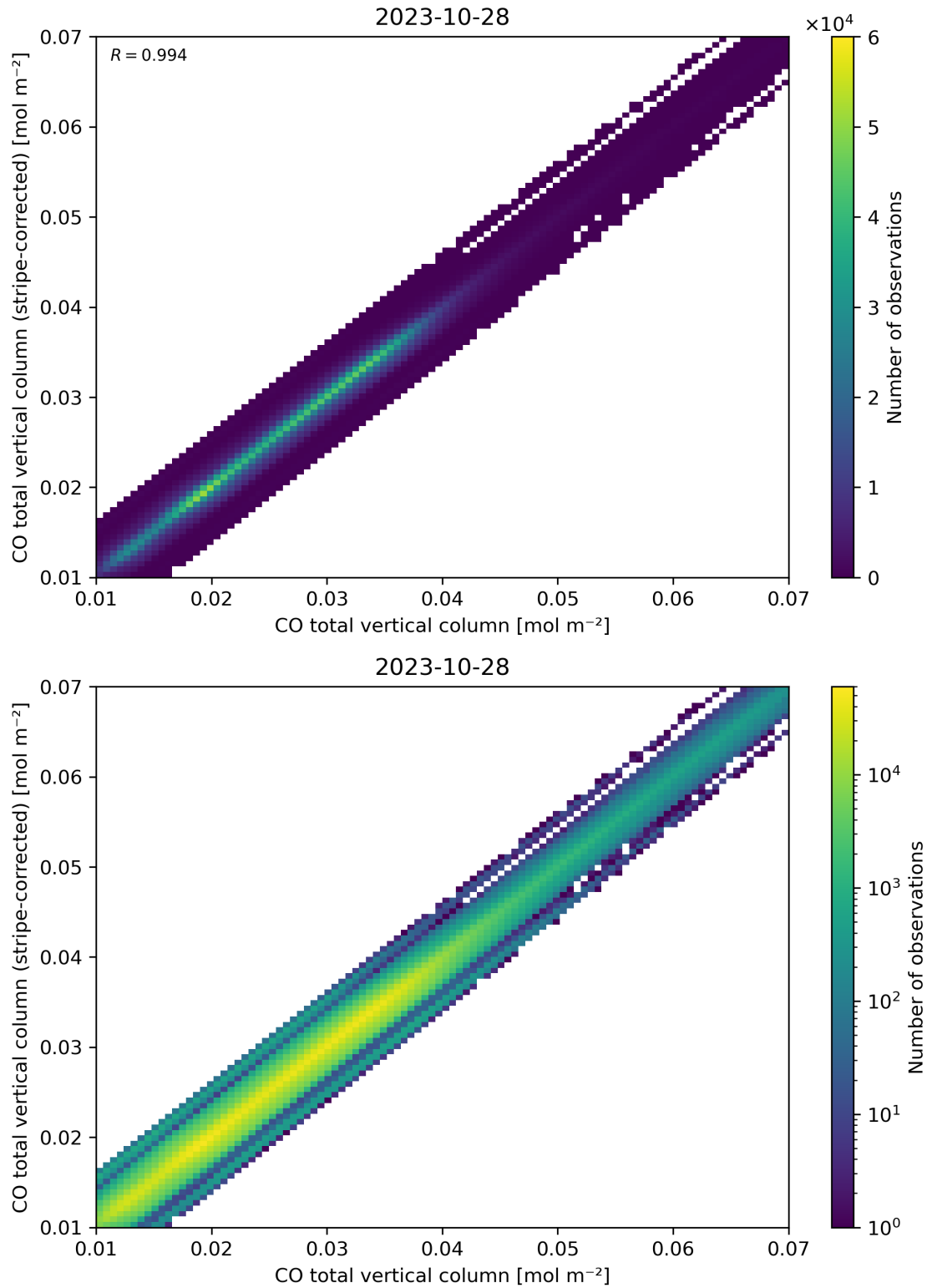
Figure 33: Scatter density plot of “CO total vertical column” against “CO total vertical column (stripe-corrected)” for 2023-10-28 to 2023-10-29.
