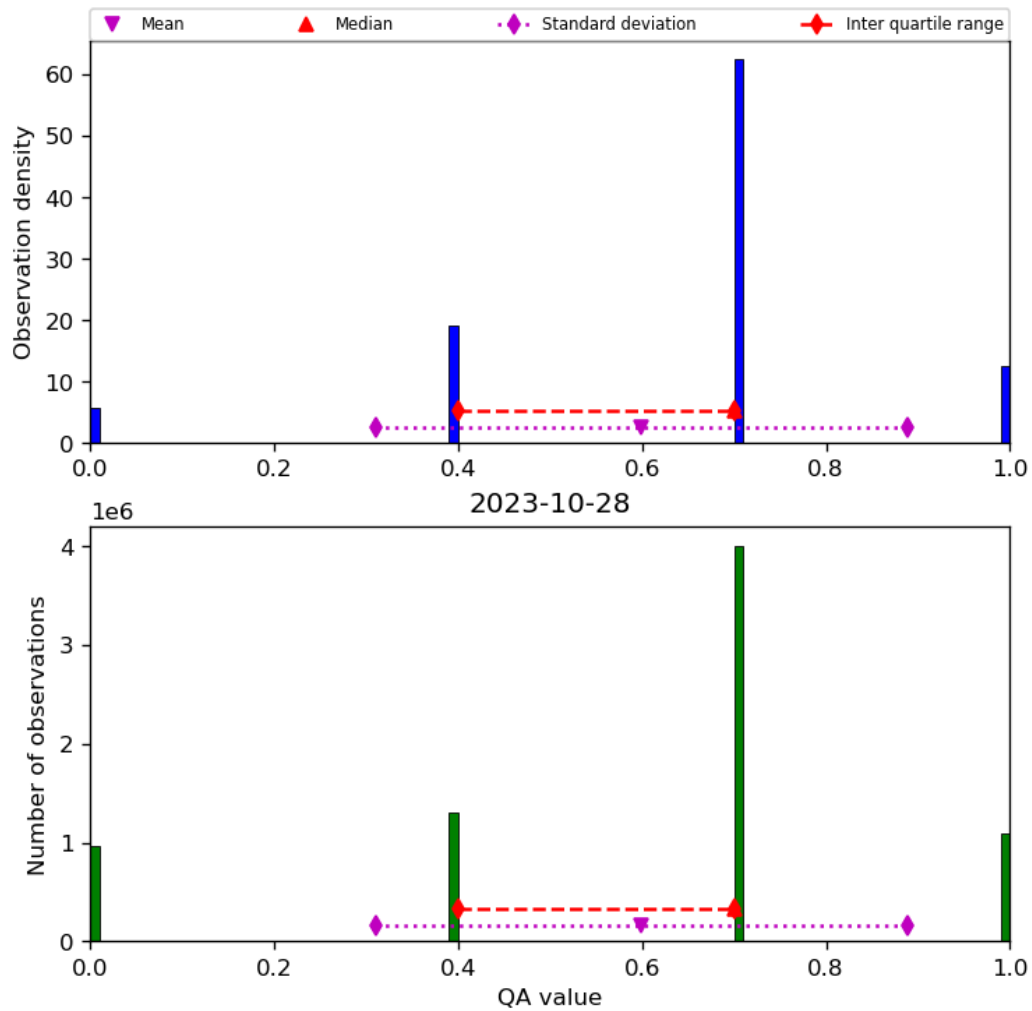
Figure 17: Histogram of “QA value” for 2023-10-28 to 2023-10-29
