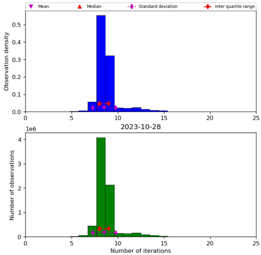
Figure 24: Histogram of “Number of iterations” for 2023-10-28 to 2023-10-29
