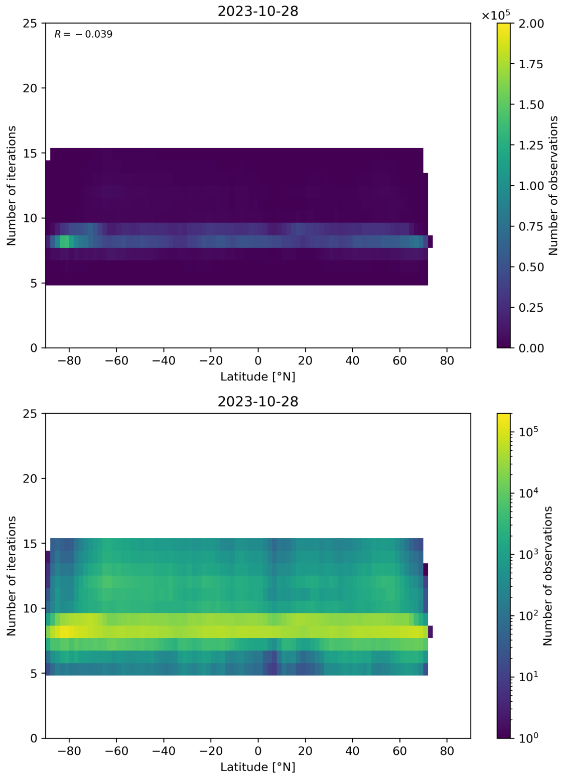
Figure 56: Scatter density plot of “Latitude” against “Number of iterations” for 2023-10-28 to 2023-10-29.
