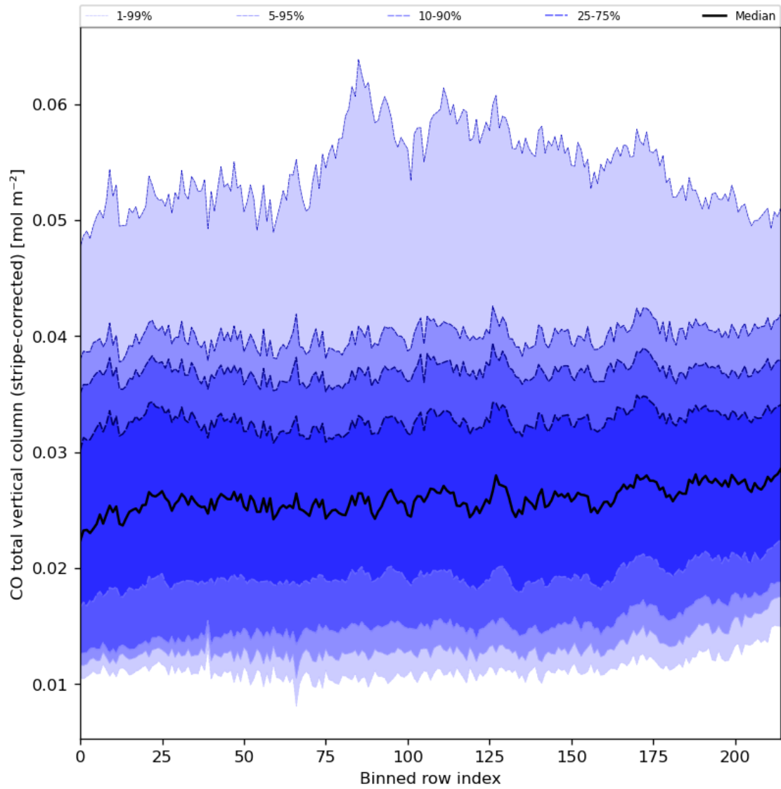
Figure 27: Along track statistics of “CO total vertical column (stripe-corrected)” for 2023-10-28 to 2023-10-29
