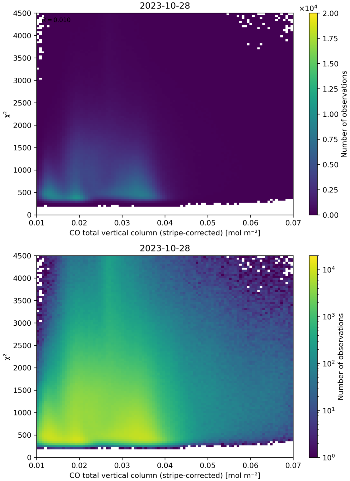
Figure 37: Scatter density plot of “CO total vertical column (stripe-corrected)” against “ \chi^2 ” for 2023-10-28 to 2023-10-29.
