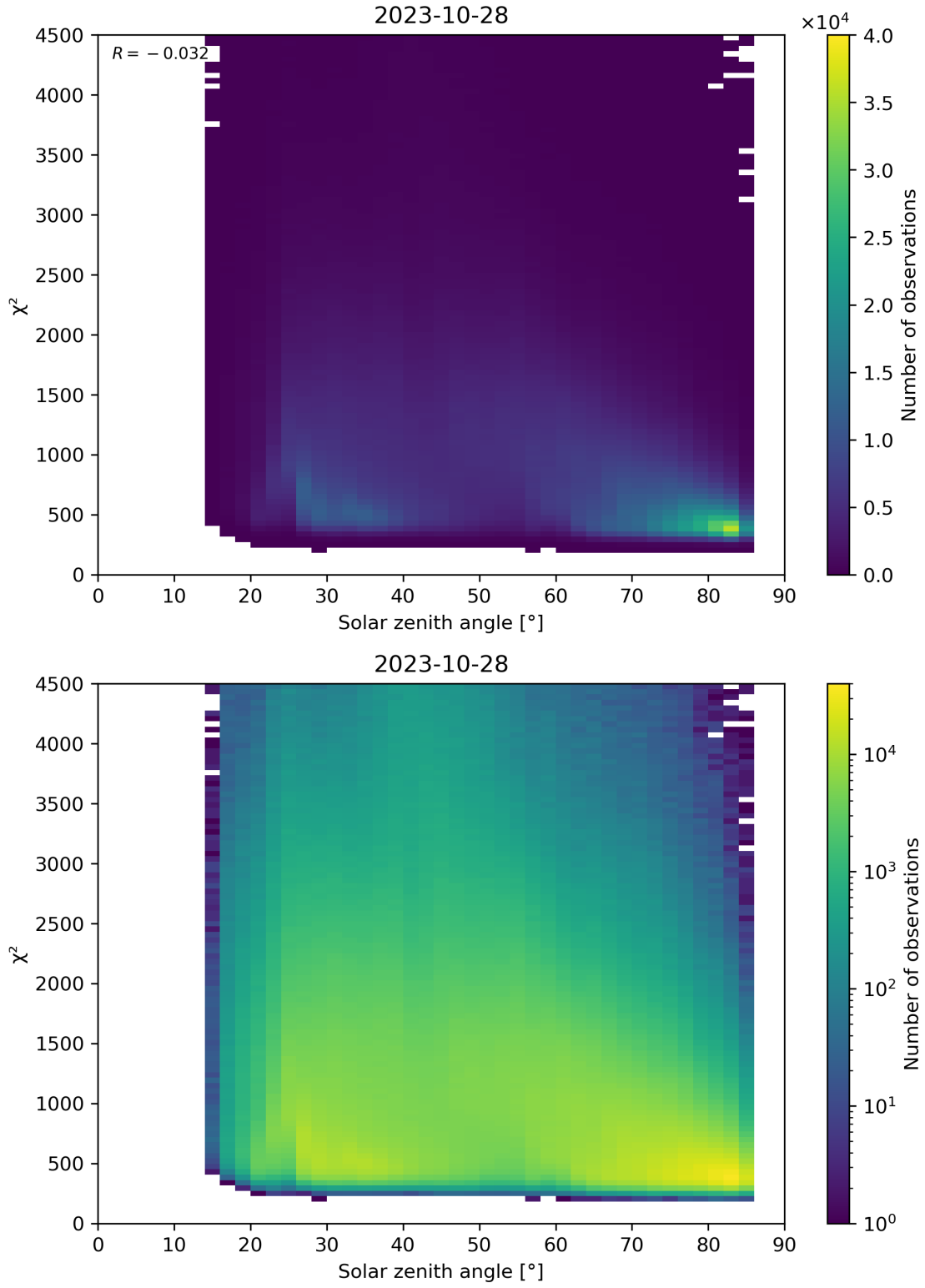
Figure 64: Scatter density plot of “Solar zenith angle” against “ \chi^2 ” for 2023-10-28 to 2023-10-29.
