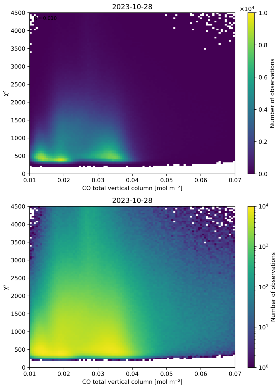
Figure 35: Scatter density plot of “CO total vertical column” against “ \chi^2 ” for 2023-10-28 to 2023-10-29.
