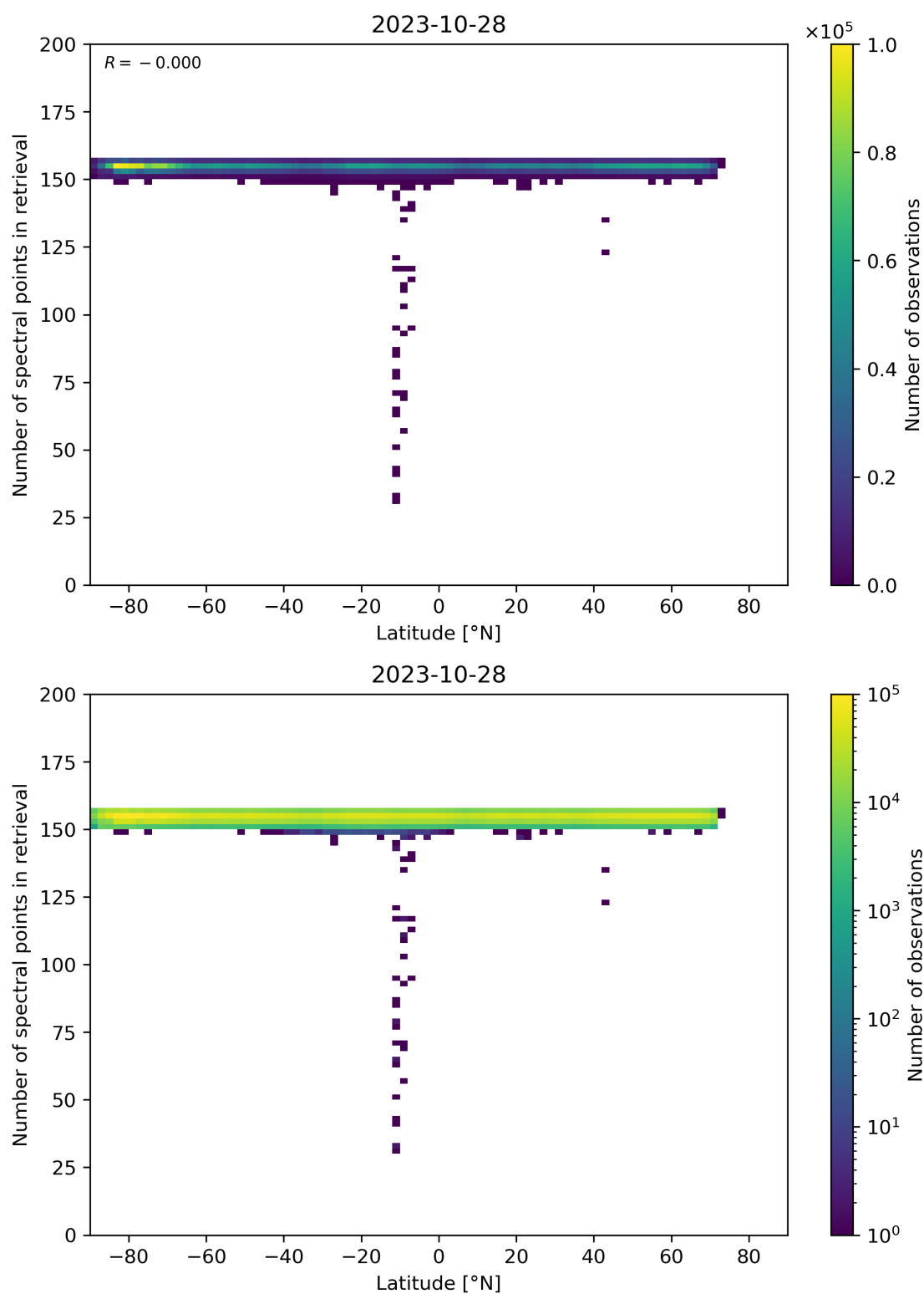
Figure 57: Scatter density plot of “Latitude” against “Number of spectral points in retrieval” for 2023-10-28 to 2023-10-29.
