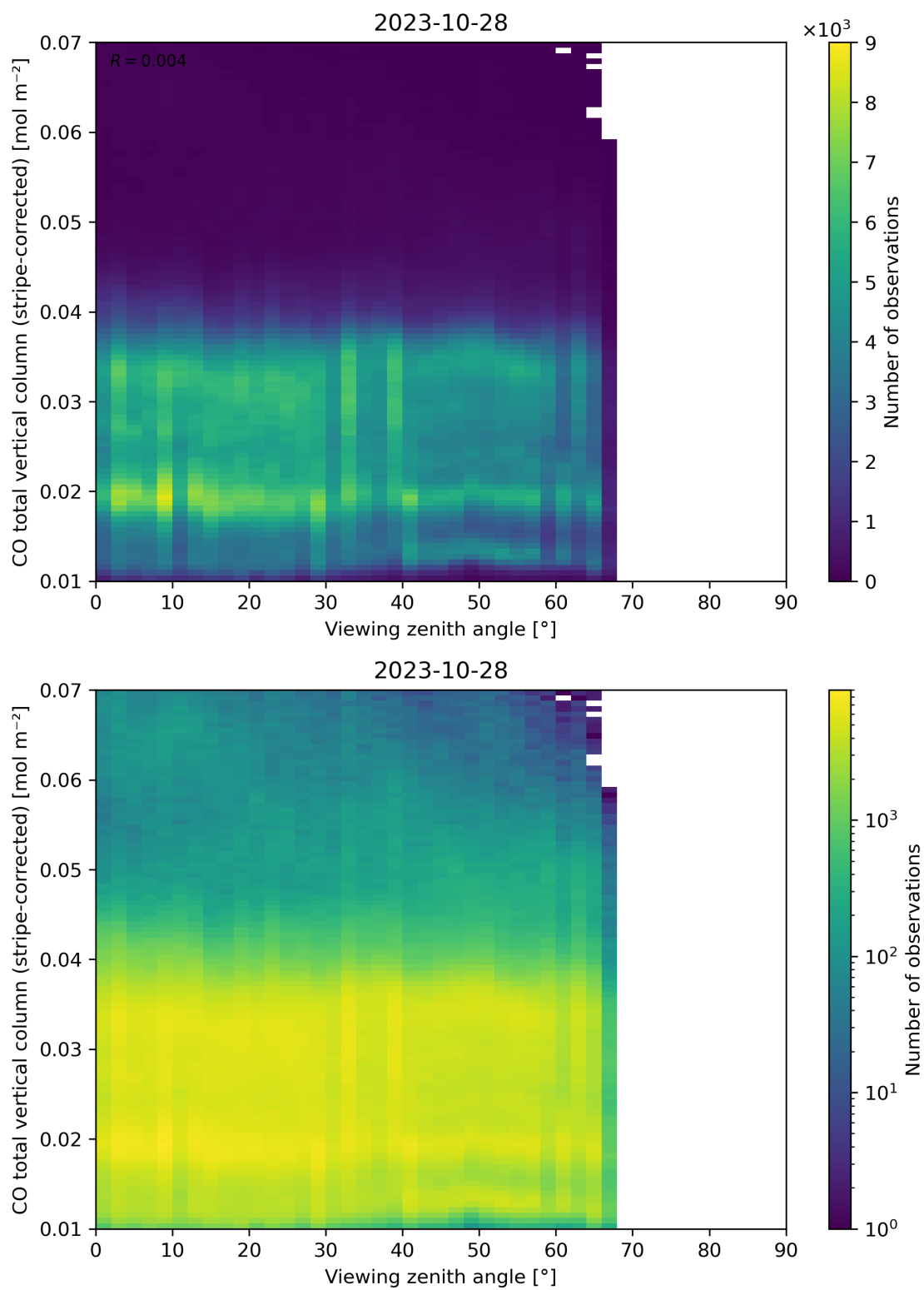
Figure 70: Scatter density plot of “Viewing zenith angle” against “CO total vertical column (stripe-corrected)” for 2023-10-28 to 2023-10-29.
