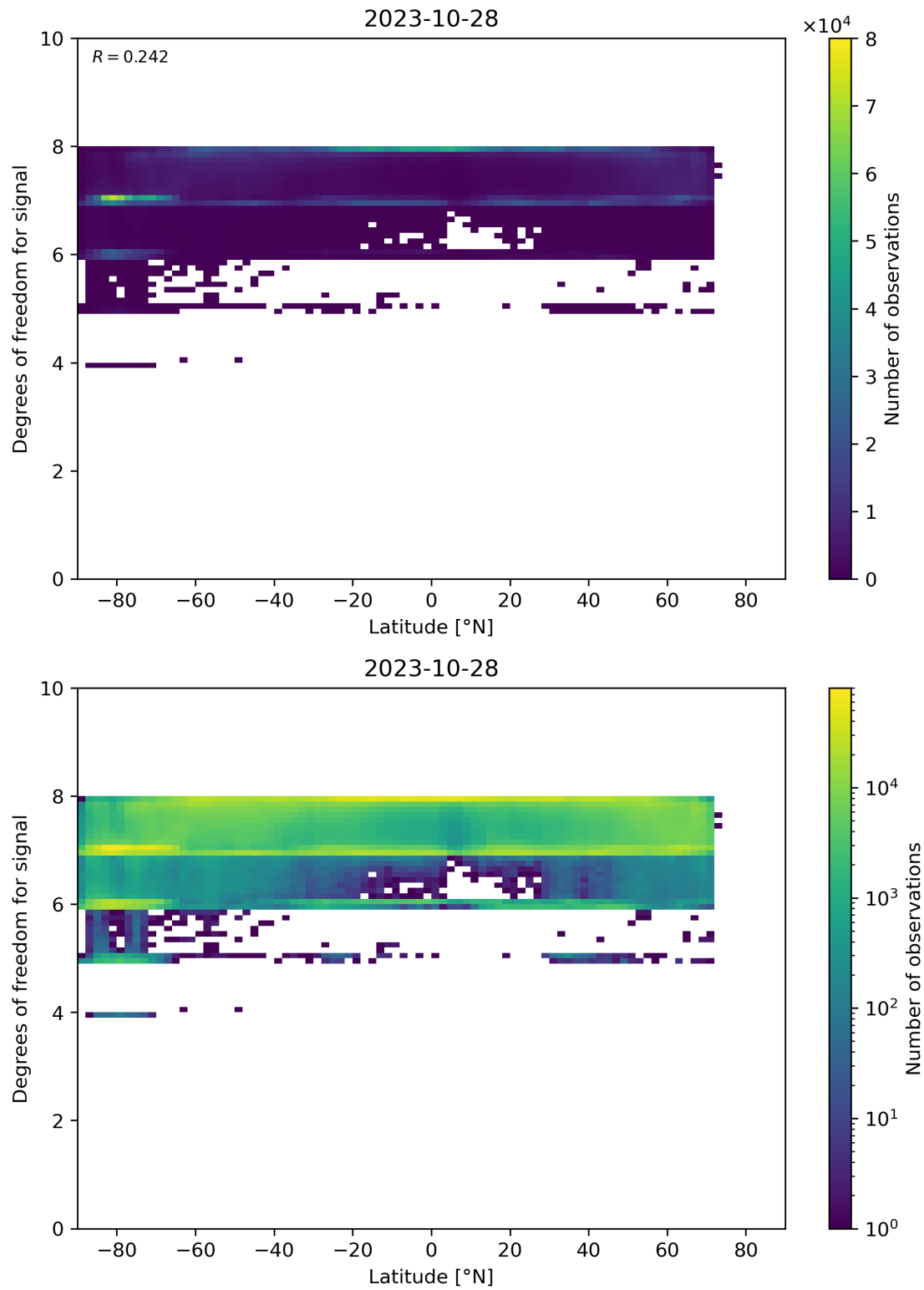
Figure 55: Scatter density plot of “Latitude” against “Degrees of freedom for signal” for 2023-10-28 to 2023-10-29.
