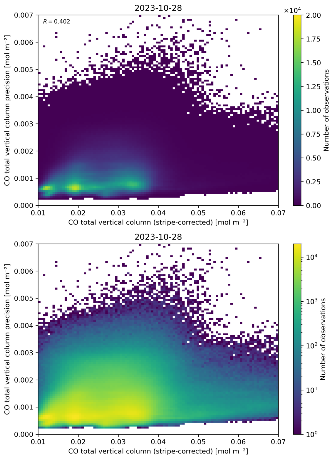
Figure 36: Scatter density plot of “CO total vertical column (stripe-corrected)” against “CO total vertical column precision” for 2023-10-28 to 2023-10-29.
