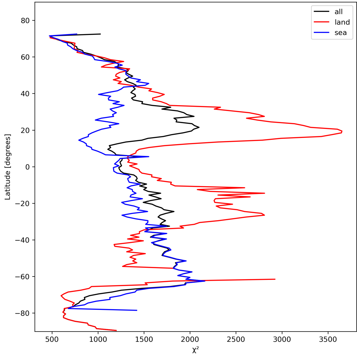
Figure 14: Zonal average of “ \chi^2 ” for 2023-10-28 to 2023-10-29.
