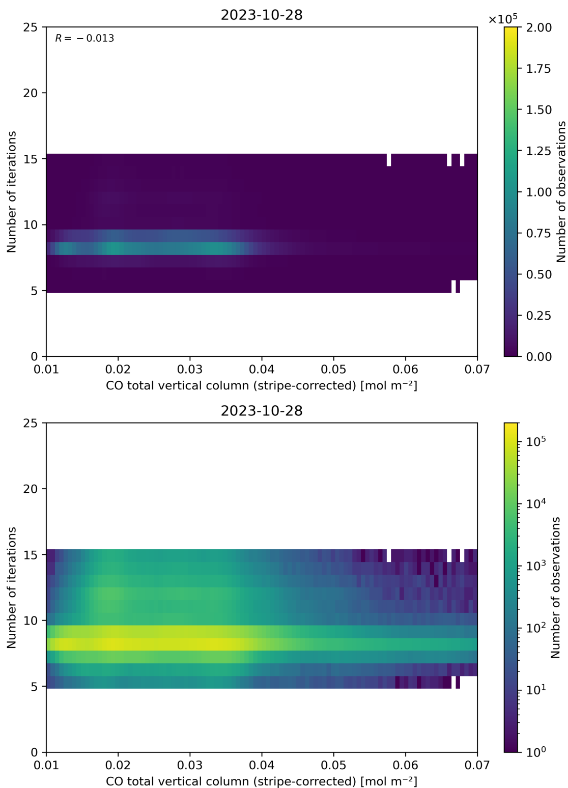
Figure 39: Scatter density plot of “CO total vertical column (stripe-corrected)” against “Number of iterations” for 2023-10-28 to 2023-10-29.
