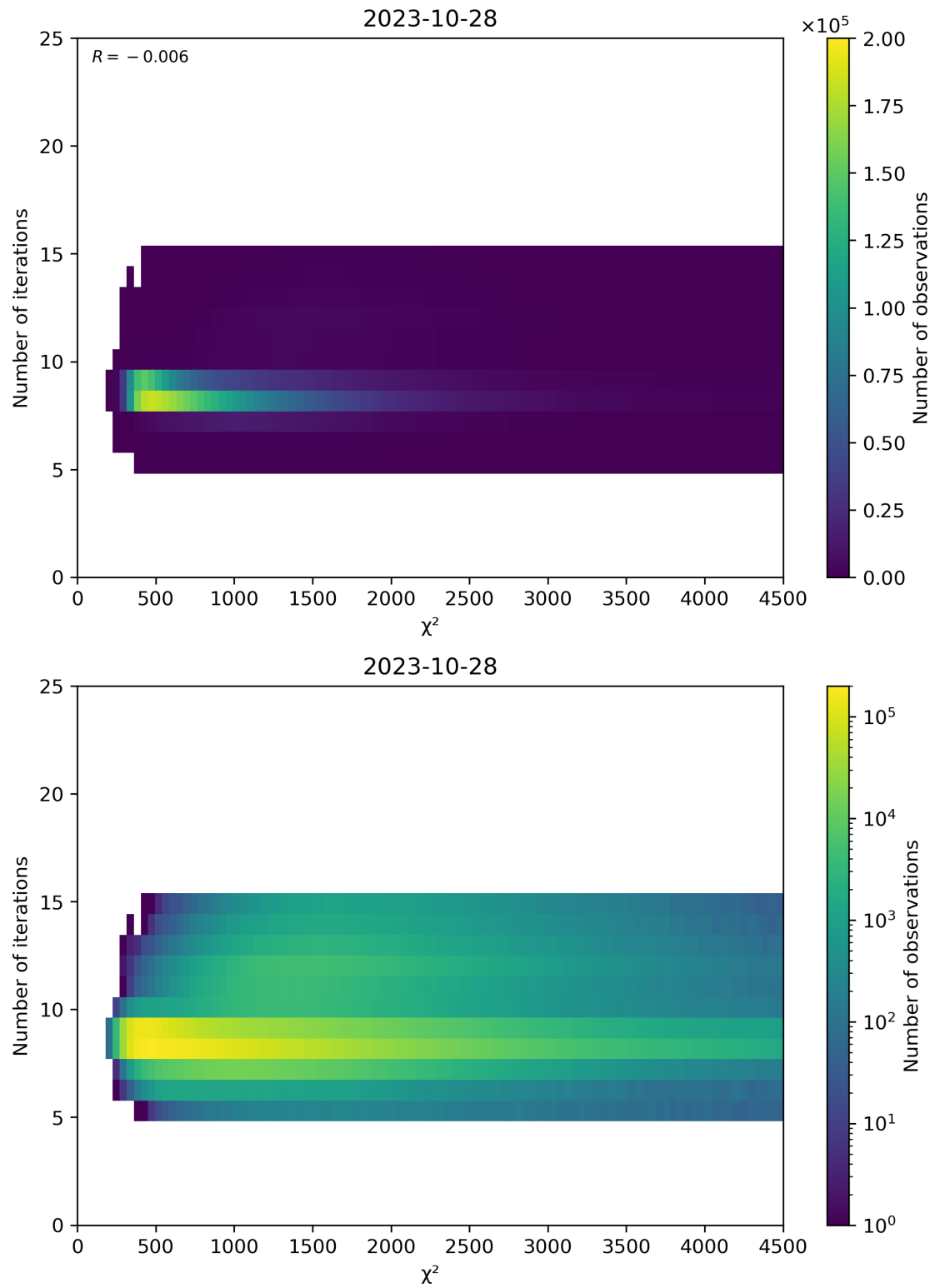
Figure 49: Scatter density plot of “ \chi^2 ” against “Number of iterations” for 2023-10-28 to 2023-10-29.
