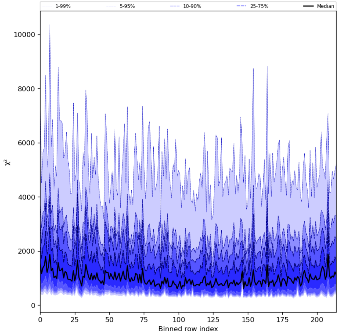
Figure 30: Along track statistics of “ \chi^2 ” for 2023-10-28 to 2023-10-29
