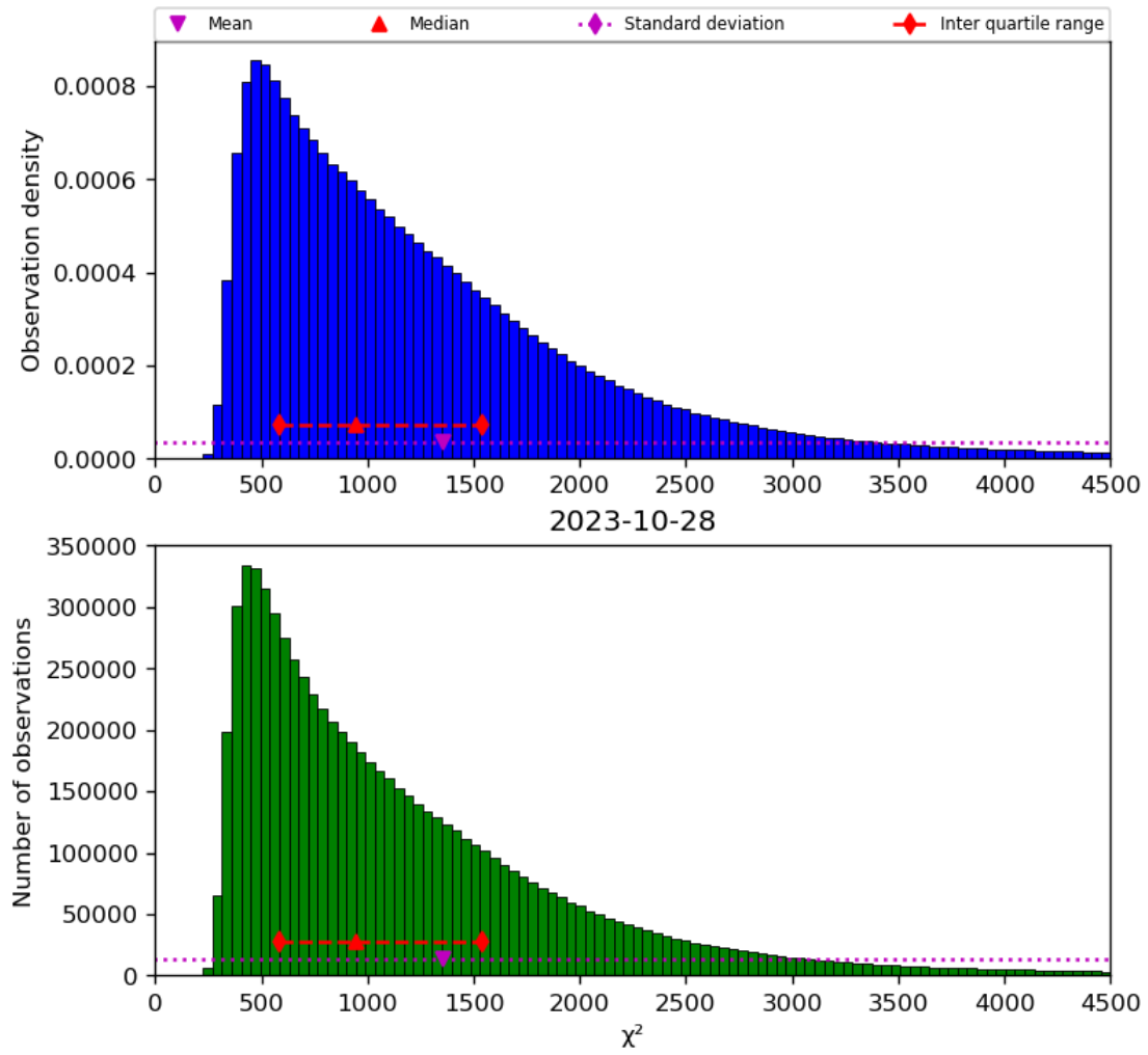
Figure 22: Histogram of “ \chi^2 ” for 2023-10-28 to 2023-10-29
