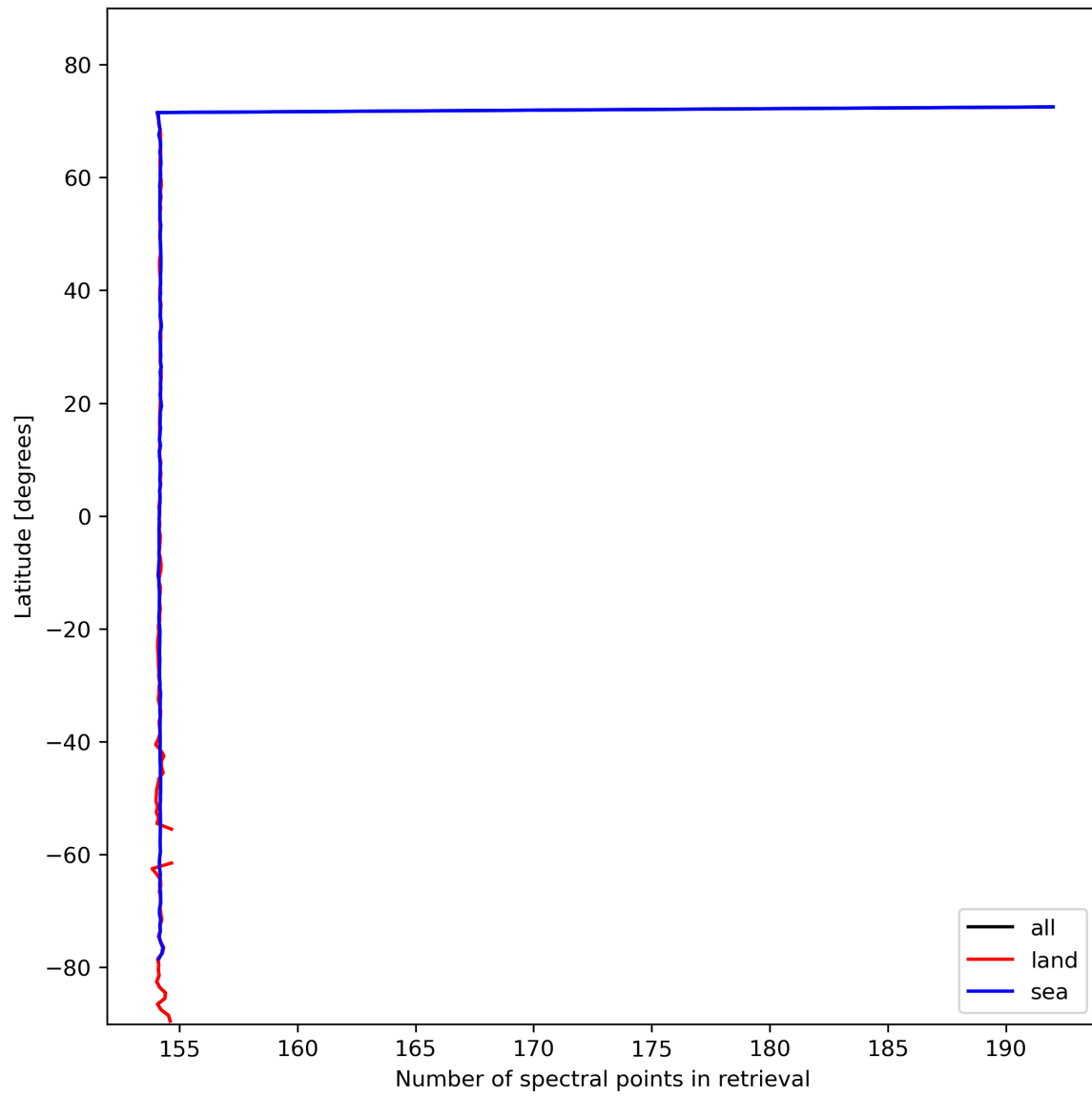
Figure 13: Zonal average of “Number of spectral points in retrieval” for 2023-10-28 to 2023-10-29.
