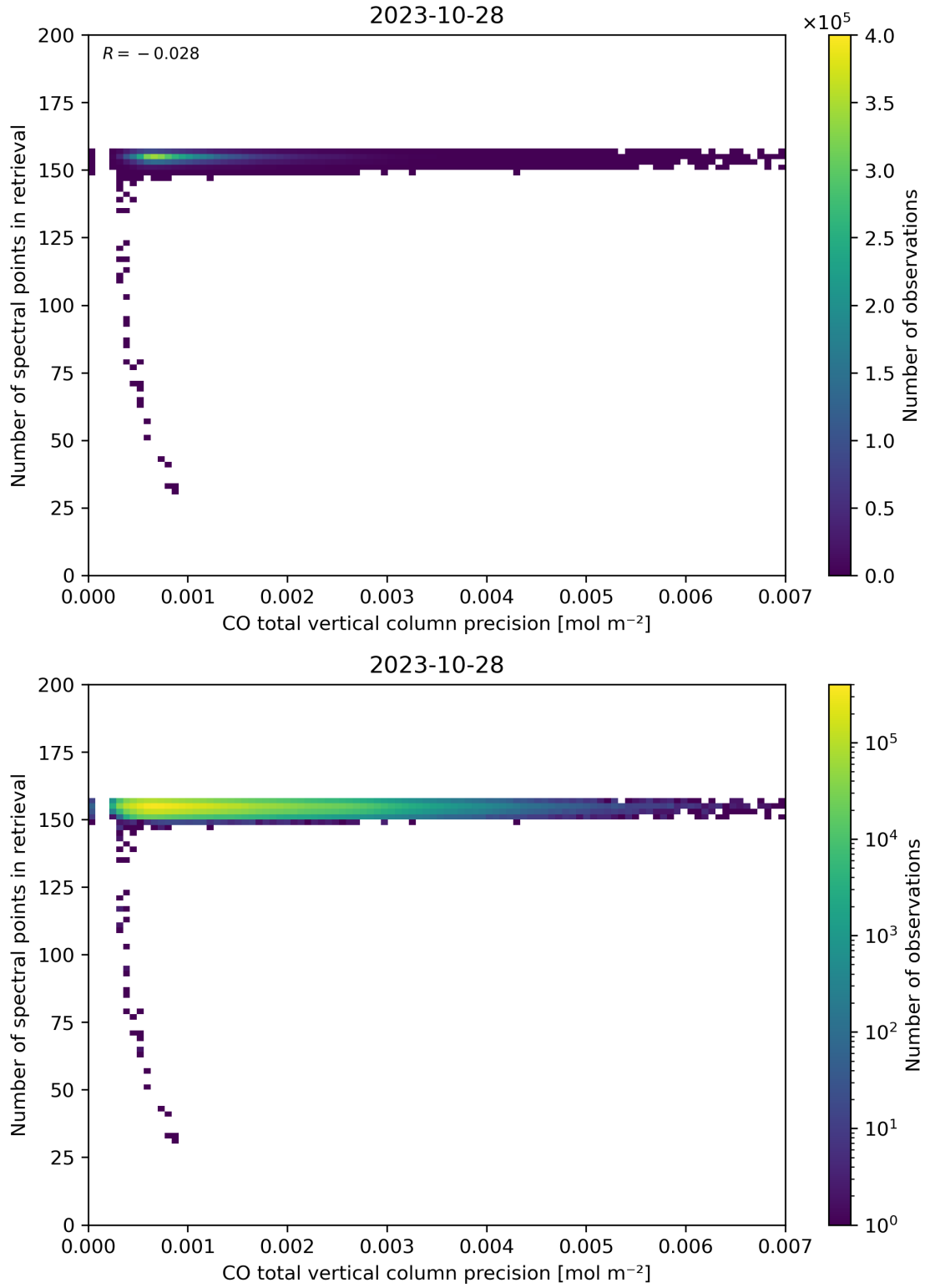
Figure 47: Scatter density plot of “CO total vertical column precision” against “Number of spectral points in retrieval” for 2023-10-28 to 2023-10-29.
