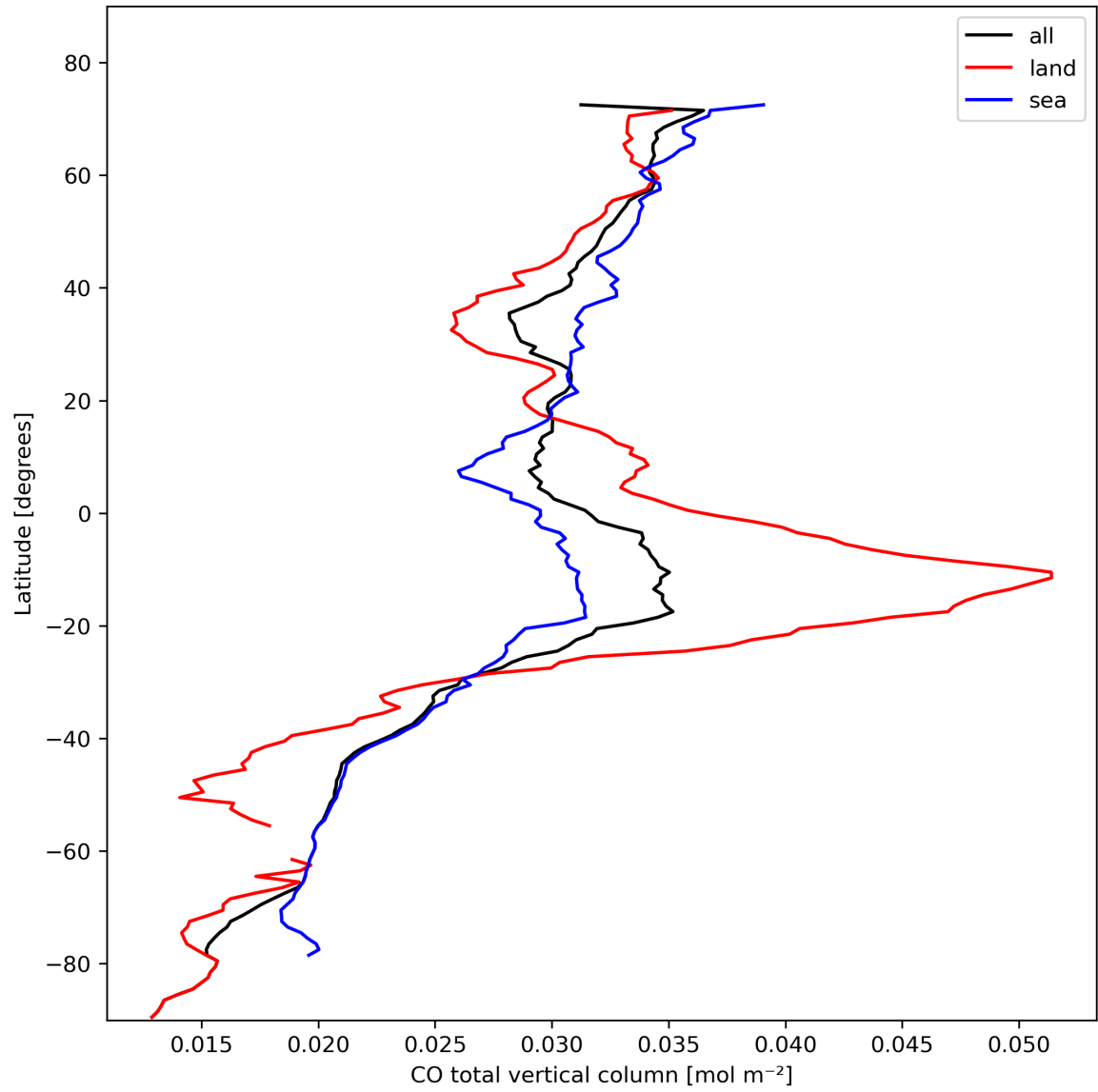
Figure 10: Zonal average of “CO total vertical column” for 2023-10-28 to 2023-10-29.
