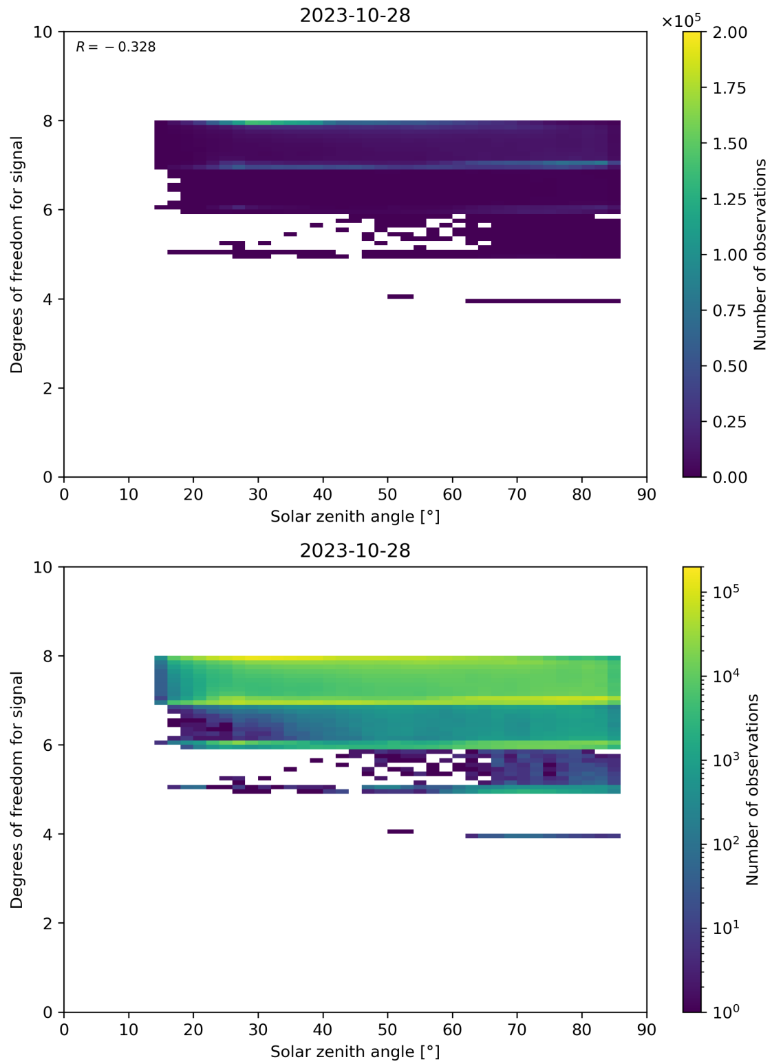
Figure 65: Scatter density plot of “Solar zenith angle” against “Degrees of freedom for signal” for 2023-10-28 to 2023-10-29.
