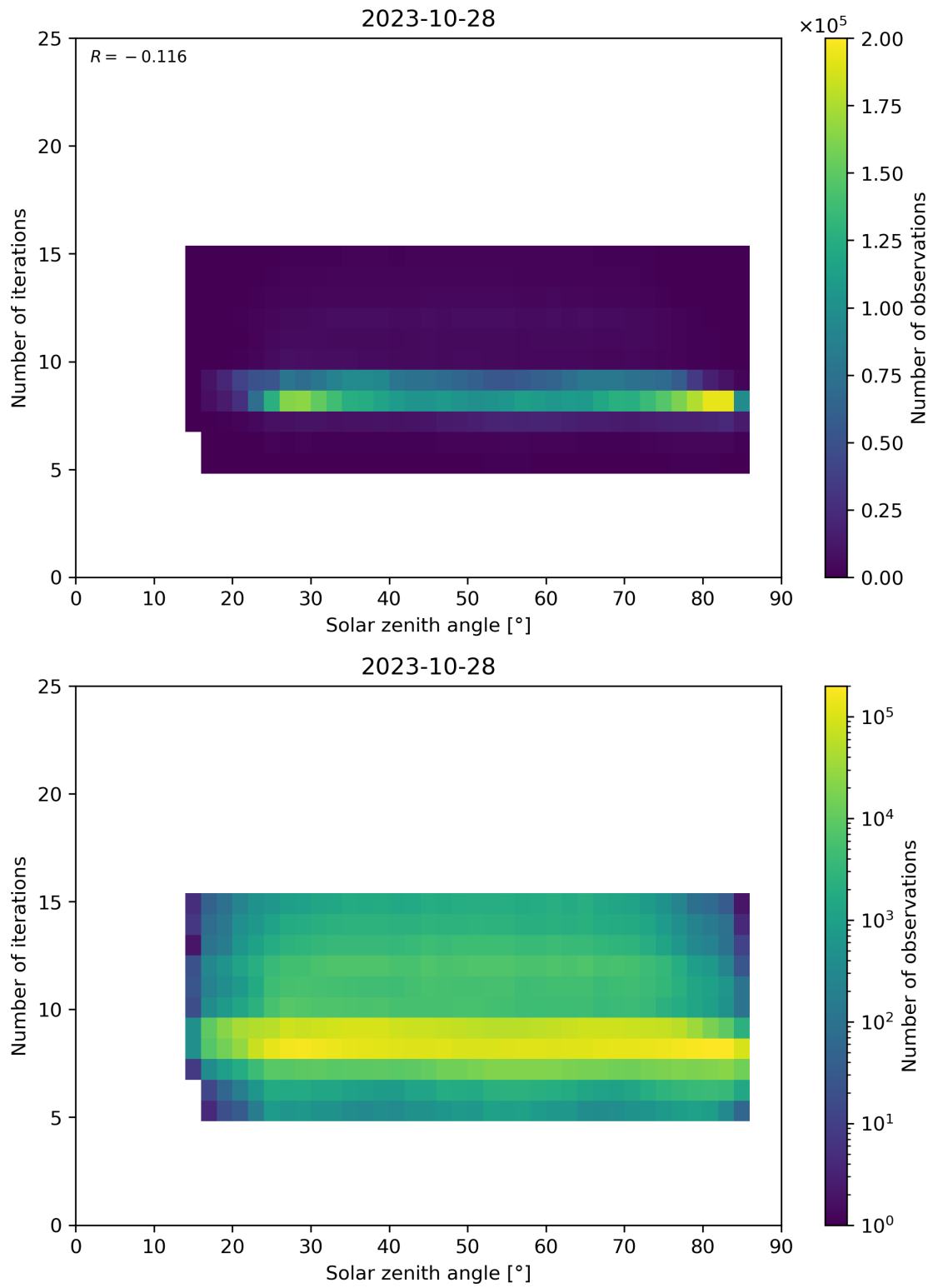
Figure 67: Scatter density plot of “Solar zenith angle” against “Number of iterations” for 2023-10-28 to 2023-10-29.
