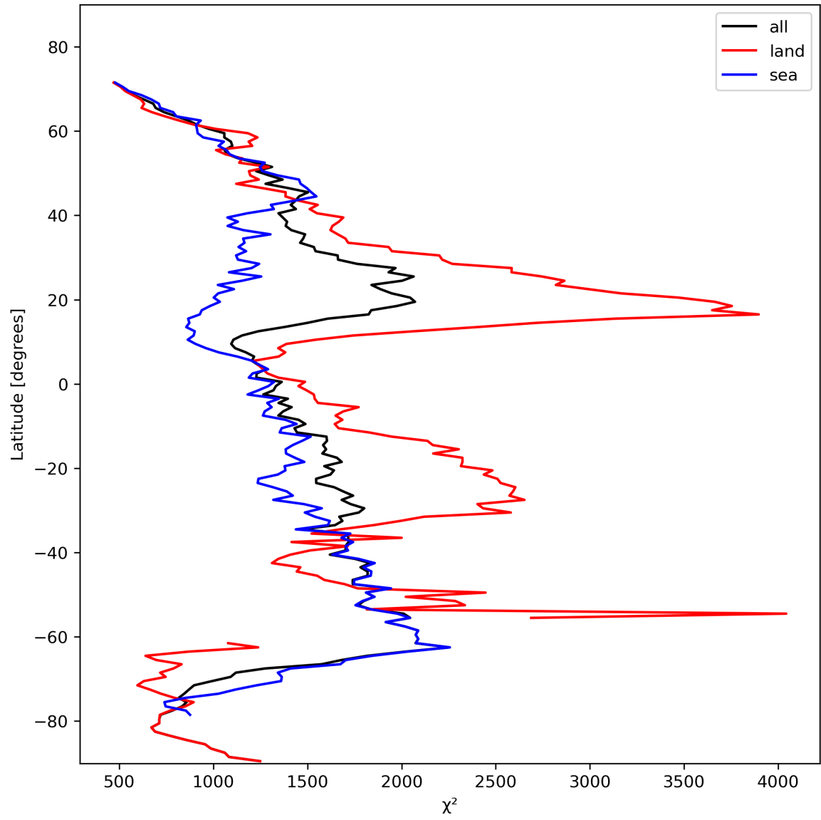
Figure 14: Zonal average of “ \chi^2 ” for 2023-10-28 to 2023-10-30.
