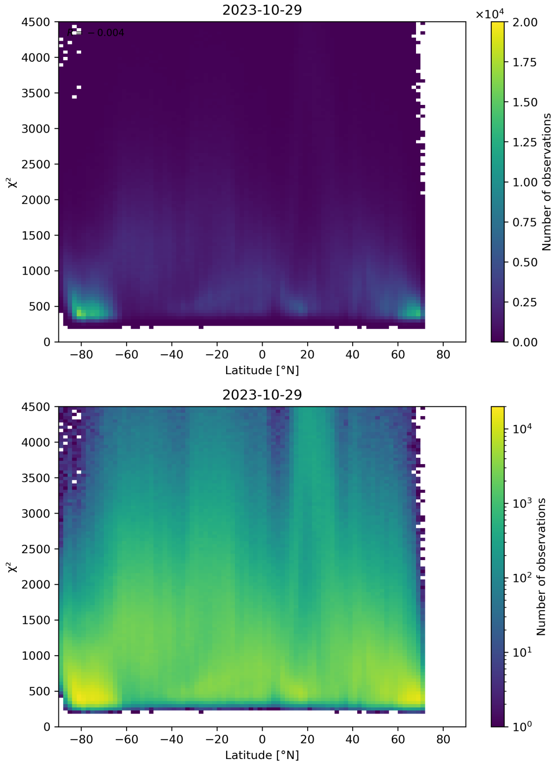
Figure 54: Scatter density plot of “Latitude” against “ \chi^2 ” for 2023-10-28 to 2023-10-30.
