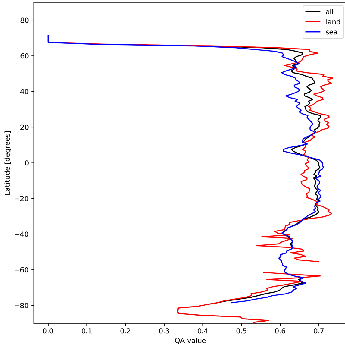
Figure 9: Zonal average of “QA value” for 2023-10-28 to 2023-10-30.
