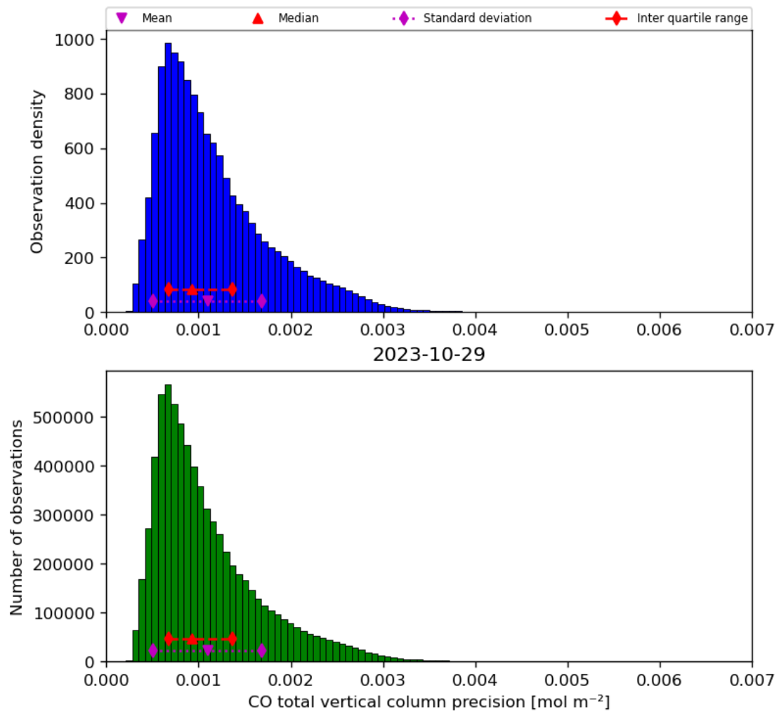
Figure 20: Histogram of “CO total vertical column precision” for 2023-10-28 to 2023-10-30
