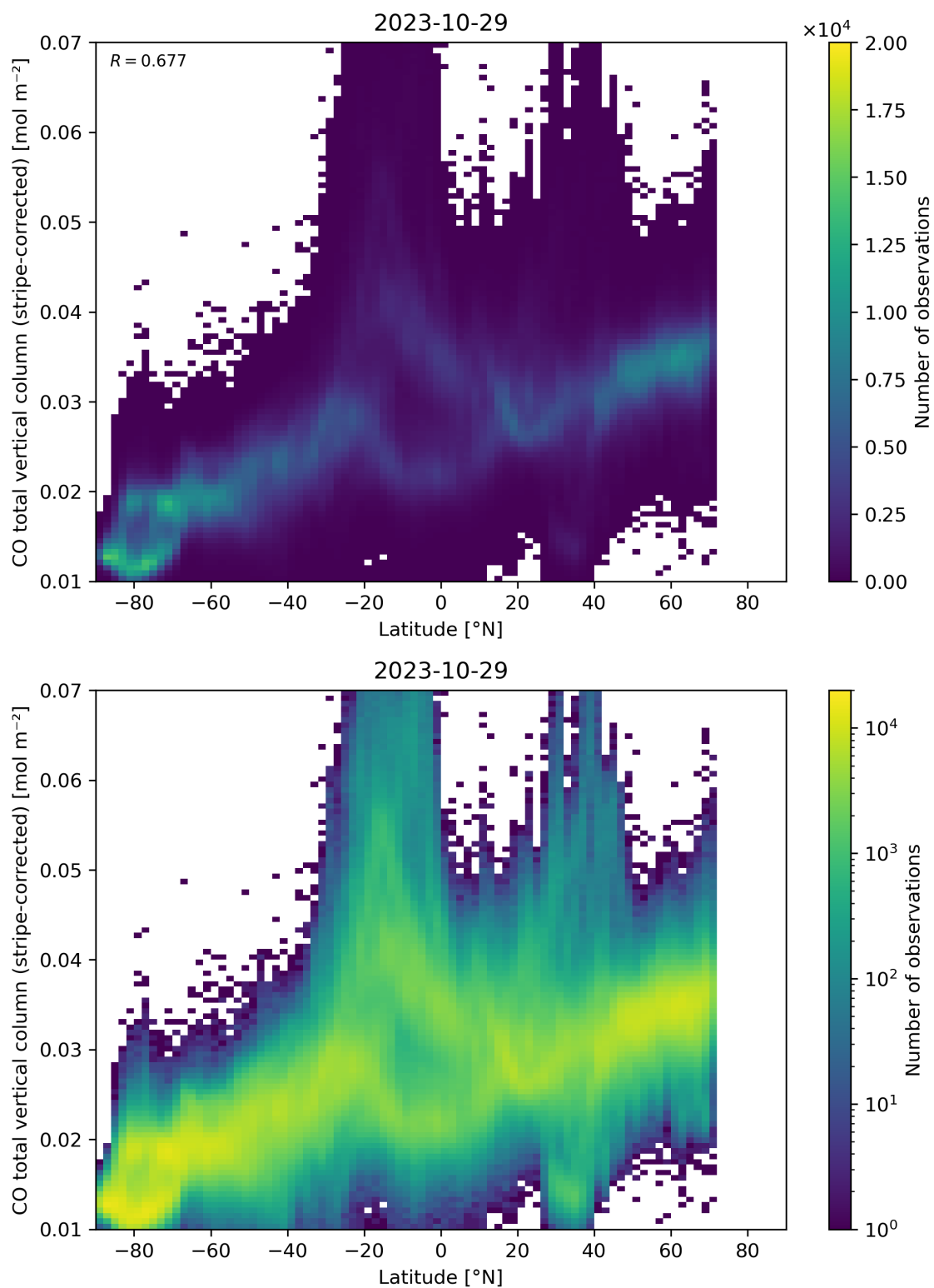
Figure 52: Scatter density plot of “Latitude” against “CO total vertical column (stripe-corrected)” for 2023-10-28 to 2023-10-30.
