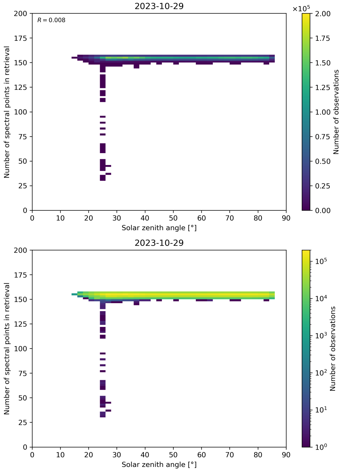
Figure 68: Scatter density plot of “Solar zenith angle” against “Number of spectral points in retrieval” for 2023-10-28 to 2023-10-30.
