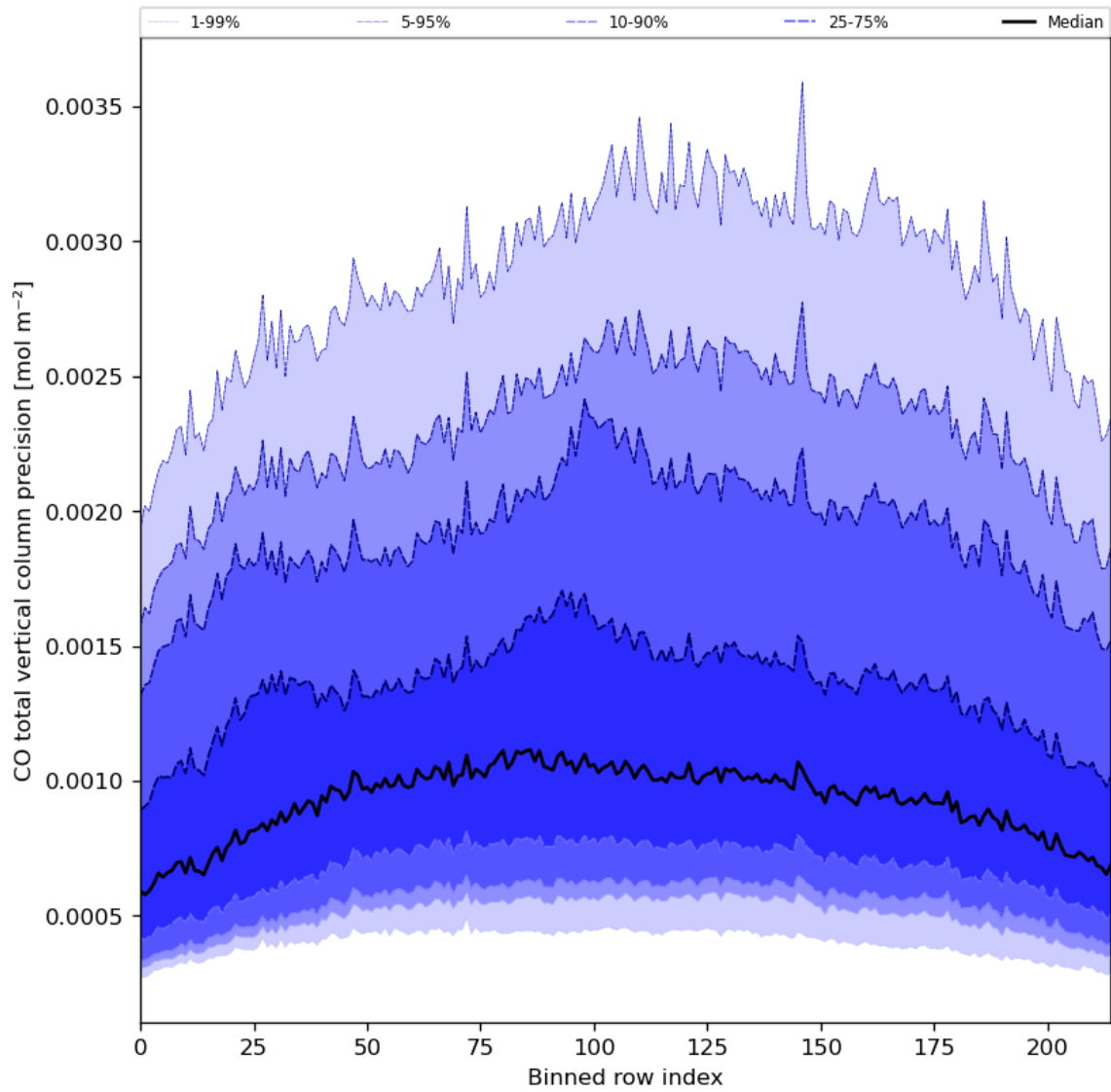
Figure 28: Along track statistics of “CO total vertical column precision” for 2023-10-28 to 2023-10-30
