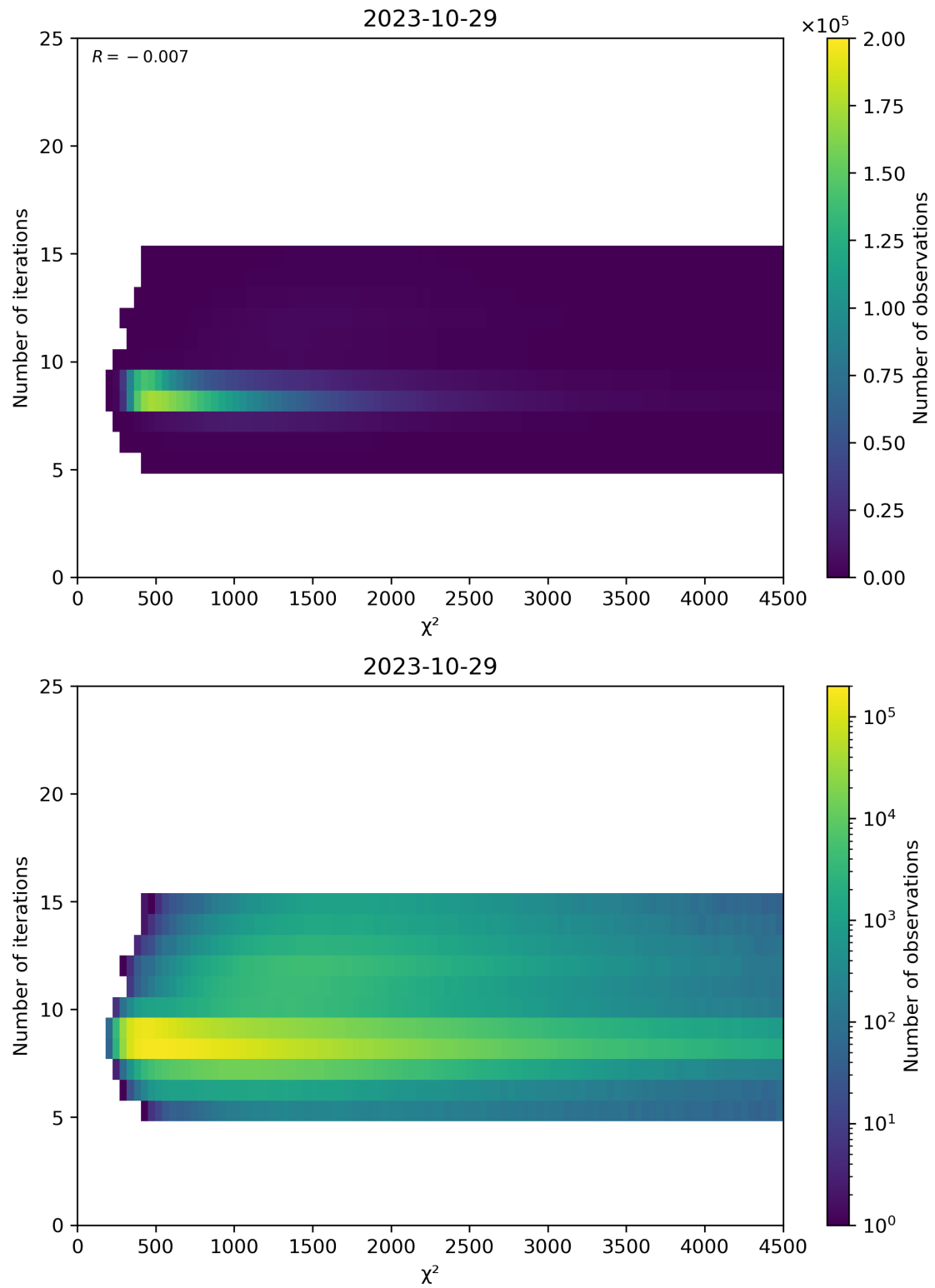
Figure 49: Scatter density plot of “ \chi^2 ” against “Number of iterations” for 2023-10-28 to 2023-10-30.
