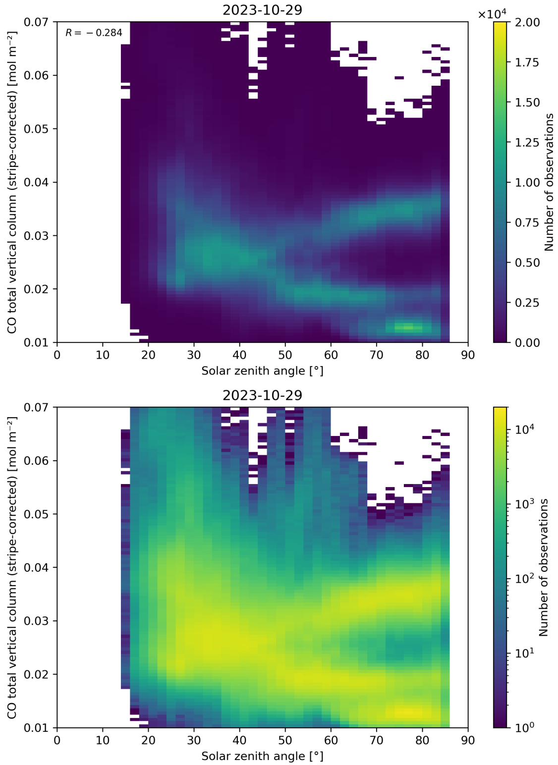
Figure 62: Scatter density plot of “Solar zenith angle” against “CO total vertical column (stripe-corrected)” for 2023-10-28 to 2023-10-30.
