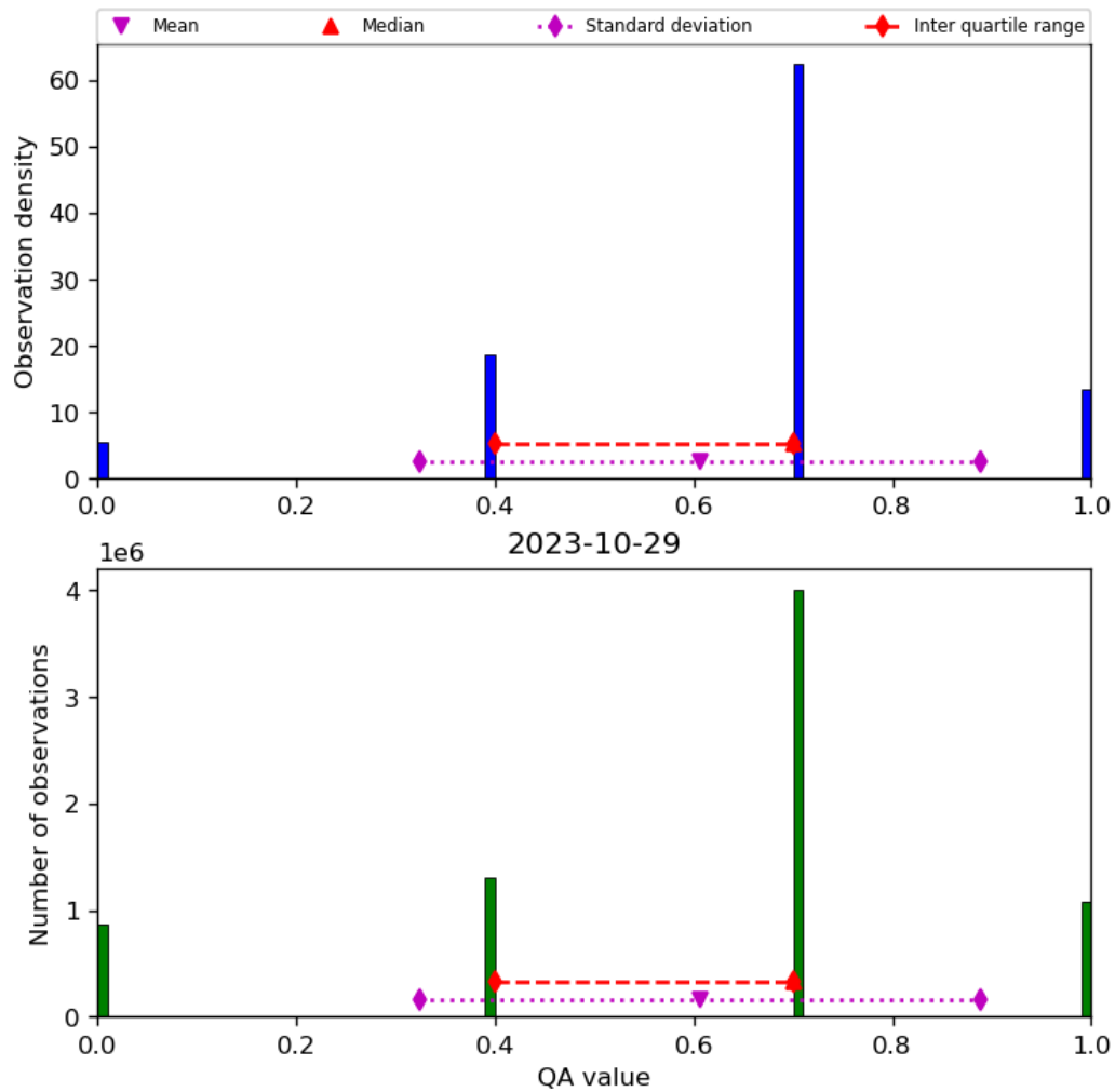
Figure 17: Histogram of “QA value” for 2023-10-28 to 2023-10-30
