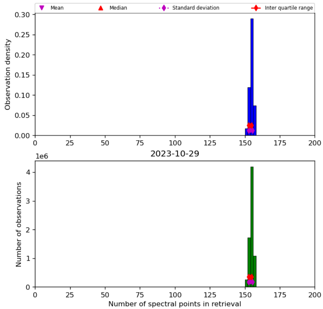
Figure 21: Histogram of “Number of spectral points in retrieval” for 2023-10-28 to 2023-10-30
