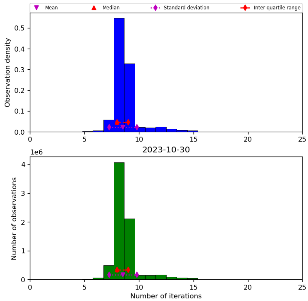
Figure 24: Histogram of “Number of iterations” for 2023-10-29 to 2023-10-31
