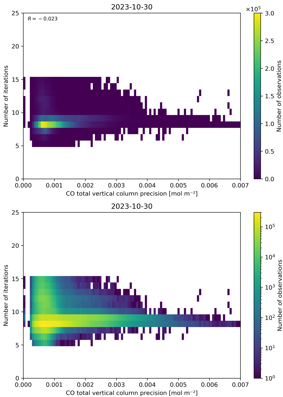
Figure 46: Scatter density plot of “CO total vertical column precision” against “Number of iterations” for 2023-10-29 to 2023-10-31.
