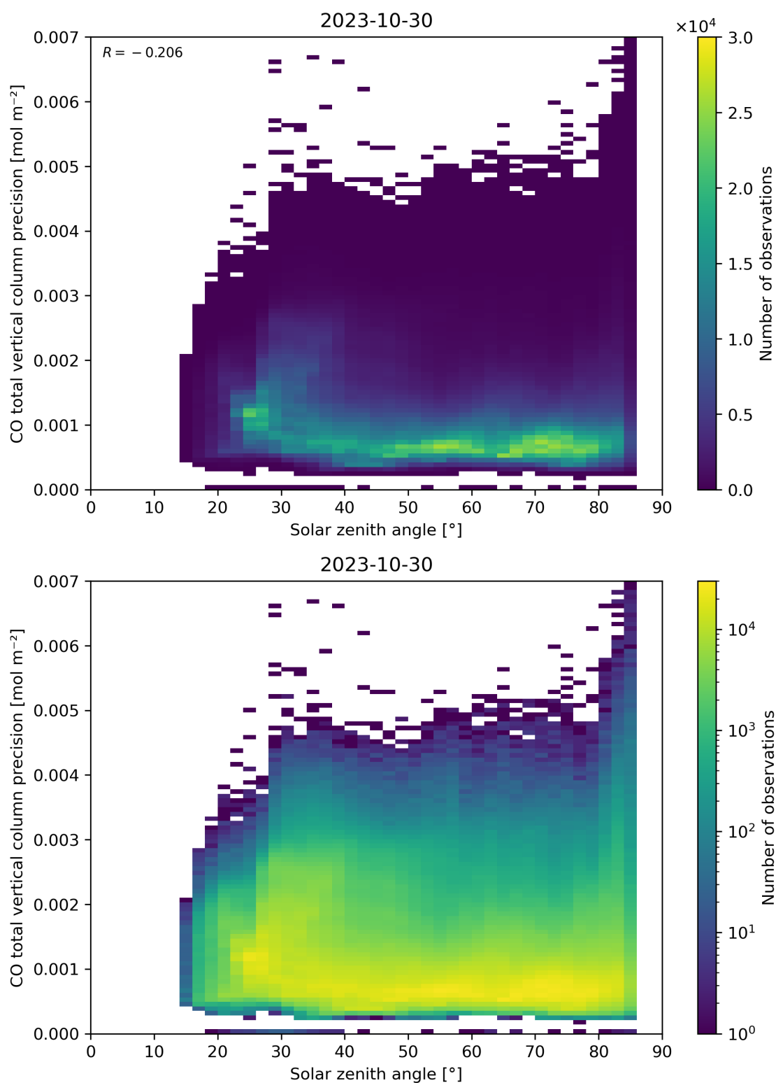
Figure 63: Scatter density plot of “Solar zenith angle” against “CO total vertical column precision” for 2023-10-29 to 2023-10-31.
