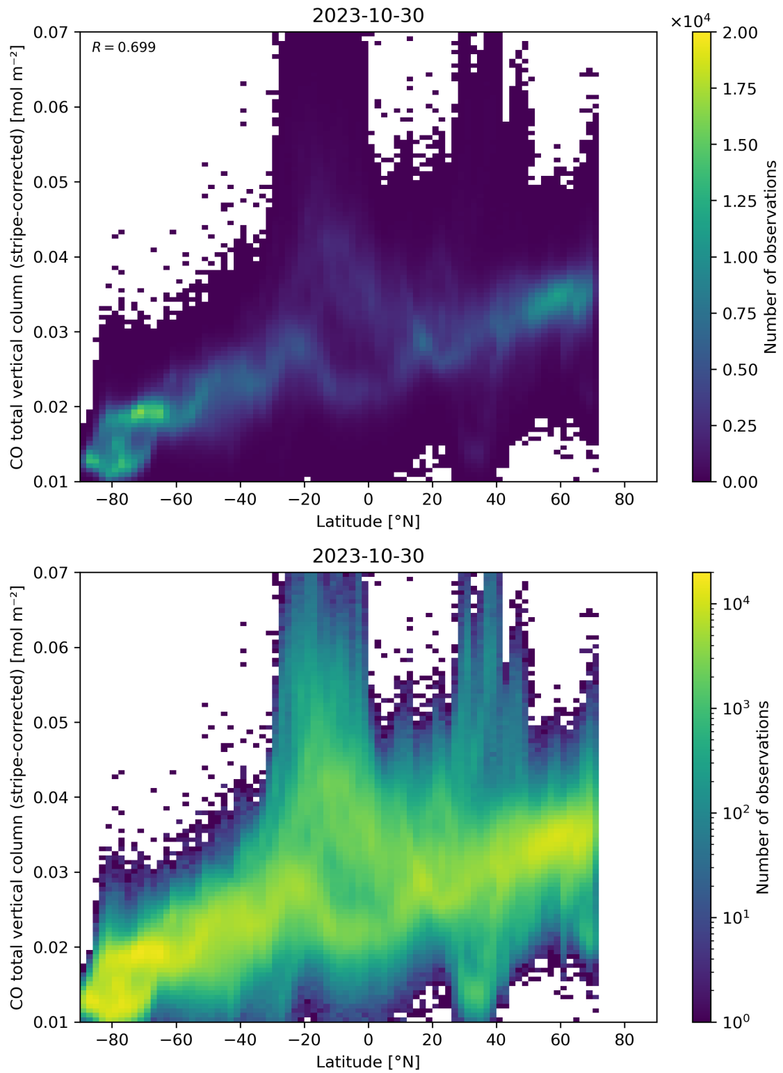
Figure 52: Scatter density plot of “Latitude” against “CO total vertical column (stripe-corrected)” for 2023-10-29 to 2023-10-31.
