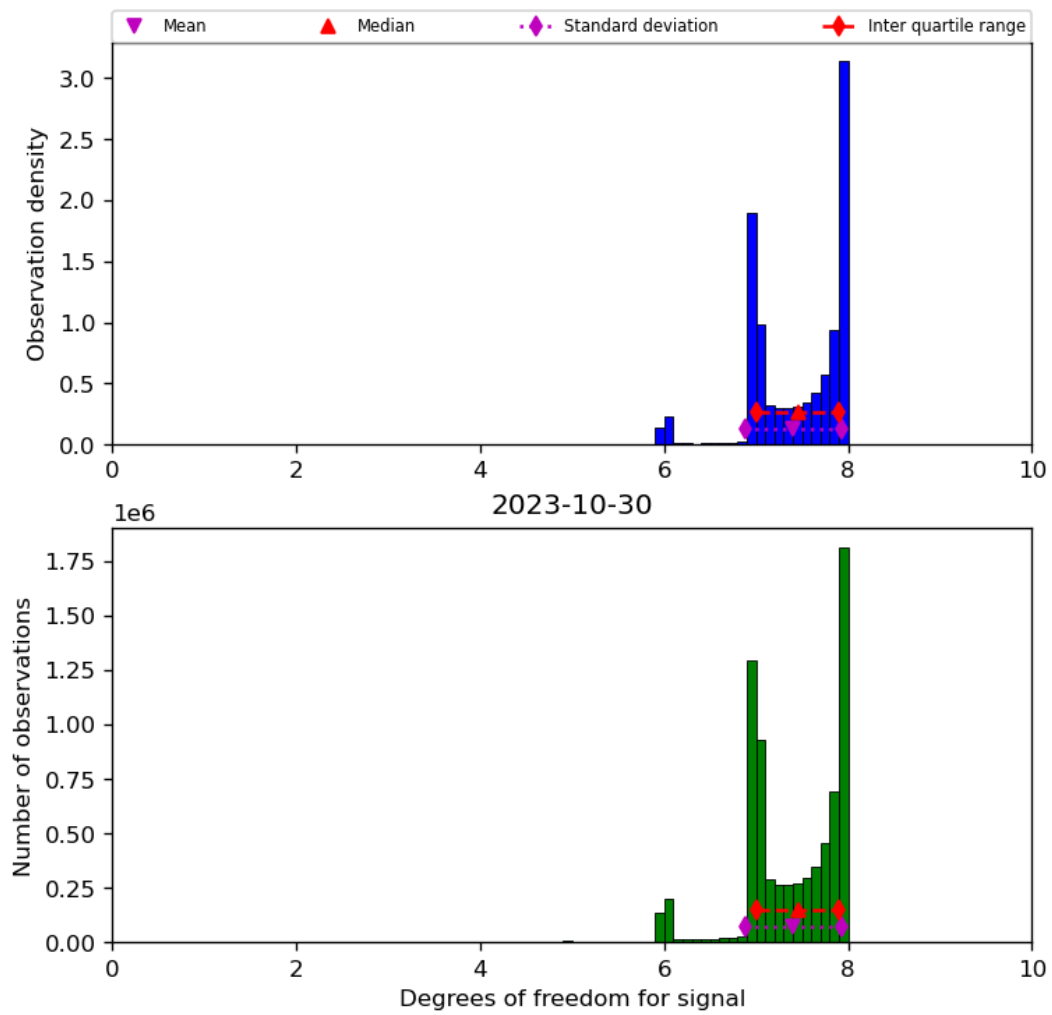
Figure 23: Histogram of “Degrees of freedom for signal” for 2023-10-29 to 2023-10-31
