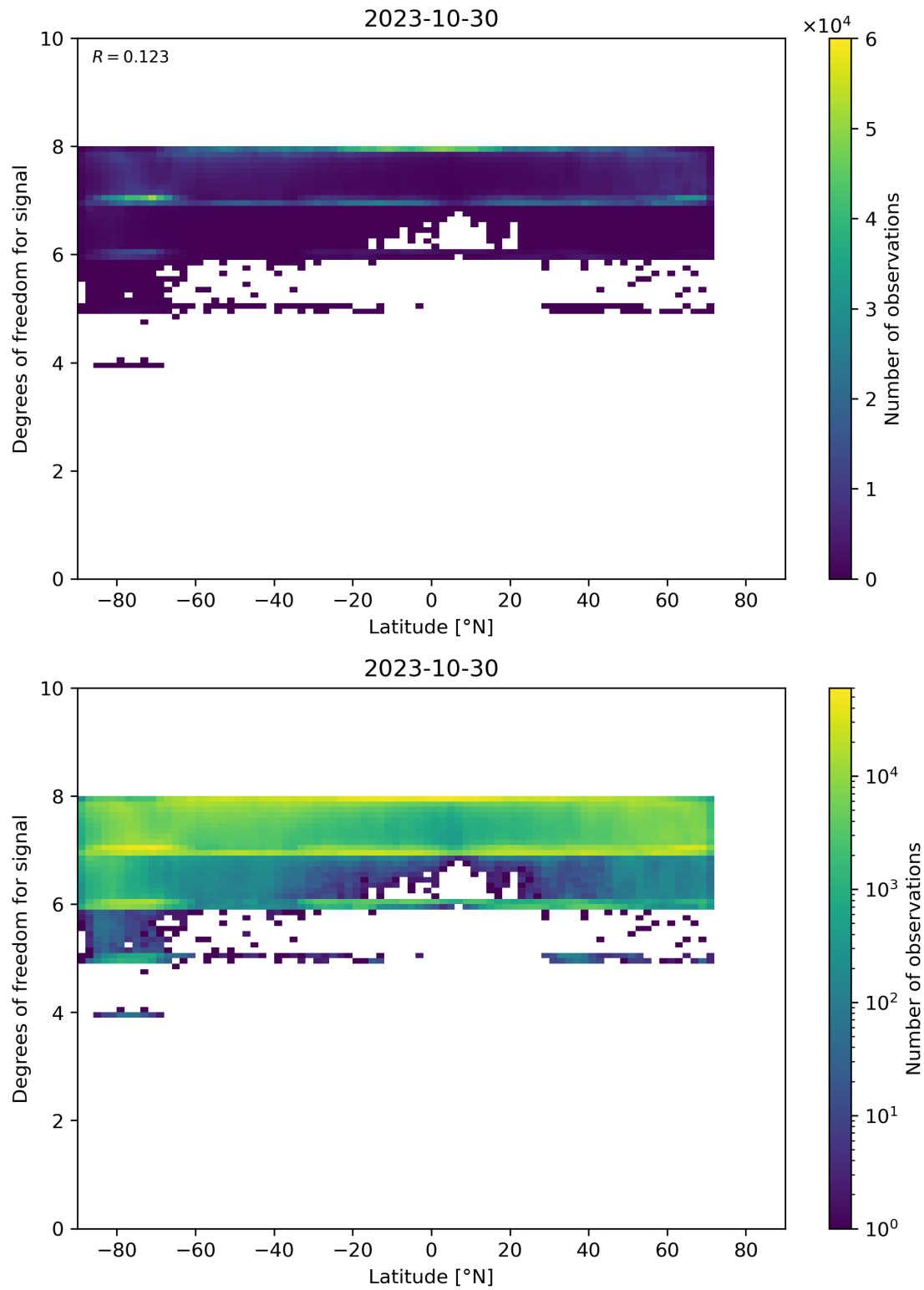
Figure 55: Scatter density plot of “Latitude” against “Degrees of freedom for signal” for 2023-10-29 to 2023-10-31.
