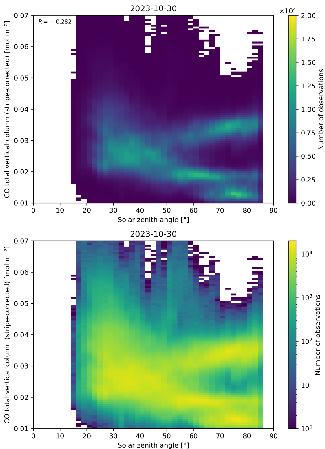
Figure 62: Scatter density plot of “Solar zenith angle” against “CO total vertical column (stripe-corrected)” for 2023-10-29 to 2023-10-31.
