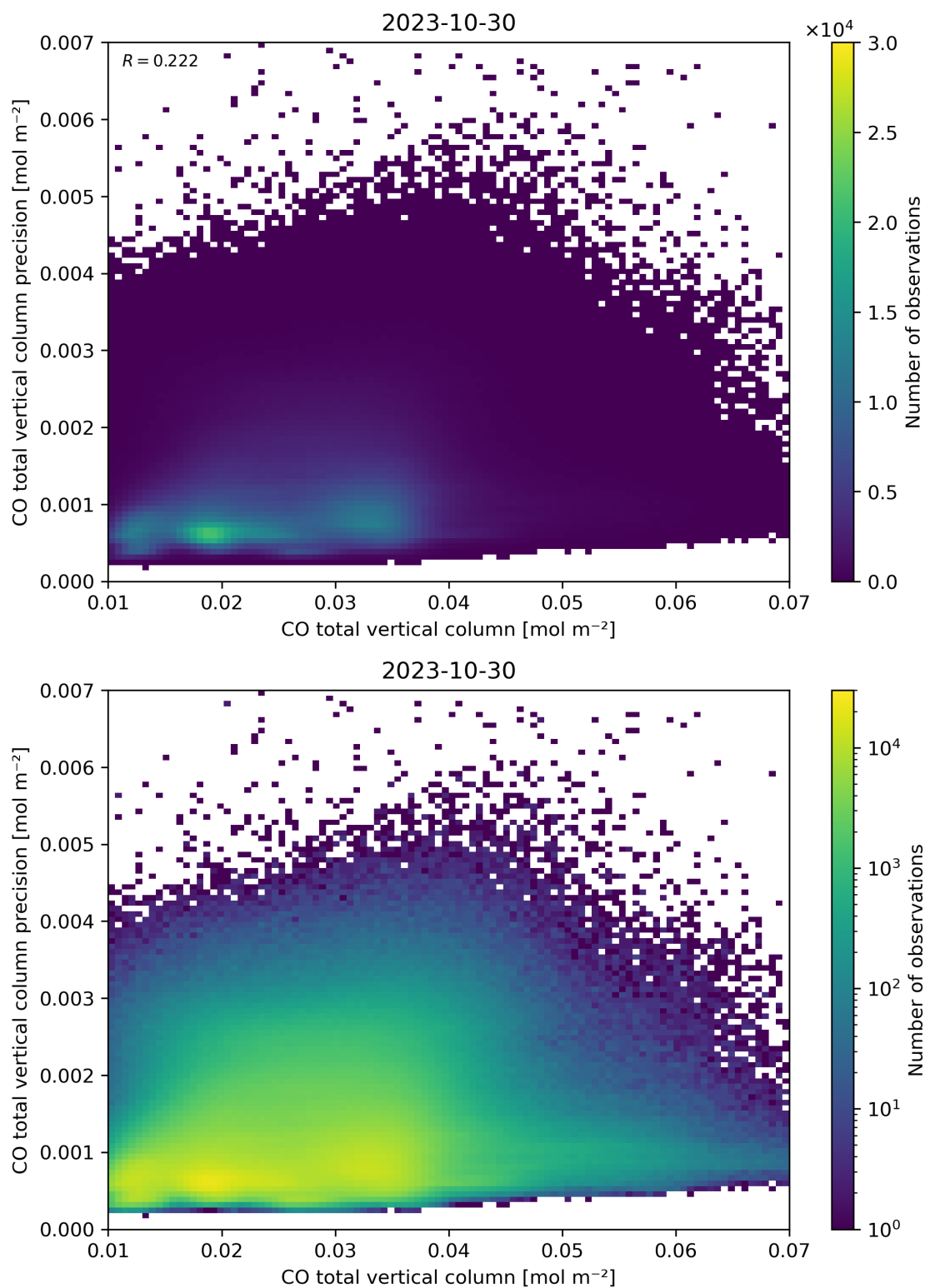
Figure 34: Scatter density plot of “CO total vertical column” against “CO total vertical column precision” for 2023-10-29 to 2023-10-31.
