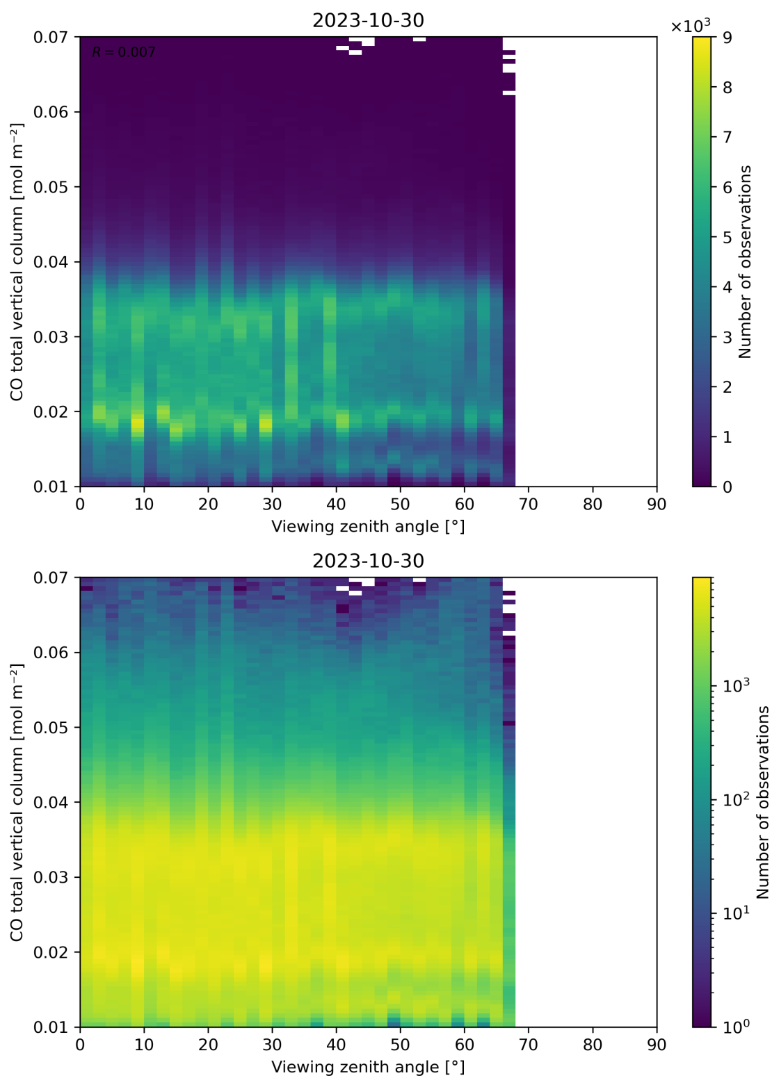
Figure 69: Scatter density plot of “Viewing zenith angle” against “CO total vertical column” for 2023-10-29 to 2023-10-31.
