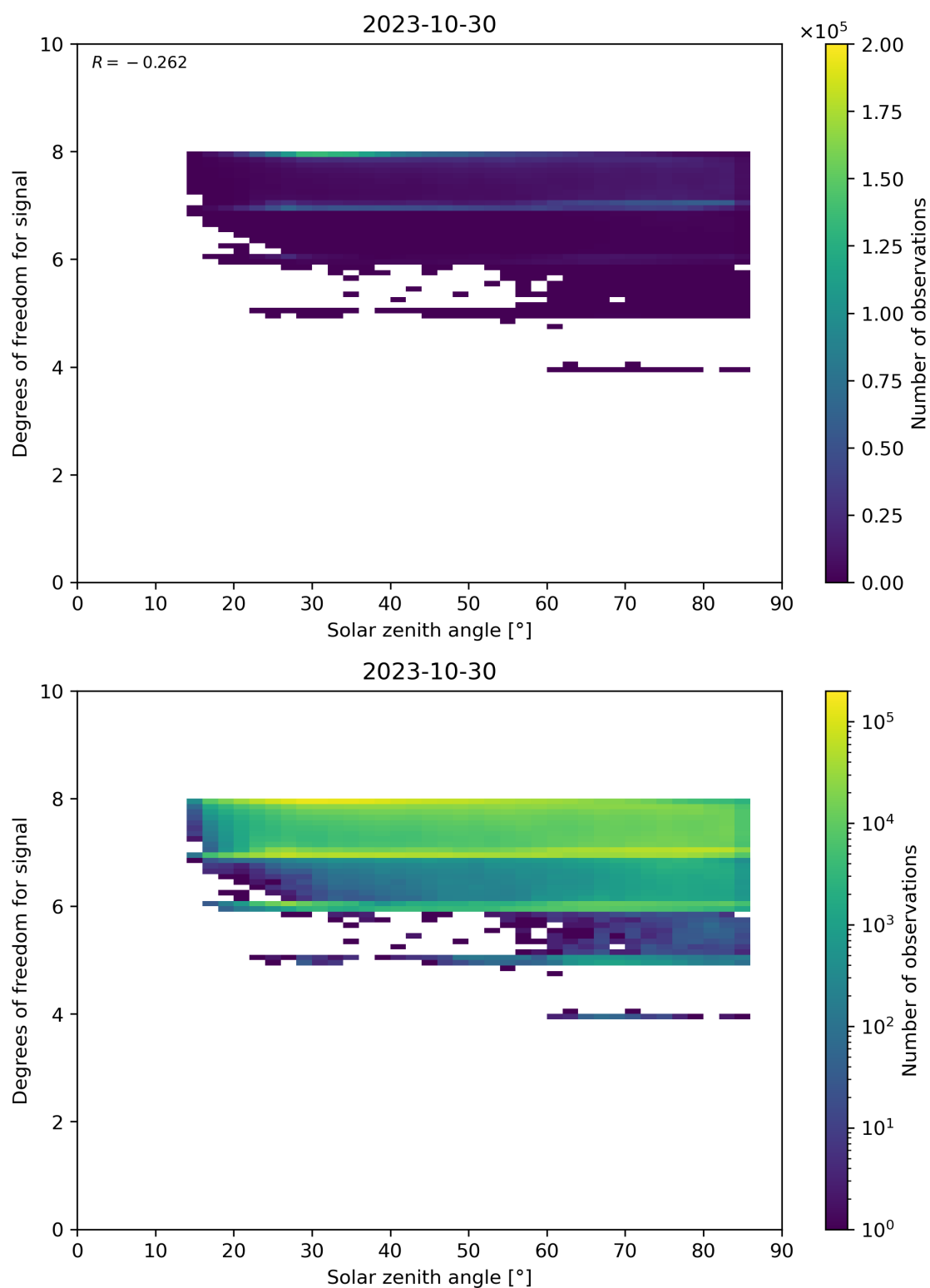
Figure 65: Scatter density plot of “Solar zenith angle” against “Degrees of freedom for signal” for 2023-10-29 to 2023-10-31.
