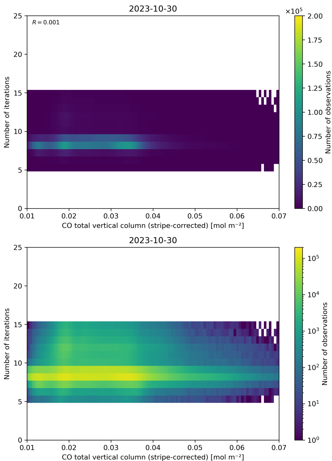
Figure 39: Scatter density plot of “CO total vertical column (stripe-corrected)” against “Number of iterations” for 2023-10-29 to 2023-10-31.
