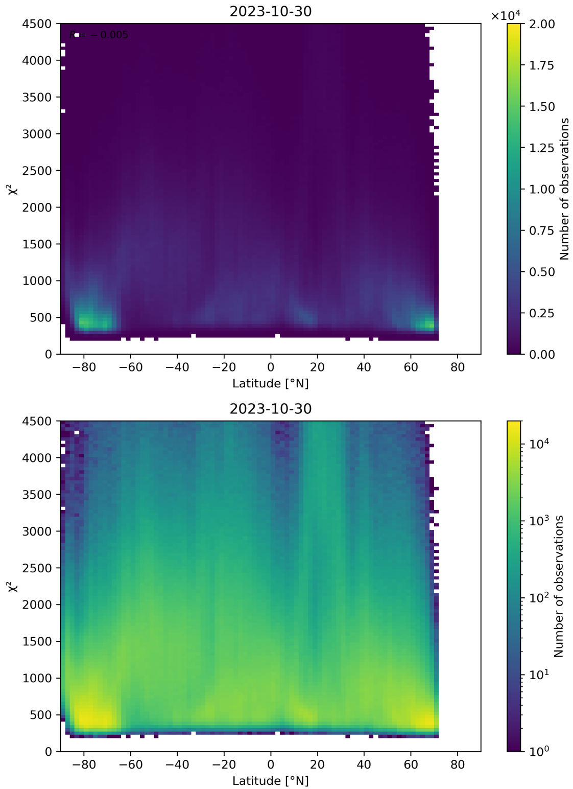
Figure 54: Scatter density plot of “Latitude” against “ \chi^2 ” for 2023-10-29 to 2023-10-31.
