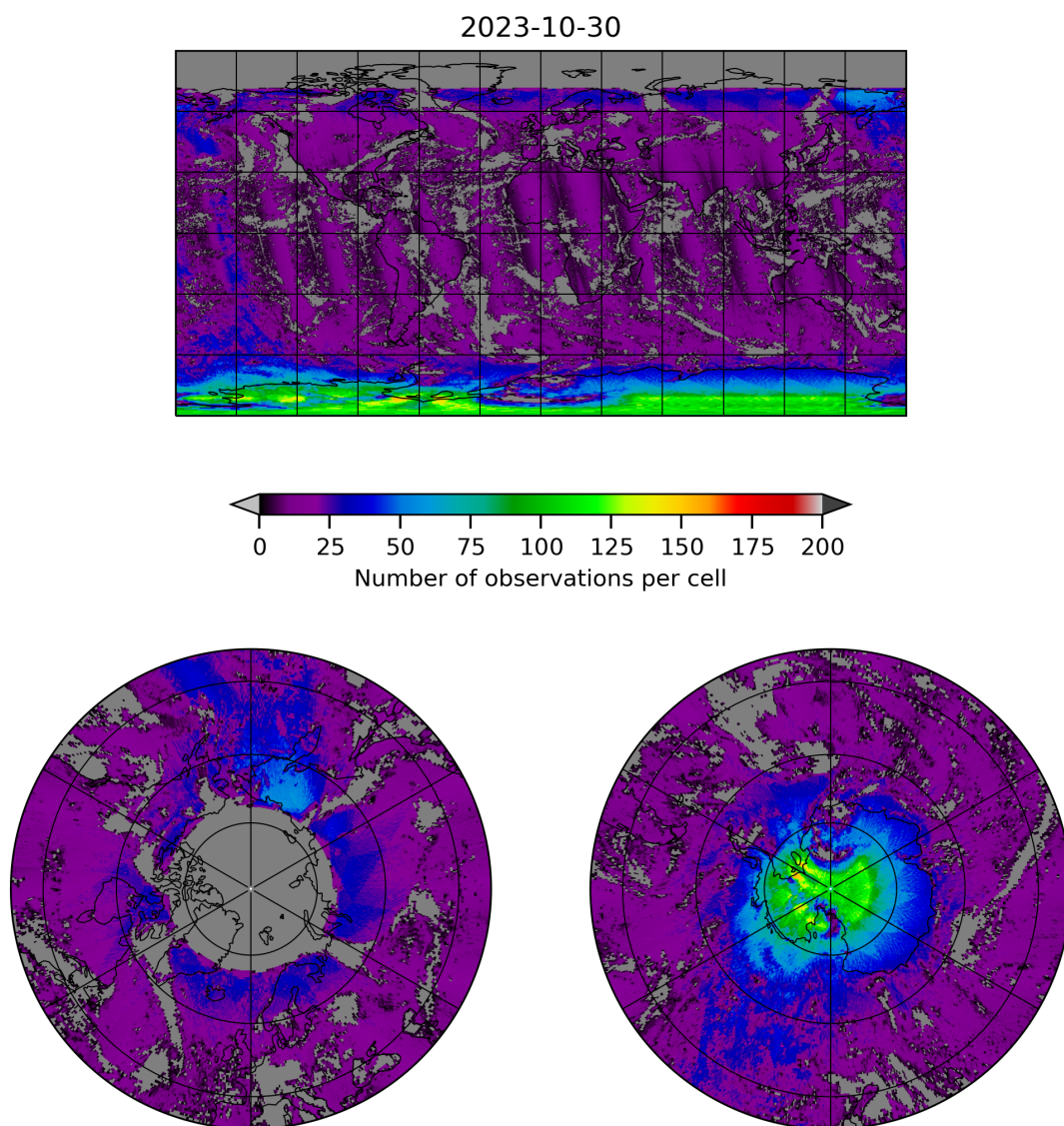
Figure 8: Map of the number of observations for 2023-10-29 to 2023-10-31
