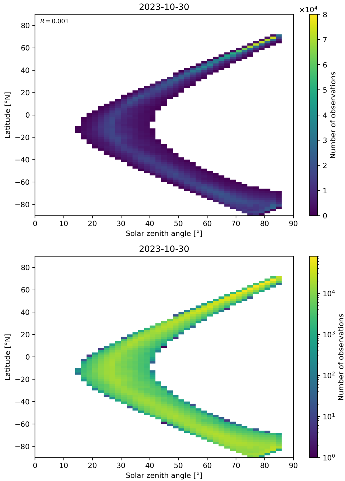
Figure 66: Scatter density plot of “Solar zenith angle” against “Latitude” for 2023-10-29 to 2023-10-31.
