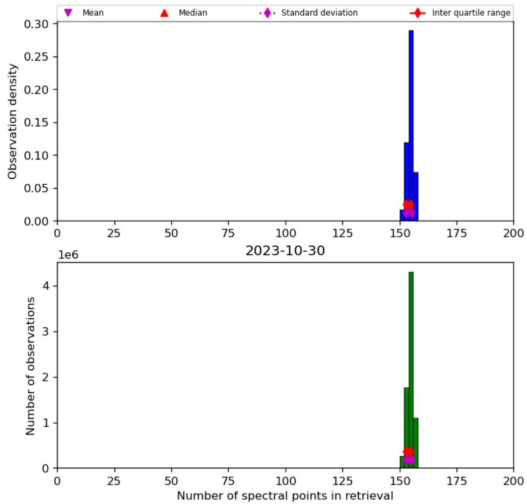
Figure 21: Histogram of “Number of spectral points in retrieval” for 2023-10-29 to 2023-10-31
