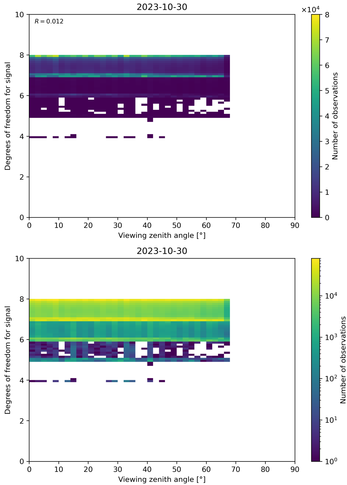
Figure 73: Scatter density plot of “Viewing zenith angle” against “Degrees of freedom for signal” for 2023-10-29 to 2023-10-31.
