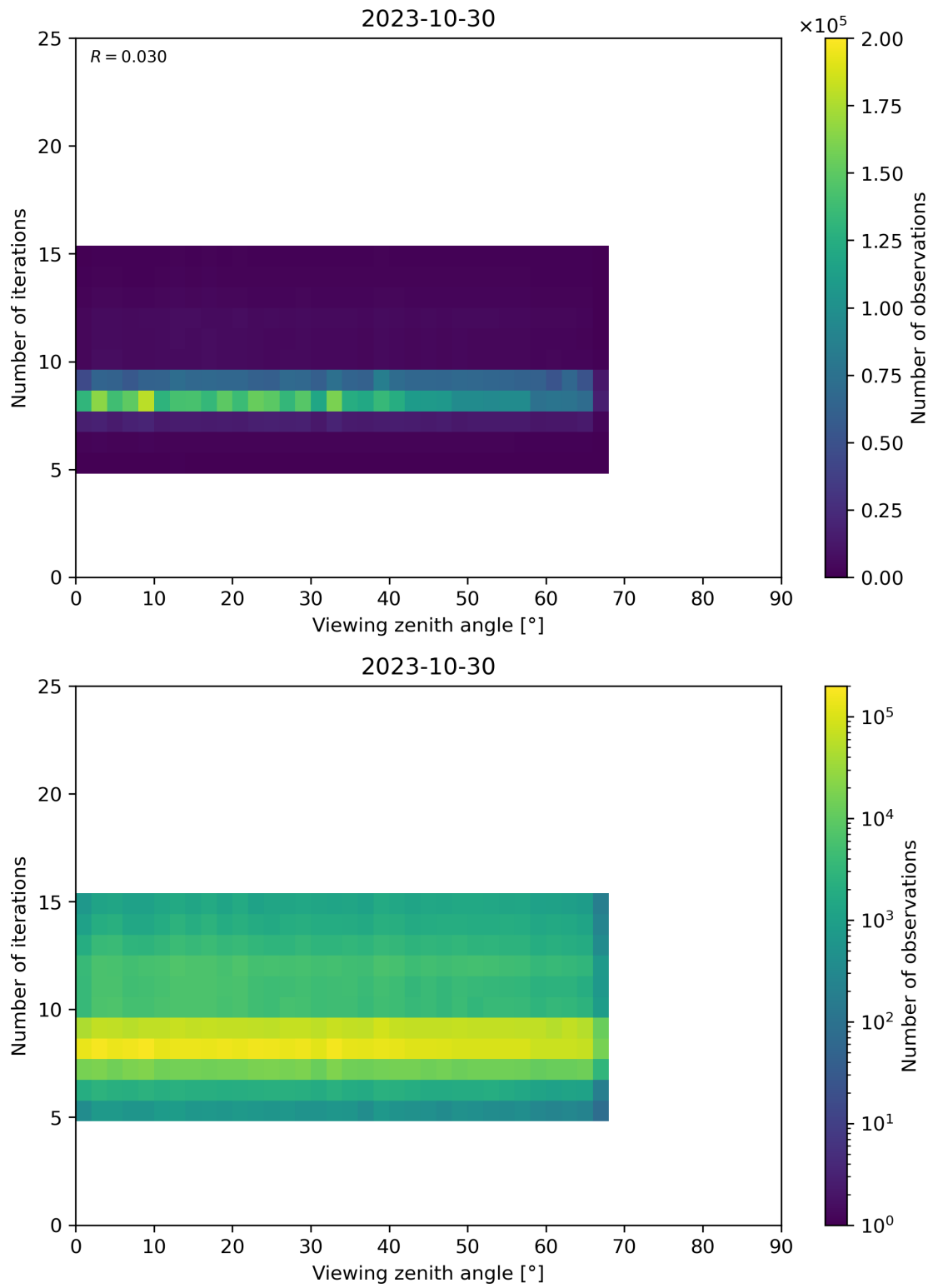
Figure 75: Scatter density plot of “Viewing zenith angle” against “Number of iterations” for 2023-10-29 to 2023-10-31.
