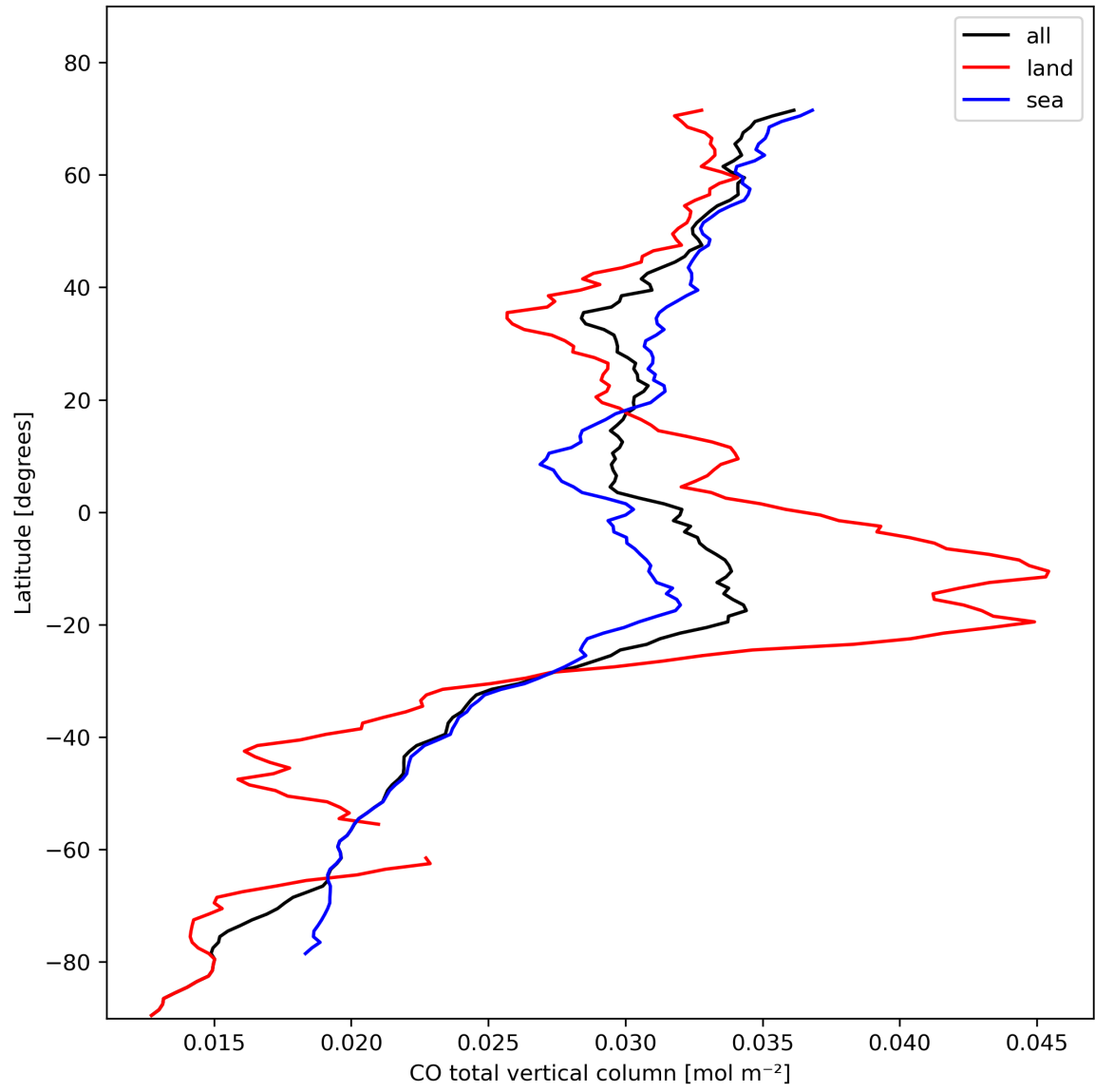
Figure 10: Zonal average of “CO total vertical column” for 2023-10-29 to 2023-10-31.
