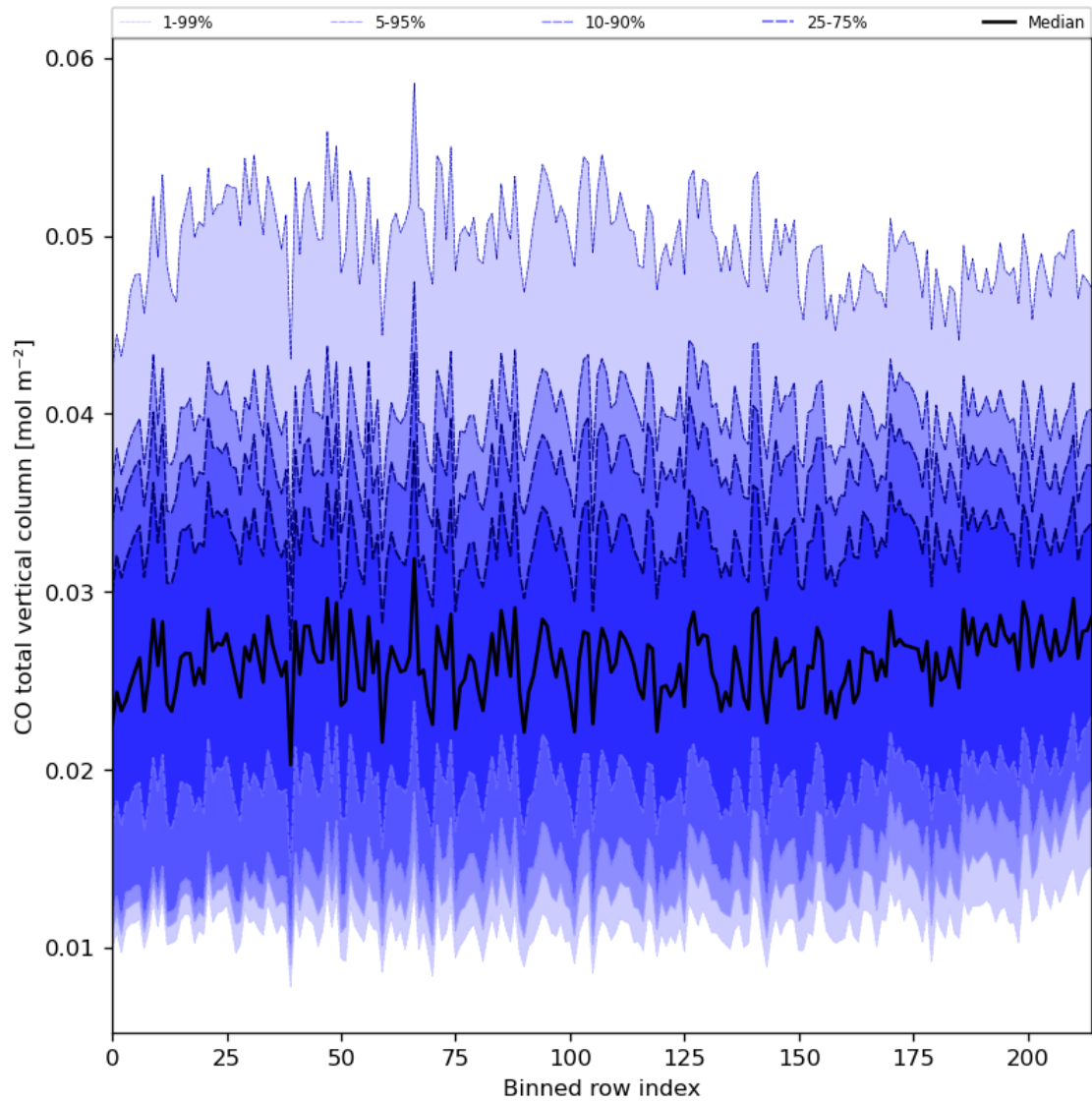
Figure 26: Along track statistics of “CO total vertical column” for 2023-10-29 to 2023-10-31
