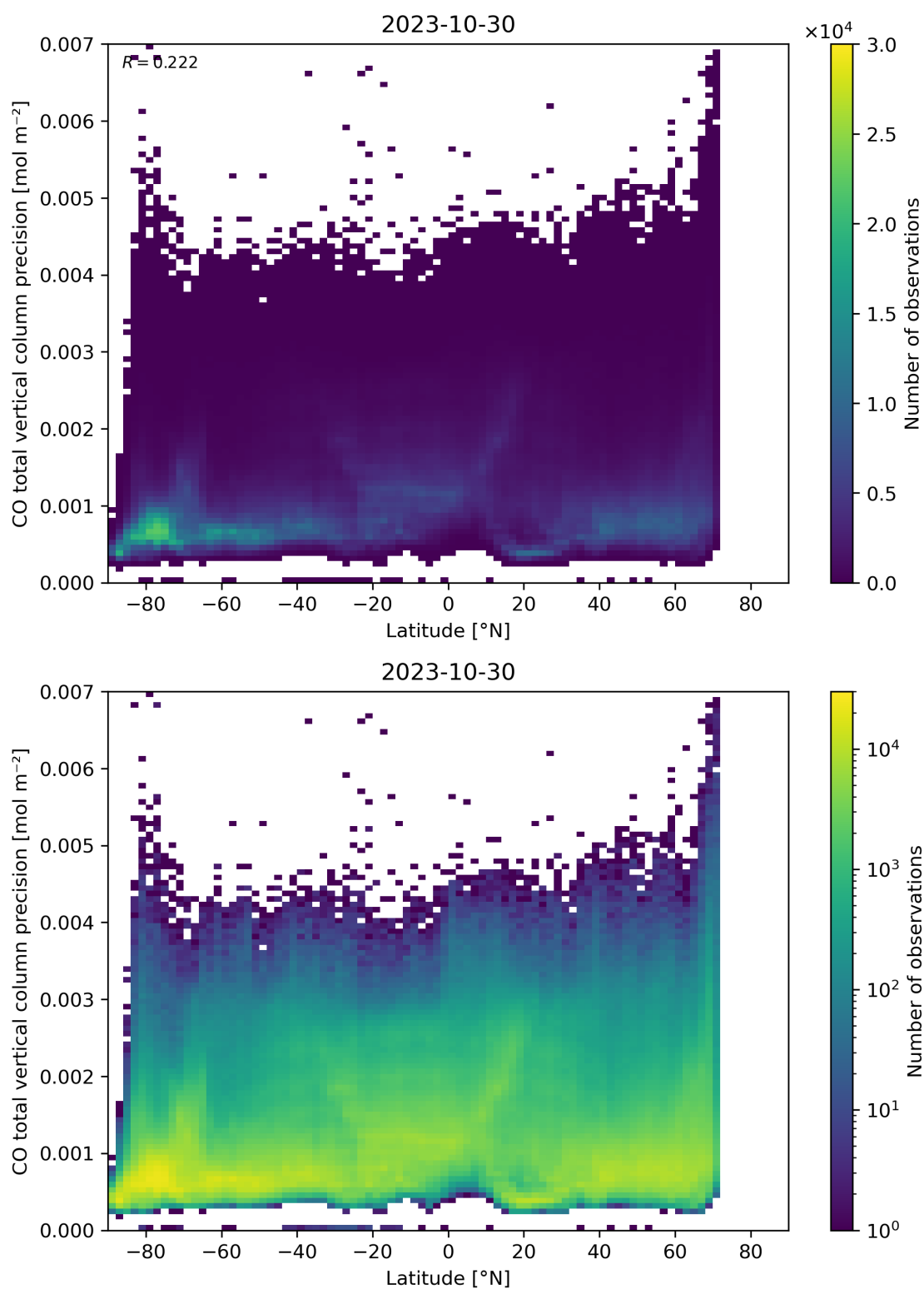
Figure 53: Scatter density plot of “Latitude” against “CO total vertical column precision” for 2023-10-29 to 2023-10-31.
