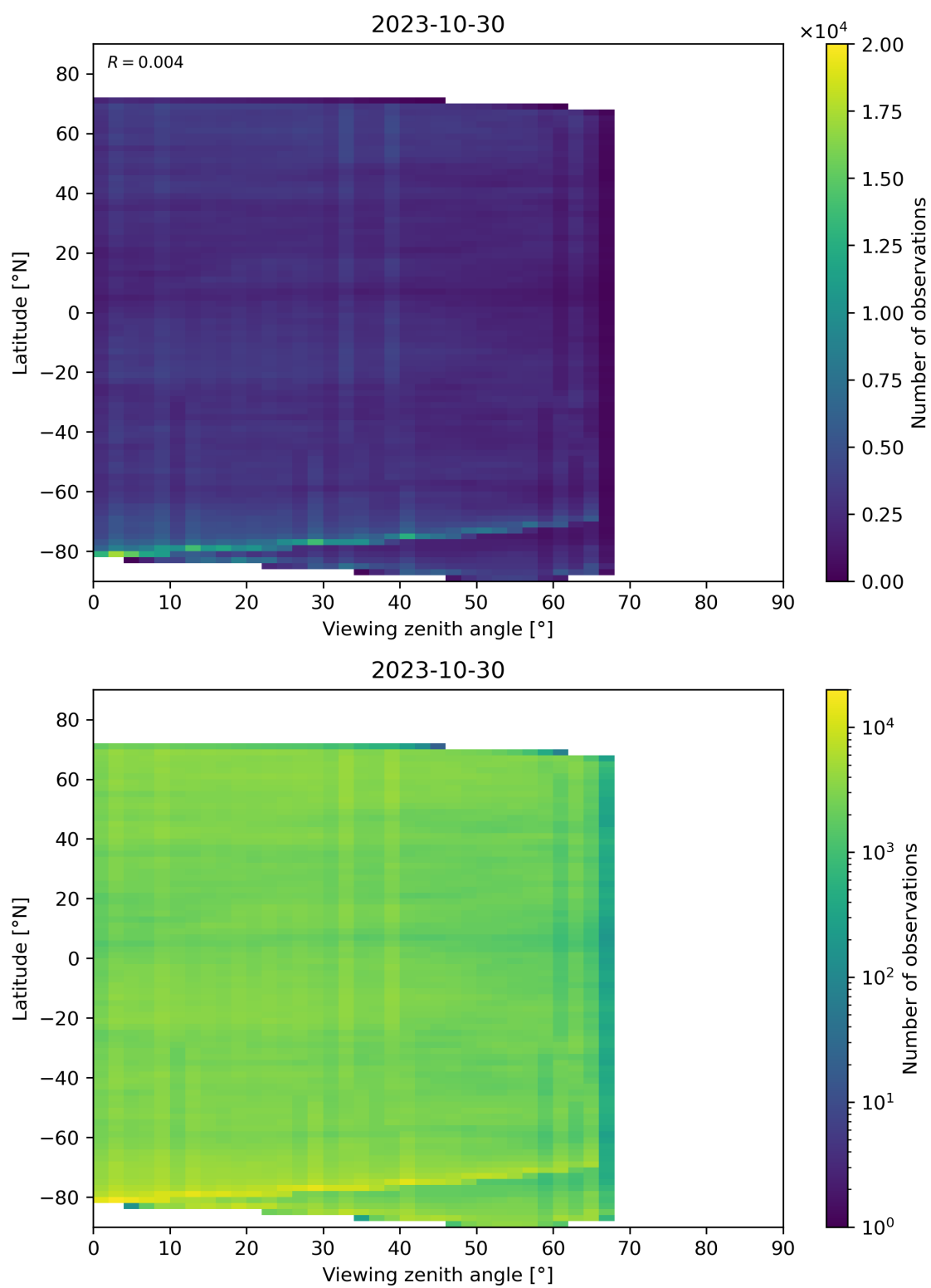
Figure 74: Scatter density plot of “Viewing zenith angle” against “Latitude” for 2023-10-29 to 2023-10-31.
