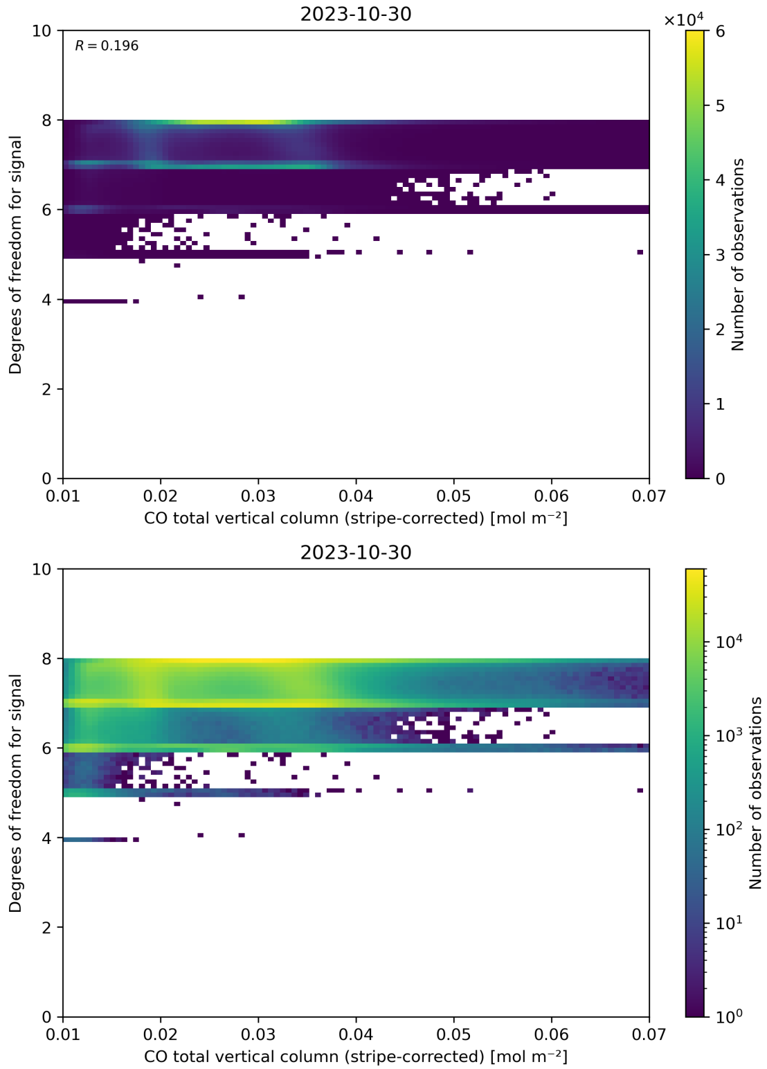
Figure 38: Scatter density plot of “CO total vertical column (stripe-corrected)” against “Degrees of freedom for signal” for 2023-10-29 to 2023-10-31.
