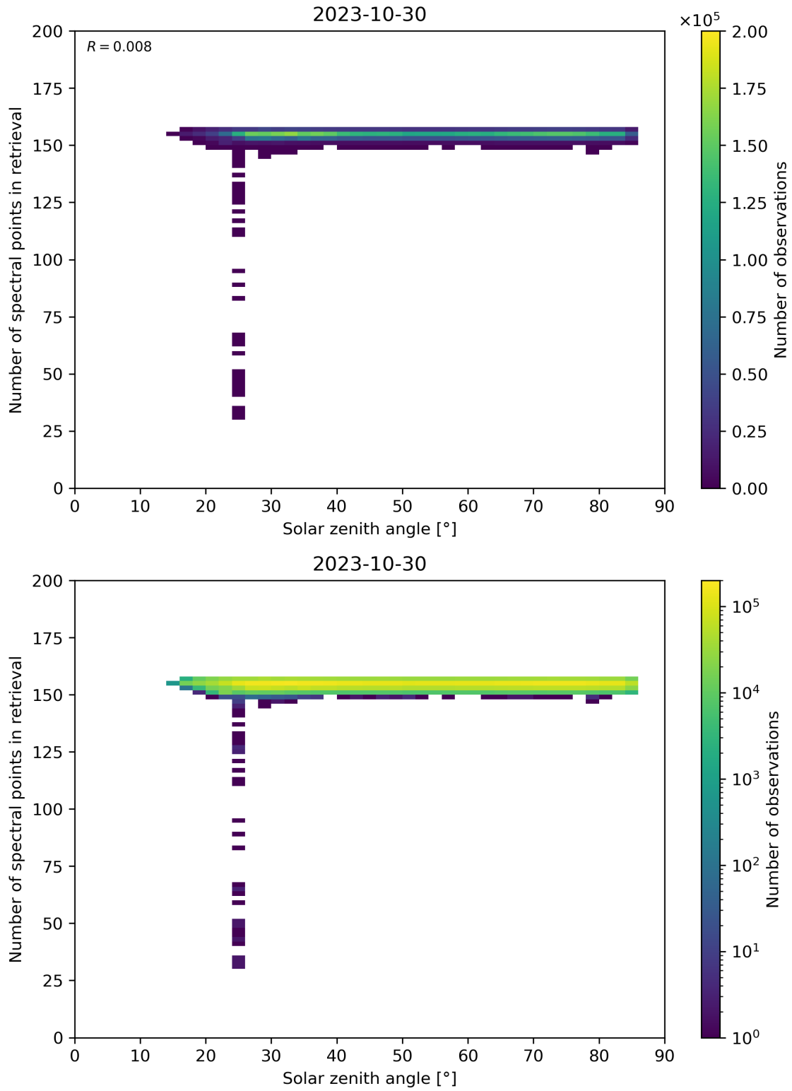
Figure 68: Scatter density plot of “Solar zenith angle” against “Number of spectral points in retrieval” for 2023-10-29 to 2023-10-31.
