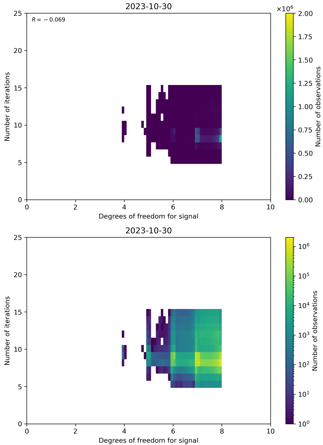
Figure 50: Scatter density plot of “Degrees of freedom for signal” against “Number of iterations” for 2023-10-29 to 2023-10-31.
