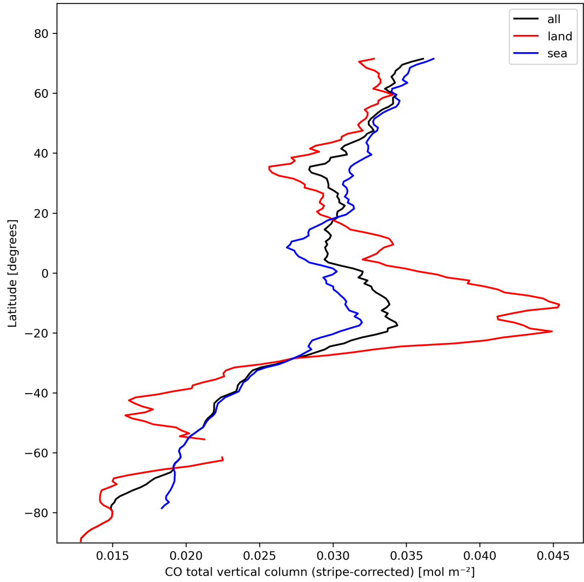
Figure 11: Zonal average of “CO total vertical column (stripe-corrected)” for 2023-10-29 to 2023-10-31.
