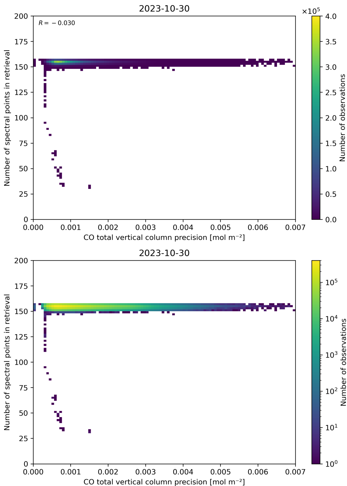
Figure 47: Scatter density plot of “CO total vertical column precision” against “Number of spectral points in retrieval” for 2023-10-29 to 2023-10-31.
