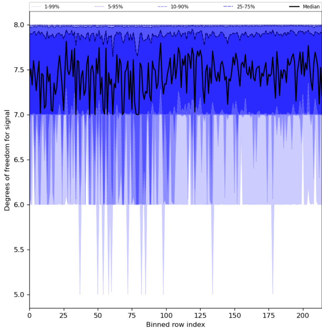
Figure 31: Along track statistics of “Degrees of freedom for signal” for 2023-10-29 to 2023-10-31
