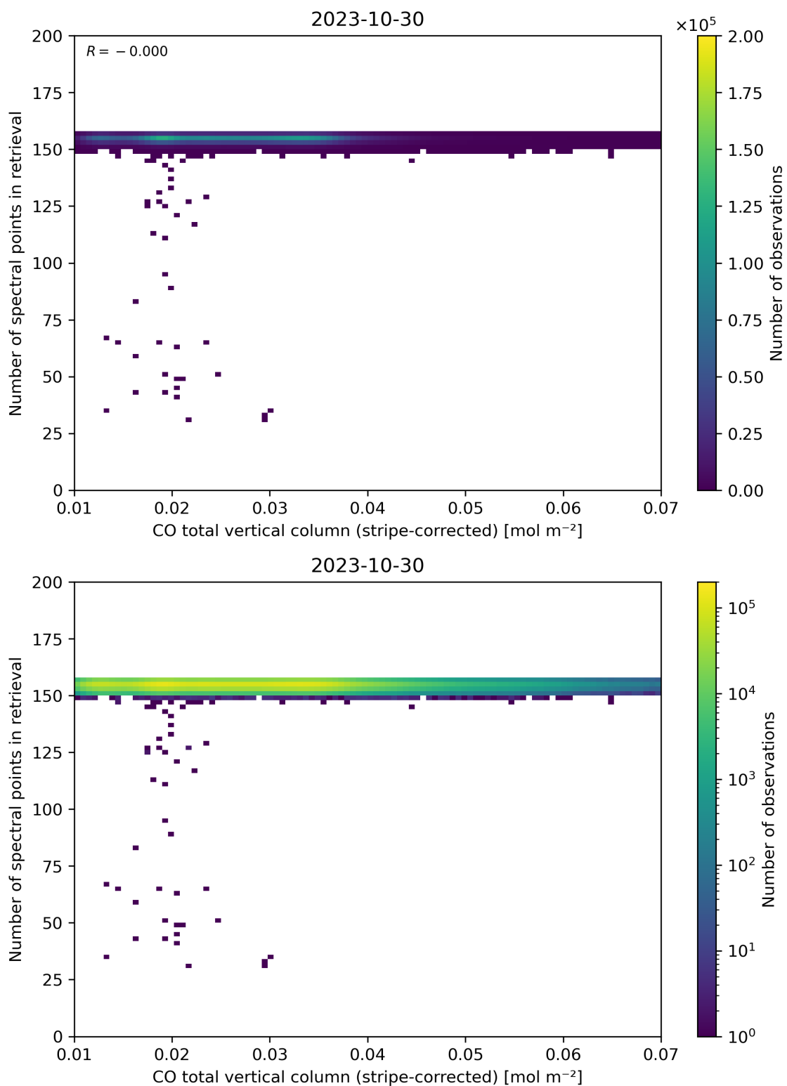
Figure 40: Scatter density plot of “CO total vertical column (stripe-corrected)” against “Number of spectral points in retrieval” for 2023-10-29 to 2023-10-31.
