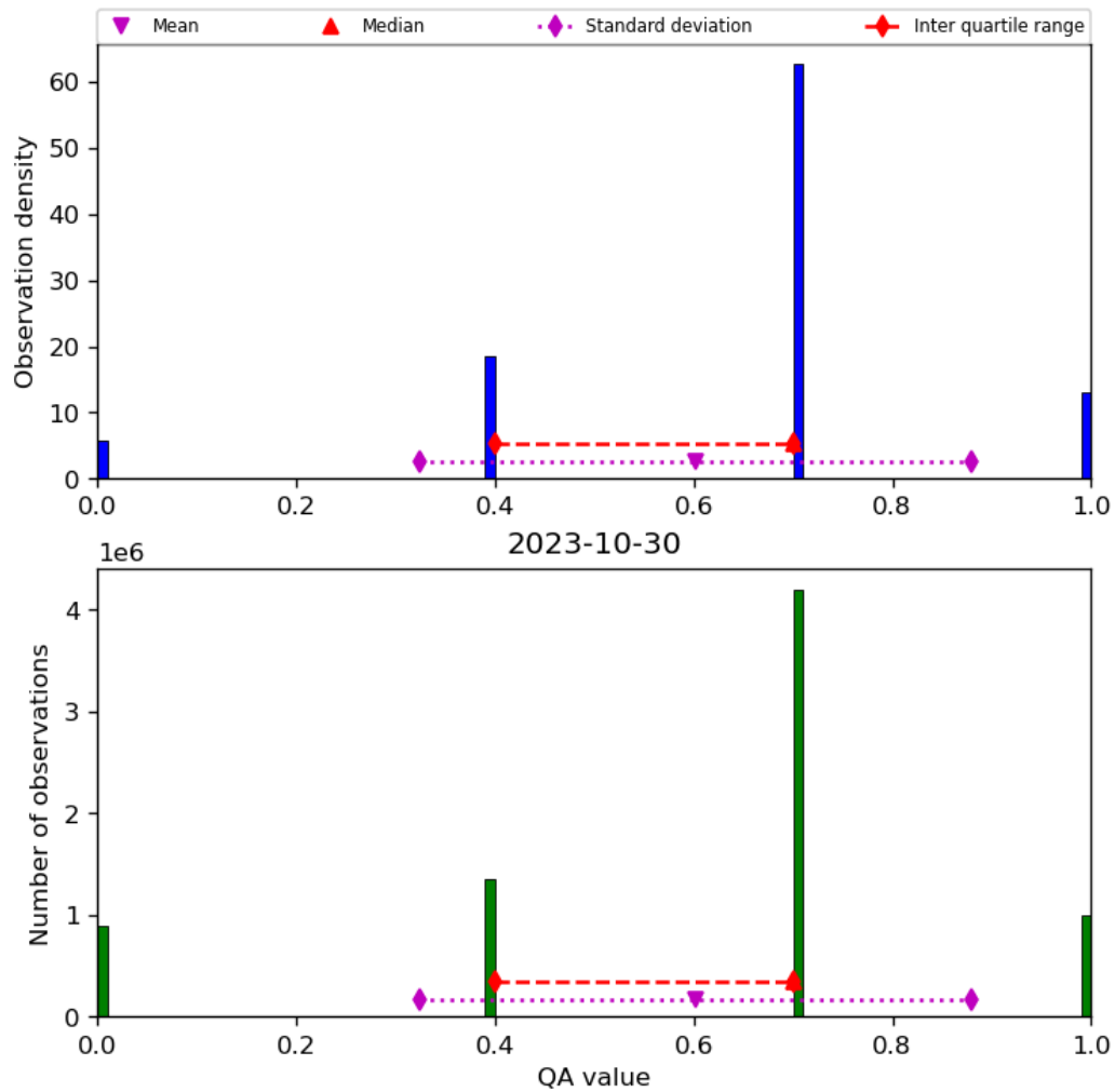
Figure 17: Histogram of “QA value” for 2023-10-29 to 2023-10-31
