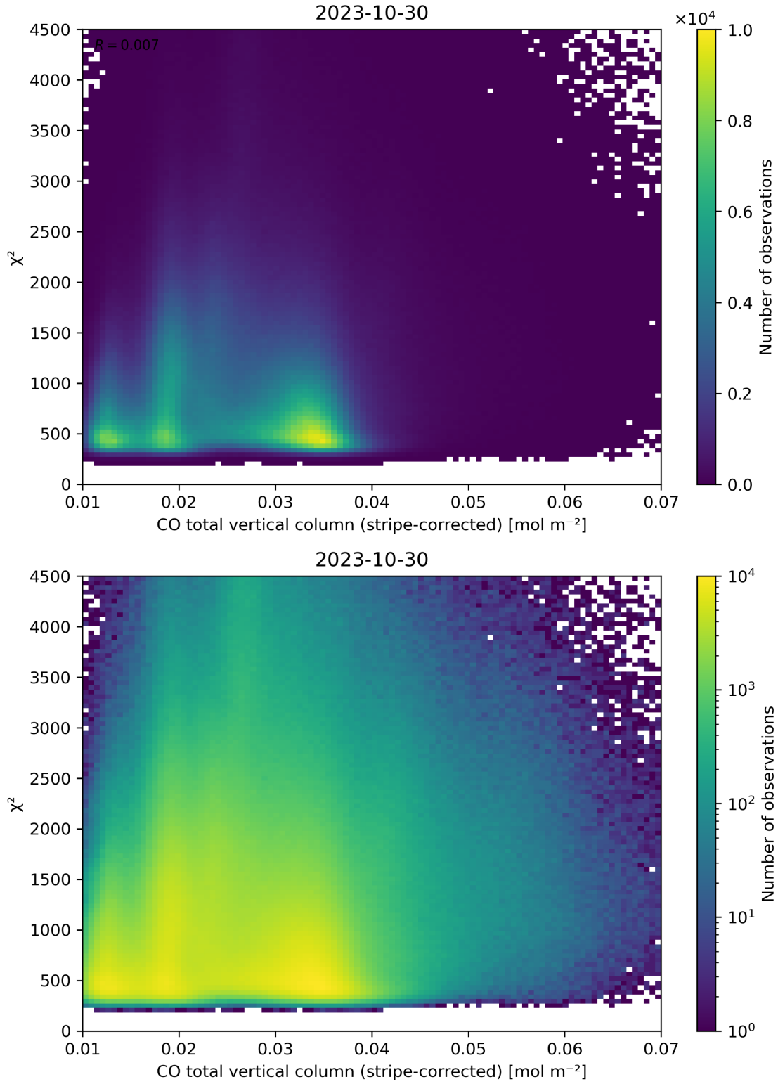
Figure 37: Scatter density plot of “CO total vertical column (stripe-corrected)” against “ \chi^2 ” for 2023-10-29 to 2023-10-31.
