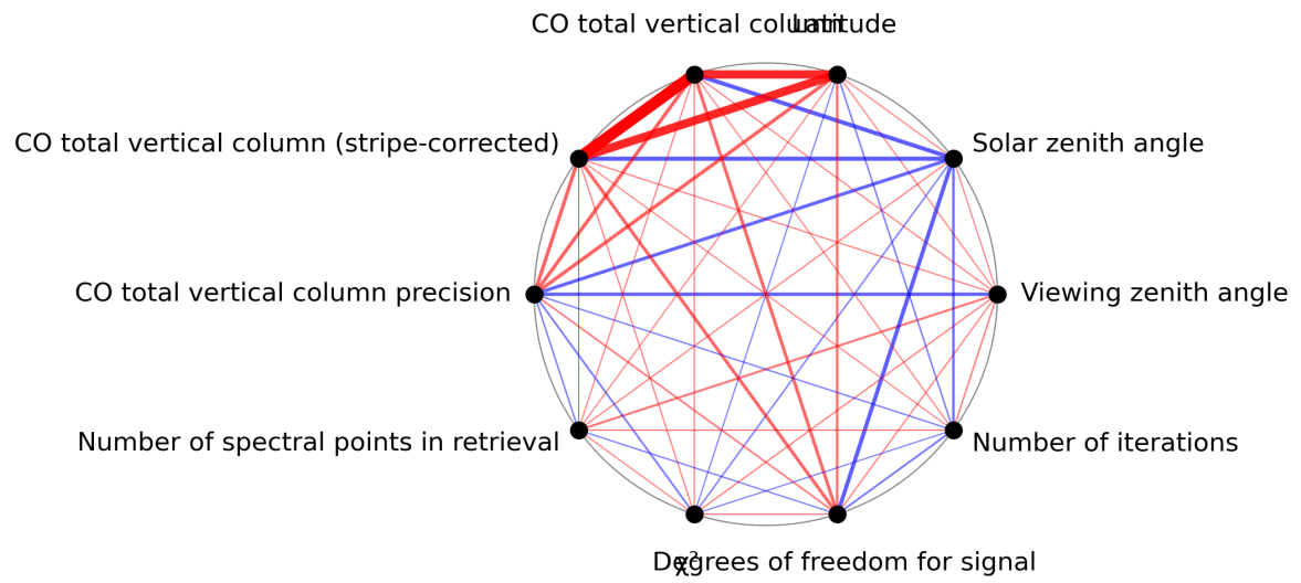
Figure 1: Map of correlation graph for 2023-10-29 to 2023-10-31.
