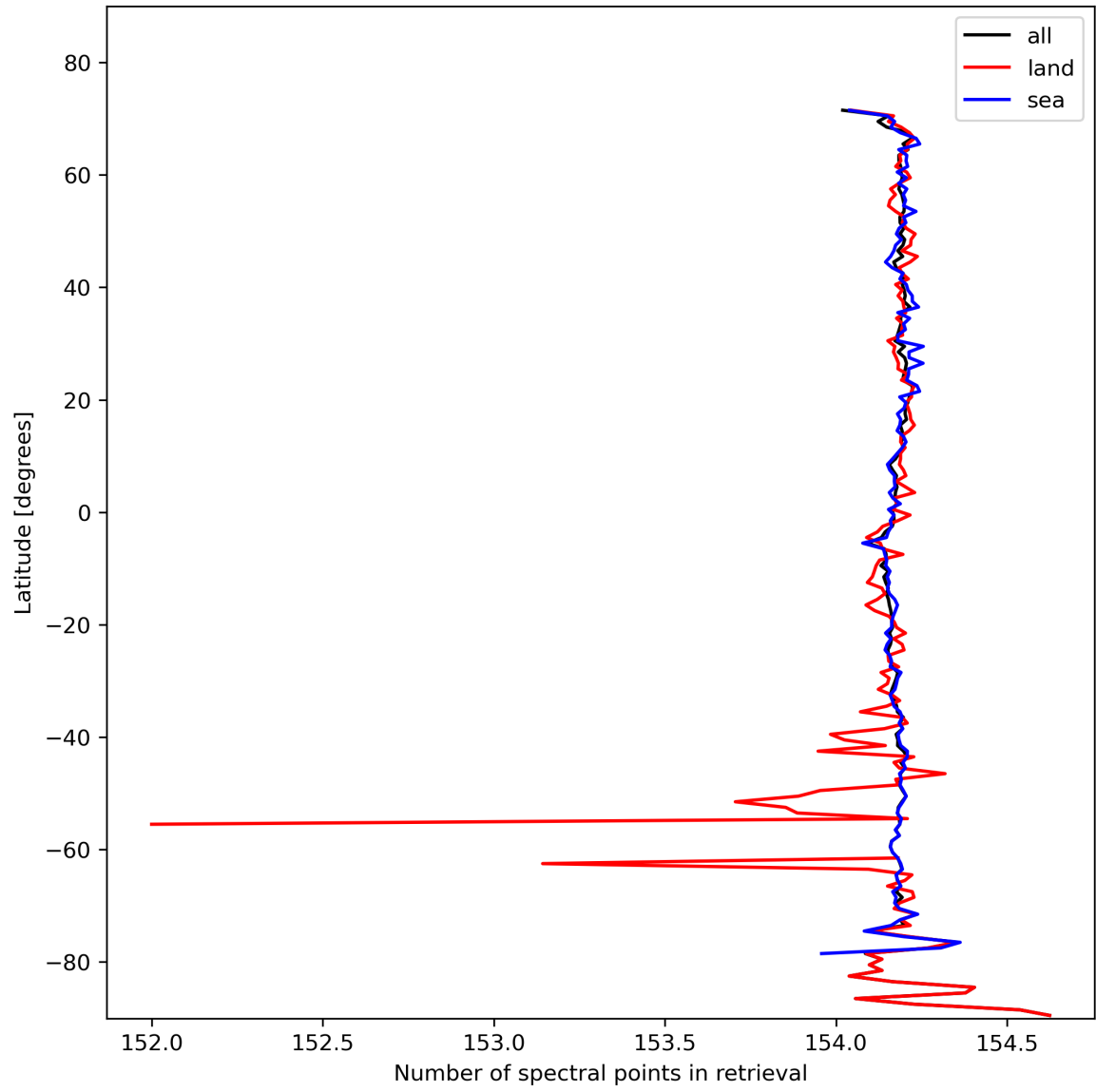
Figure 13: Zonal average of “Number of spectral points in retrieval” for 2023-10-29 to 2023-10-31.
