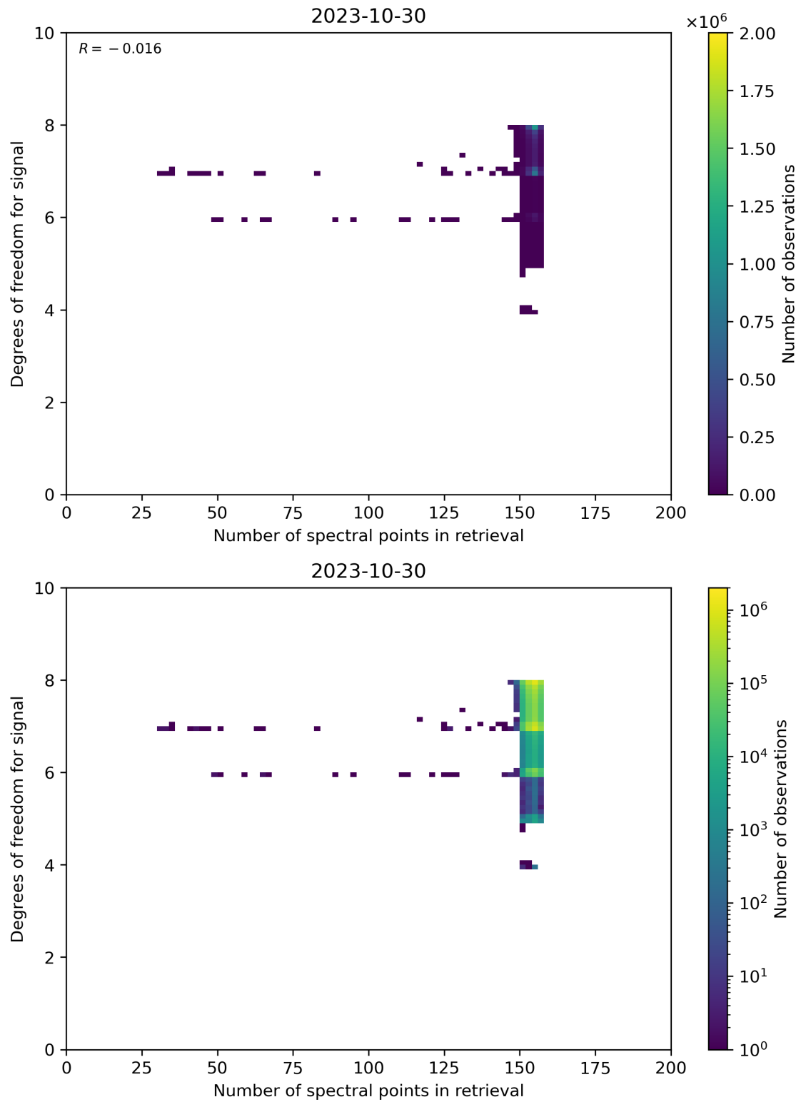
Figure 59: Scatter density plot of “Number of spectral points in retrieval” against “Degrees of freedom for signal” for 2023-10-29 to 2023-10-31.
