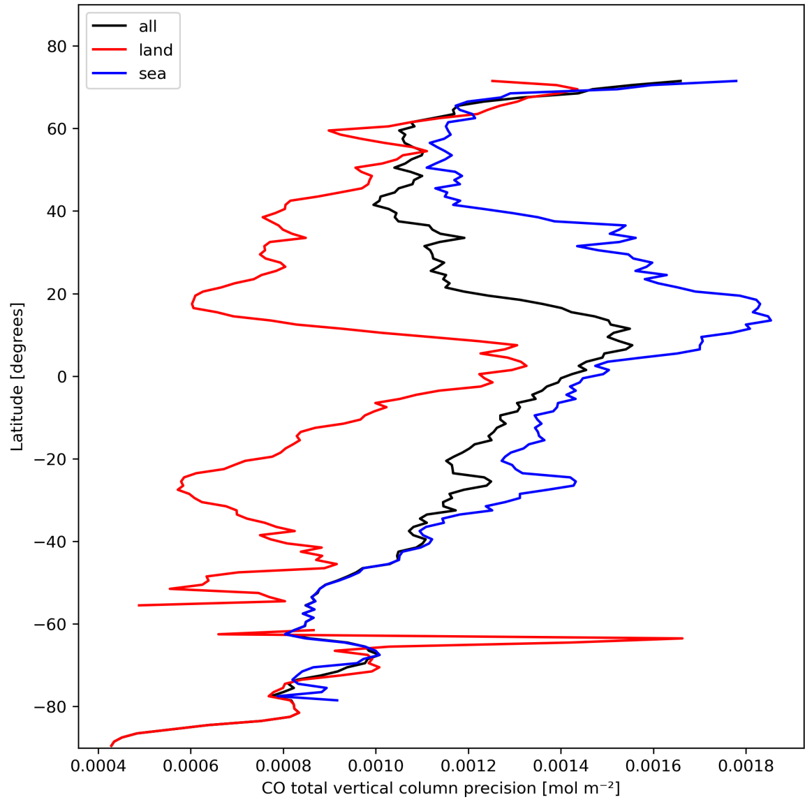
Figure 12: Zonal average of “CO total vertical column precision” for 2023-10-29 to 2023-10-31.
