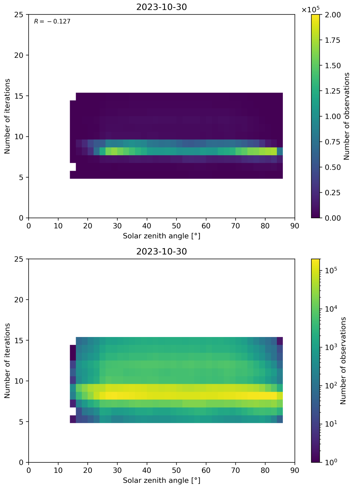
Figure 67: Scatter density plot of “Solar zenith angle” against “Number of iterations” for 2023-10-29 to 2023-10-31.
