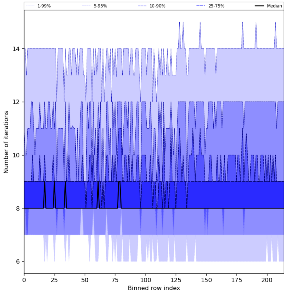
Figure 32: Along track statistics of “Number of iterations” for 2023-10-29 to 2023-10-31
