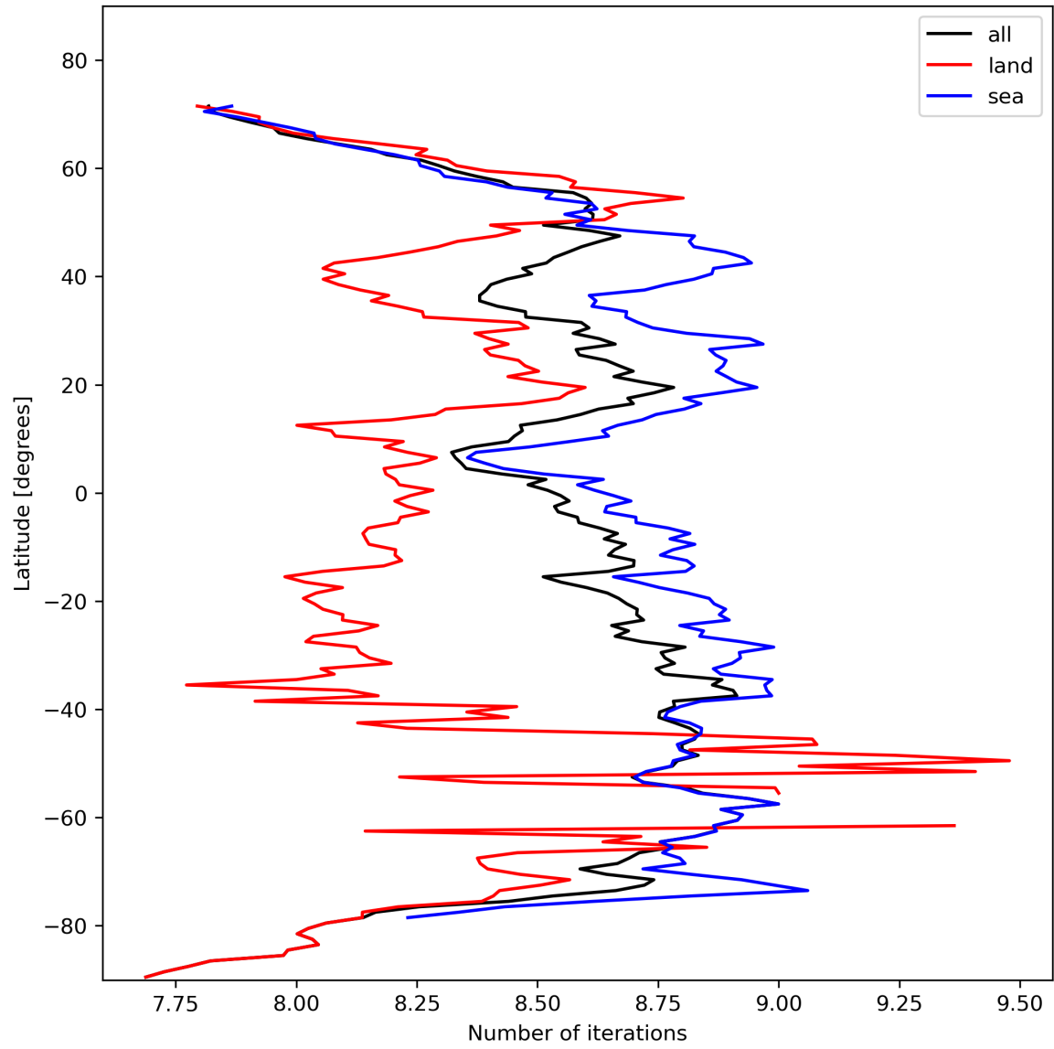
Figure 16: Zonal average of “Number of iterations” for 2023-10-29 to 2023-10-31.
