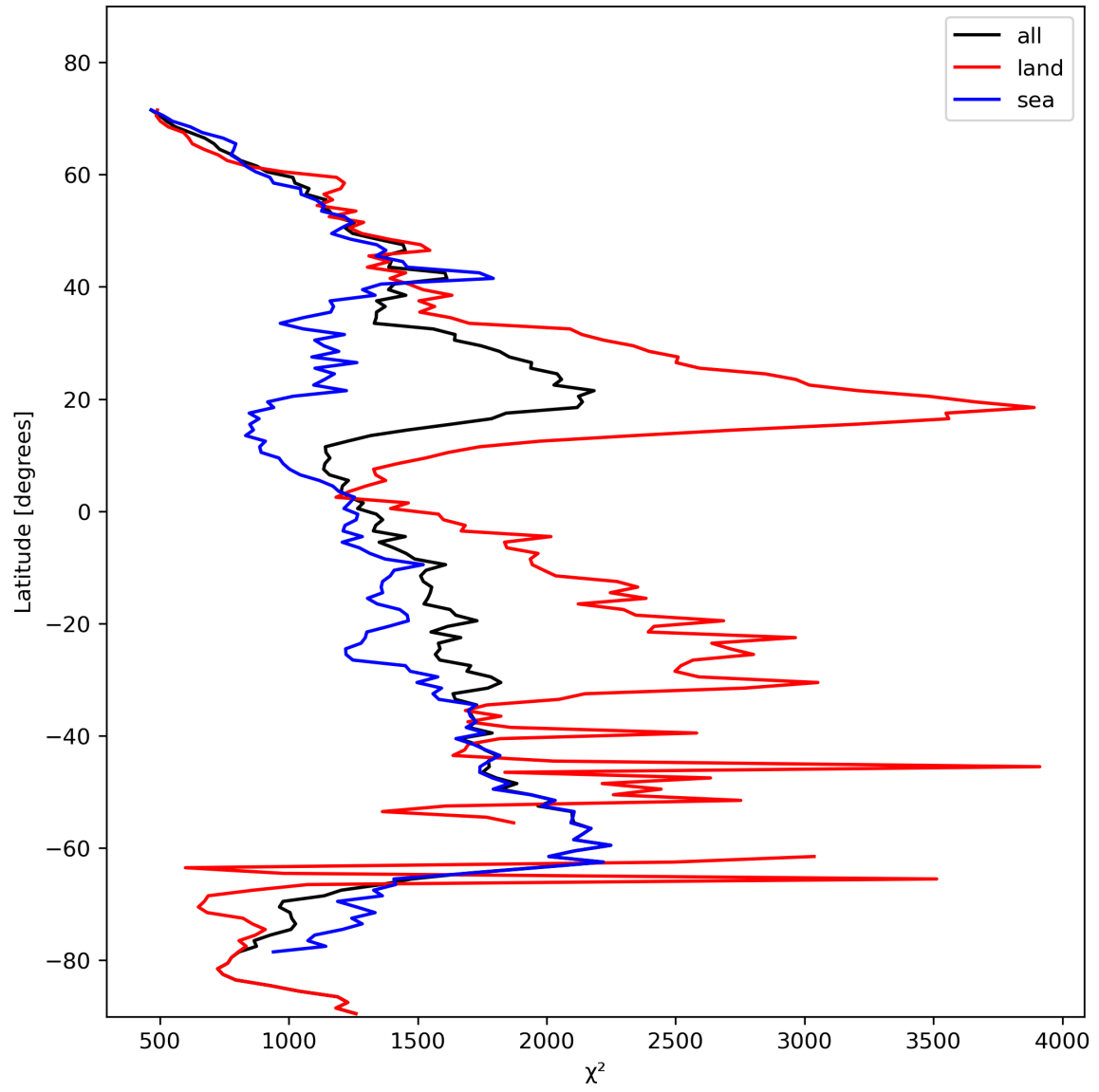
Figure 14: Zonal average of “ \chi^2 ” for 2023-10-29 to 2023-10-31.
