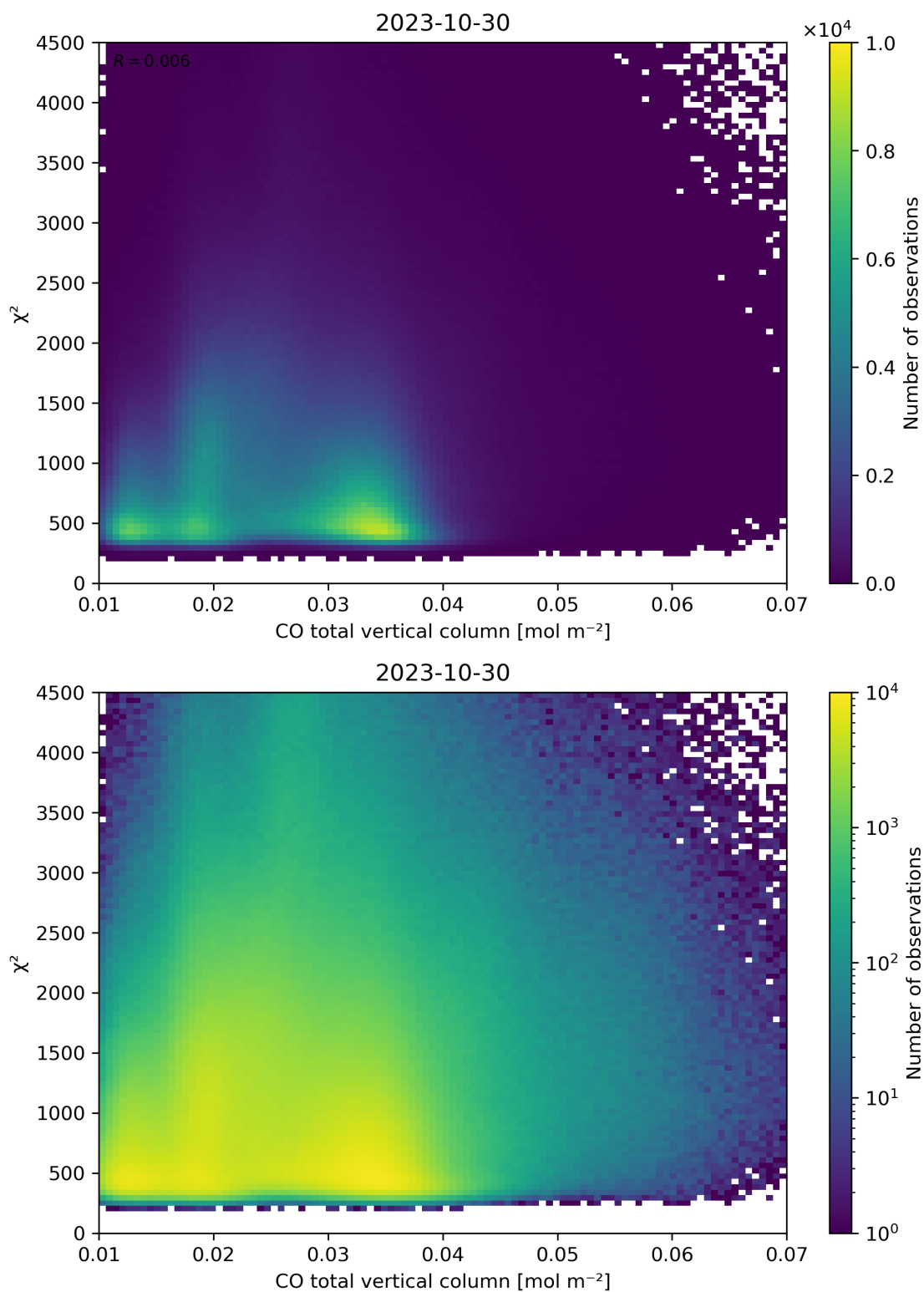
Figure 35: Scatter density plot of “CO total vertical column” against “ \chi^2 ” for 2023-10-29 to 2023-10-31.
