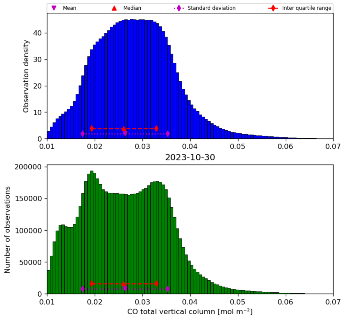
Figure 18: Histogram of “CO total vertical column” for 2023-10-29 to 2023-10-31
