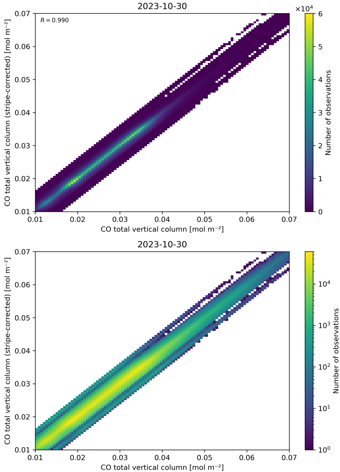
Figure 33: Scatter density plot of “CO total vertical column” against “CO total vertical column (stripe-corrected)” for 2023-10-29 to 2023-10-31.
