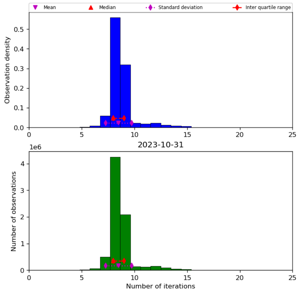
Figure 24: Histogram of “Number of iterations” for 2023-10-30 to 2023-11-01
