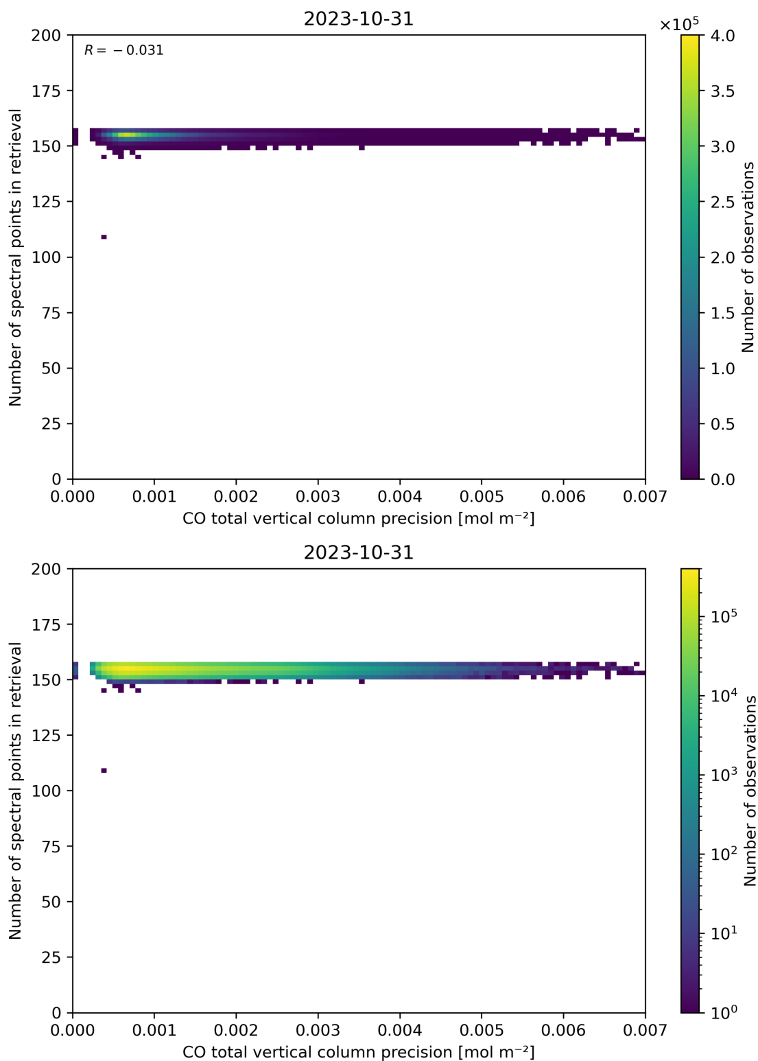
Figure 47: Scatter density plot of “CO total vertical column precision” against “Number of spectral points in retrieval” for 2023-10-30 to 2023-11-01.
