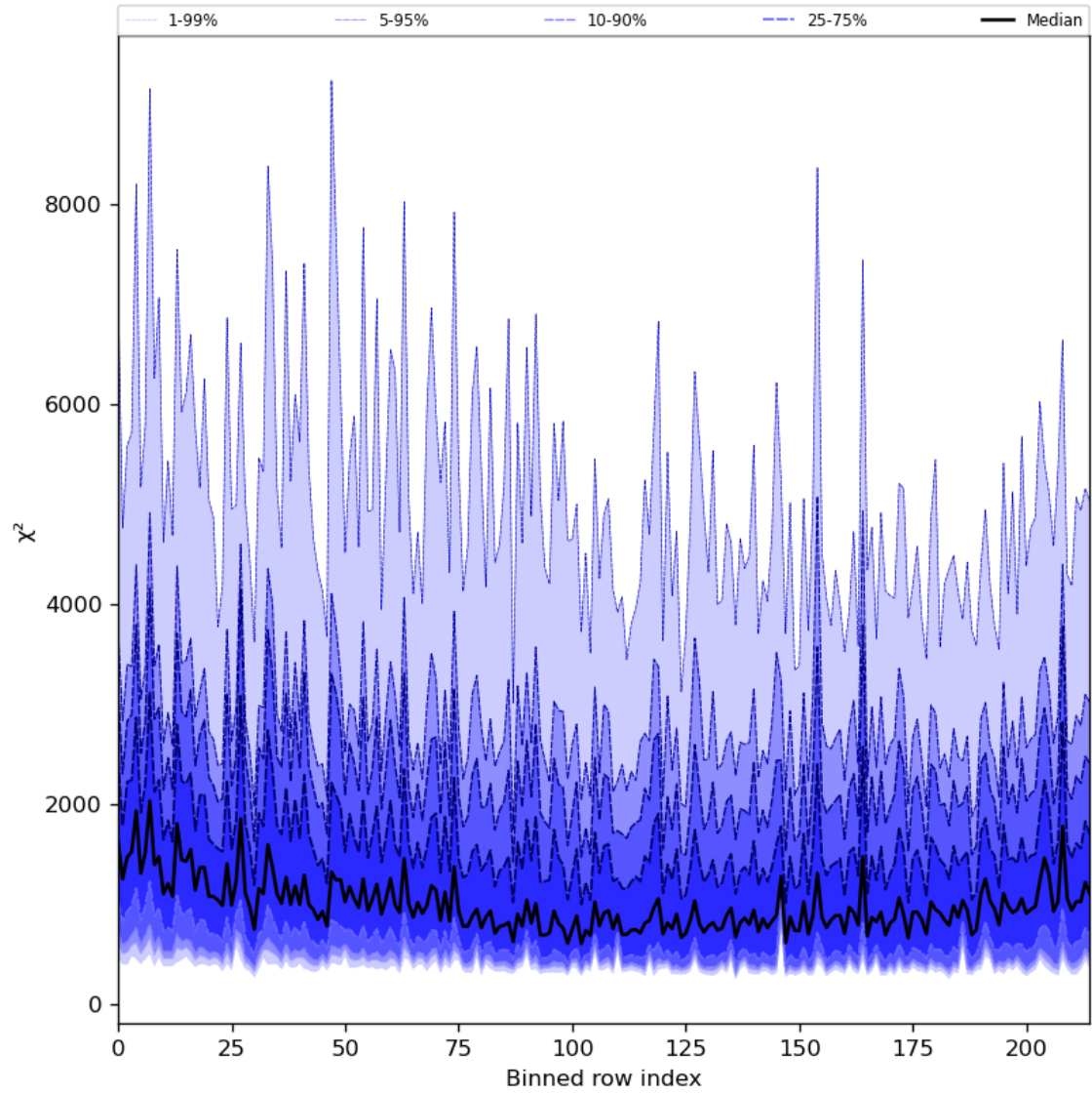
Figure 30: Along track statistics of “ \chi^2 ” for 2023-10-30 to 2023-11-01
