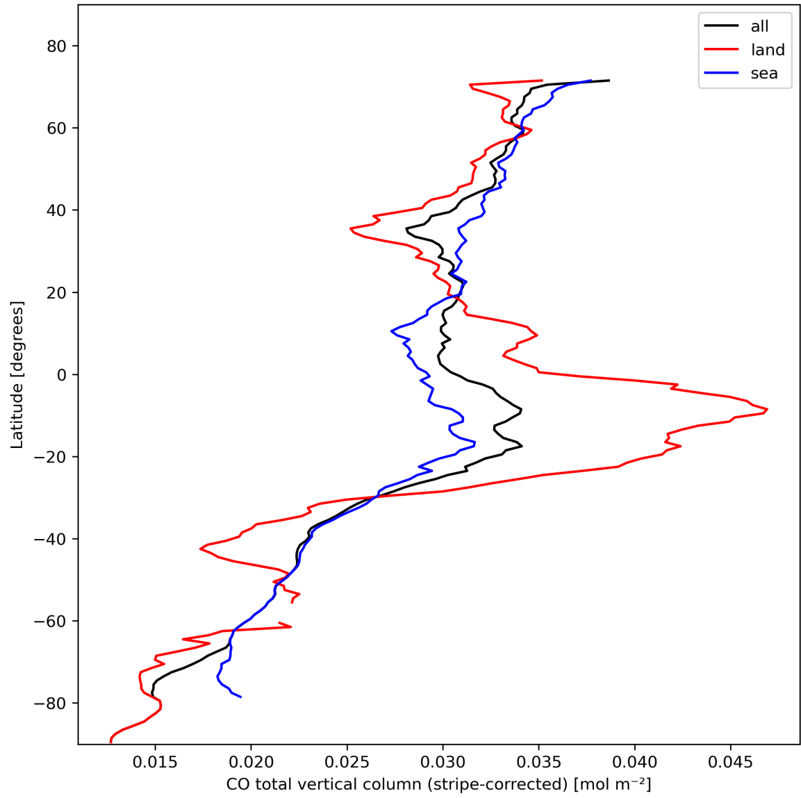
Figure 11: Zonal average of “CO total vertical column (stripe-corrected)” for 2023-10-30 to 2023-11-01.
