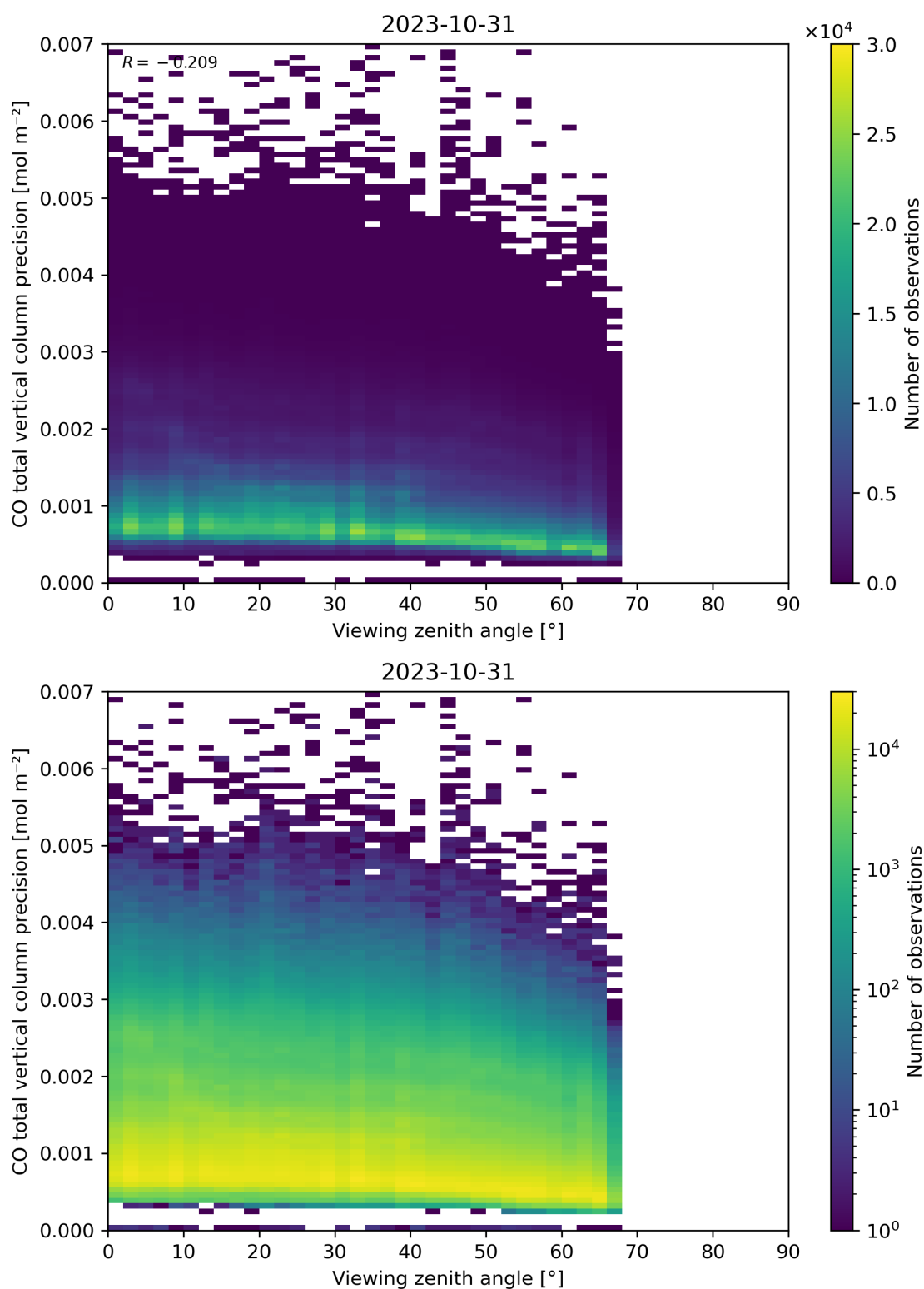
Figure 71: Scatter density plot of “Viewing zenith angle” against “CO total vertical column precision” for 2023-10-30 to 2023-11-01.
