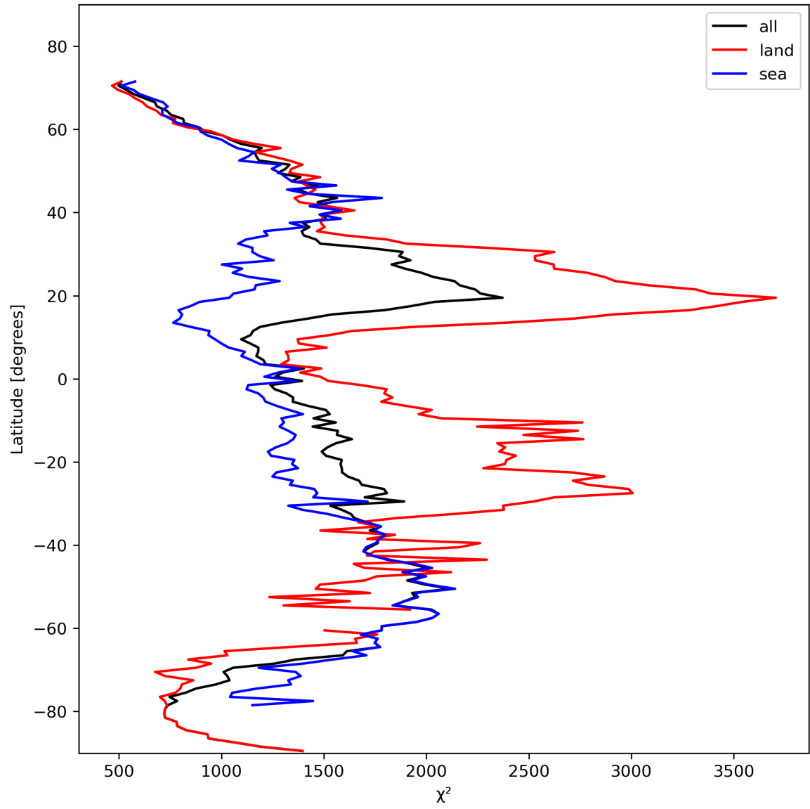
Figure 14: Zonal average of “ \chi^2 ” for 2023-10-30 to 2023-11-01.
