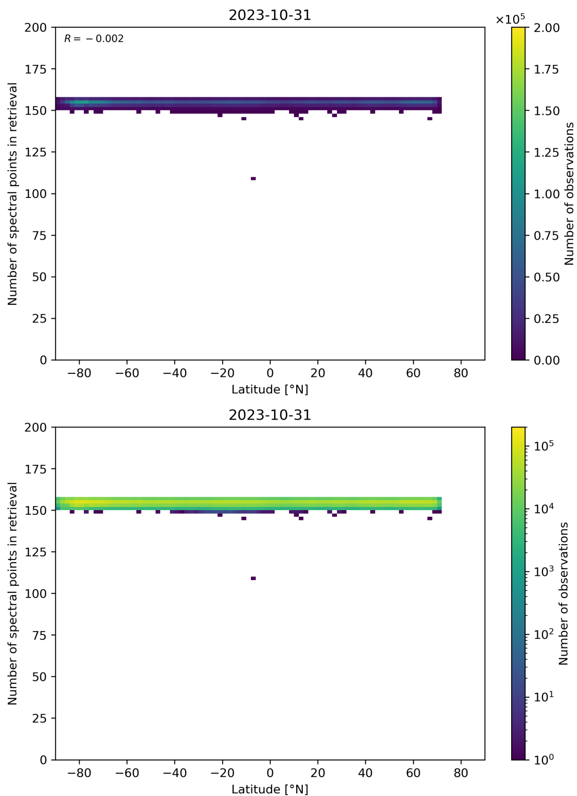
Figure 57: Scatter density plot of “Latitude” against “Number of spectral points in retrieval” for 2023-10-30 to 2023-11-01.
