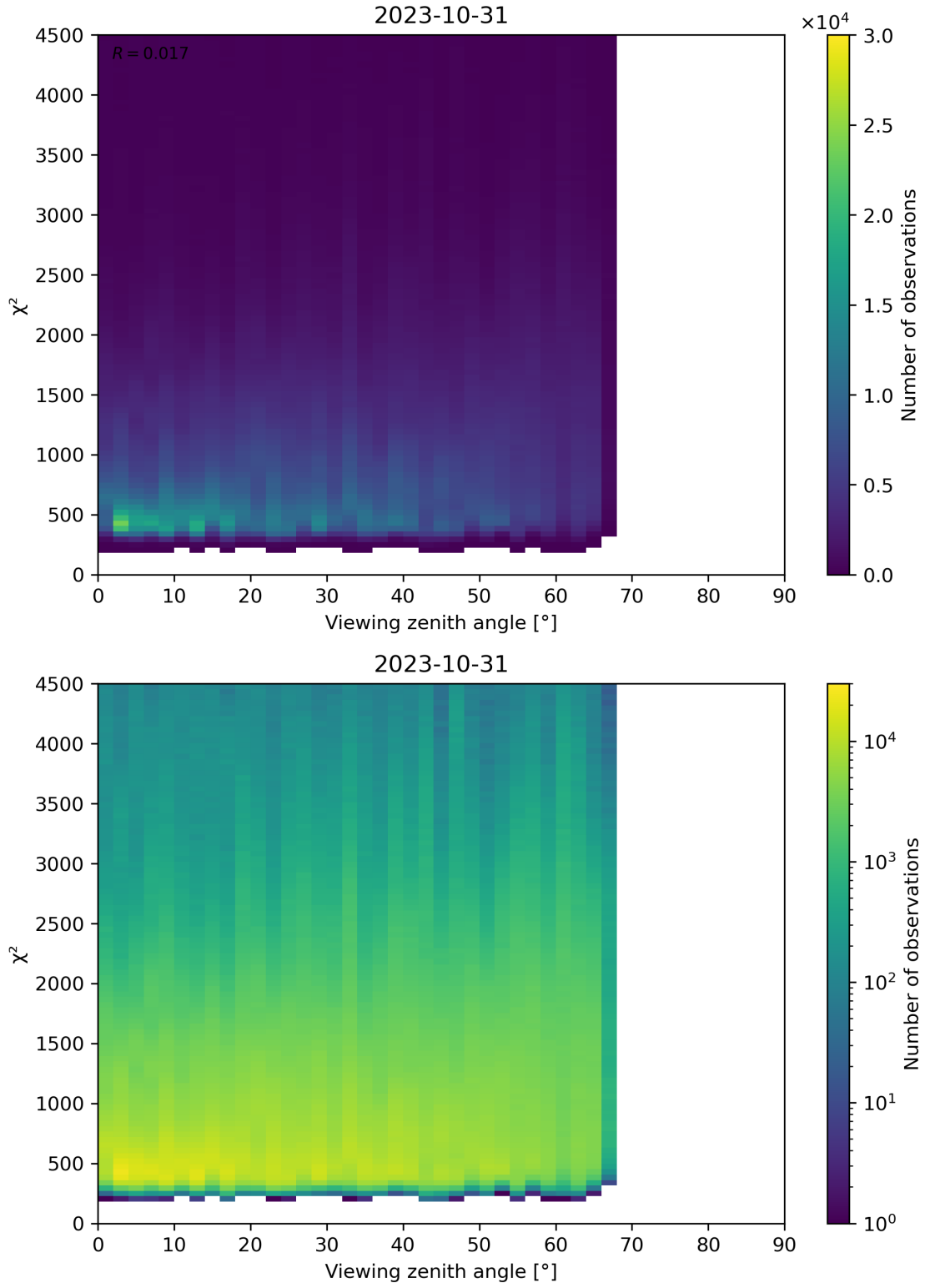
Figure 72: Scatter density plot of “Viewing zenith angle” against “ \chi^2 ” for 2023-10-30 to 2023-11-01.
