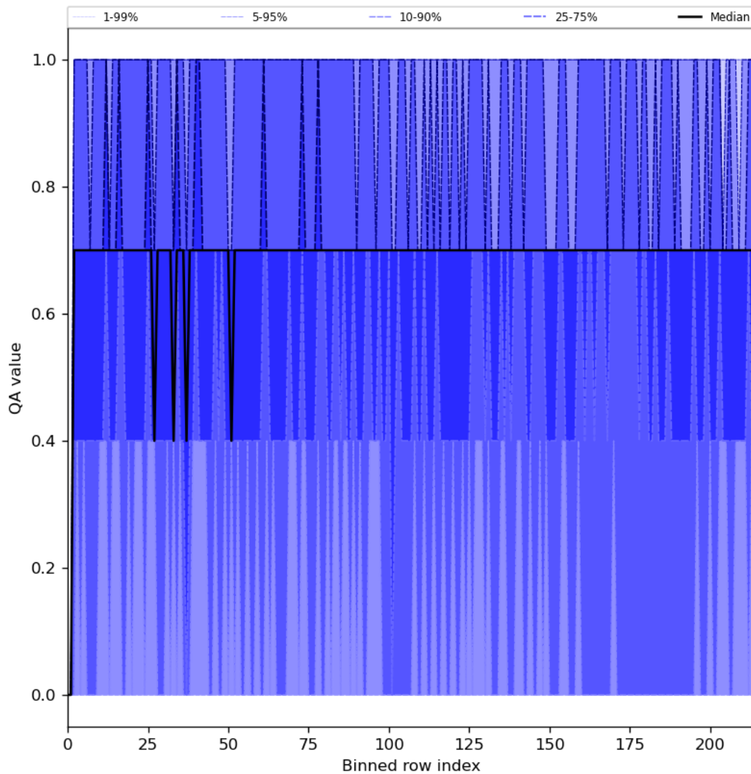
Figure 25: Along track statistics of “QA value” for 2023-10-30 to 2023-11-01
