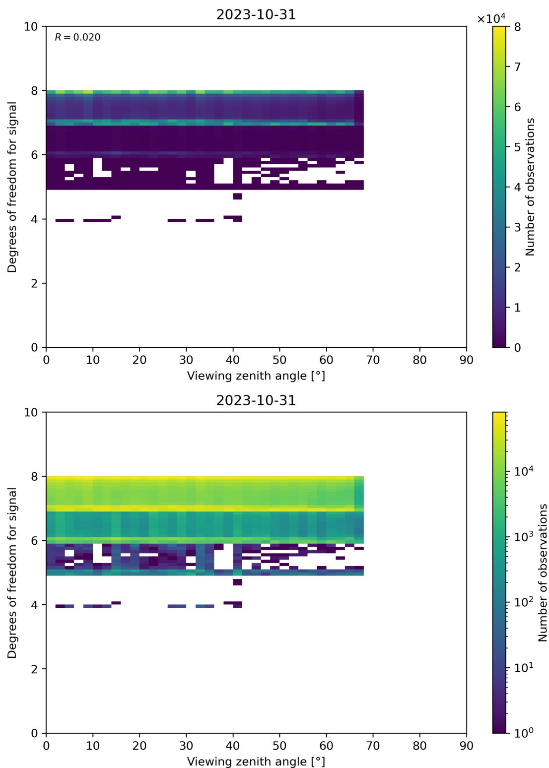
Figure 73: Scatter density plot of “Viewing zenith angle” against “Degrees of freedom for signal” for 2023-10-30 to 2023-11-01.
