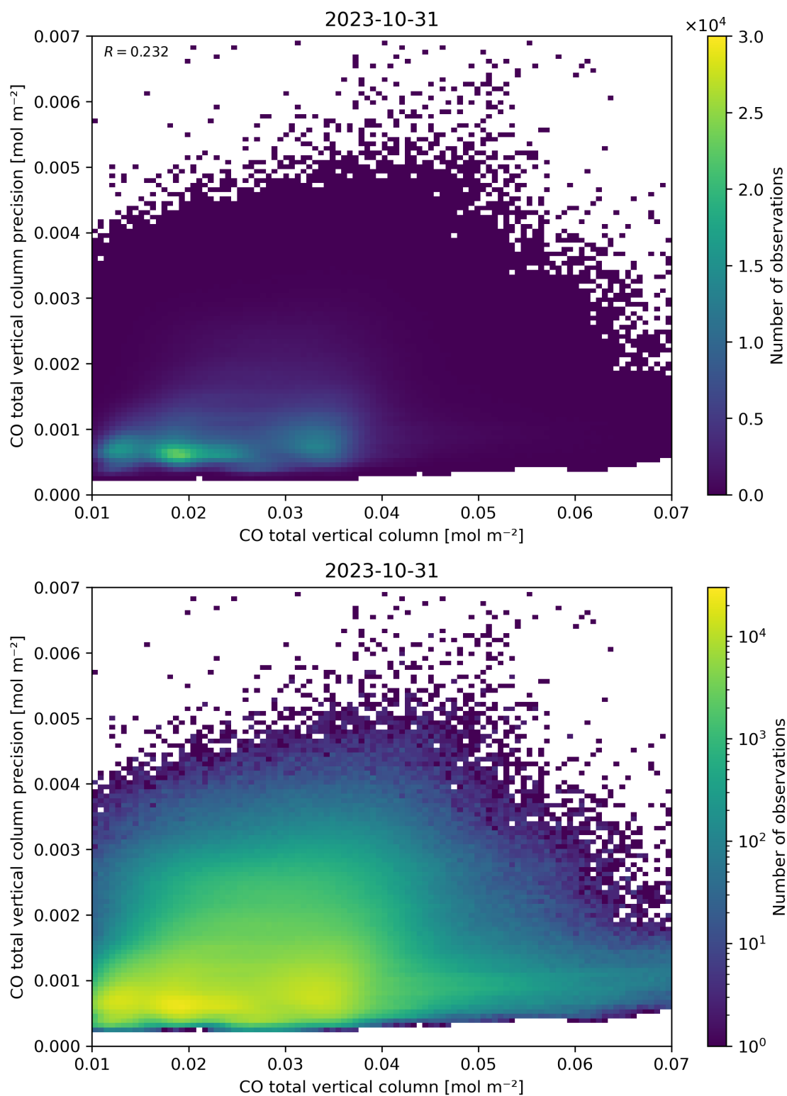
Figure 34: Scatter density plot of “CO total vertical column” against “CO total vertical column precision” for 2023-10-30 to 2023-11-01.
