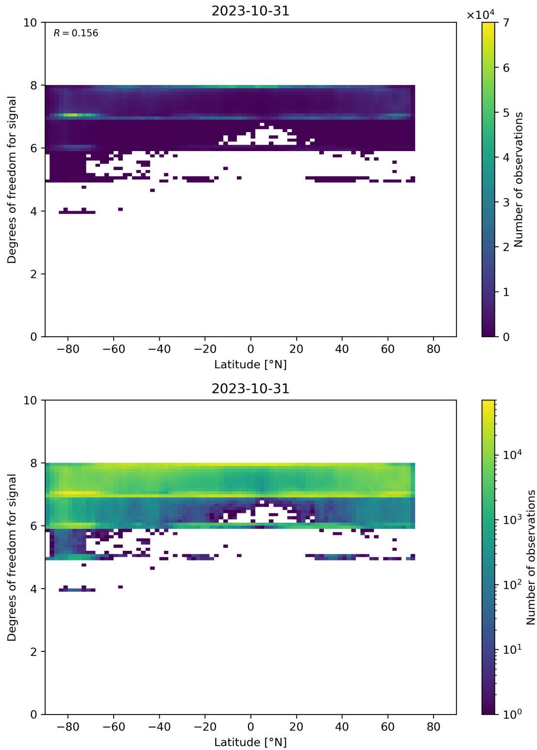
Figure 55: Scatter density plot of “Latitude” against “Degrees of freedom for signal” for 2023-10-30 to 2023-11-01.
