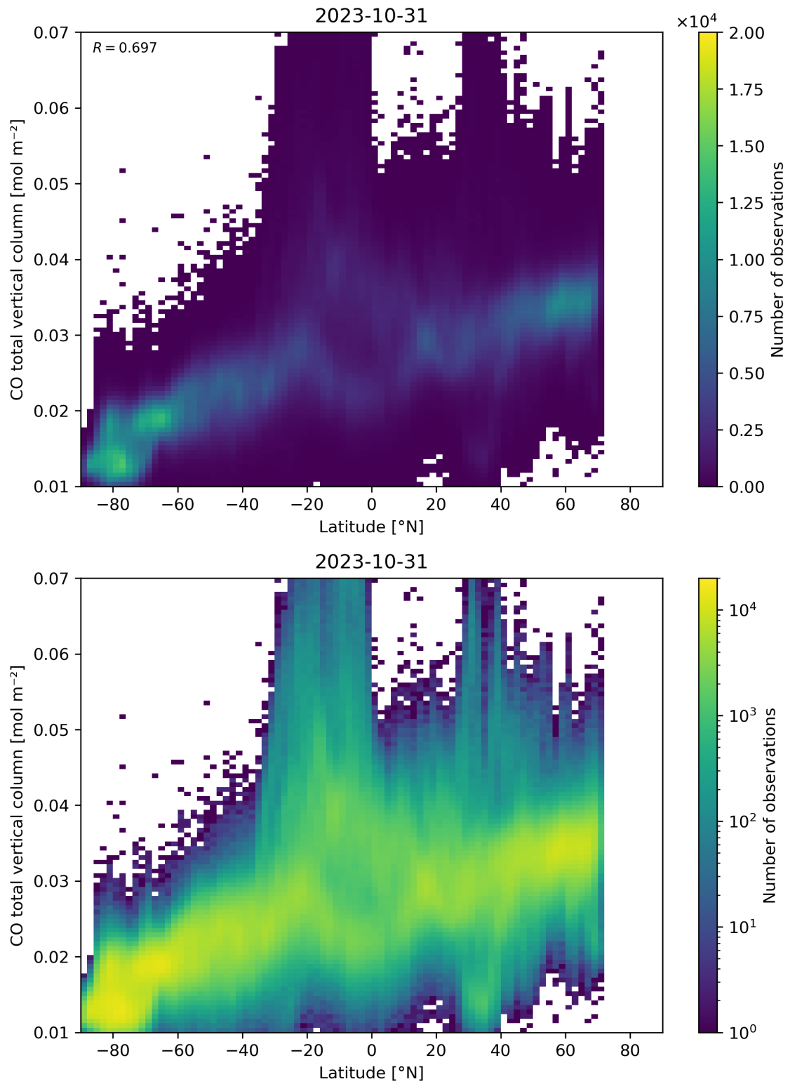
Figure 51: Scatter density plot of “Latitude” against “CO total vertical column” for 2023-10-30 to 2023-11-01.
