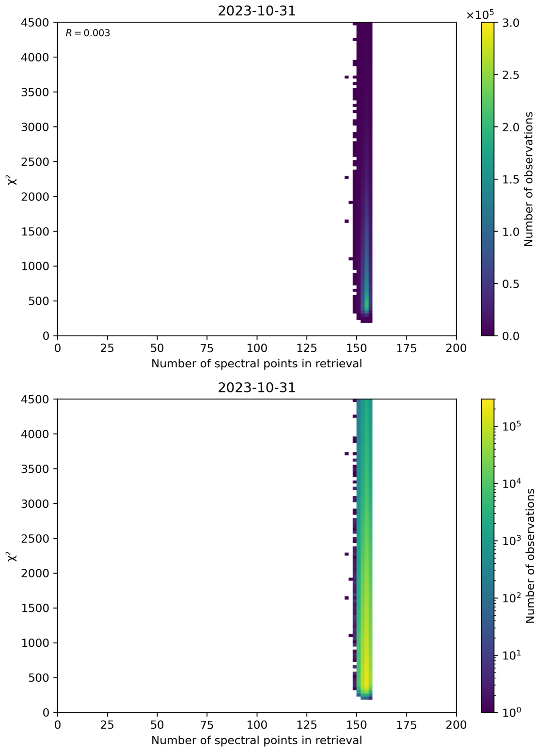
Figure 58: Scatter density plot of “Number of spectral points in retrieval” against “ \chi^2 ” for 2023-10-30 to 2023-11-01.
