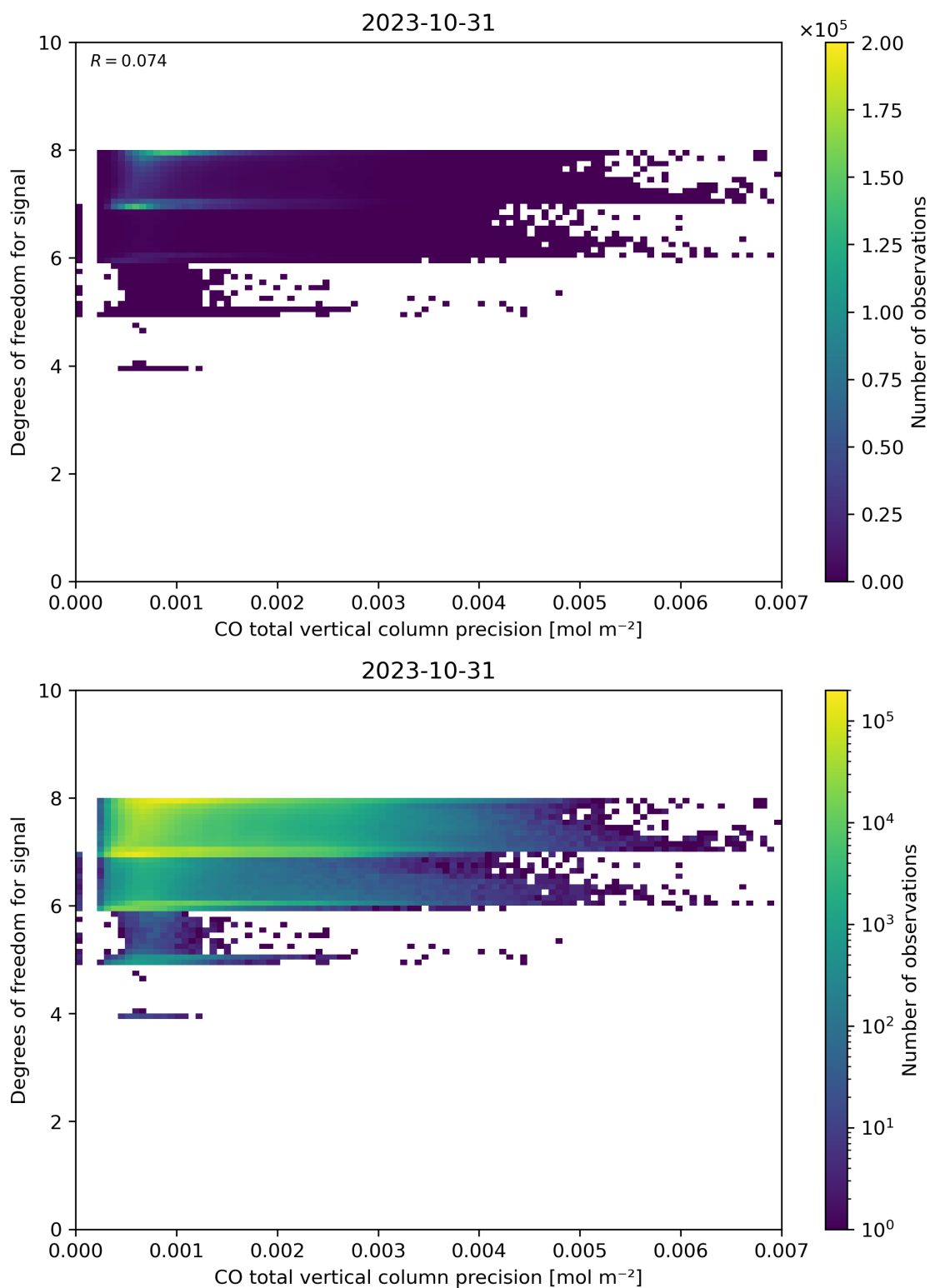
Figure 45: Scatter density plot of “CO total vertical column precision” against “Degrees of freedom for signal” for 2023-10-30 to 2023-11-01.
