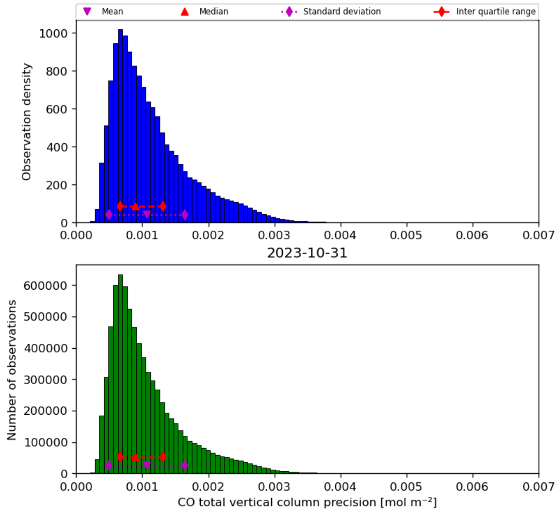
Figure 20: Histogram of “CO total vertical column precision” for 2023-10-30 to 2023-11-01
