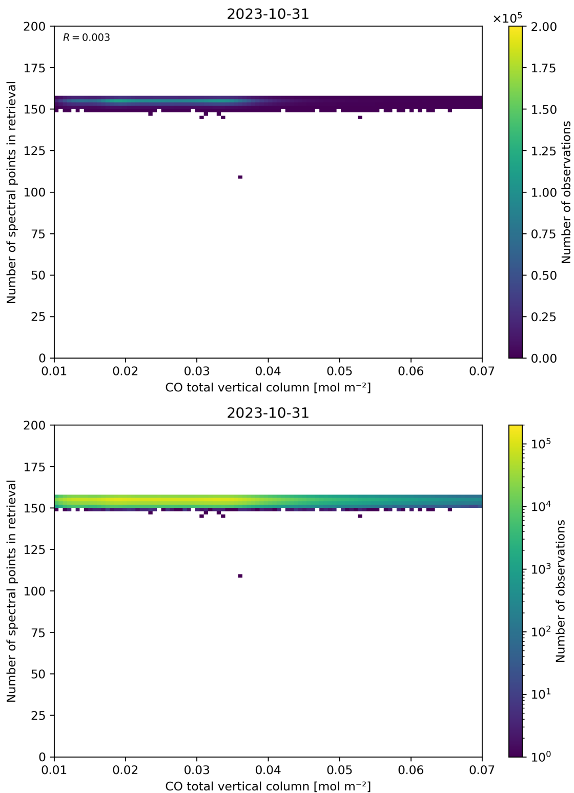
Figure 43: Scatter density plot of “CO total vertical column” against “Number of spectral points in retrieval” for 2023-10-30 to 2023-11-01.
