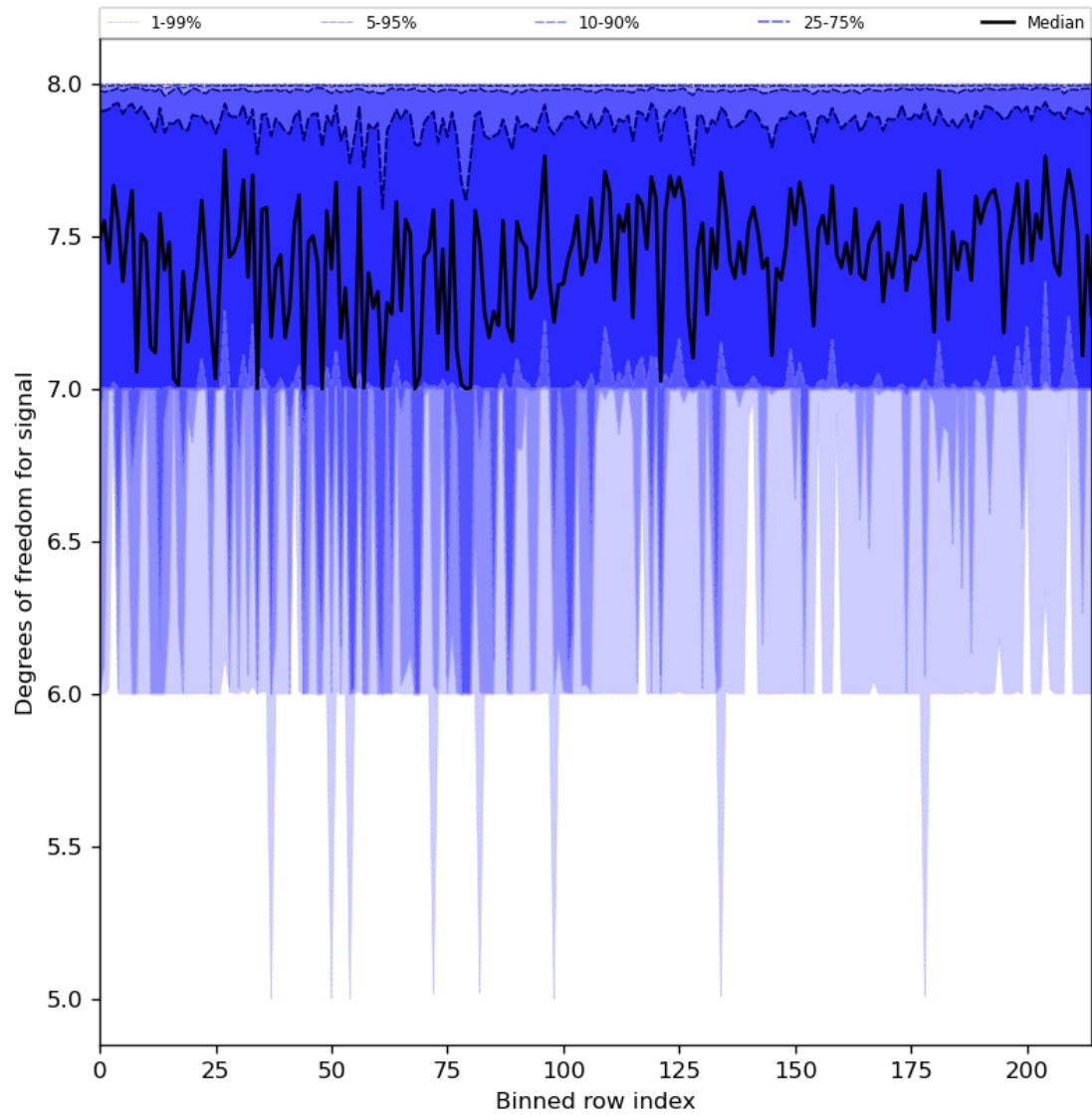
Figure 31: Along track statistics of “Degrees of freedom for signal” for 2023-10-30 to 2023-11-01
