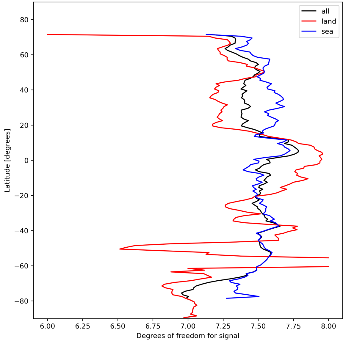
Figure 15: Zonal average of “Degrees of freedom for signal” for 2023-10-30 to 2023-11-01.
