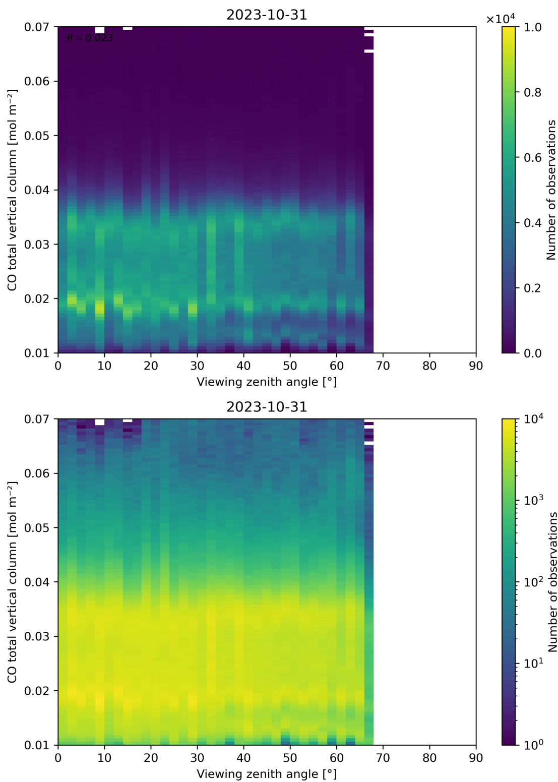
Figure 69: Scatter density plot of “Viewing zenith angle” against “CO total vertical column” for 2023-10-30 to 2023-11-01.
