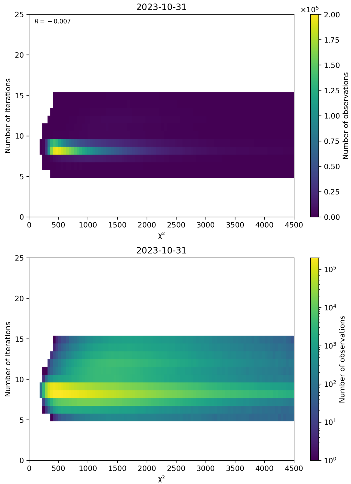
Figure 49: Scatter density plot of “ \chi^2 ” against “Number of iterations” for 2023-10-30 to 2023-11-01.
