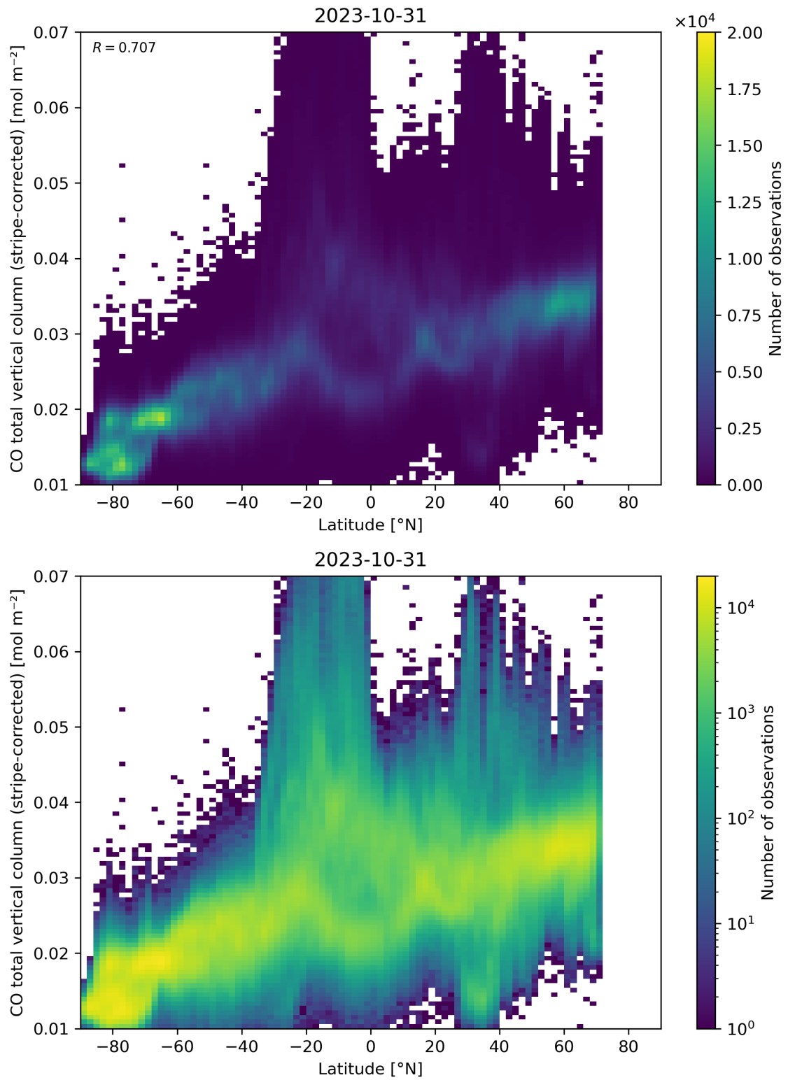
Figure 52: Scatter density plot of “Latitude” against “CO total vertical column (stripe-corrected)” for 2023-10-30 to 2023-11-01.
