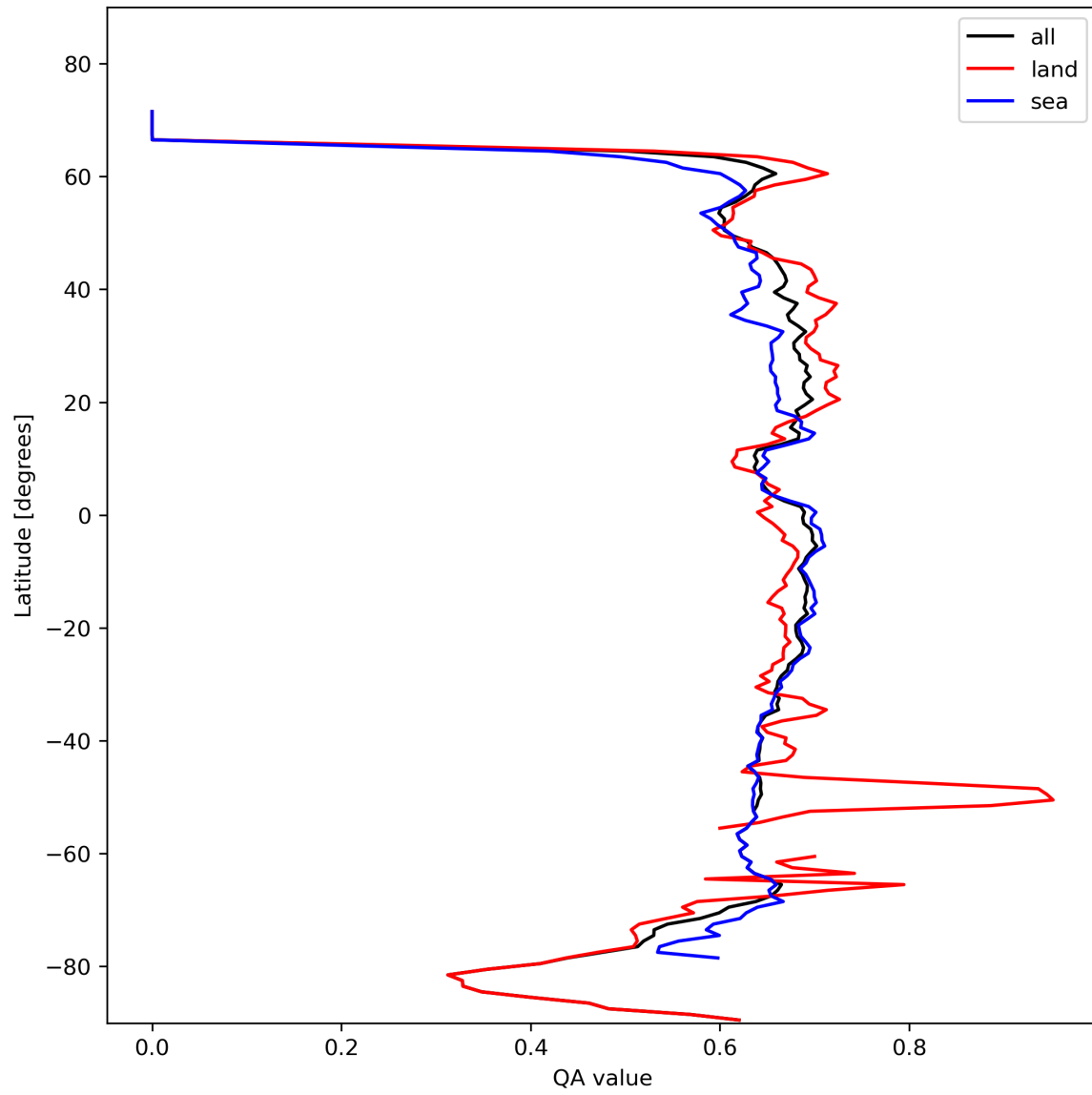
Figure 9: Zonal average of “QA value” for 2023-10-30 to 2023-11-01.
