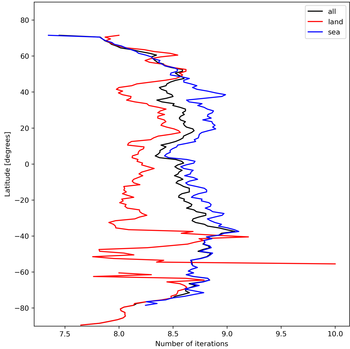
Figure 16: Zonal average of “Number of iterations” for 2023-10-30 to 2023-11-01.
