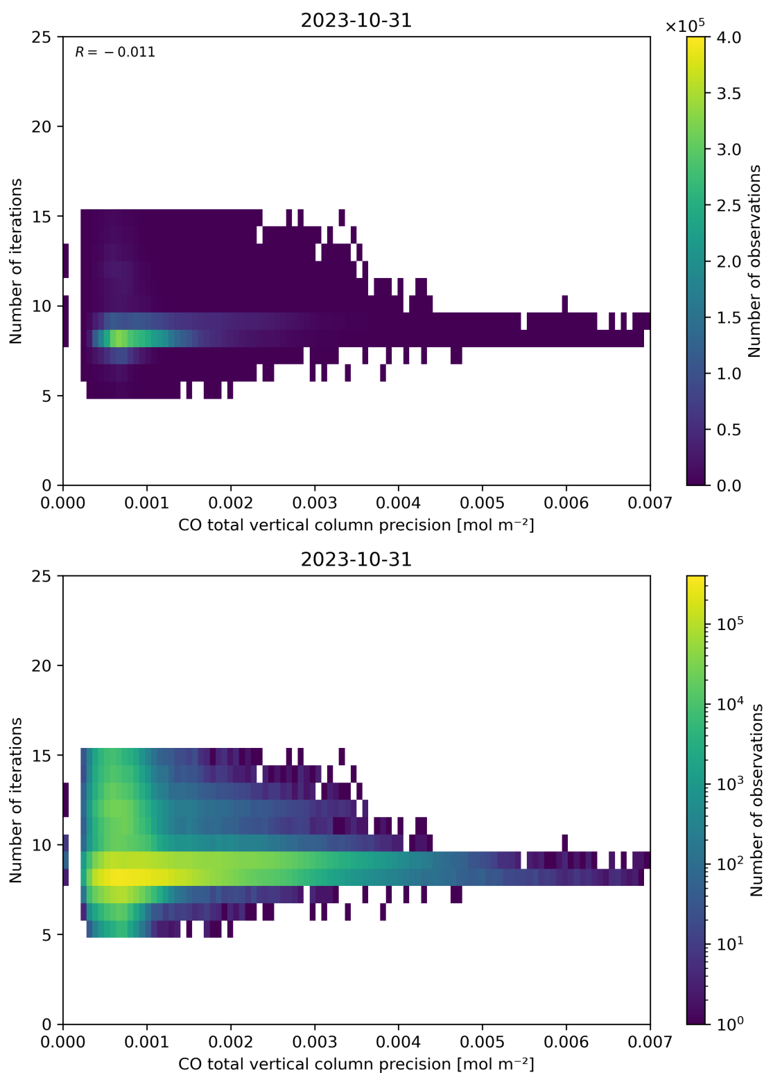
Figure 46: Scatter density plot of “CO total vertical column precision” against “Number of iterations” for 2023-10-30 to 2023-11-01.
