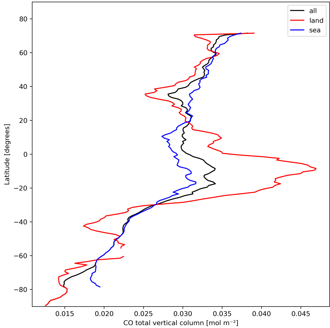
Figure 10: Zonal average of “CO total vertical column” for 2023-10-30 to 2023-11-01.
