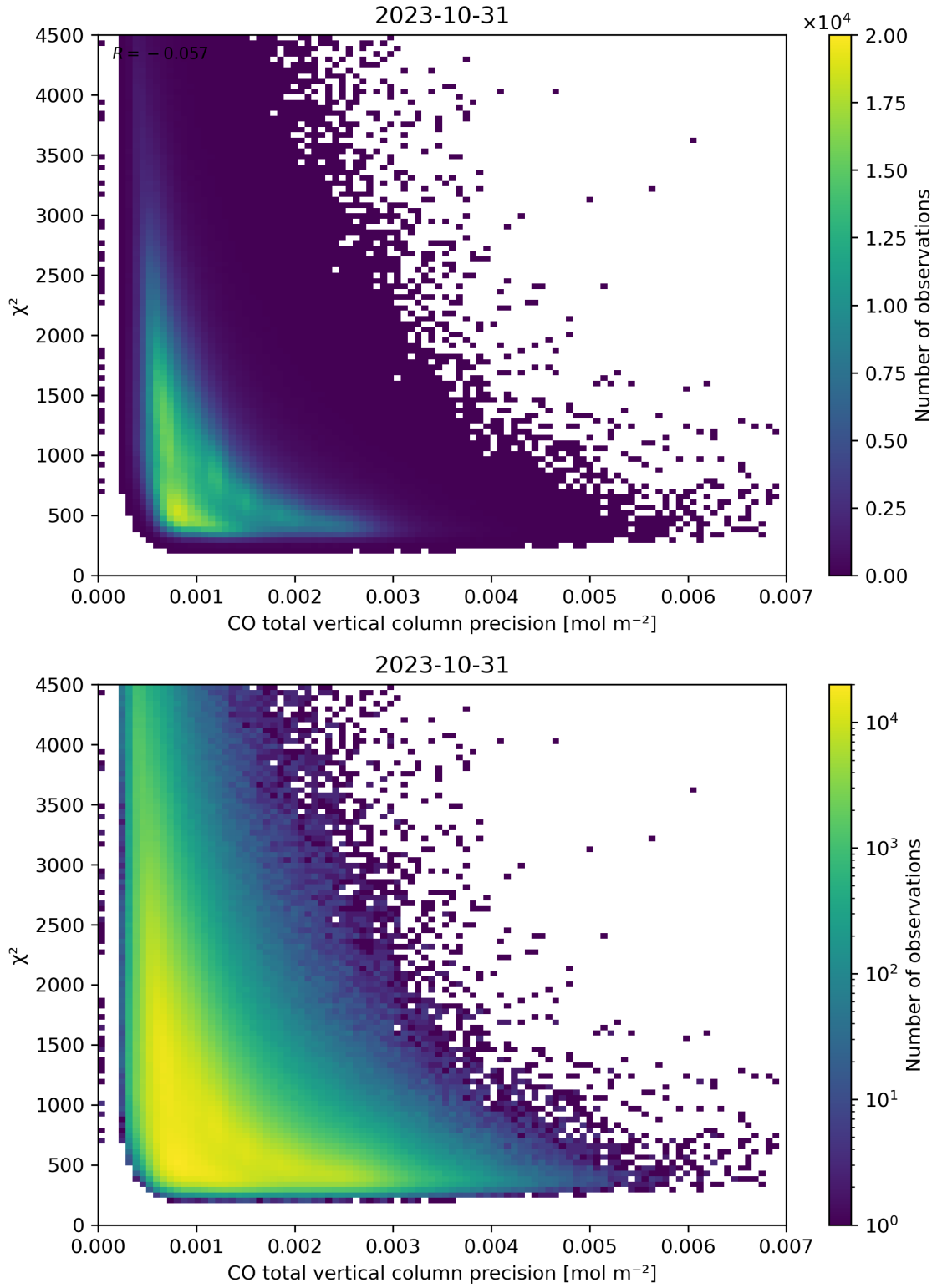
Figure 44: Scatter density plot of “CO total vertical column precision” against “ \chi^2 ” for 2023-10-30 to 2023-11-01.
