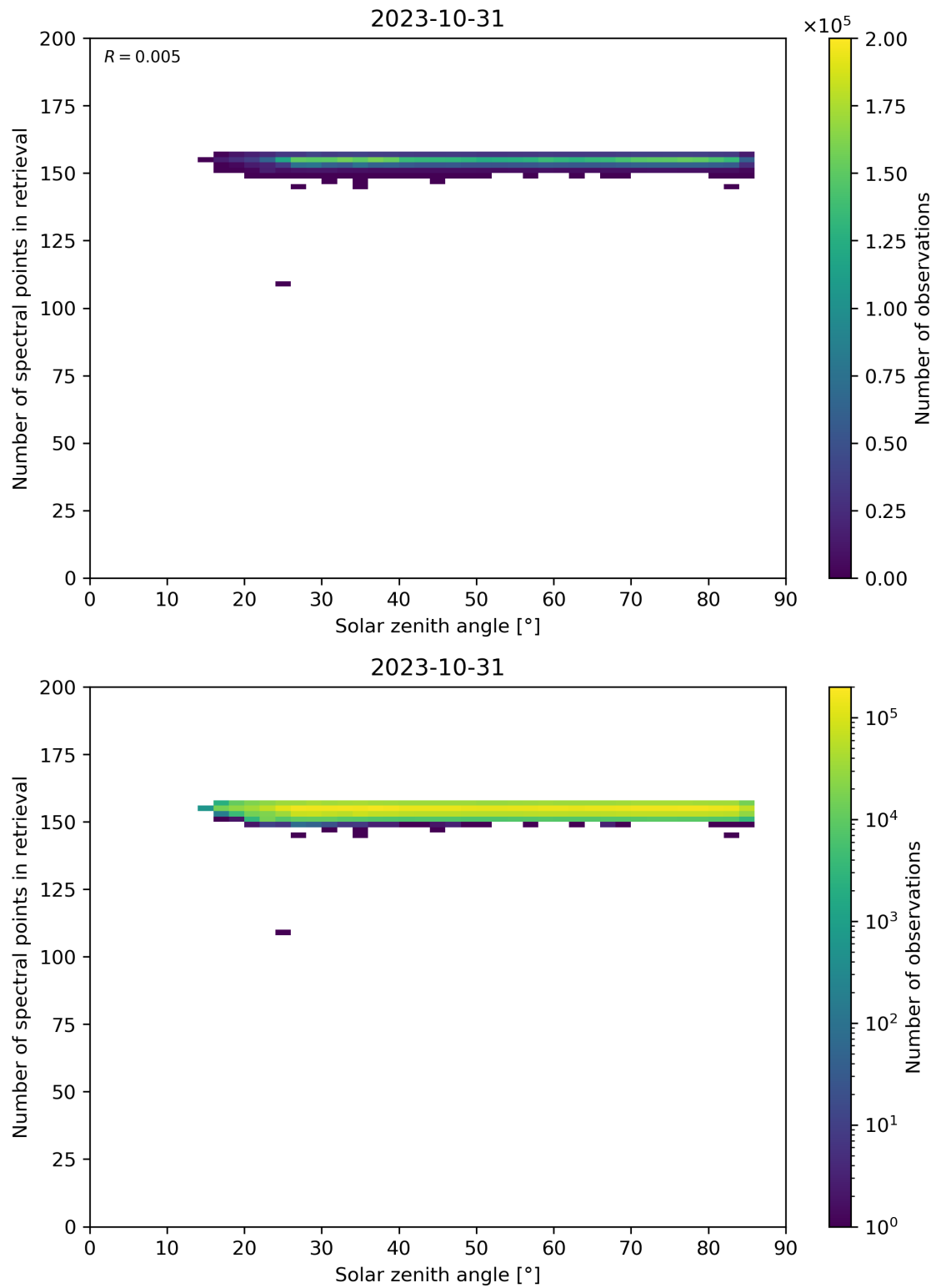
Figure 68: Scatter density plot of “Solar zenith angle” against “Number of spectral points in retrieval” for 2023-10-30 to 2023-11-01.
