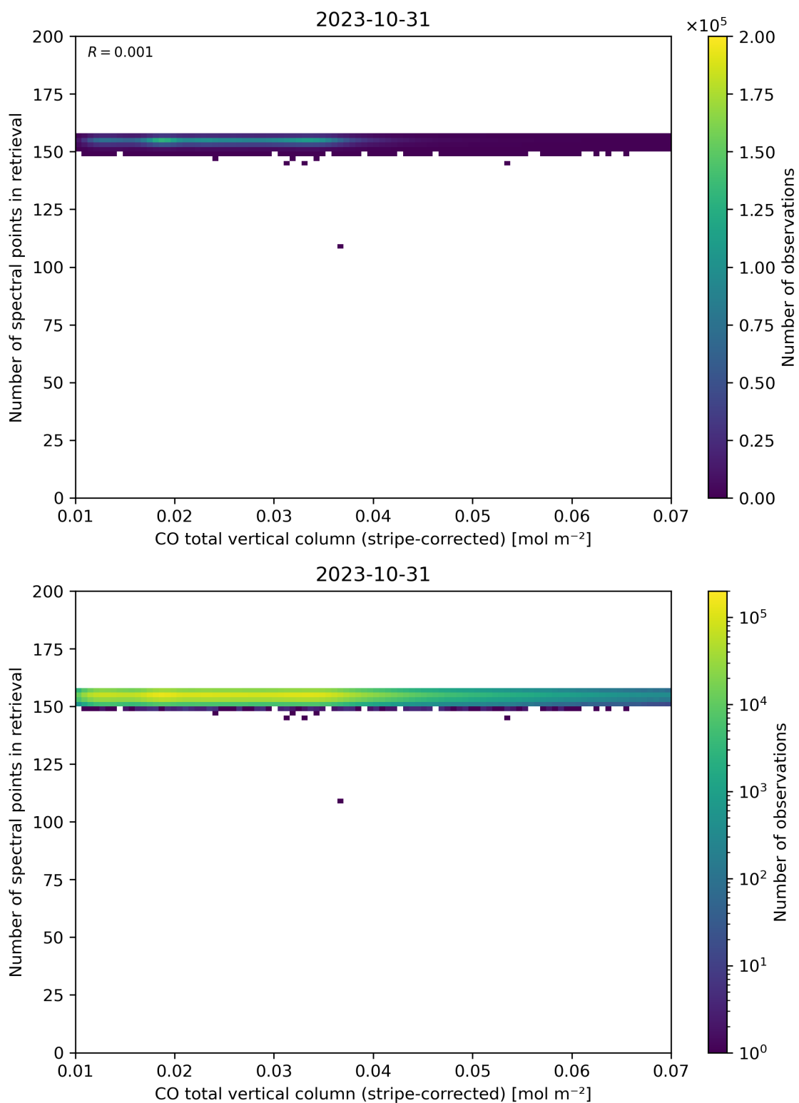
Figure 40: Scatter density plot of “CO total vertical column (stripe-corrected)” against “Number of spectral points in retrieval” for 2023-10-30 to 2023-11-01.
