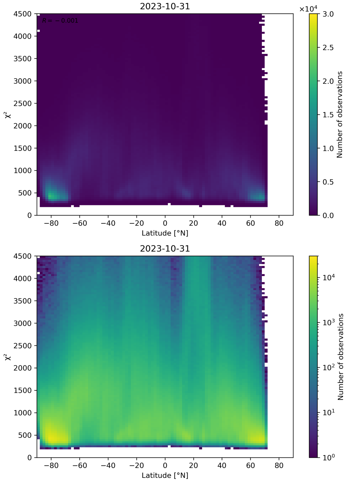
Figure 54: Scatter density plot of “Latitude” against “ \chi^2 ” for 2023-10-30 to 2023-11-01.
