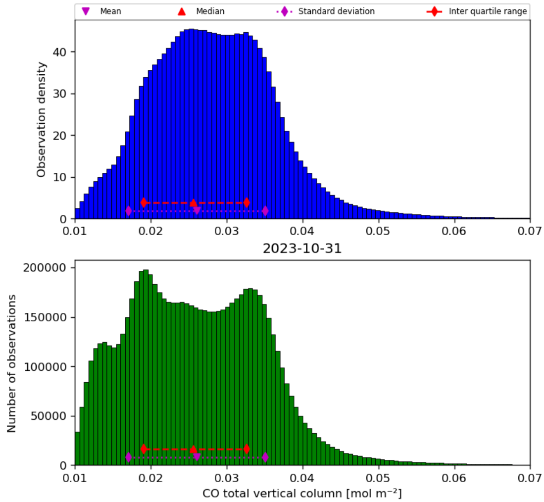
Figure 18: Histogram of “CO total vertical column” for 2023-10-30 to 2023-11-01
