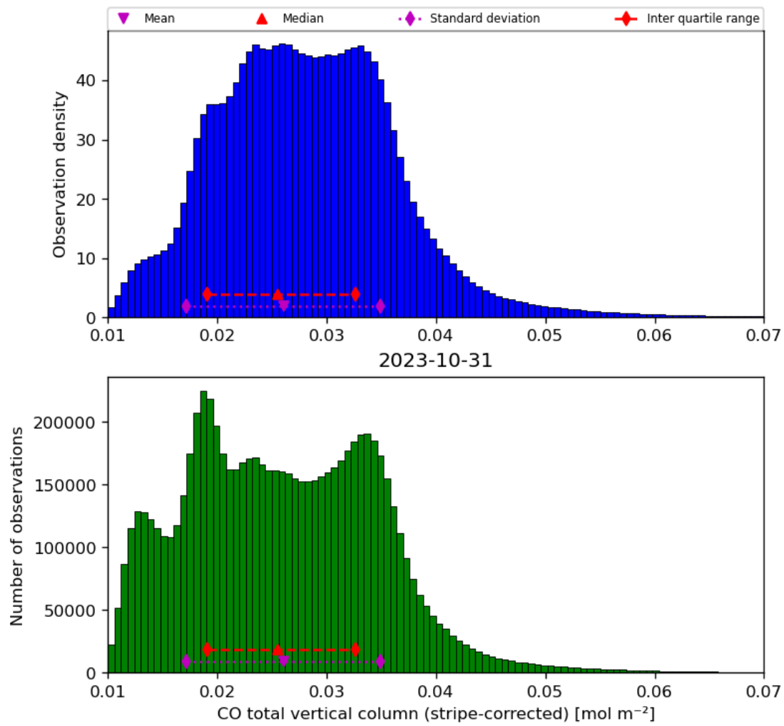
Figure 19: Histogram of “CO total vertical column (stripe-corrected)” for 2023-10-30 to 2023-11-01
