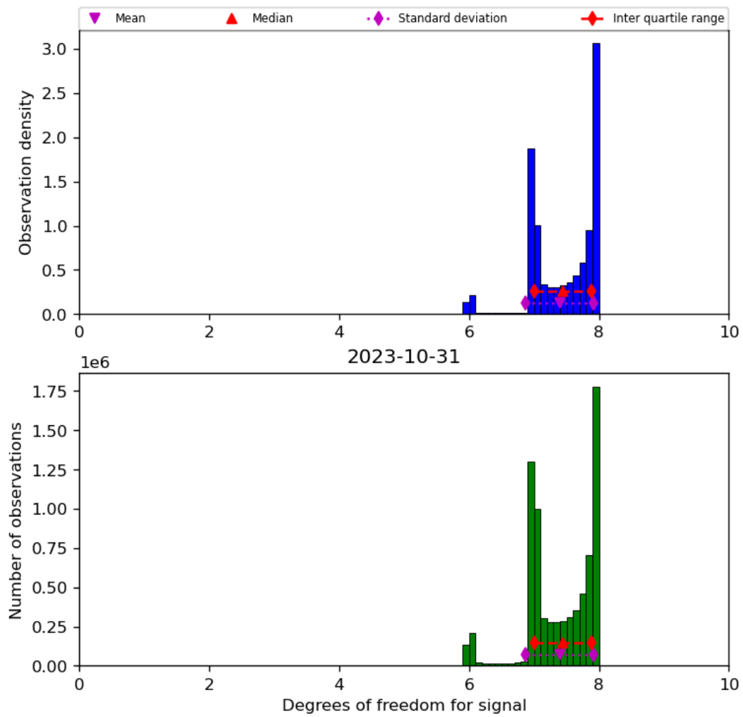
Figure 23: Histogram of “Degrees of freedom for signal” for 2023-10-30 to 2023-11-01
