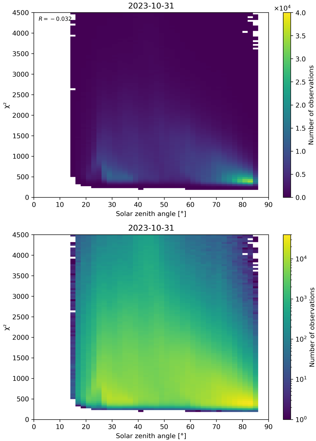
Figure 64: Scatter density plot of “Solar zenith angle” against “ \chi^2 ” for 2023-10-30 to 2023-11-01.
