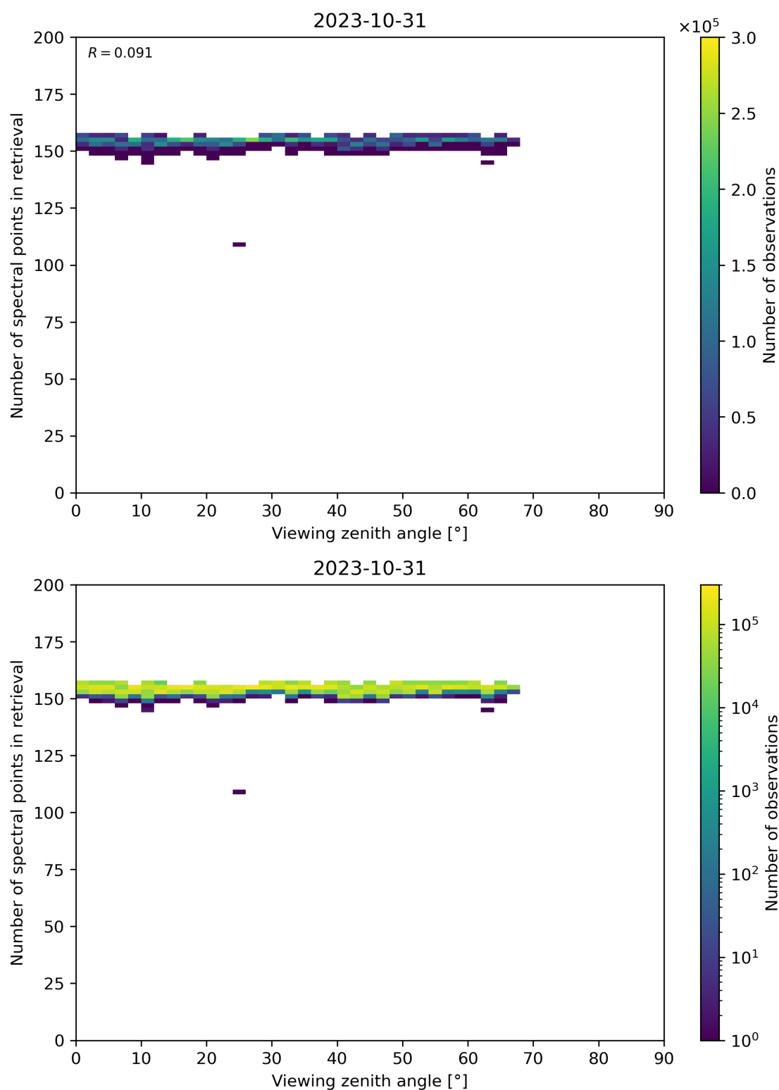
Figure 76: Scatter density plot of “Viewing zenith angle” against “Number of spectral points in retrieval” for 2023-10-30 to 2023-11-01.
