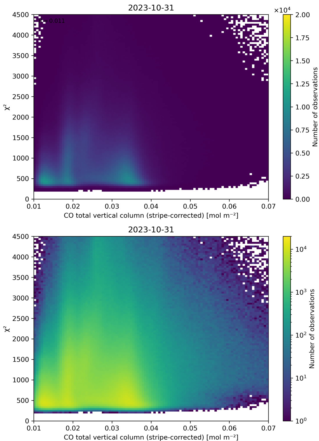
Figure 37: Scatter density plot of “CO total vertical column (stripe-corrected)” against “ \chi^2 ” for 2023-10-30 to 2023-11-01.
