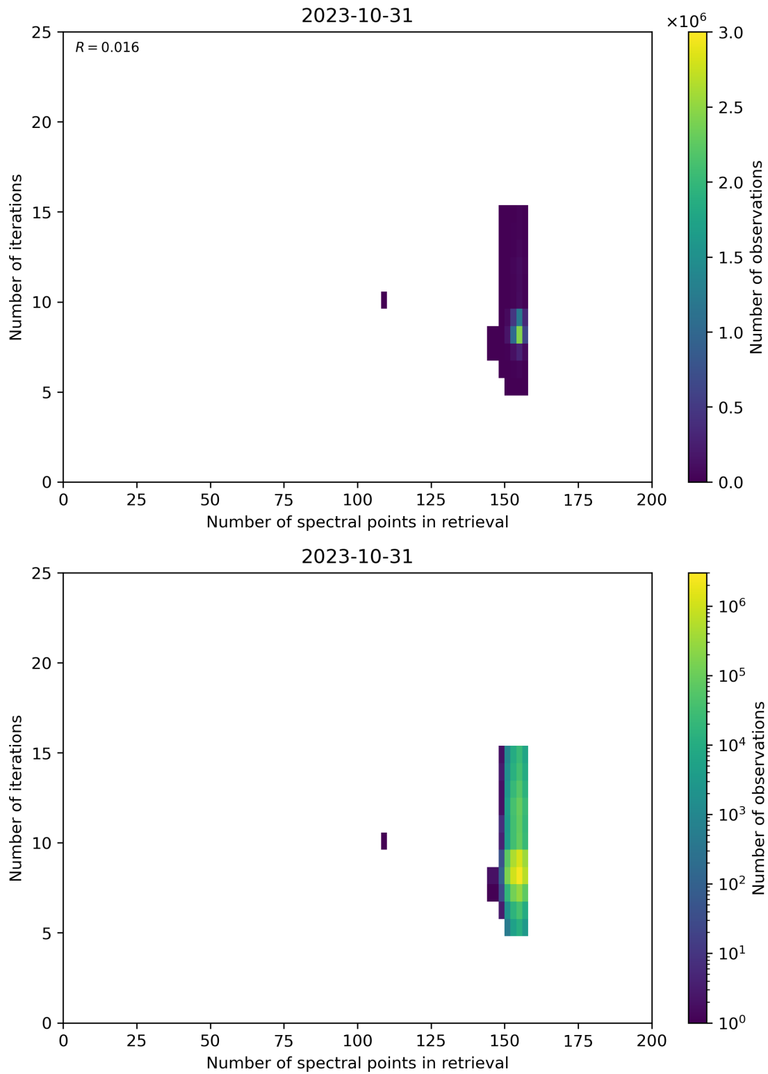
Figure 60: Scatter density plot of “Number of spectral points in retrieval” against “Number of iterations” for 2023-10-30 to 2023-11-01.
