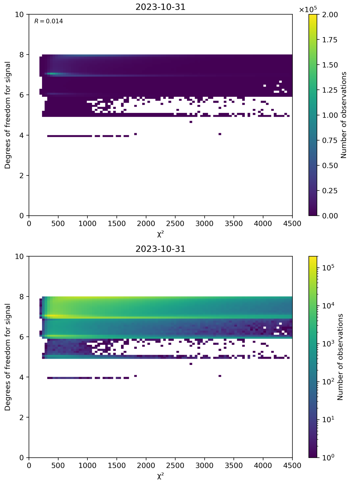
Figure 48: Scatter density plot of " \chi^2 " against "Degrees of freedom for signal" for 2023-10-30 to 2023-11-01.
