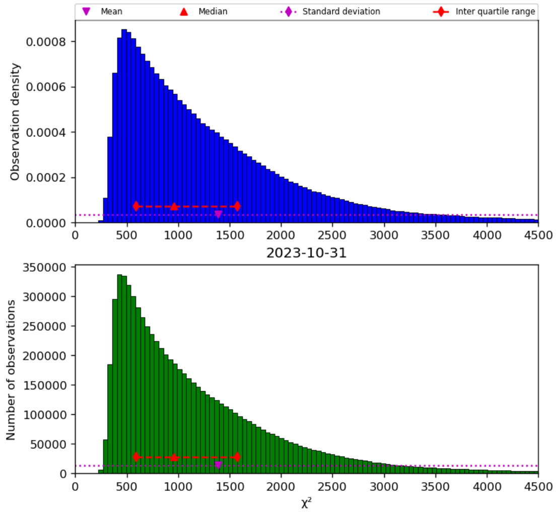
Figure 22: Histogram of " \chi^2 " for 2023-10-30 to 2023-11-01
