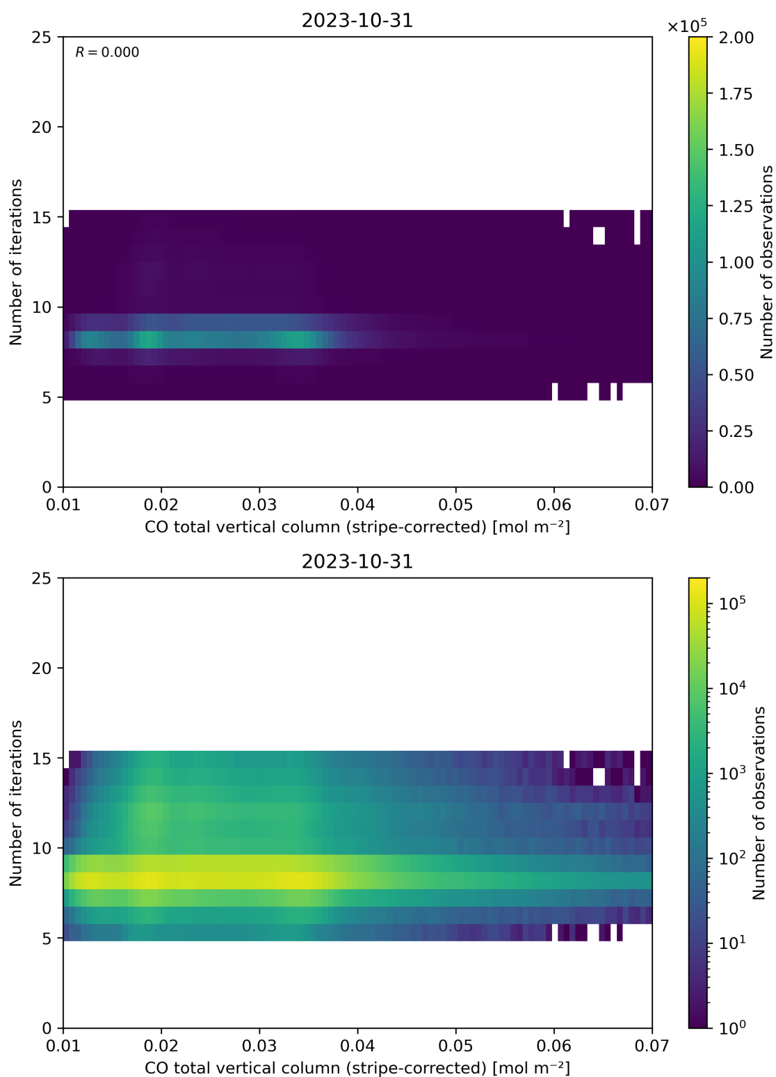
Figure 39: Scatter density plot of “CO total vertical column (stripe-corrected)” against “Number of iterations” for 2023-10-30 to 2023-11-01.
