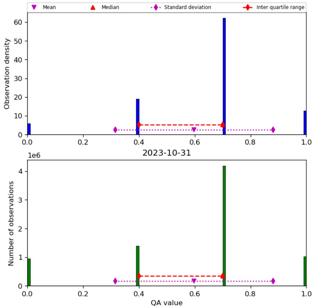
Figure 17: Histogram of “QA value” for 2023-10-30 to 2023-11-01
