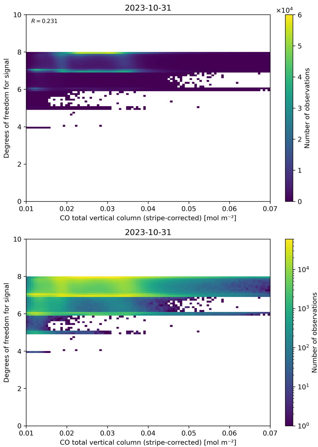
Figure 38: Scatter density plot of “CO total vertical column (stripe-corrected)” against “Degrees of freedom for signal” for 2023-10-30 to 2023-11-01.
