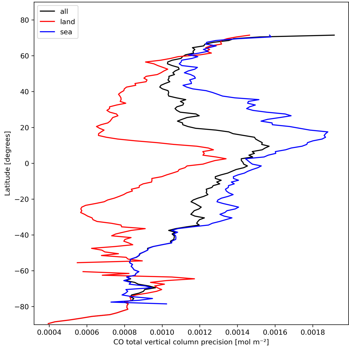
Figure 12: Zonal average of “CO total vertical column precision” for 2023-10-30 to 2023-11-01.
