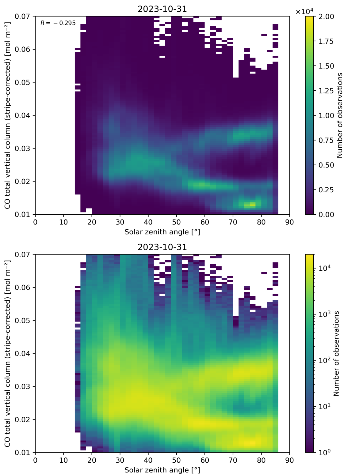
Figure 62: Scatter density plot of “Solar zenith angle” against “CO total vertical column (stripe-corrected)” for 2023-10-30 to 2023-11-01.
