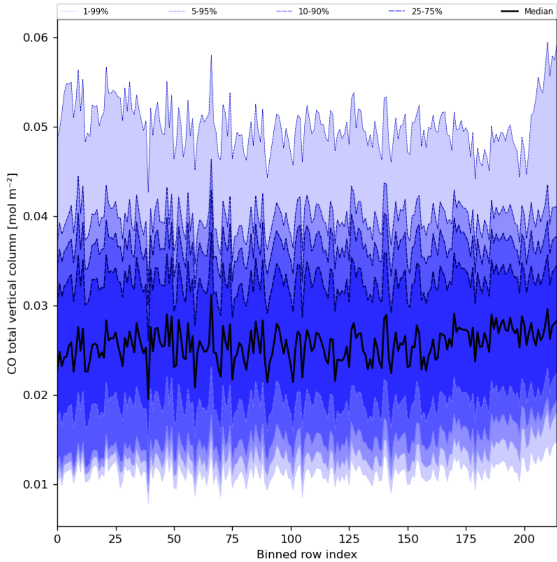
Figure 26: Along track statistics of “CO total vertical column” for 2023-10-30 to 2023-11-01
