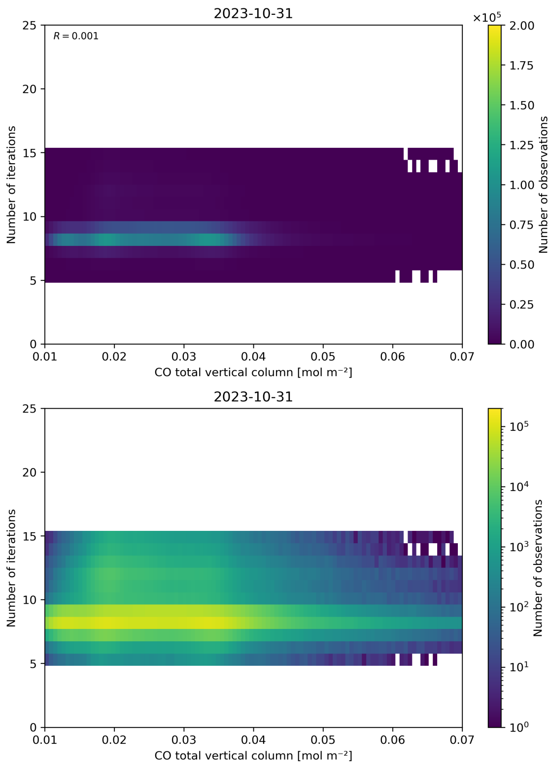
Figure 42: Scatter density plot of “CO total vertical column” against “Number of iterations” for 2023-10-30 to 2023-11-01.
