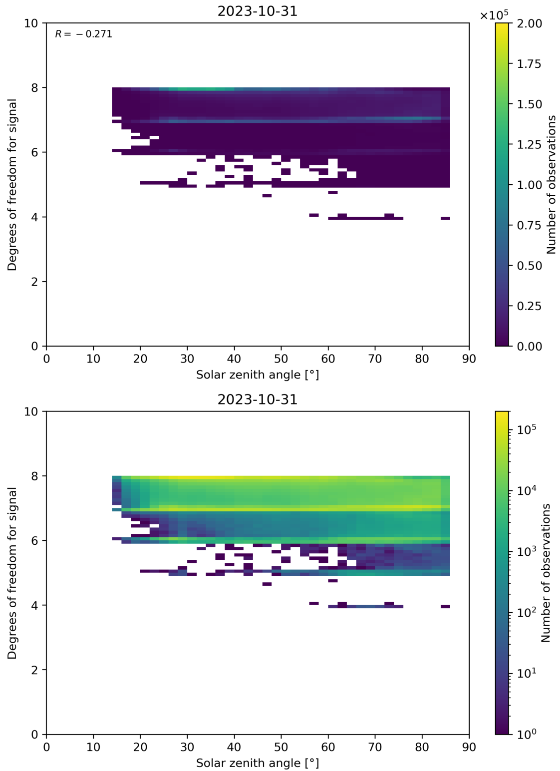
Figure 65: Scatter density plot of “Solar zenith angle” against “Degrees of freedom for signal” for 2023-10-30 to 2023-11-01.
