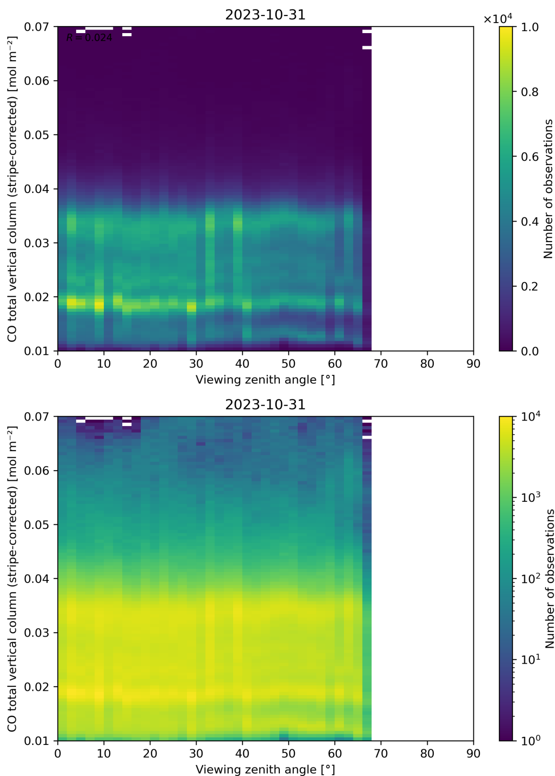
Figure 70: Scatter density plot of “Viewing zenith angle” against “CO total vertical column (stripe-corrected)” for 2023-10-30 to 2023-11-01.
