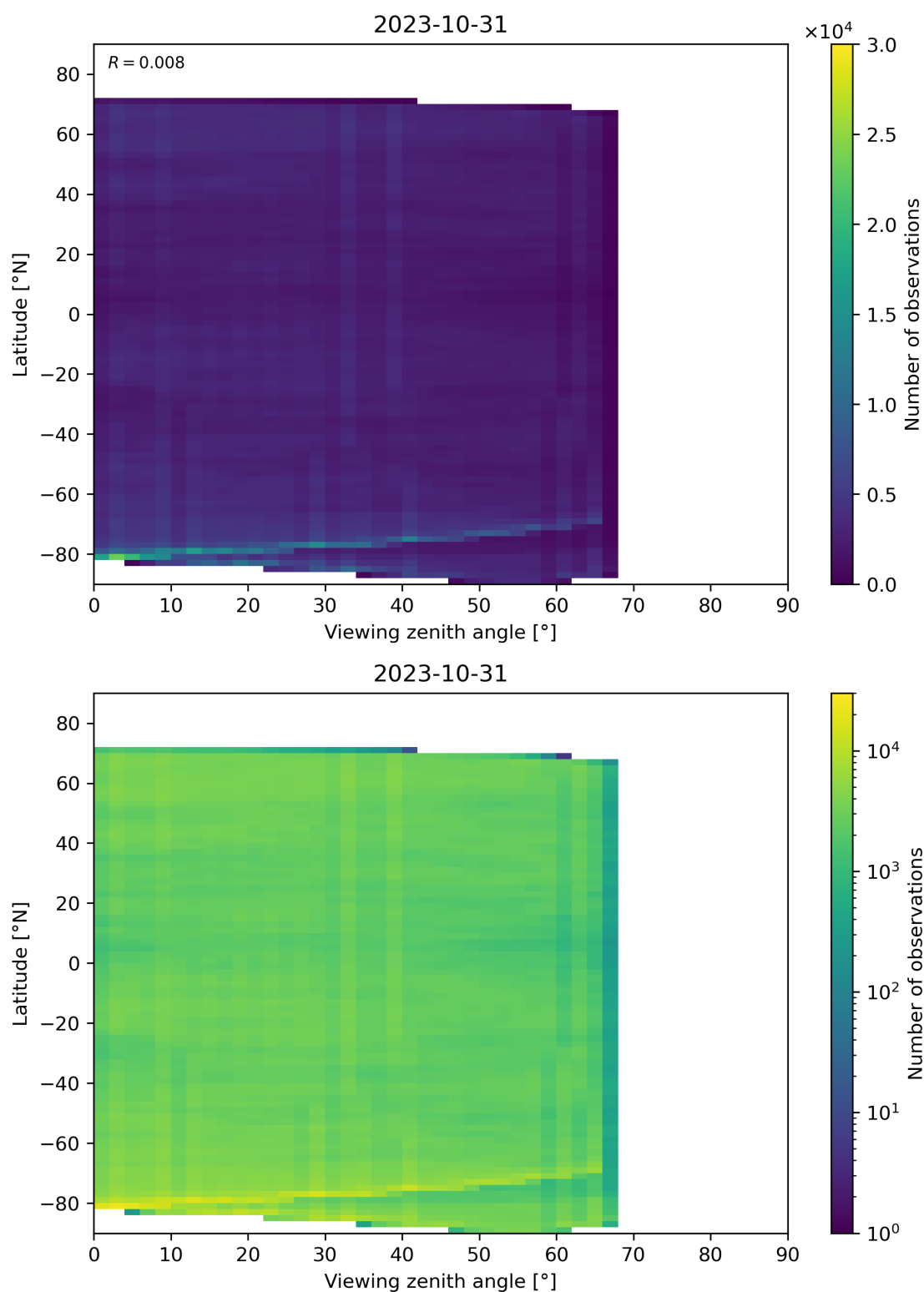
Figure 74: Scatter density plot of “Viewing zenith angle” against “Latitude” for 2023-10-30 to 2023-11-01.
