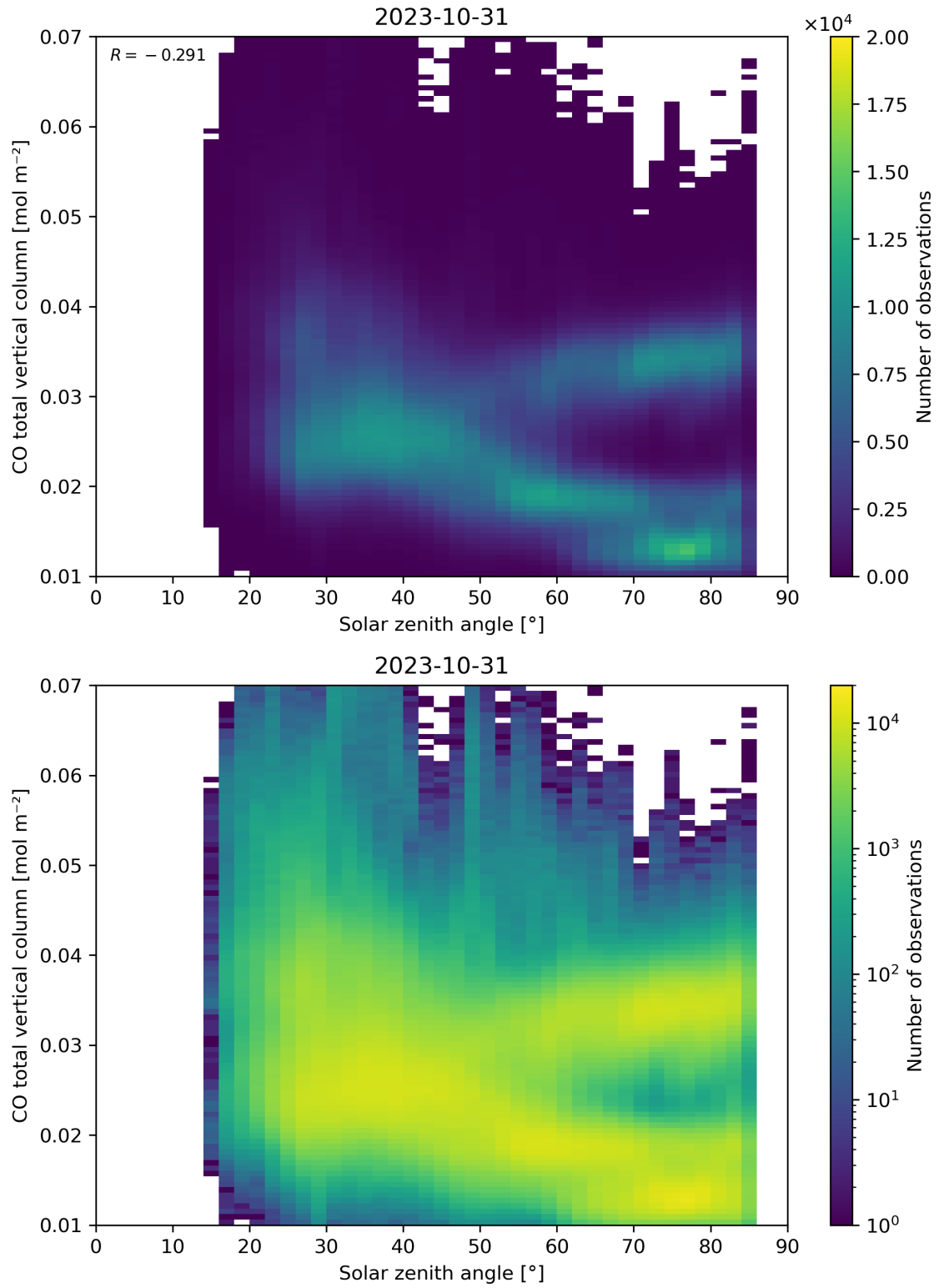
Figure 61: Scatter density plot of “Solar zenith angle” against “CO total vertical column” for 2023-10-30 to 2023-11-01.
