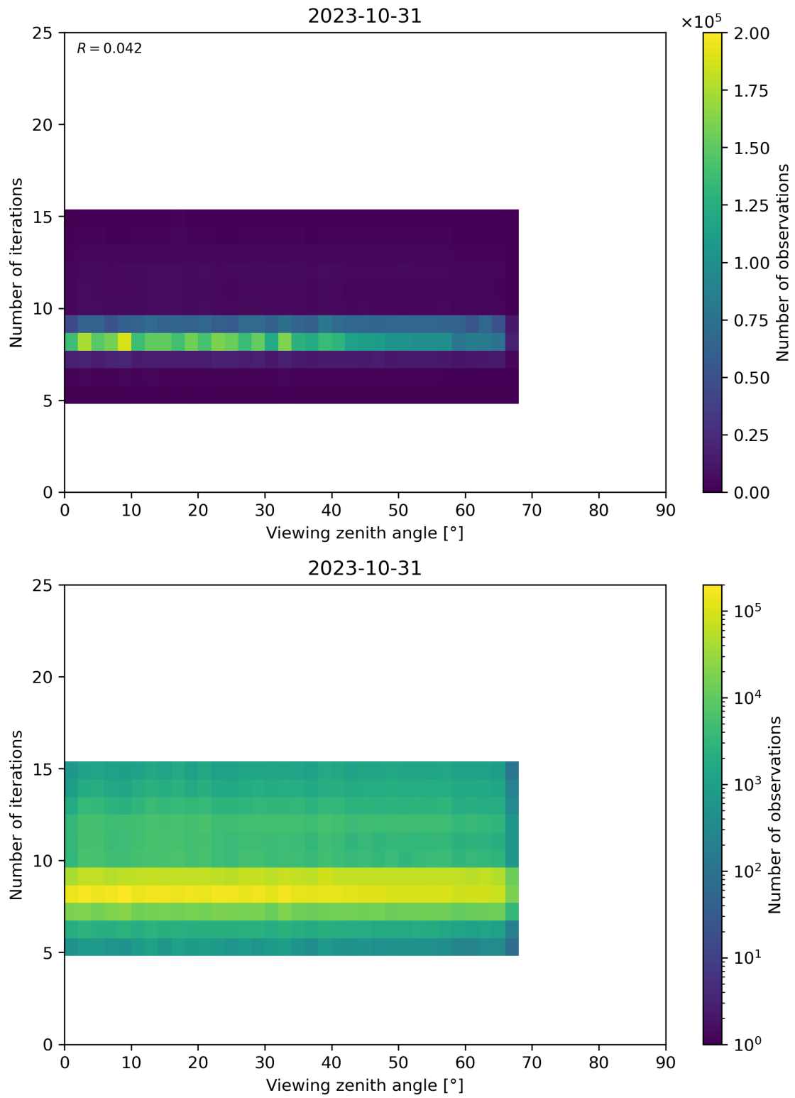
Figure 75: Scatter density plot of “Viewing zenith angle” against “Number of iterations” for 2023-10-30 to 2023-11-01.
