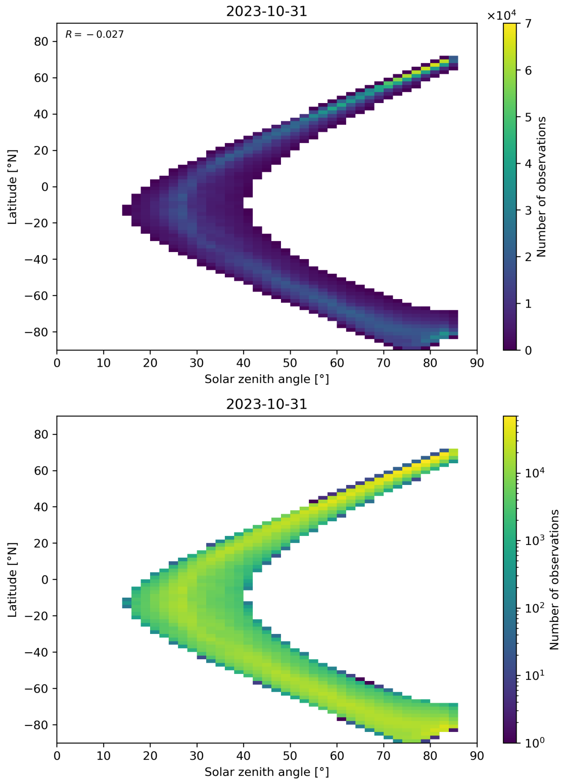
Figure 66: Scatter density plot of “Solar zenith angle” against “Latitude” for 2023-10-30 to 2023-11-01.
