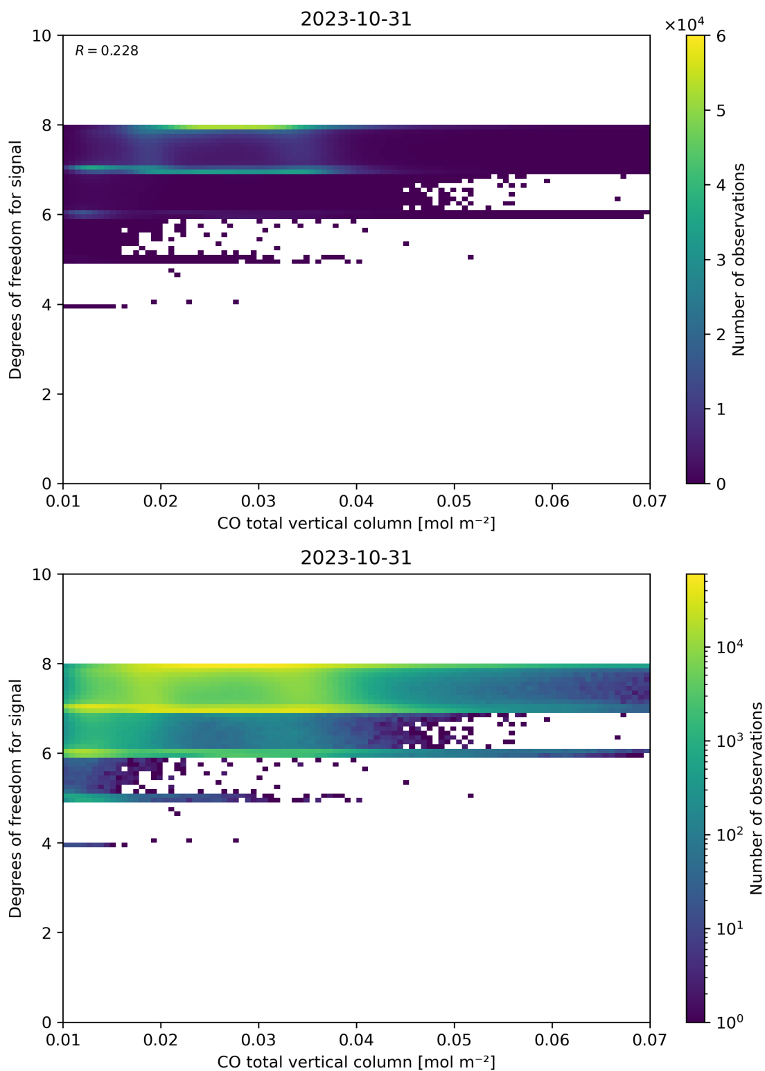
Figure 41: Scatter density plot of “CO total vertical column” against “Degrees of freedom for signal” for 2023-10-30 to 2023-11-01.
