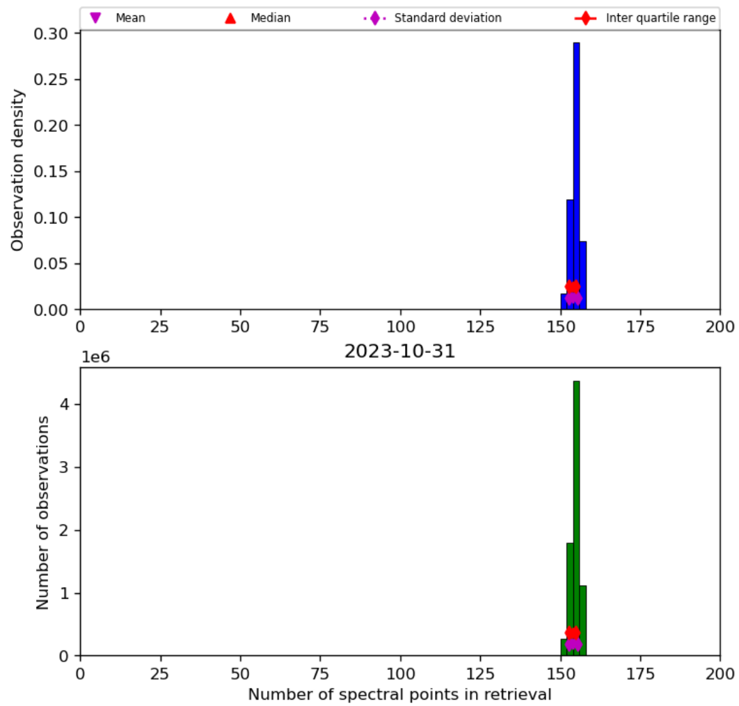
Figure 21: Histogram of “Number of spectral points in retrieval” for 2023-10-30 to 2023-11-01
