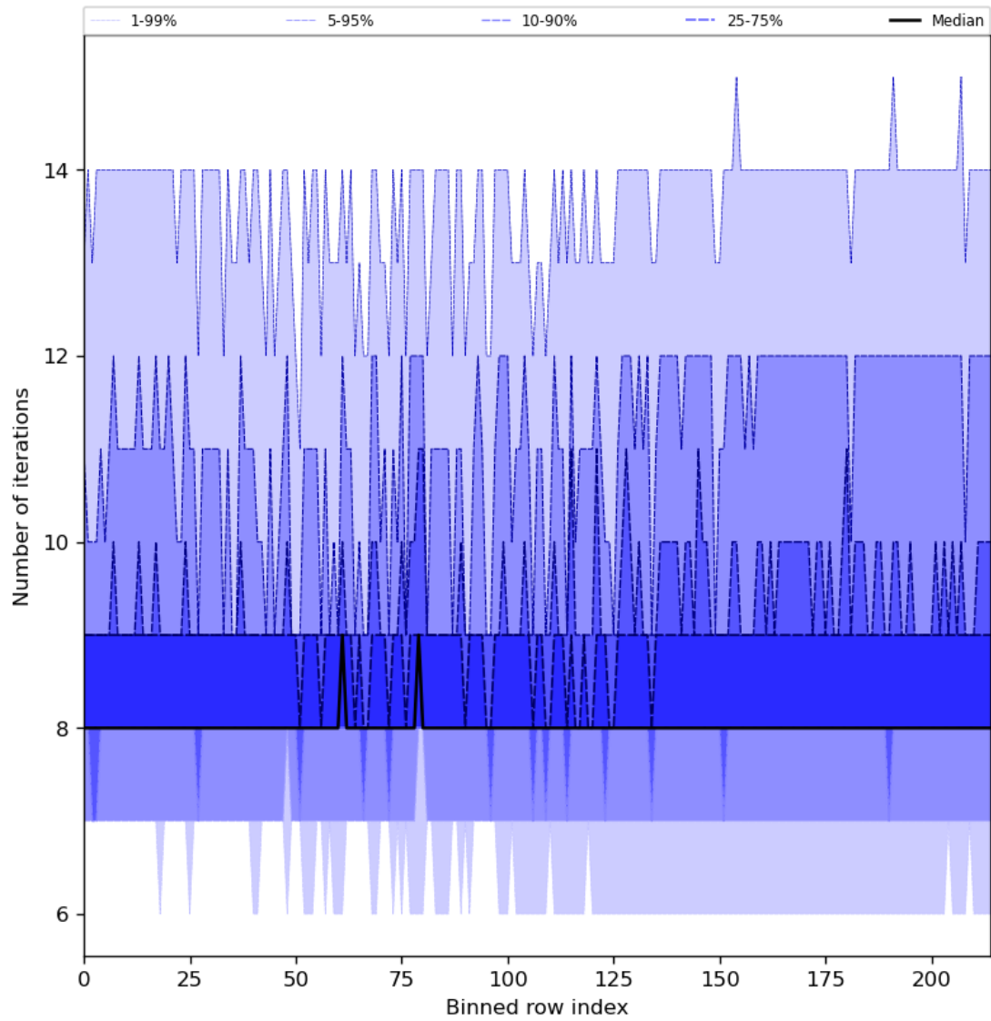
Figure 32: Along track statistics of “Number of iterations” for 2023-10-30 to 2023-11-01
