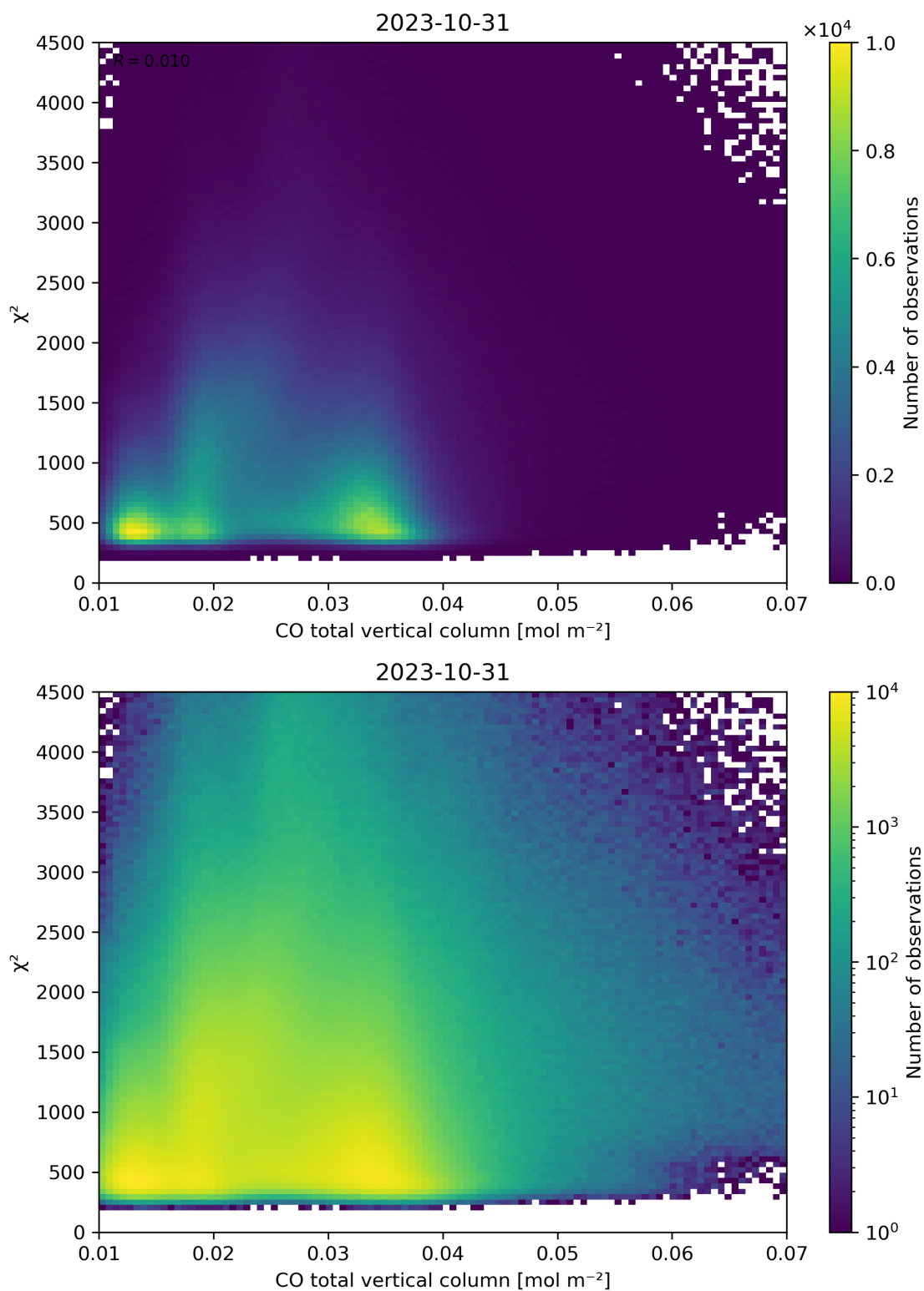
Figure 35: Scatter density plot of “CO total vertical column” against “ \chi^2 ” for 2023-10-30 to 2023-11-01.
