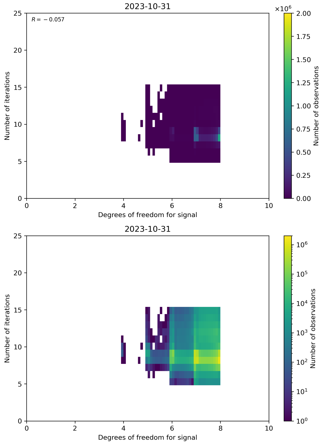
Figure 50: Scatter density plot of “Degrees of freedom for signal” against “Number of iterations” for 2023-10-30 to 2023-11-01.
