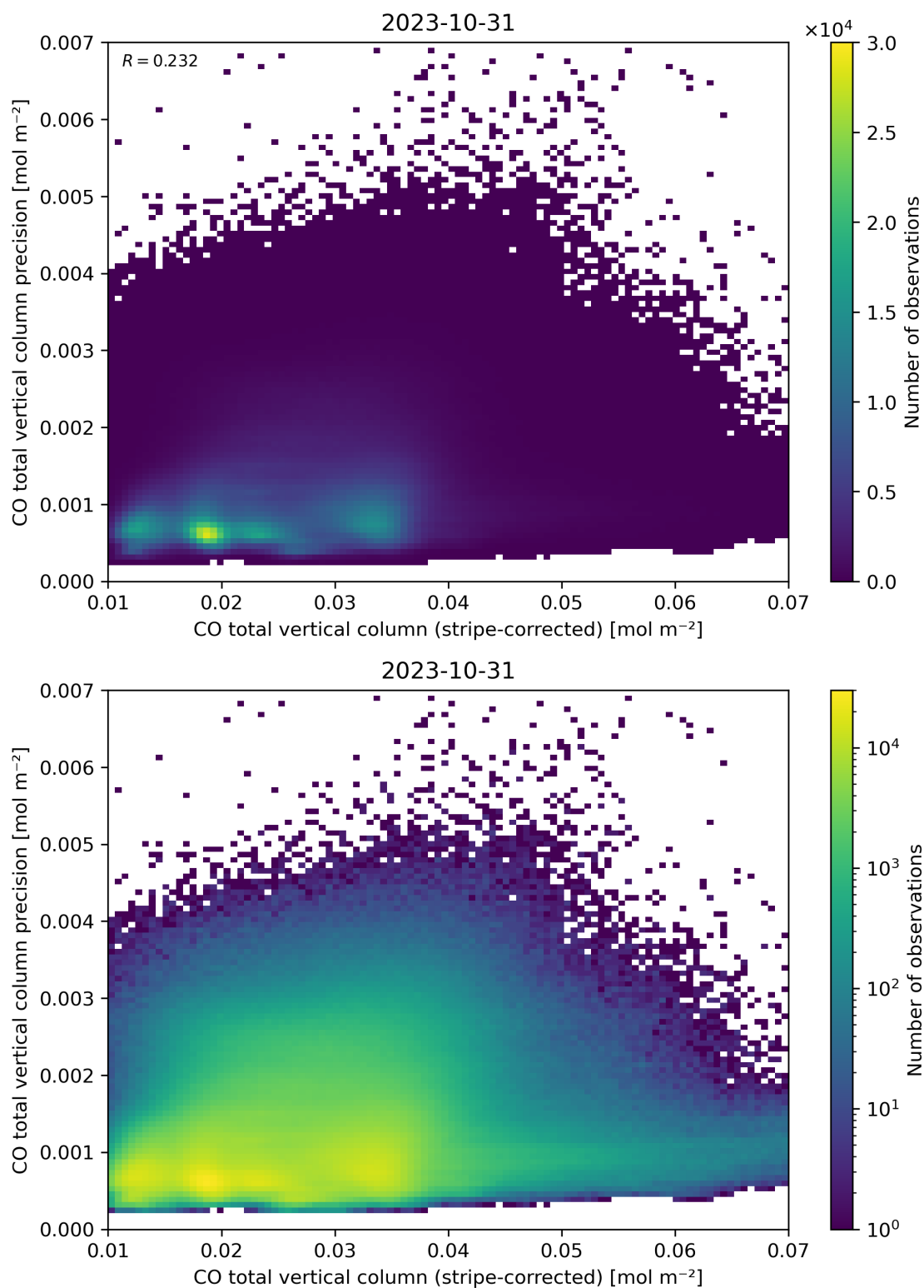
Figure 36: Scatter density plot of “CO total vertical column (stripe-corrected)” against “CO total vertical column precision” for 2023-10-30 to 2023-11-01.
