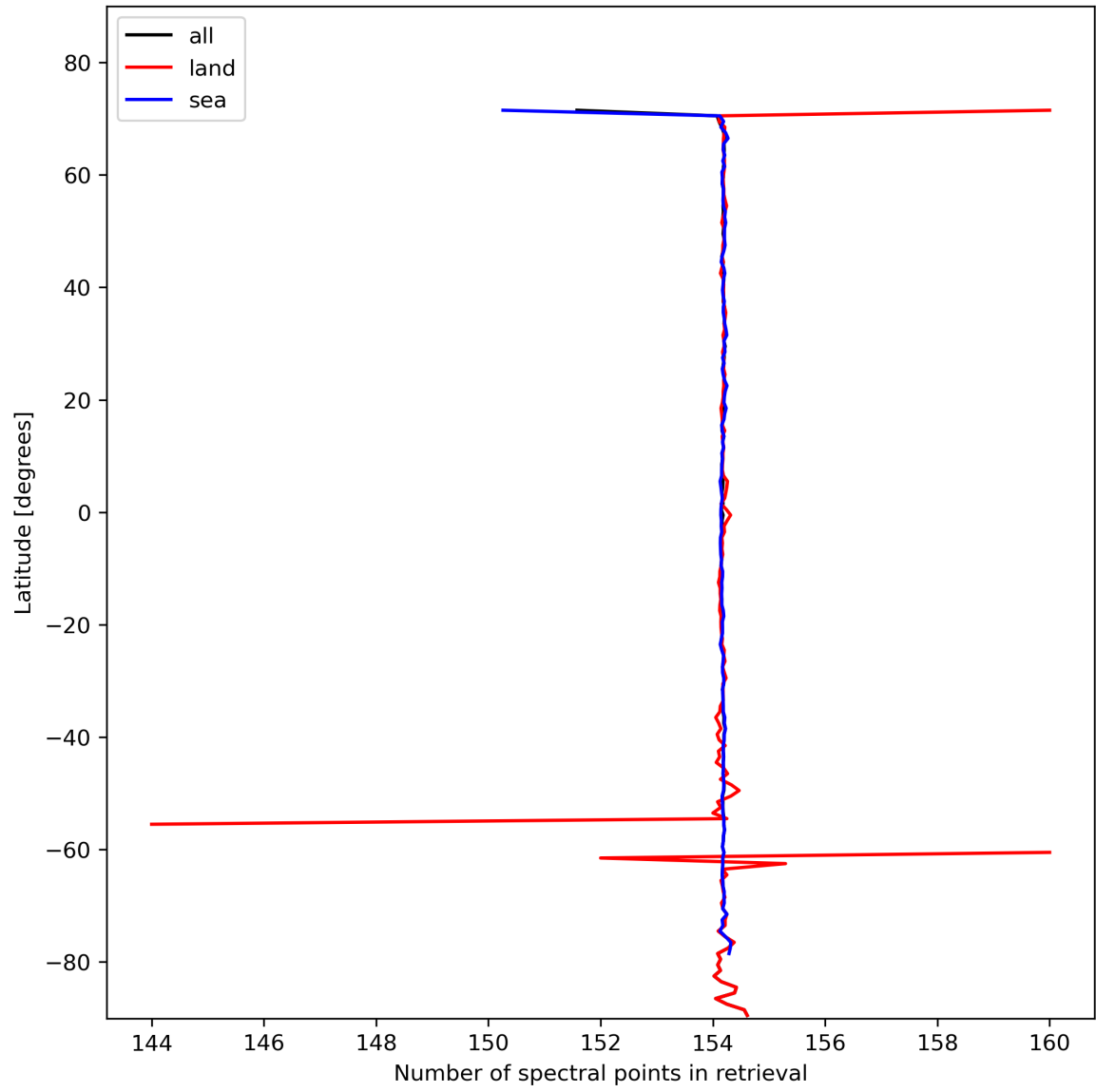
Figure 13: Zonal average of “Number of spectral points in retrieval” for 2023-10-30 to 2023-11-01.
