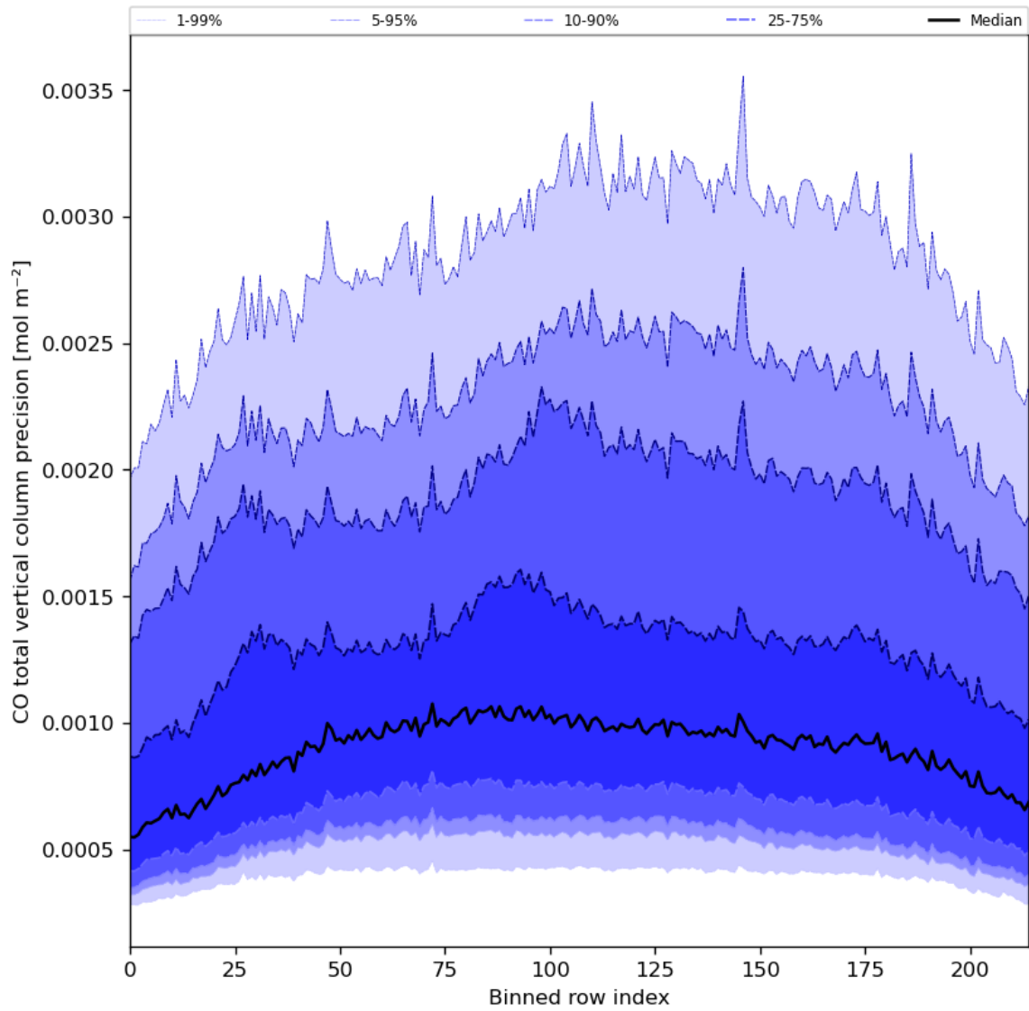
Figure 28: Along track statistics of “CO total vertical column precision” for 2023-10-30 to 2023-11-01
