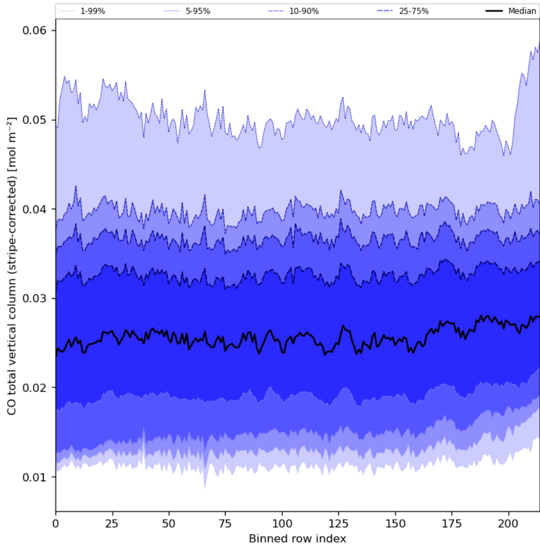
Figure 27: Along track statistics of “CO total vertical column (stripe-corrected)” for 2023-10-30 to 2023-11-01
