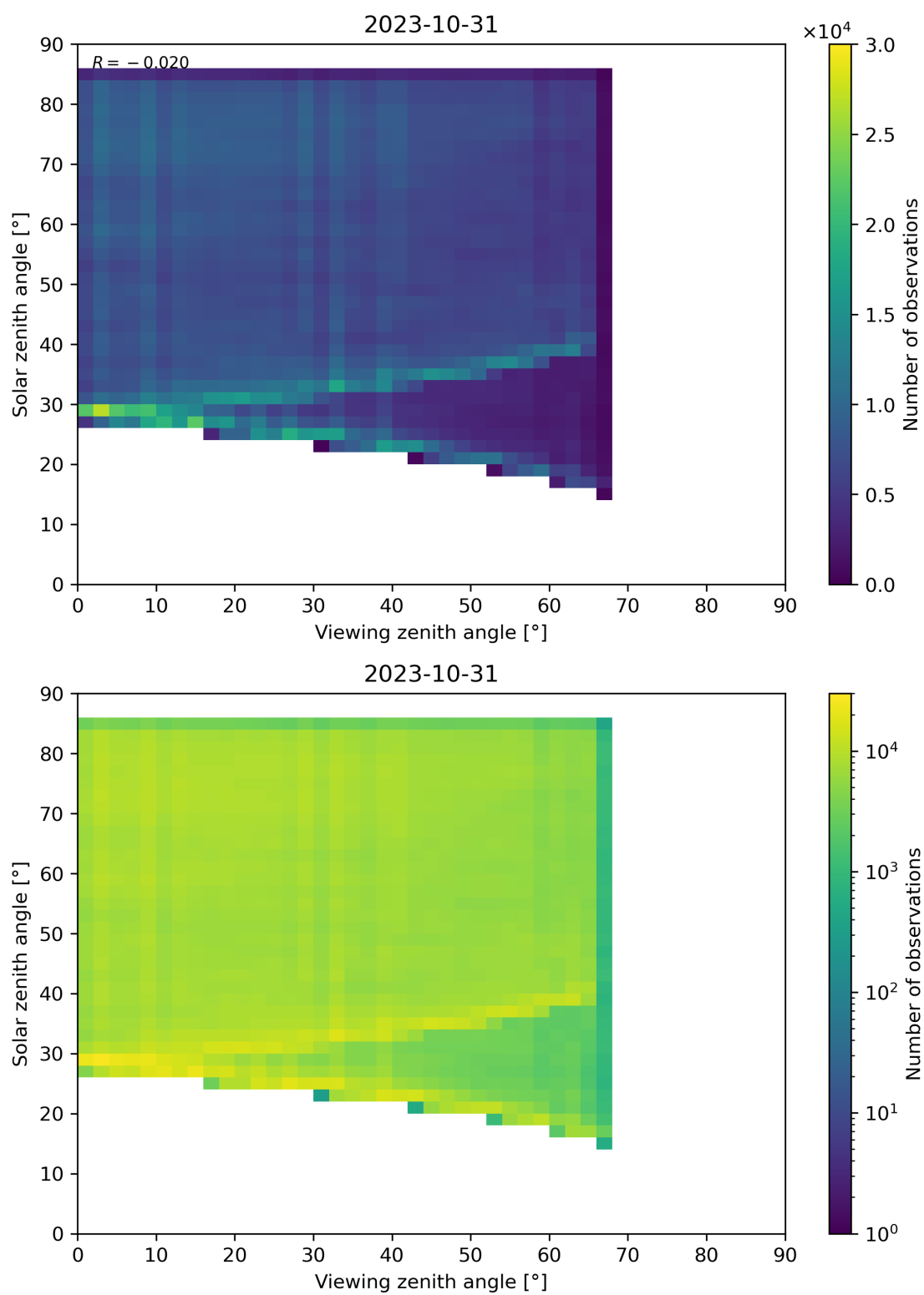
Figure 77: Scatter density plot of “Viewing zenith angle” against “Solar zenith angle” for 2023-10-30 to 2023-11-01.
