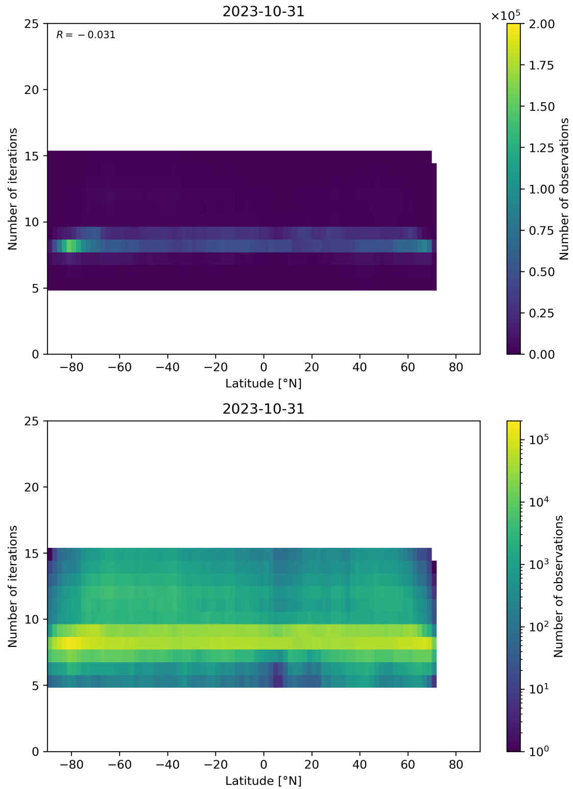
Figure 56: Scatter density plot of “Latitude” against “Number of iterations” for 2023-10-30 to 2023-11-01.
