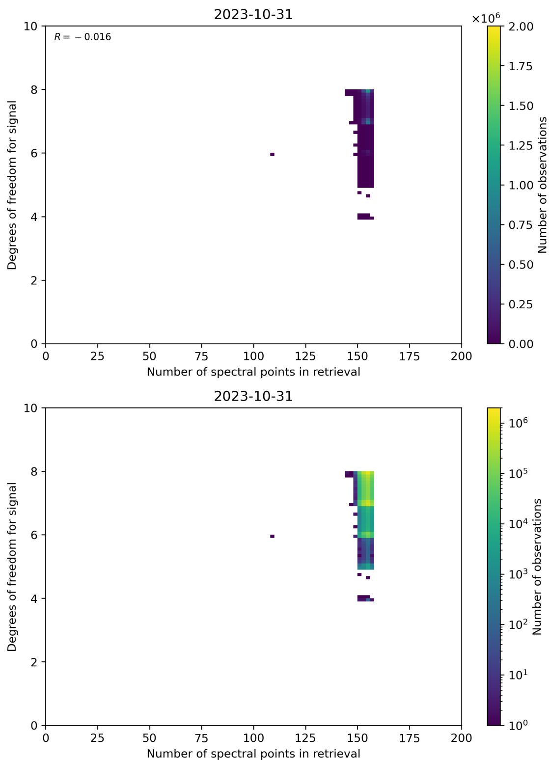
Figure 59: Scatter density plot of “Number of spectral points in retrieval” against “Degrees of freedom for signal” for 2023-10-30 to 2023-11-01.
