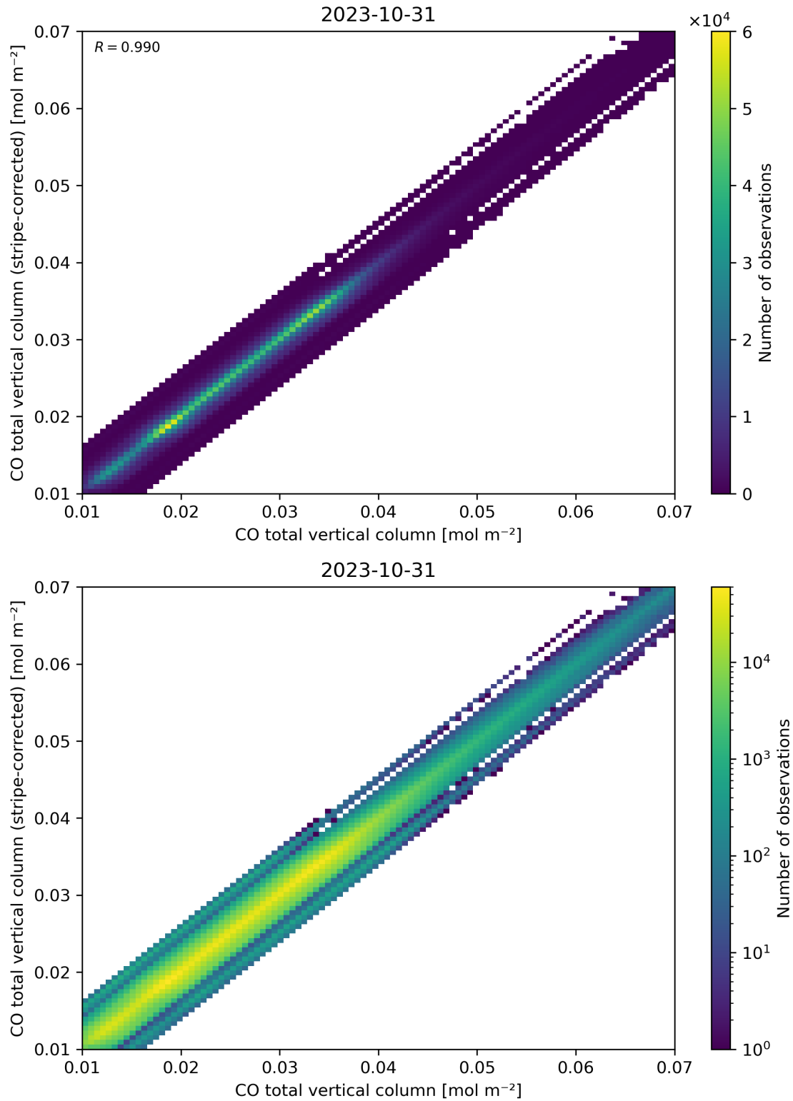
Figure 33: Scatter density plot of “CO total vertical column” against “CO total vertical column (stripe-corrected)” for 2023-10-30 to 2023-11-01.
