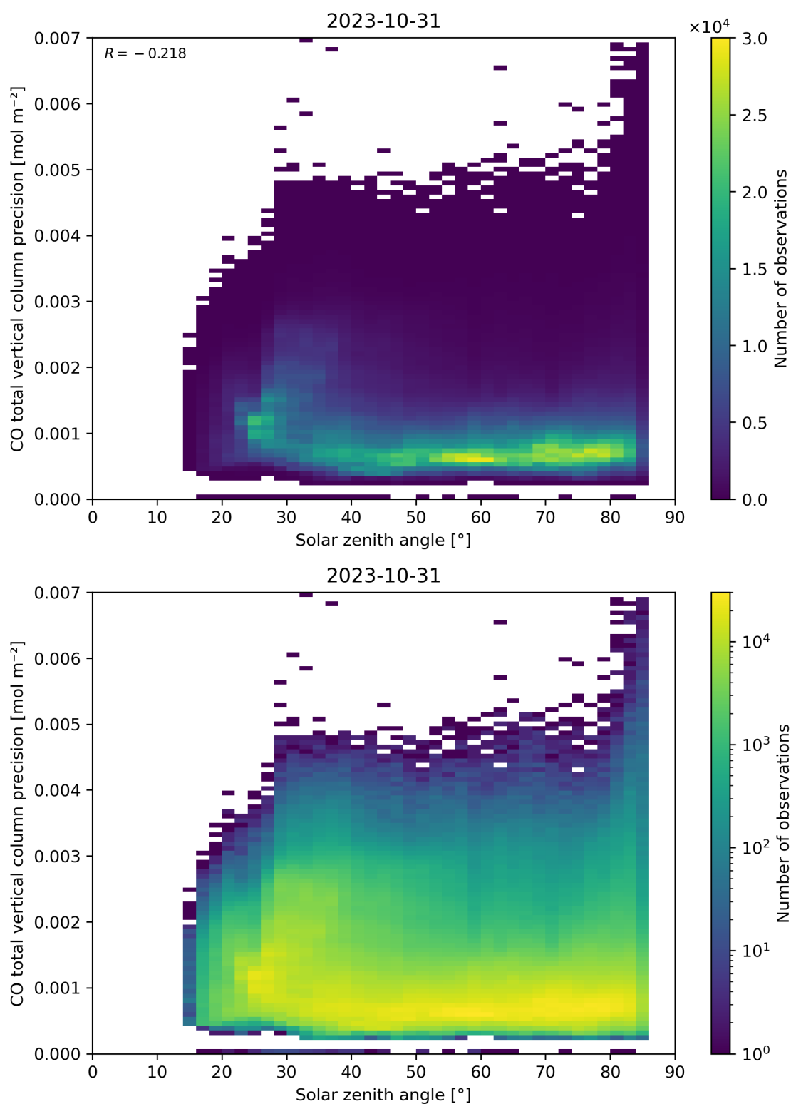
Figure 63: Scatter density plot of “Solar zenith angle” against “CO total vertical column precision” for 2023-10-30 to 2023-11-01.
