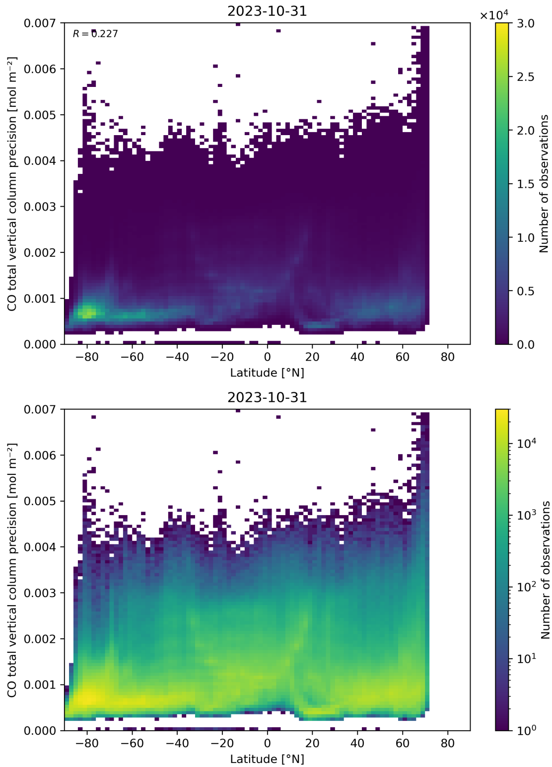
Figure 53: Scatter density plot of “Latitude” against “CO total vertical column precision” for 2023-10-30 to 2023-11-01.
