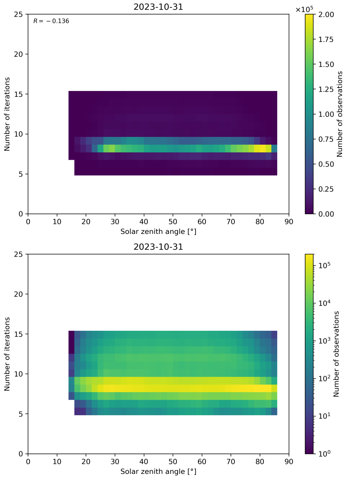
Figure 67: Scatter density plot of “Solar zenith angle” against “Number of iterations” for 2023-10-30 to 2023-11-01.
