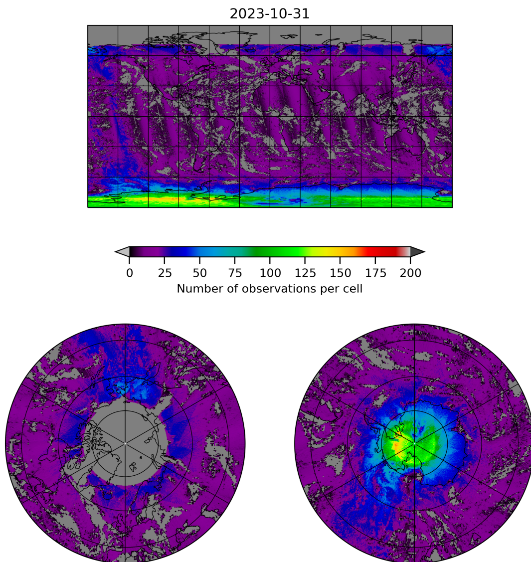
Figure 8: Map of the number of observations for 2023-10-30 to 2023-11-01
