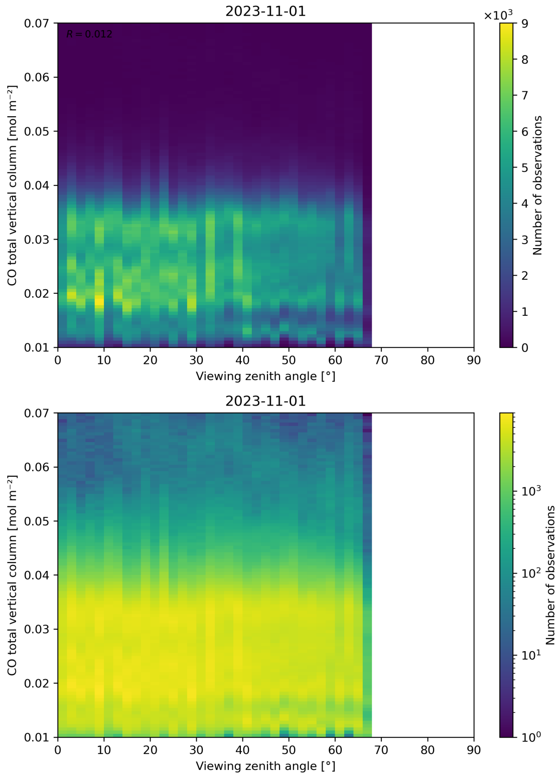
Figure 69: Scatter density plot of “Viewing zenith angle” against “CO total vertical column” for 2023-10-31 to 2023-11-02.
