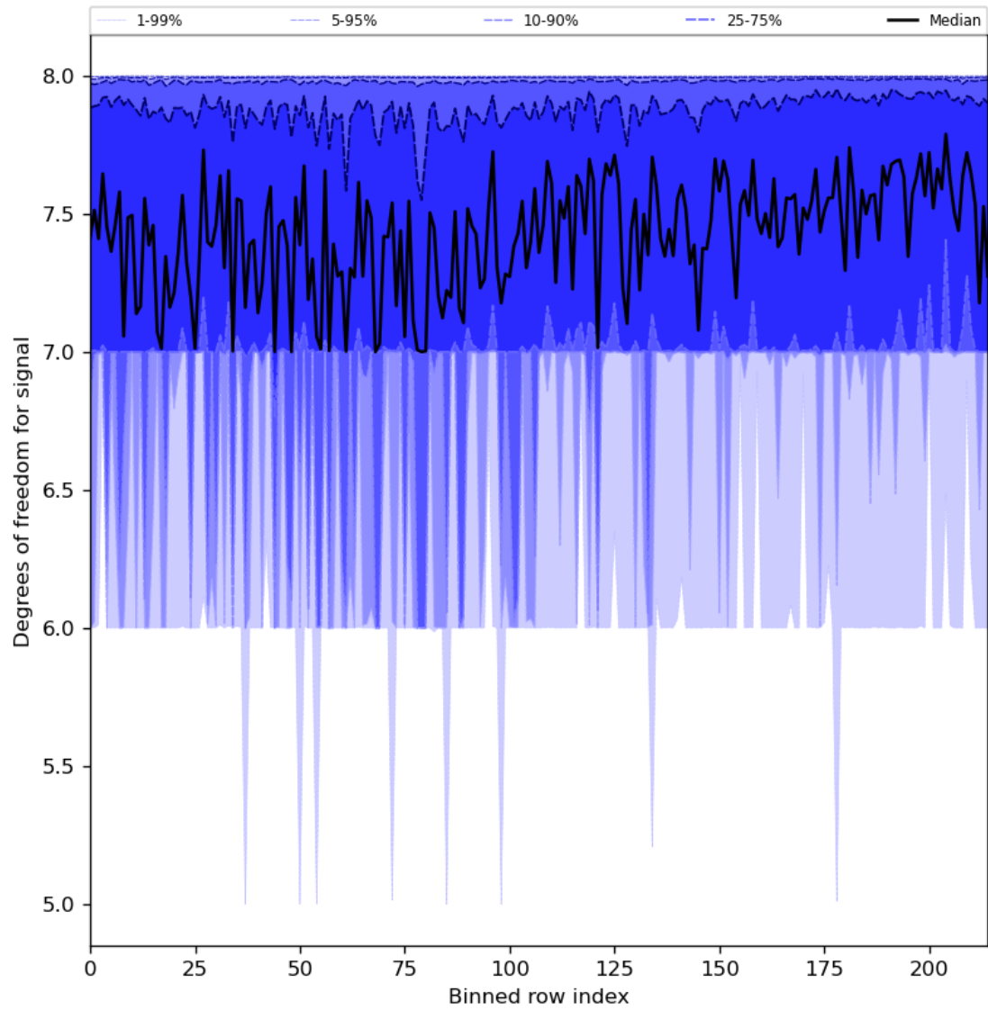
Figure 31: Along track statistics of “Degrees of freedom for signal” for 2023-10-31 to 2023-11-02
