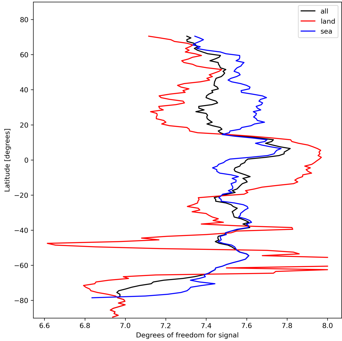
Figure 15: Zonal average of “Degrees of freedom for signal” for 2023-10-31 to 2023-11-02.
