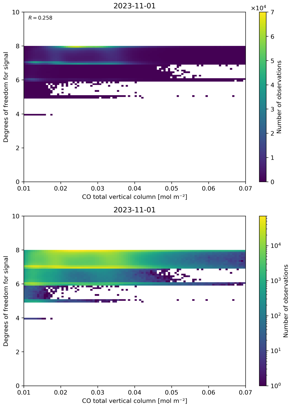
Figure 41: Scatter density plot of “CO total vertical column” against “Degrees of freedom for signal” for 2023-10-31 to 2023-11-02.
