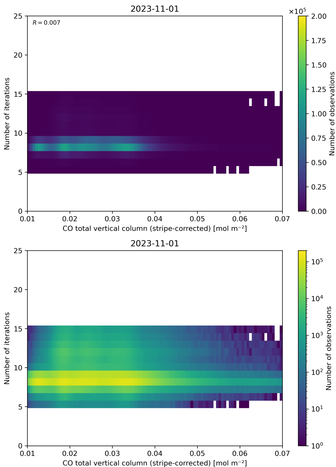
Figure 39: Scatter density plot of “CO total vertical column (stripe-corrected)” against “Number of iterations” for 2023-10-31 to 2023-11-02.
