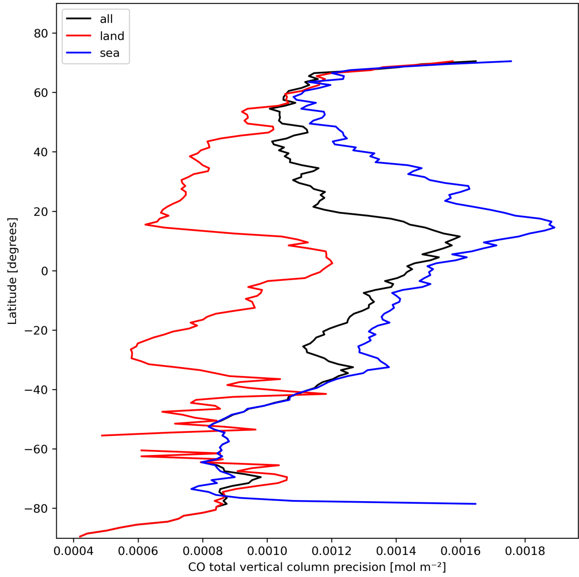
Figure 12: Zonal average of “CO total vertical column precision” for 2023-10-31 to 2023-11-02.
