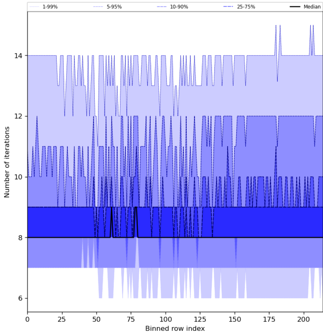
Figure 32: Along track statistics of “Number of iterations” for 2023-10-31 to 2023-11-02
