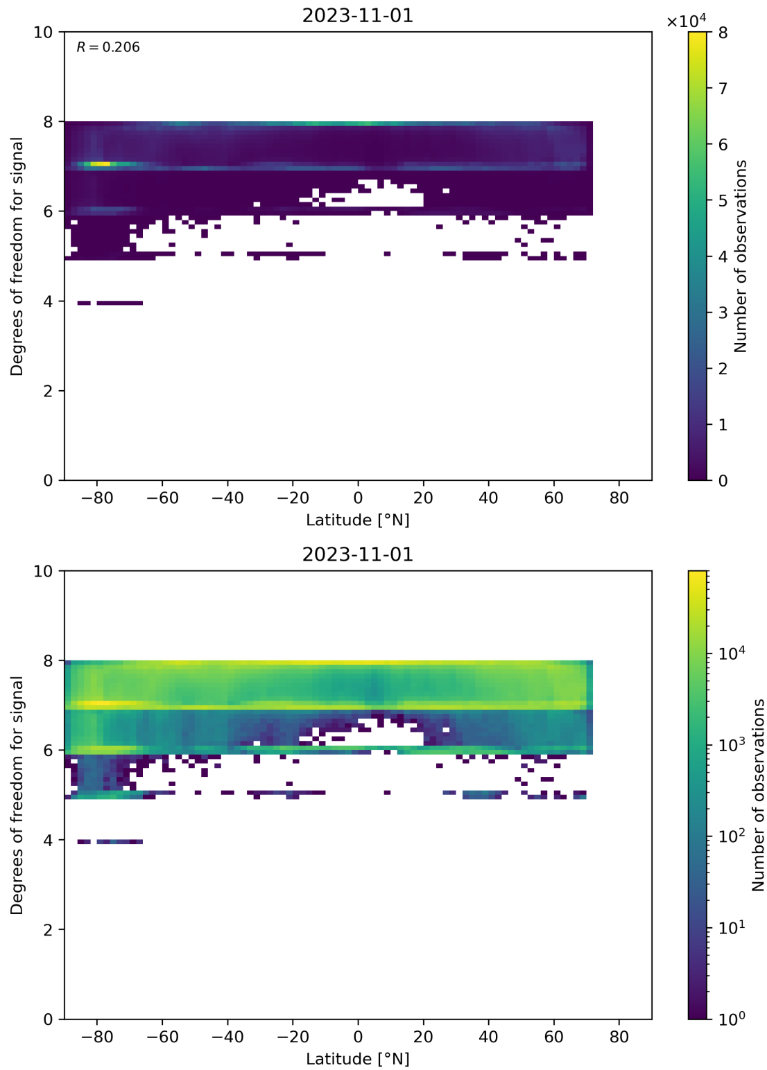
Figure 55: Scatter density plot of “Latitude” against “Degrees of freedom for signal” for 2023-10-31 to 2023-11-02.
