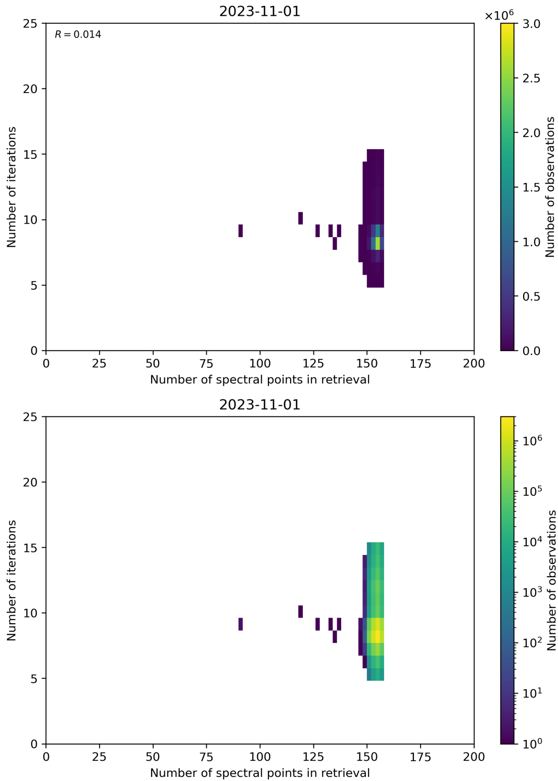
Figure 60: Scatter density plot of “Number of spectral points in retrieval” against “Number of iterations” for 2023-10-31 to 2023-11-02.
