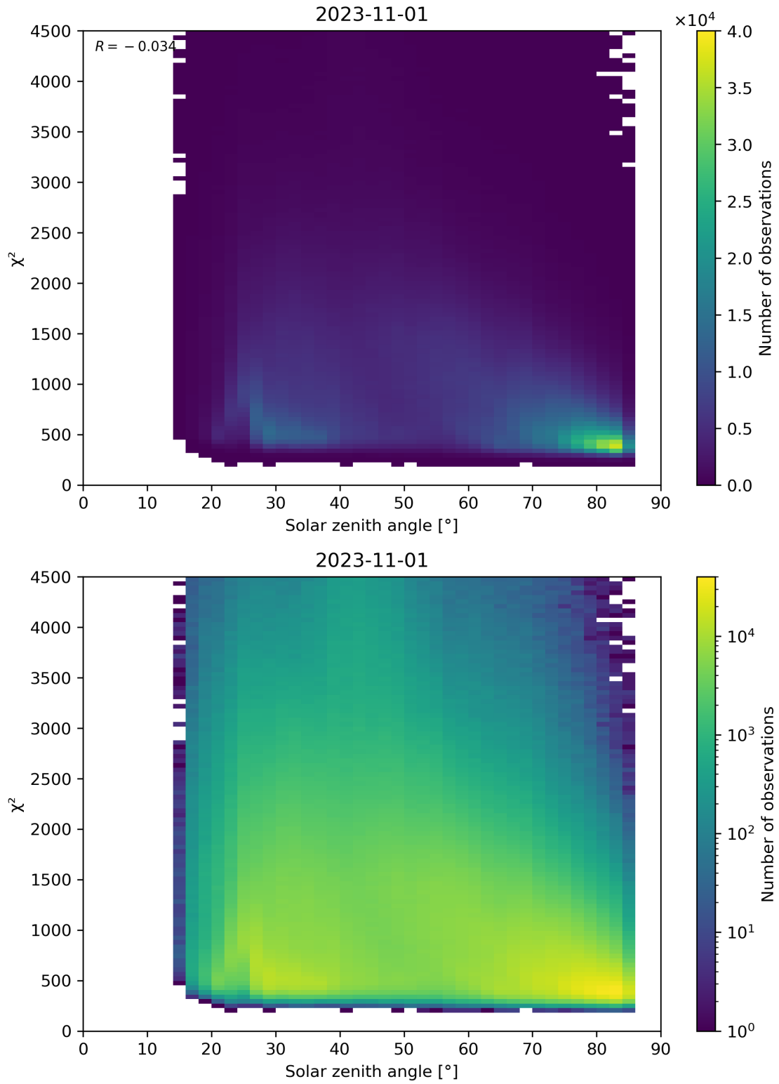
Figure 64: Scatter density plot of “Solar zenith angle” against “ \chi^2 ” for 2023-10-31 to 2023-11-02.
