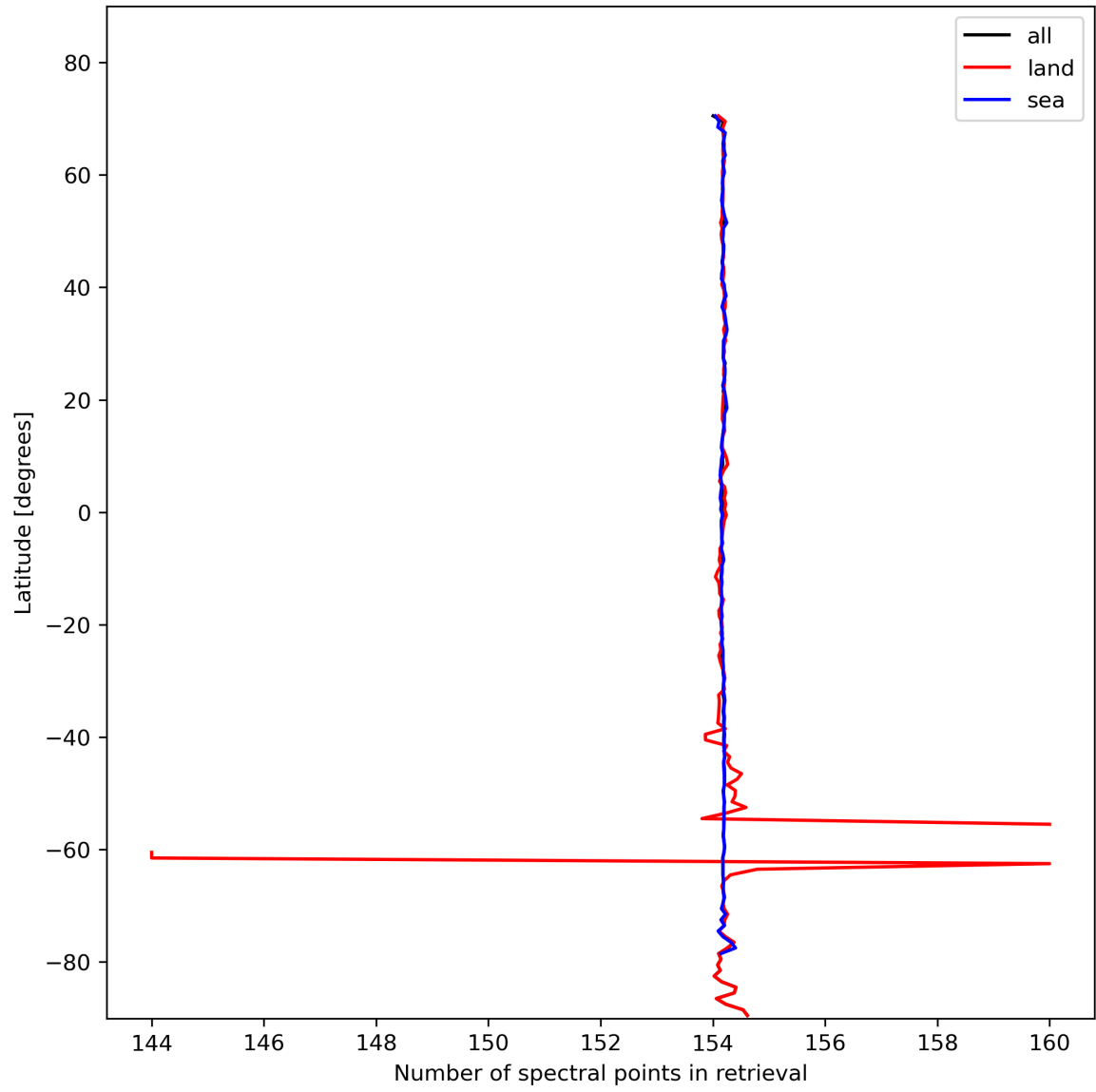
Figure 13: Zonal average of “Number of spectral points in retrieval” for 2023-10-31 to 2023-11-02.
