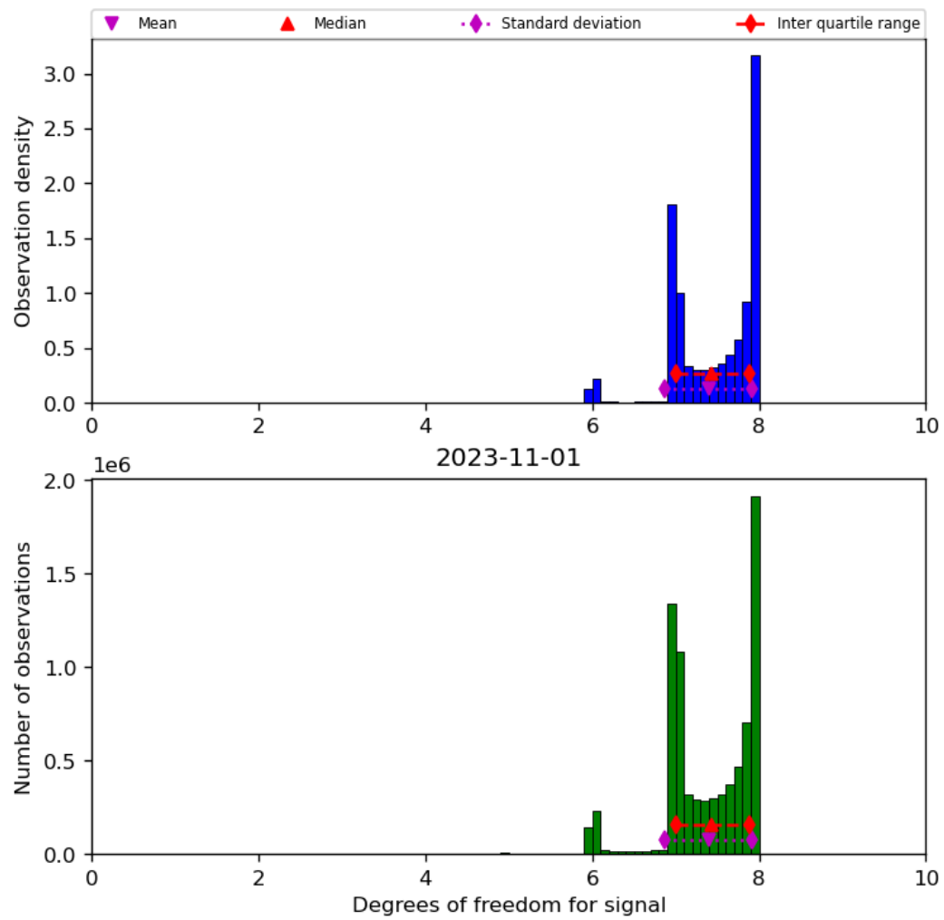
Figure 23: Histogram of “Degrees of freedom for signal” for 2023-10-31 to 2023-11-02
