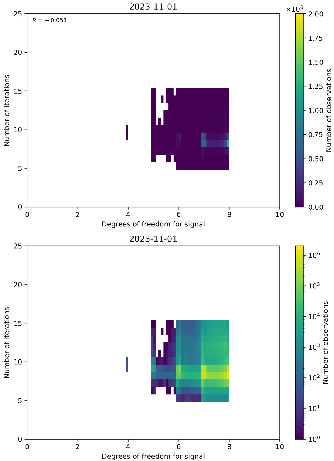
Figure 50: Scatter density plot of “Degrees of freedom for signal” against “Number of iterations” for 2023-10-31 to 2023-11-02.
