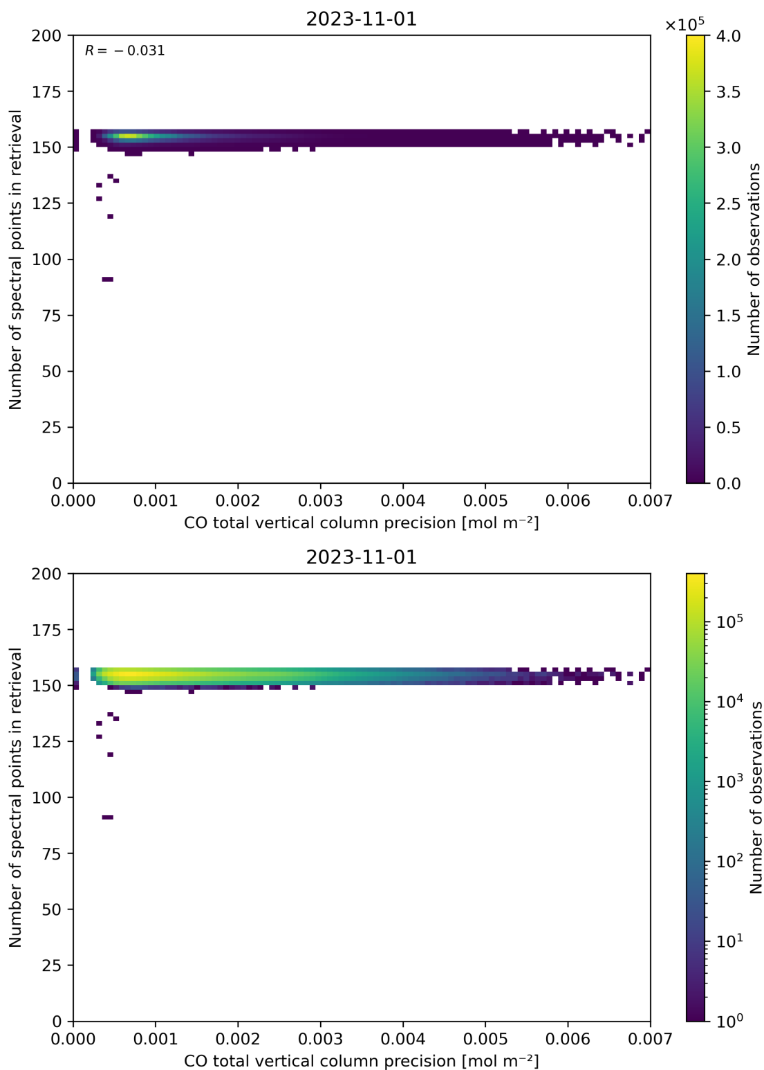
Figure 47: Scatter density plot of “CO total vertical column precision” against “Number of spectral points in retrieval” for 2023-10-31 to 2023-11-02.
