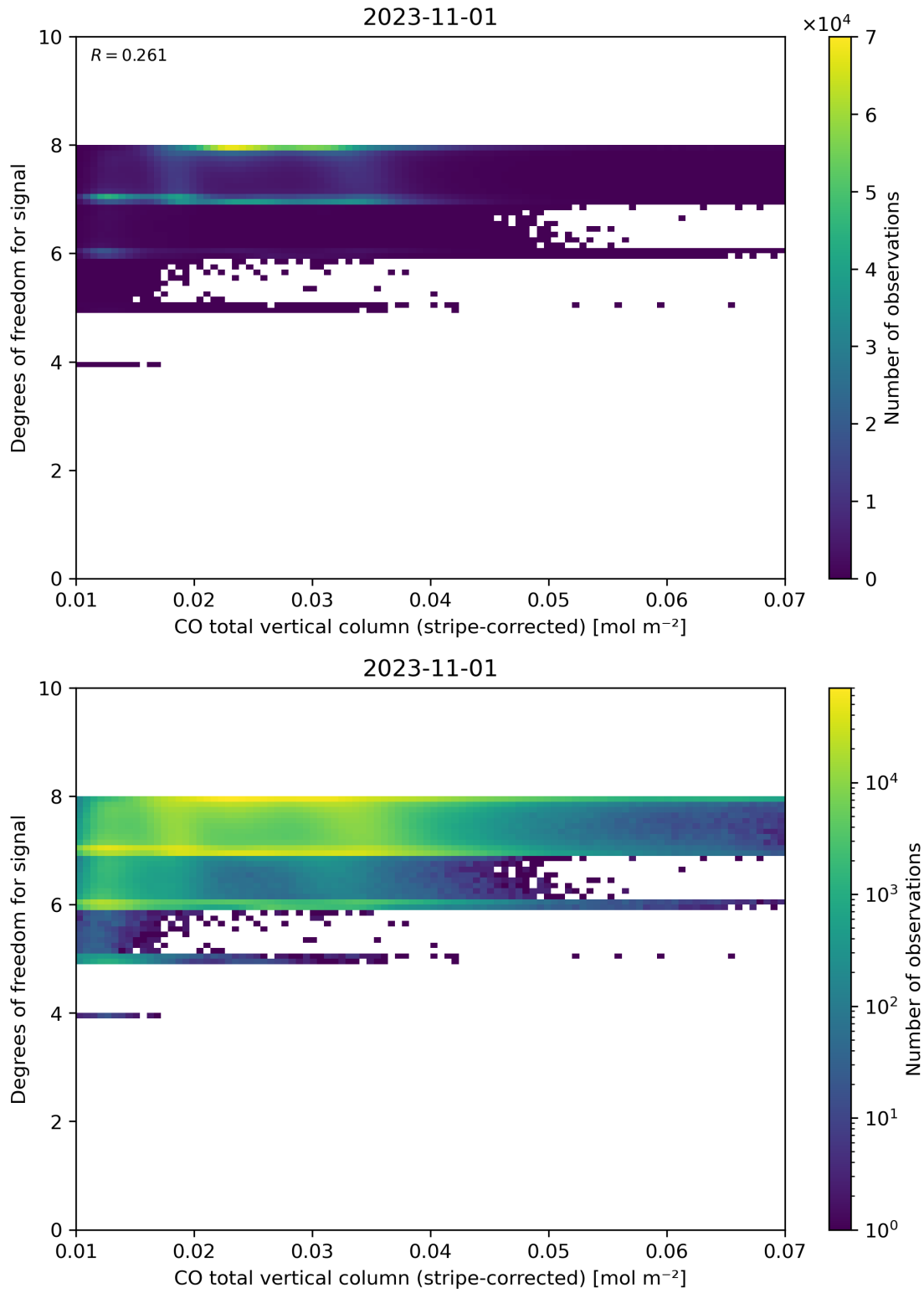
Figure 38: Scatter density plot of “CO total vertical column (stripe-corrected)” against “Degrees of freedom for signal” for 2023-10-31 to 2023-11-02.
