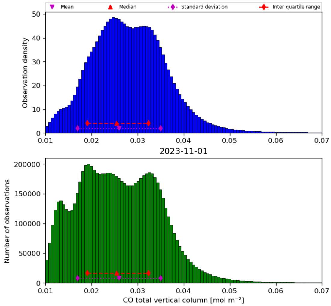
Figure 18: Histogram of “CO total vertical column” for 2023-10-31 to 2023-11-02
