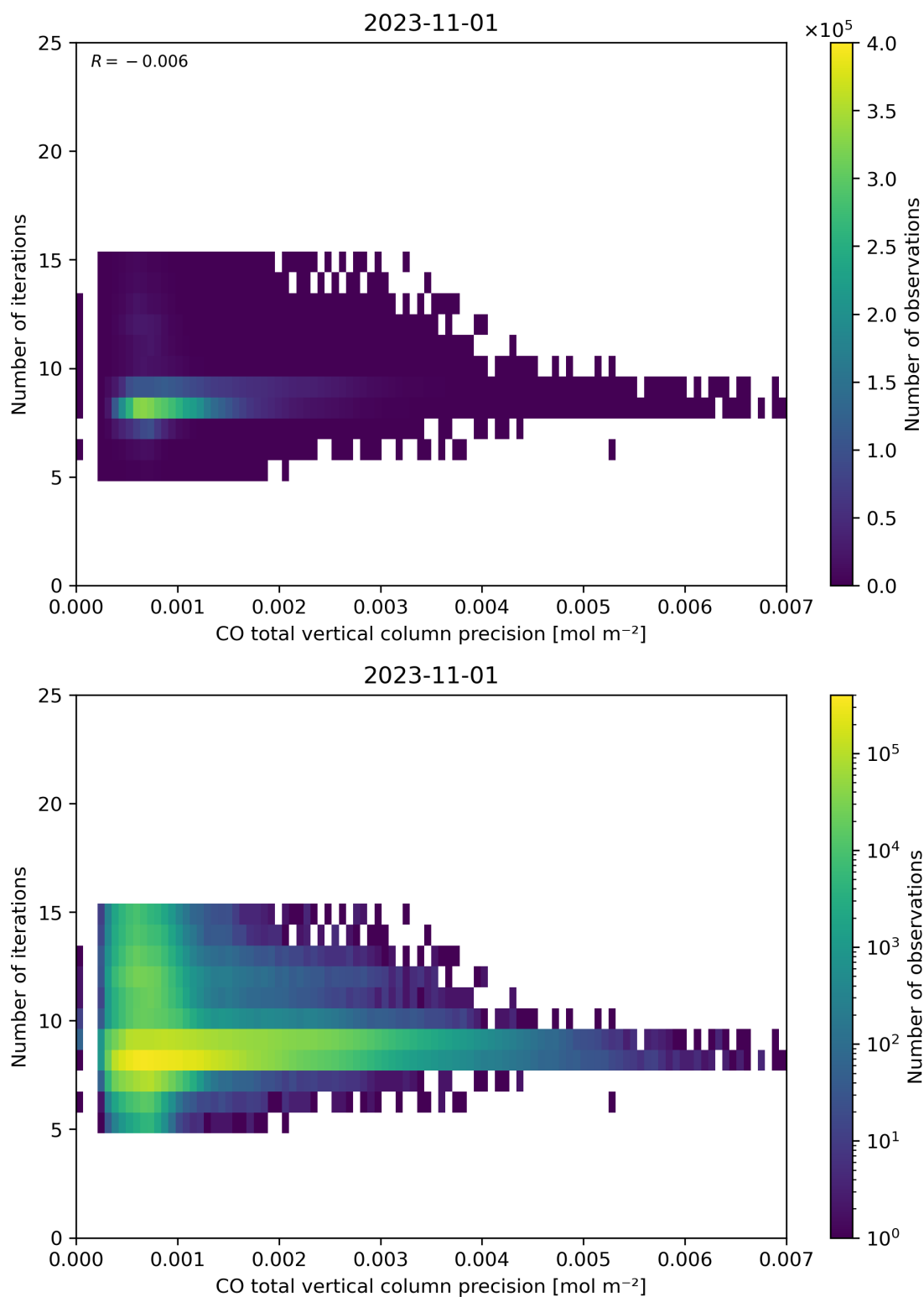
Figure 46: Scatter density plot of “CO total vertical column precision” against “Number of iterations” for 2023-10-31 to 2023-11-02.
