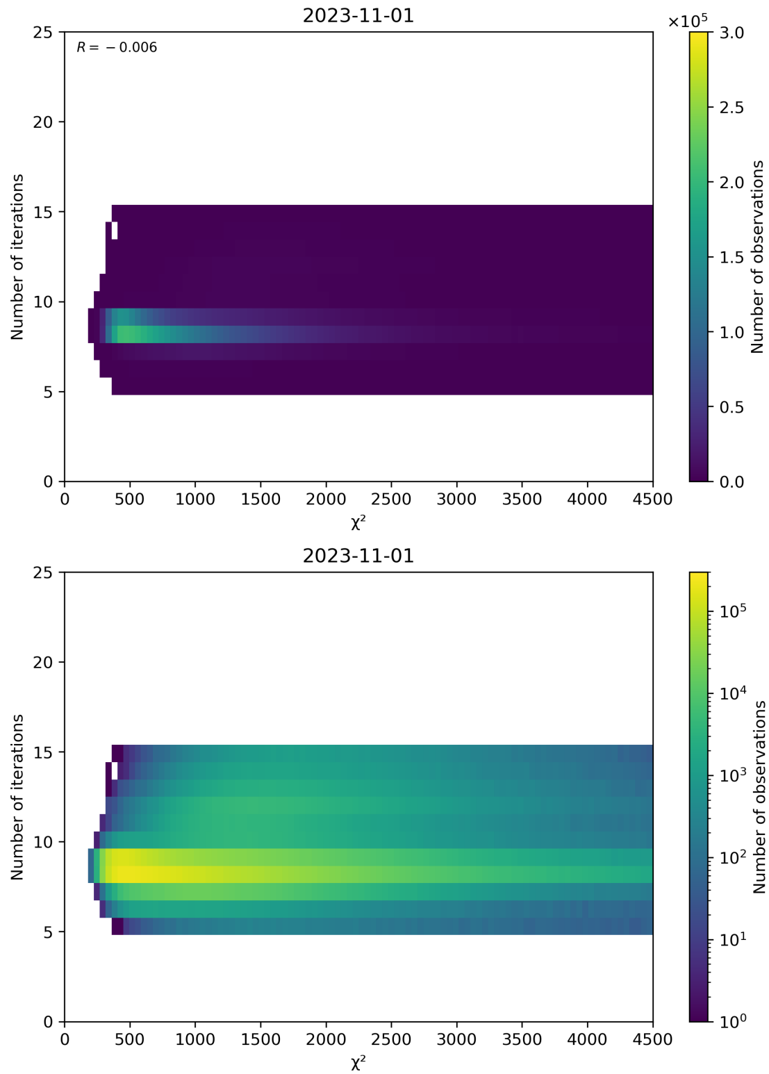
Figure 49: Scatter density plot of “ \chi^2 ” against “Number of iterations” for 2023-10-31 to 2023-11-02.
