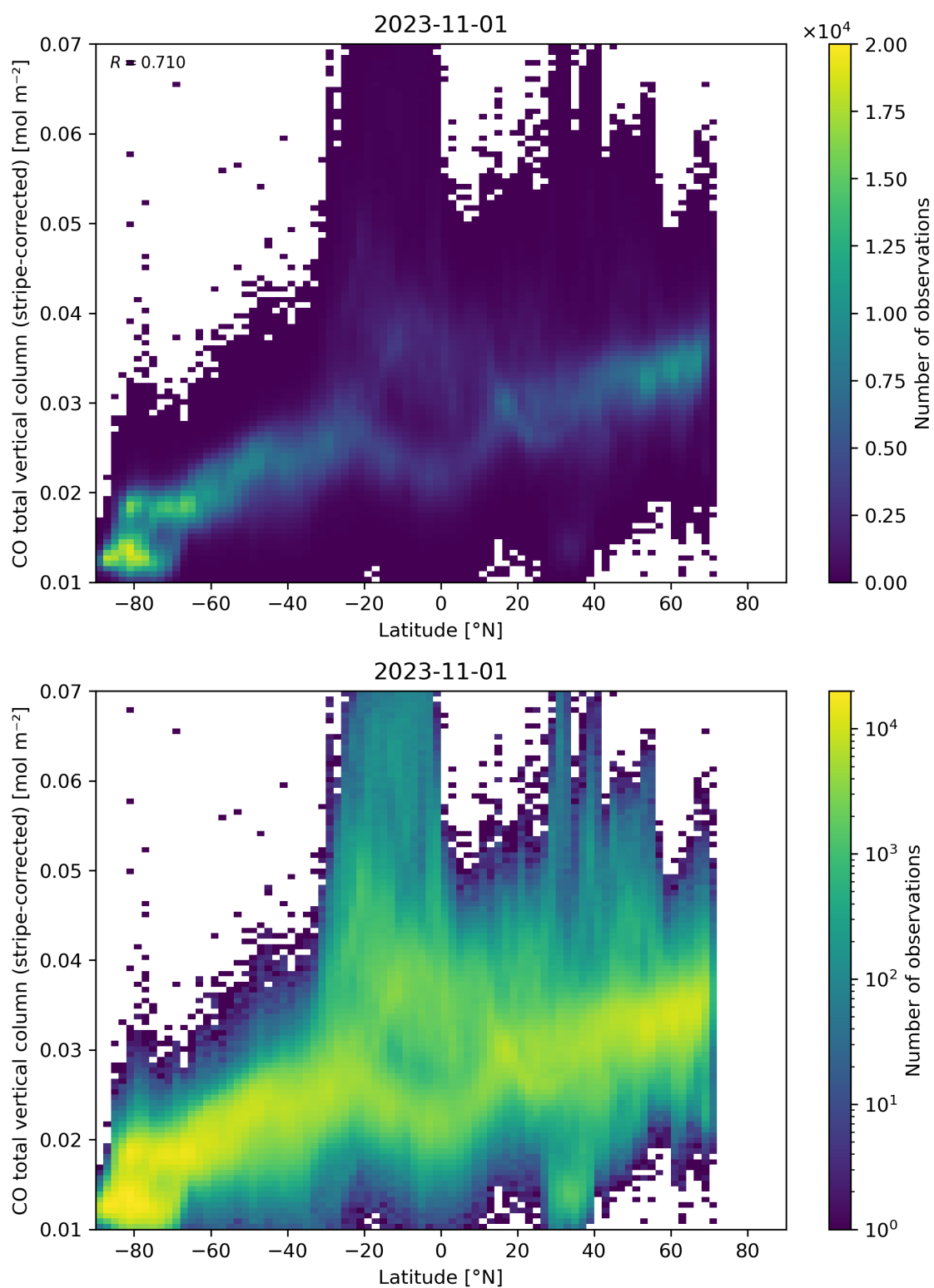
Figure 52: Scatter density plot of “Latitude” against “CO total vertical column (stripe-corrected)” for 2023-10-31 to 2023-11-02.
