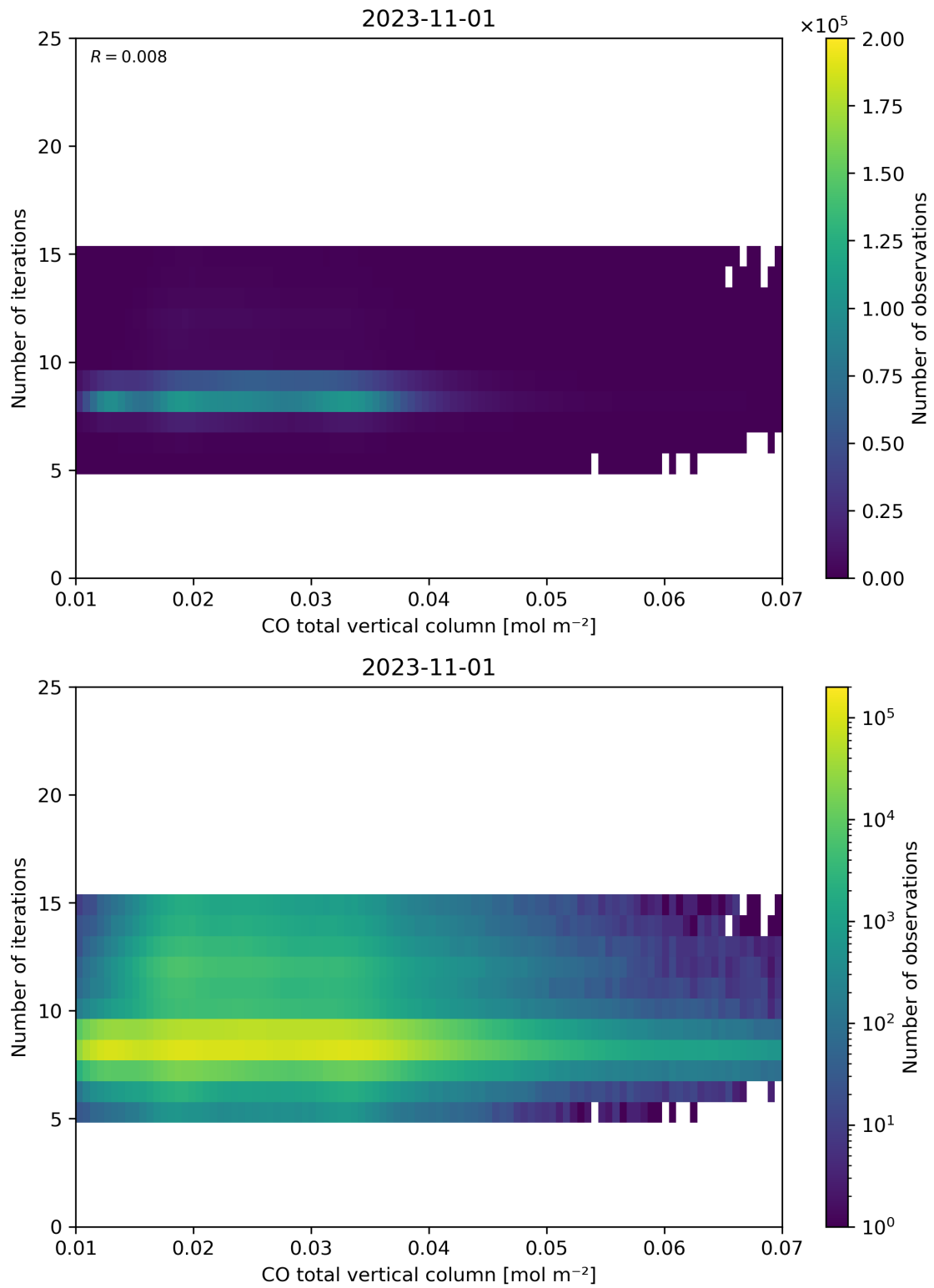
Figure 42: Scatter density plot of “CO total vertical column” against “Number of iterations” for 2023-10-31 to 2023-11-02.
