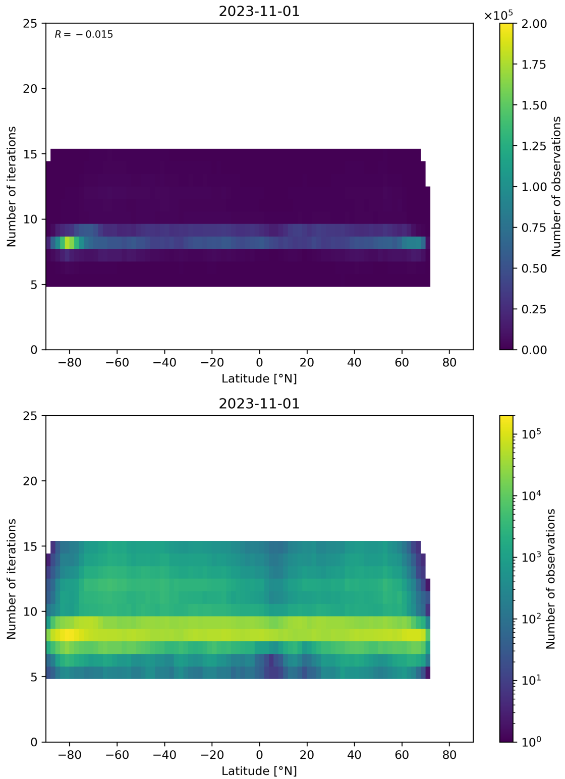
Figure 56: Scatter density plot of “Latitude” against “Number of iterations” for 2023-10-31 to 2023-11-02.
