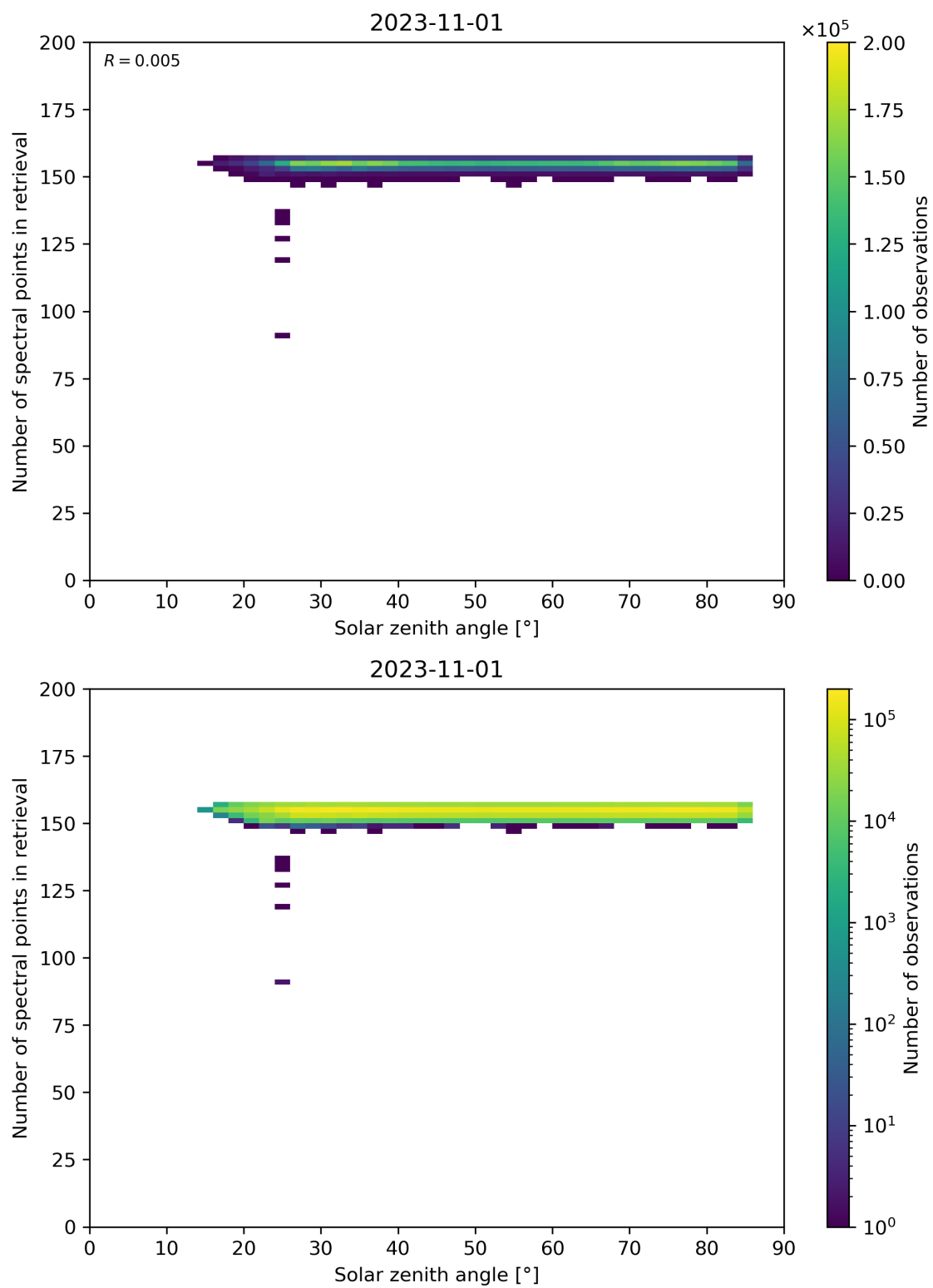
Figure 68: Scatter density plot of “Solar zenith angle” against “Number of spectral points in retrieval” for 2023-10-31 to 2023-11-02.
