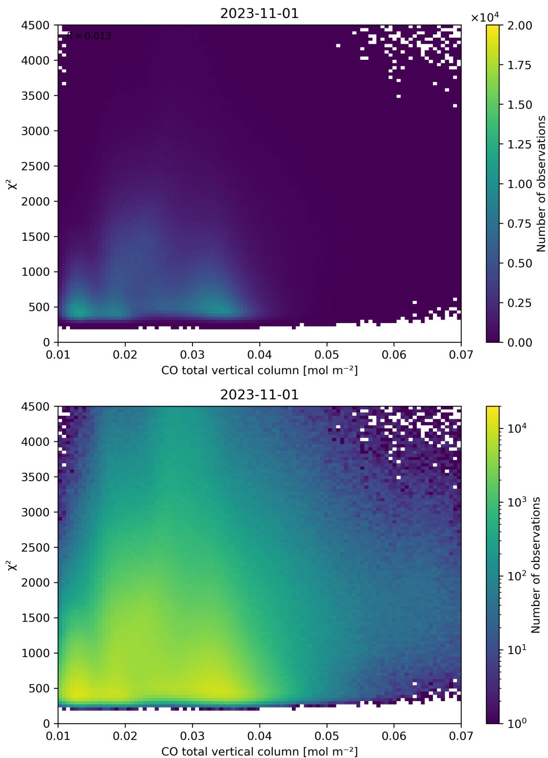
Figure 35: Scatter density plot of “CO total vertical column” against “ \chi^2 ” for 2023-10-31 to 2023-11-02.
