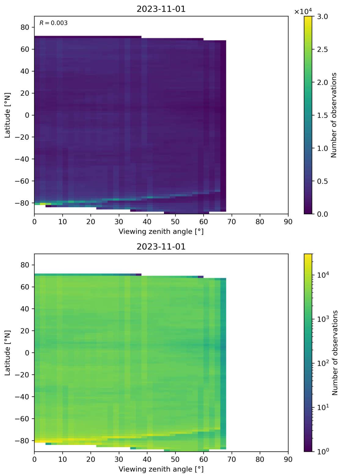
Figure 74: Scatter density plot of “Viewing zenith angle” against “Latitude” for 2023-10-31 to 2023-11-02.
