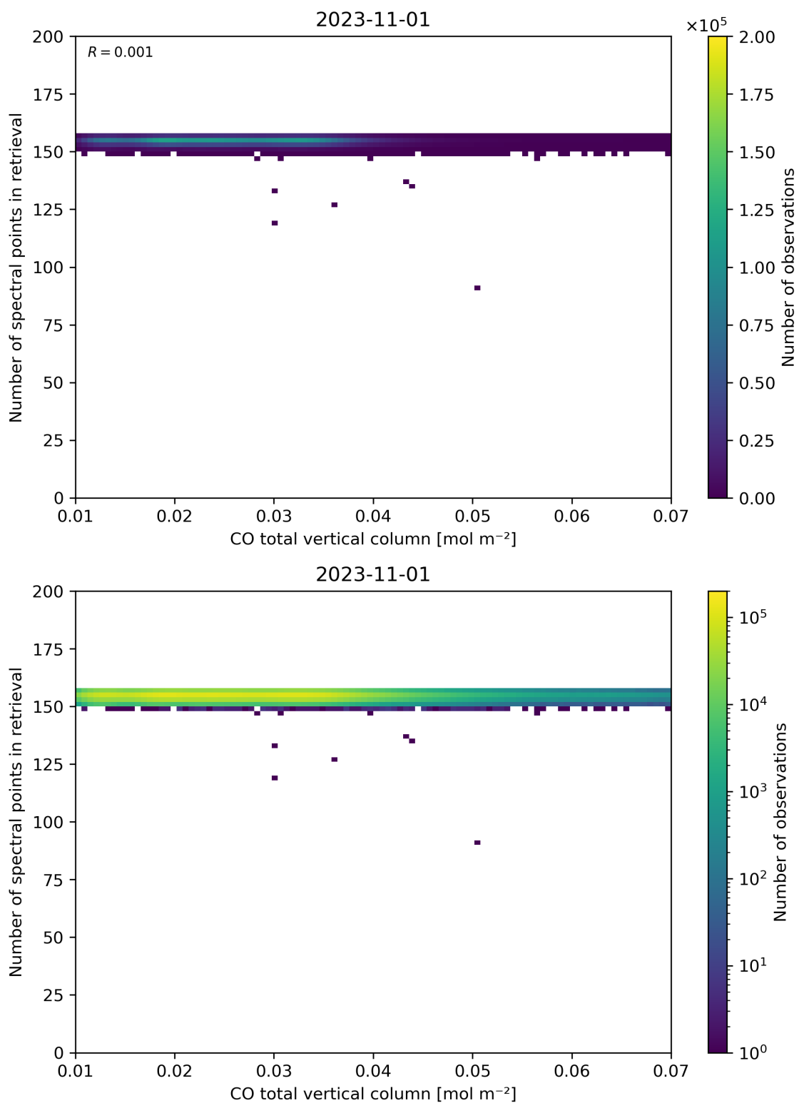
Figure 43: Scatter density plot of “CO total vertical column” against “Number of spectral points in retrieval” for 2023-10-31 to 2023-11-02.
