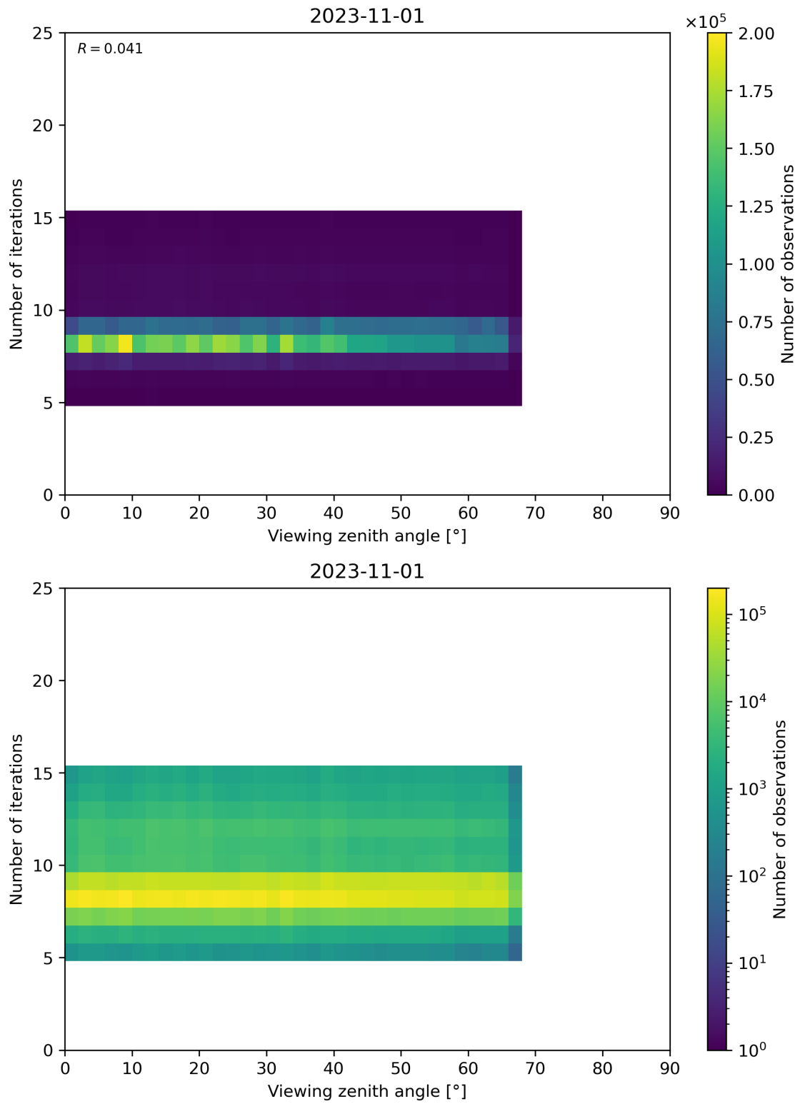
Figure 75: Scatter density plot of “Viewing zenith angle” against “Number of iterations” for 2023-10-31 to 2023-11-02.
