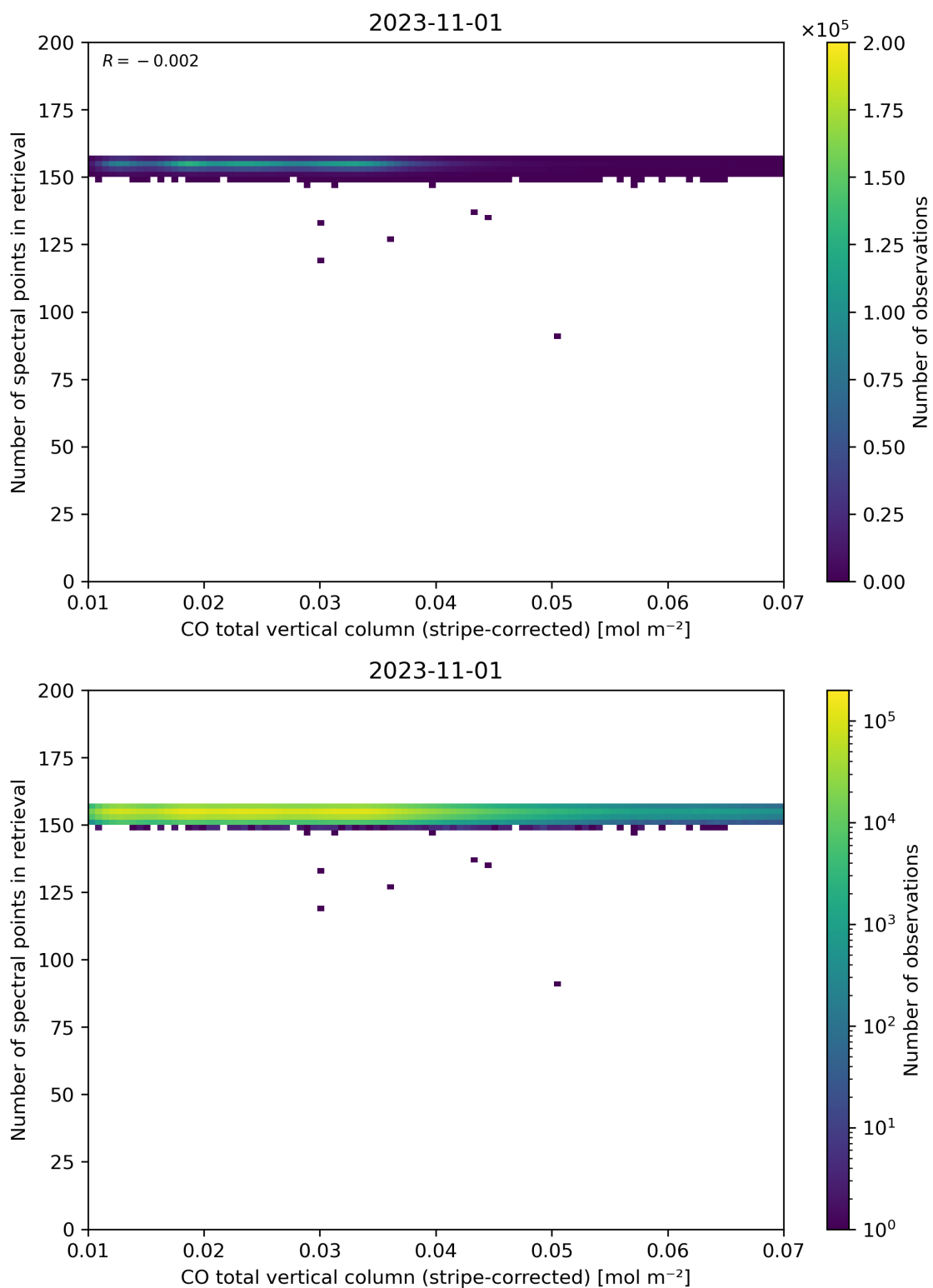
Figure 40: Scatter density plot of “CO total vertical column (stripe-corrected)” against “Number of spectral points in retrieval” for 2023-10-31 to 2023-11-02.
