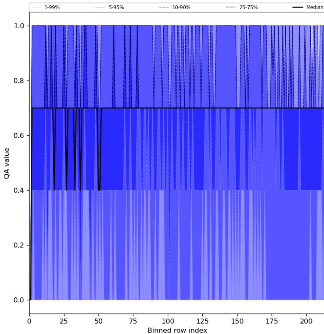
Figure 25: Along track statistics of “QA value” for 2023-10-31 to 2023-11-02
