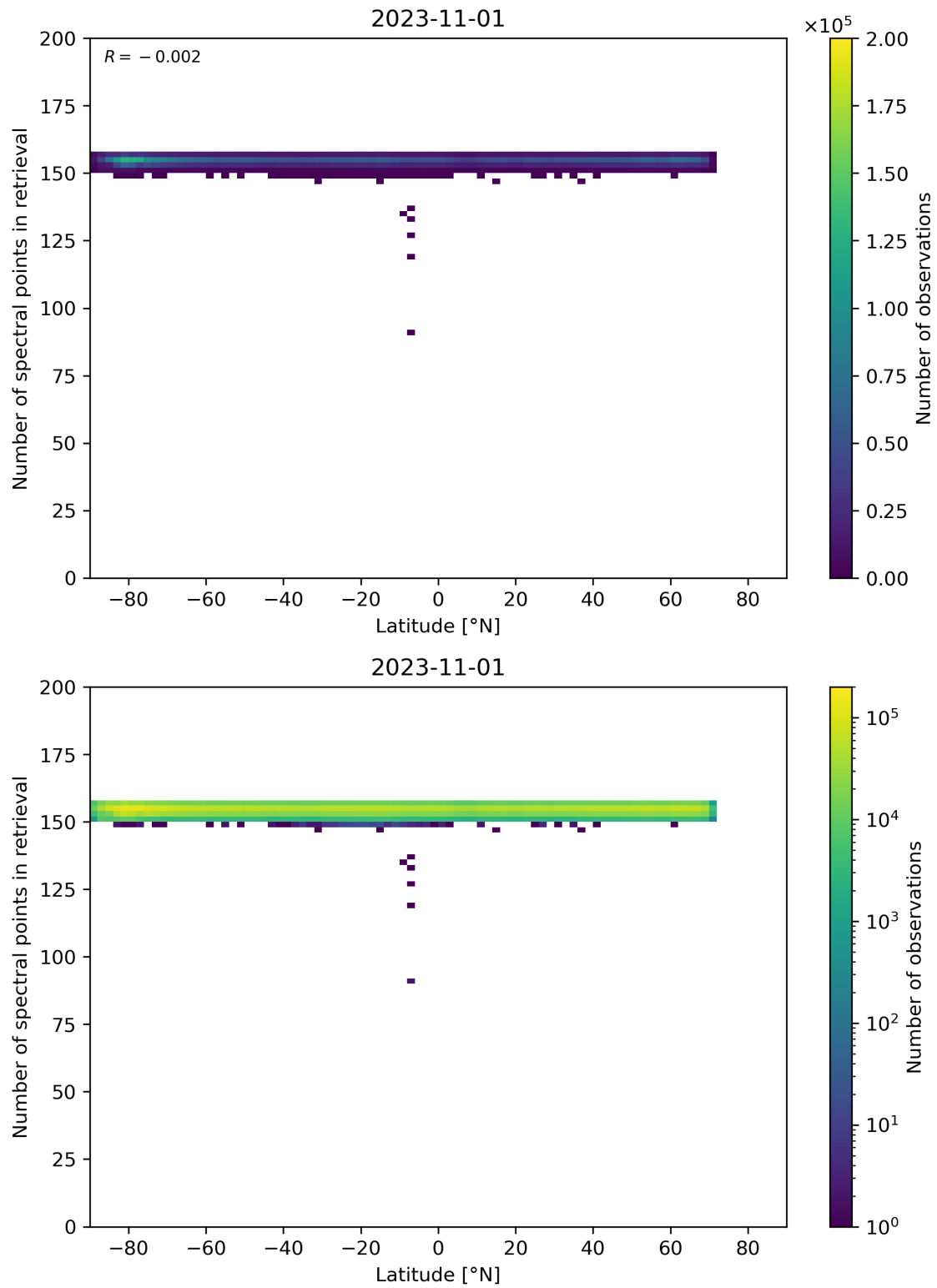
Figure 57: Scatter density plot of “Latitude” against “Number of spectral points in retrieval” for 2023-10-31 to 2023-11-02.
