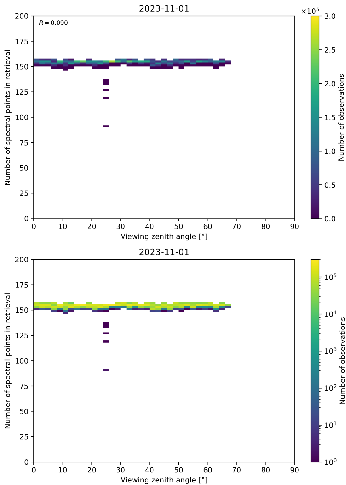
Figure 76: Scatter density plot of “Viewing zenith angle” against “Number of spectral points in retrieval” for 2023-10-31 to 2023-11-02.
