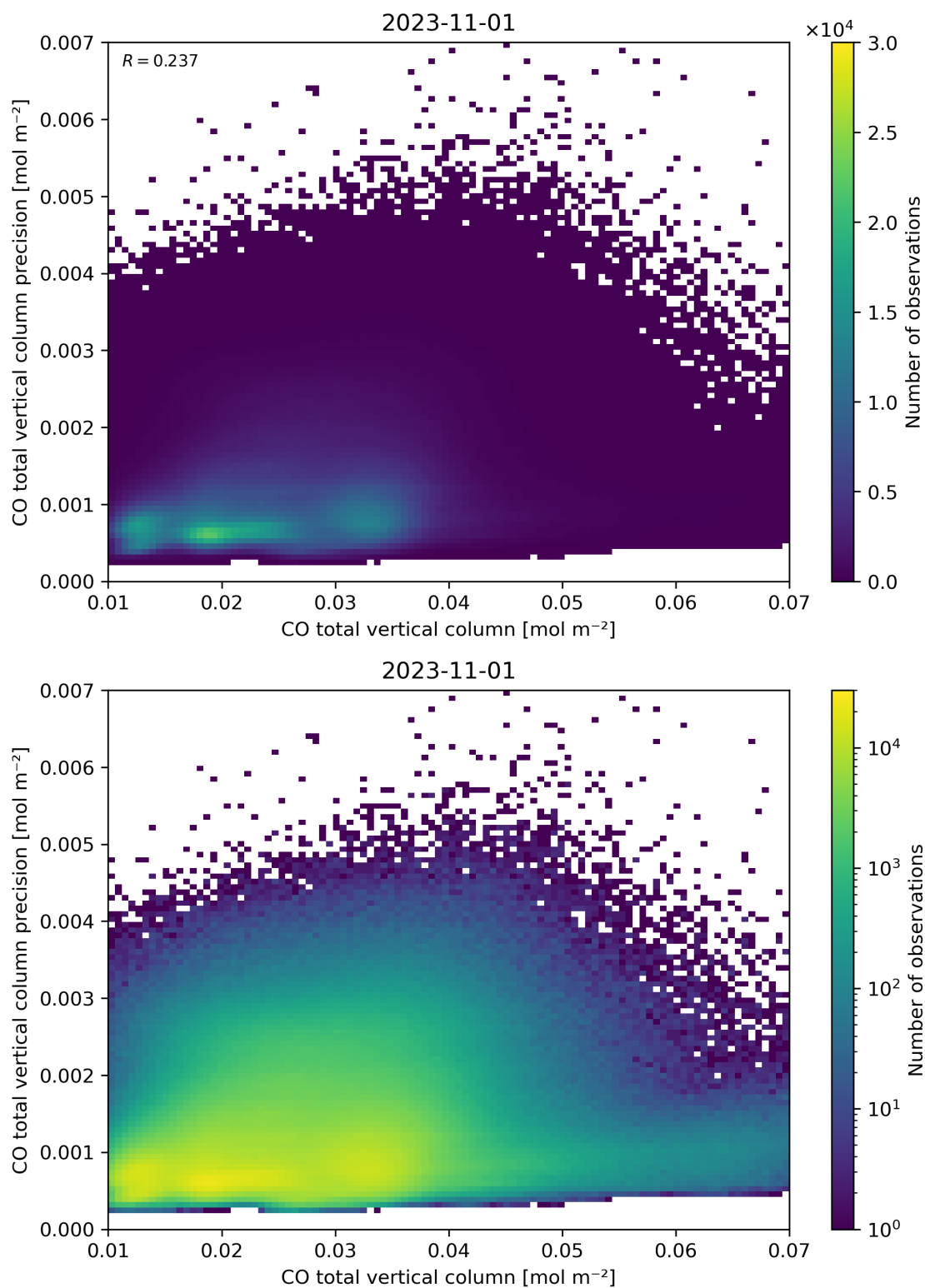
Figure 34: Scatter density plot of “CO total vertical column” against “CO total vertical column precision” for 2023-10-31 to 2023-11-02.
