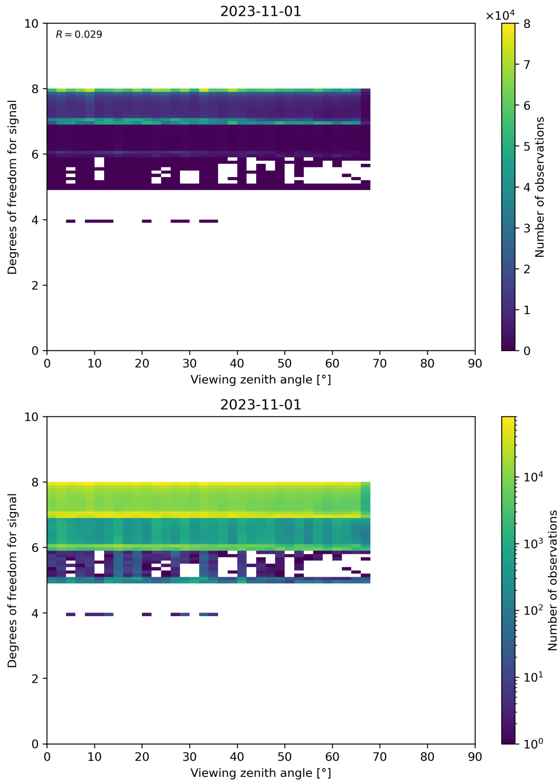
Figure 73: Scatter density plot of “Viewing zenith angle” against “Degrees of freedom for signal” for 2023-10-31 to 2023-11-02.
