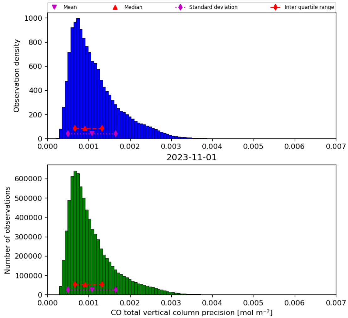
Figure 20: Histogram of “CO total vertical column precision” for 2023-10-31 to 2023-11-02
