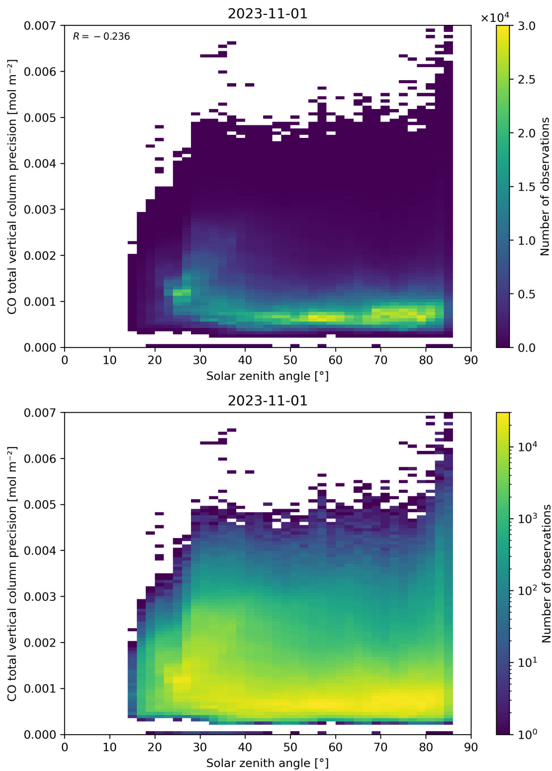
Figure 63: Scatter density plot of “Solar zenith angle” against “CO total vertical column precision” for 2023-10-31 to 2023-11-02.
