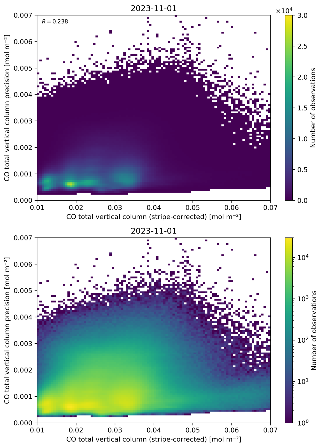
Figure 36: Scatter density plot of “CO total vertical column (stripe-corrected)” against “CO total vertical column precision” for 2023-10-31 to 2023-11-02.
