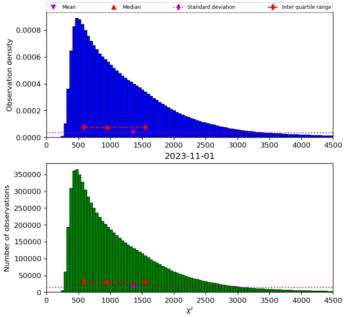
Figure 22: Histogram of “ \chi^2 ” for 2023-10-31 to 2023-11-02
