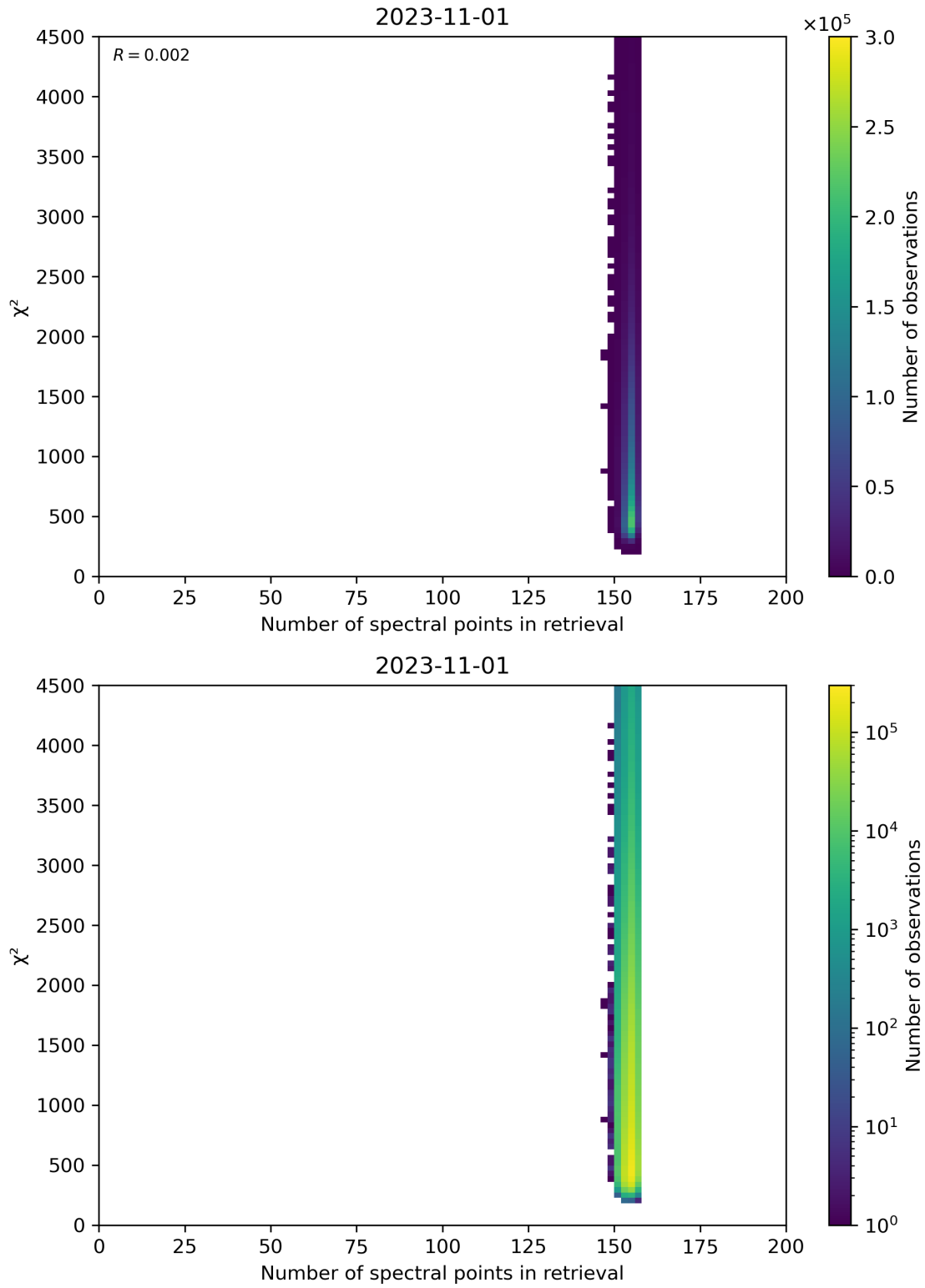
Figure 58: Scatter density plot of “Number of spectral points in retrieval” against “ \chi^2 ” for 2023-10-31 to 2023-11-02.
