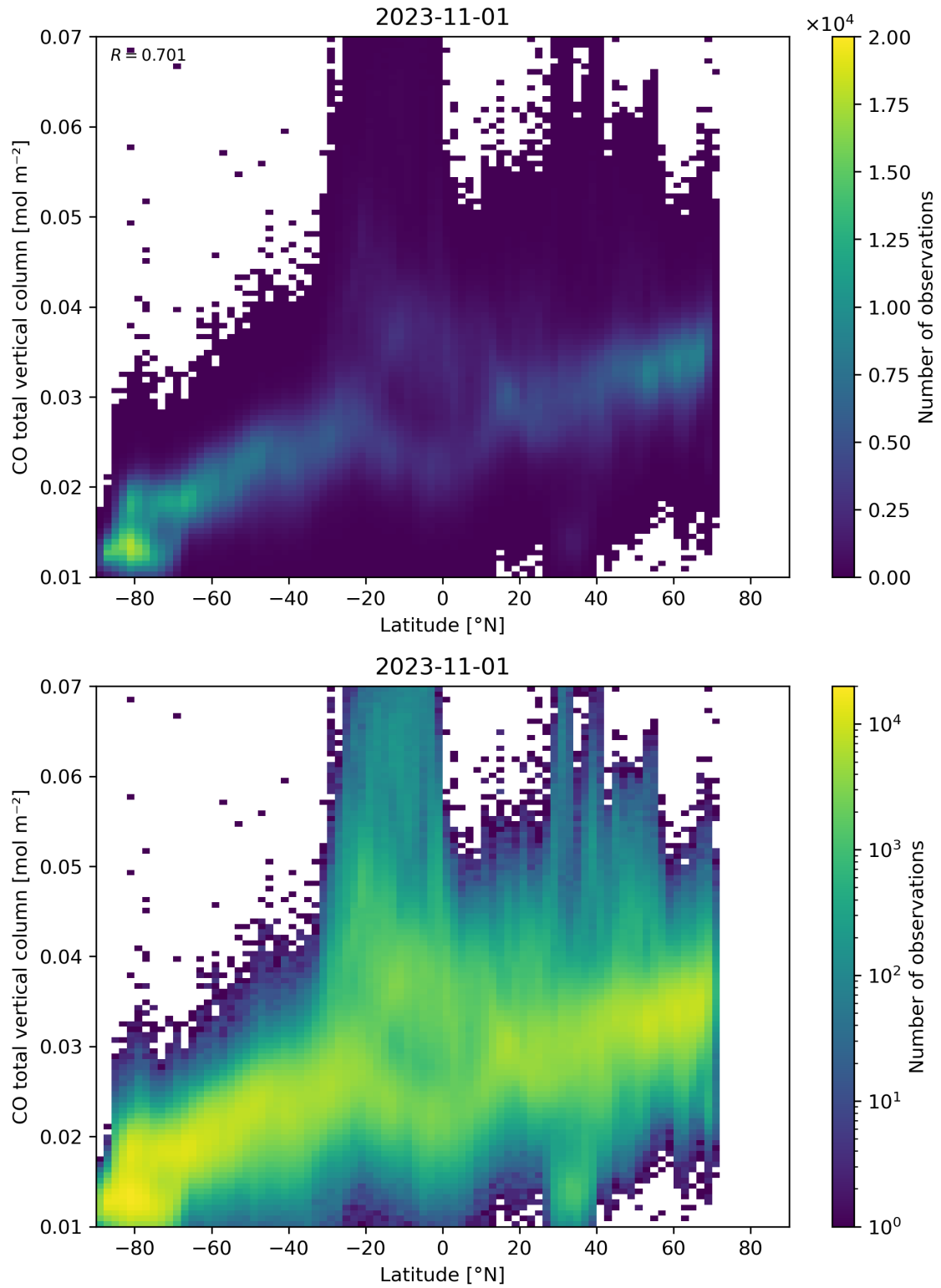
Figure 51: Scatter density plot of “Latitude” against “CO total vertical column” for 2023-10-31 to 2023-11-02.
