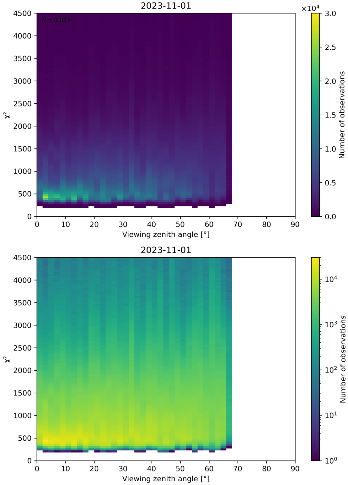
Figure 72: Scatter density plot of “Viewing zenith angle” against “ \chi^2 ” for 2023-10-31 to 2023-11-02.
