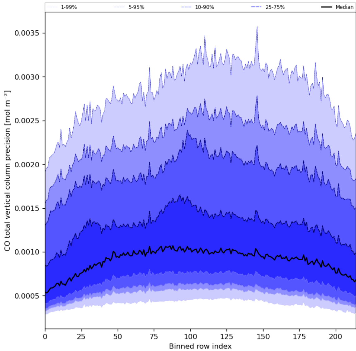
Figure 28: Along track statistics of “CO total vertical column precision” for 2023-10-31 to 2023-11-02
