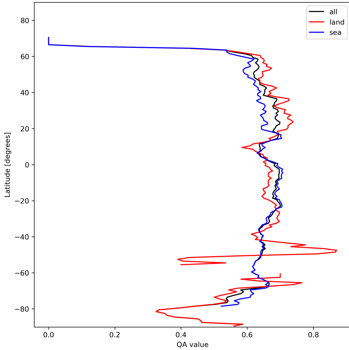
Figure 9: Zonal average of “QA value” for 2023-10-31 to 2023-11-02.
