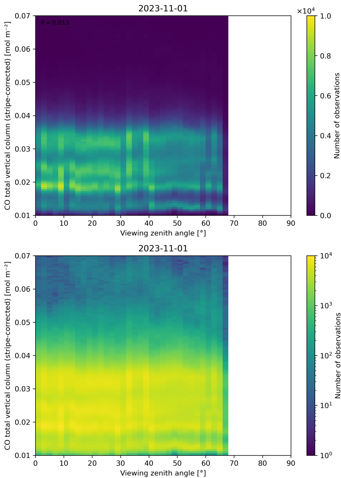
Figure 70: Scatter density plot of “Viewing zenith angle” against “CO total vertical column (stripe-corrected)” for 2023-10-31 to 2023-11-02.
