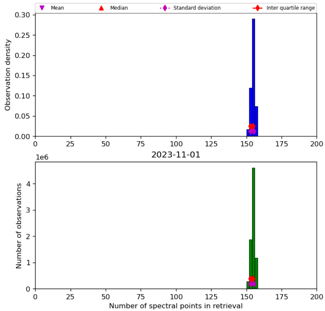
Figure 21: Histogram of “Number of spectral points in retrieval” for 2023-10-31 to 2023-11-02
