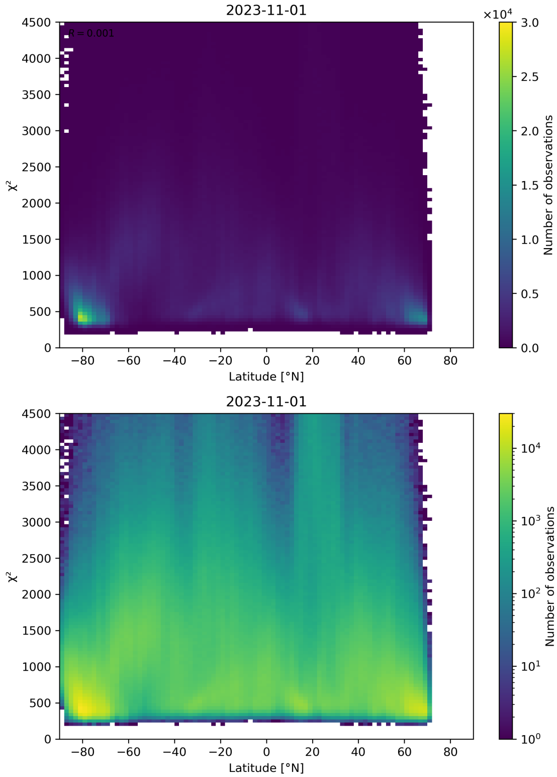
Figure 54: Scatter density plot of “Latitude” against “ \chi^2 ” for 2023-10-31 to 2023-11-02.
