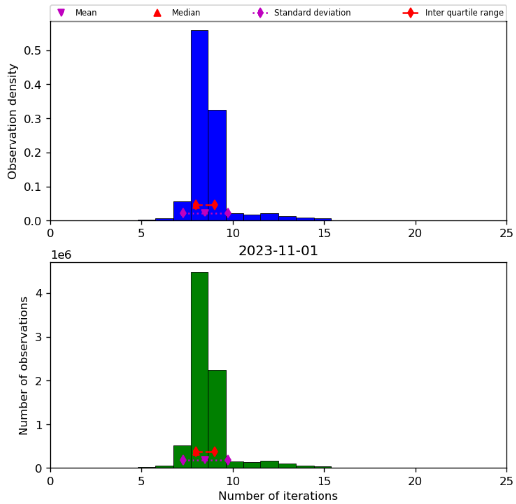
Figure 24: Histogram of “Number of iterations” for 2023-10-31 to 2023-11-02
