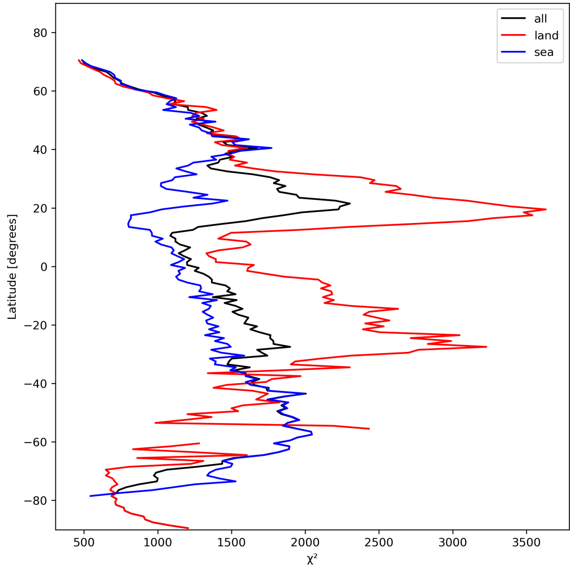
Figure 14: Zonal average of “ \chi^2 ” for 2023-10-31 to 2023-11-02.
