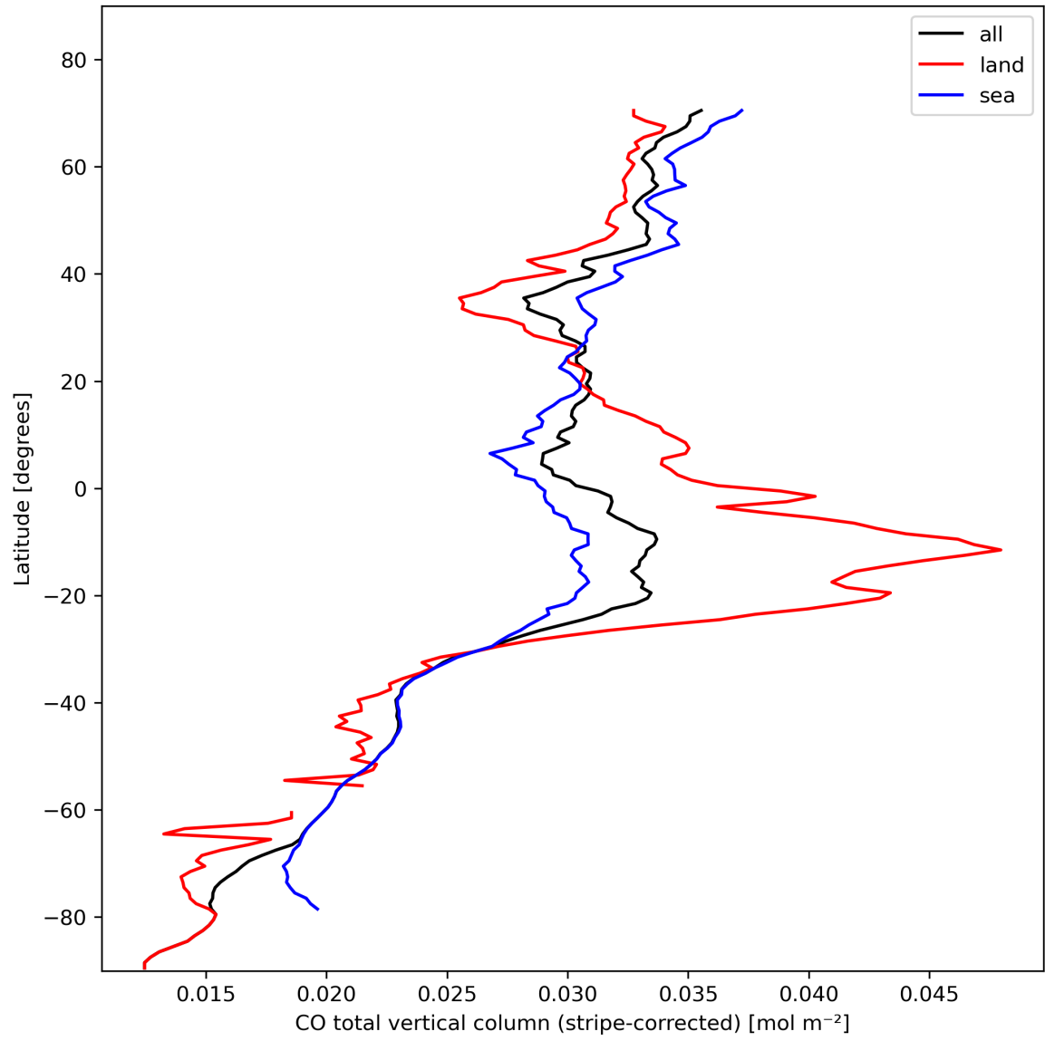
Figure 11: Zonal average of “CO total vertical column (stripe-corrected)” for 2023-10-31 to 2023-11-02.
