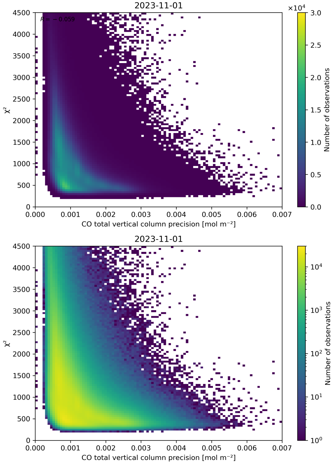
Figure 44: Scatter density plot of “CO total vertical column precision” against “ \chi^2 ” for 2023-10-31 to 2023-11-02.
