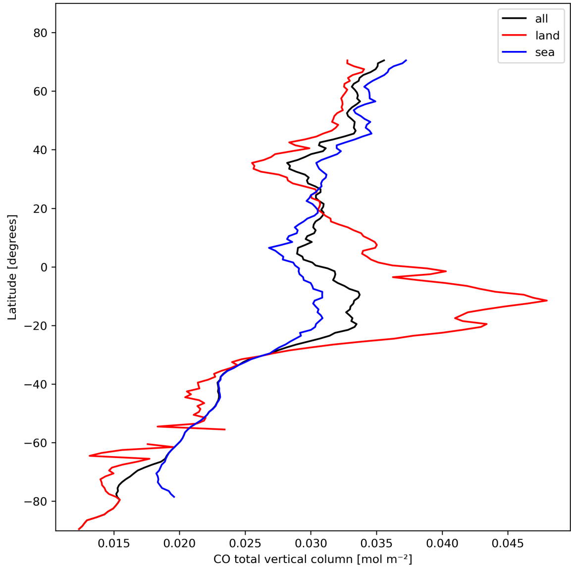
Figure 10: Zonal average of “CO total vertical column” for 2023-10-31 to 2023-11-02.
