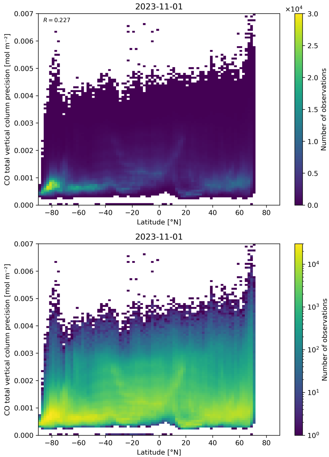
Figure 53: Scatter density plot of “Latitude” against “CO total vertical column precision” for 2023-10-31 to 2023-11-02.
