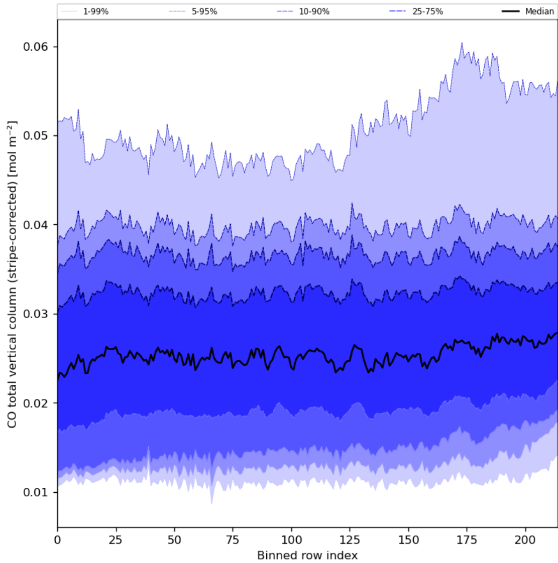
Figure 27: Along track statistics of “CO total vertical column (stripe-corrected)” for 2023-10-31 to 2023-11-02
