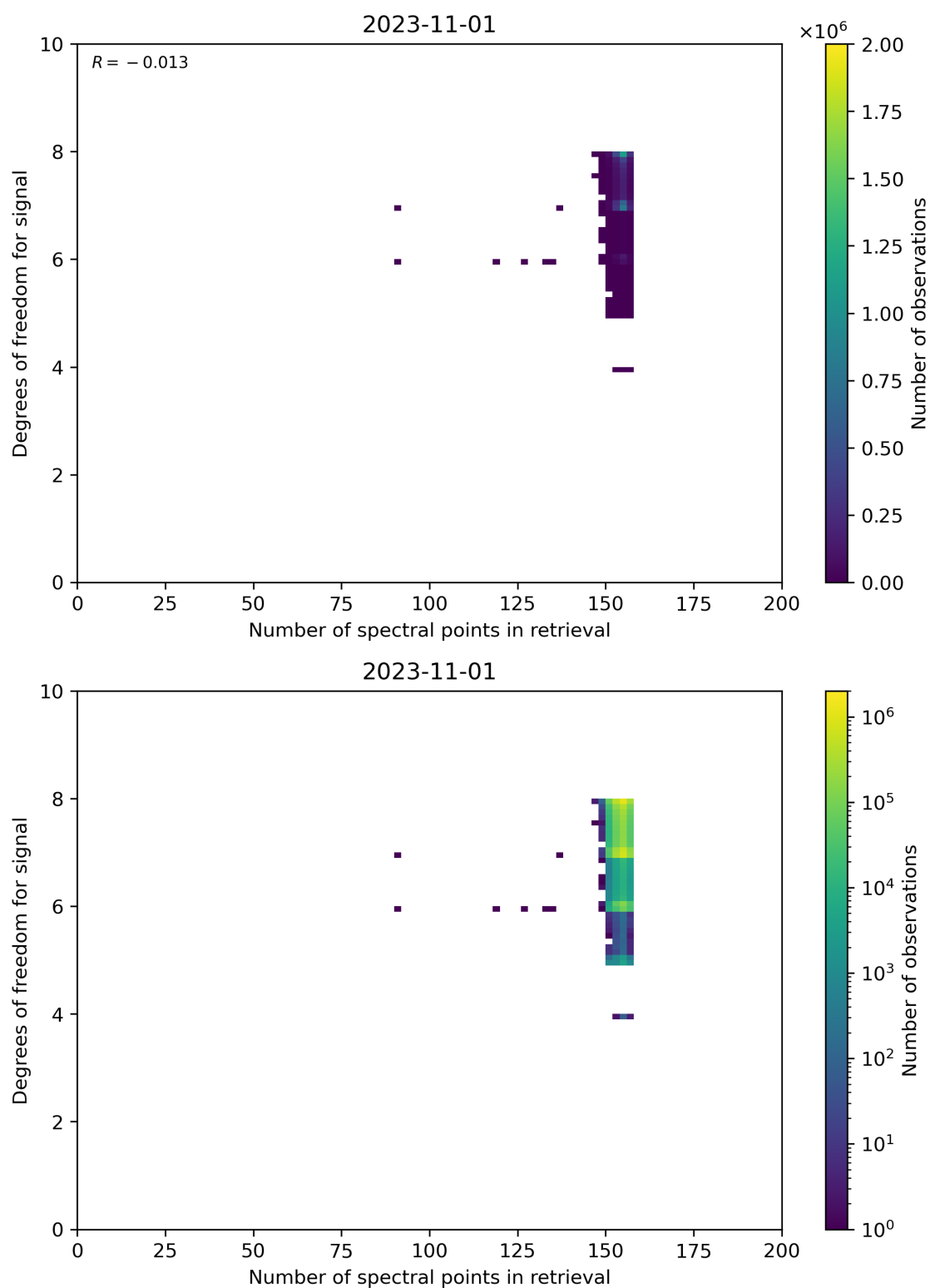
Figure 59: Scatter density plot of “Number of spectral points in retrieval” against “Degrees of freedom for signal” for 2023-10-31 to 2023-11-02.
