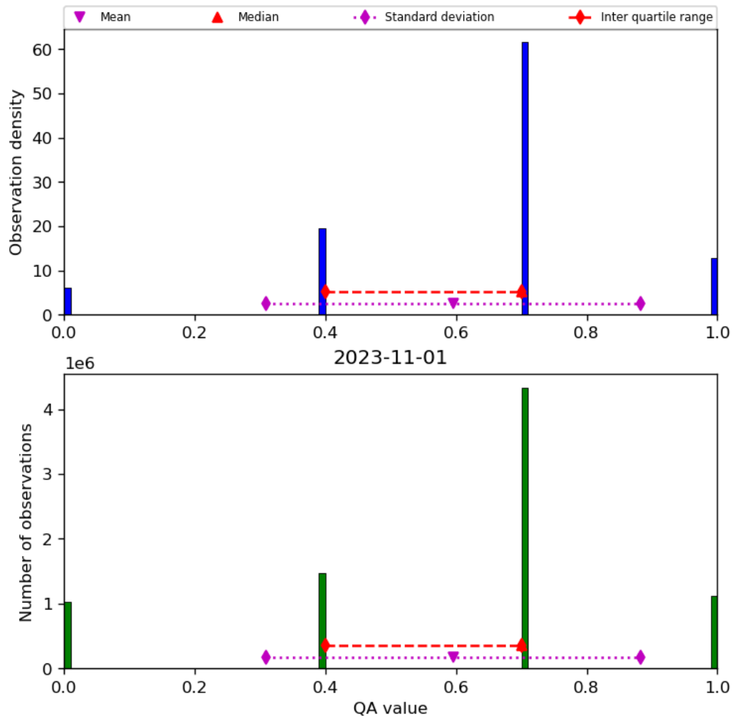
Figure 17: Histogram of “QA value” for 2023-10-31 to 2023-11-02
