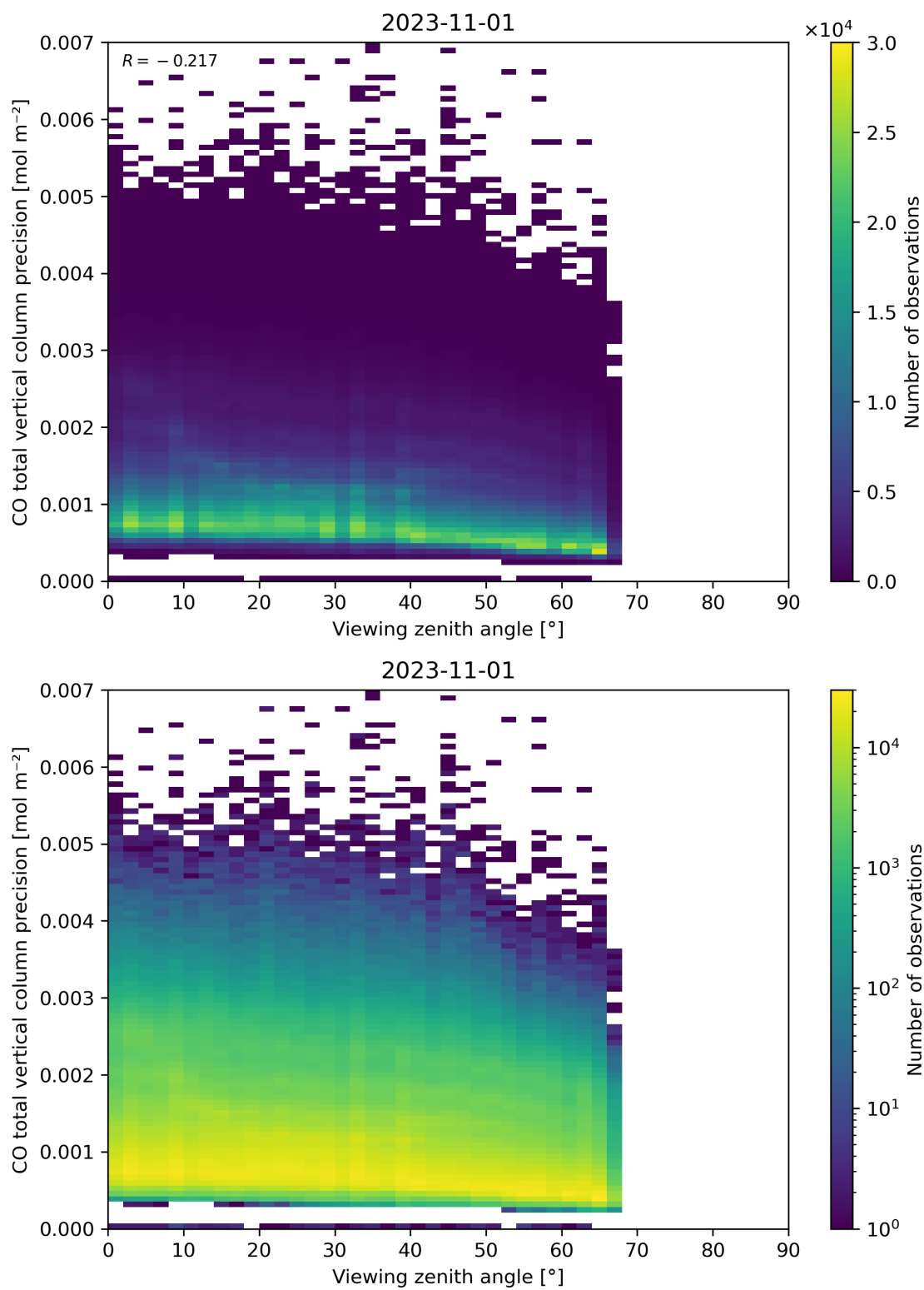
Figure 71: Scatter density plot of “Viewing zenith angle” against “CO total vertical column precision” for 2023-10-31 to 2023-11-02.
