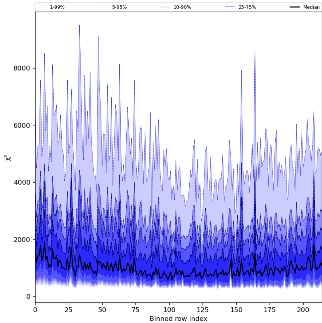
Figure 30: Along track statistics of “ \chi^2 ” for 2023-10-31 to 2023-11-02
