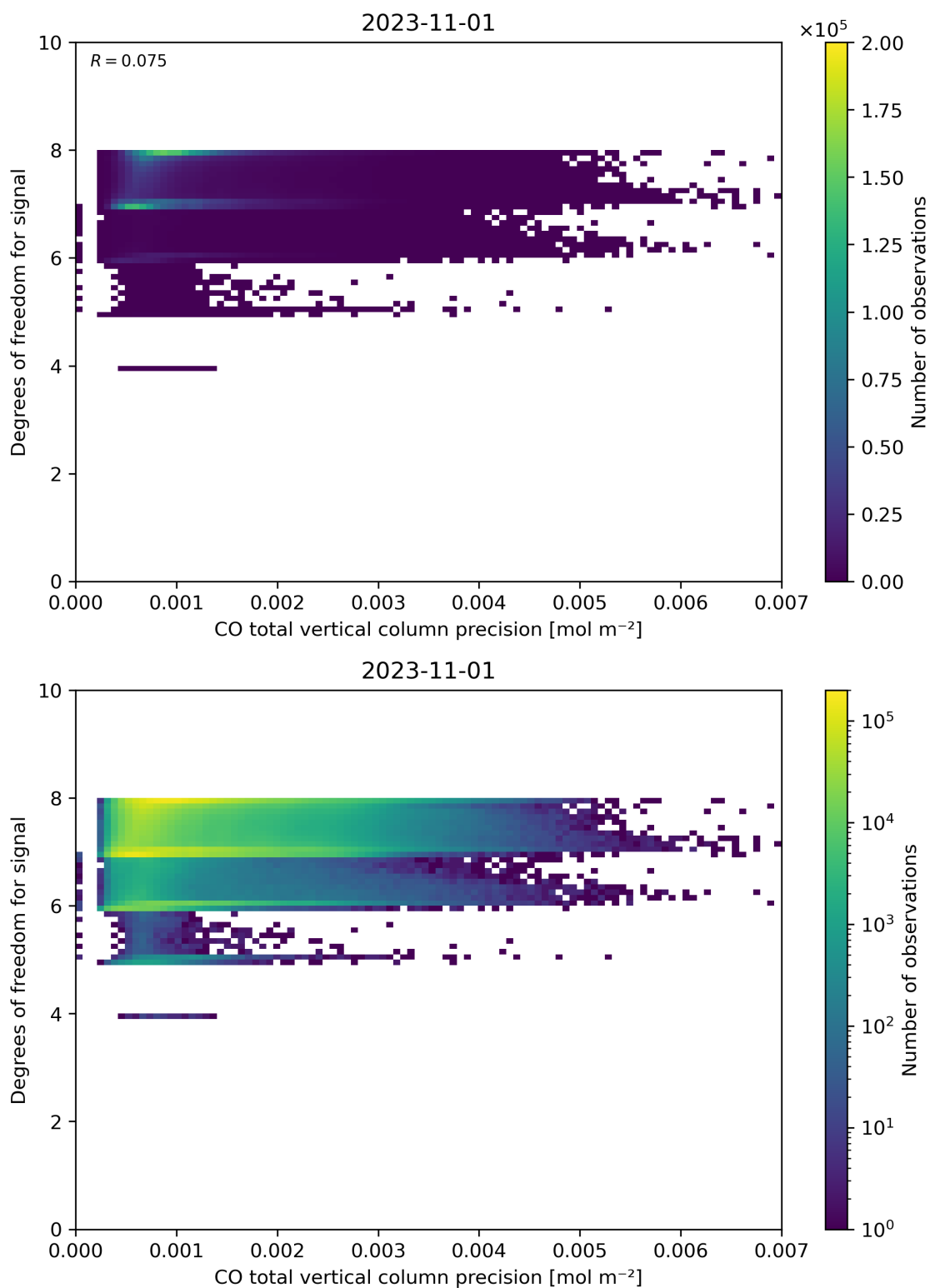
Figure 45: Scatter density plot of “CO total vertical column precision” against “Degrees of freedom for signal” for 2023-10-31 to 2023-11-02.
