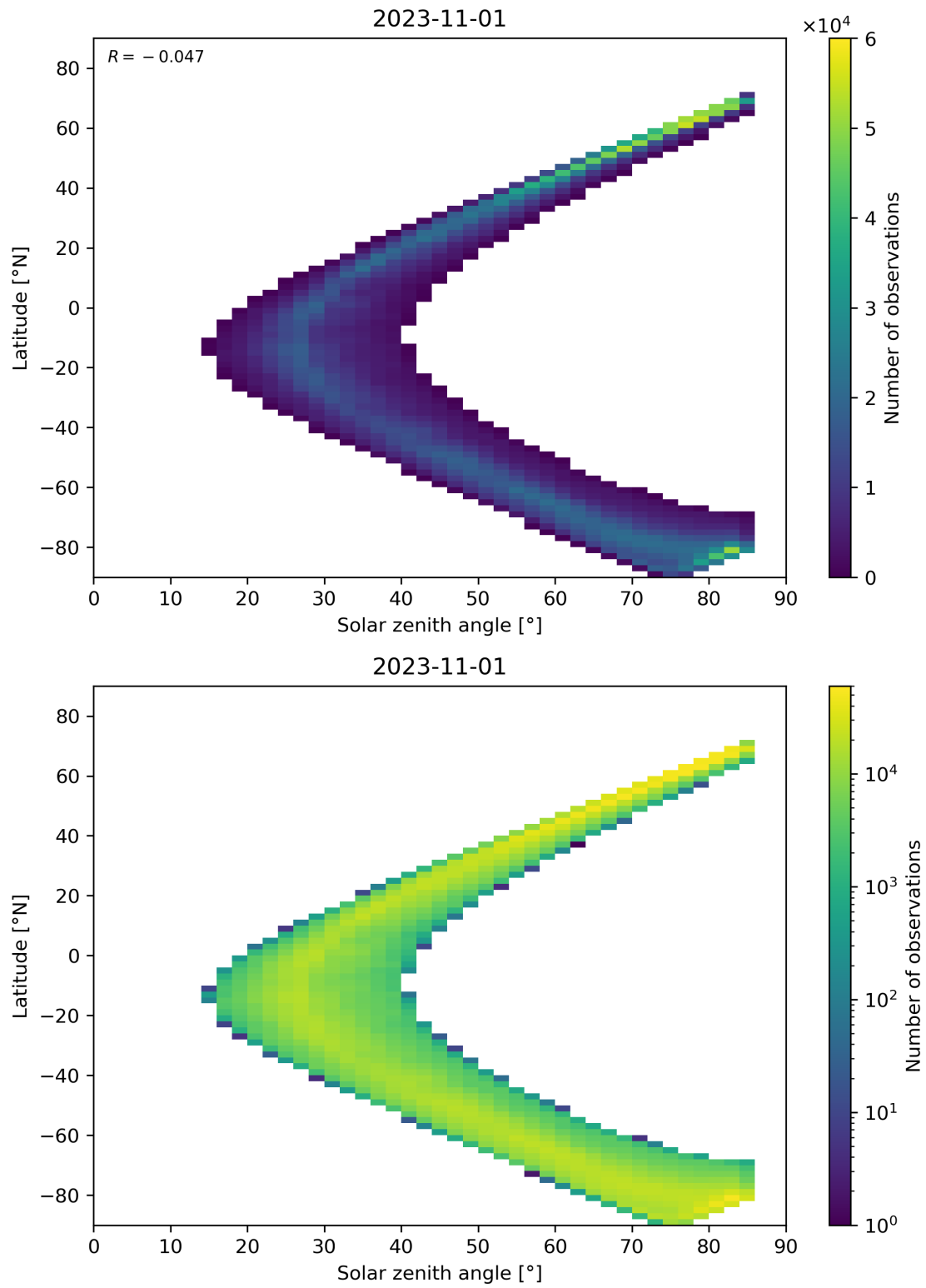
Figure 66: Scatter density plot of “Solar zenith angle” against “Latitude” for 2023-10-31 to 2023-11-02.
