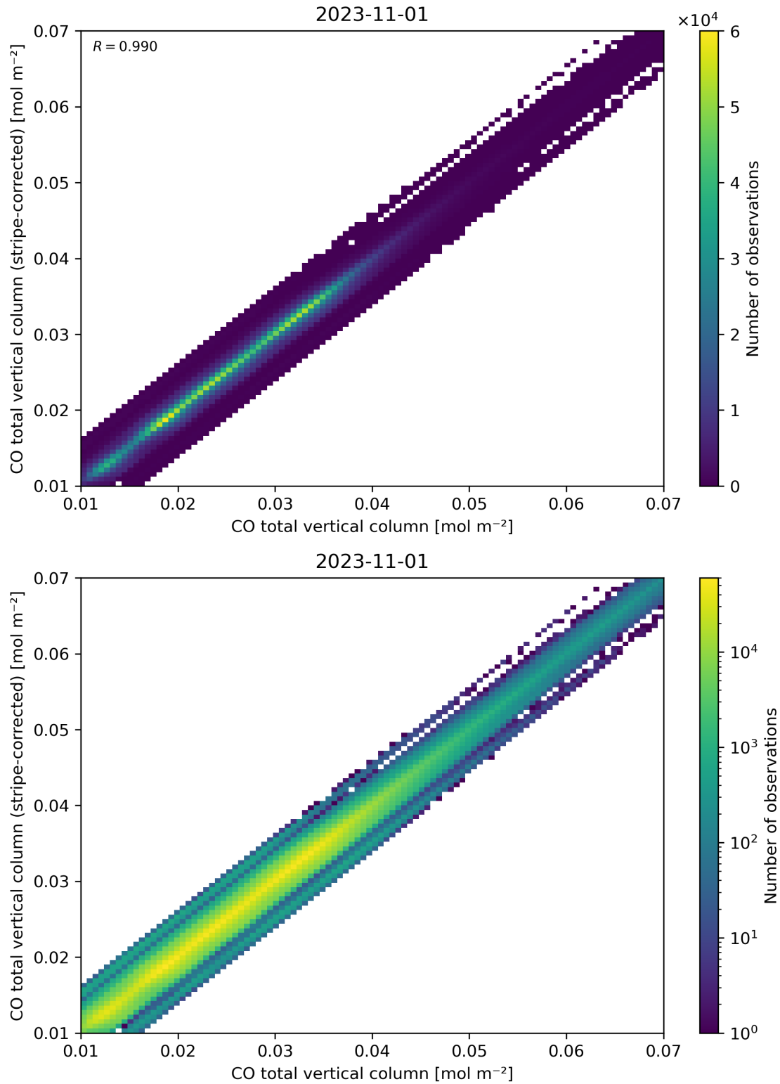
Figure 33: Scatter density plot of “CO total vertical column” against “CO total vertical column (stripe-corrected)” for 2023-10-31 to 2023-11-02.
