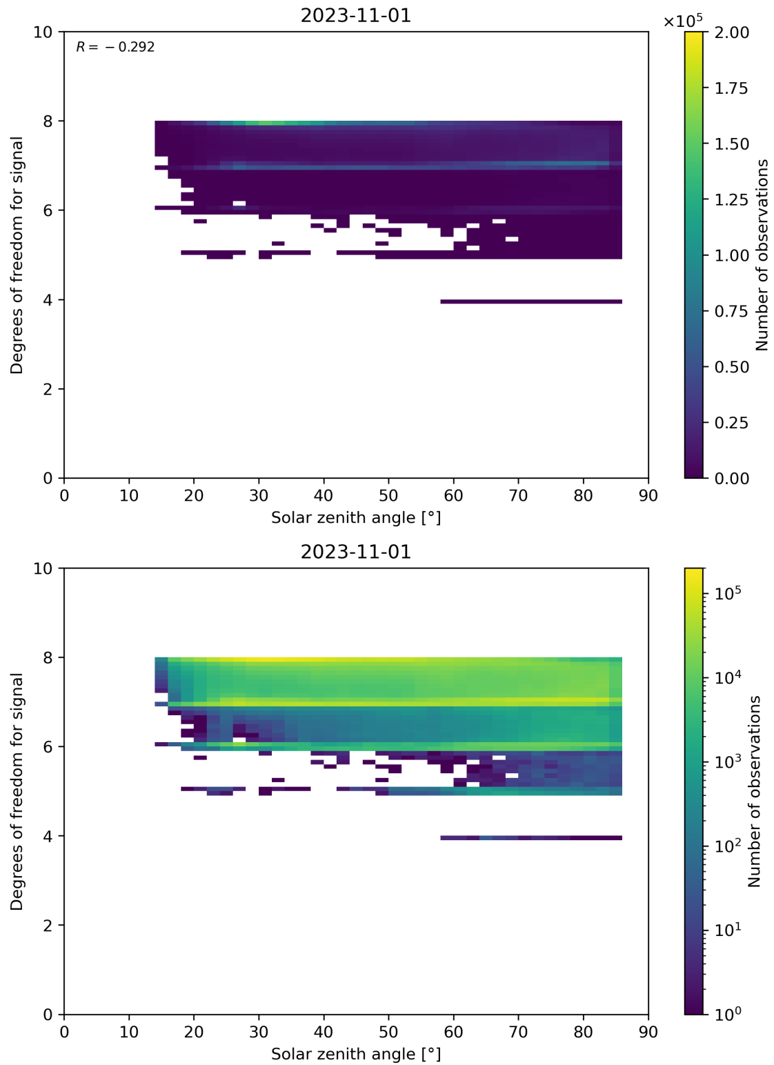
Figure 65: Scatter density plot of “Solar zenith angle” against “Degrees of freedom for signal” for 2023-10-31 to 2023-11-02.
