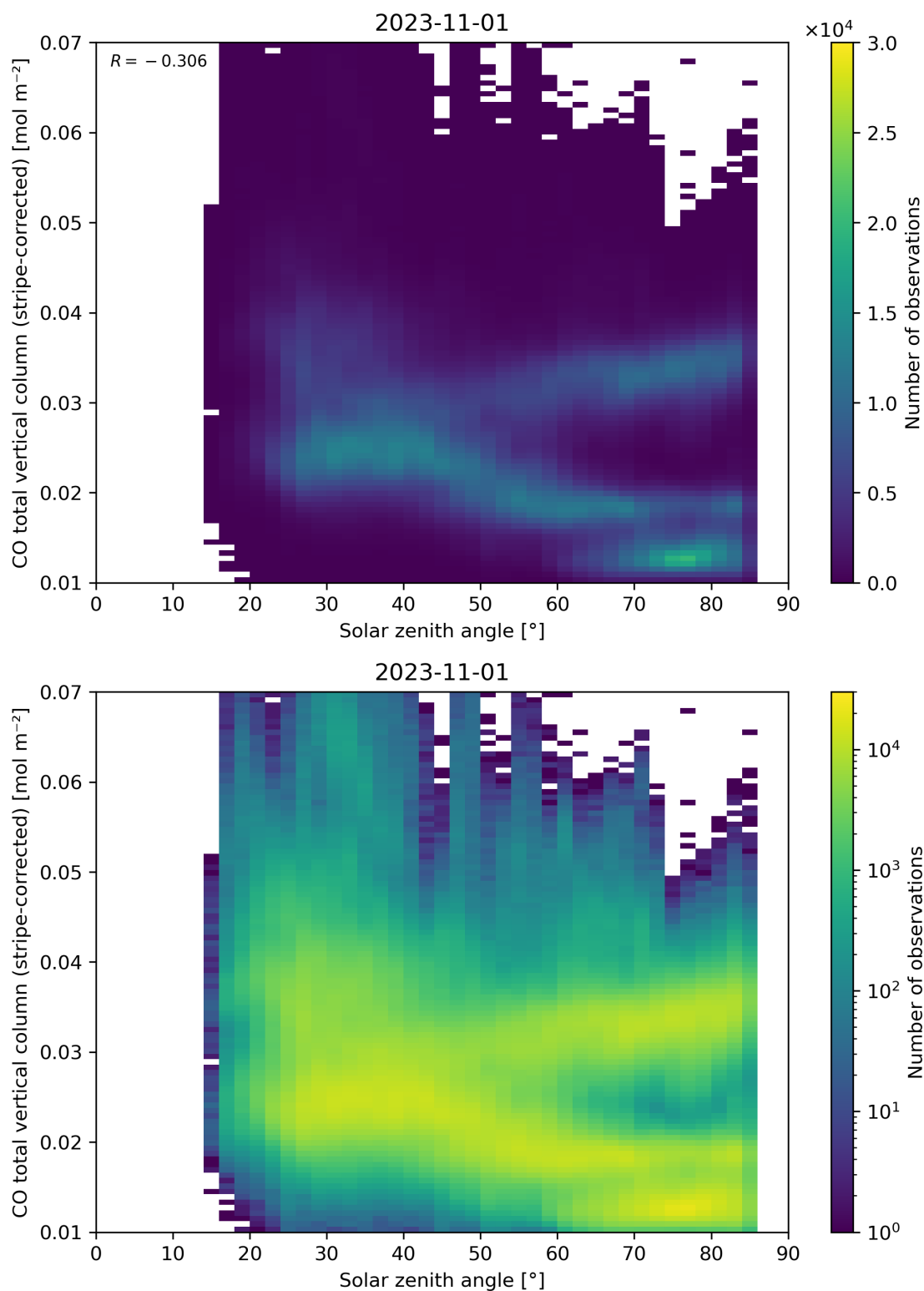
Figure 62: Scatter density plot of “Solar zenith angle” against “CO total vertical column (stripe-corrected)” for 2023-10-31 to 2023-11-02.
