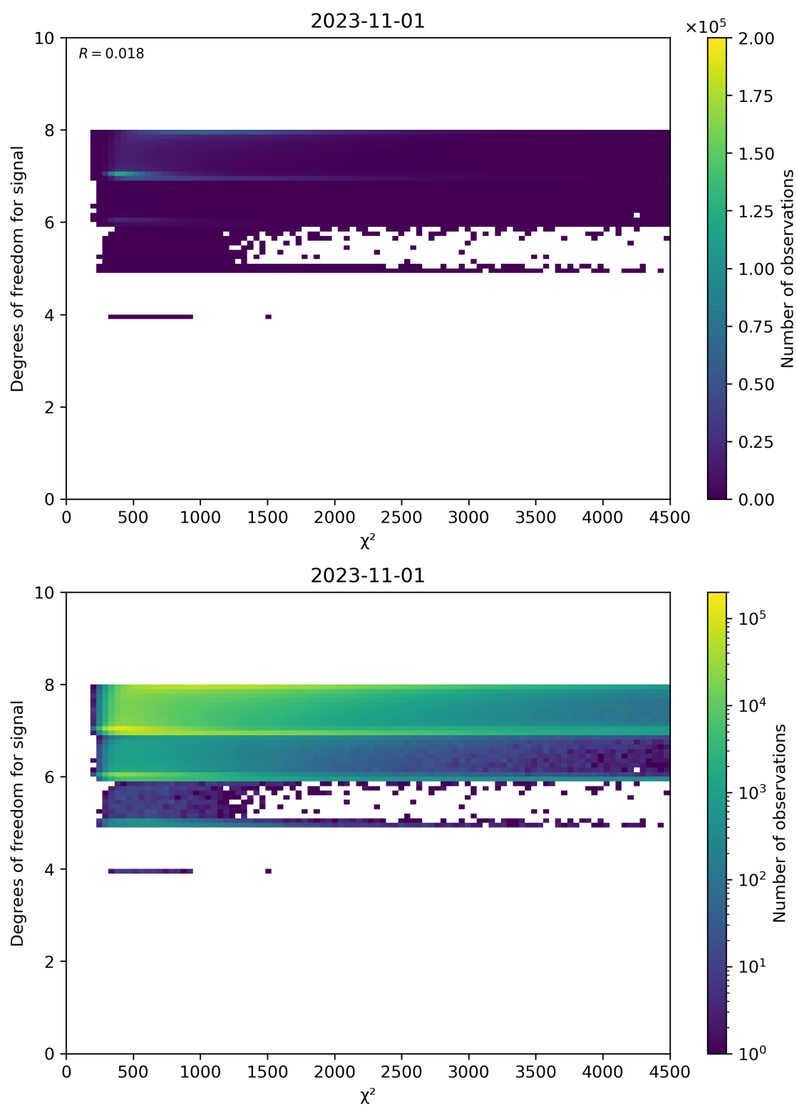
Figure 48: Scatter density plot of “ \chi^2 ” against “Degrees of freedom for signal” for 2023-10-31 to 2023-11-02.
