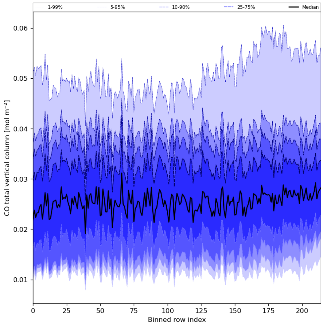
Figure 26: Along track statistics of “CO total vertical column” for 2023-10-31 to 2023-11-02
