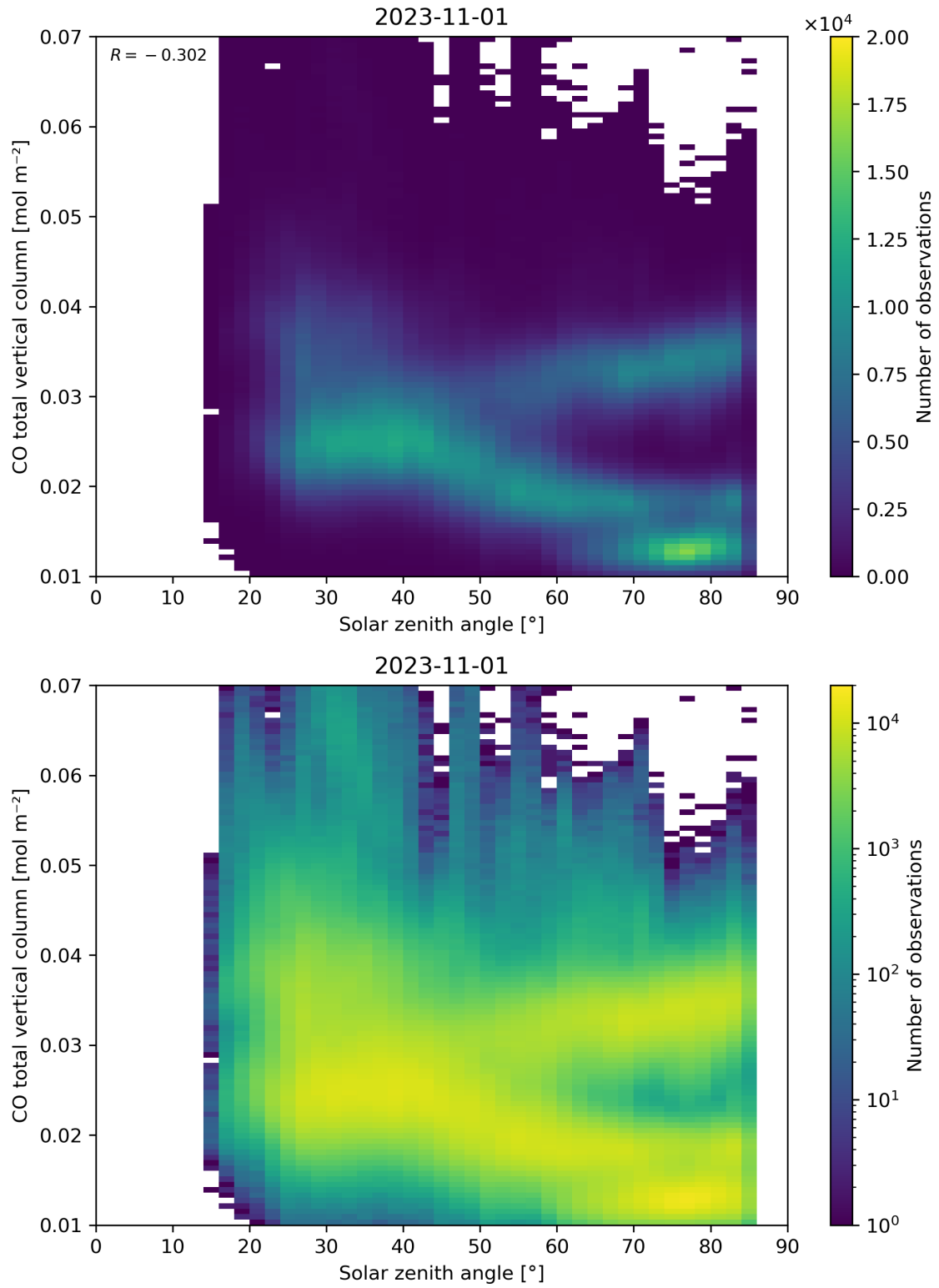
Figure 61: Scatter density plot of “Solar zenith angle” against “CO total vertical column” for 2023-10-31 to 2023-11-02.
