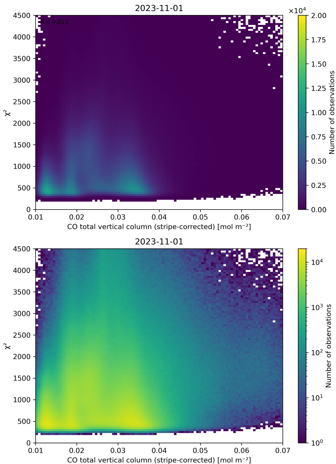
Figure 37: Scatter density plot of “CO total vertical column (stripe-corrected)” against “ \chi^2 ” for 2023-10-31 to 2023-11-02.
