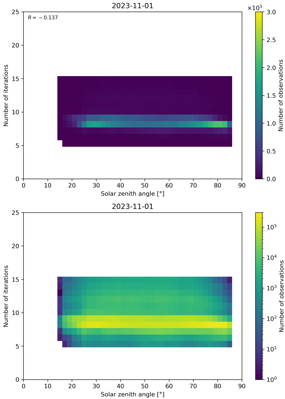
Figure 67: Scatter density plot of “Solar zenith angle” against “Number of iterations” for 2023-10-31 to 2023-11-02.
