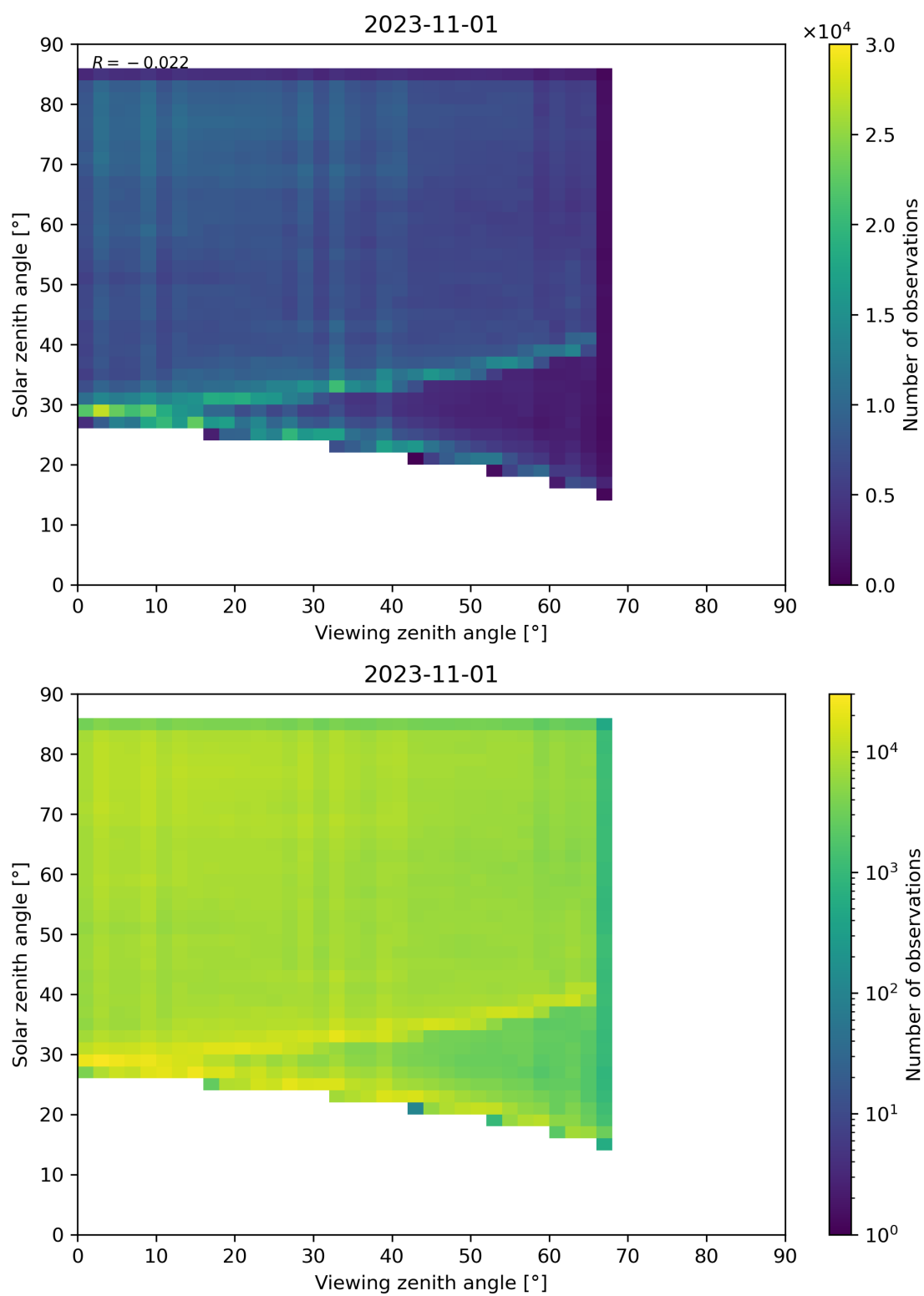
Figure 77: Scatter density plot of “Viewing zenith angle” against “Solar zenith angle” for 2023-10-31 to 2023-11-02.
