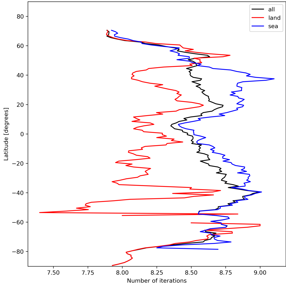
Figure 16: Zonal average of “Number of iterations” for 2023-10-31 to 2023-11-02.
