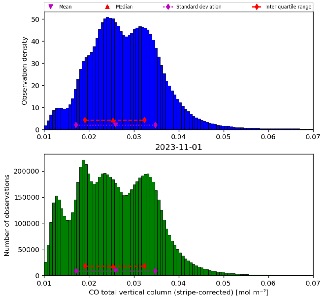
Figure 19: Histogram of “CO total vertical column (stripe-corrected)” for 2023-10-31 to 2023-11-02
