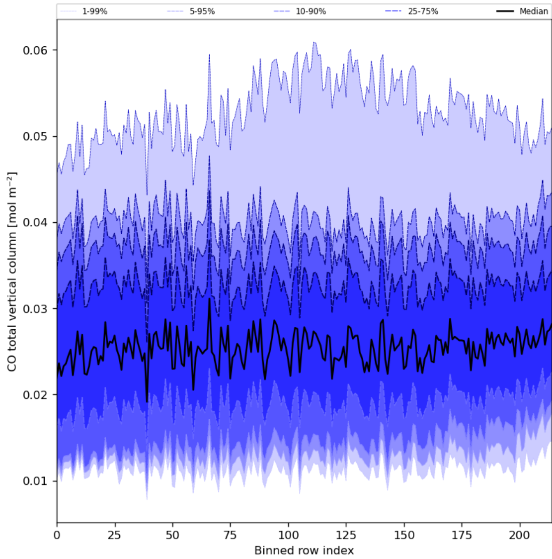
Figure 26: Along track statistics of “CO total vertical column” for 2023-11-02 to 2023-11-03
