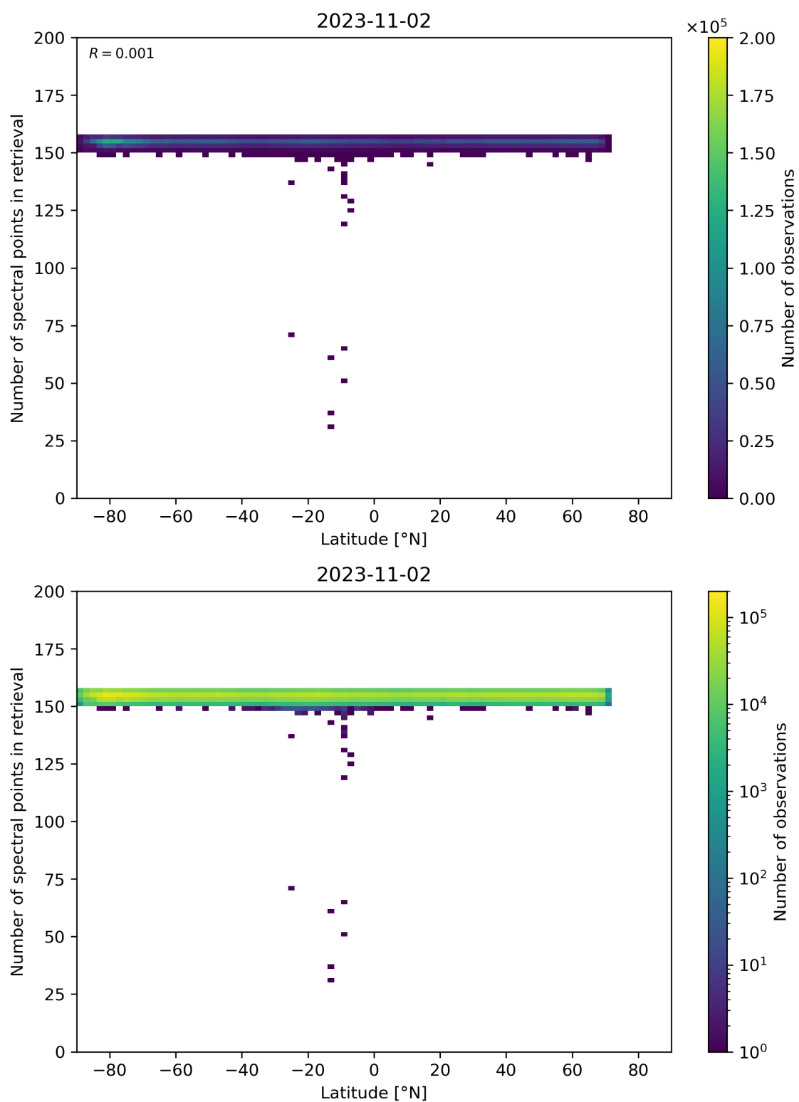
Figure 57: Scatter density plot of “Latitude” against “Number of spectral points in retrieval” for 2023-11-02 to 2023-11-03.
