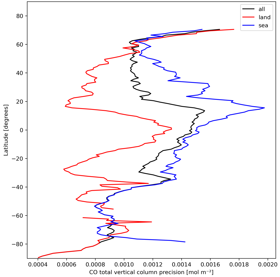
Figure 12: Zonal average of “CO total vertical column precision” for 2023-11-02 to 2023-11-03.
