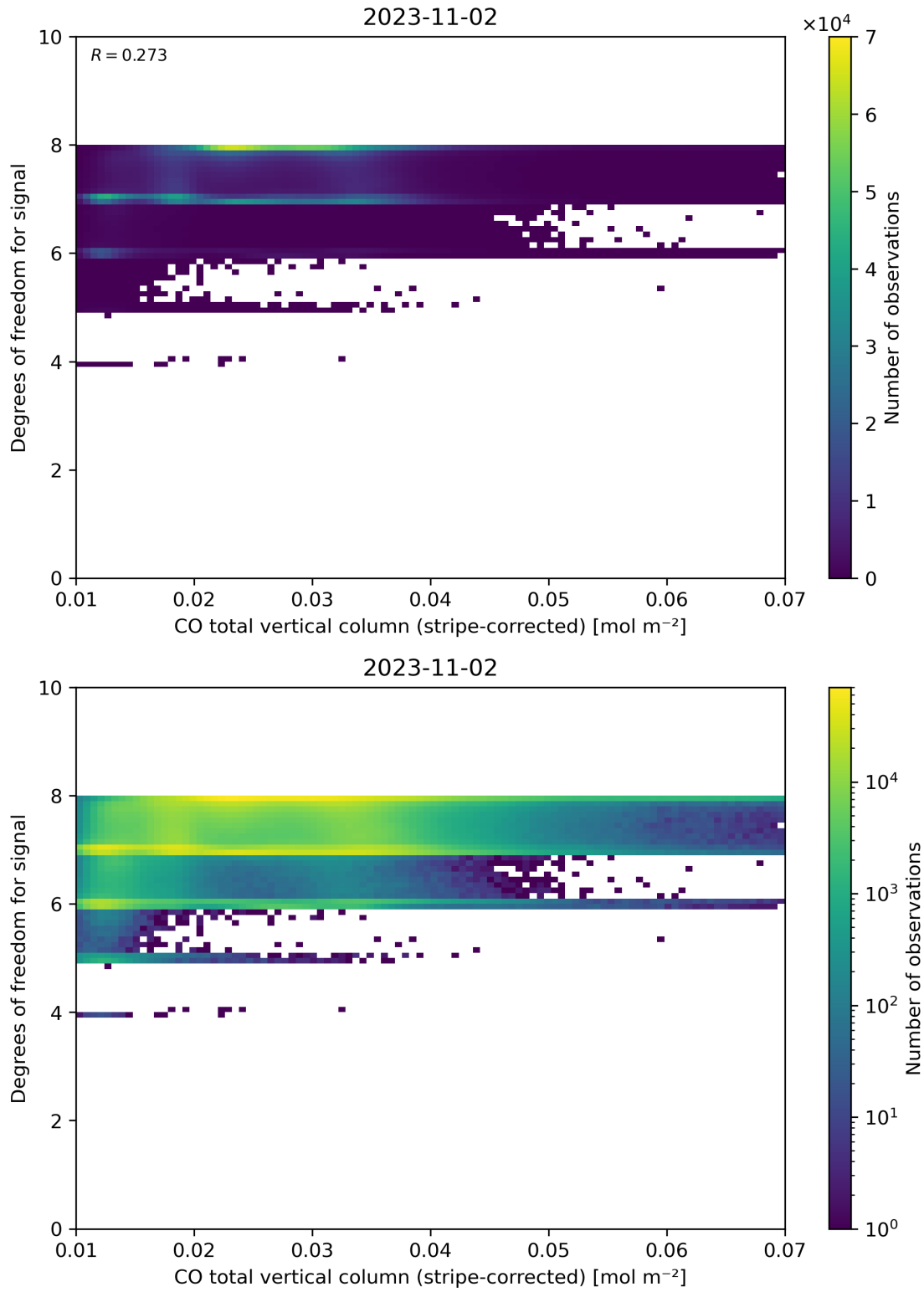
Figure 38: Scatter density plot of “CO total vertical column (stripe-corrected)” against “Degrees of freedom for signal” for 2023-11-02 to 2023-11-03.
