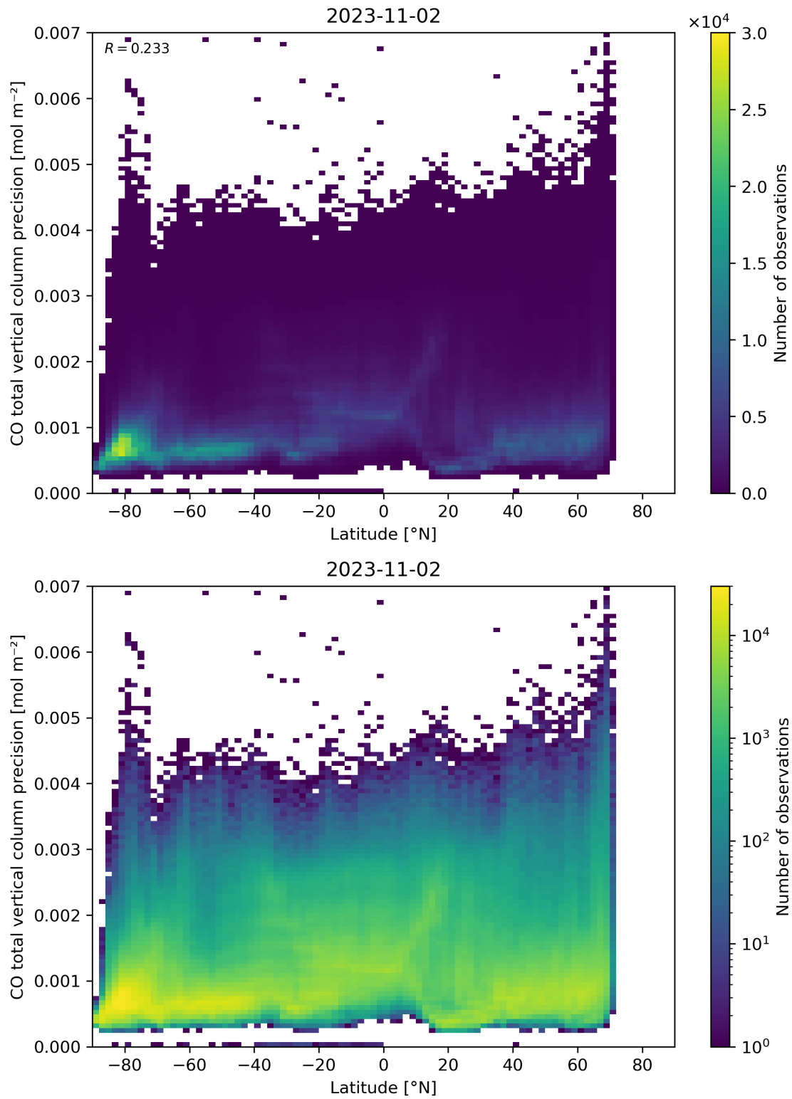
Figure 53: Scatter density plot of “Latitude” against “CO total vertical column precision” for 2023-11-02 to 2023-11-03.
