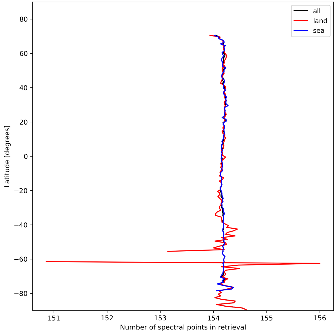
Figure 13: Zonal average of “Number of spectral points in retrieval” for 2023-11-02 to 2023-11-03.
