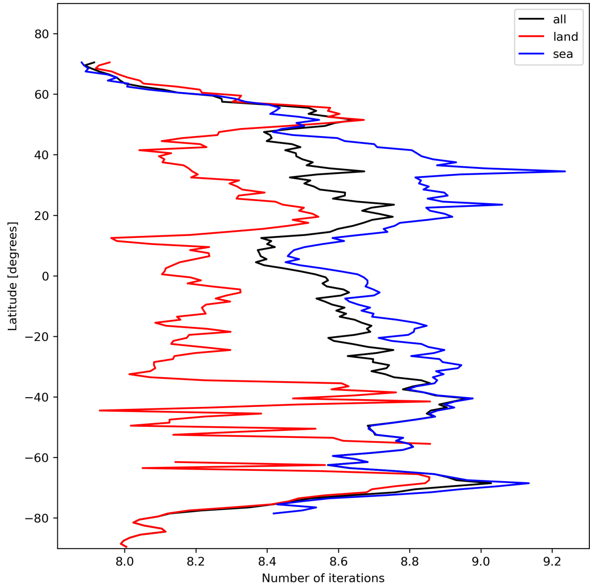
Figure 16: Zonal average of “Number of iterations” for 2023-11-02 to 2023-11-03.
