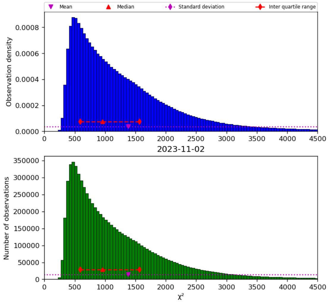
Figure 22: Histogram of “ \chi^2 ” for 2023-11-02 to 2023-11-03
