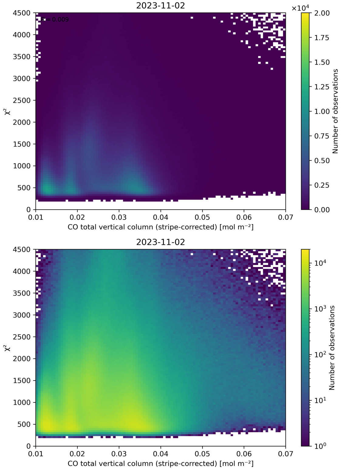
Figure 37: Scatter density plot of “CO total vertical column (stripe-corrected)” against “ \chi^2 ” for 2023-11-02 to 2023-11-03.
