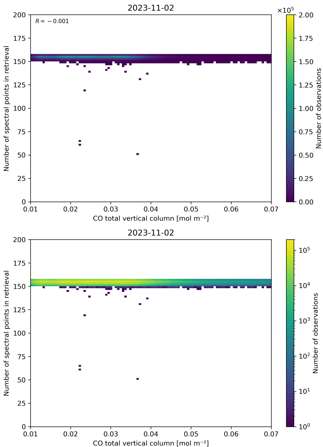
Figure 43: Scatter density plot of “CO total vertical column” against “Number of spectral points in retrieval” for 2023-11-02 to 2023-11-03.
