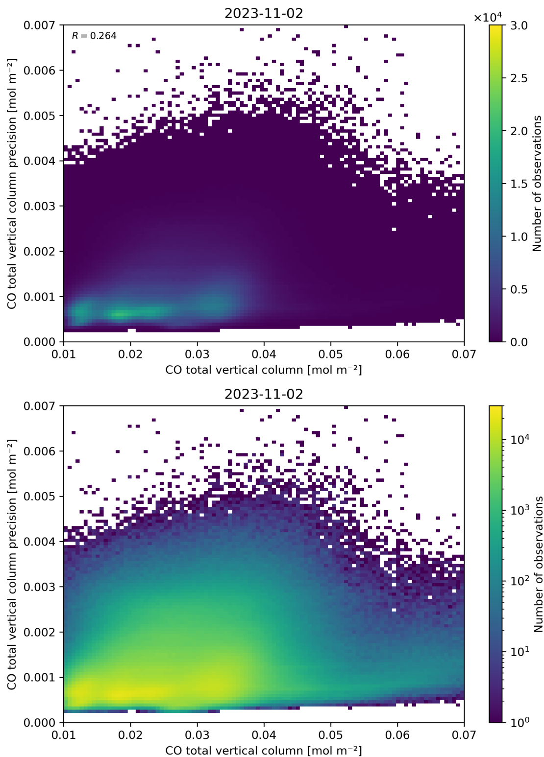
Figure 34: Scatter density plot of “CO total vertical column” against “CO total vertical column precision” for 2023-11-02 to 2023-11-03.
