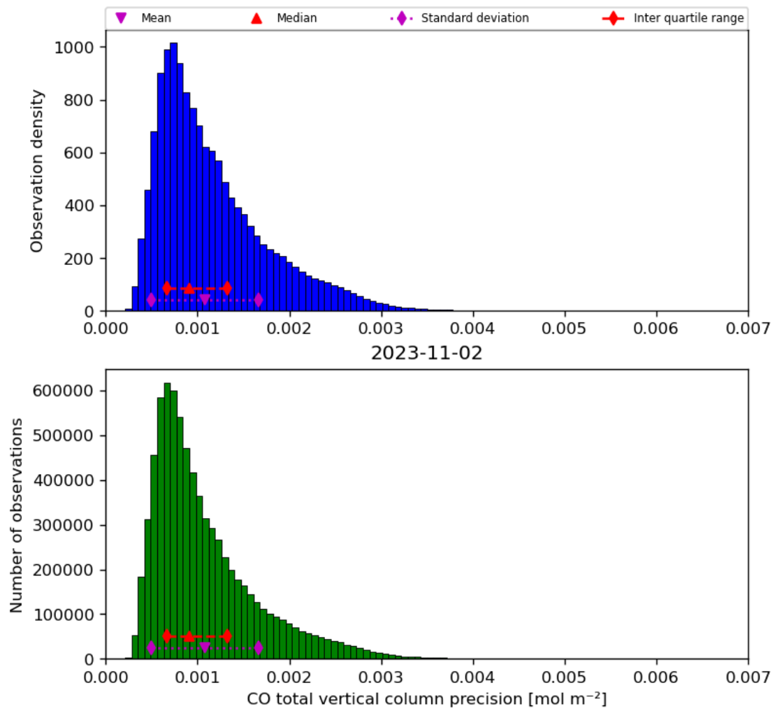
Figure 20: Histogram of “CO total vertical column precision” for 2023-11-02 to 2023-11-03
