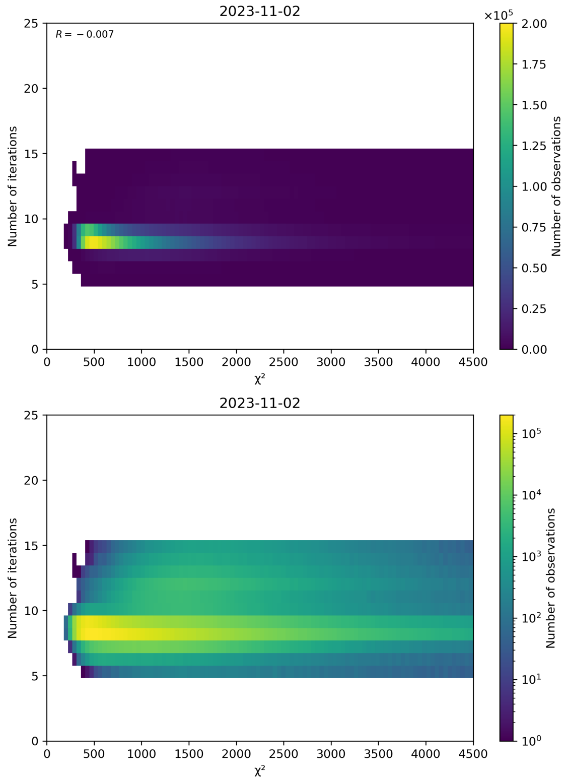
Figure 49: Scatter density plot of “ \chi^2 ” against “Number of iterations” for 2023-11-02 to 2023-11-03.
