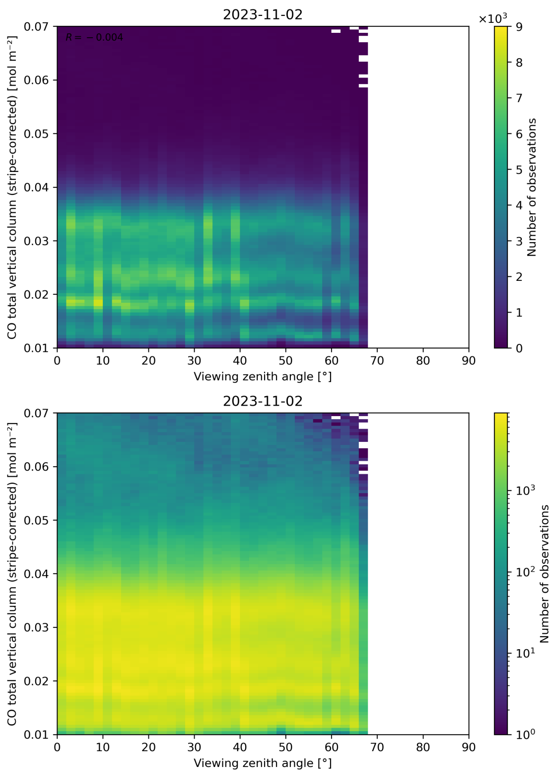
Figure 70: Scatter density plot of “Viewing zenith angle” against “CO total vertical column (stripe-corrected)” for 2023-11-02 to 2023-11-03.
