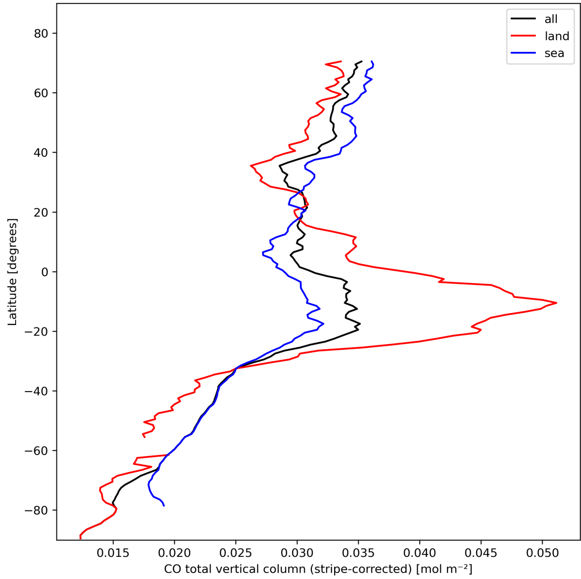
Figure 11: Zonal average of “CO total vertical column (stripe-corrected)” for 2023-11-02 to 2023-11-03.
