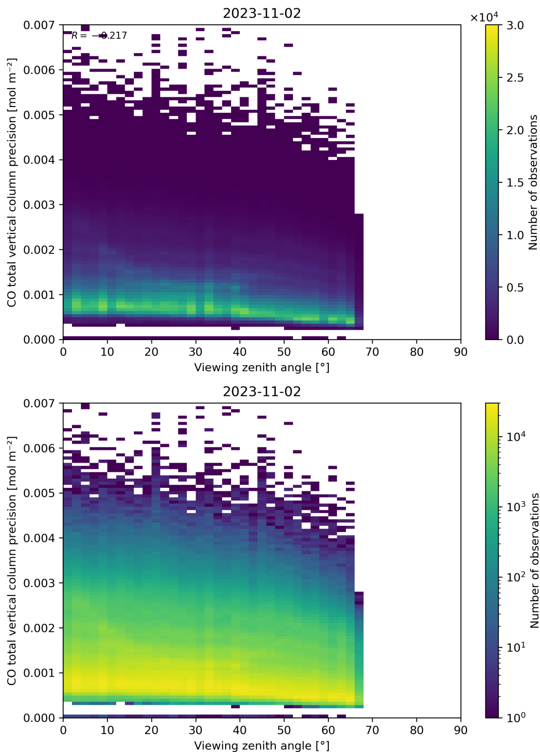
Figure 71: Scatter density plot of “Viewing zenith angle” against “CO total vertical column precision” for 2023-11-02 to 2023-11-03.
