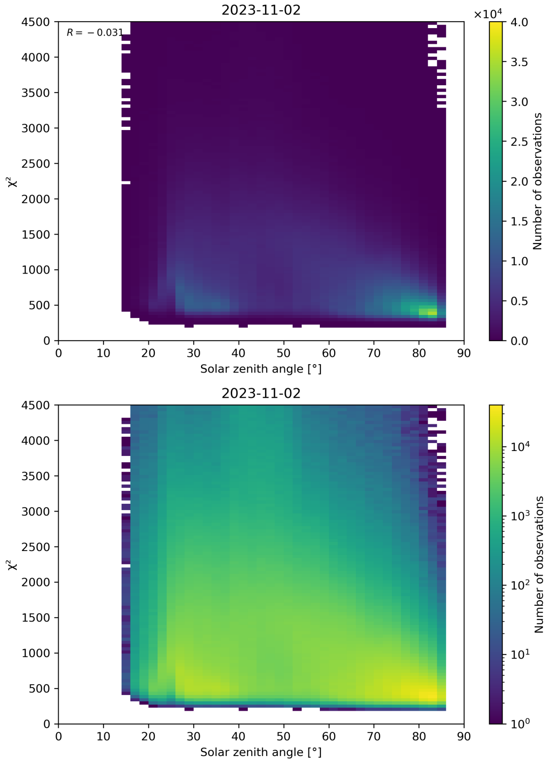
Figure 64: Scatter density plot of “Solar zenith angle” against “ \chi^2 ” for 2023-11-02 to 2023-11-03.
