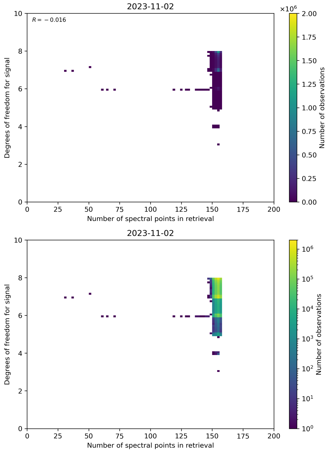
Figure 59: Scatter density plot of “Number of spectral points in retrieval” against “Degrees of freedom for signal” for 2023-11-02 to 2023-11-03.
