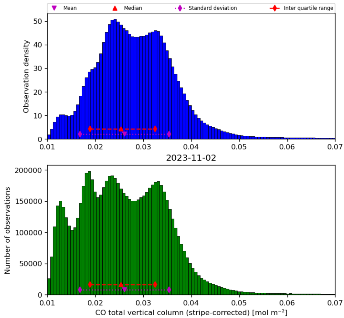
Figure 19: Histogram of “CO total vertical column (stripe-corrected)” for 2023-11-02 to 2023-11-03
