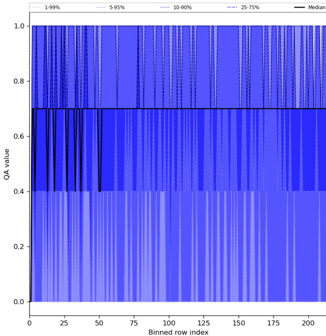
Figure 25: Along track statistics of “QA value” for 2023-11-02 to 2023-11-03
