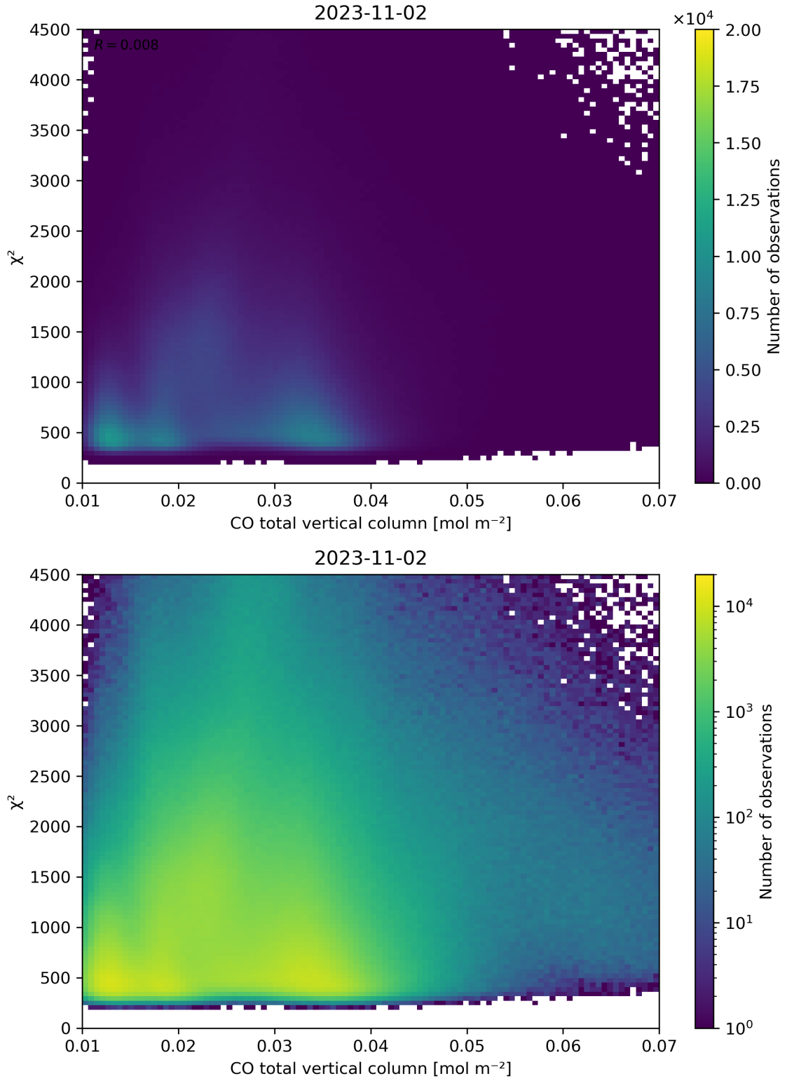
Figure 35: Scatter density plot of “CO total vertical column” against “ \chi^2 ” for 2023-11-02 to 2023-11-03.
