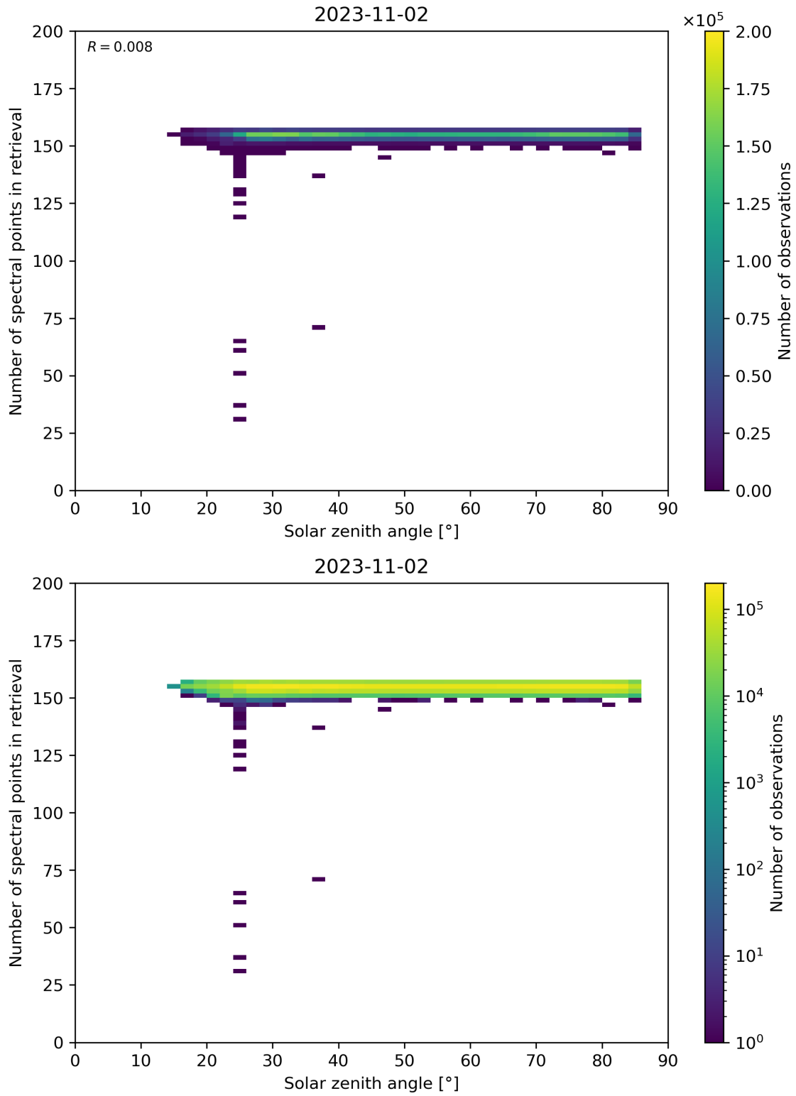
Figure 68: Scatter density plot of “Solar zenith angle” against “Number of spectral points in retrieval” for 2023-11-02 to 2023-11-03.
