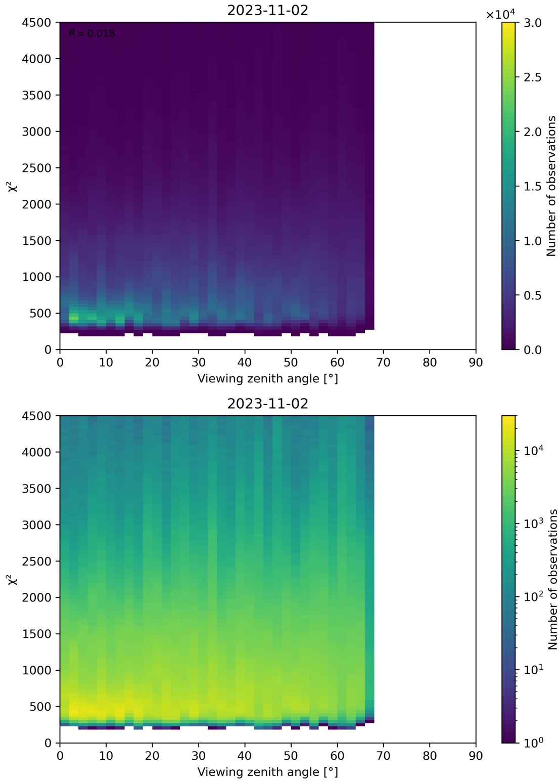
Figure 72: Scatter density plot of “Viewing zenith angle” against “ \chi^2 ” for 2023-11-02 to 2023-11-03.
