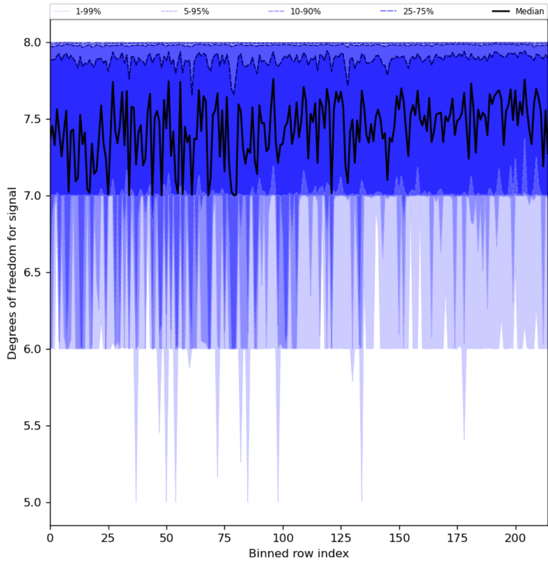
Figure 31: Along track statistics of “Degrees of freedom for signal” for 2023-11-02 to 2023-11-03
