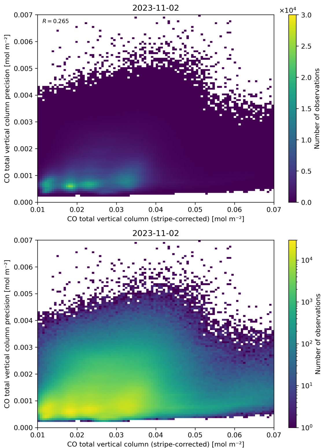
Figure 36: Scatter density plot of “CO total vertical column (stripe-corrected)” against “CO total vertical column precision” for 2023-11-02 to 2023-11-03.
