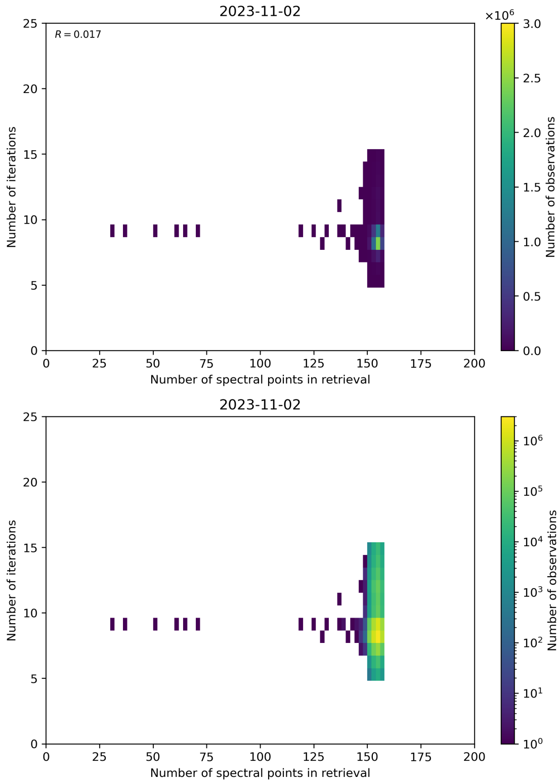
Figure 60: Scatter density plot of “Number of spectral points in retrieval” against “Number of iterations” for 2023-11-02 to 2023-11-03.
