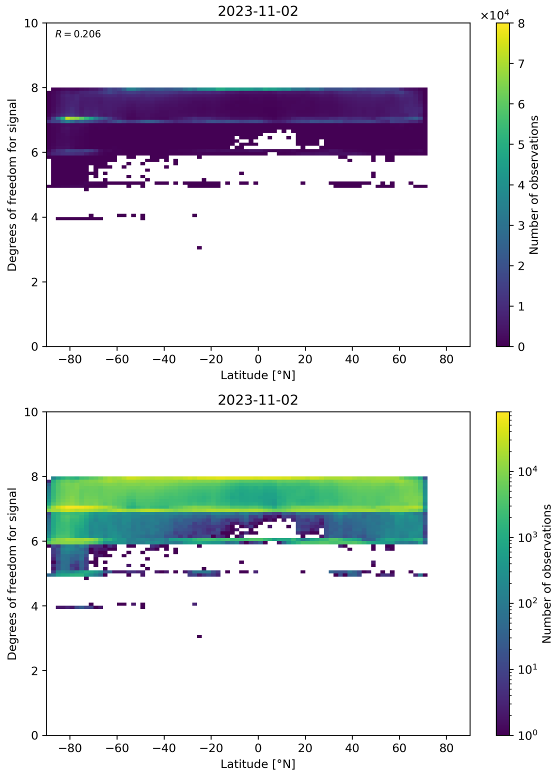
Figure 55: Scatter density plot of “Latitude” against “Degrees of freedom for signal” for 2023-11-02 to 2023-11-03.
