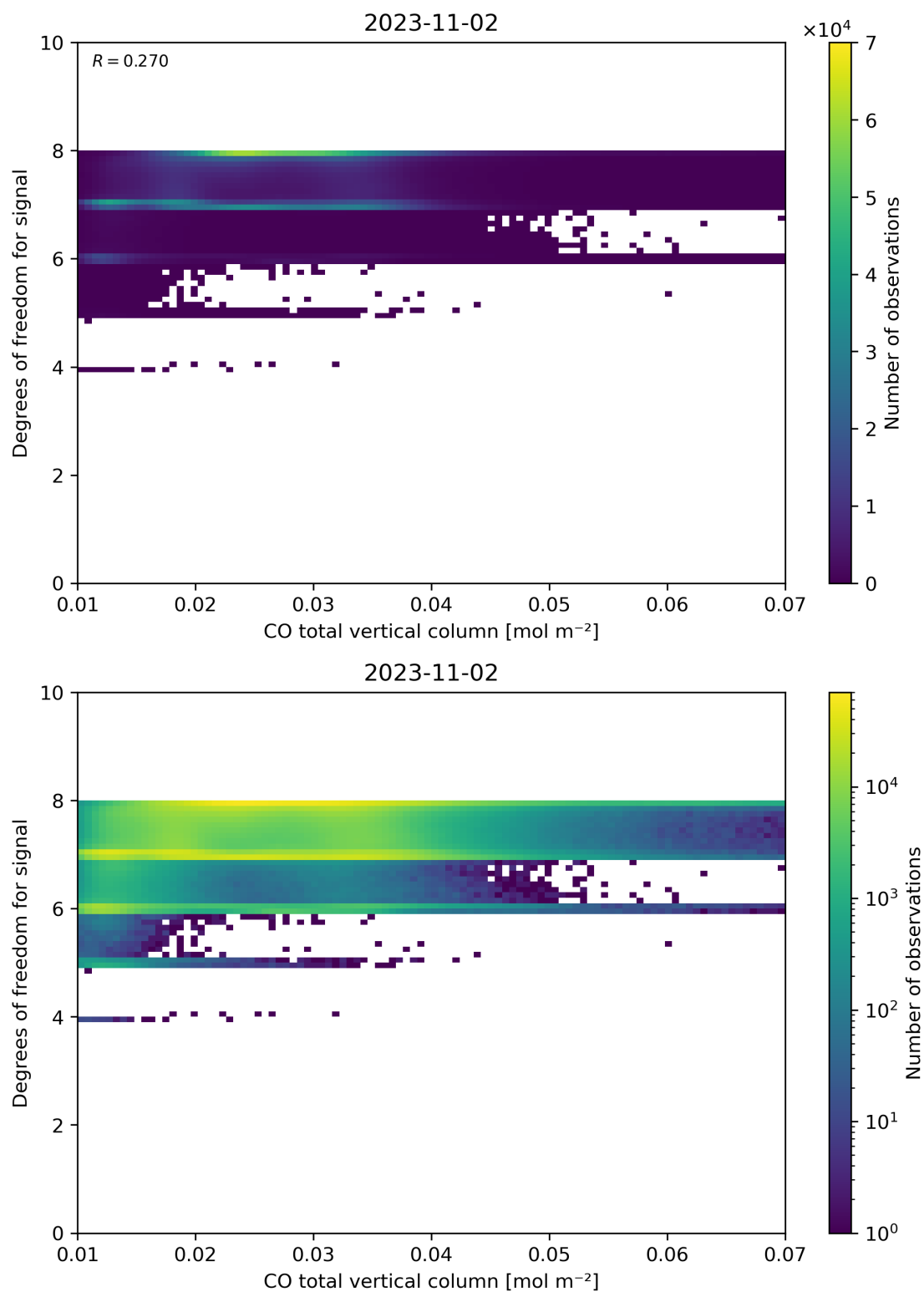
Figure 41: Scatter density plot of “CO total vertical column” against “Degrees of freedom for signal” for 2023-11-02 to 2023-11-03.
