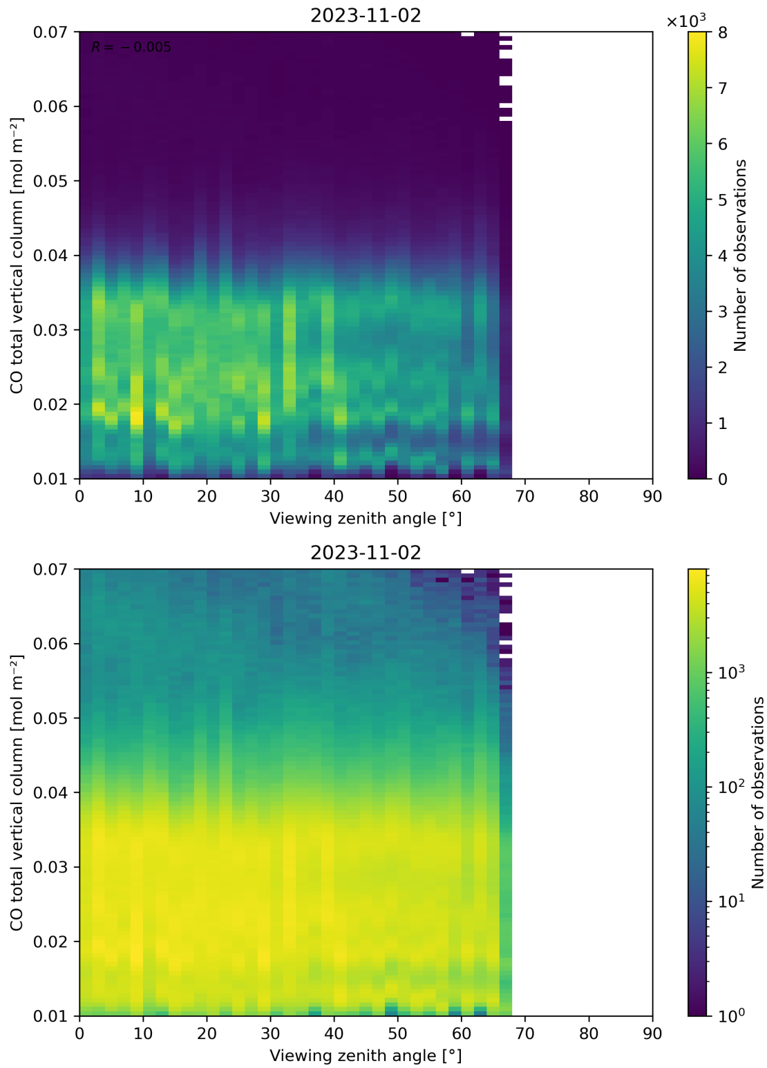
Figure 69: Scatter density plot of “Viewing zenith angle” against “CO total vertical column” for 2023-11-02 to 2023-11-03.
