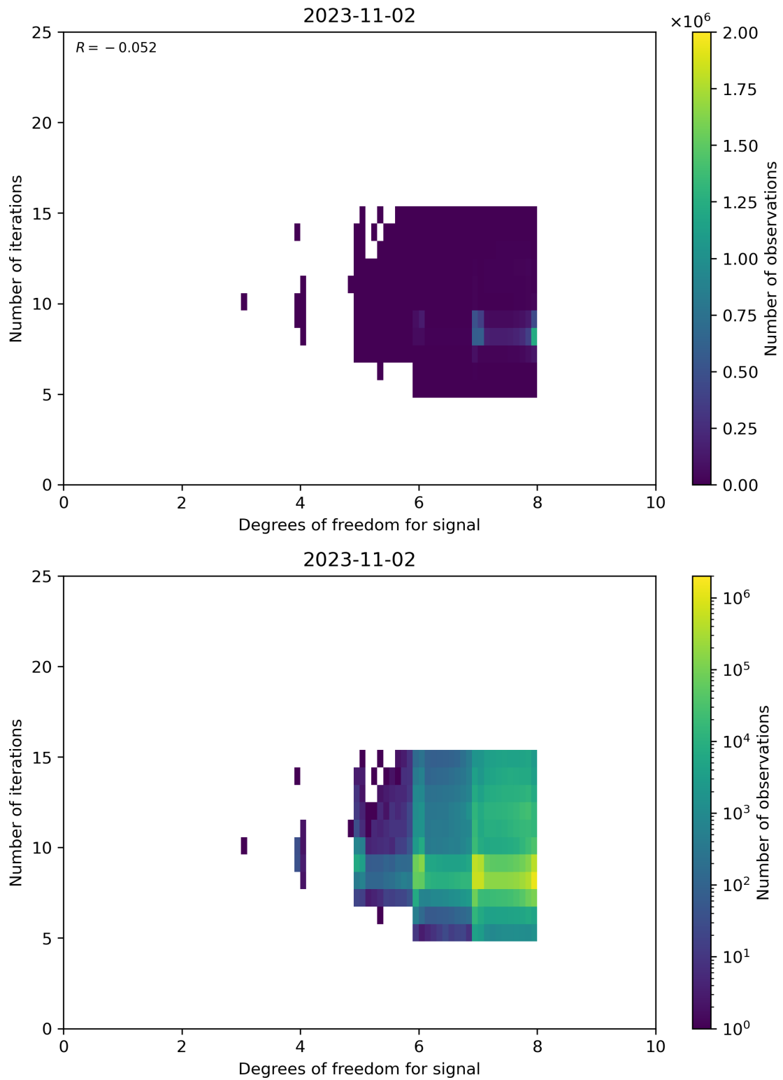
Figure 50: Scatter density plot of “Degrees of freedom for signal” against “Number of iterations” for 2023-11-02 to 2023-11-03.
