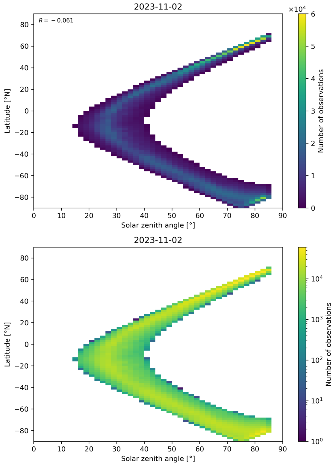
Figure 66: Scatter density plot of “Solar zenith angle” against “Latitude” for 2023-11-02 to 2023-11-03.
