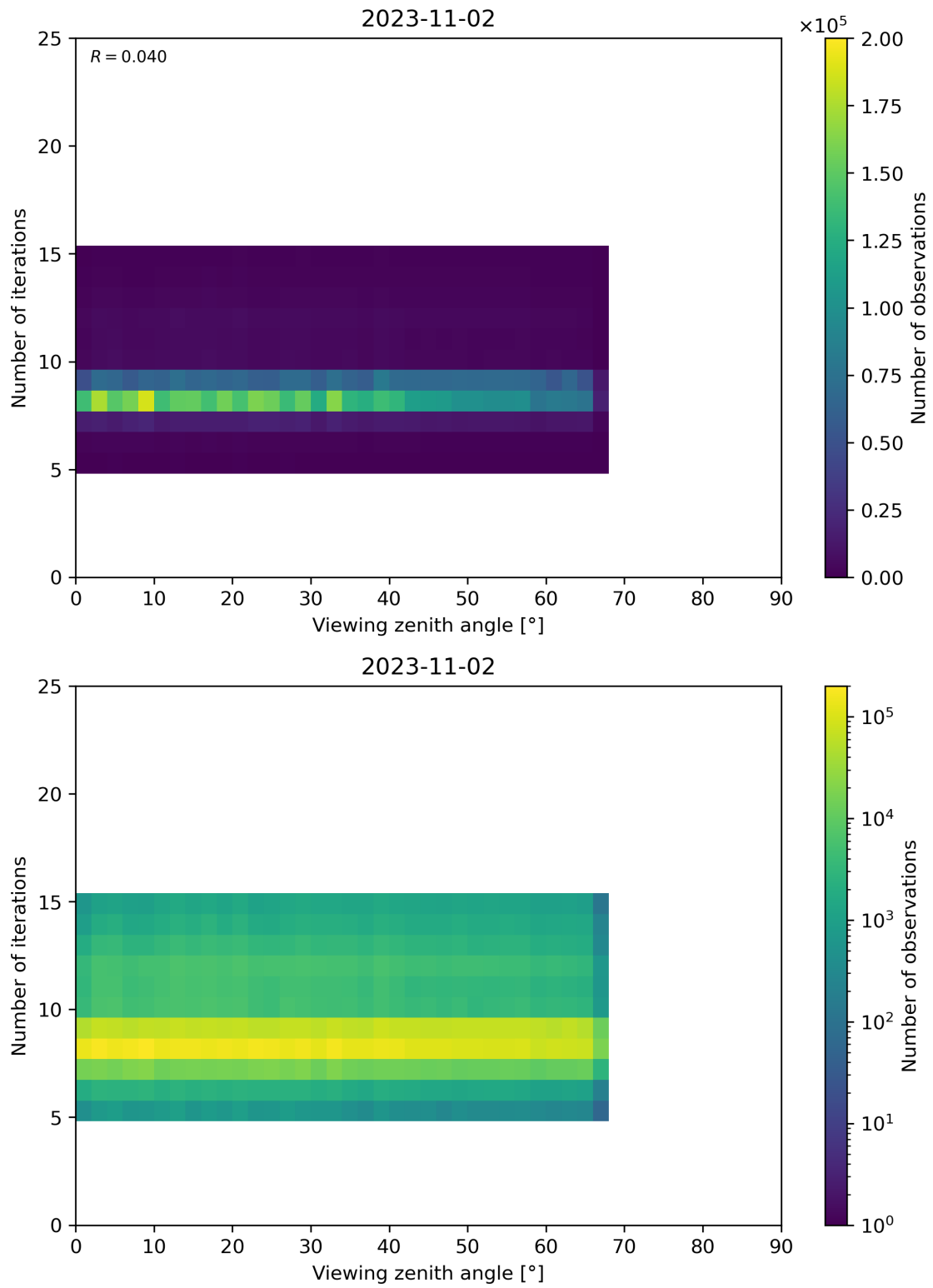
Figure 75: Scatter density plot of “Viewing zenith angle” against “Number of iterations” for 2023-11-02 to 2023-11-03.
