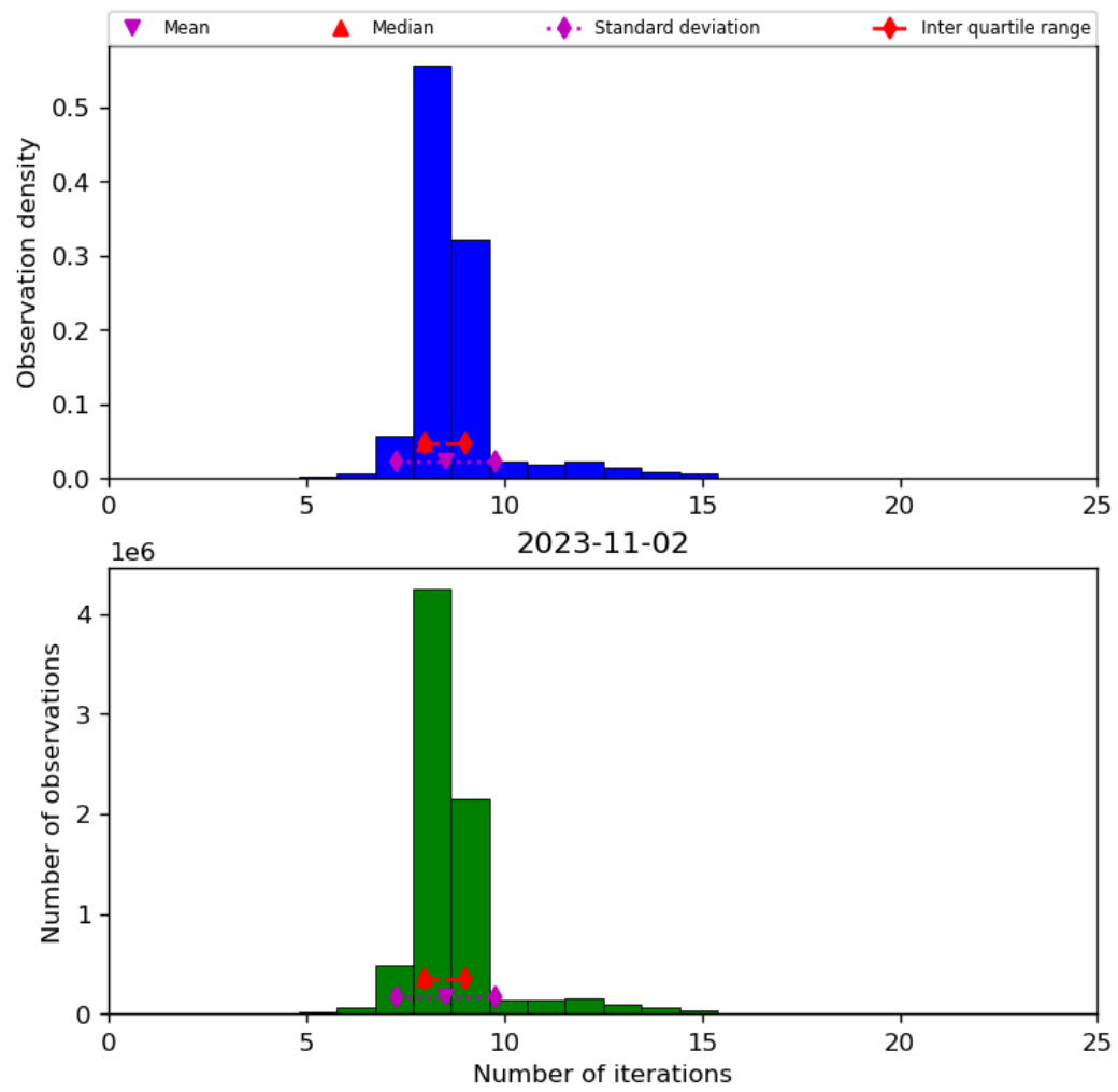
Figure 24: Histogram of “Number of iterations” for 2023-11-02 to 2023-11-03
