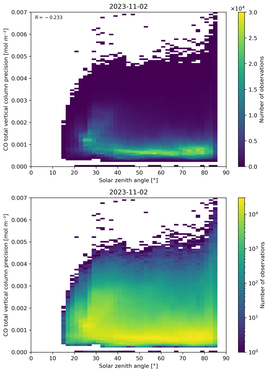
Figure 63: Scatter density plot of “Solar zenith angle” against “CO total vertical column precision” for 2023-11-02 to 2023-11-03.
