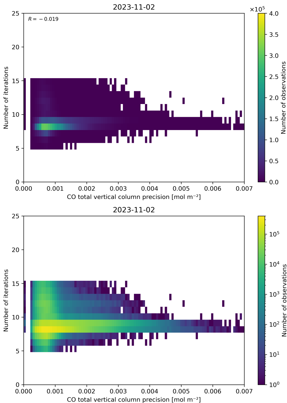
Figure 46: Scatter density plot of “CO total vertical column precision” against “Number of iterations” for 2023-11-02 to 2023-11-03.
