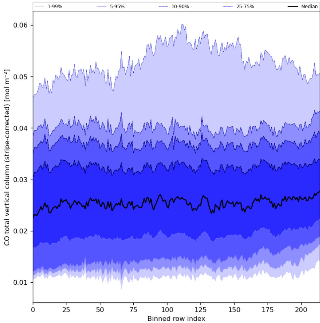
Figure 27: Along track statistics of “CO total vertical column (stripe-corrected)” for 2023-11-02 to 2023-11-03
