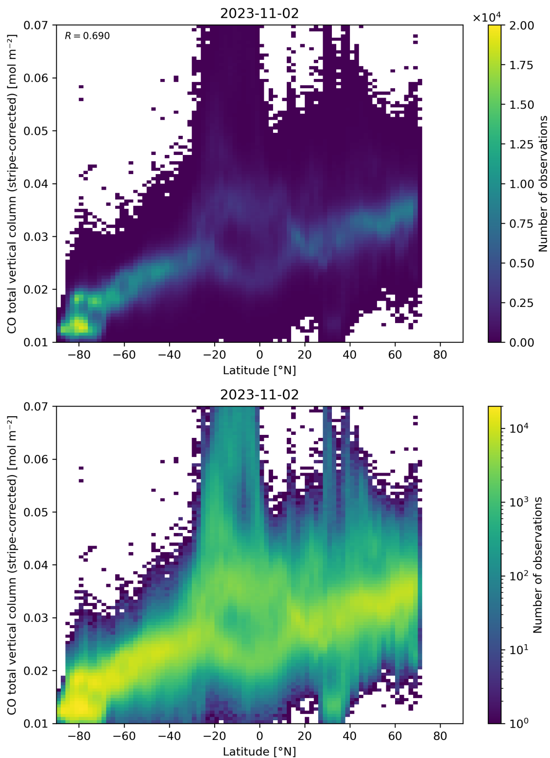
Figure 52: Scatter density plot of “Latitude” against “CO total vertical column (stripe-corrected)” for 2023-11-02 to 2023-11-03.
