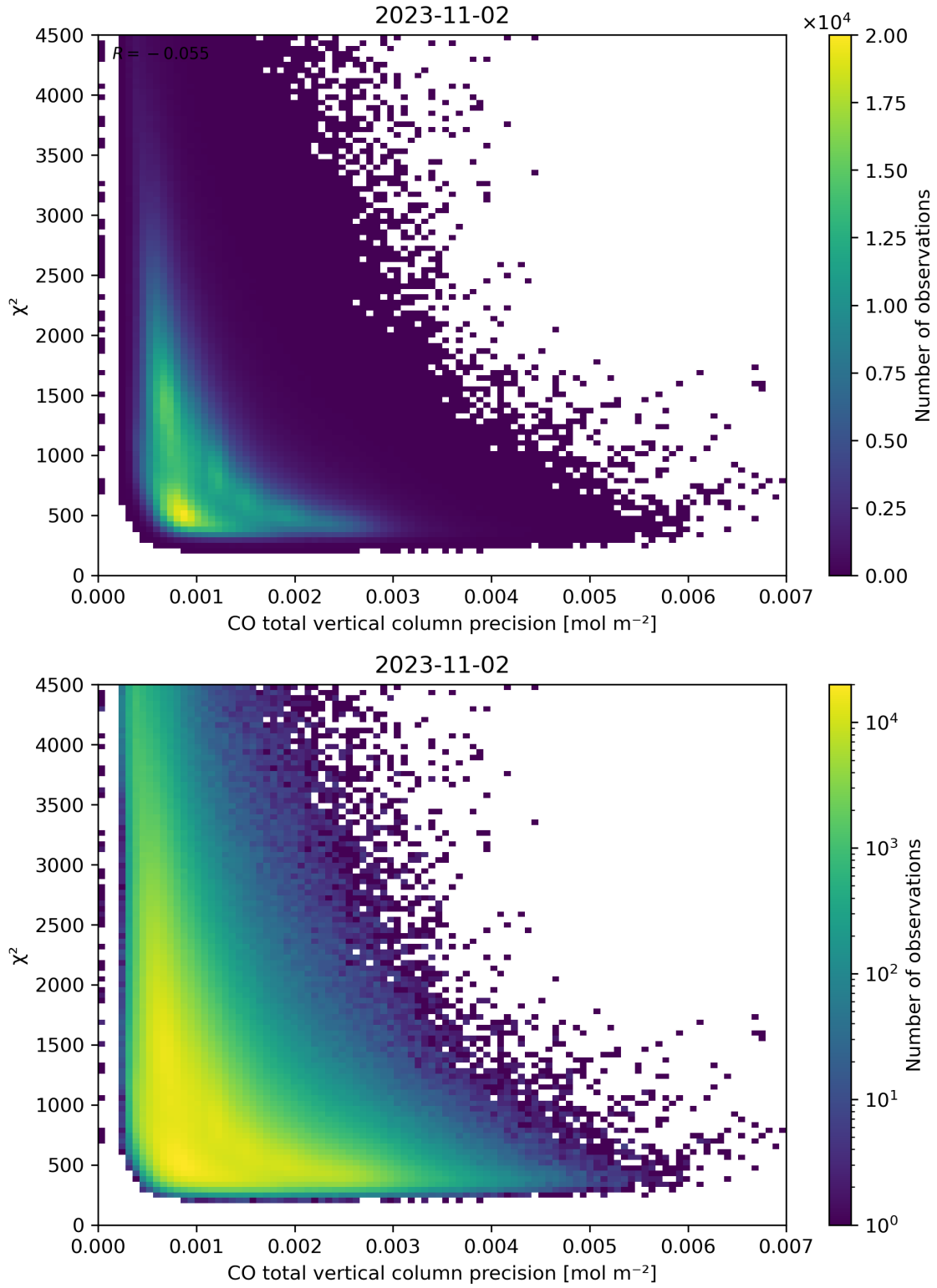
Figure 44: Scatter density plot of “CO total vertical column precision” against “ \chi^2 ” for 2023-11-02 to 2023-11-03.
