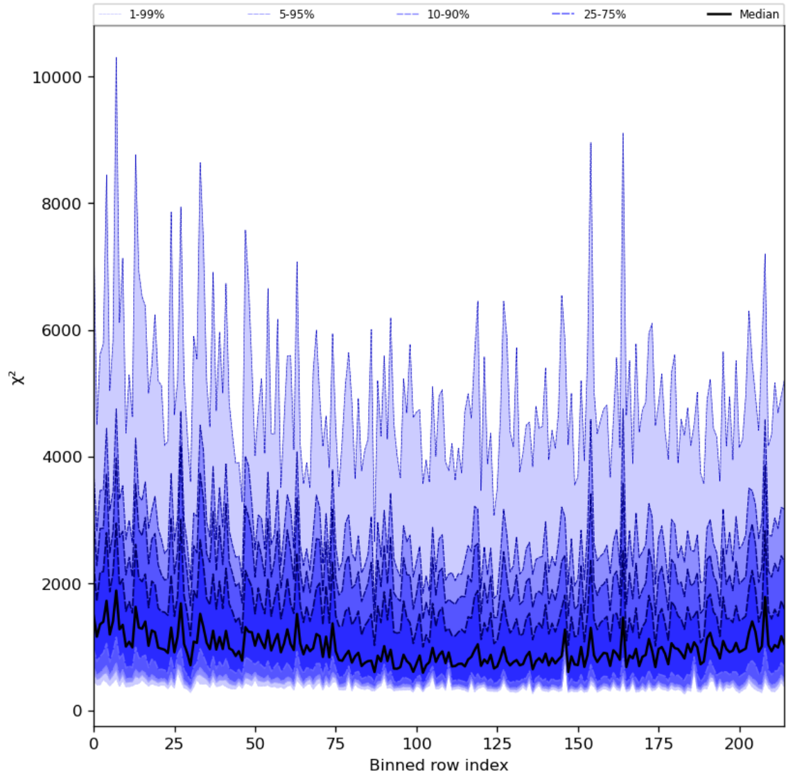
Figure 30: Along track statistics of “ \chi^2 ” for 2023-11-02 to 2023-11-03
