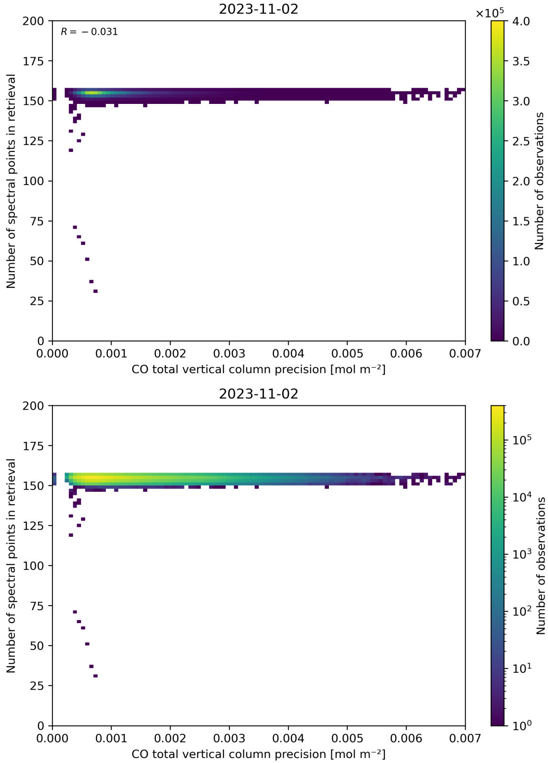
Figure 47: Scatter density plot of “CO total vertical column precision” against “Number of spectral points in retrieval” for 2023-11-02 to 2023-11-03.
