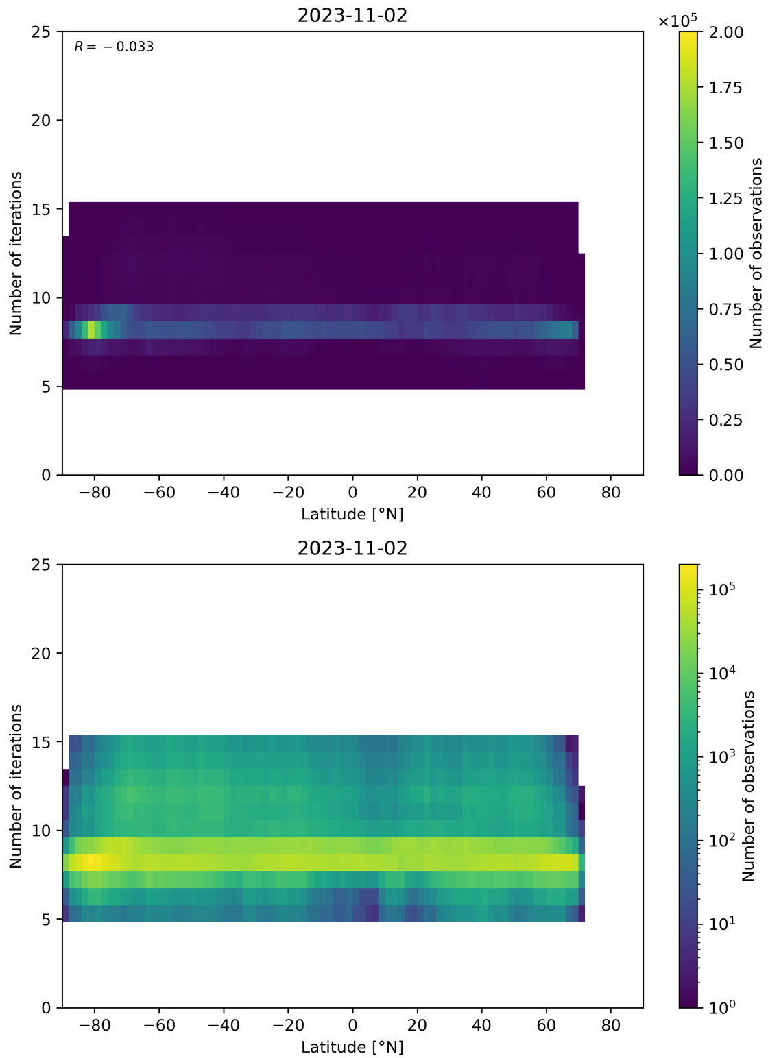
Figure 56: Scatter density plot of “Latitude” against “Number of iterations” for 2023-11-02 to 2023-11-03.
