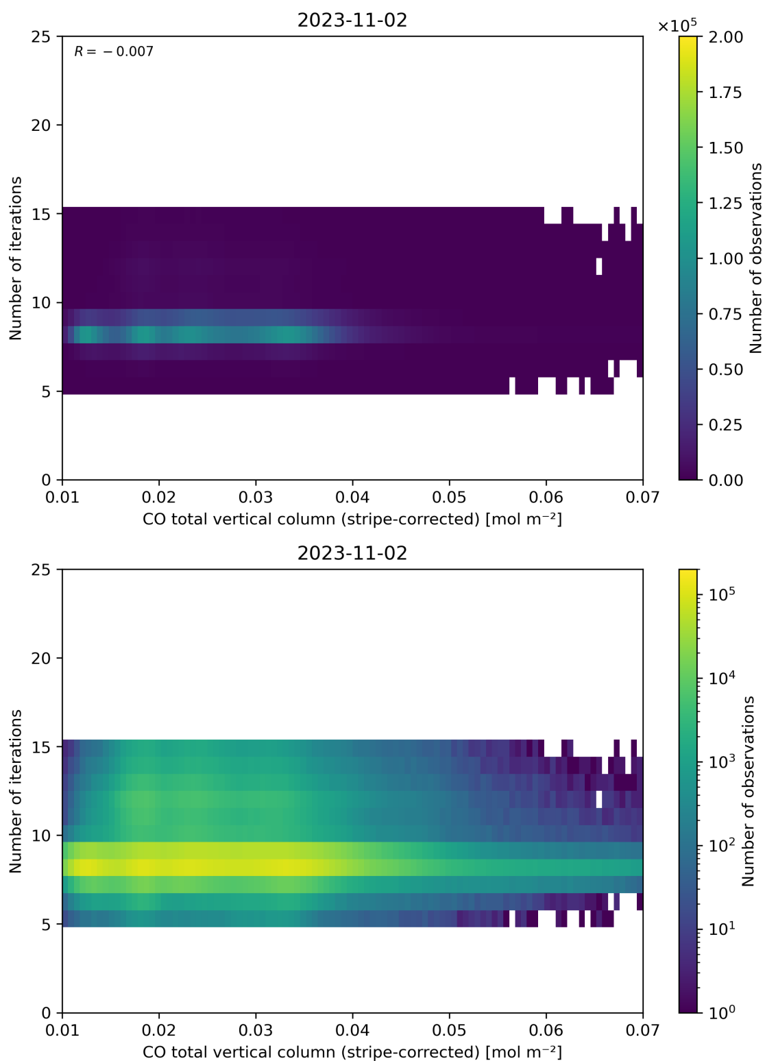
Figure 39: Scatter density plot of “CO total vertical column (stripe-corrected)” against “Number of iterations” for 2023-11-02 to 2023-11-03.
