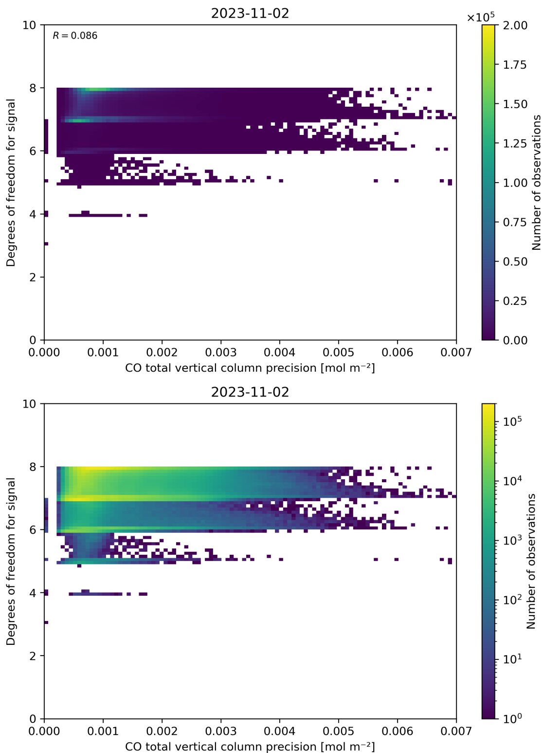
Figure 45: Scatter density plot of “CO total vertical column precision” against “Degrees of freedom for signal” for 2023-11-02 to 2023-11-03.
