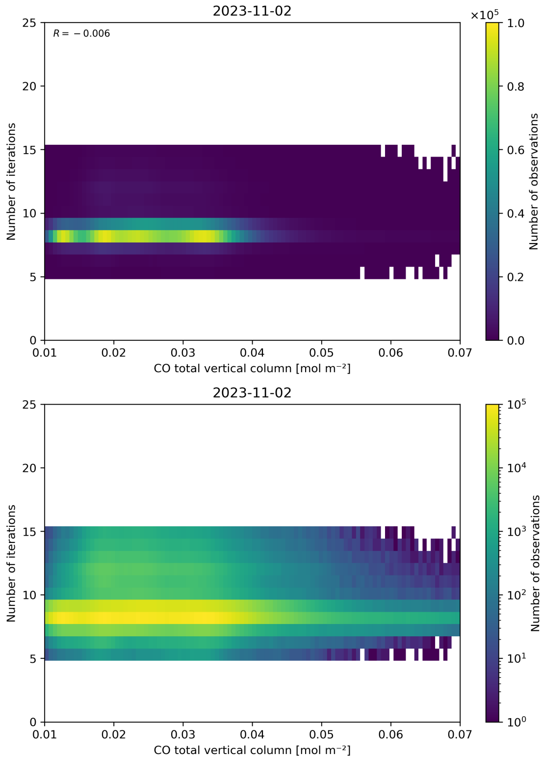
Figure 42: Scatter density plot of “CO total vertical column” against “Number of iterations” for 2023-11-02 to 2023-11-03.
