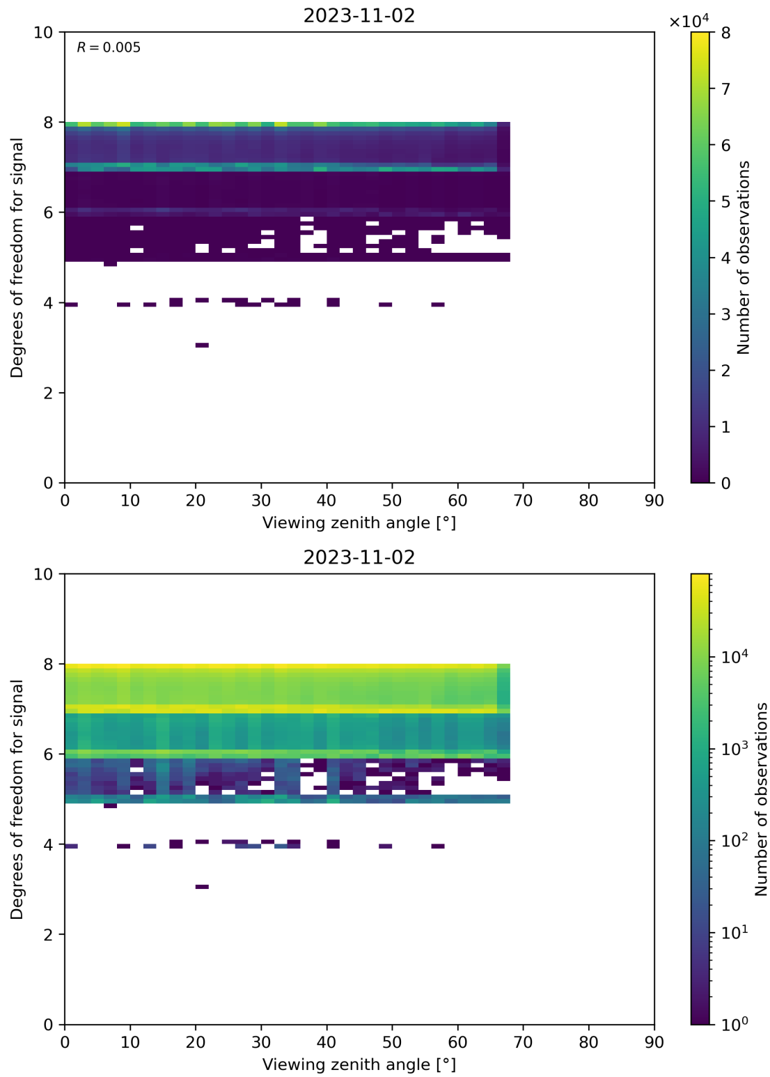
Figure 73: Scatter density plot of “Viewing zenith angle” against “Degrees of freedom for signal” for 2023-11-02 to 2023-11-03.
