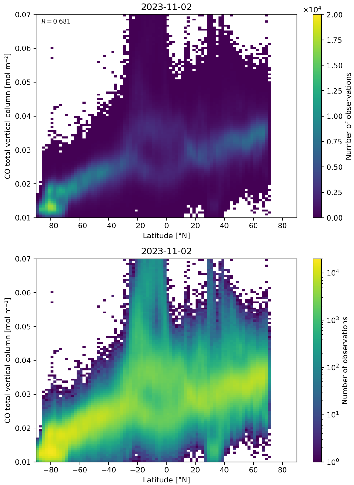
Figure 51: Scatter density plot of “Latitude” against “CO total vertical column” for 2023-11-02 to 2023-11-03.
