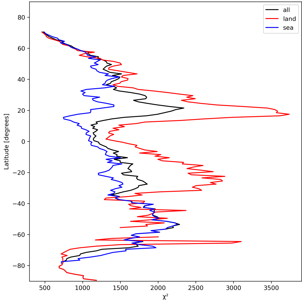
Figure 14: Zonal average of “ \chi^2 ” for 2023-11-02 to 2023-11-03.
