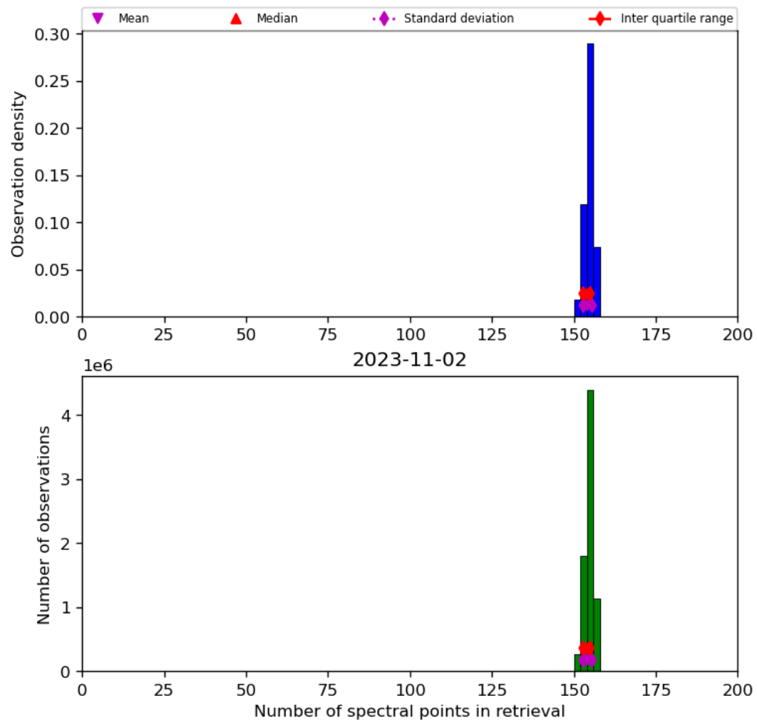
Figure 21: Histogram of “Number of spectral points in retrieval” for 2023-11-02 to 2023-11-03
