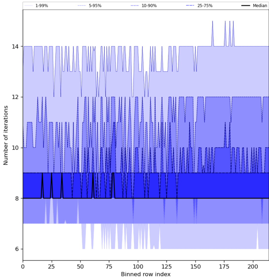
Figure 32: Along track statistics of “Number of iterations” for 2023-11-02 to 2023-11-03
