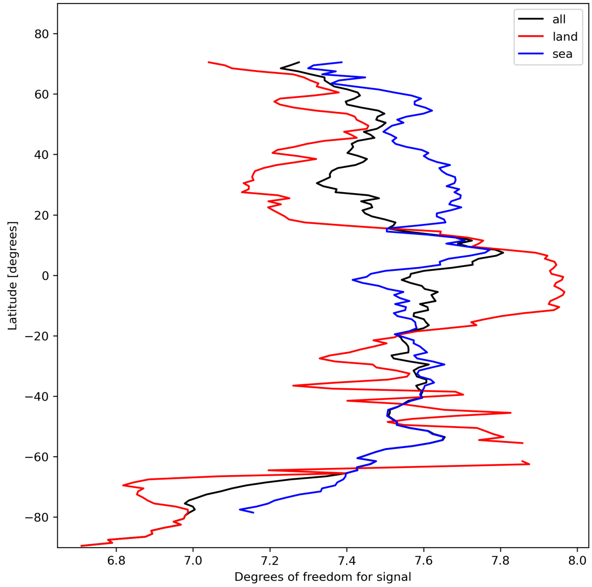
Figure 15: Zonal average of “Degrees of freedom for signal” for 2023-11-02 to 2023-11-03.
