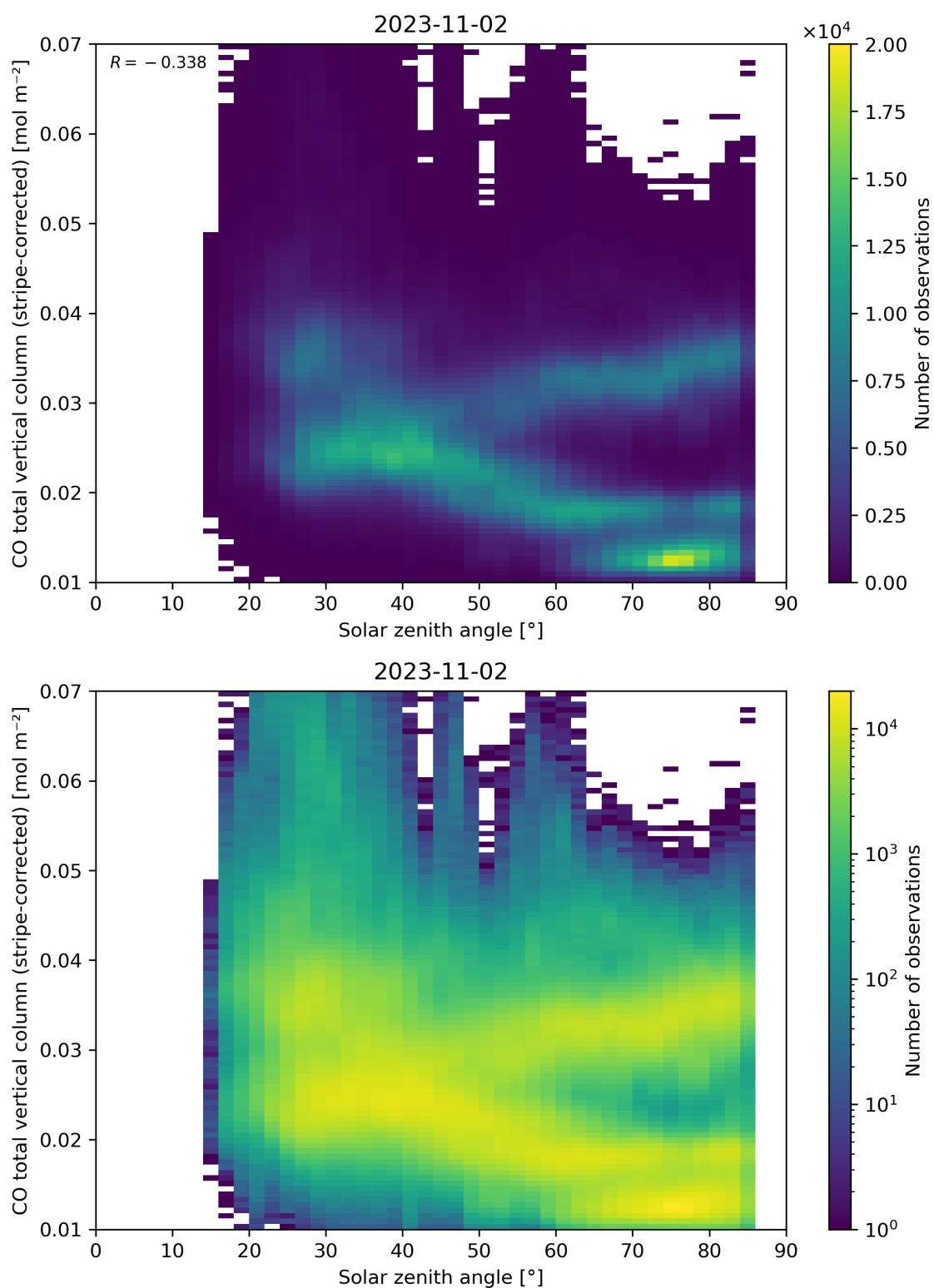
Figure 62: Scatter density plot of “Solar zenith angle” against “CO total vertical column (stripe-corrected)” for 2023-11-02 to 2023-11-03.
