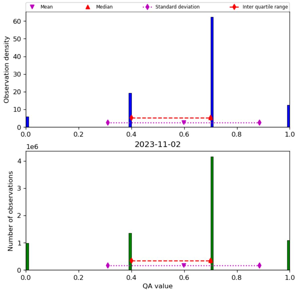
Figure 17: Histogram of “QA value” for 2023-11-02 to 2023-11-03
