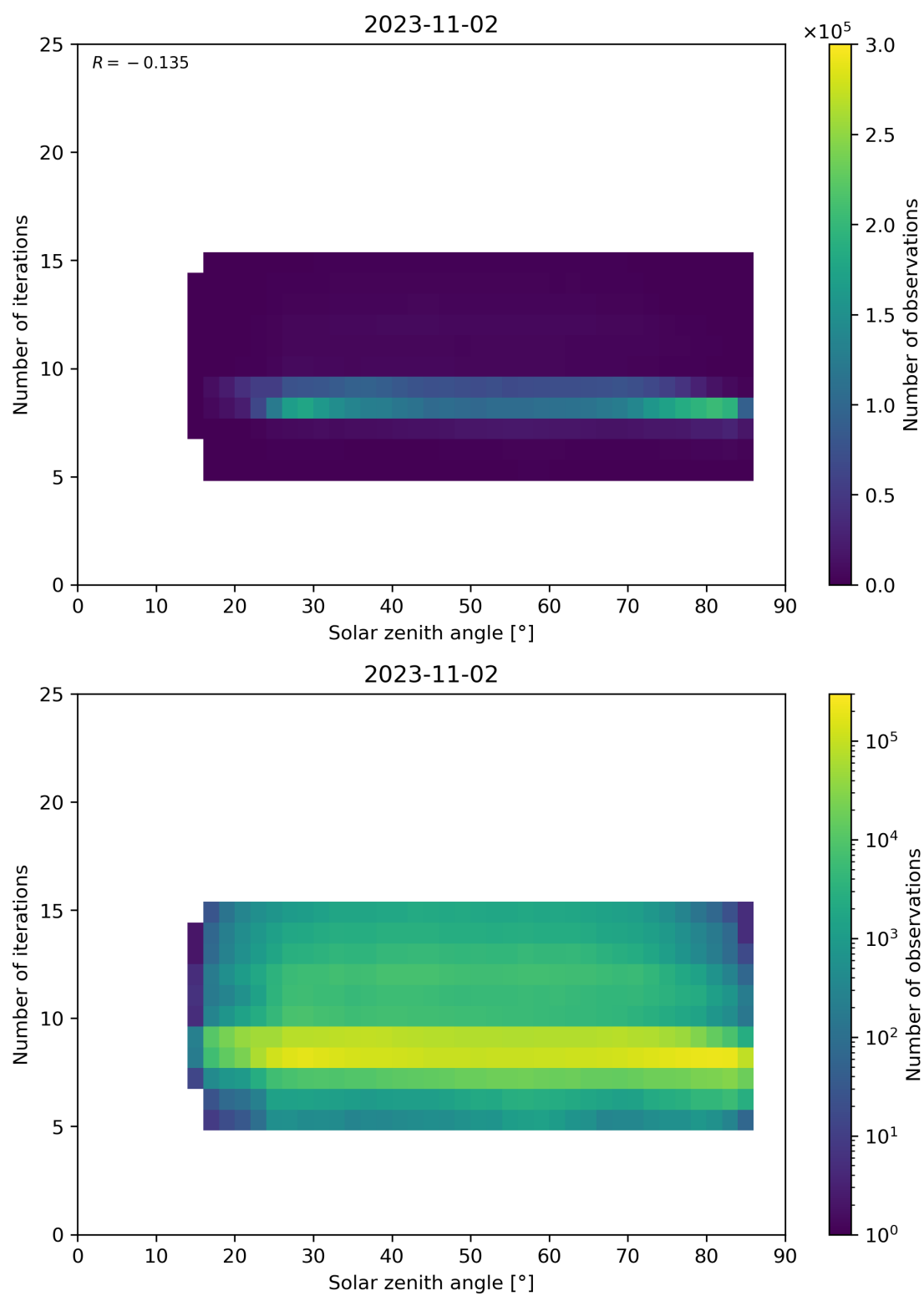
Figure 67: Scatter density plot of “Solar zenith angle” against “Number of iterations” for 2023-11-02 to 2023-11-03.
