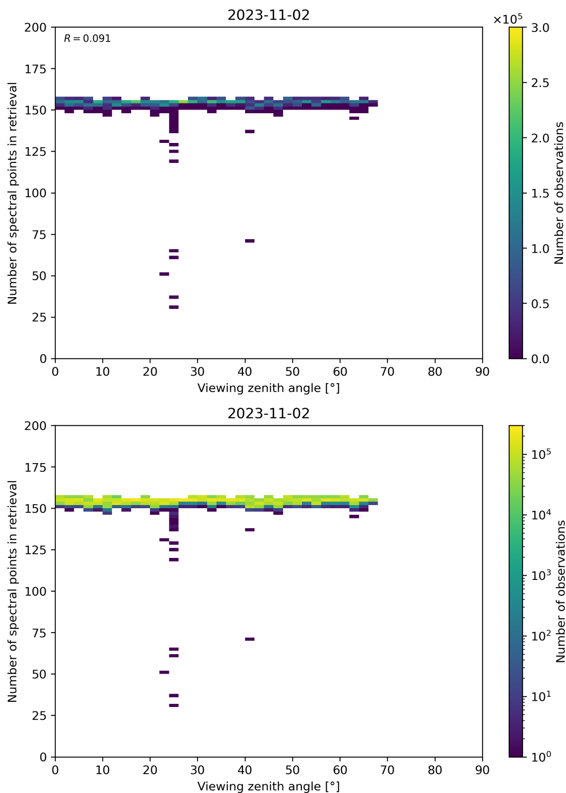
Figure 76: Scatter density plot of “Viewing zenith angle” against “Number of spectral points in retrieval” for 2023-11-02 to 2023-11-03.
