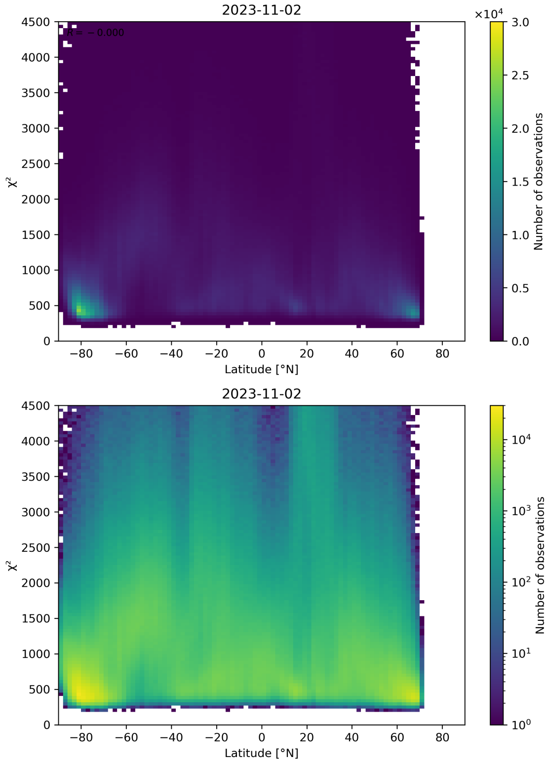
Figure 54: Scatter density plot of “Latitude” against “ \chi^2 ” for 2023-11-02 to 2023-11-03.
