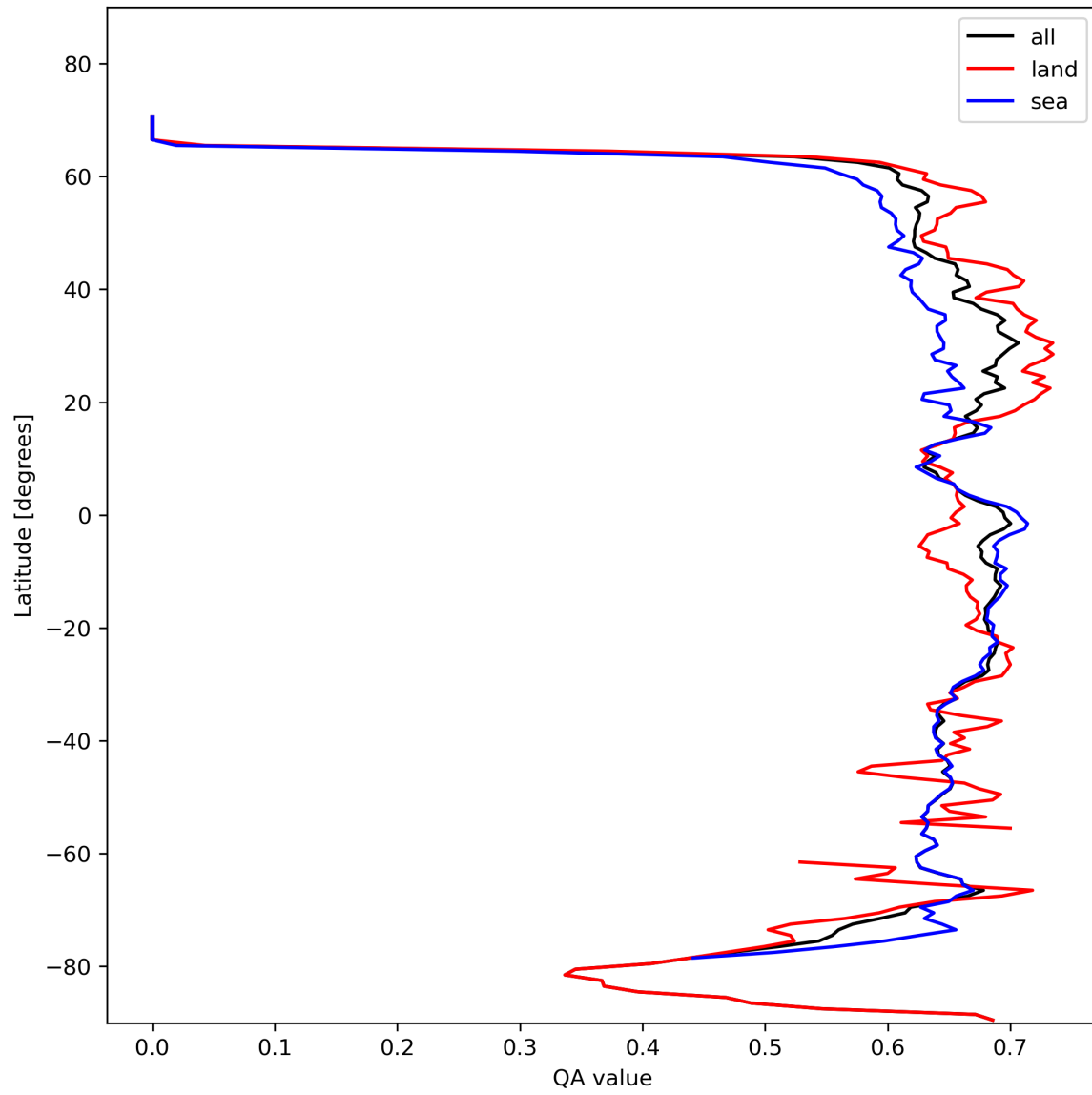
Figure 9: Zonal average of “QA value” for 2023-11-02 to 2023-11-03.
