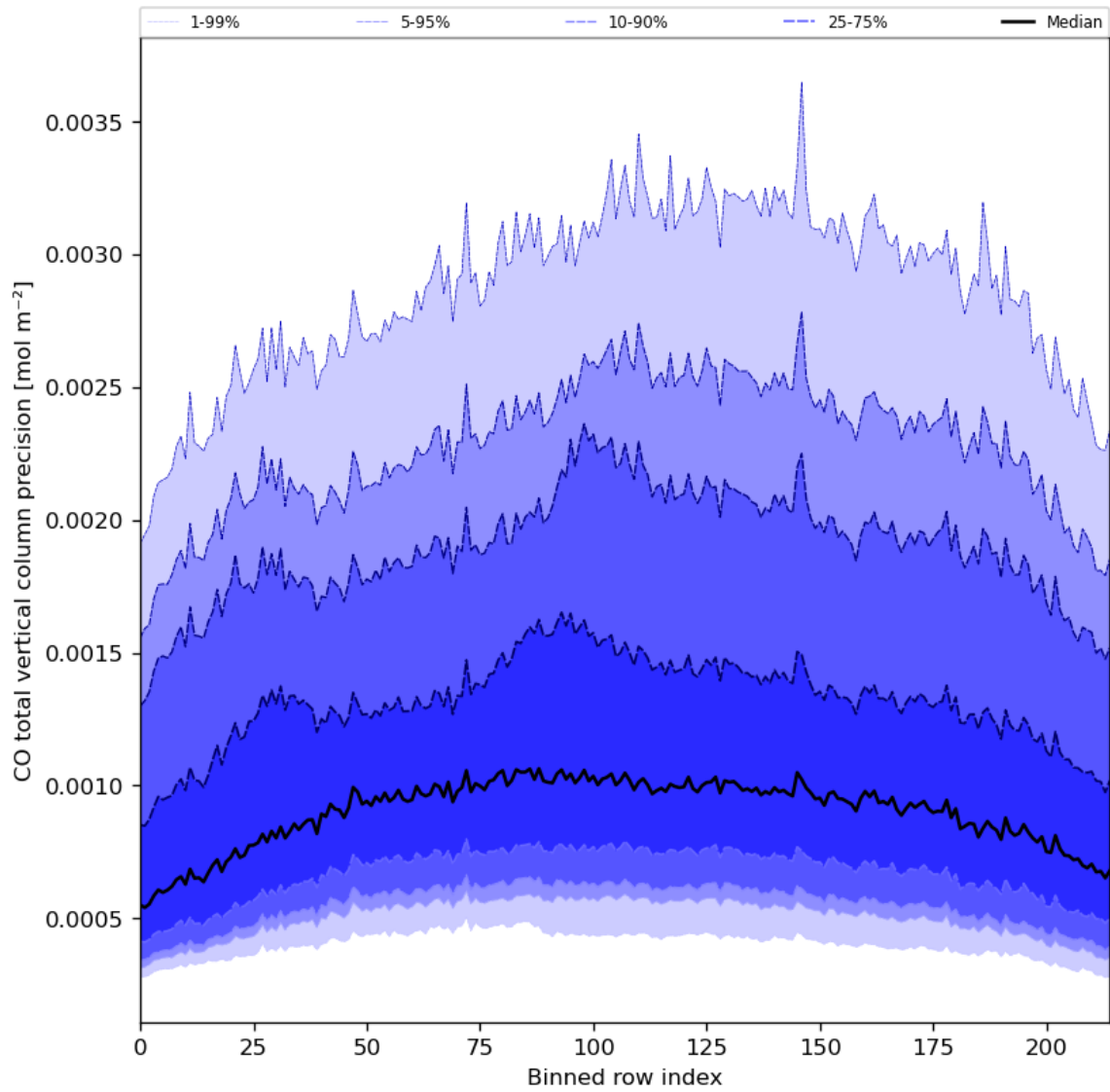
Figure 28: Along track statistics of “CO total vertical column precision” for 2023-11-02 to 2023-11-03
