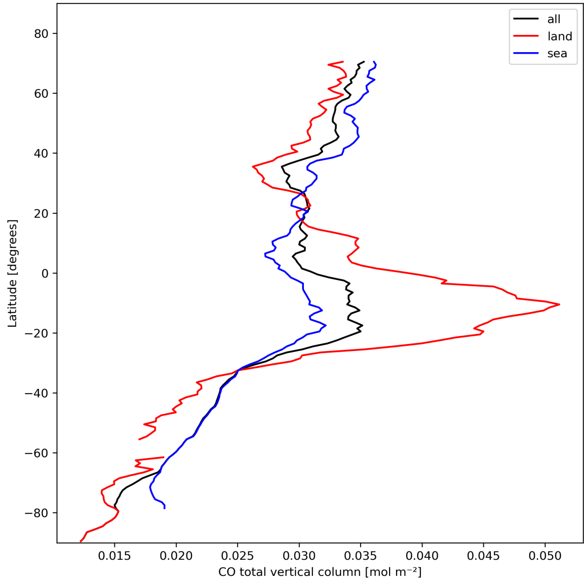
Figure 10: Zonal average of “CO total vertical column” for 2023-11-02 to 2023-11-03.
