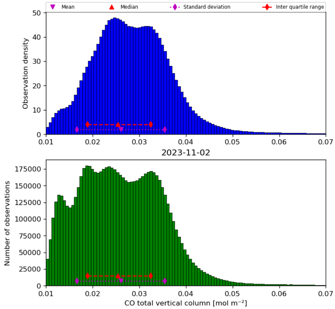
Figure 18: Histogram of “CO total vertical column” for 2023-11-02 to 2023-11-03
