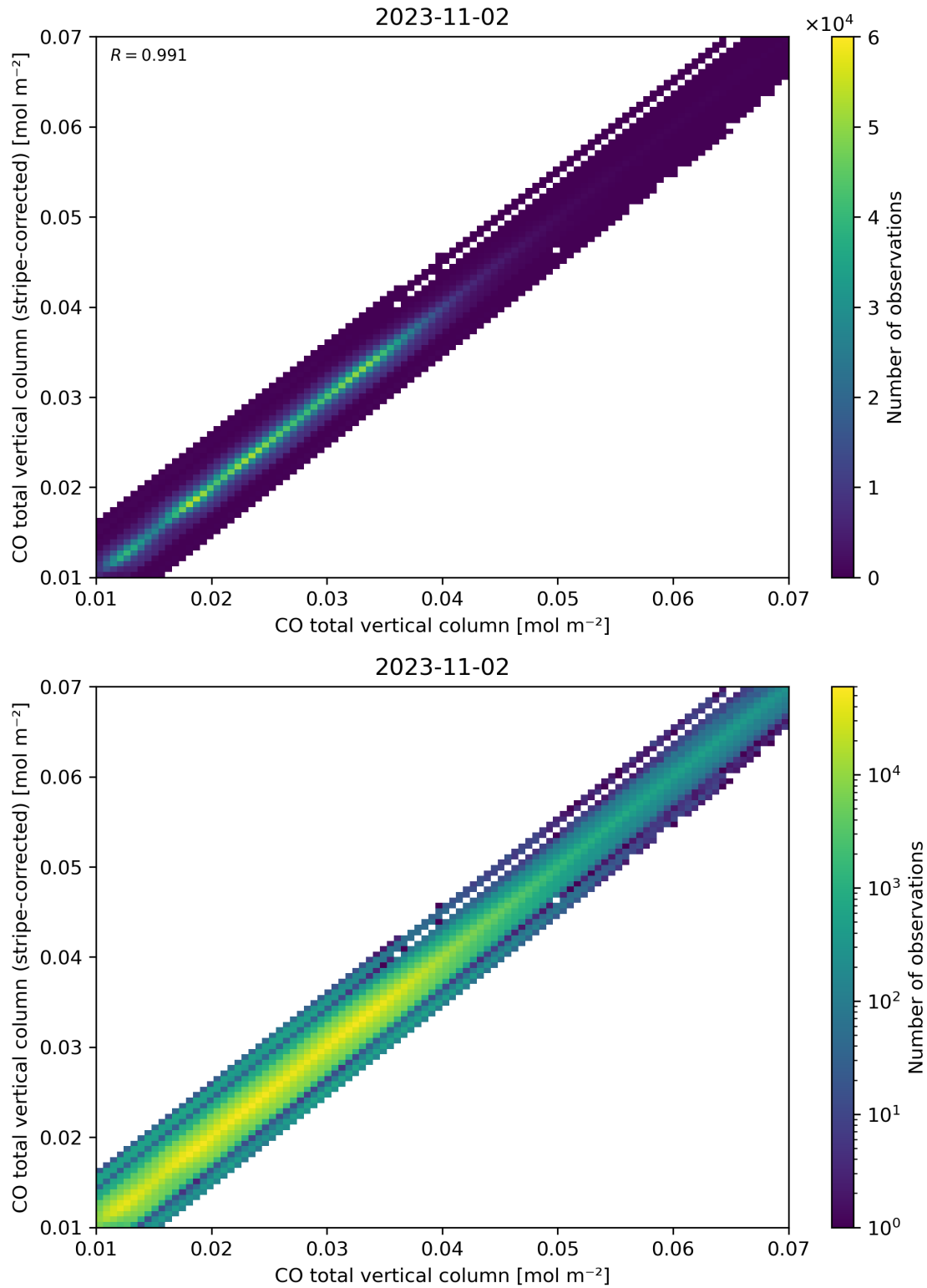
Figure 33: Scatter density plot of “CO total vertical column” against “CO total vertical column (stripe-corrected)” for 2023-11-02 to 2023-11-03.
