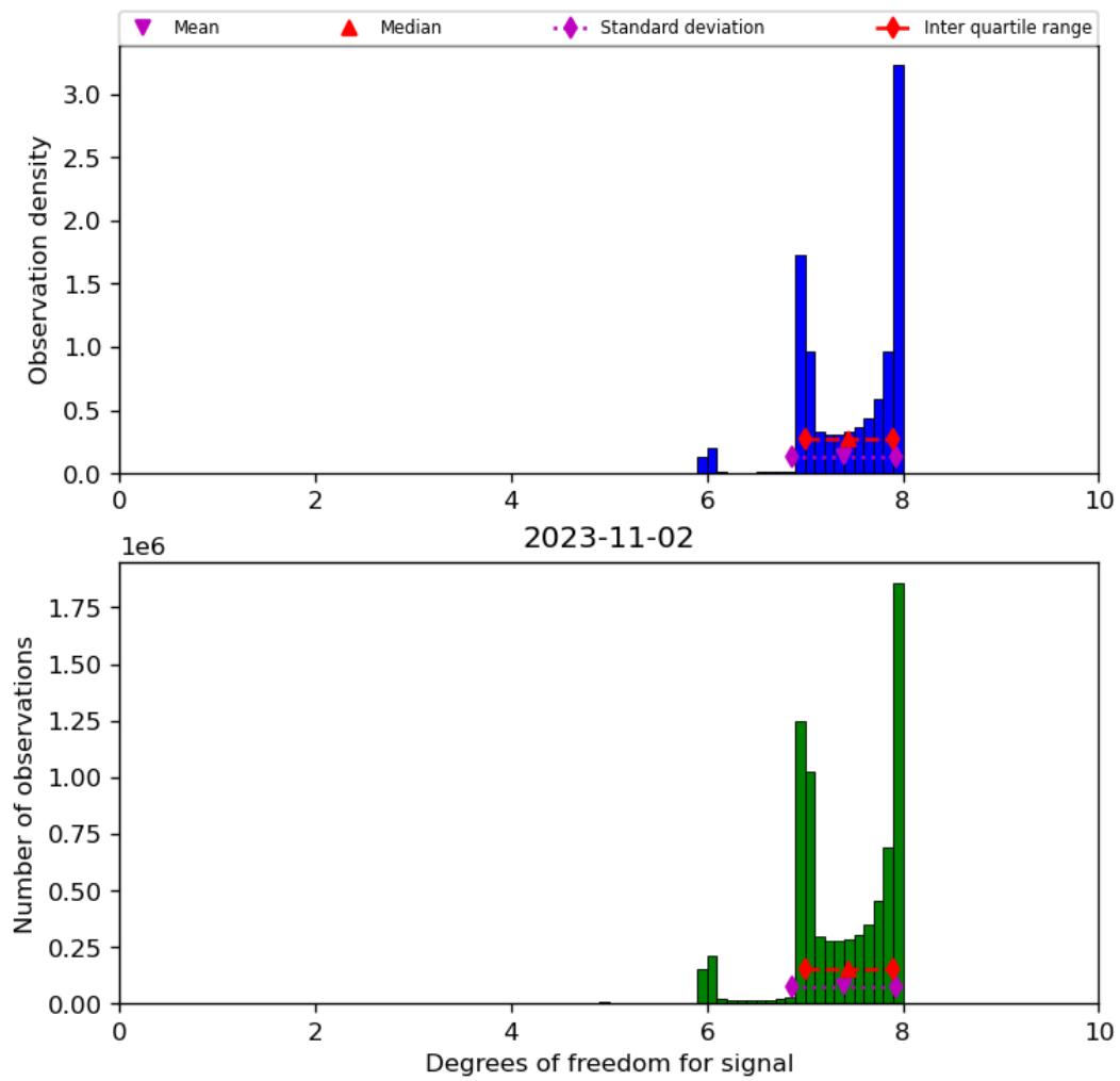
Figure 23: Histogram of “Degrees of freedom for signal” for 2023-11-02 to 2023-11-03
