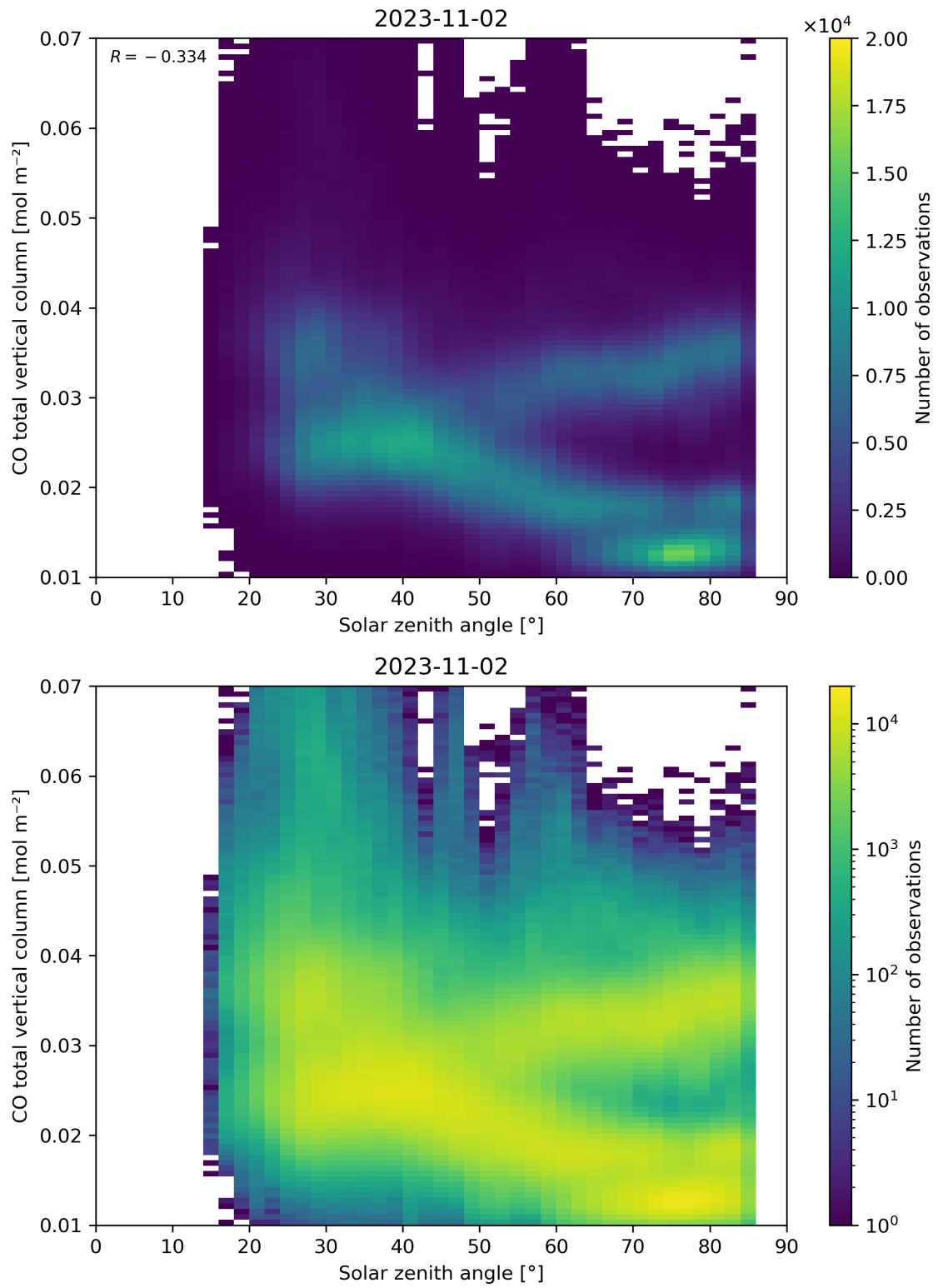
Figure 61: Scatter density plot of “Solar zenith angle” against “CO total vertical column” for 2023-11-02 to 2023-11-03.
