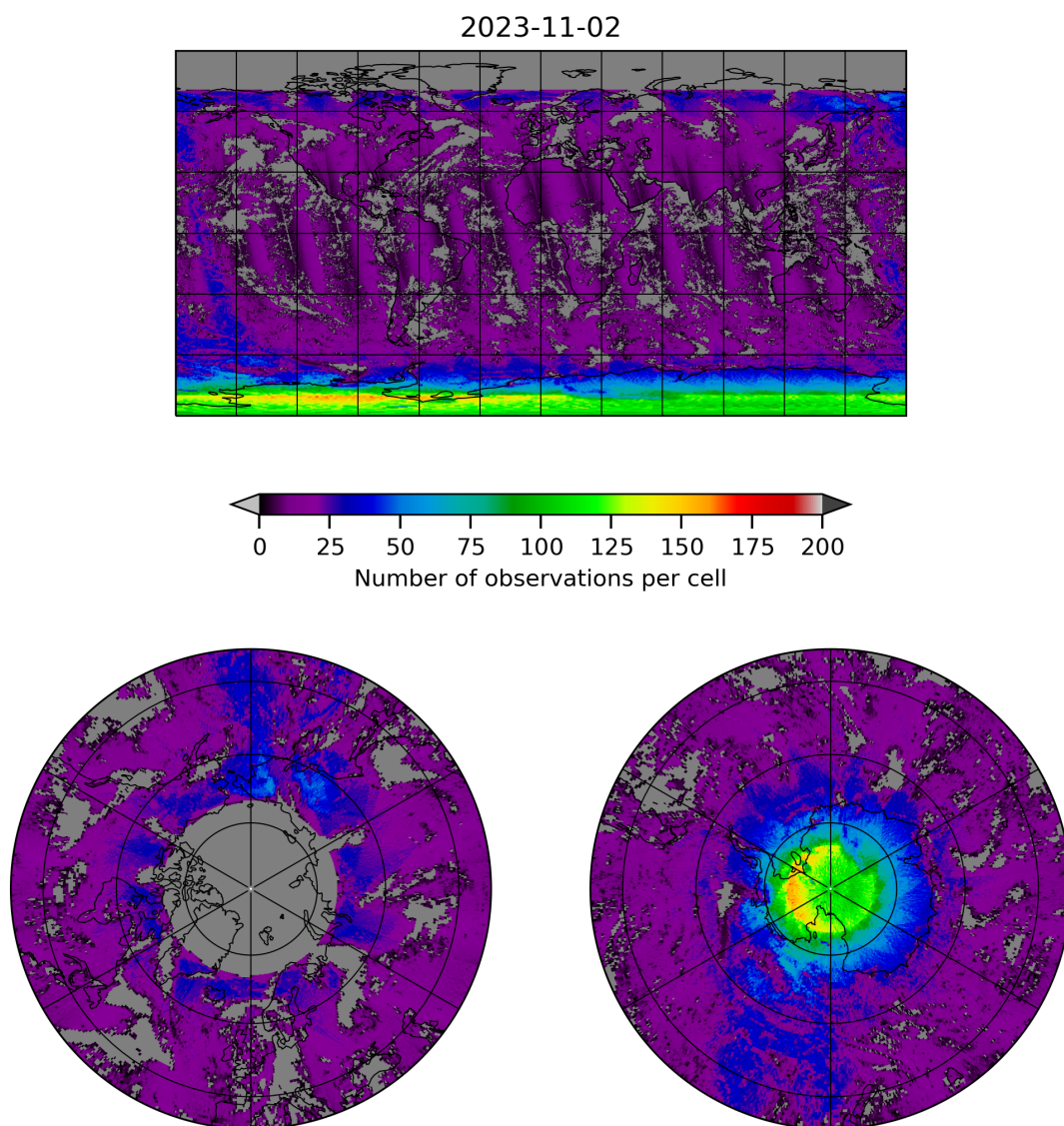
Figure 8: Map of the number of observations for 2023-11-02 to 2023-11-03
