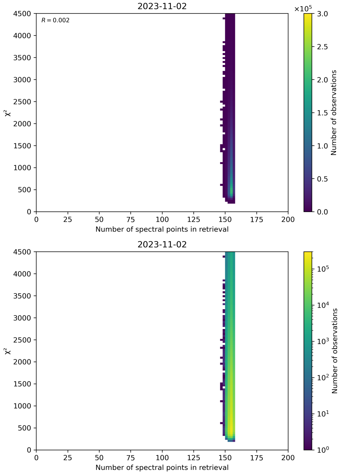
Figure 58: Scatter density plot of “Number of spectral points in retrieval” against “ \chi^2 ” for 2023-11-02 to 2023-11-03.
