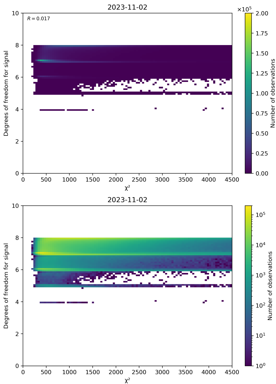
Figure 48: Scatter density plot of “ \chi^2 ” against “Degrees of freedom for signal” for 2023-11-02 to 2023-11-03.
