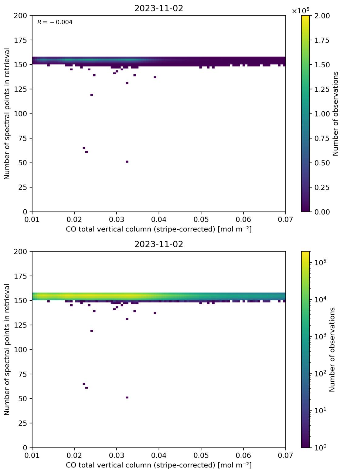
Figure 40: Scatter density plot of “CO total vertical column (stripe-corrected)” against “Number of spectral points in retrieval” for 2023-11-02 to 2023-11-03.
