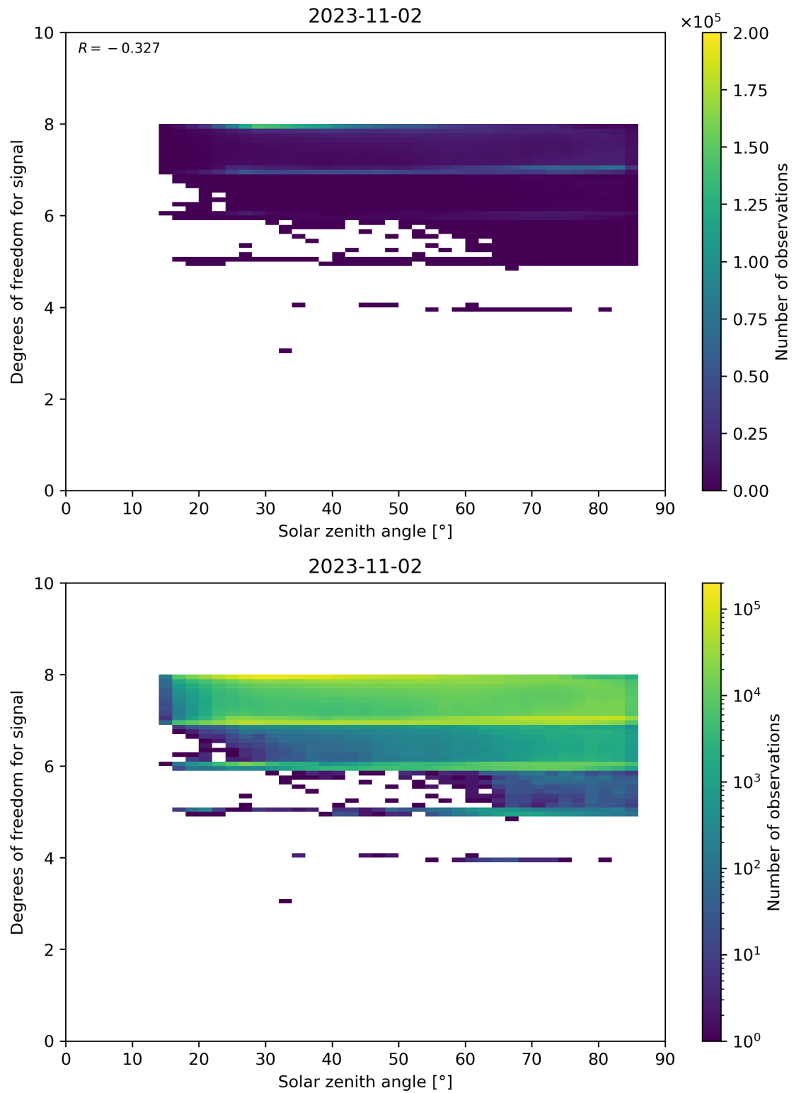
Figure 65: Scatter density plot of “Solar zenith angle” against “Degrees of freedom for signal” for 2023-11-02 to 2023-11-03.
