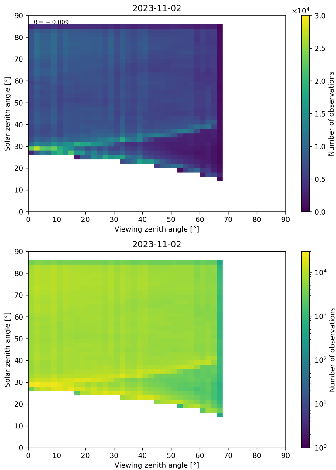
Figure 77: Scatter density plot of “Viewing zenith angle” against “Solar zenith angle” for 2023-11-02 to 2023-11-03.
