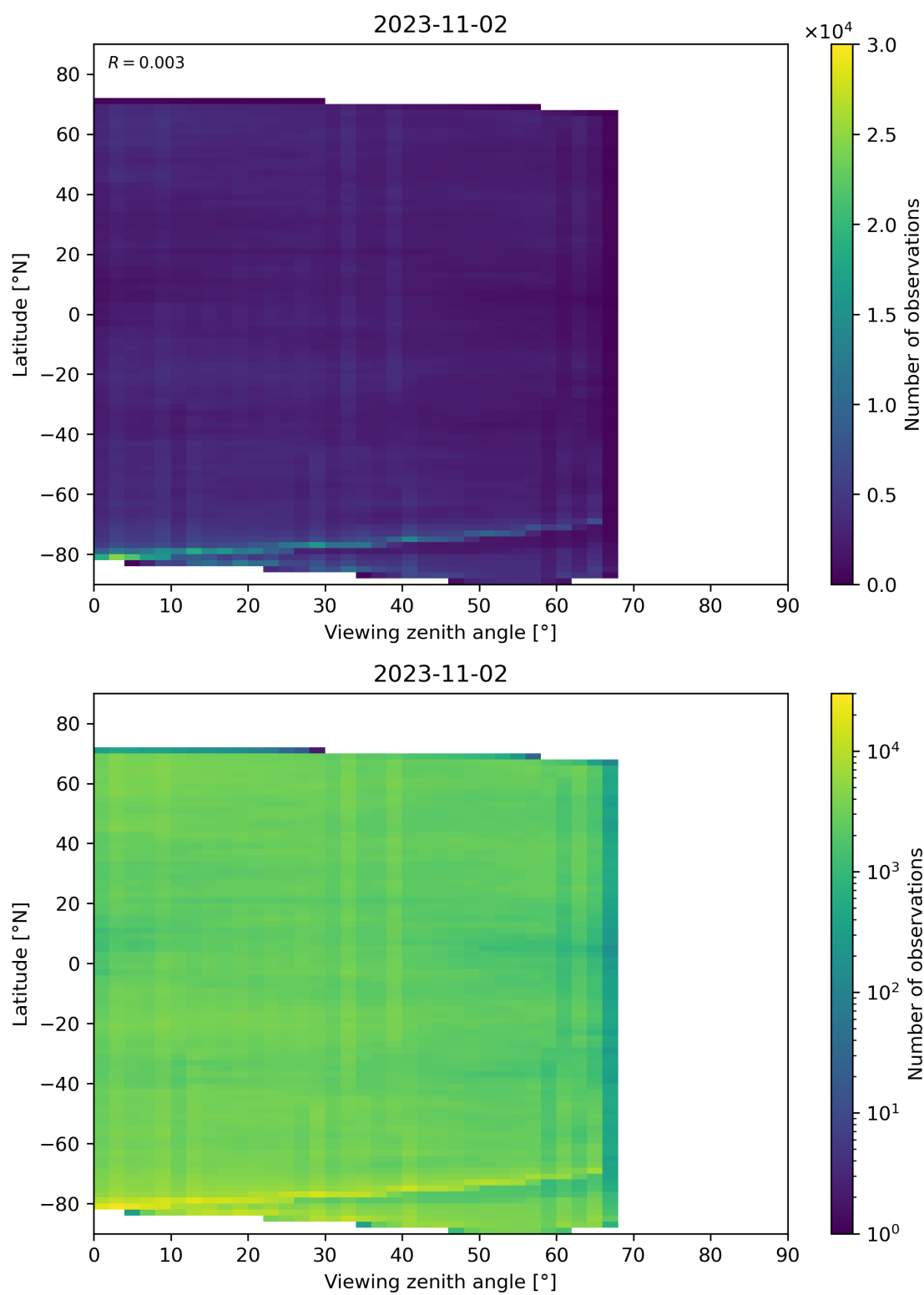
Figure 74: Scatter density plot of “Viewing zenith angle” against “Latitude” for 2023-11-02 to 2023-11-03.
