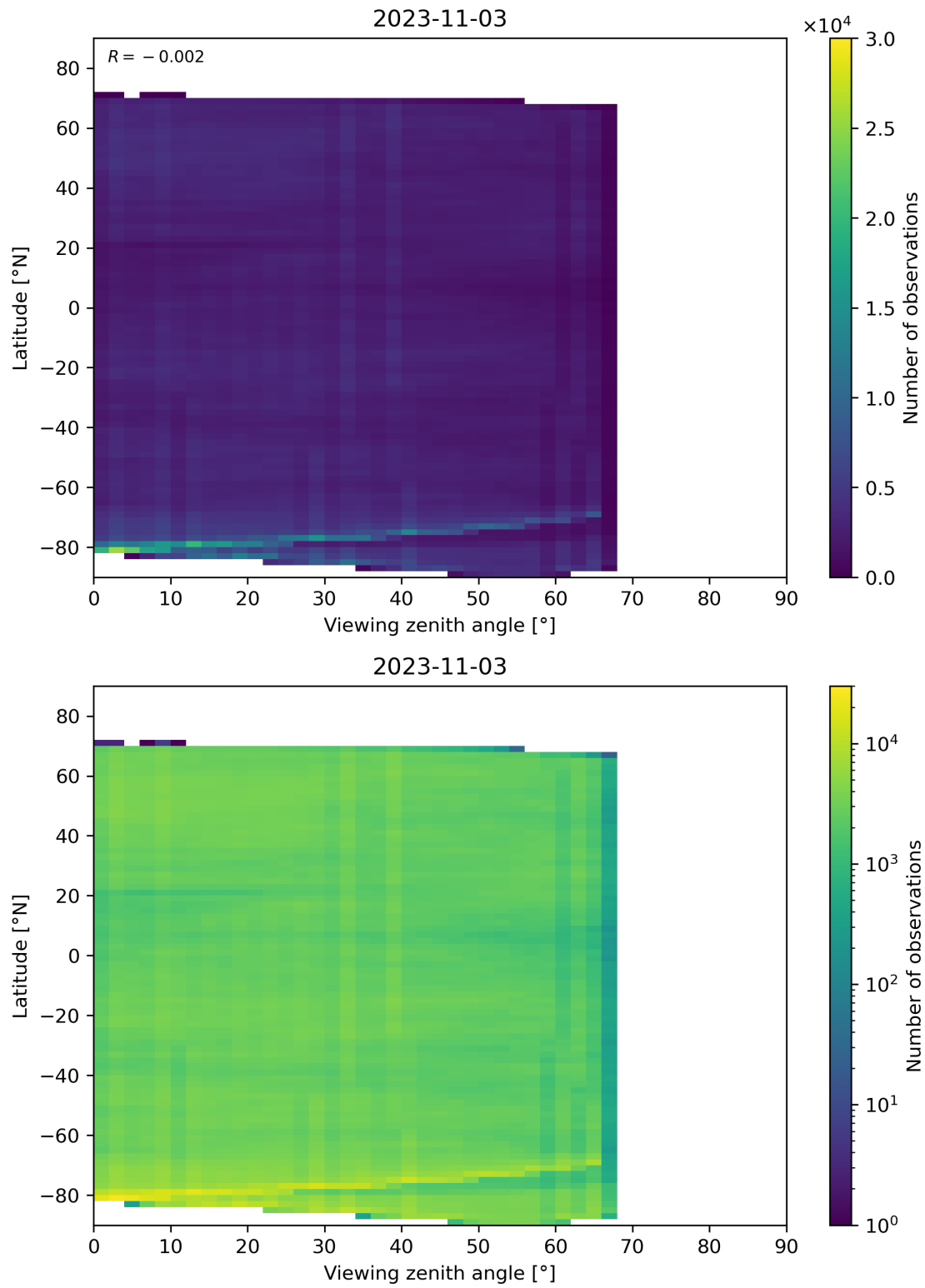
Figure 74: Scatter density plot of “Viewing zenith angle” against “Latitude” for 2023-11-02 to 2023-11-04.
