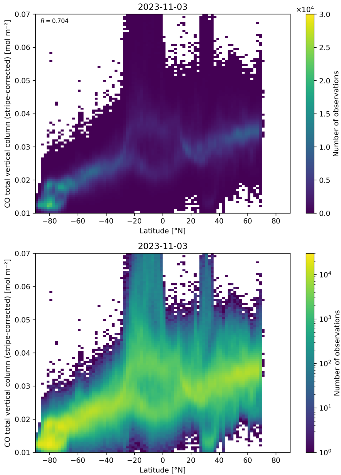
Figure 52: Scatter density plot of “Latitude” against “CO total vertical column (stripe-corrected)” for 2023-11-02 to 2023-11-04.
