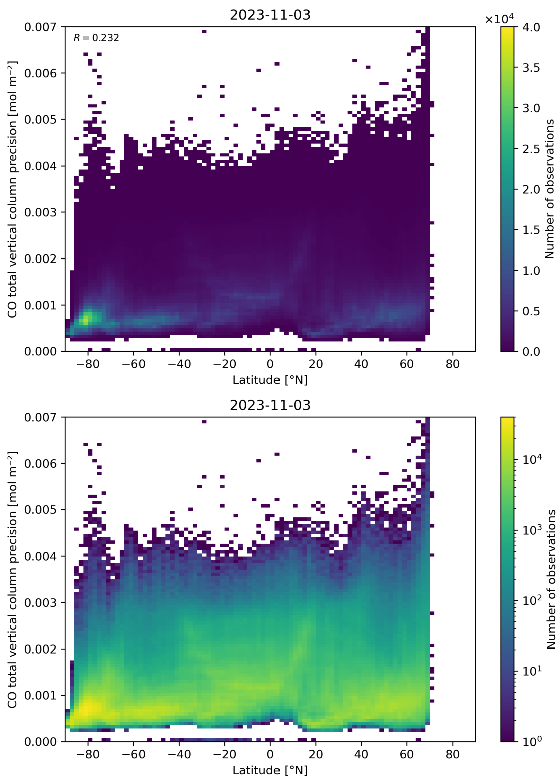
Figure 53: Scatter density plot of “Latitude” against “CO total vertical column precision” for 2023-11-02 to 2023-11-04.
