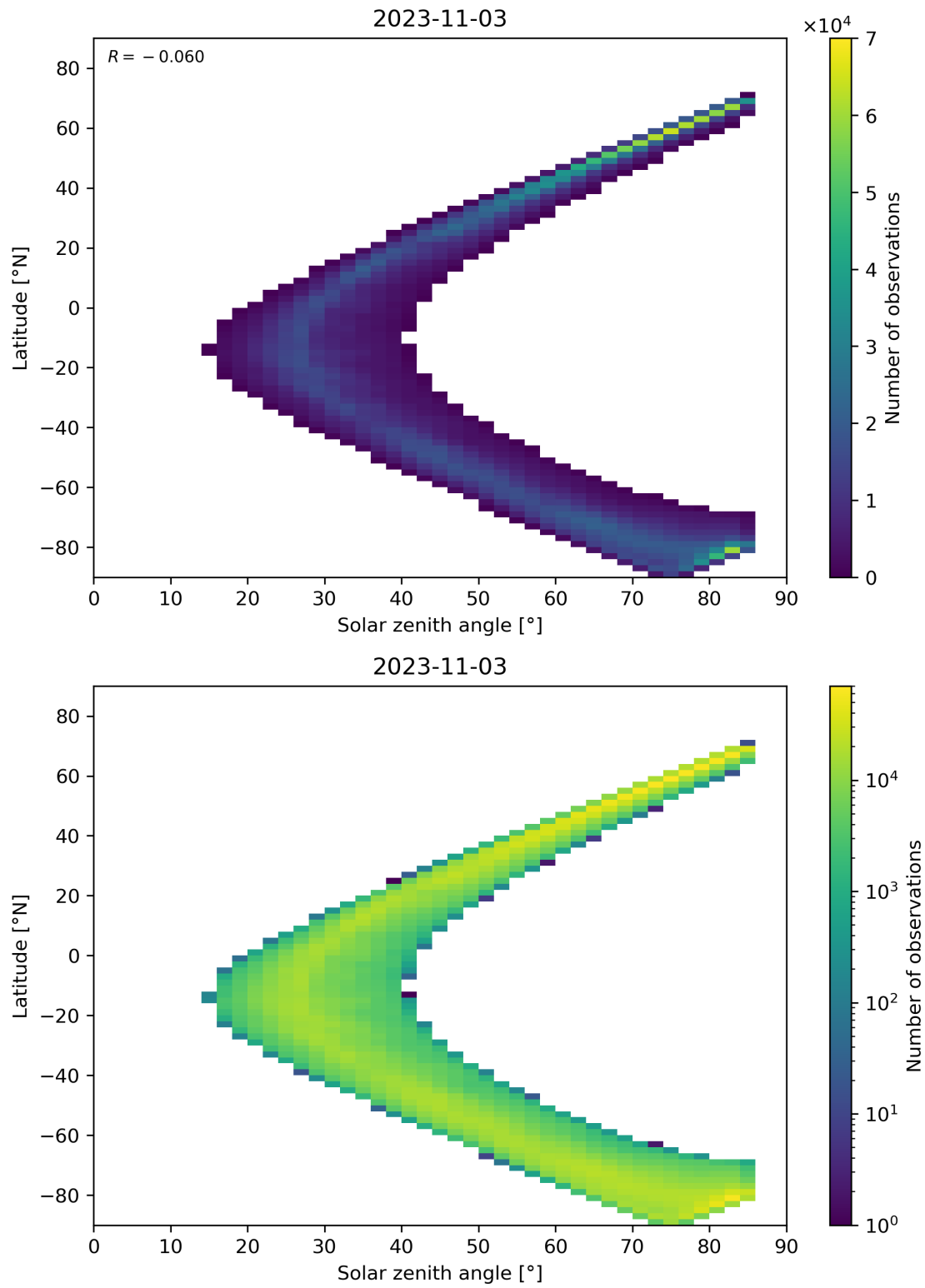
Figure 66: Scatter density plot of “Solar zenith angle” against “Latitude” for 2023-11-02 to 2023-11-04.
