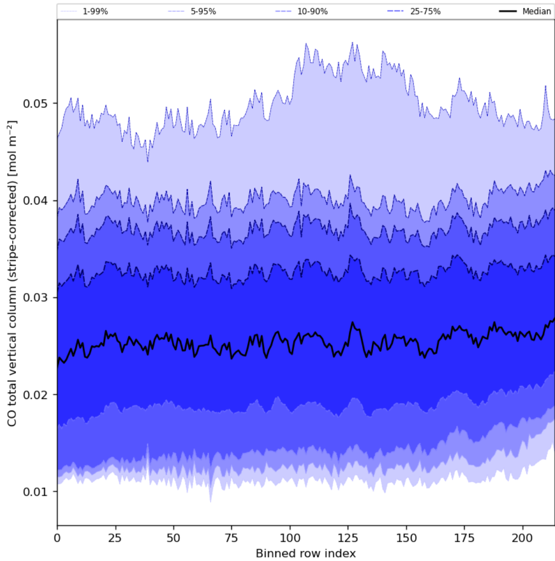
Figure 27: Along track statistics of “CO total vertical column (stripe-corrected)” for 2023-11-02 to 2023-11-04
