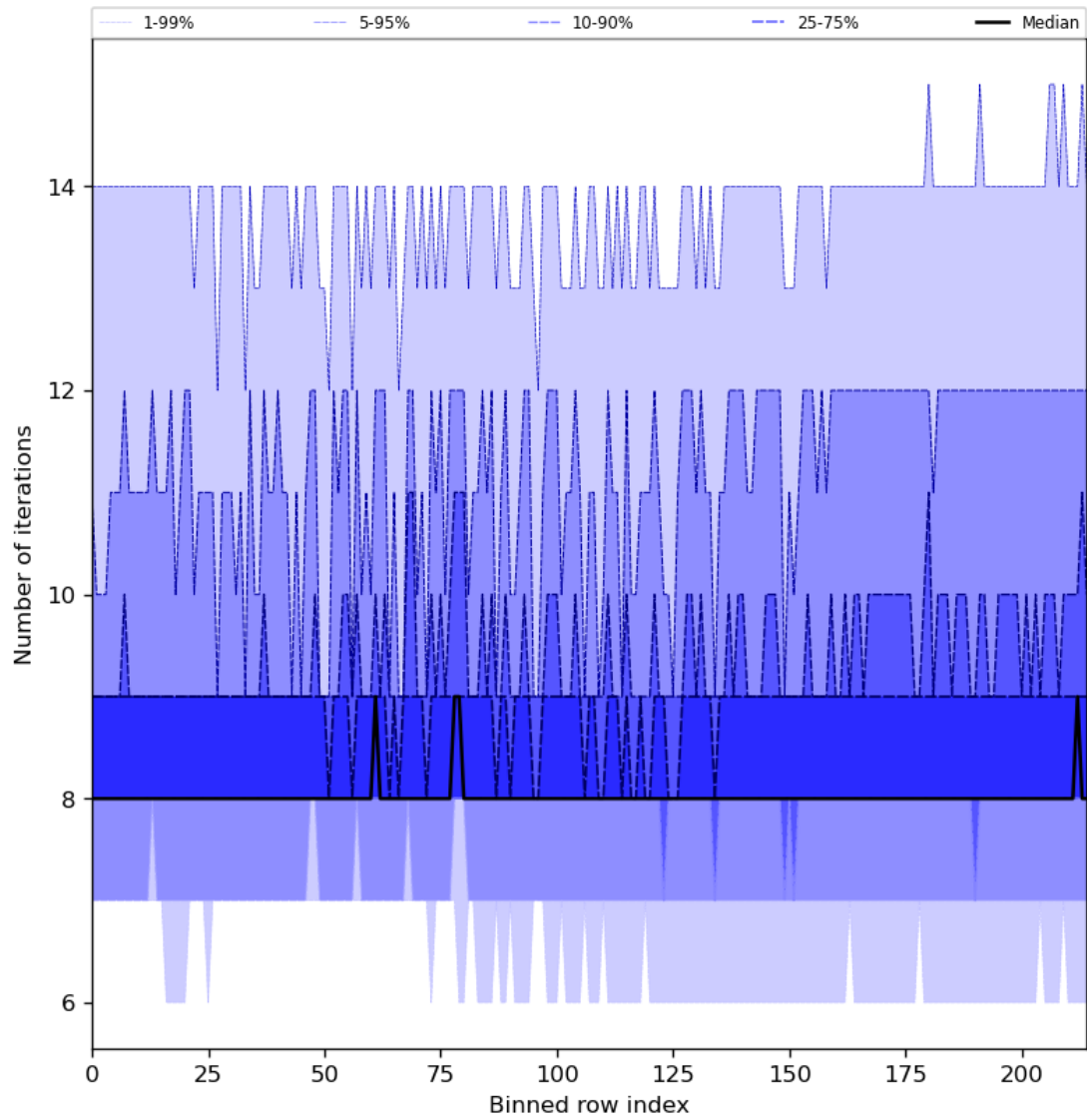
Figure 32: Along track statistics of “Number of iterations” for 2023-11-02 to 2023-11-04
