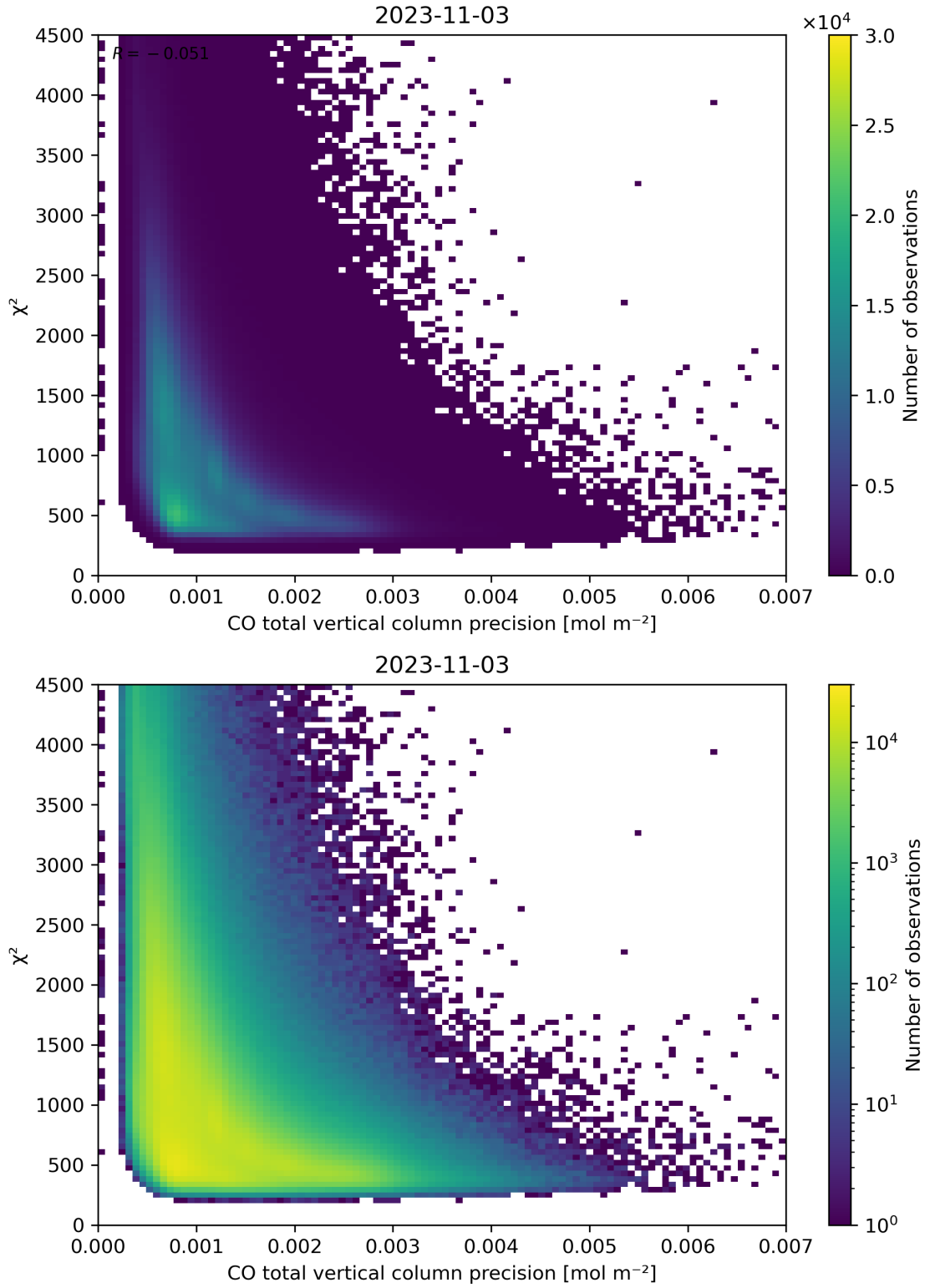
Figure 44: Scatter density plot of “CO total vertical column precision” against “ \chi^2 ” for 2023-11-02 to 2023-11-04.
