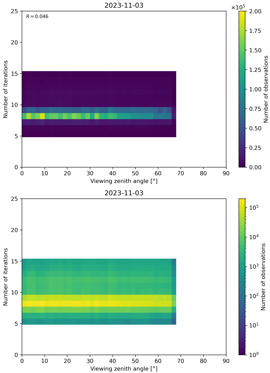
Figure 75: Scatter density plot of “Viewing zenith angle” against “Number of iterations” for 2023-11-02 to 2023-11-04.
