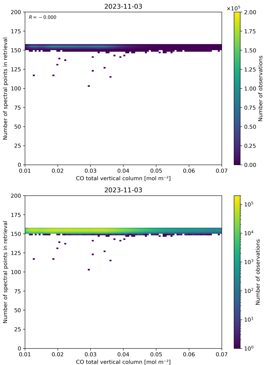
Figure 43: Scatter density plot of “CO total vertical column” against “Number of spectral points in retrieval” for 2023-11-02 to 2023-11-04.
