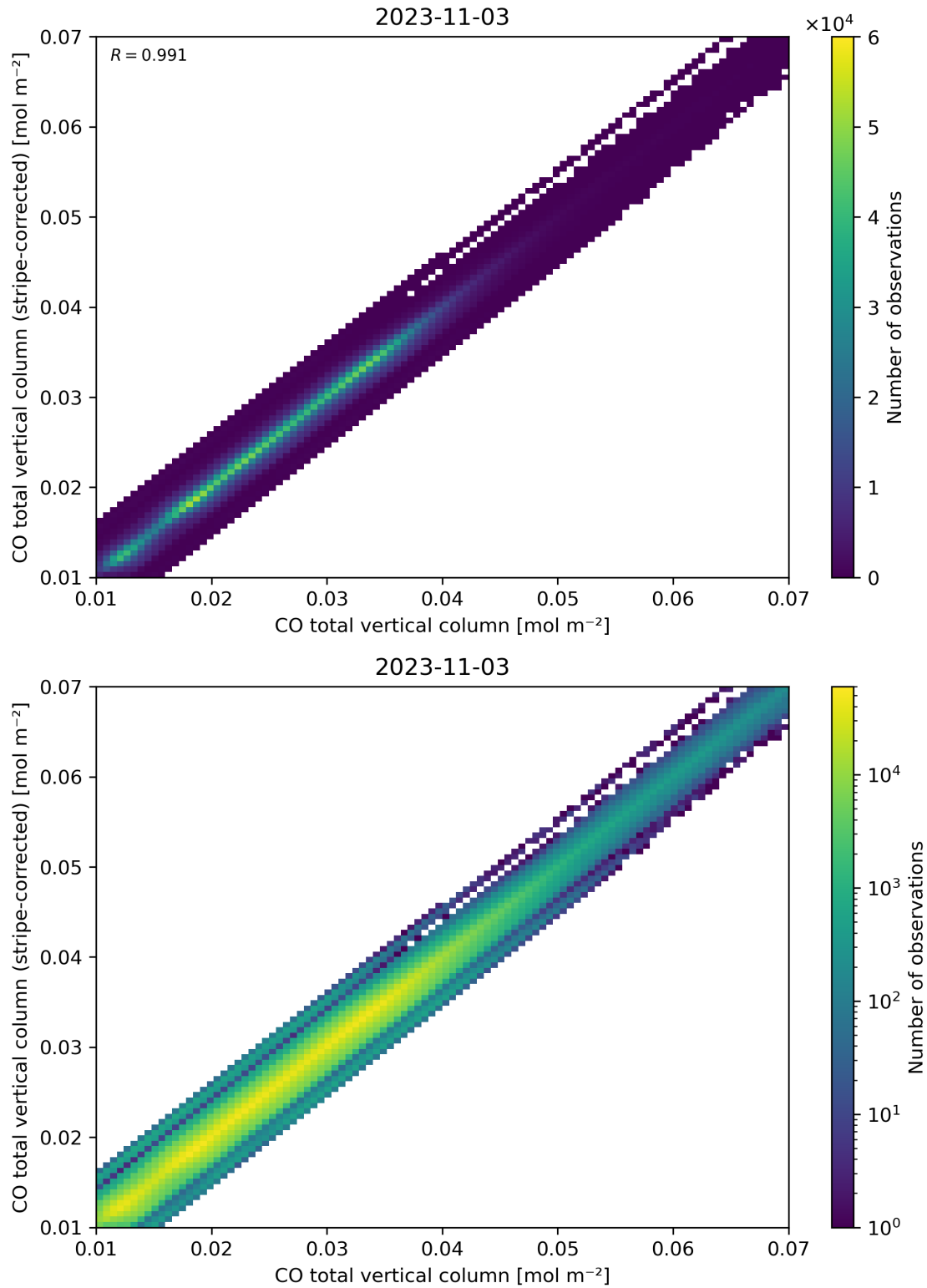
Figure 33: Scatter density plot of “CO total vertical column” against “CO total vertical column (stripe-corrected)” for 2023-11-02 to 2023-11-04.
