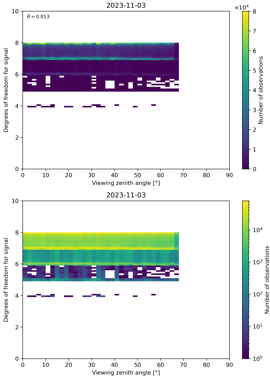
Figure 73: Scatter density plot of “Viewing zenith angle” against “Degrees of freedom for signal” for 2023-11-02 to 2023-11-04.
