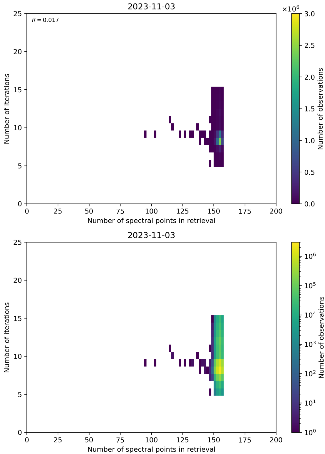
Figure 60: Scatter density plot of “Number of spectral points in retrieval” against “Number of iterations” for 2023-11-02 to 2023-11-04.
