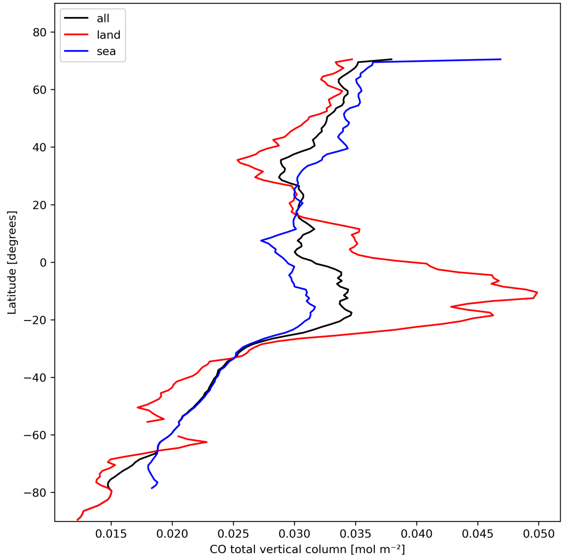
Figure 10: Zonal average of “CO total vertical column” for 2023-11-02 to 2023-11-04.
