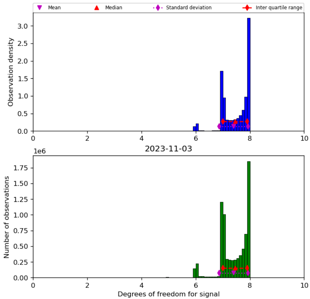
Figure 23: Histogram of “Degrees of freedom for signal” for 2023-11-02 to 2023-11-04
