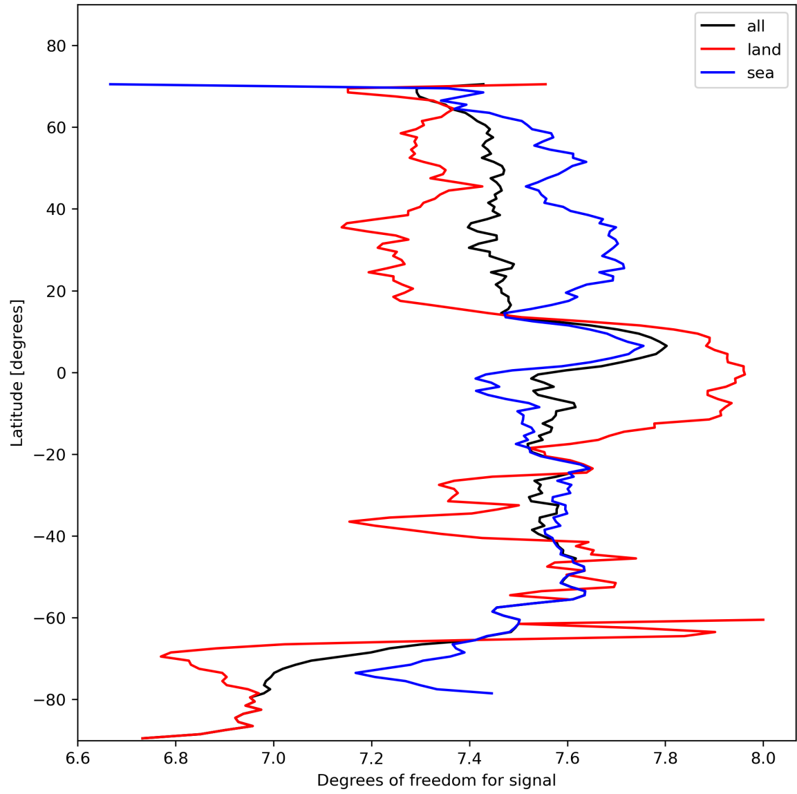
Figure 15: Zonal average of “Degrees of freedom for signal” for 2023-11-02 to 2023-11-04.
