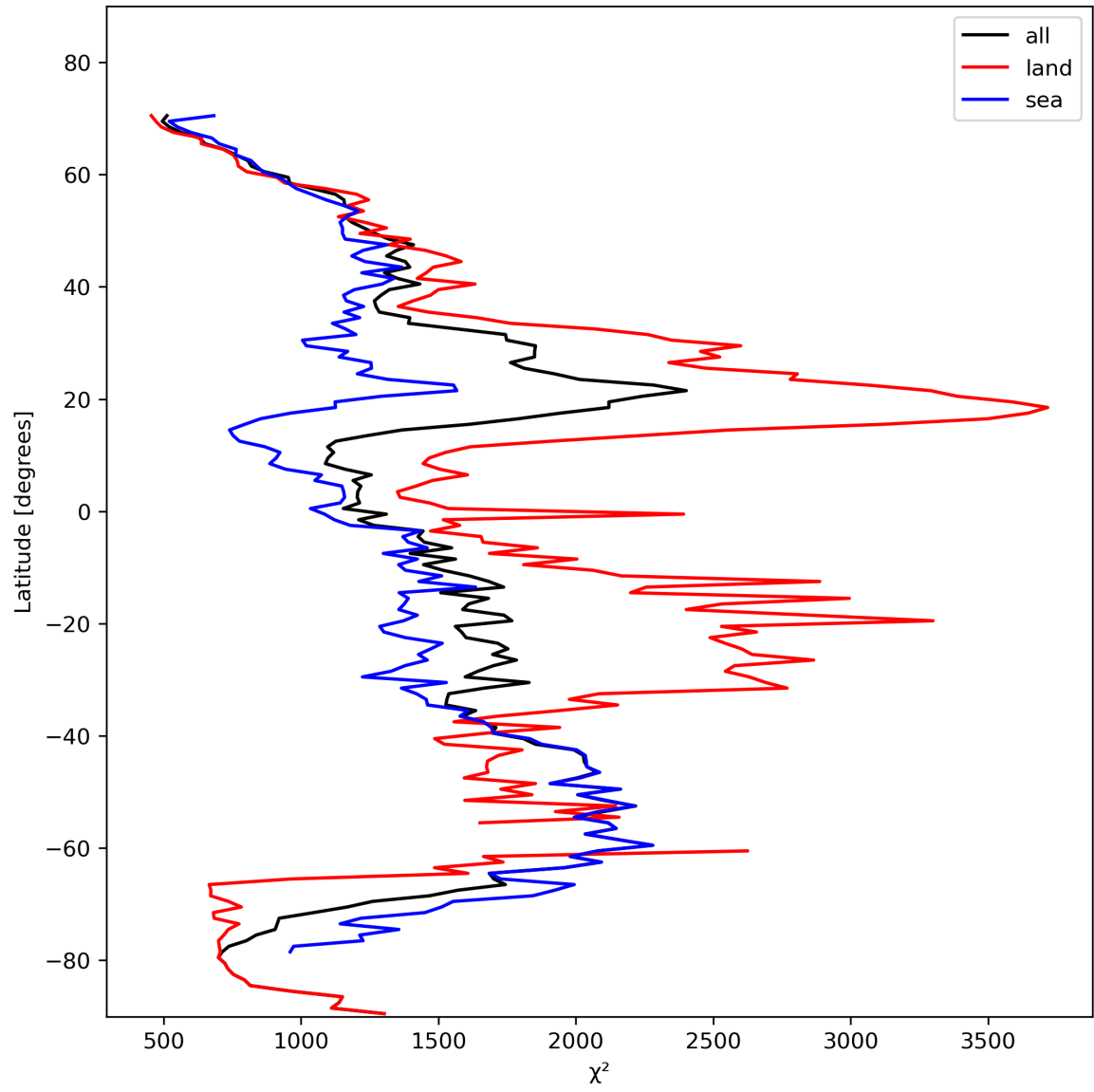
Figure 14: Zonal average of “ \chi^2 ” for 2023-11-02 to 2023-11-04.
