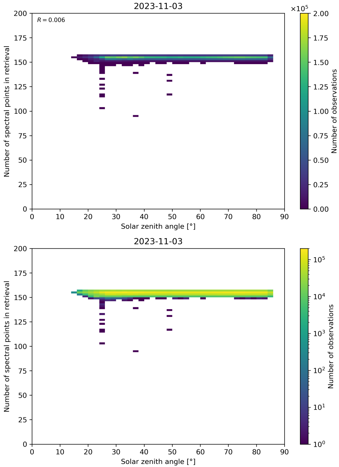
Figure 68: Scatter density plot of “Solar zenith angle” against “Number of spectral points in retrieval” for 2023-11-02 to 2023-11-04.
