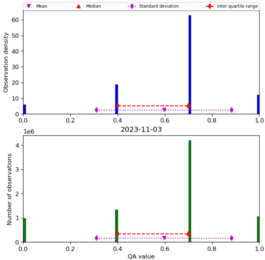
Figure 17: Histogram of “QA value” for 2023-11-02 to 2023-11-04
