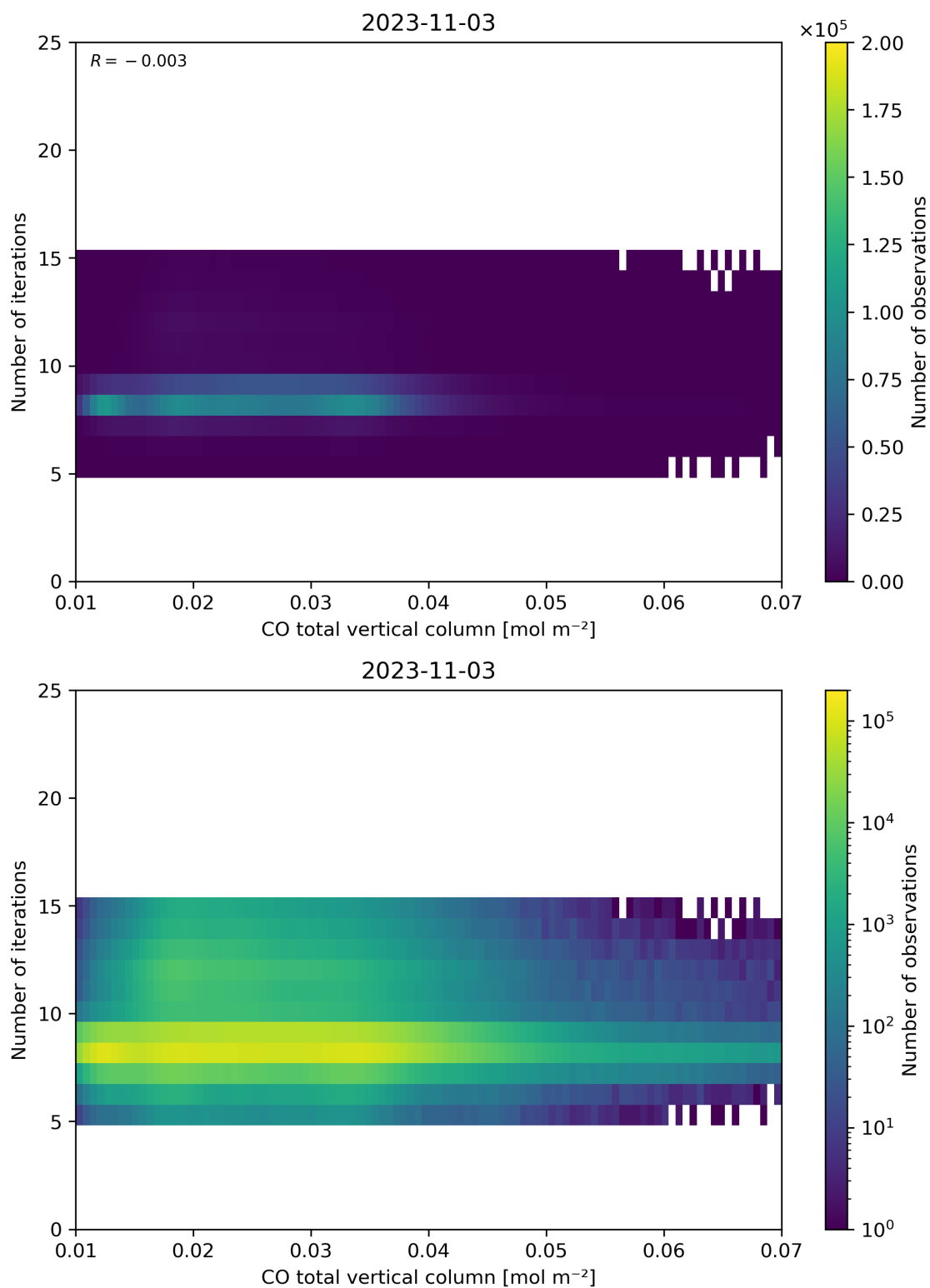
Figure 42: Scatter density plot of “CO total vertical column” against “Number of iterations” for 2023-11-02 to 2023-11-04.
