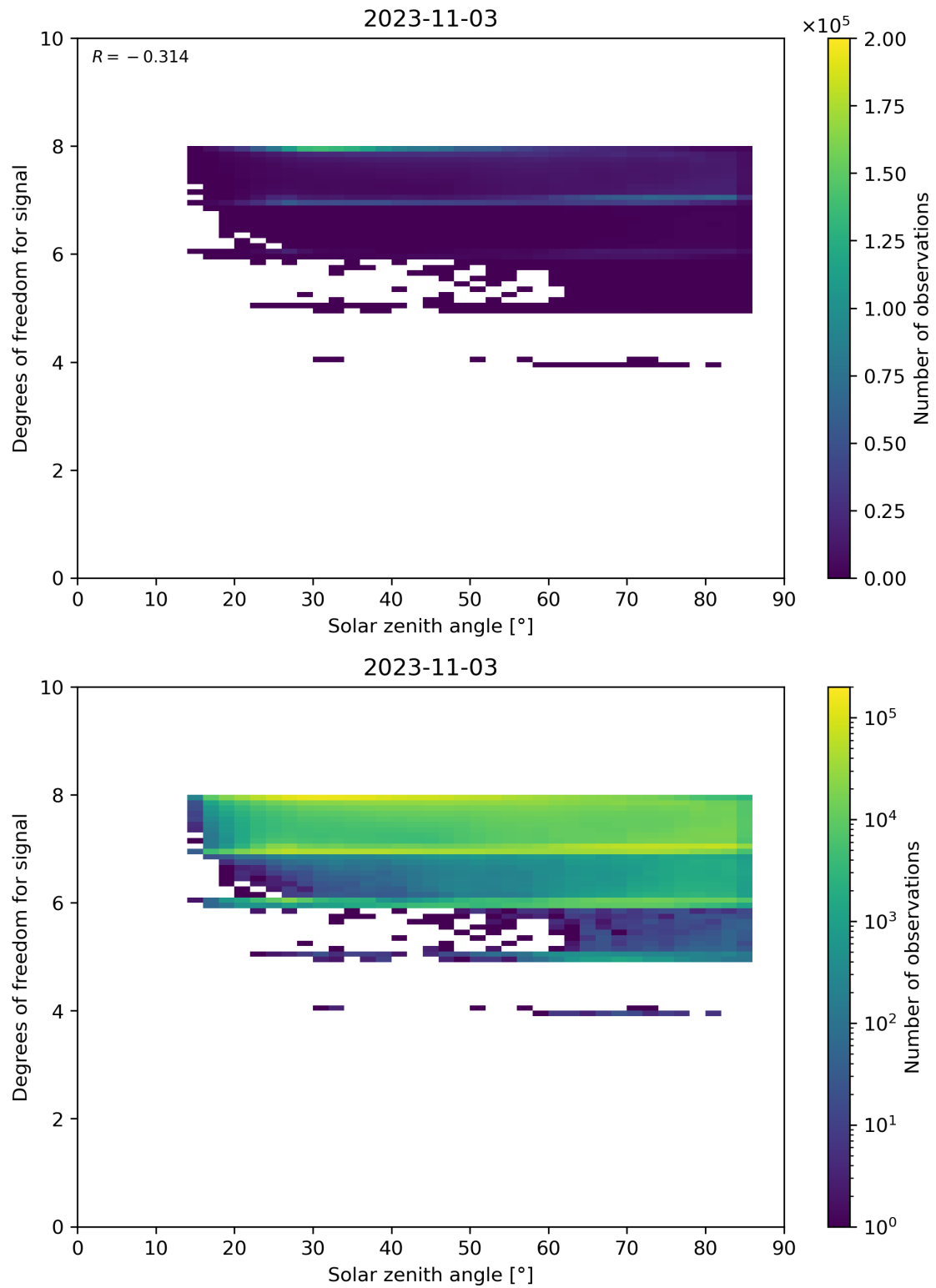
Figure 65: Scatter density plot of “Solar zenith angle” against “Degrees of freedom for signal” for 2023-11-02 to 2023-11-04.
