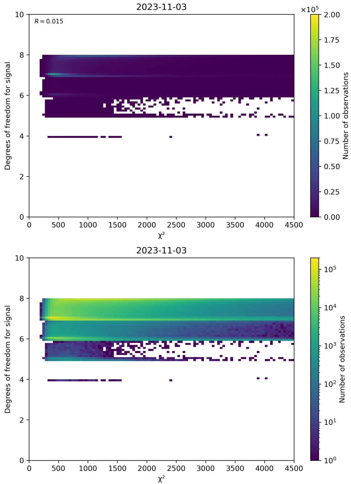
Figure 48: Scatter density plot of “ \chi^2 ” against “Degrees of freedom for signal” for 2023-11-02 to 2023-11-04.
