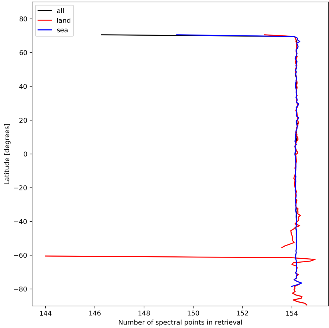
Figure 13: Zonal average of “Number of spectral points in retrieval” for 2023-11-02 to 2023-11-04.
