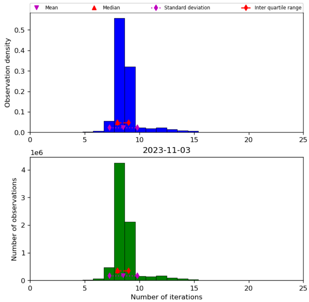
Figure 24: Histogram of “Number of iterations” for 2023-11-02 to 2023-11-04
