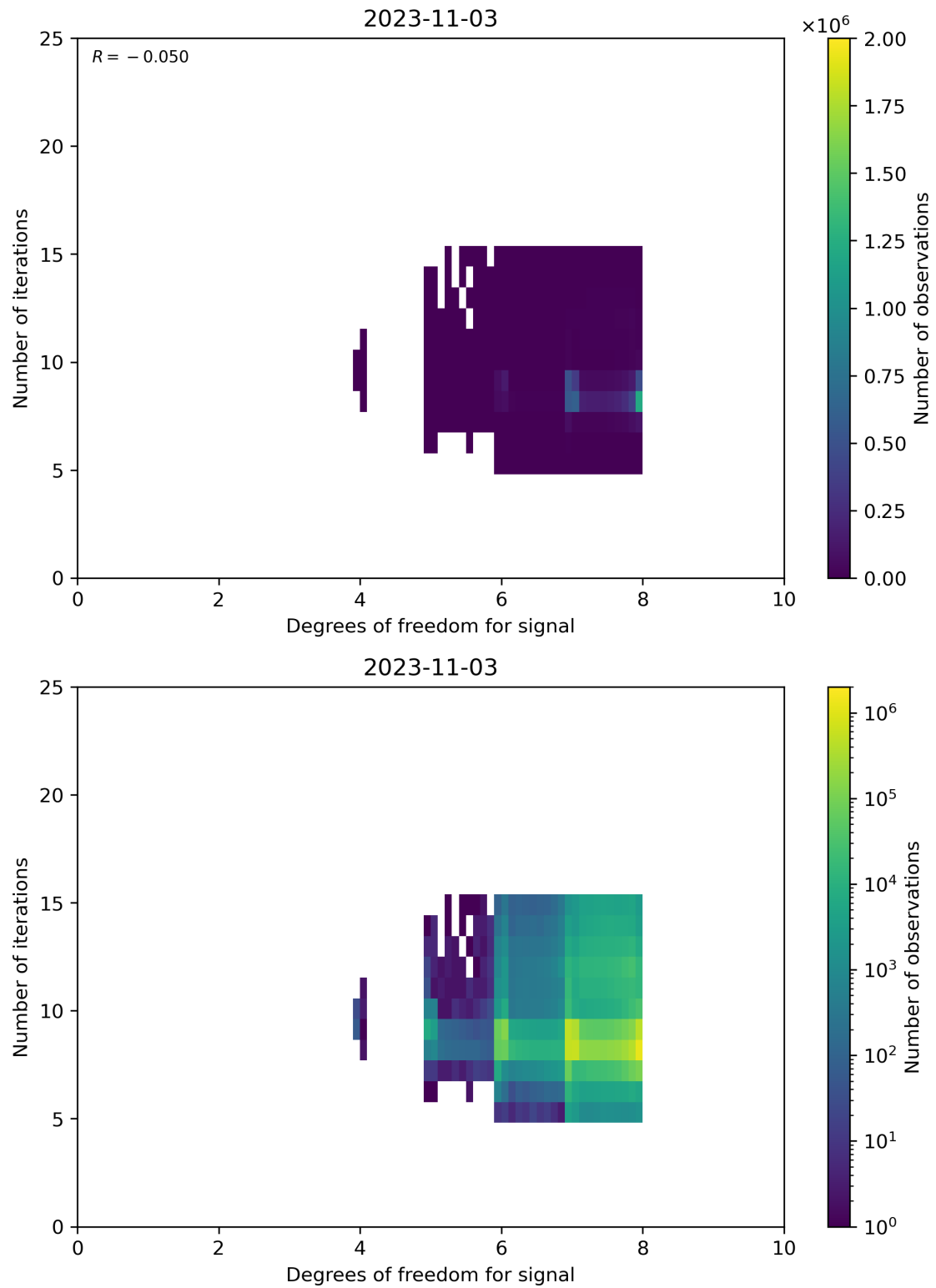
Figure 50: Scatter density plot of “Degrees of freedom for signal” against “Number of iterations” for 2023-11-02 to 2023-11-04.
