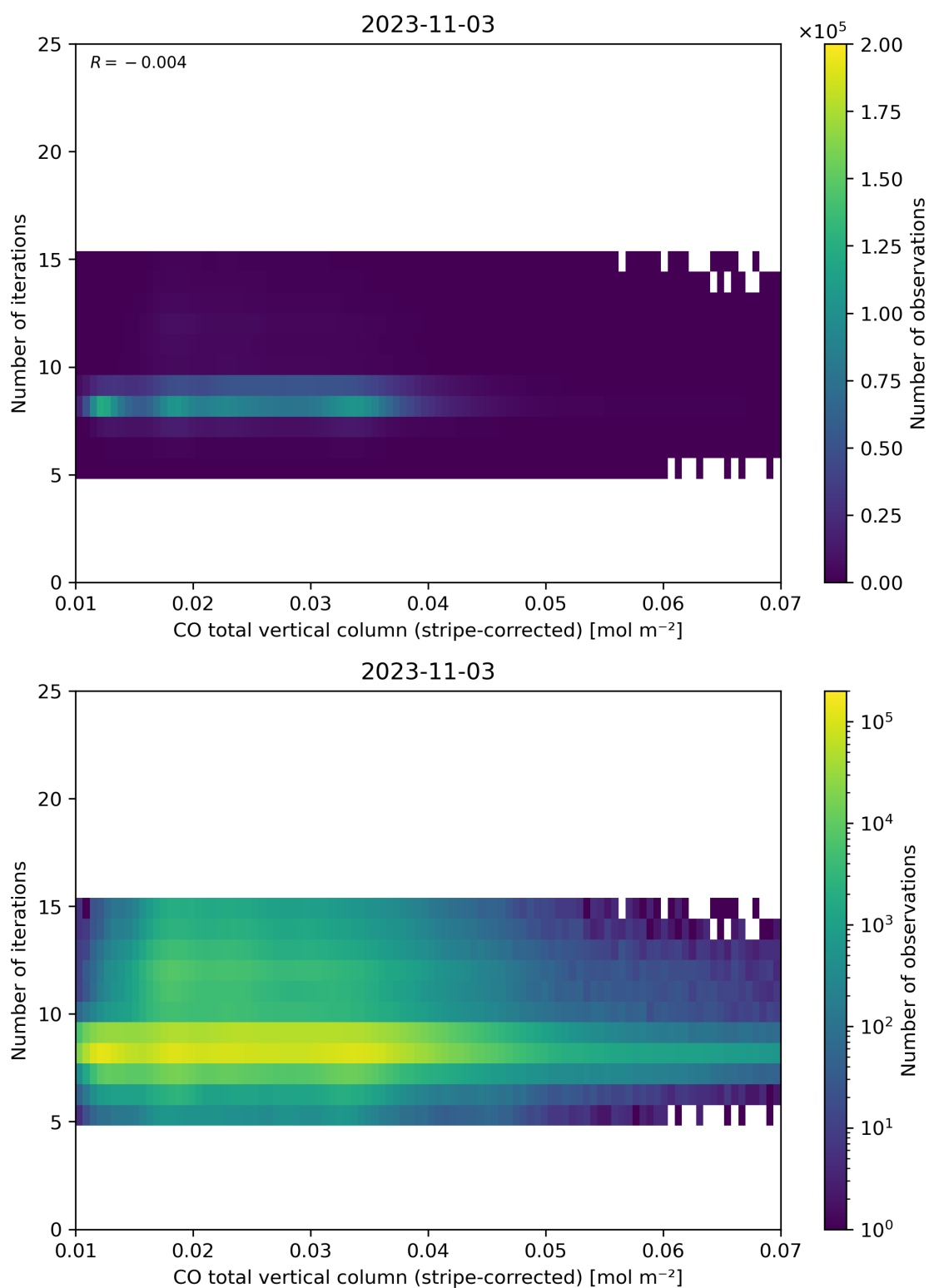
Figure 39: Scatter density plot of “CO total vertical column (stripe-corrected)” against “Number of iterations” for 2023-11-02 to 2023-11-04.
