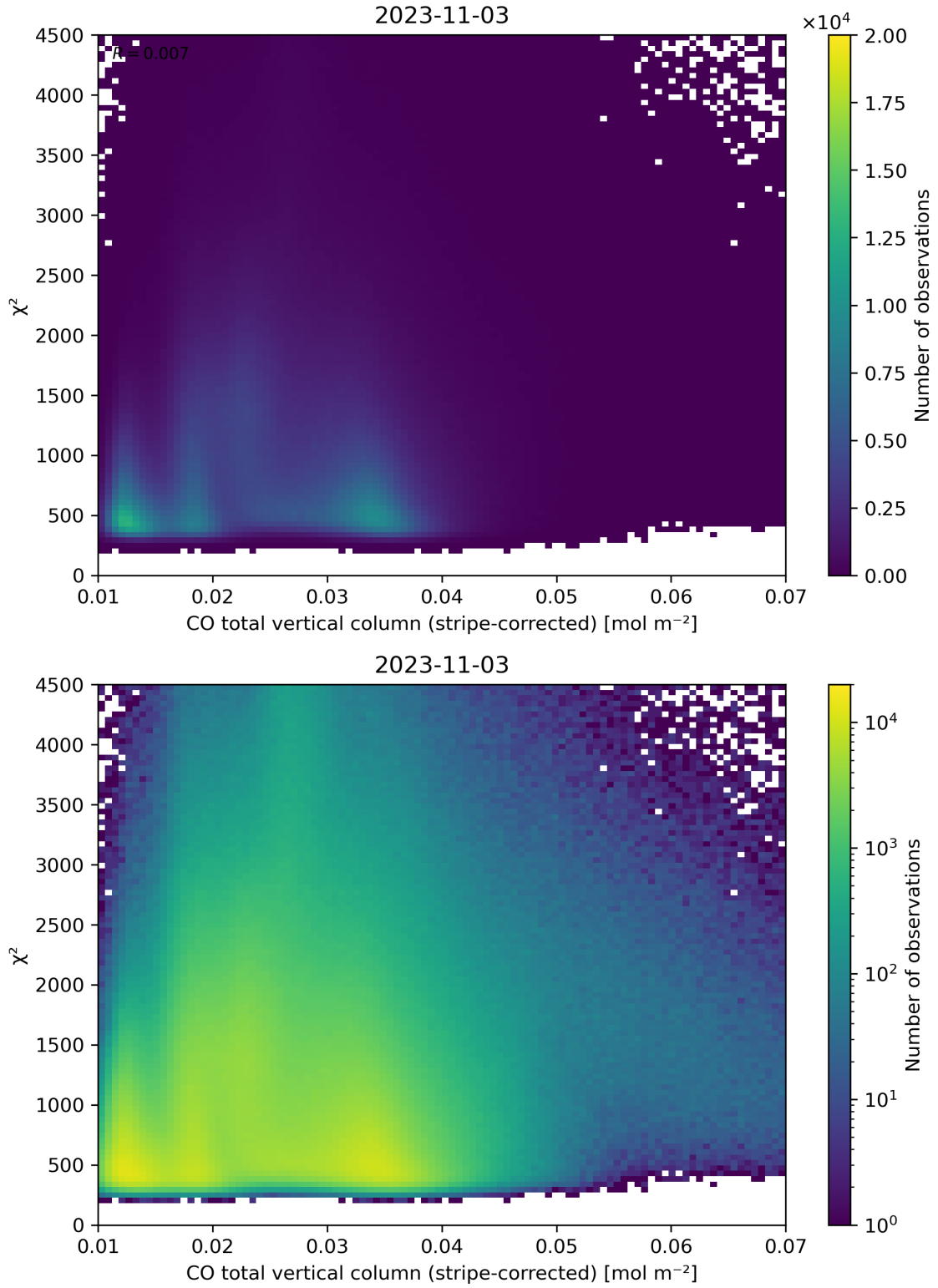
Figure 37: Scatter density plot of “CO total vertical column (stripe-corrected)” against “ \chi^2 ” for 2023-11-02 to 2023-11-04.
