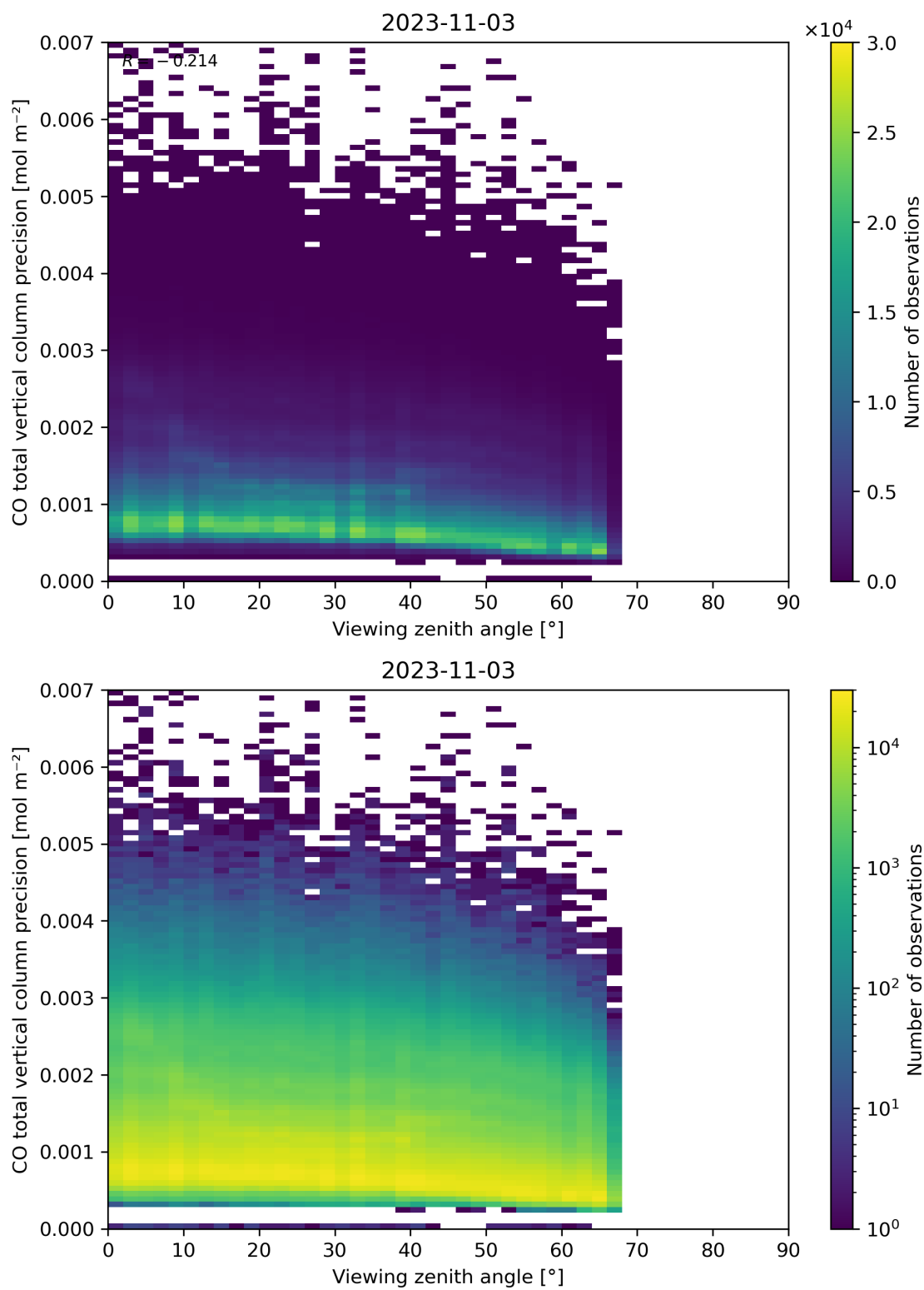
Figure 71: Scatter density plot of “Viewing zenith angle” against “CO total vertical column precision” for 2023-11-02 to 2023-11-04.
