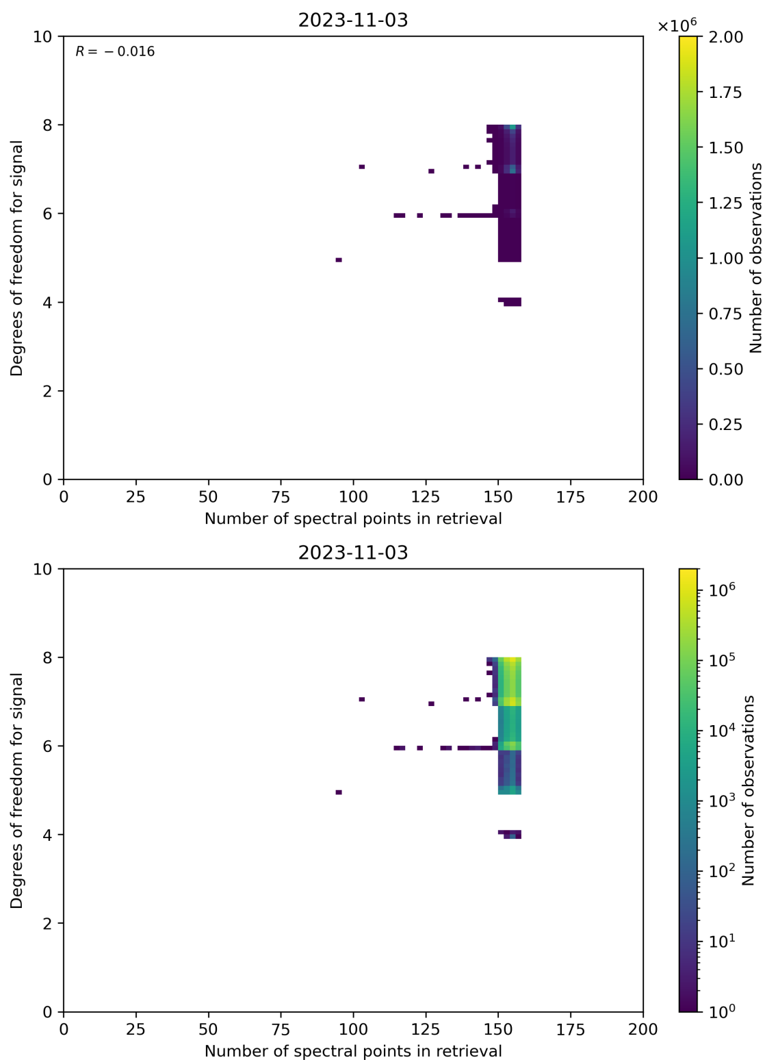
Figure 59: Scatter density plot of “Number of spectral points in retrieval” against “Degrees of freedom for signal” for 2023-11-02 to 2023-11-04.
