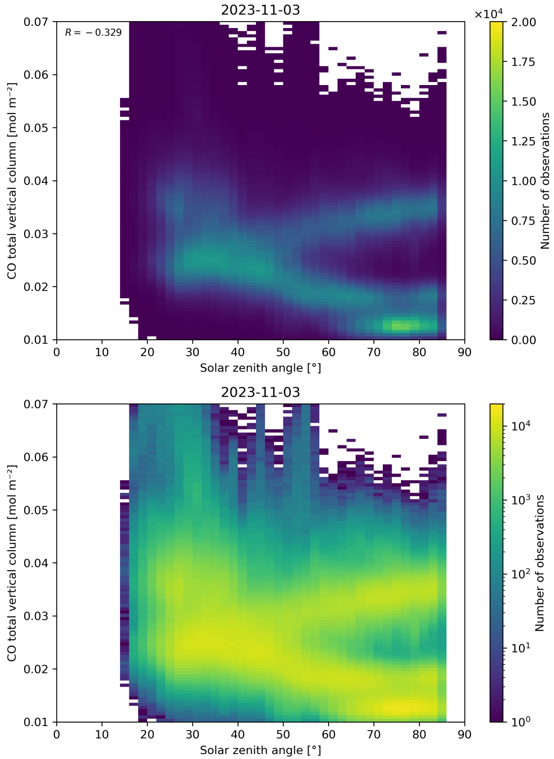
Figure 61: Scatter density plot of “Solar zenith angle” against “CO total vertical column” for 2023-11-02 to 2023-11-04.
