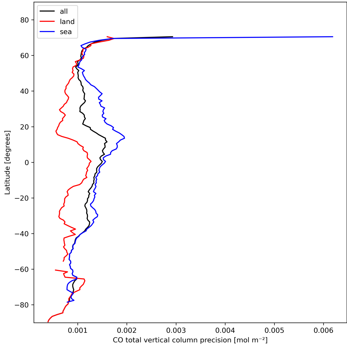
Figure 12: Zonal average of “CO total vertical column precision” for 2023-11-02 to 2023-11-04.
