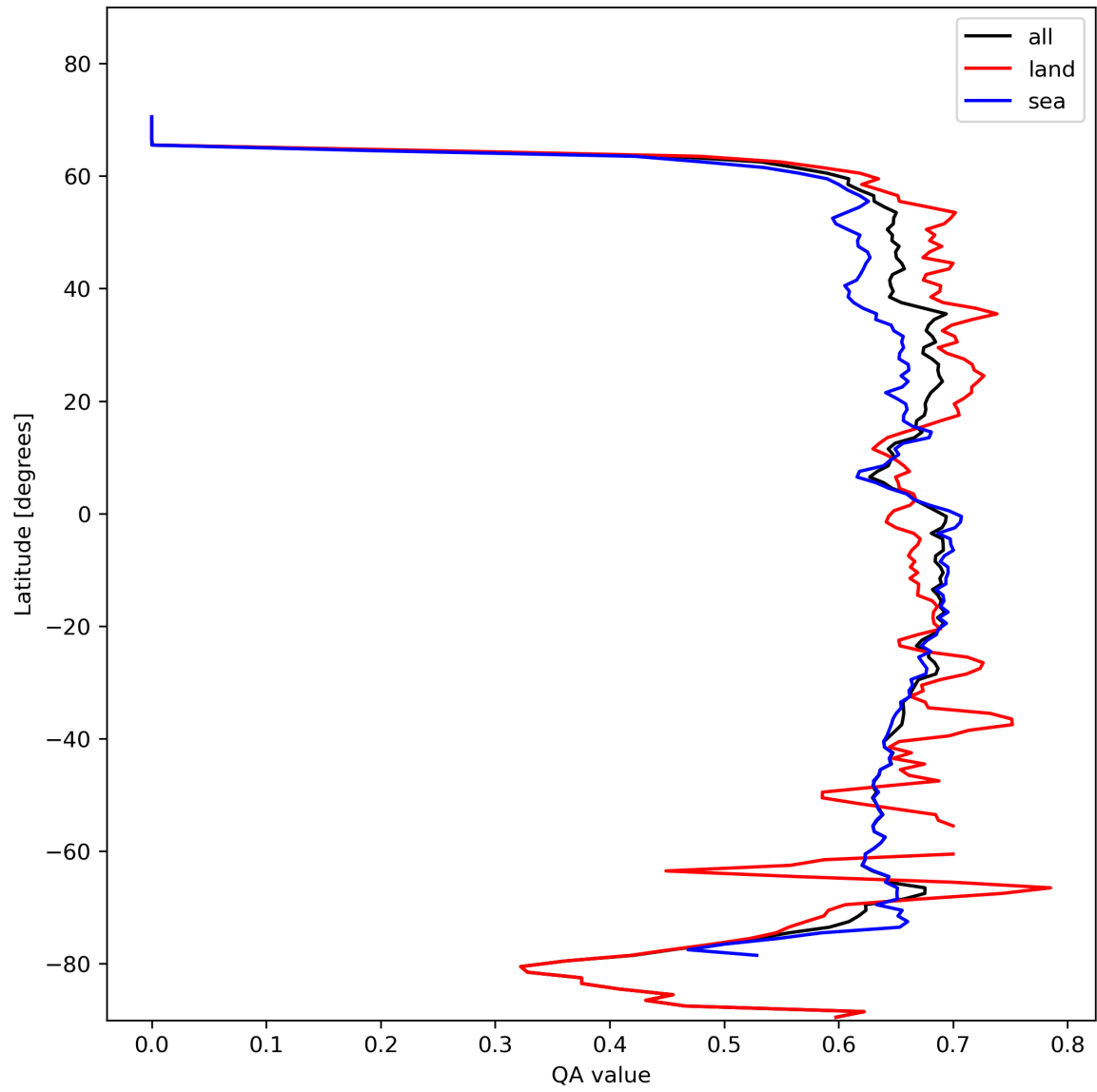
Figure 9: Zonal average of “QA value” for 2023-11-02 to 2023-11-04.
