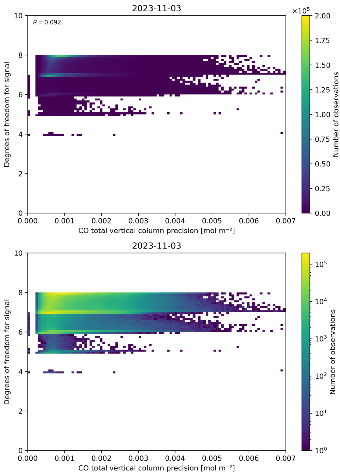
Figure 45: Scatter density plot of “CO total vertical column precision” against “Degrees of freedom for signal” for 2023-11-02 to 2023-11-04.
