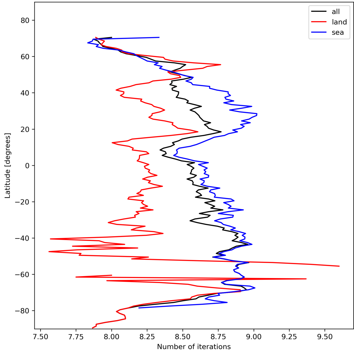
Figure 16: Zonal average of “Number of iterations” for 2023-11-02 to 2023-11-04.
