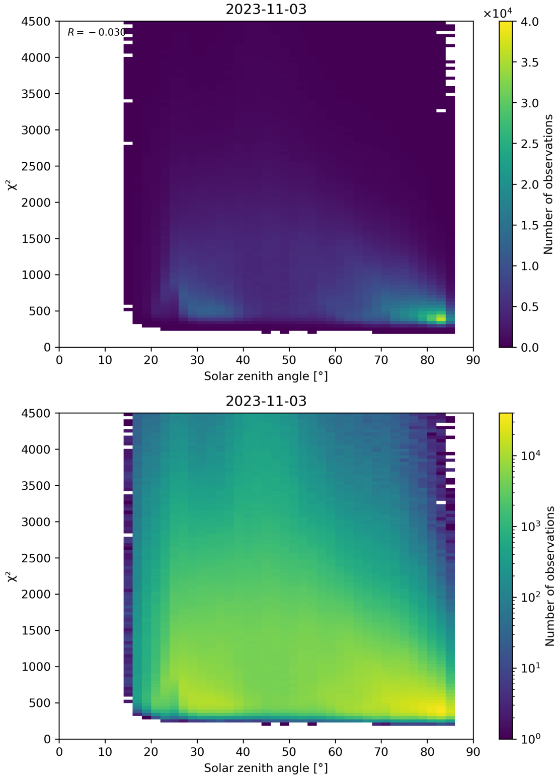
Figure 64: Scatter density plot of “Solar zenith angle” against “ \chi^2 ” for 2023-11-02 to 2023-11-04.
