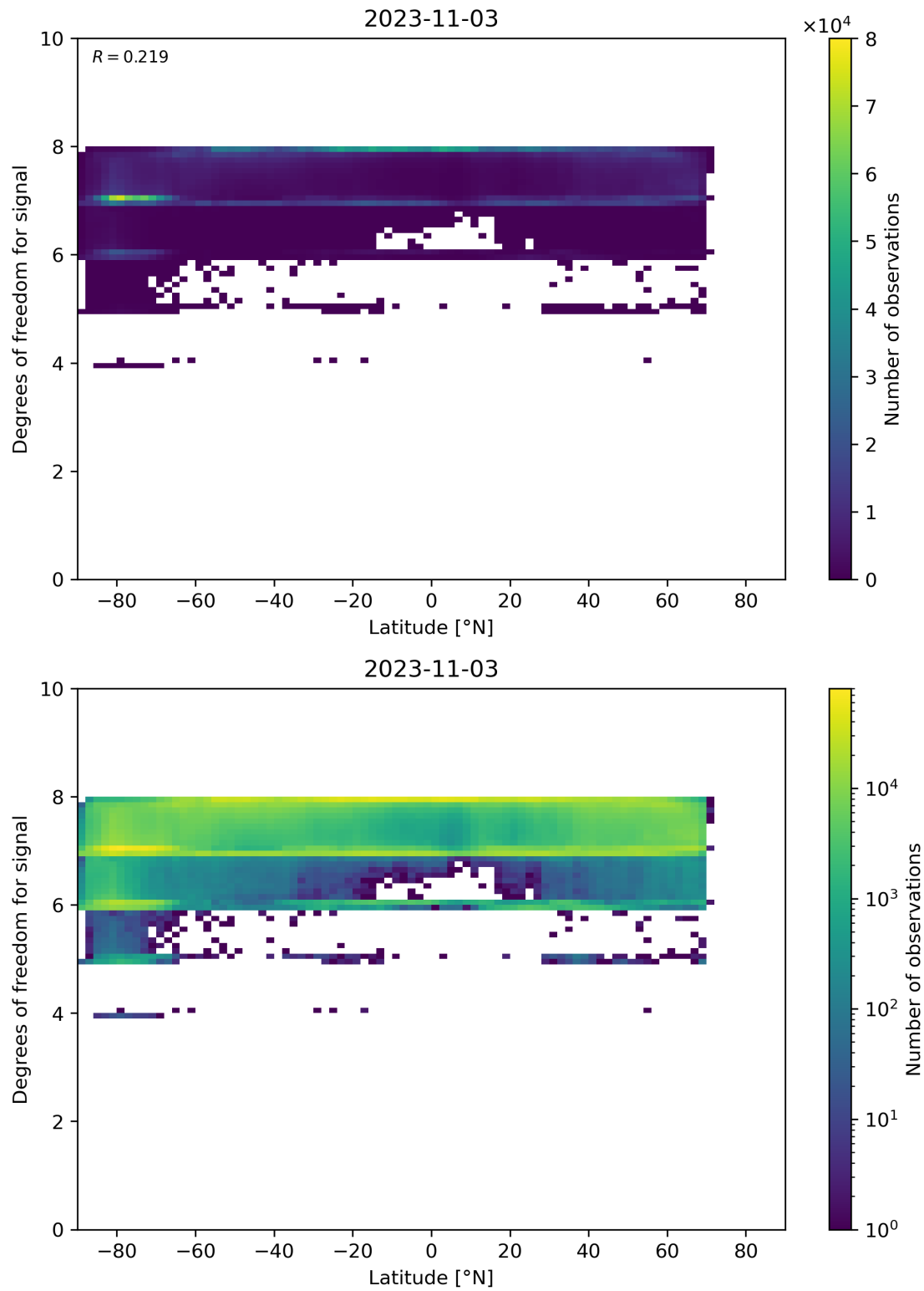
Figure 55: Scatter density plot of “Latitude” against “Degrees of freedom for signal” for 2023-11-02 to 2023-11-04.
