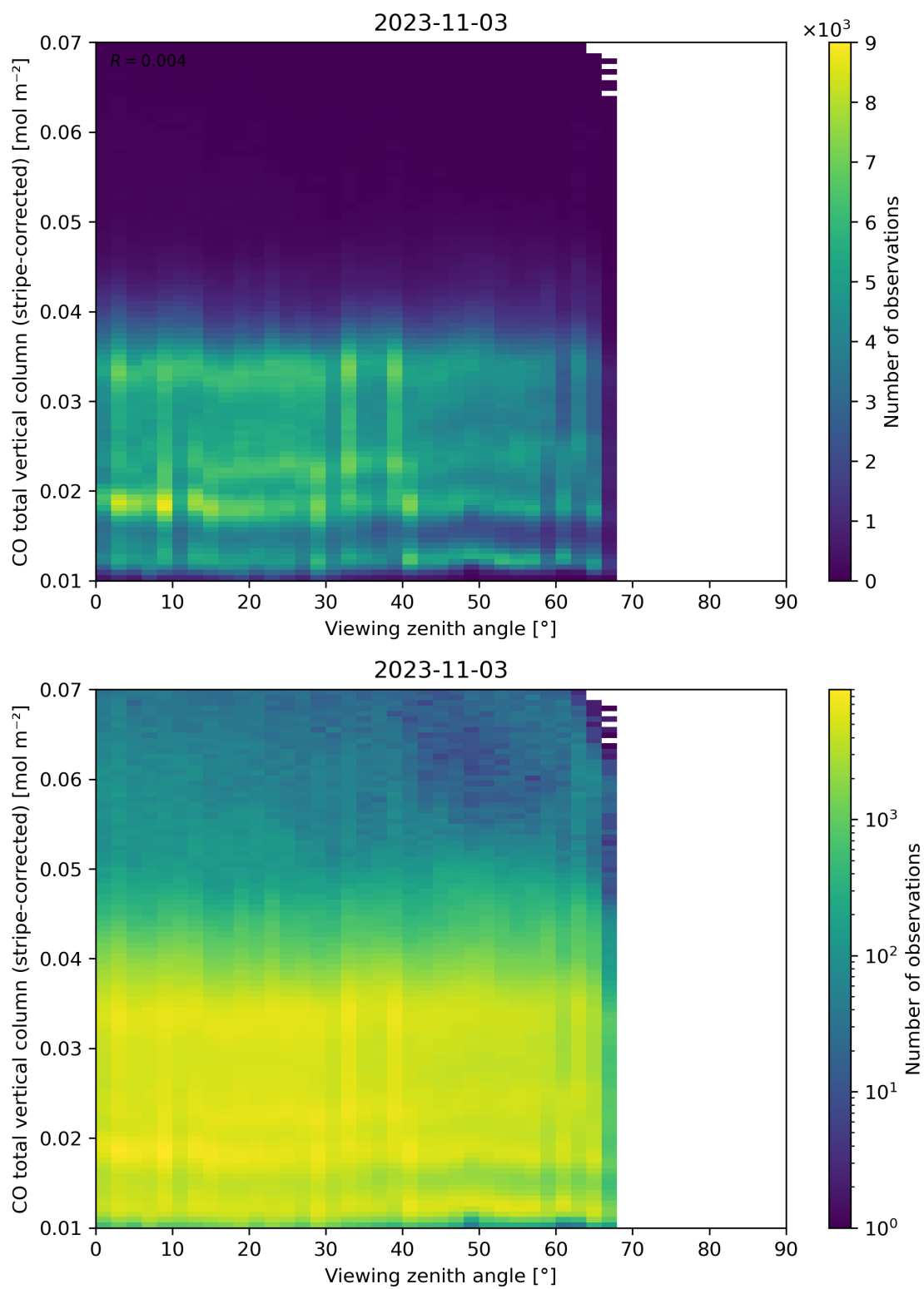
Figure 70: Scatter density plot of “Viewing zenith angle” against “CO total vertical column (stripe-corrected)” for 2023-11-02 to 2023-11-04.
