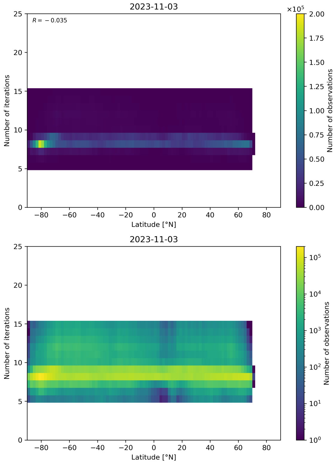
Figure 56: Scatter density plot of “Latitude” against “Number of iterations” for 2023-11-02 to 2023-11-04.
