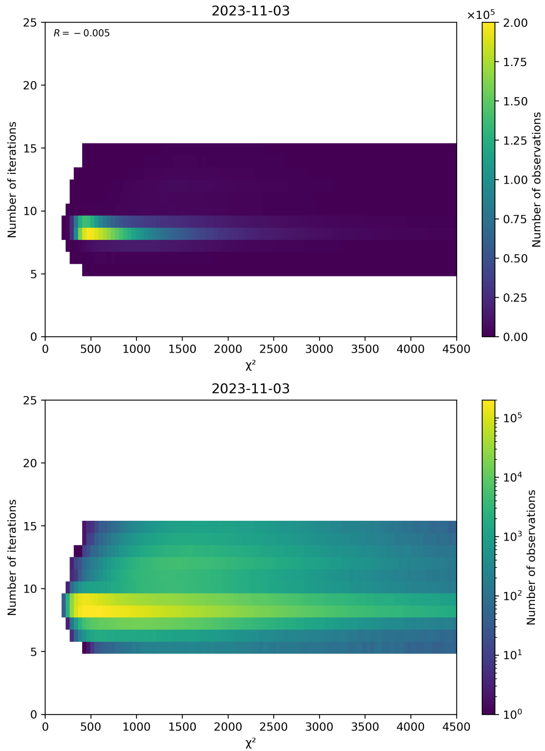
Figure 49: Scatter density plot of “ \chi^2 ” against “Number of iterations” for 2023-11-02 to 2023-11-04.
