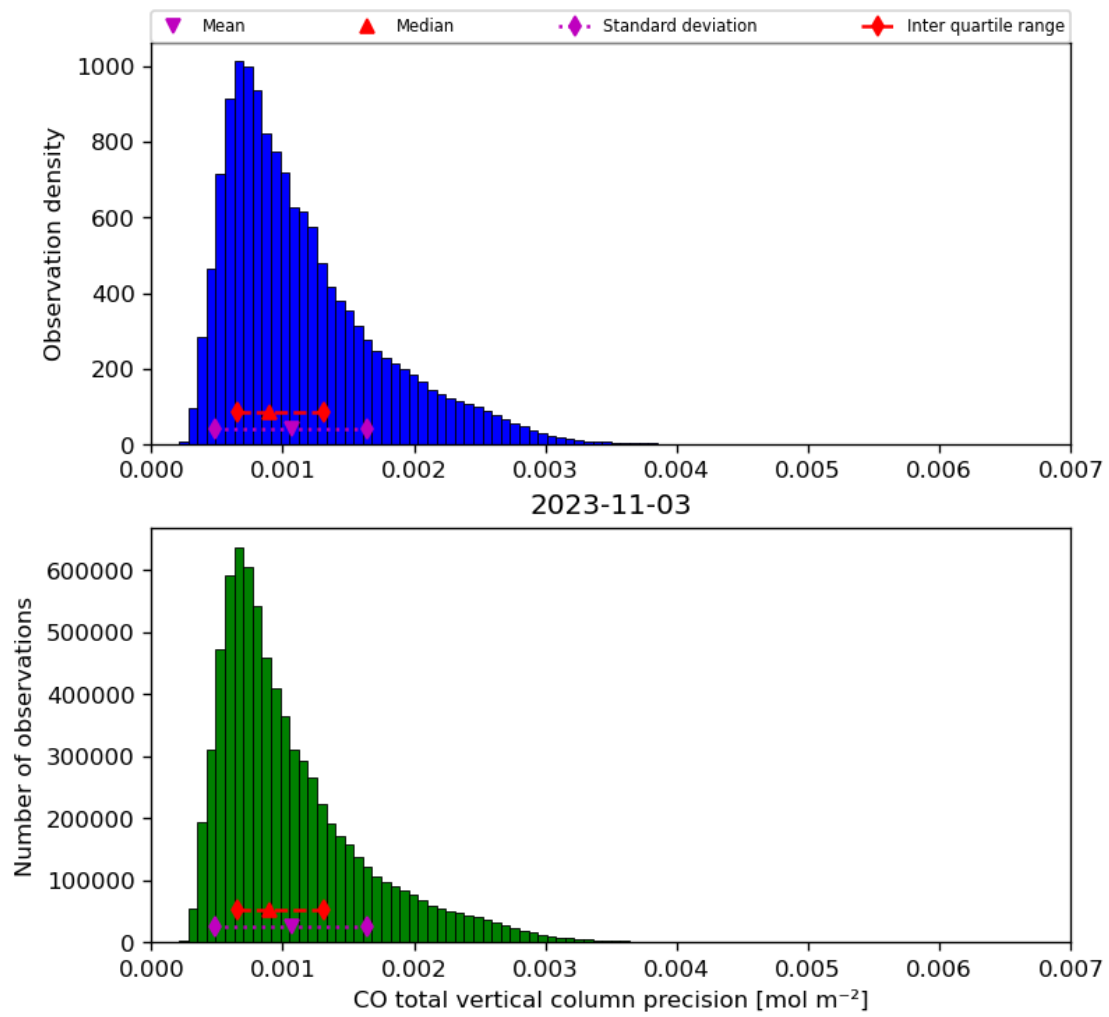
Figure 20: Histogram of “CO total vertical column precision” for 2023-11-02 to 2023-11-04
