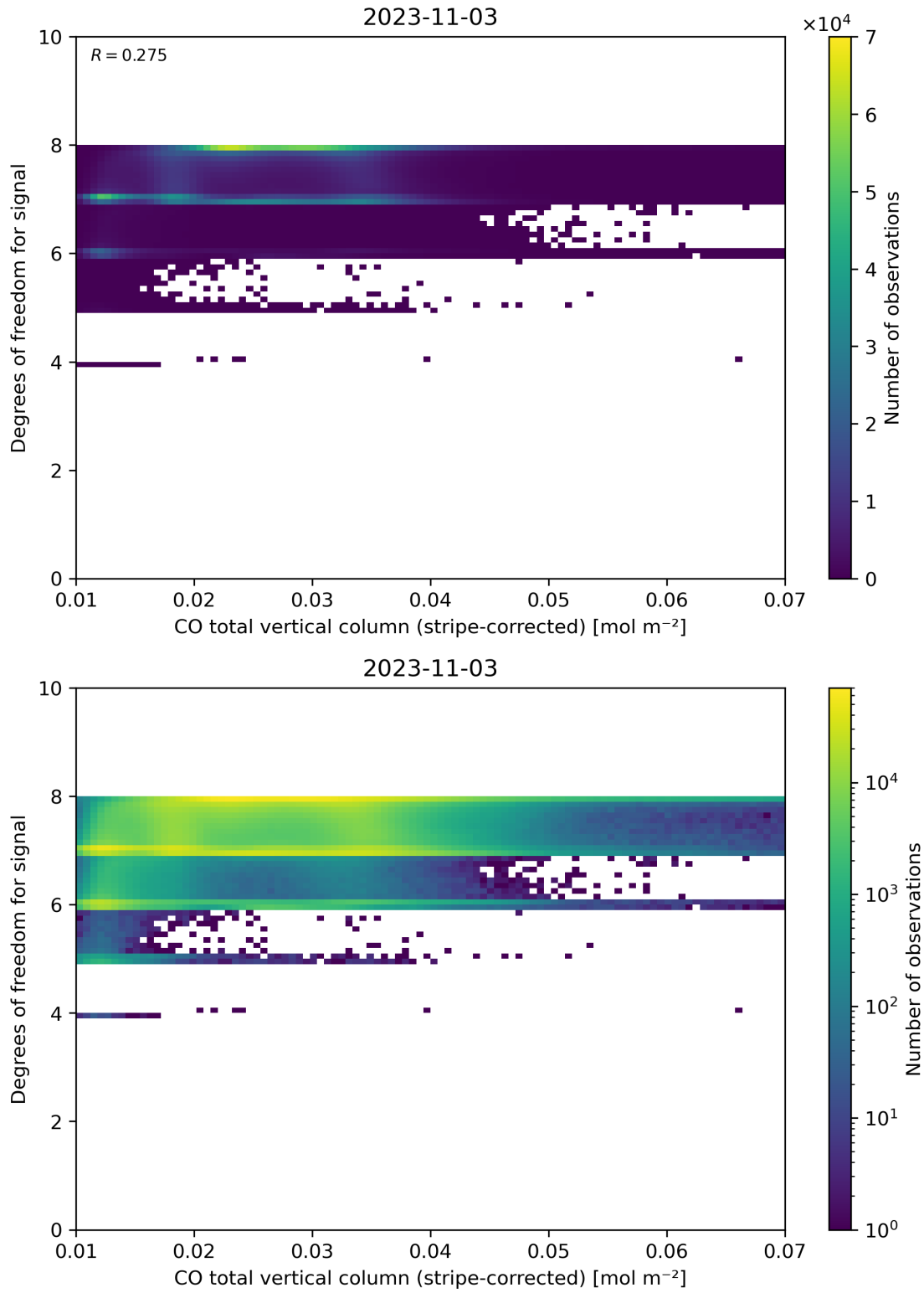
Figure 38: Scatter density plot of “CO total vertical column (stripe-corrected)” against “Degrees of freedom for signal” for 2023-11-02 to 2023-11-04.
