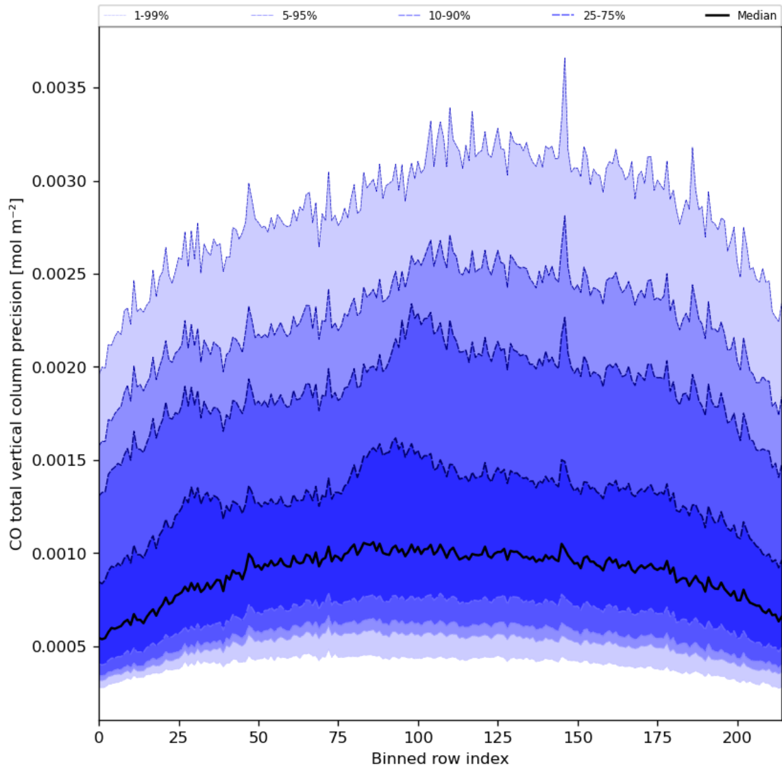
Figure 28: Along track statistics of “CO total vertical column precision” for 2023-11-02 to 2023-11-04
