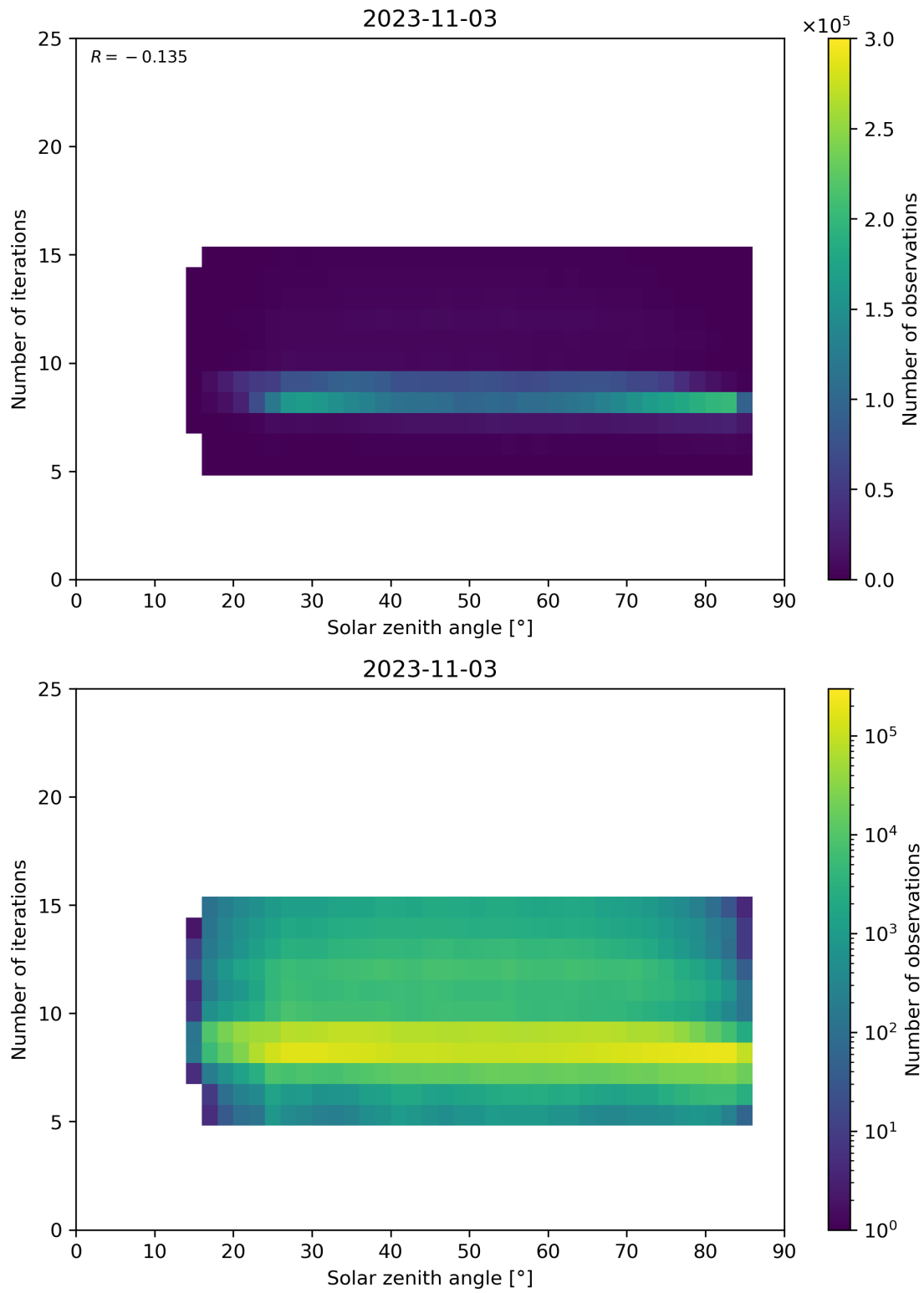
Figure 67: Scatter density plot of “Solar zenith angle” against “Number of iterations” for 2023-11-02 to 2023-11-04.
