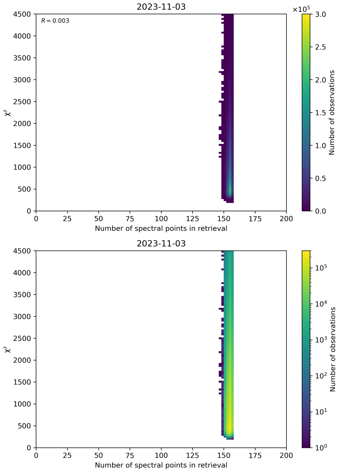
Figure 58: Scatter density plot of “Number of spectral points in retrieval” against “ \chi^2 ” for 2023-11-02 to 2023-11-04.
