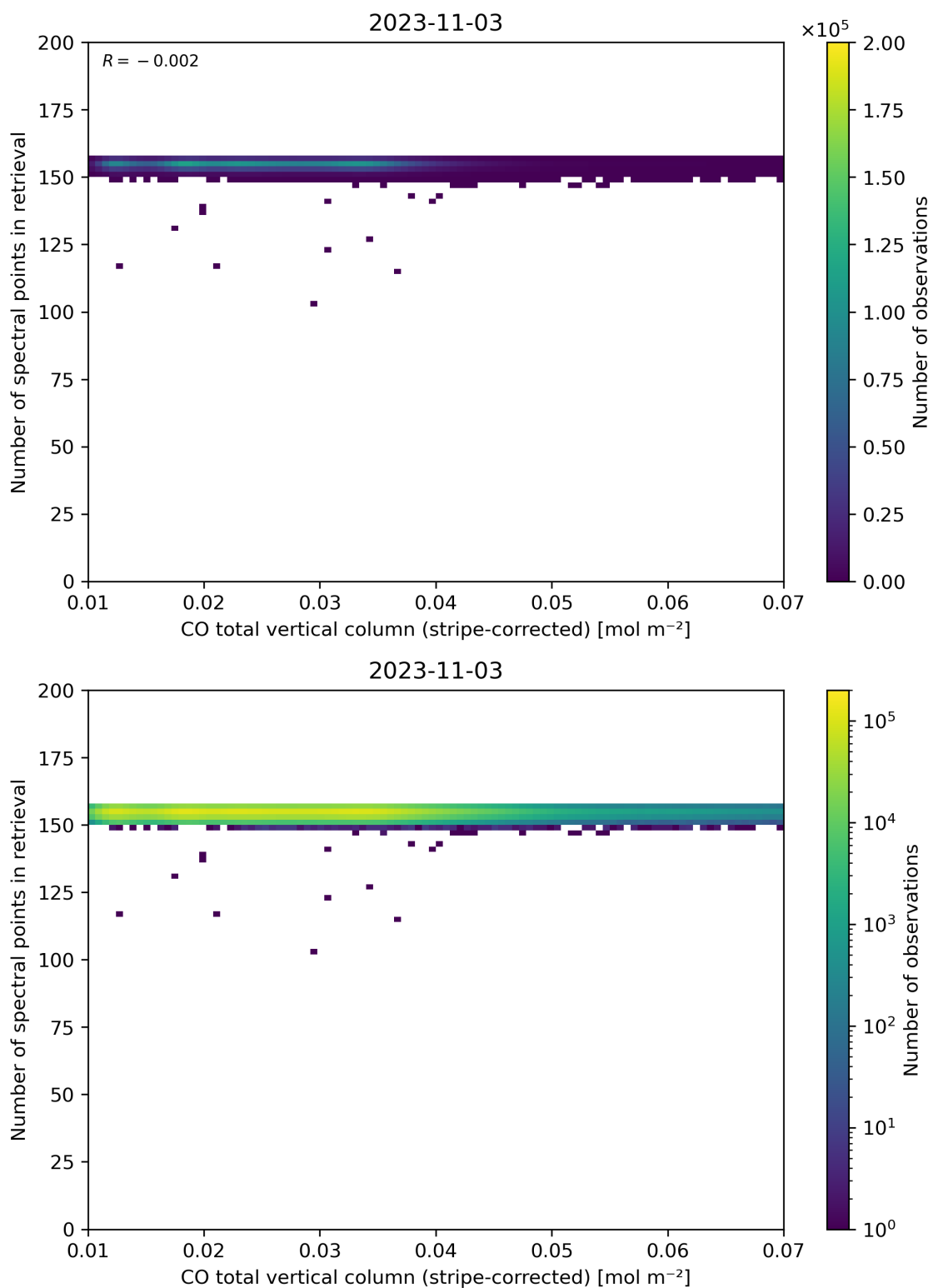
Figure 40: Scatter density plot of “CO total vertical column (stripe-corrected)” against “Number of spectral points in retrieval” for 2023-11-02 to 2023-11-04.
