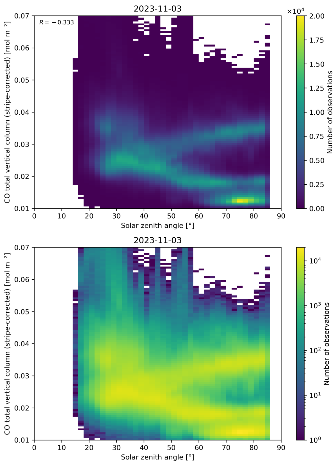
Figure 62: Scatter density plot of “Solar zenith angle” against “CO total vertical column (stripe-corrected)” for 2023-11-02 to 2023-11-04.
