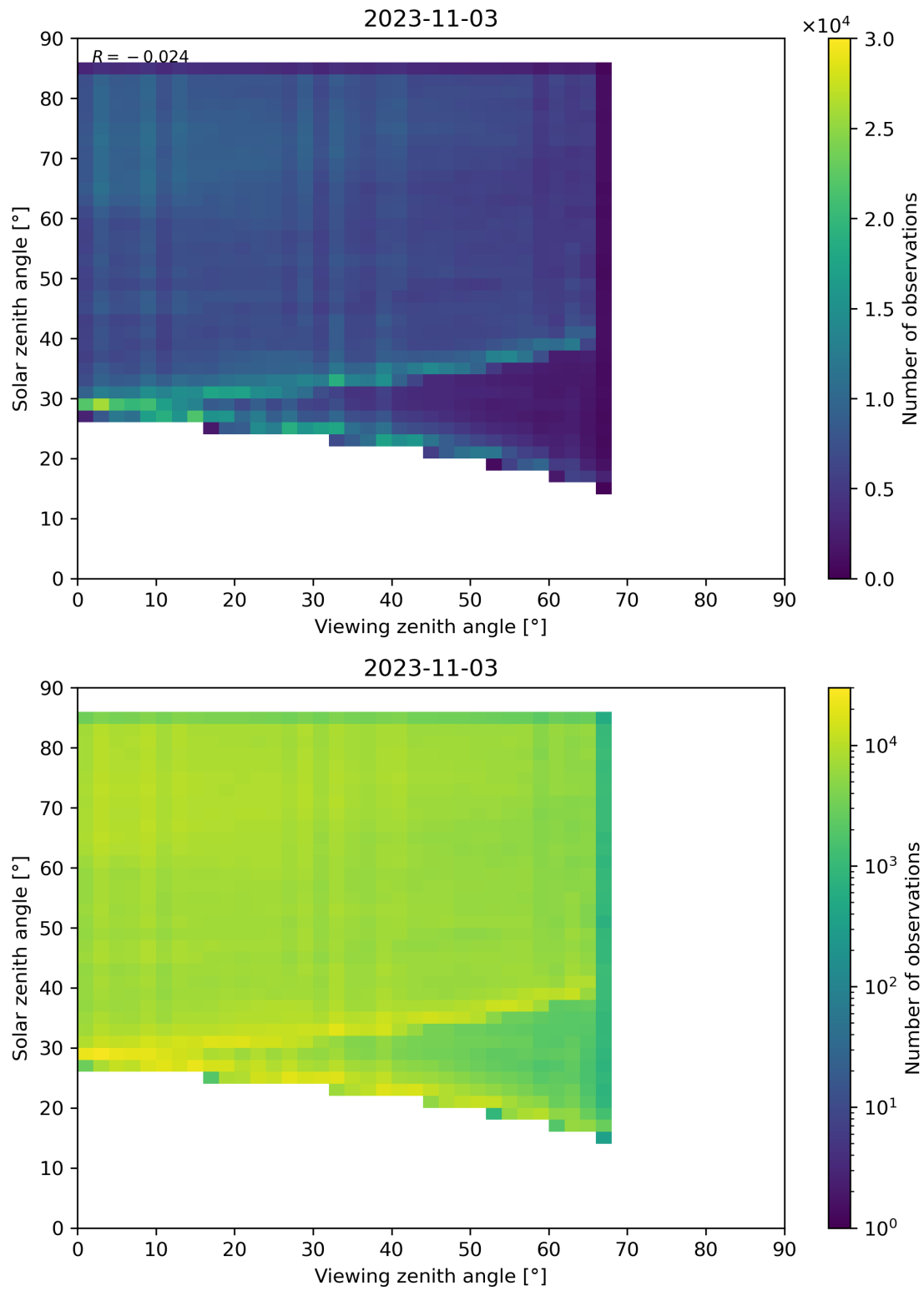
Figure 77: Scatter density plot of “Viewing zenith angle” against “Solar zenith angle” for 2023-11-02 to 2023-11-04.
