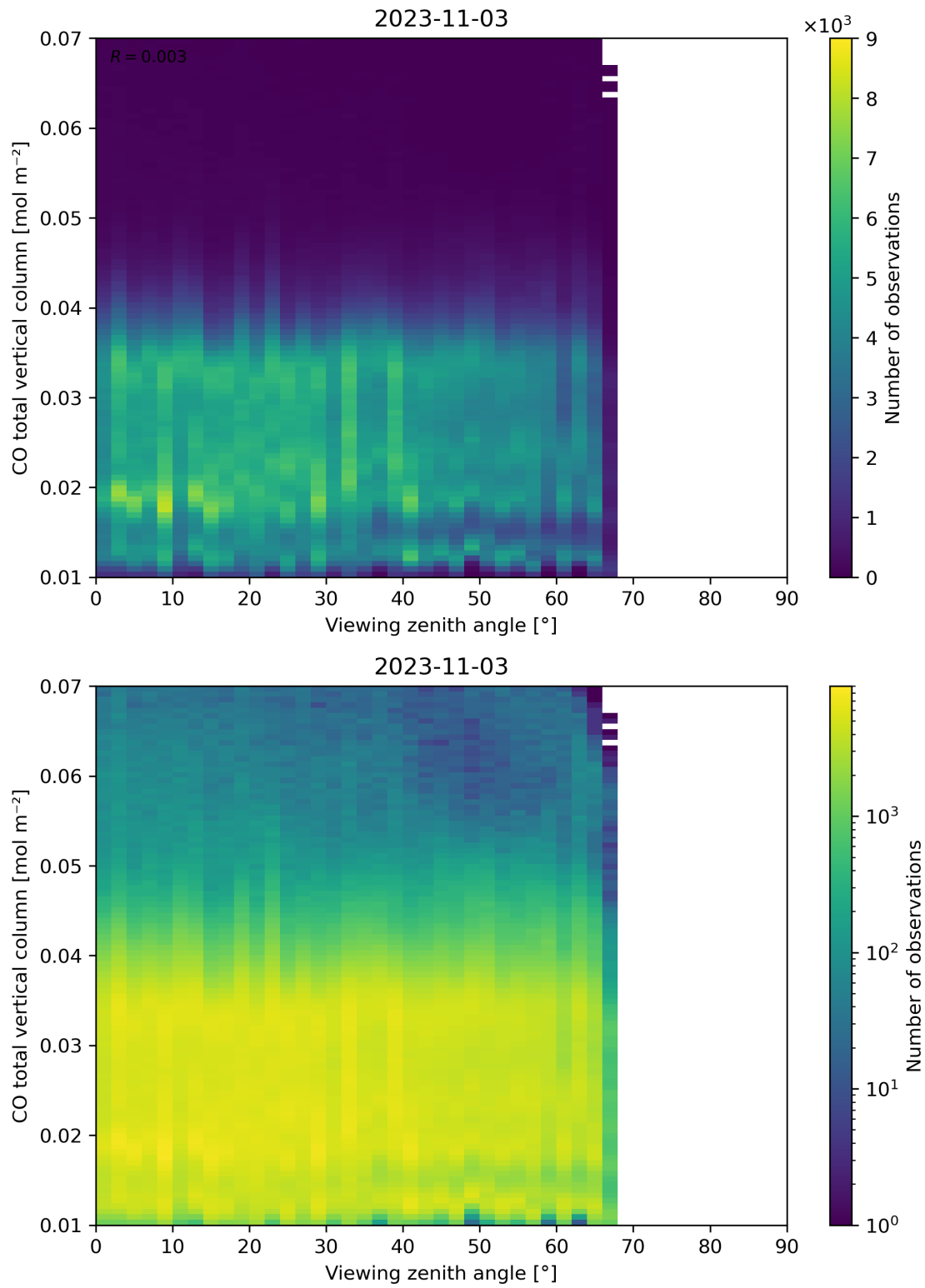
Figure 69: Scatter density plot of “Viewing zenith angle” against “CO total vertical column” for 2023-11-02 to 2023-11-04.
