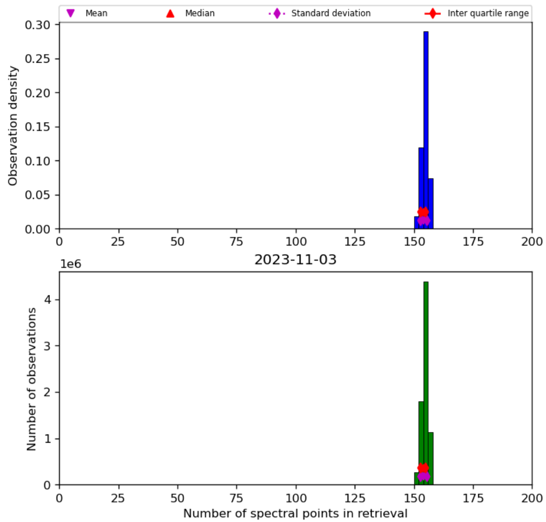
Figure 21: Histogram of “Number of spectral points in retrieval” for 2023-11-02 to 2023-11-04
