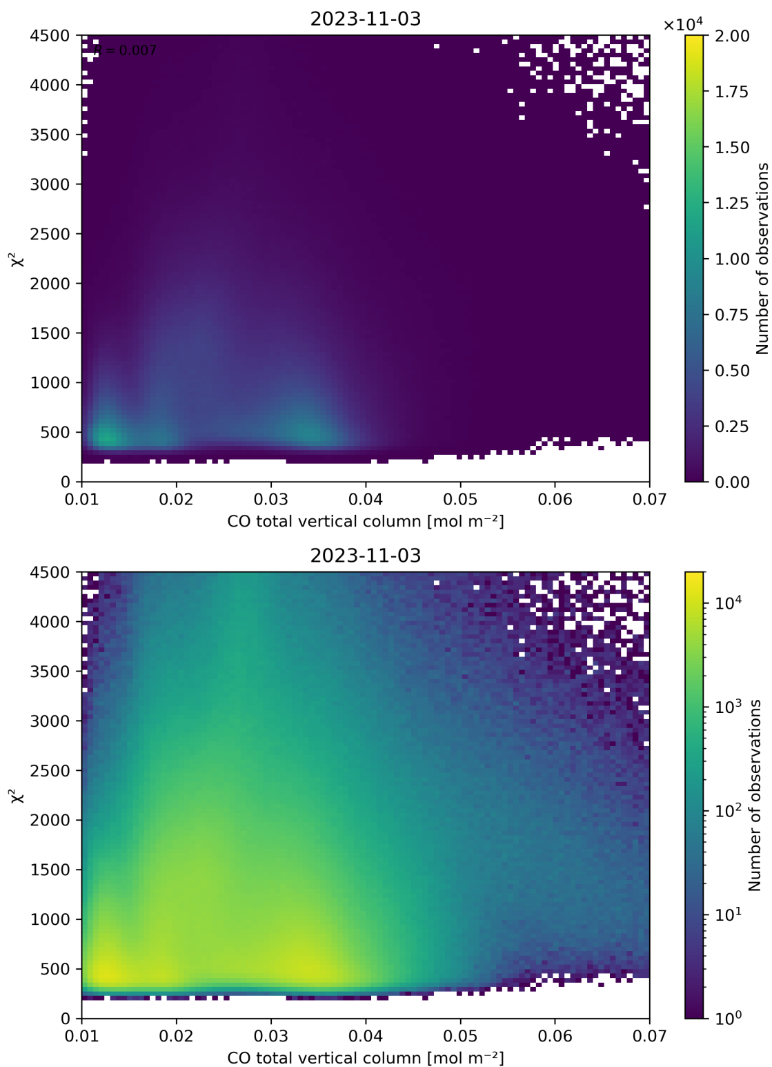
Figure 35: Scatter density plot of “CO total vertical column” against “ \chi^2 ” for 2023-11-02 to 2023-11-04.
