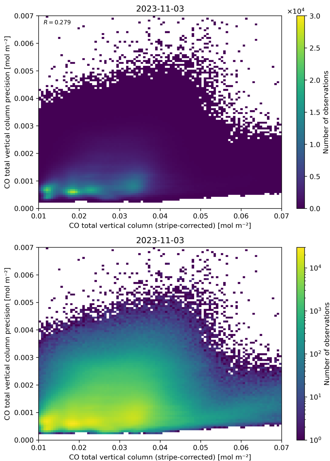
Figure 36: Scatter density plot of “CO total vertical column (stripe-corrected)” against “CO total vertical column precision” for 2023-11-02 to 2023-11-04.
