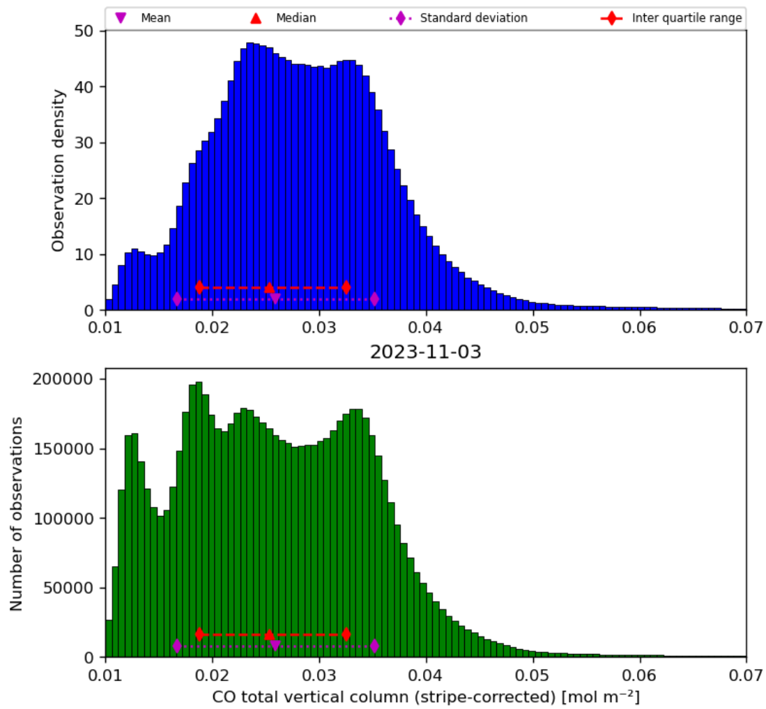
Figure 19: Histogram of “CO total vertical column (stripe-corrected)” for 2023-11-02 to 2023-11-04
