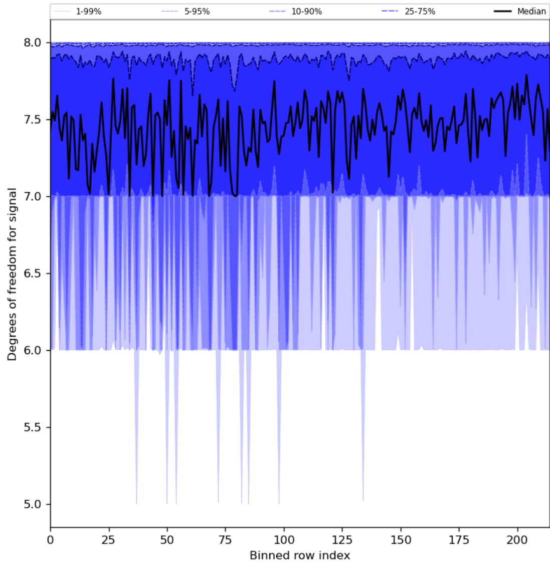
Figure 31: Along track statistics of “Degrees of freedom for signal” for 2023-11-02 to 2023-11-04
