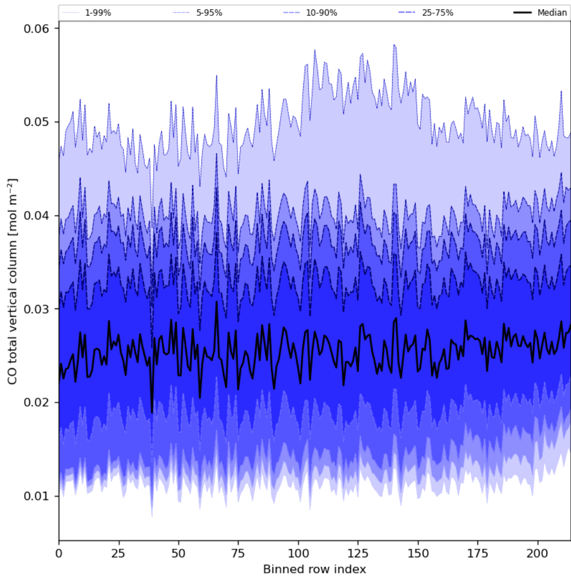
Figure 26: Along track statistics of “CO total vertical column” for 2023-11-02 to 2023-11-04
