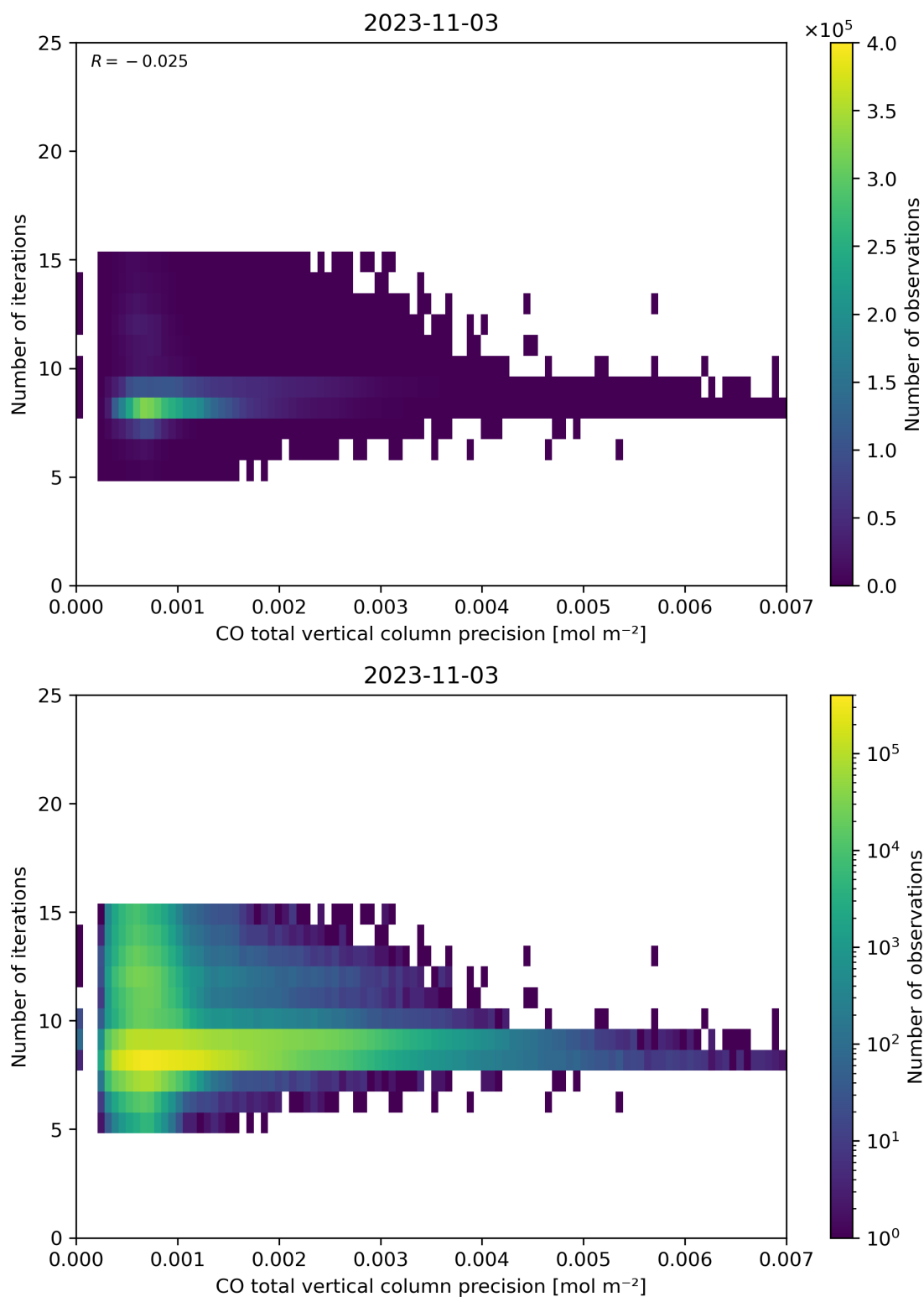
Figure 46: Scatter density plot of “CO total vertical column precision” against “Number of iterations” for 2023-11-02 to 2023-11-04.
