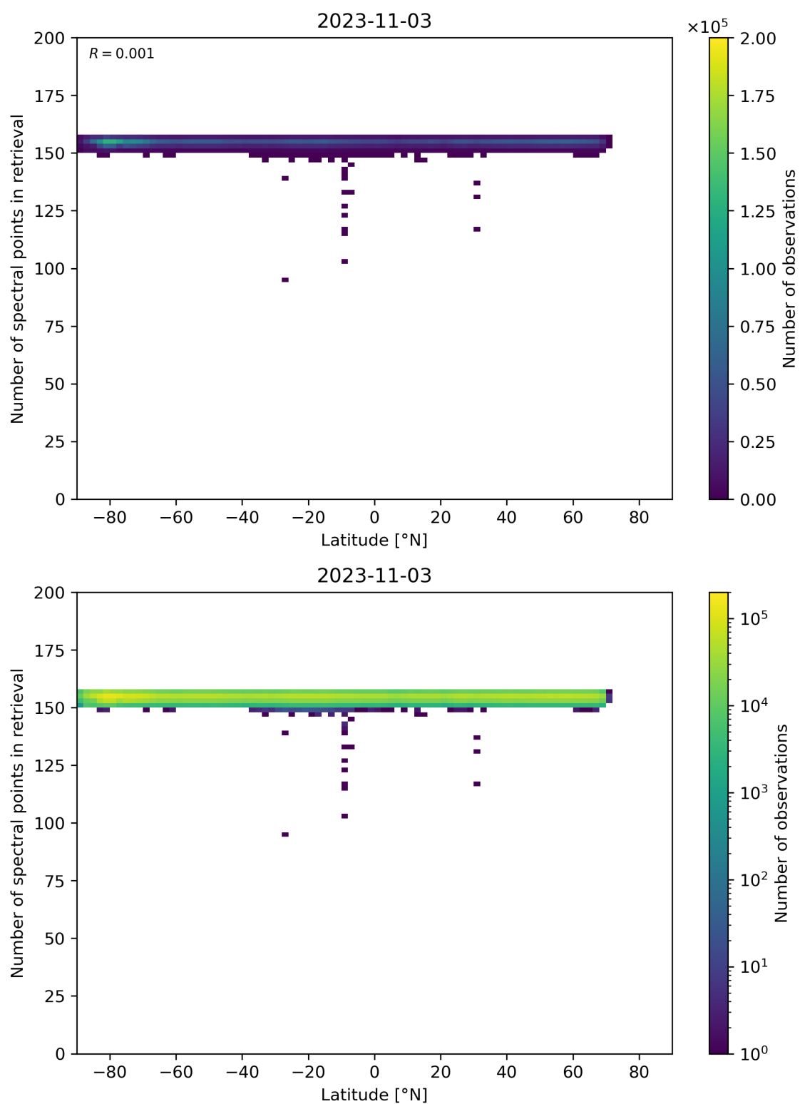
Figure 57: Scatter density plot of “Latitude” against “Number of spectral points in retrieval” for 2023-11-02 to 2023-11-04.
