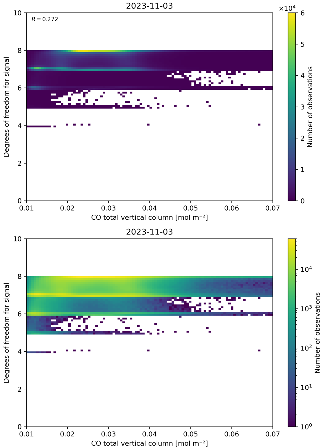
Figure 41: Scatter density plot of “CO total vertical column” against “Degrees of freedom for signal” for 2023-11-02 to 2023-11-04.
