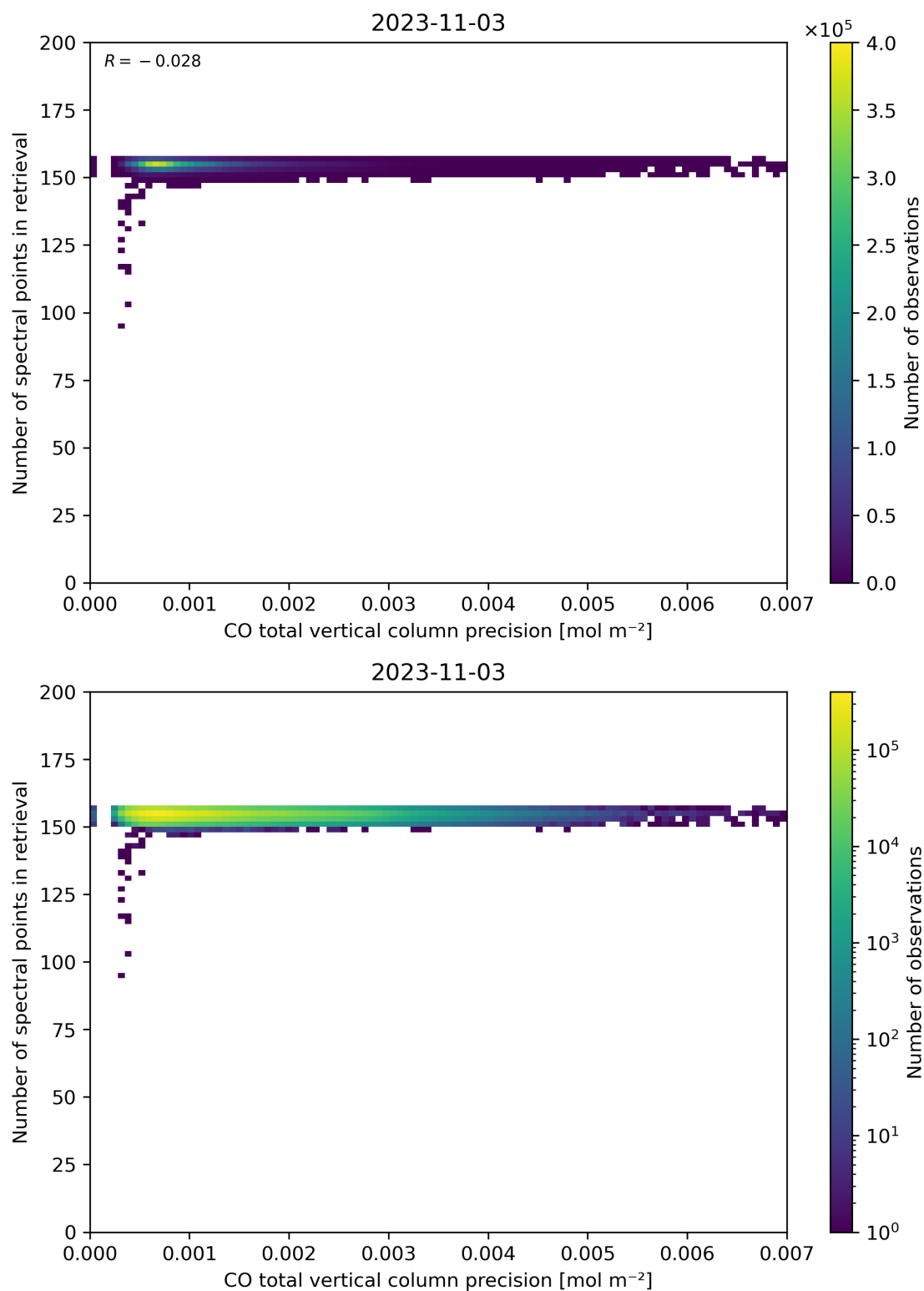
Figure 47: Scatter density plot of “CO total vertical column precision” against “Number of spectral points in retrieval” for 2023-11-02 to 2023-11-04.
