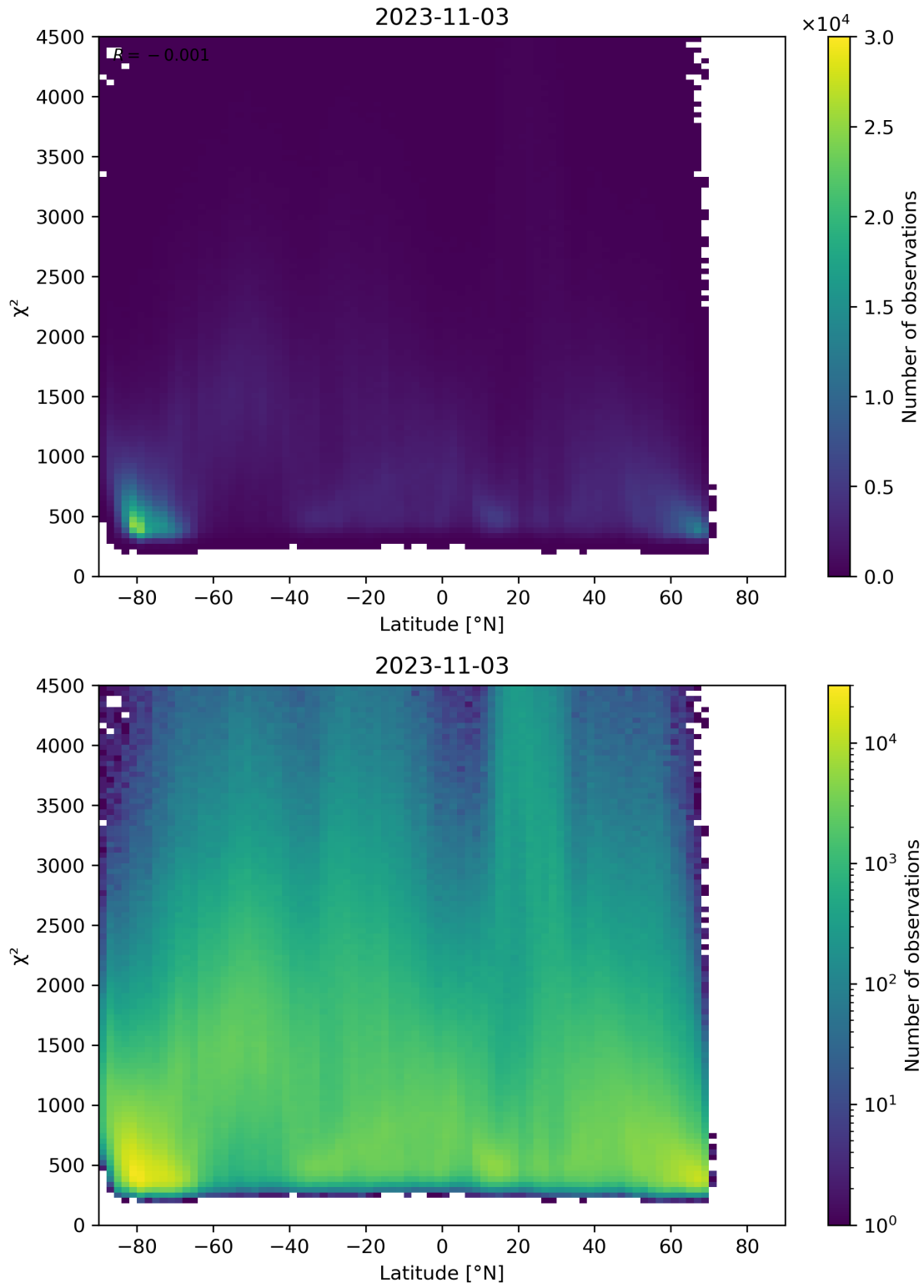
Figure 54: Scatter density plot of “Latitude” against “ \chi^2 ” for 2023-11-02 to 2023-11-04.
