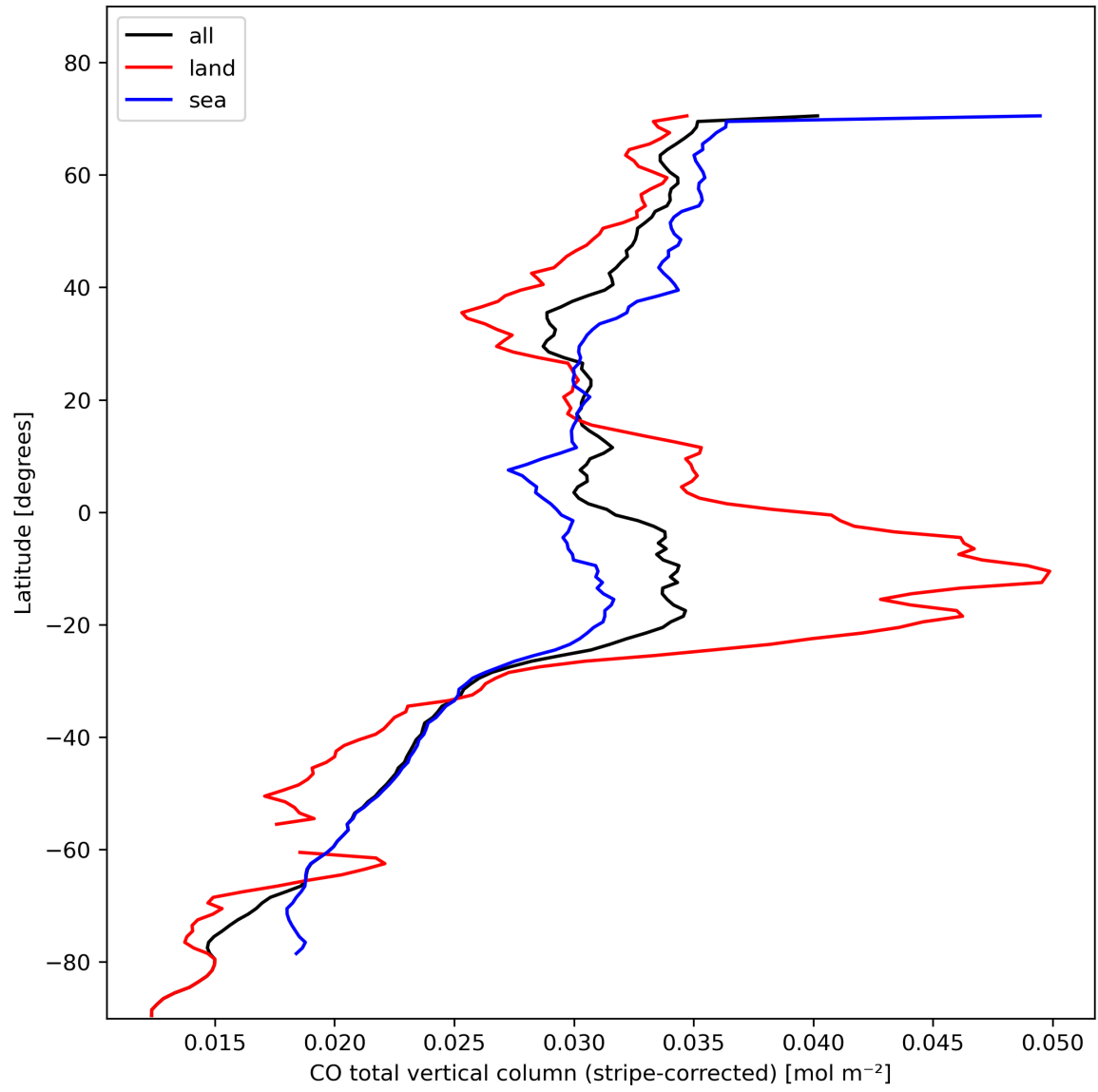
Figure 11: Zonal average of “CO total vertical column (stripe-corrected)” for 2023-11-02 to 2023-11-04.
