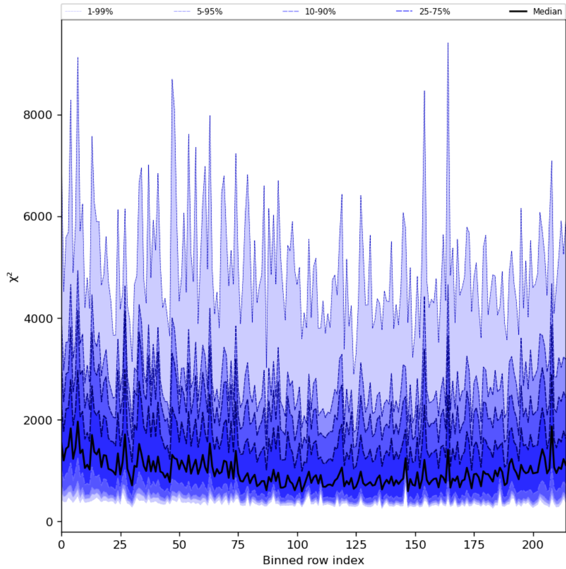
Figure 30: Along track statistics of “ \chi^2 ” for 2023-11-02 to 2023-11-04
