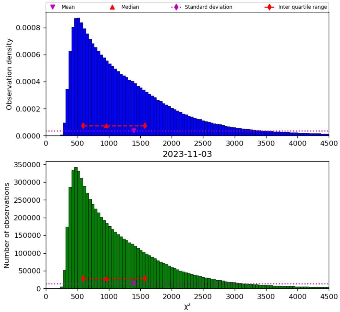
Figure 22: Histogram of “ \chi^2 ” for 2023-11-02 to 2023-11-04
