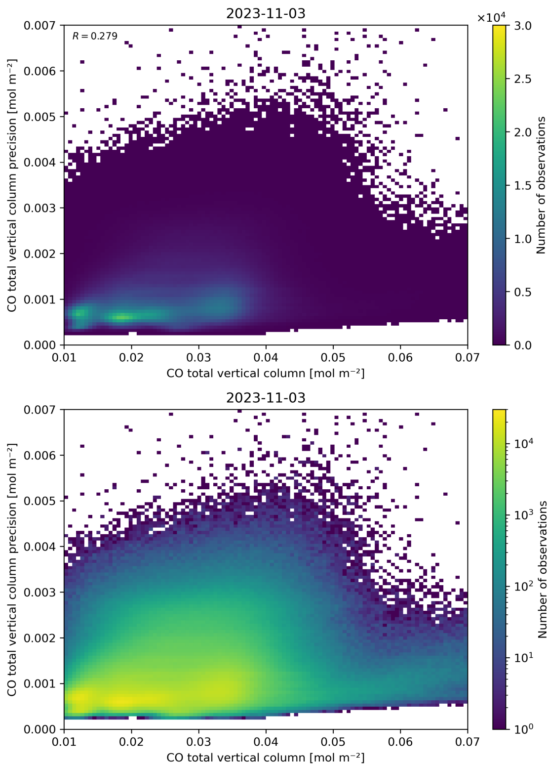
Figure 34: Scatter density plot of “CO total vertical column” against “CO total vertical column precision” for 2023-11-02 to 2023-11-04.
