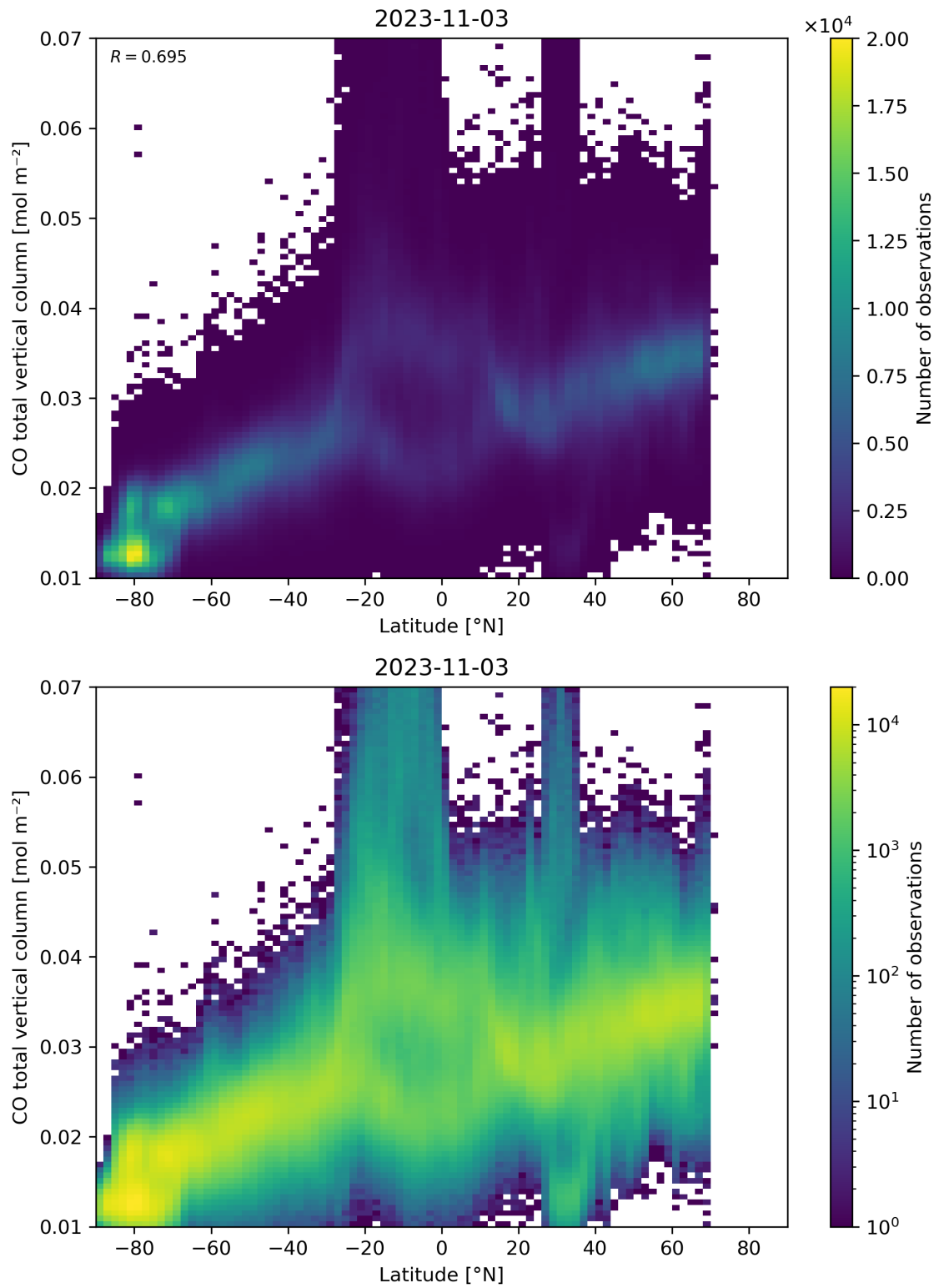
Figure 51: Scatter density plot of “Latitude” against “CO total vertical column” for 2023-11-02 to 2023-11-04.
