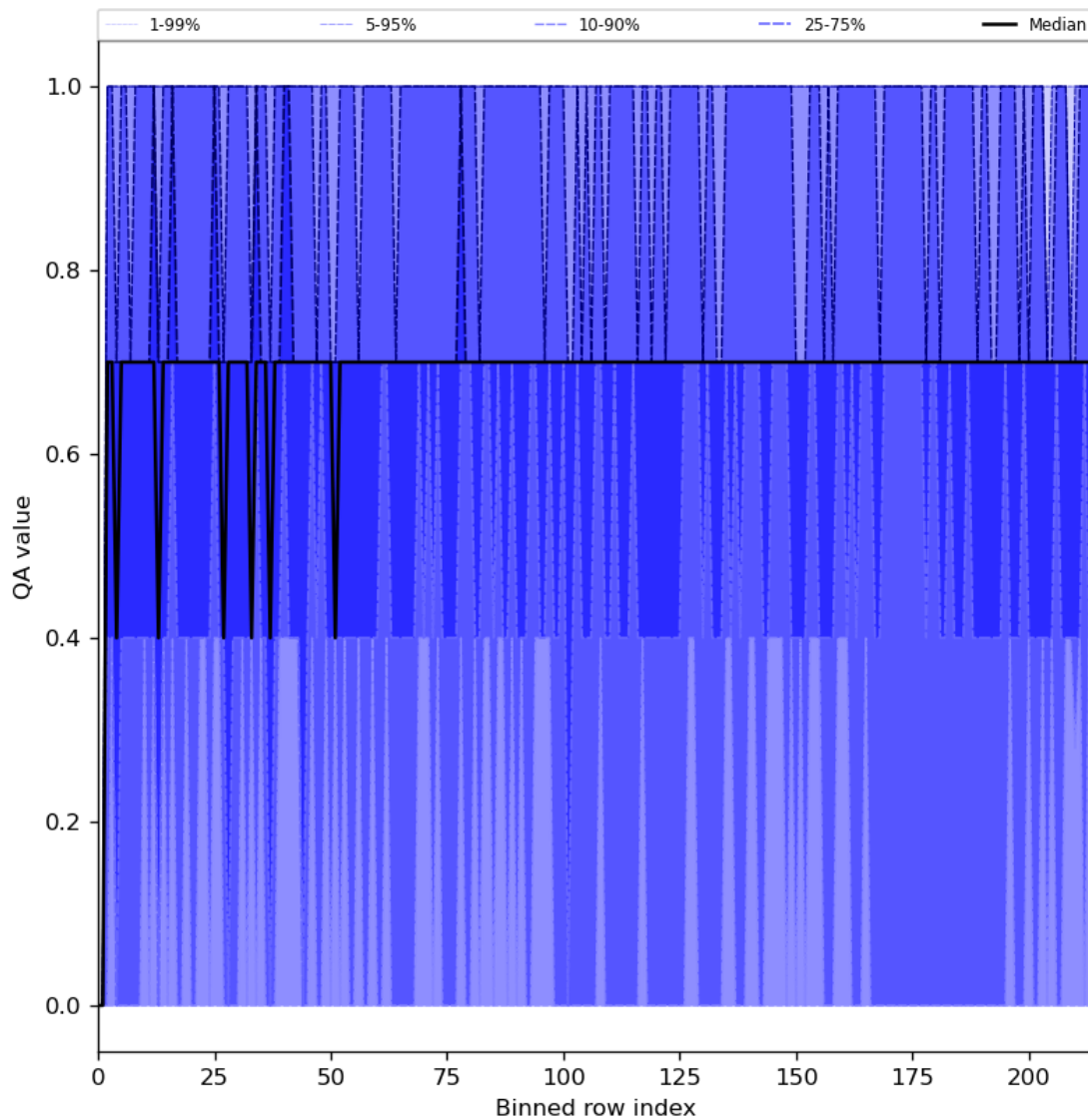
Figure 25: Along track statistics of “QA value” for 2023-11-02 to 2023-11-04
