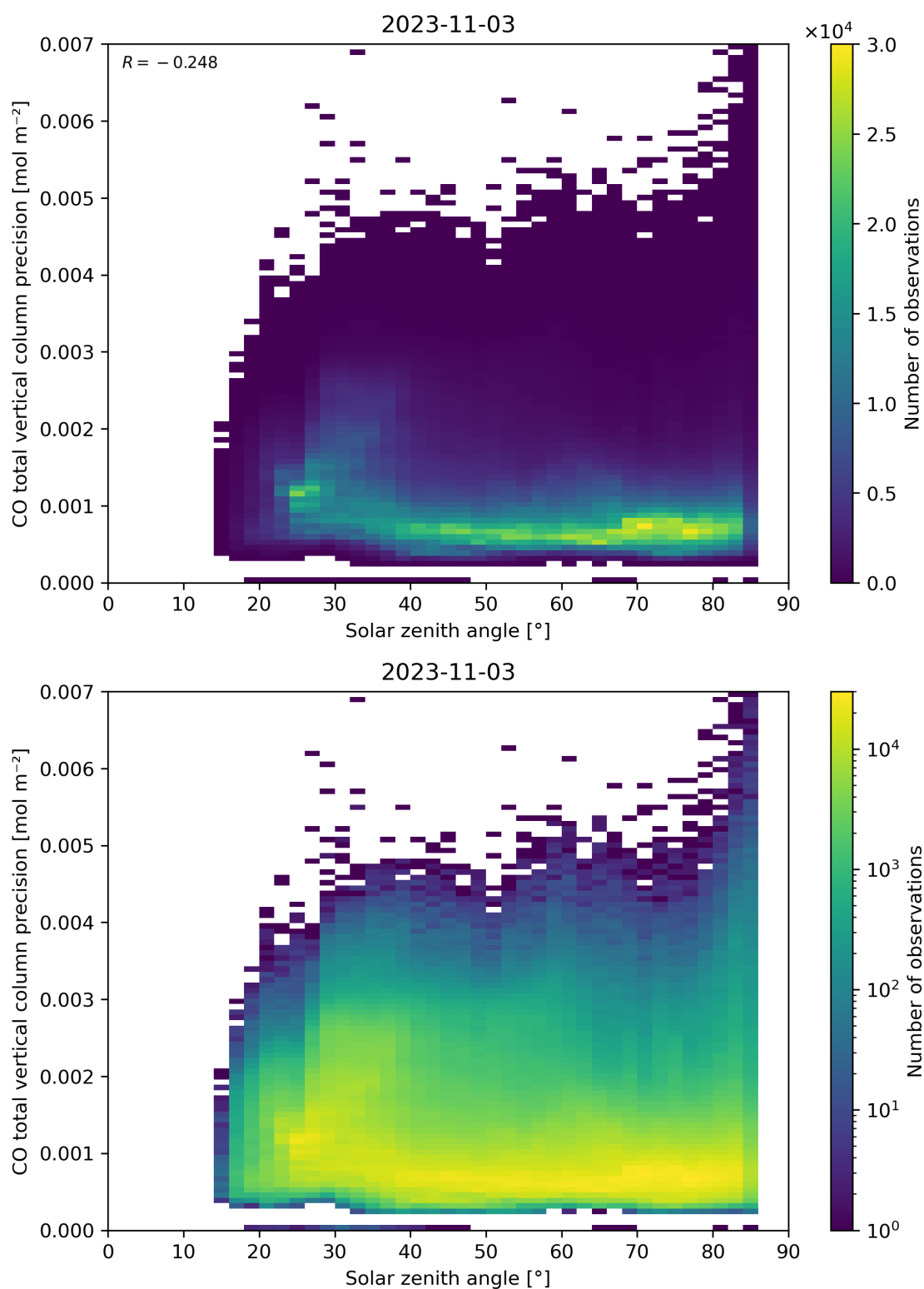
Figure 63: Scatter density plot of “Solar zenith angle” against “CO total vertical column precision” for 2023-11-02 to 2023-11-04.
