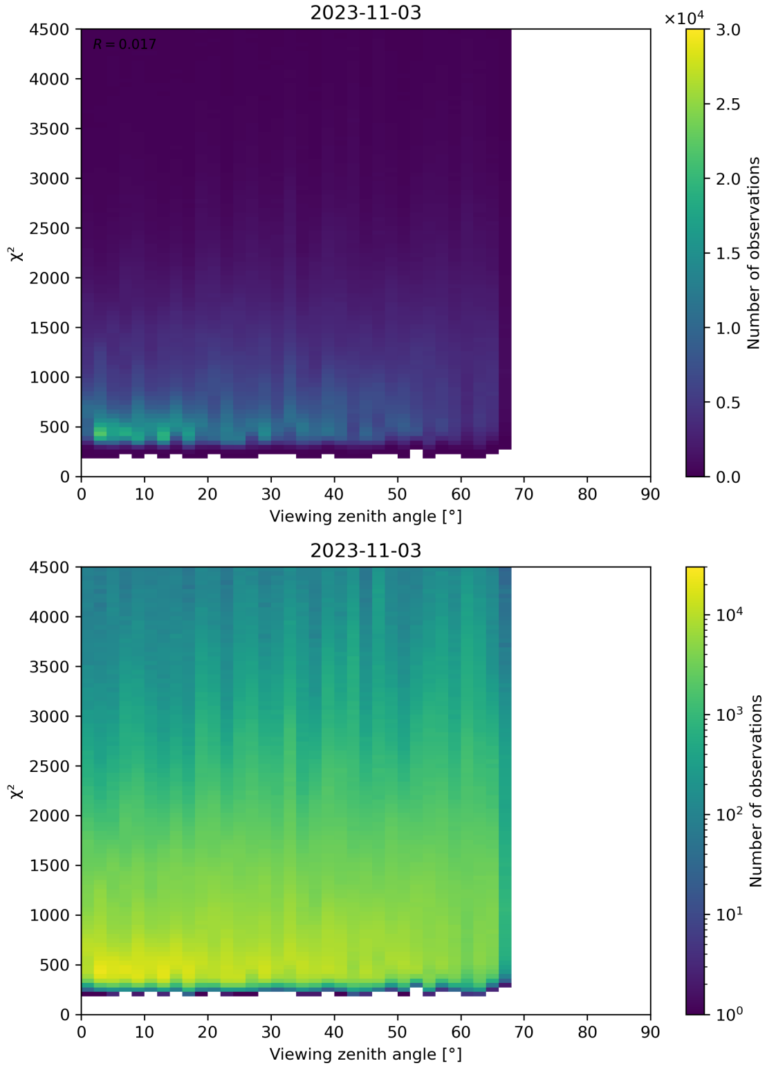
Figure 72: Scatter density plot of “Viewing zenith angle” against “ \chi^2 ” for 2023-11-02 to 2023-11-04.
