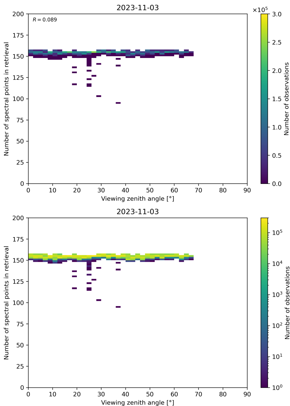
Figure 76: Scatter density plot of “Viewing zenith angle” against “Number of spectral points in retrieval” for 2023-11-02 to 2023-11-04.
