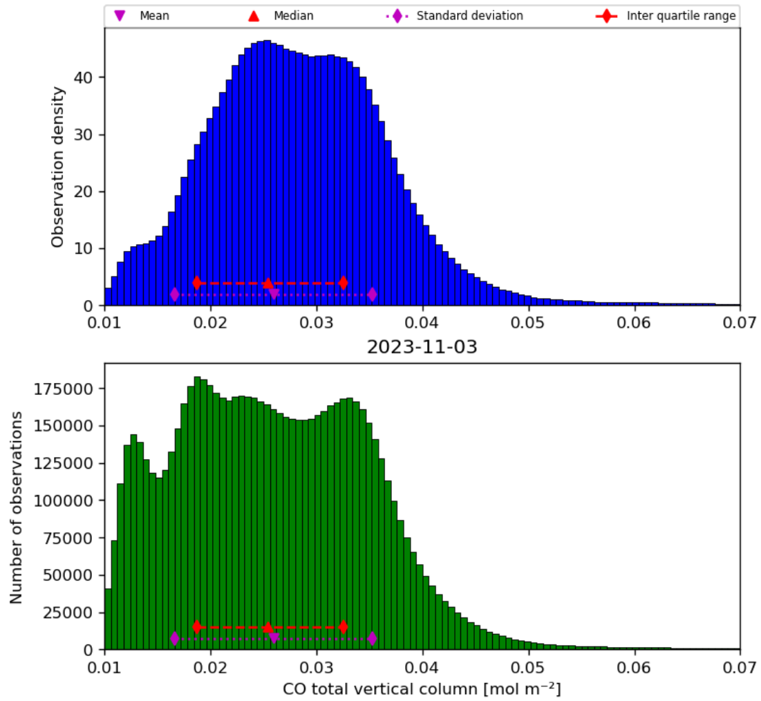
Figure 18: Histogram of “CO total vertical column” for 2023-11-02 to 2023-11-04
