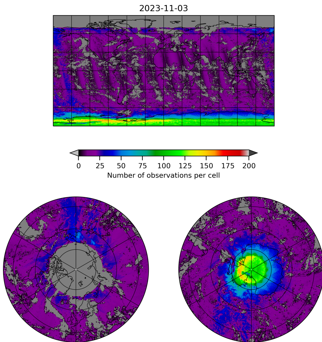
Figure 8: Map of the number of observations for 2023-11-02 to 2023-11-04
