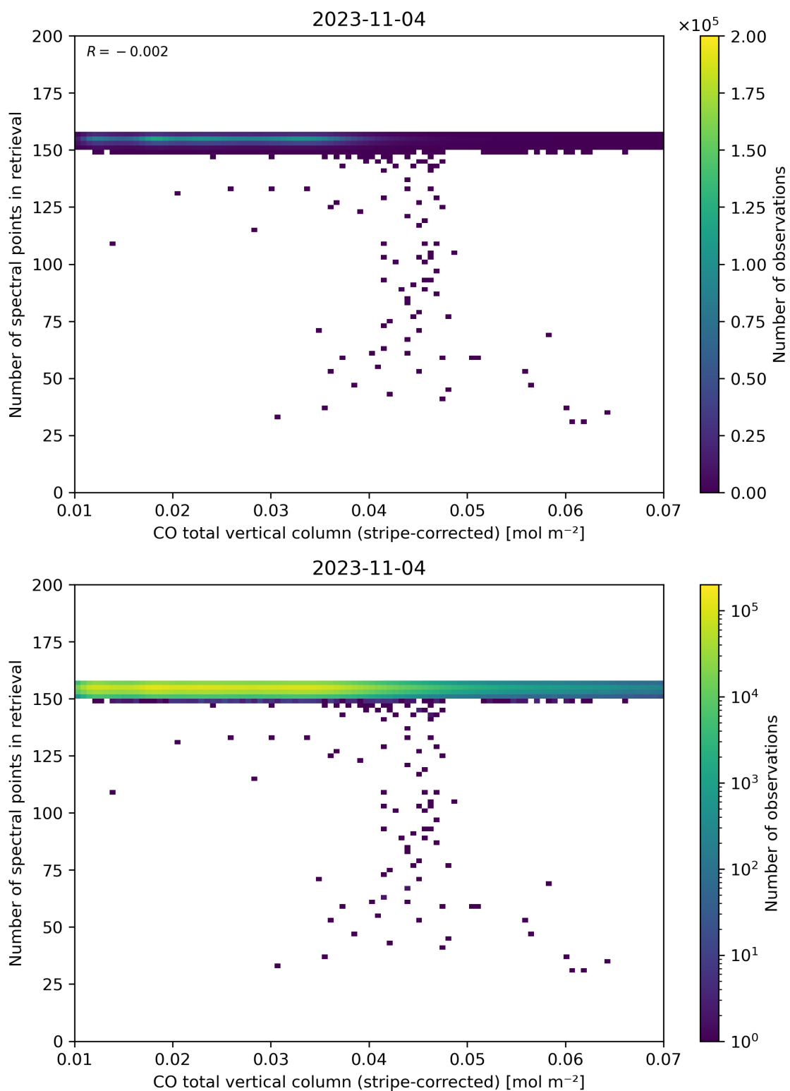
Figure 40: Scatter density plot of “CO total vertical column (stripe-corrected)” against “Number of spectral points in retrieval” for 2023-11-03 to 2023-11-05.
