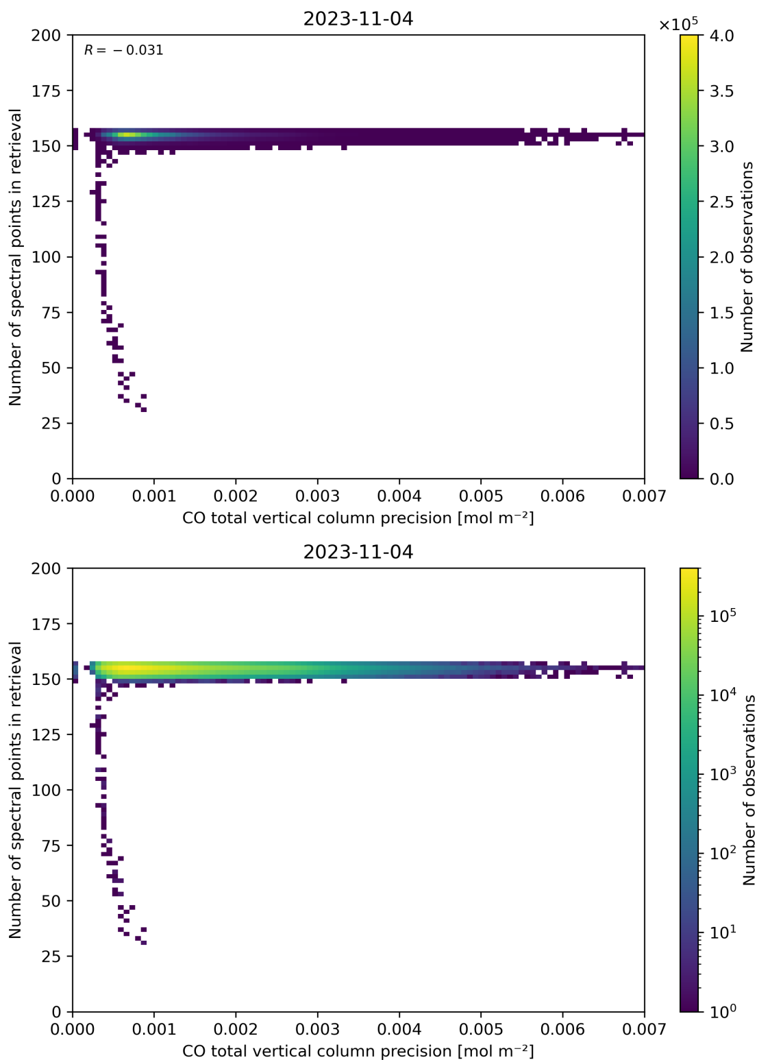
Figure 47: Scatter density plot of “CO total vertical column precision” against “Number of spectral points in retrieval” for 2023-11-03 to 2023-11-05.
