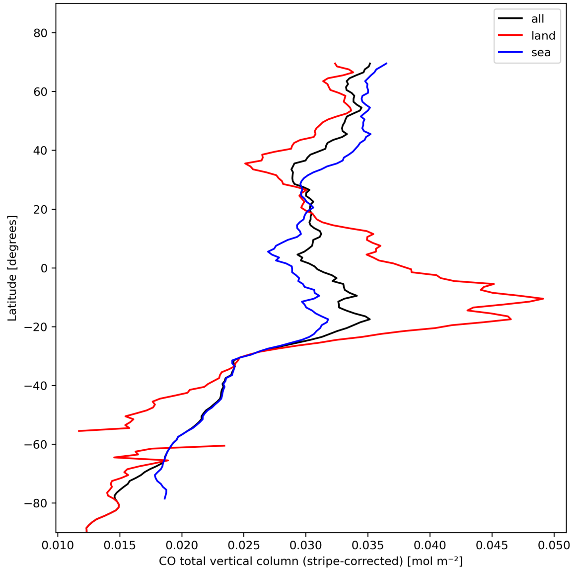
Figure 11: Zonal average of “CO total vertical column (stripe-corrected)” for 2023-11-03 to 2023-11-05.
