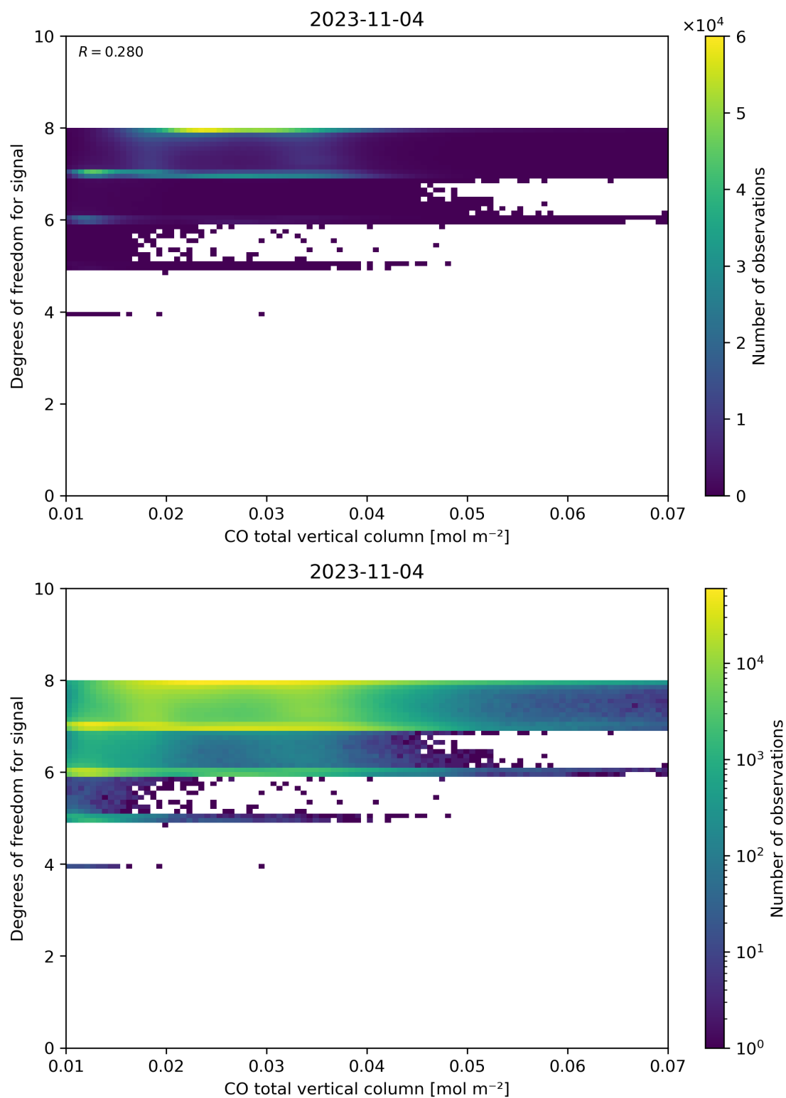
Figure 41: Scatter density plot of “CO total vertical column” against “Degrees of freedom for signal” for 2023-11-03 to 2023-11-05.
