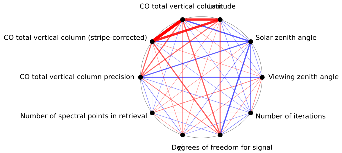
Figure 1: Map of correlation graph for 2023-11-03 to 2023-11-05.
