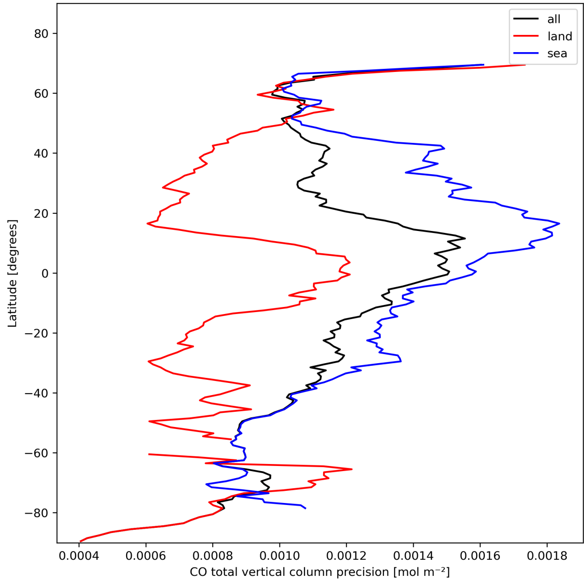
Figure 12: Zonal average of “CO total vertical column precision” for 2023-11-03 to 2023-11-05.
