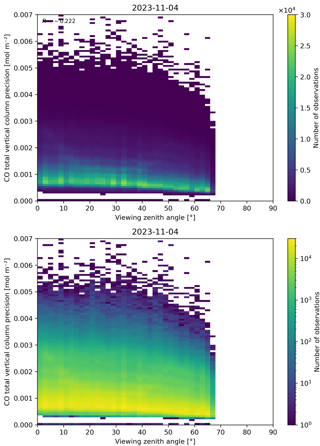
Figure 71: Scatter density plot of “Viewing zenith angle” against “CO total vertical column precision” for 2023-11-03 to 2023-11-05.
