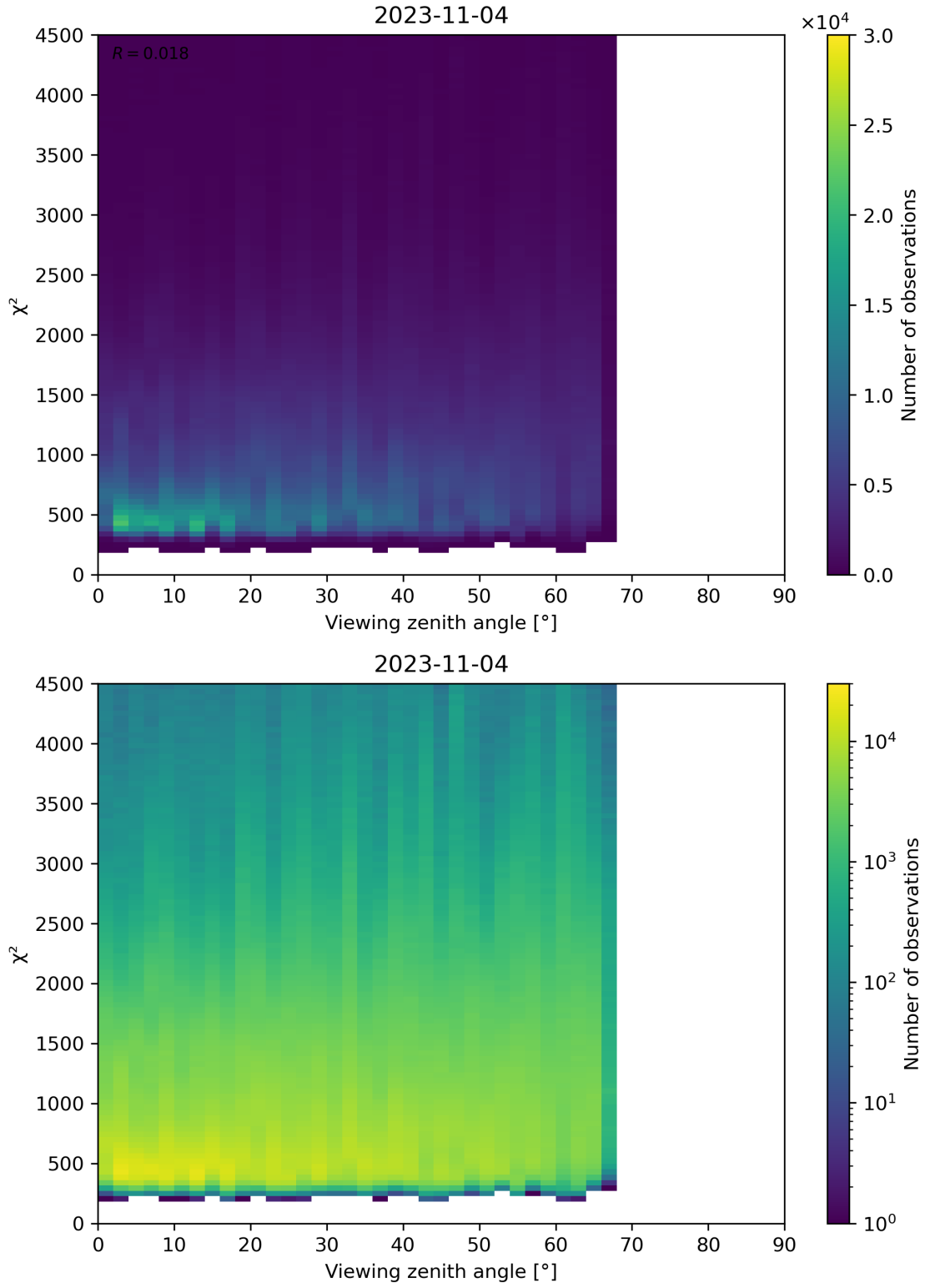
Figure 72: Scatter density plot of “Viewing zenith angle” against “ \chi^2 ” for 2023-11-03 to 2023-11-05.
