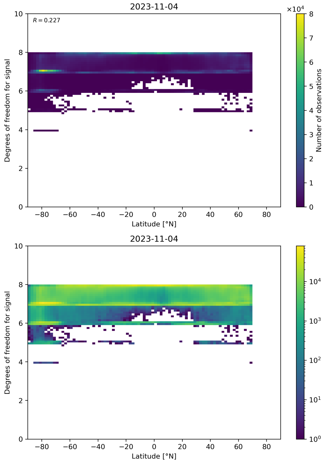
Figure 55: Scatter density plot of “Latitude” against “Degrees of freedom for signal” for 2023-11-03 to 2023-11-05.
