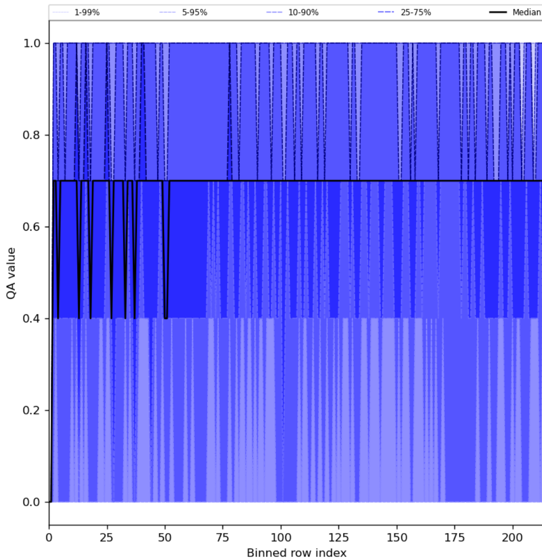
Figure 25: Along track statistics of “QA value” for 2023-11-03 to 2023-11-05
