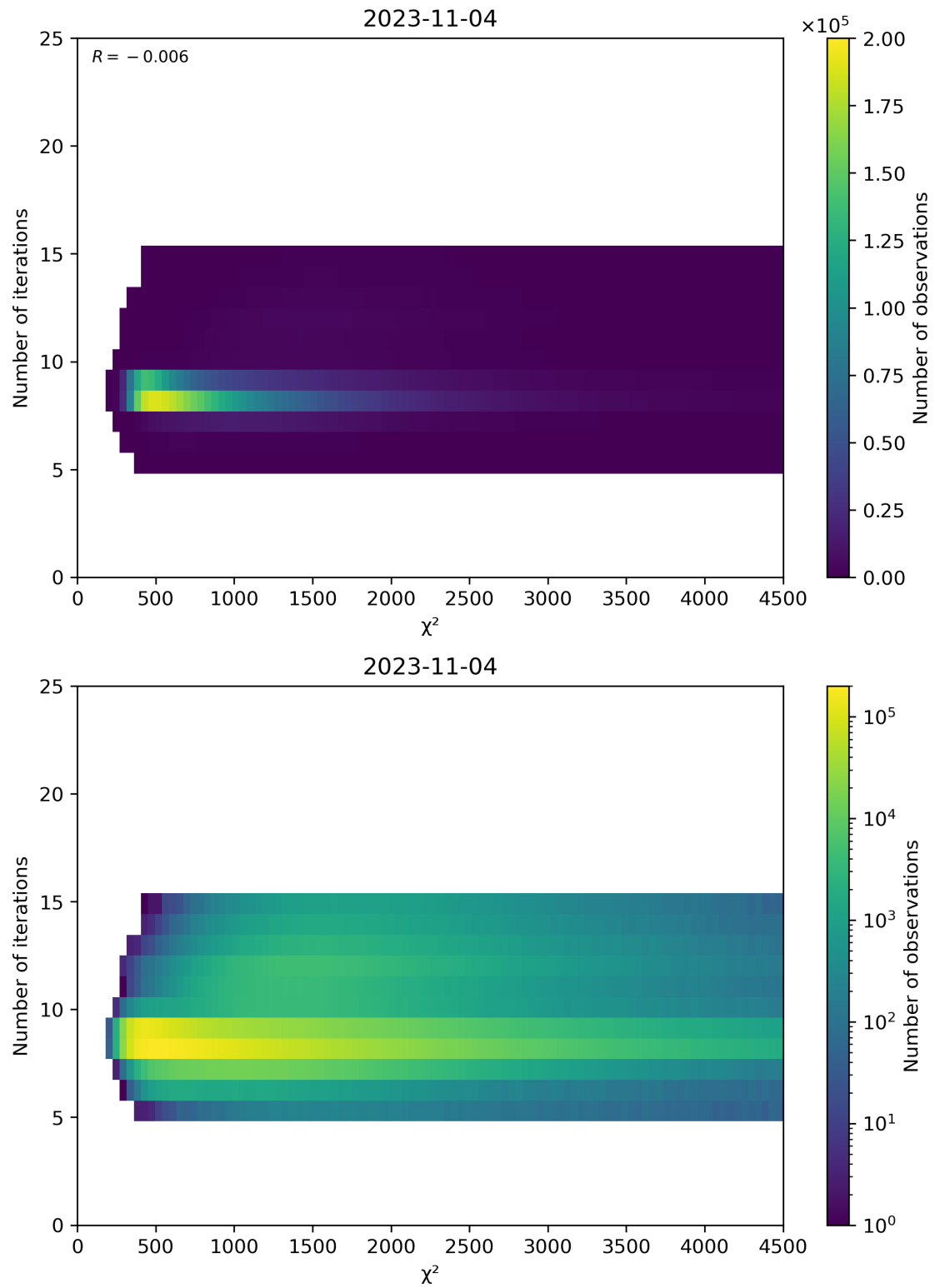
Figure 49: Scatter density plot of “ \chi^2 ” against “Number of iterations” for 2023-11-03 to 2023-11-05.
