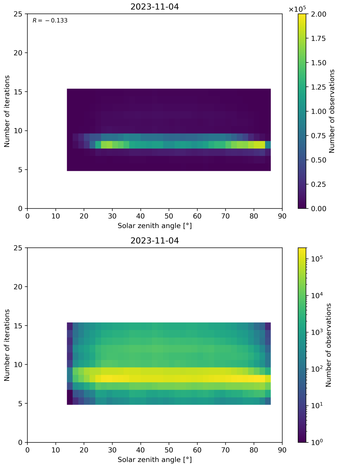
Figure 67: Scatter density plot of “Solar zenith angle” against “Number of iterations” for 2023-11-03 to 2023-11-05.
