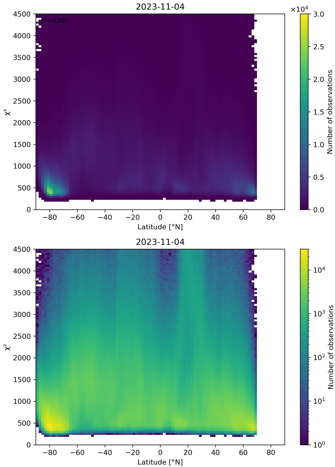
Figure 54: Scatter density plot of “Latitude” against “ \chi^2 ” for 2023-11-03 to 2023-11-05.
