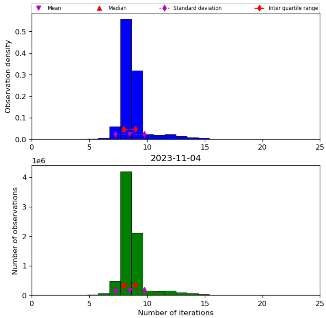
Figure 24: Histogram of “Number of iterations” for 2023-11-03 to 2023-11-05
