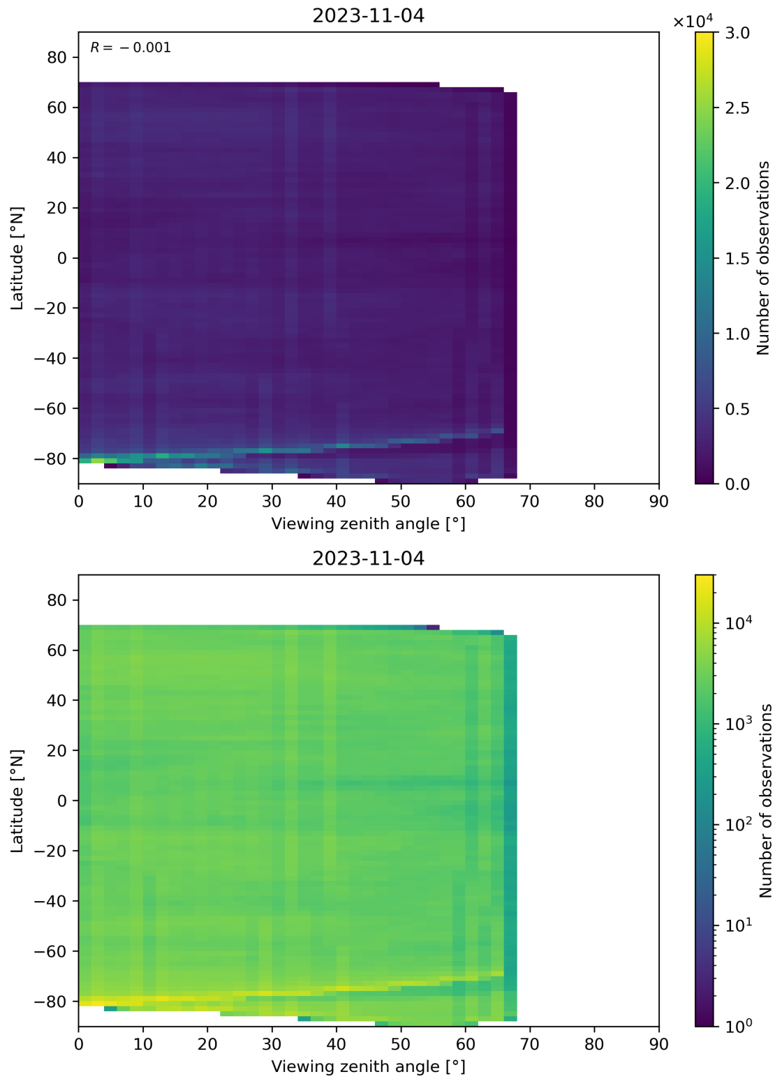
Figure 74: Scatter density plot of “Viewing zenith angle” against “Latitude” for 2023-11-03 to 2023-11-05.
