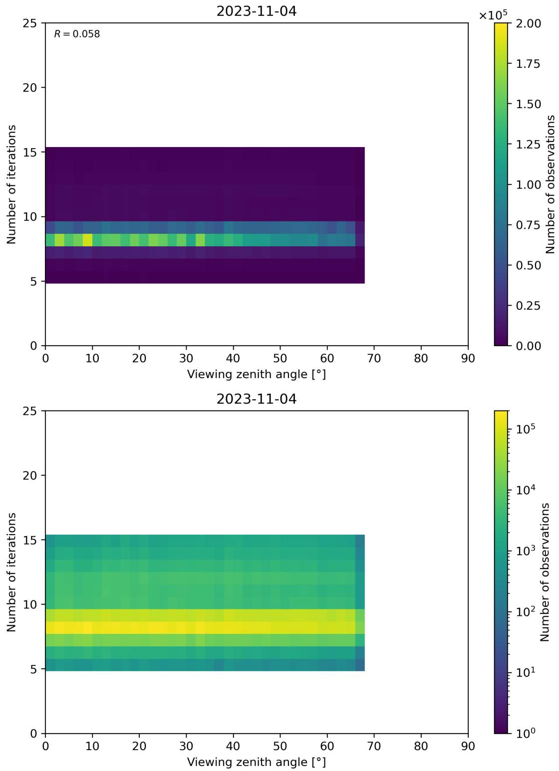
Figure 75: Scatter density plot of “Viewing zenith angle” against “Number of iterations” for 2023-11-03 to 2023-11-05.
