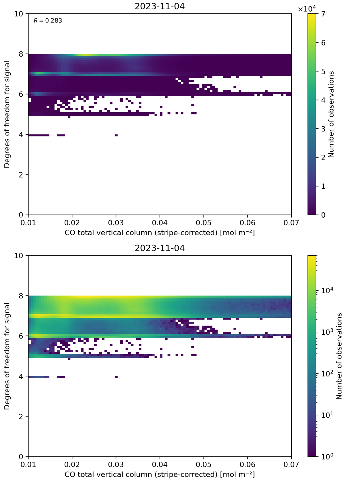
Figure 38: Scatter density plot of “CO total vertical column (stripe-corrected)” against “Degrees of freedom for signal” for 2023-11-03 to 2023-11-05.
