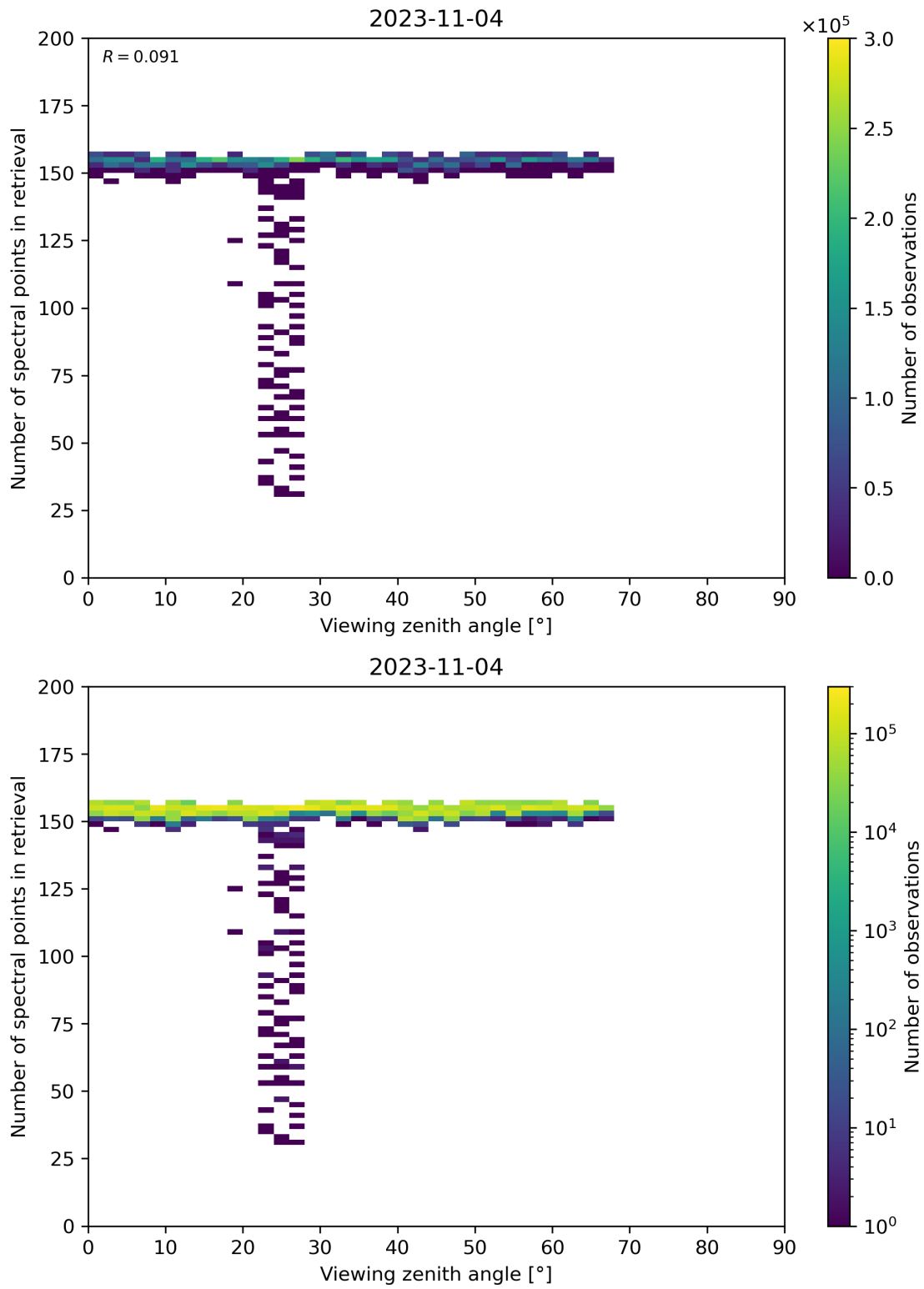
Figure 76: Scatter density plot of “Viewing zenith angle” against “Number of spectral points in retrieval” for 2023-11-03 to 2023-11-05.
