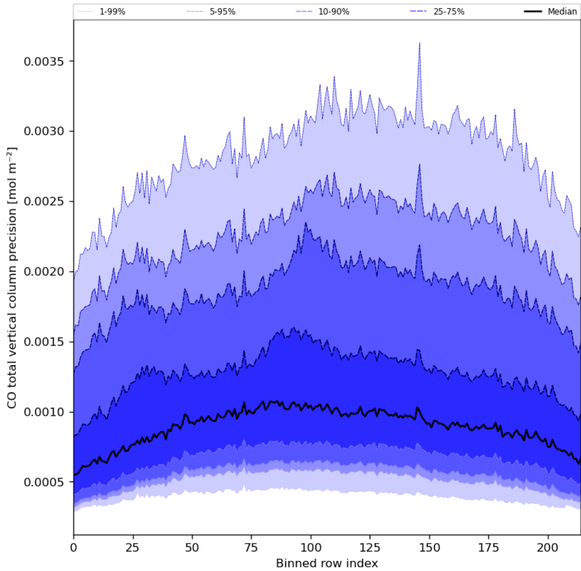
Figure 28: Along track statistics of “CO total vertical column precision” for 2023-11-03 to 2023-11-05
