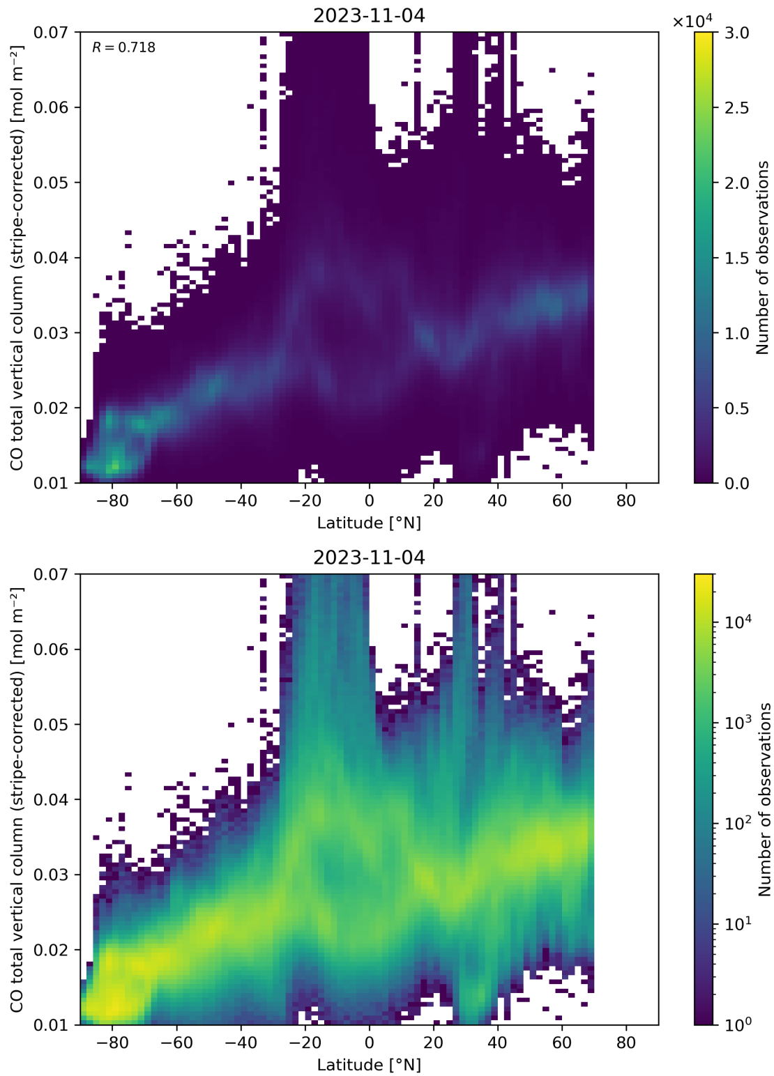
Figure 52: Scatter density plot of “Latitude” against “CO total vertical column (stripe-corrected)” for 2023-11-03 to 2023-11-05.
