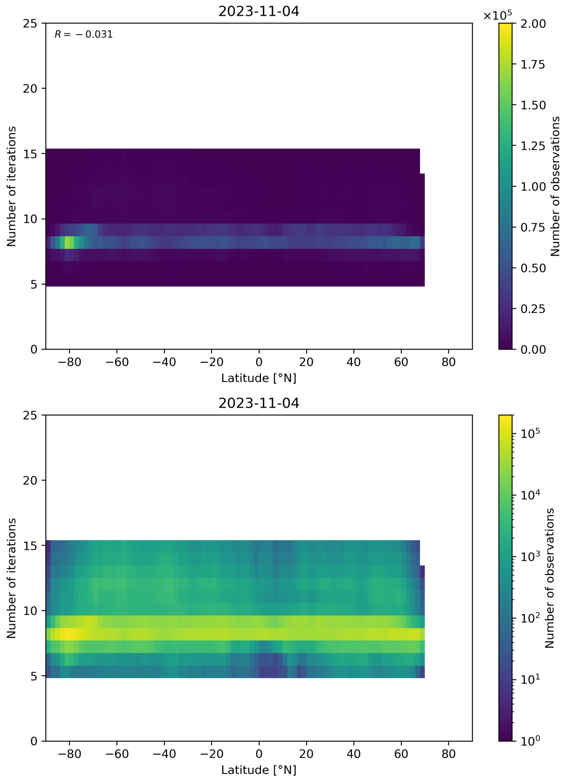
Figure 56: Scatter density plot of “Latitude” against “Number of iterations” for 2023-11-03 to 2023-11-05.
