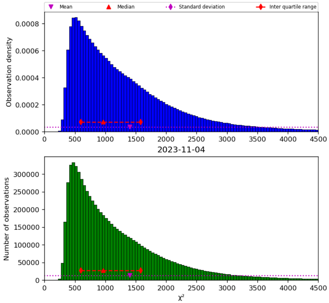
Figure 22: Histogram of “ \chi^2 ” for 2023-11-03 to 2023-11-05
