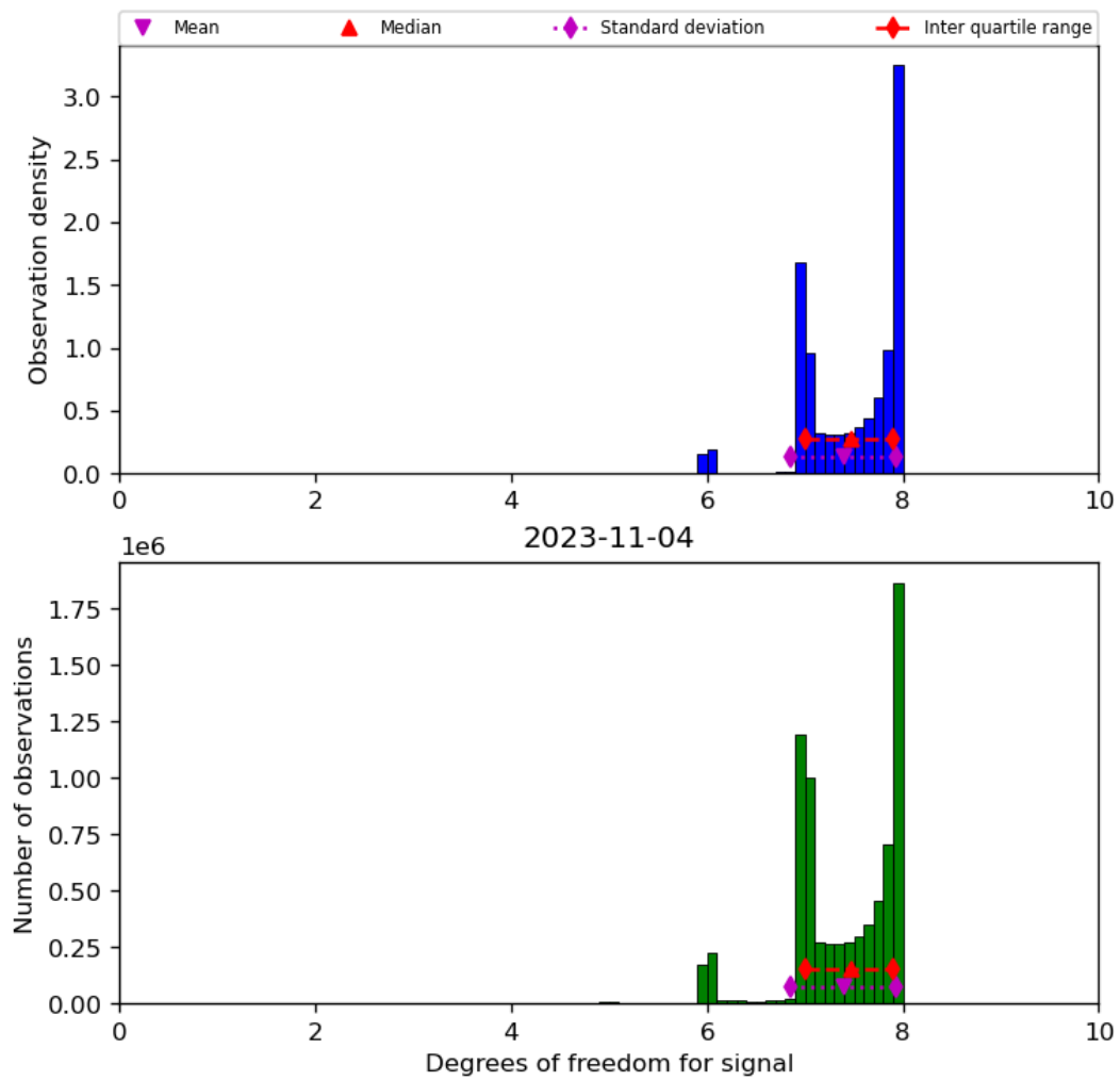
Figure 23: Histogram of “Degrees of freedom for signal” for 2023-11-03 to 2023-11-05
