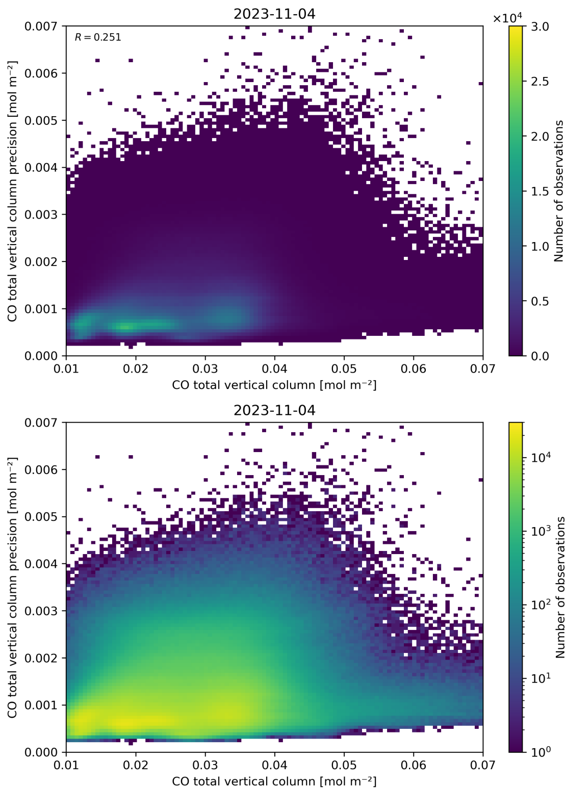
Figure 34: Scatter density plot of “CO total vertical column” against “CO total vertical column precision” for 2023-11-03 to 2023-11-05.
