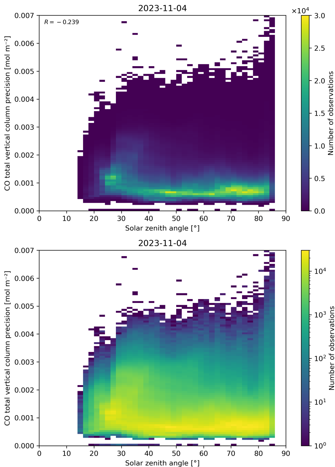
Figure 63: Scatter density plot of “Solar zenith angle” against “CO total vertical column precision” for 2023-11-03 to 2023-11-05.
