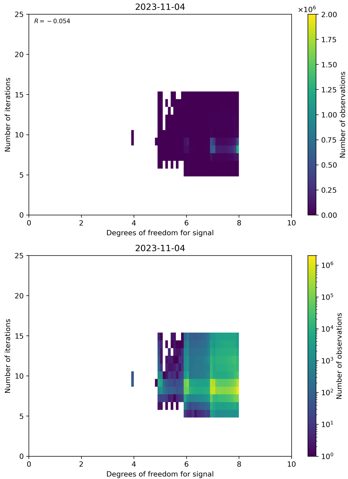
Figure 50: Scatter density plot of “Degrees of freedom for signal” against “Number of iterations” for 2023-11-03 to 2023-11-05.
