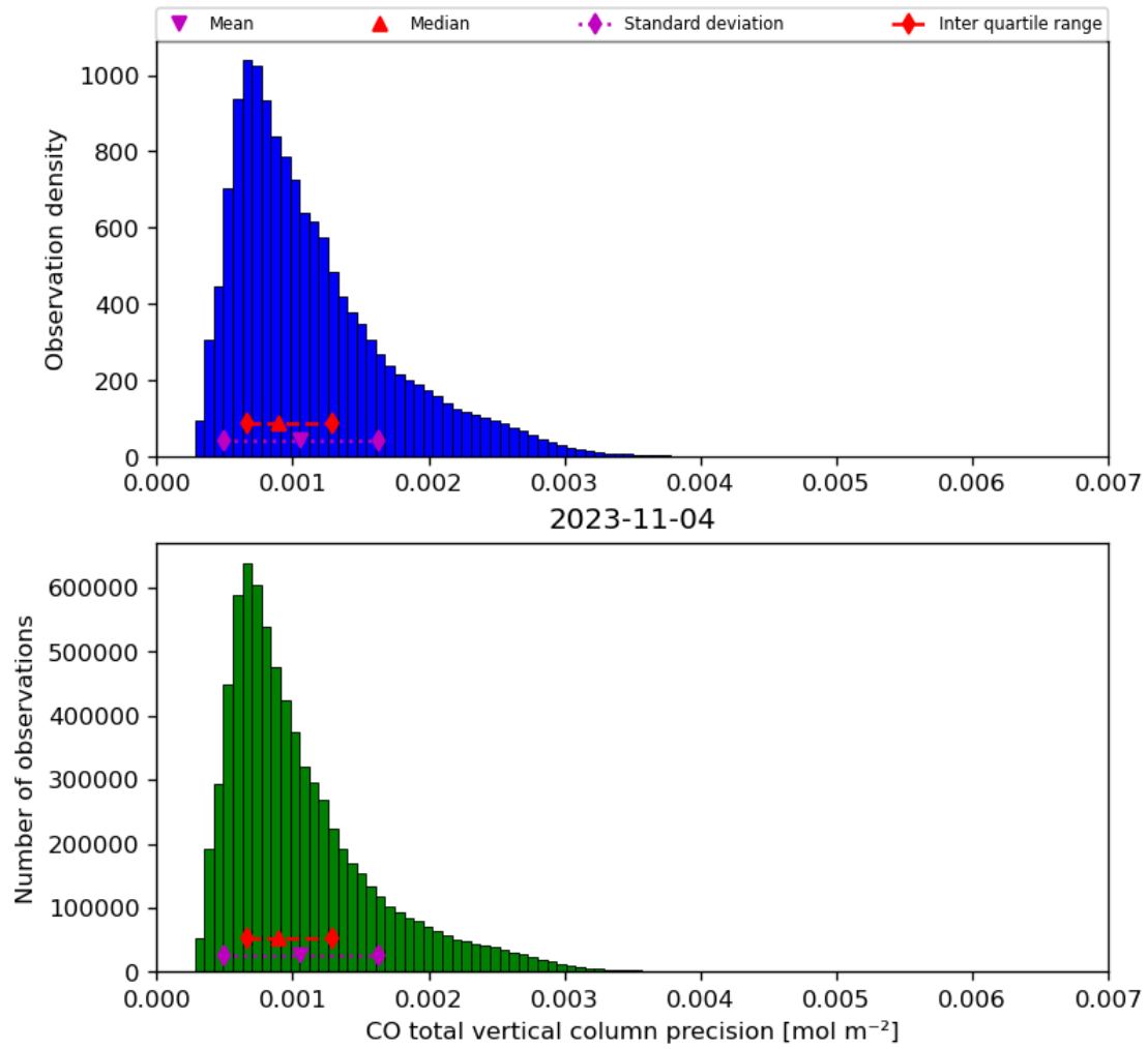
Figure 20: Histogram of “CO total vertical column precision” for 2023-11-03 to 2023-11-05
