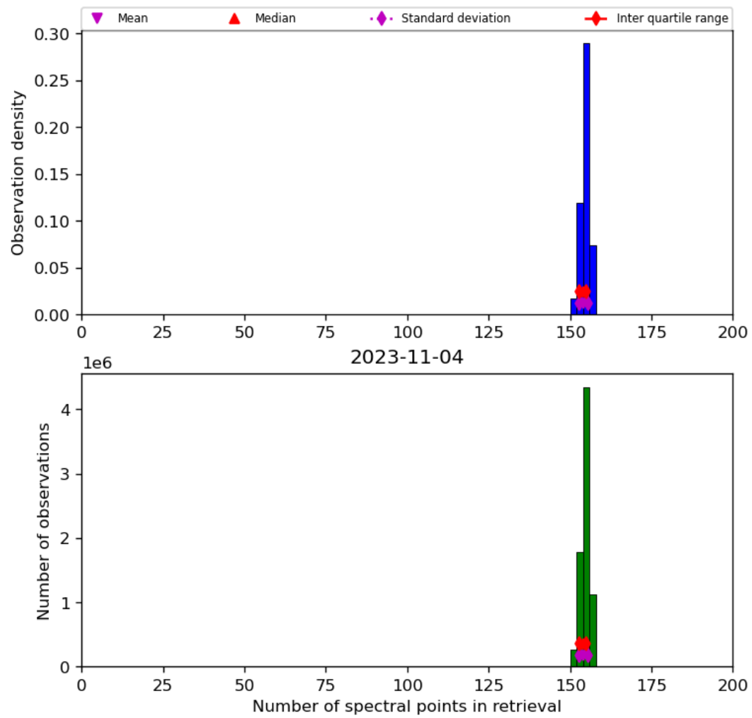
Figure 21: Histogram of “Number of spectral points in retrieval” for 2023-11-03 to 2023-11-05
