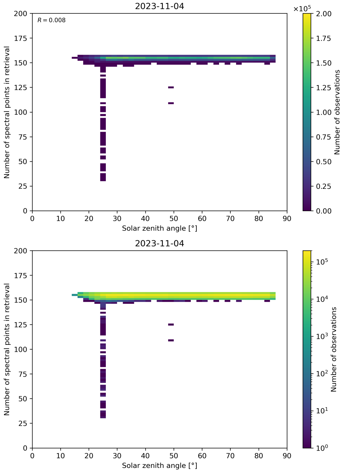
Figure 68: Scatter density plot of “Solar zenith angle” against “Number of spectral points in retrieval” for 2023-11-03 to 2023-11-05.
