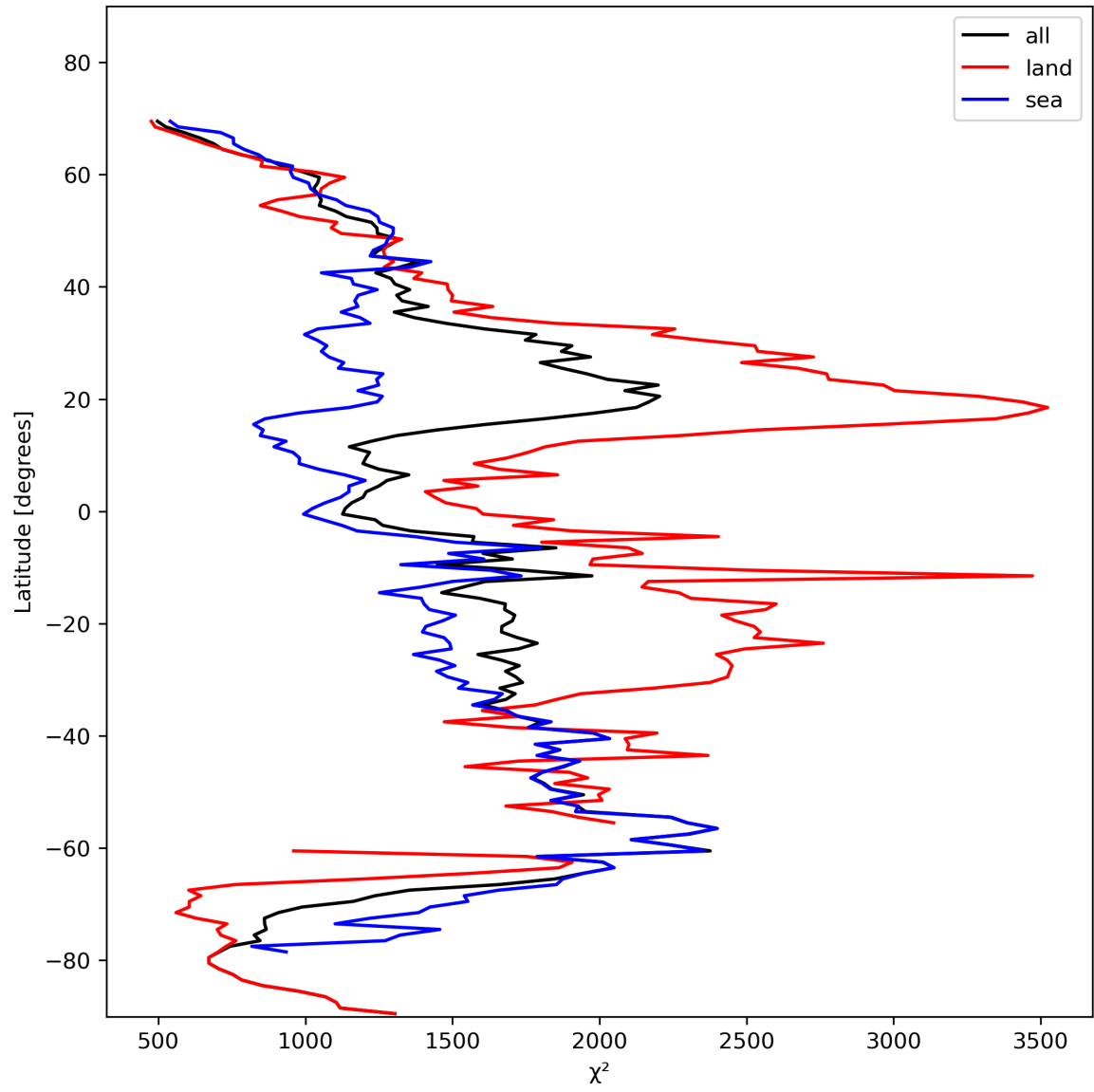
Figure 14: Zonal average of “ \chi^2 ” for 2023-11-03 to 2023-11-05.
