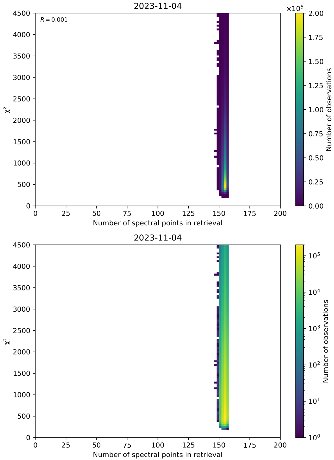
Figure 58: Scatter density plot of “Number of spectral points in retrieval” against “ \chi^2 ” for 2023-11-03 to 2023-11-05.
