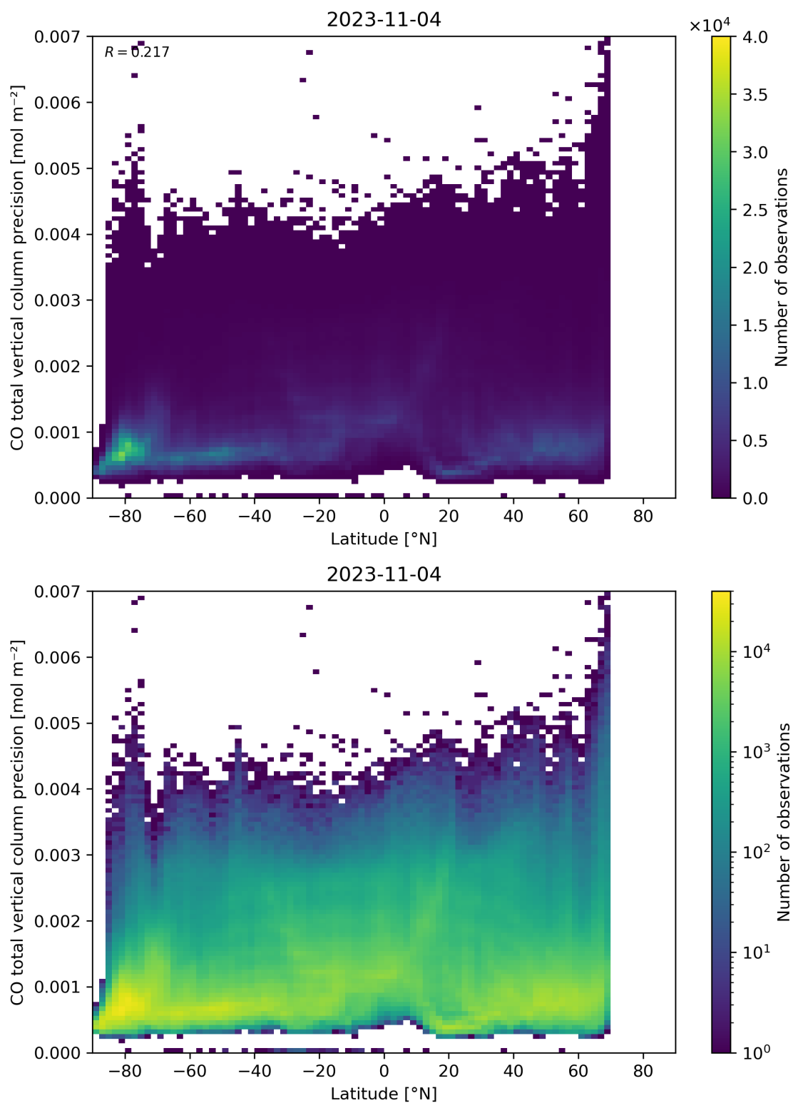
Figure 53: Scatter density plot of “Latitude” against “CO total vertical column precision” for 2023-11-03 to 2023-11-05.
