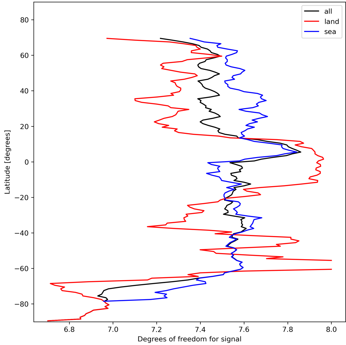
Figure 15: Zonal average of “Degrees of freedom for signal” for 2023-11-03 to 2023-11-05.
