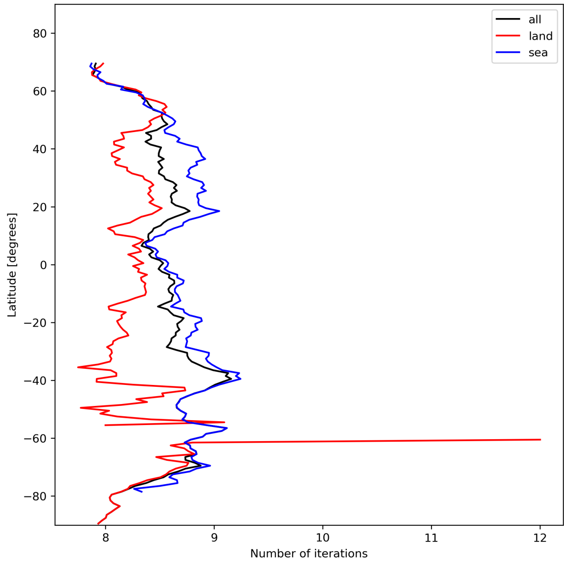
Figure 16: Zonal average of “Number of iterations” for 2023-11-03 to 2023-11-05.
