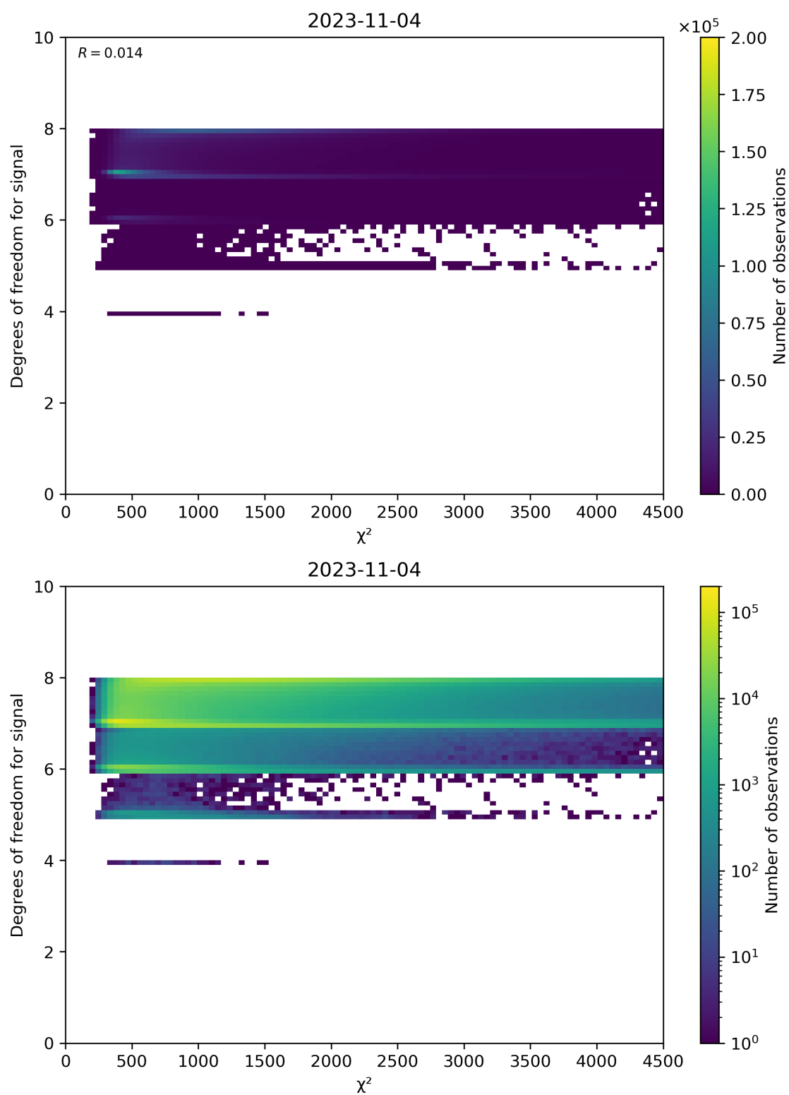
Figure 48: Scatter density plot of “ \chi^2 ” against “Degrees of freedom for signal” for 2023-11-03 to 2023-11-05.
