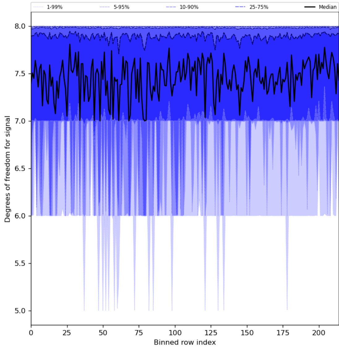
Figure 31: Along track statistics of “Degrees of freedom for signal” for 2023-11-03 to 2023-11-05
