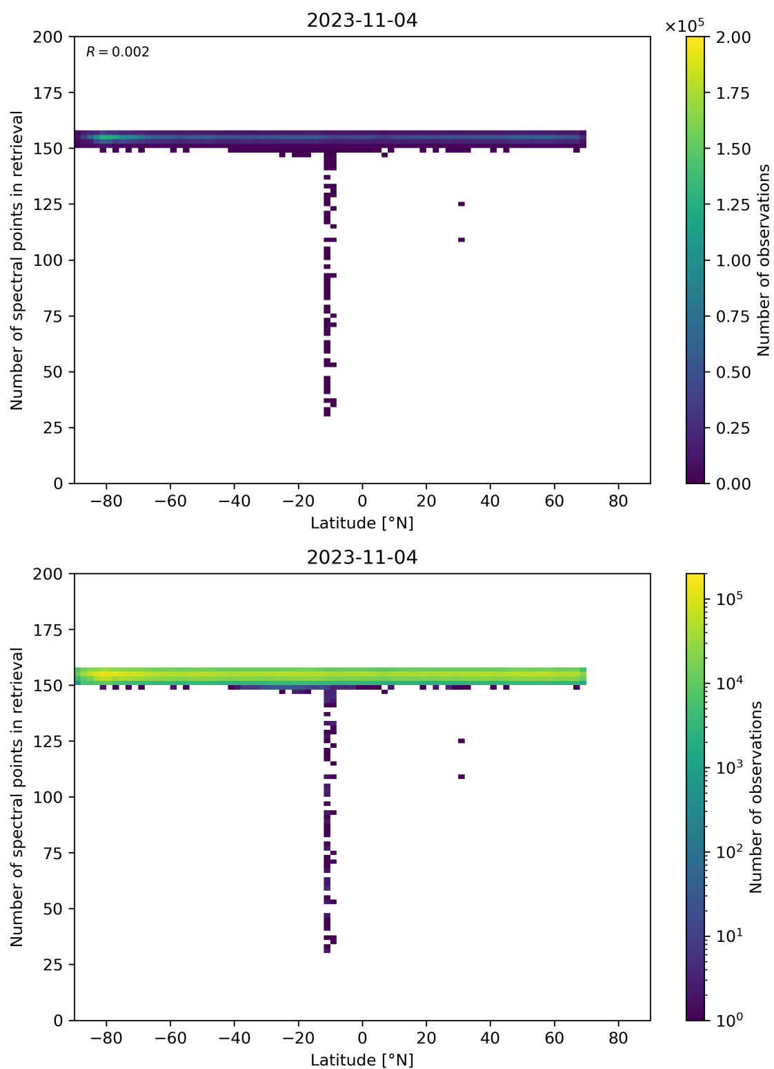
Figure 57: Scatter density plot of “Latitude” against “Number of spectral points in retrieval” for 2023-11-03 to 2023-11-05.
