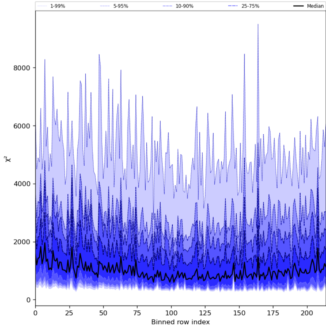
Figure 30: Along track statistics of “ \chi^2 ” for 2023-11-03 to 2023-11-05
