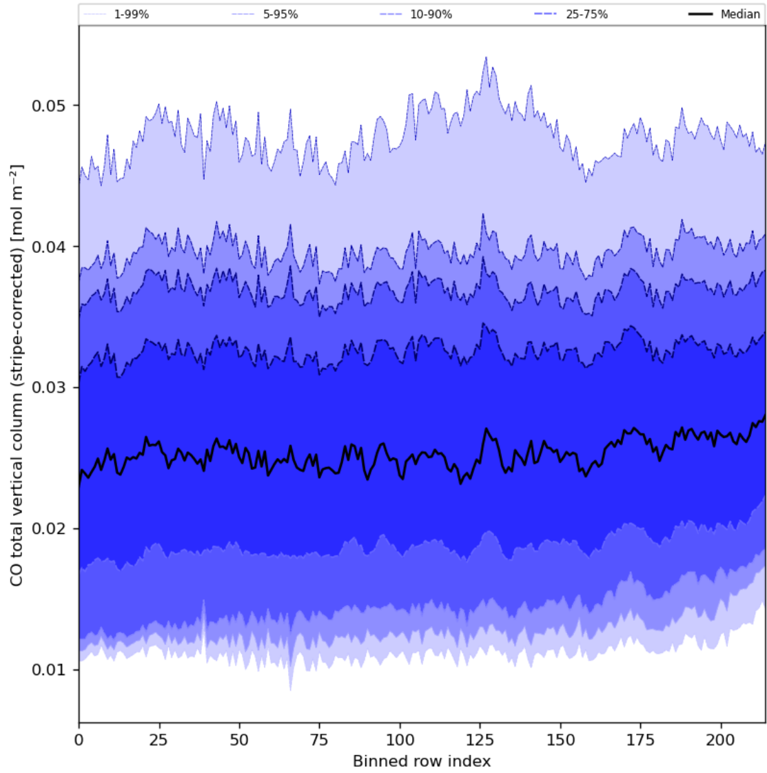
Figure 27: Along track statistics of “CO total vertical column (stripe-corrected)” for 2023-11-03 to 2023-11-05
