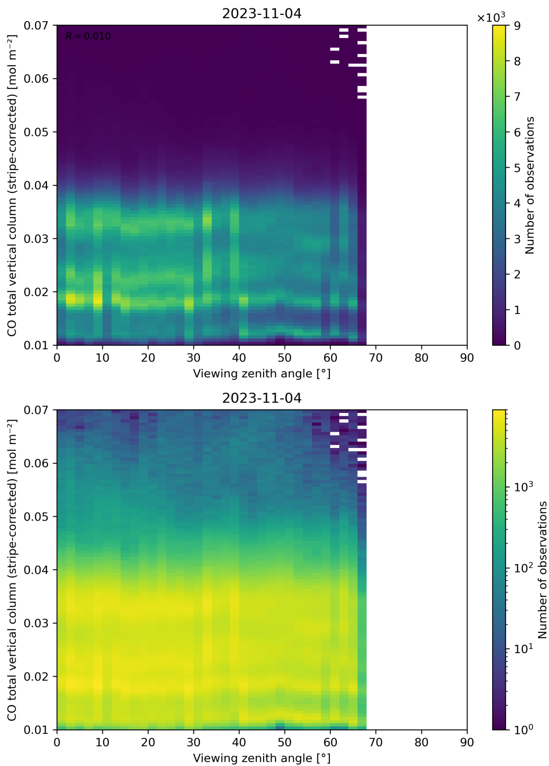
Figure 70: Scatter density plot of “Viewing zenith angle” against “CO total vertical column (stripe-corrected)” for 2023-11-03 to 2023-11-05.
