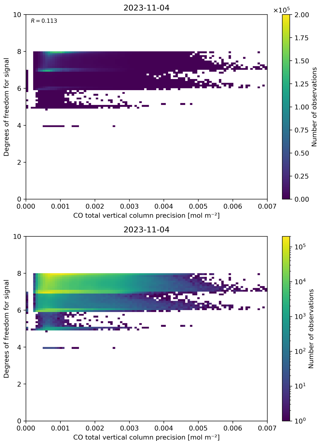
Figure 45: Scatter density plot of “CO total vertical column precision” against “Degrees of freedom for signal” for 2023-11-03 to 2023-11-05.
