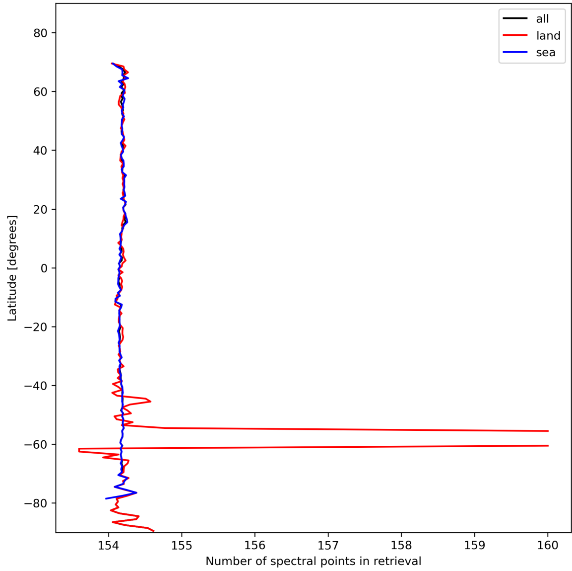
Figure 13: Zonal average of “Number of spectral points in retrieval” for 2023-11-03 to 2023-11-05.
