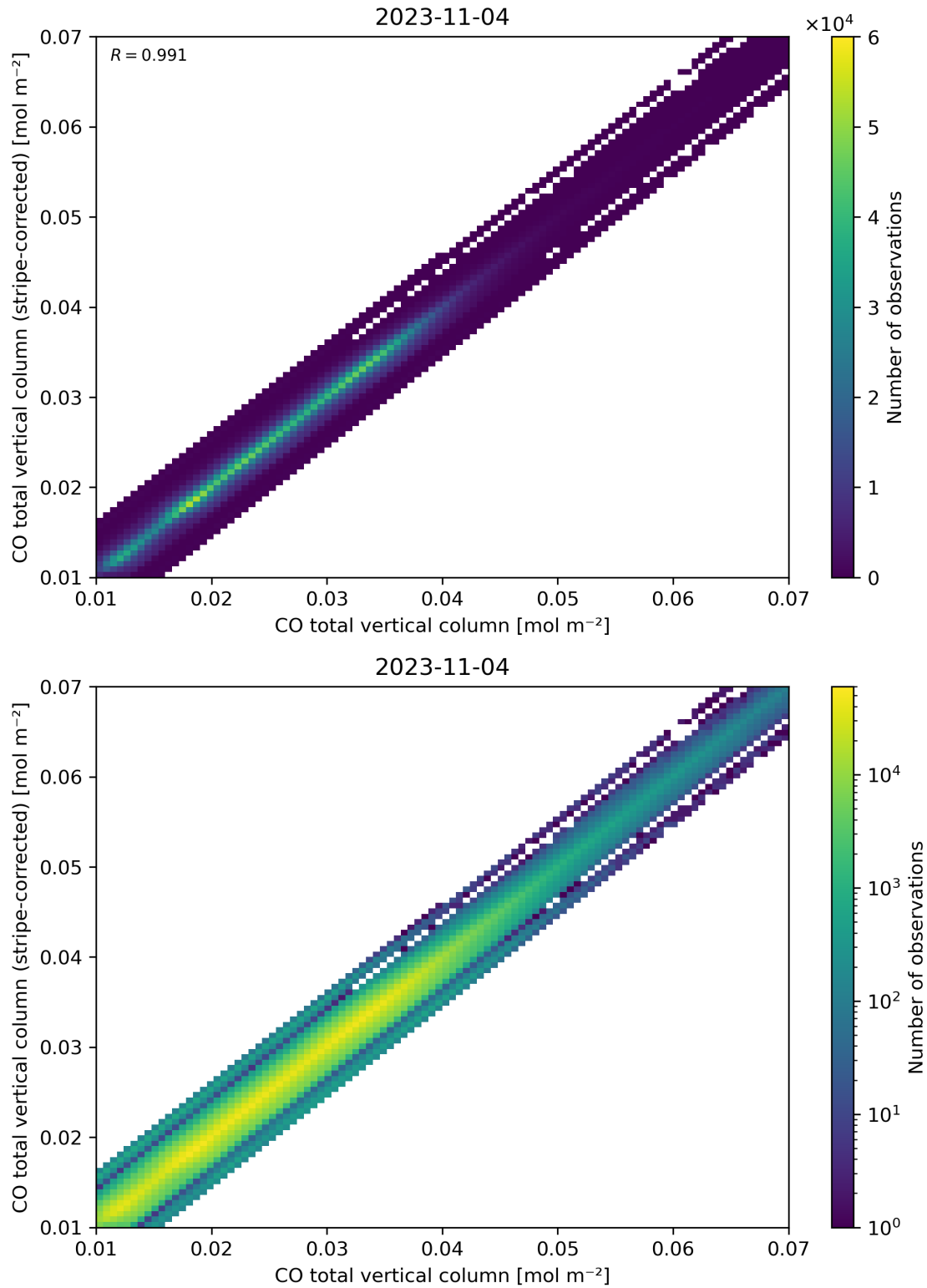
Figure 33: Scatter density plot of “CO total vertical column” against “CO total vertical column (stripe-corrected)” for 2023-11-03 to 2023-11-05.
