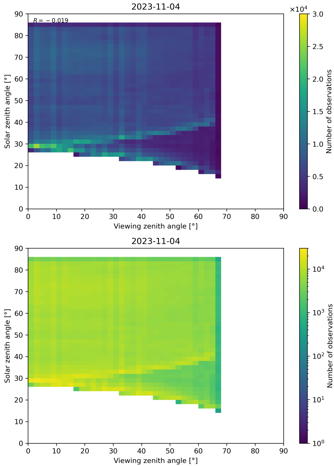
Figure 77: Scatter density plot of “Viewing zenith angle” against “Solar zenith angle” for 2023-11-03 to 2023-11-05.
