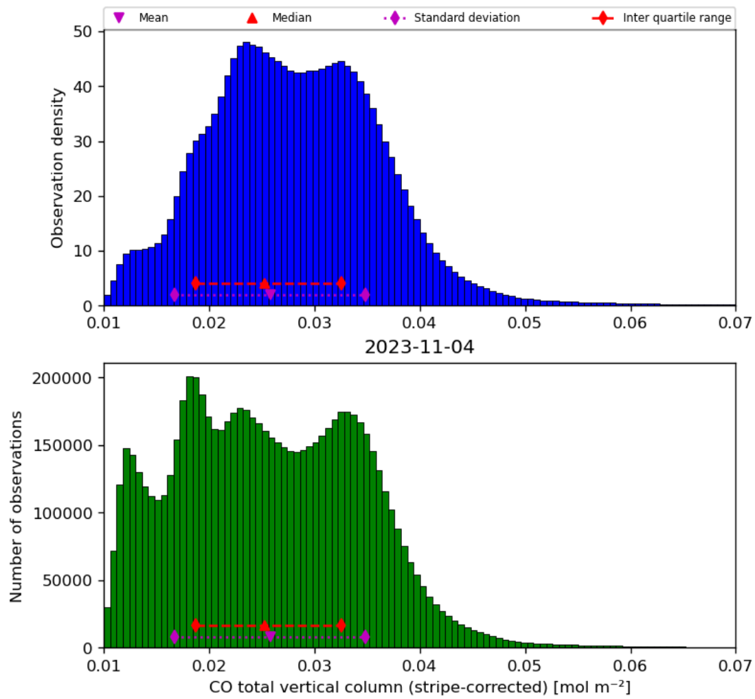
Figure 19: Histogram of “CO total vertical column (stripe-corrected)” for 2023-11-03 to 2023-11-05
