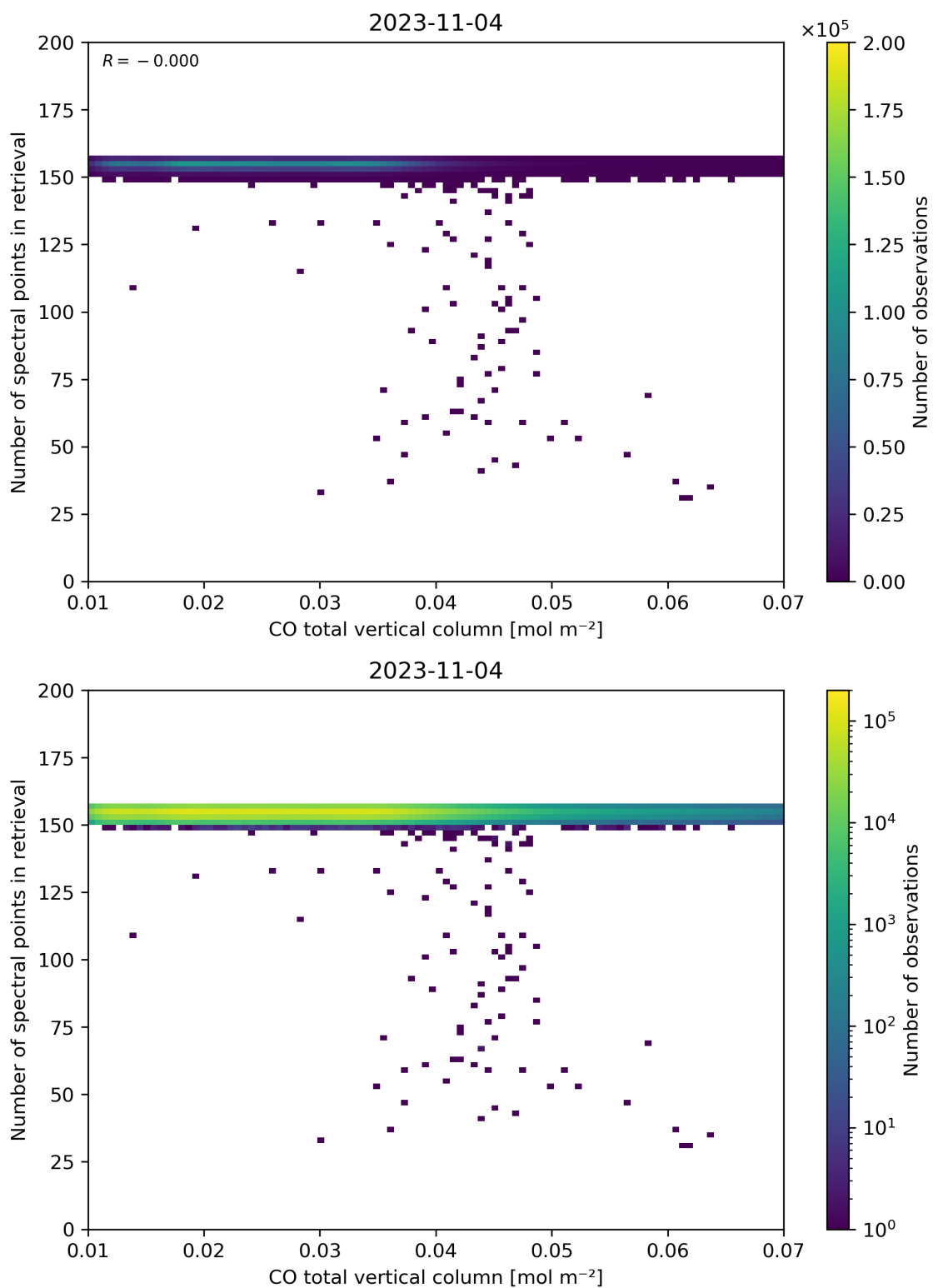
Figure 43: Scatter density plot of “CO total vertical column” against “Number of spectral points in retrieval” for 2023-11-03 to 2023-11-05.
