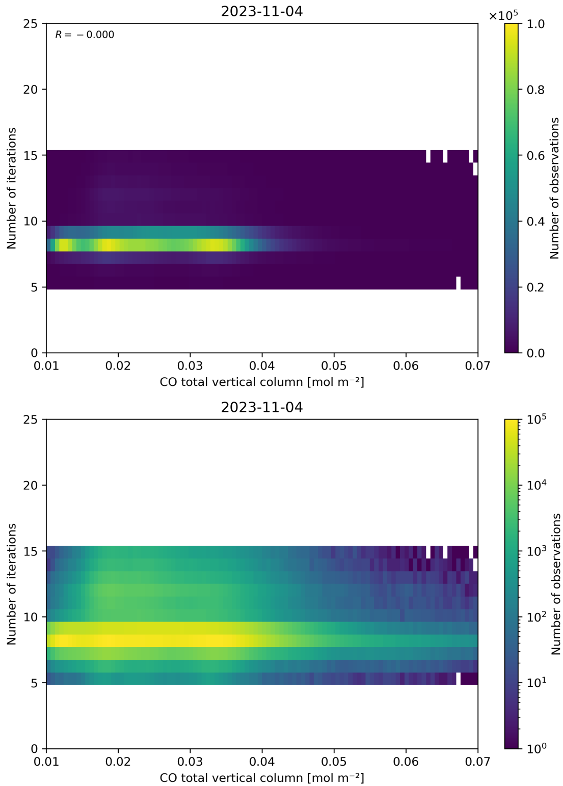
Figure 42: Scatter density plot of “CO total vertical column” against “Number of iterations” for 2023-11-03 to 2023-11-05.
