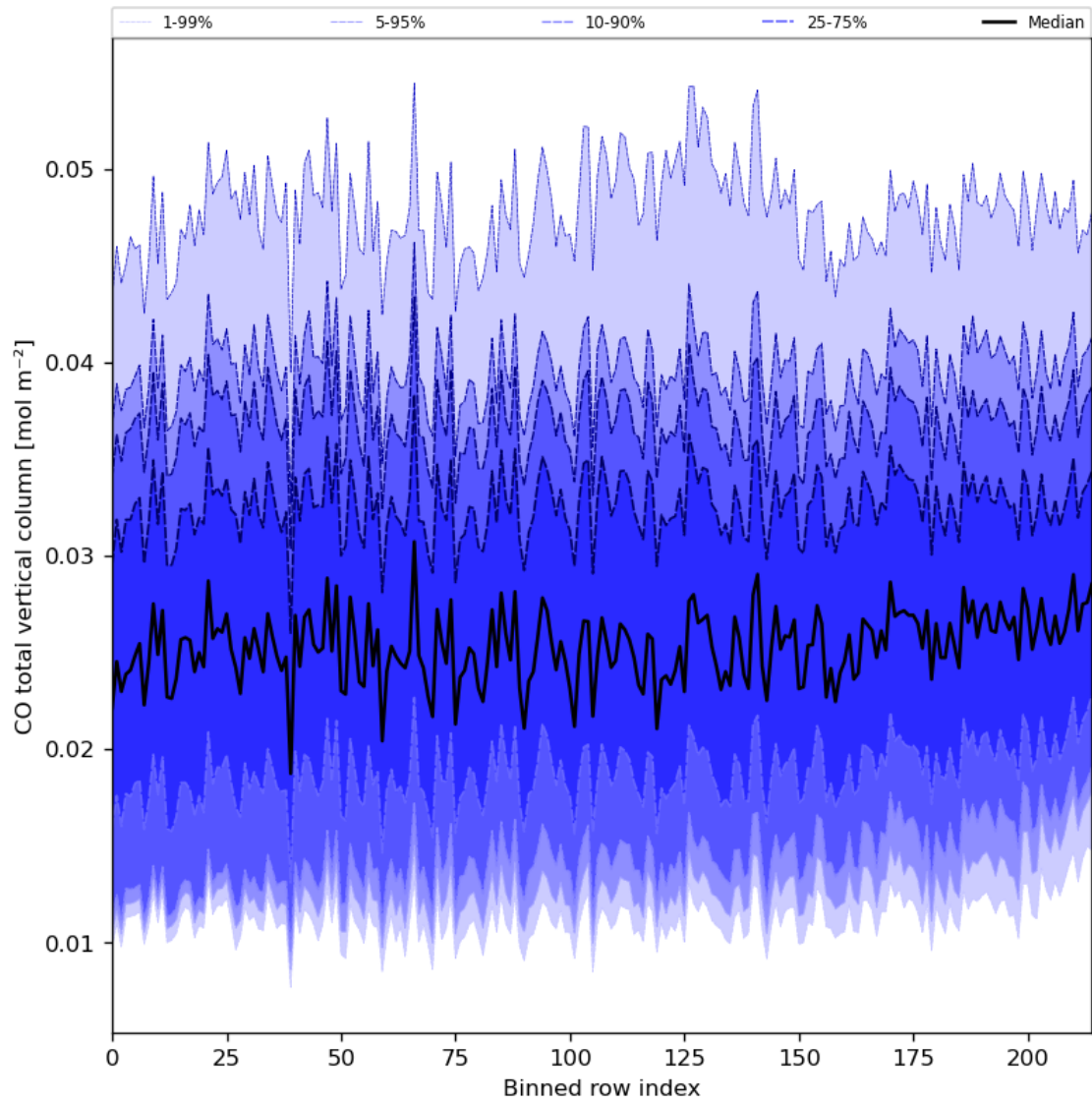
Figure 26: Along track statistics of “CO total vertical column” for 2023-11-03 to 2023-11-05
