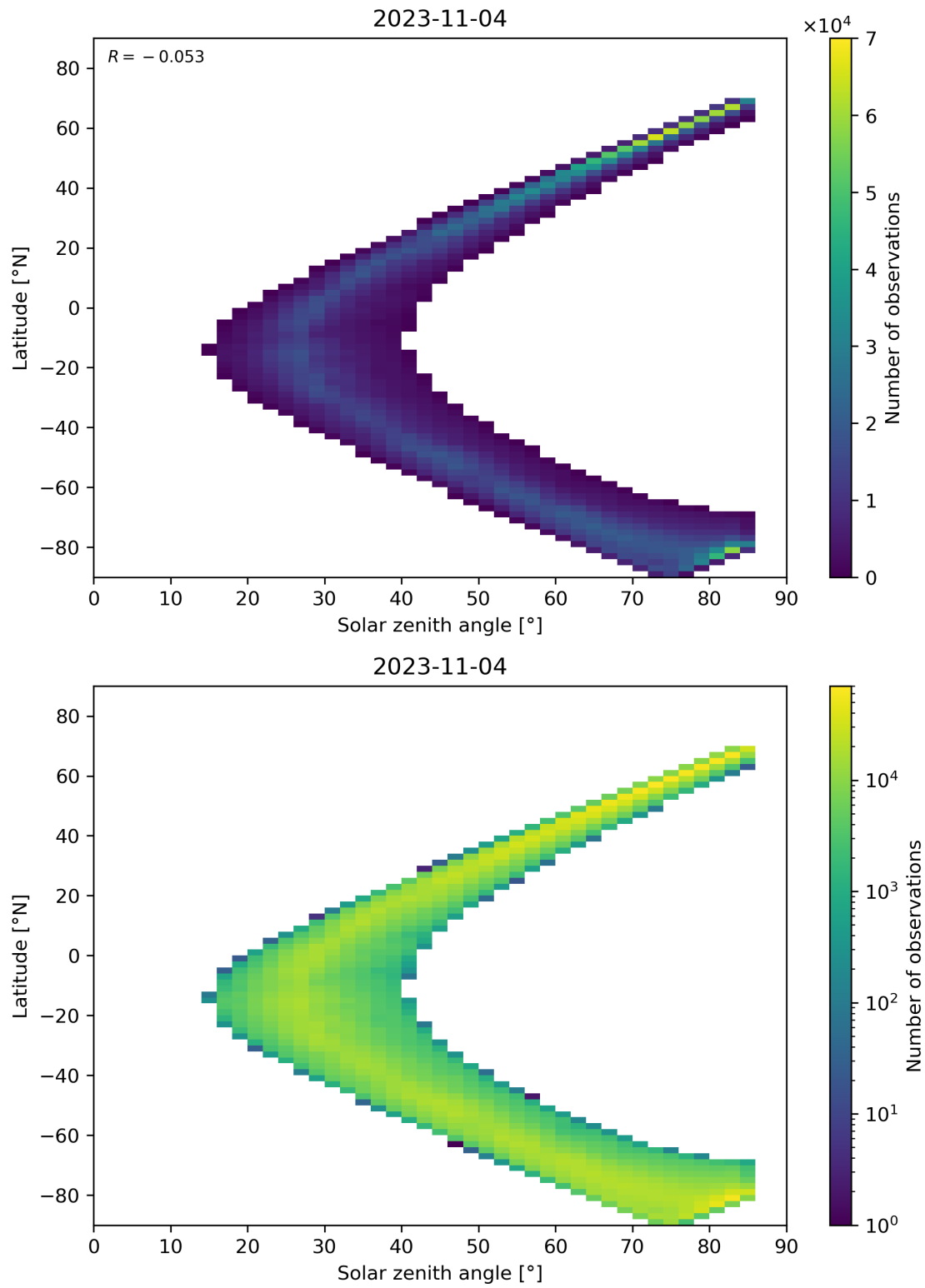
Figure 66: Scatter density plot of “Solar zenith angle” against “Latitude” for 2023-11-03 to 2023-11-05.
