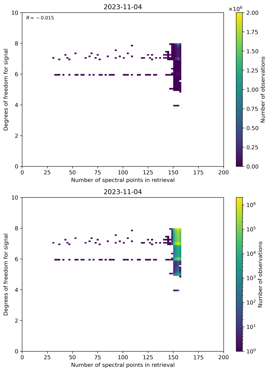
Figure 59: Scatter density plot of “Number of spectral points in retrieval” against “Degrees of freedom for signal” for 2023-11-03 to 2023-11-05.
