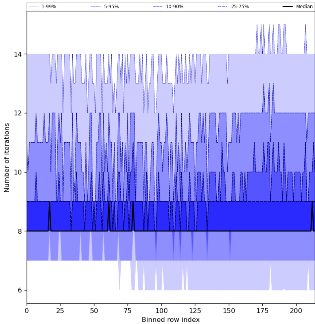
Figure 32: Along track statistics of “Number of iterations” for 2023-11-03 to 2023-11-05
