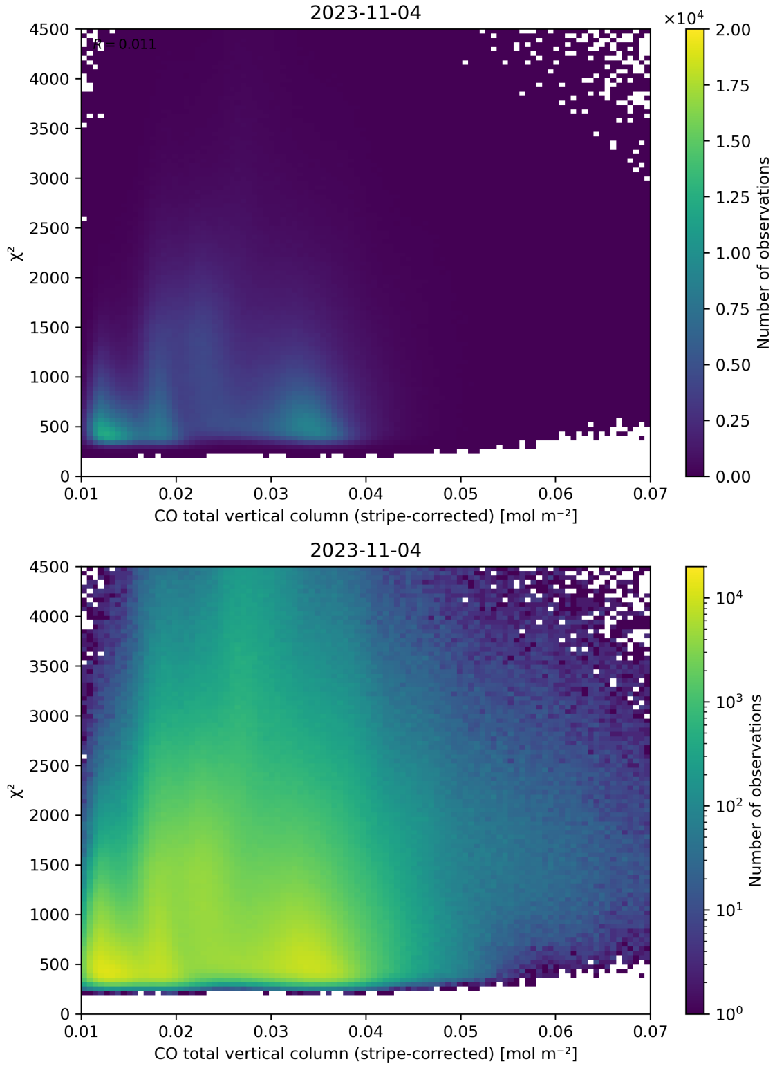
Figure 37: Scatter density plot of “CO total vertical column (stripe-corrected)” against “ \chi^2 ” for 2023-11-03 to 2023-11-05.
