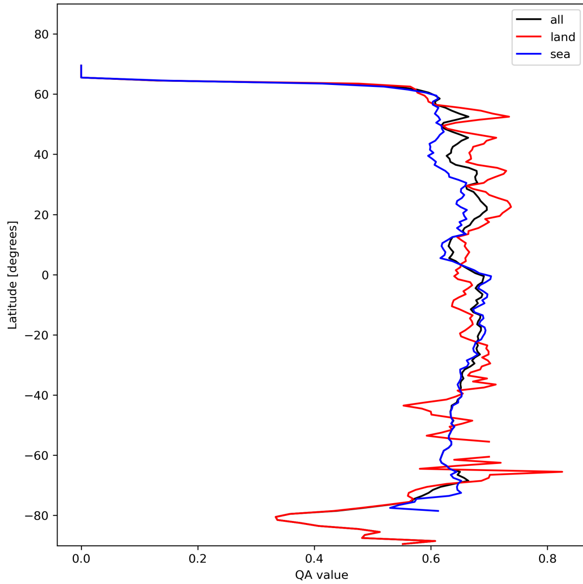
Figure 9: Zonal average of “QA value” for 2023-11-03 to 2023-11-05.
