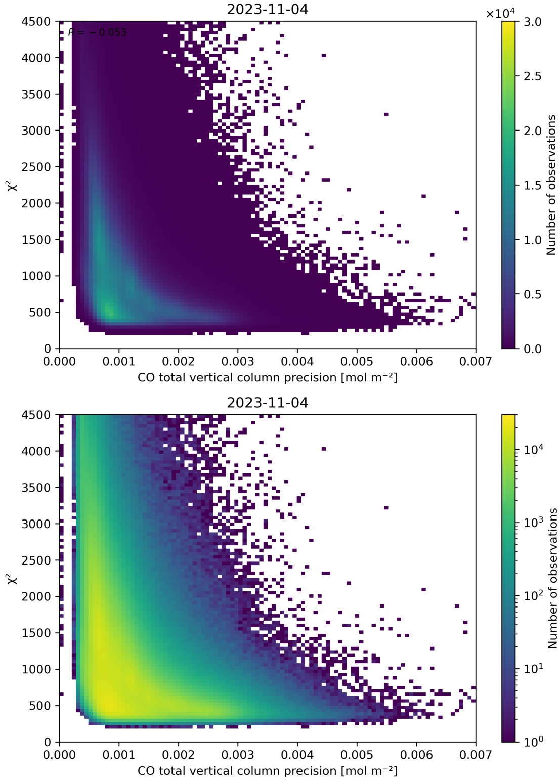
Figure 44: Scatter density plot of “CO total vertical column precision” against “ \chi^2 ” for 2023-11-03 to 2023-11-05.
