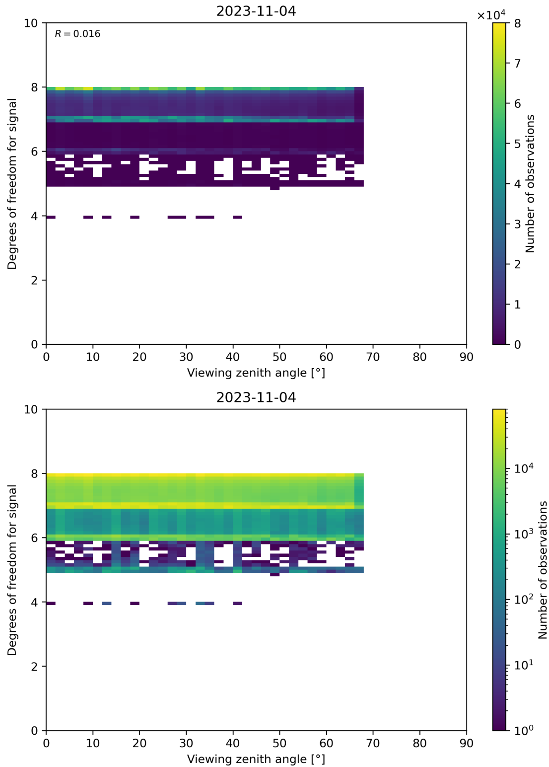
Figure 73: Scatter density plot of “Viewing zenith angle” against “Degrees of freedom for signal” for 2023-11-03 to 2023-11-05.
