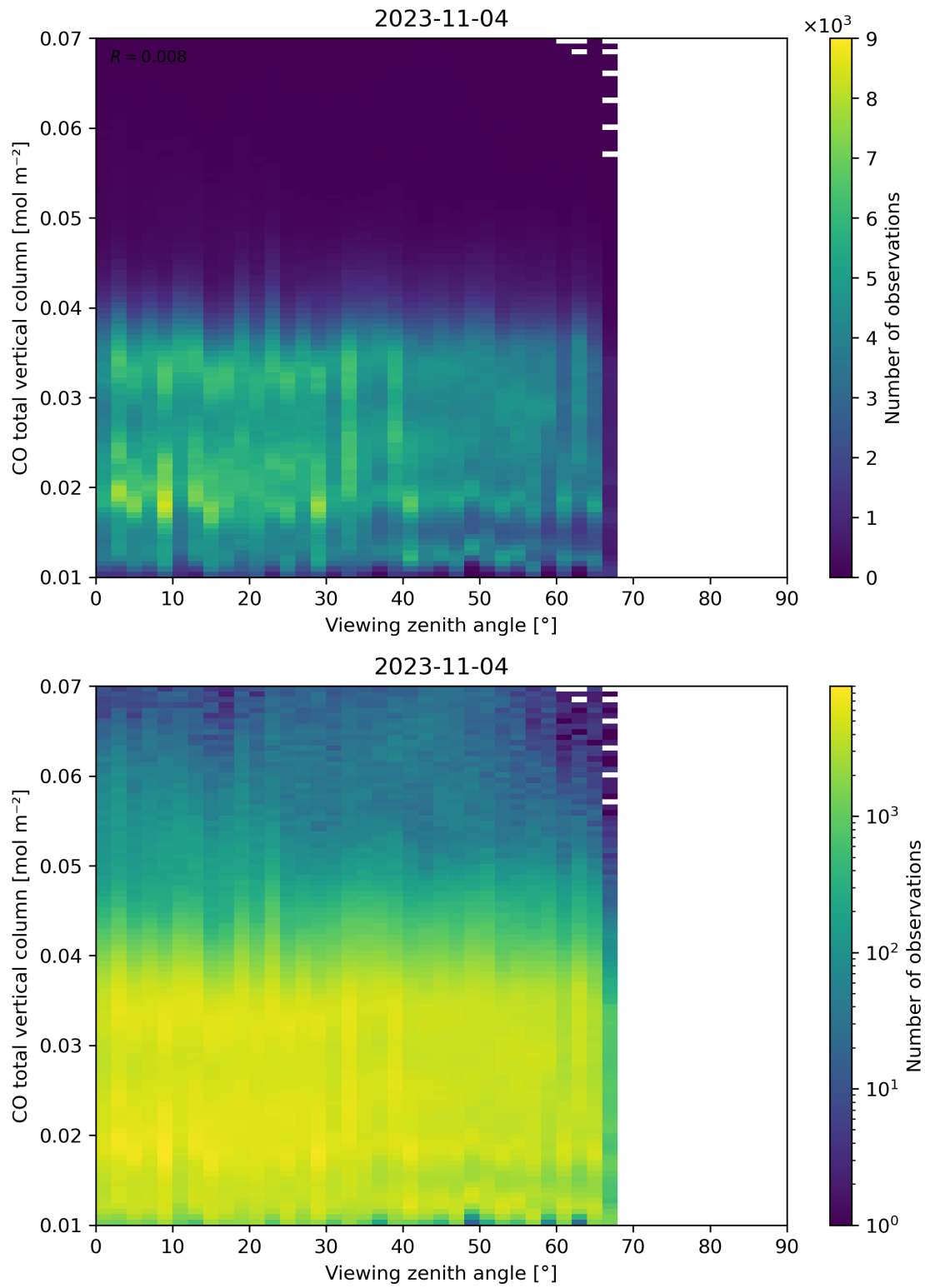
Figure 69: Scatter density plot of “Viewing zenith angle” against “CO total vertical column” for 2023-11-03 to 2023-11-05.
