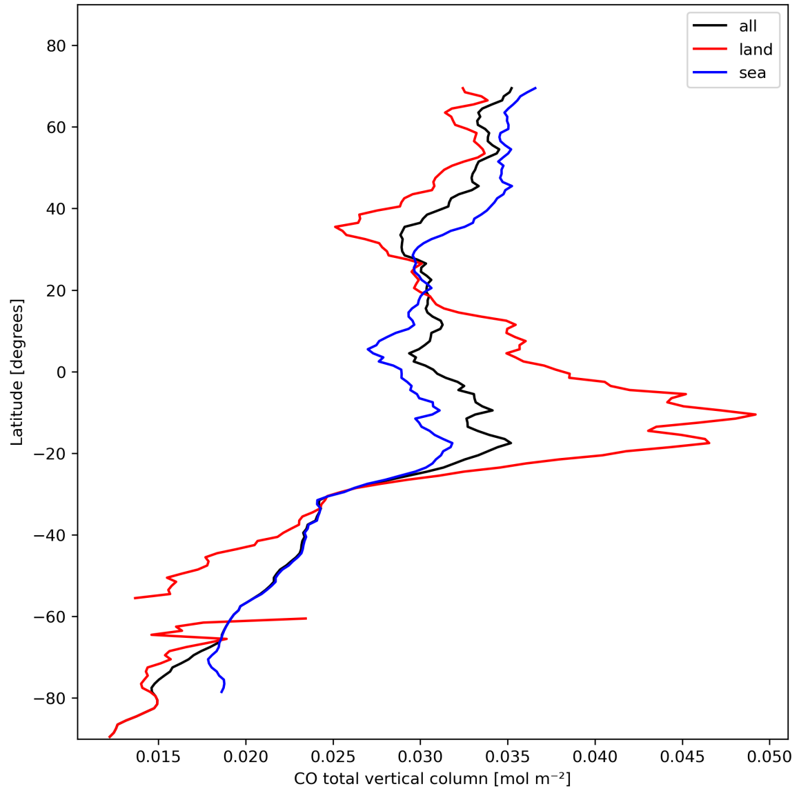
Figure 10: Zonal average of “CO total vertical column” for 2023-11-03 to 2023-11-05.
