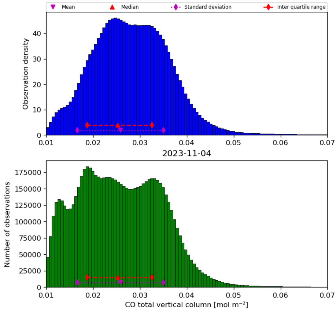
Figure 18: Histogram of “CO total vertical column” for 2023-11-03 to 2023-11-05
