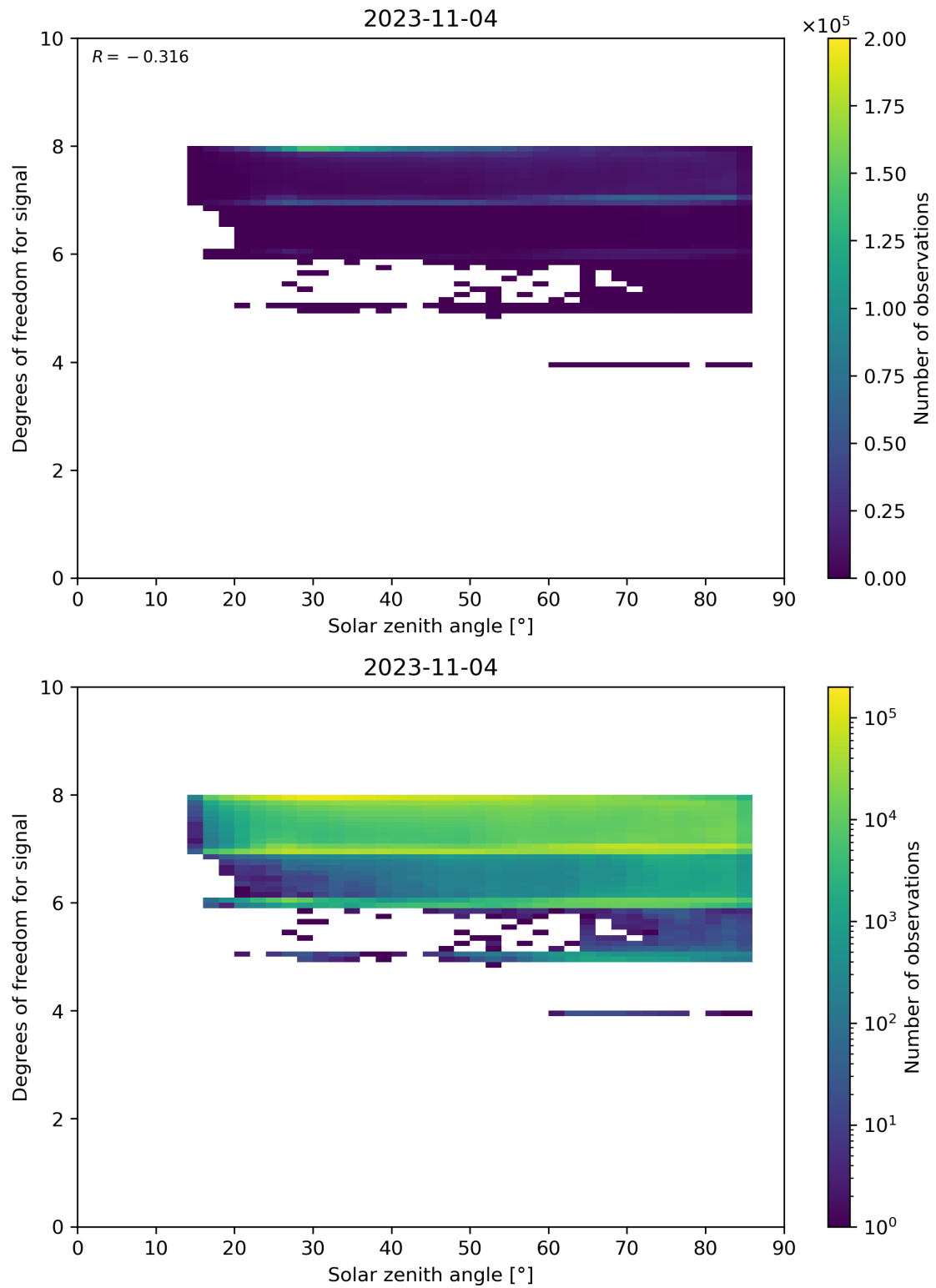
Figure 65: Scatter density plot of “Solar zenith angle” against “Degrees of freedom for signal” for 2023-11-03 to 2023-11-05.
