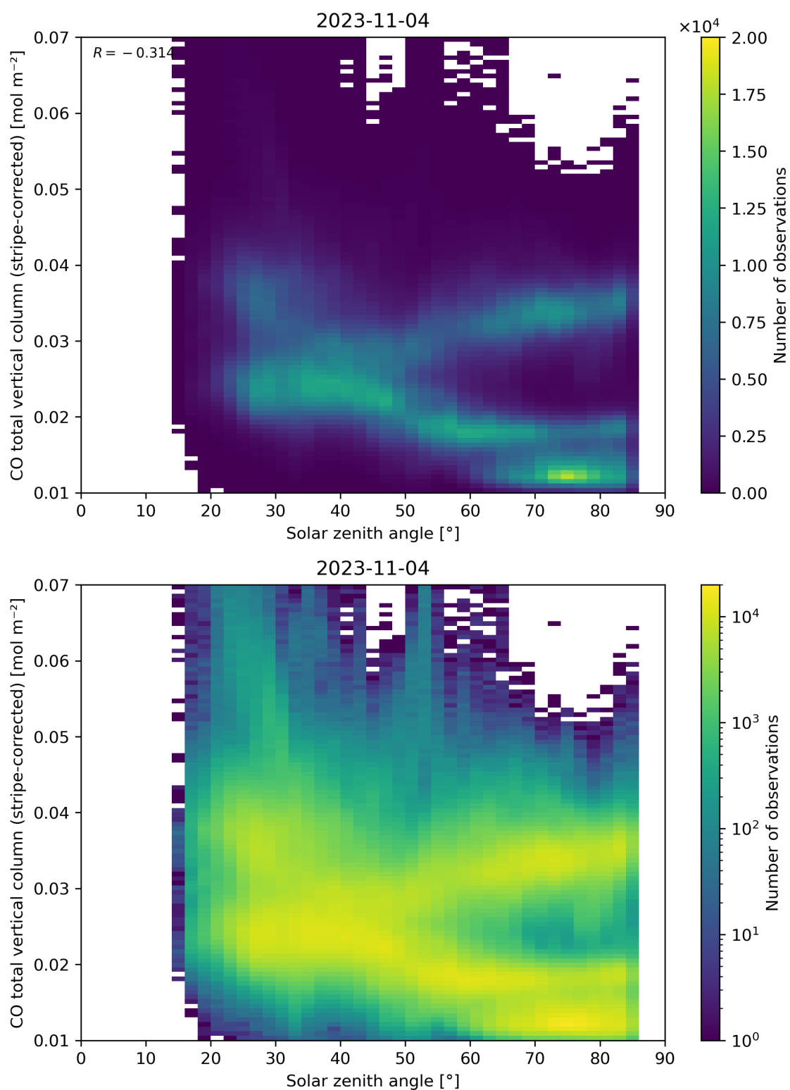
Figure 62: Scatter density plot of “Solar zenith angle” against “CO total vertical column (stripe-corrected)” for 2023-11-03 to 2023-11-05.
