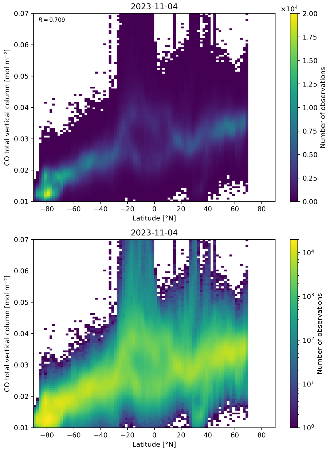
Figure 51: Scatter density plot of “Latitude” against “CO total vertical column” for 2023-11-03 to 2023-11-05.
