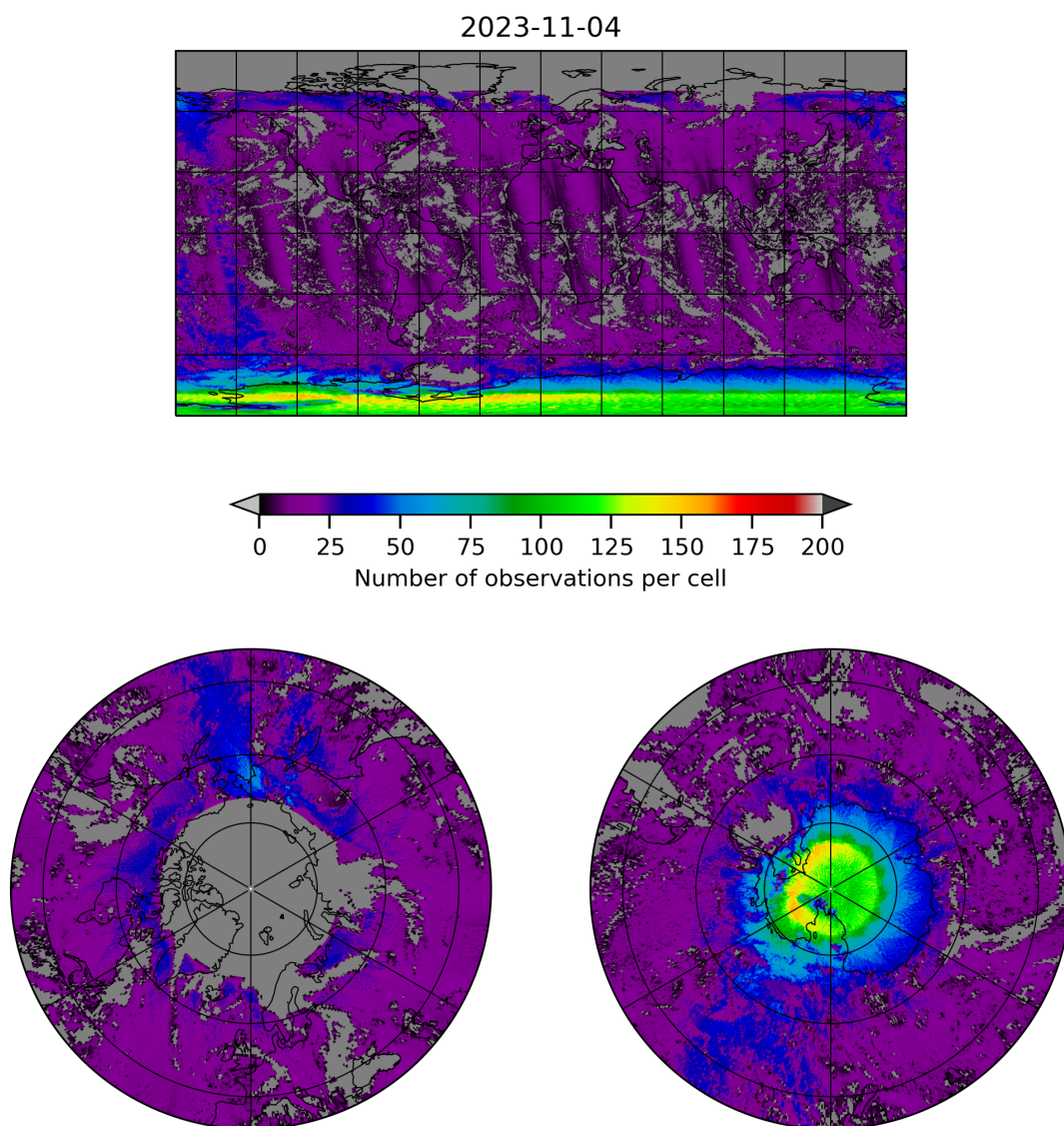
Figure 8: Map of the number of observations for 2023-11-03 to 2023-11-05
