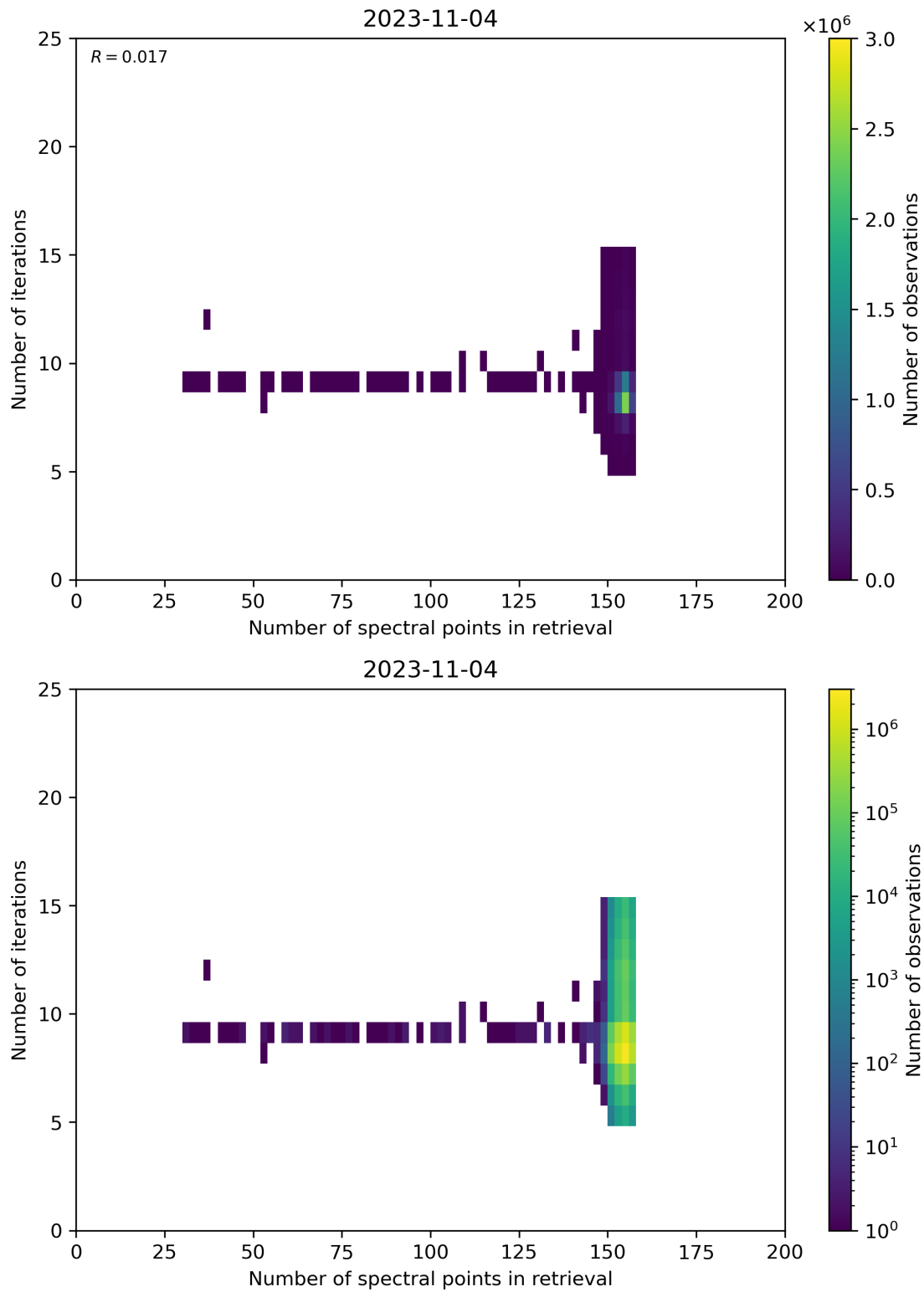
Figure 60: Scatter density plot of “Number of spectral points in retrieval” against “Number of iterations” for 2023-11-03 to 2023-11-05.
