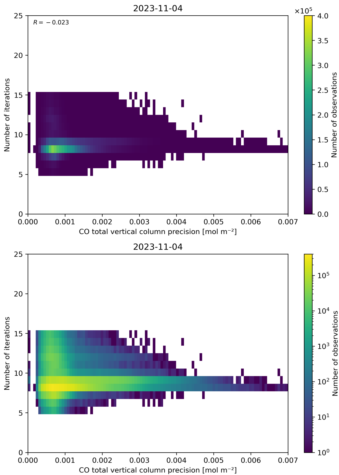
Figure 46: Scatter density plot of “CO total vertical column precision” against “Number of iterations” for 2023-11-03 to 2023-11-05.
