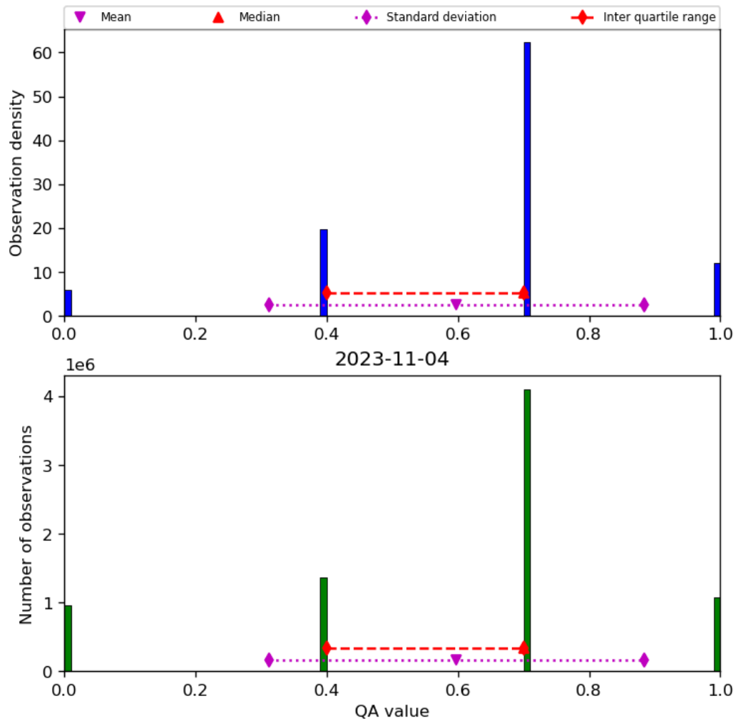
Figure 17: Histogram of “QA value” for 2023-11-03 to 2023-11-05
