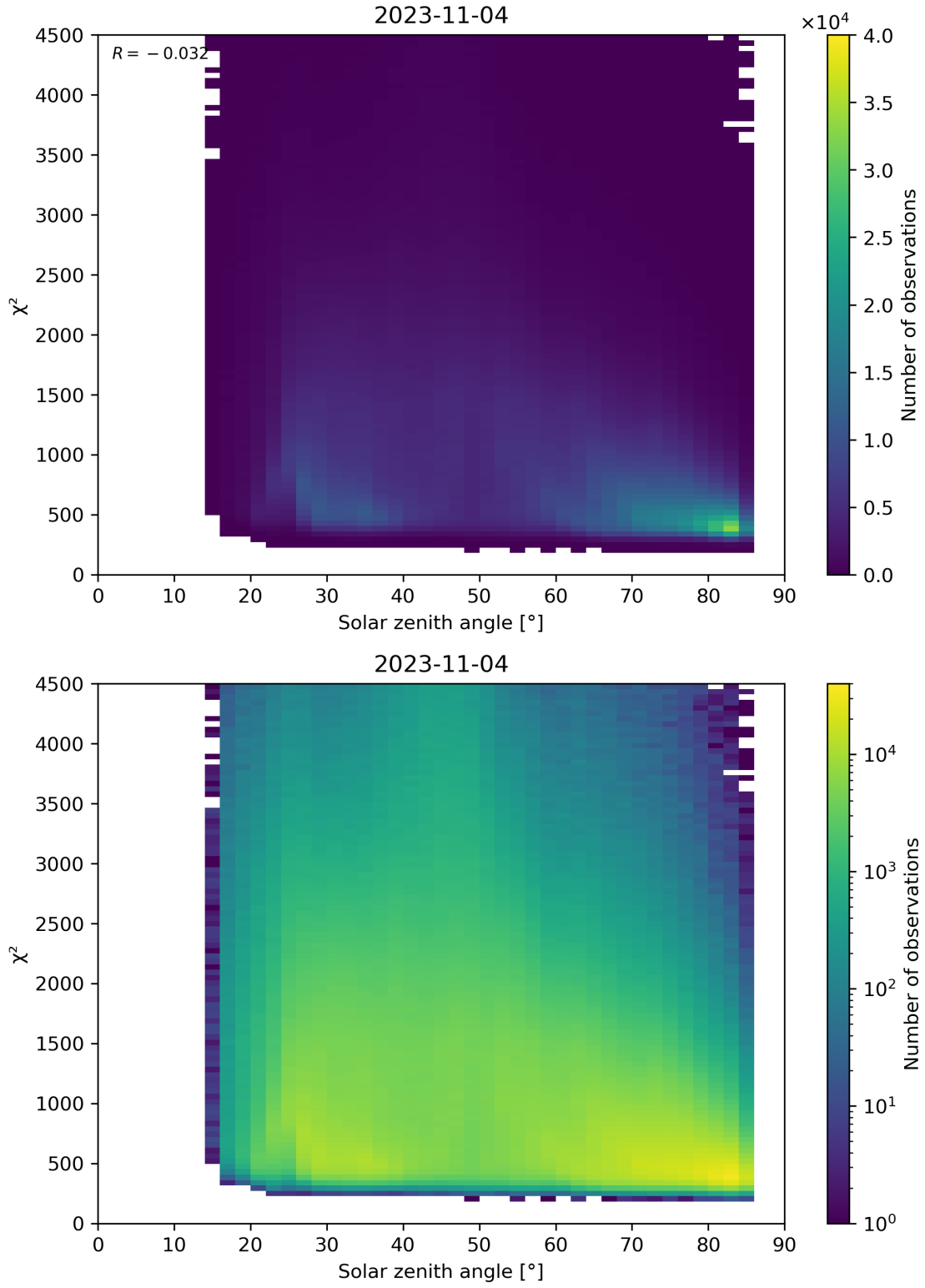
Figure 64: Scatter density plot of “Solar zenith angle” against “ \chi^2 ” for 2023-11-03 to 2023-11-05.
