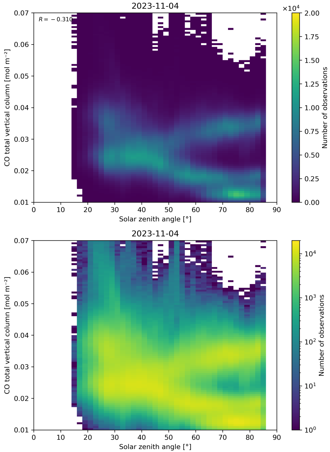
Figure 61: Scatter density plot of “Solar zenith angle” against “CO total vertical column” for 2023-11-03 to 2023-11-05.
