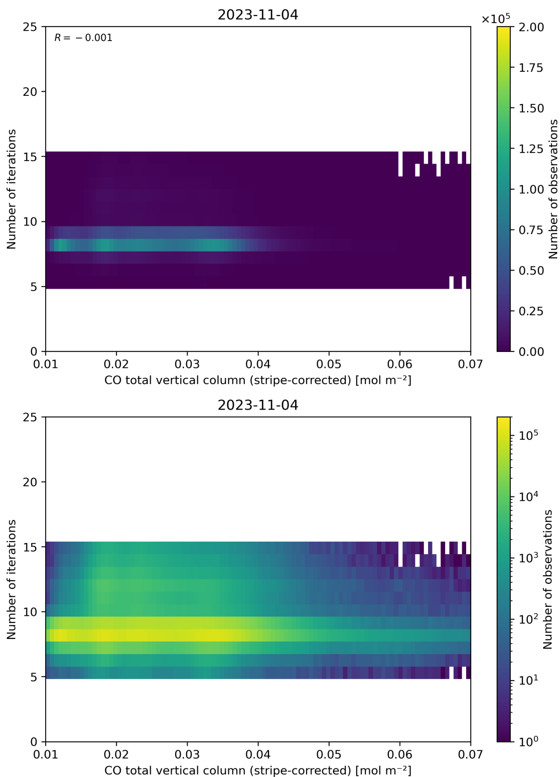
Figure 39: Scatter density plot of “CO total vertical column (stripe-corrected)” against “Number of iterations” for 2023-11-03 to 2023-11-05.
