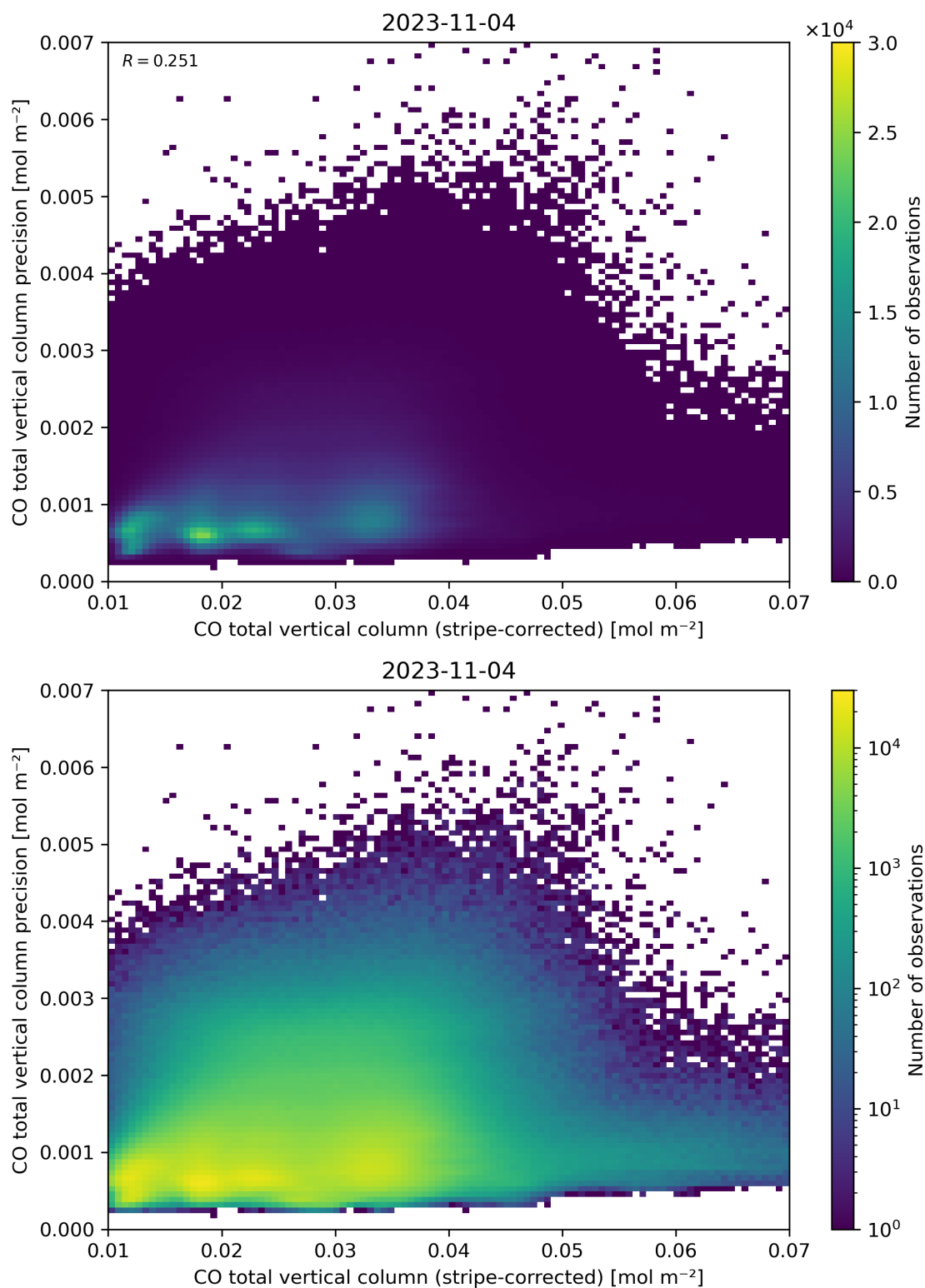
Figure 36: Scatter density plot of “CO total vertical column (stripe-corrected)” against “CO total vertical column precision” for 2023-11-03 to 2023-11-05.
