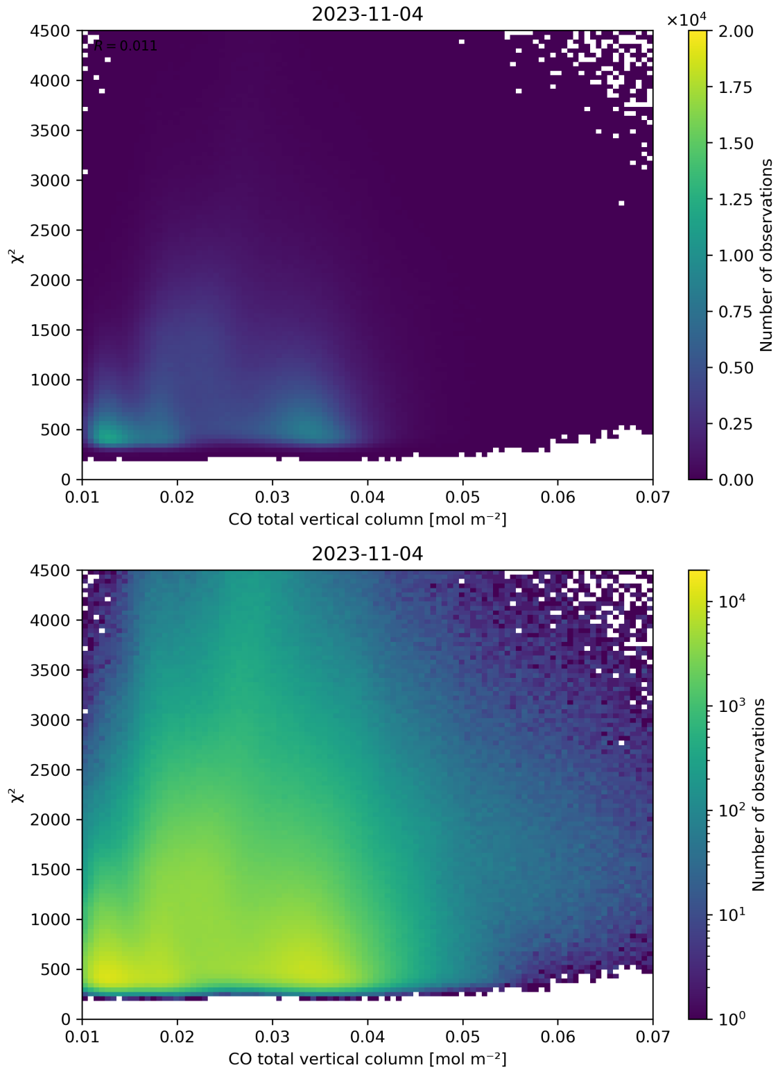
Figure 35: Scatter density plot of “CO total vertical column” against “ \chi^2 ” for 2023-11-03 to 2023-11-05.
