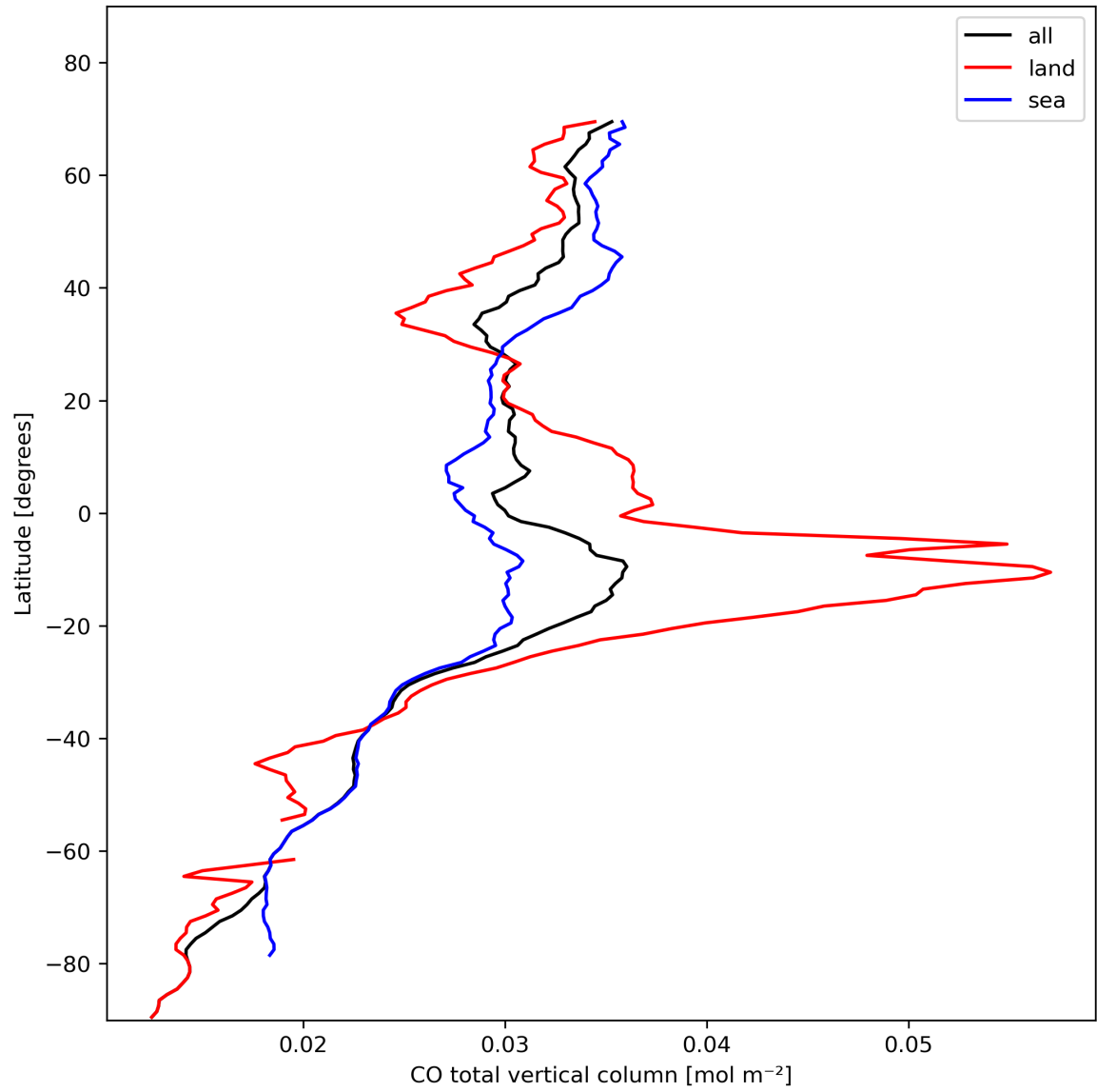
Figure 10: Zonal average of “CO total vertical column” for 2023-11-04 to 2023-11-06.
