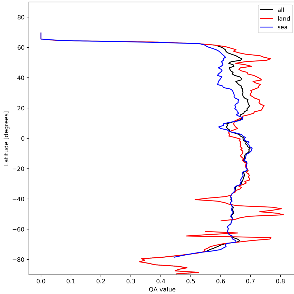
Figure 9: Zonal average of “QA value” for 2023-11-04 to 2023-11-06.
