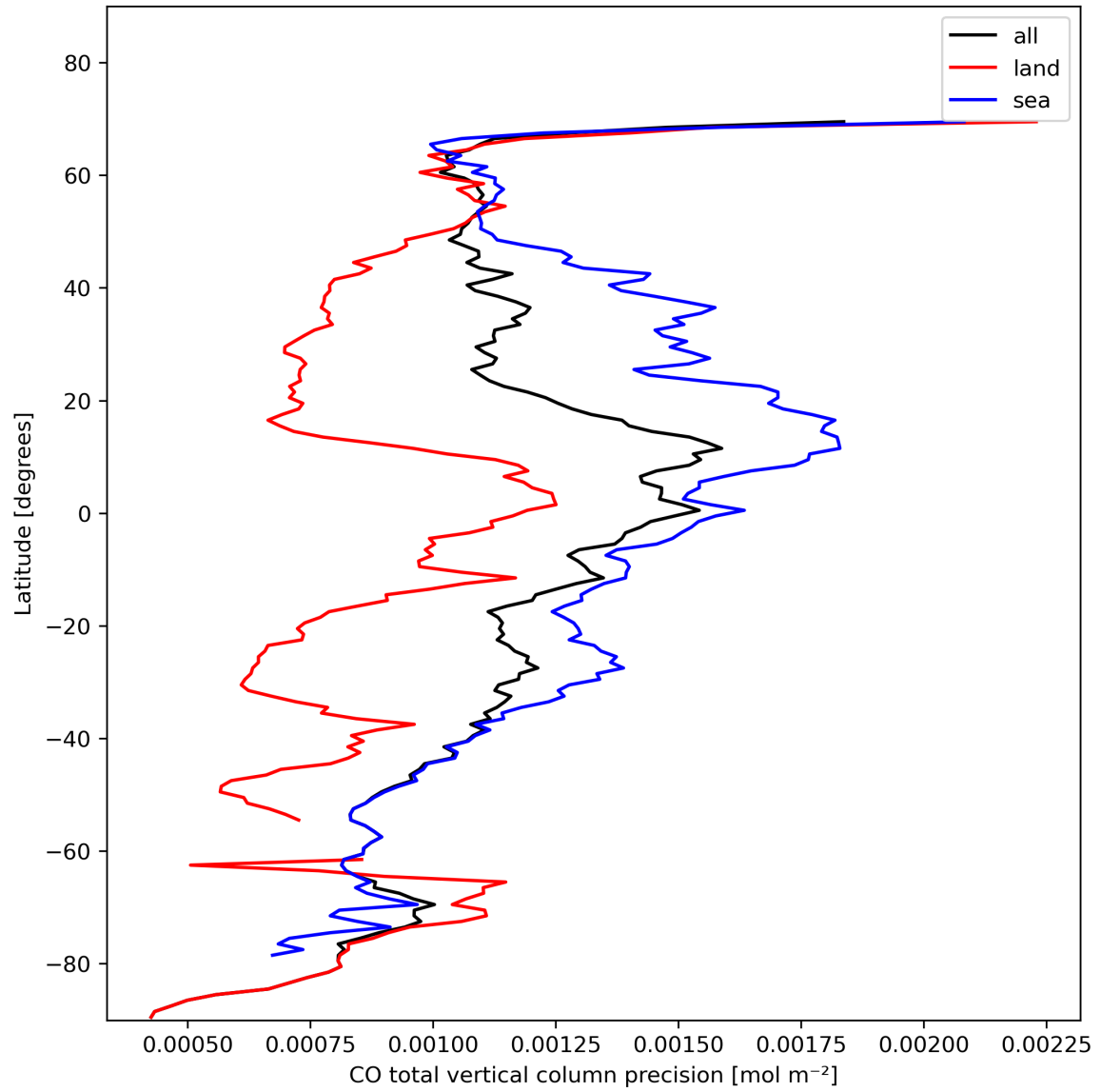
Figure 12: Zonal average of “CO total vertical column precision” for 2023-11-04 to 2023-11-06.
