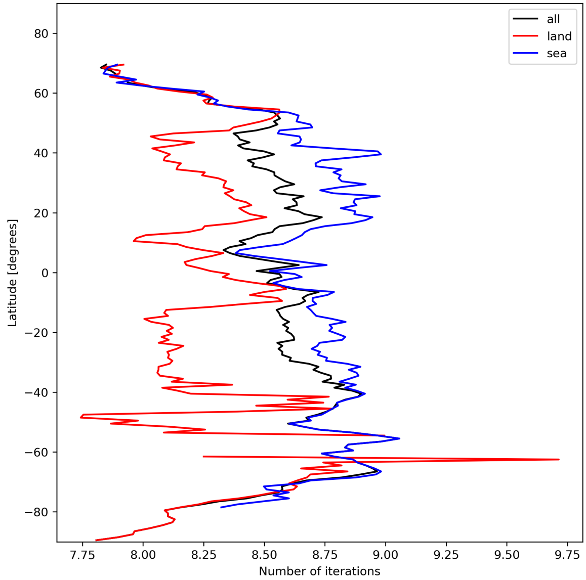
Figure 16: Zonal average of “Number of iterations” for 2023-11-04 to 2023-11-06.
