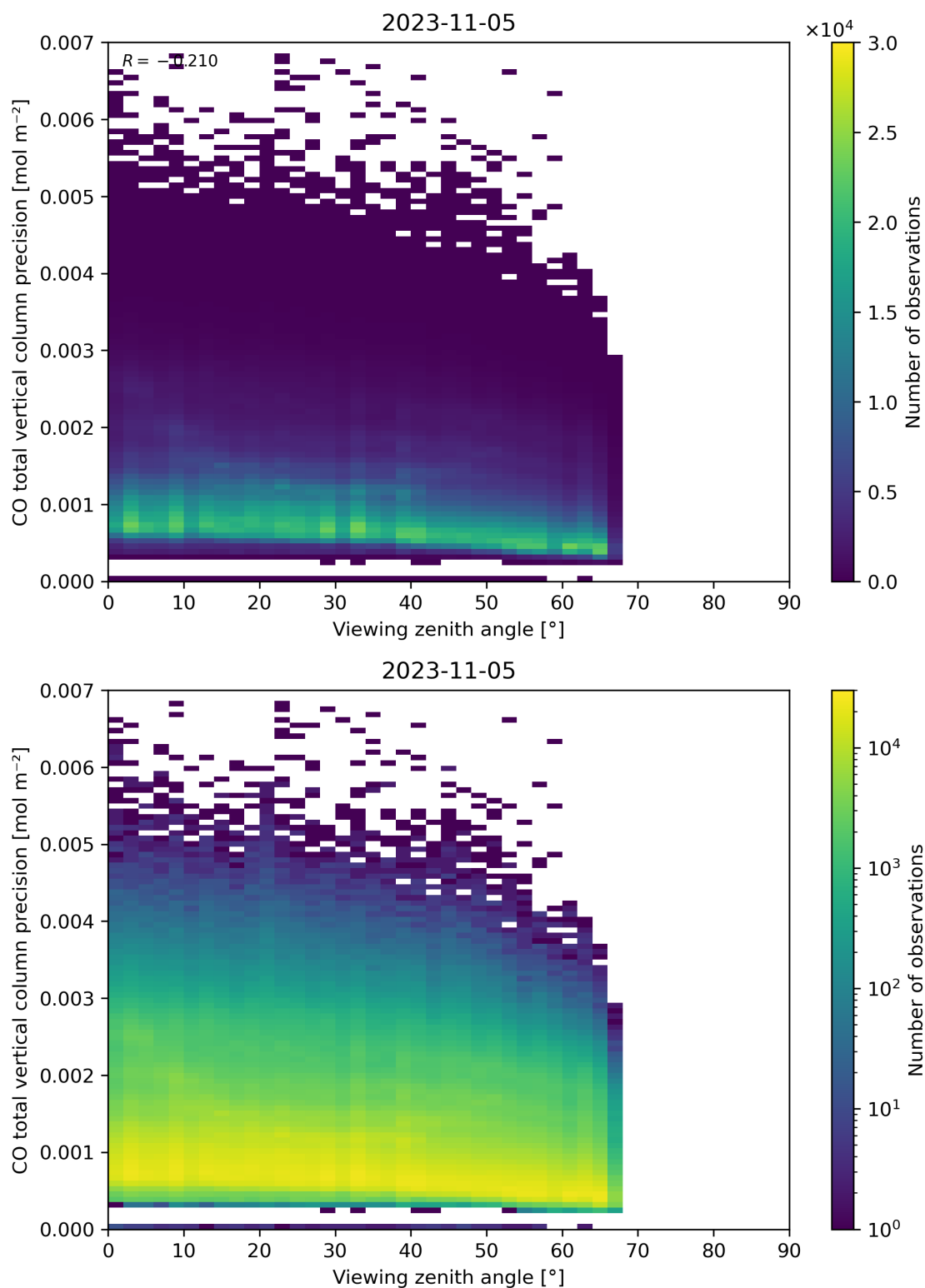
Figure 71: Scatter density plot of “Viewing zenith angle” against “CO total vertical column precision” for 2023-11-04 to 2023-11-06.
