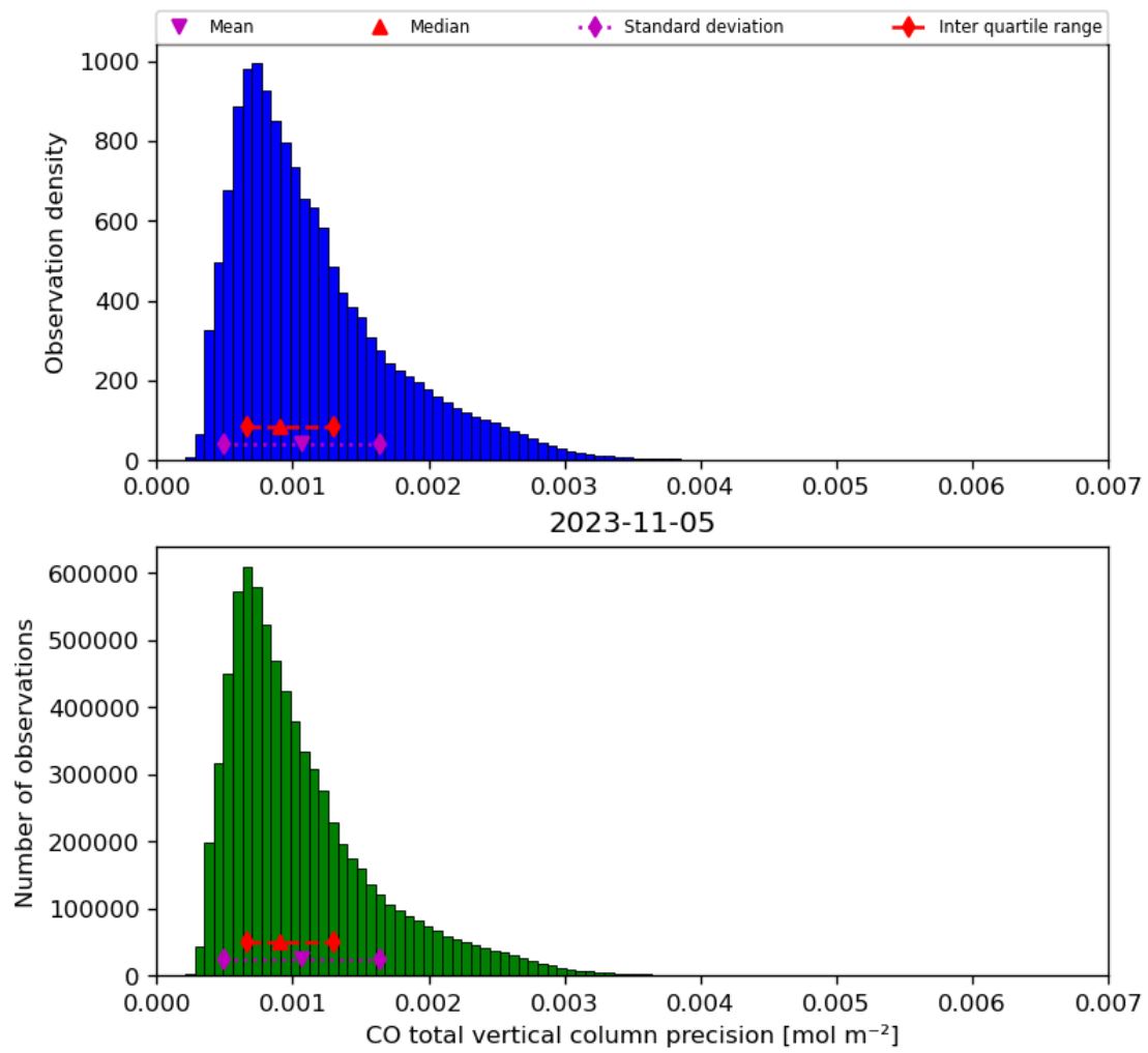
Figure 20: Histogram of “CO total vertical column precision” for 2023-11-04 to 2023-11-06
