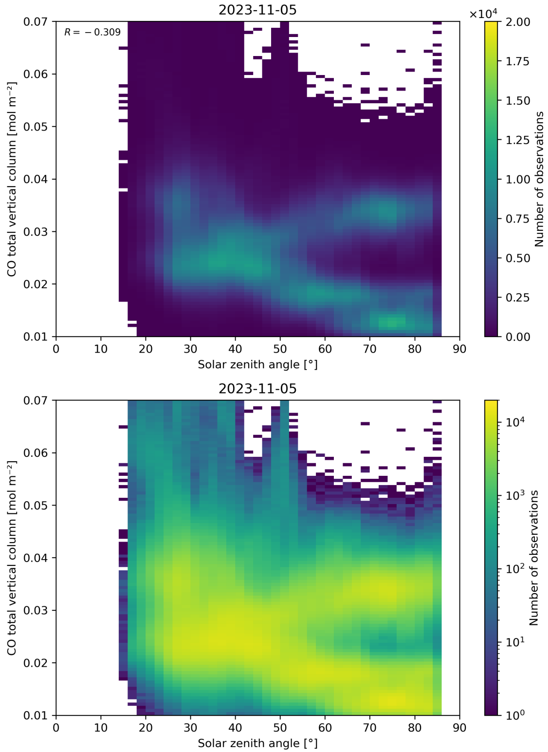
Figure 61: Scatter density plot of “Solar zenith angle” against “CO total vertical column” for 2023-11-04 to 2023-11-06.
