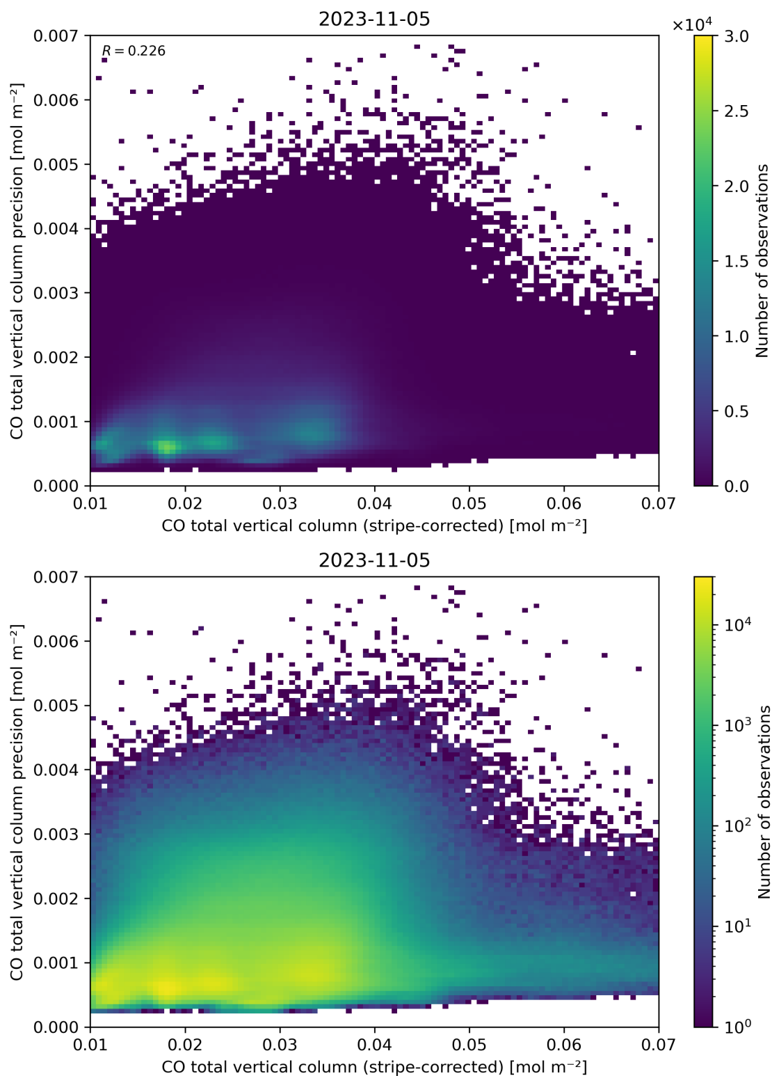
Figure 36: Scatter density plot of “CO total vertical column (stripe-corrected)” against “CO total vertical column precision” for 2023-11-04 to 2023-11-06.
