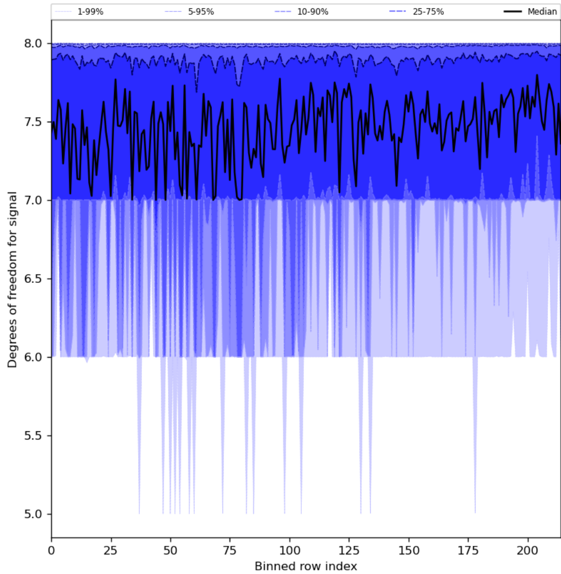
Figure 31: Along track statistics of “Degrees of freedom for signal” for 2023-11-04 to 2023-11-06
