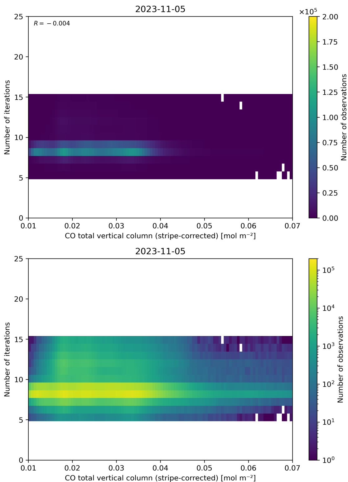
Figure 39: Scatter density plot of “CO total vertical column (stripe-corrected)” against “Number of iterations” for 2023-11-04 to 2023-11-06.
