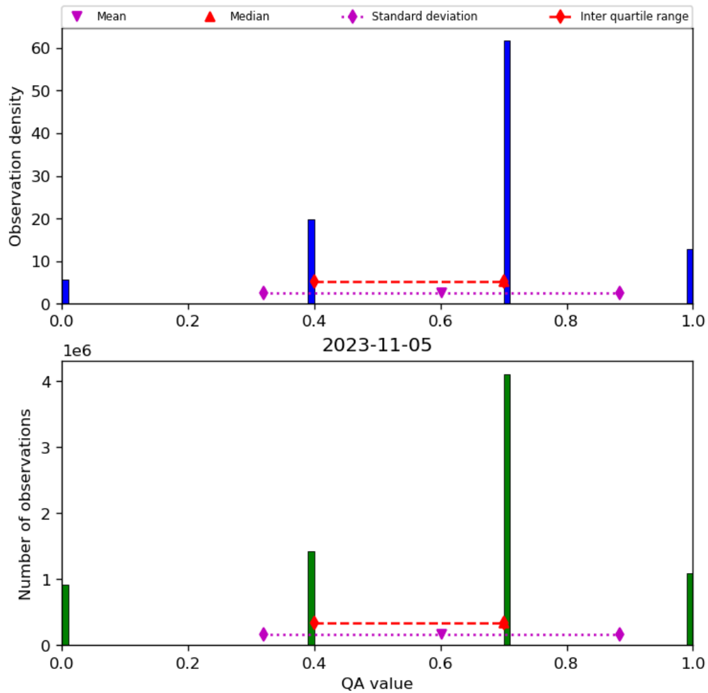
Figure 17: Histogram of “QA value” for 2023-11-04 to 2023-11-06
