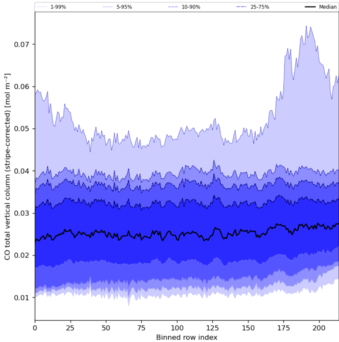
Figure 27: Along track statistics of “CO total vertical column (stripe-corrected)” for 2023-11-04 to 2023-11-06
