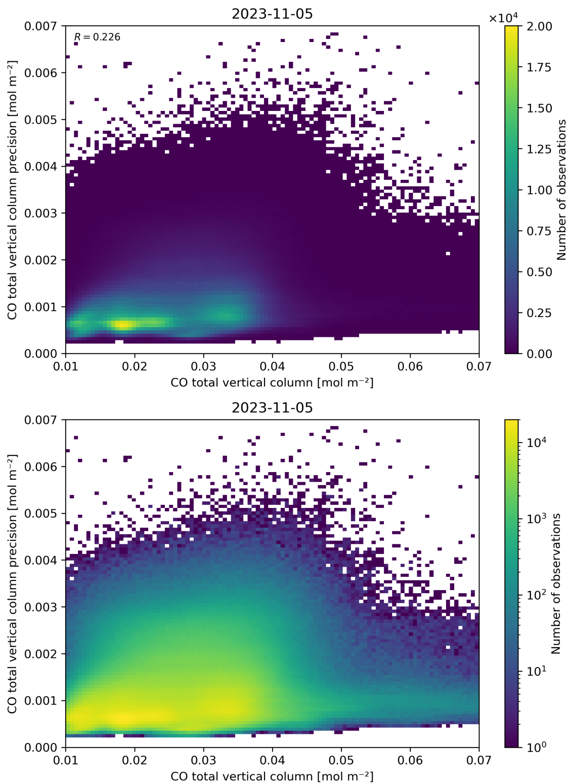
Figure 34: Scatter density plot of “CO total vertical column” against “CO total vertical column precision” for 2023-11-04 to 2023-11-06.
