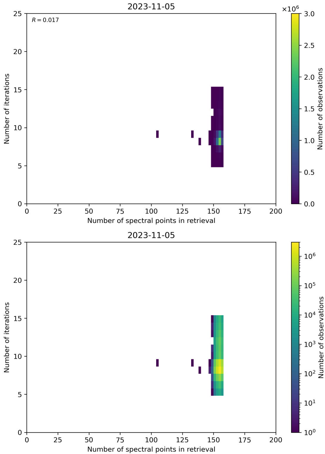
Figure 60: Scatter density plot of “Number of spectral points in retrieval” against “Number of iterations” for 2023-11-04 to 2023-11-06.
