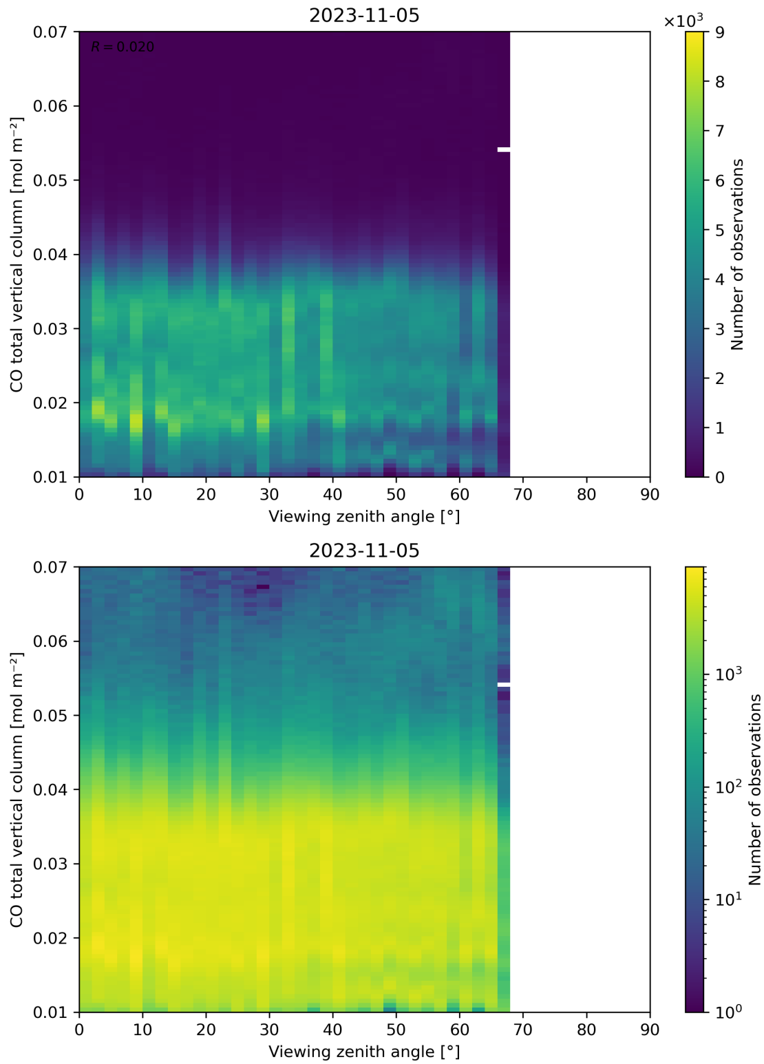
Figure 69: Scatter density plot of “Viewing zenith angle” against “CO total vertical column” for 2023-11-04 to 2023-11-06.
