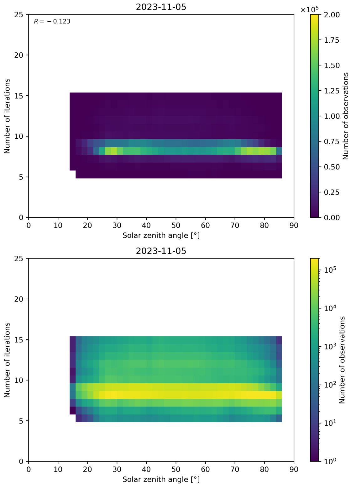
Figure 67: Scatter density plot of “Solar zenith angle” against “Number of iterations” for 2023-11-04 to 2023-11-06.
