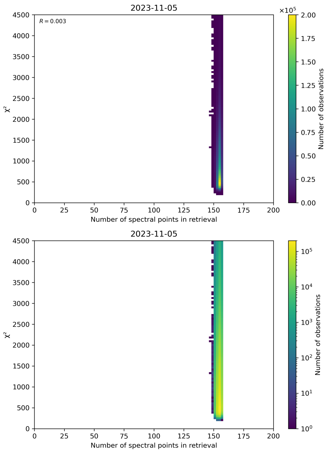
Figure 58: Scatter density plot of “Number of spectral points in retrieval” against “ \chi^2 ” for 2023-11-04 to 2023-11-06.
