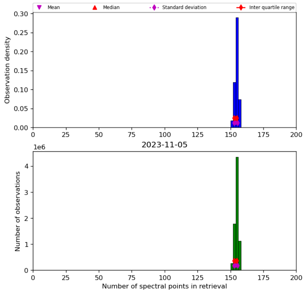
Figure 21: Histogram of “Number of spectral points in retrieval” for 2023-11-04 to 2023-11-06
