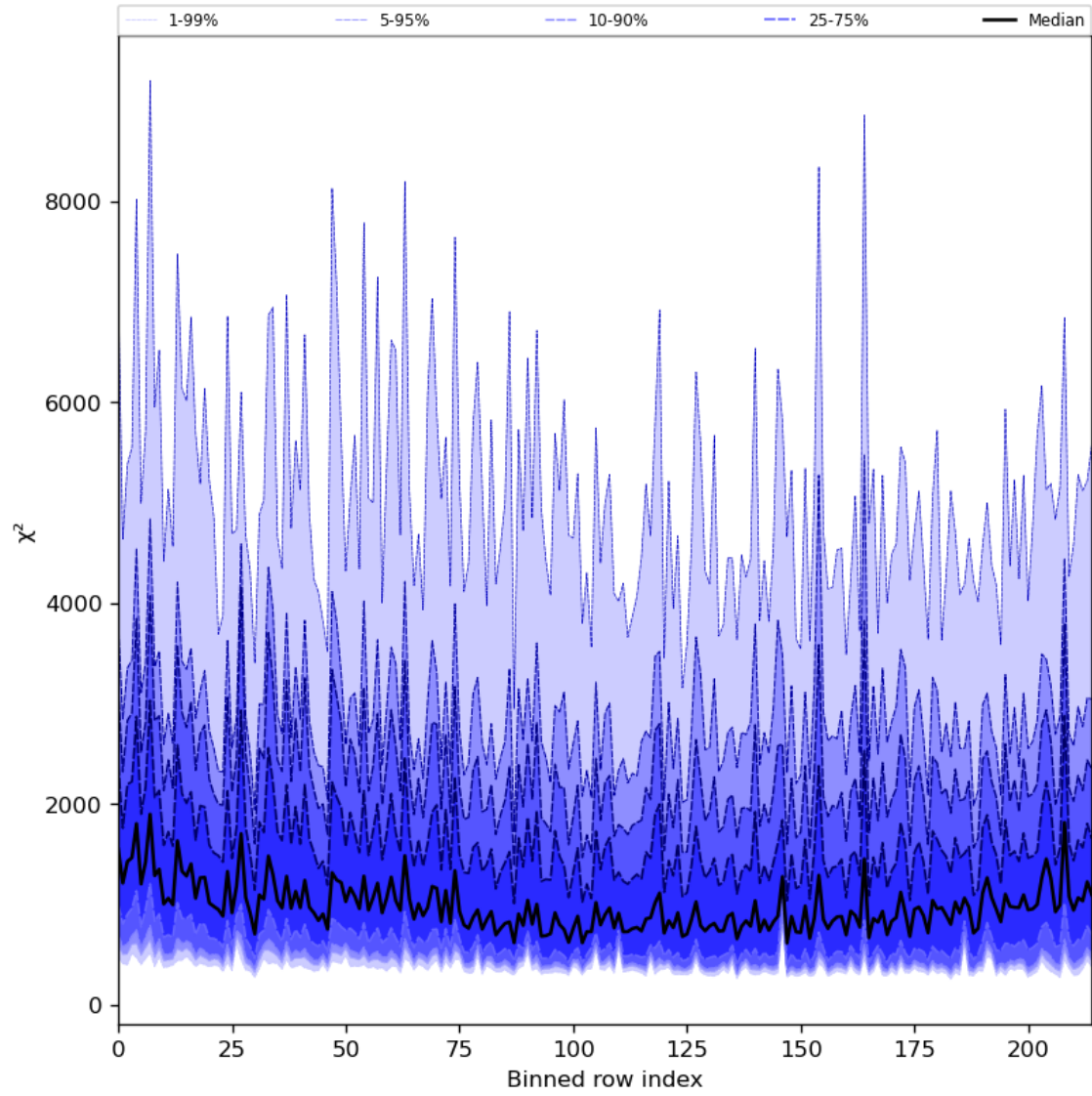
Figure 30: Along track statistics of “ \chi^2 ” for 2023-11-04 to 2023-11-06
