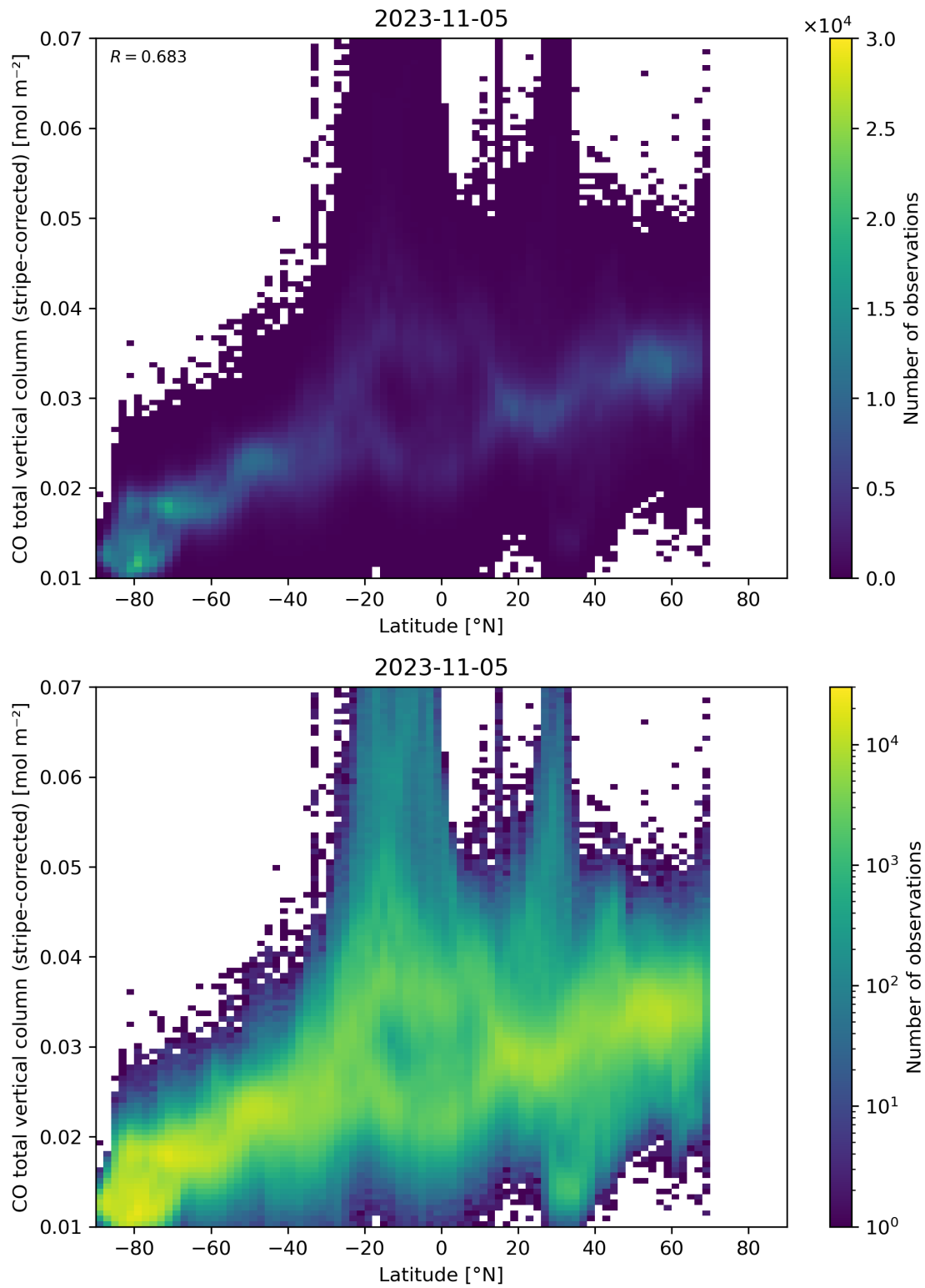
Figure 52: Scatter density plot of “Latitude” against “CO total vertical column (stripe-corrected)” for 2023-11-04 to 2023-11-06.
