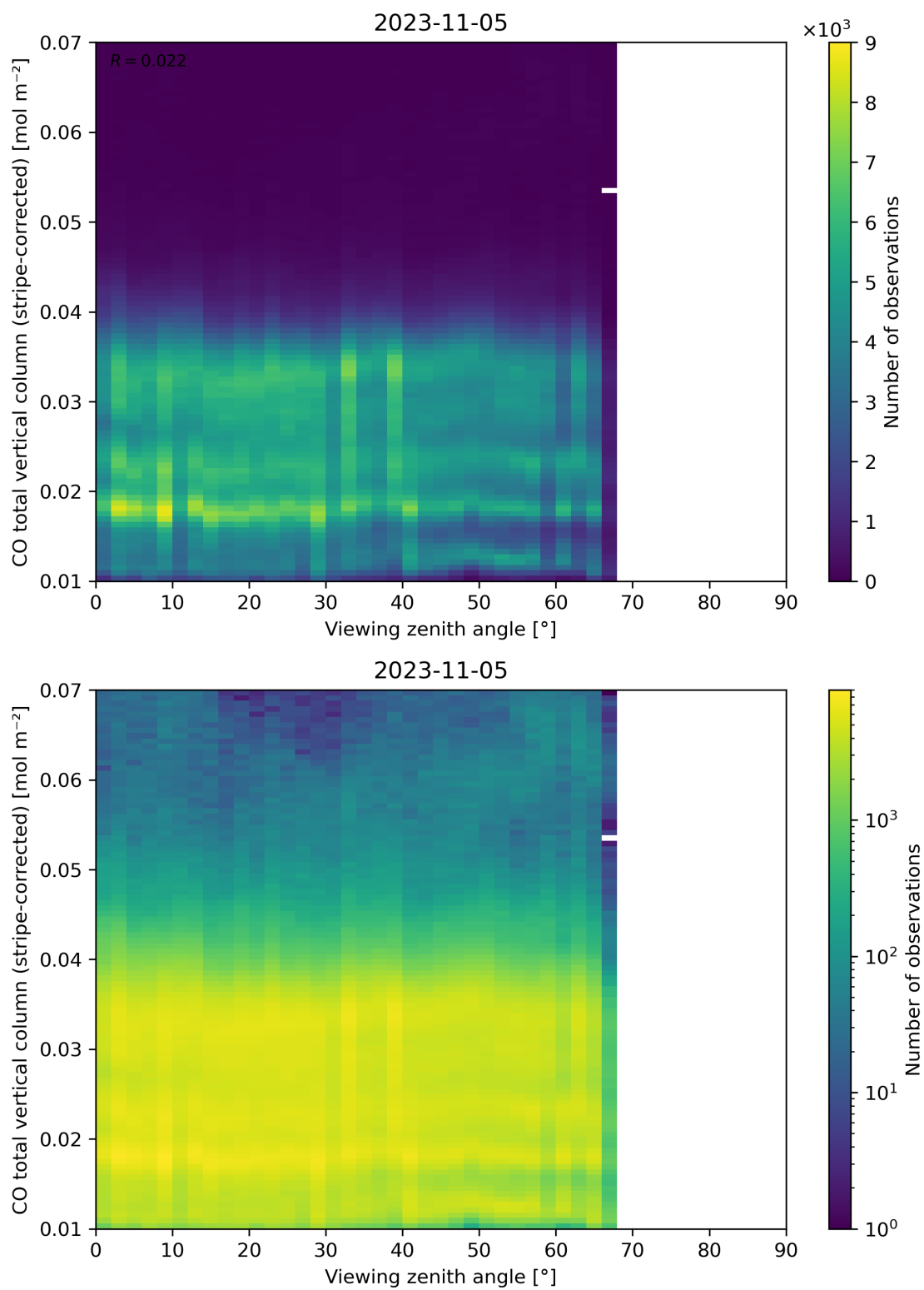
Figure 70: Scatter density plot of “Viewing zenith angle” against “CO total vertical column (stripe-corrected)” for 2023-11-04 to 2023-11-06.
