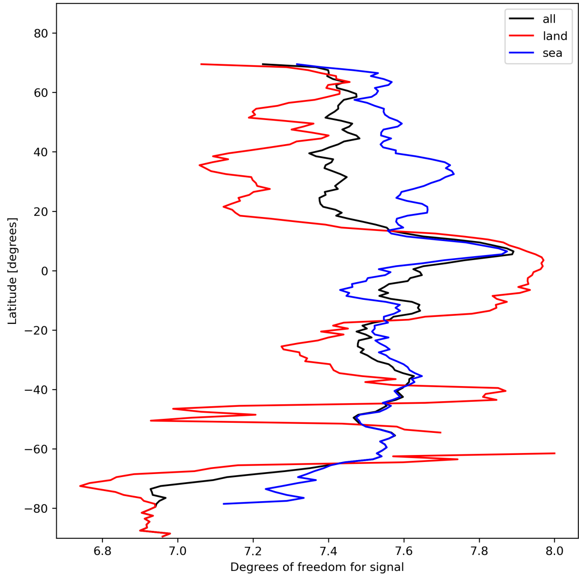
Figure 15: Zonal average of “Degrees of freedom for signal” for 2023-11-04 to 2023-11-06.
