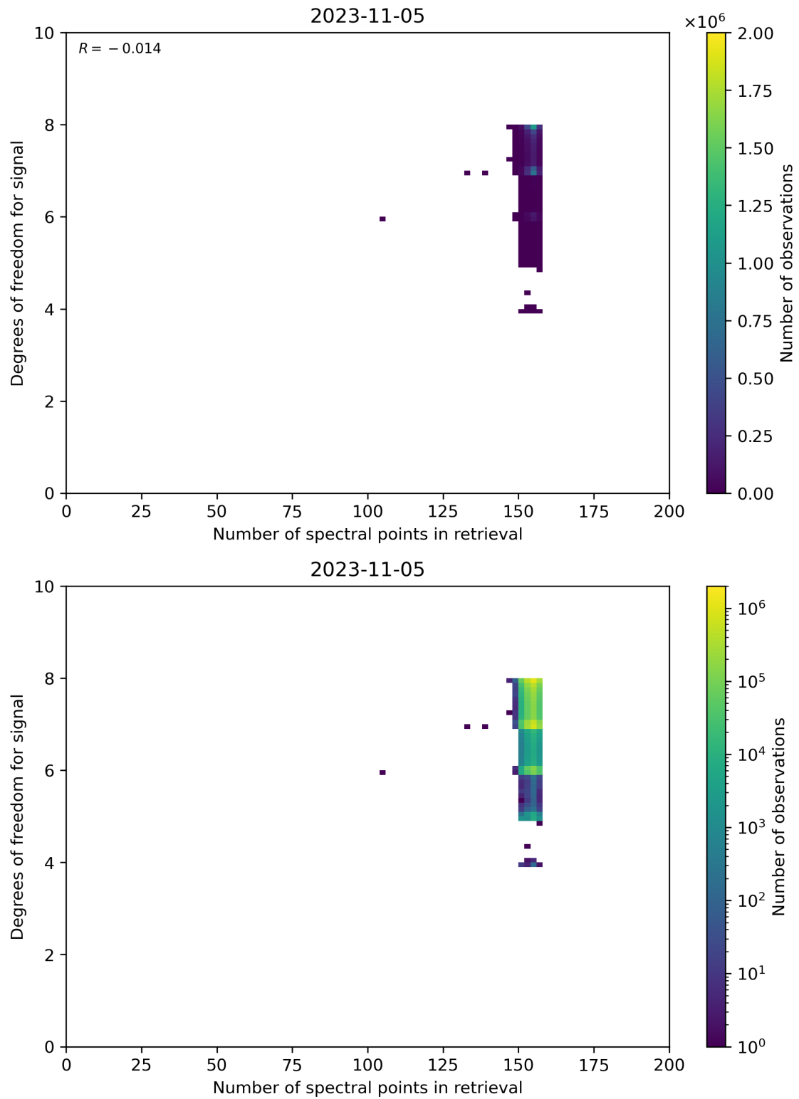
Figure 59: Scatter density plot of “Number of spectral points in retrieval” against “Degrees of freedom for signal” for 2023-11-04 to 2023-11-06.
