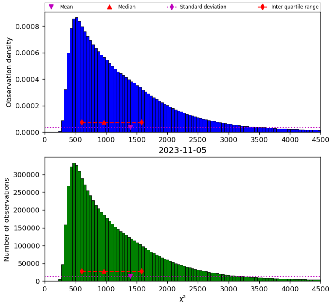
Figure 22: Histogram of “ \chi^2 ” for 2023-11-04 to 2023-11-06
