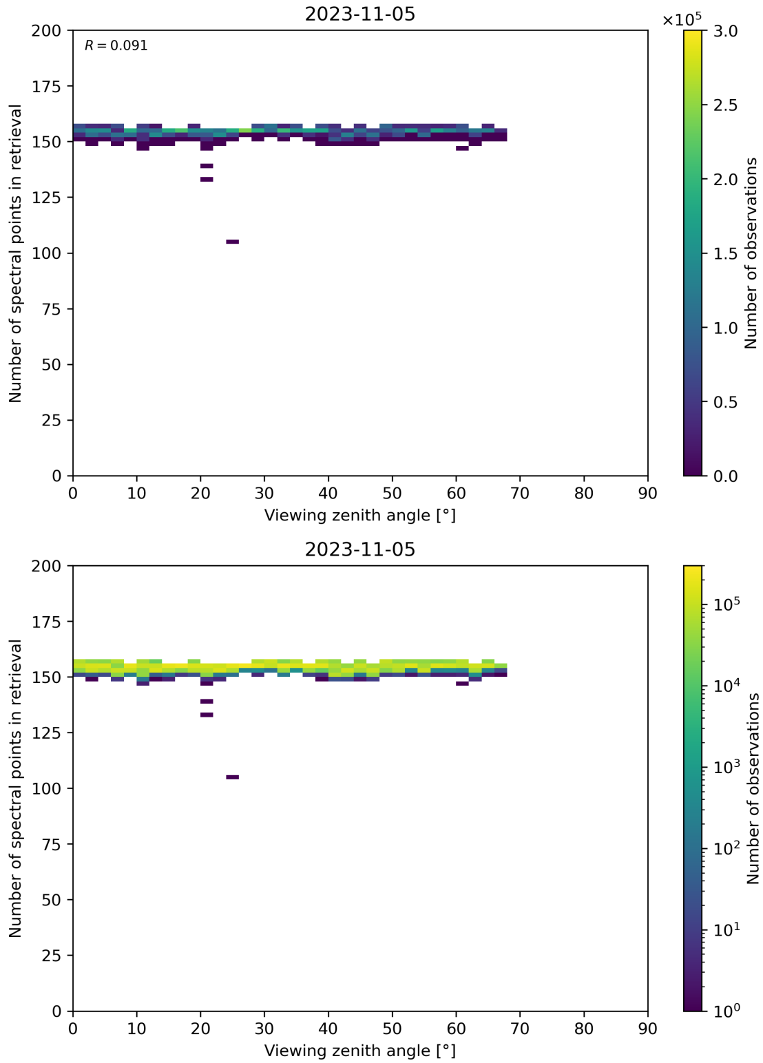
Figure 76: Scatter density plot of “Viewing zenith angle” against “Number of spectral points in retrieval” for 2023-11-04 to 2023-11-06.
