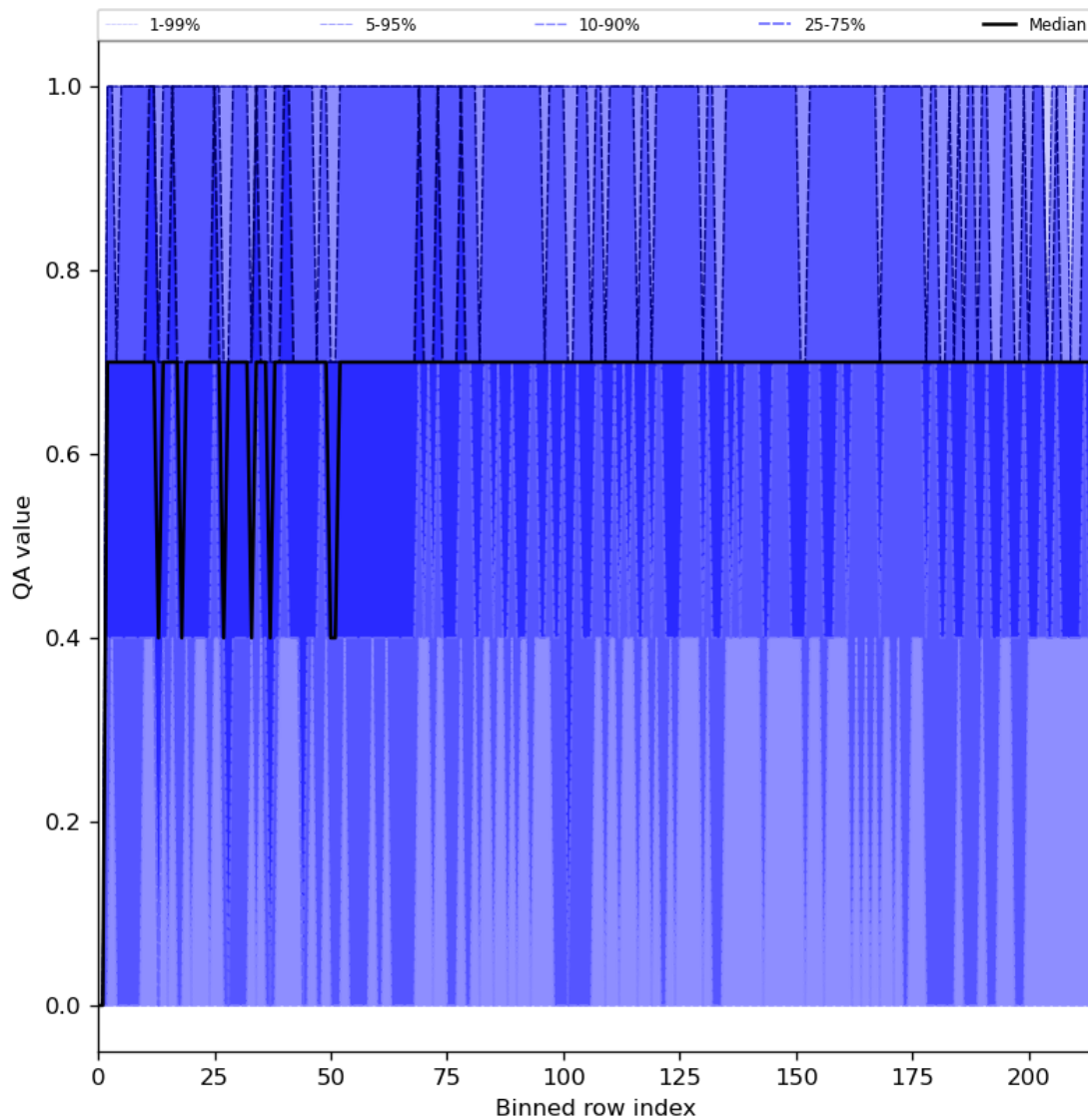
Figure 25: Along track statistics of “QA value” for 2023-11-04 to 2023-11-06
