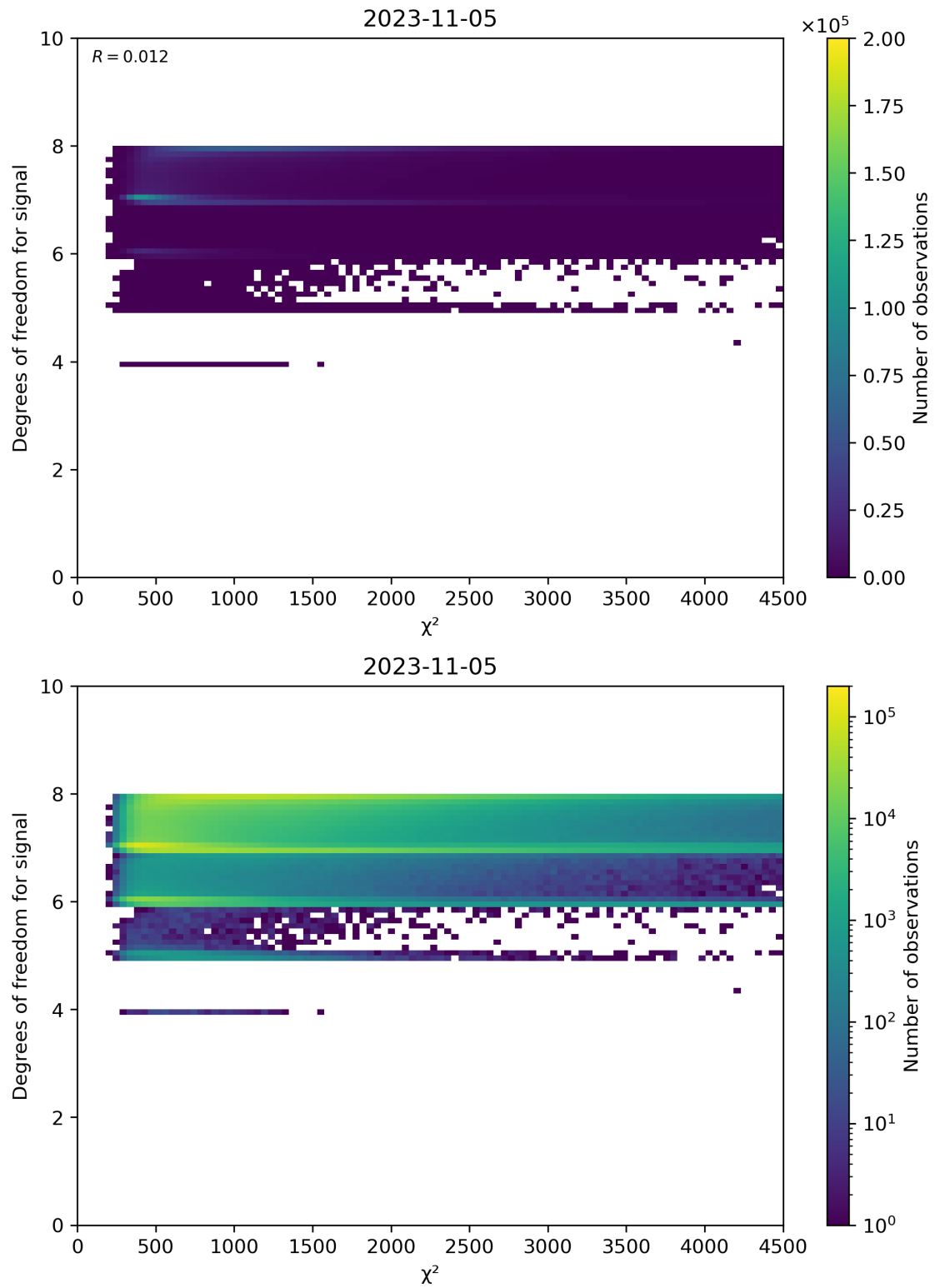
Figure 48: Scatter density plot of " \chi^2 " against "Degrees of freedom for signal" for 2023-11-04 to 2023-11-06.
