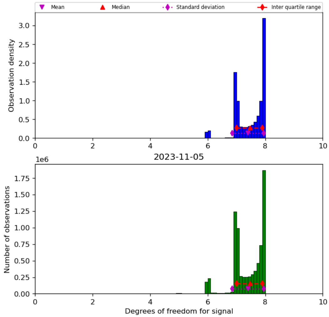
Figure 23: Histogram of “Degrees of freedom for signal” for 2023-11-04 to 2023-11-06
