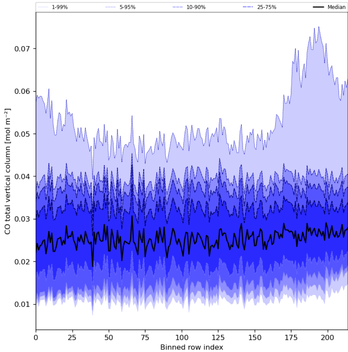
Figure 26: Along track statistics of “CO total vertical column” for 2023-11-04 to 2023-11-06
