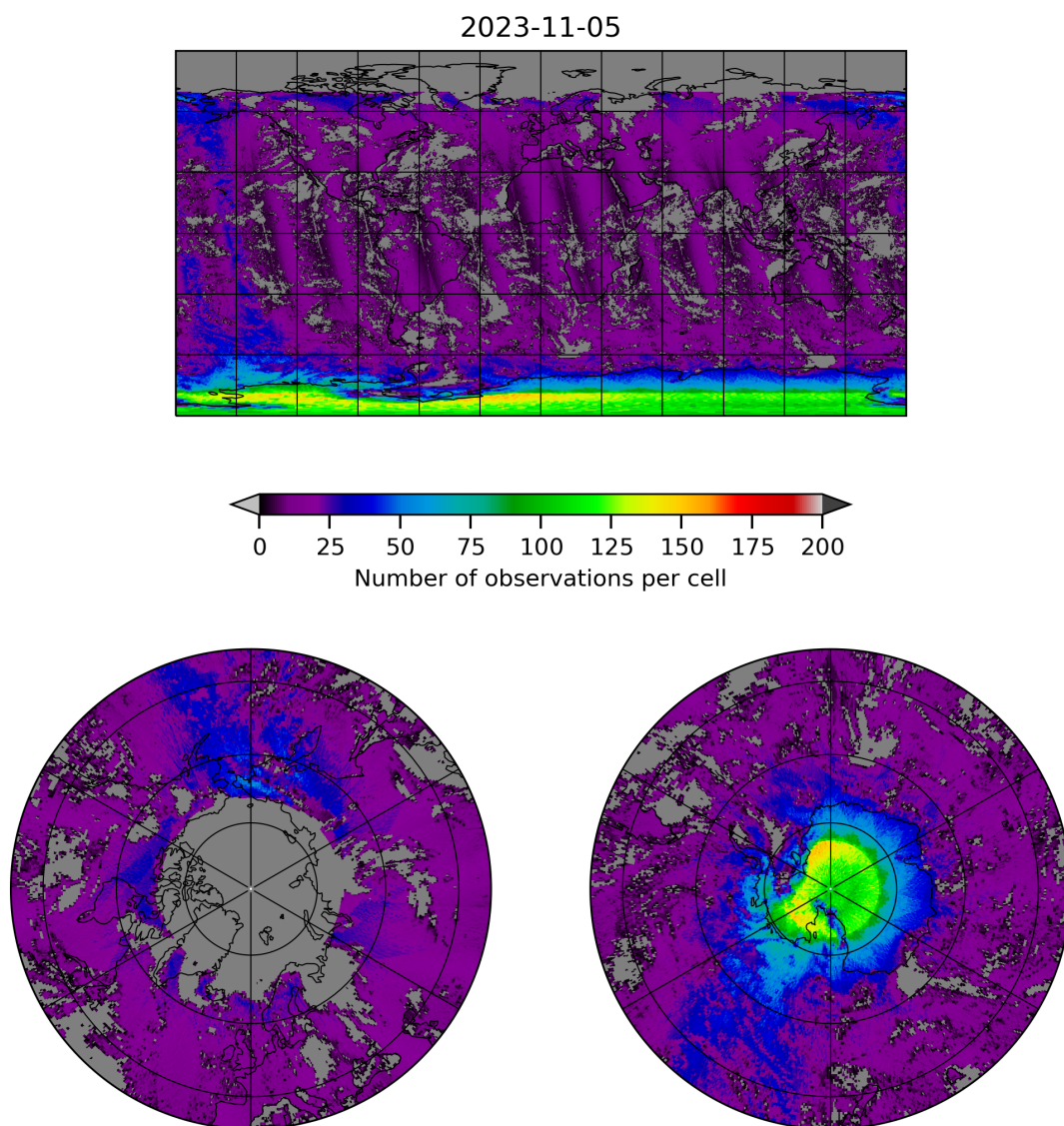
Figure 8: Map of the number of observations for 2023-11-04 to 2023-11-06
