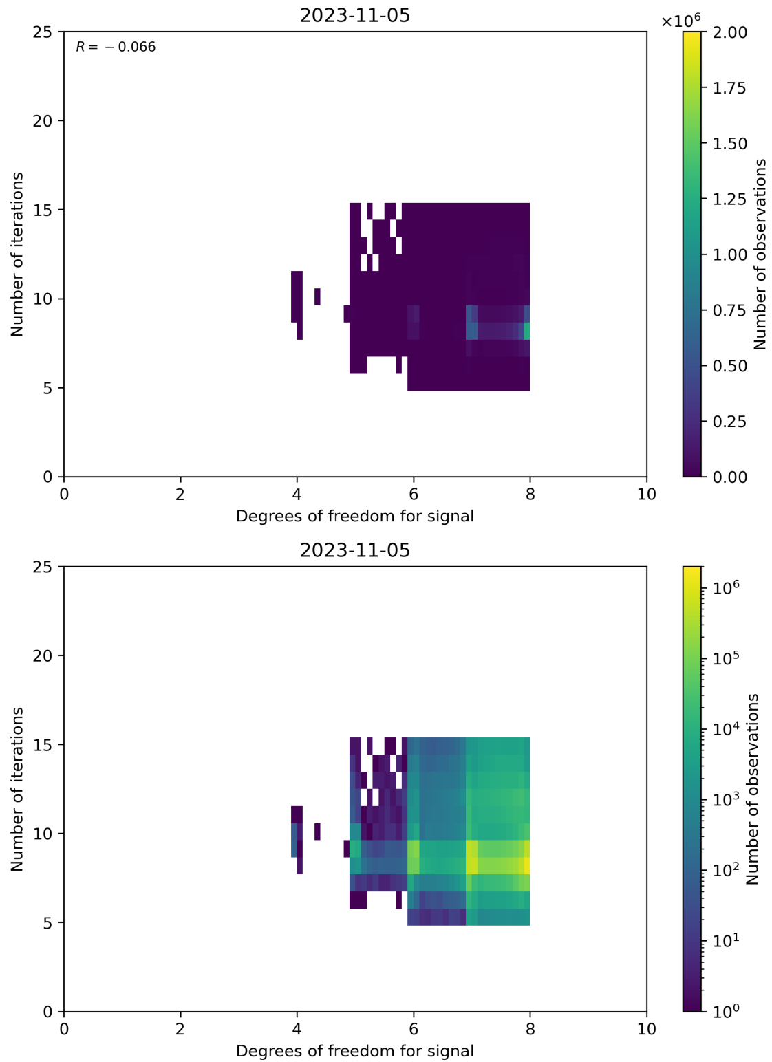
Figure 50: Scatter density plot of “Degrees of freedom for signal” against “Number of iterations” for 2023-11-04 to 2023-11-06.
