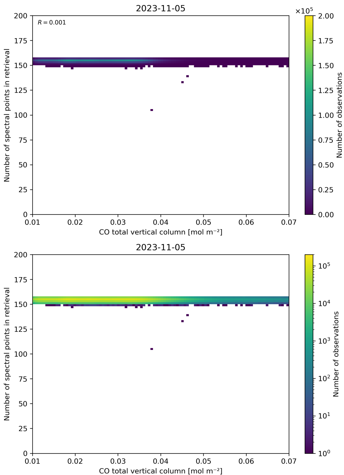
Figure 43: Scatter density plot of “CO total vertical column” against “Number of spectral points in retrieval” for 2023-11-04 to 2023-11-06.
