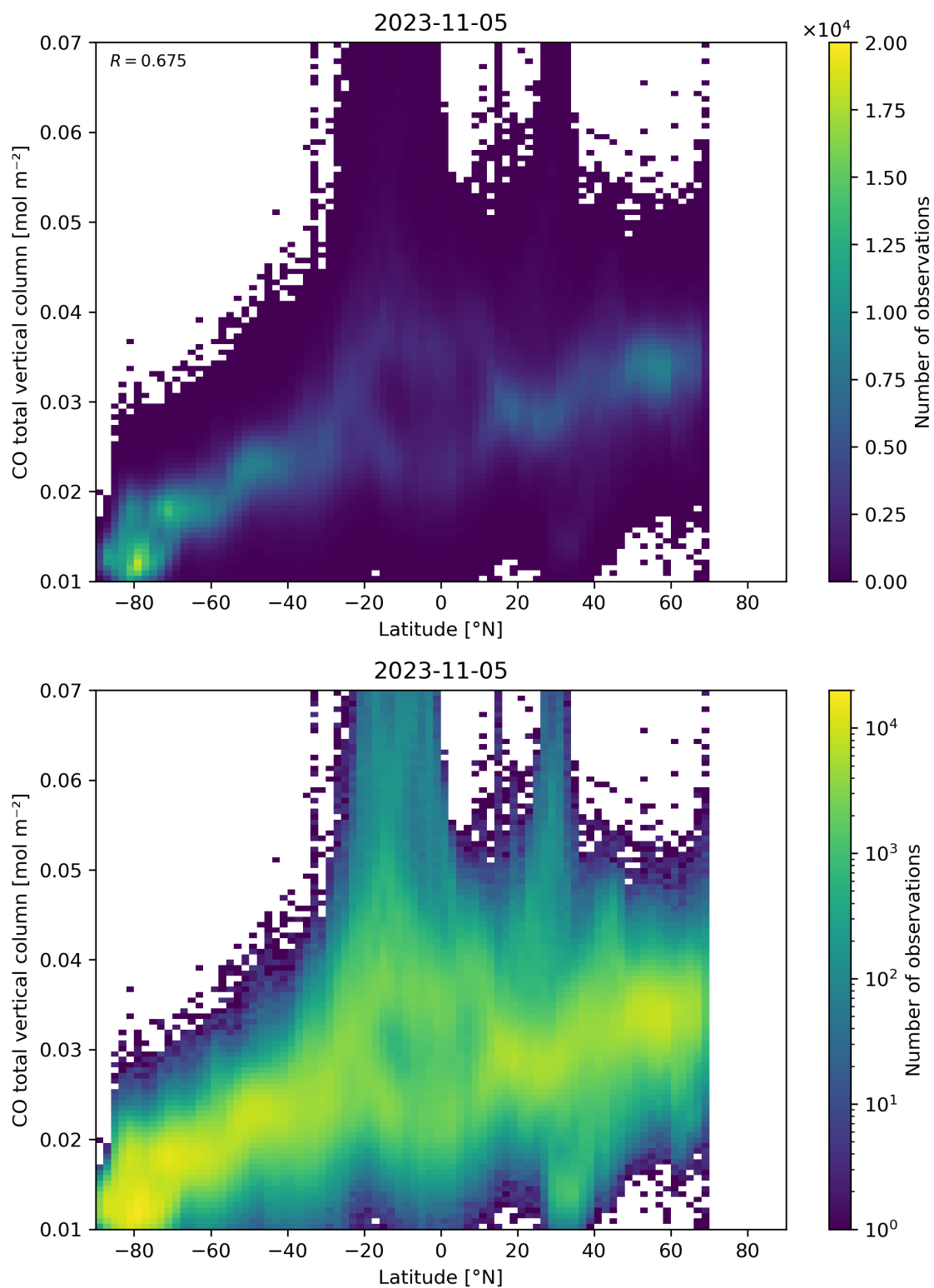
Figure 51: Scatter density plot of “Latitude” against “CO total vertical column” for 2023-11-04 to 2023-11-06.
