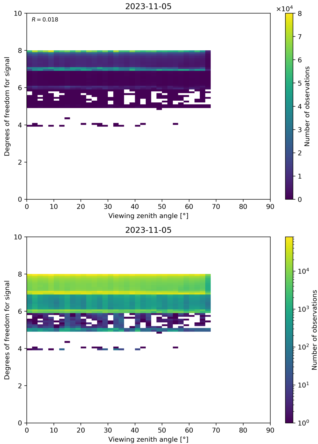
Figure 73: Scatter density plot of “Viewing zenith angle” against “Degrees of freedom for signal” for 2023-11-04 to 2023-11-06.
