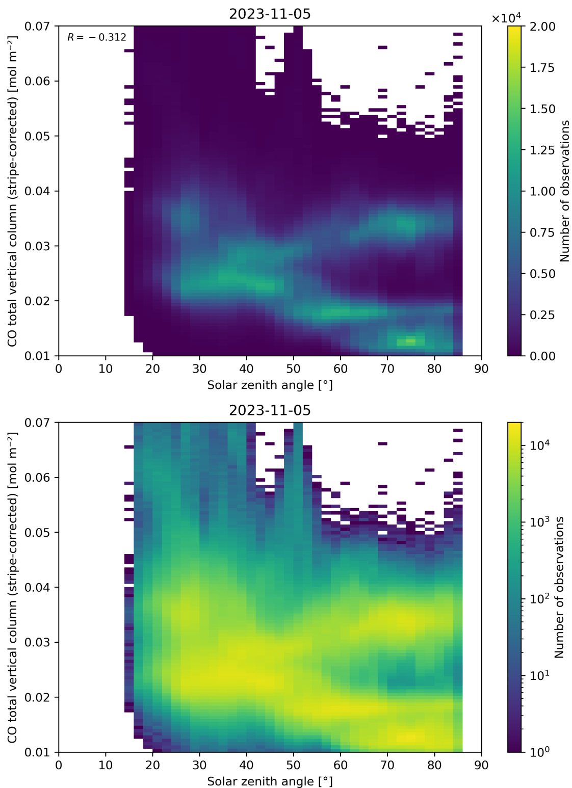
Figure 62: Scatter density plot of “Solar zenith angle” against “CO total vertical column (stripe-corrected)” for 2023-11-04 to 2023-11-06.
