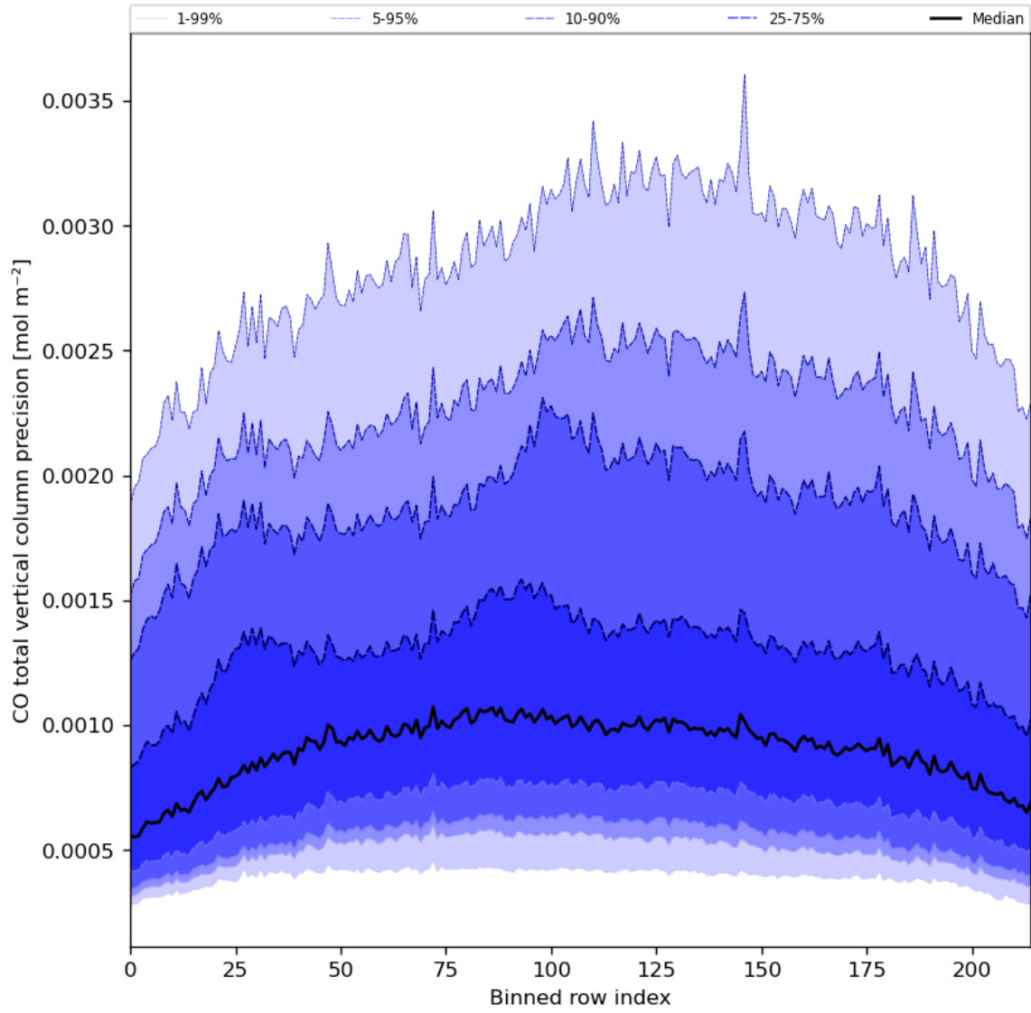
Figure 28: Along track statistics of “CO total vertical column precision” for 2023-11-04 to 2023-11-06
