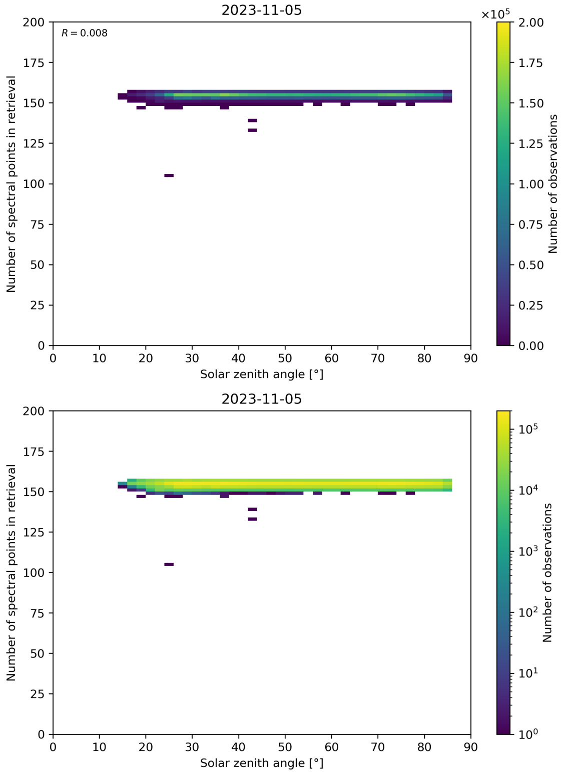
Figure 68: Scatter density plot of “Solar zenith angle” against “Number of spectral points in retrieval” for 2023-11-04 to 2023-11-06.
