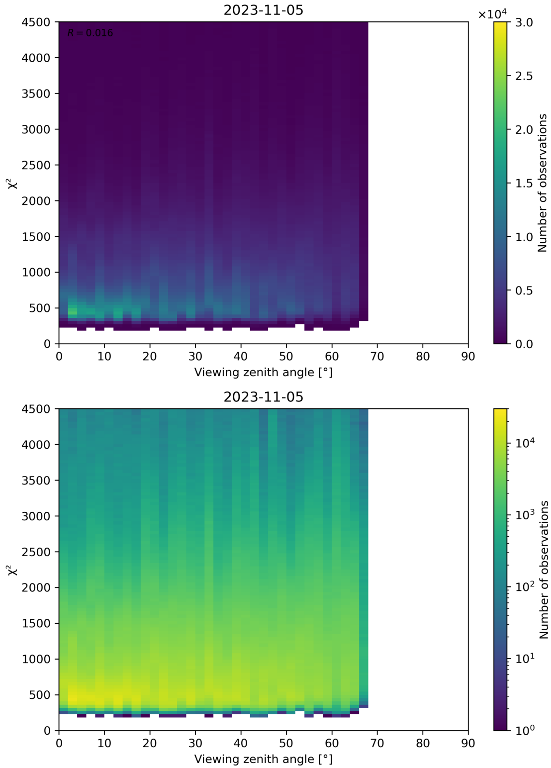
Figure 72: Scatter density plot of “Viewing zenith angle” against “ \chi^2 ” for 2023-11-04 to 2023-11-06.
