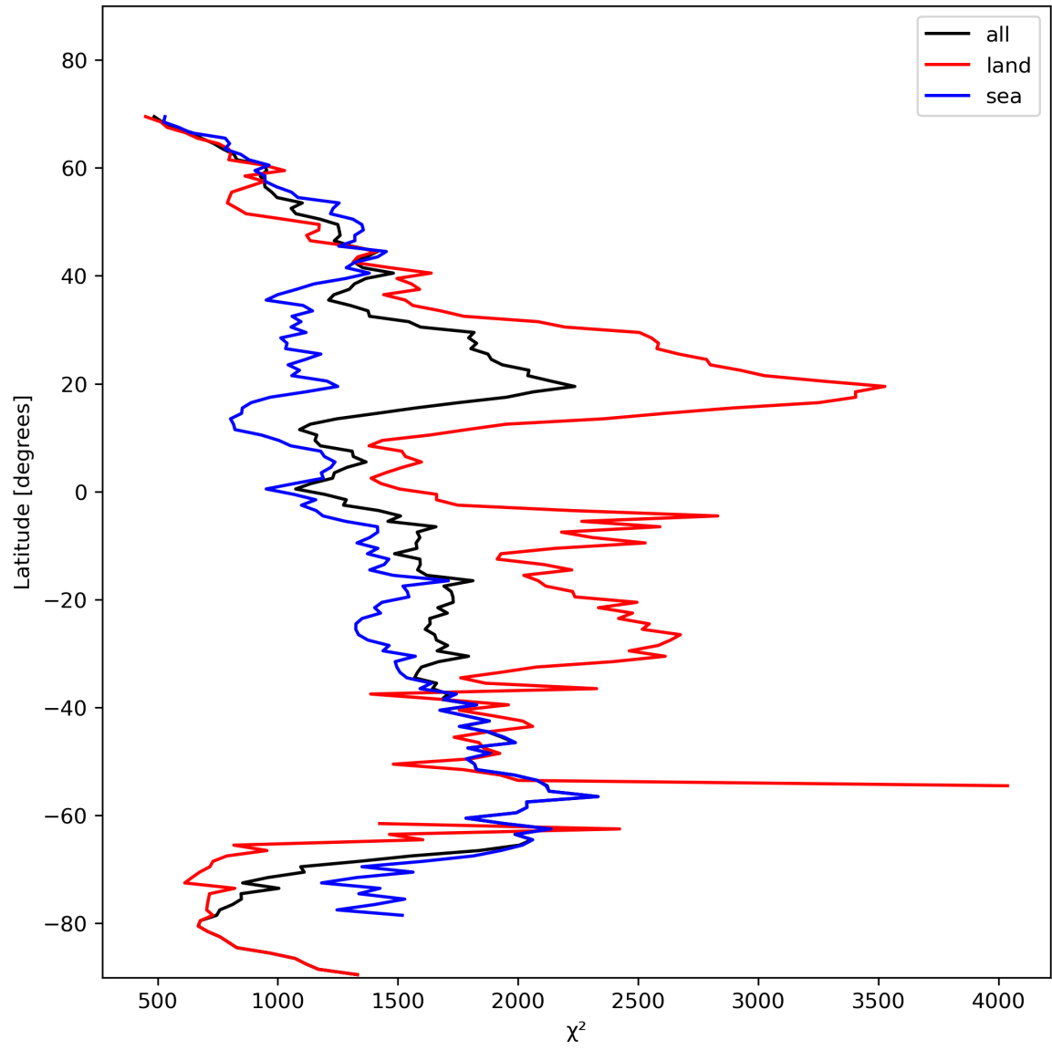
Figure 14: Zonal average of “ \chi^2 ” for 2023-11-04 to 2023-11-06.
