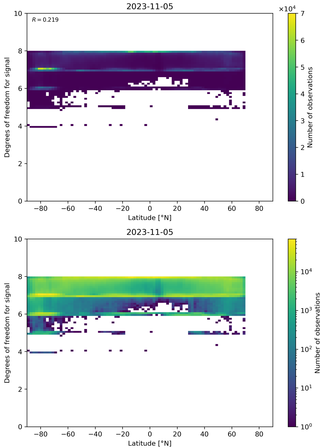
Figure 55: Scatter density plot of “Latitude” against “Degrees of freedom for signal” for 2023-11-04 to 2023-11-06.
