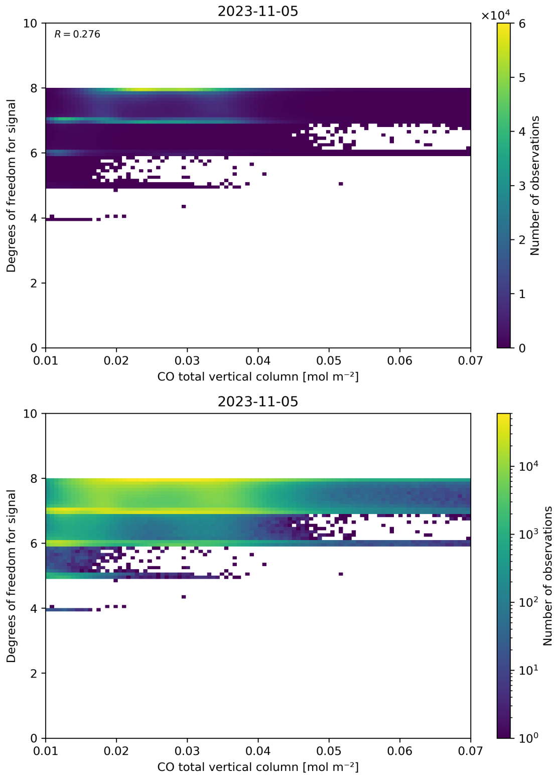
Figure 41: Scatter density plot of “CO total vertical column” against “Degrees of freedom for signal” for 2023-11-04 to 2023-11-06.
