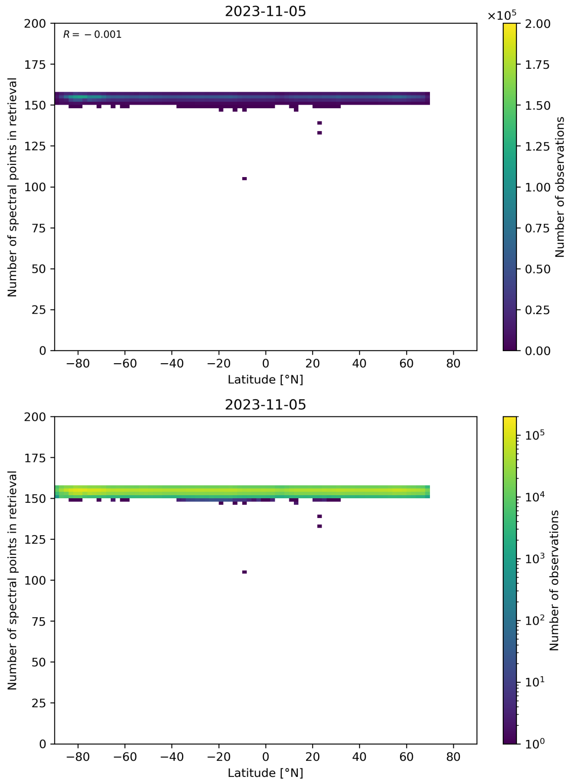
Figure 57: Scatter density plot of “Latitude” against “Number of spectral points in retrieval” for 2023-11-04 to 2023-11-06.
