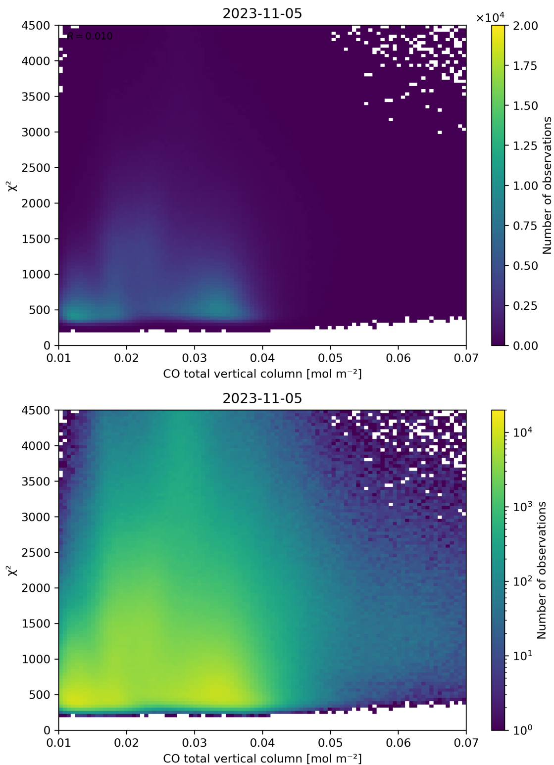
Figure 35: Scatter density plot of “CO total vertical column” against “ \chi^2 ” for 2023-11-04 to 2023-11-06.
