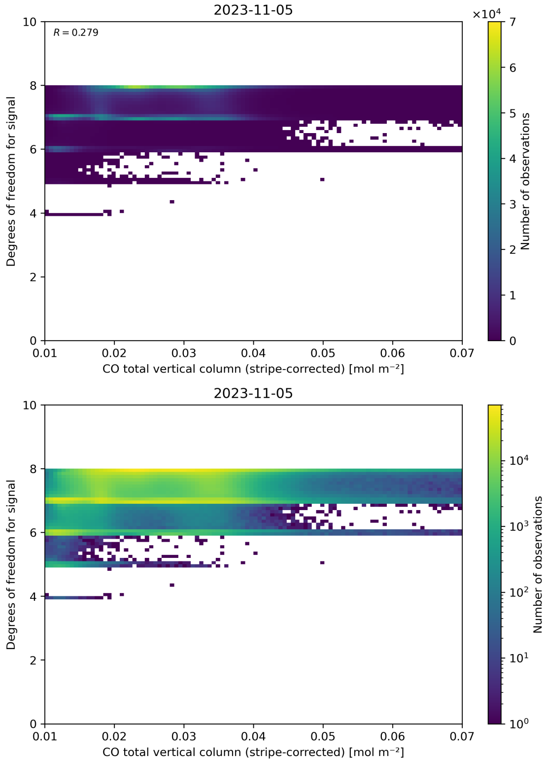
Figure 38: Scatter density plot of “CO total vertical column (stripe-corrected)” against “Degrees of freedom for signal” for 2023-11-04 to 2023-11-06.
