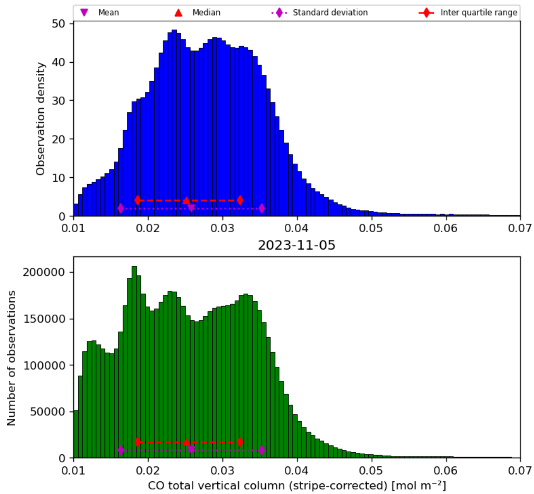
Figure 19: Histogram of “CO total vertical column (stripe-corrected)” for 2023-11-04 to 2023-11-06
