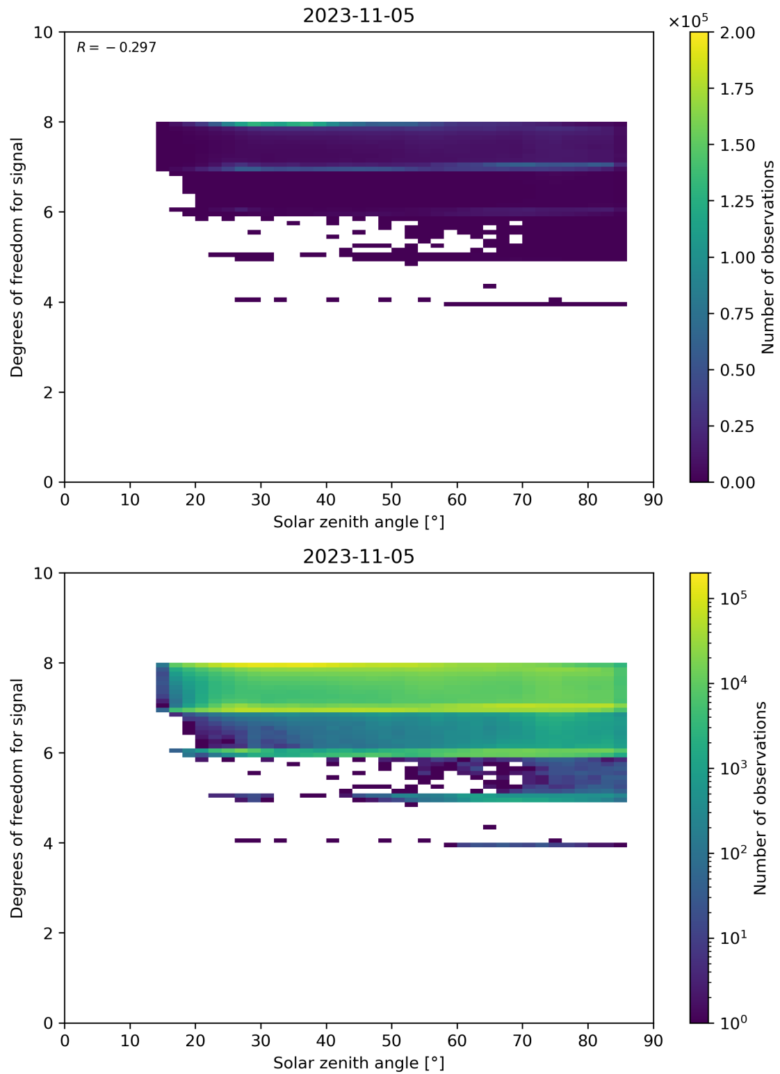
Figure 65: Scatter density plot of “Solar zenith angle” against “Degrees of freedom for signal” for 2023-11-04 to 2023-11-06.
