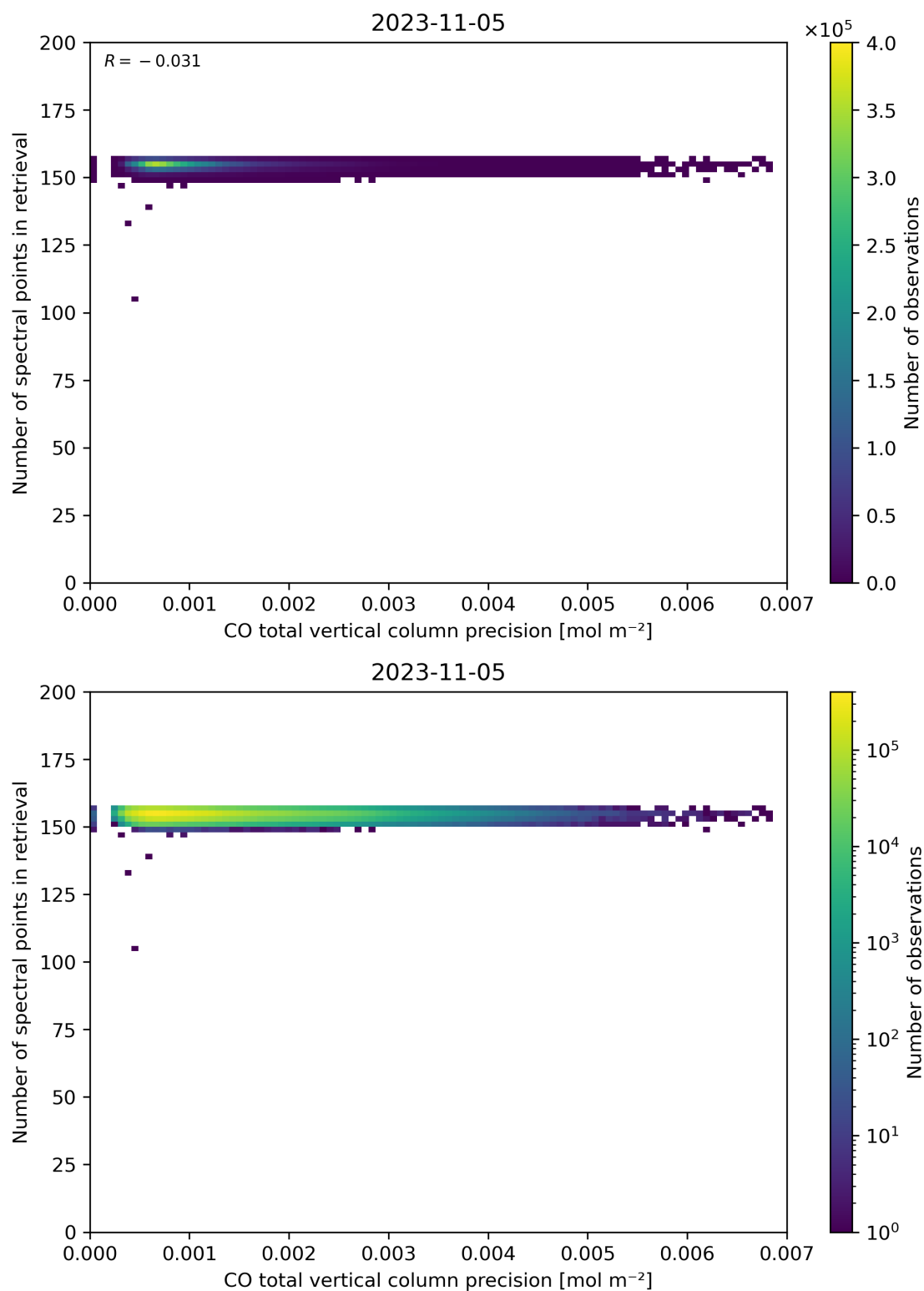
Figure 47: Scatter density plot of “CO total vertical column precision” against “Number of spectral points in retrieval” for 2023-11-04 to 2023-11-06.
