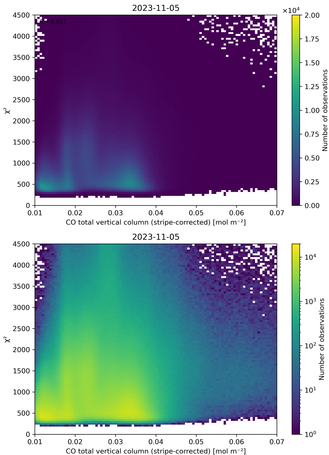
Figure 37: Scatter density plot of “CO total vertical column (stripe-corrected)” against “ \chi^2 ” for 2023-11-04 to 2023-11-06.
