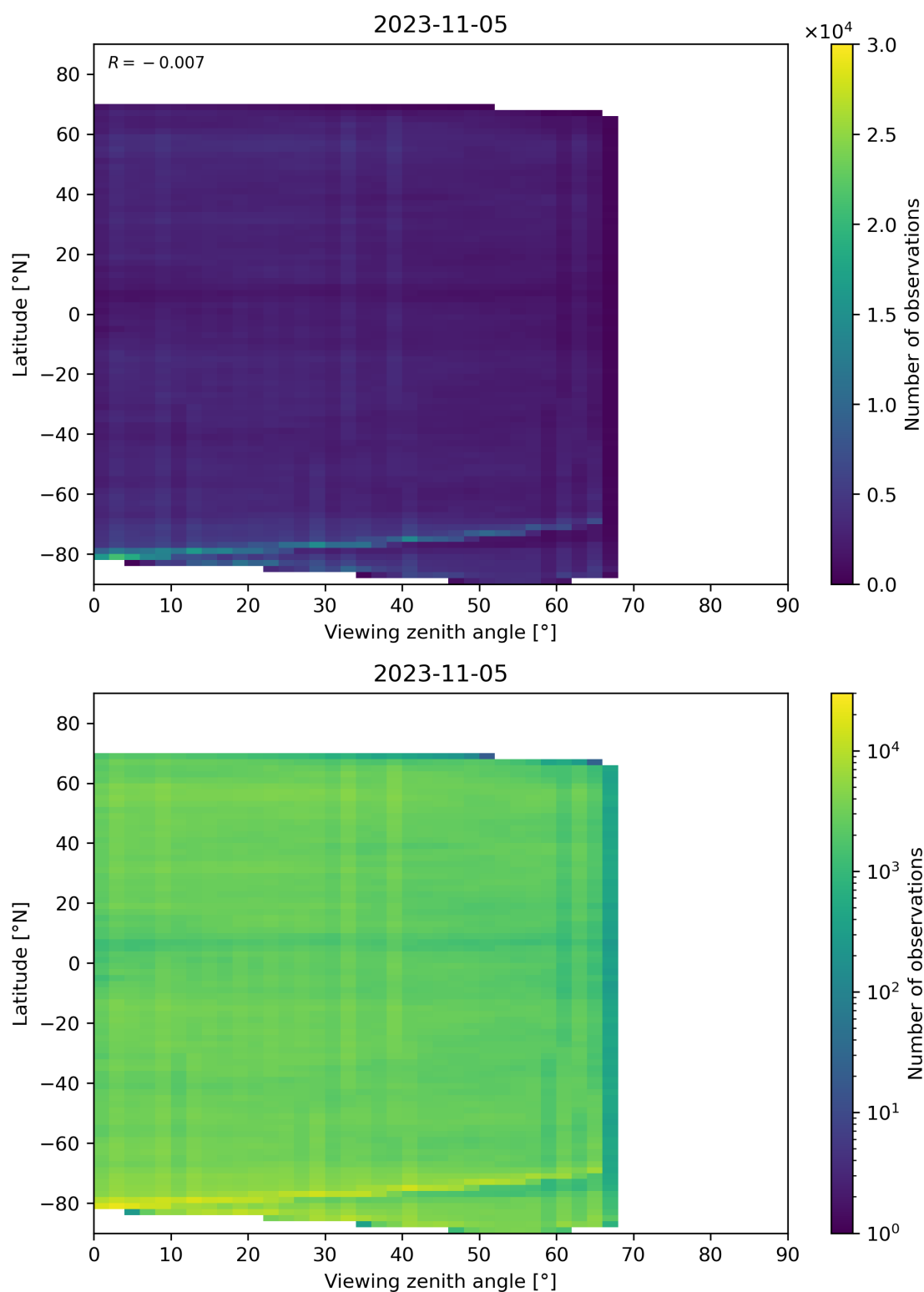
Figure 74: Scatter density plot of “Viewing zenith angle” against “Latitude” for 2023-11-04 to 2023-11-06.
