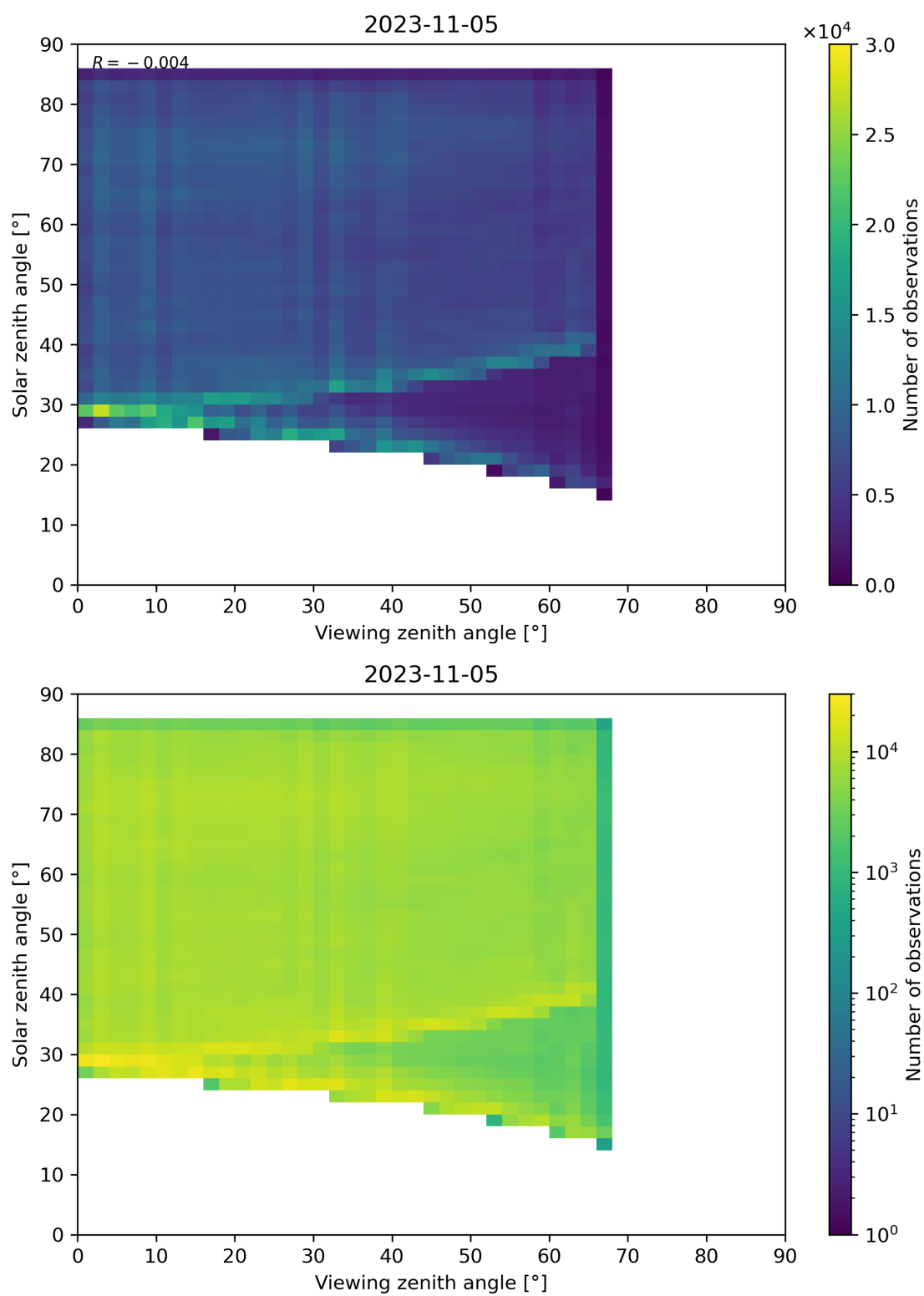
Figure 77: Scatter density plot of “Viewing zenith angle” against “Solar zenith angle” for 2023-11-04 to 2023-11-06.
