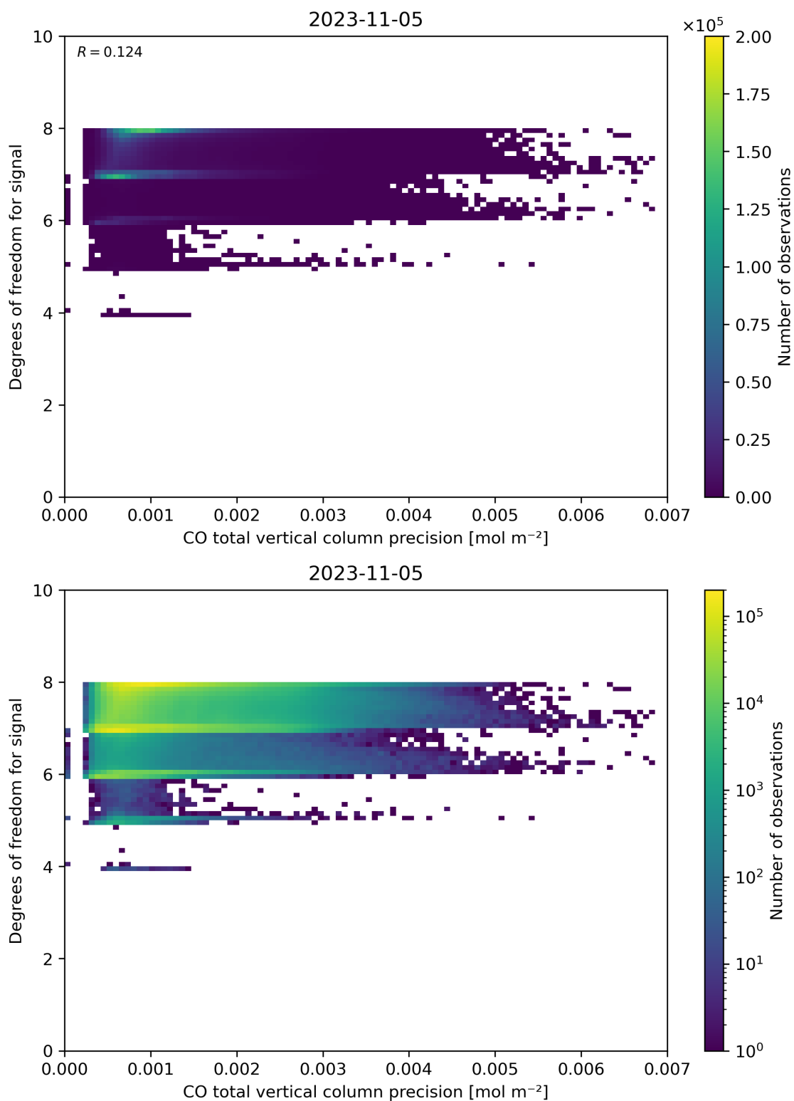
Figure 45: Scatter density plot of “CO total vertical column precision” against “Degrees of freedom for signal” for 2023-11-04 to 2023-11-06.
