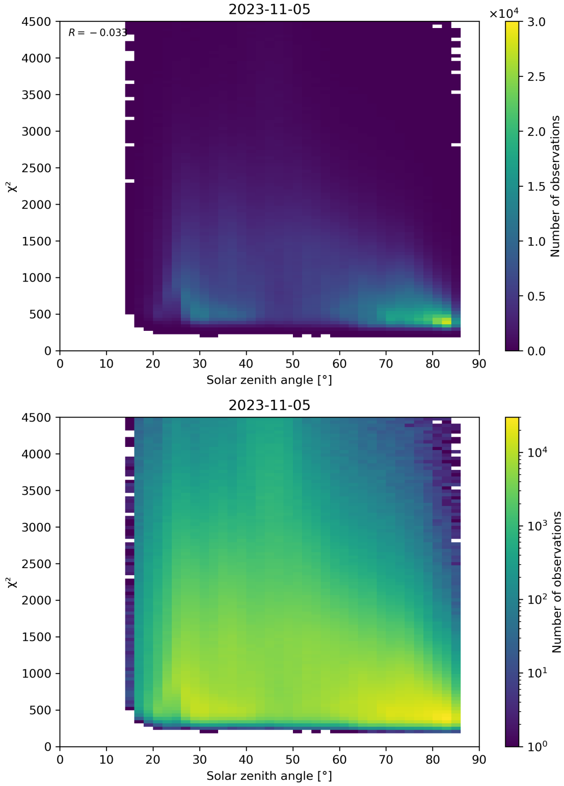
Figure 64: Scatter density plot of “Solar zenith angle” against “ \chi^2 ” for 2023-11-04 to 2023-11-06.
