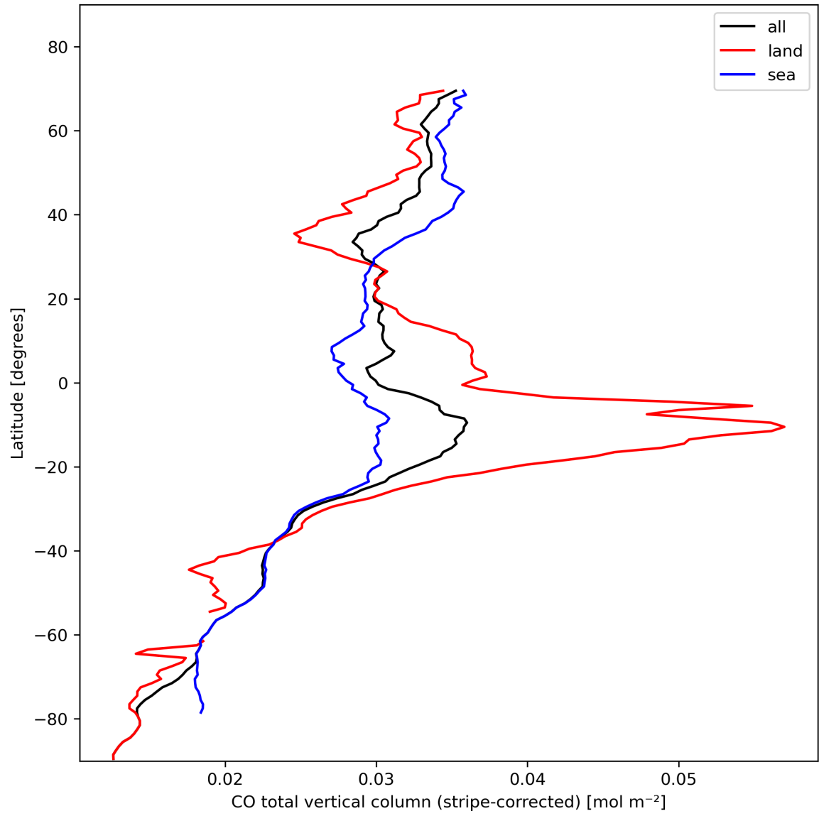
Figure 11: Zonal average of “CO total vertical column (stripe-corrected)” for 2023-11-04 to 2023-11-06.
