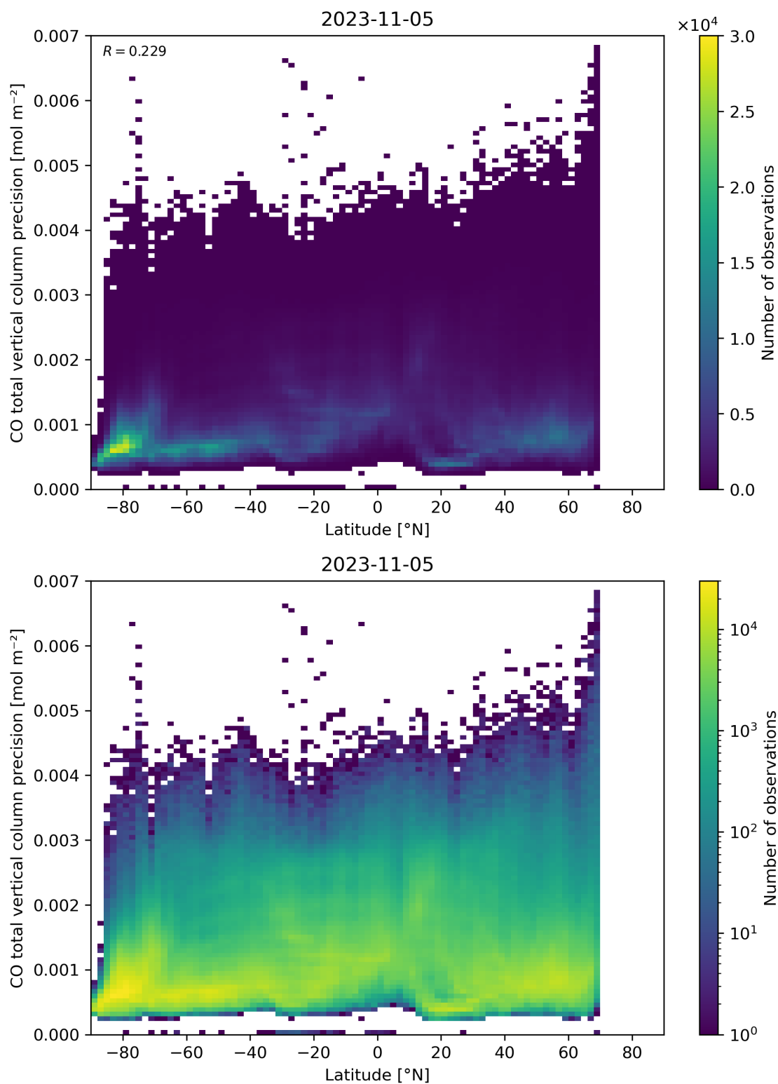
Figure 53: Scatter density plot of “Latitude” against “CO total vertical column precision” for 2023-11-04 to 2023-11-06.
