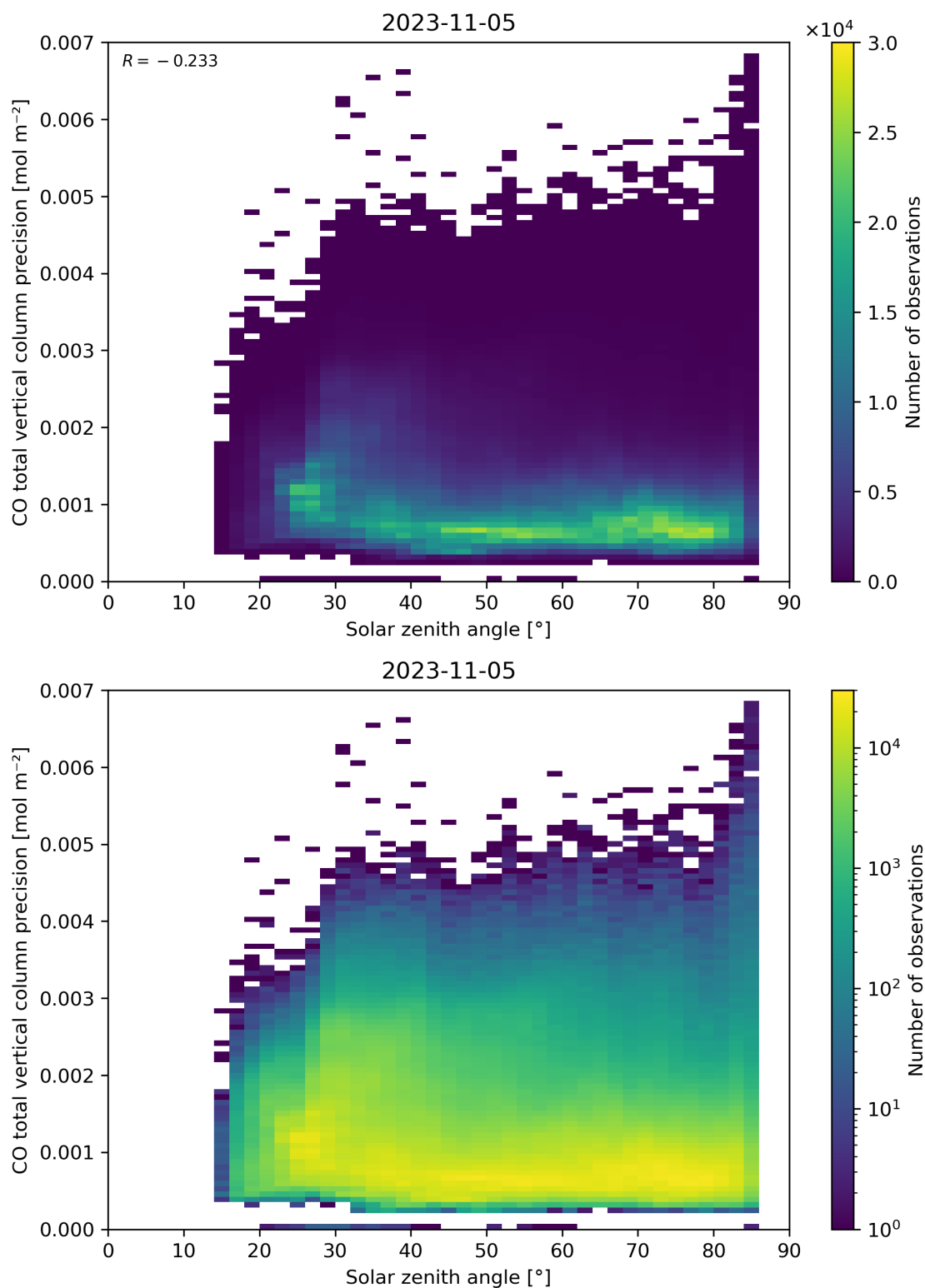
Figure 63: Scatter density plot of “Solar zenith angle” against “CO total vertical column precision” for 2023-11-04 to 2023-11-06.
