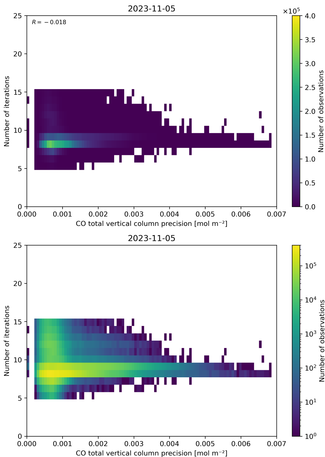
Figure 46: Scatter density plot of “CO total vertical column precision” against “Number of iterations” for 2023-11-04 to 2023-11-06.
