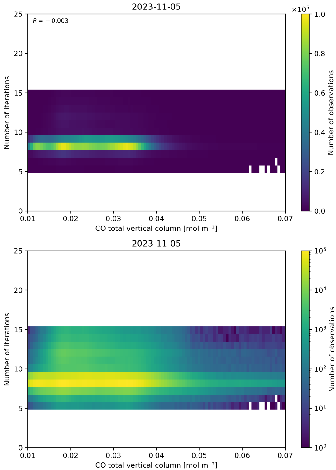
Figure 42: Scatter density plot of “CO total vertical column” against “Number of iterations” for 2023-11-04 to 2023-11-06.
