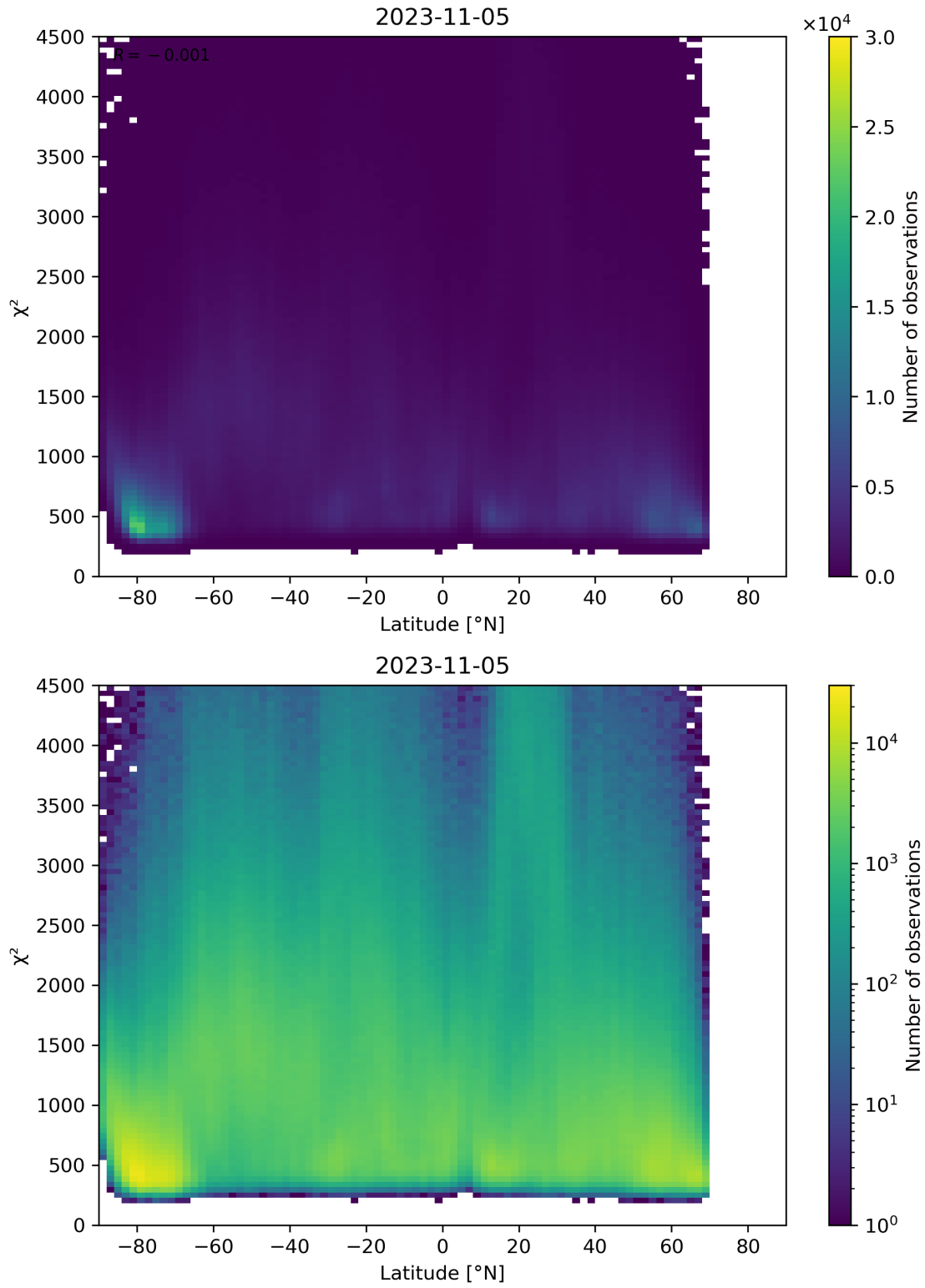
Figure 54: Scatter density plot of “Latitude” against “ \chi^2 ” for 2023-11-04 to 2023-11-06.
