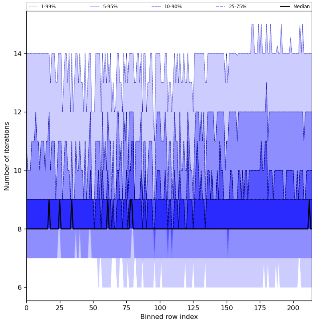
Figure 32: Along track statistics of “Number of iterations” for 2023-11-04 to 2023-11-06
