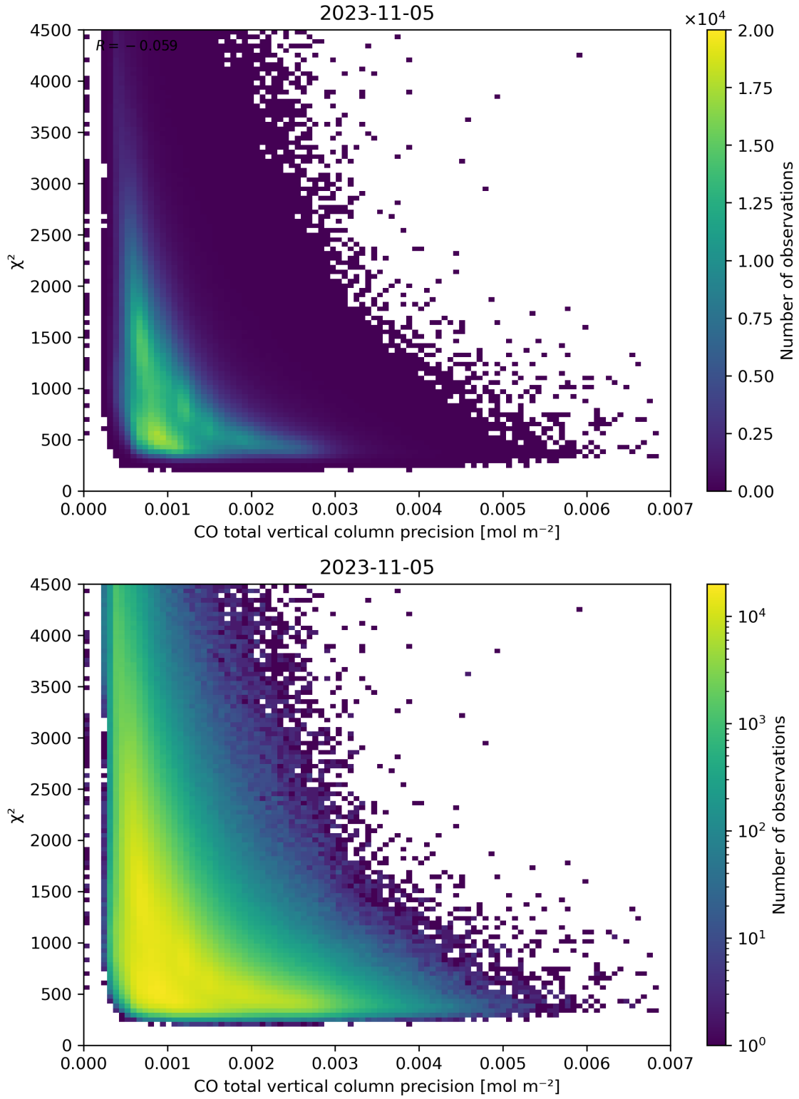
Figure 44: Scatter density plot of “CO total vertical column precision” against “ \chi^2 ” for 2023-11-04 to 2023-11-06.
