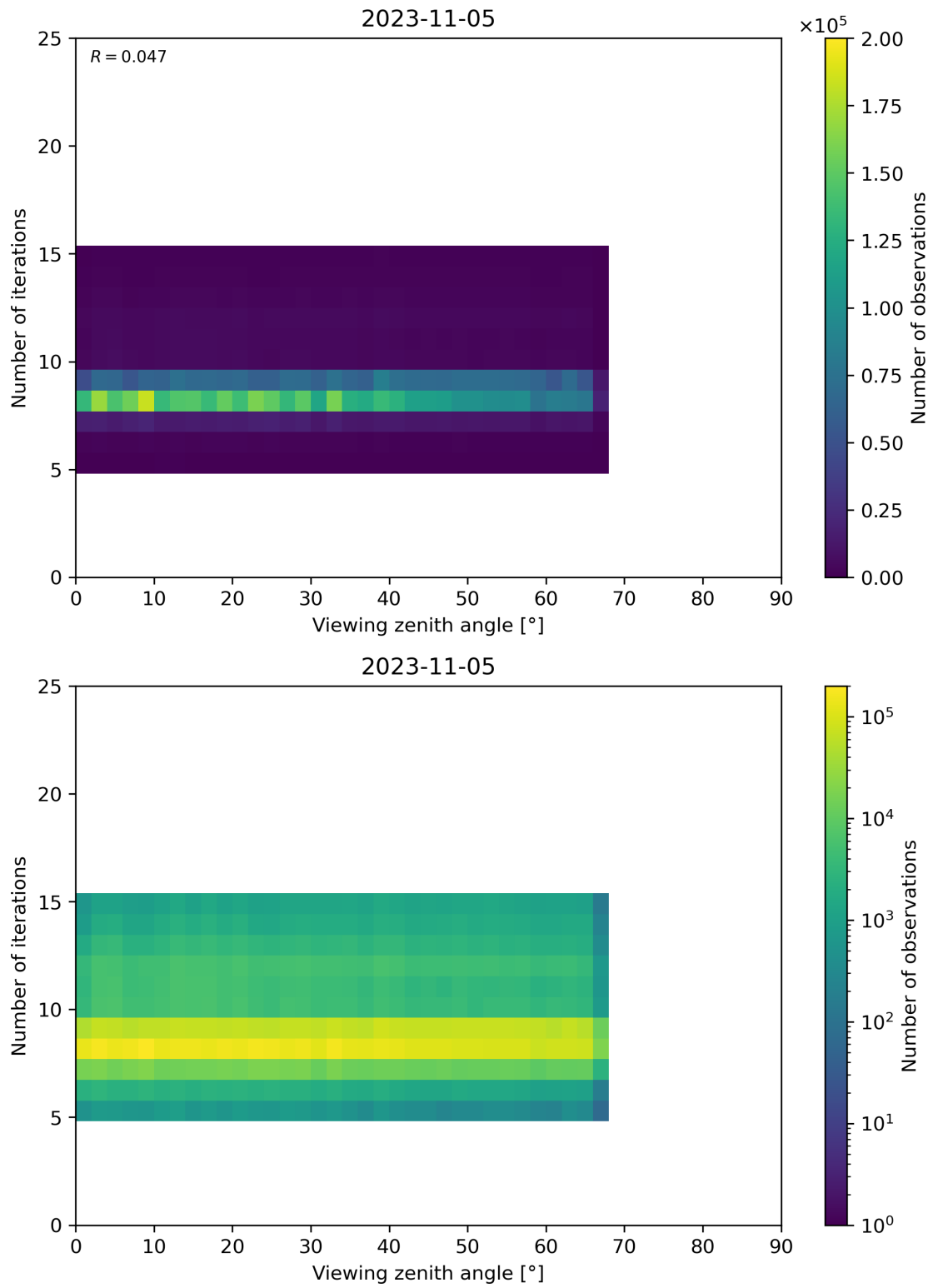
Figure 75: Scatter density plot of “Viewing zenith angle” against “Number of iterations” for 2023-11-04 to 2023-11-06.
