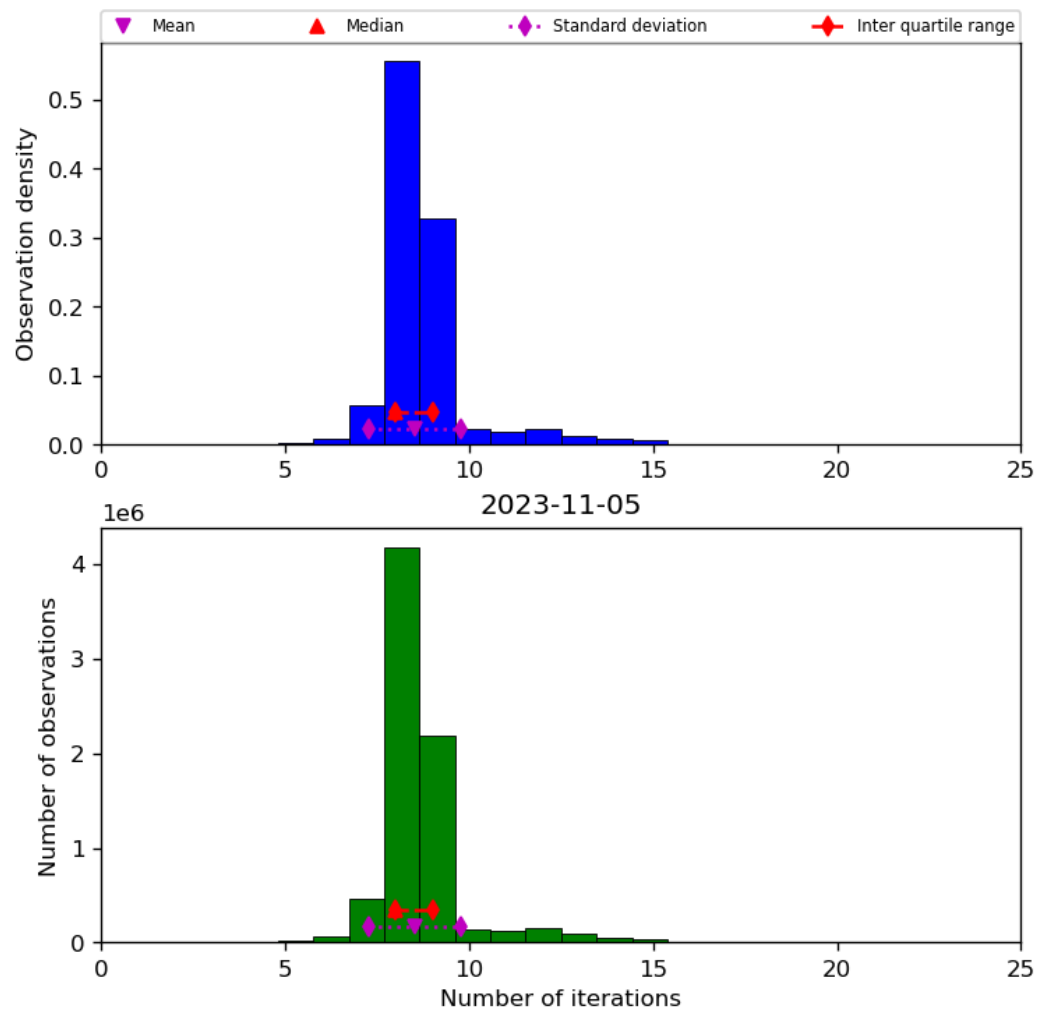
Figure 24: Histogram of “Number of iterations” for 2023-11-04 to 2023-11-06
