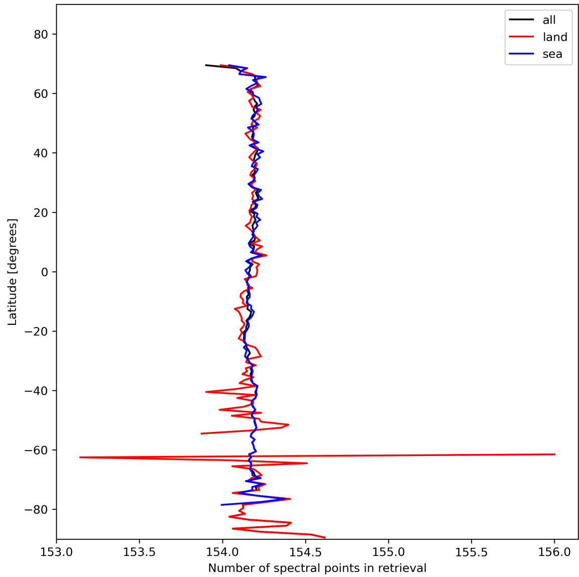
Figure 13: Zonal average of “Number of spectral points in retrieval” for 2023-11-04 to 2023-11-06.
