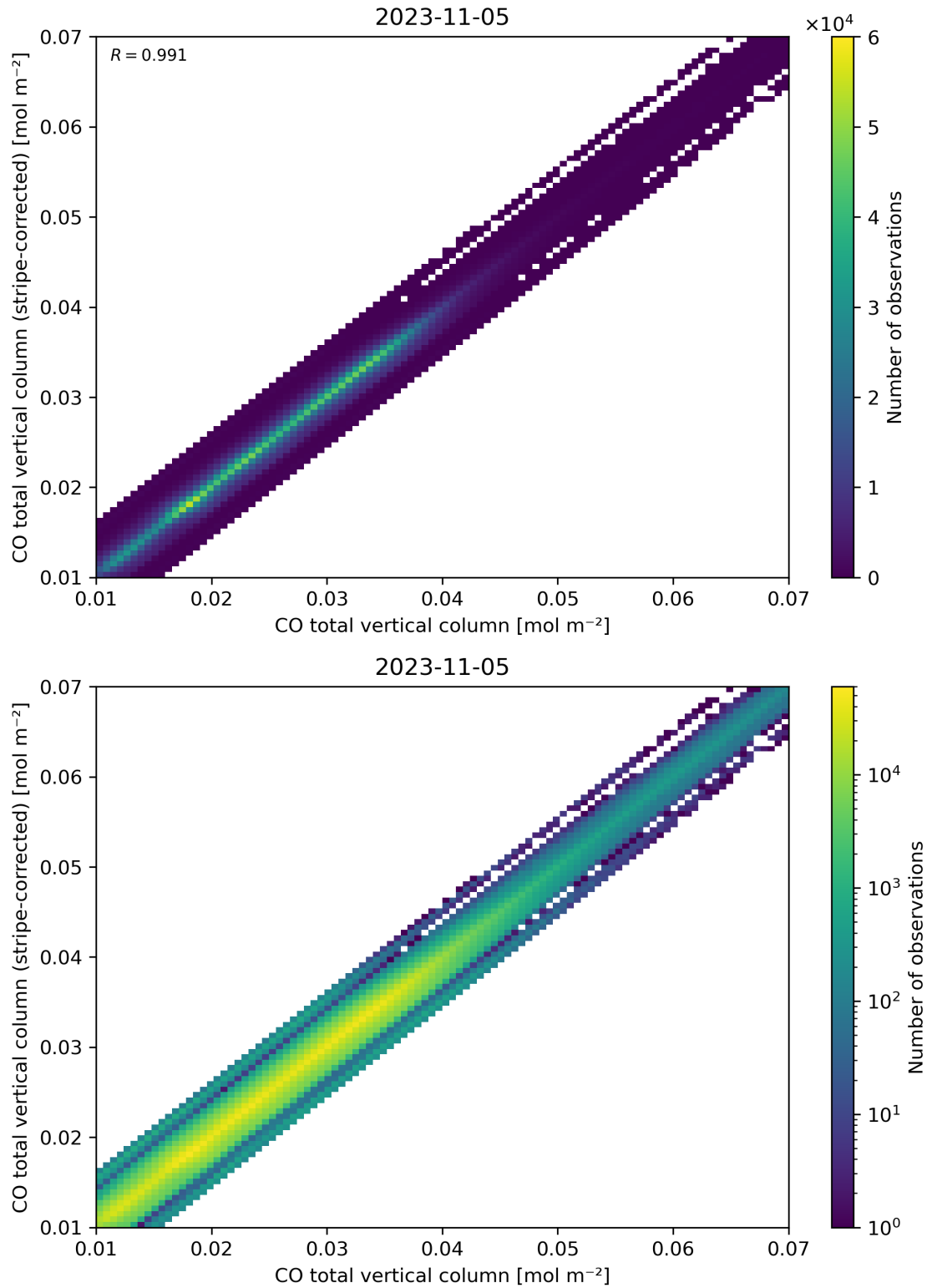
Figure 33: Scatter density plot of “CO total vertical column” against “CO total vertical column (stripe-corrected)” for 2023-11-04 to 2023-11-06.
