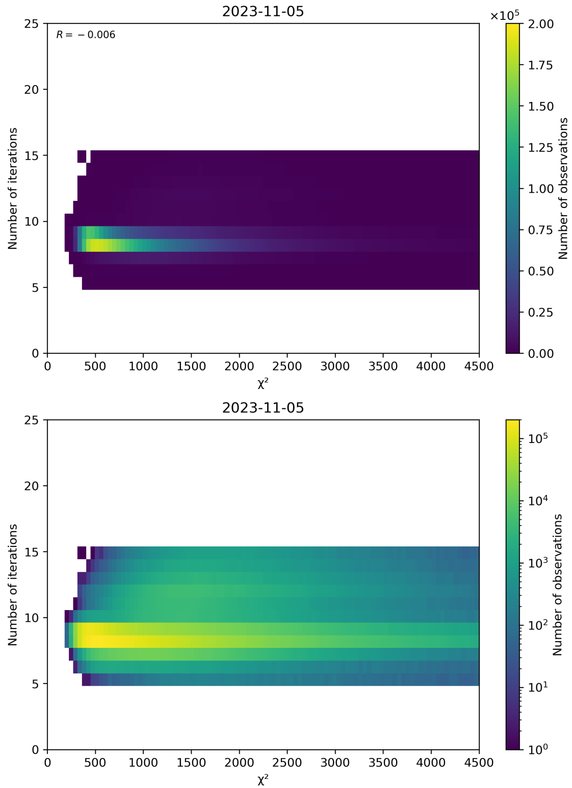
Figure 49: Scatter density plot of “ \chi^2 ” against “Number of iterations” for 2023-11-04 to 2023-11-06.
