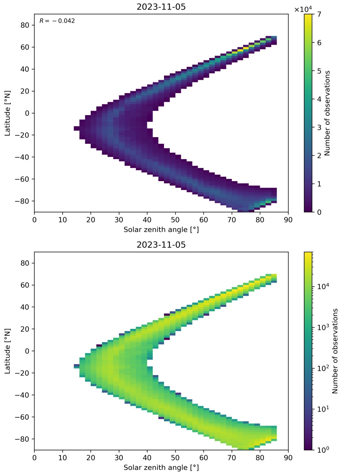
Figure 66: Scatter density plot of “Solar zenith angle” against “Latitude” for 2023-11-04 to 2023-11-06.
