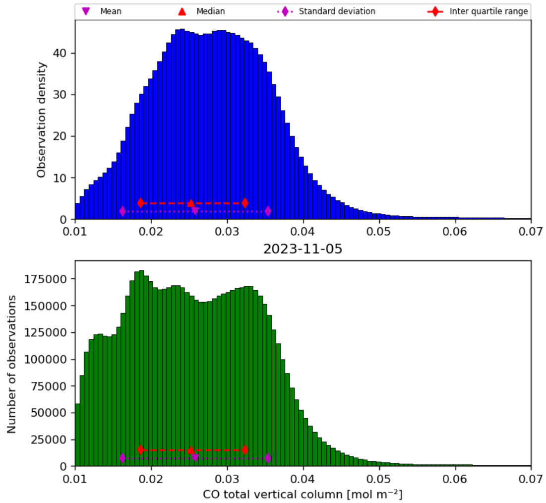
Figure 18: Histogram of “CO total vertical column” for 2023-11-04 to 2023-11-06
