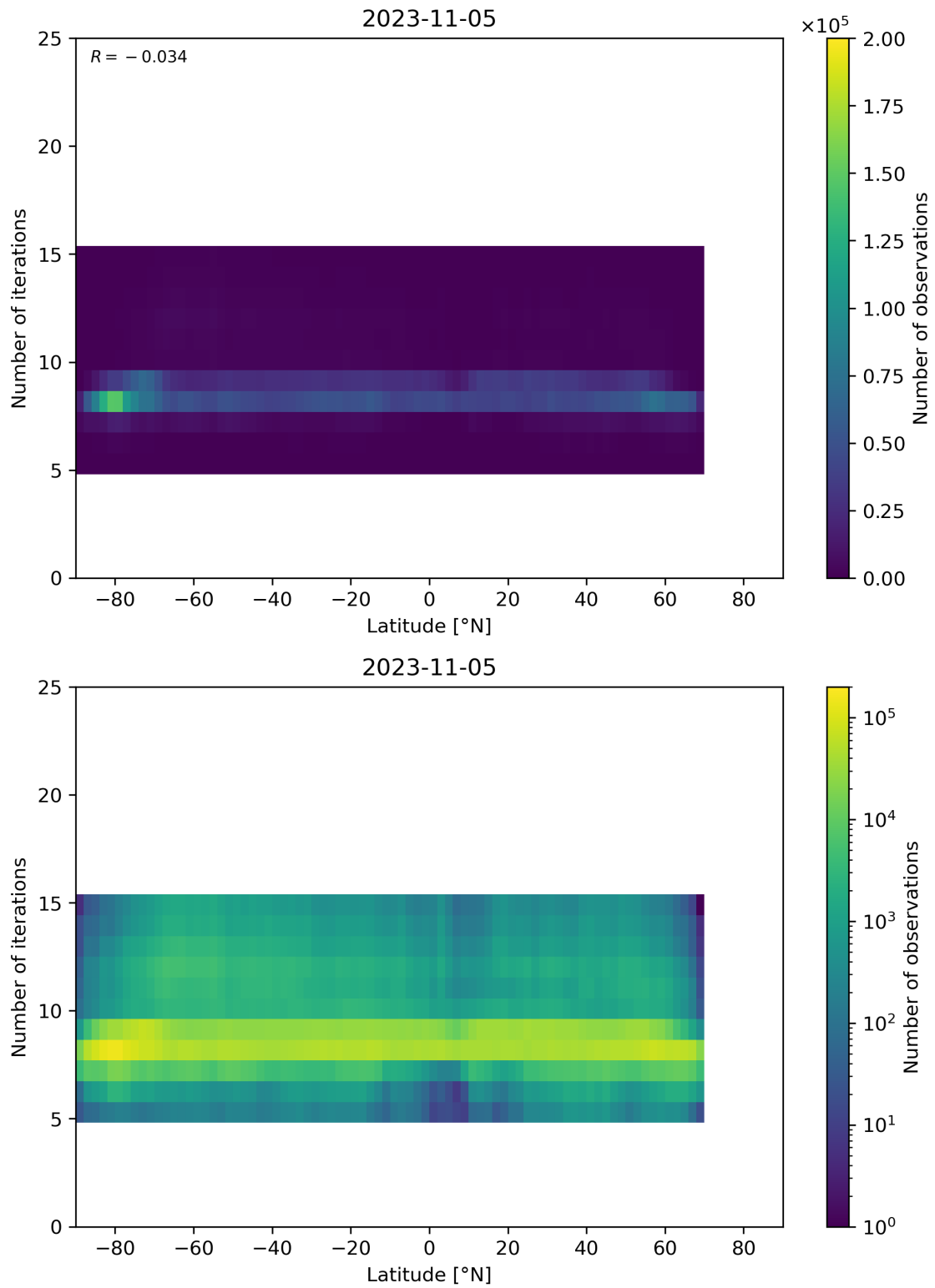
Figure 56: Scatter density plot of “Latitude” against “Number of iterations” for 2023-11-04 to 2023-11-06.
