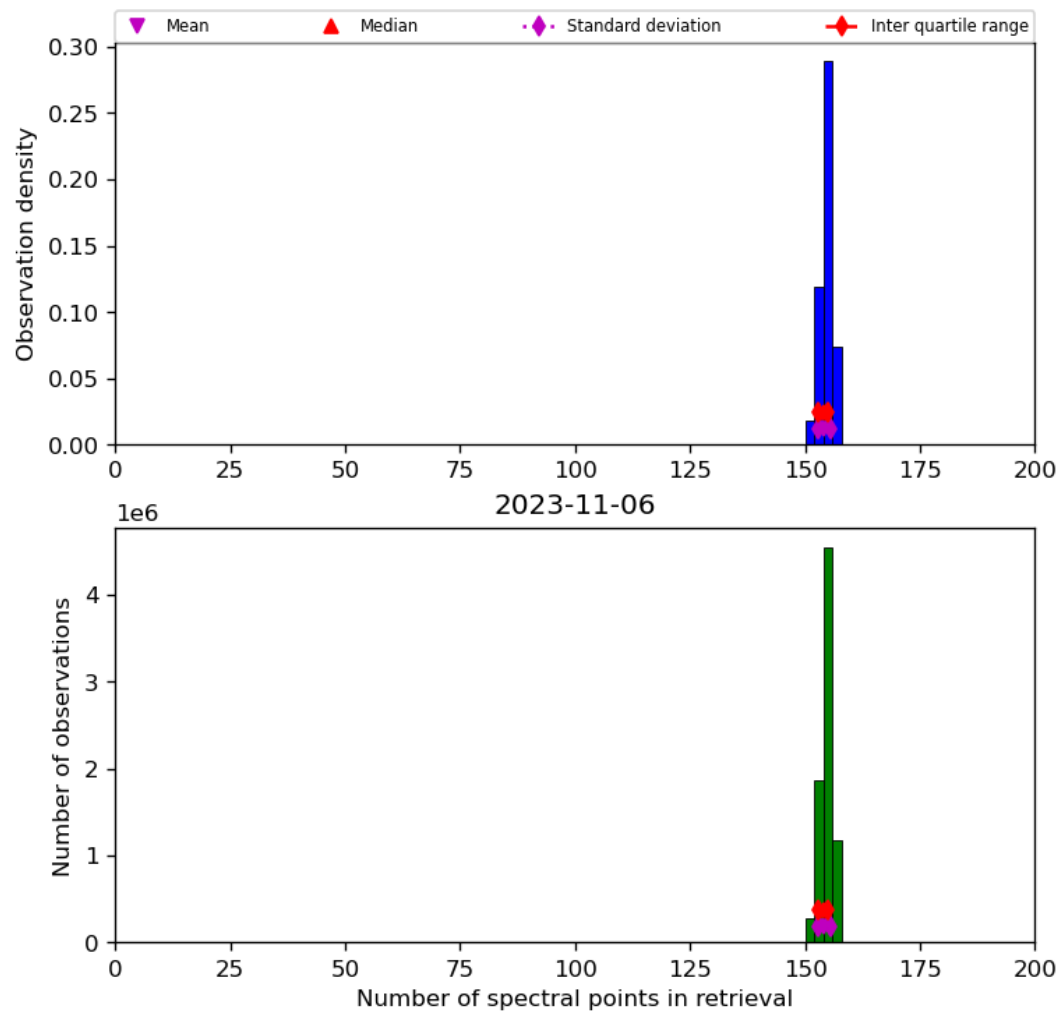
Figure 21: Histogram of “Number of spectral points in retrieval” for 2023-11-05 to 2023-11-07
