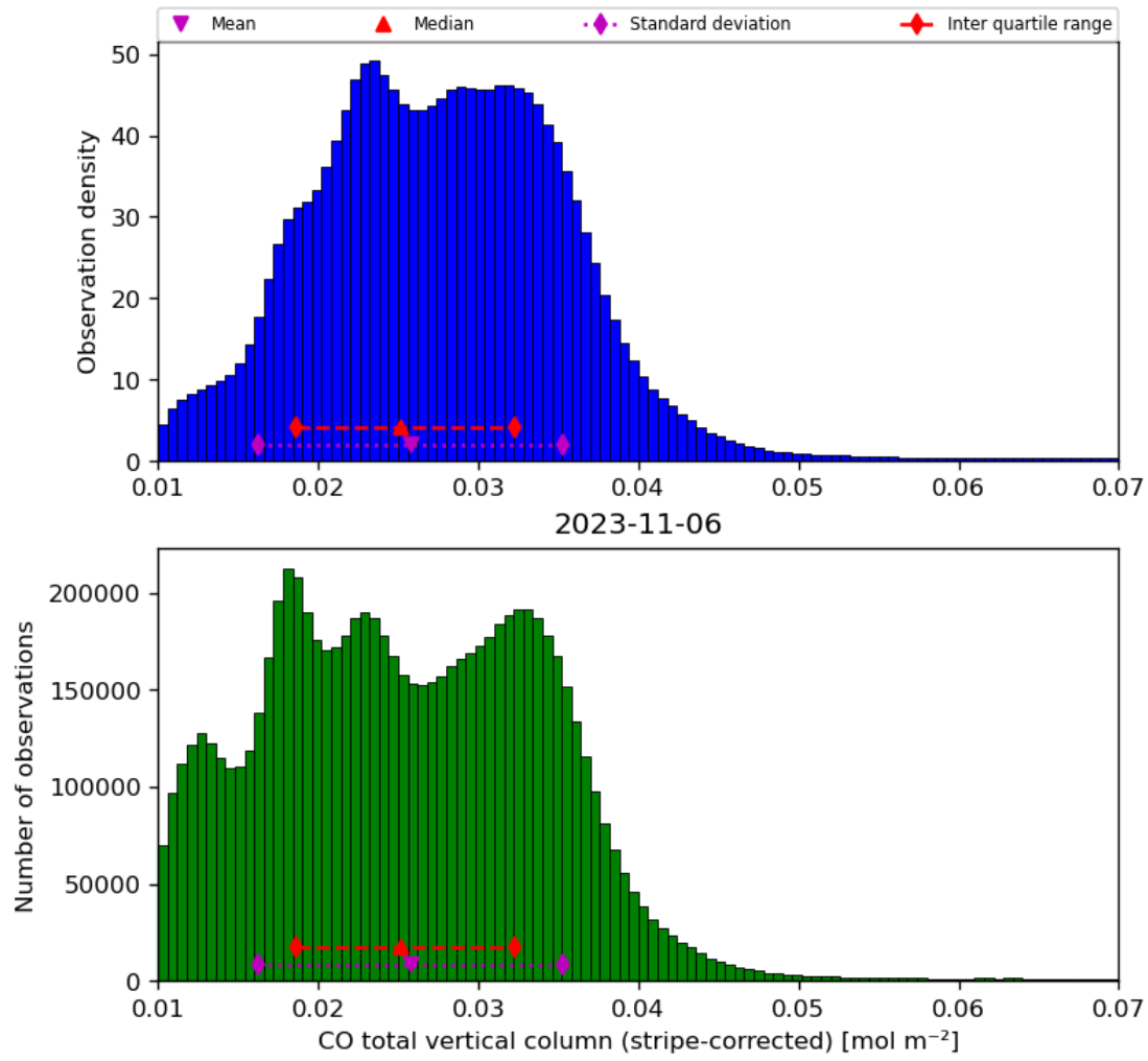
Figure 19: Histogram of “CO total vertical column (stripe-corrected)” for 2023-11-05 to 2023-11-07
