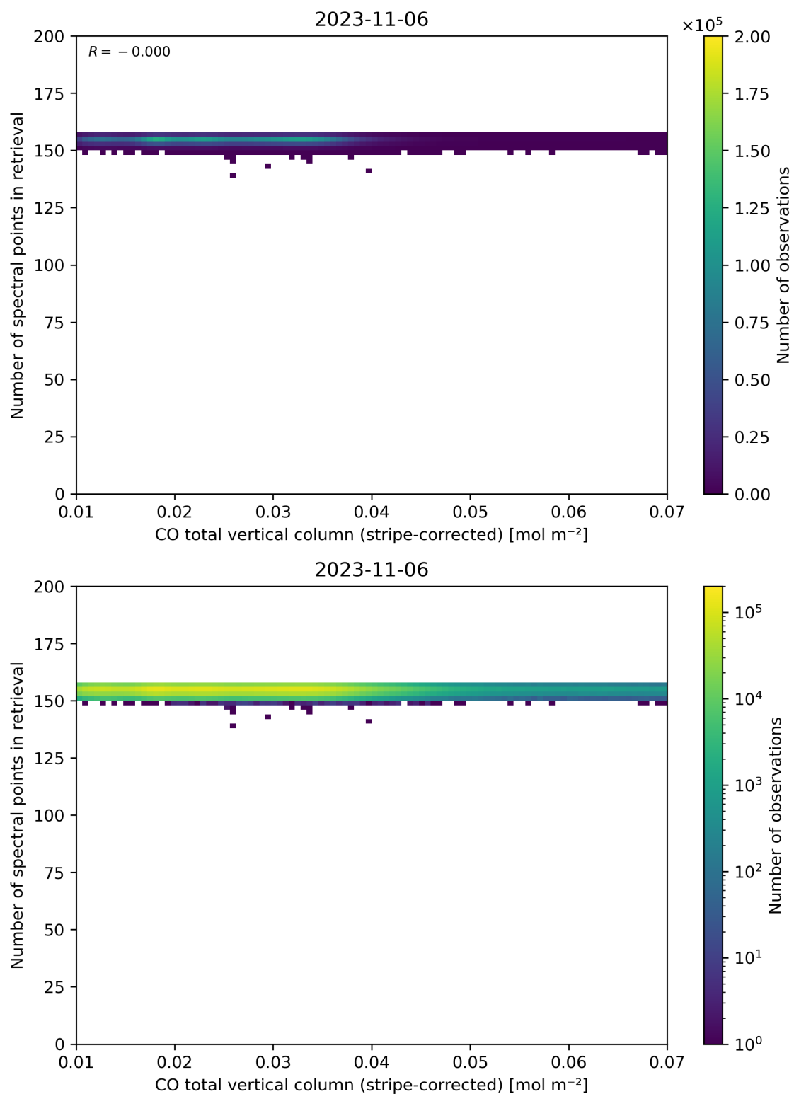
Figure 40: Scatter density plot of “CO total vertical column (stripe-corrected)” against “Number of spectral points in retrieval” for 2023-11-05 to 2023-11-07.
