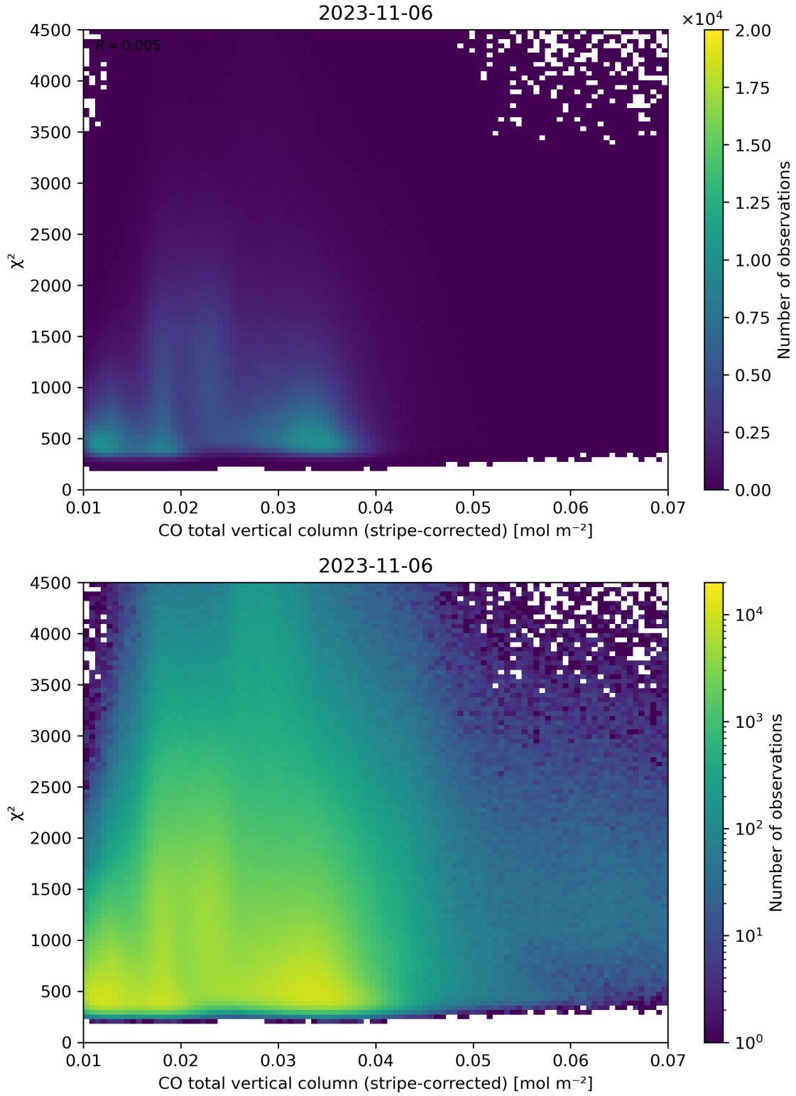
Figure 37: Scatter density plot of “CO total vertical column (stripe-corrected)” against “ \chi^2 ” for 2023-11-05 to 2023-11-07.
