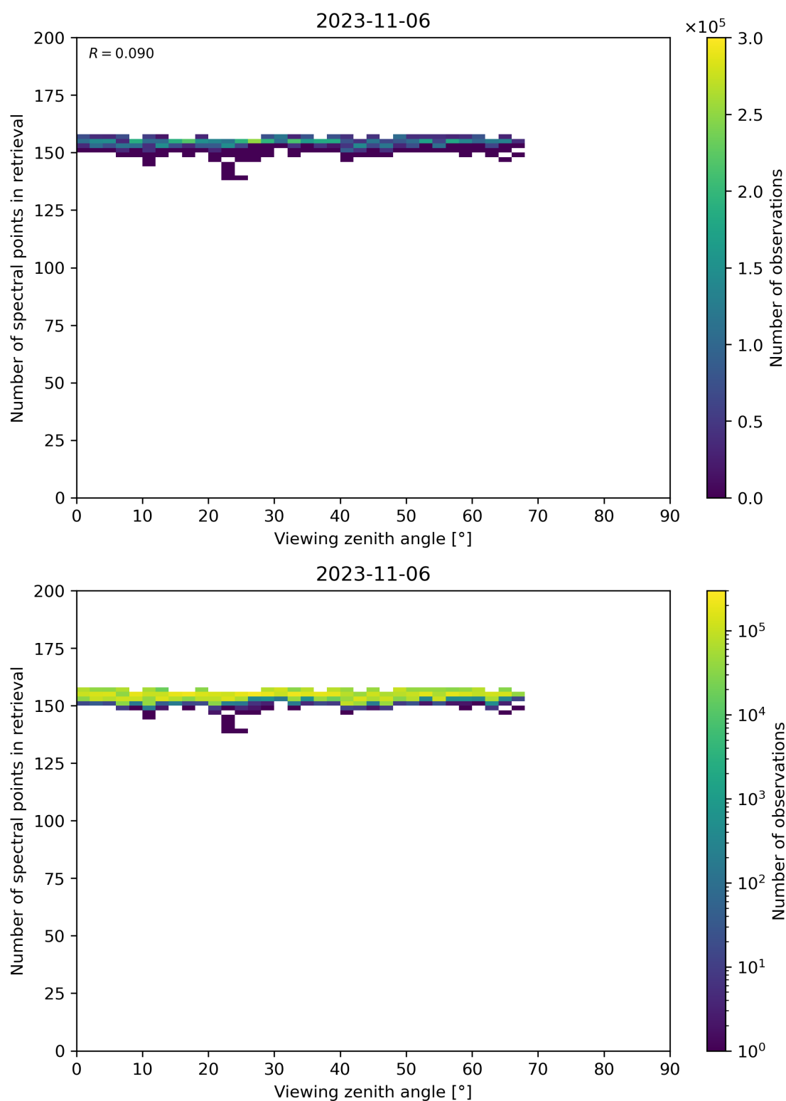
Figure 76: Scatter density plot of “Viewing zenith angle” against “Number of spectral points in retrieval” for 2023-11-05 to 2023-11-07.
