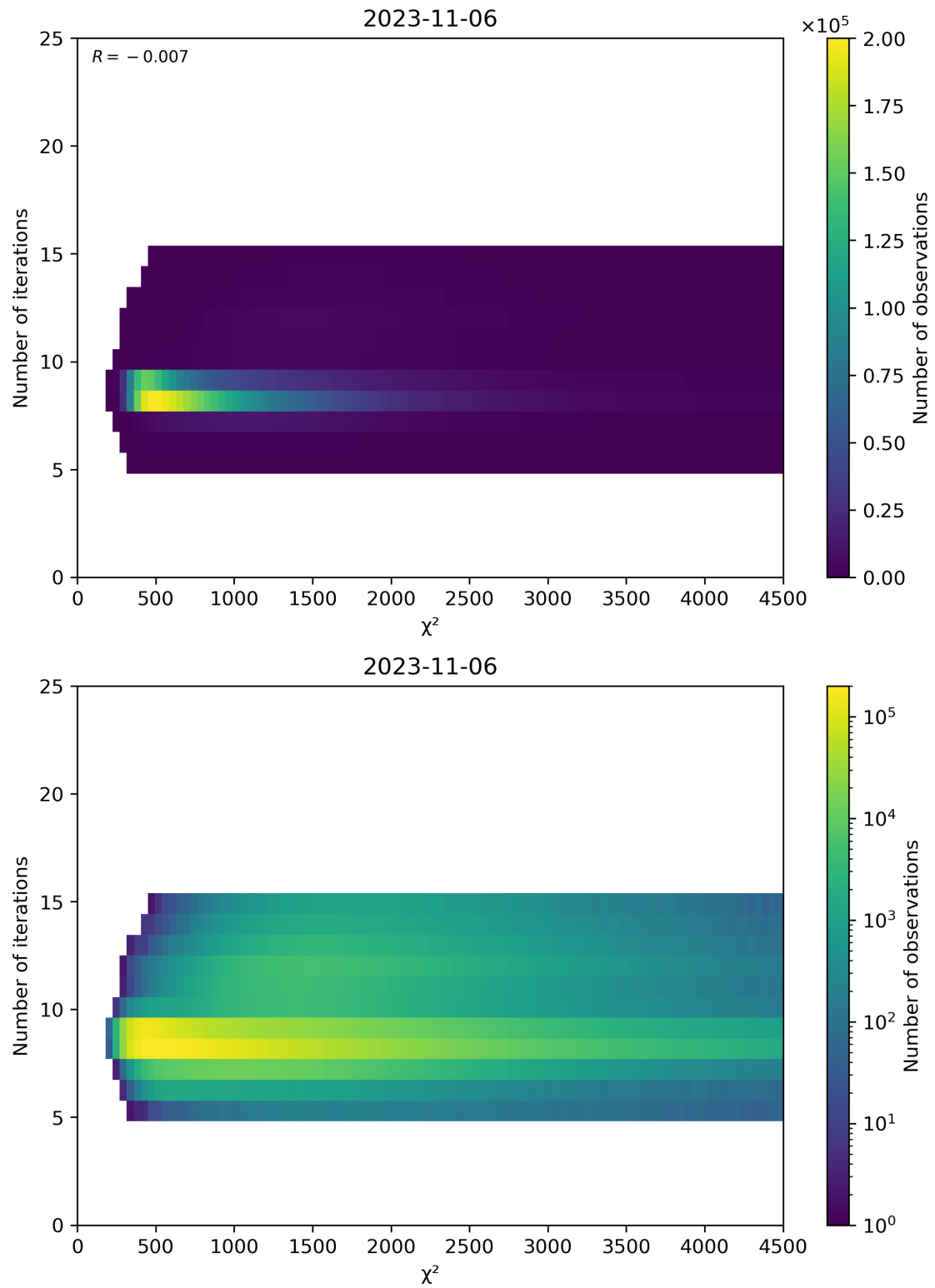
Figure 49: Scatter density plot of “ \chi^2 ” against “Number of iterations” for 2023-11-05 to 2023-11-07.
