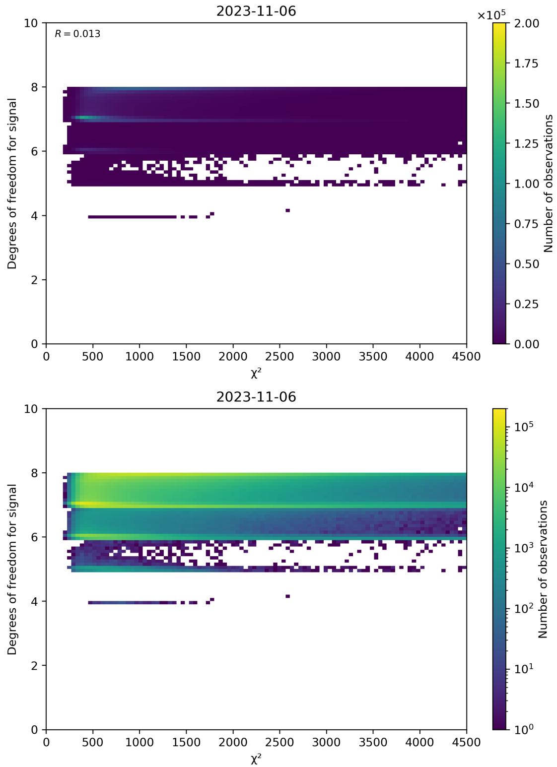
Figure 48: Scatter density plot of “ \chi^2 ” against “Degrees of freedom for signal” for 2023-11-05 to 2023-11-07.
