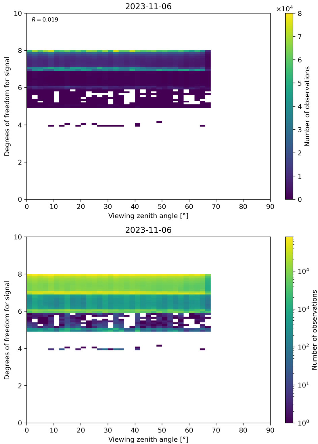
Figure 73: Scatter density plot of “Viewing zenith angle” against “Degrees of freedom for signal” for 2023-11-05 to 2023-11-07.
