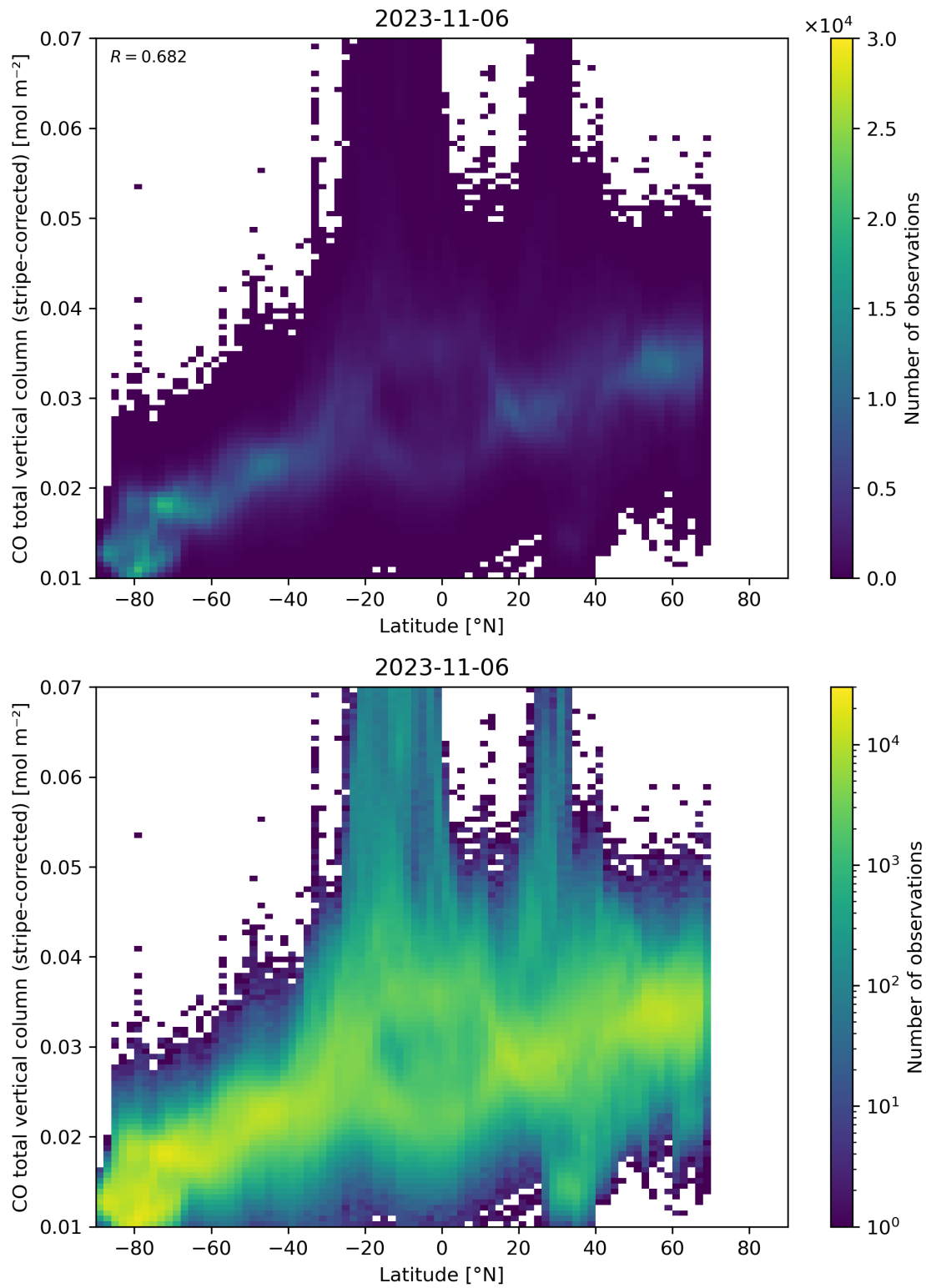
Figure 52: Scatter density plot of “Latitude” against “CO total vertical column (stripe-corrected)” for 2023-11-05 to 2023-11-07.
