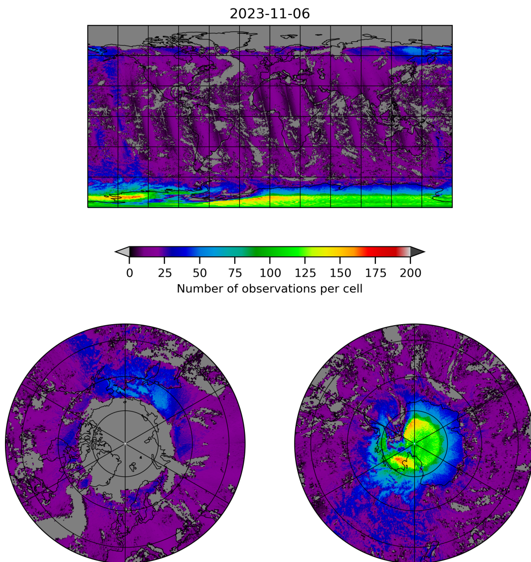
Figure 8: Map of the number of observations for 2023-11-05 to 2023-11-07
