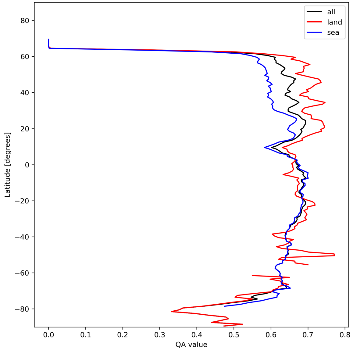
Figure 9: Zonal average of “QA value” for 2023-11-05 to 2023-11-07.
