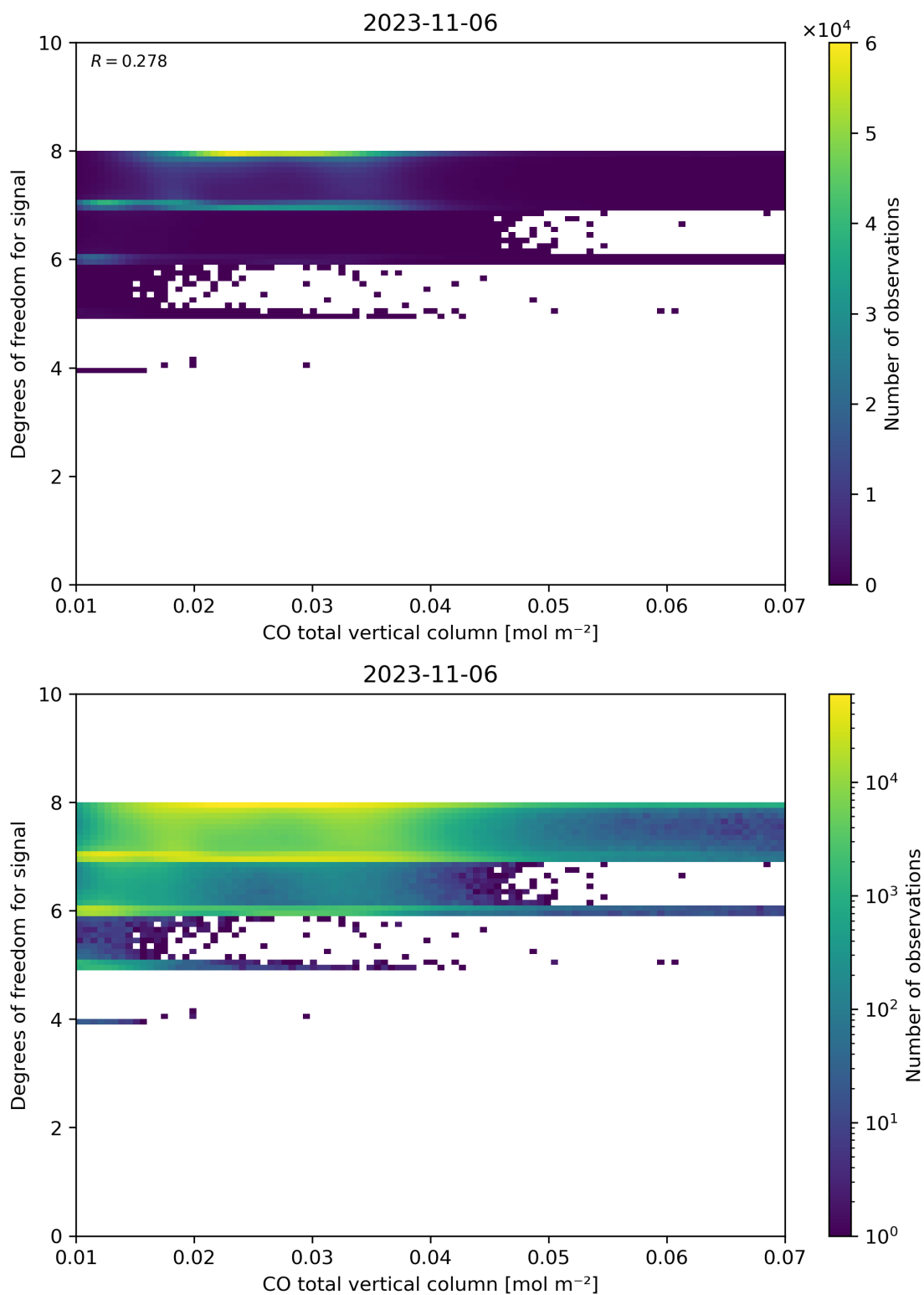
Figure 41: Scatter density plot of “CO total vertical column” against “Degrees of freedom for signal” for 2023-11-05 to 2023-11-07.
