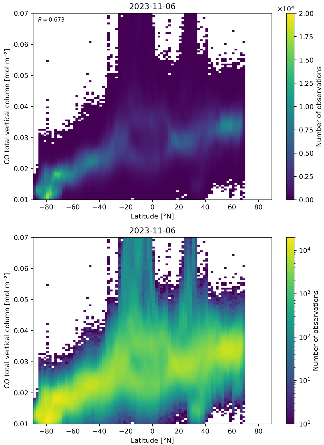
Figure 51: Scatter density plot of “Latitude” against “CO total vertical column” for 2023-11-05 to 2023-11-07.
