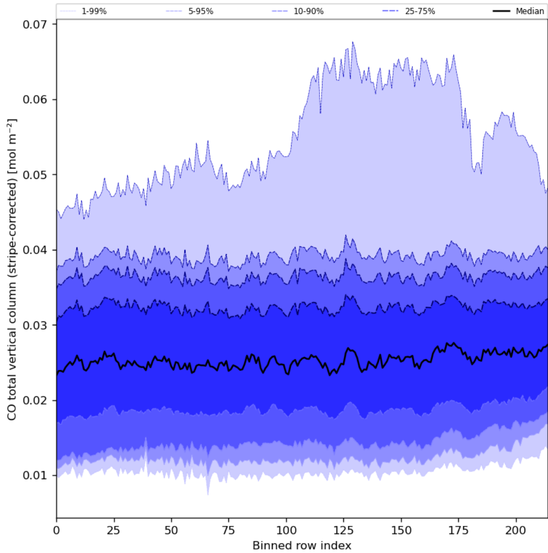
Figure 27: Along track statistics of “CO total vertical column (stripe-corrected)” for 2023-11-05 to 2023-11-07
