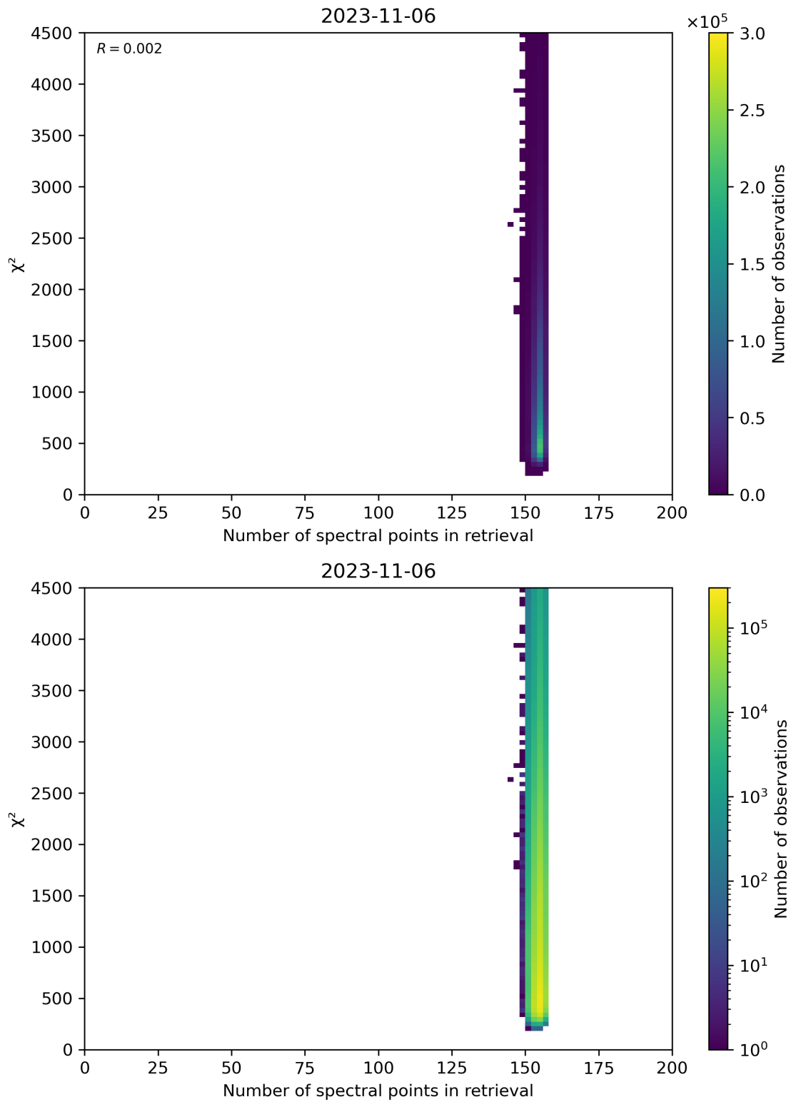
Figure 58: Scatter density plot of “Number of spectral points in retrieval” against “ \chi^2 ” for 2023-11-05 to 2023-11-07.
