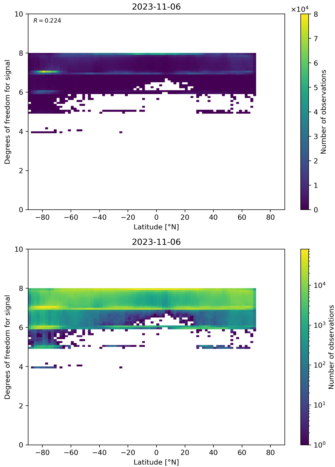
Figure 55: Scatter density plot of “Latitude” against “Degrees of freedom for signal” for 2023-11-05 to 2023-11-07.
