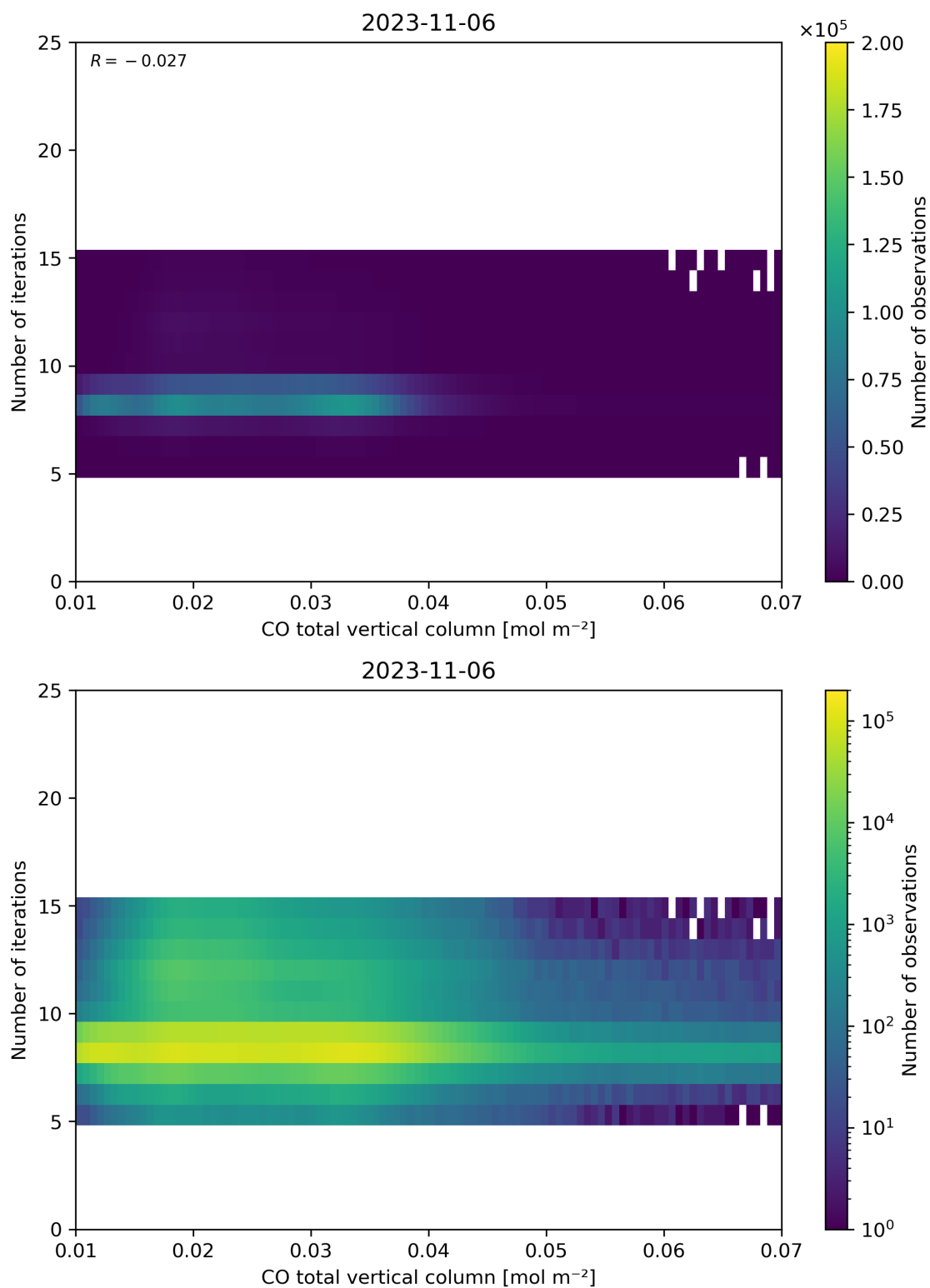
Figure 42: Scatter density plot of “CO total vertical column” against “Number of iterations” for 2023-11-05 to 2023-11-07.
