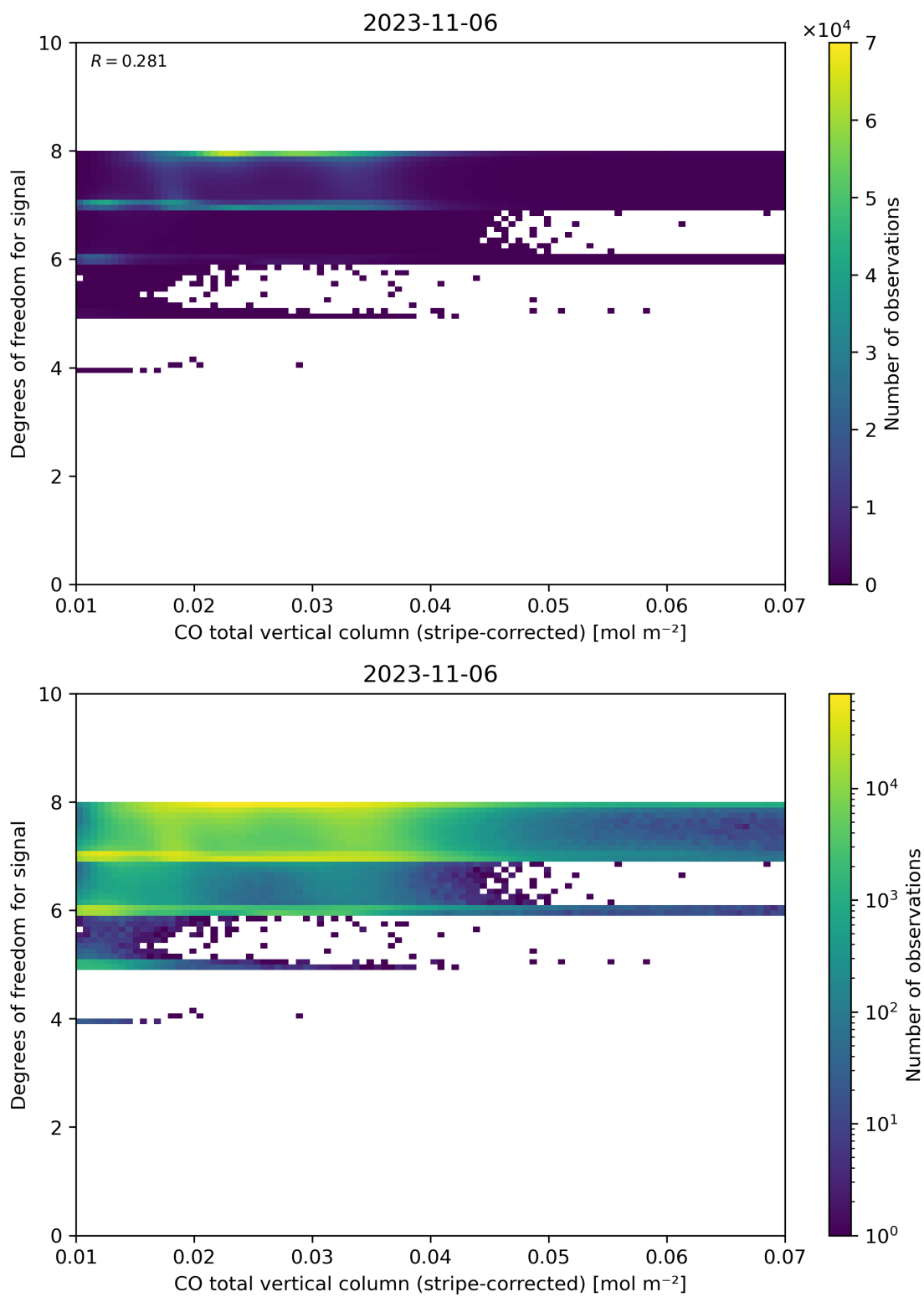
Figure 38: Scatter density plot of “CO total vertical column (stripe-corrected)” against “Degrees of freedom for signal” for 2023-11-05 to 2023-11-07.
