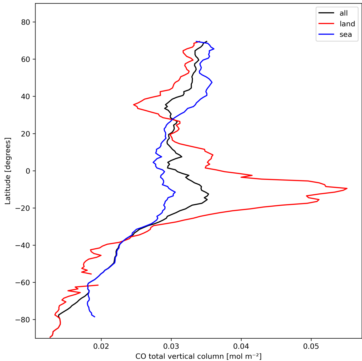
Figure 10: Zonal average of “CO total vertical column” for 2023-11-05 to 2023-11-07.
