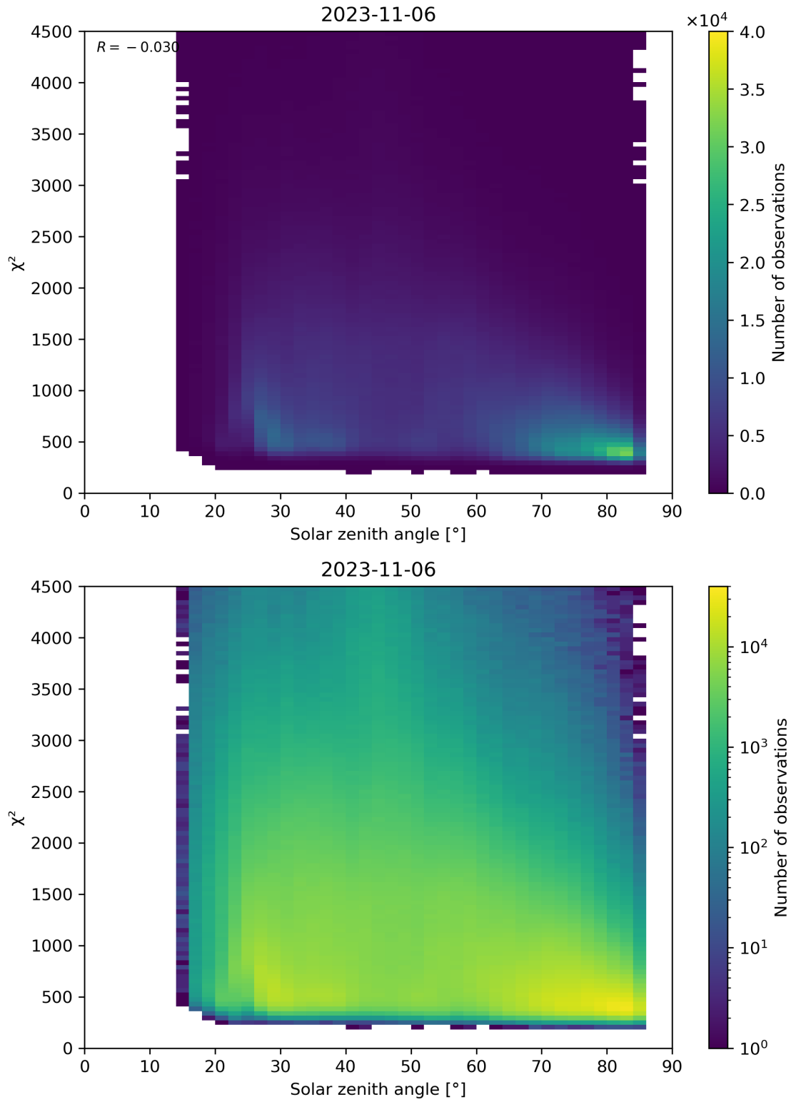
Figure 64: Scatter density plot of “Solar zenith angle” against “ \chi^2 ” for 2023-11-05 to 2023-11-07.
