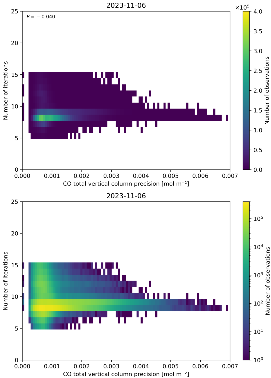
Figure 46: Scatter density plot of “CO total vertical column precision” against “Number of iterations” for 2023-11-05 to 2023-11-07.
