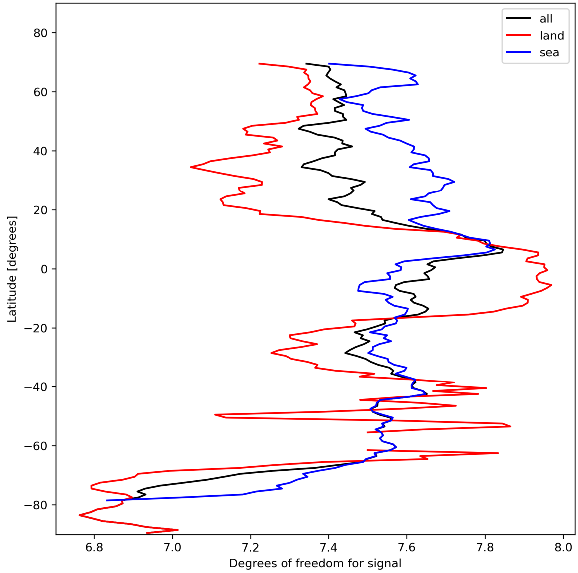
Figure 15: Zonal average of “Degrees of freedom for signal” for 2023-11-05 to 2023-11-07.
