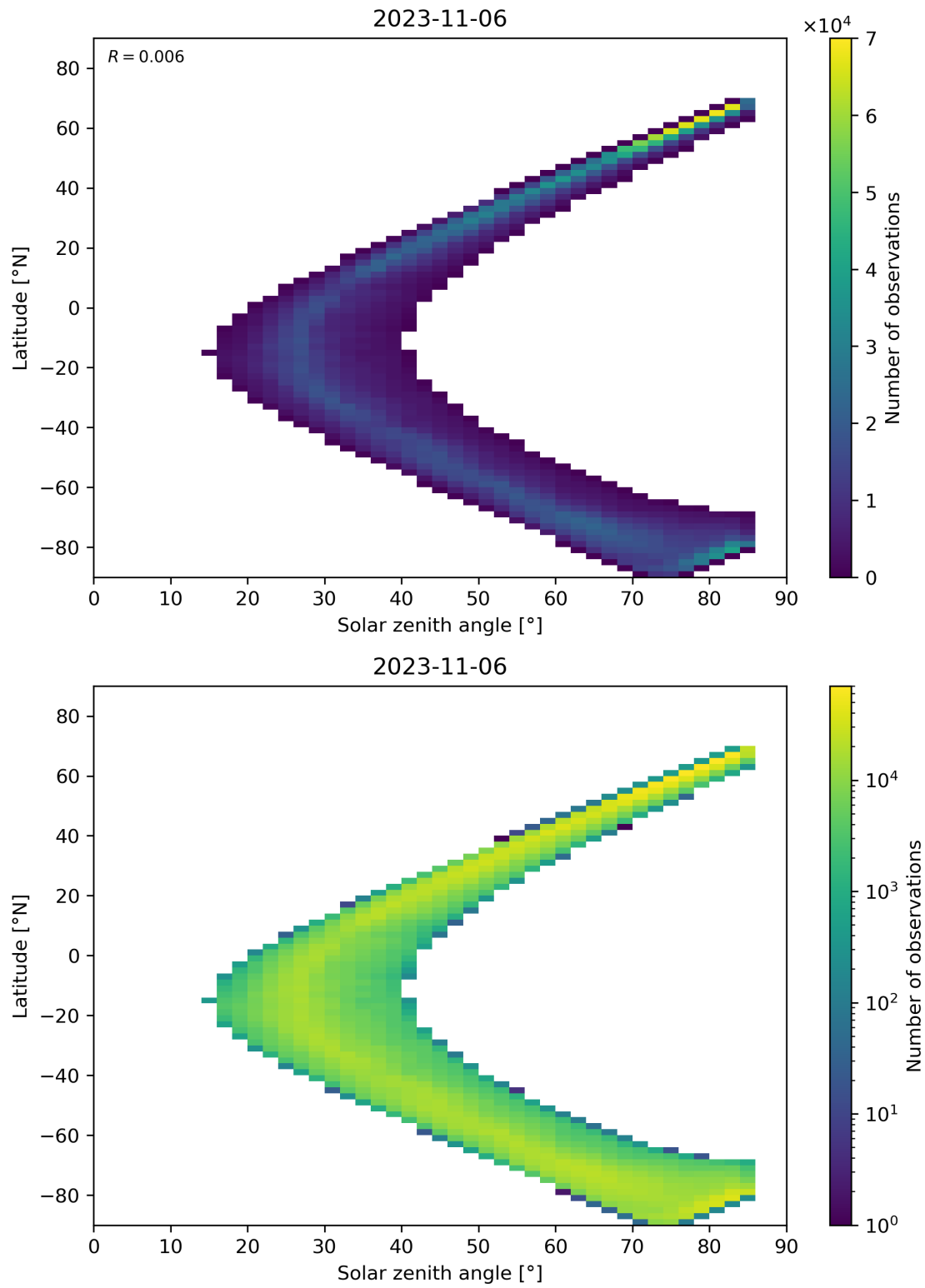
Figure 66: Scatter density plot of “Solar zenith angle” against “Latitude” for 2023-11-05 to 2023-11-07.
