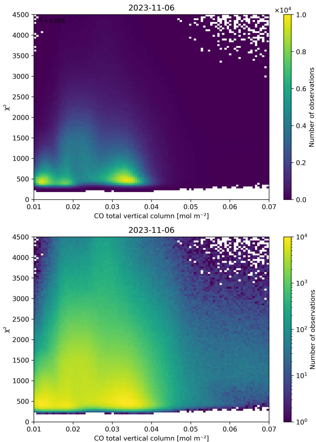
Figure 35: Scatter density plot of “CO total vertical column” against “ \chi^2 ” for 2023-11-05 to 2023-11-07.
