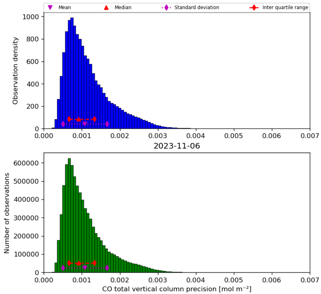
Figure 20: Histogram of “CO total vertical column precision” for 2023-11-05 to 2023-11-07
