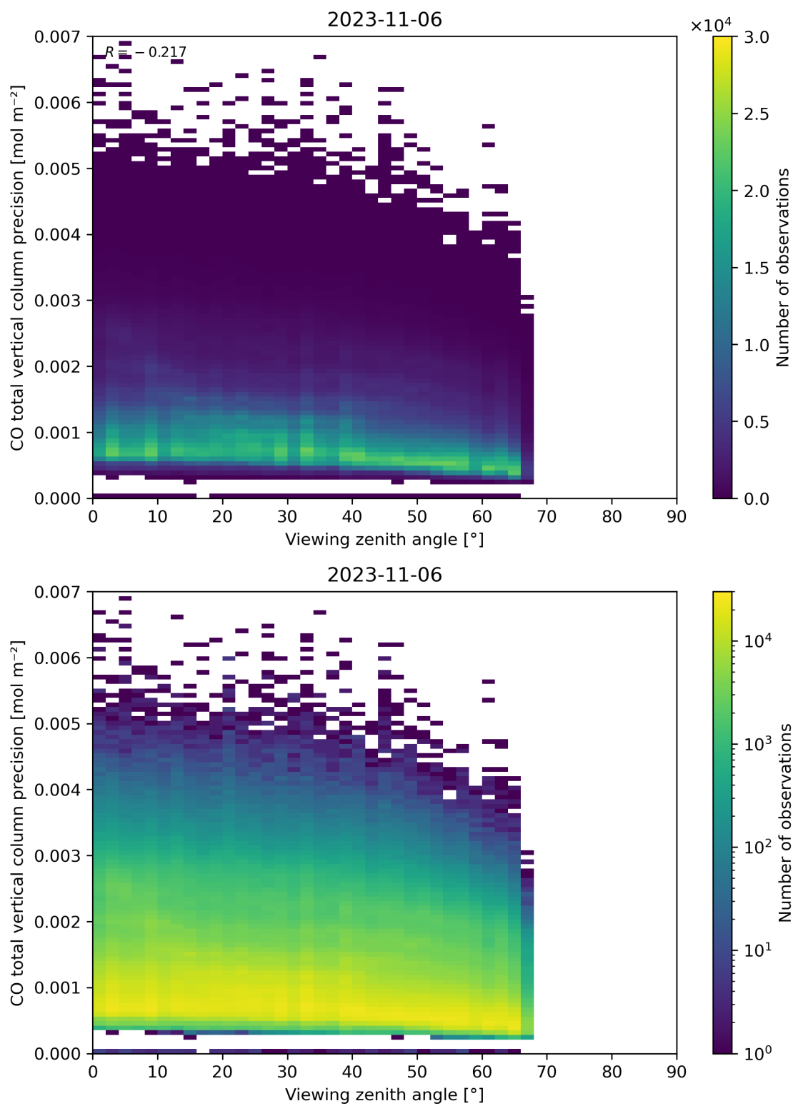
Figure 71: Scatter density plot of “Viewing zenith angle” against “CO total vertical column precision” for 2023-11-05 to 2023-11-07.
