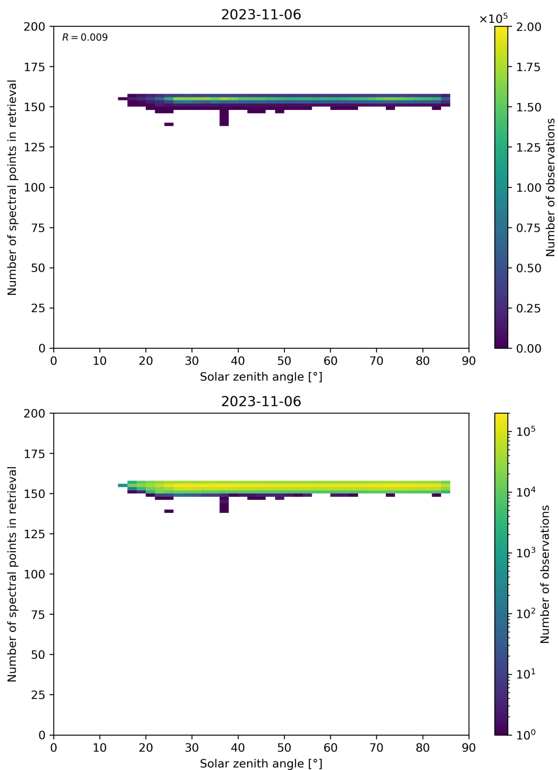
Figure 68: Scatter density plot of “Solar zenith angle” against “Number of spectral points in retrieval” for 2023-11-05 to 2023-11-07.
