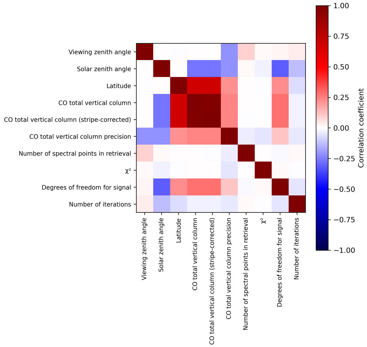
Figure 2: Map of correlation matrix for 2023-11-05 to 2023-11-07.
