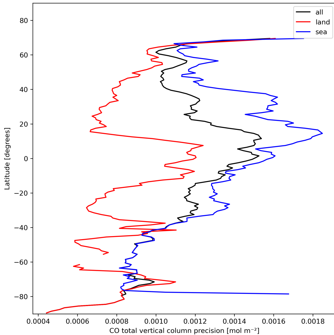
Figure 12: Zonal average of “CO total vertical column precision” for 2023-11-05 to 2023-11-07.
