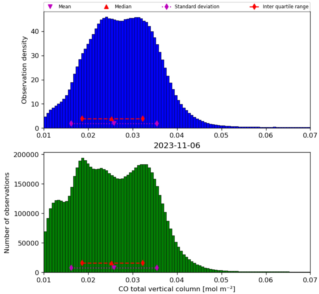
Figure 18: Histogram of “CO total vertical column” for 2023-11-05 to 2023-11-07
