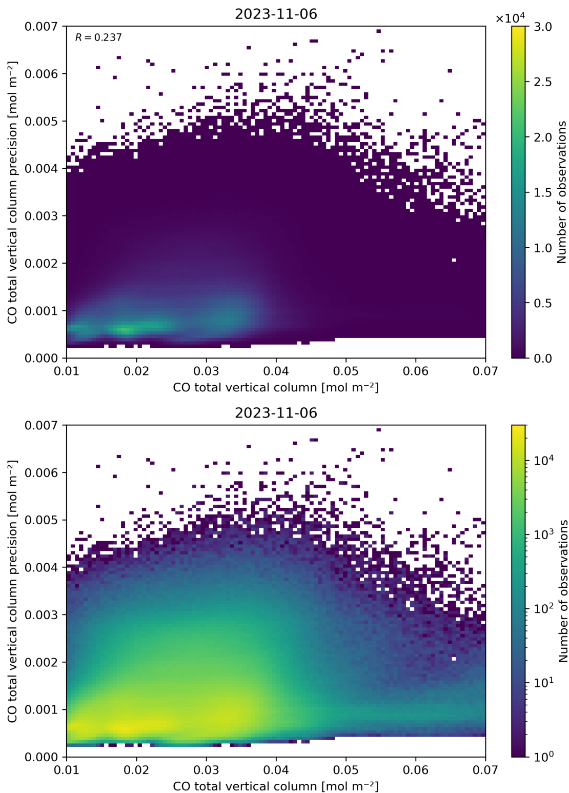
Figure 34: Scatter density plot of “CO total vertical column” against “CO total vertical column precision” for 2023-11-05 to 2023-11-07.
