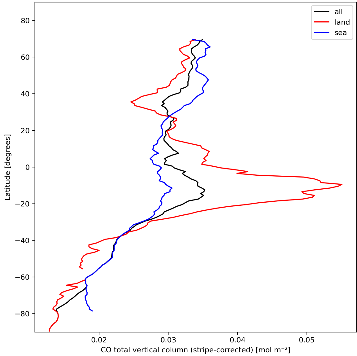
Figure 11: Zonal average of “CO total vertical column (stripe-corrected)” for 2023-11-05 to 2023-11-07.
