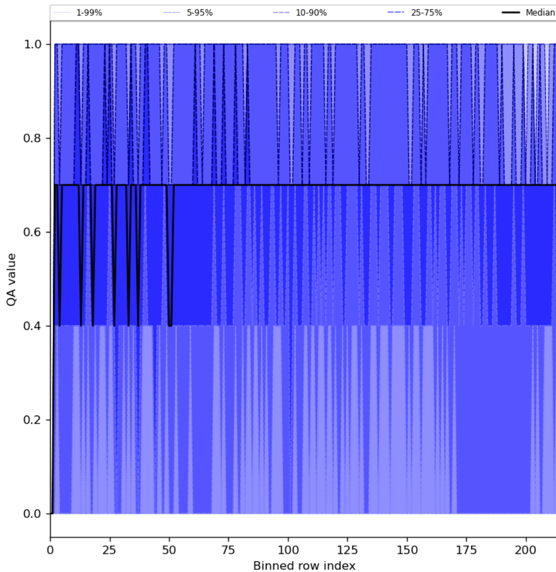
Figure 25: Along track statistics of “QA value” for 2023-11-05 to 2023-11-07
