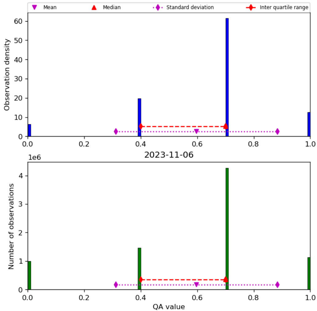
Figure 17: Histogram of “QA value” for 2023-11-05 to 2023-11-07
