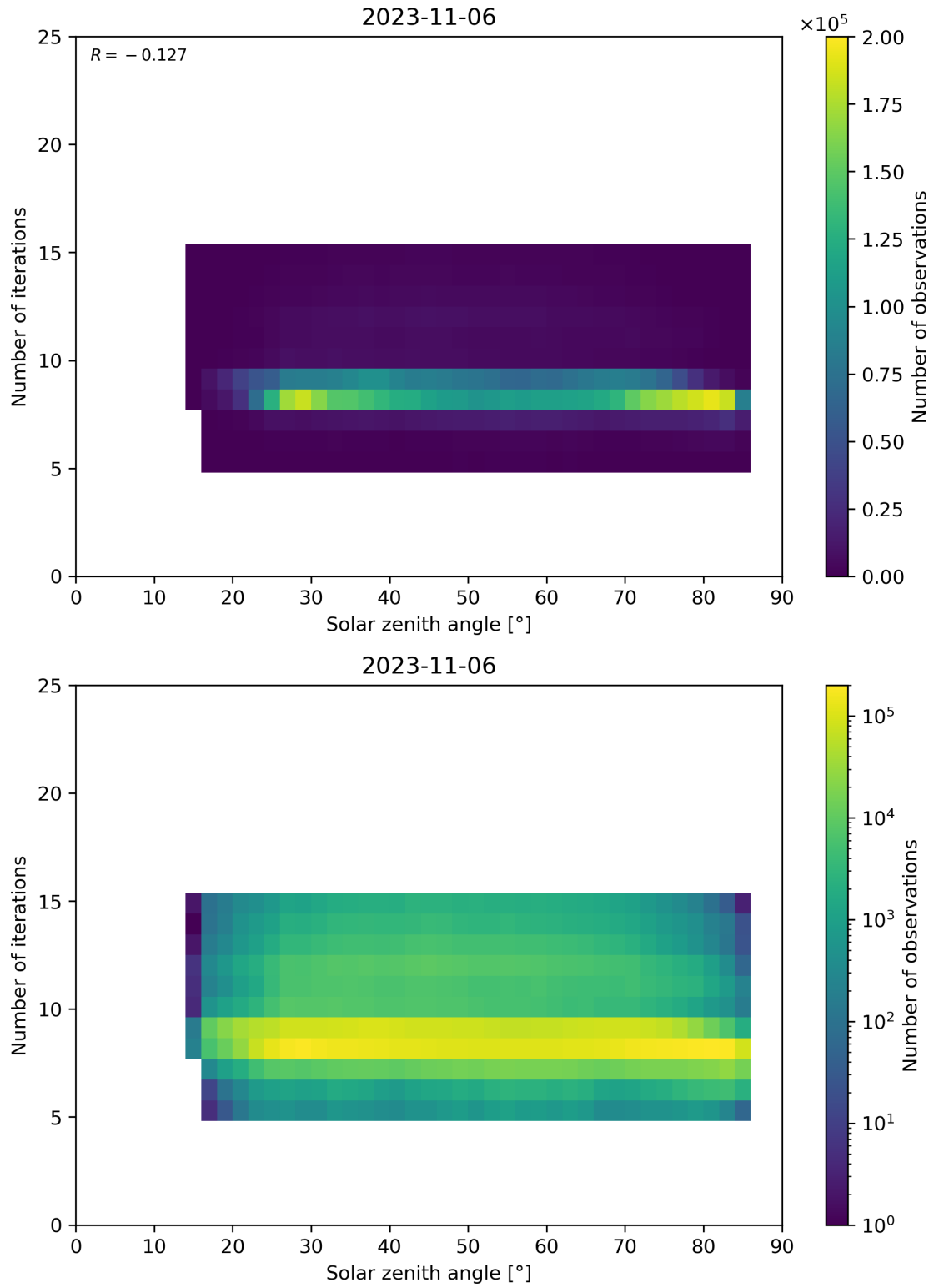
Figure 67: Scatter density plot of “Solar zenith angle” against “Number of iterations” for 2023-11-05 to 2023-11-07.
