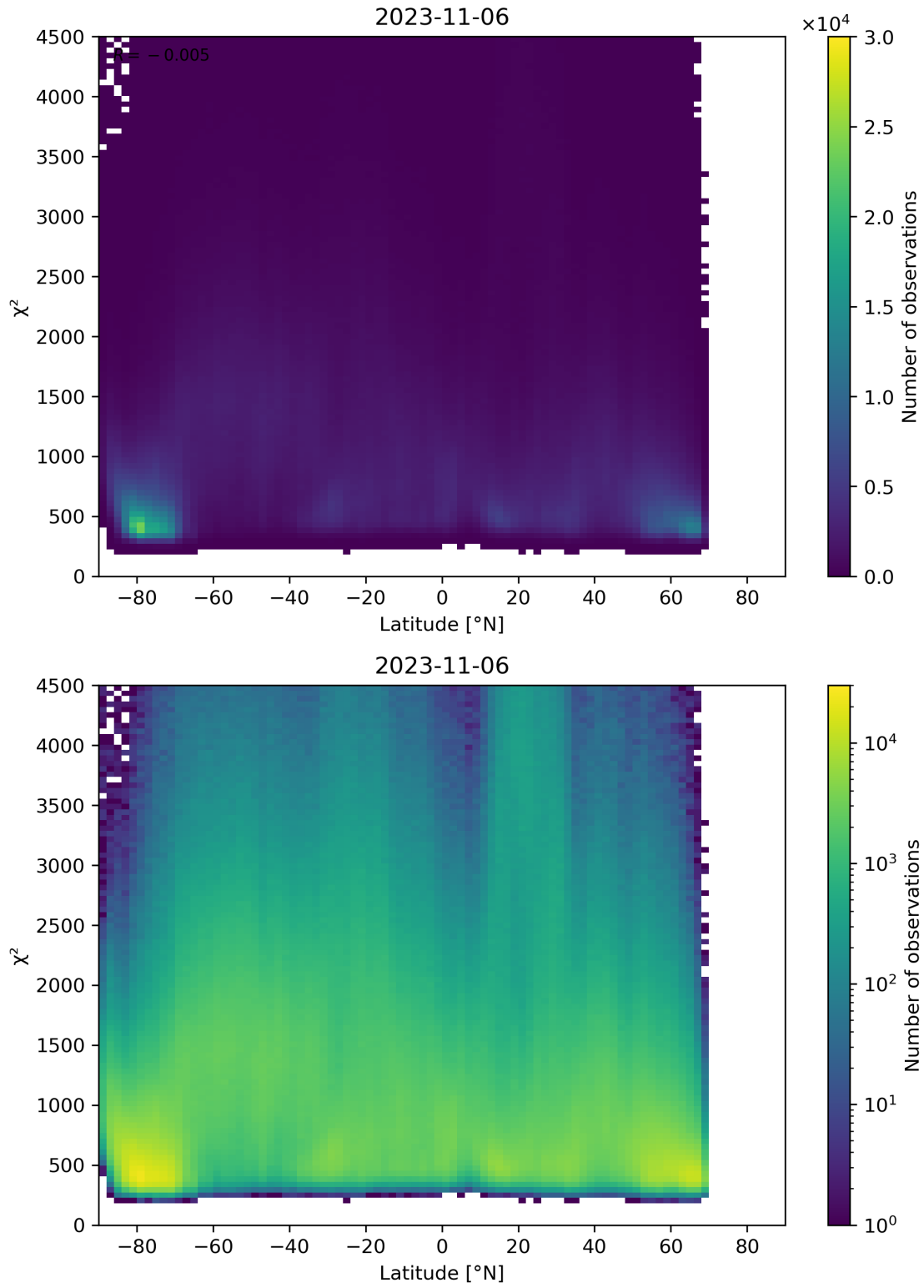
Figure 54: Scatter density plot of “Latitude” against “ \chi^2 ” for 2023-11-05 to 2023-11-07.
