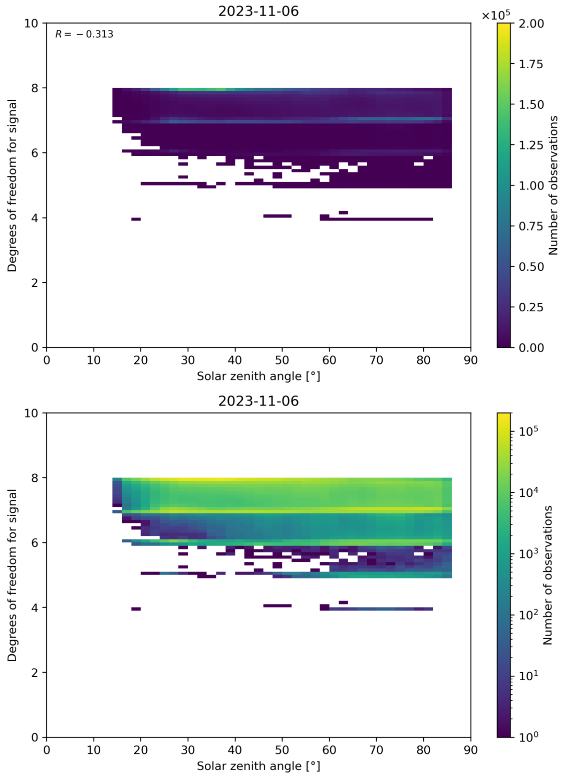
Figure 65: Scatter density plot of “Solar zenith angle” against “Degrees of freedom for signal” for 2023-11-05 to 2023-11-07.
