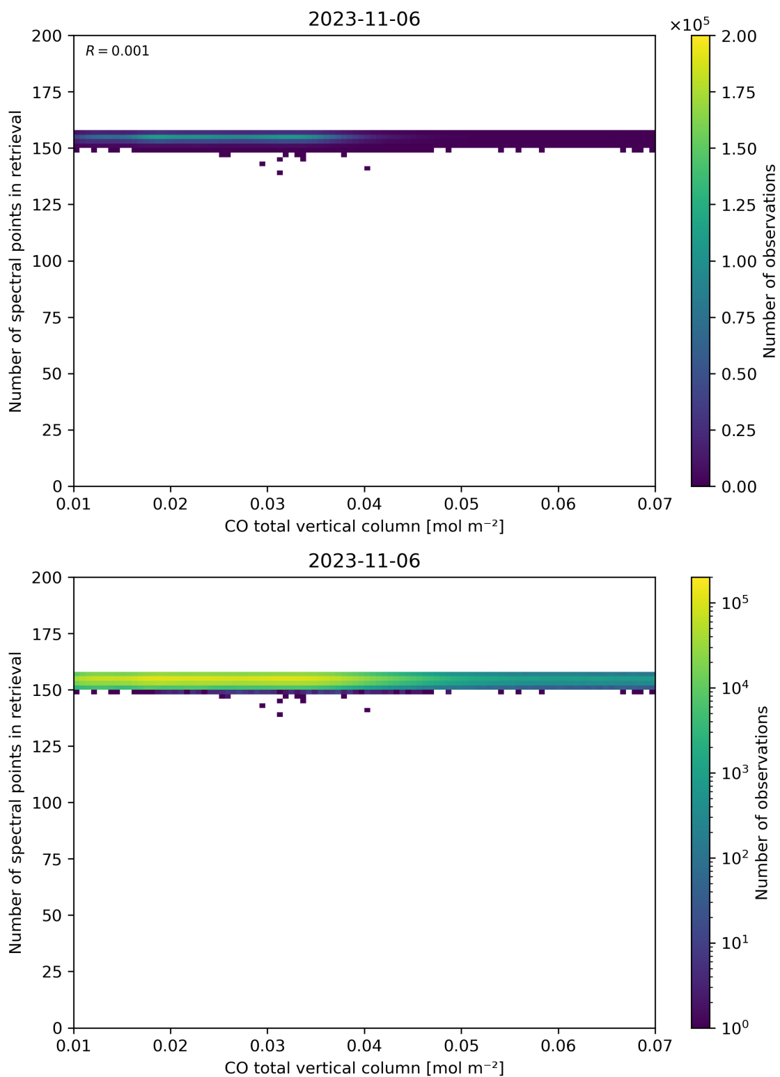
Figure 43: Scatter density plot of “CO total vertical column” against “Number of spectral points in retrieval” for 2023-11-05 to 2023-11-07.
