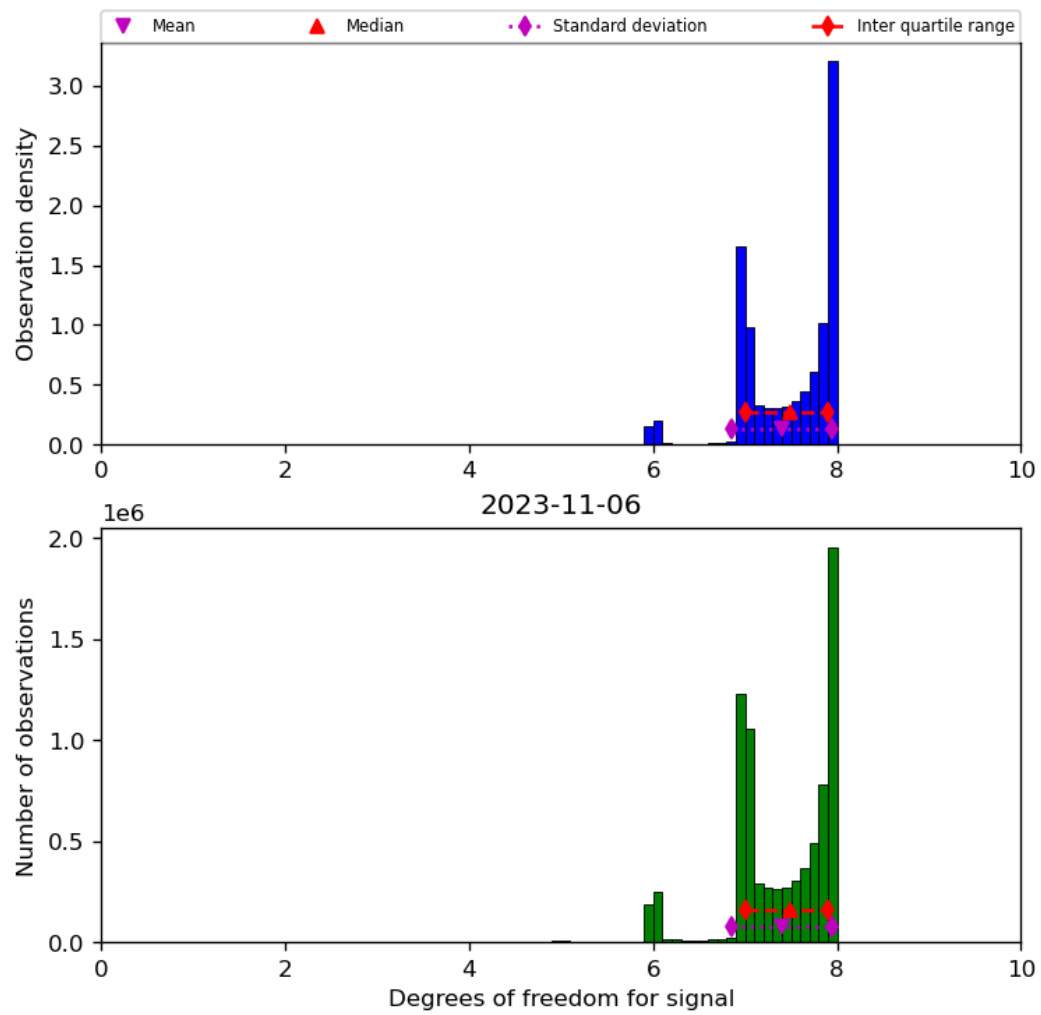
Figure 23: Histogram of “Degrees of freedom for signal” for 2023-11-05 to 2023-11-07
