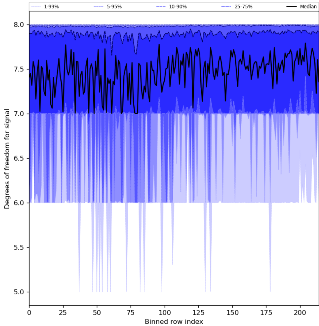
Figure 31: Along track statistics of “Degrees of freedom for signal” for 2023-11-05 to 2023-11-07
