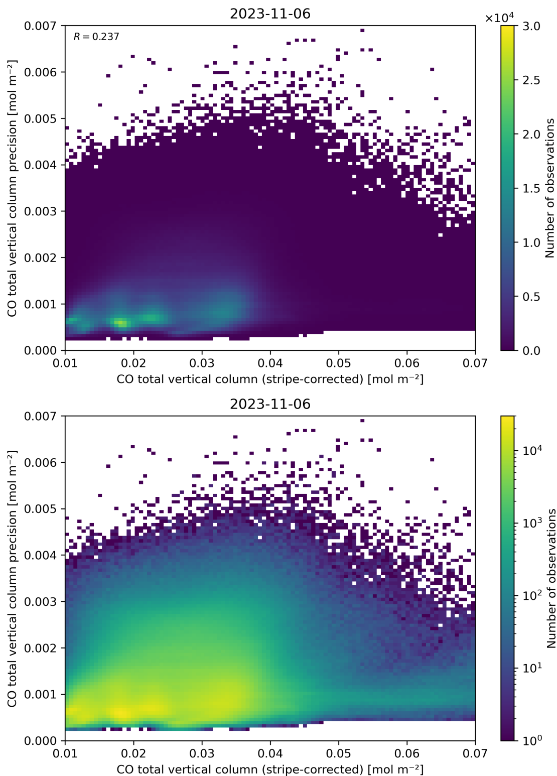
Figure 36: Scatter density plot of “CO total vertical column (stripe-corrected)” against “CO total vertical column precision” for 2023-11-05 to 2023-11-07.
