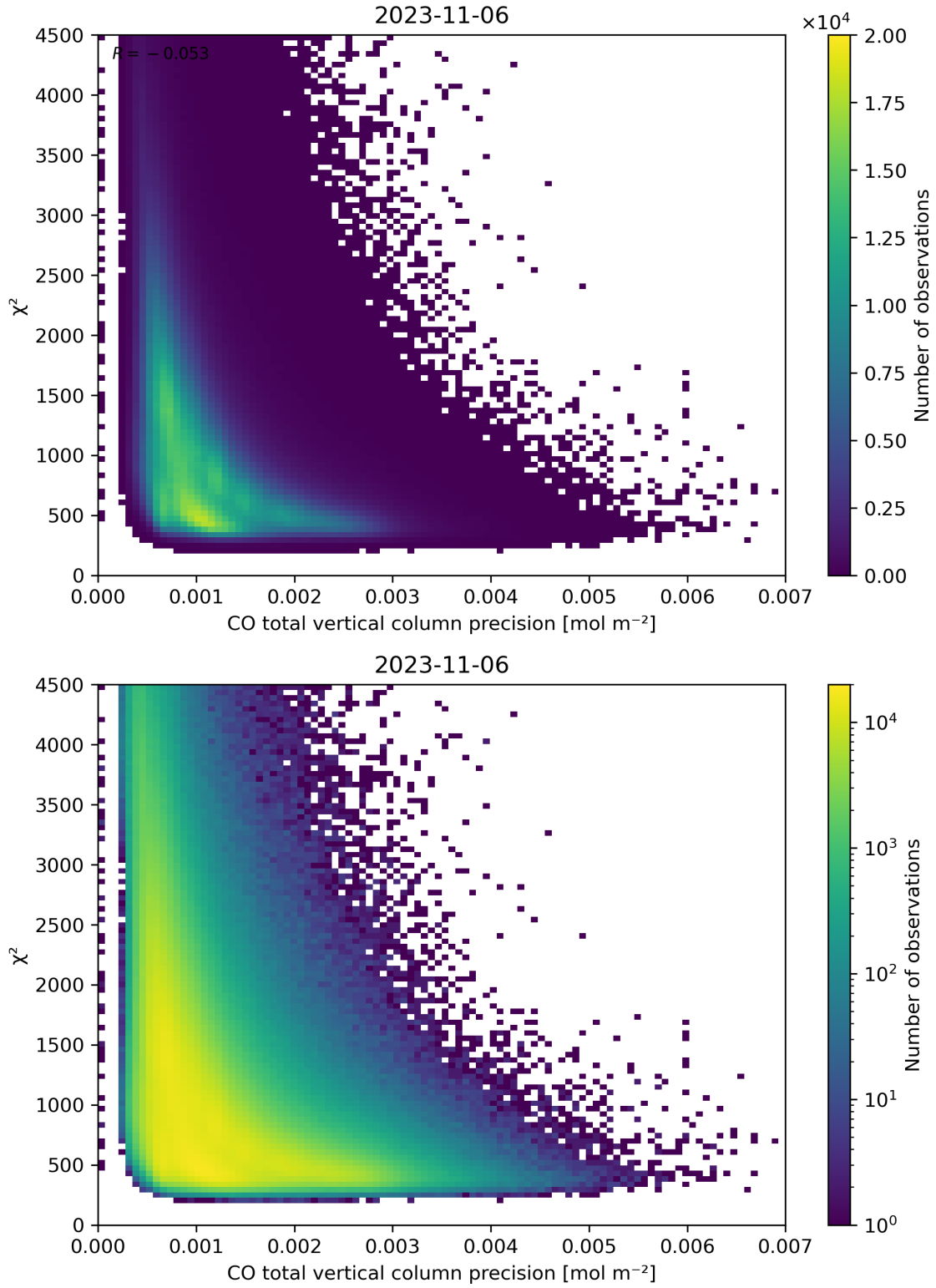
Figure 44: Scatter density plot of “CO total vertical column precision” against “ \chi^2 ” for 2023-11-05 to 2023-11-07.
