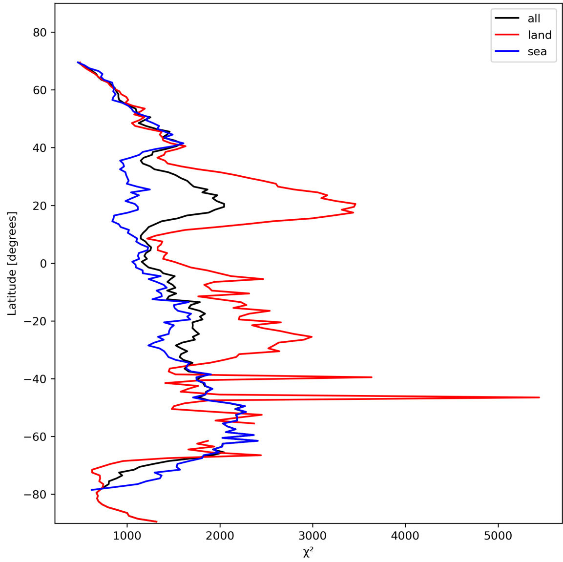
Figure 14: Zonal average of “ \chi^2 ” for 2023-11-05 to 2023-11-07.
