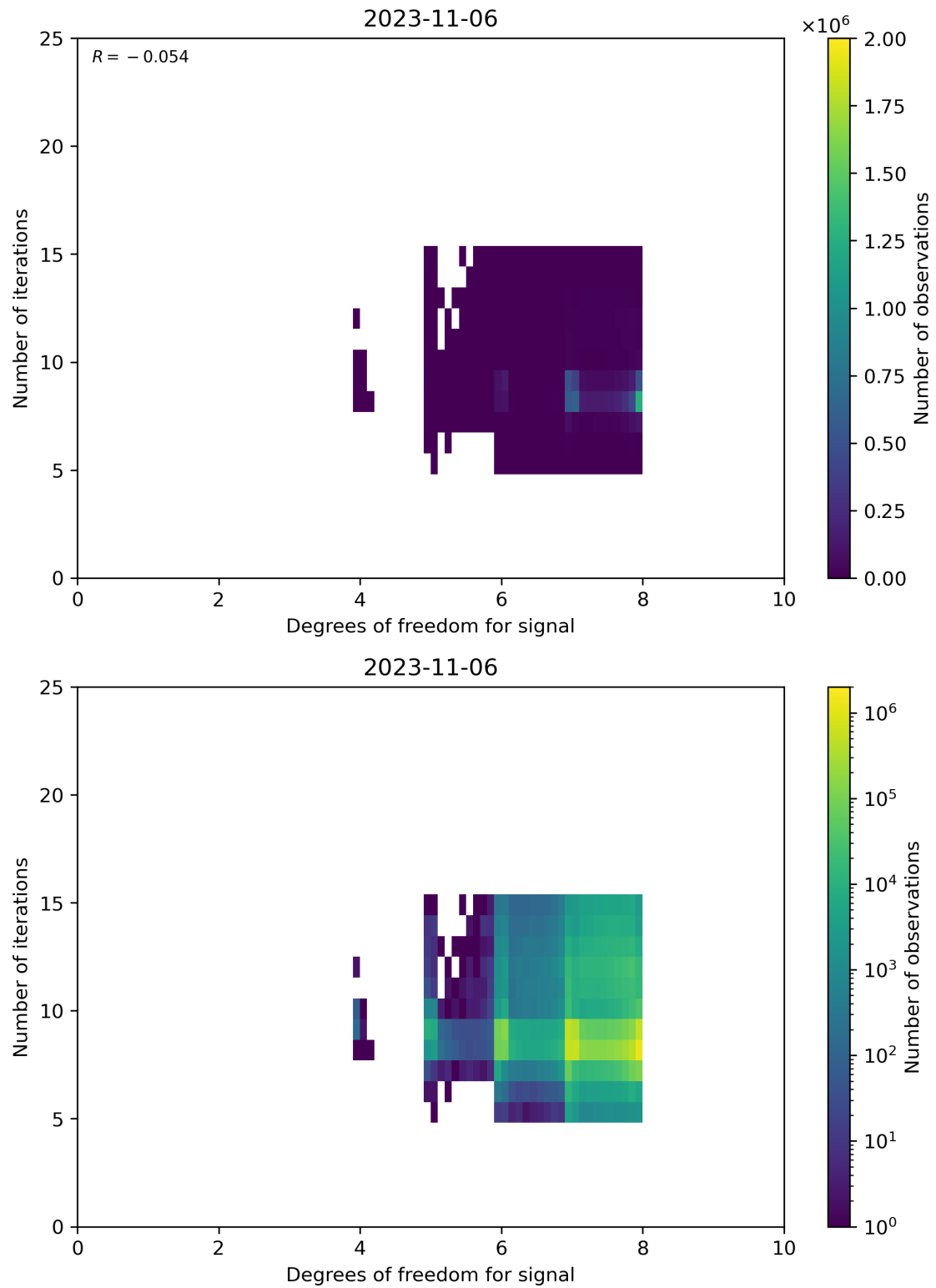
Figure 50: Scatter density plot of “Degrees of freedom for signal” against “Number of iterations” for 2023-11-05 to 2023-11-07.
