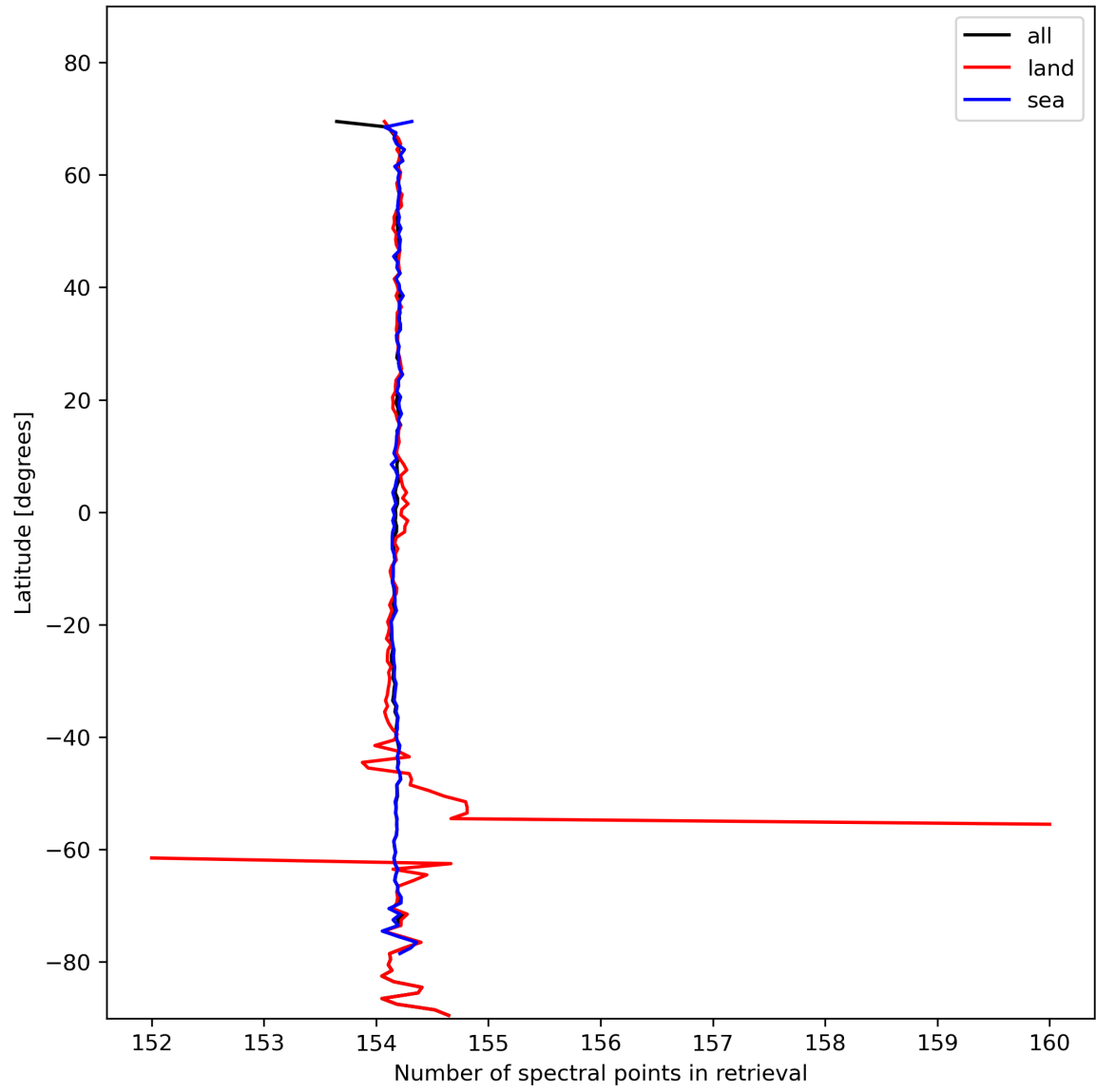
Figure 13: Zonal average of “Number of spectral points in retrieval” for 2023-11-05 to 2023-11-07.
