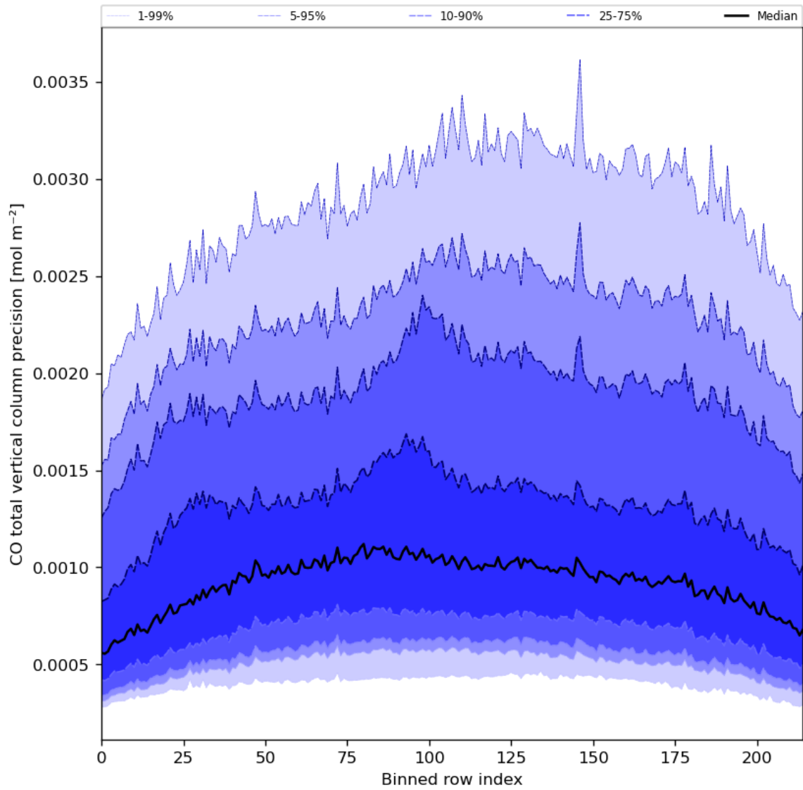
Figure 28: Along track statistics of “CO total vertical column precision” for 2023-11-05 to 2023-11-07
