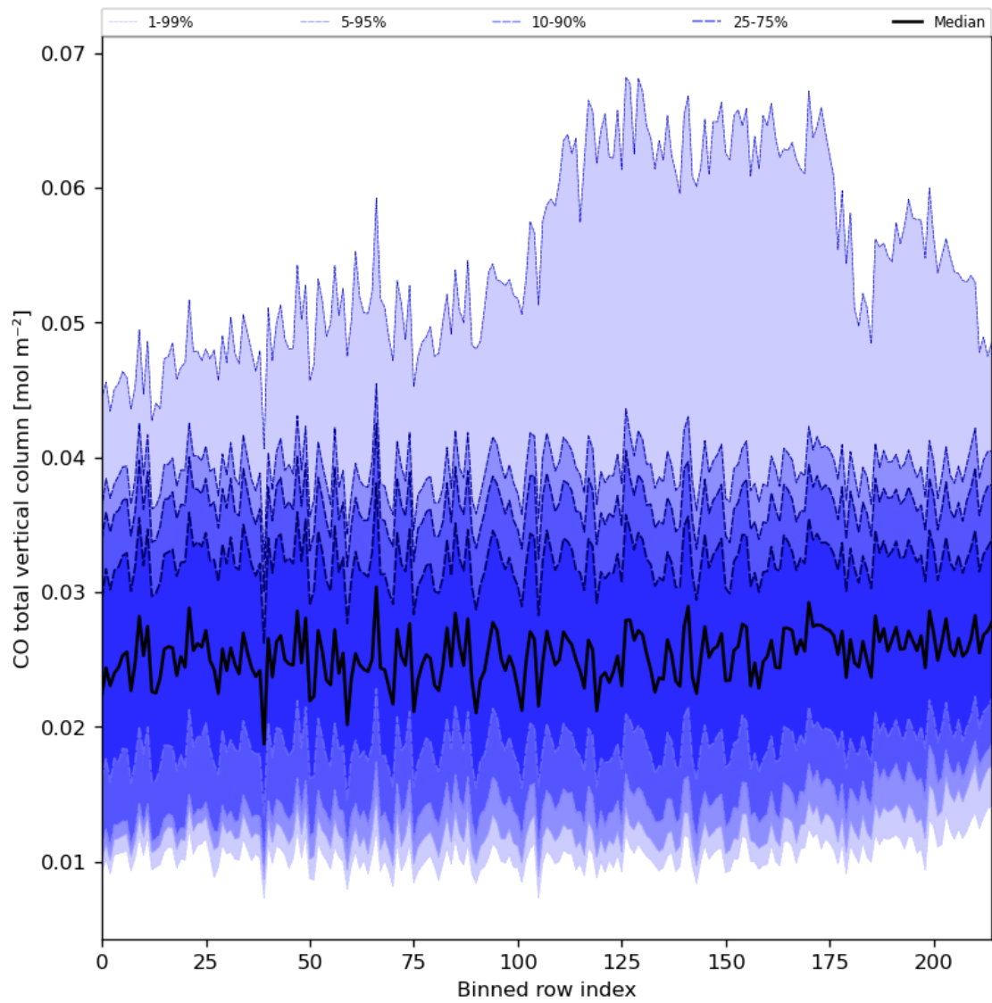
Figure 26: Along track statistics of “CO total vertical column” for 2023-11-05 to 2023-11-07
