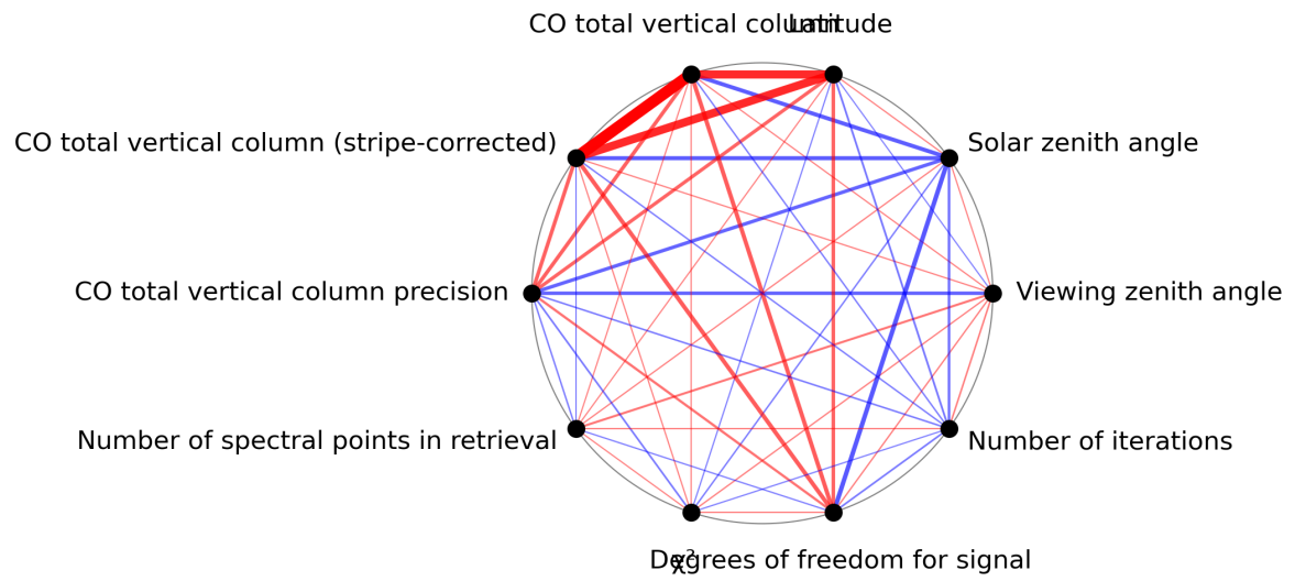
Figure 1: Map of correlation graph for 2023-11-05 to 2023-11-07.
