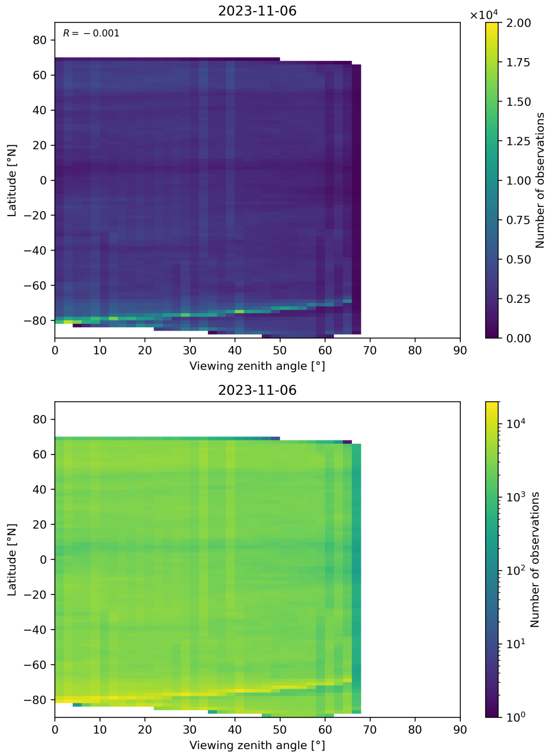
Figure 74: Scatter density plot of “Viewing zenith angle” against “Latitude” for 2023-11-05 to 2023-11-07.
