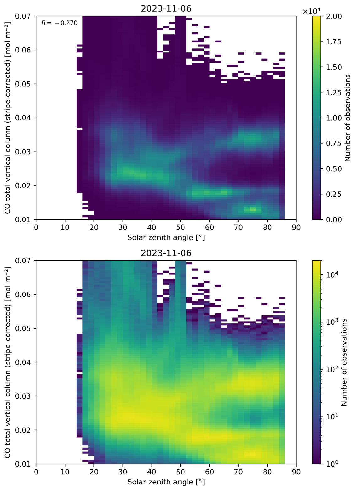
Figure 62: Scatter density plot of “Solar zenith angle” against “CO total vertical column (stripe-corrected)” for 2023-11-05 to 2023-11-07.
