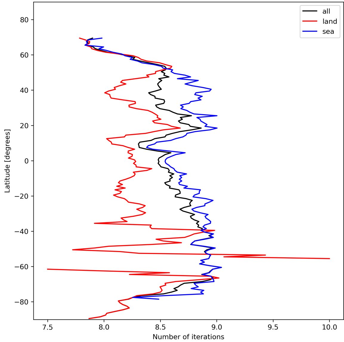
Figure 16: Zonal average of “Number of iterations” for 2023-11-05 to 2023-11-07.
