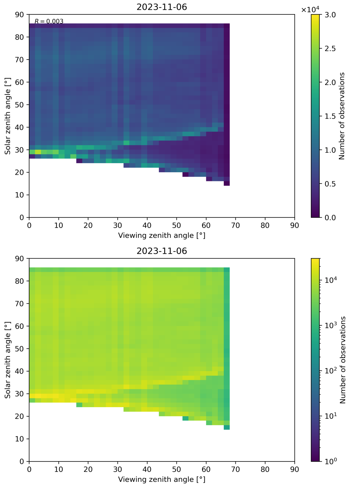
Figure 77: Scatter density plot of “Viewing zenith angle” against “Solar zenith angle” for 2023-11-05 to 2023-11-07.
