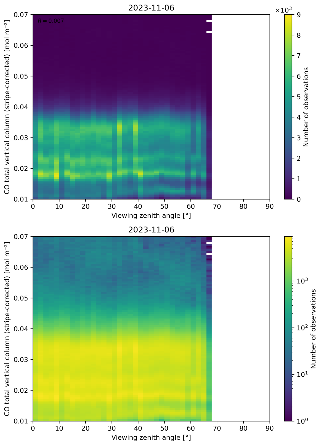
Figure 70: Scatter density plot of “Viewing zenith angle” against “CO total vertical column (stripe-corrected)” for 2023-11-05 to 2023-11-07.
