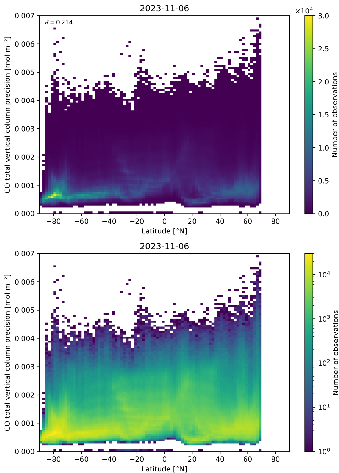
Figure 53: Scatter density plot of “Latitude” against “CO total vertical column precision” for 2023-11-05 to 2023-11-07.
