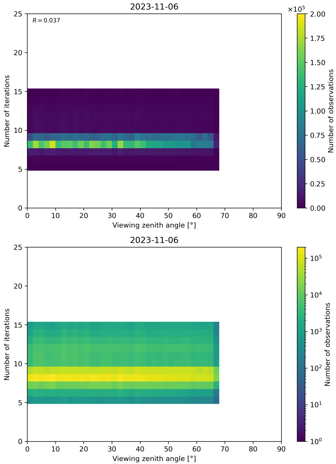
Figure 75: Scatter density plot of “Viewing zenith angle” against “Number of iterations” for 2023-11-05 to 2023-11-07.
