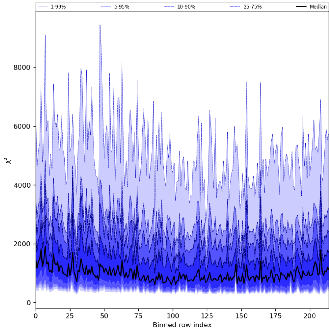
Figure 30: Along track statistics of “ \chi^2 ” for 2023-11-05 to 2023-11-07
