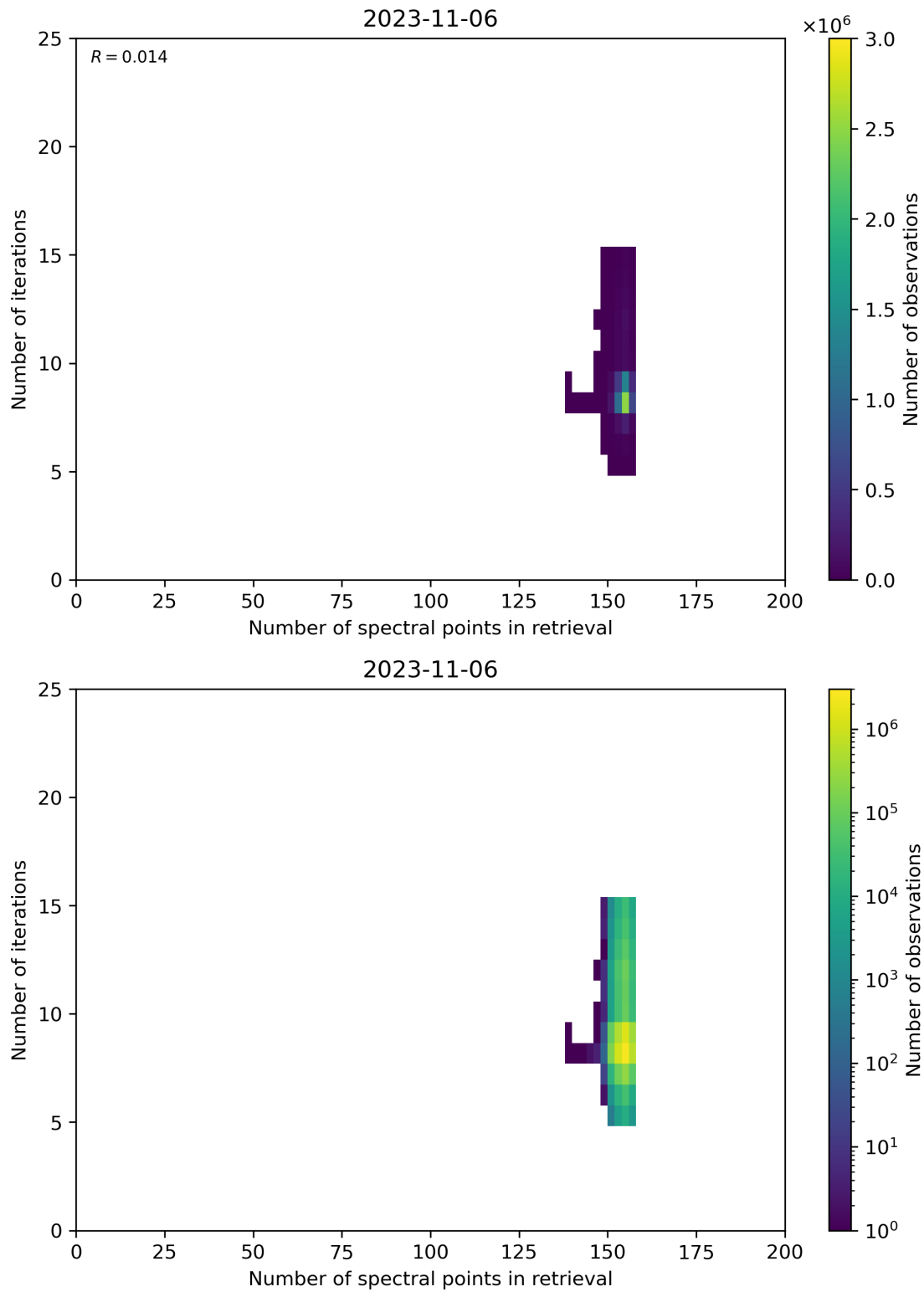
Figure 60: Scatter density plot of “Number of spectral points in retrieval” against “Number of iterations” for 2023-11-05 to 2023-11-07.
