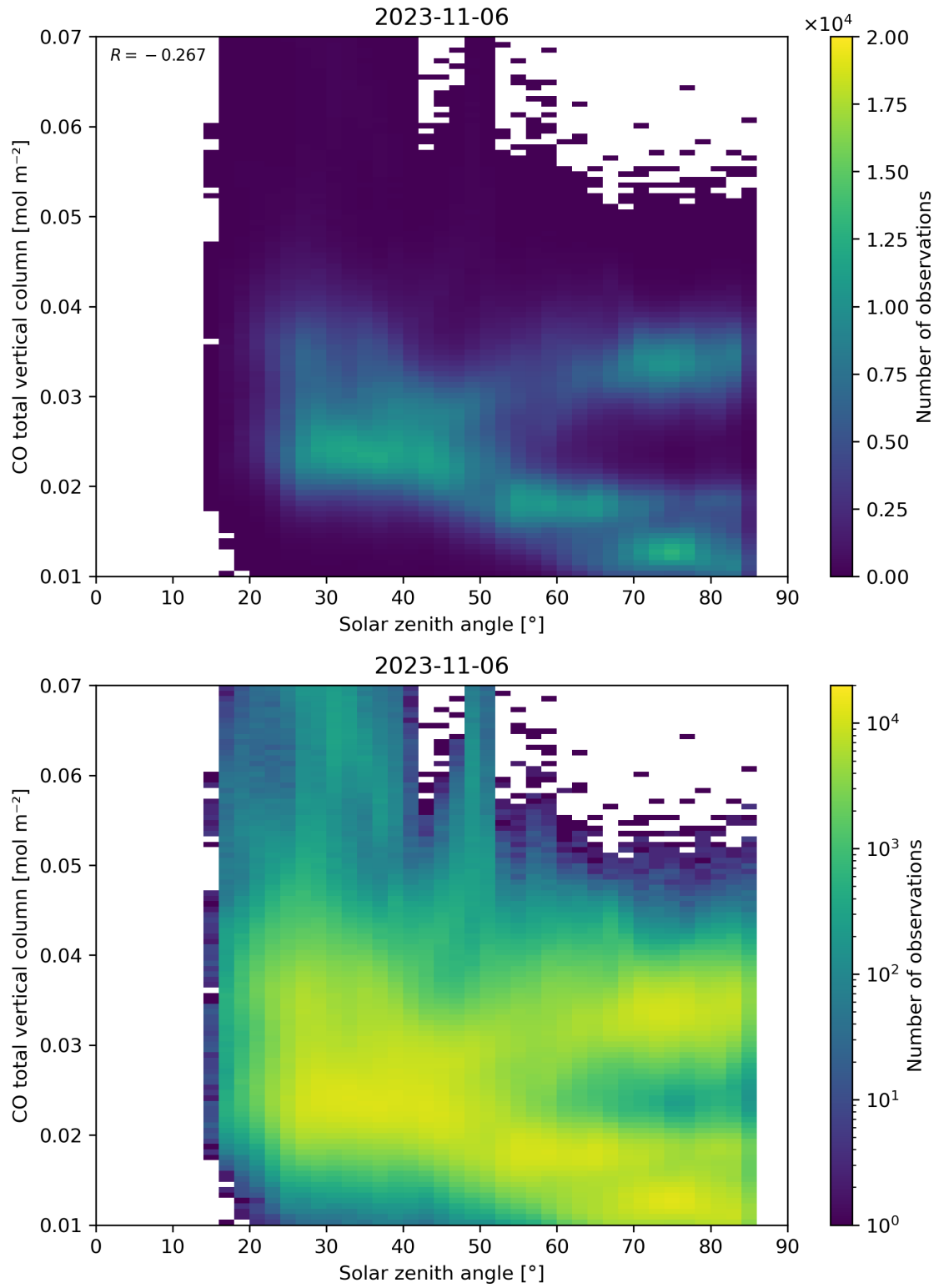
Figure 61: Scatter density plot of “Solar zenith angle” against “CO total vertical column” for 2023-11-05 to 2023-11-07.
