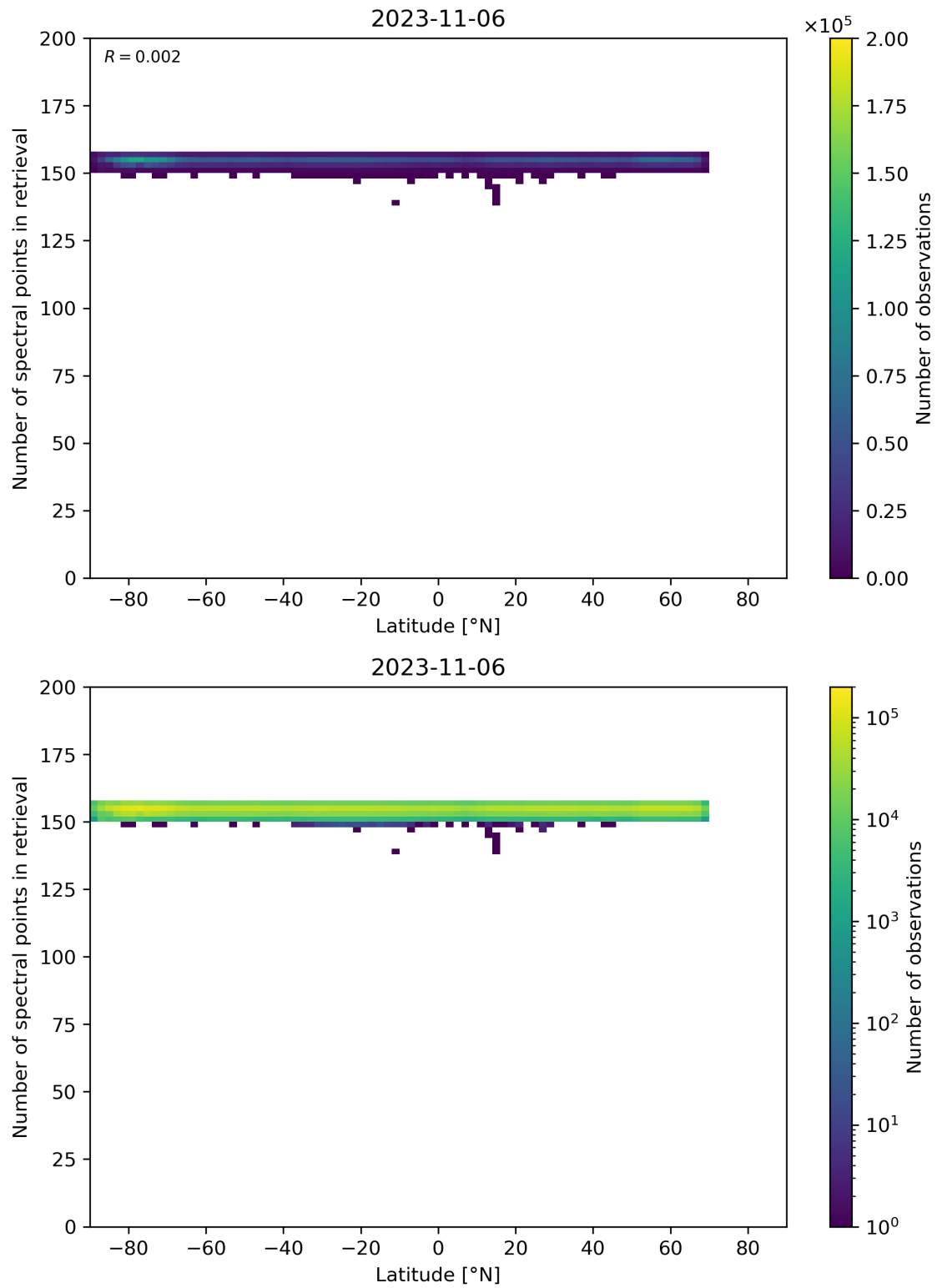
Figure 57: Scatter density plot of “Latitude” against “Number of spectral points in retrieval” for 2023-11-05 to 2023-11-07.
