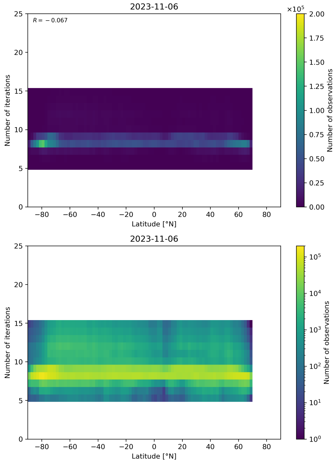
Figure 56: Scatter density plot of “Latitude” against “Number of iterations” for 2023-11-05 to 2023-11-07.
