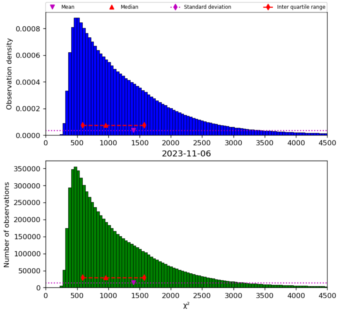
Figure 22: Histogram of “ \chi^2 ” for 2023-11-05 to 2023-11-07
