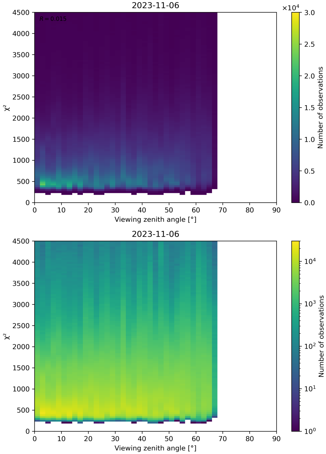
Figure 72: Scatter density plot of “Viewing zenith angle” against “ \chi^2 ” for 2023-11-05 to 2023-11-07.
