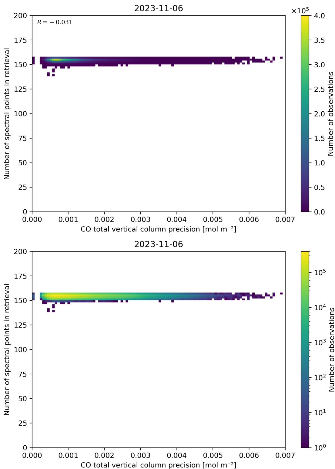
Figure 47: Scatter density plot of “CO total vertical column precision” against “Number of spectral points in retrieval” for 2023-11-05 to 2023-11-07.
