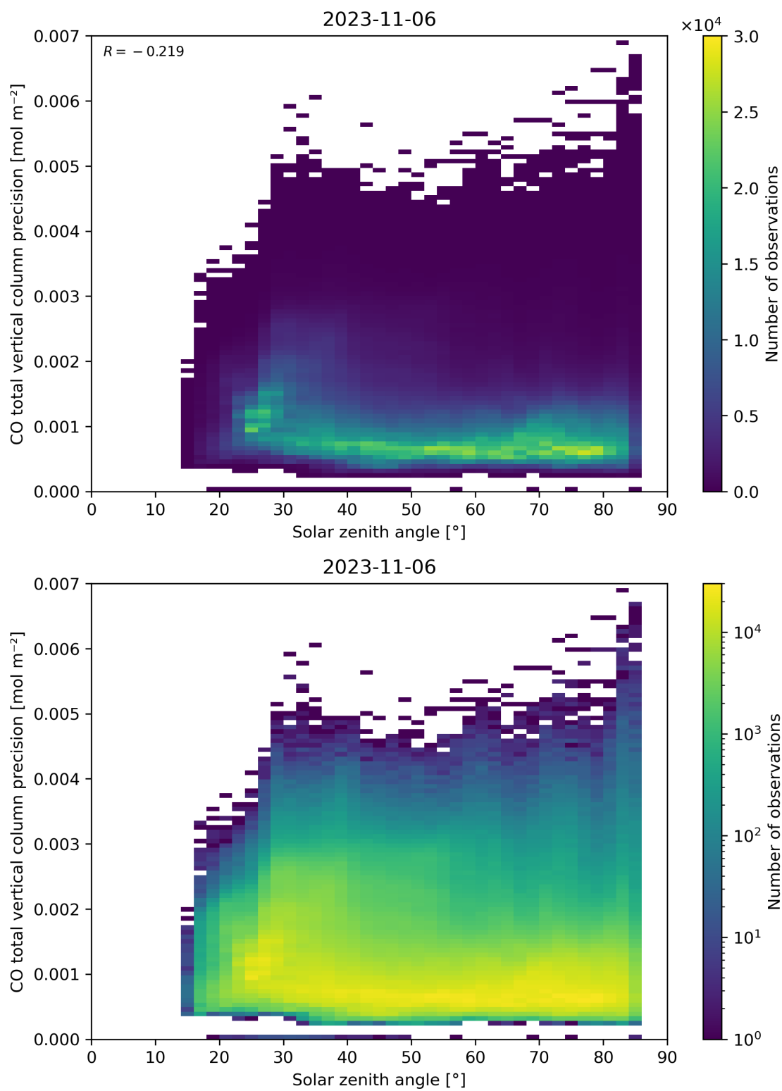
Figure 63: Scatter density plot of “Solar zenith angle” against “CO total vertical column precision” for 2023-11-05 to 2023-11-07.
