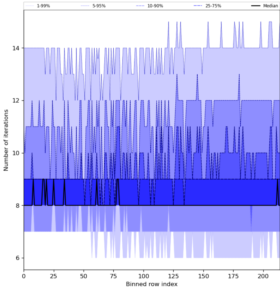
Figure 32: Along track statistics of “Number of iterations” for 2023-11-05 to 2023-11-07
