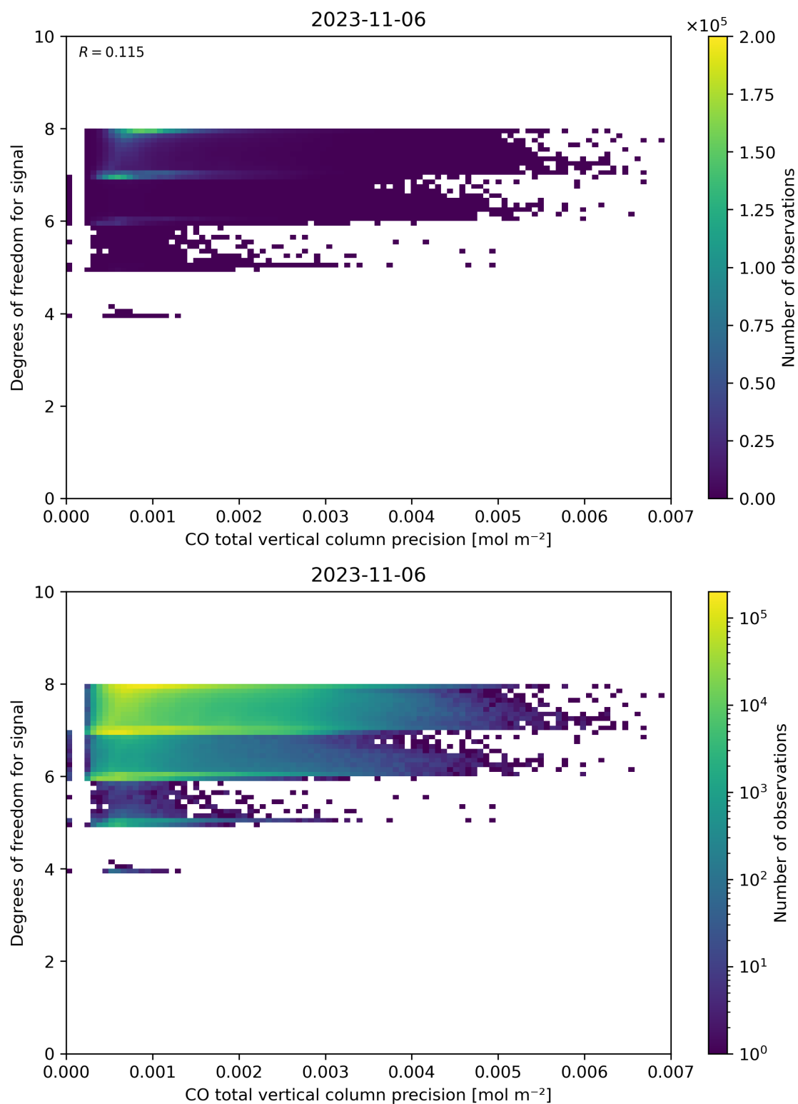
Figure 45: Scatter density plot of “CO total vertical column precision” against “Degrees of freedom for signal” for 2023-11-05 to 2023-11-07.
