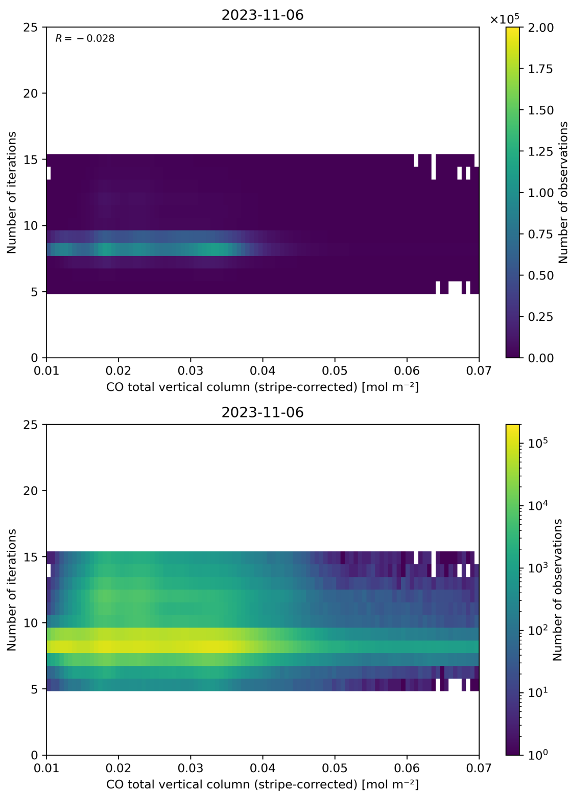
Figure 39: Scatter density plot of “CO total vertical column (stripe-corrected)” against “Number of iterations” for 2023-11-05 to 2023-11-07.
