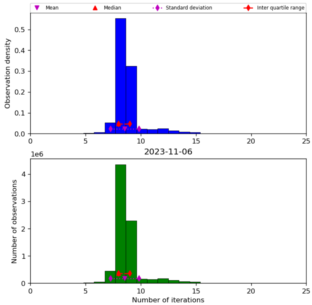
Figure 24: Histogram of “Number of iterations” for 2023-11-05 to 2023-11-07
