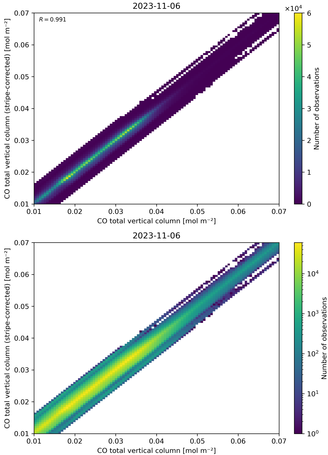
Figure 33: Scatter density plot of “CO total vertical column” against “CO total vertical column (stripe-corrected)” for 2023-11-05 to 2023-11-07.
