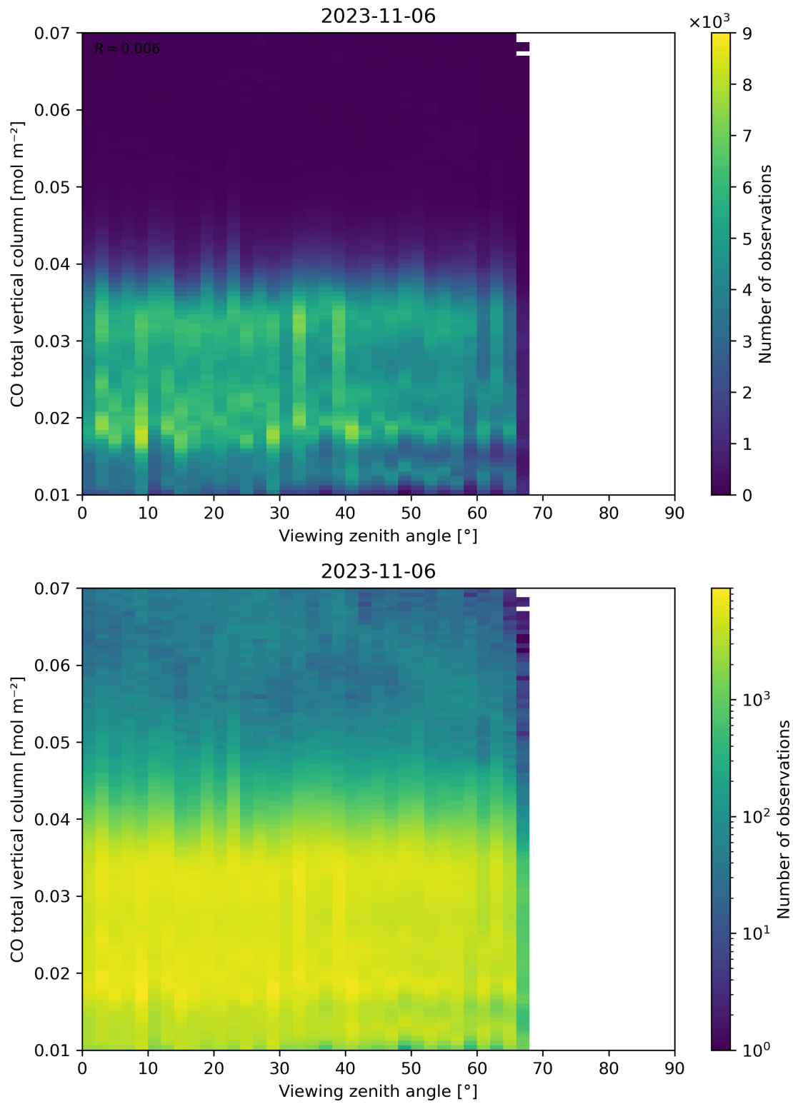
Figure 69: Scatter density plot of “Viewing zenith angle” against “CO total vertical column” for 2023-11-05 to 2023-11-07.
