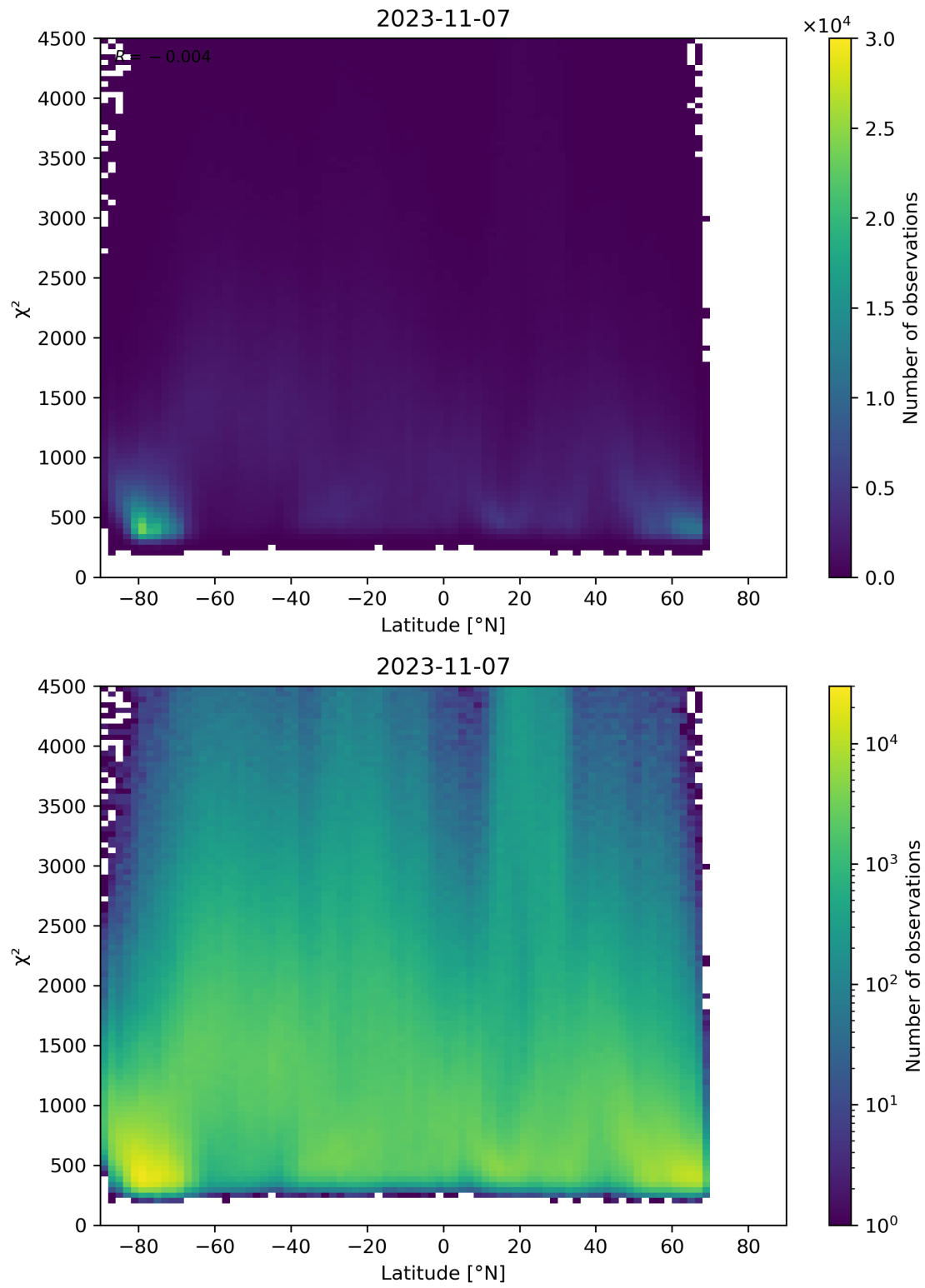
Figure 54: Scatter density plot of “Latitude” against “ \chi^2 ” for 2023-11-07 to 2023-11-08.
