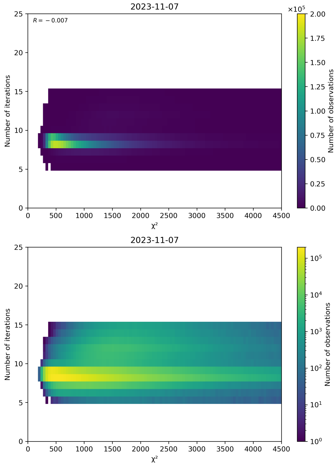
Figure 49: Scatter density plot of “ \chi^2 ” against “Number of iterations” for 2023-11-07 to 2023-11-08.
