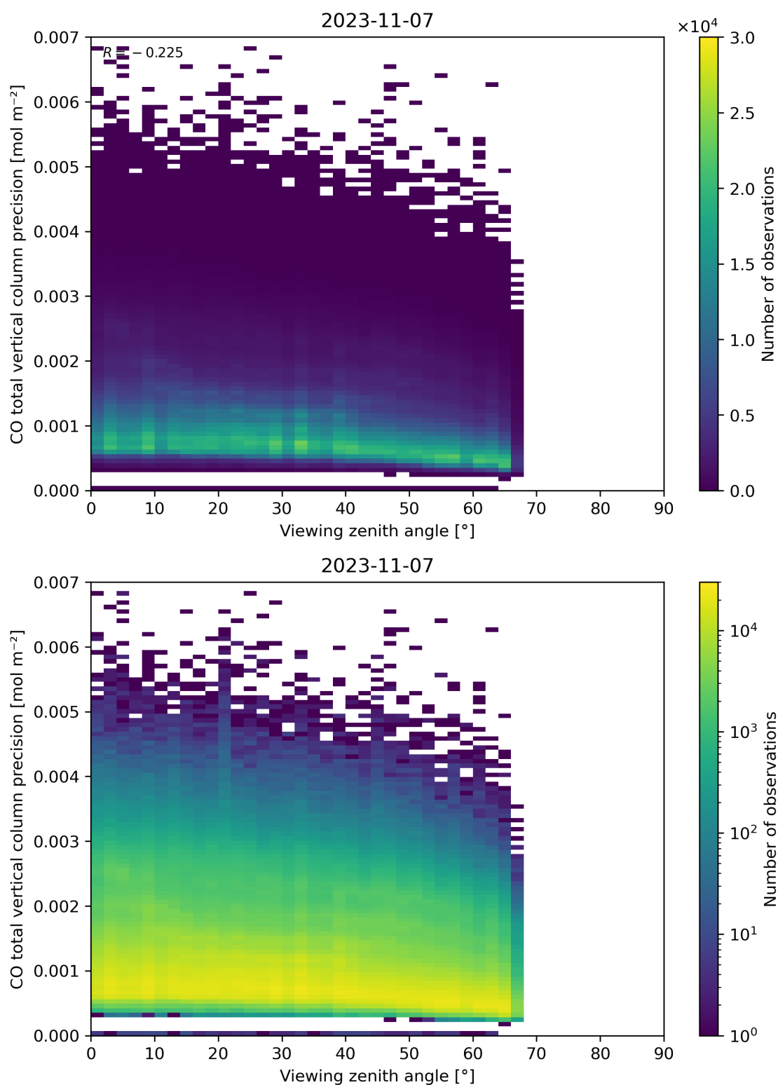
Figure 71: Scatter density plot of “Viewing zenith angle” against “CO total vertical column precision” for 2023-11-07 to 2023-11-08.
