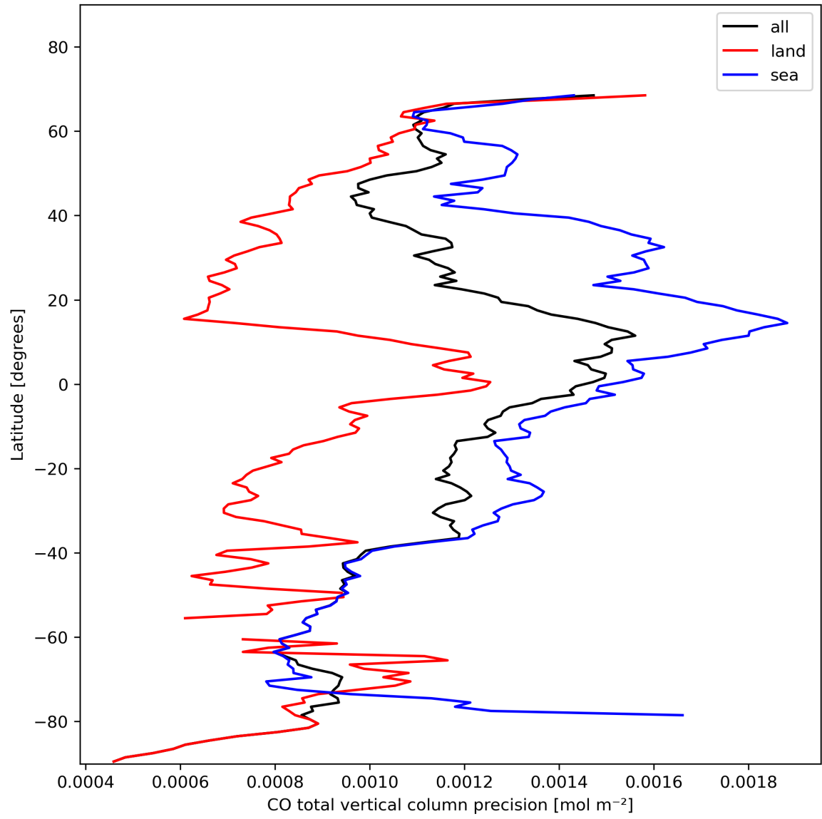
Figure 12: Zonal average of “CO total vertical column precision” for 2023-11-07 to 2023-11-08.
