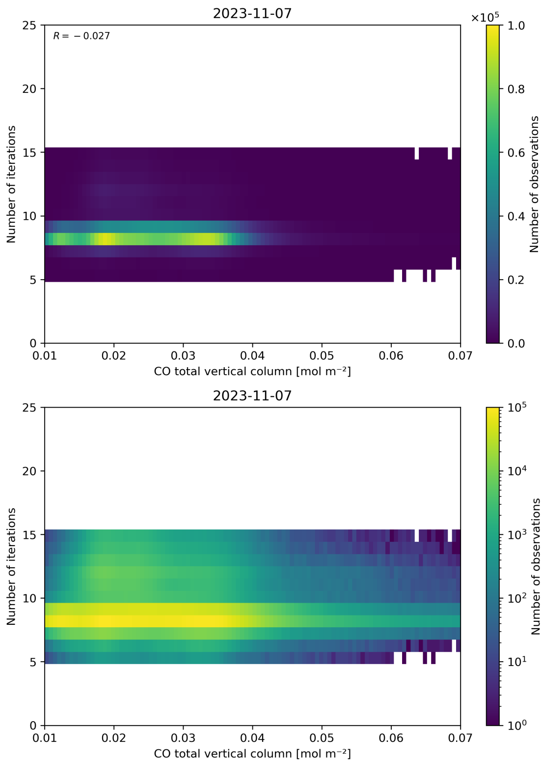
Figure 42: Scatter density plot of “CO total vertical column” against “Number of iterations” for 2023-11-07 to 2023-11-08.
