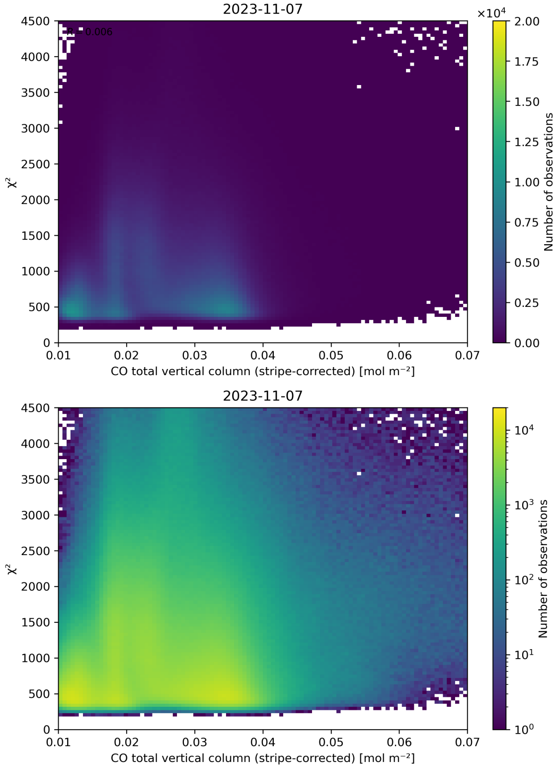
Figure 37: Scatter density plot of “CO total vertical column (stripe-corrected)” against “ \chi^2 ” for 2023-11-07 to 2023-11-08.
