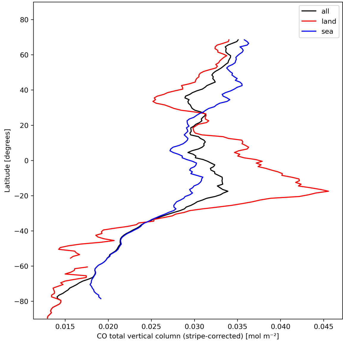
Figure 11: Zonal average of “CO total vertical column (stripe-corrected)” for 2023-11-07 to 2023-11-08.
