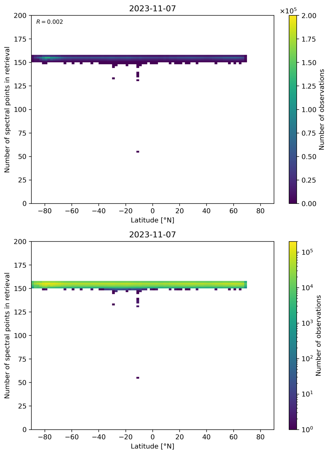
Figure 57: Scatter density plot of “Latitude” against “Number of spectral points in retrieval” for 2023-11-07 to 2023-11-08.
