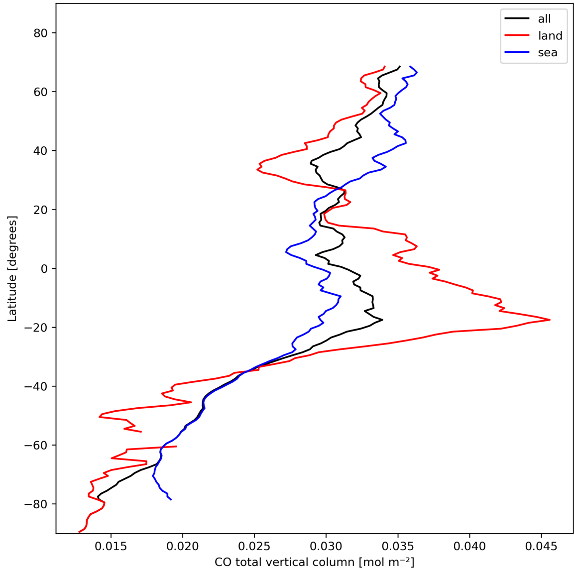
Figure 10: Zonal average of “CO total vertical column” for 2023-11-07 to 2023-11-08.
