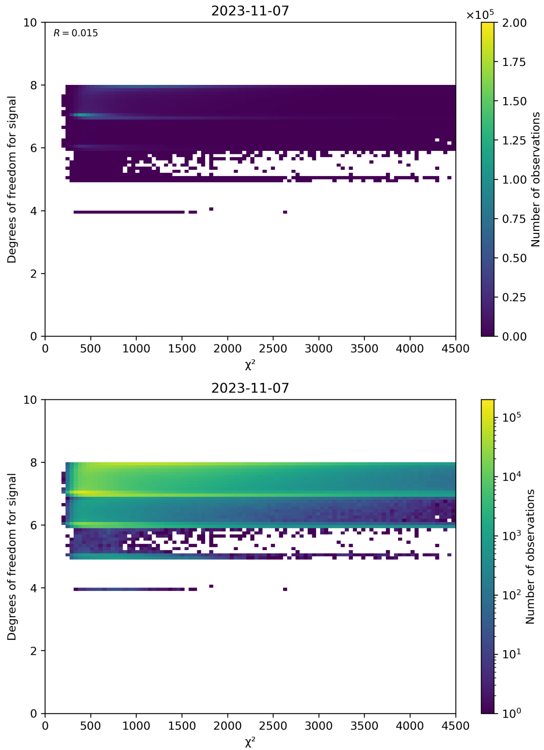
Figure 48: Scatter density plot of " \chi^2 " against "Degrees of freedom for signal" for 2023-11-07 to 2023-11-08.
