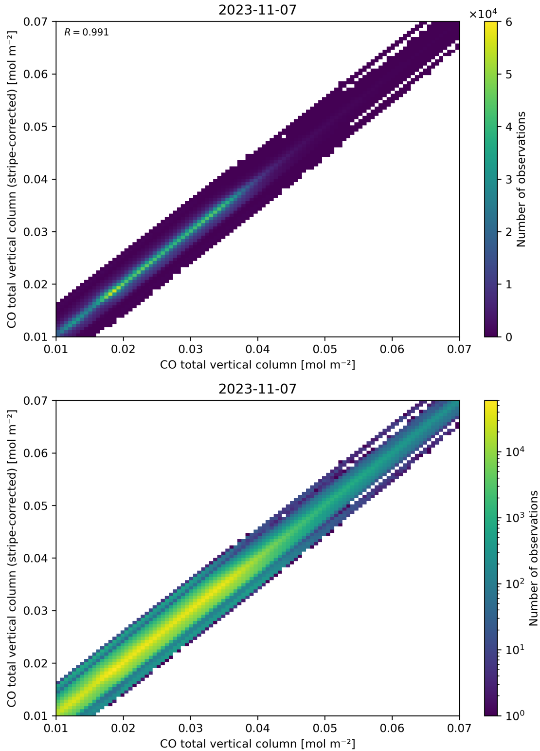
Figure 33: Scatter density plot of “CO total vertical column” against “CO total vertical column (stripe-corrected)” for 2023-11-07 to 2023-11-08.
