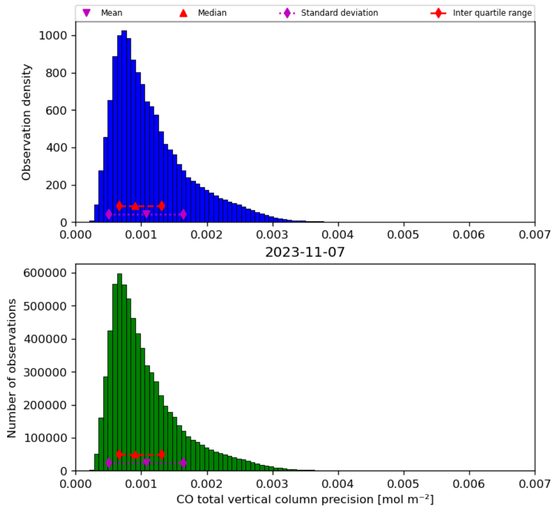
Figure 20: Histogram of “CO total vertical column precision” for 2023-11-07 to 2023-11-08
