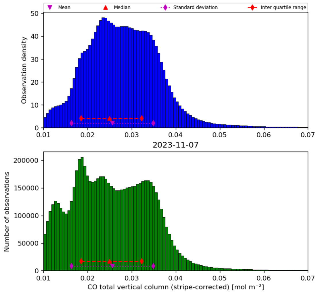
Figure 19: Histogram of “CO total vertical column (stripe-corrected)” for 2023-11-07 to 2023-11-08
