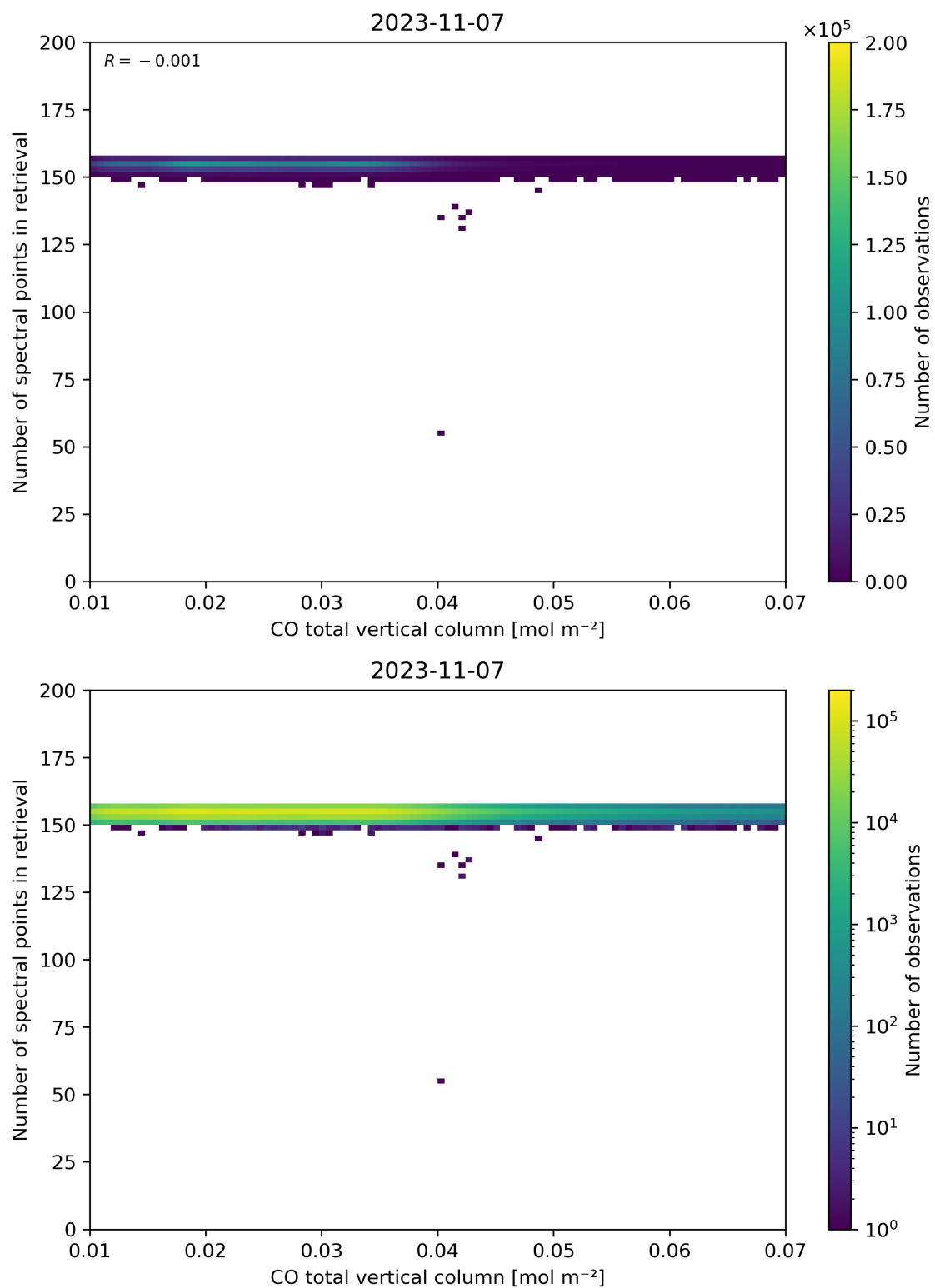
Figure 43: Scatter density plot of “CO total vertical column” against “Number of spectral points in retrieval” for 2023-11-07 to 2023-11-08.
