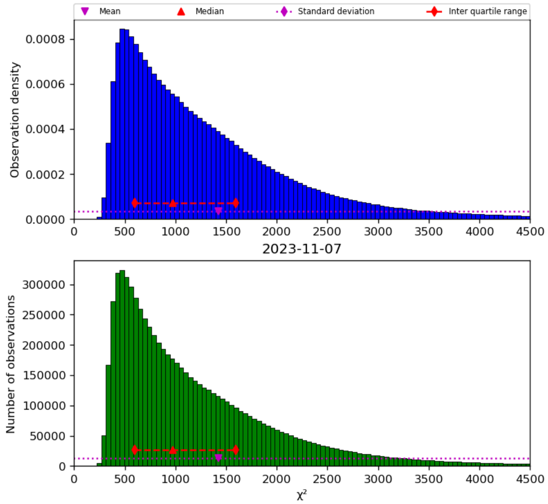
Figure 22: Histogram of “ \chi^2 ” for 2023-11-07 to 2023-11-08
