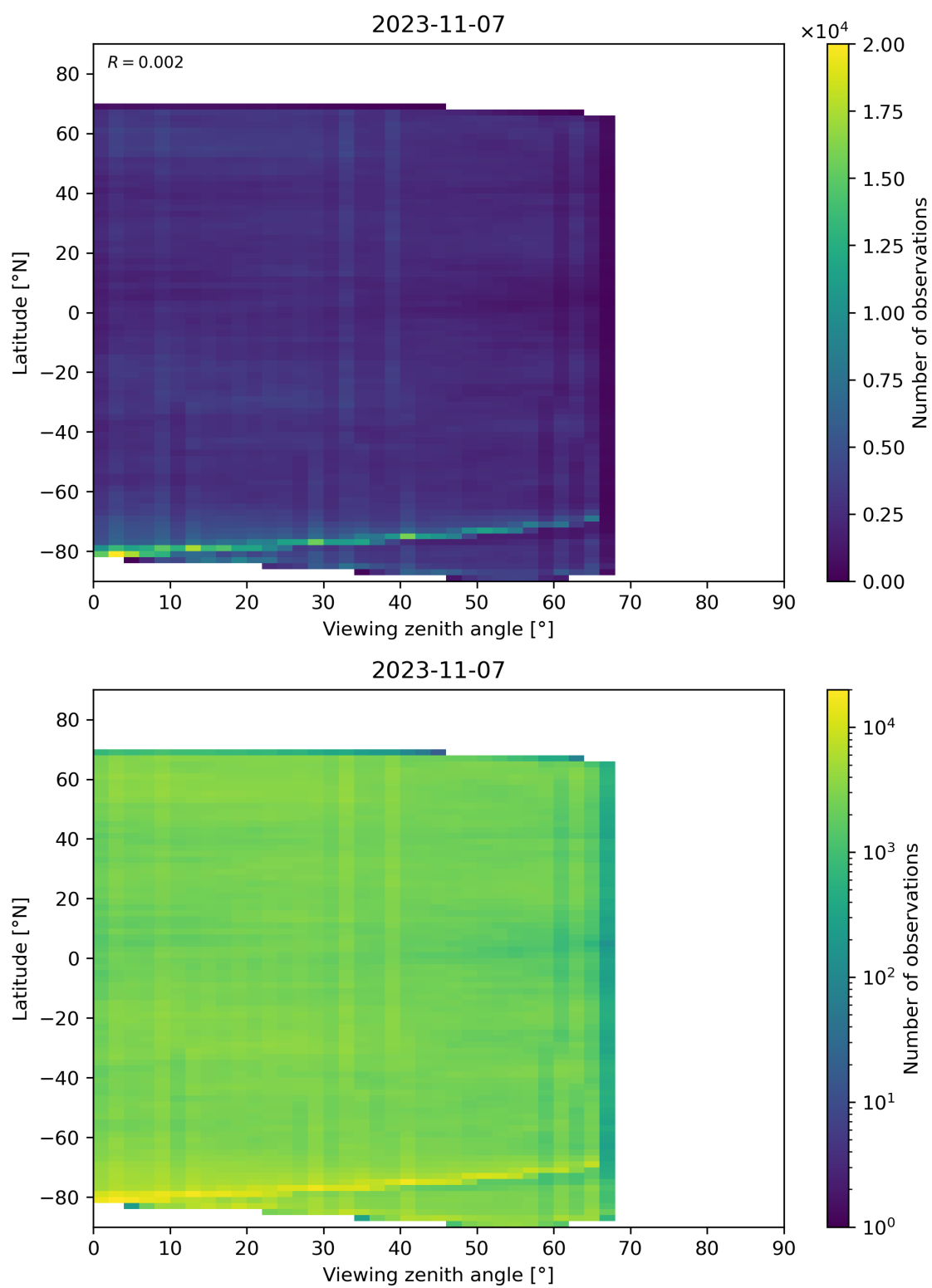
Figure 74: Scatter density plot of “Viewing zenith angle” against “Latitude” for 2023-11-07 to 2023-11-08.
