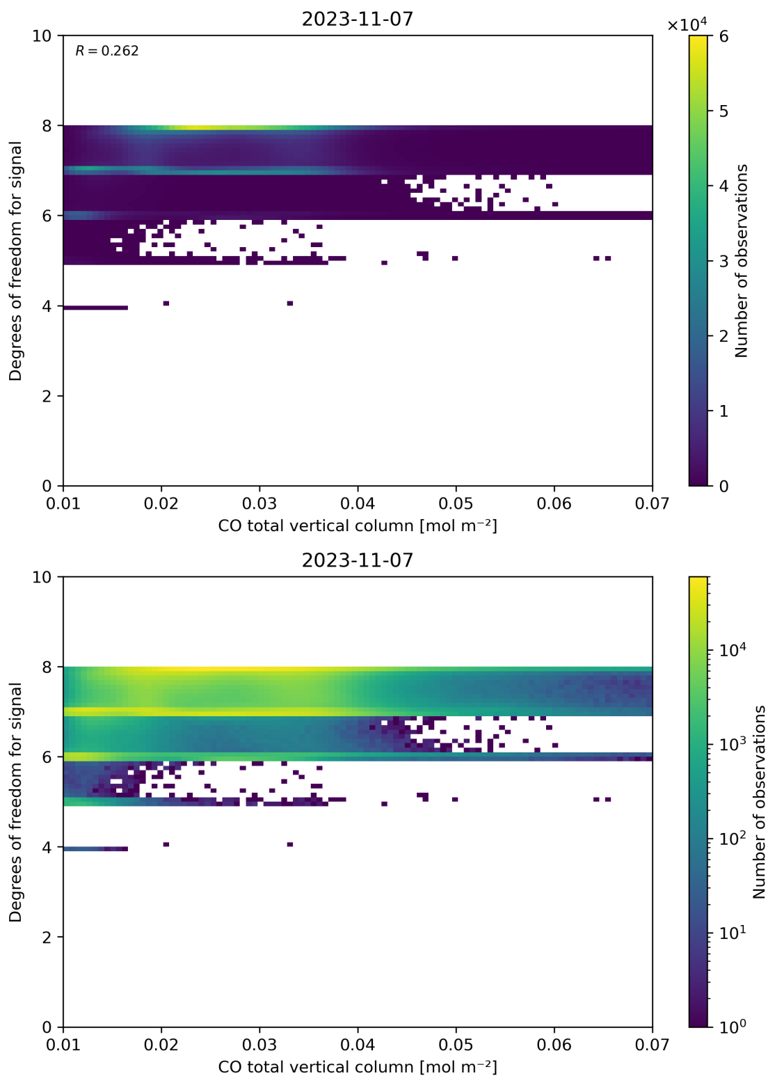
Figure 41: Scatter density plot of “CO total vertical column” against “Degrees of freedom for signal” for 2023-11-07 to 2023-11-08.
