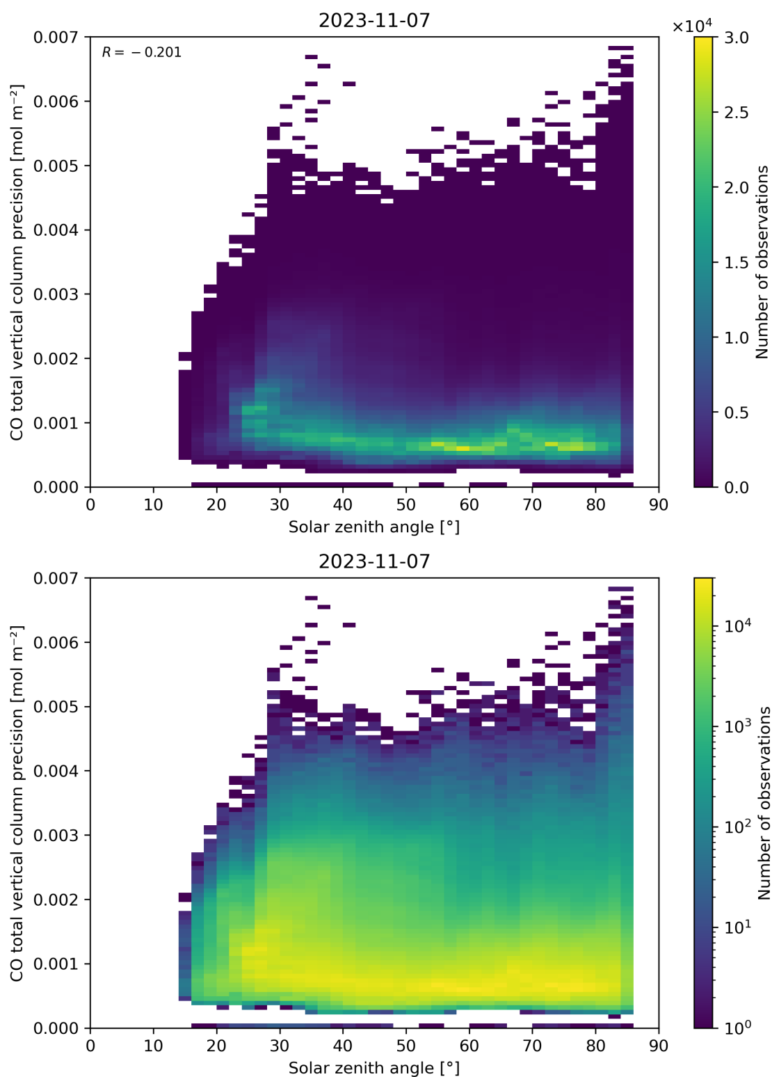
Figure 63: Scatter density plot of “Solar zenith angle” against “CO total vertical column precision” for 2023-11-07 to 2023-11-08.
