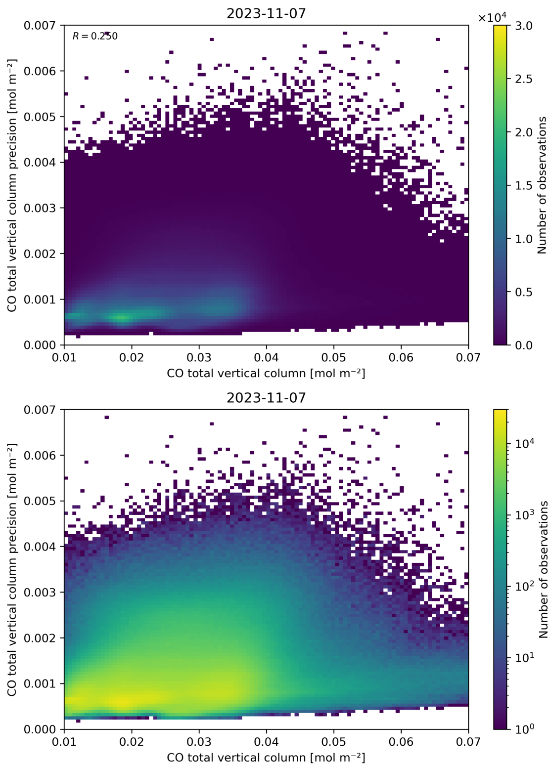
Figure 34: Scatter density plot of “CO total vertical column” against “CO total vertical column precision” for 2023-11-07 to 2023-11-08.
