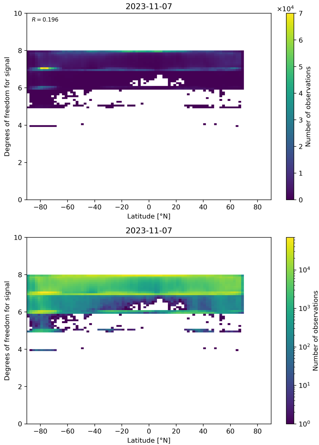
Figure 55: Scatter density plot of “Latitude” against “Degrees of freedom for signal” for 2023-11-07 to 2023-11-08.
