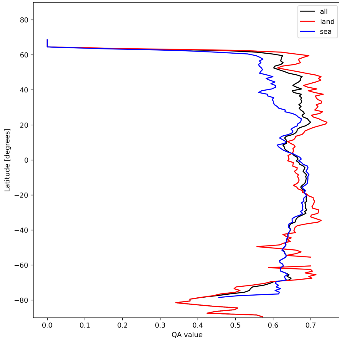
Figure 9: Zonal average of “QA value” for 2023-11-07 to 2023-11-08.
