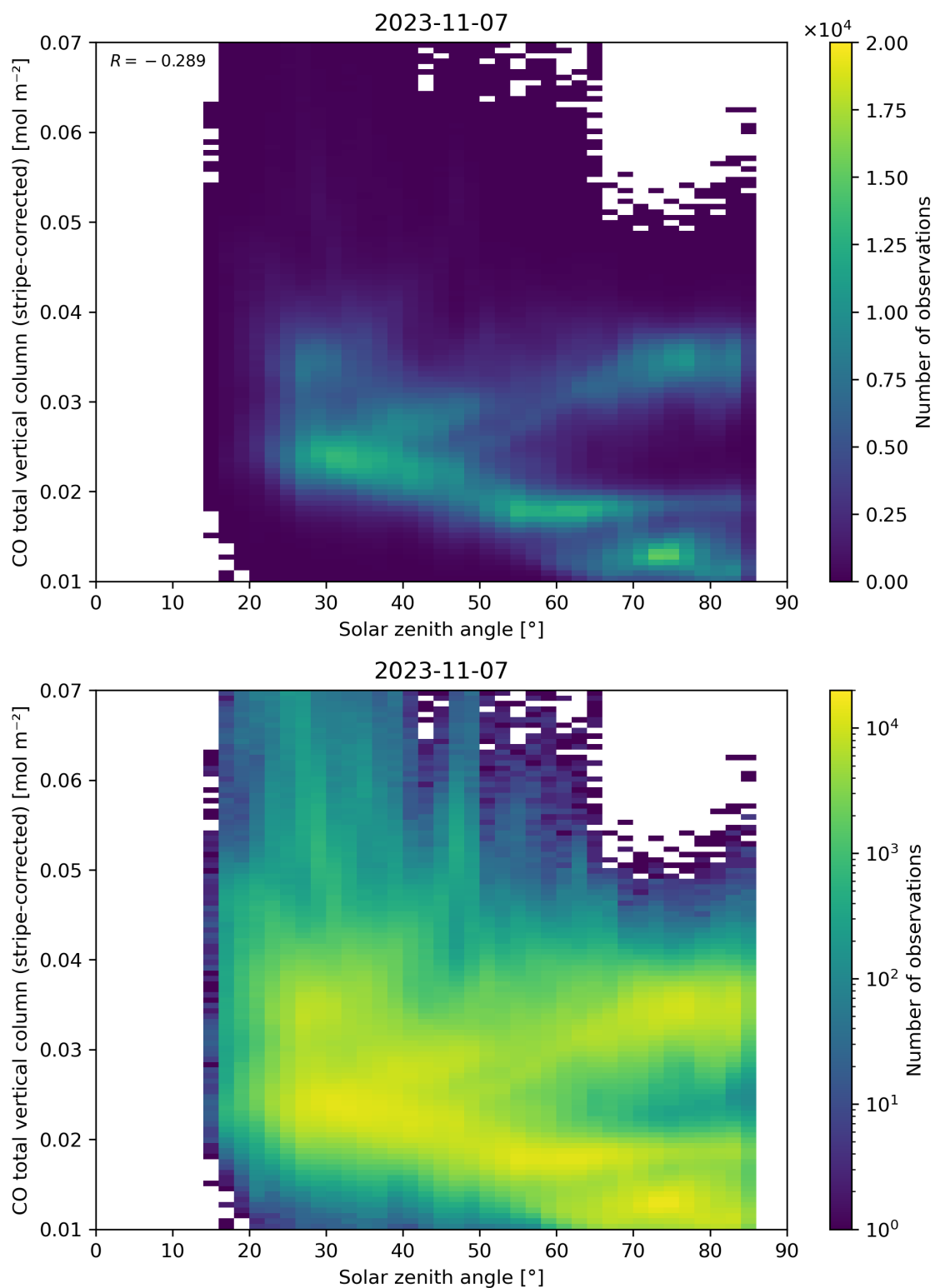
Figure 62: Scatter density plot of “Solar zenith angle” against “CO total vertical column (stripe-corrected)” for 2023-11-07 to 2023-11-08.
