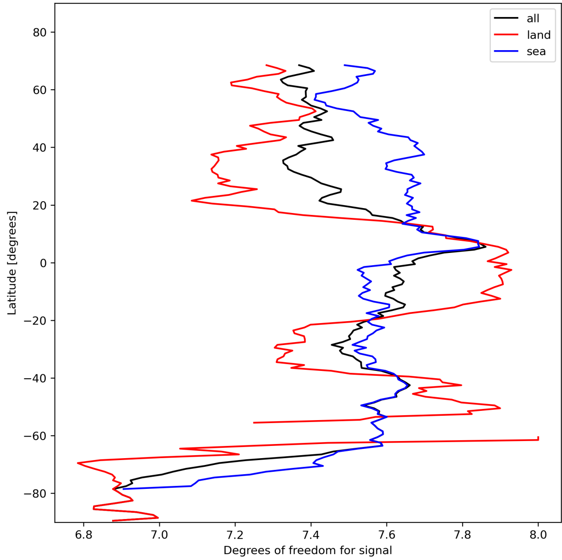
Figure 15: Zonal average of “Degrees of freedom for signal” for 2023-11-07 to 2023-11-08.
