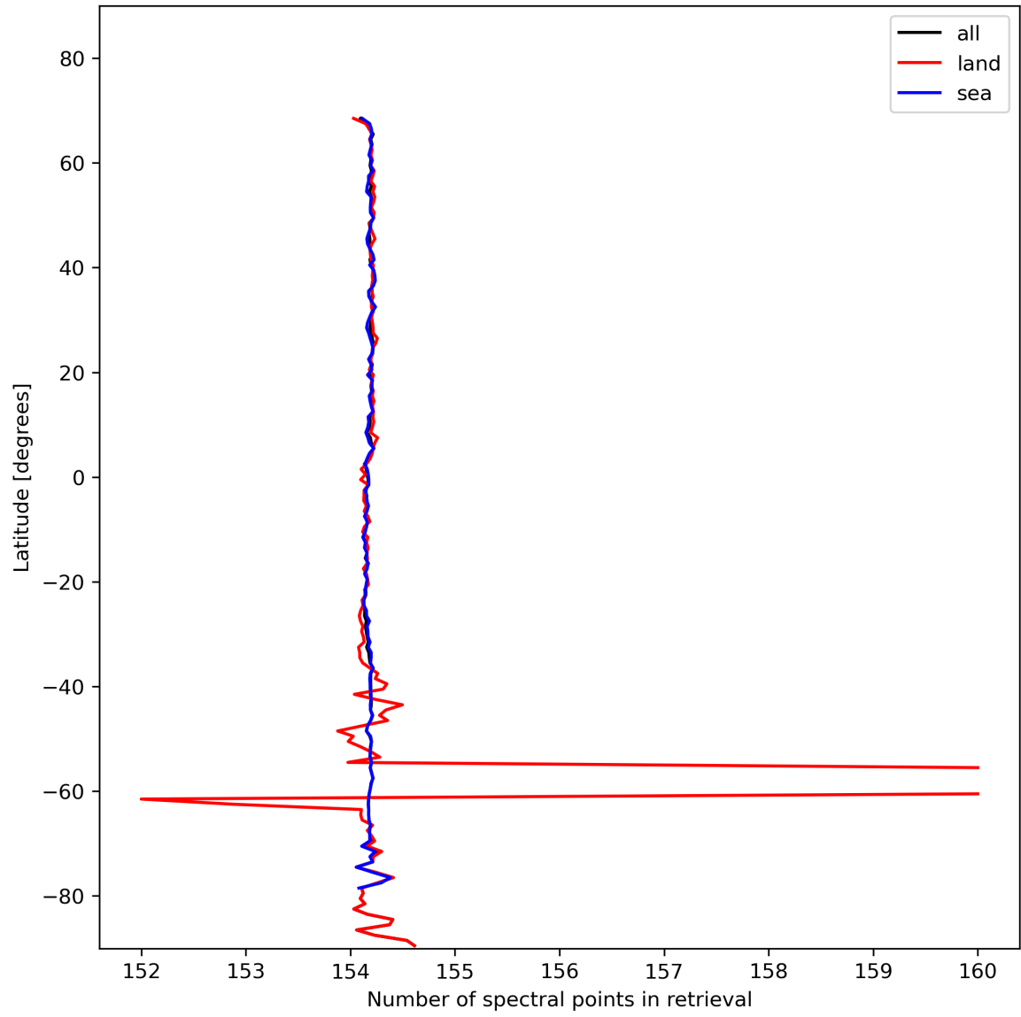
Figure 13: Zonal average of “Number of spectral points in retrieval” for 2023-11-07 to 2023-11-08.
