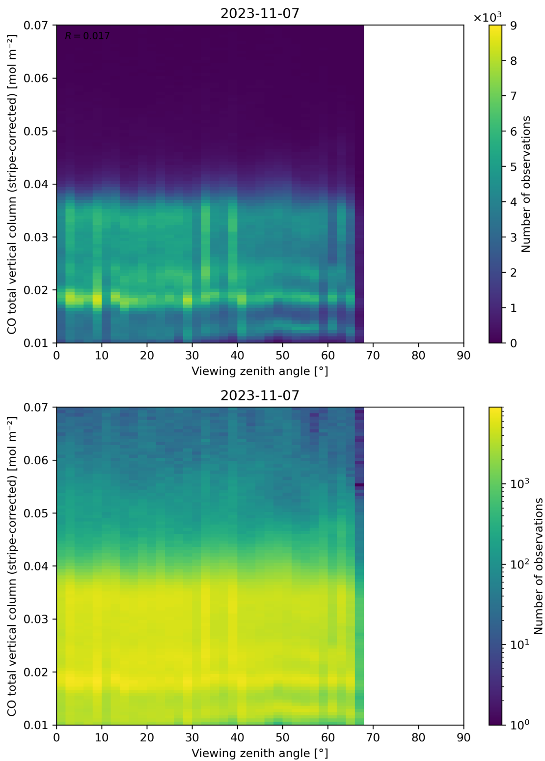
Figure 70: Scatter density plot of “Viewing zenith angle” against “CO total vertical column (stripe-corrected)” for 2023-11-07 to 2023-11-08.
