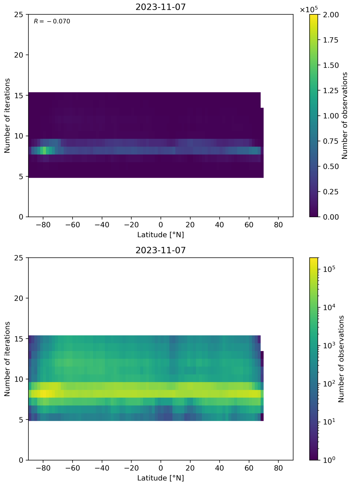
Figure 56: Scatter density plot of “Latitude” against “Number of iterations” for 2023-11-07 to 2023-11-08.
