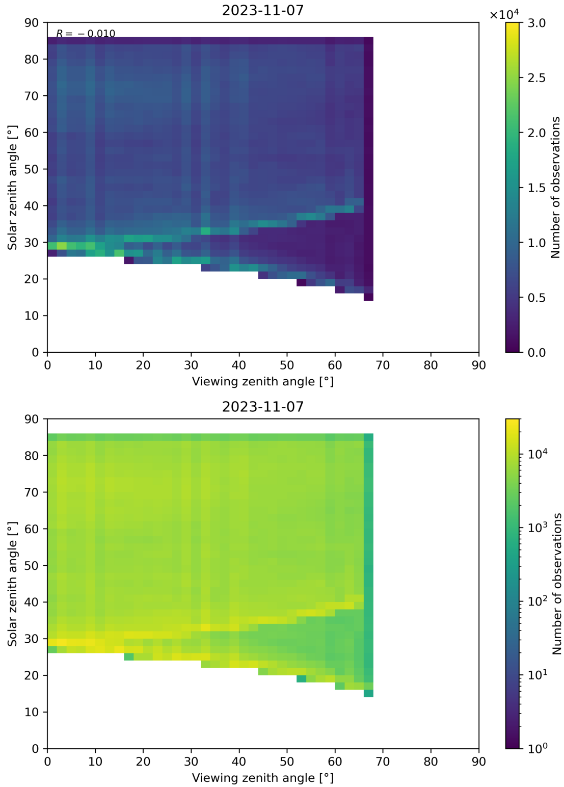
Figure 77: Scatter density plot of “Viewing zenith angle” against “Solar zenith angle” for 2023-11-07 to 2023-11-08.
