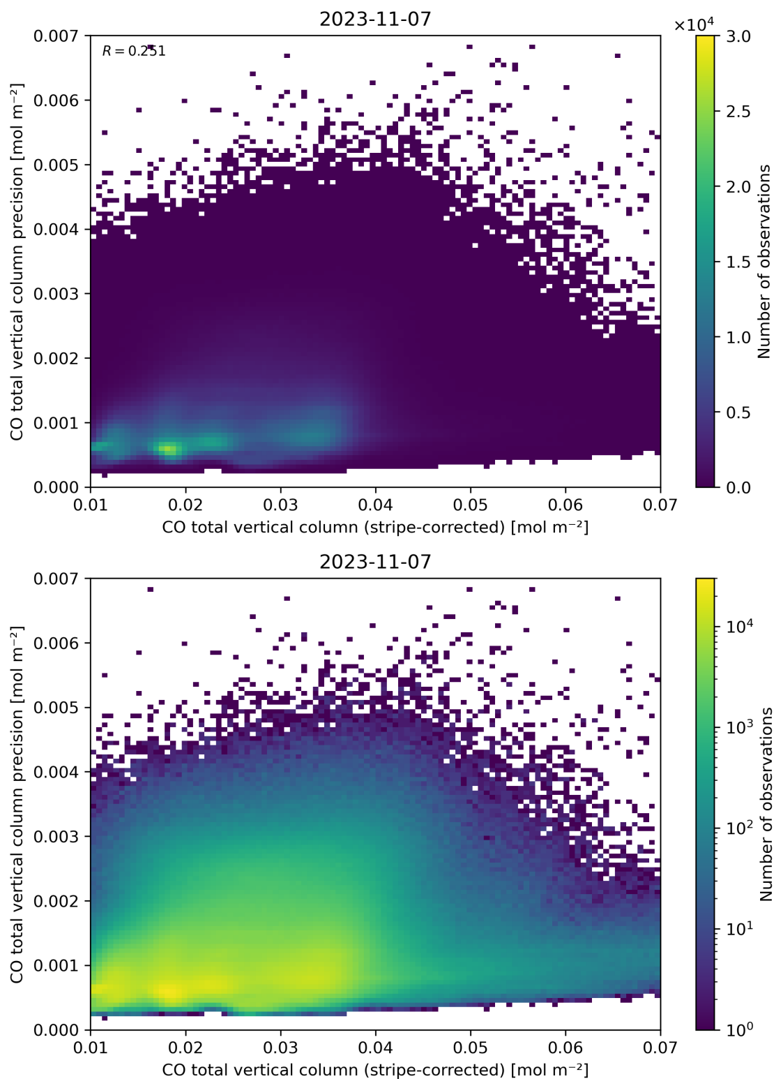
Figure 36: Scatter density plot of “CO total vertical column (stripe-corrected)” against “CO total vertical column precision” for 2023-11-07 to 2023-11-08.
