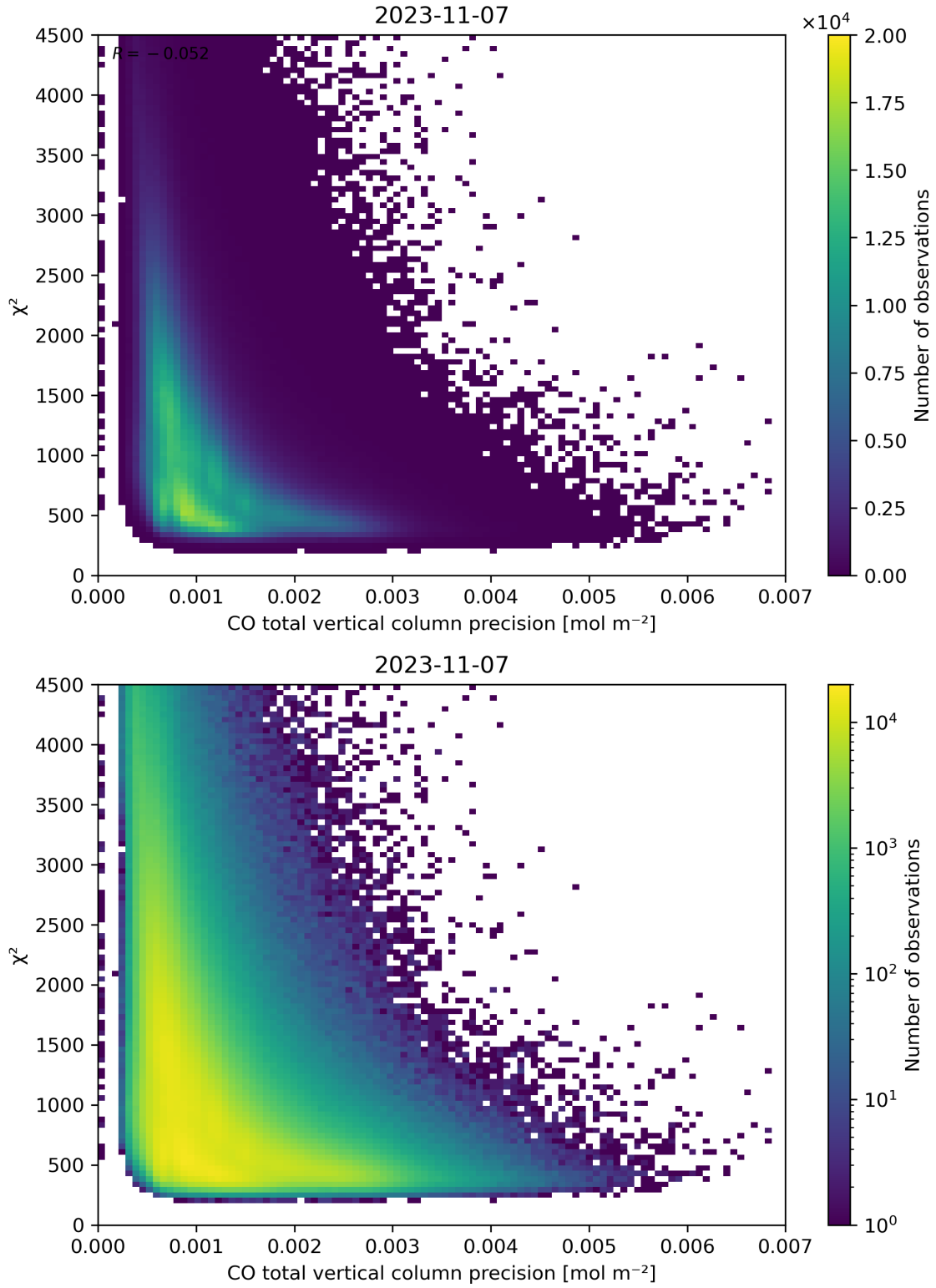
Figure 44: Scatter density plot of “CO total vertical column precision” against “ \chi^2 ” for 2023-11-07 to 2023-11-08.
