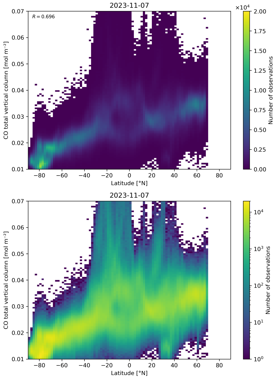
Figure 51: Scatter density plot of “Latitude” against “CO total vertical column” for 2023-11-07 to 2023-11-08.
