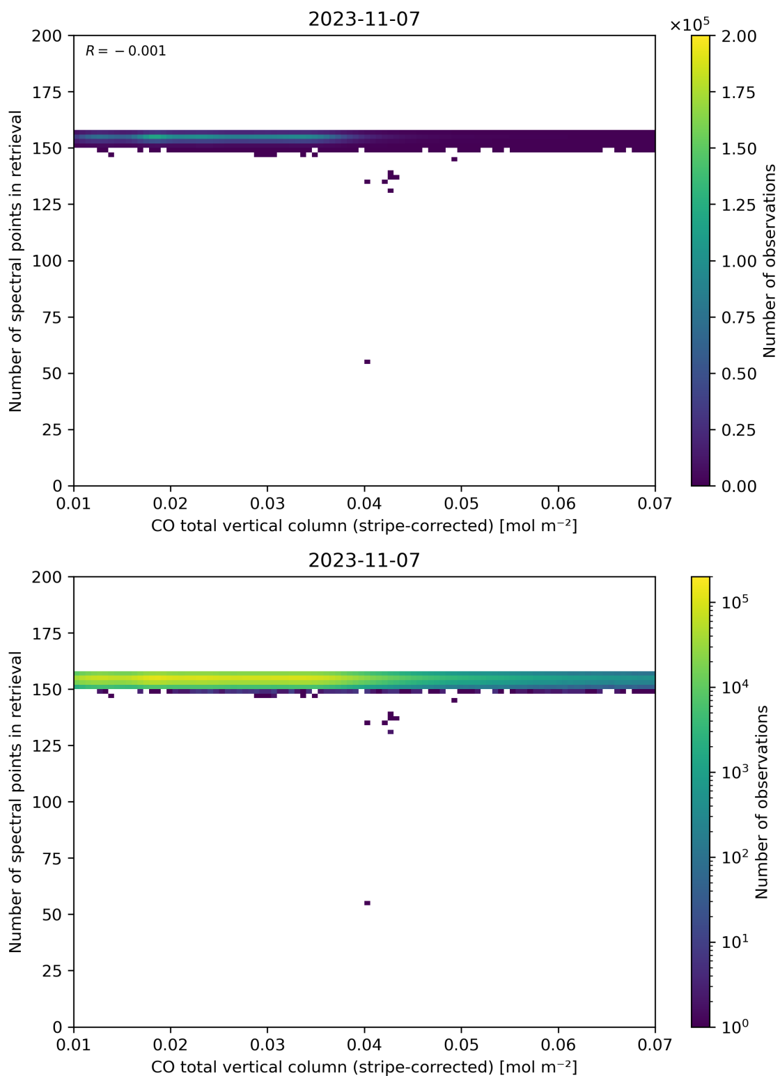
Figure 40: Scatter density plot of “CO total vertical column (stripe-corrected)” against “Number of spectral points in retrieval” for 2023-11-07 to 2023-11-08.
