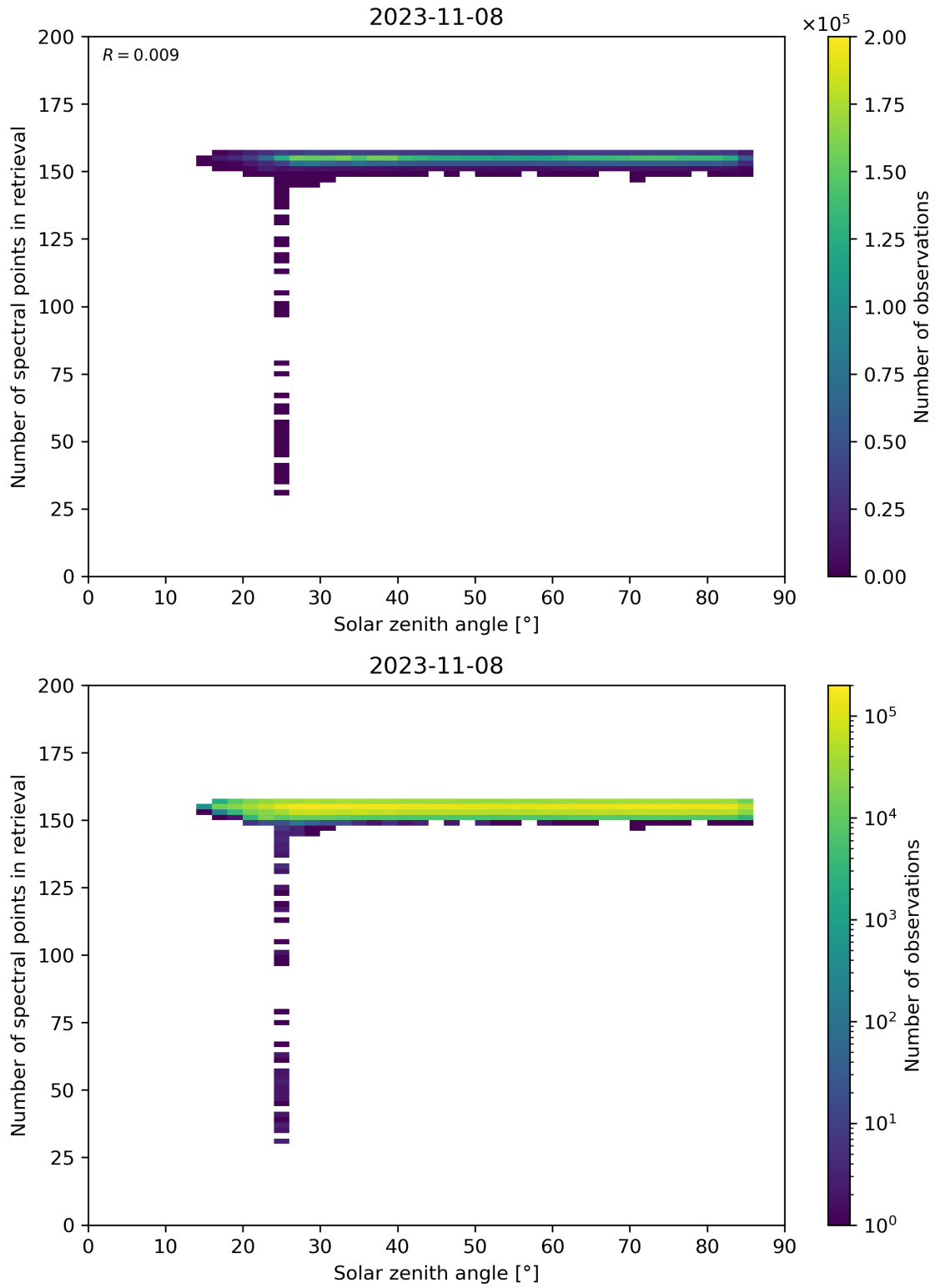
Figure 68: Scatter density plot of “Solar zenith angle” against “Number of spectral points in retrieval” for 2023-11-07 to 2023-11-09.
