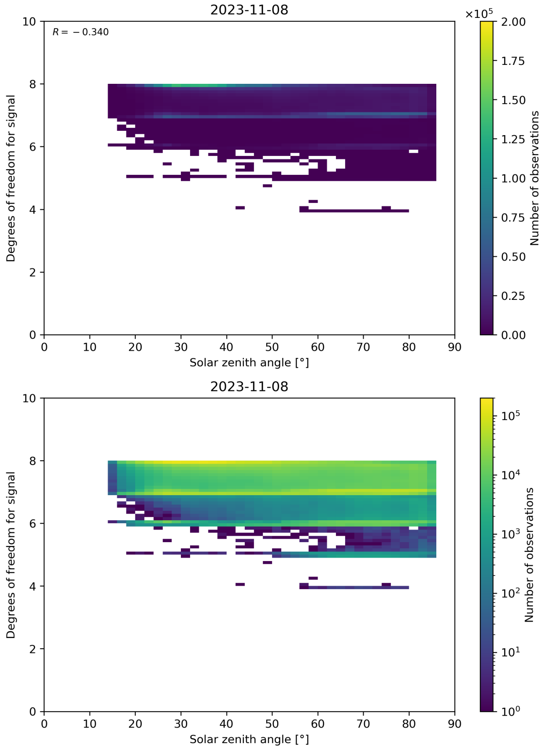
Figure 65: Scatter density plot of “Solar zenith angle” against “Degrees of freedom for signal” for 2023-11-07 to 2023-11-09.
