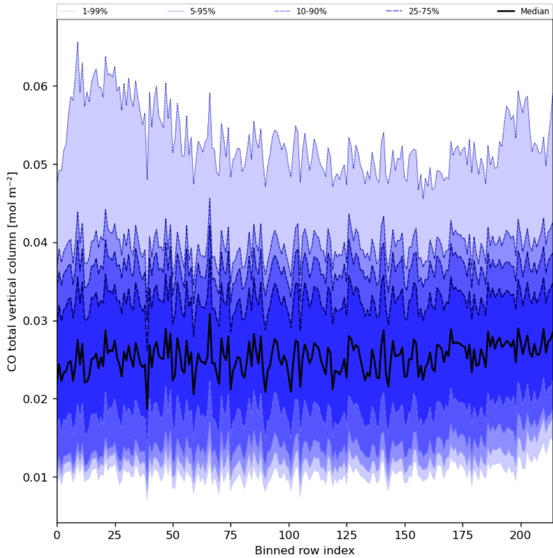
Figure 26: Along track statistics of “CO total vertical column” for 2023-11-07 to 2023-11-09
