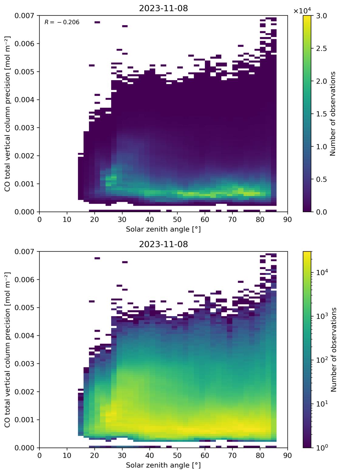
Figure 63: Scatter density plot of “Solar zenith angle” against “CO total vertical column precision” for 2023-11-07 to 2023-11-09.
