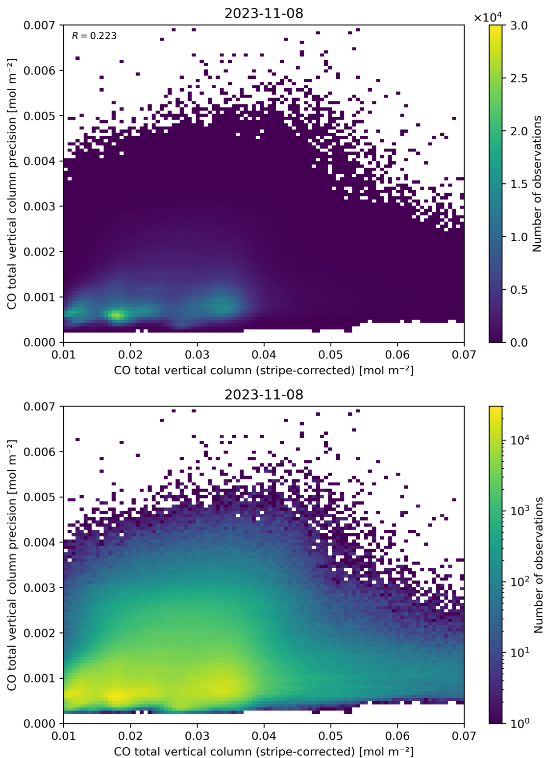
Figure 36: Scatter density plot of “CO total vertical column (stripe-corrected)” against “CO total vertical column precision” for 2023-11-07 to 2023-11-09.
