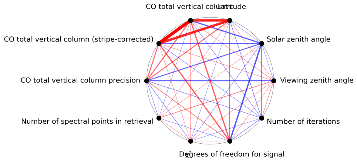
Figure 1: Map of correlation graph for 2023-11-07 to 2023-11-09.
