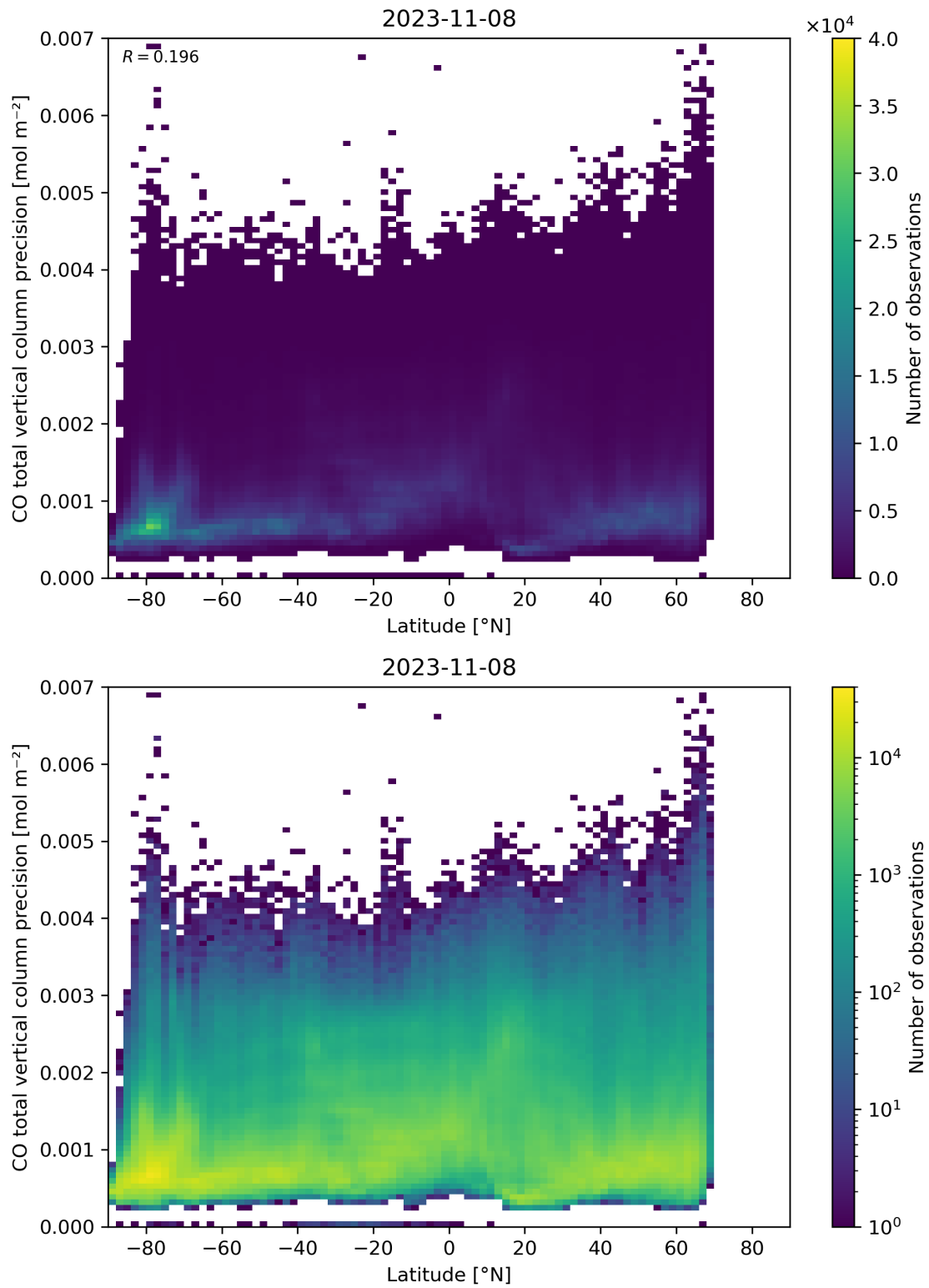
Figure 53: Scatter density plot of “Latitude” against “CO total vertical column precision” for 2023-11-07 to 2023-11-09.
