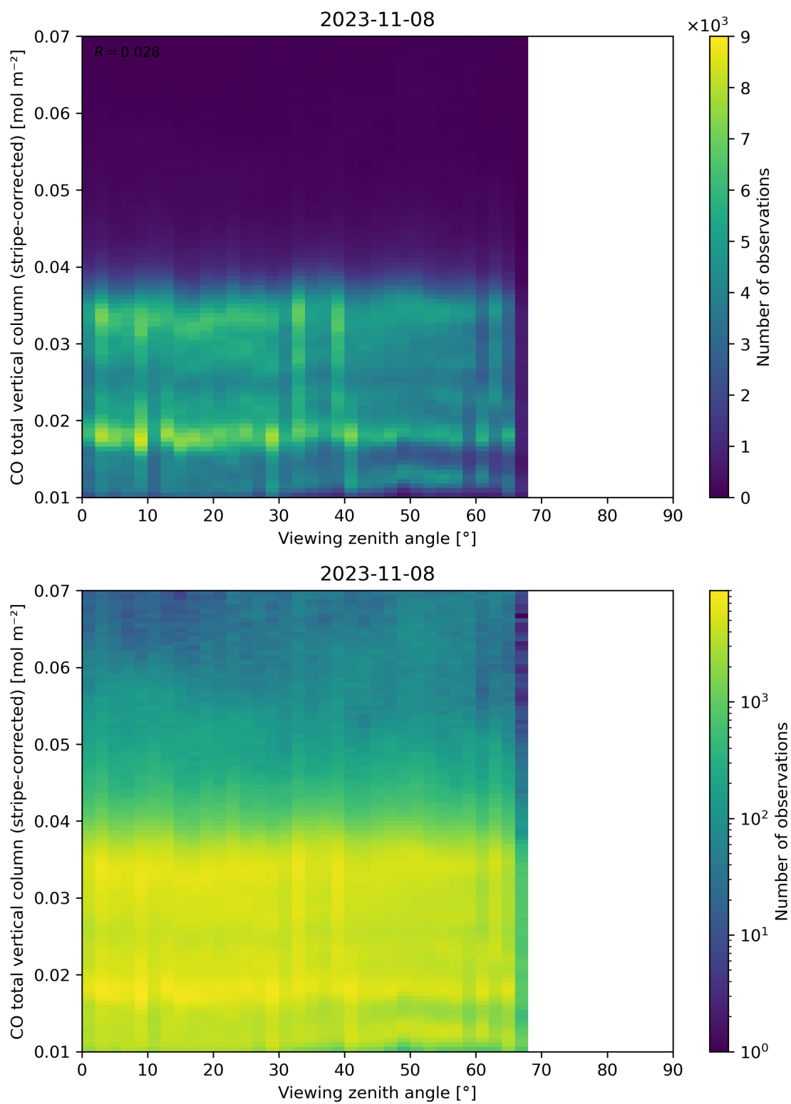
Figure 70: Scatter density plot of “Viewing zenith angle” against “CO total vertical column (stripe-corrected)” for 2023-11-07 to 2023-11-09.
