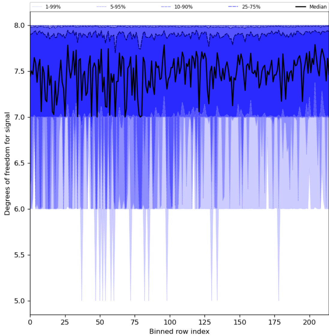
Figure 31: Along track statistics of “Degrees of freedom for signal” for 2023-11-07 to 2023-11-09
