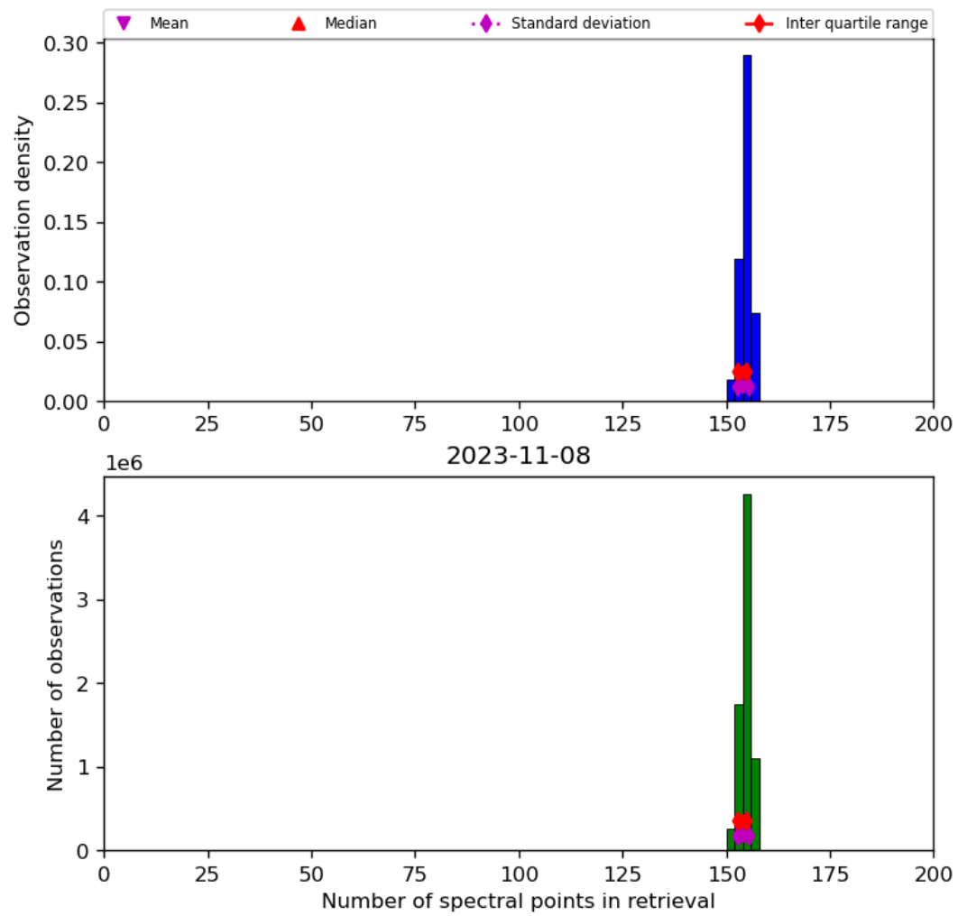
Figure 21: Histogram of “Number of spectral points in retrieval” for 2023-11-07 to 2023-11-09
