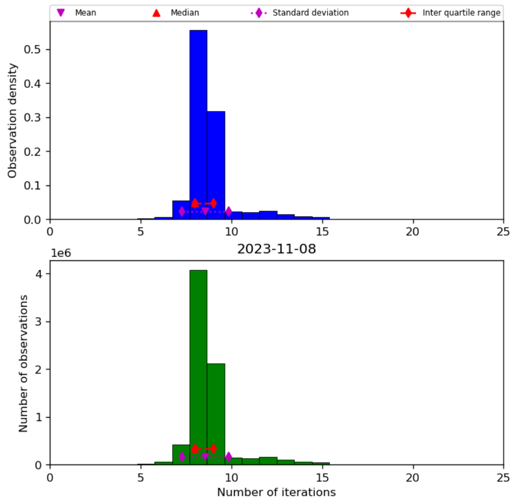
Figure 24: Histogram of “Number of iterations” for 2023-11-07 to 2023-11-09
