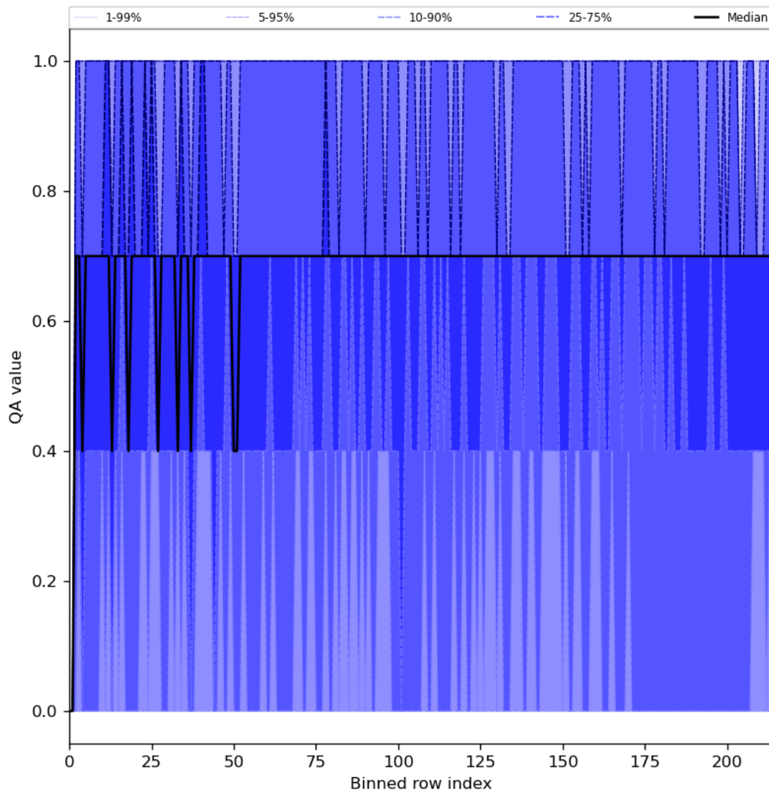
Figure 25: Along track statistics of “QA value” for 2023-11-07 to 2023-11-09
