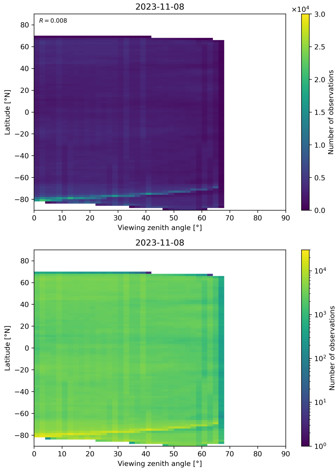
Figure 74: Scatter density plot of “Viewing zenith angle” against “Latitude” for 2023-11-07 to 2023-11-09.
