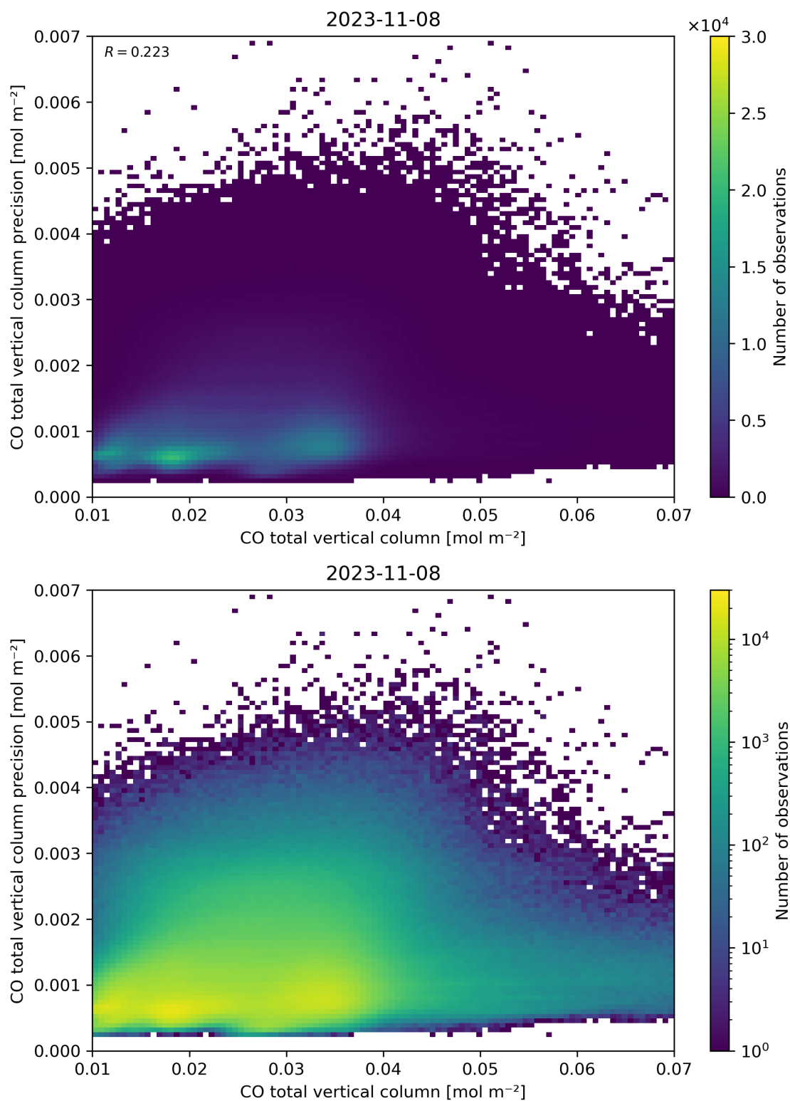
Figure 34: Scatter density plot of “CO total vertical column” against “CO total vertical column precision” for 2023-11-07 to 2023-11-09.
