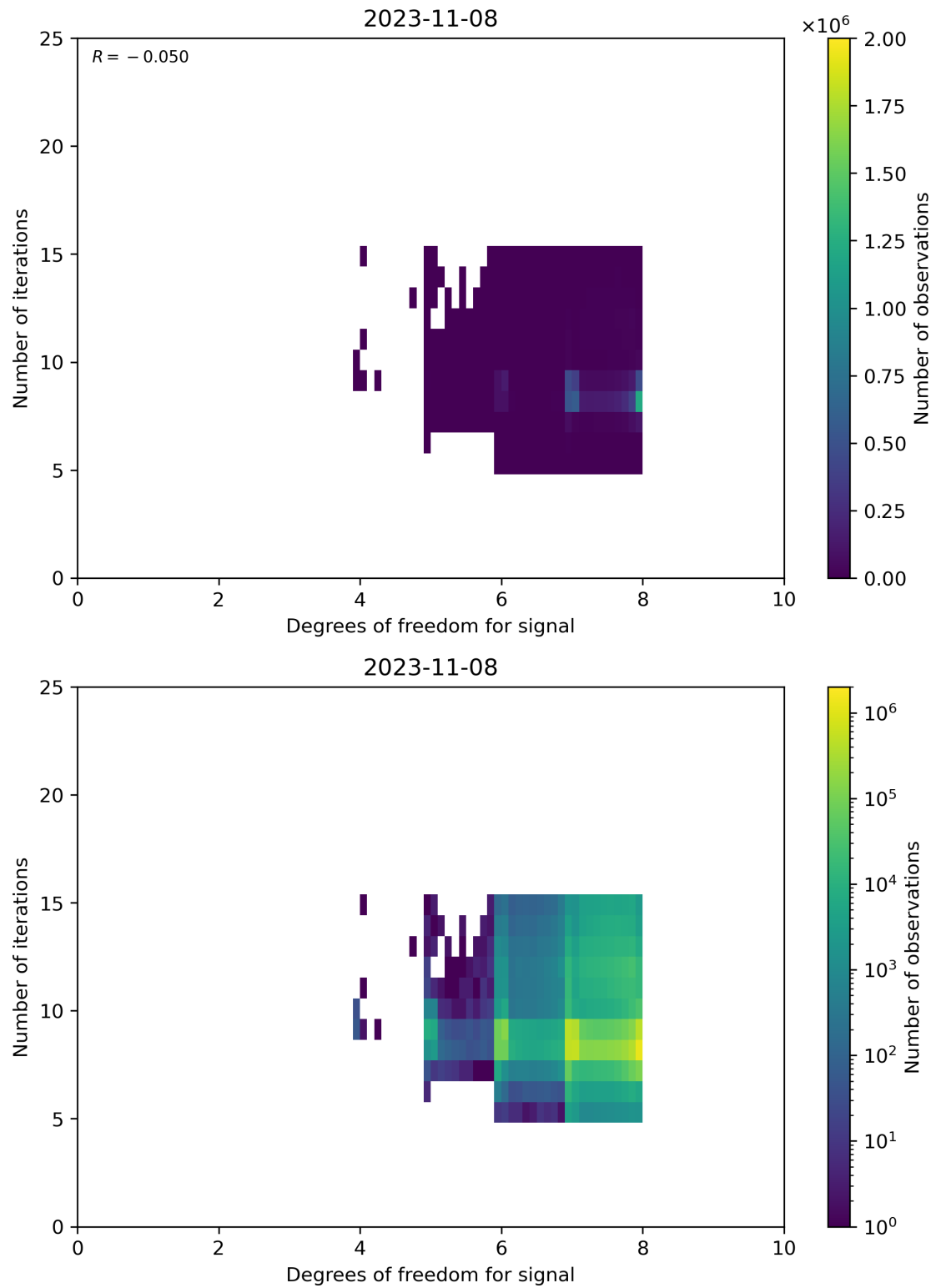
Figure 50: Scatter density plot of “Degrees of freedom for signal” against “Number of iterations” for 2023-11-07 to 2023-11-09.
