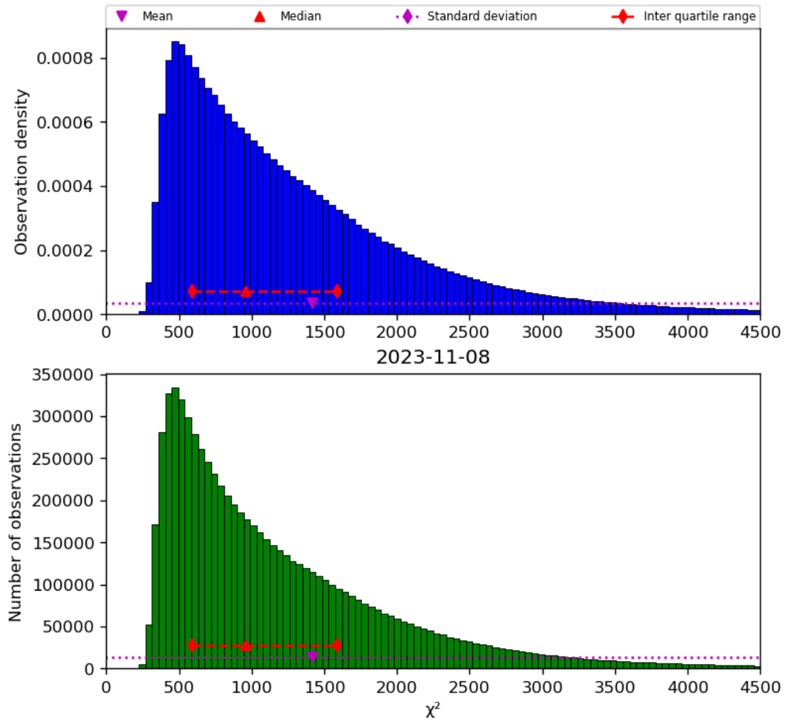
Figure 22: Histogram of “ \chi^2 ” for 2023-11-07 to 2023-11-09
