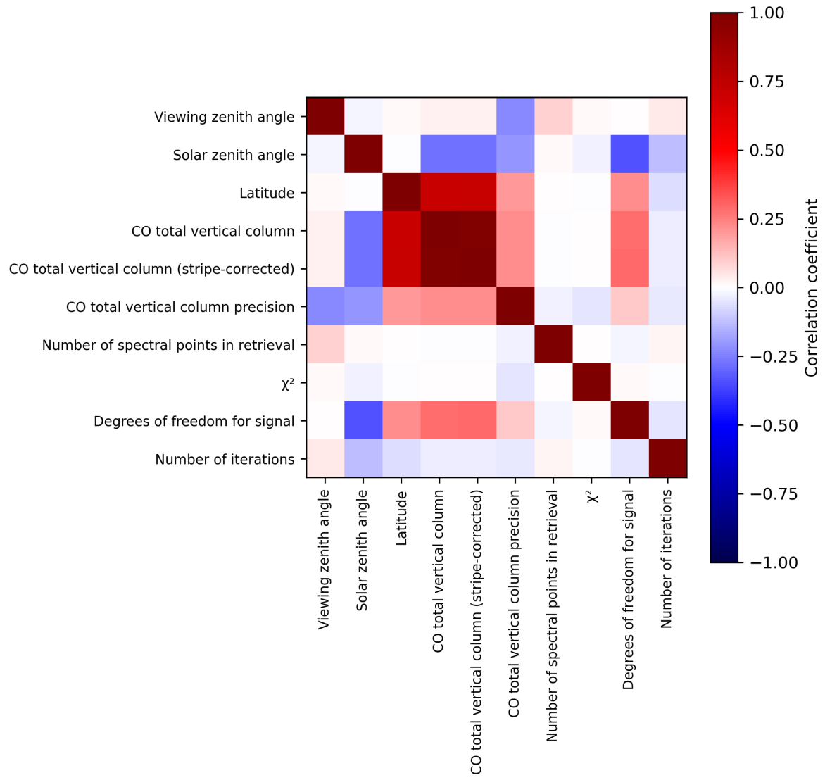
Figure 2: Map of correlation matrix for 2023-11-07 to 2023-11-09.
