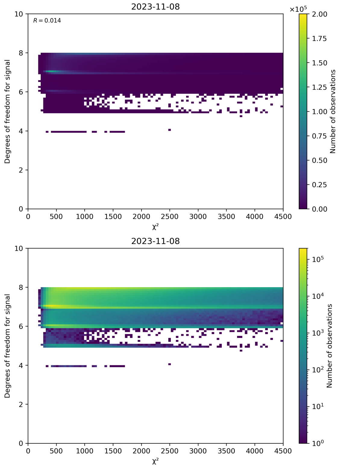
Figure 48: Scatter density plot of “ \chi^2 ” against “Degrees of freedom for signal” for 2023-11-07 to 2023-11-09.
