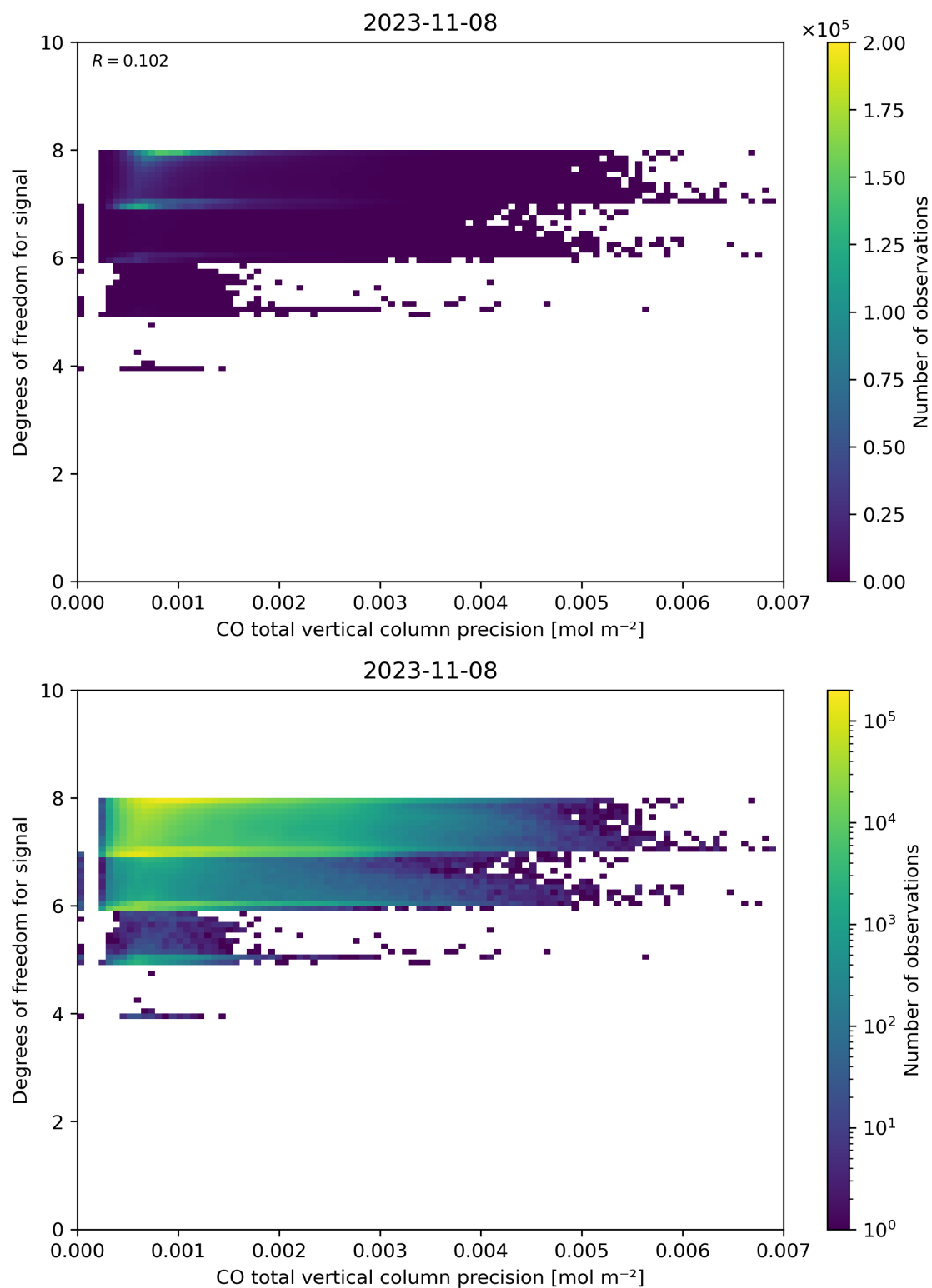
Figure 45: Scatter density plot of “CO total vertical column precision” against “Degrees of freedom for signal” for 2023-11-07 to 2023-11-09.
