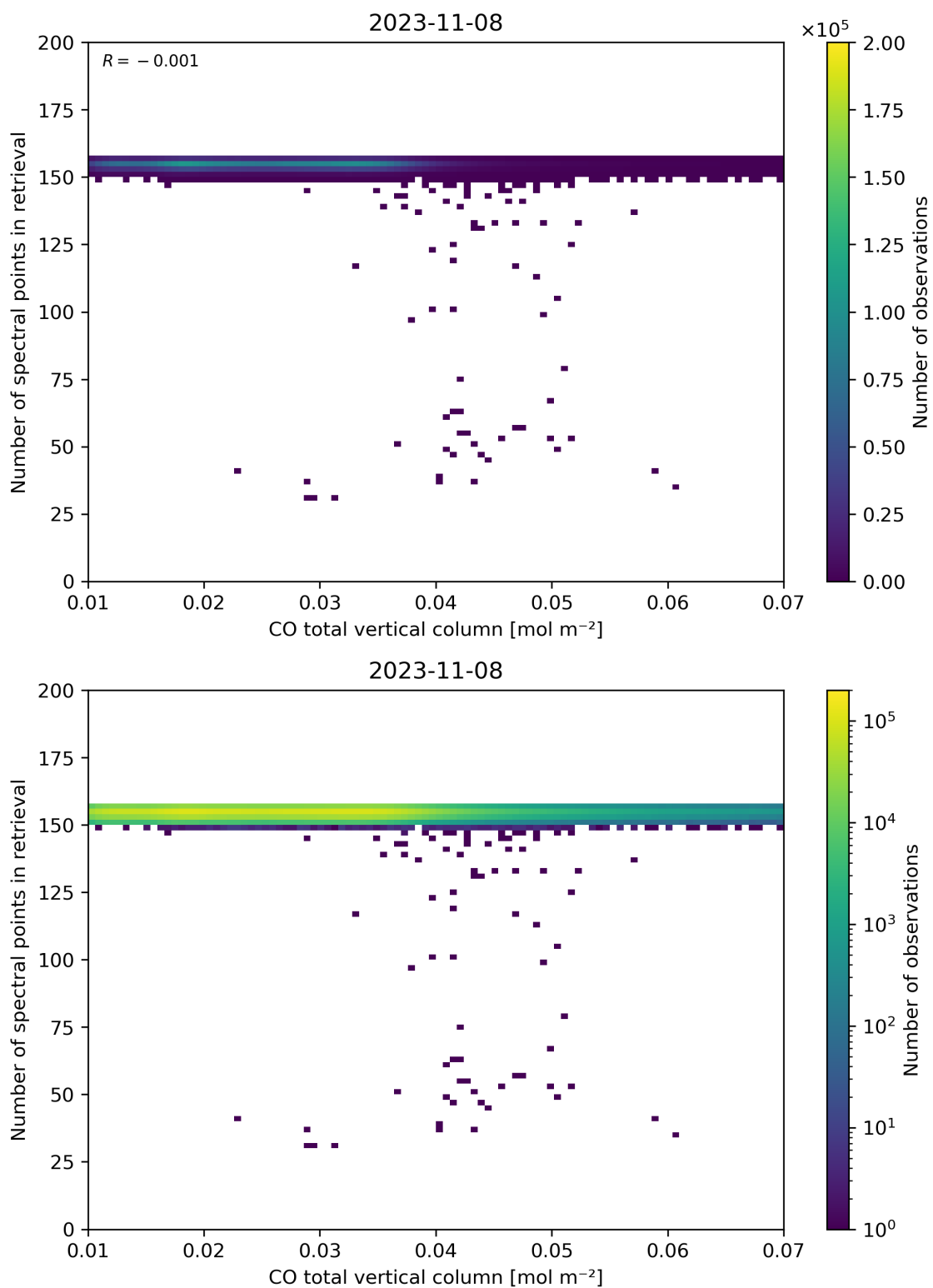
Figure 43: Scatter density plot of “CO total vertical column” against “Number of spectral points in retrieval” for 2023-11-07 to 2023-11-09.
