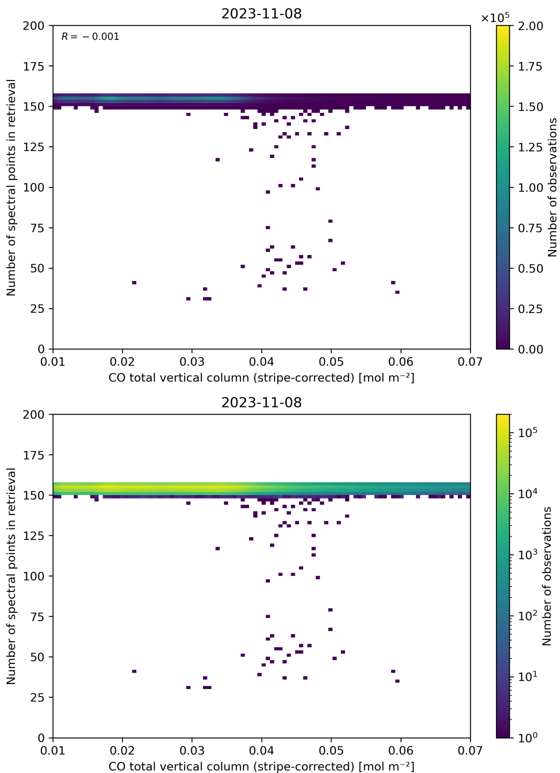
Figure 40: Scatter density plot of “CO total vertical column (stripe-corrected)” against “Number of spectral points in retrieval” for 2023-11-07 to 2023-11-09.
