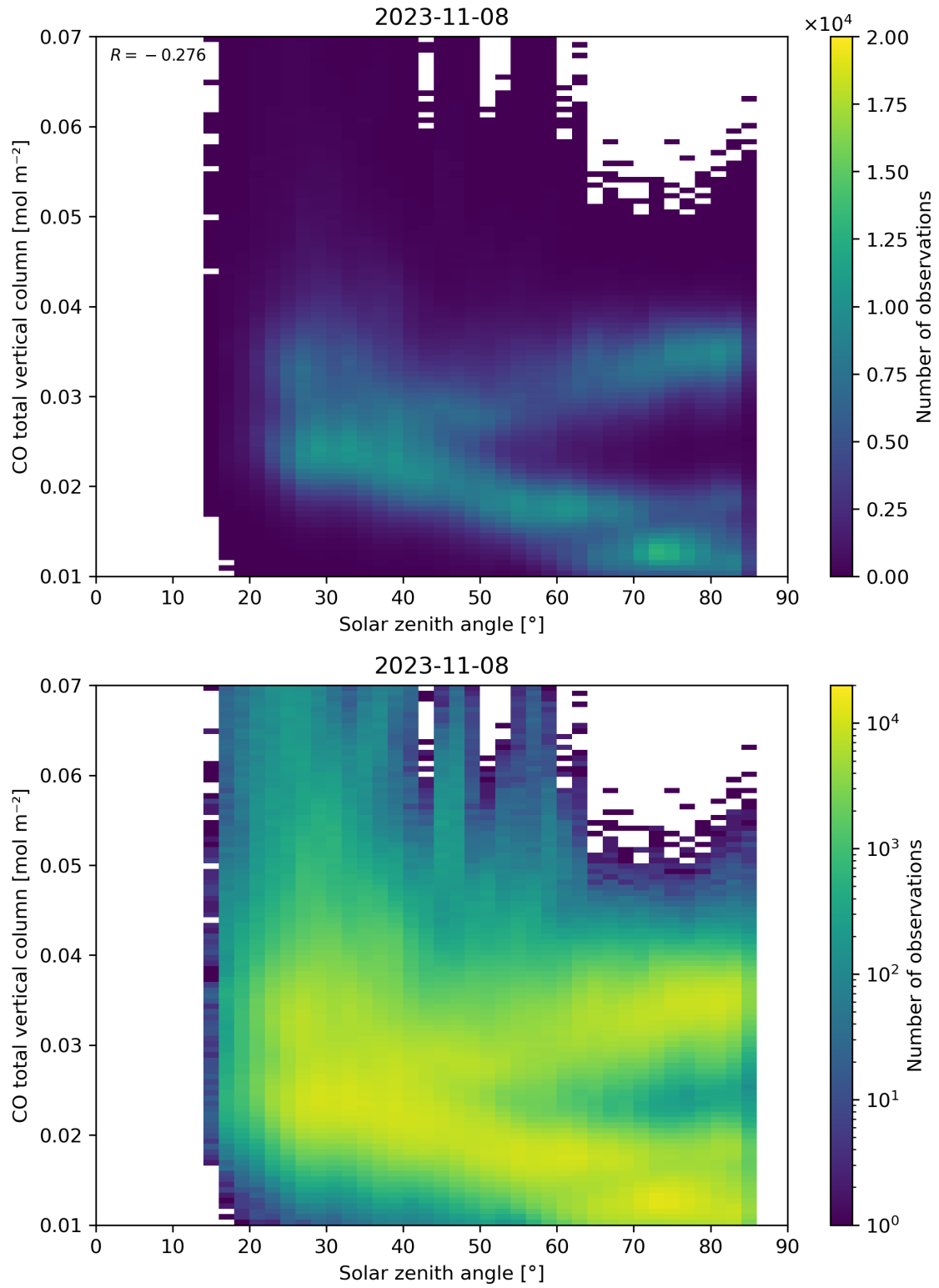
Figure 61: Scatter density plot of “Solar zenith angle” against “CO total vertical column” for 2023-11-07 to 2023-11-09.
