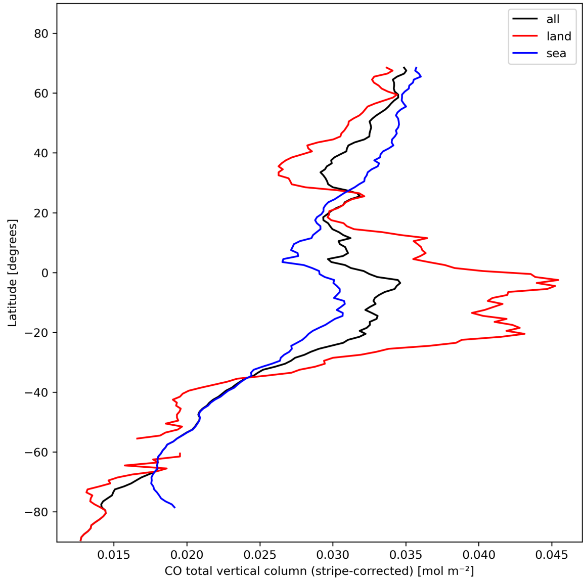
Figure 11: Zonal average of “CO total vertical column (stripe-corrected)” for 2023-11-07 to 2023-11-09.
