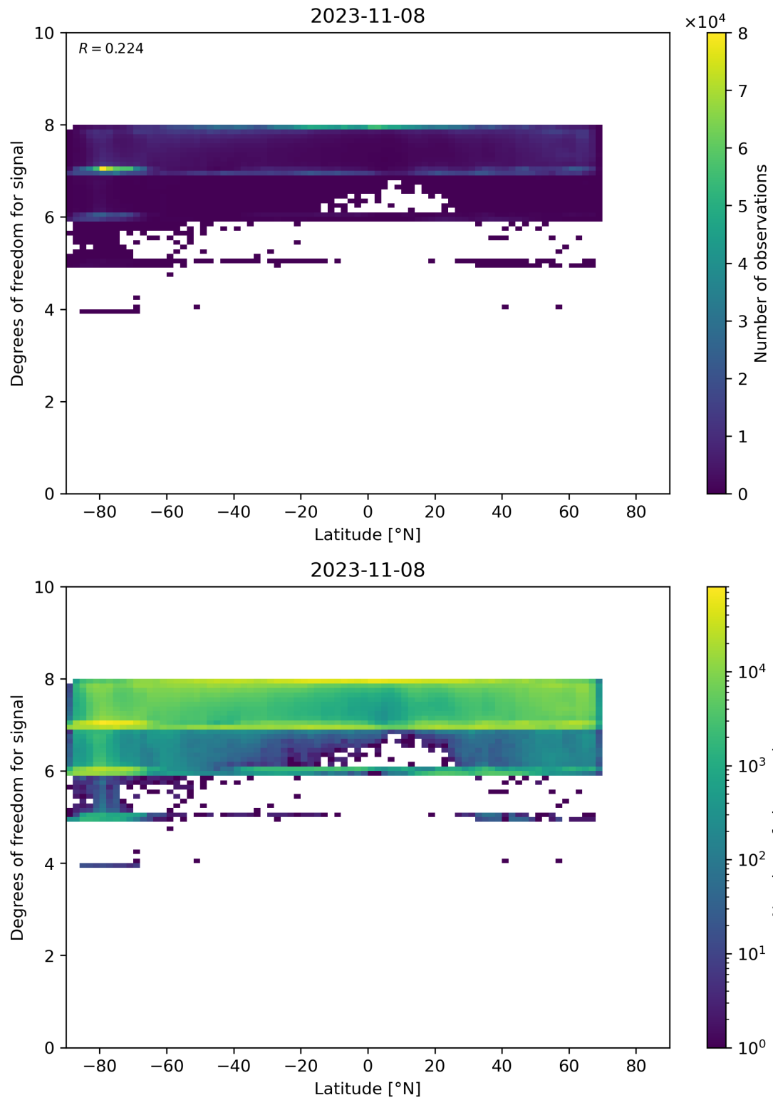
Figure 55: Scatter density plot of “Latitude” against “Degrees of freedom for signal” for 2023-11-07 to 2023-11-09.
