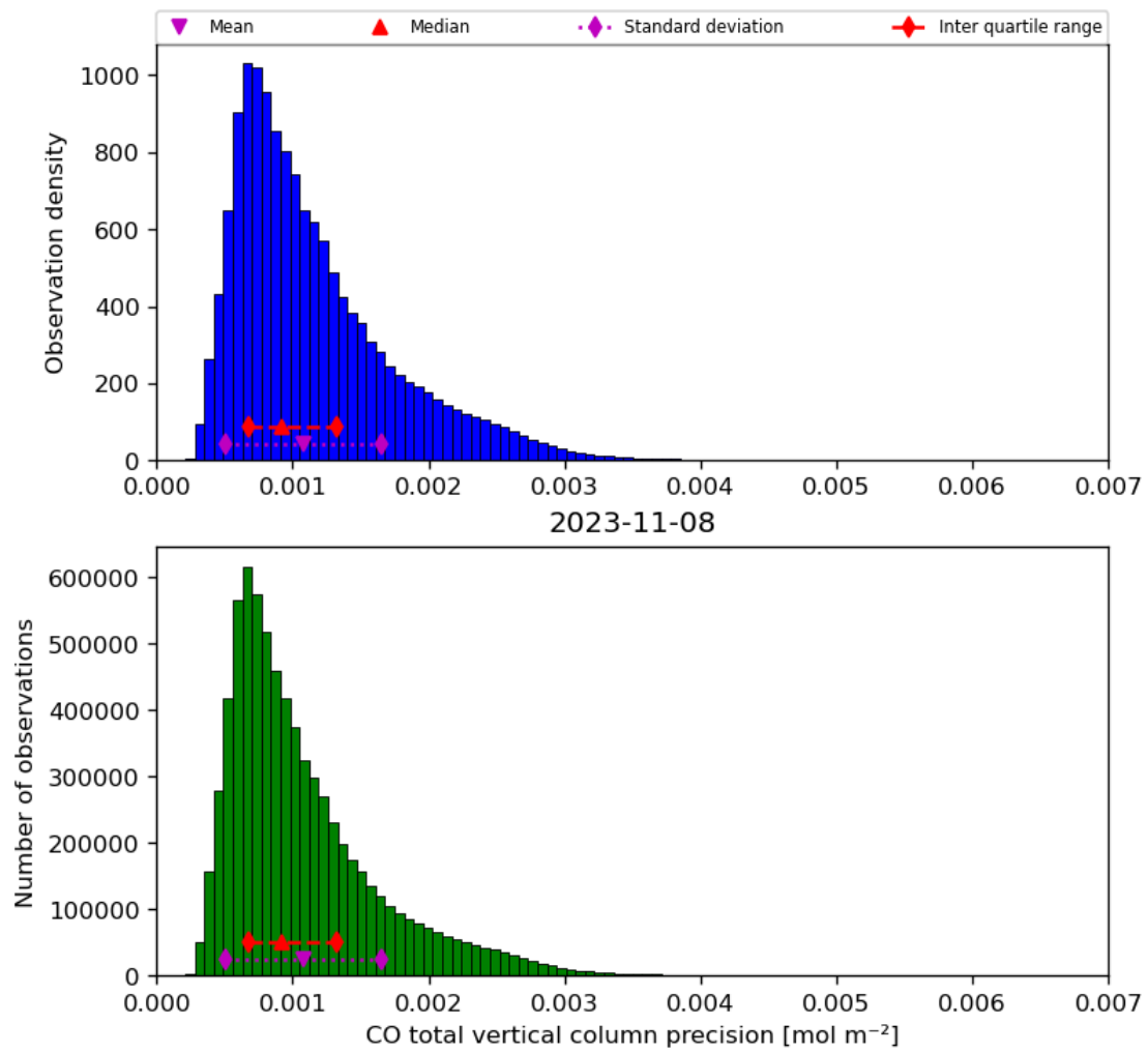
Figure 20: Histogram of “CO total vertical column precision” for 2023-11-07 to 2023-11-09
