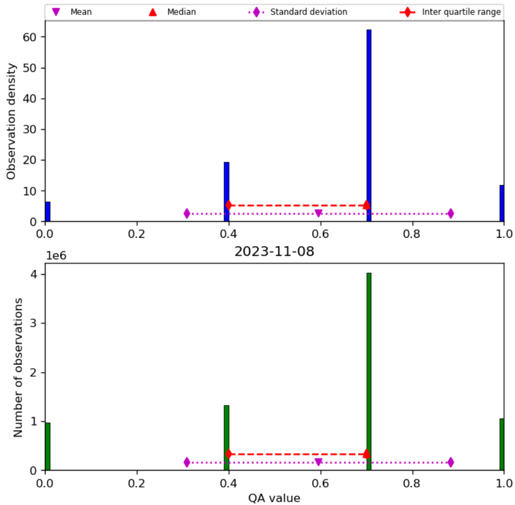
Figure 17: Histogram of “QA value” for 2023-11-07 to 2023-11-09
