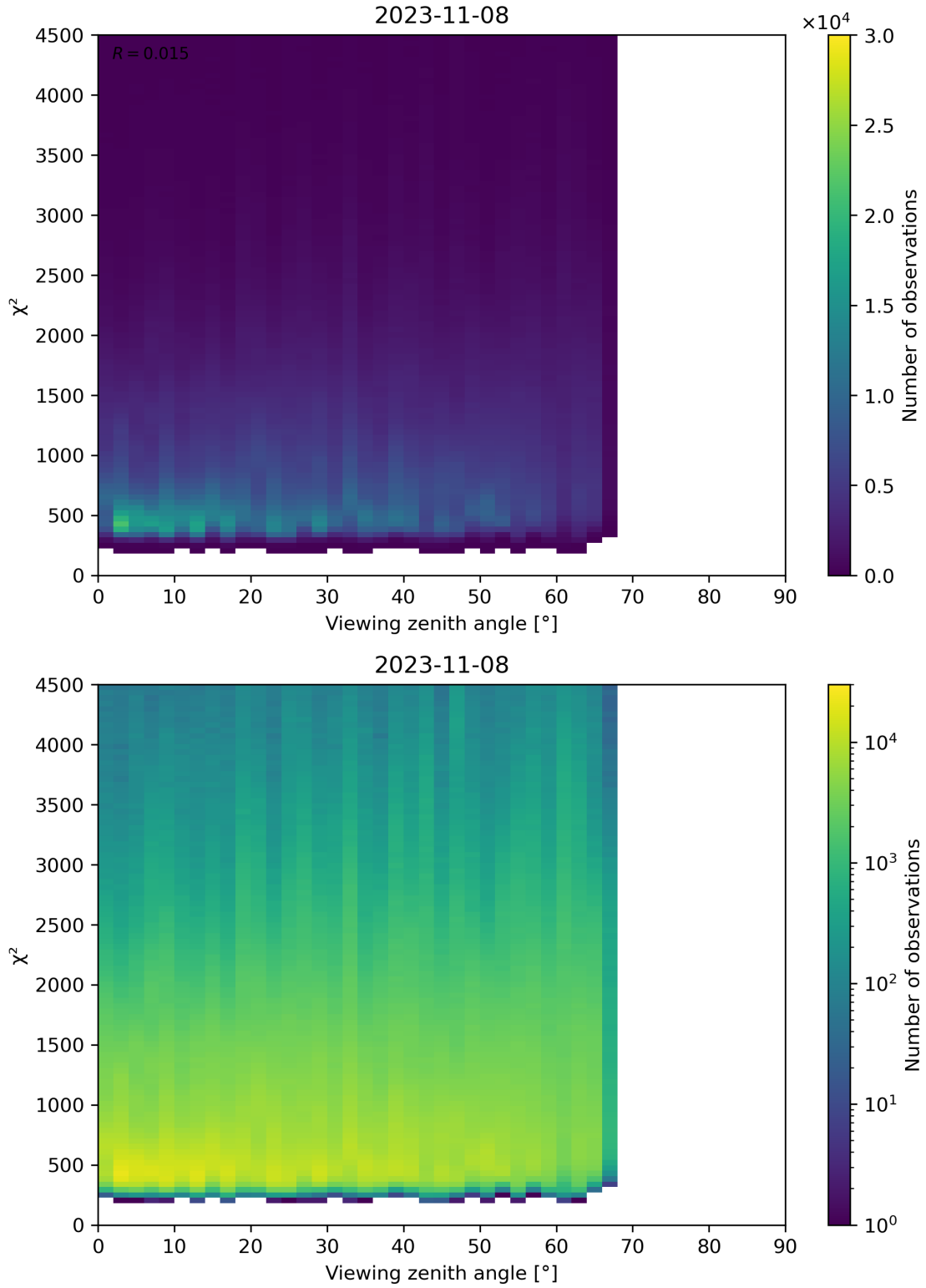
Figure 72: Scatter density plot of “Viewing zenith angle” against “ \chi^2 ” for 2023-11-07 to 2023-11-09.
