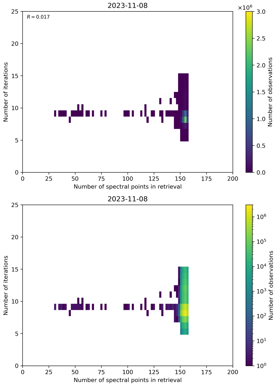
Figure 60: Scatter density plot of “Number of spectral points in retrieval” against “Number of iterations” for 2023-11-07 to 2023-11-09.
