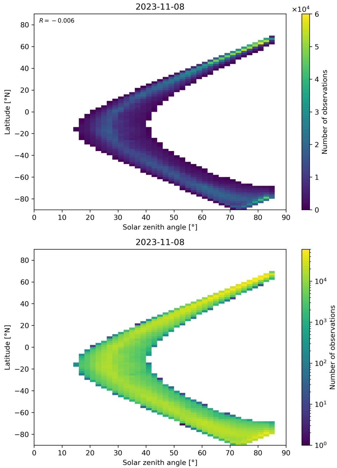
Figure 66: Scatter density plot of “Solar zenith angle” against “Latitude” for 2023-11-07 to 2023-11-09.
