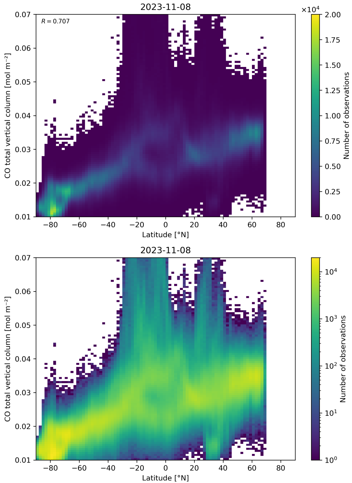
Figure 51: Scatter density plot of “Latitude” against “CO total vertical column” for 2023-11-07 to 2023-11-09.
