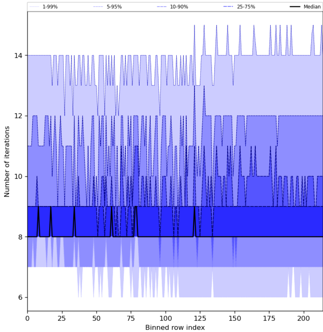
Figure 32: Along track statistics of “Number of iterations” for 2023-11-07 to 2023-11-09
