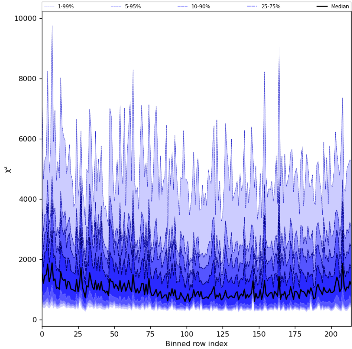
Figure 30: Along track statistics of “ \chi^2 ” for 2023-11-07 to 2023-11-09
