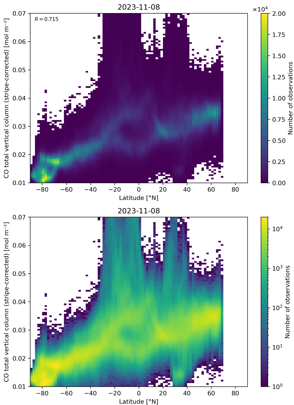
Figure 52: Scatter density plot of “Latitude” against “CO total vertical column (stripe-corrected)” for 2023-11-07 to 2023-11-09.
