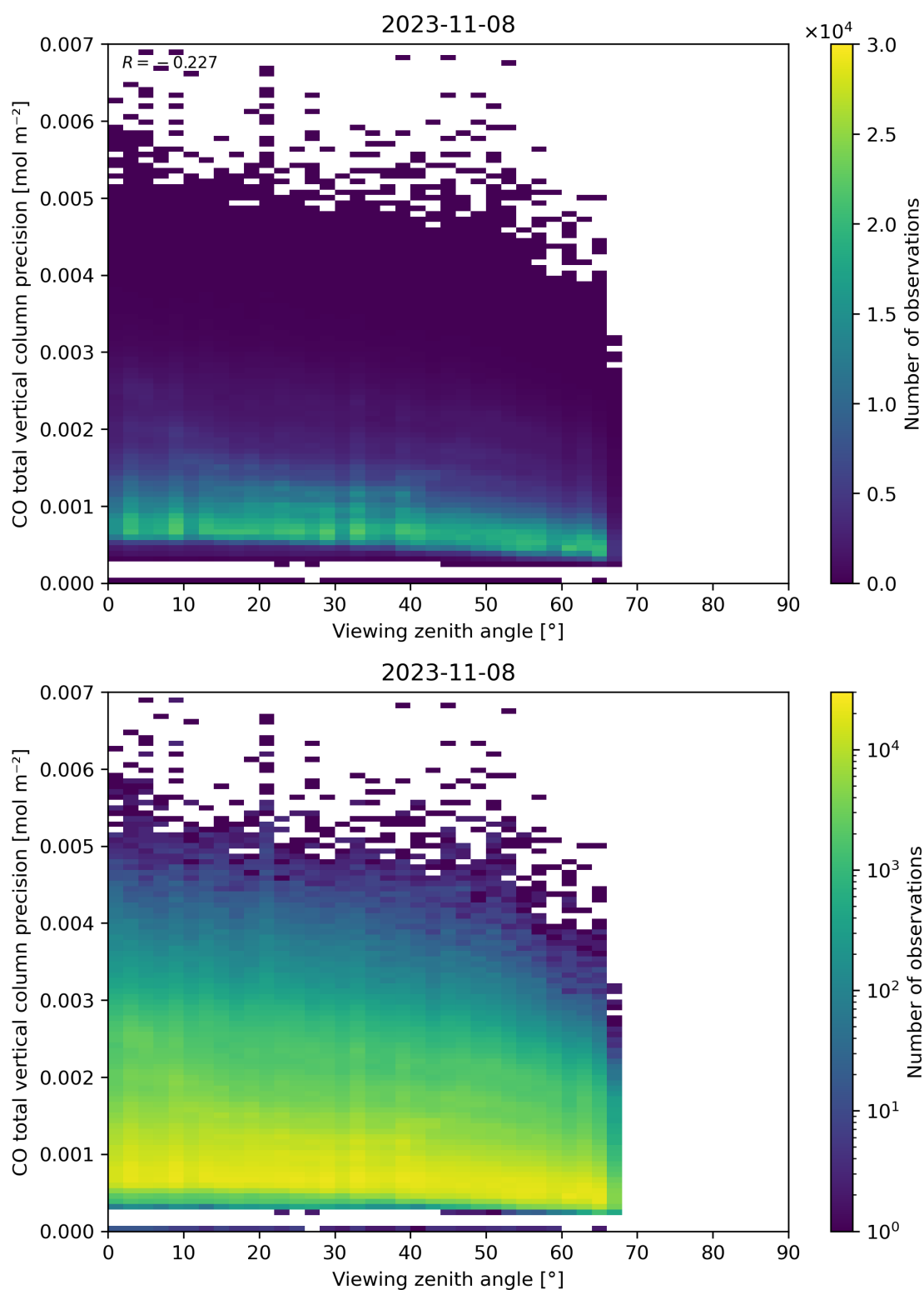
Figure 71: Scatter density plot of “Viewing zenith angle” against “CO total vertical column precision” for 2023-11-07 to 2023-11-09.
