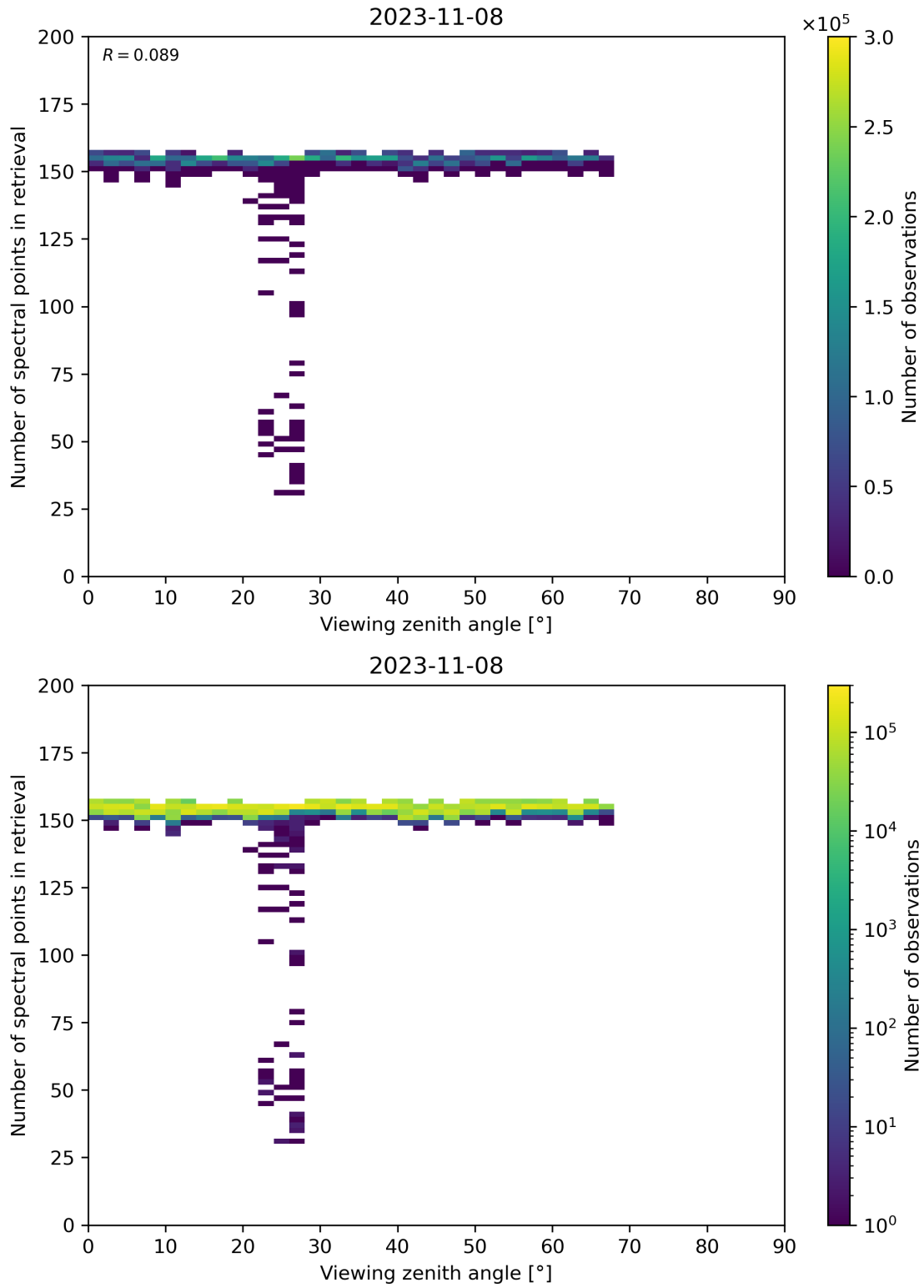
Figure 76: Scatter density plot of “Viewing zenith angle” against “Number of spectral points in retrieval” for 2023-11-07 to 2023-11-09.
