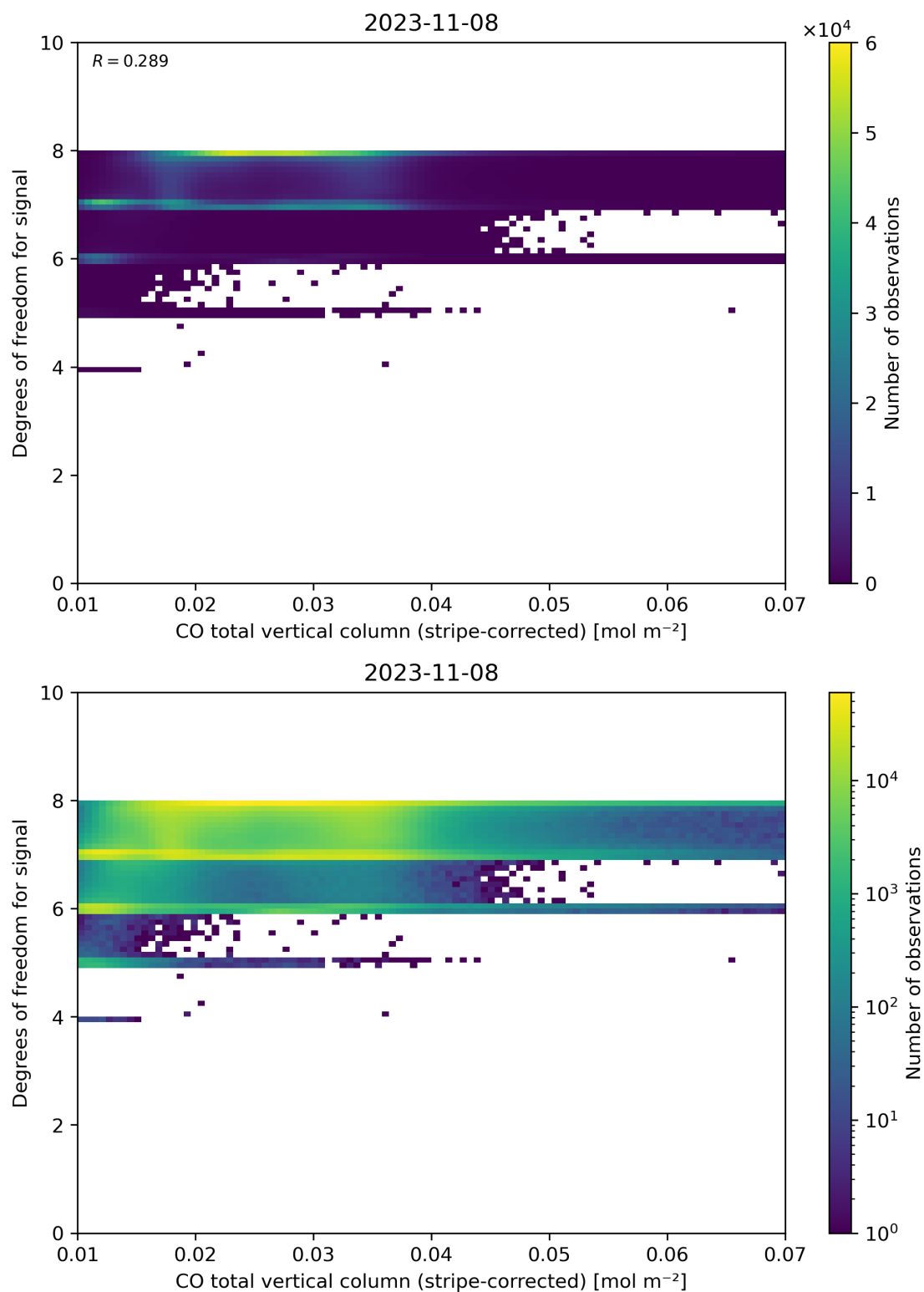
Figure 38: Scatter density plot of “CO total vertical column (stripe-corrected)” against “Degrees of freedom for signal” for 2023-11-07 to 2023-11-09.
