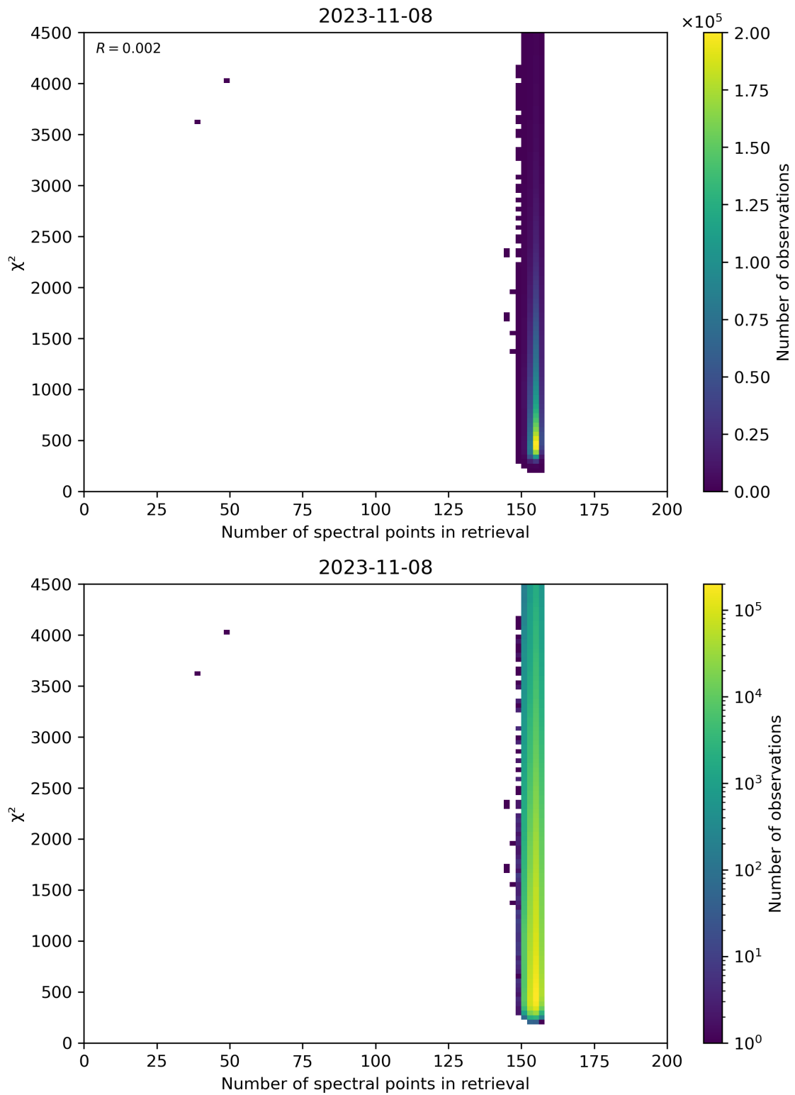
Figure 58: Scatter density plot of “Number of spectral points in retrieval” against “ \chi^2 ” for 2023-11-07 to 2023-11-09.
