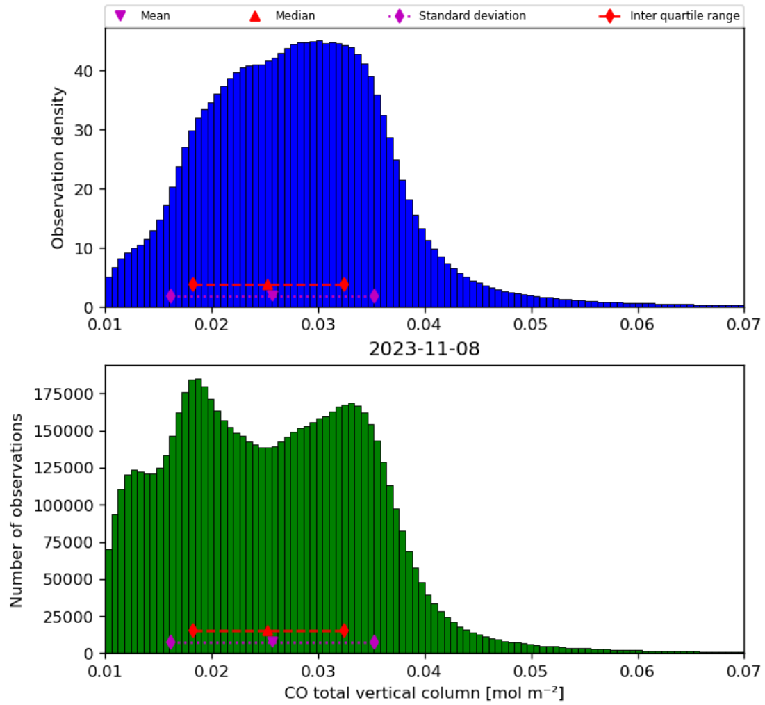
Figure 18: Histogram of “CO total vertical column” for 2023-11-07 to 2023-11-09
