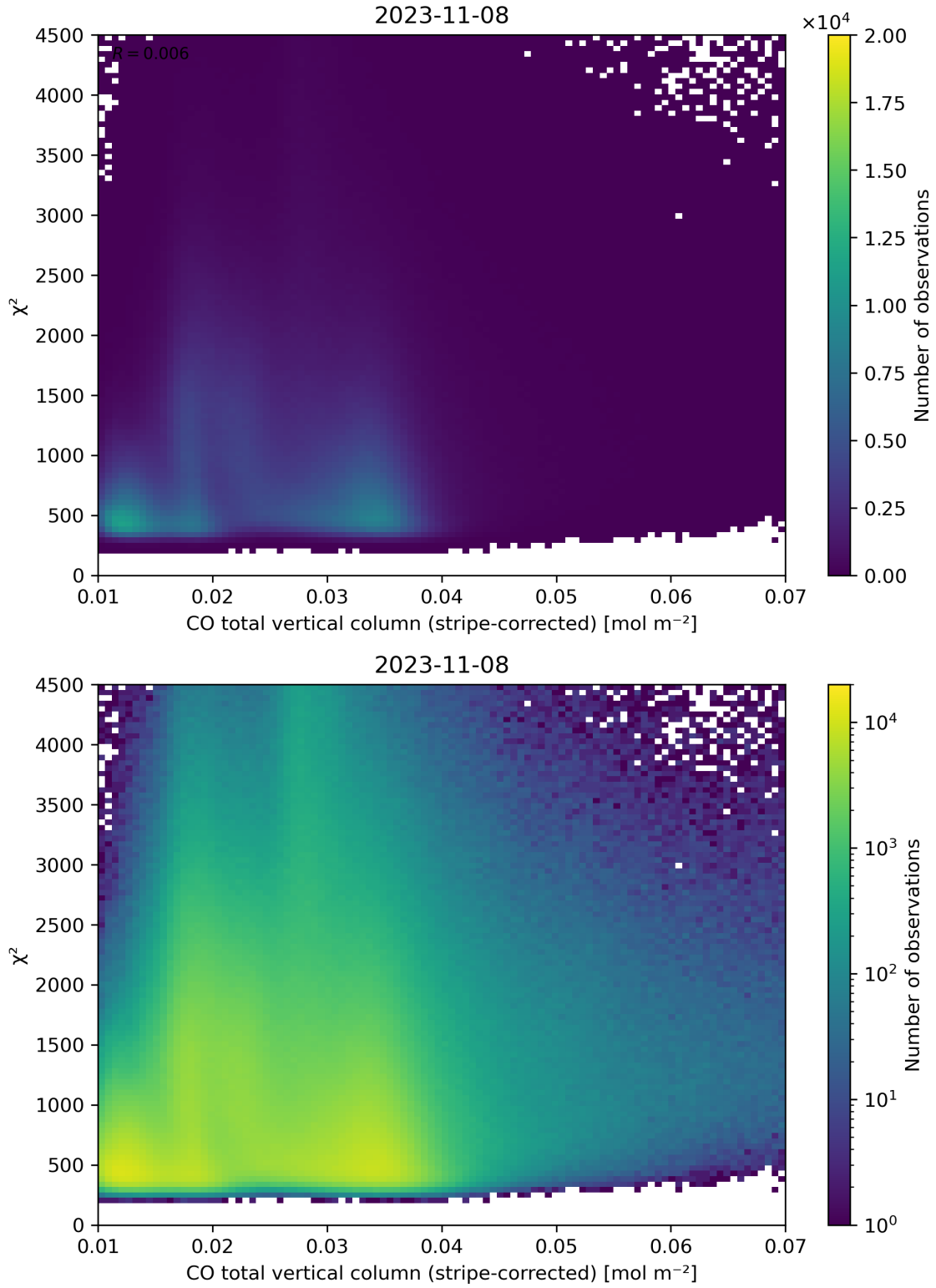
Figure 37: Scatter density plot of “CO total vertical column (stripe-corrected)” against “ \chi^2 ” for 2023-11-07 to 2023-11-09.
