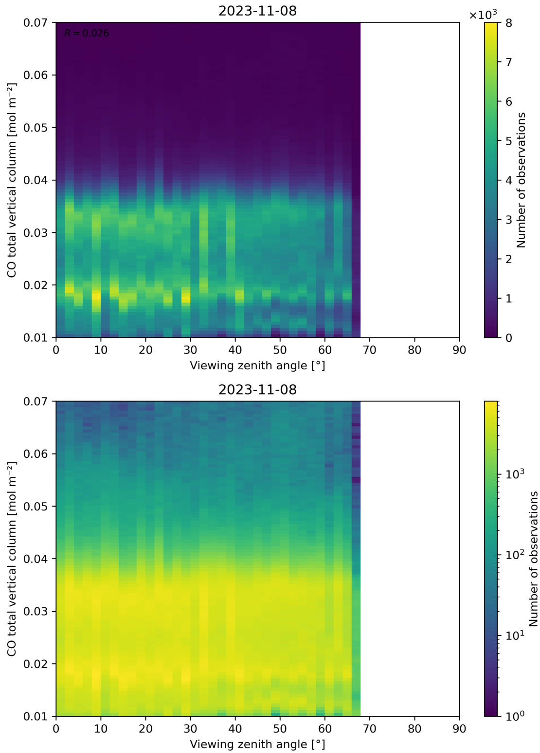
Figure 69: Scatter density plot of “Viewing zenith angle” against “CO total vertical column” for 2023-11-07 to 2023-11-09.
