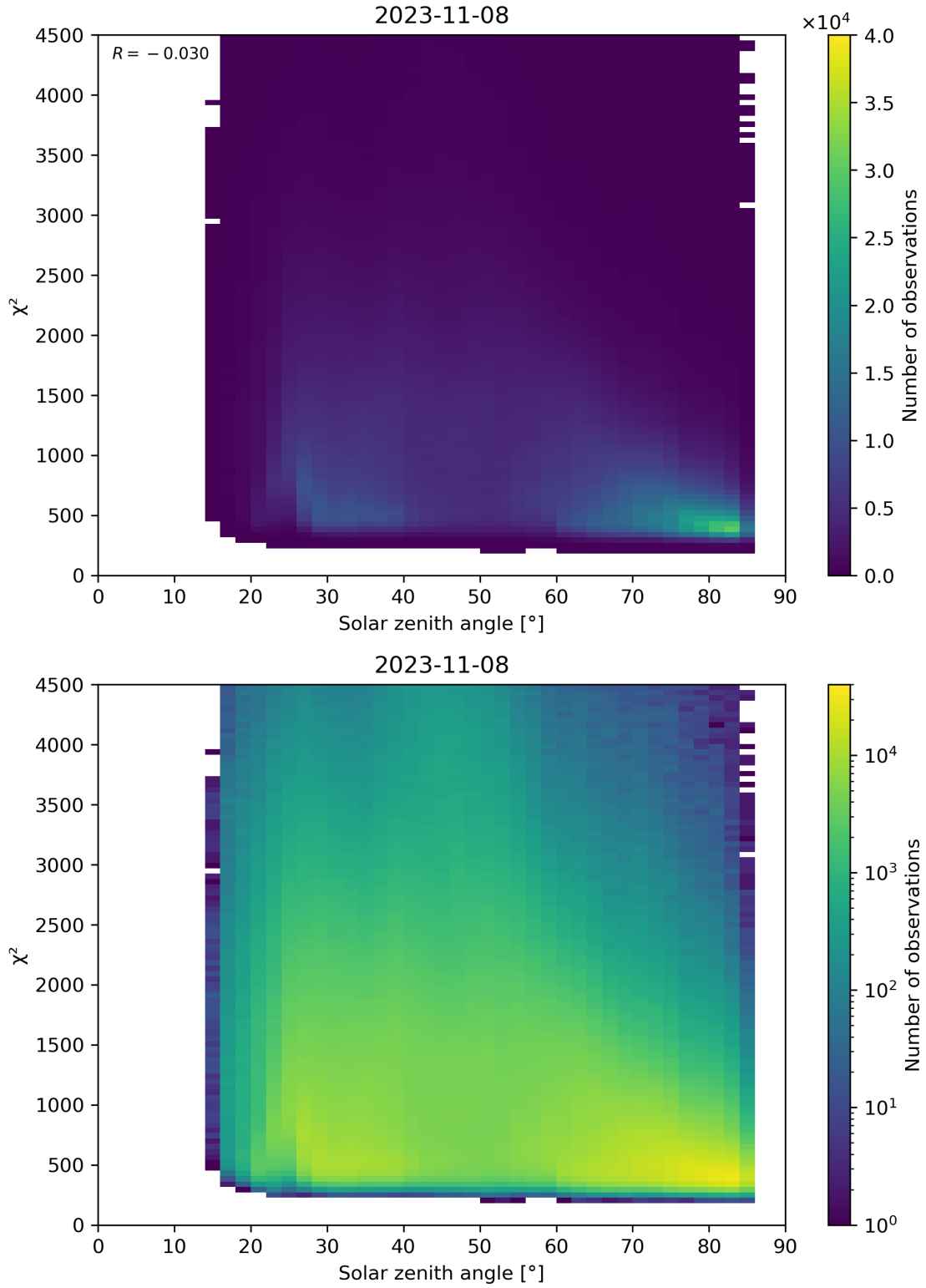
Figure 64: Scatter density plot of “Solar zenith angle” against “ \chi^2 ” for 2023-11-07 to 2023-11-09.
