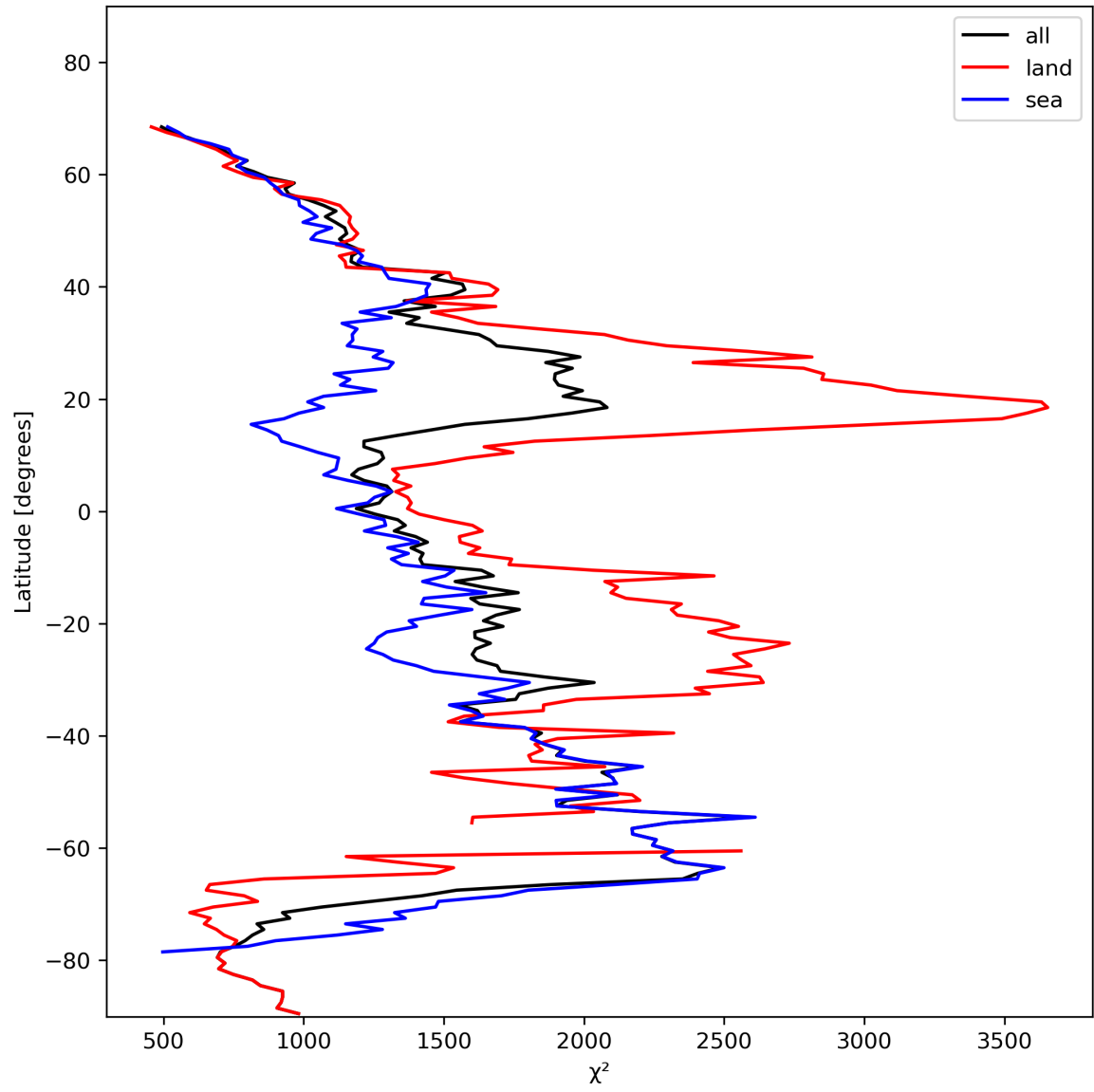
Figure 14: Zonal average of “ \chi^2 ” for 2023-11-07 to 2023-11-09.
