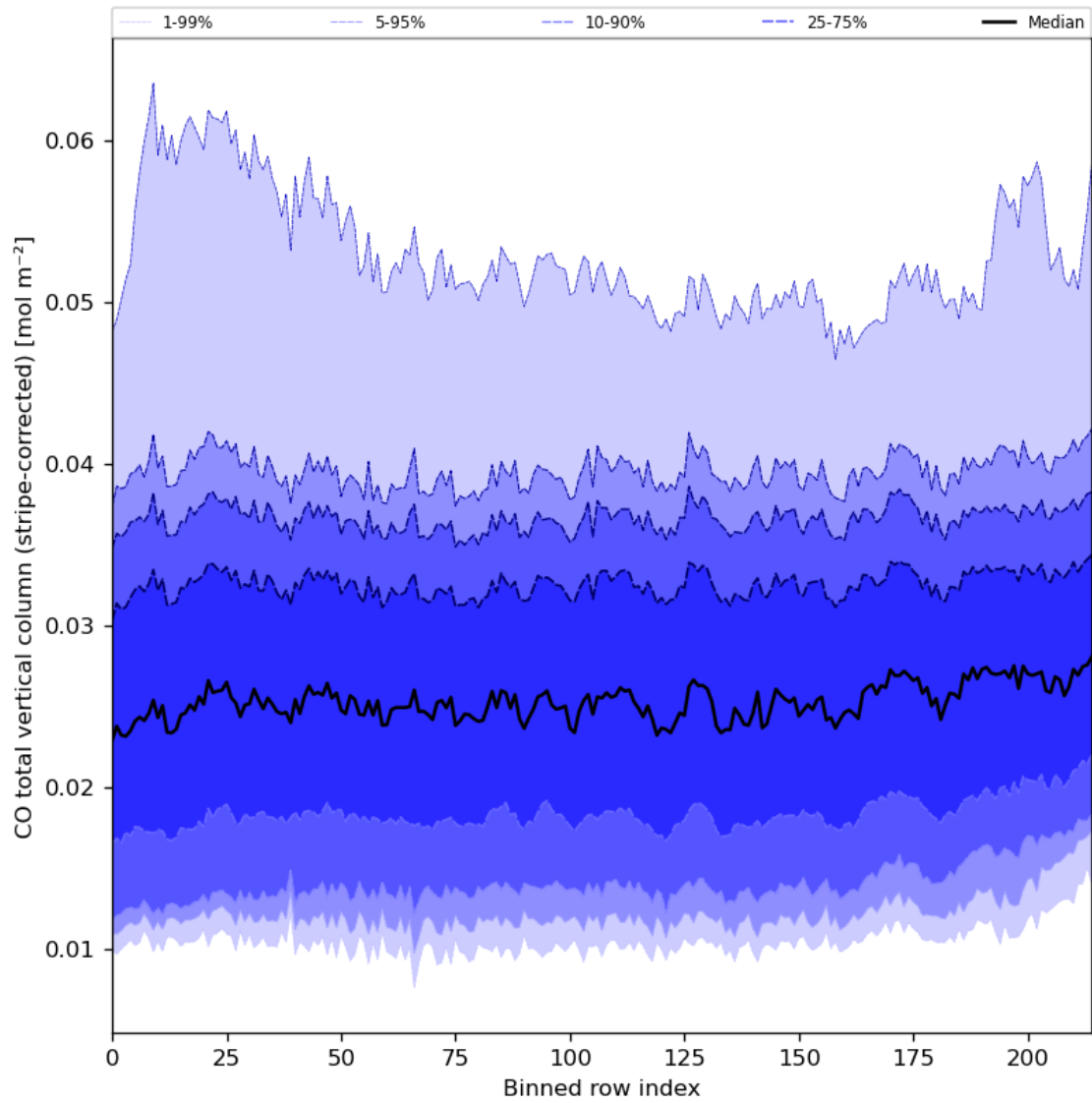
Figure 27: Along track statistics of “CO total vertical column (stripe-corrected)” for 2023-11-07 to 2023-11-09
