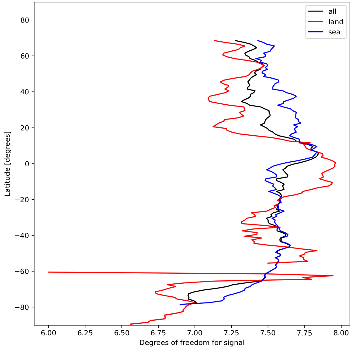
Figure 15: Zonal average of “Degrees of freedom for signal” for 2023-11-07 to 2023-11-09.
