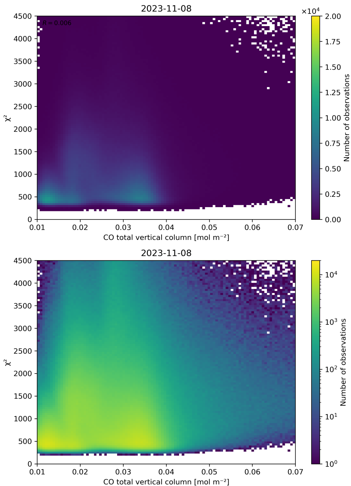
Figure 35: Scatter density plot of “CO total vertical column” against “ \chi^2 ” for 2023-11-07 to 2023-11-09.
