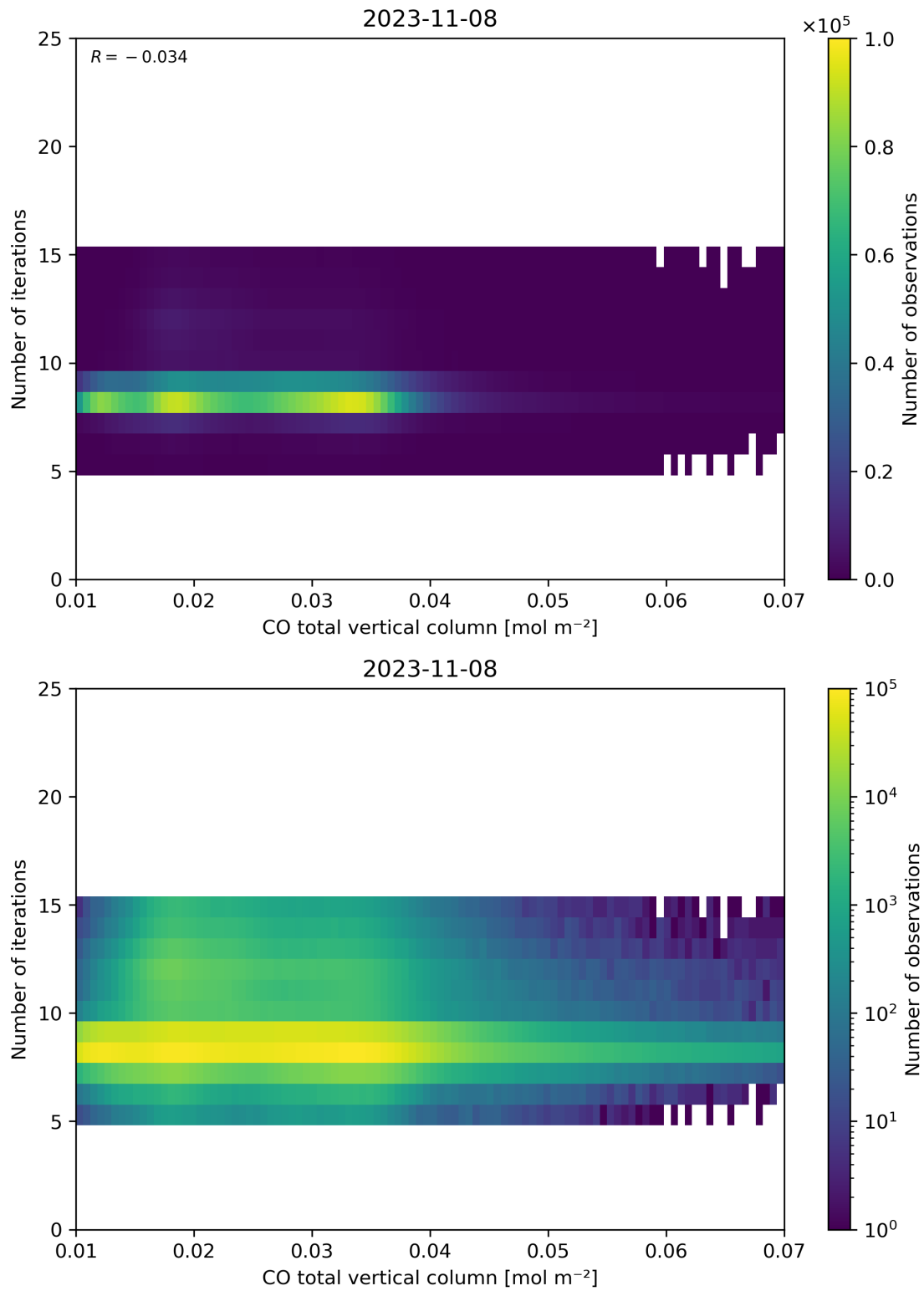
Figure 42: Scatter density plot of “CO total vertical column” against “Number of iterations” for 2023-11-07 to 2023-11-09.
