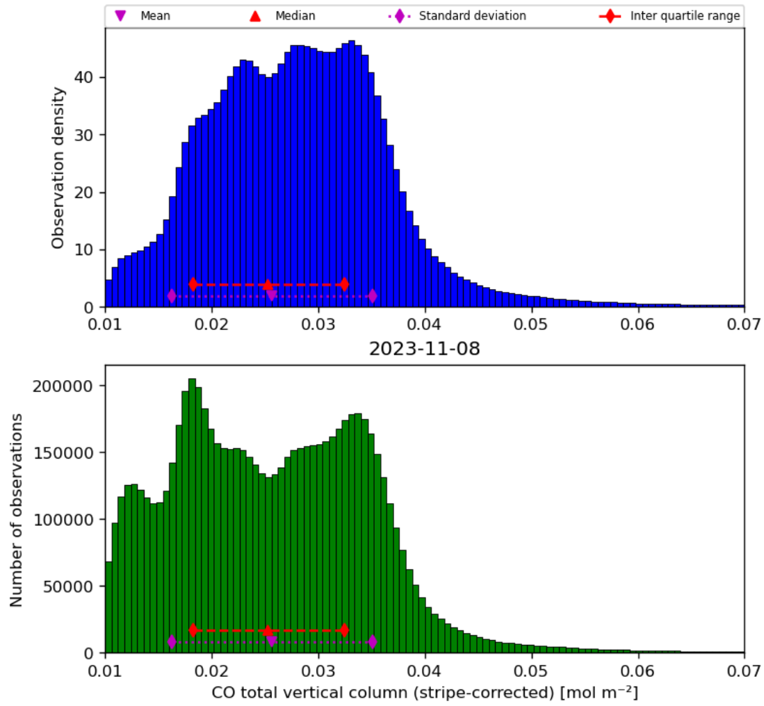
Figure 19: Histogram of “CO total vertical column (stripe-corrected)” for 2023-11-07 to 2023-11-09
