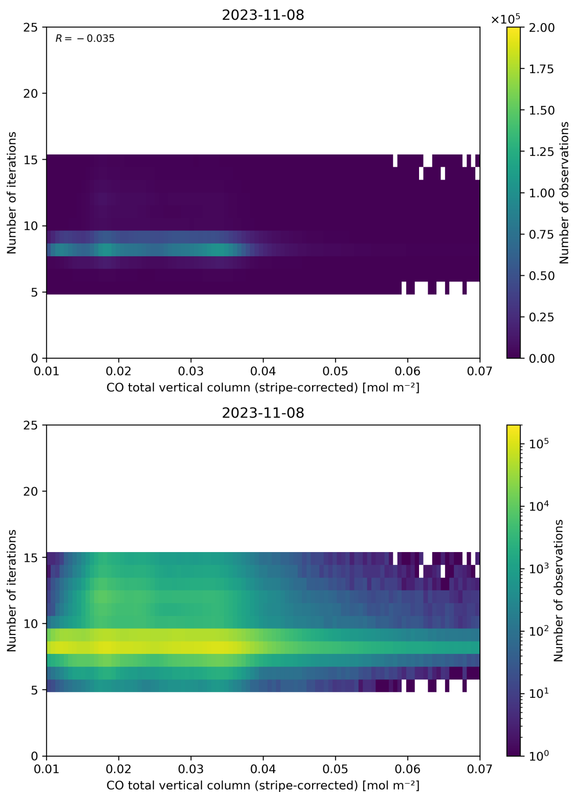
Figure 39: Scatter density plot of “CO total vertical column (stripe-corrected)” against “Number of iterations” for 2023-11-07 to 2023-11-09.
