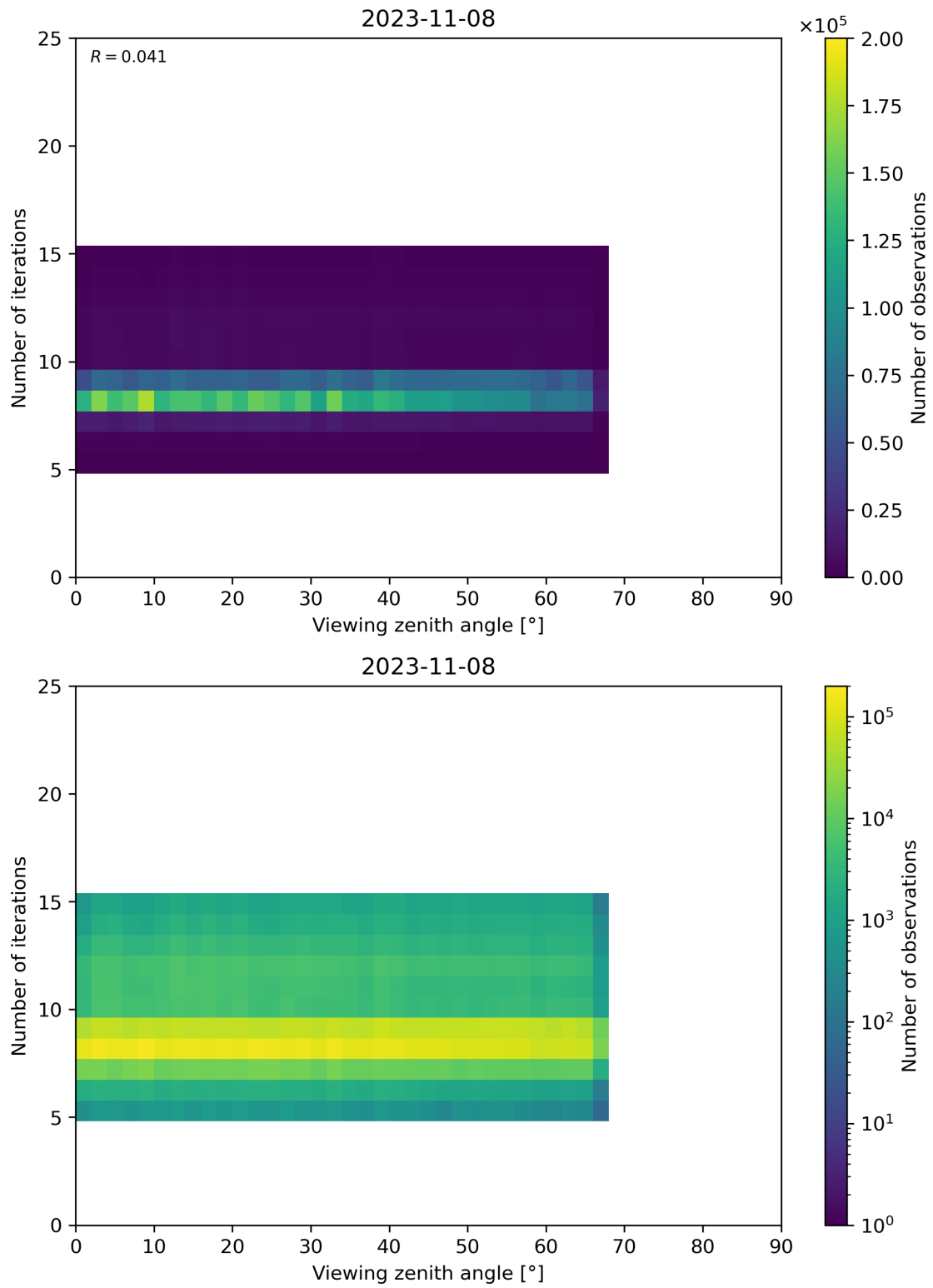
Figure 75: Scatter density plot of “Viewing zenith angle” against “Number of iterations” for 2023-11-07 to 2023-11-09.
