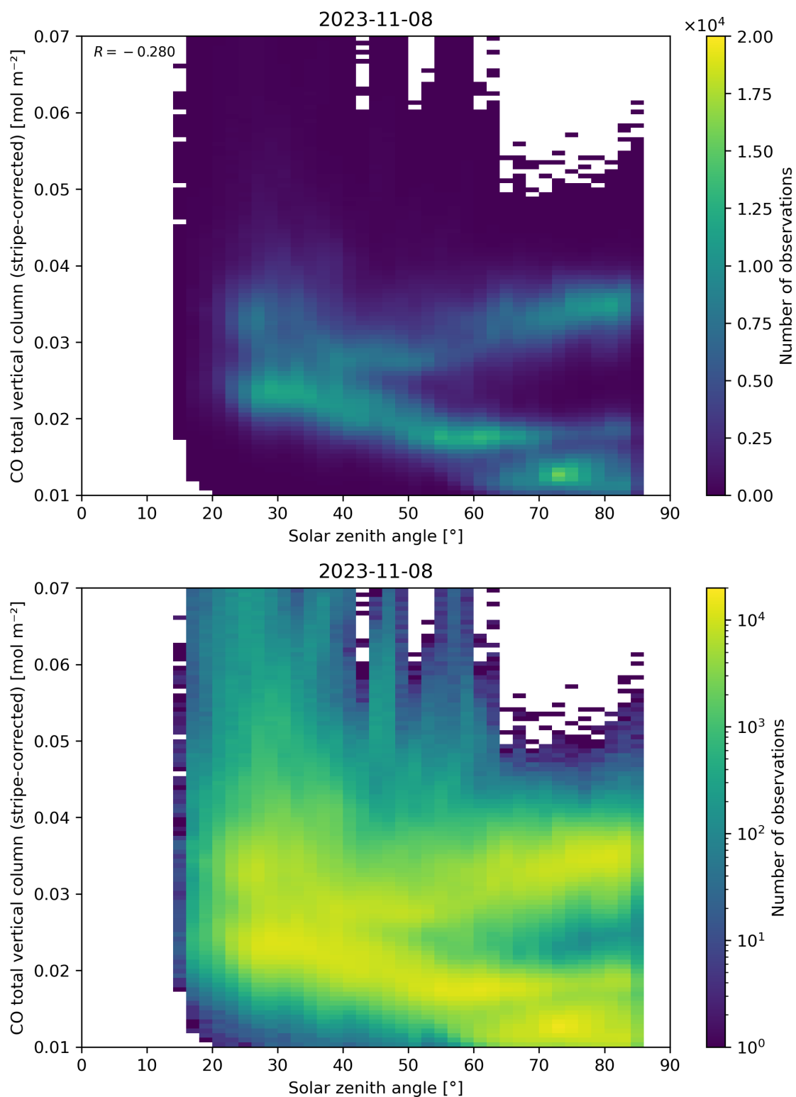
Figure 62: Scatter density plot of “Solar zenith angle” against “CO total vertical column (stripe-corrected)” for 2023-11-07 to 2023-11-09.
