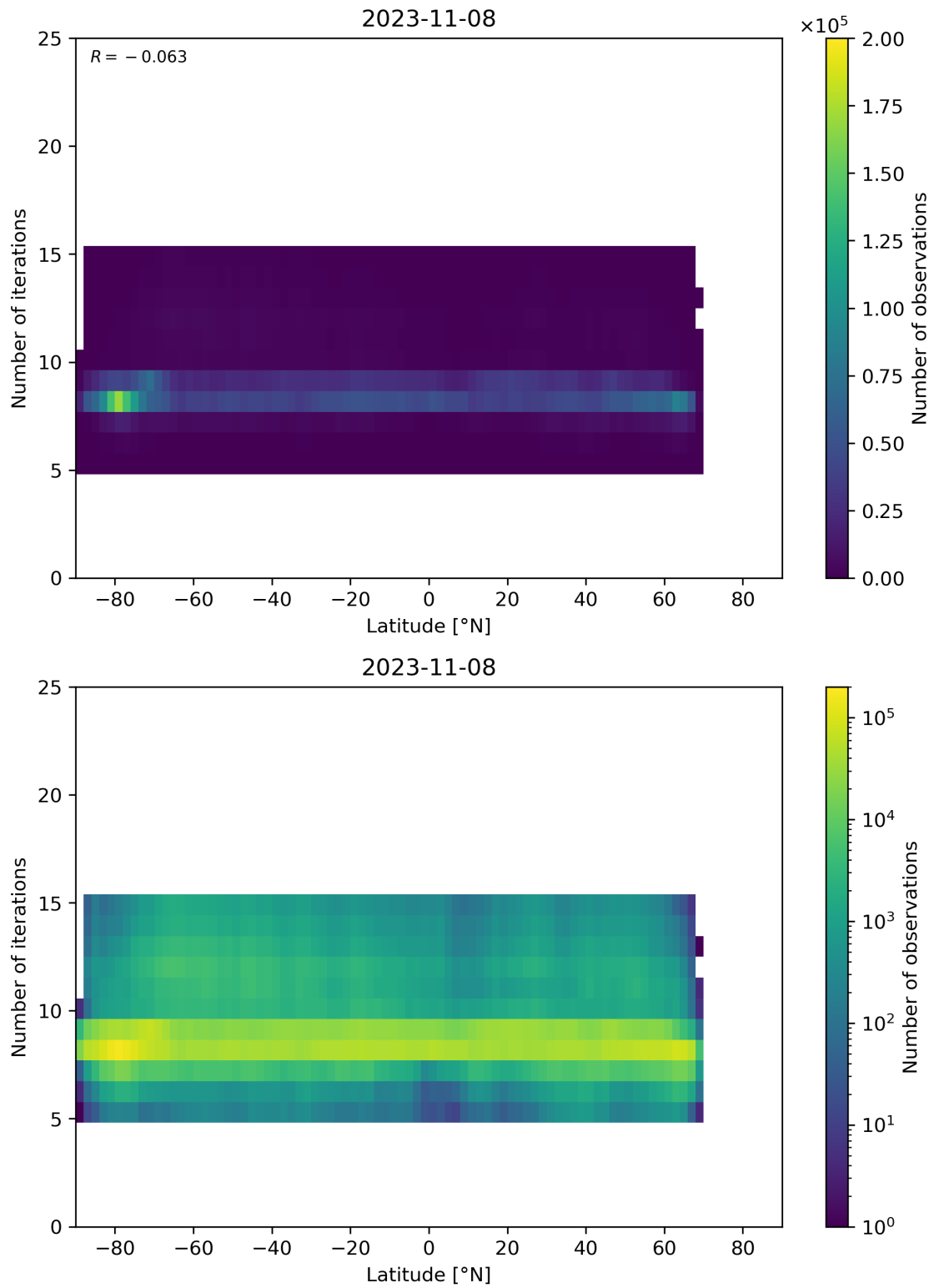
Figure 56: Scatter density plot of “Latitude” against “Number of iterations” for 2023-11-07 to 2023-11-09.
