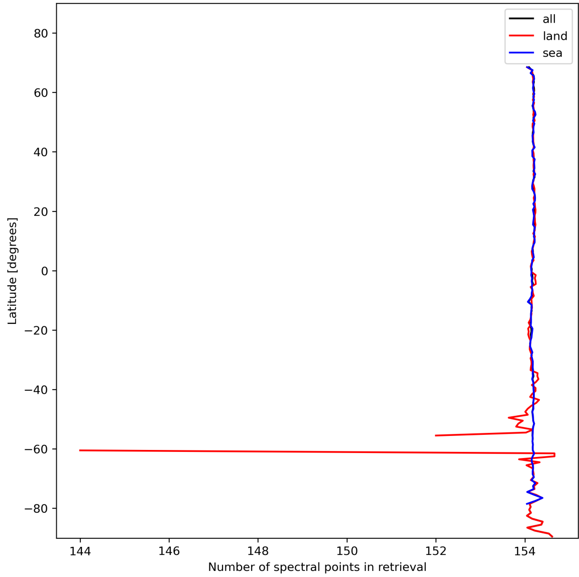
Figure 13: Zonal average of “Number of spectral points in retrieval” for 2023-11-07 to 2023-11-09.
