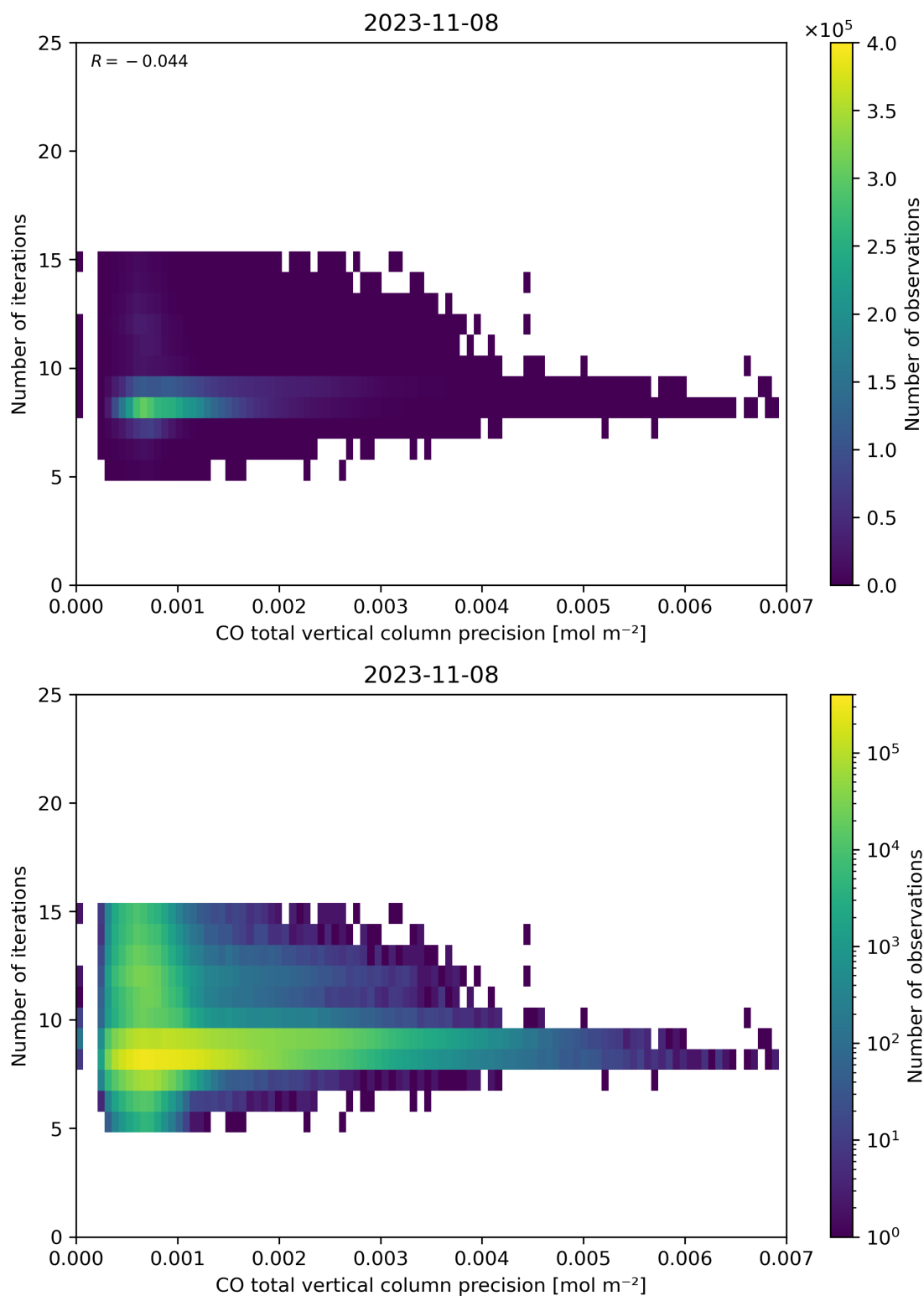
Figure 46: Scatter density plot of “CO total vertical column precision” against “Number of iterations” for 2023-11-07 to 2023-11-09.
