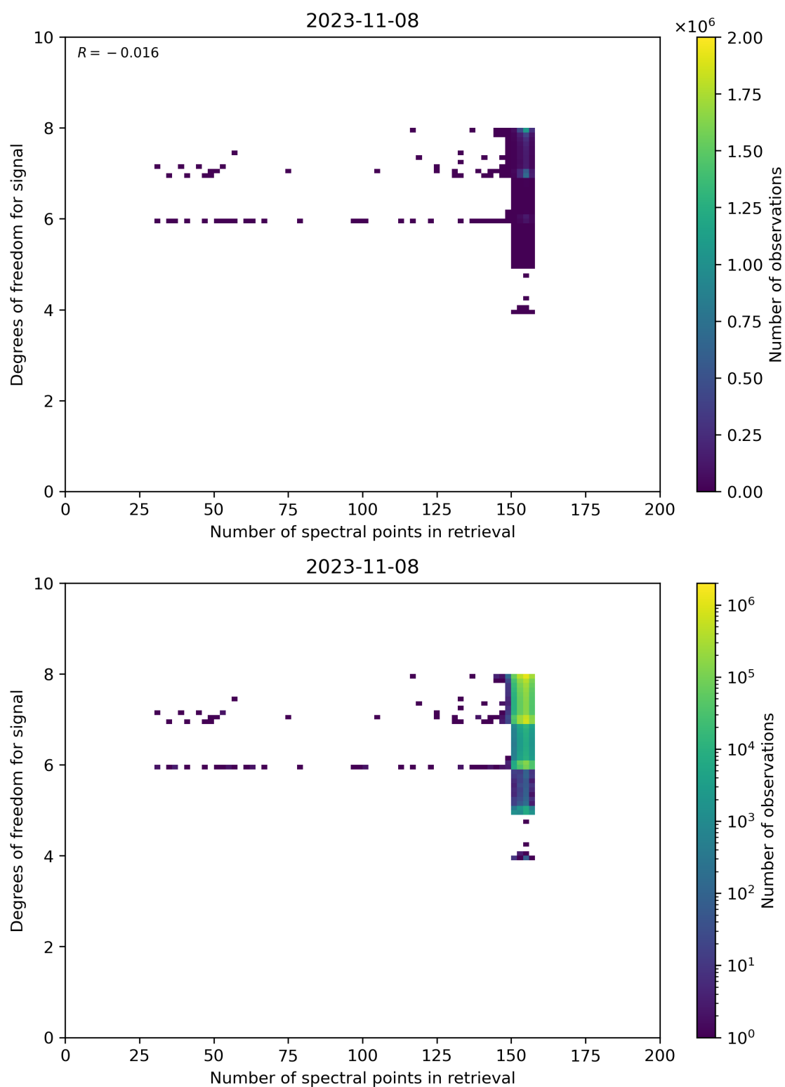
Figure 59: Scatter density plot of “Number of spectral points in retrieval” against “Degrees of freedom for signal” for 2023-11-07 to 2023-11-09.
