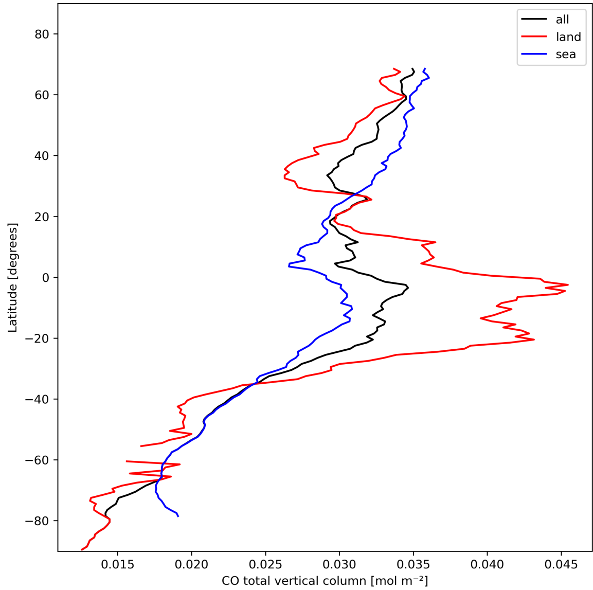
Figure 10: Zonal average of “CO total vertical column” for 2023-11-07 to 2023-11-09.
