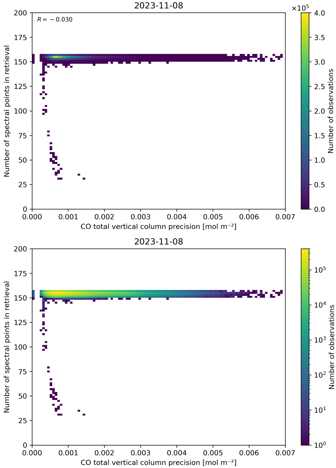
Figure 47: Scatter density plot of “CO total vertical column precision” against “Number of spectral points in retrieval” for 2023-11-07 to 2023-11-09.
