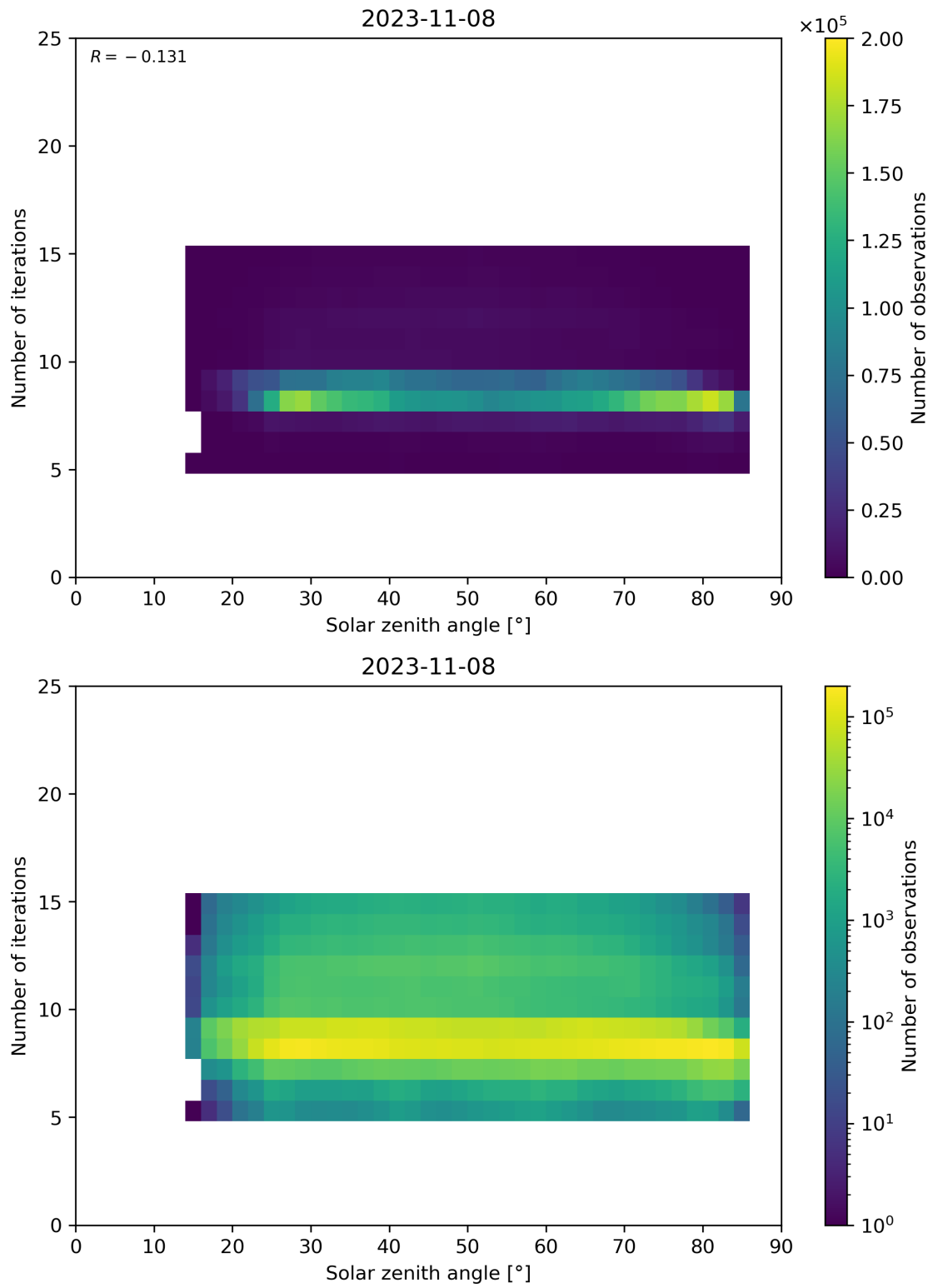
Figure 67: Scatter density plot of “Solar zenith angle” against “Number of iterations” for 2023-11-07 to 2023-11-09.
