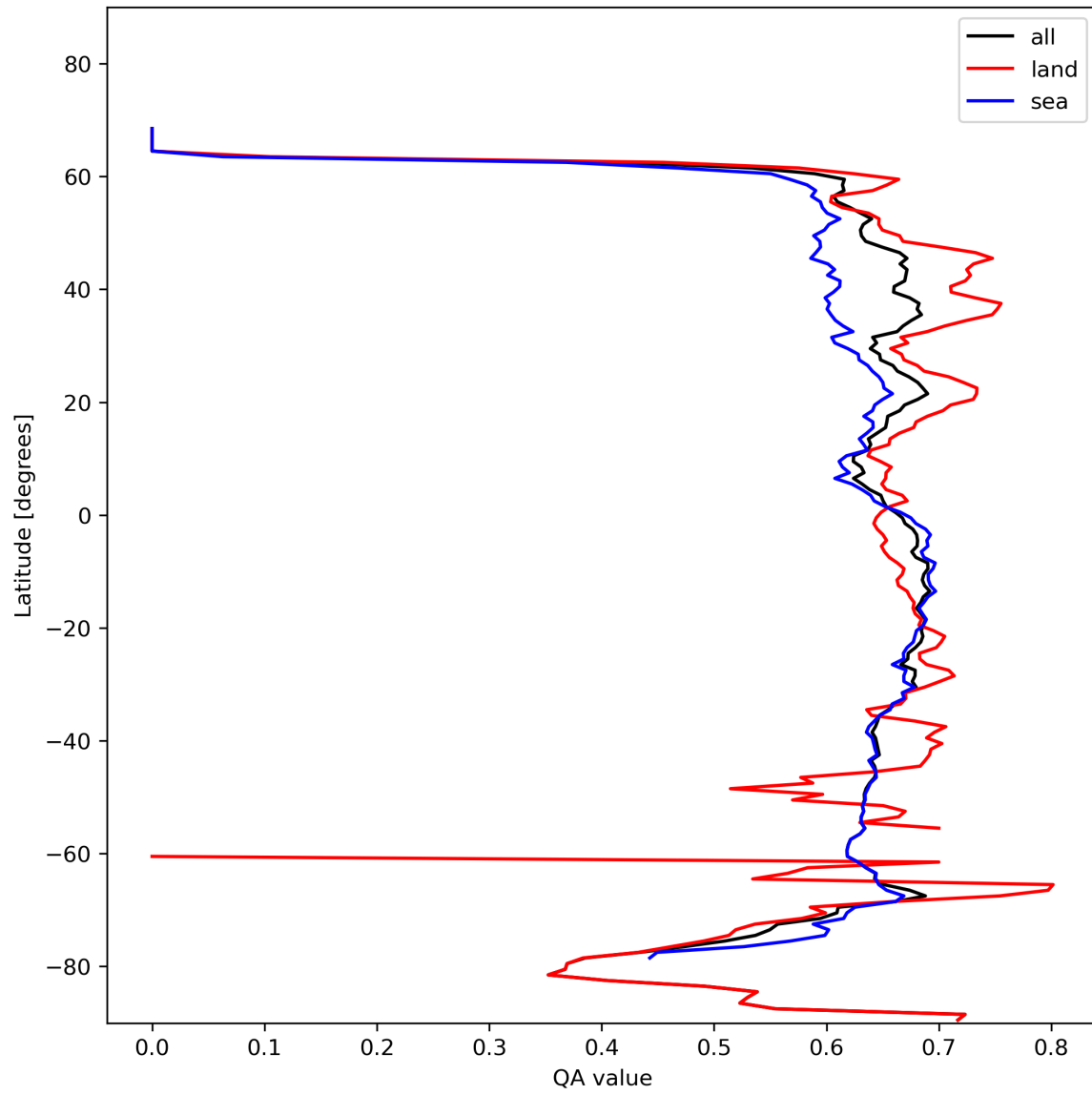
Figure 9: Zonal average of “QA value” for 2023-11-07 to 2023-11-09.
