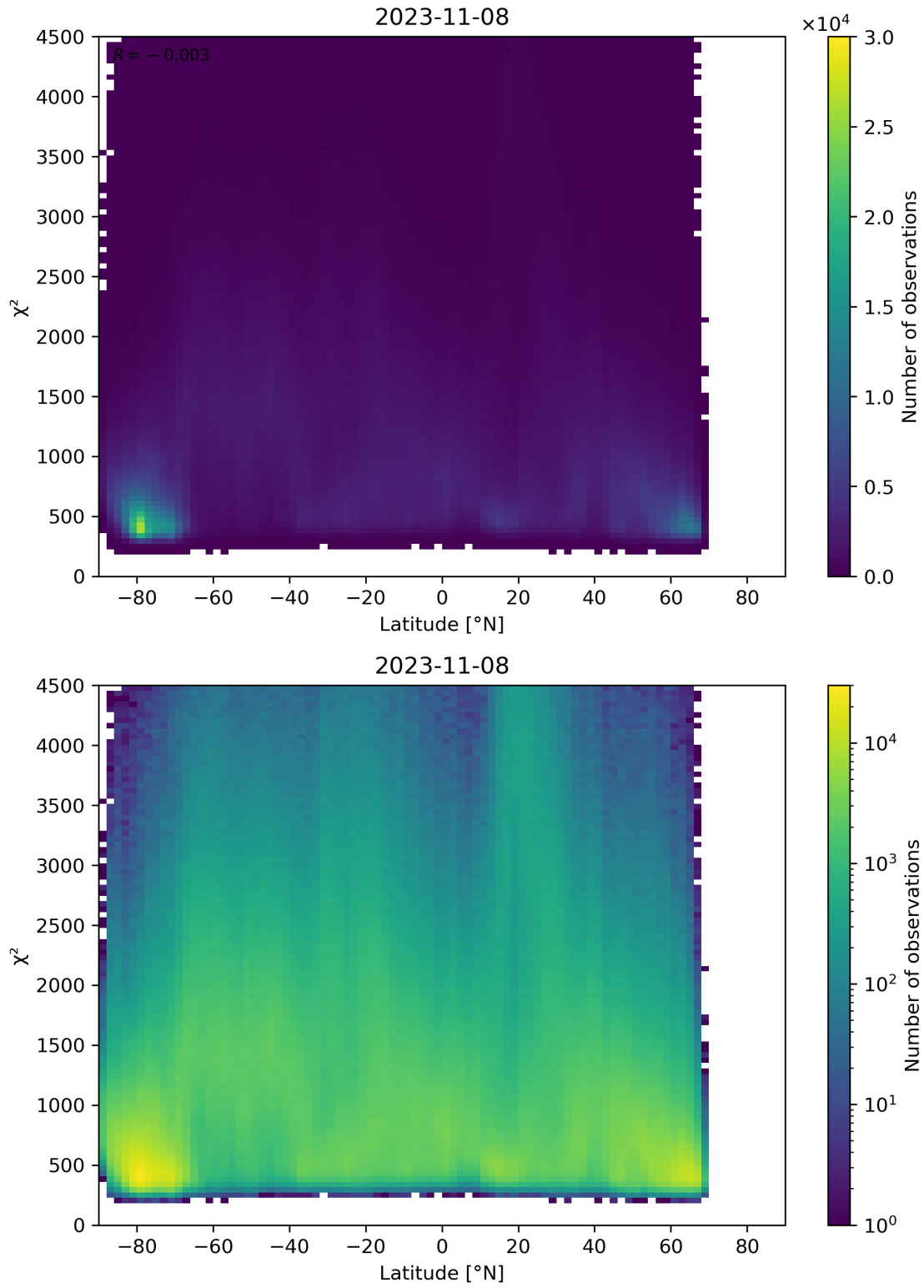
Figure 54: Scatter density plot of “Latitude” against “ \chi^2 ” for 2023-11-07 to 2023-11-09.
