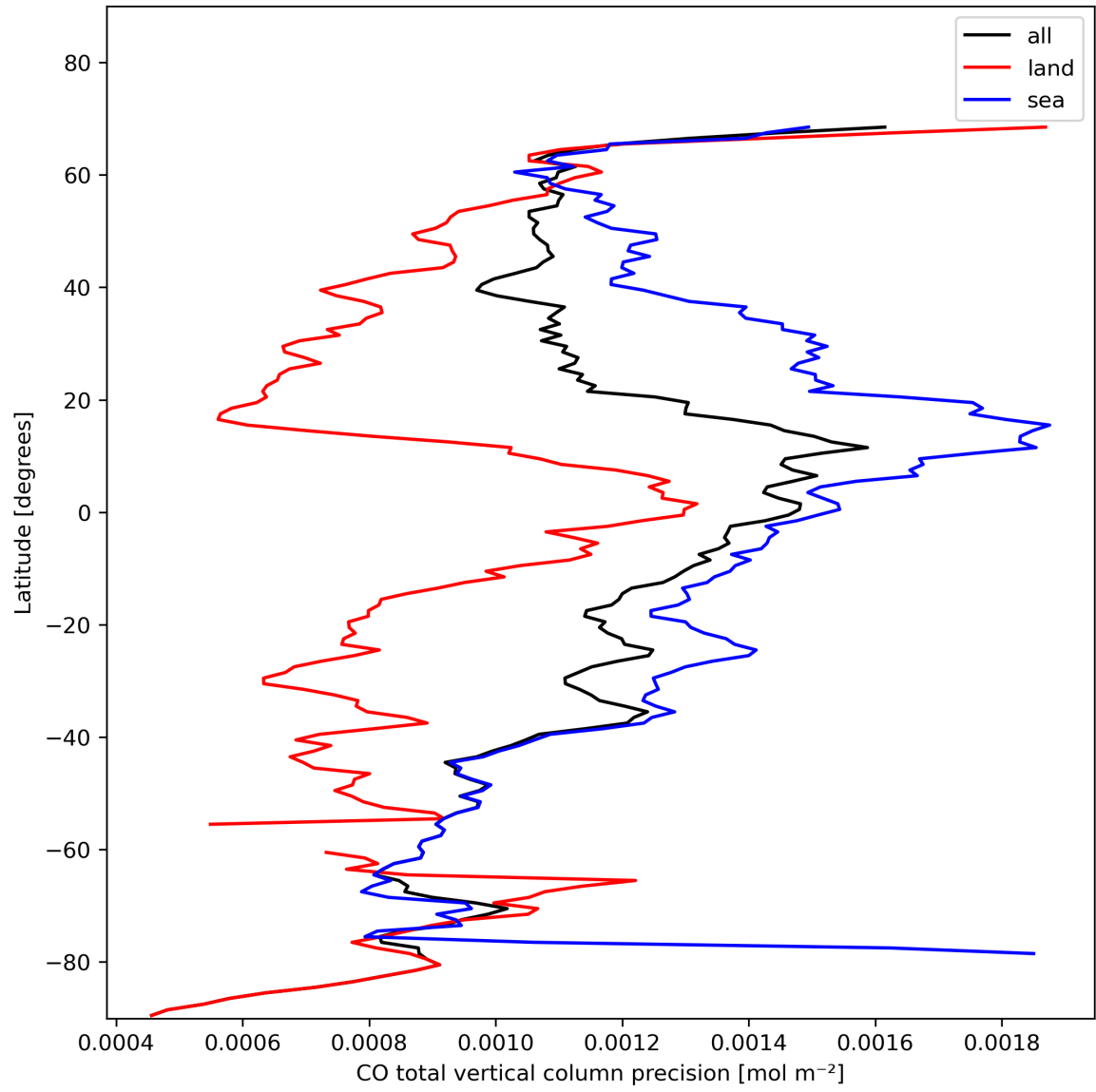
Figure 12: Zonal average of “CO total vertical column precision” for 2023-11-07 to 2023-11-09.
