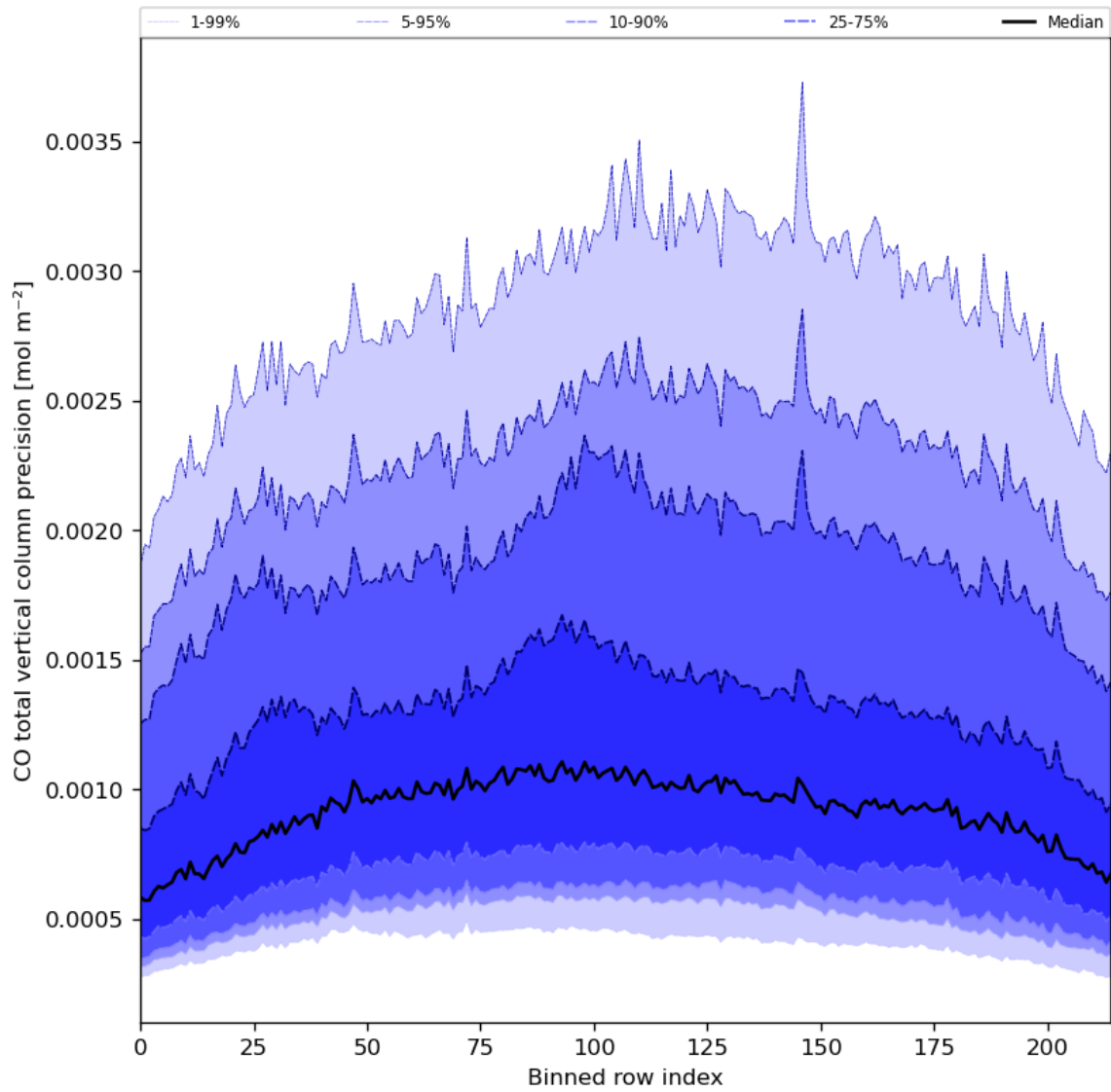
Figure 28: Along track statistics of “CO total vertical column precision” for 2023-11-07 to 2023-11-09
