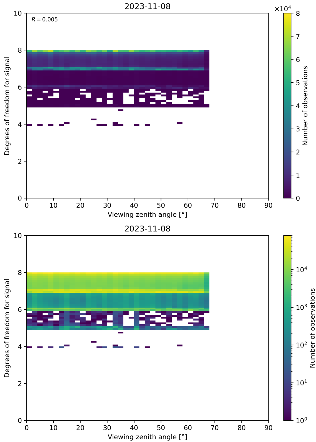
Figure 73: Scatter density plot of “Viewing zenith angle” against “Degrees of freedom for signal” for 2023-11-07 to 2023-11-09.
