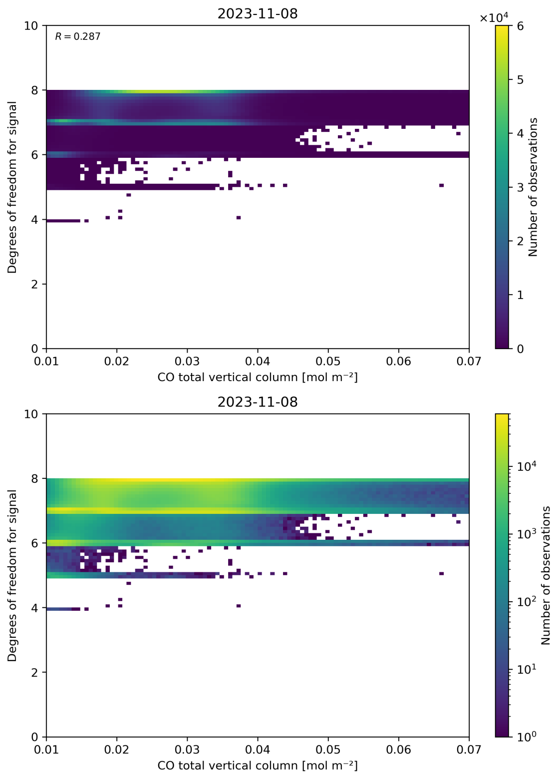
Figure 41: Scatter density plot of “CO total vertical column” against “Degrees of freedom for signal” for 2023-11-07 to 2023-11-09.
