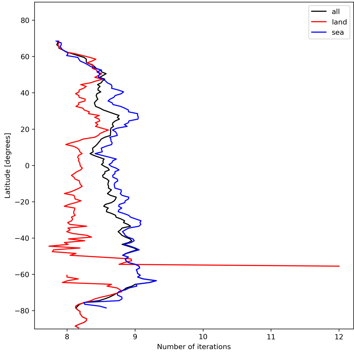
Figure 16: Zonal average of “Number of iterations” for 2023-11-07 to 2023-11-09.
