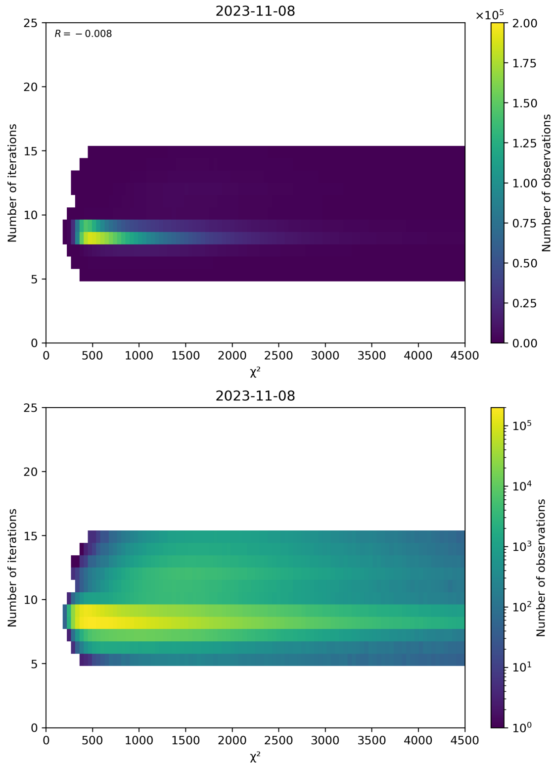
Figure 49: Scatter density plot of “ \chi^2 ” against “Number of iterations” for 2023-11-07 to 2023-11-09.
