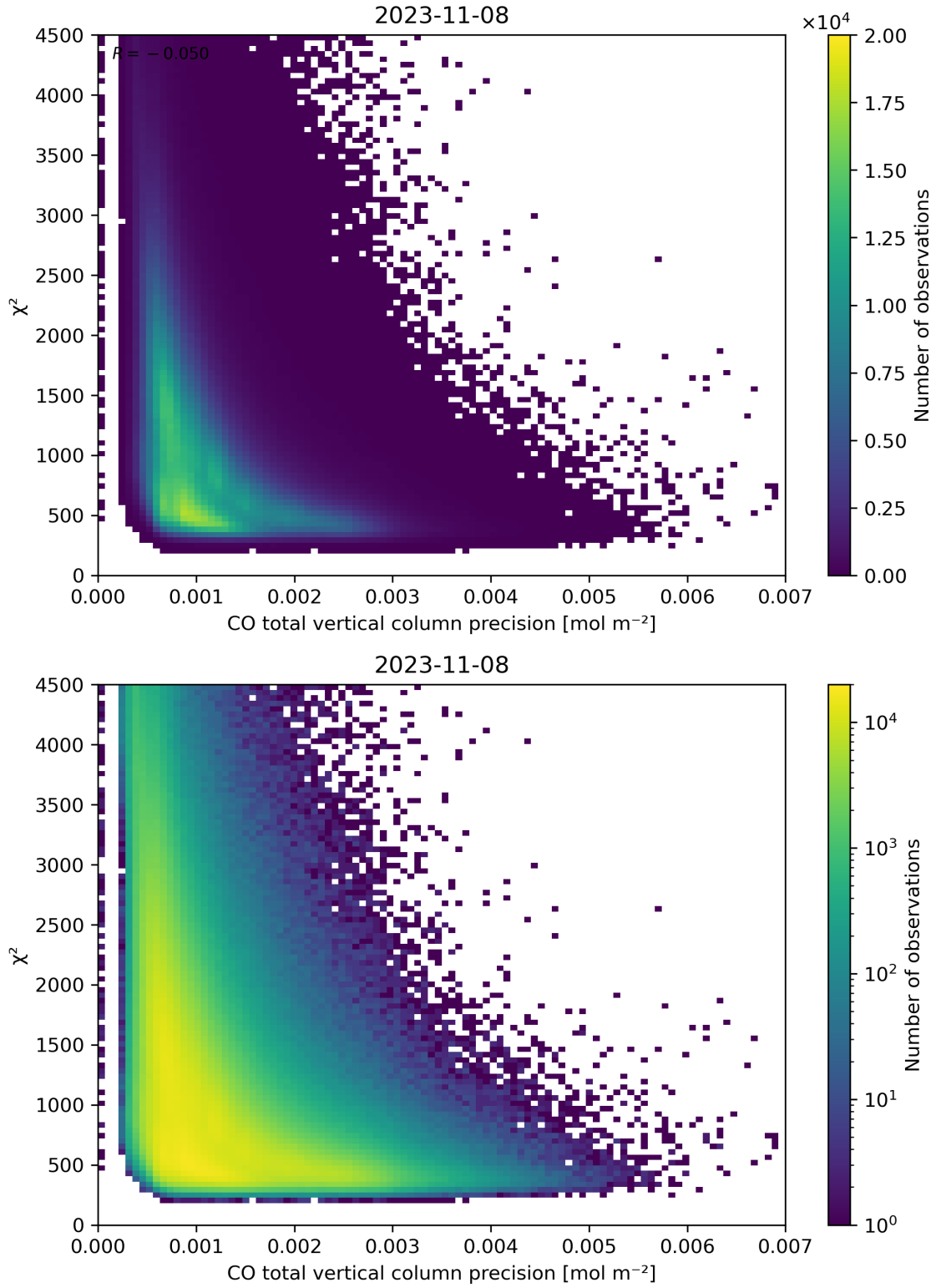
Figure 44: Scatter density plot of “CO total vertical column precision” against “ \chi^2 ” for 2023-11-07 to 2023-11-09.
