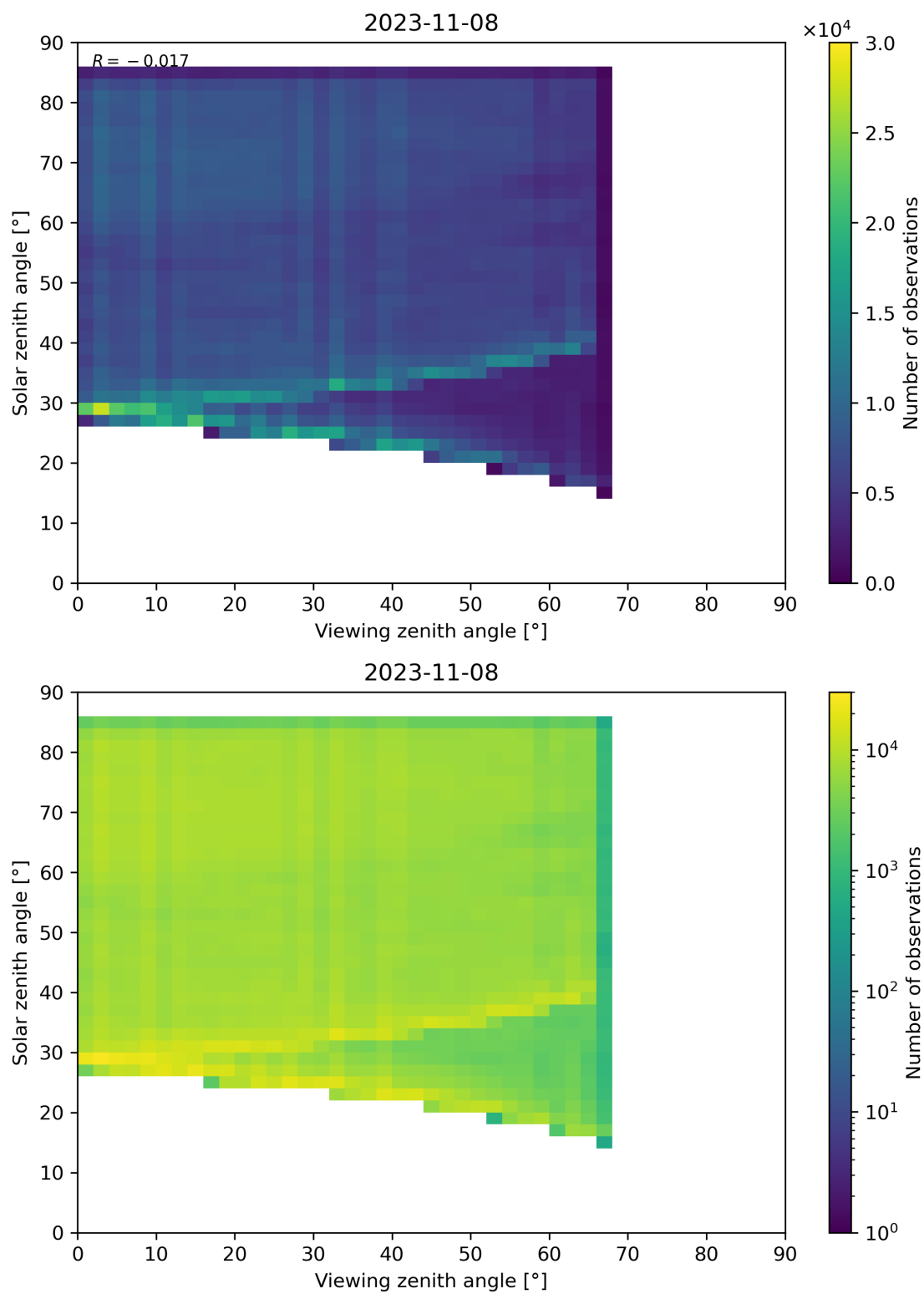
Figure 77: Scatter density plot of “Viewing zenith angle” against “Solar zenith angle” for 2023-11-07 to 2023-11-09.
