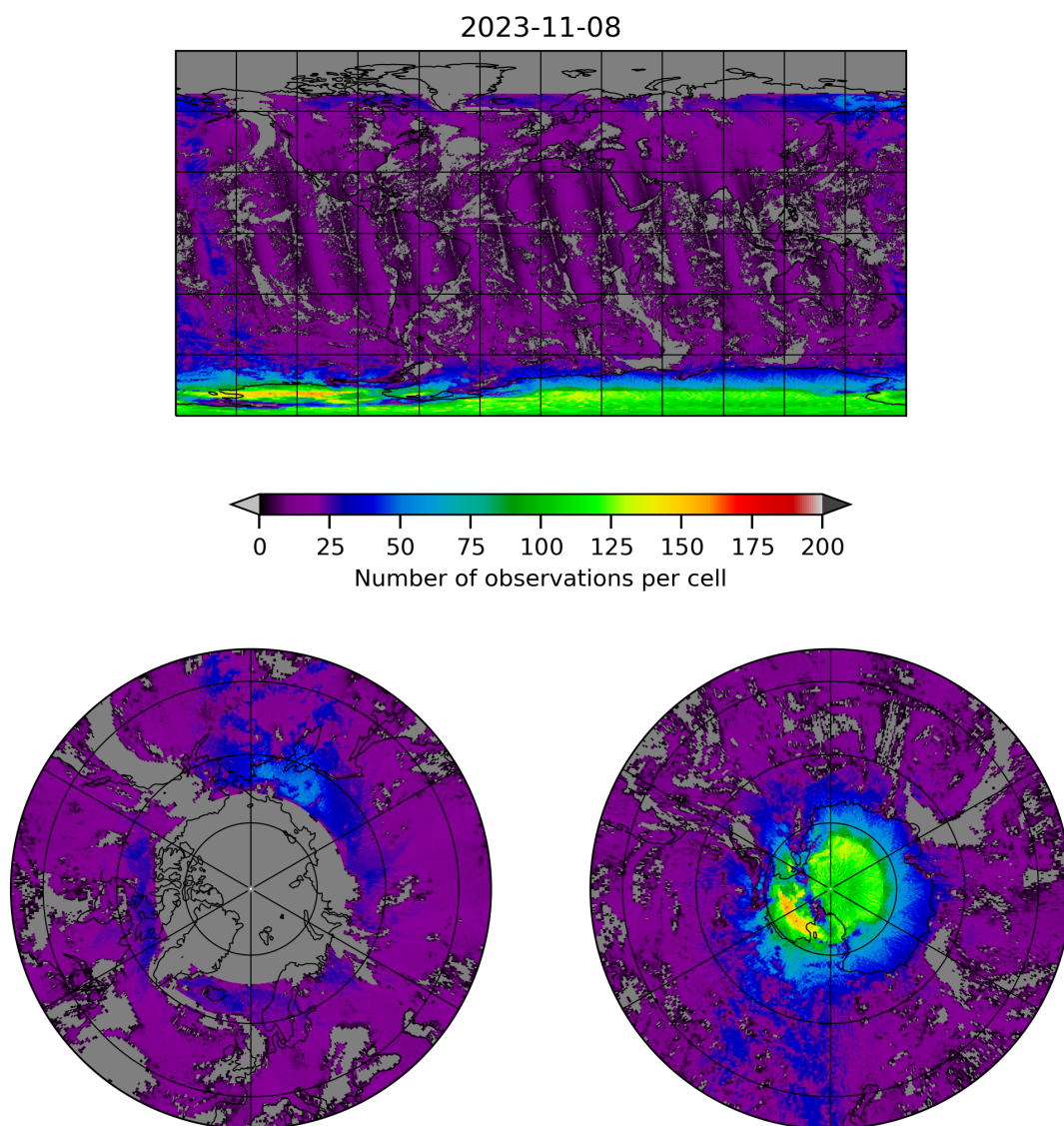
Figure 8: Map of the number of observations for 2023-11-07 to 2023-11-09
