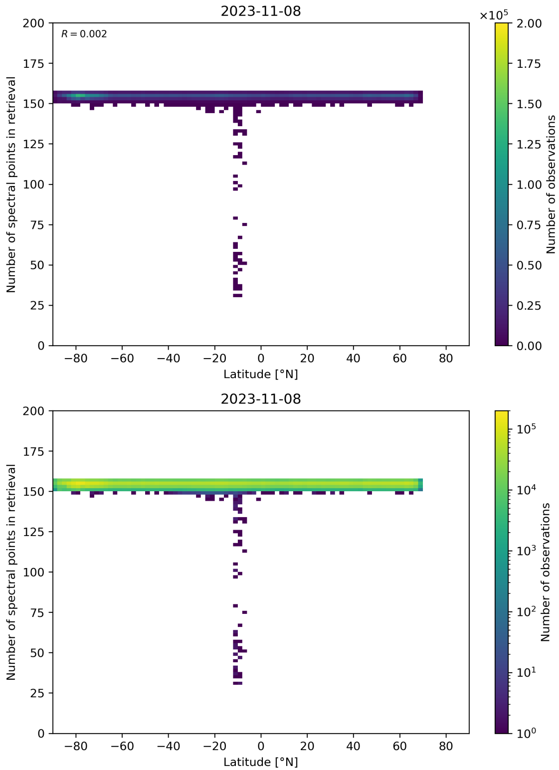
Figure 57: Scatter density plot of “Latitude” against “Number of spectral points in retrieval” for 2023-11-07 to 2023-11-09.
