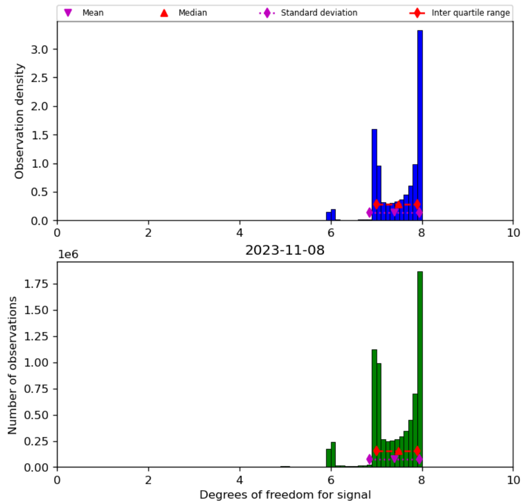
Figure 23: Histogram of “Degrees of freedom for signal” for 2023-11-07 to 2023-11-09
