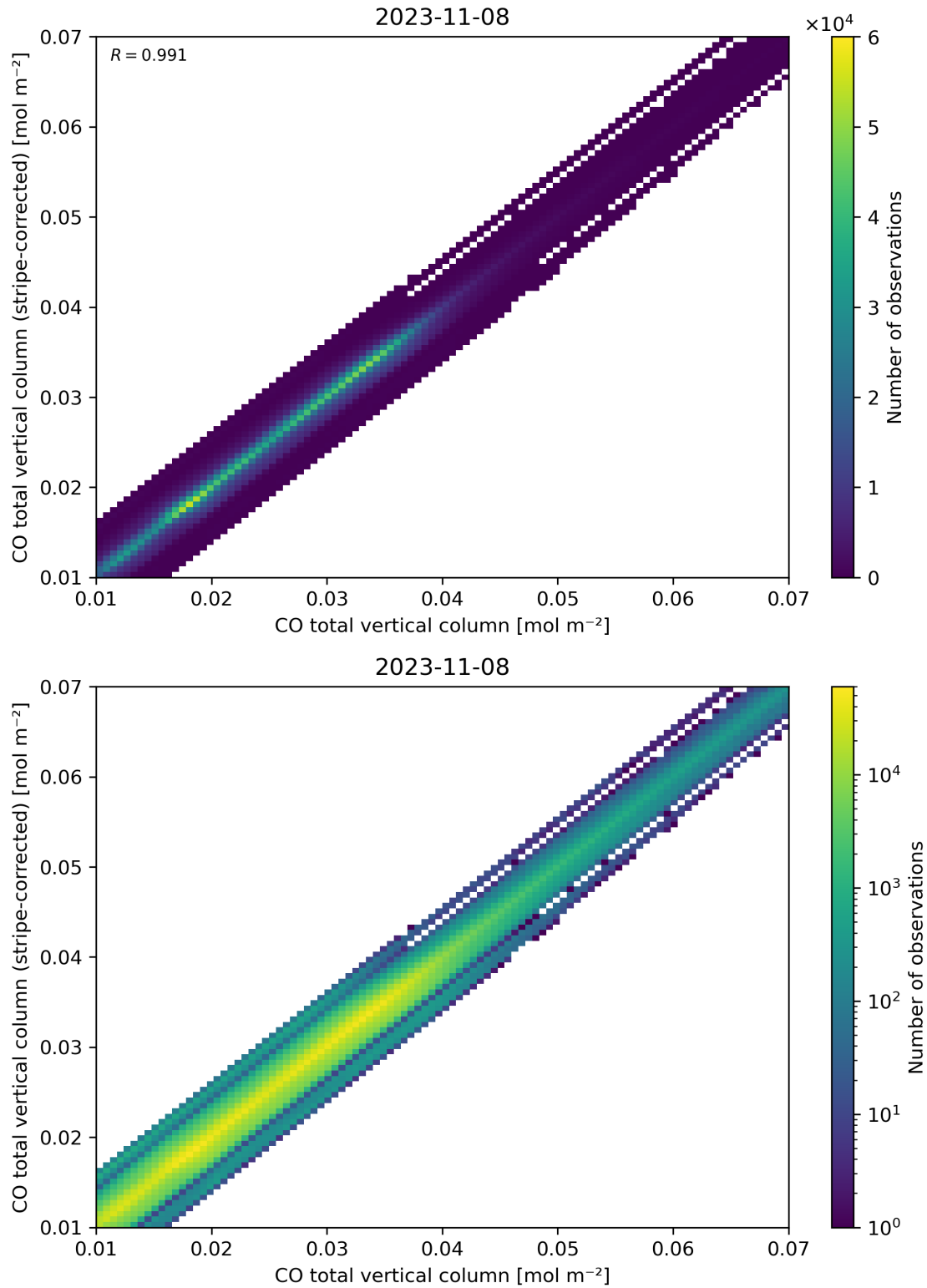
Figure 33: Scatter density plot of “CO total vertical column” against “CO total vertical column (stripe-corrected)” for 2023-11-07 to 2023-11-09.
