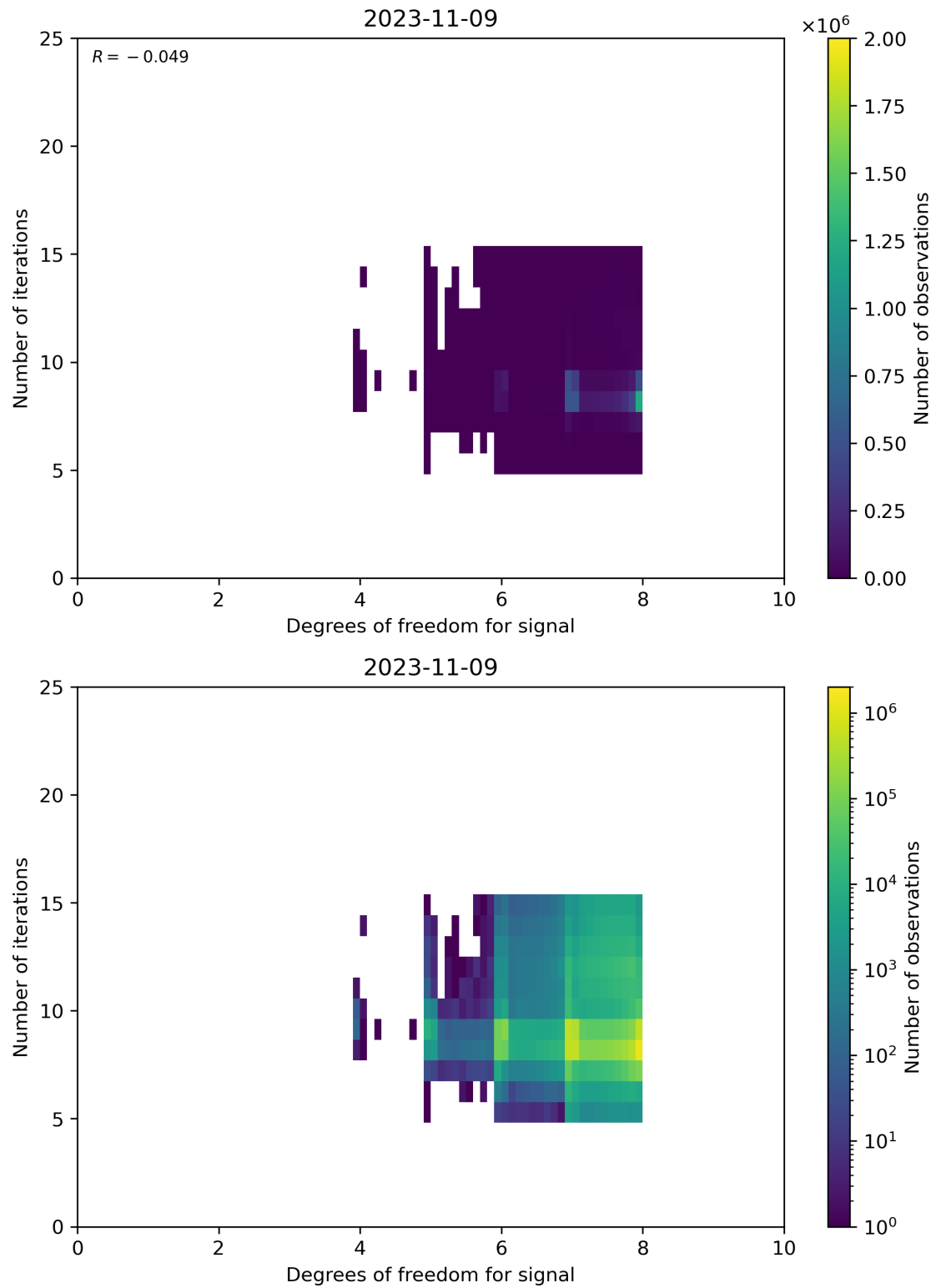
Figure 50: Scatter density plot of “Degrees of freedom for signal” against “Number of iterations” for 2023-11-08 to 2023-11-10.
