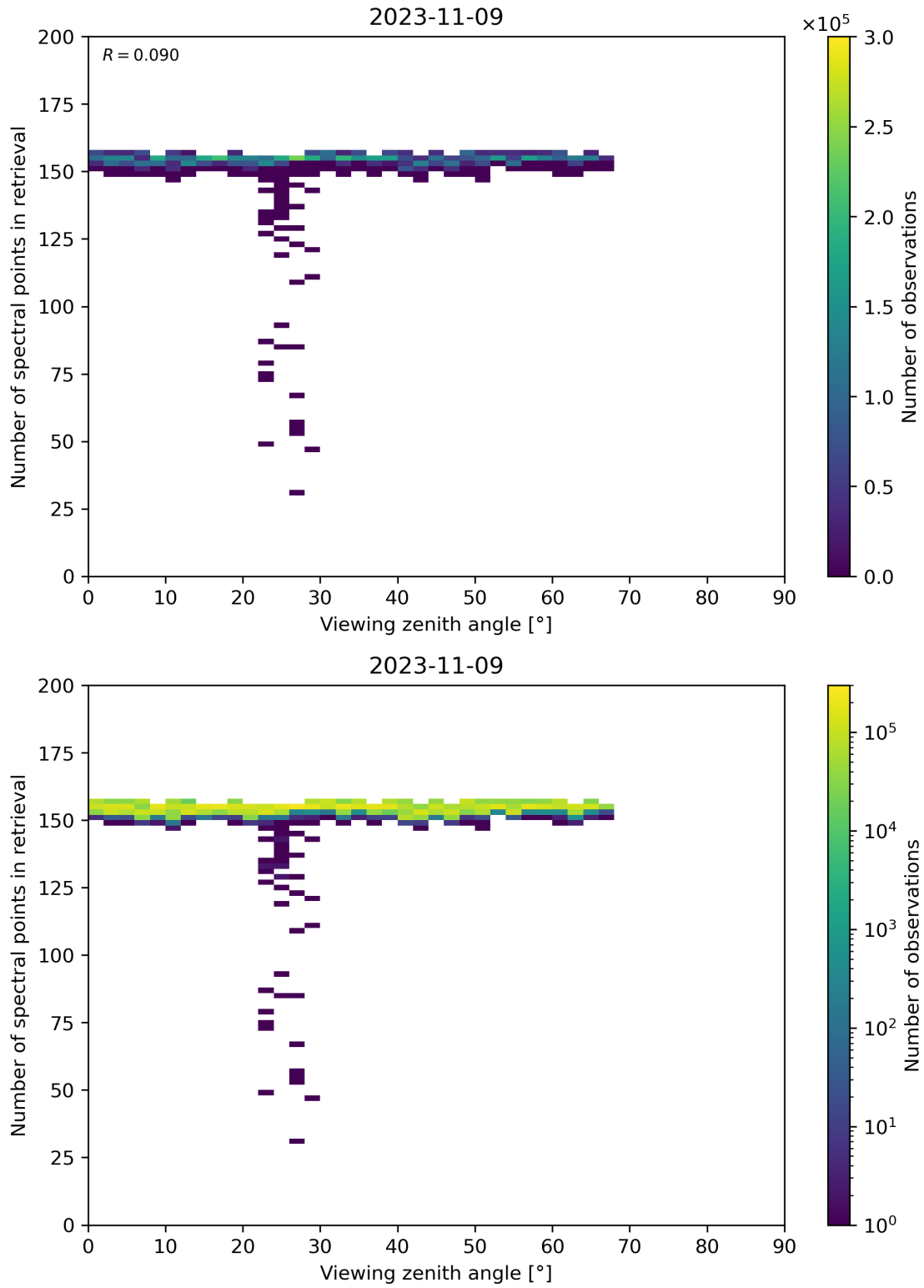
Figure 76: Scatter density plot of “Viewing zenith angle” against “Number of spectral points in retrieval” for 2023-11-08 to 2023-11-10.
