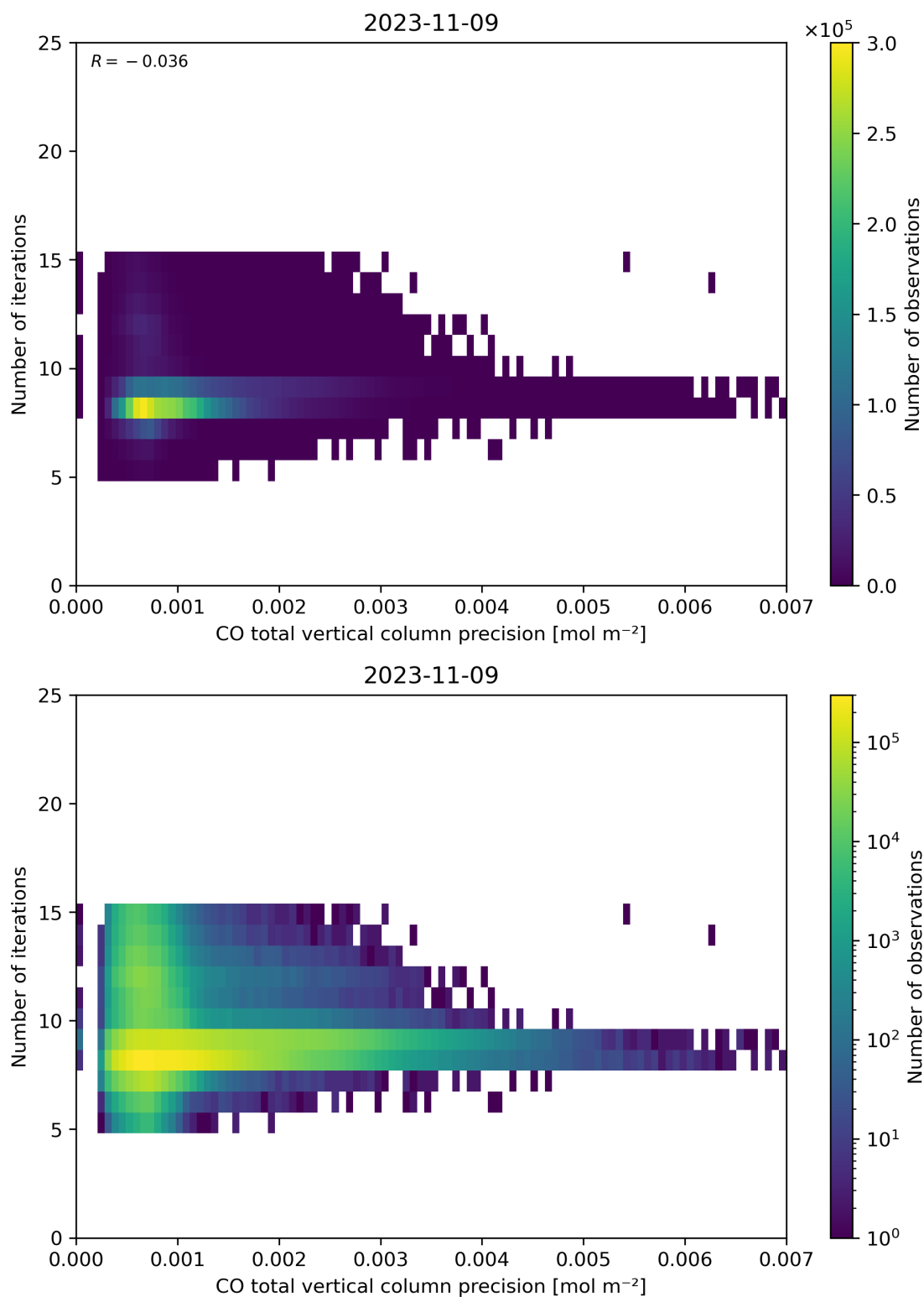
Figure 46: Scatter density plot of “CO total vertical column precision” against “Number of iterations” for 2023-11-08 to 2023-11-10.
