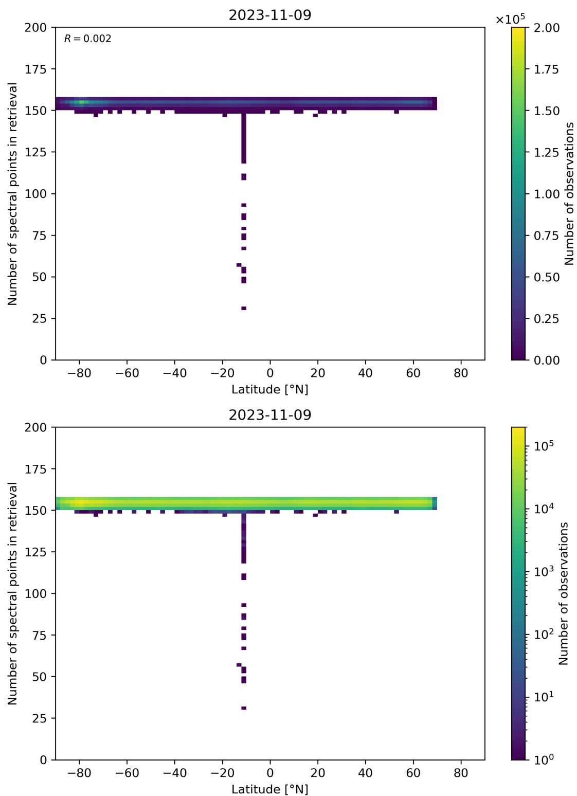
Figure 57: Scatter density plot of “Latitude” against “Number of spectral points in retrieval” for 2023-11-08 to 2023-11-10.
