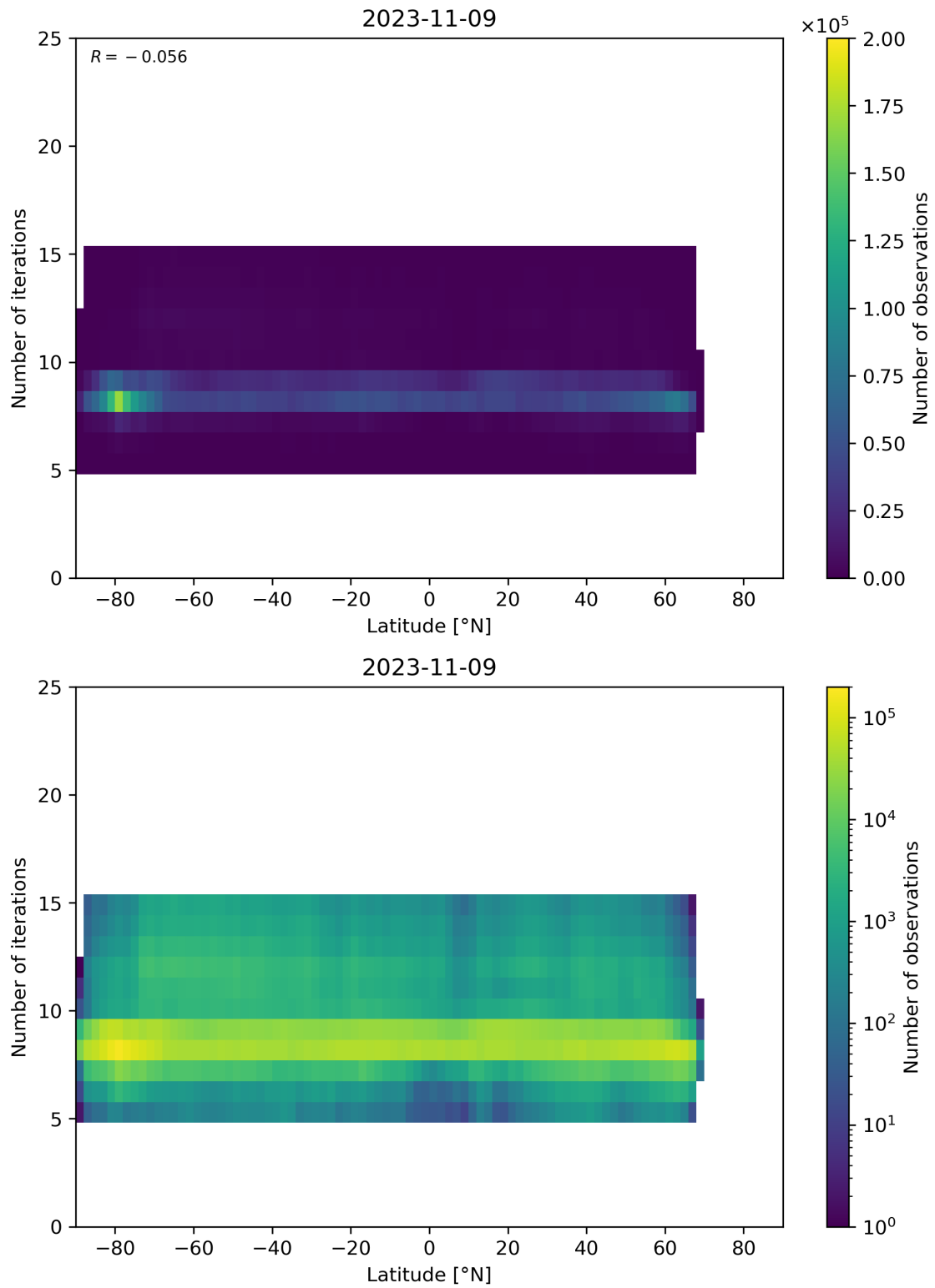
Figure 56: Scatter density plot of “Latitude” against “Number of iterations” for 2023-11-08 to 2023-11-10.
