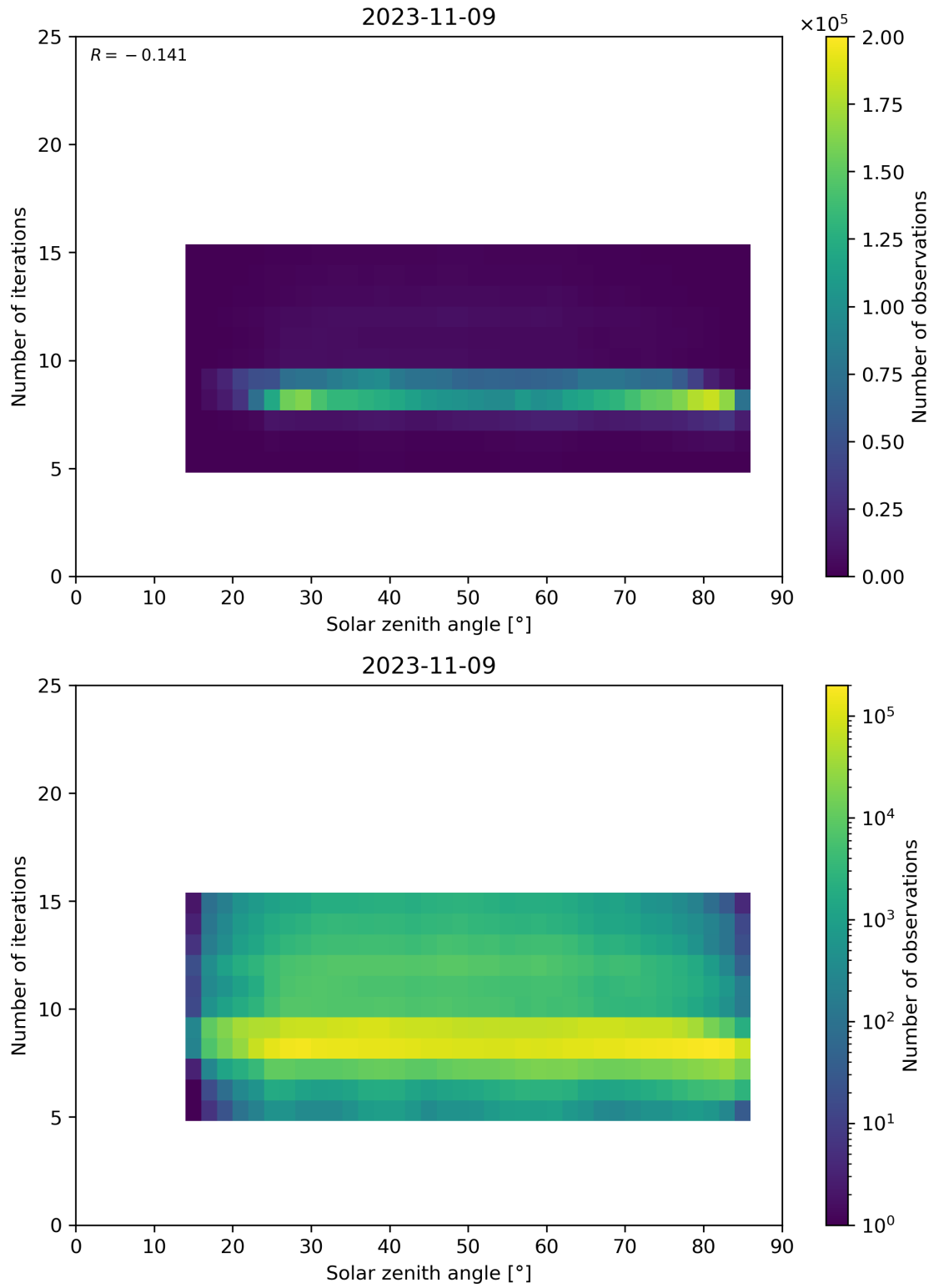
Figure 67: Scatter density plot of “Solar zenith angle” against “Number of iterations” for 2023-11-08 to 2023-11-10.
