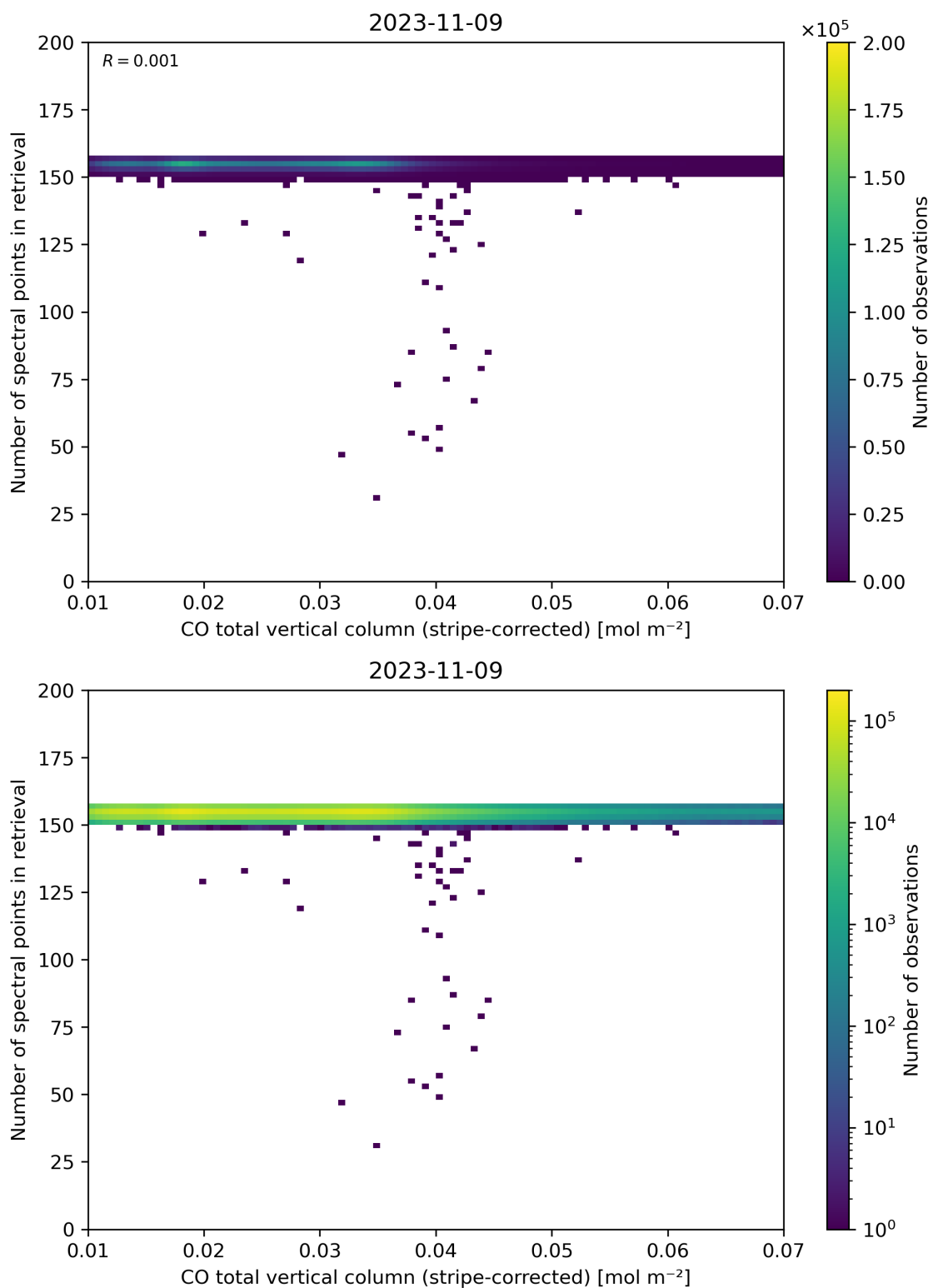
Figure 40: Scatter density plot of “CO total vertical column (stripe-corrected)” against “Number of spectral points in retrieval” for 2023-11-08 to 2023-11-10.
