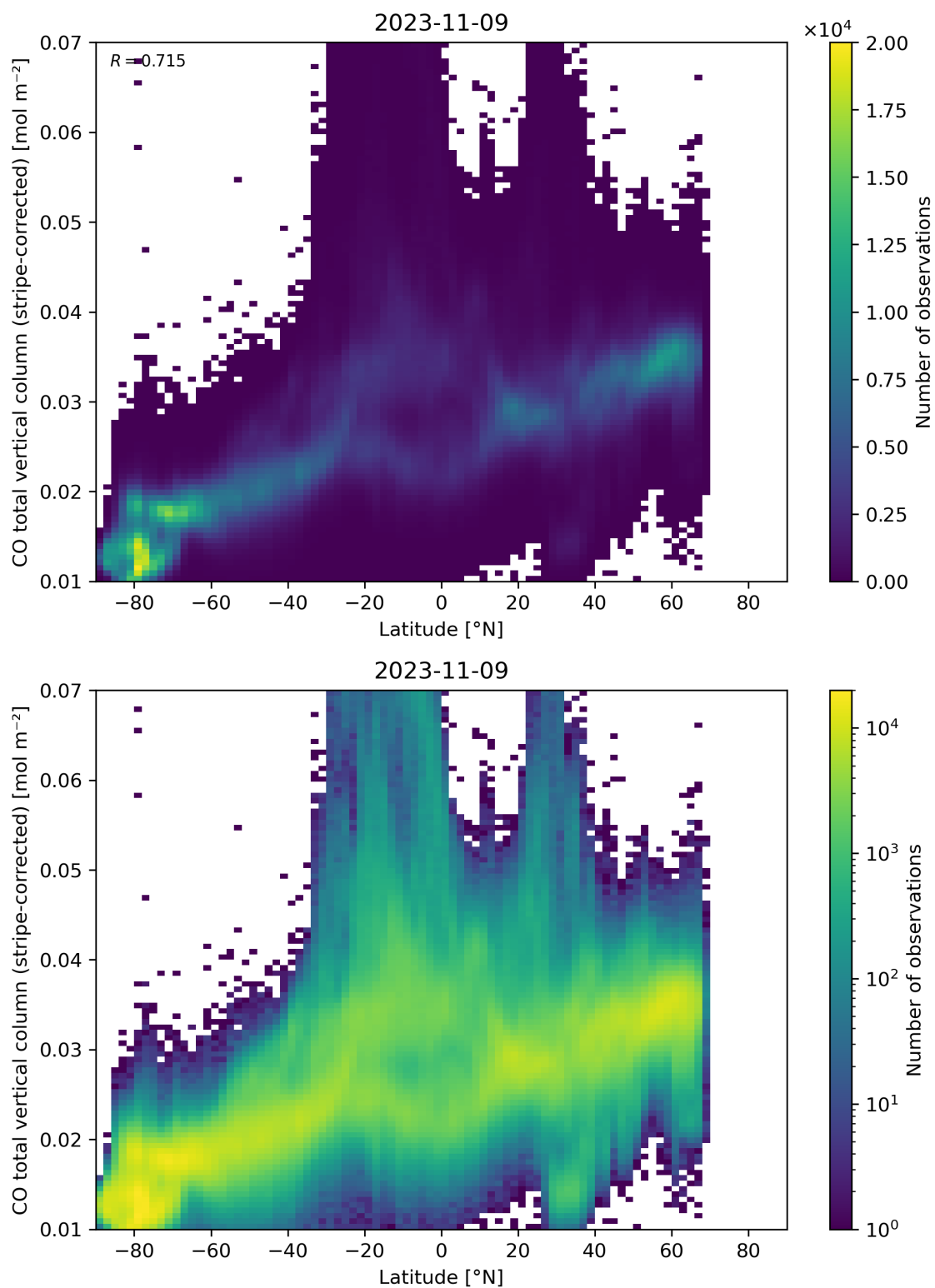
Figure 52: Scatter density plot of “Latitude” against “CO total vertical column (stripe-corrected)” for 2023-11-08 to 2023-11-10.
