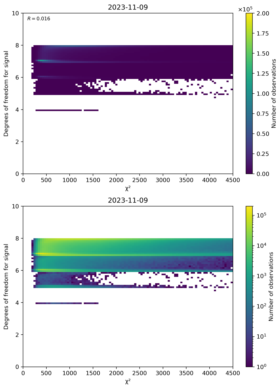
Figure 48: Scatter density plot of “ \chi^2 ” against “Degrees of freedom for signal” for 2023-11-08 to 2023-11-10.
