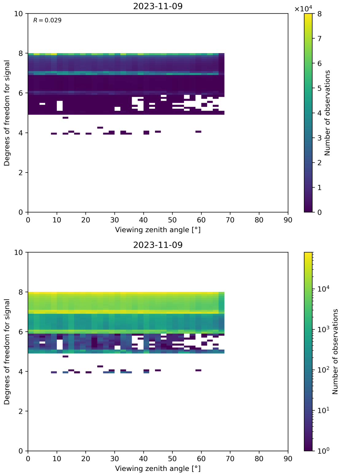
Figure 73: Scatter density plot of “Viewing zenith angle” against “Degrees of freedom for signal” for 2023-11-08 to 2023-11-10.
