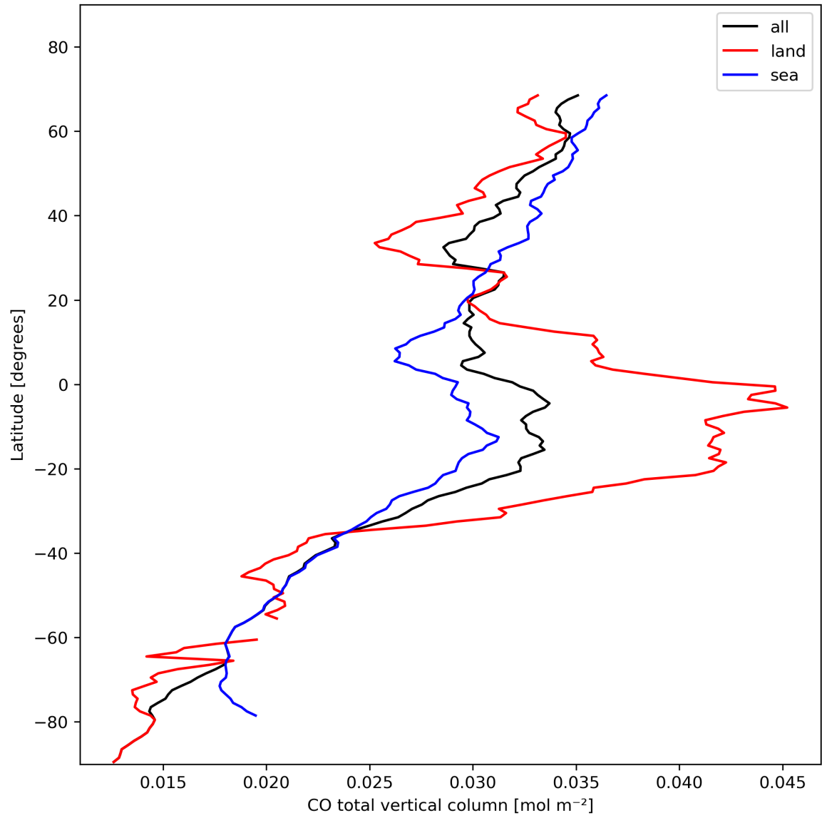
Figure 10: Zonal average of “CO total vertical column” for 2023-11-08 to 2023-11-10.
