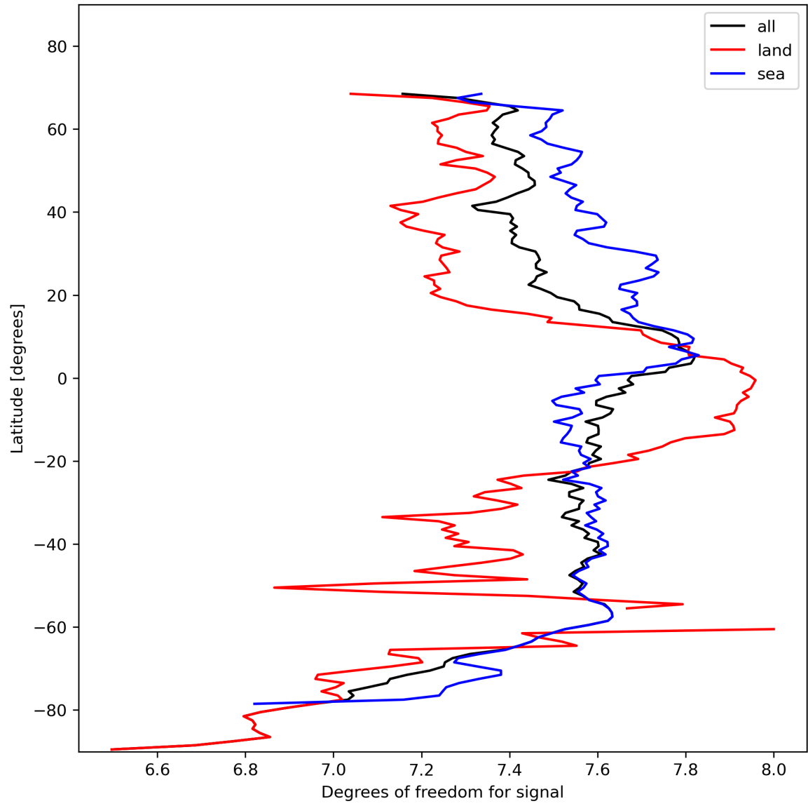
Figure 15: Zonal average of “Degrees of freedom for signal” for 2023-11-08 to 2023-11-10.
