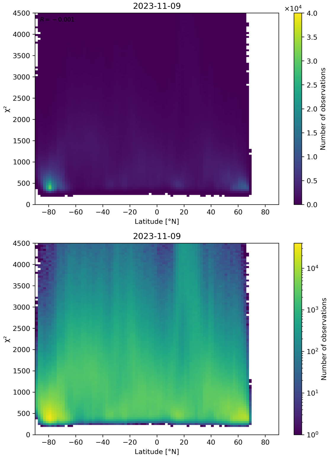
Figure 54: Scatter density plot of “Latitude” against “ \chi^2 ” for 2023-11-08 to 2023-11-10.
