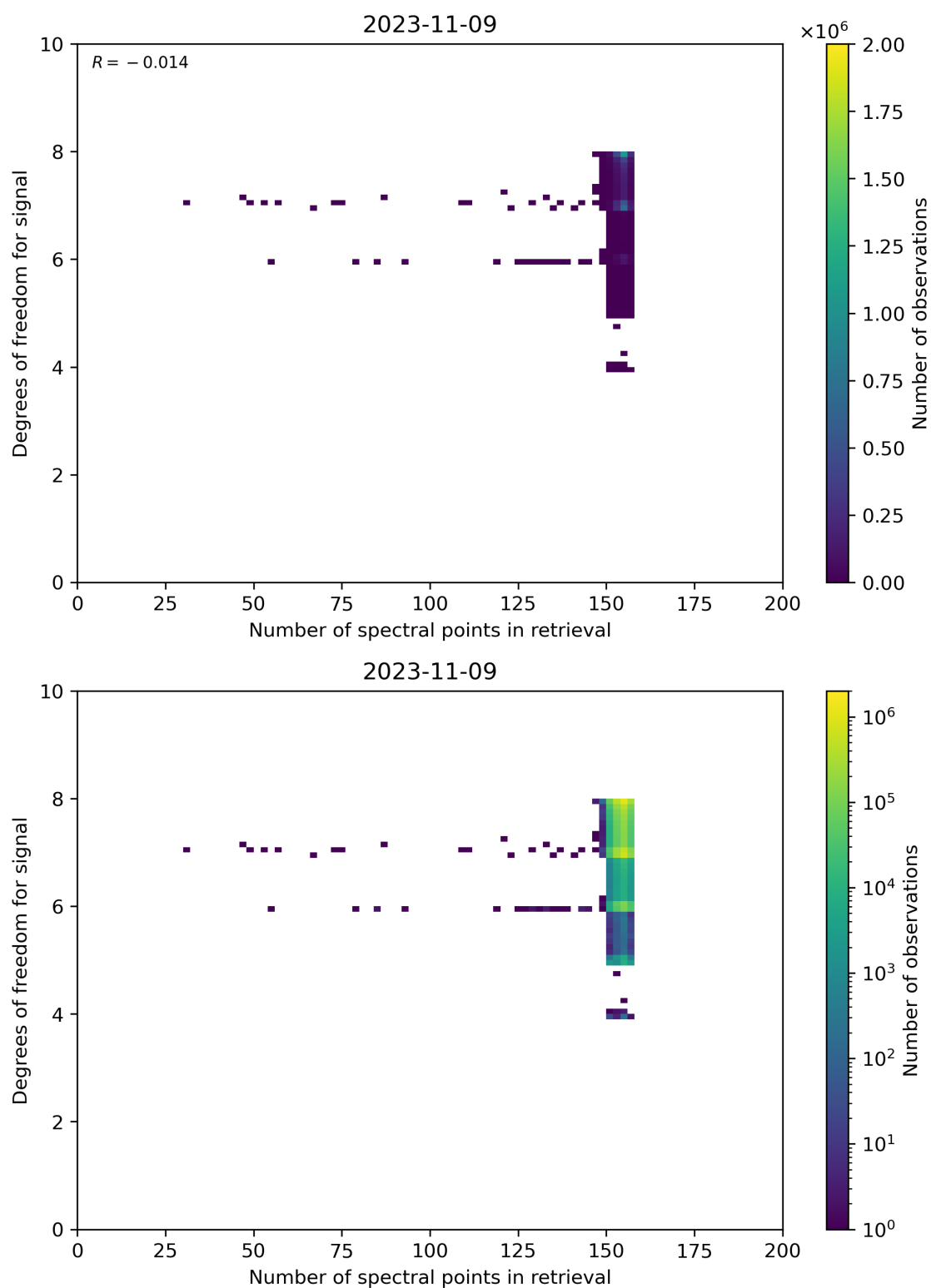
Figure 59: Scatter density plot of “Number of spectral points in retrieval” against “Degrees of freedom for signal” for 2023-11-08 to 2023-11-10.
