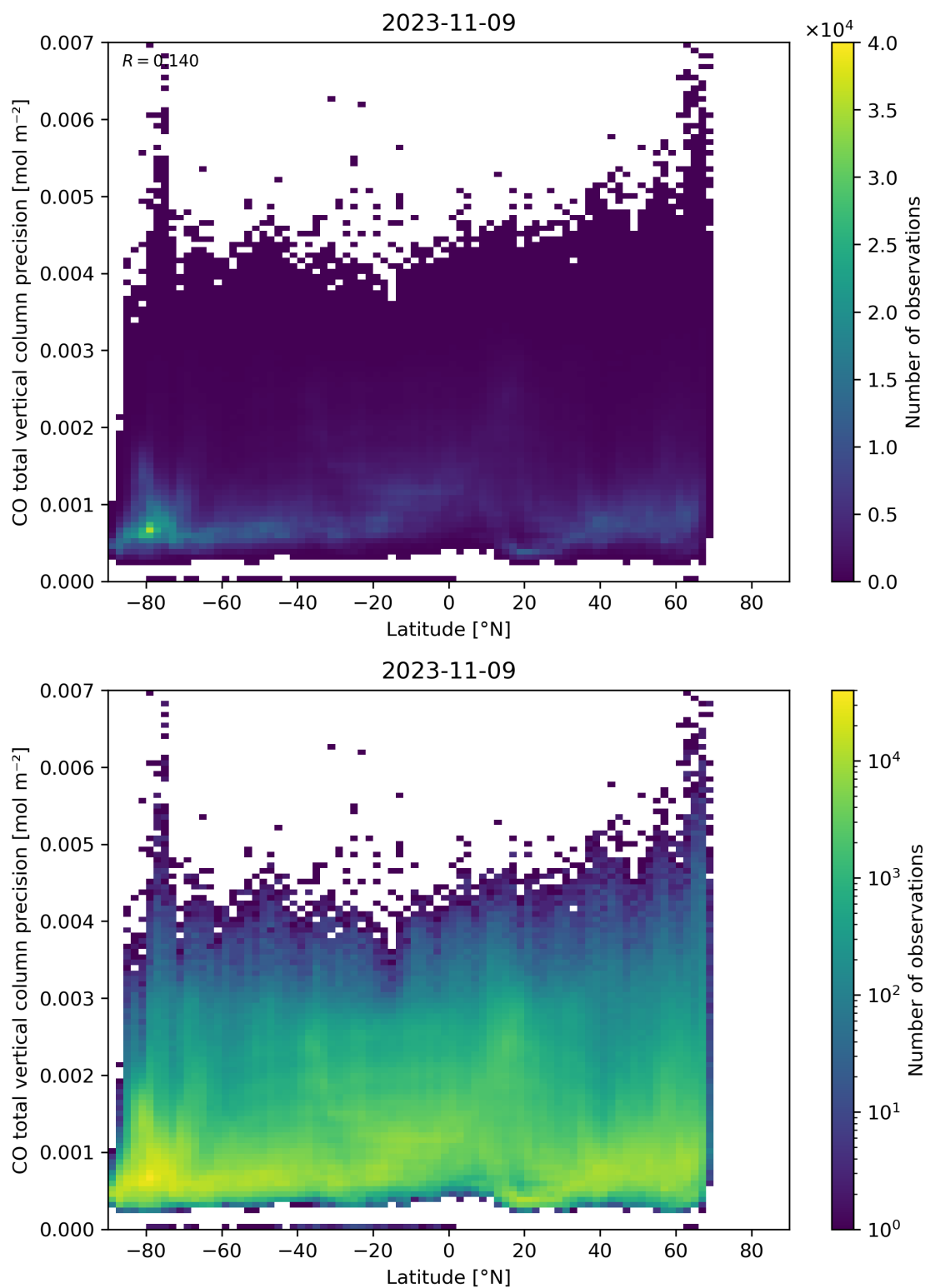
Figure 53: Scatter density plot of “Latitude” against “CO total vertical column precision” for 2023-11-08 to 2023-11-10.
