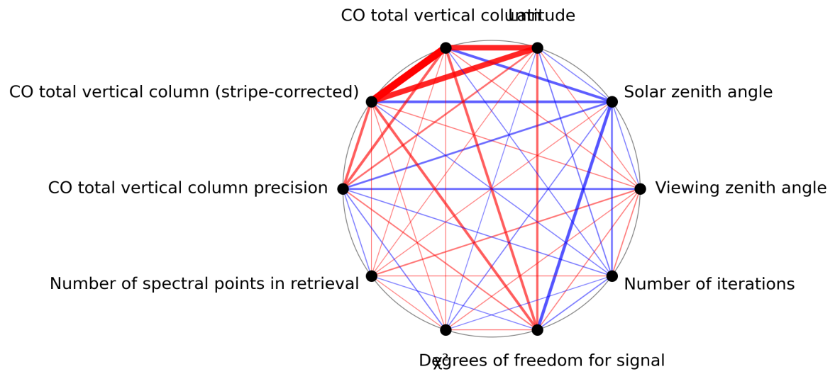
Figure 1: Map of correlation graph for 2023-11-08 to 2023-11-10.
