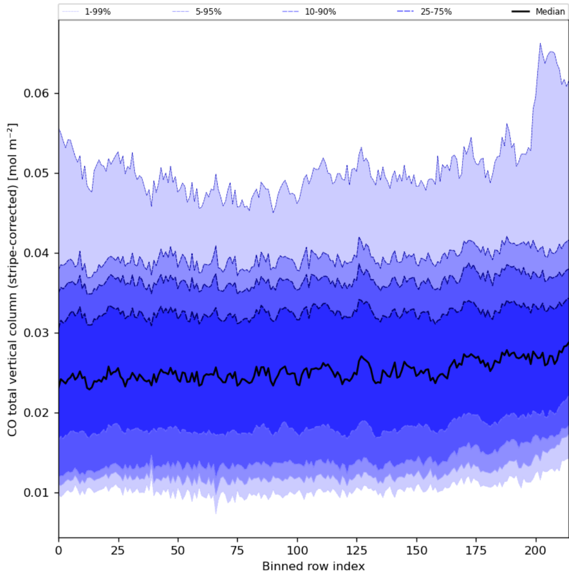
Figure 27: Along track statistics of “CO total vertical column (stripe-corrected)” for 2023-11-08 to 2023-11-10
