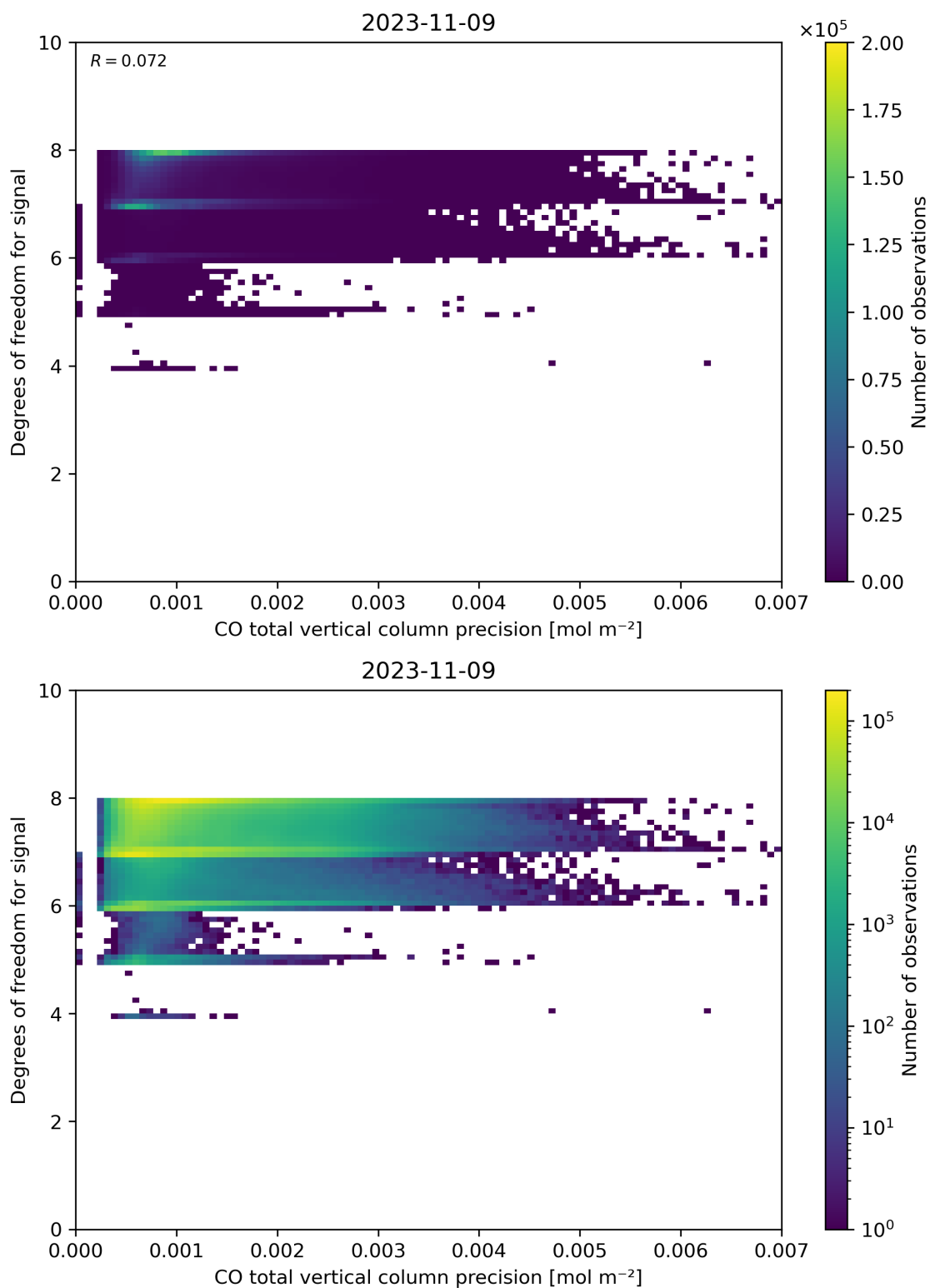
Figure 45: Scatter density plot of “CO total vertical column precision” against “Degrees of freedom for signal” for 2023-11-08 to 2023-11-10.
