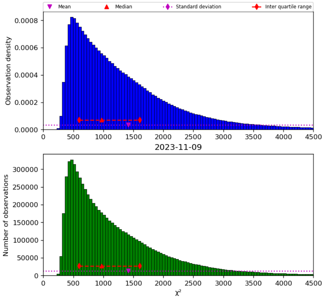
Figure 22: Histogram of “ \chi^2 ” for 2023-11-08 to 2023-11-10
