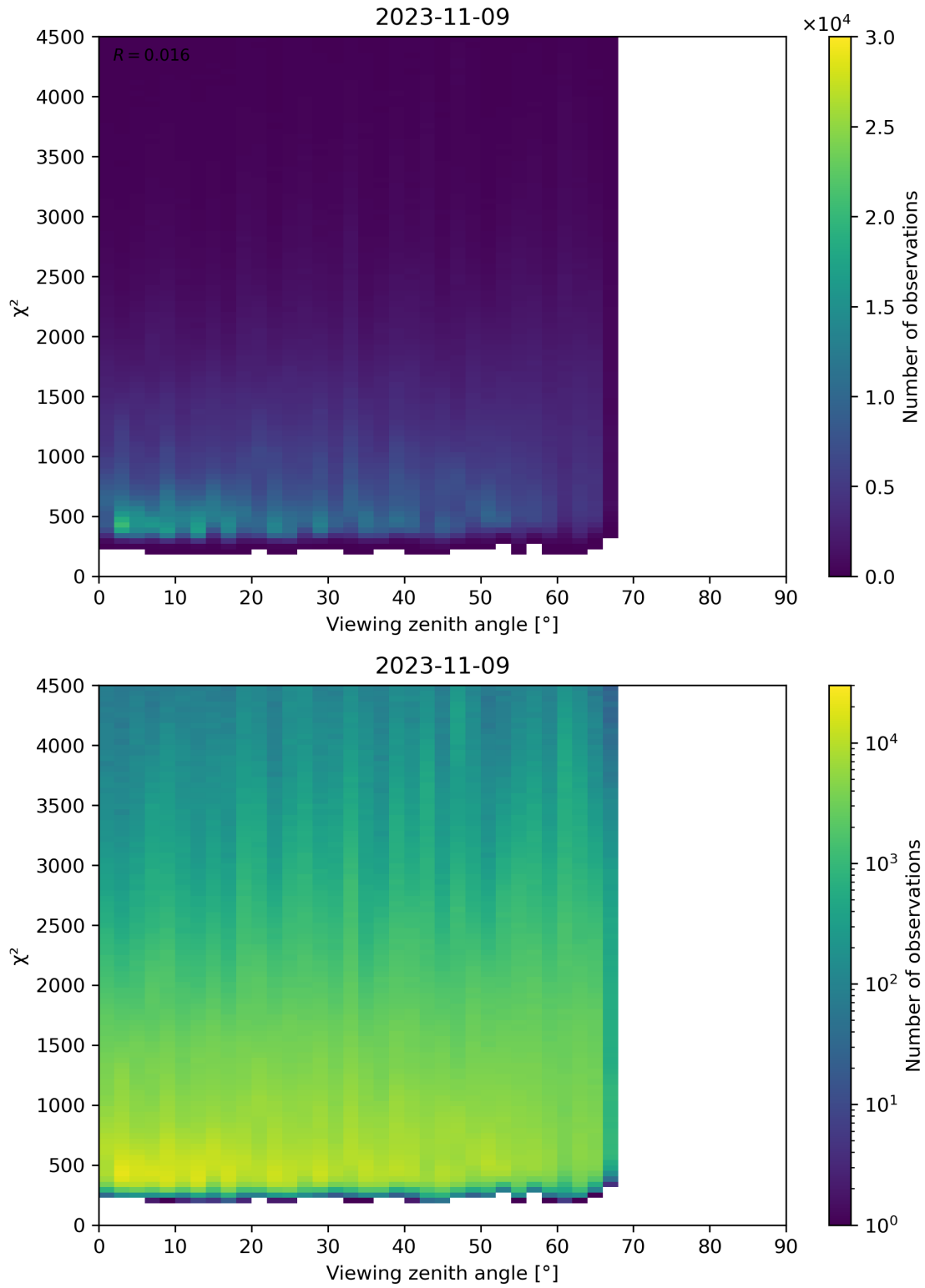
Figure 72: Scatter density plot of “Viewing zenith angle” against “ \chi^2 ” for 2023-11-08 to 2023-11-10.
