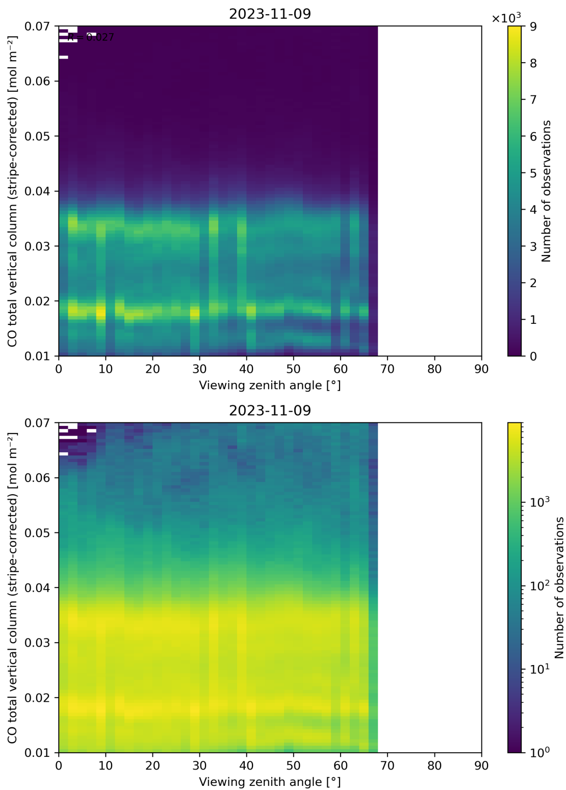
Figure 70: Scatter density plot of “Viewing zenith angle” against “CO total vertical column (stripe-corrected)” for 2023-11-08 to 2023-11-10.
