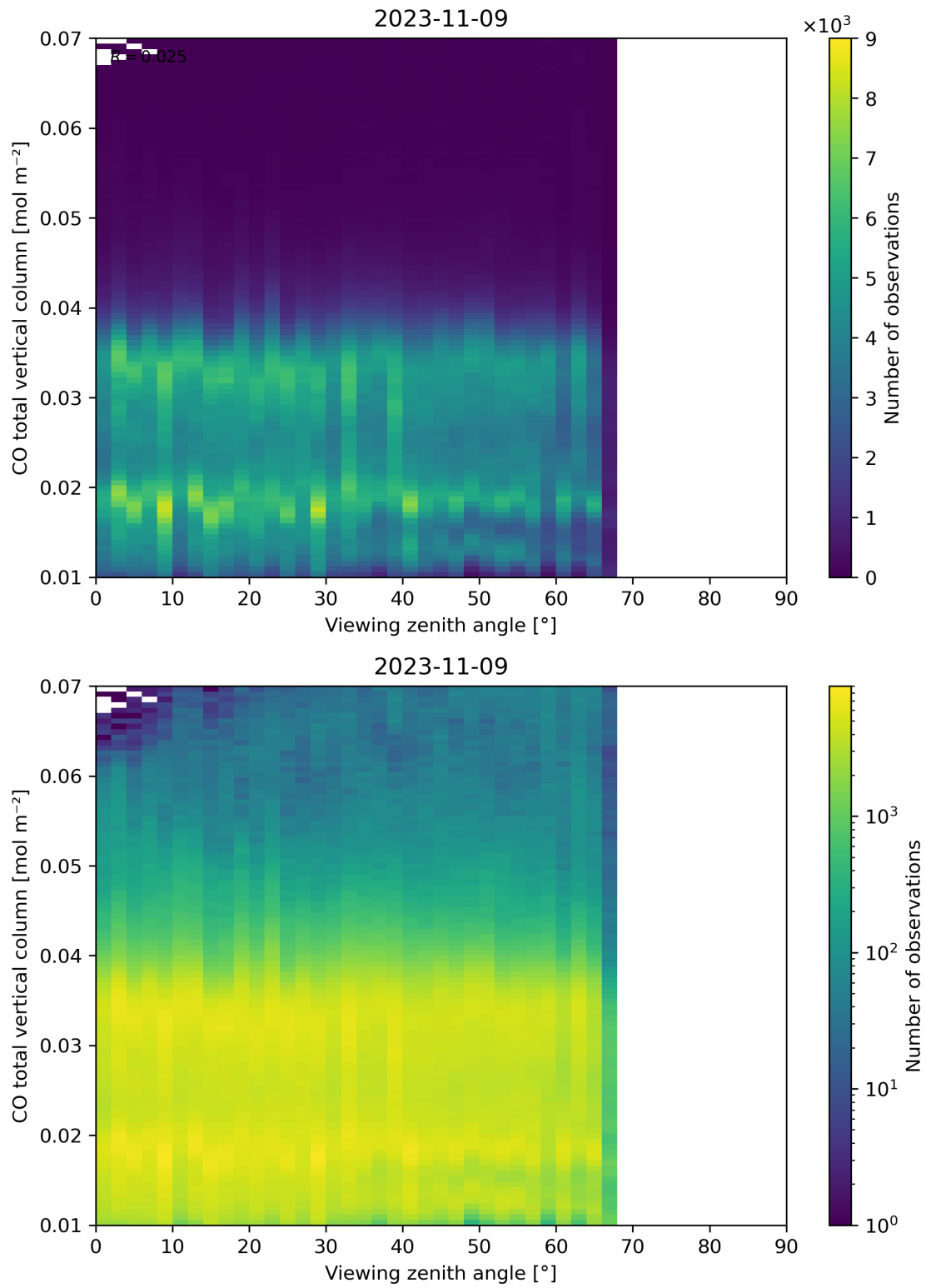
Figure 69: Scatter density plot of “Viewing zenith angle” against “CO total vertical column” for 2023-11-08 to 2023-11-10.
