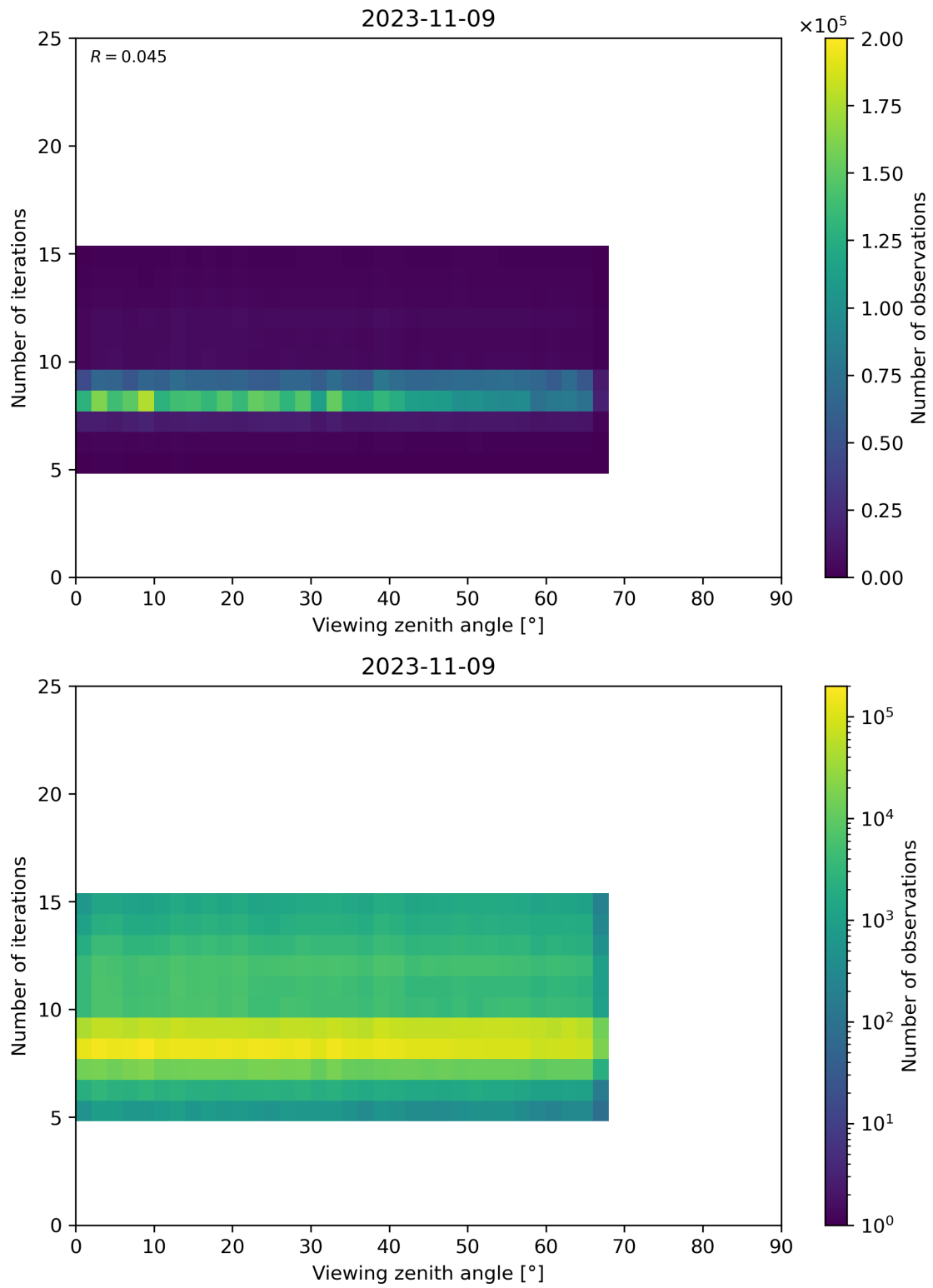
Figure 75: Scatter density plot of “Viewing zenith angle” against “Number of iterations” for 2023-11-08 to 2023-11-10.
