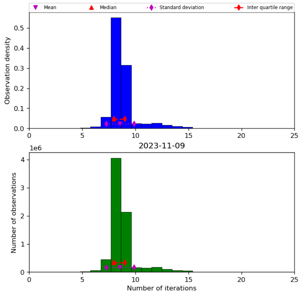
Figure 24: Histogram of “Number of iterations” for 2023-11-08 to 2023-11-10
