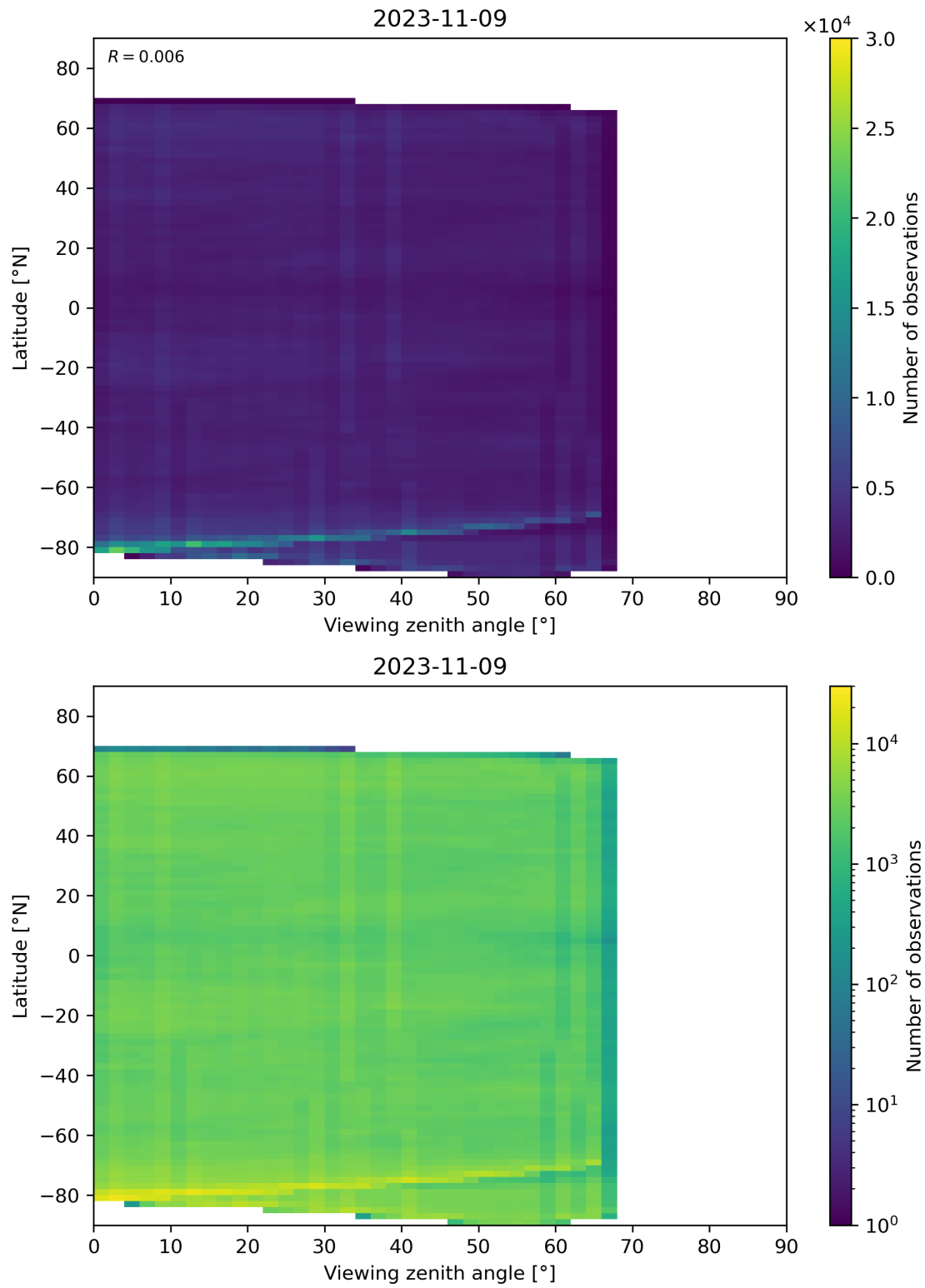
Figure 74: Scatter density plot of “Viewing zenith angle” against “Latitude” for 2023-11-08 to 2023-11-10.
