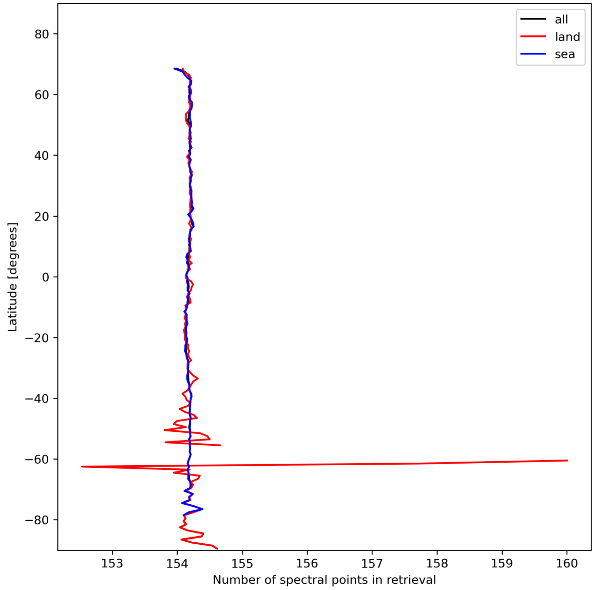
Figure 13: Zonal average of “Number of spectral points in retrieval” for 2023-11-08 to 2023-11-10.
