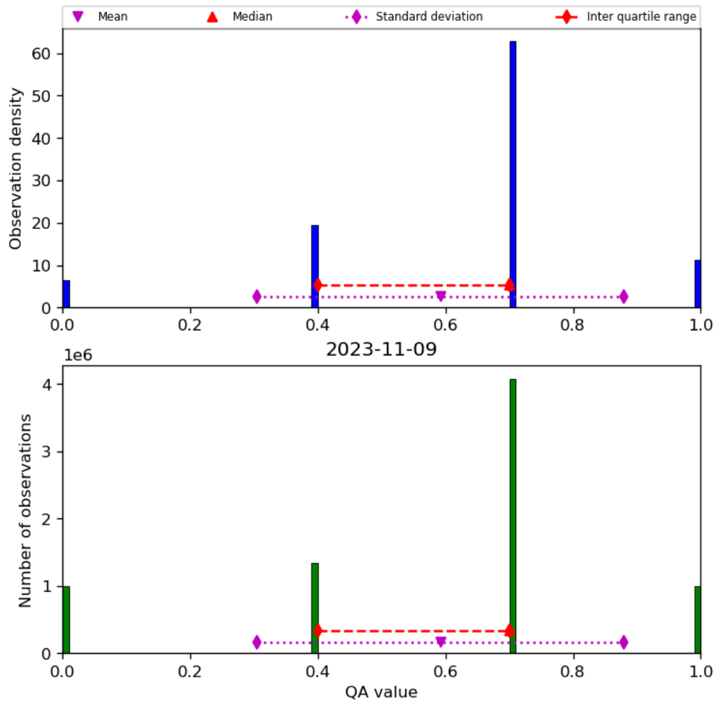
Figure 17: Histogram of “QA value” for 2023-11-08 to 2023-11-10
