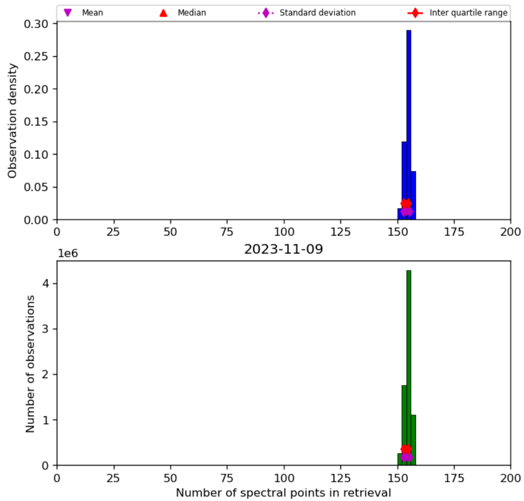
Figure 21: Histogram of “Number of spectral points in retrieval” for 2023-11-08 to 2023-11-10
