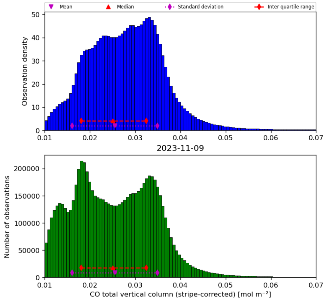
Figure 19: Histogram of “CO total vertical column (stripe-corrected)” for 2023-11-08 to 2023-11-10
