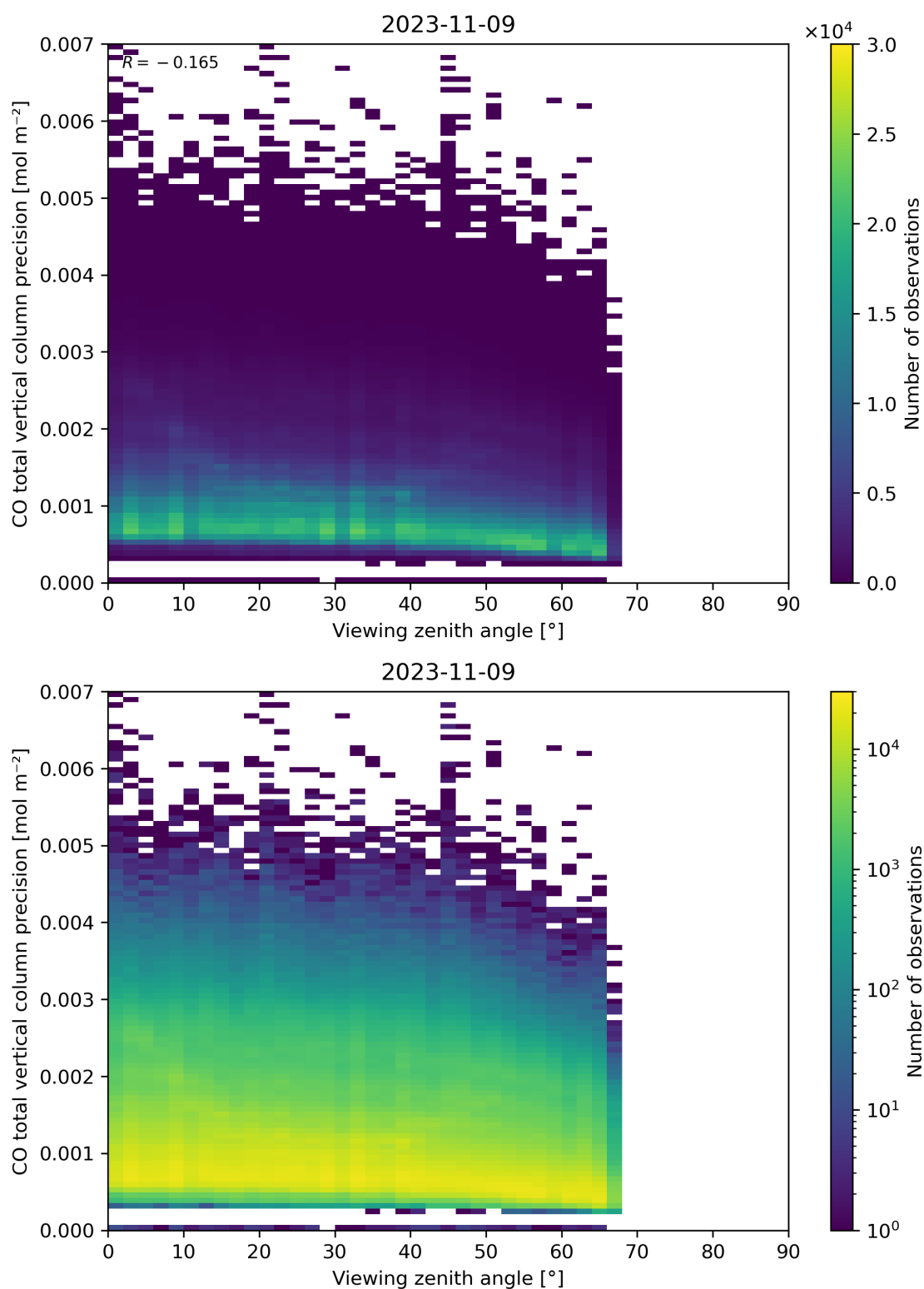
Figure 71: Scatter density plot of “Viewing zenith angle” against “CO total vertical column precision” for 2023-11-08 to 2023-11-10.
