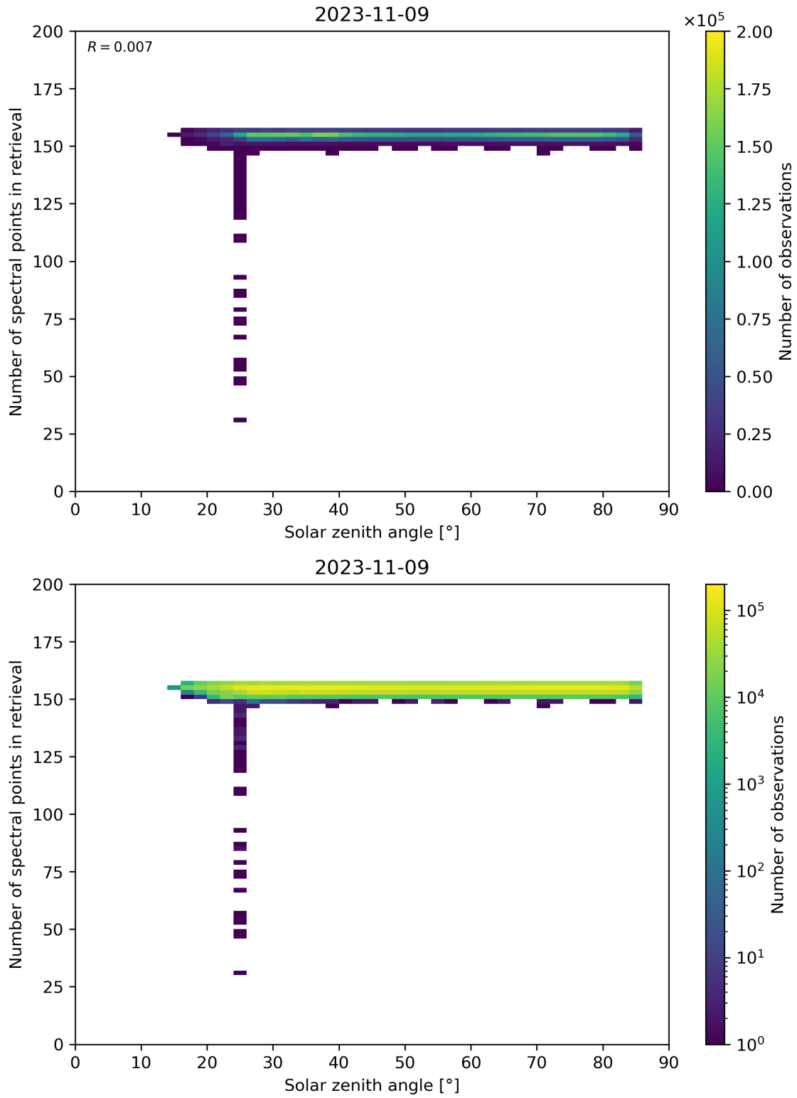
Figure 68: Scatter density plot of “Solar zenith angle” against “Number of spectral points in retrieval” for 2023-11-08 to 2023-11-10.
