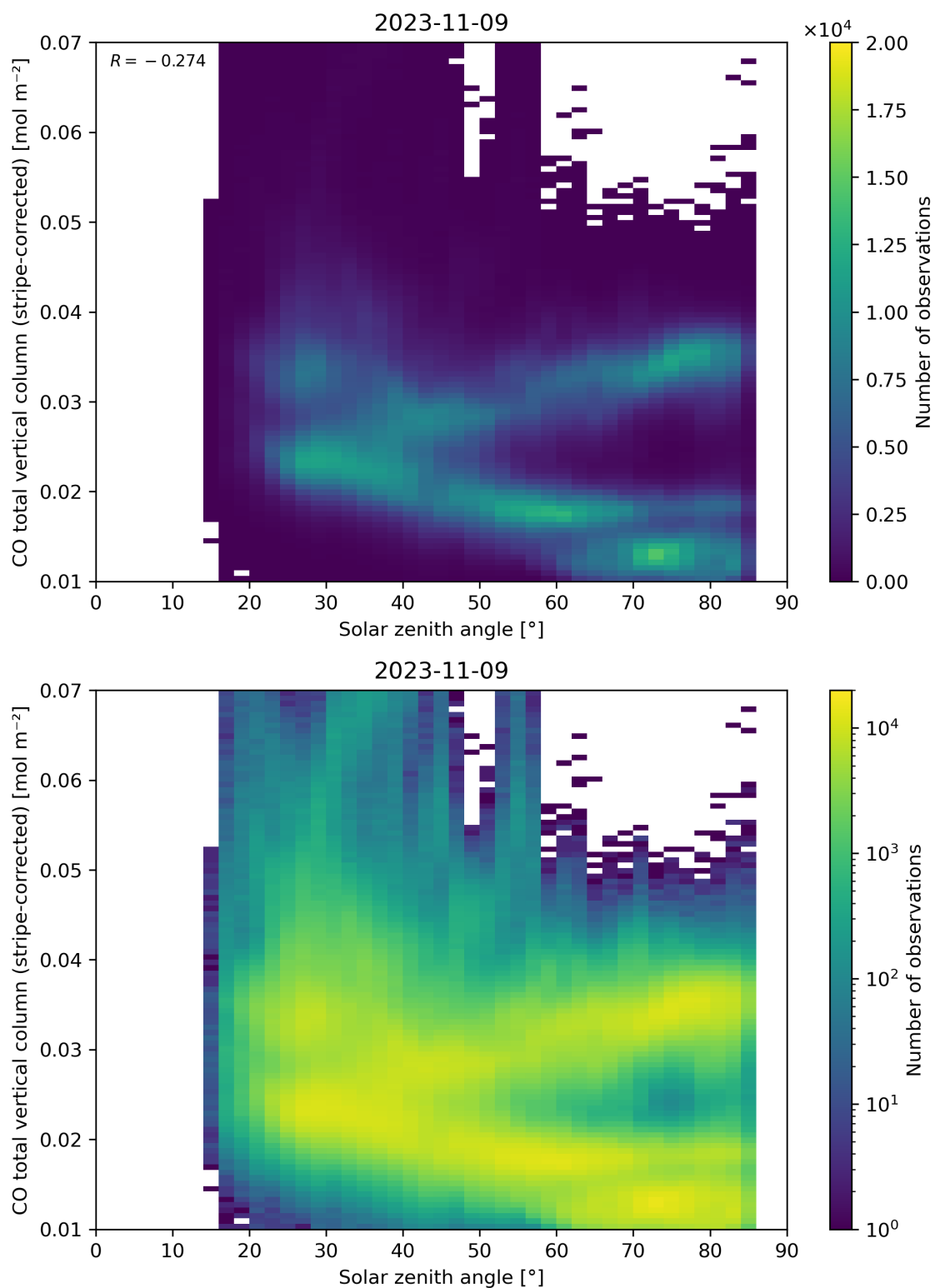
Figure 62: Scatter density plot of “Solar zenith angle” against “CO total vertical column (stripe-corrected)” for 2023-11-08 to 2023-11-10.
