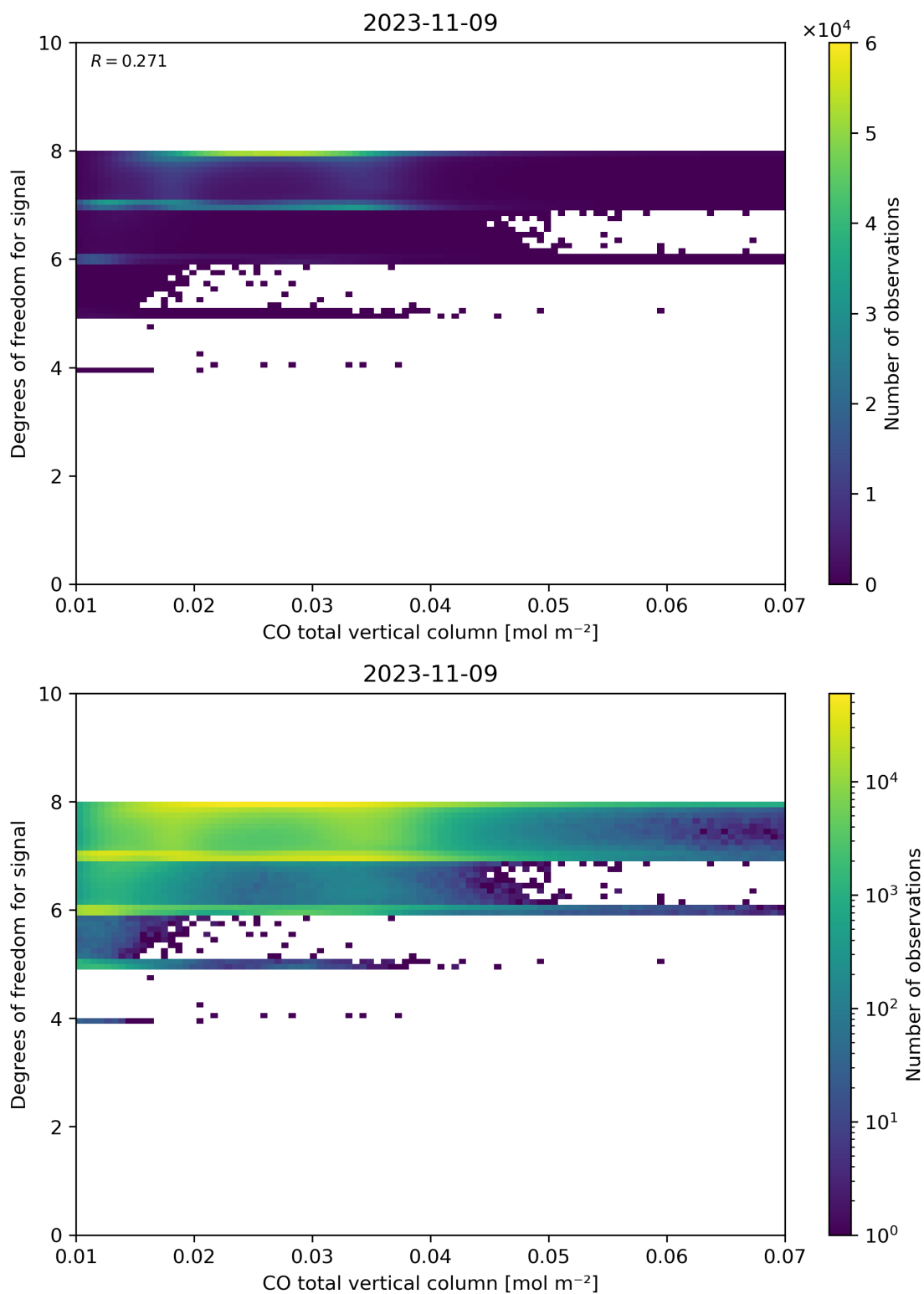
Figure 41: Scatter density plot of “CO total vertical column” against “Degrees of freedom for signal” for 2023-11-08 to 2023-11-10.
