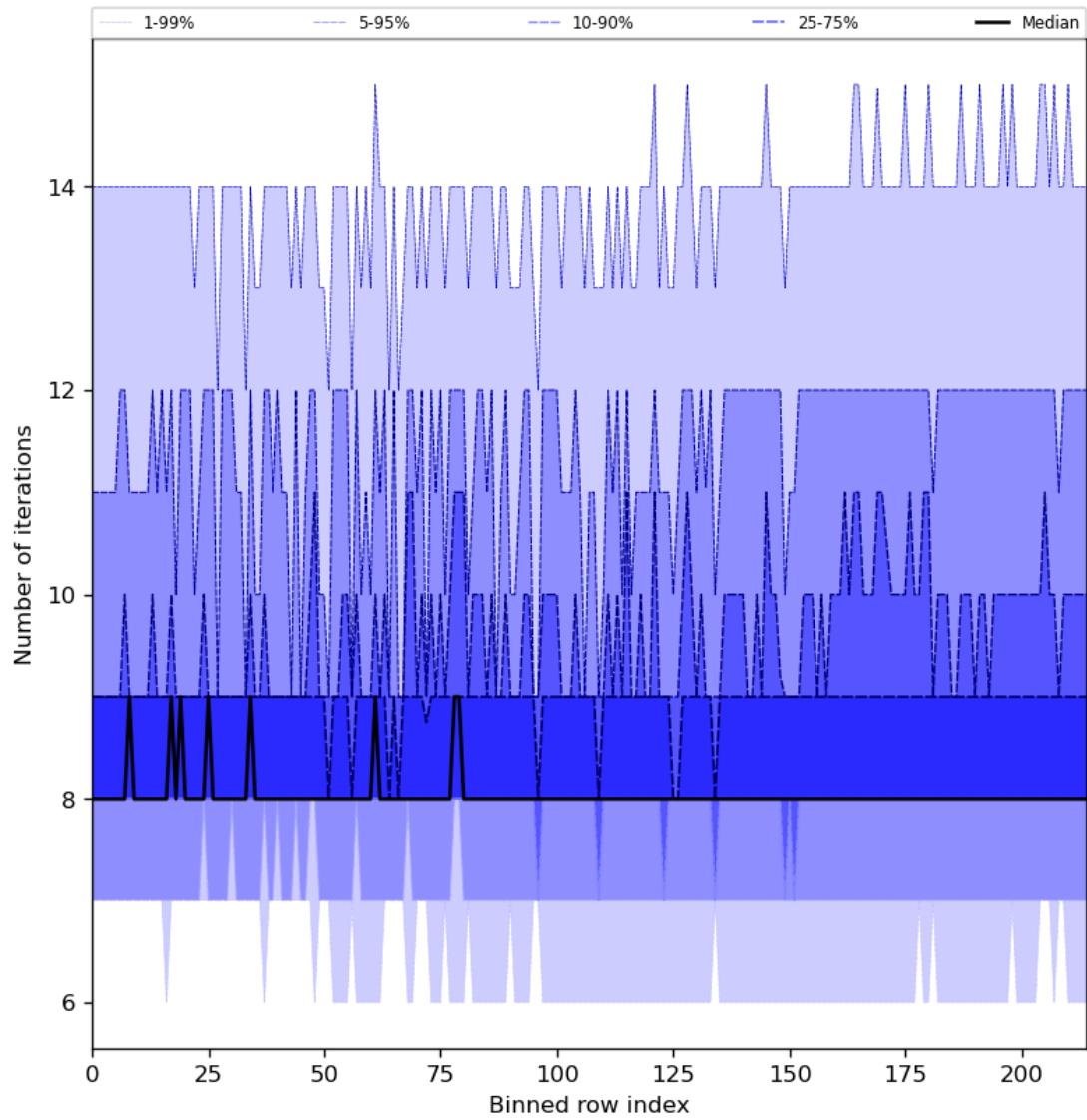
Figure 32: Along track statistics of “Number of iterations” for 2023-11-08 to 2023-11-10
