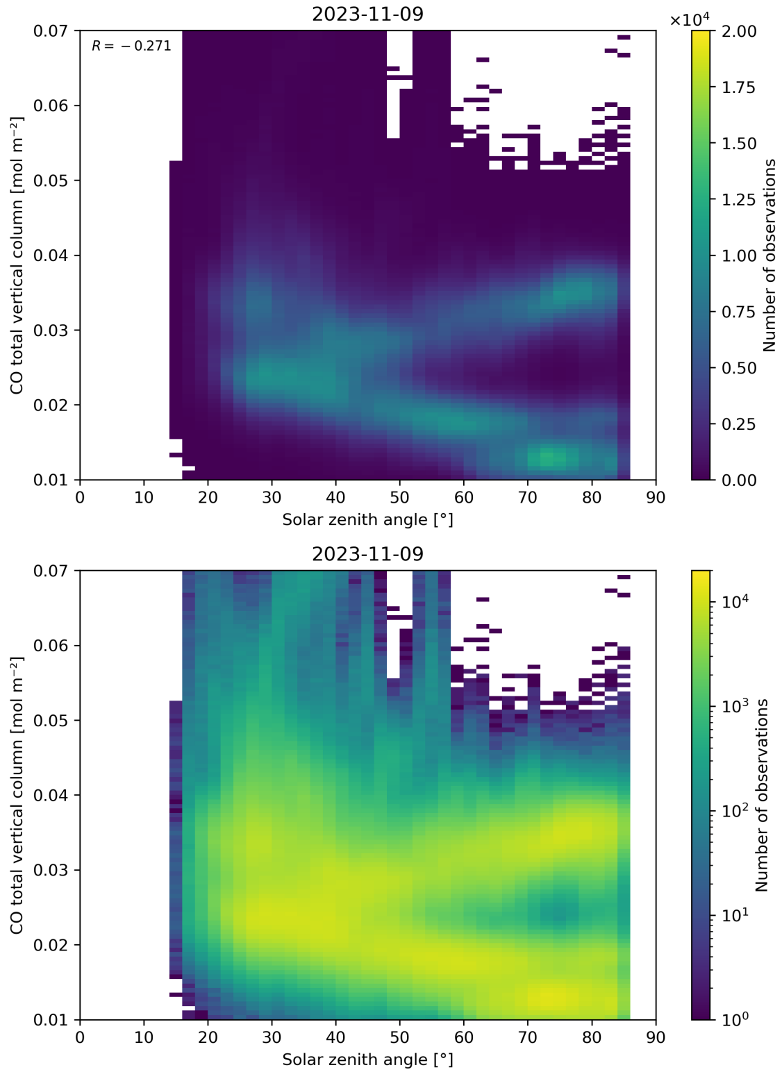
Figure 61: Scatter density plot of “Solar zenith angle” against “CO total vertical column” for 2023-11-08 to 2023-11-10.
