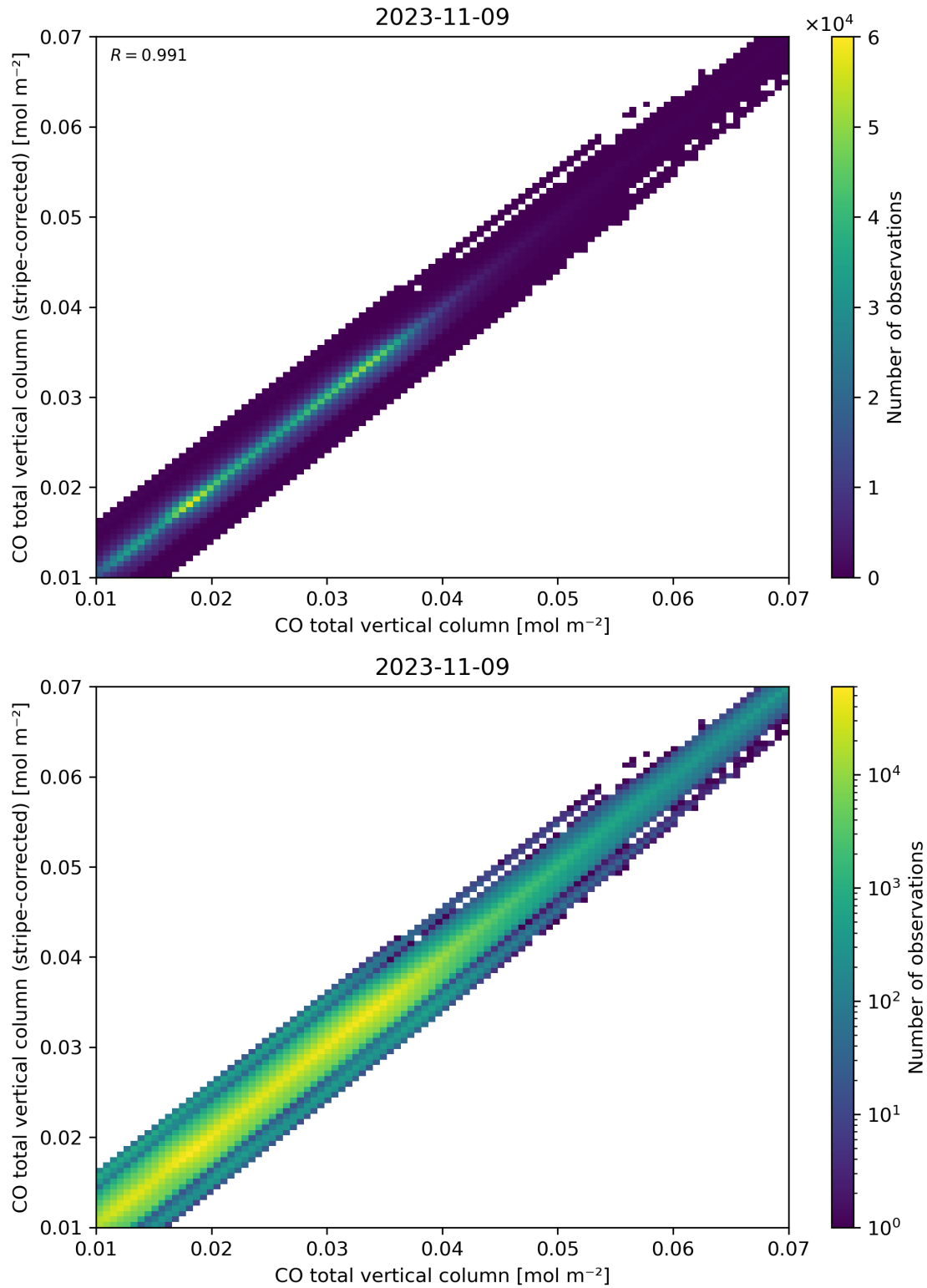
Figure 33: Scatter density plot of “CO total vertical column” against “CO total vertical column (stripe-corrected)” for 2023-11-08 to 2023-11-10.
