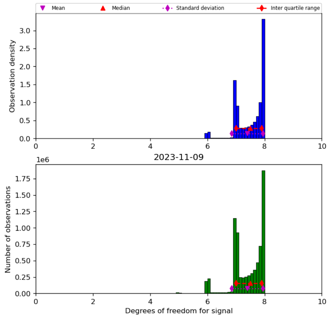
Figure 23: Histogram of “Degrees of freedom for signal” for 2023-11-08 to 2023-11-10
