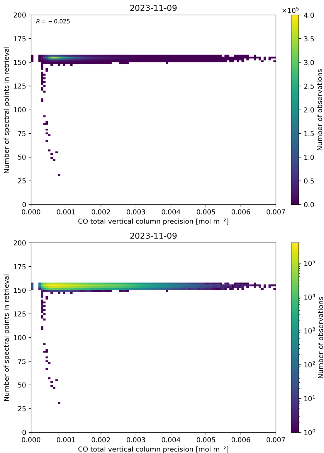
Figure 47: Scatter density plot of “CO total vertical column precision” against “Number of spectral points in retrieval” for 2023-11-08 to 2023-11-10.
