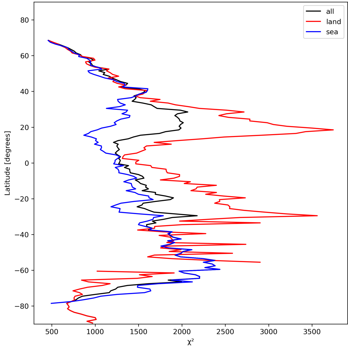
Figure 14: Zonal average of “ \chi^2 ” for 2023-11-08 to 2023-11-10.
