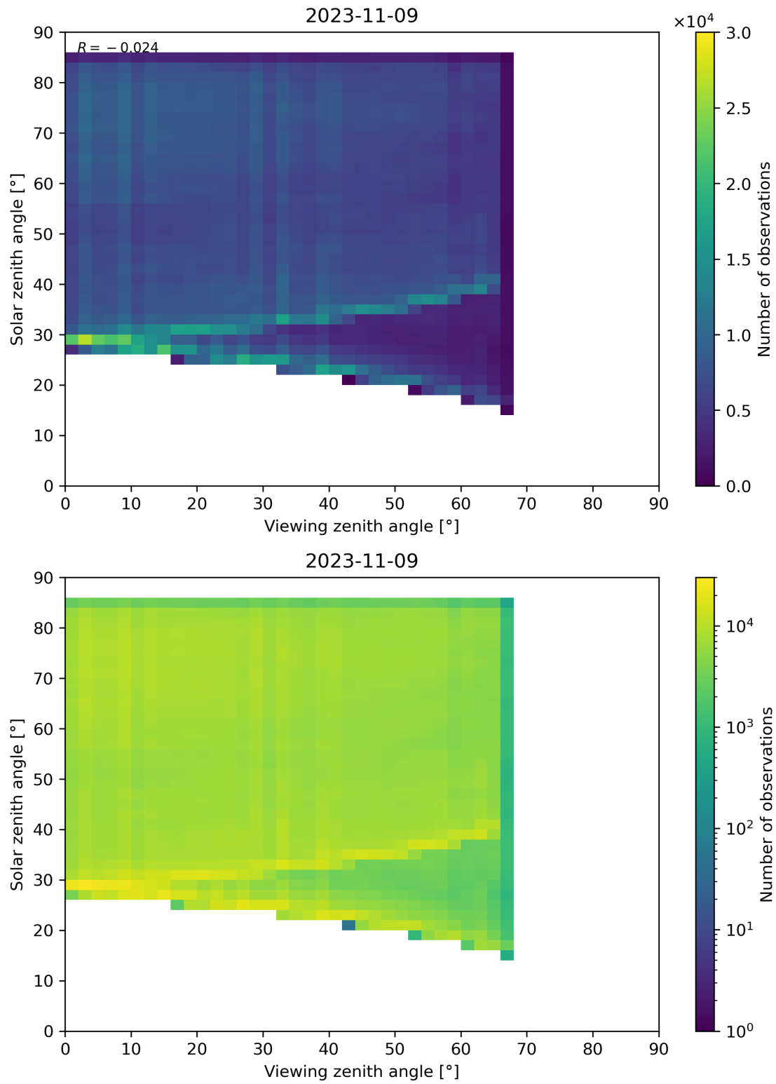
Figure 77: Scatter density plot of “Viewing zenith angle” against “Solar zenith angle” for 2023-11-08 to 2023-11-10.
