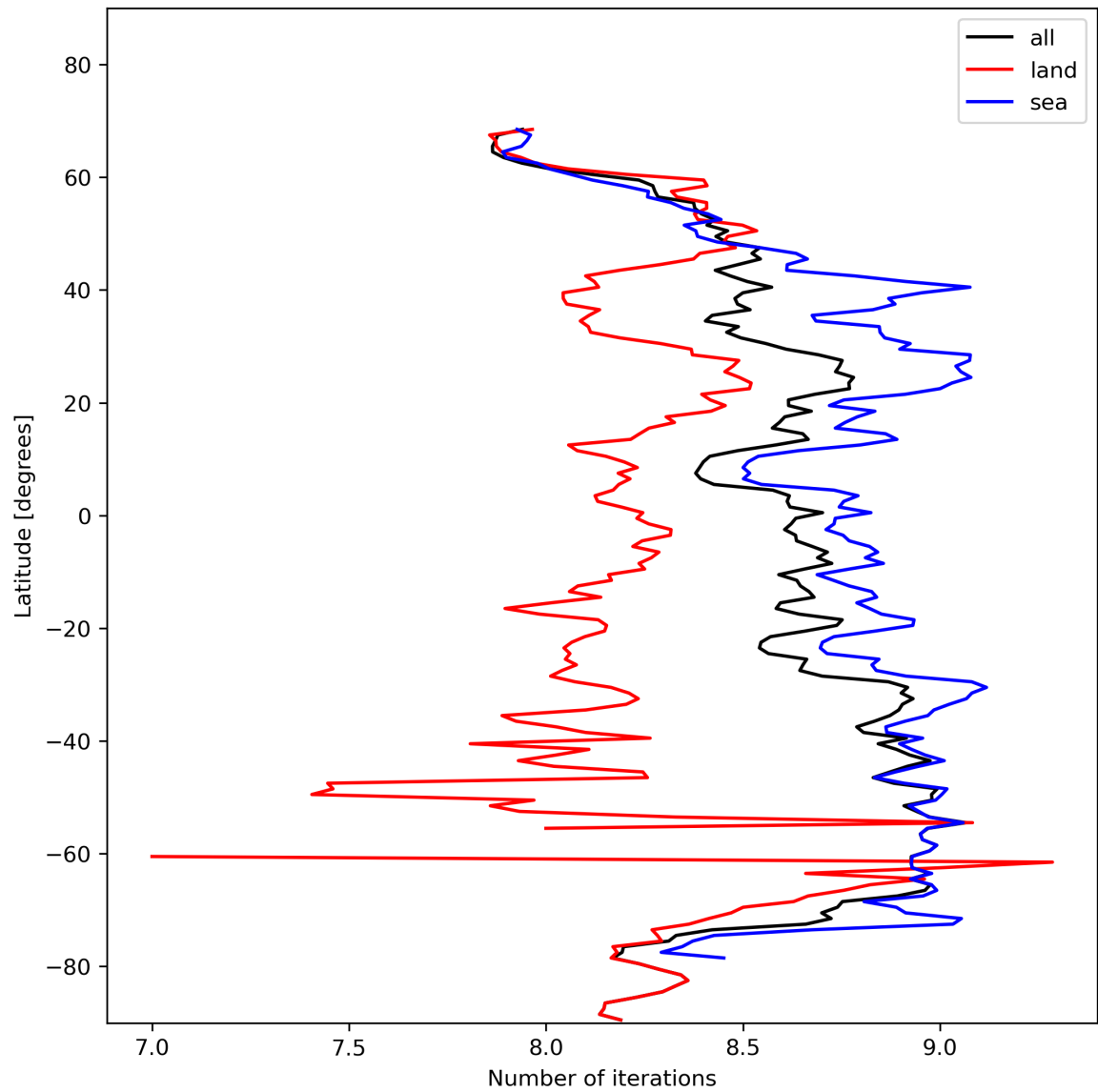
Figure 16: Zonal average of “Number of iterations” for 2023-11-08 to 2023-11-10.
