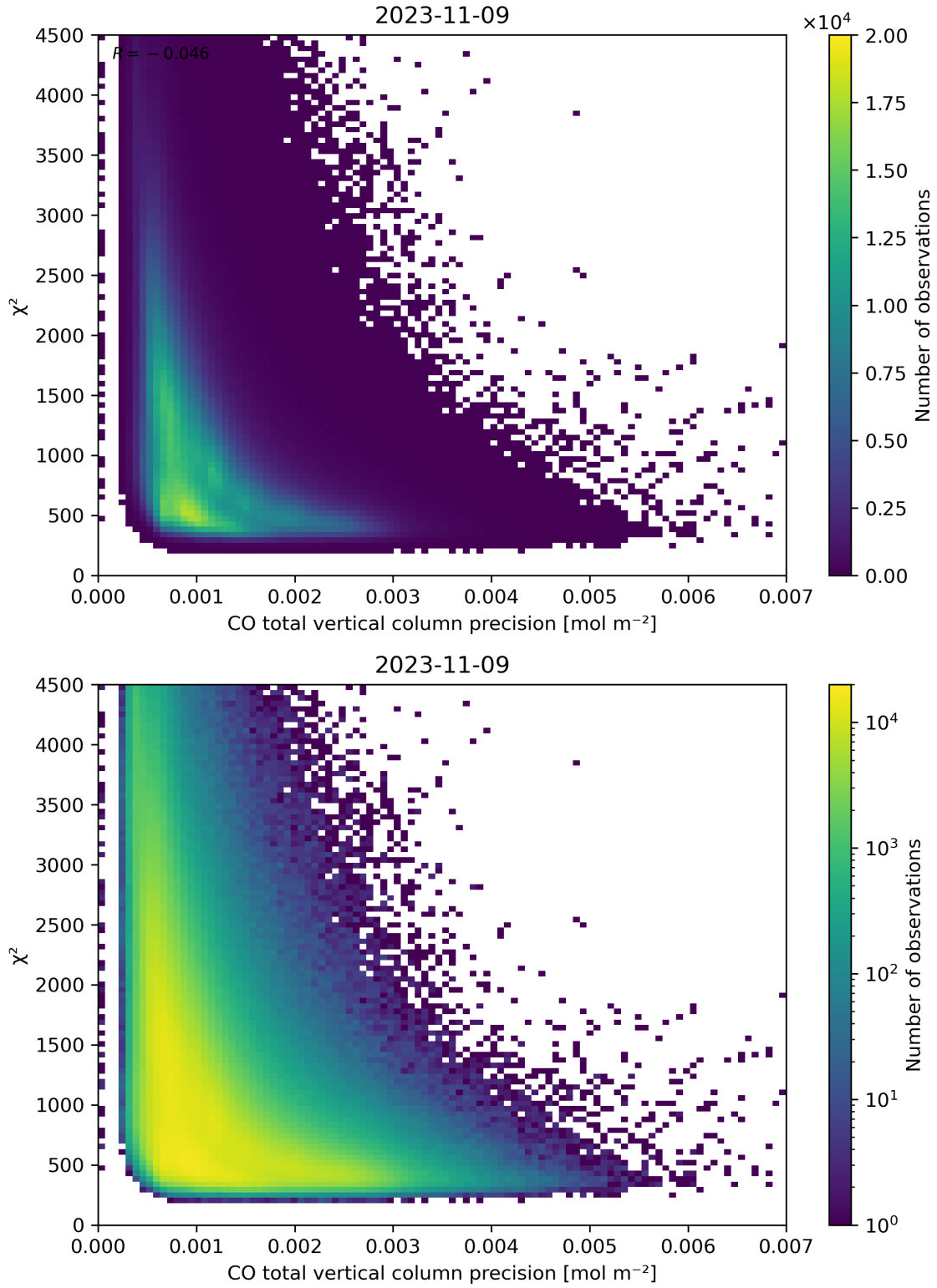
Figure 44: Scatter density plot of “CO total vertical column precision” against “ \chi^2 ” for 2023-11-08 to 2023-11-10.
