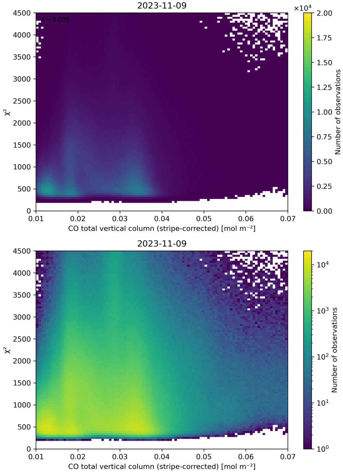
Figure 37: Scatter density plot of “CO total vertical column (stripe-corrected)” against “ \chi^2 ” for 2023-11-08 to 2023-11-10.
