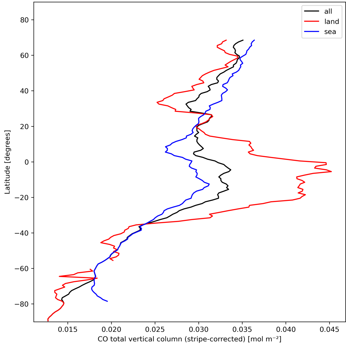
Figure 11: Zonal average of “CO total vertical column (stripe-corrected)” for 2023-11-08 to 2023-11-10.
