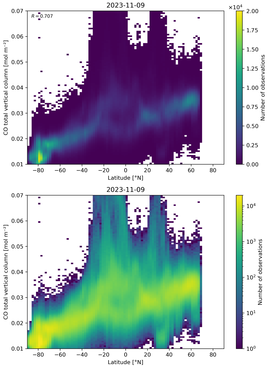
Figure 51: Scatter density plot of “Latitude” against “CO total vertical column” for 2023-11-08 to 2023-11-10.
