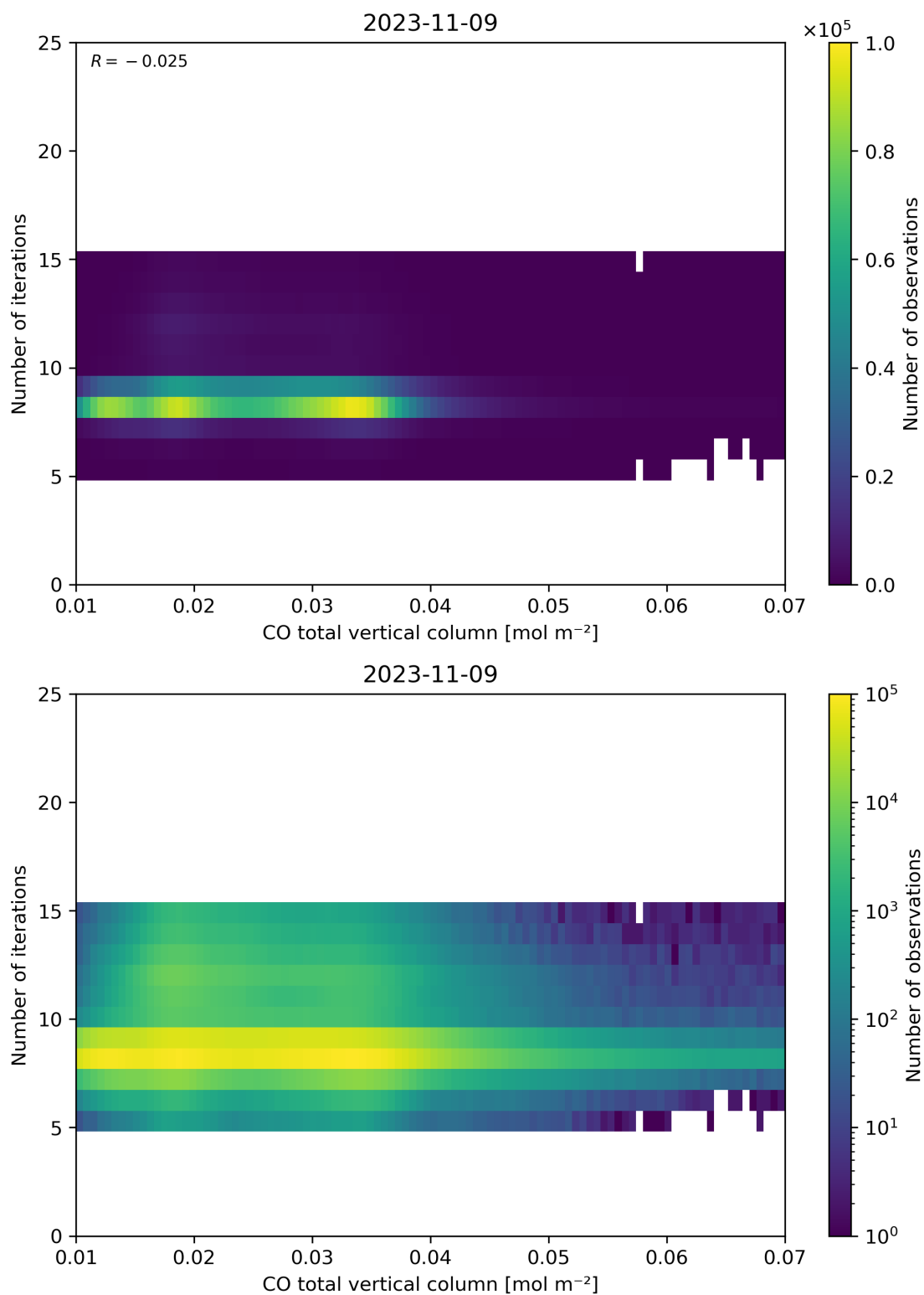
Figure 42: Scatter density plot of “CO total vertical column” against “Number of iterations” for 2023-11-08 to 2023-11-10.
