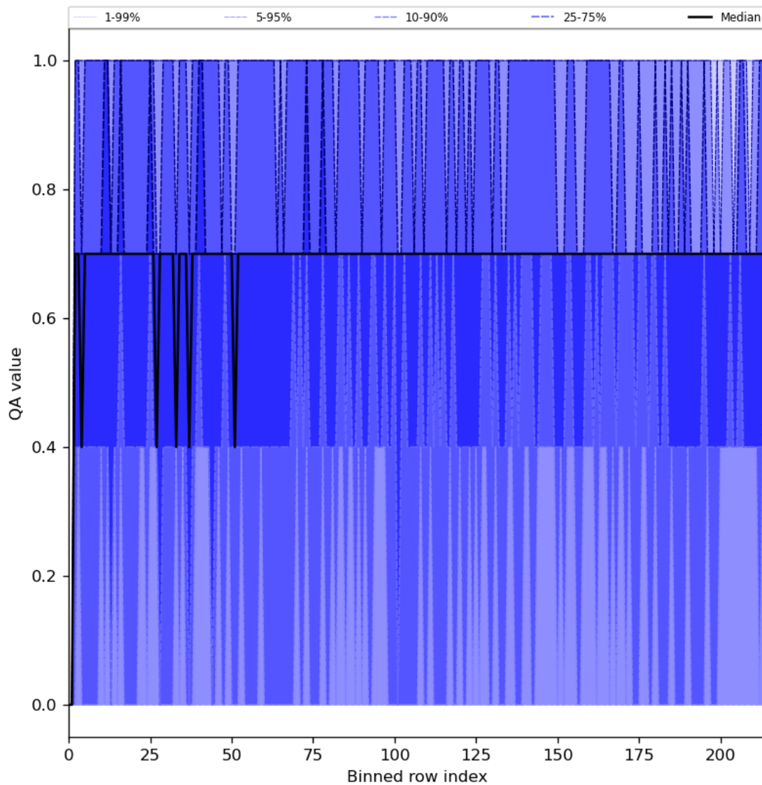
Figure 25: Along track statistics of “QA value” for 2023-11-08 to 2023-11-10
