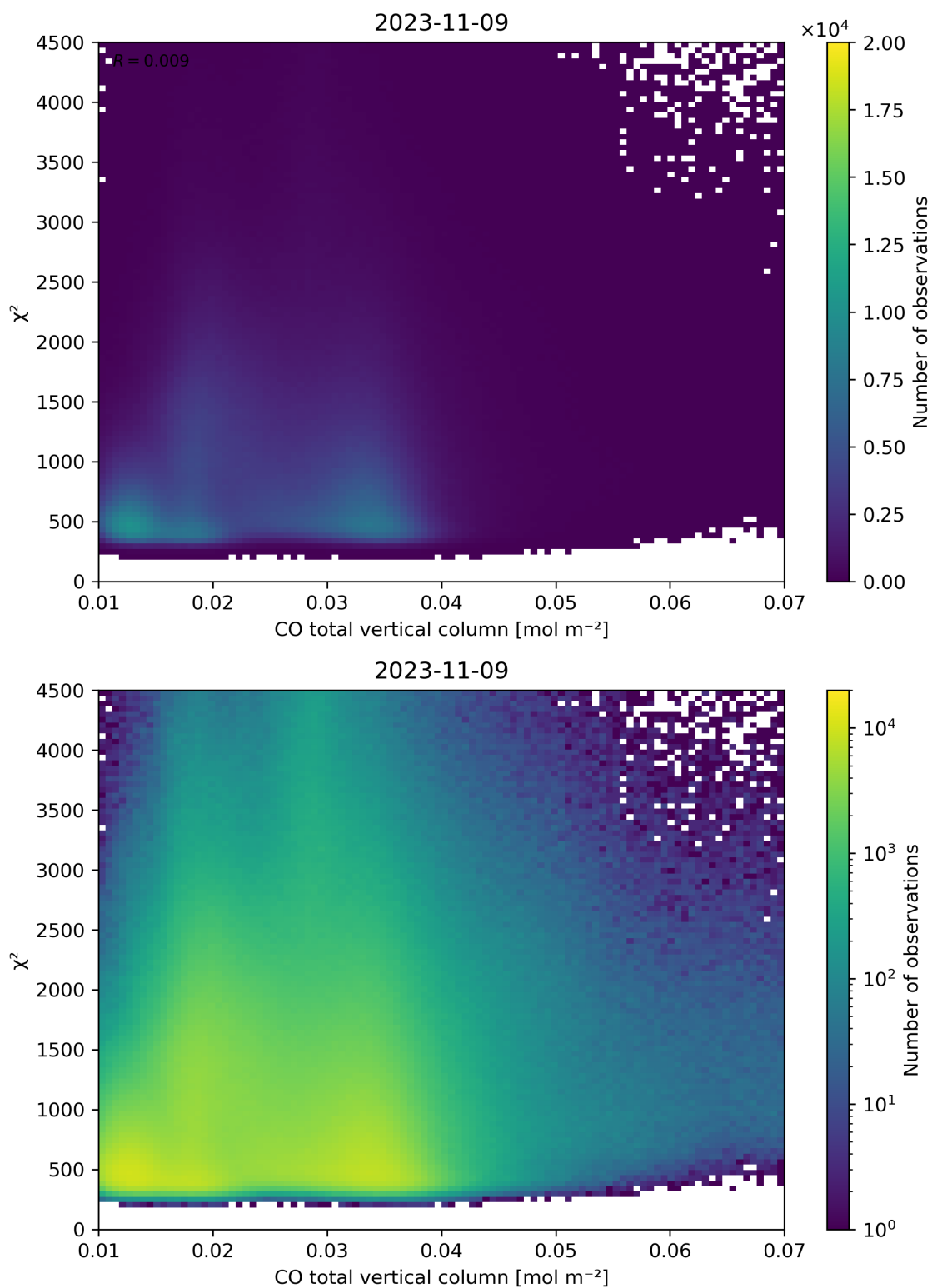
Figure 35: Scatter density plot of “CO total vertical column” against “ \chi^2 ” for 2023-11-08 to 2023-11-10.
