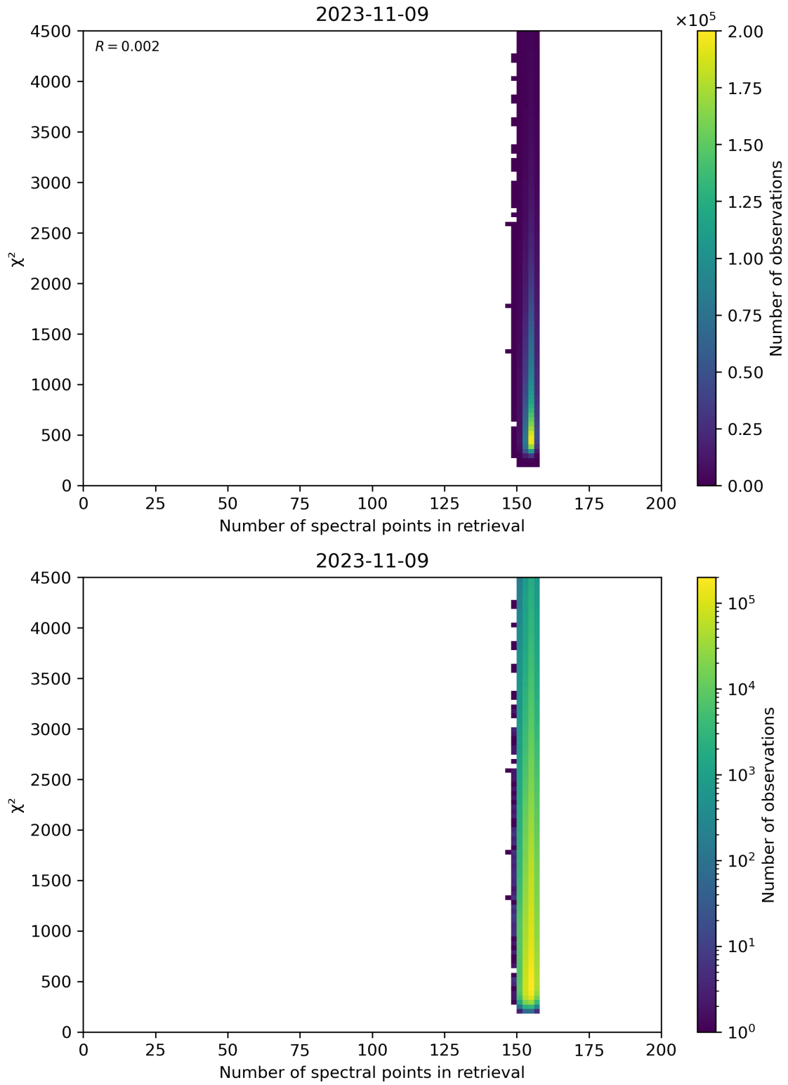
Figure 58: Scatter density plot of “Number of spectral points in retrieval” against “ \chi^2 ” for 2023-11-08 to 2023-11-10.
