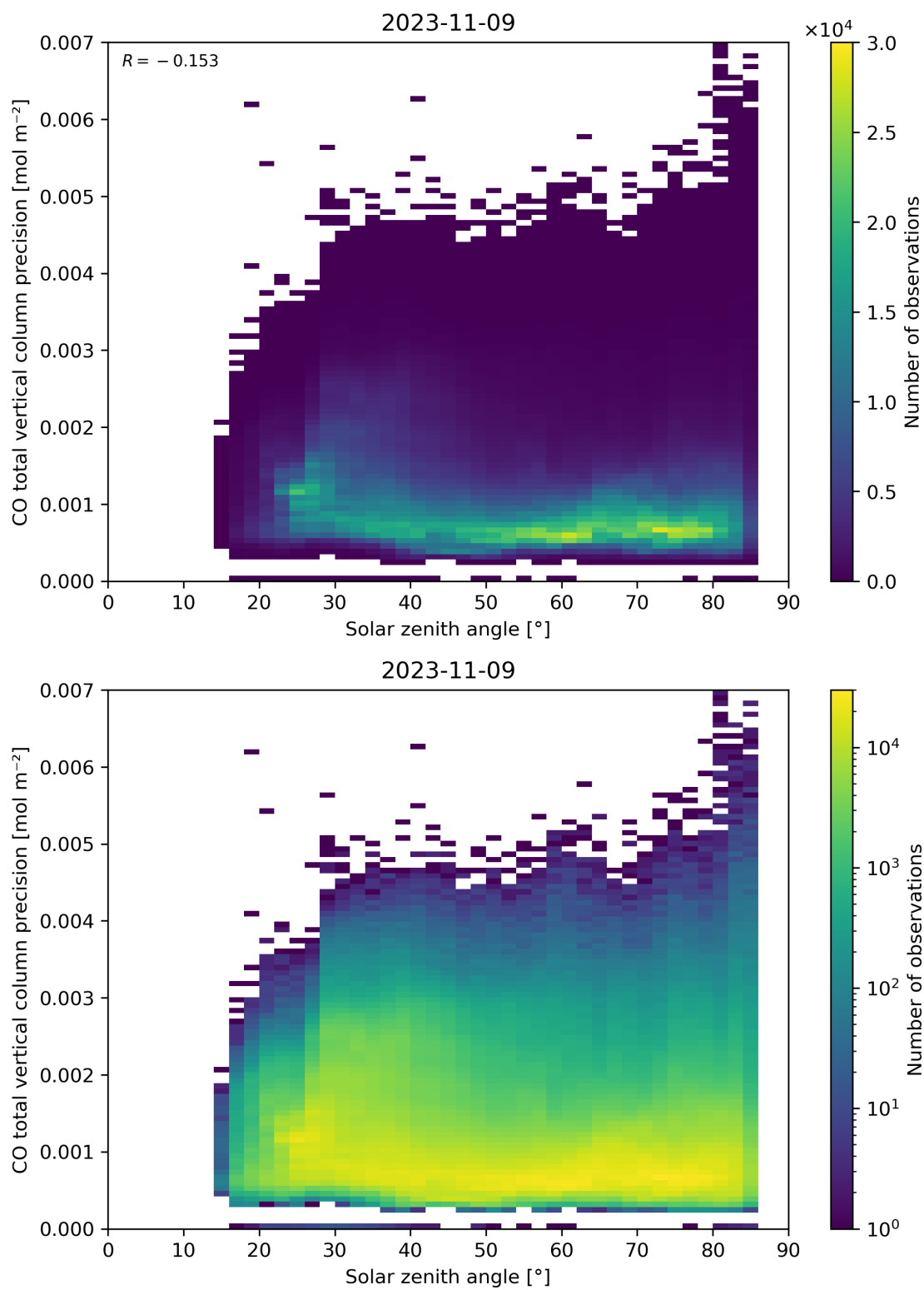
Figure 63: Scatter density plot of “Solar zenith angle” against “CO total vertical column precision” for 2023-11-08 to 2023-11-10.
