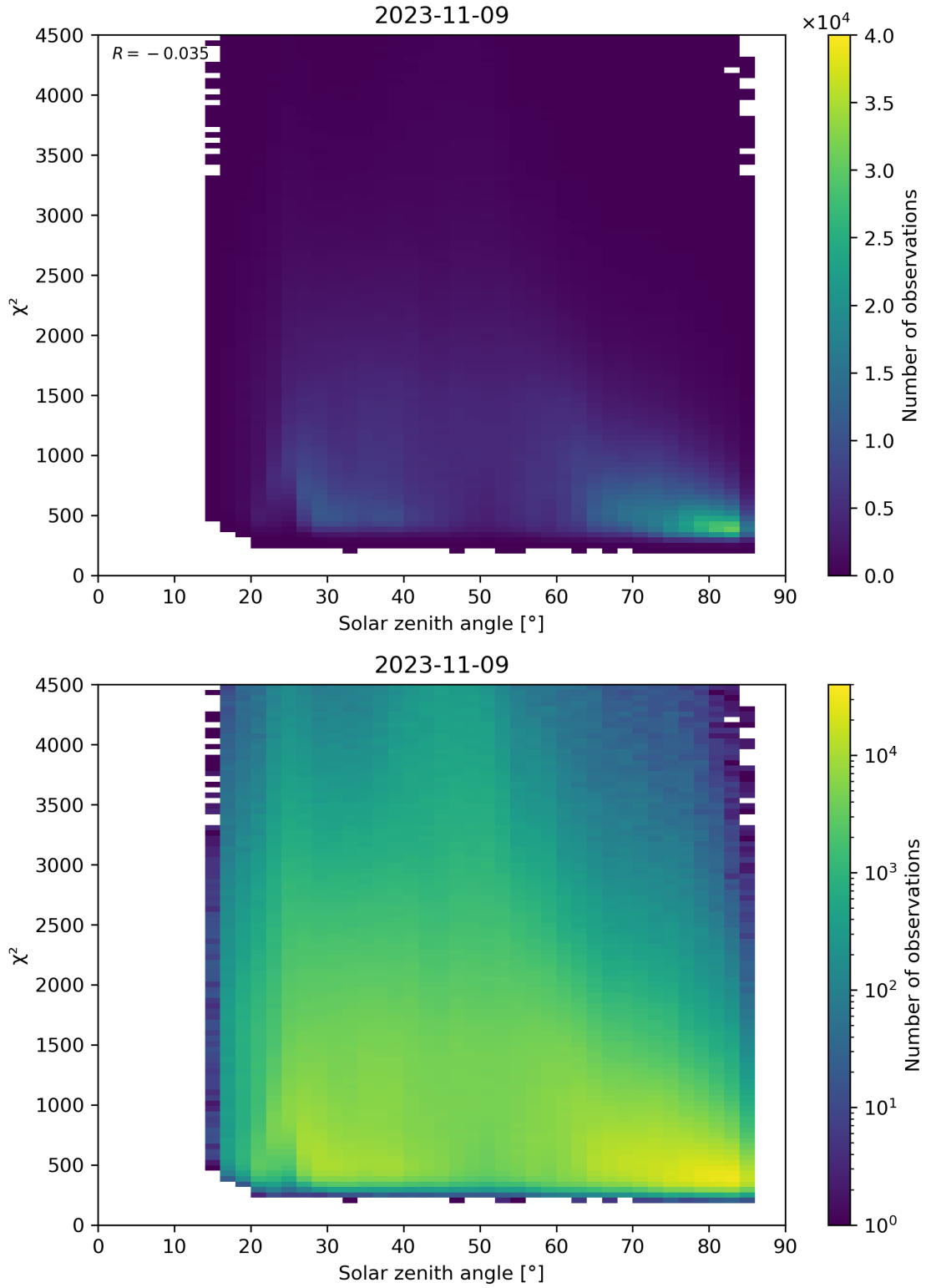
Figure 64: Scatter density plot of “Solar zenith angle” against “ \chi^2 ” for 2023-11-08 to 2023-11-10.
