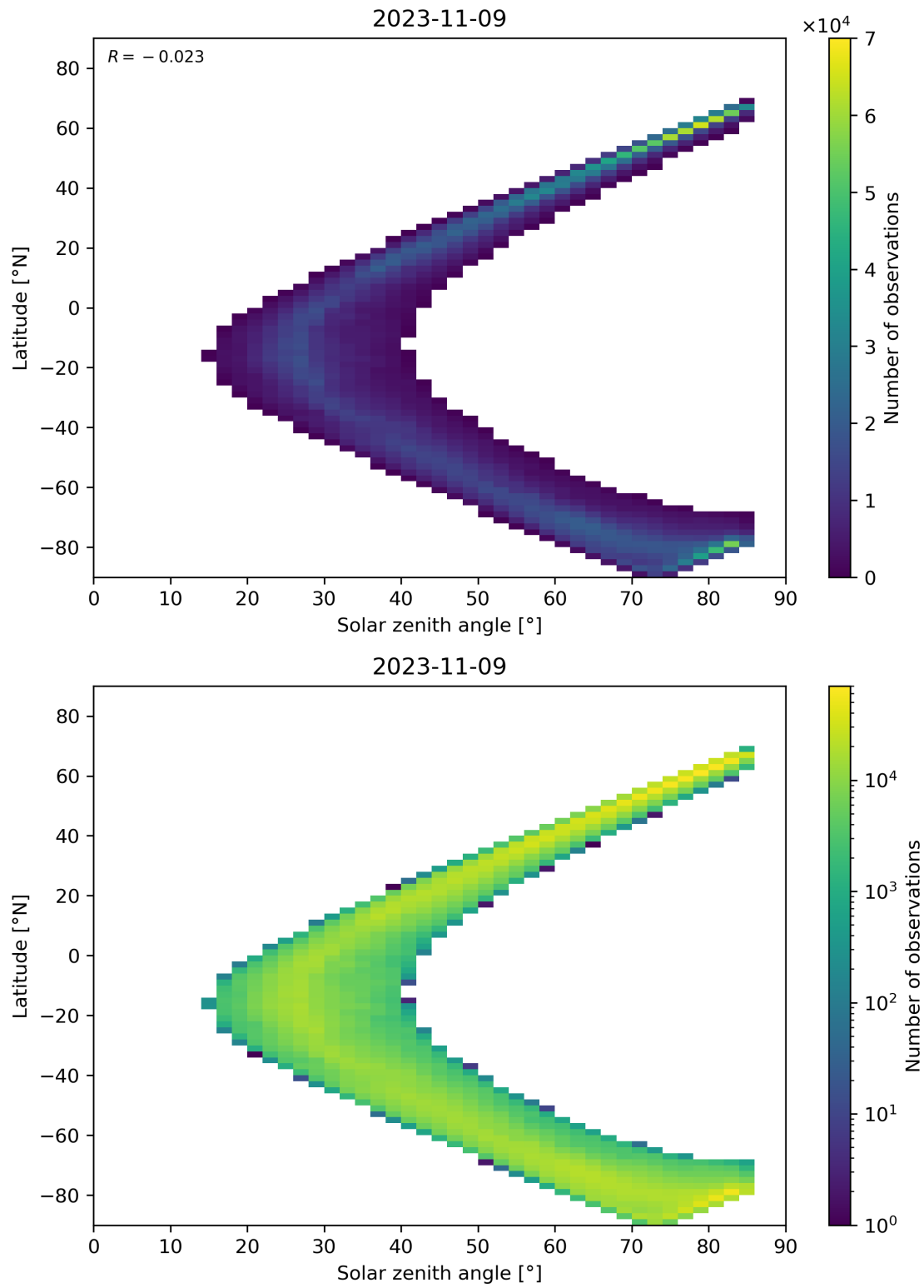
Figure 66: Scatter density plot of “Solar zenith angle” against “Latitude” for 2023-11-08 to 2023-11-10.
