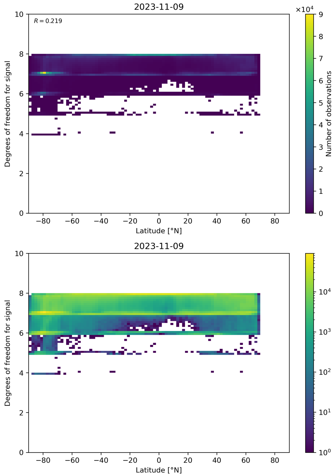
Figure 55: Scatter density plot of “Latitude” against “Degrees of freedom for signal” for 2023-11-08 to 2023-11-10.
