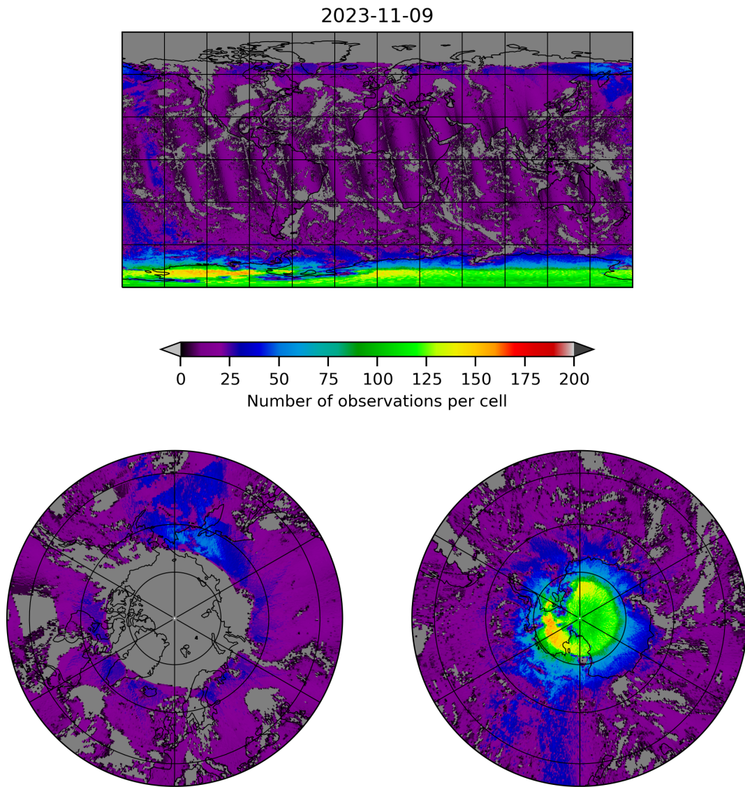
Figure 8: Map of the number of observations for 2023-11-08 to 2023-11-10
