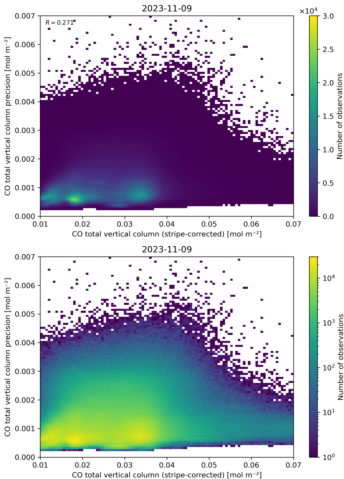
Figure 36: Scatter density plot of “CO total vertical column (stripe-corrected)” against “CO total vertical column precision” for 2023-11-08 to 2023-11-10.
