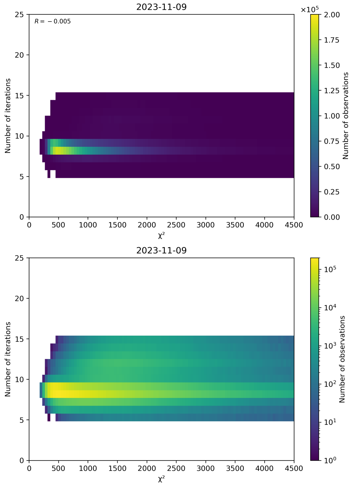
Figure 49: Scatter density plot of “ \chi^2 ” against “Number of iterations” for 2023-11-08 to 2023-11-10.
