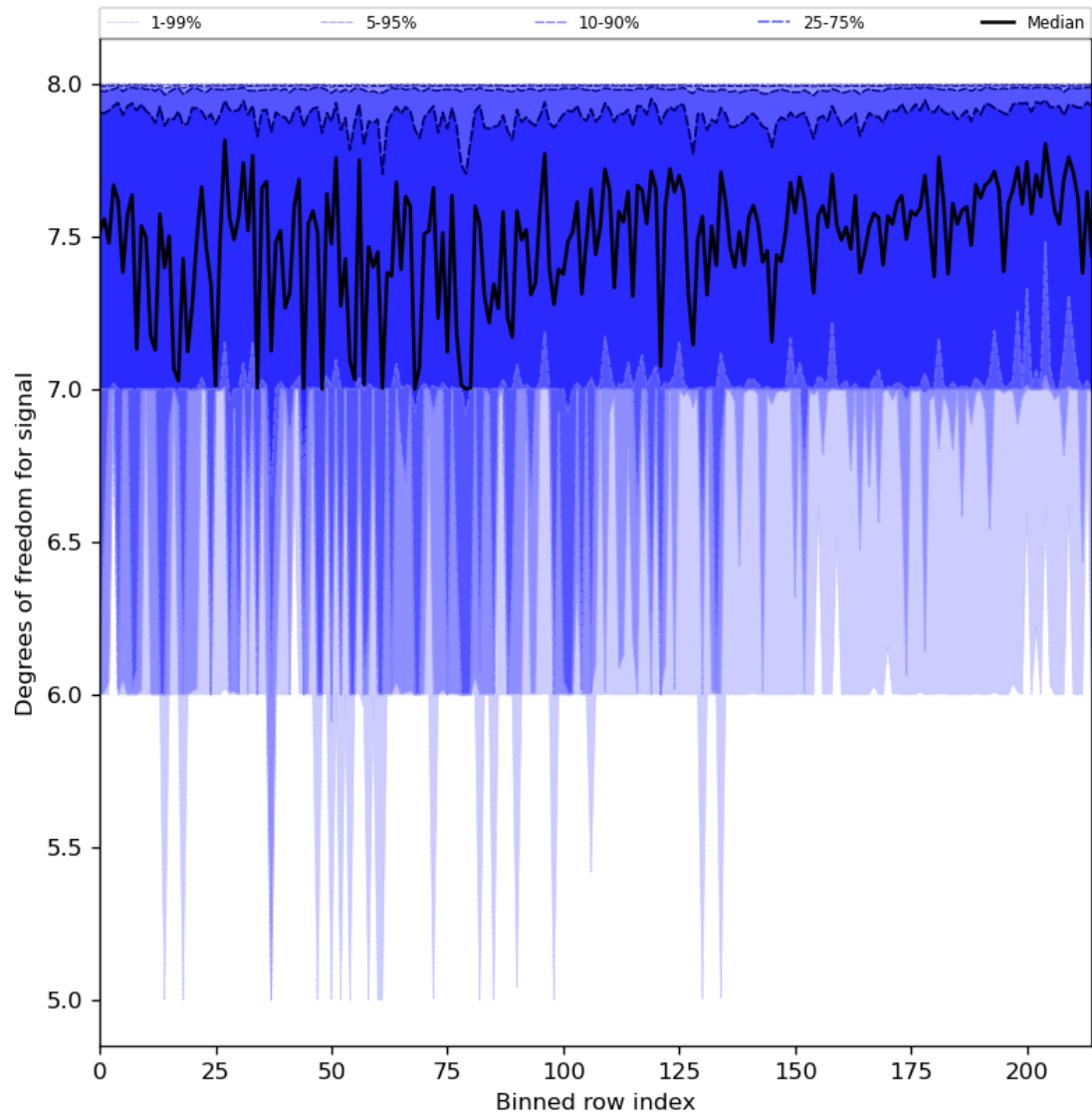
Figure 31: Along track statistics of “Degrees of freedom for signal” for 2023-11-08 to 2023-11-10
