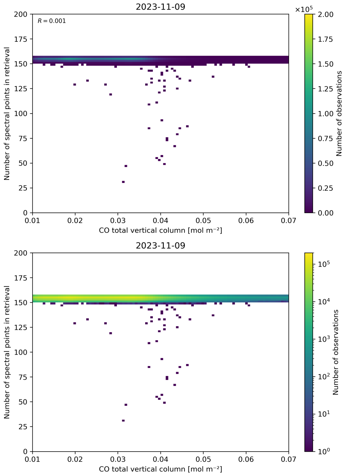
Figure 43: Scatter density plot of “CO total vertical column” against “Number of spectral points in retrieval” for 2023-11-08 to 2023-11-10.
