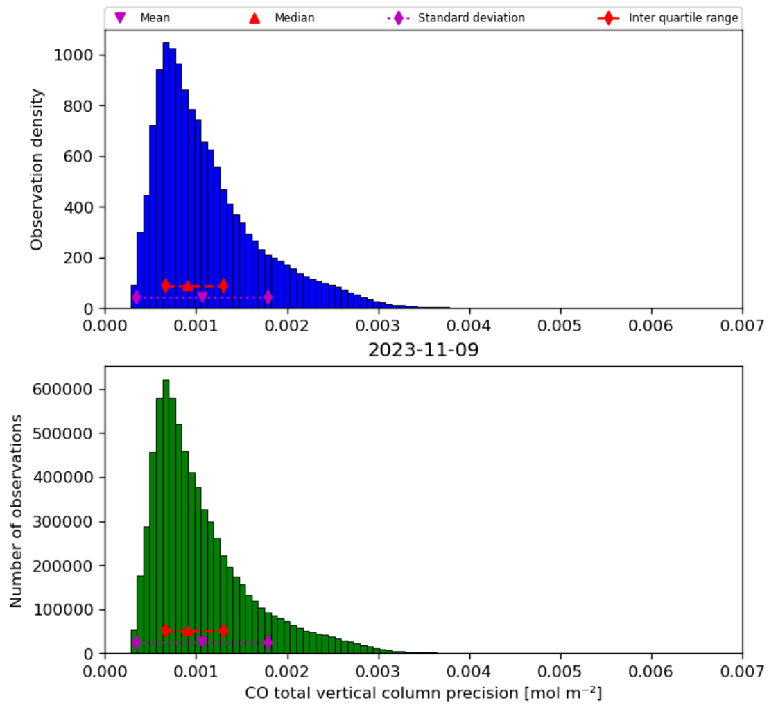
Figure 20: Histogram of “CO total vertical column precision” for 2023-11-08 to 2023-11-10
