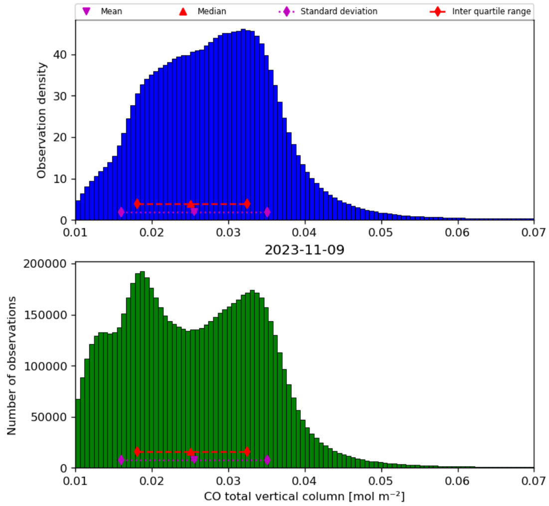
Figure 18: Histogram of “CO total vertical column” for 2023-11-08 to 2023-11-10
