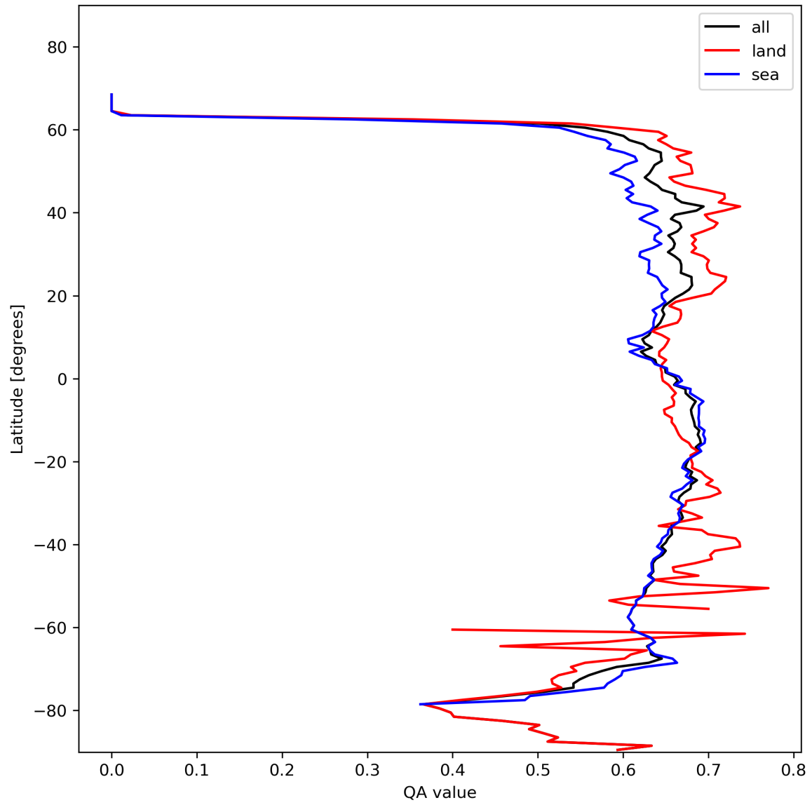
Figure 9: Zonal average of “QA value” for 2023-11-08 to 2023-11-10.
