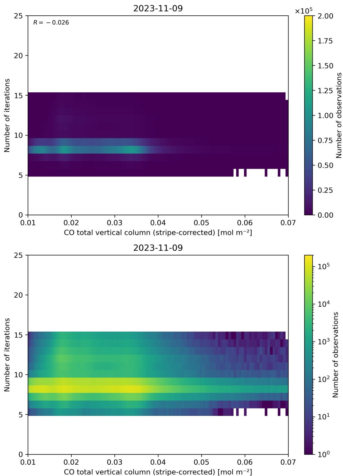
Figure 39: Scatter density plot of “CO total vertical column (stripe-corrected)” against “Number of iterations” for 2023-11-08 to 2023-11-10.
