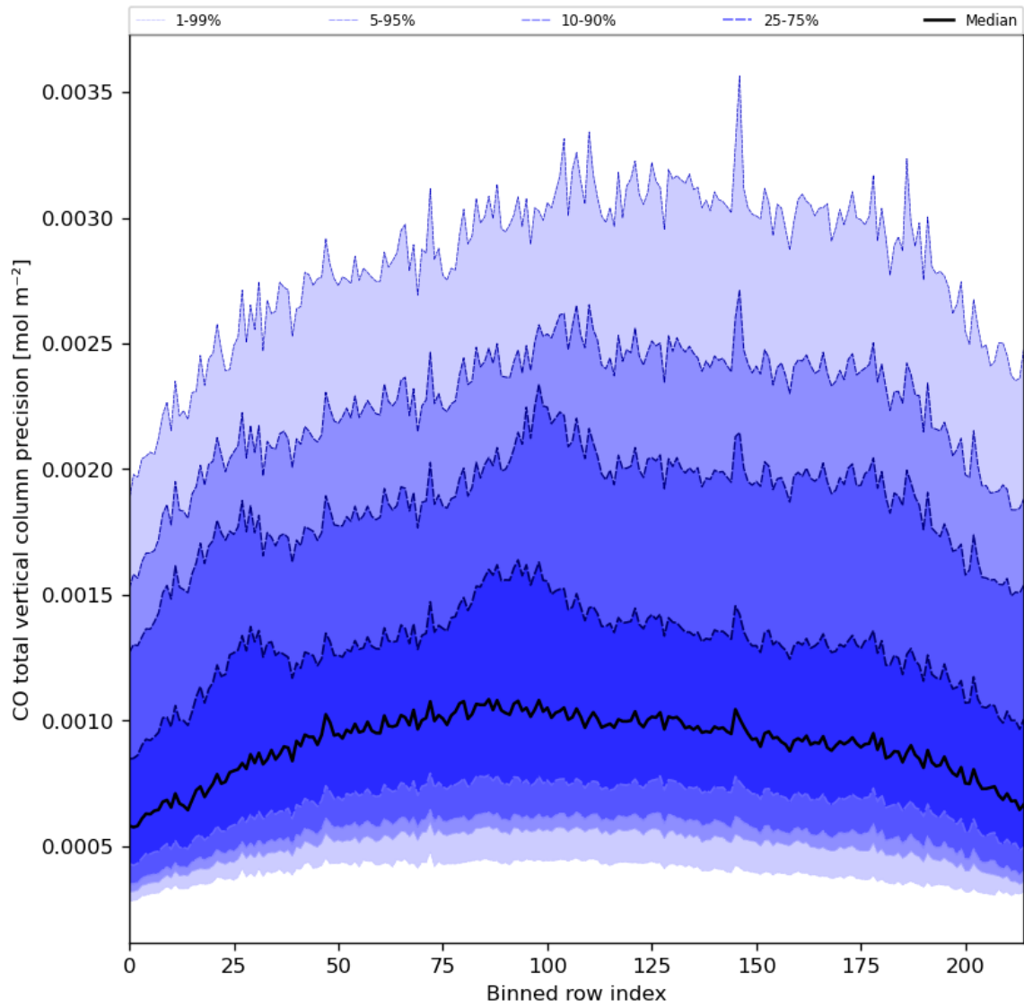
Figure 28: Along track statistics of “CO total vertical column precision” for 2023-11-08 to 2023-11-10
