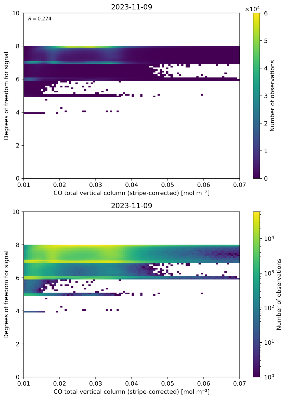
Figure 38: Scatter density plot of “CO total vertical column (stripe-corrected)” against “Degrees of freedom for signal” for 2023-11-08 to 2023-11-10.
