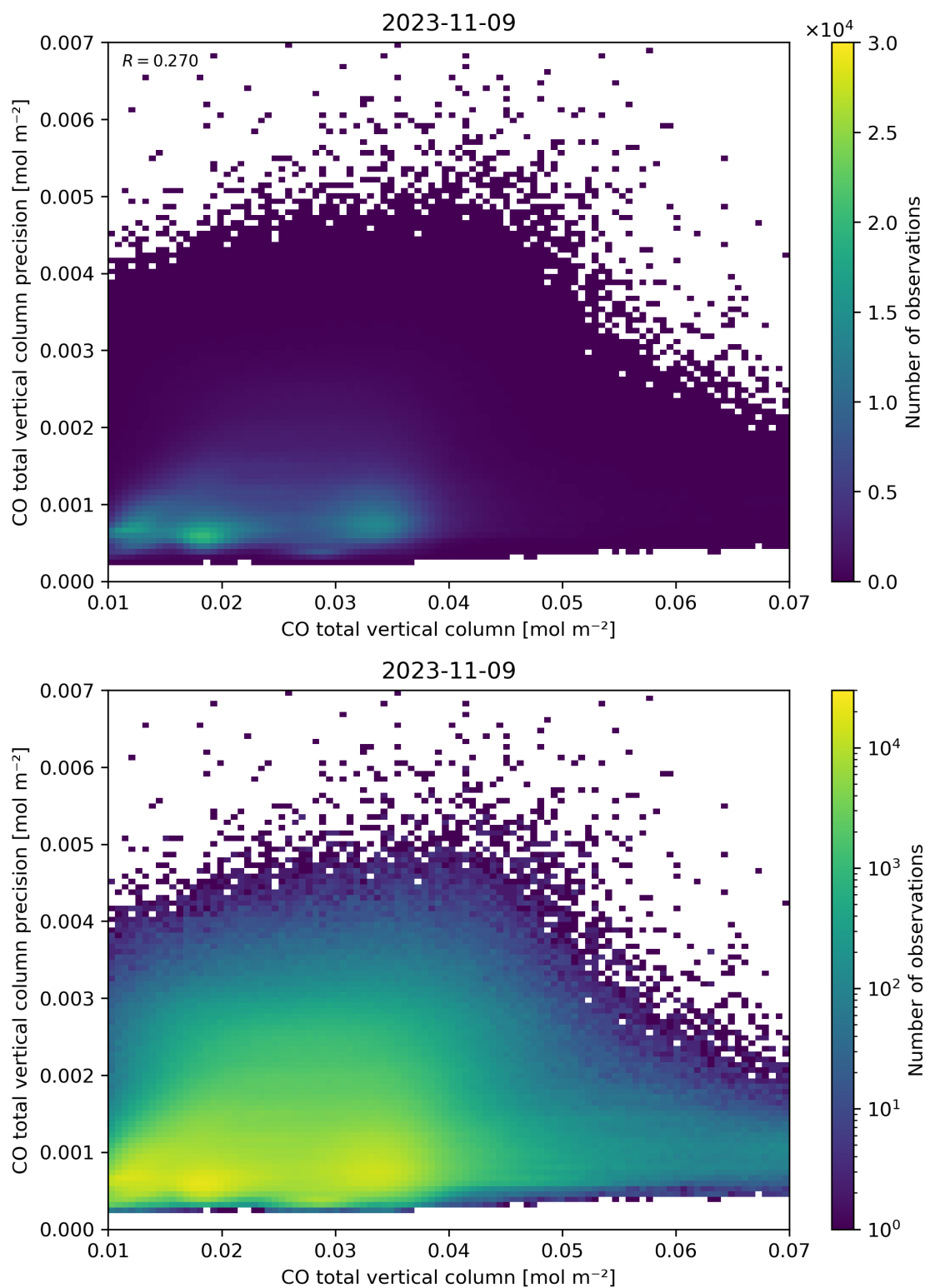
Figure 34: Scatter density plot of “CO total vertical column” against “CO total vertical column precision” for 2023-11-08 to 2023-11-10.
