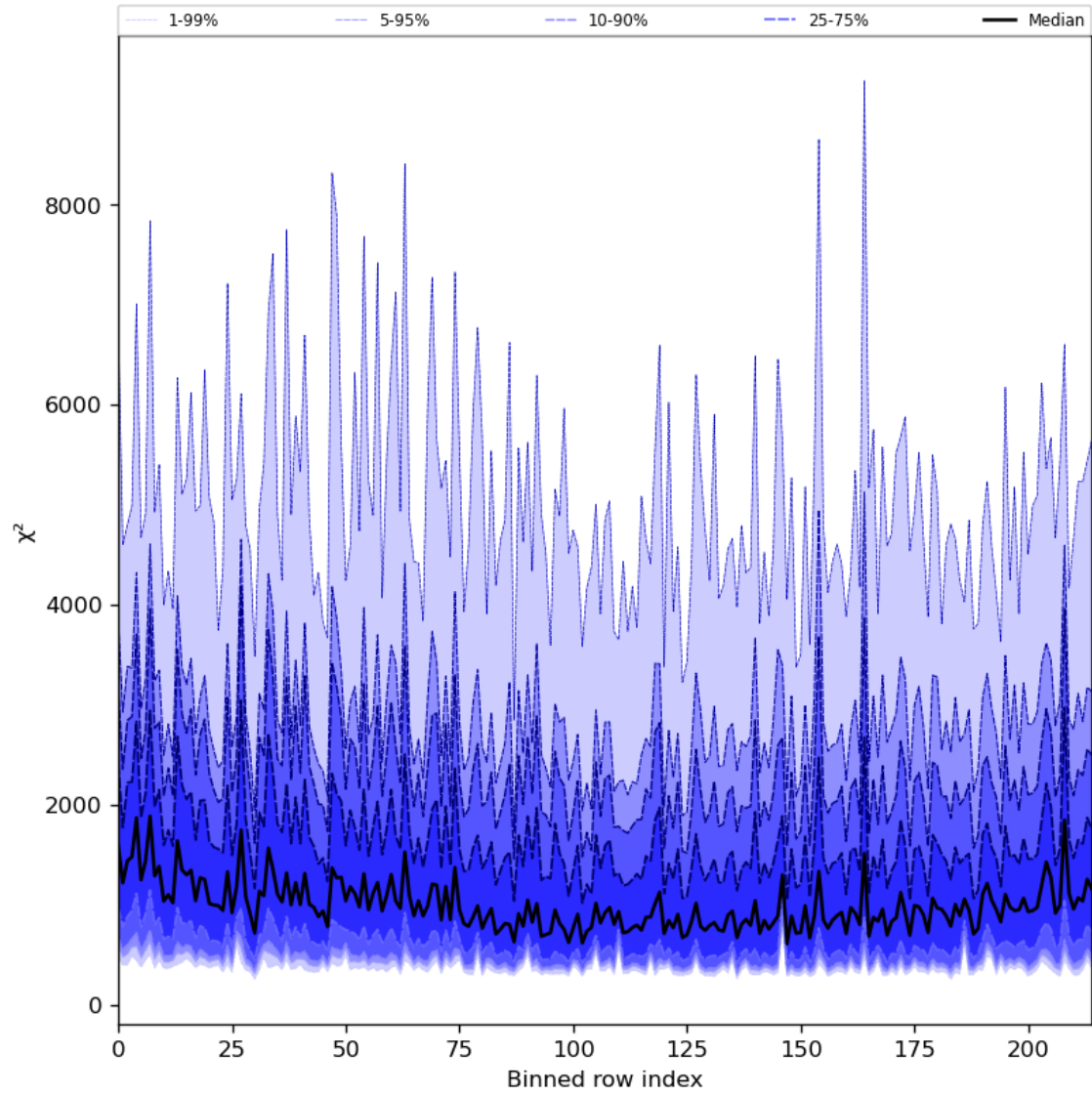
Figure 30: Along track statistics of “ \chi^2 ” for 2023-11-08 to 2023-11-10
