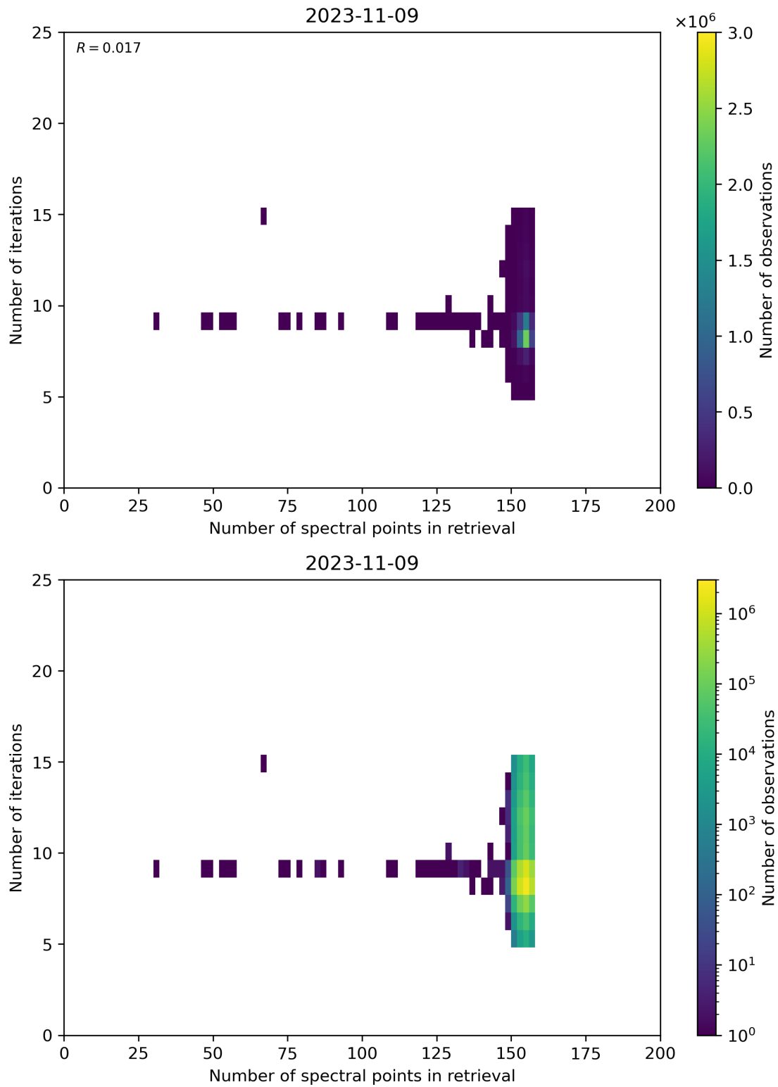
Figure 60: Scatter density plot of “Number of spectral points in retrieval” against “Number of iterations” for 2023-11-08 to 2023-11-10.
