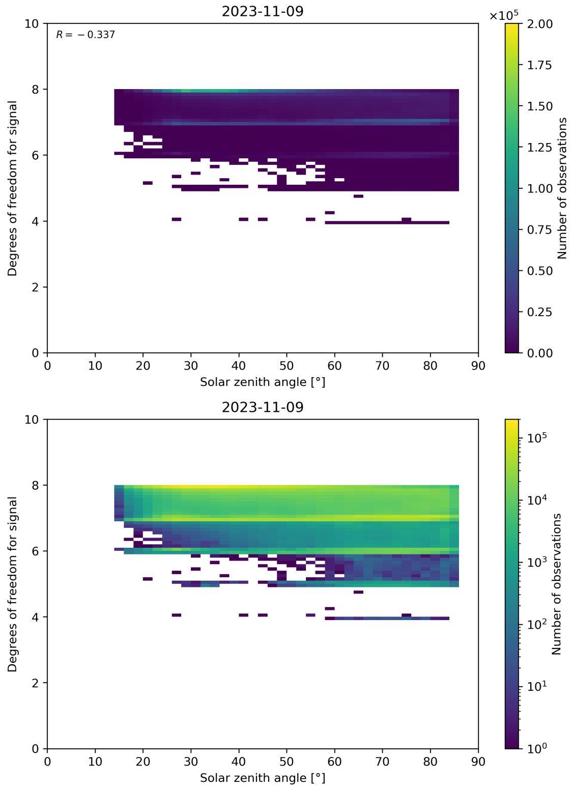
Figure 65: Scatter density plot of “Solar zenith angle” against “Degrees of freedom for signal” for 2023-11-08 to 2023-11-10.
