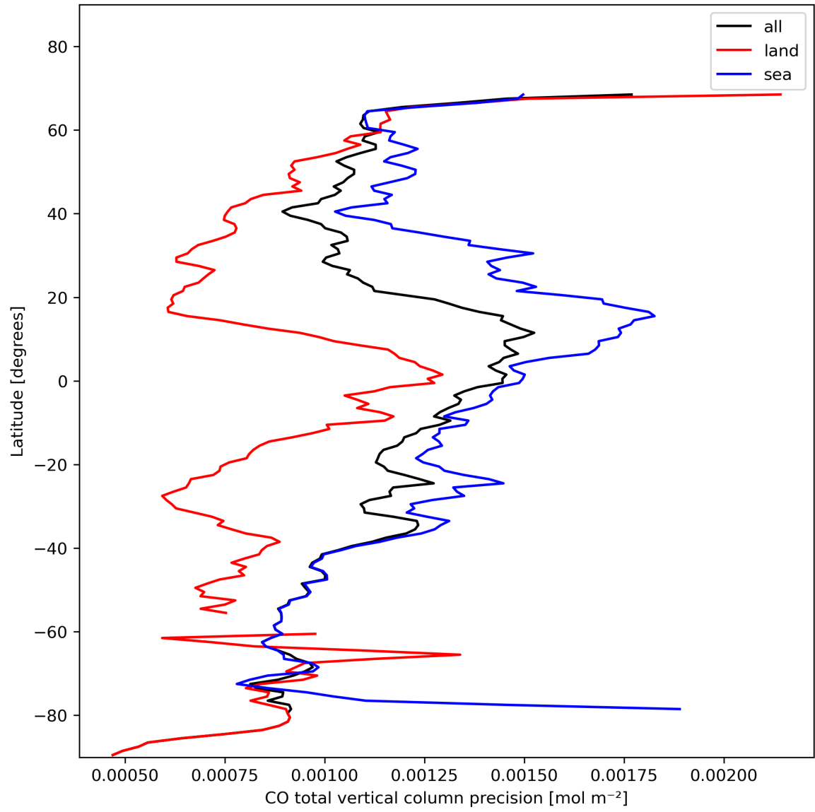
Figure 12: Zonal average of “CO total vertical column precision” for 2023-11-08 to 2023-11-10.
