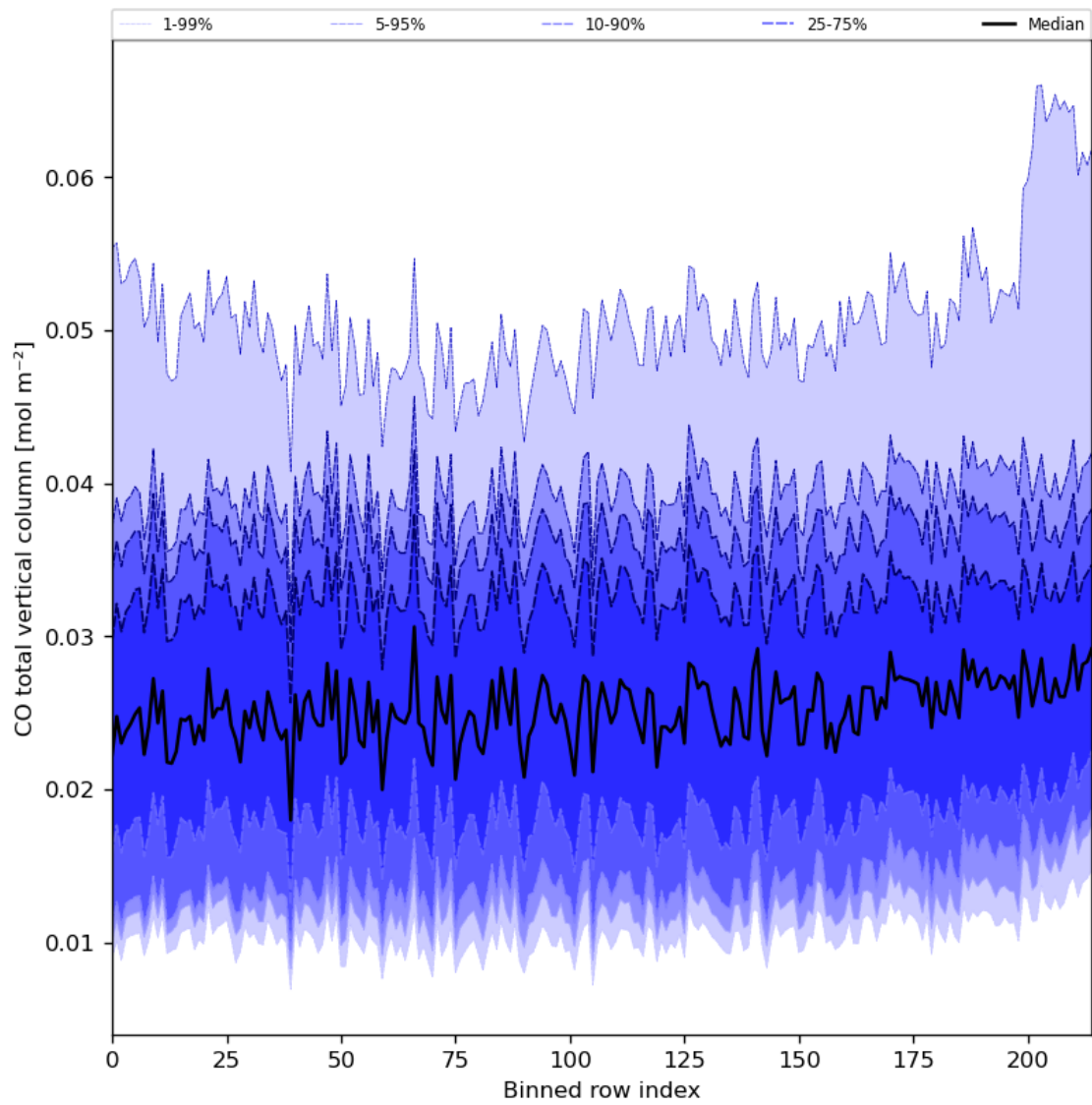
Figure 26: Along track statistics of “CO total vertical column” for 2023-11-08 to 2023-11-10
