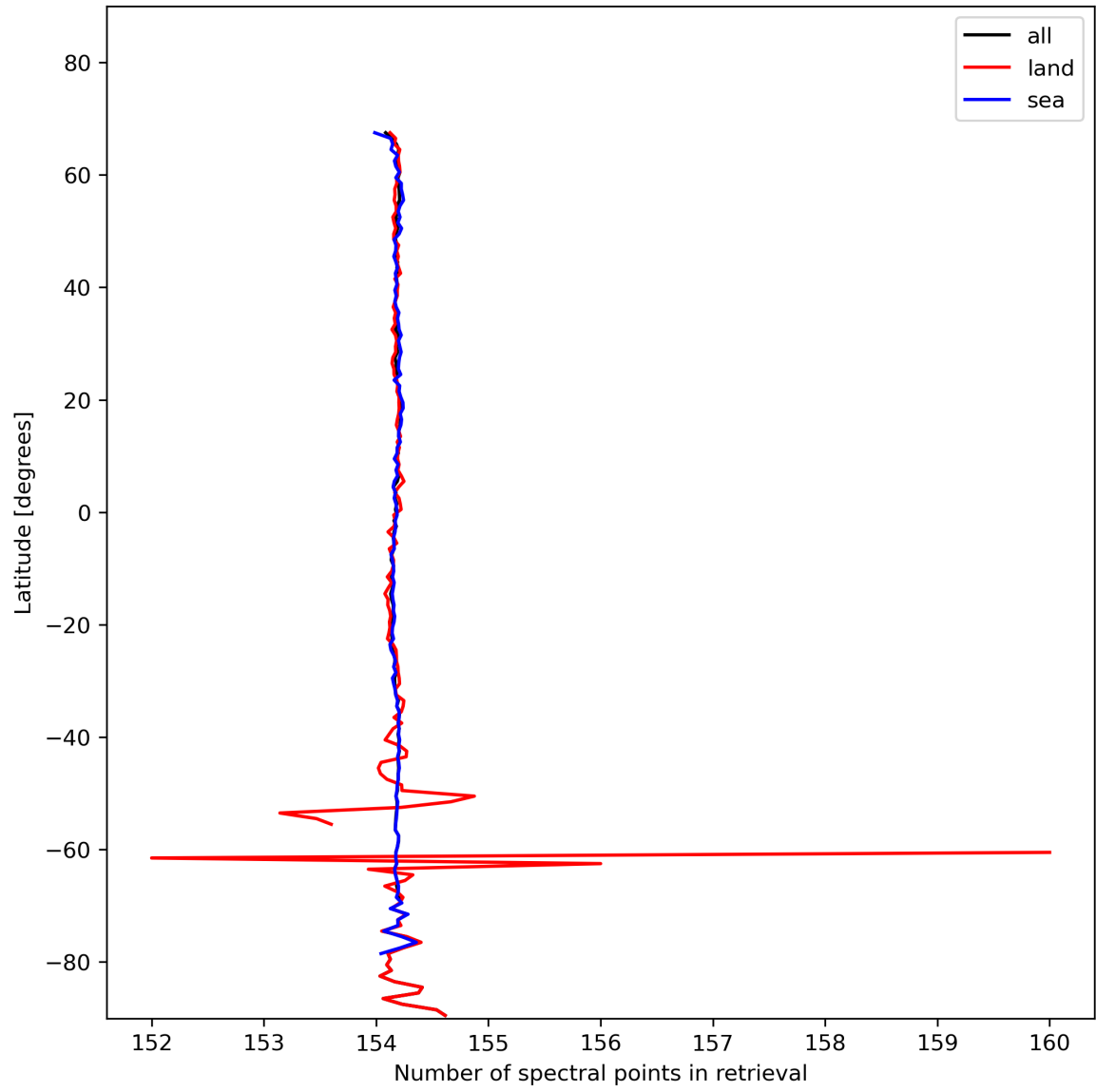
Figure 13: Zonal average of “Number of spectral points in retrieval” for 2023-11-09 to 2023-11-11.
