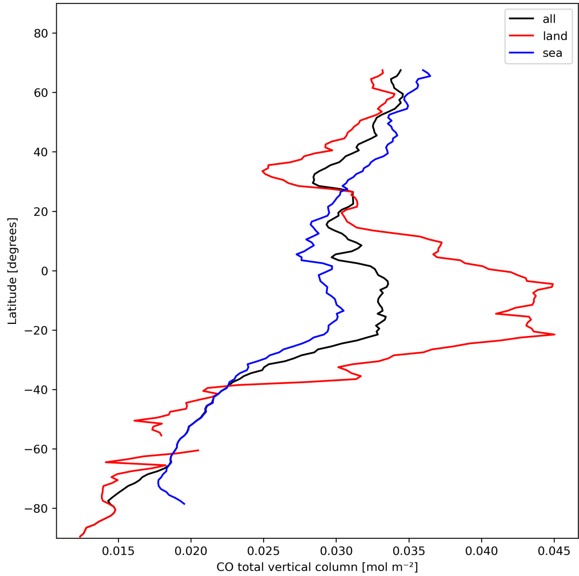
Figure 10: Zonal average of “CO total vertical column” for 2023-11-09 to 2023-11-11.
