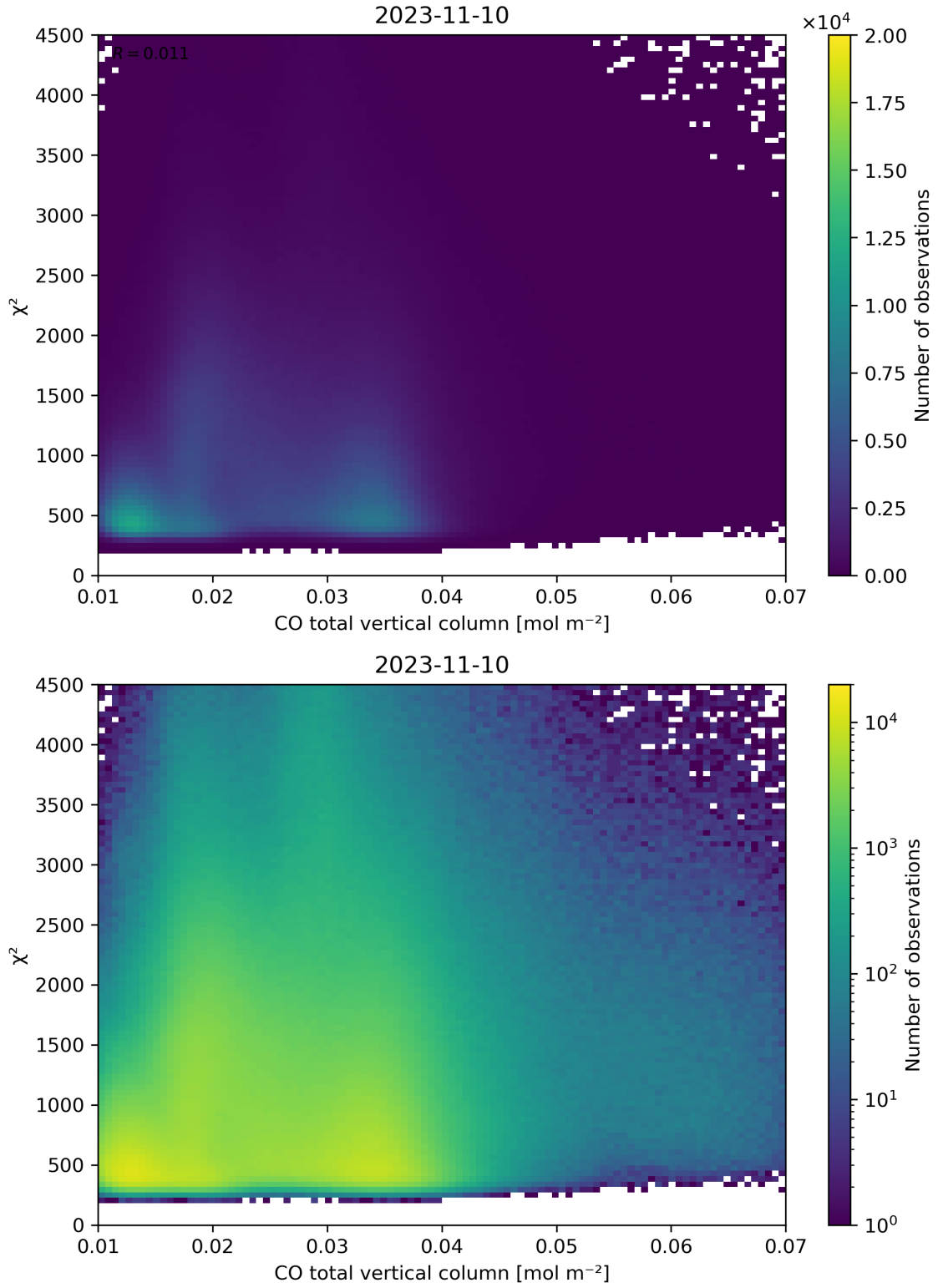
Figure 35: Scatter density plot of “CO total vertical column” against “ \chi^2 ” for 2023-11-09 to 2023-11-11.
