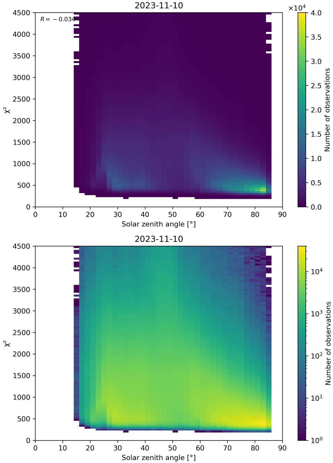
Figure 64: Scatter density plot of “Solar zenith angle” against “ \chi^2 ” for 2023-11-09 to 2023-11-11.
