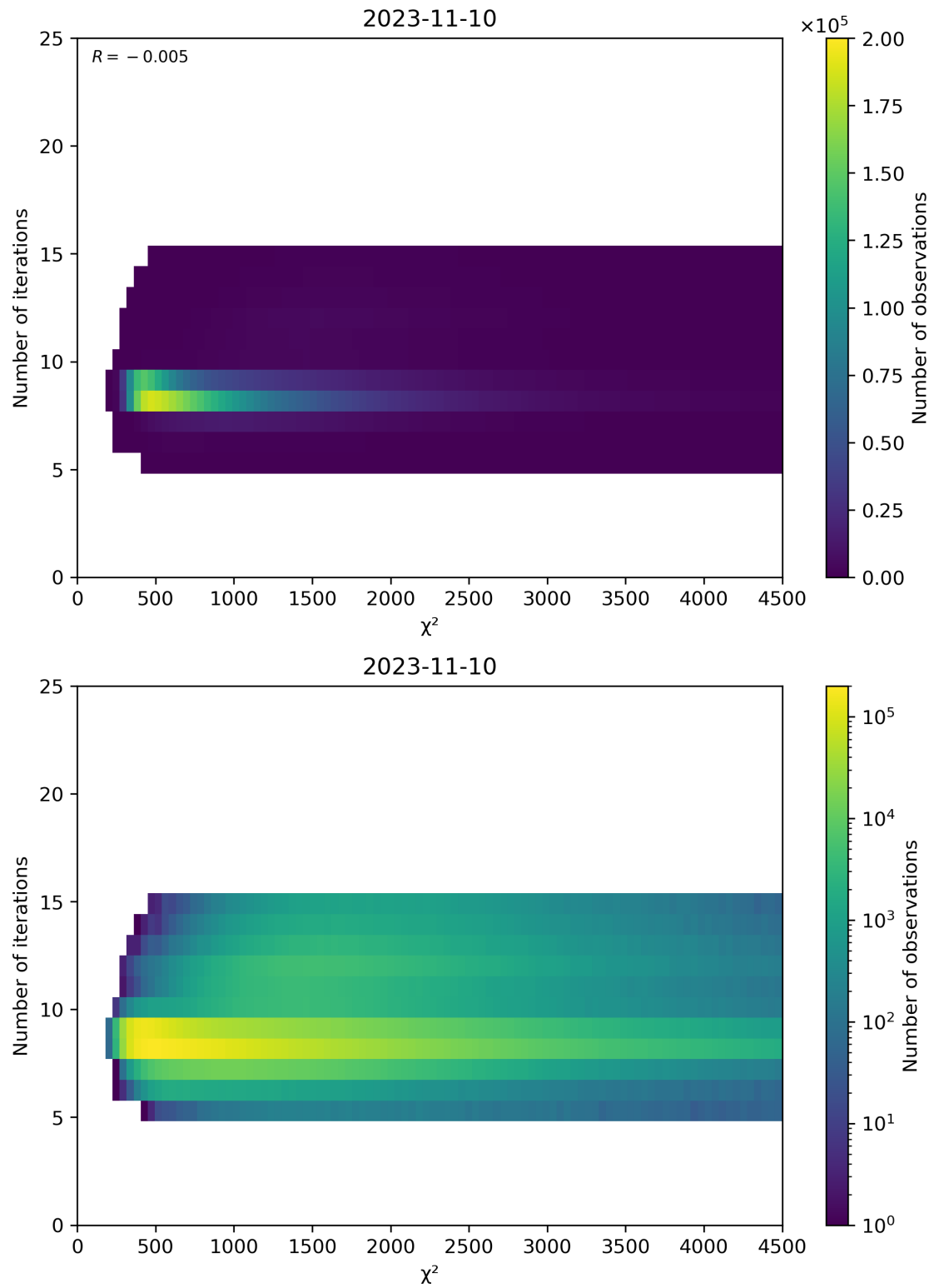
Figure 49: Scatter density plot of “ \chi^2 ” against “Number of iterations” for 2023-11-09 to 2023-11-11.
