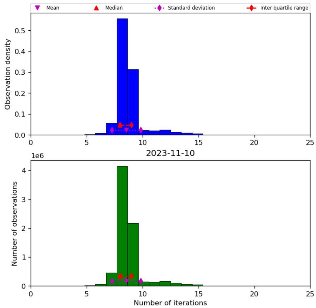
Figure 24: Histogram of “Number of iterations” for 2023-11-09 to 2023-11-11
