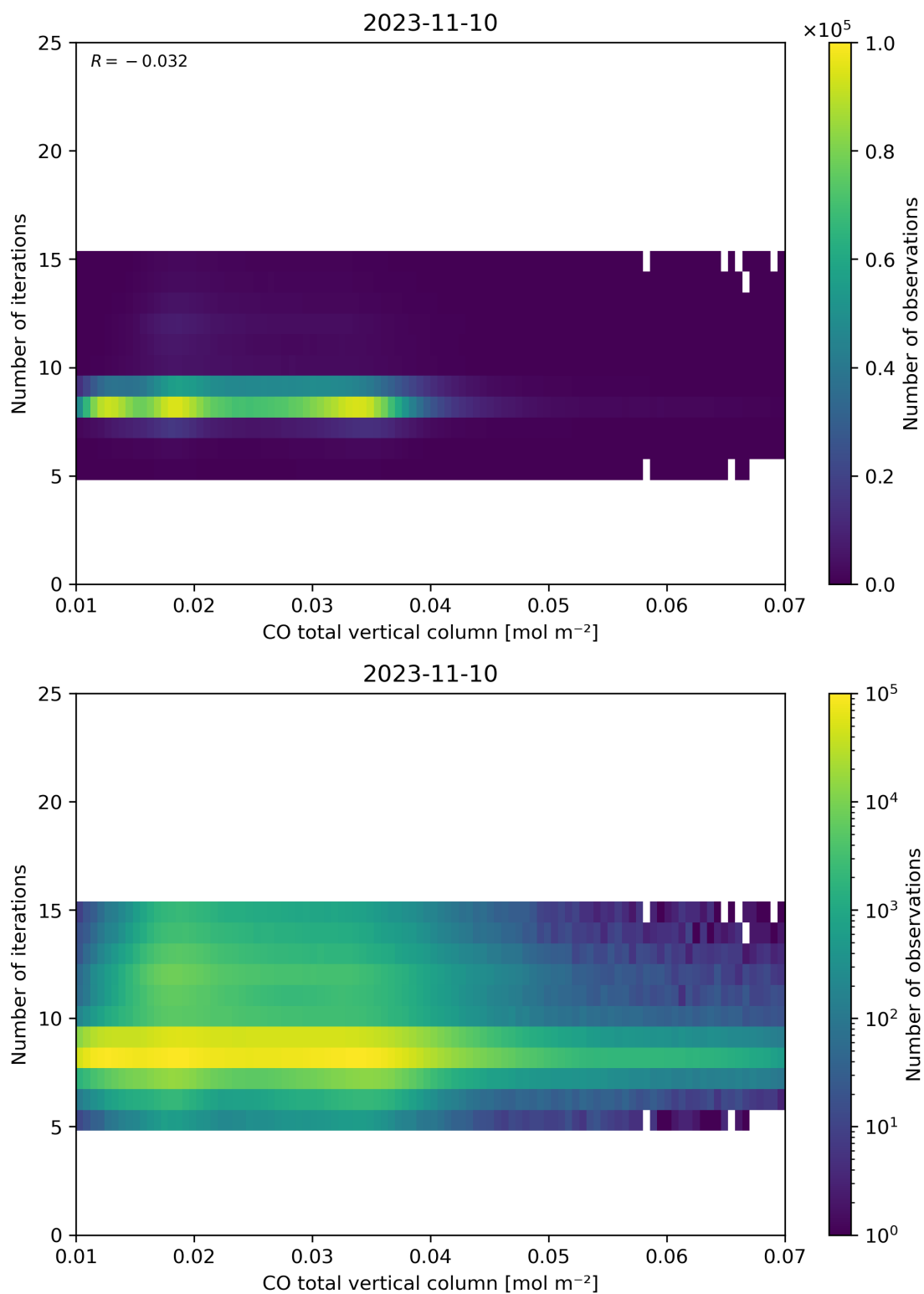
Figure 42: Scatter density plot of “CO total vertical column” against “Number of iterations” for 2023-11-09 to 2023-11-11.
