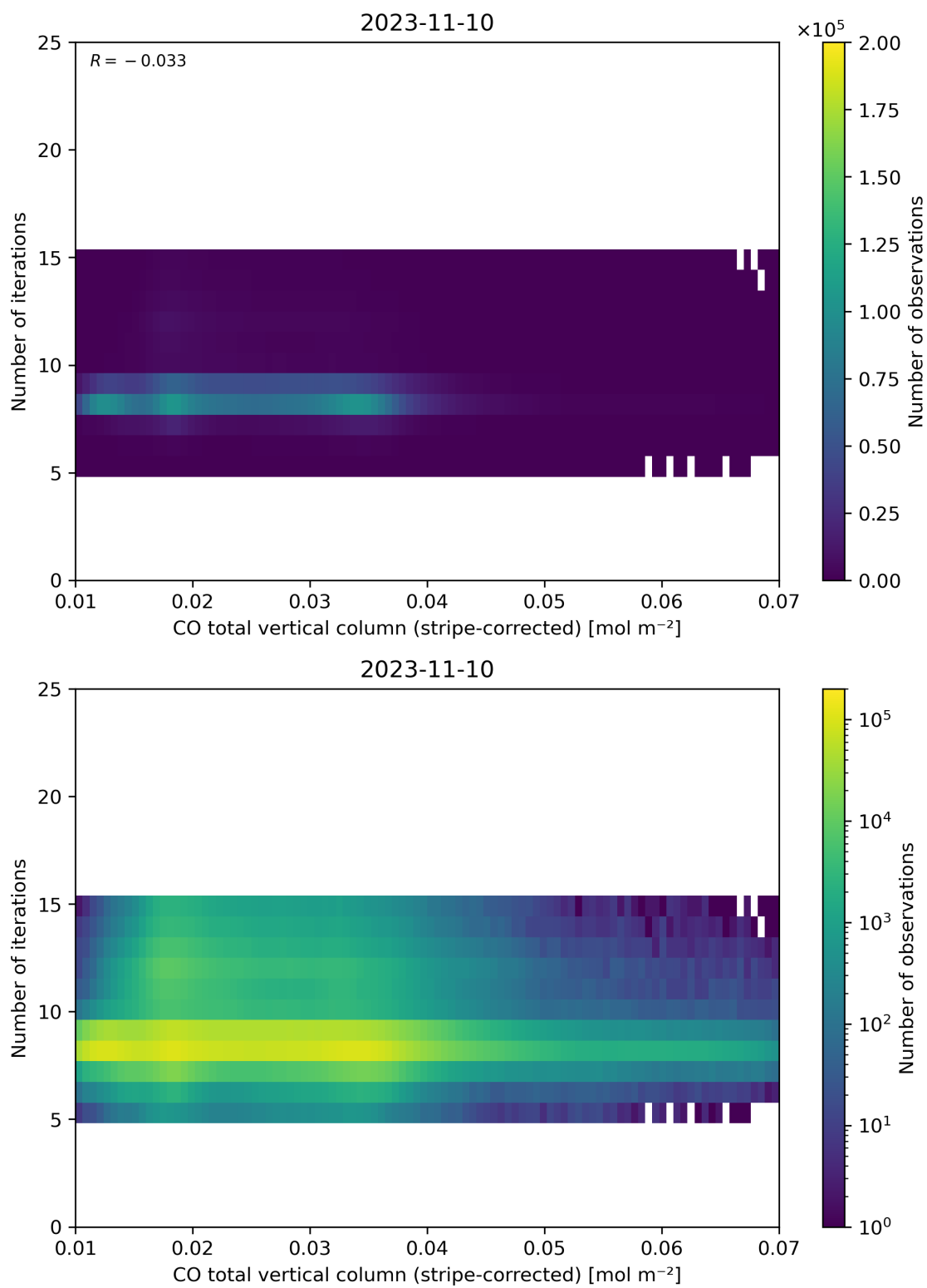
Figure 39: Scatter density plot of “CO total vertical column (stripe-corrected)” against “Number of iterations” for 2023-11-09 to 2023-11-11.
