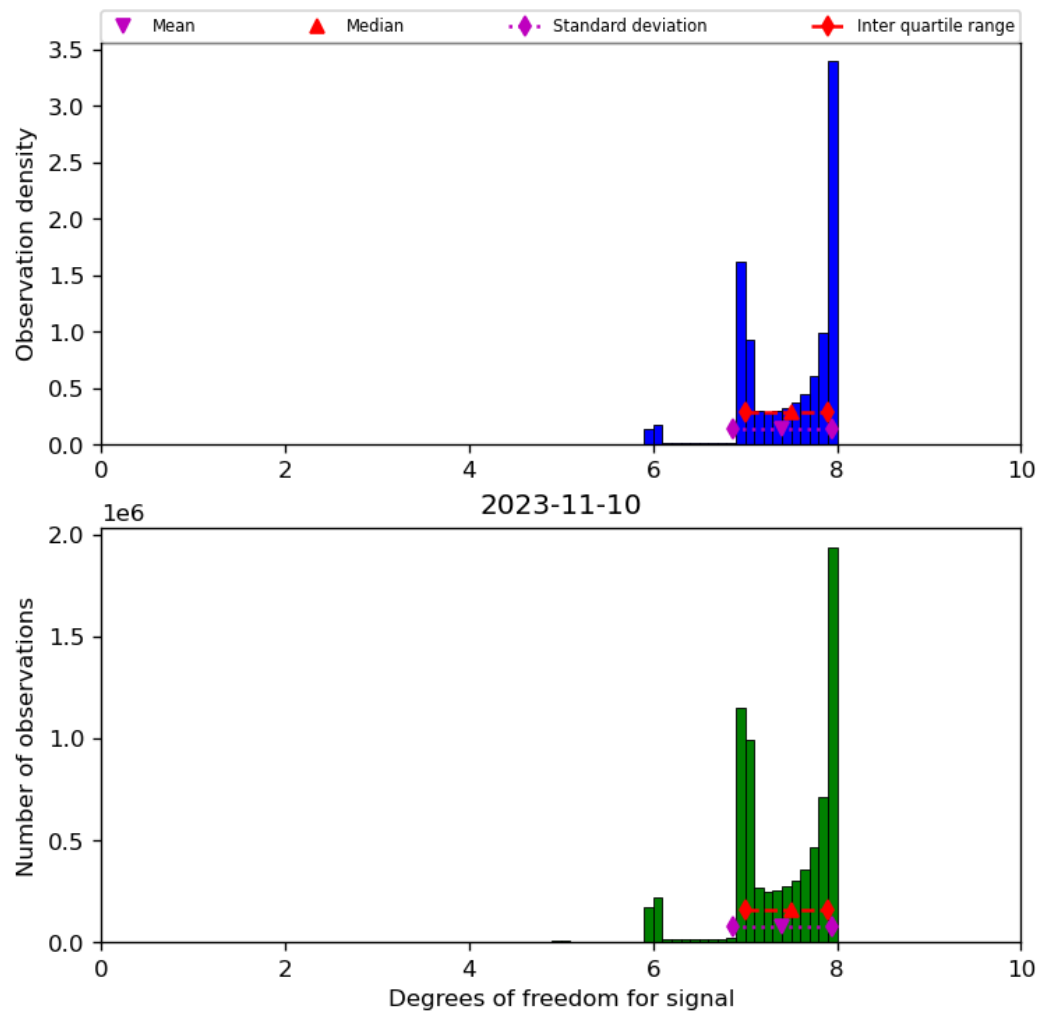
Figure 23: Histogram of “Degrees of freedom for signal” for 2023-11-09 to 2023-11-11
