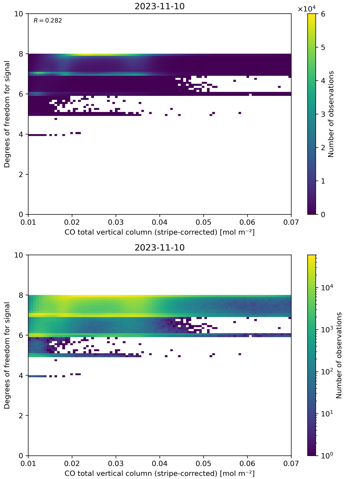
Figure 38: Scatter density plot of “CO total vertical column (stripe-corrected)” against “Degrees of freedom for signal” for 2023-11-09 to 2023-11-11.
