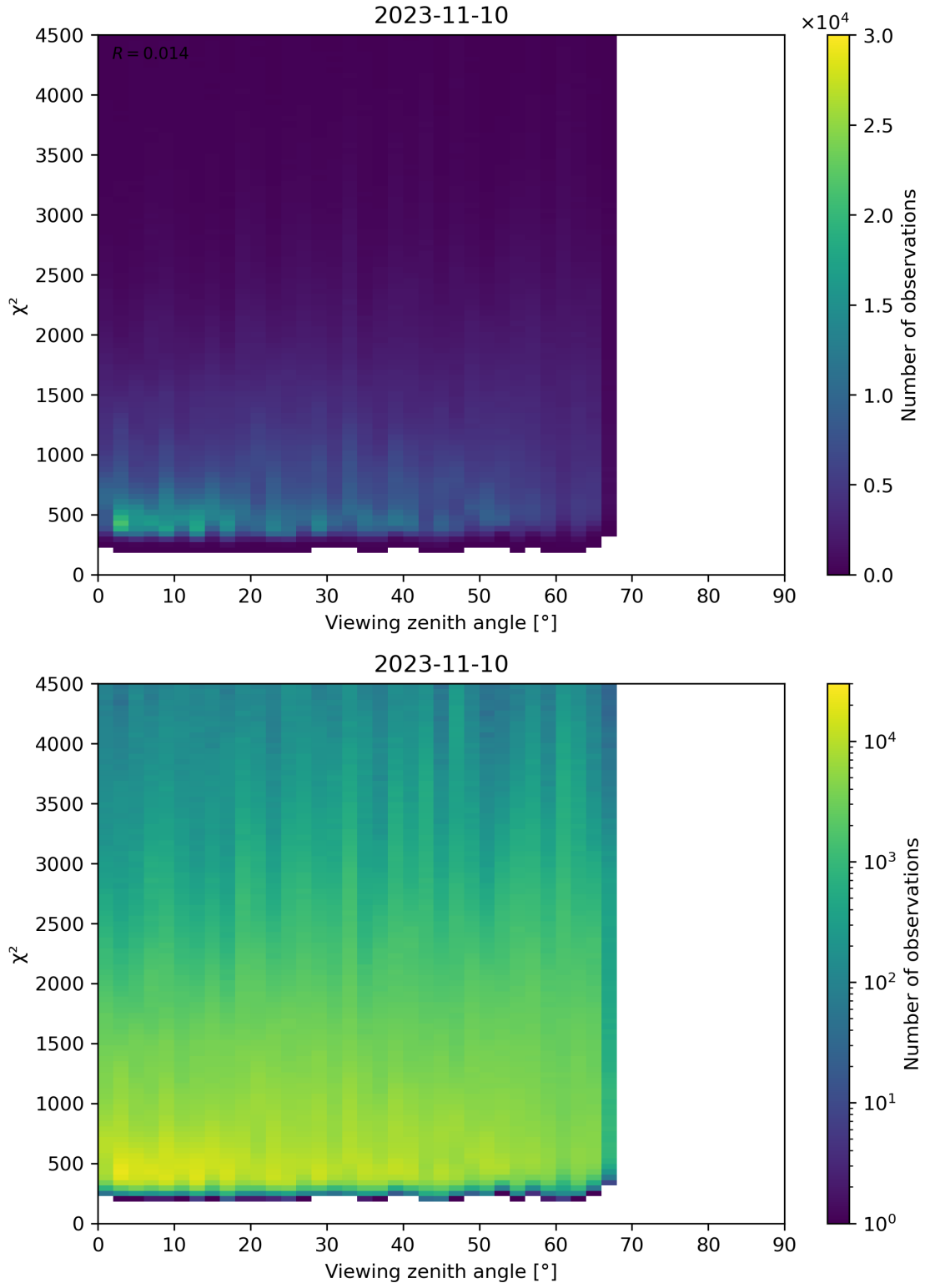
Figure 72: Scatter density plot of “Viewing zenith angle” against “ \chi^2 ” for 2023-11-09 to 2023-11-11.
