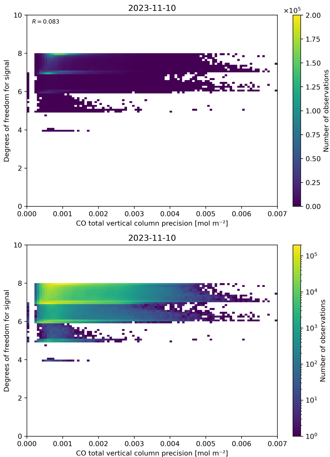
Figure 45: Scatter density plot of “CO total vertical column precision” against “Degrees of freedom for signal” for 2023-11-09 to 2023-11-11.
