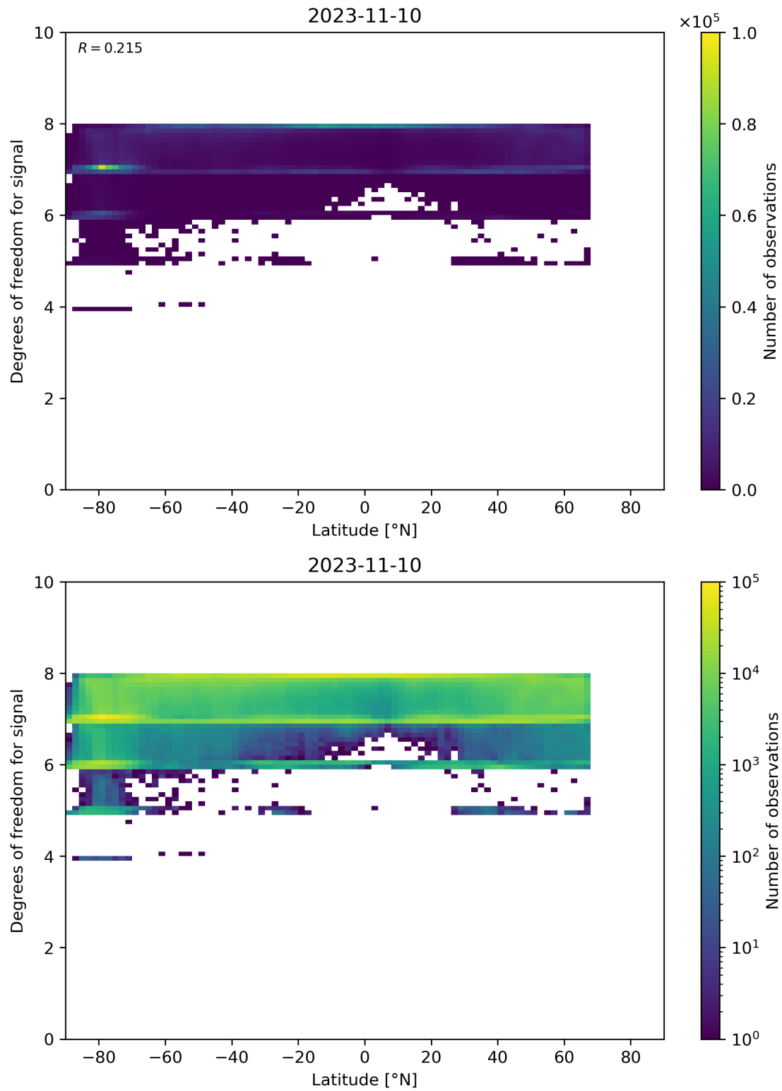
Figure 55: Scatter density plot of “Latitude” against “Degrees of freedom for signal” for 2023-11-09 to 2023-11-11.
