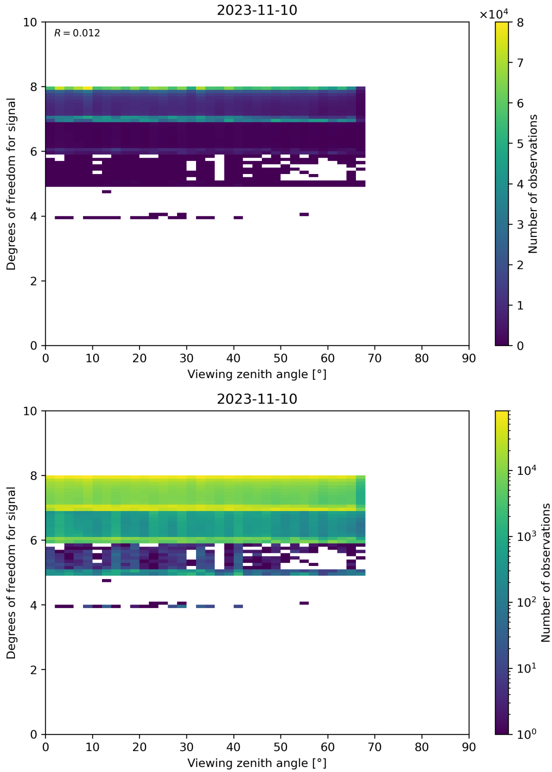
Figure 73: Scatter density plot of “Viewing zenith angle” against “Degrees of freedom for signal” for 2023-11-09 to 2023-11-11.
