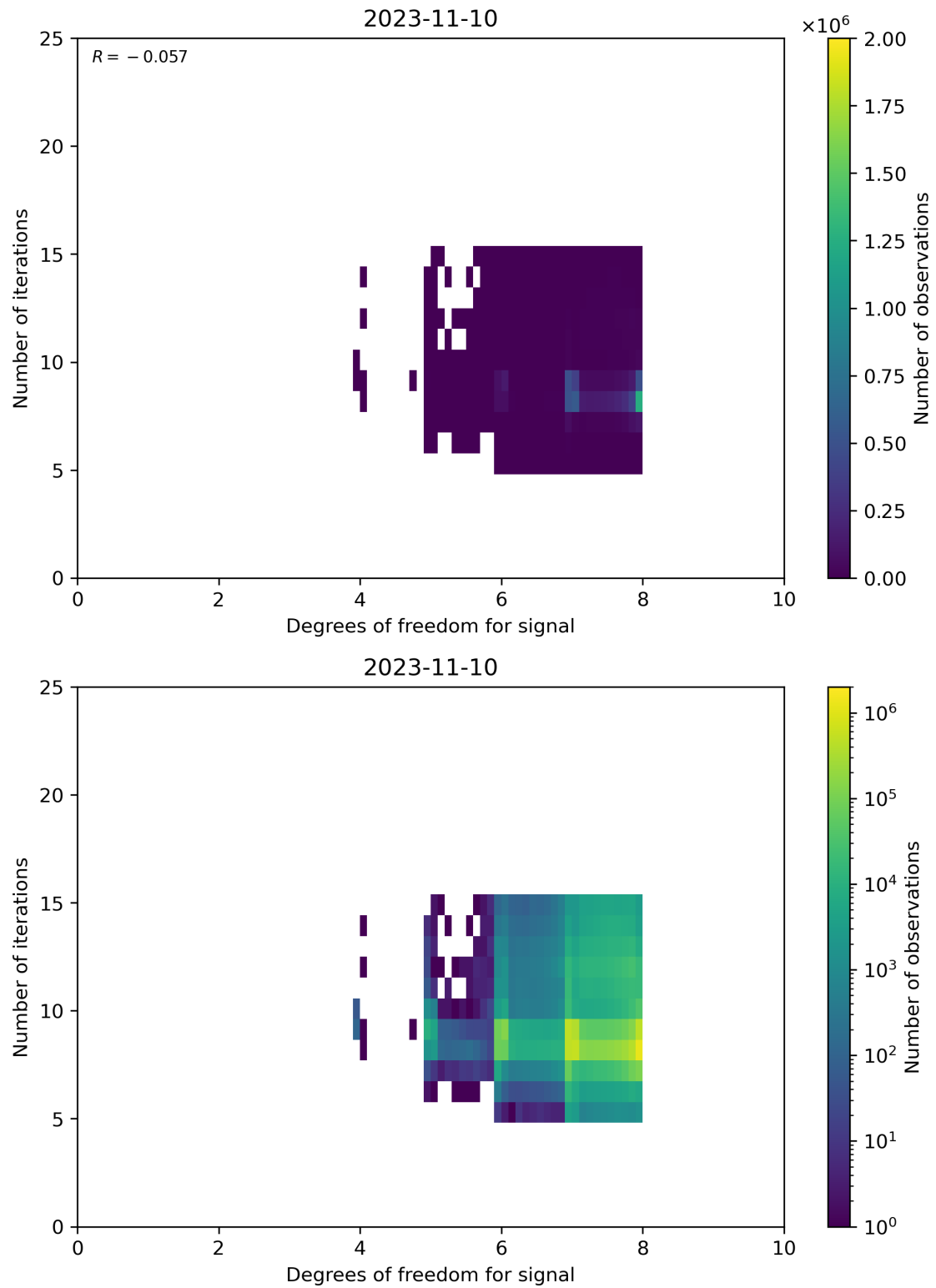
Figure 50: Scatter density plot of “Degrees of freedom for signal” against “Number of iterations” for 2023-11-09 to 2023-11-11.
