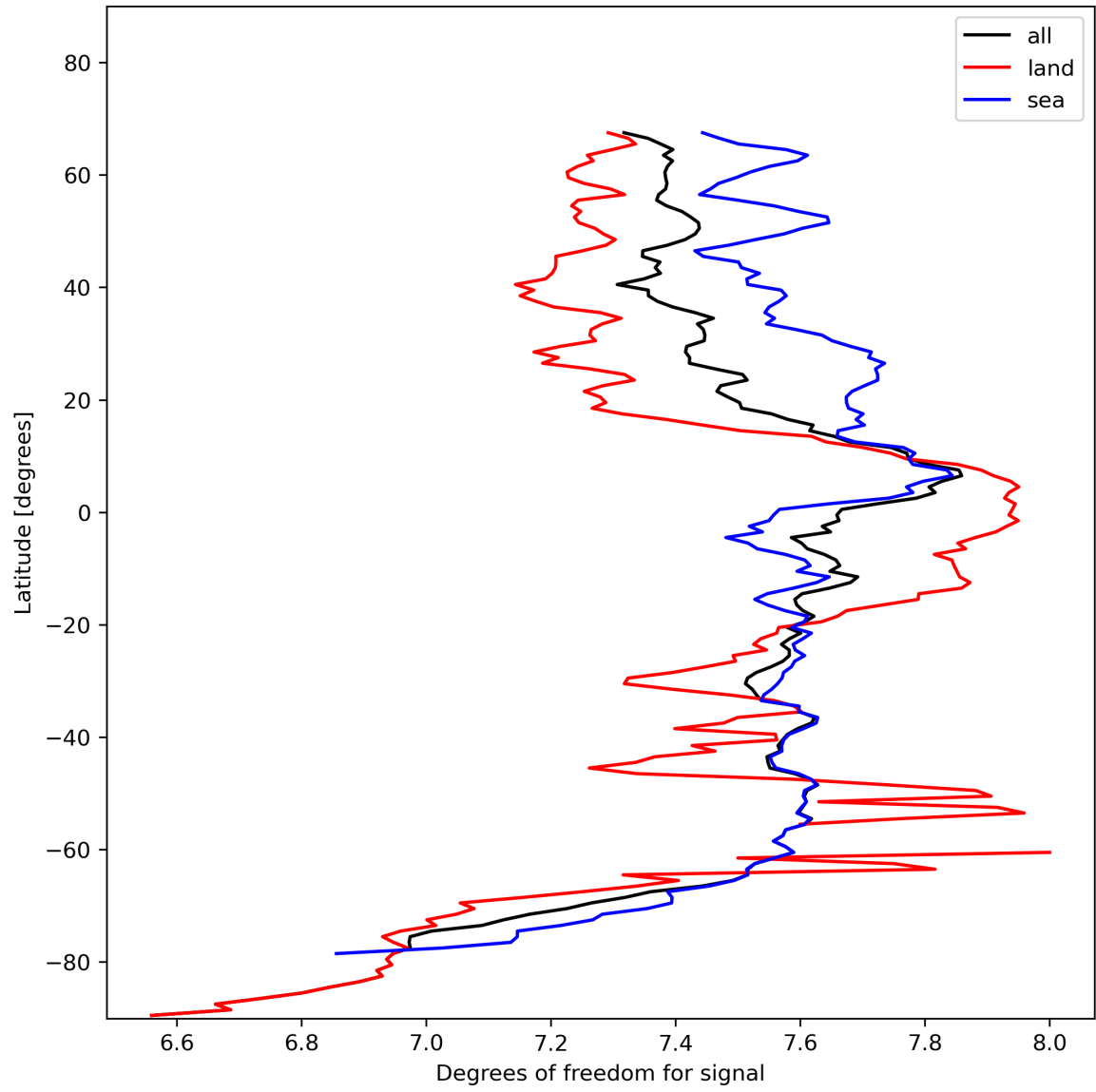
Figure 15: Zonal average of “Degrees of freedom for signal” for 2023-11-09 to 2023-11-11.
