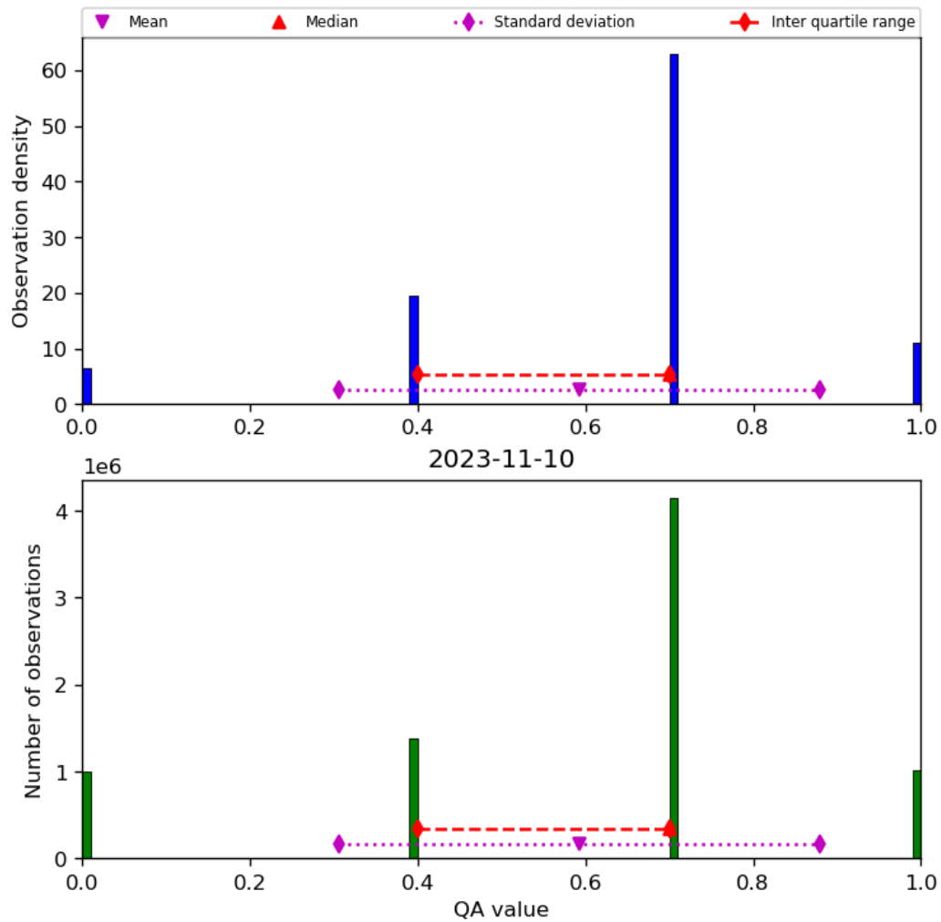
Figure 17: Histogram of “QA value” for 2023-11-09 to 2023-11-11
