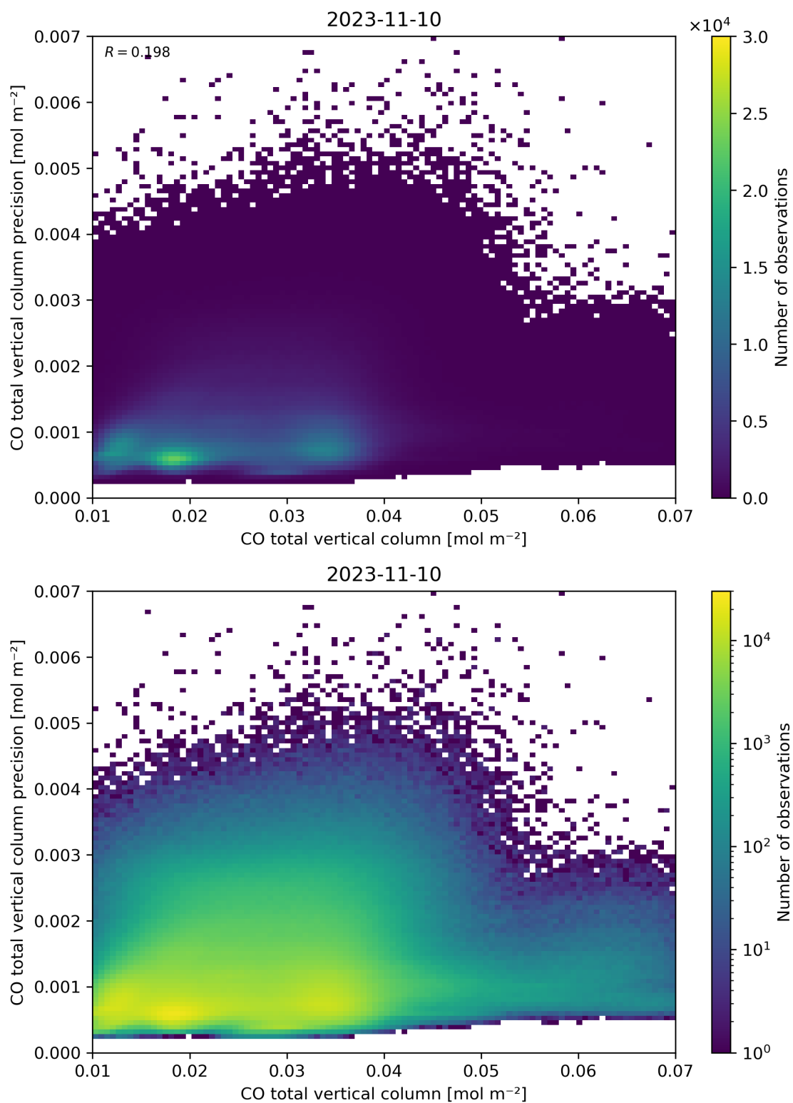
Figure 34: Scatter density plot of “CO total vertical column” against “CO total vertical column precision” for 2023-11-09 to 2023-11-11.
