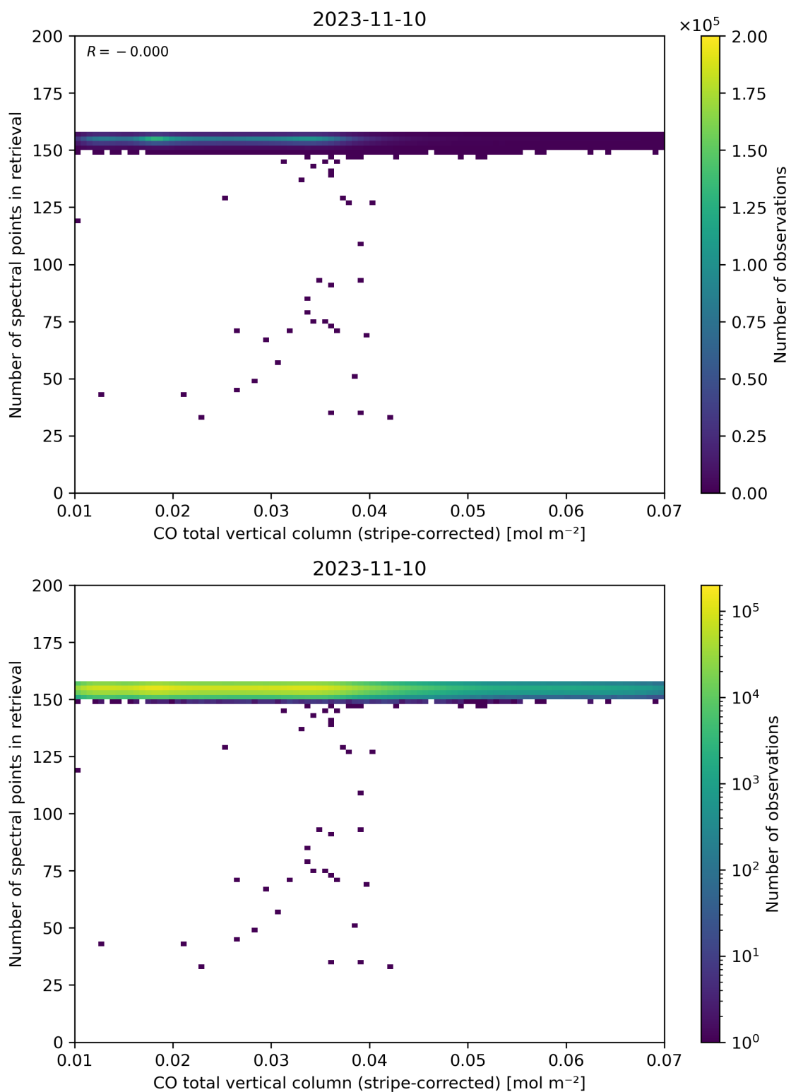
Figure 40: Scatter density plot of “CO total vertical column (stripe-corrected)” against “Number of spectral points in retrieval” for 2023-11-09 to 2023-11-11.
