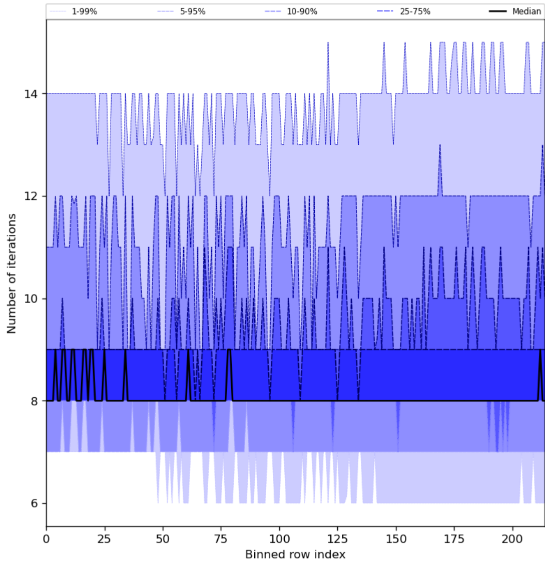
Figure 32: Along track statistics of “Number of iterations” for 2023-11-09 to 2023-11-11
