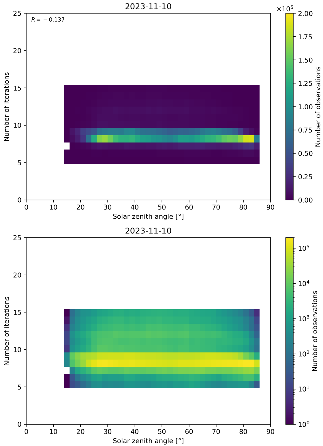
Figure 67: Scatter density plot of “Solar zenith angle” against “Number of iterations” for 2023-11-09 to 2023-11-11.
