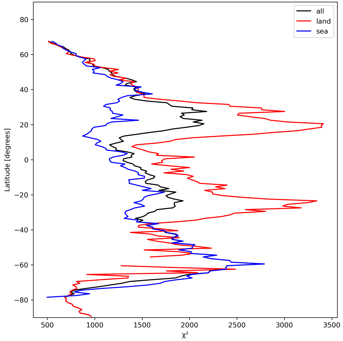
Figure 14: Zonal average of “ \chi^2 ” for 2023-11-09 to 2023-11-11.
