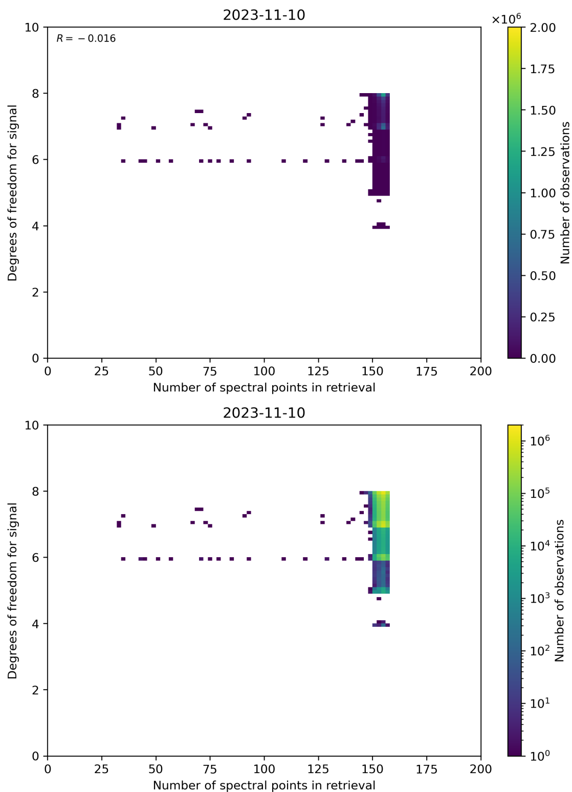
Figure 59: Scatter density plot of “Number of spectral points in retrieval” against “Degrees of freedom for signal” for 2023-11-09 to 2023-11-11.
