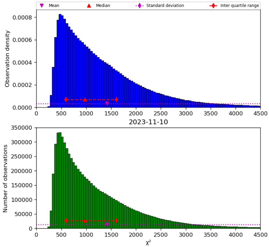
Figure 22: Histogram of “ \chi^2 ” for 2023-11-09 to 2023-11-11
