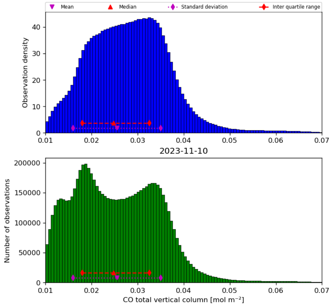
Figure 18: Histogram of “CO total vertical column” for 2023-11-09 to 2023-11-11
