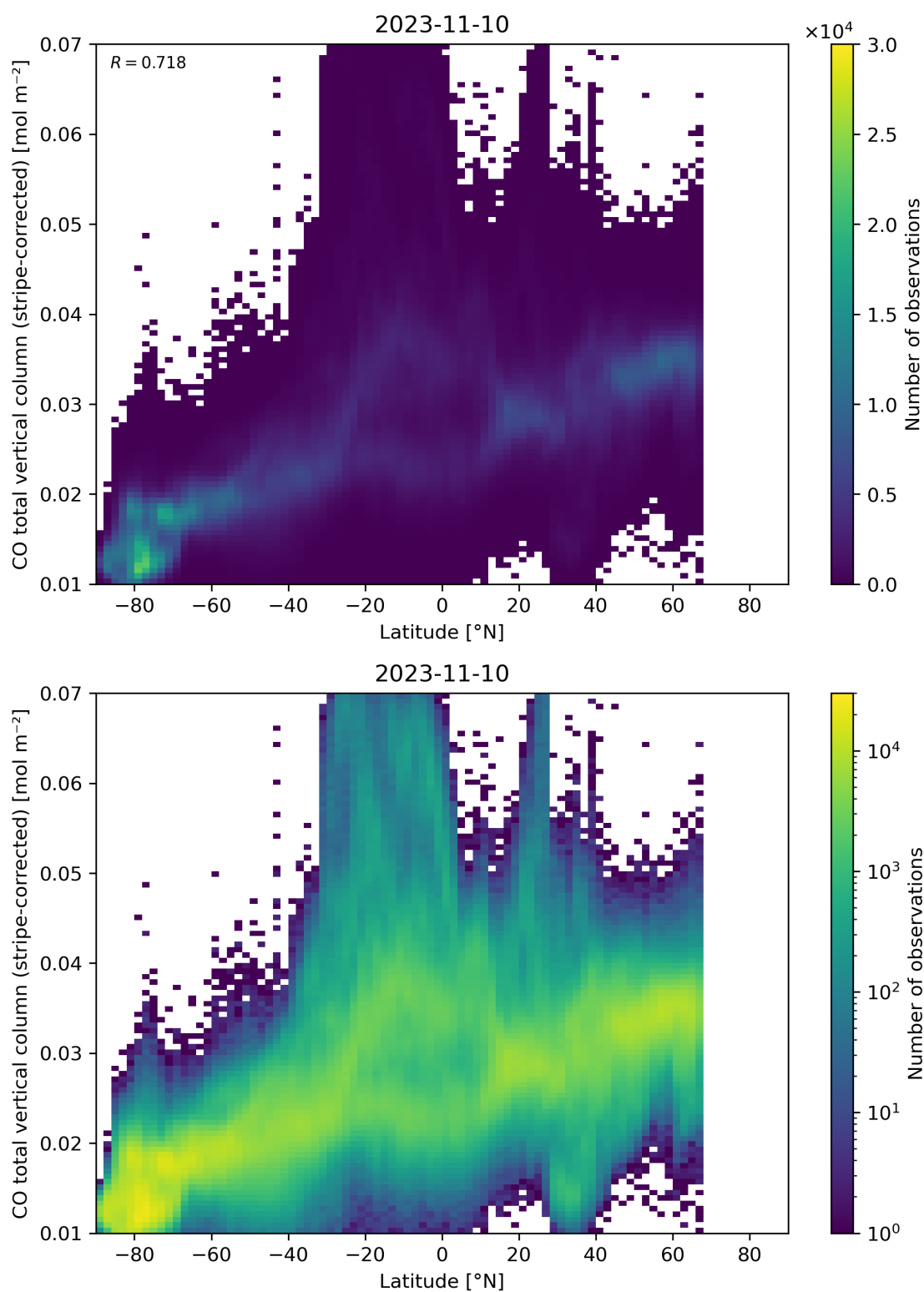
Figure 52: Scatter density plot of “Latitude” against “CO total vertical column (stripe-corrected)” for 2023-11-09 to 2023-11-11.
