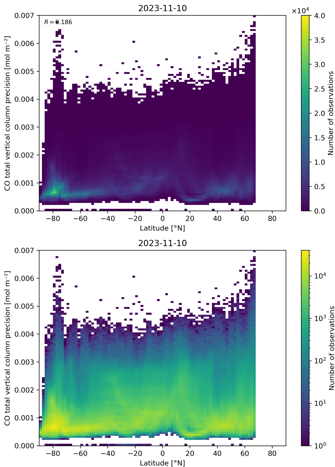
Figure 53: Scatter density plot of “Latitude” against “CO total vertical column precision” for 2023-11-09 to 2023-11-11.
