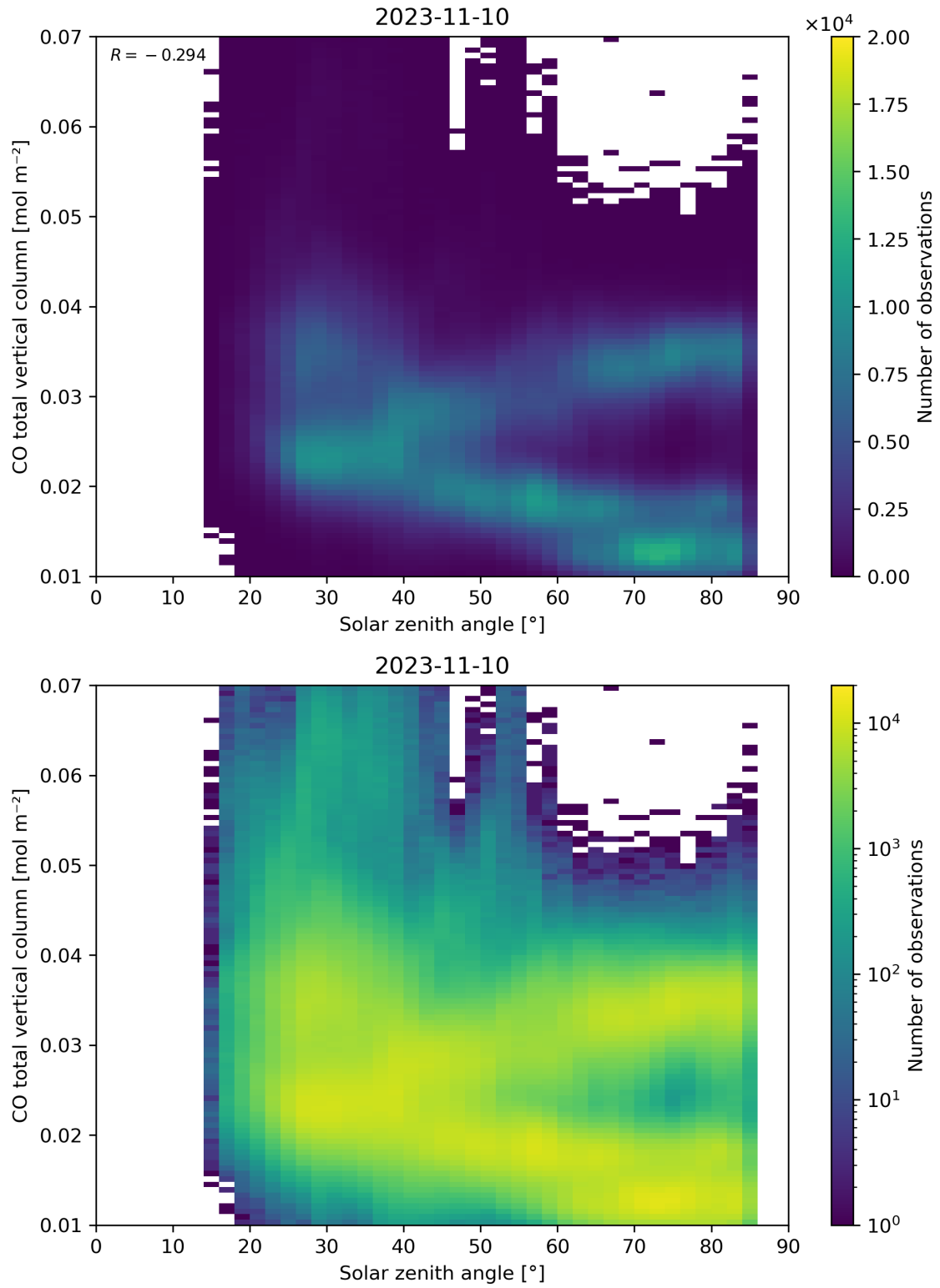
Figure 61: Scatter density plot of “Solar zenith angle” against “CO total vertical column” for 2023-11-09 to 2023-11-11.
