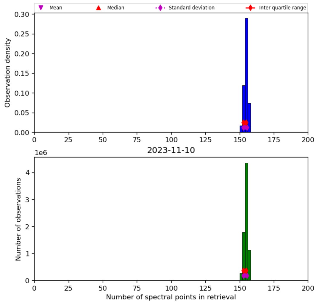
Figure 21: Histogram of “Number of spectral points in retrieval” for 2023-11-09 to 2023-11-11
