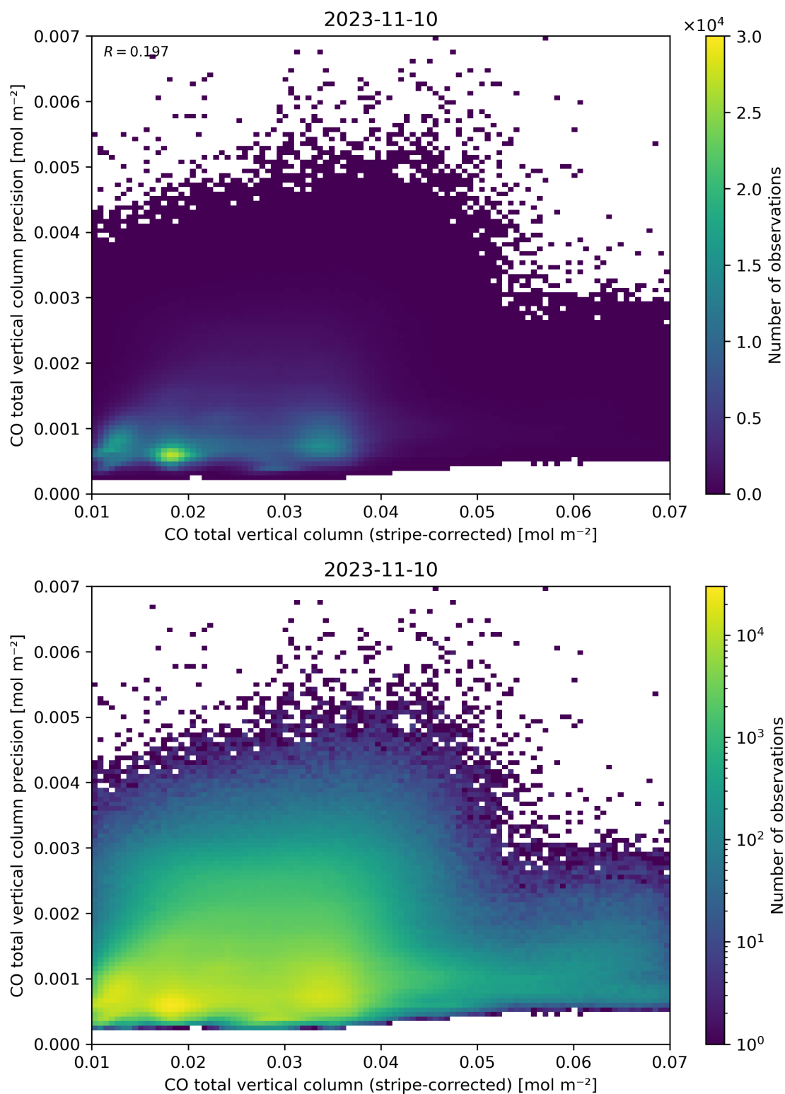
Figure 36: Scatter density plot of “CO total vertical column (stripe-corrected)” against “CO total vertical column precision” for 2023-11-09 to 2023-11-11.
