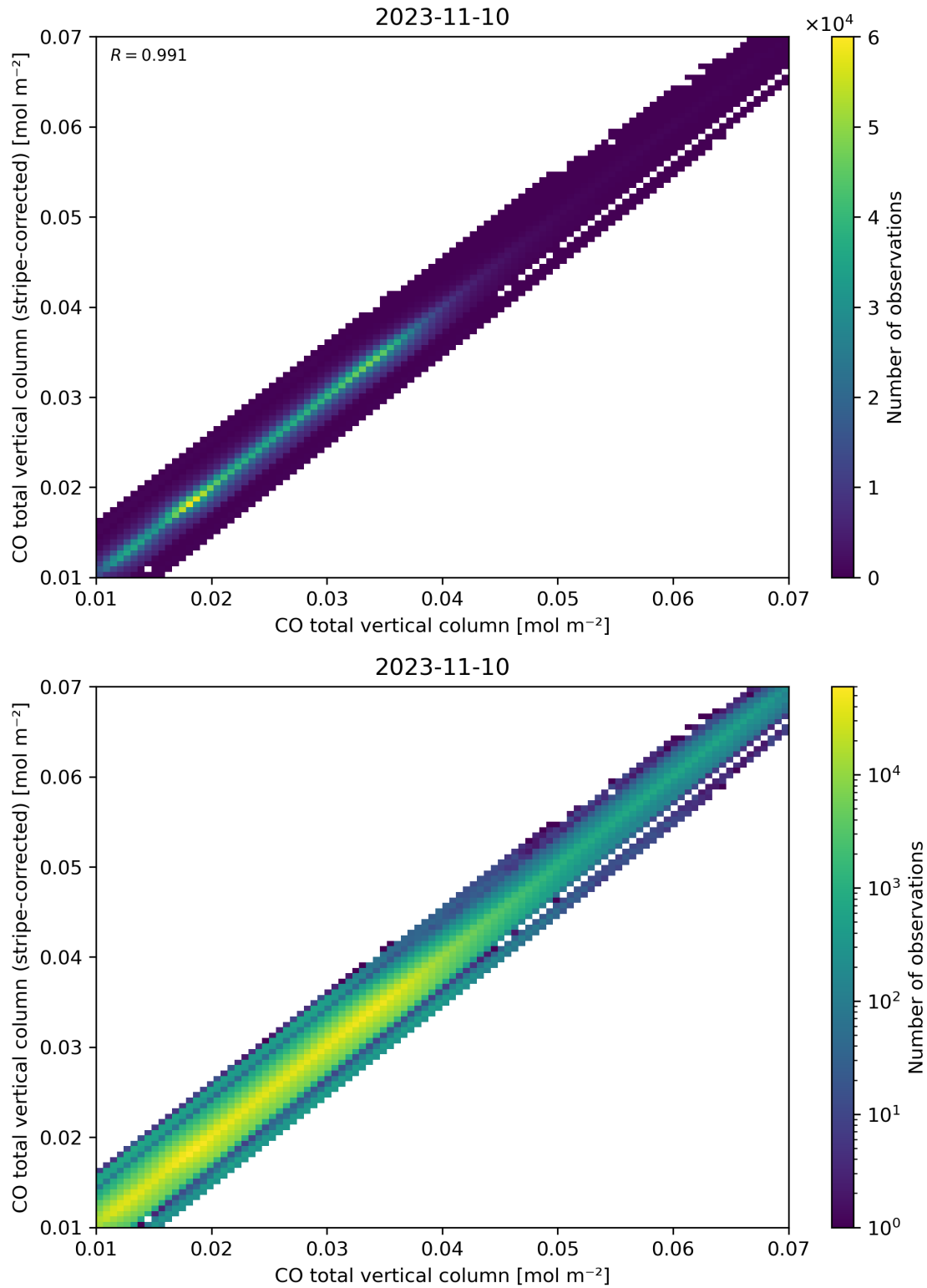
Figure 33: Scatter density plot of “CO total vertical column” against “CO total vertical column (stripe-corrected)” for 2023-11-09 to 2023-11-11.
