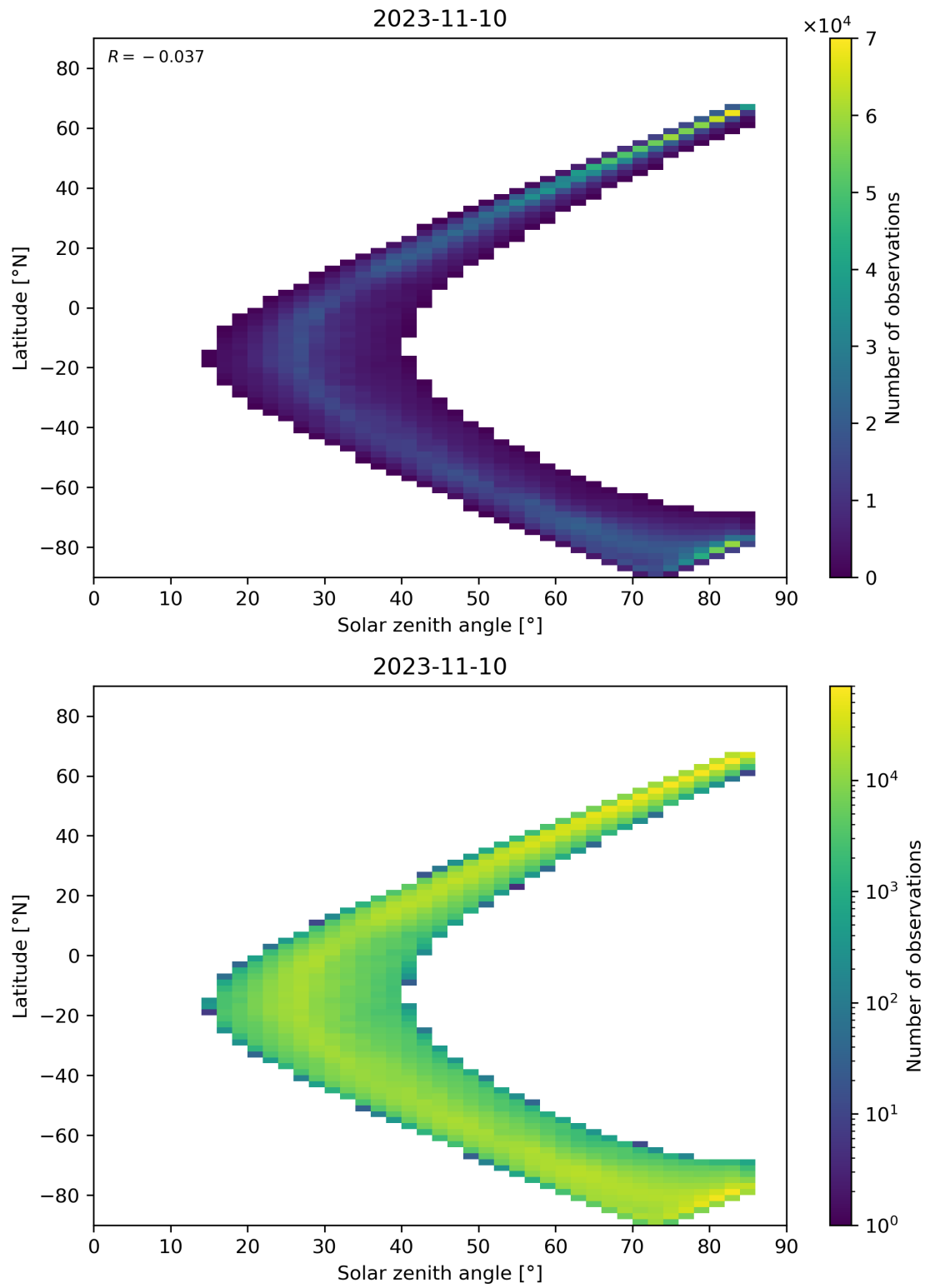
Figure 66: Scatter density plot of “Solar zenith angle” against “Latitude” for 2023-11-09 to 2023-11-11.
