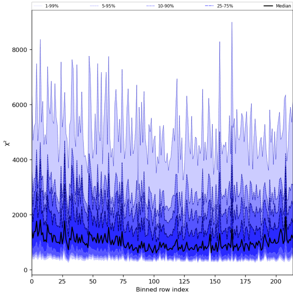
Figure 30: Along track statistics of “ \chi^2 ” for 2023-11-09 to 2023-11-11
