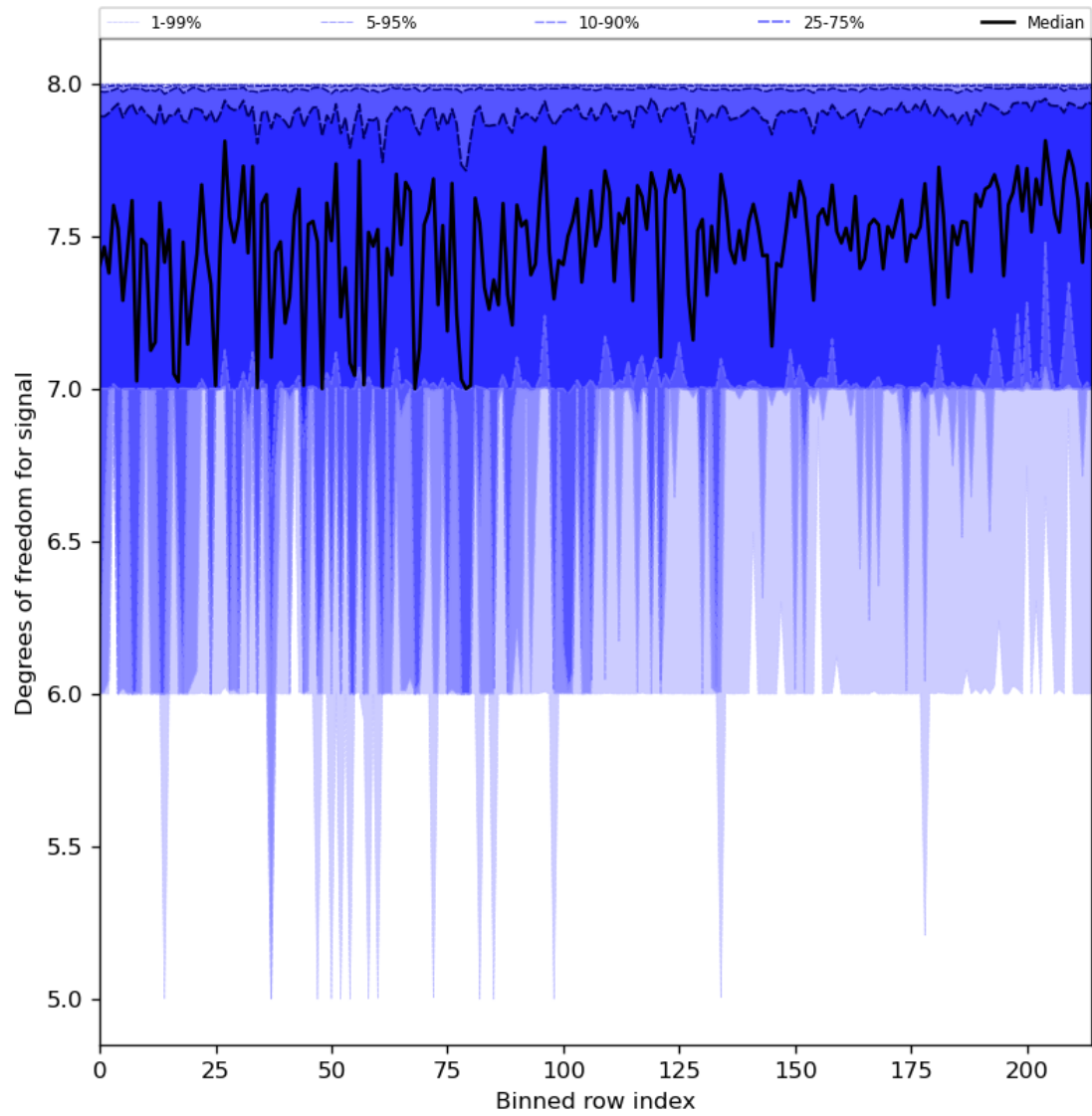
Figure 31: Along track statistics of “Degrees of freedom for signal” for 2023-11-09 to 2023-11-11
