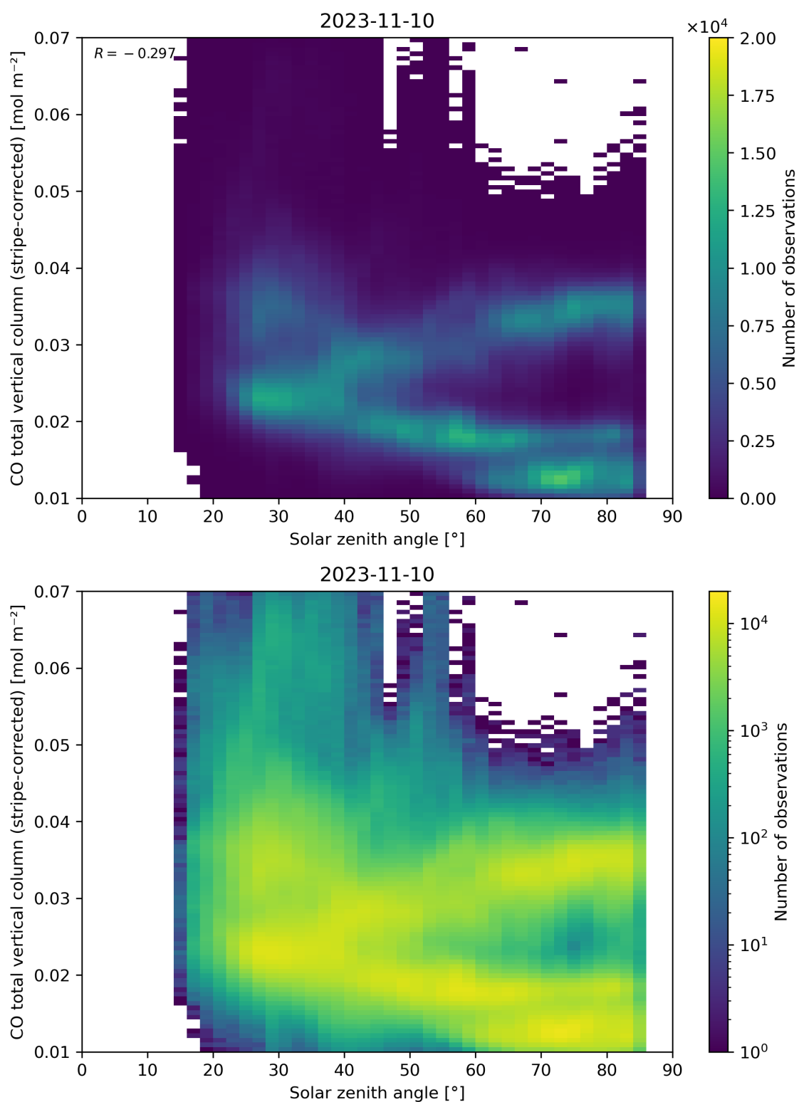
Figure 62: Scatter density plot of “Solar zenith angle” against “CO total vertical column (stripe-corrected)” for 2023-11-09 to 2023-11-11.
