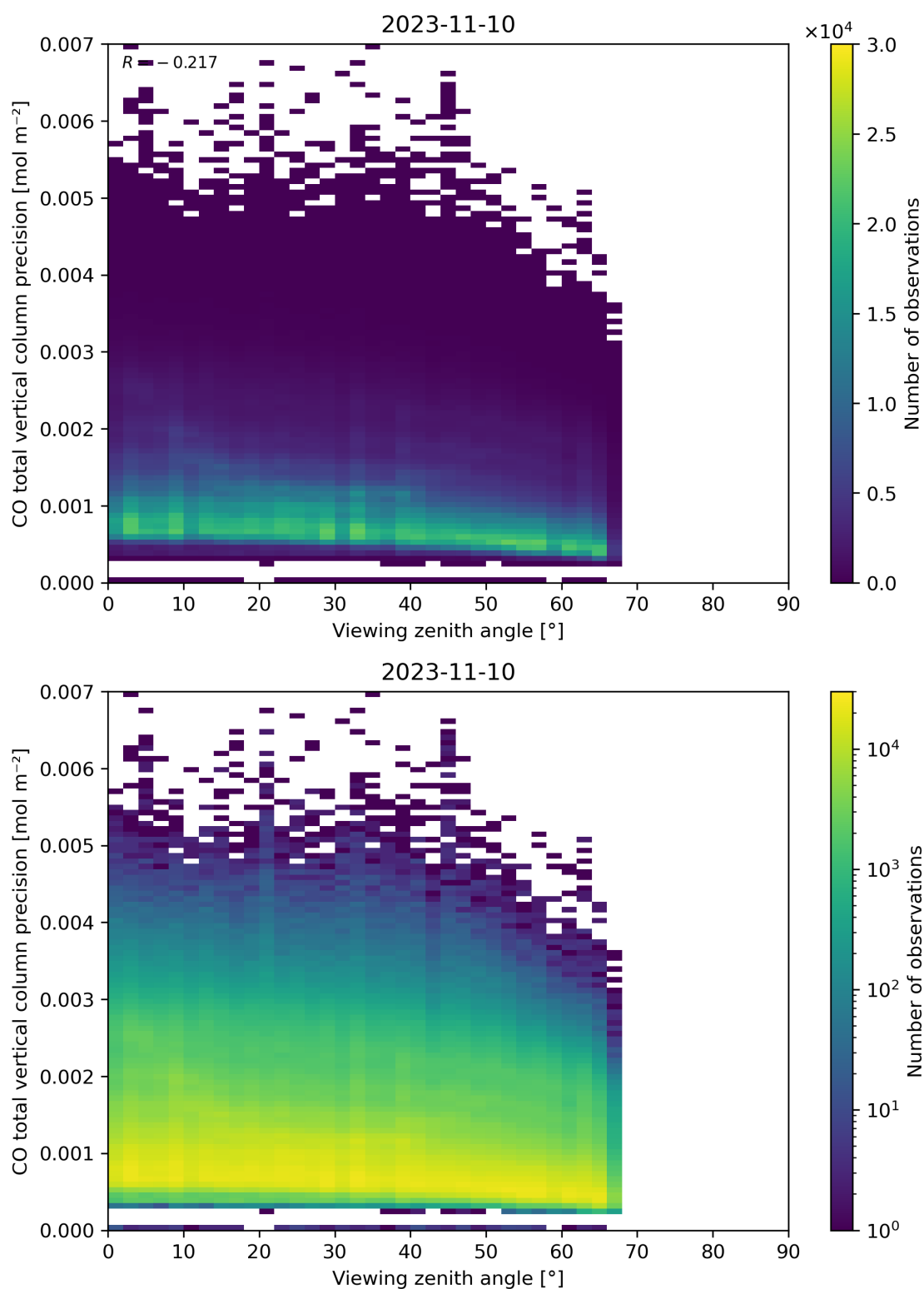
Figure 71: Scatter density plot of “Viewing zenith angle” against “CO total vertical column precision” for 2023-11-09 to 2023-11-11.
