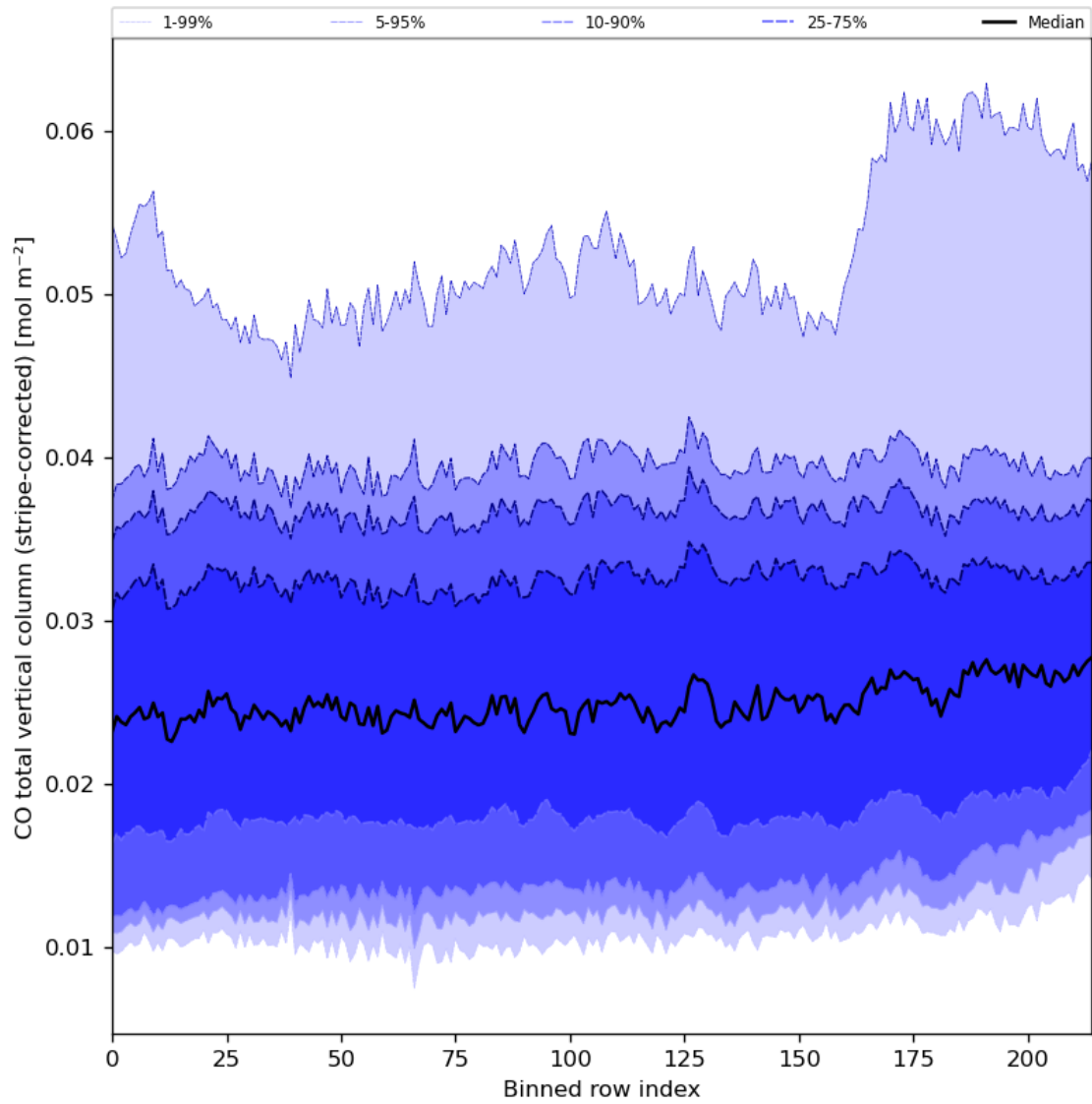
Figure 27: Along track statistics of “CO total vertical column (stripe-corrected)” for 2023-11-09 to 2023-11-11
