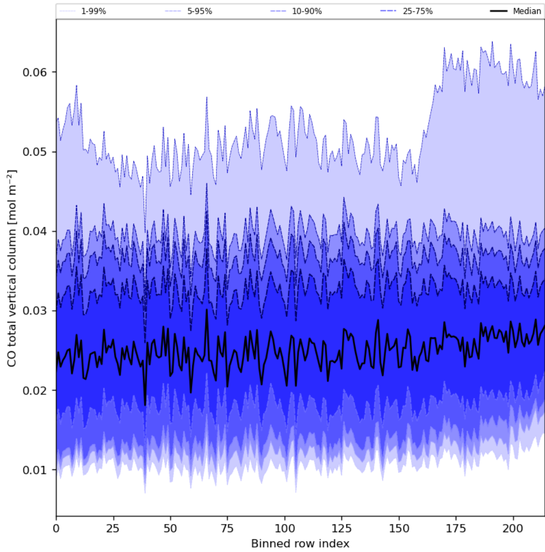
Figure 26: Along track statistics of “CO total vertical column” for 2023-11-09 to 2023-11-11
