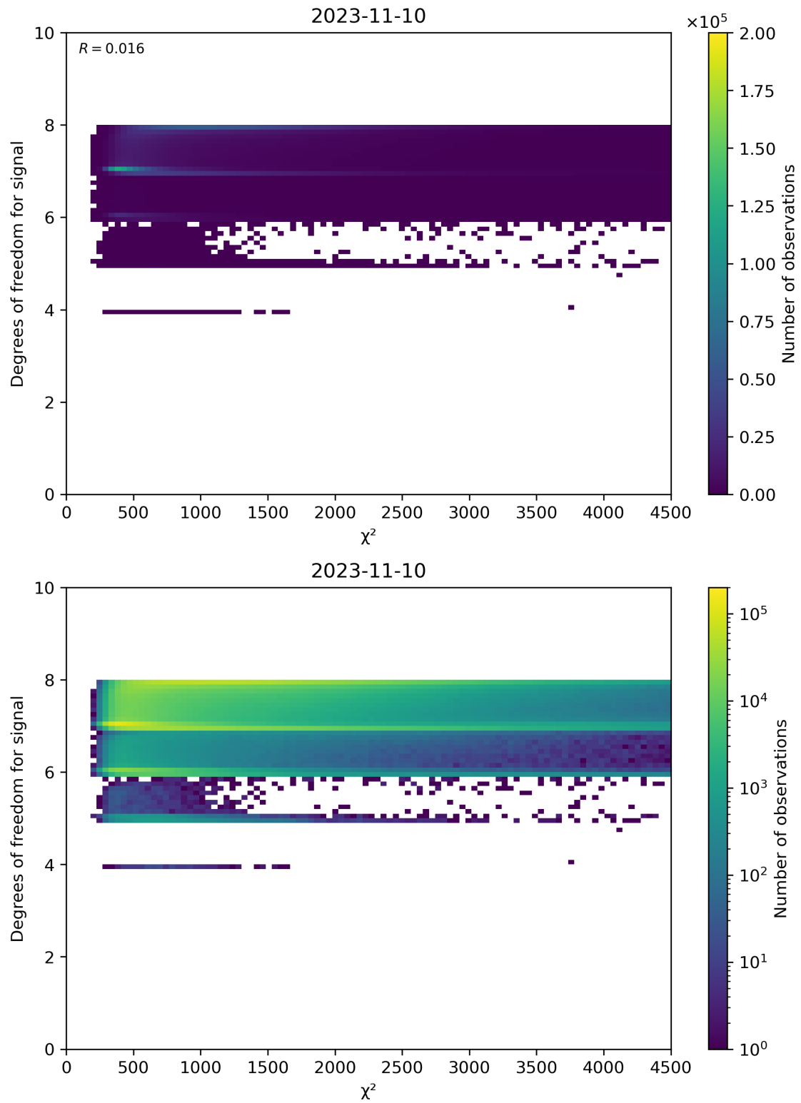
Figure 48: Scatter density plot of “ \chi^2 ” against “Degrees of freedom for signal” for 2023-11-09 to 2023-11-11.
