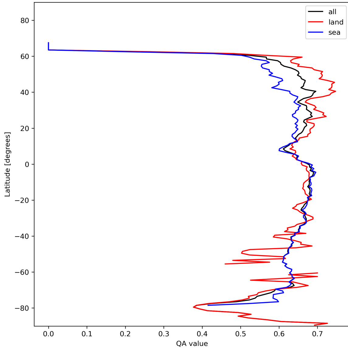
Figure 9: Zonal average of “QA value” for 2023-11-09 to 2023-11-11.
