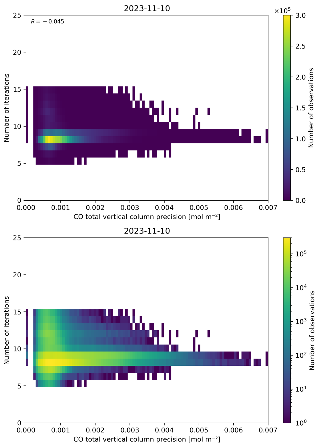
Figure 46: Scatter density plot of “CO total vertical column precision” against “Number of iterations” for 2023-11-09 to 2023-11-11.
