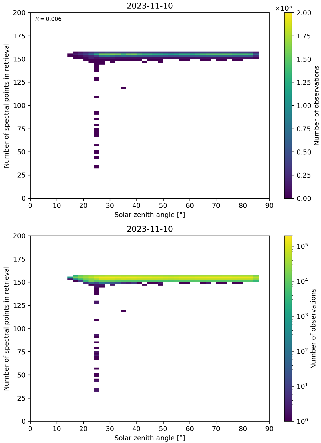
Figure 68: Scatter density plot of “Solar zenith angle” against “Number of spectral points in retrieval” for 2023-11-09 to 2023-11-11.
