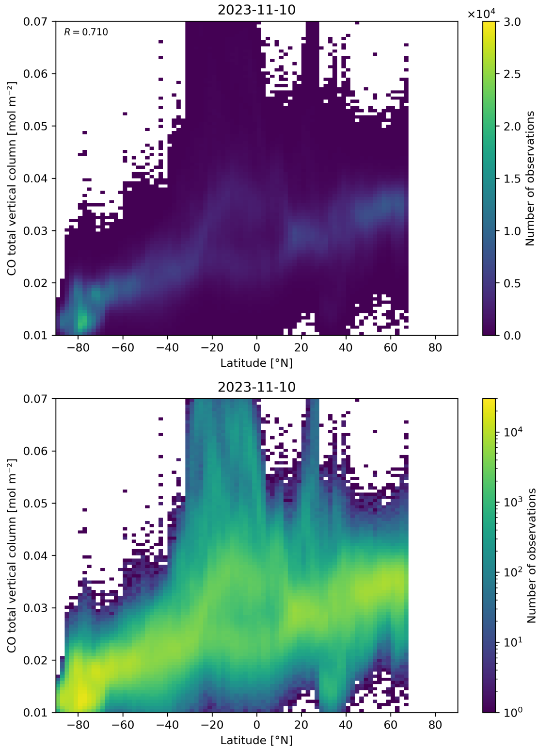
Figure 51: Scatter density plot of “Latitude” against “CO total vertical column” for 2023-11-09 to 2023-11-11.
