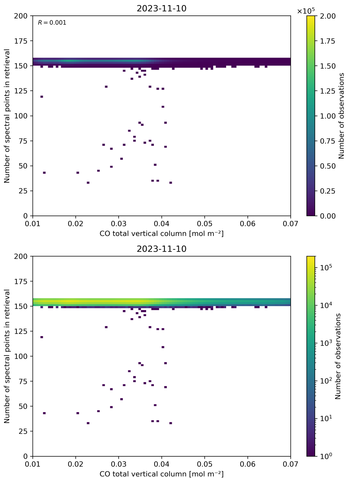
Figure 43: Scatter density plot of “CO total vertical column” against “Number of spectral points in retrieval” for 2023-11-09 to 2023-11-11.
