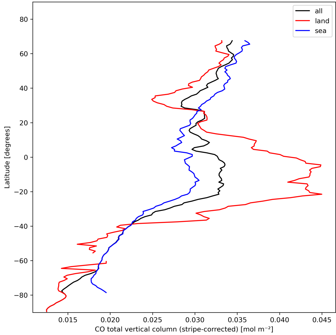
Figure 11: Zonal average of “CO total vertical column (stripe-corrected)” for 2023-11-09 to 2023-11-11.
