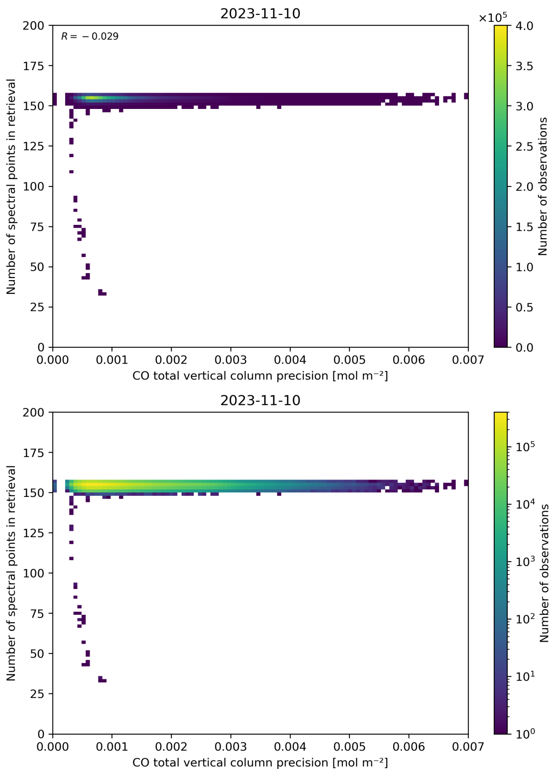
Figure 47: Scatter density plot of “CO total vertical column precision” against “Number of spectral points in retrieval” for 2023-11-09 to 2023-11-11.
