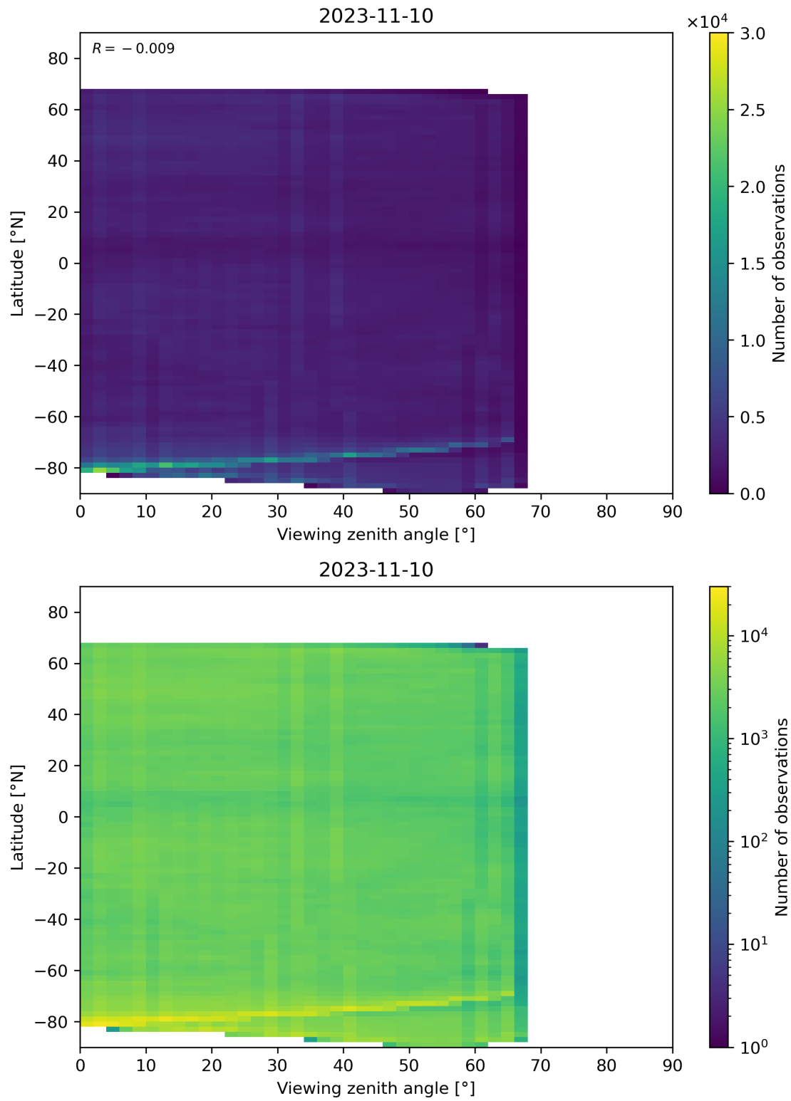
Figure 74: Scatter density plot of “Viewing zenith angle” against “Latitude” for 2023-11-09 to 2023-11-11.
