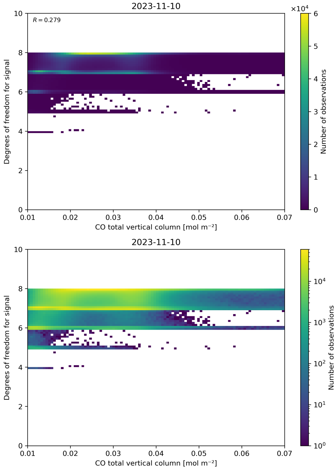
Figure 41: Scatter density plot of “CO total vertical column” against “Degrees of freedom for signal” for 2023-11-09 to 2023-11-11.
