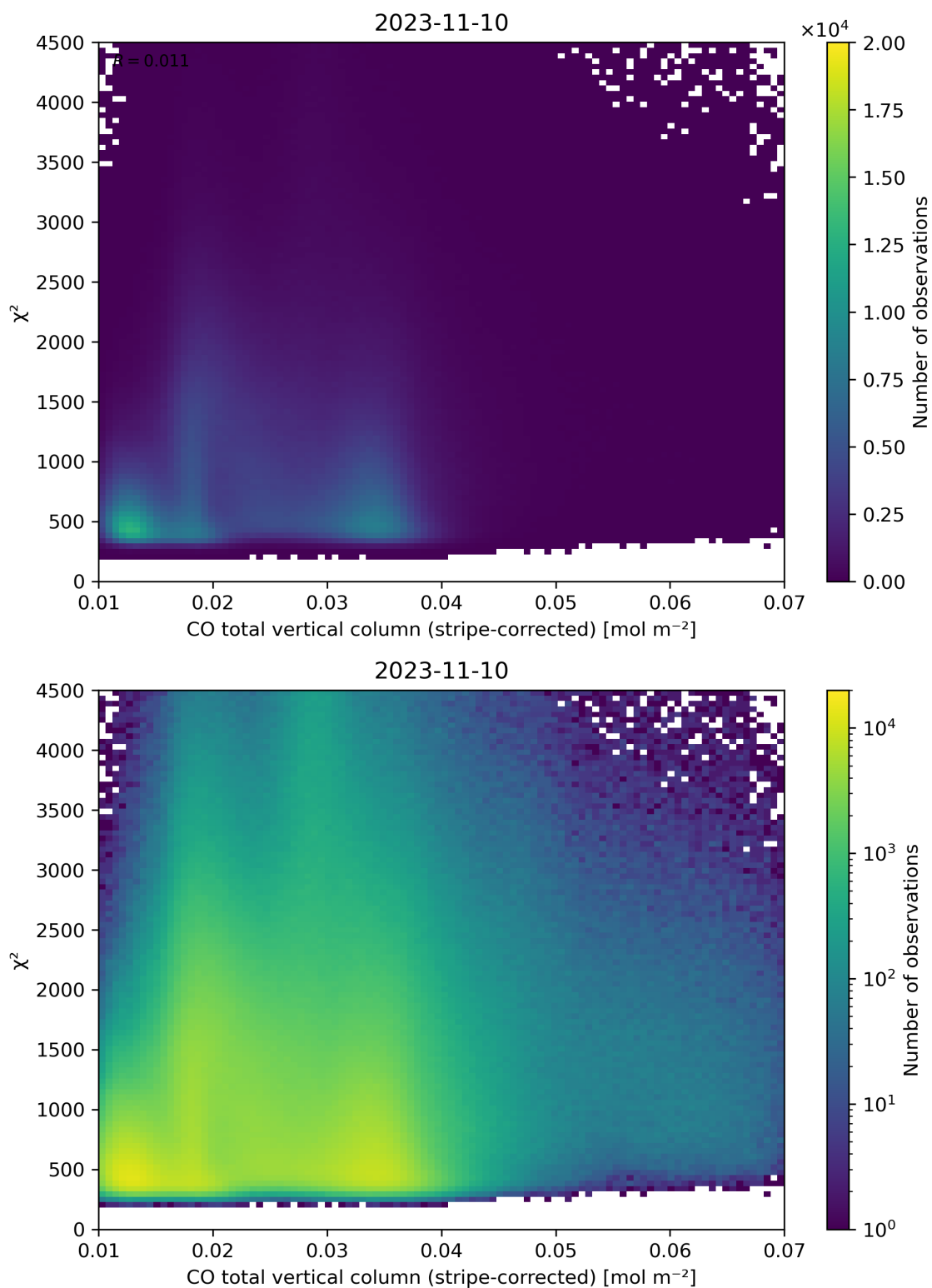
Figure 37: Scatter density plot of “CO total vertical column (stripe-corrected)” against “ \chi^2 ” for 2023-11-09 to 2023-11-11.
