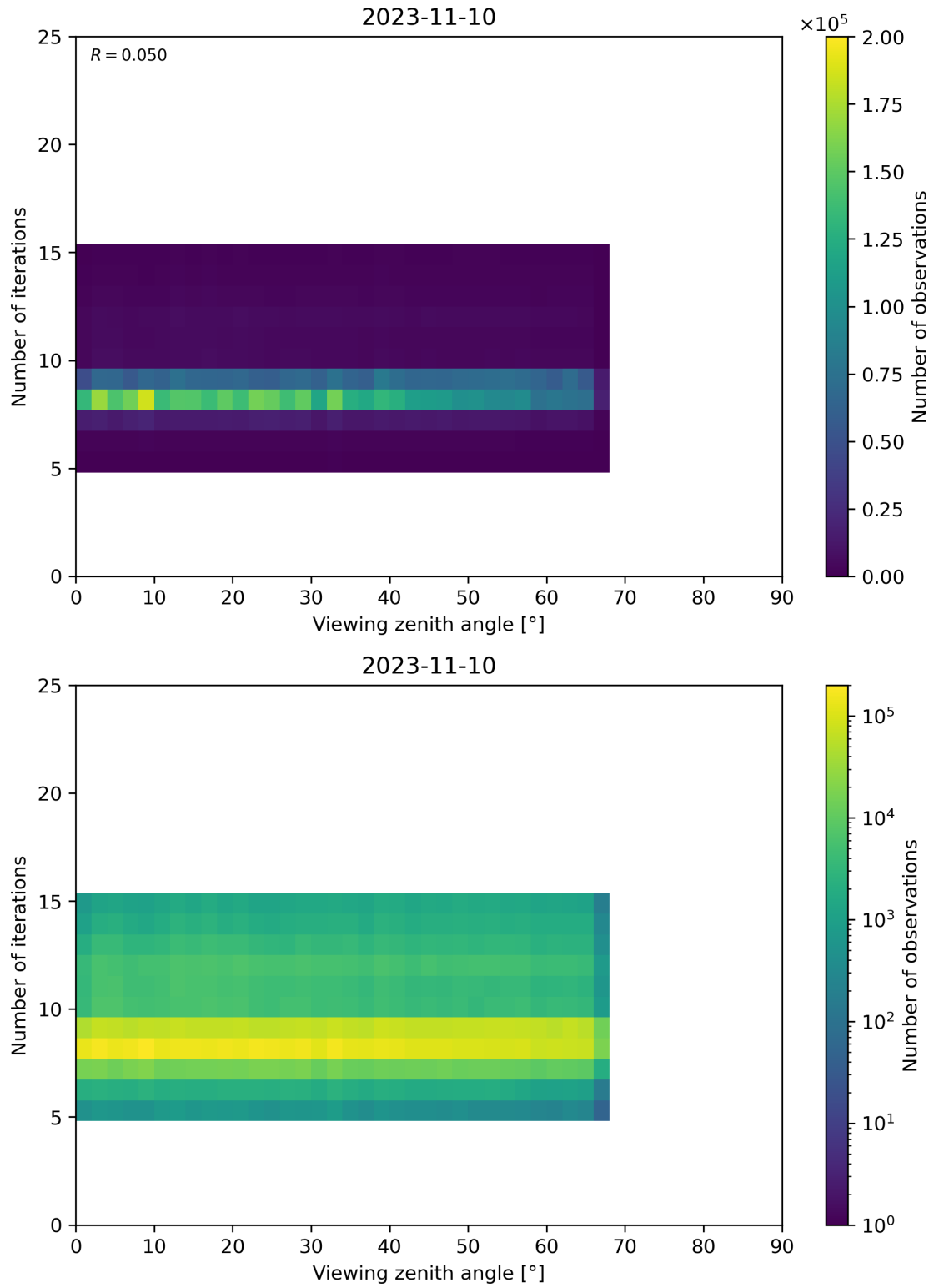
Figure 75: Scatter density plot of “Viewing zenith angle” against “Number of iterations” for 2023-11-09 to 2023-11-11.
