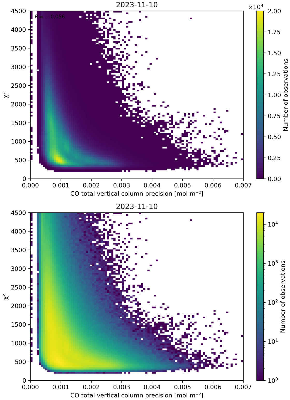
Figure 44: Scatter density plot of “CO total vertical column precision” against “ \chi^2 ” for 2023-11-09 to 2023-11-11.
