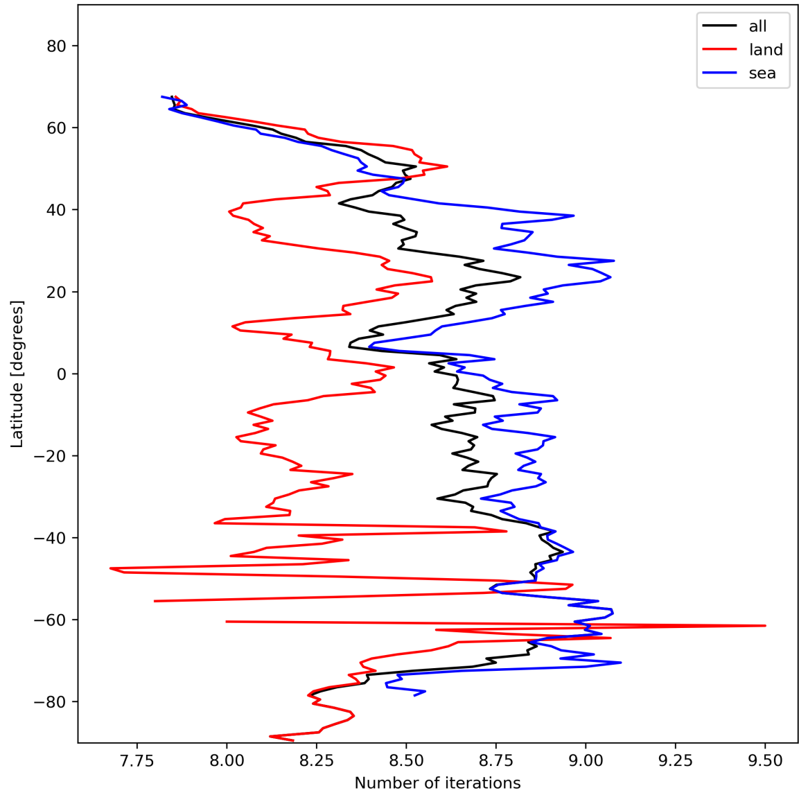
Figure 16: Zonal average of “Number of iterations” for 2023-11-09 to 2023-11-11.
