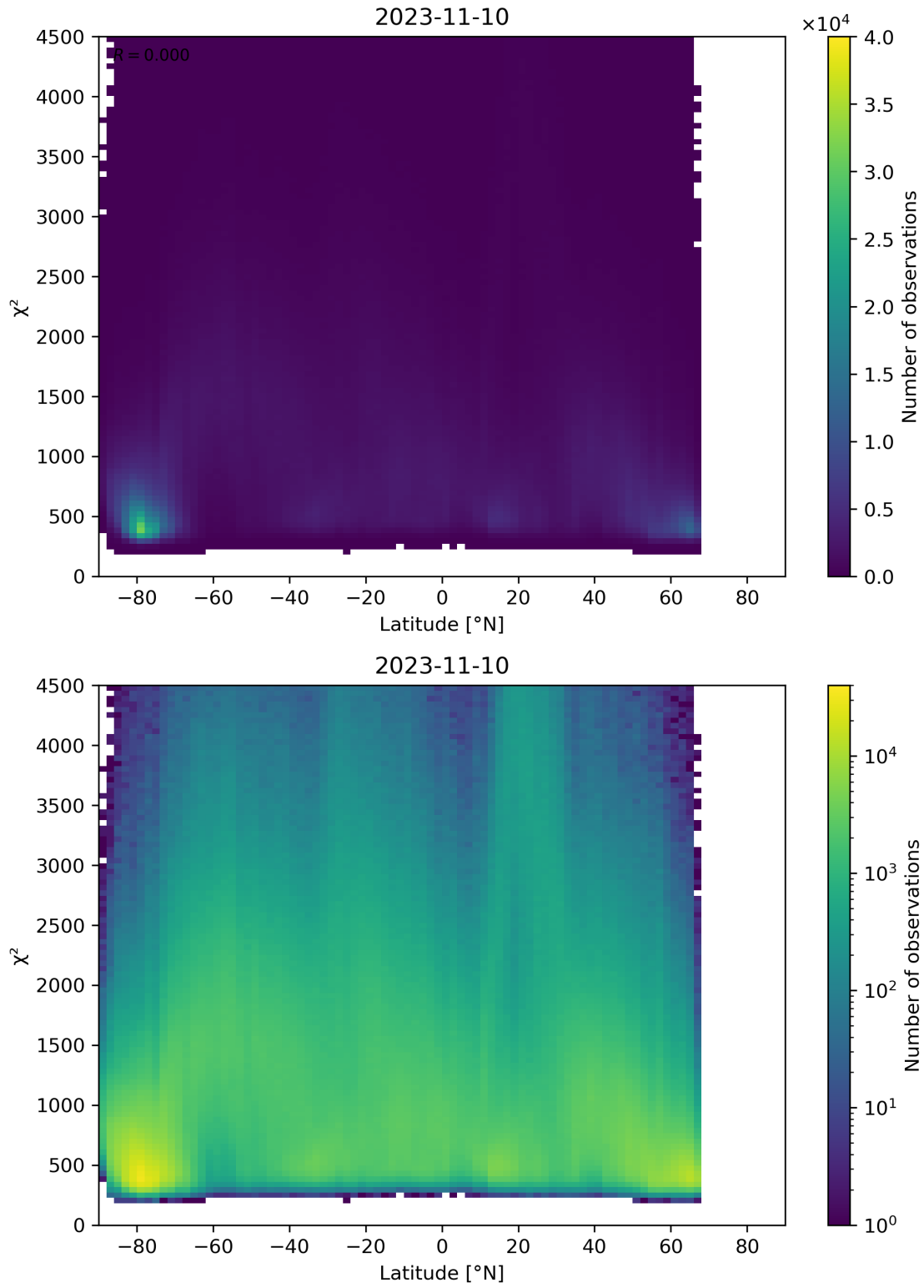
Figure 54: Scatter density plot of “Latitude” against “ \chi^2 ” for 2023-11-09 to 2023-11-11.
