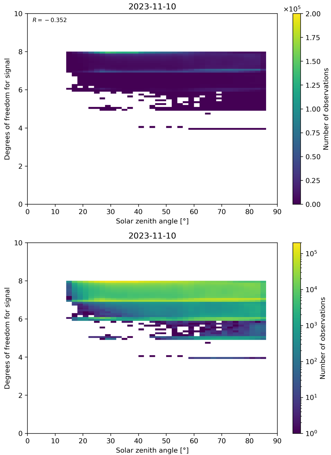
Figure 65: Scatter density plot of “Solar zenith angle” against “Degrees of freedom for signal” for 2023-11-09 to 2023-11-11.
