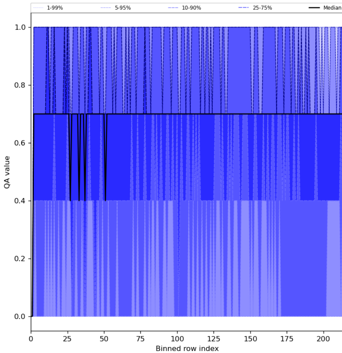
Figure 25: Along track statistics of “QA value” for 2023-11-09 to 2023-11-11
