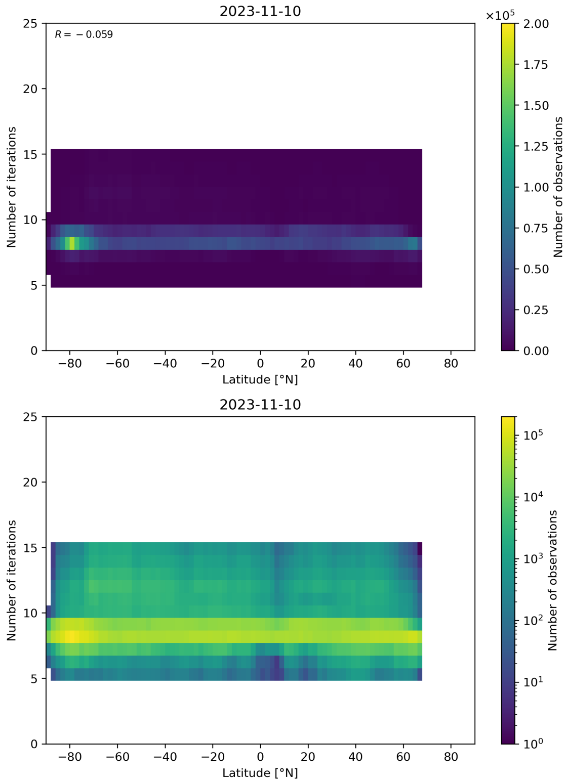
Figure 56: Scatter density plot of “Latitude” against “Number of iterations” for 2023-11-09 to 2023-11-11.
