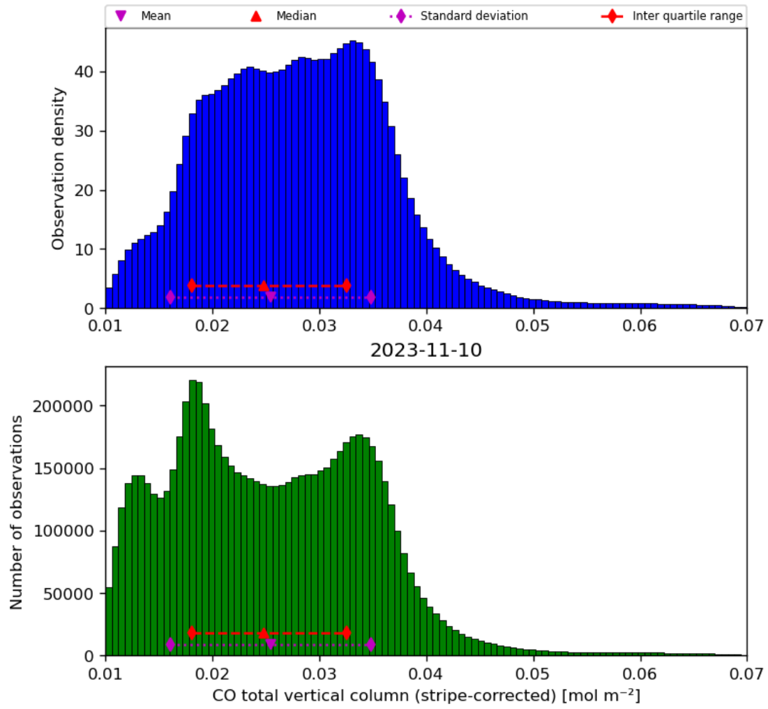
Figure 19: Histogram of “CO total vertical column (stripe-corrected)” for 2023-11-09 to 2023-11-11
