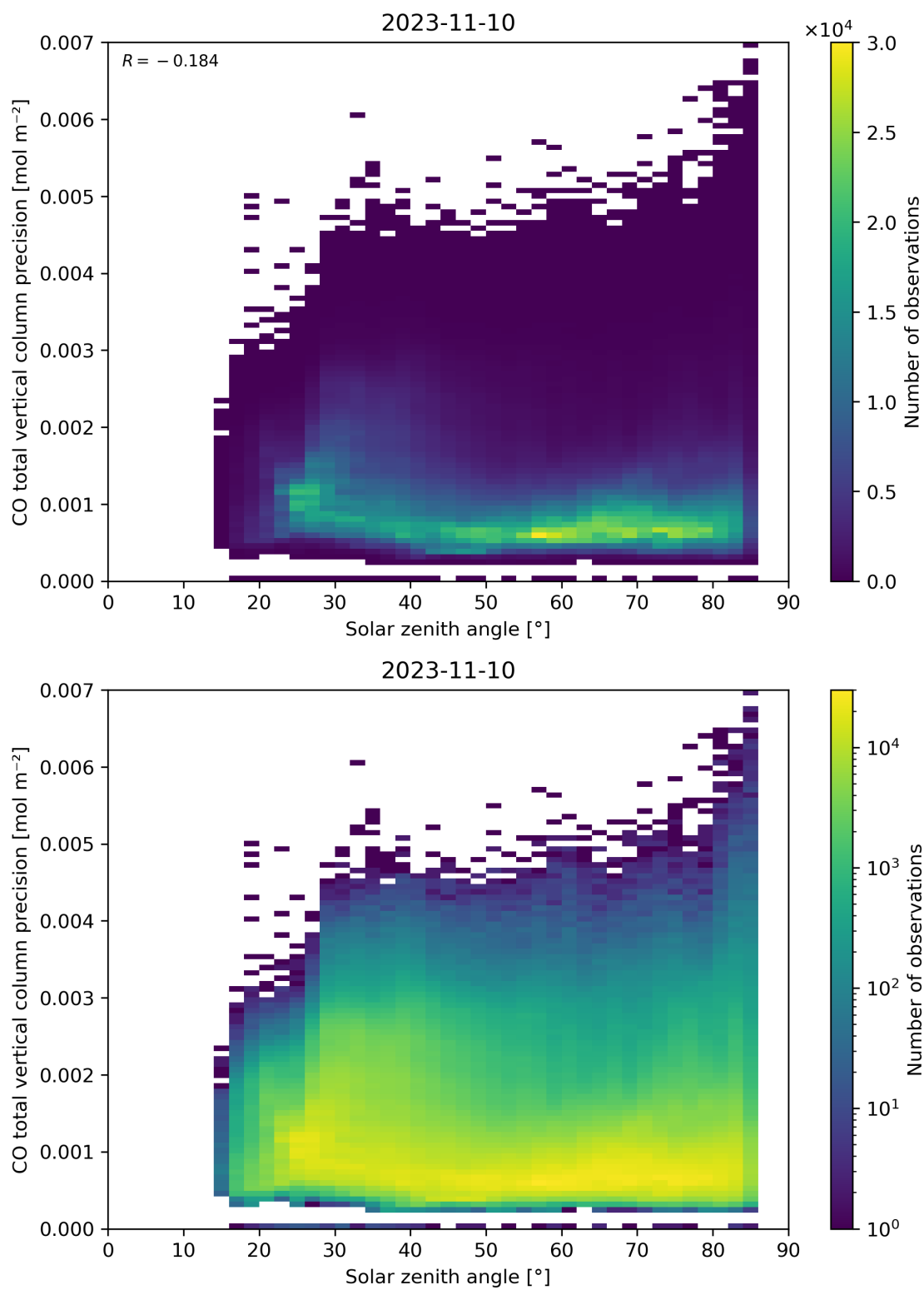
Figure 63: Scatter density plot of “Solar zenith angle” against “CO total vertical column precision” for 2023-11-09 to 2023-11-11.
