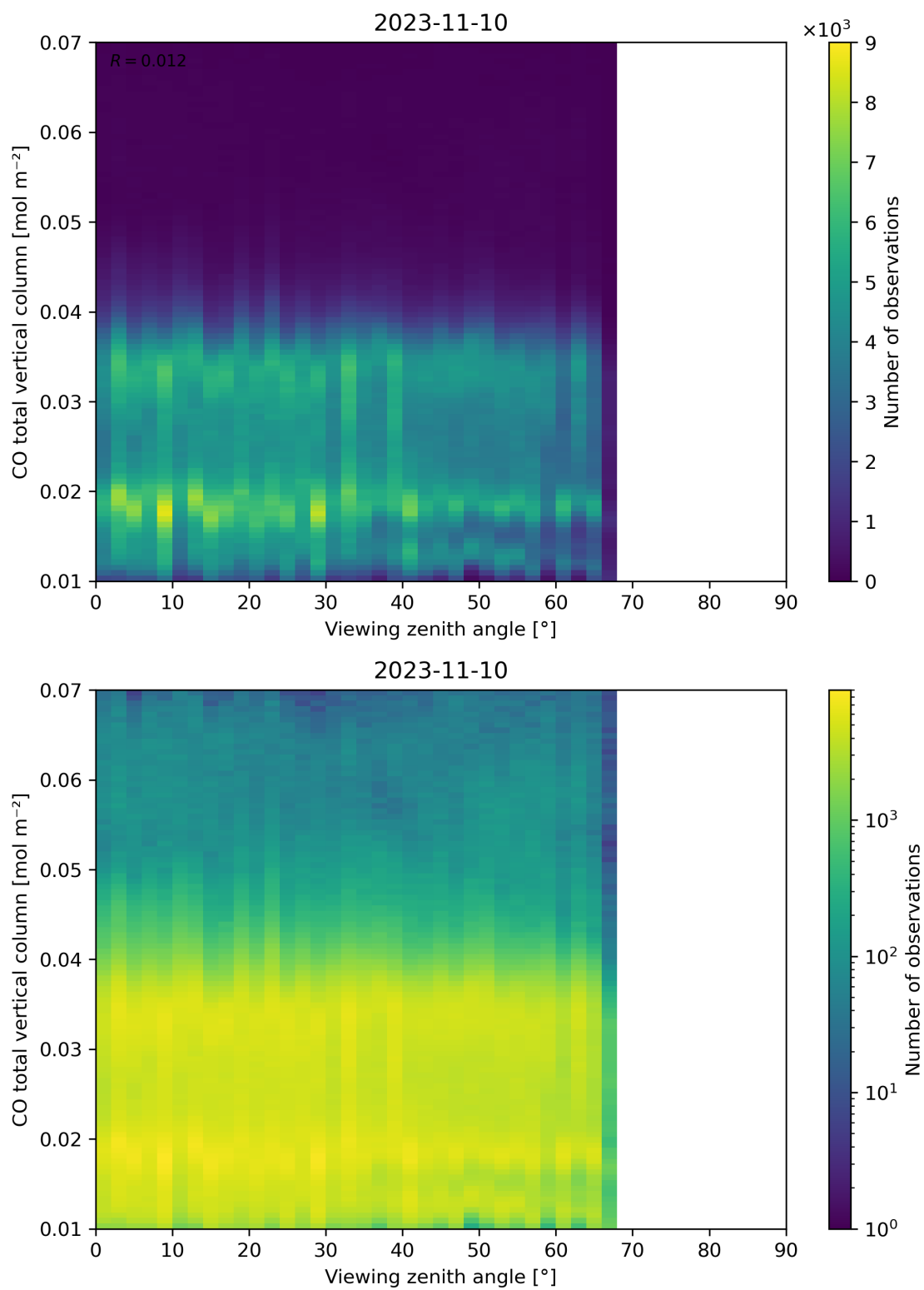
Figure 69: Scatter density plot of “Viewing zenith angle” against “CO total vertical column” for 2023-11-09 to 2023-11-11.
