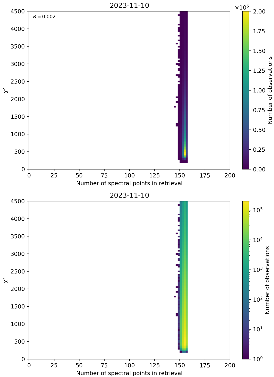
Figure 58: Scatter density plot of “Number of spectral points in retrieval” against “ \chi^2 ” for 2023-11-09 to 2023-11-11.
