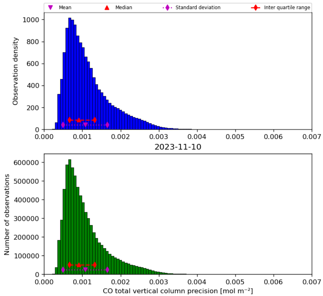
Figure 20: Histogram of “CO total vertical column precision” for 2023-11-09 to 2023-11-11
