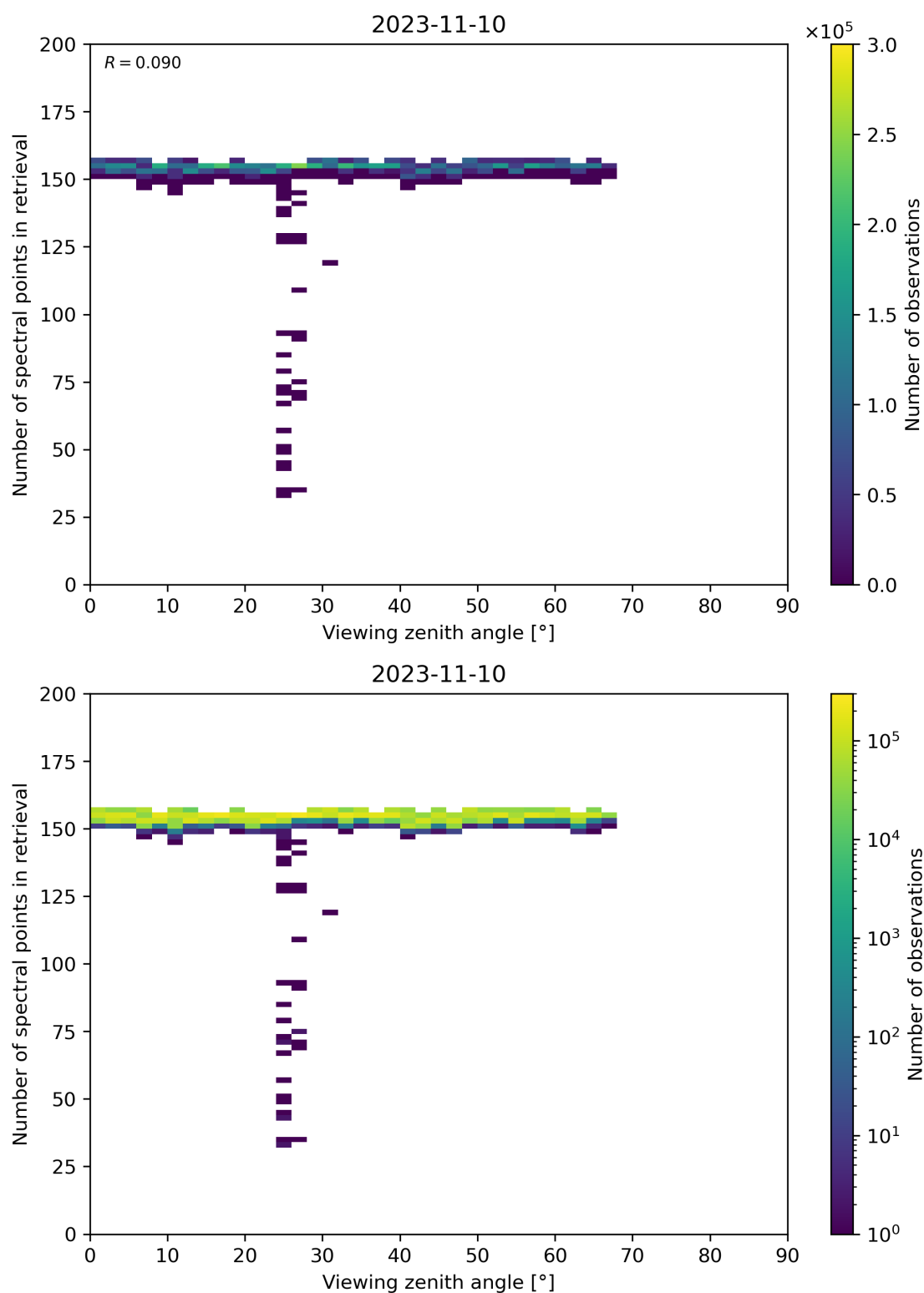
Figure 76: Scatter density plot of “Viewing zenith angle” against “Number of spectral points in retrieval” for 2023-11-09 to 2023-11-11.
