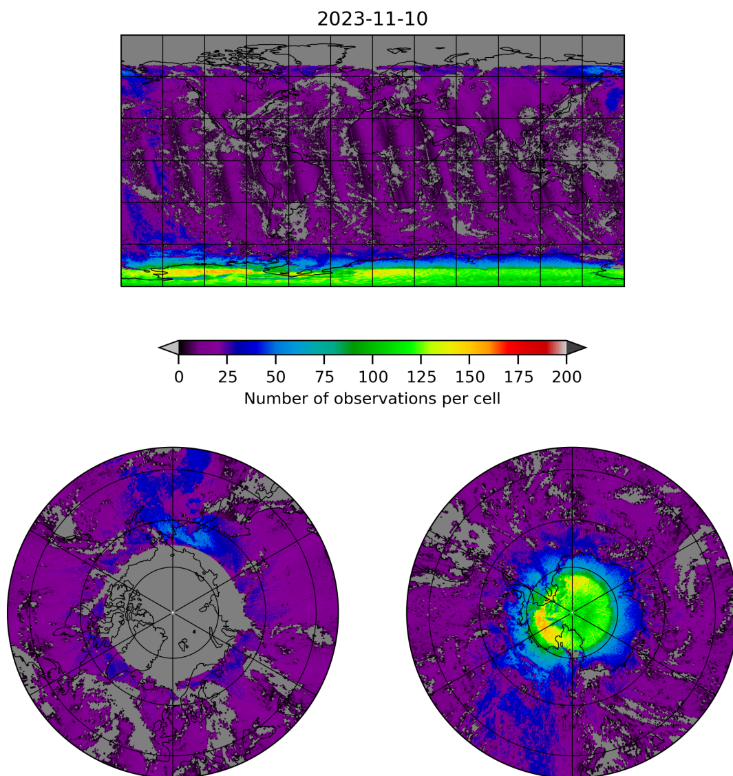
Figure 8: Map of the number of observations for 2023-11-09 to 2023-11-11
