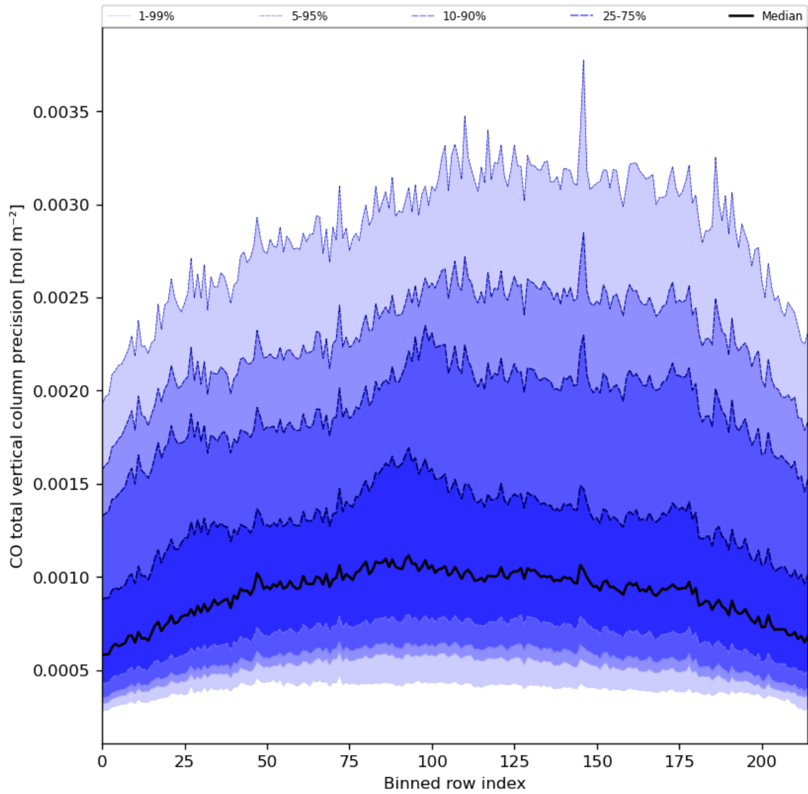
Figure 28: Along track statistics of “CO total vertical column precision” for 2023-11-09 to 2023-11-11
