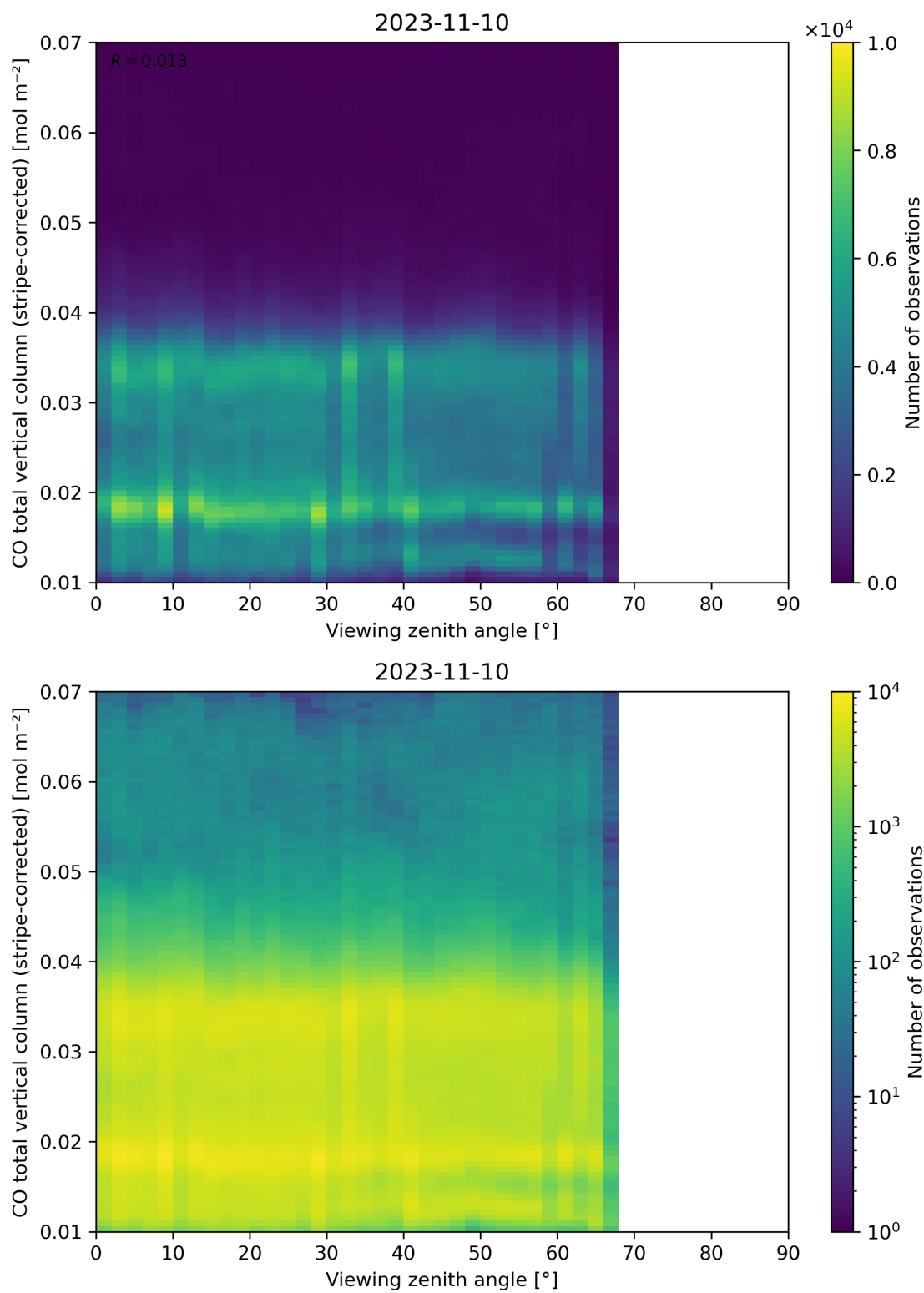
Figure 70: Scatter density plot of “Viewing zenith angle” against “CO total vertical column (stripe-corrected)” for 2023-11-09 to 2023-11-11.
