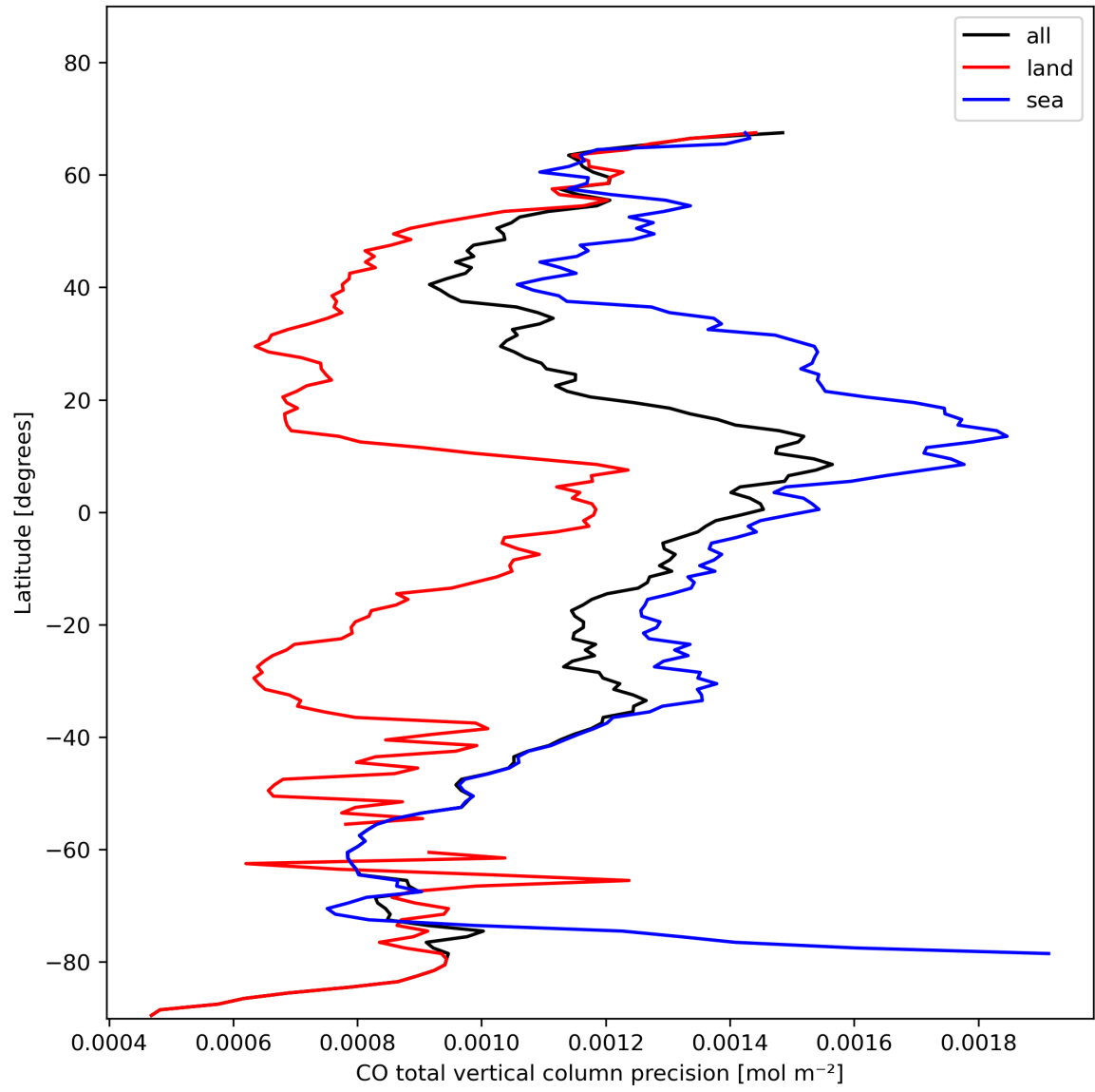
Figure 12: Zonal average of “CO total vertical column precision” for 2023-11-09 to 2023-11-11.
