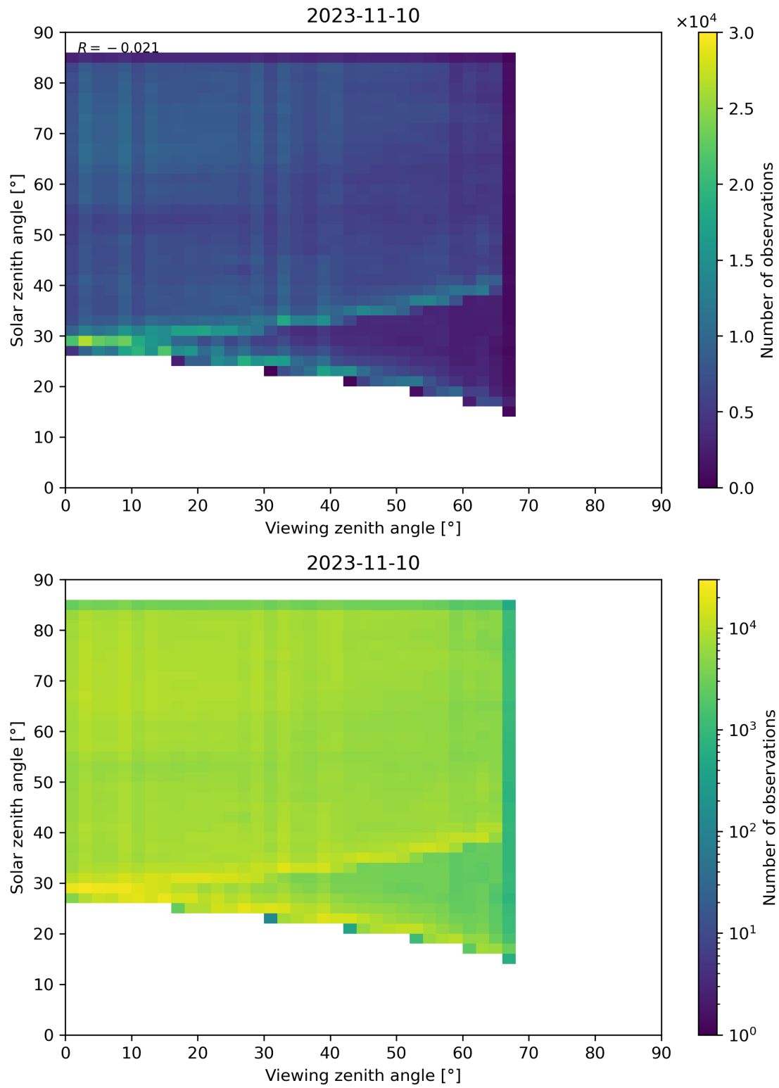
Figure 77: Scatter density plot of “Viewing zenith angle” against “Solar zenith angle” for 2023-11-09 to 2023-11-11.
