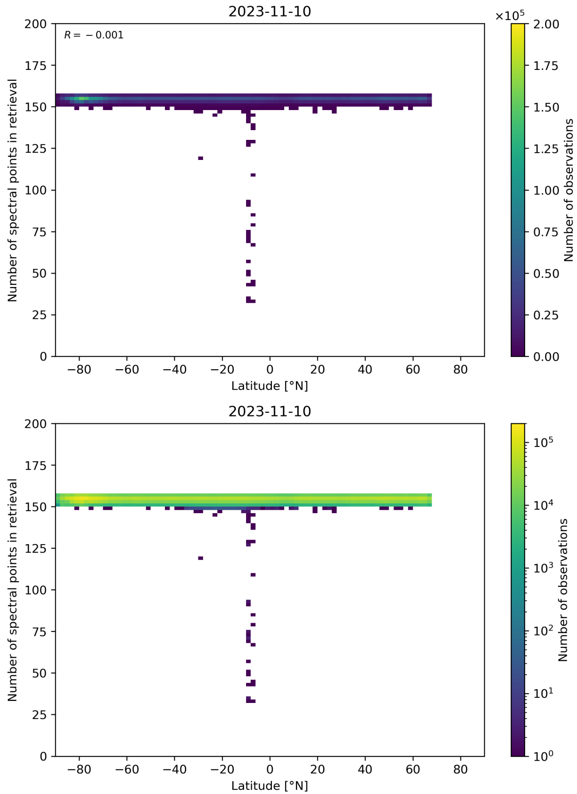
Figure 57: Scatter density plot of “Latitude” against “Number of spectral points in retrieval” for 2023-11-09 to 2023-11-11.
