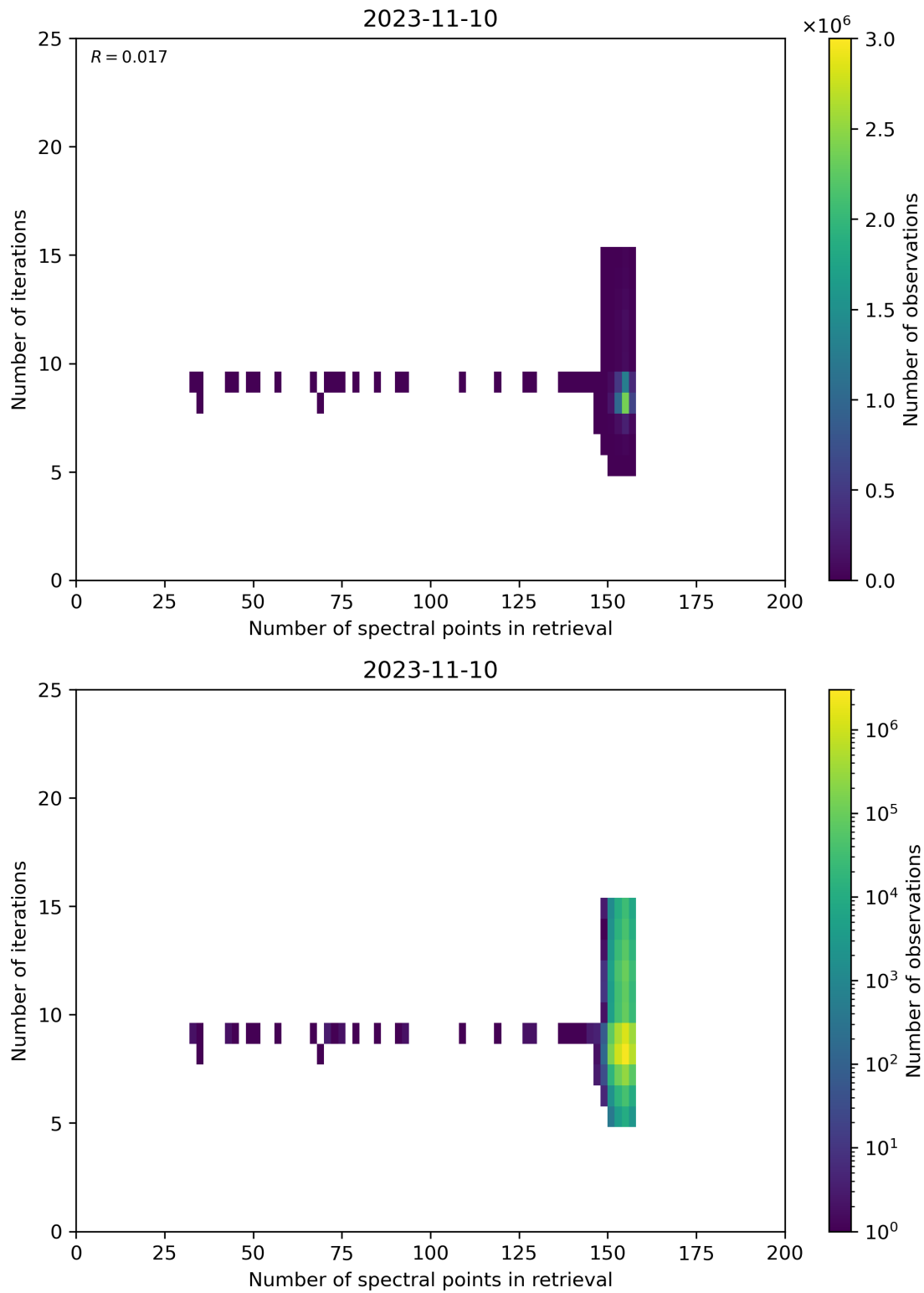
Figure 60: Scatter density plot of “Number of spectral points in retrieval” against “Number of iterations” for 2023-11-09 to 2023-11-11.
