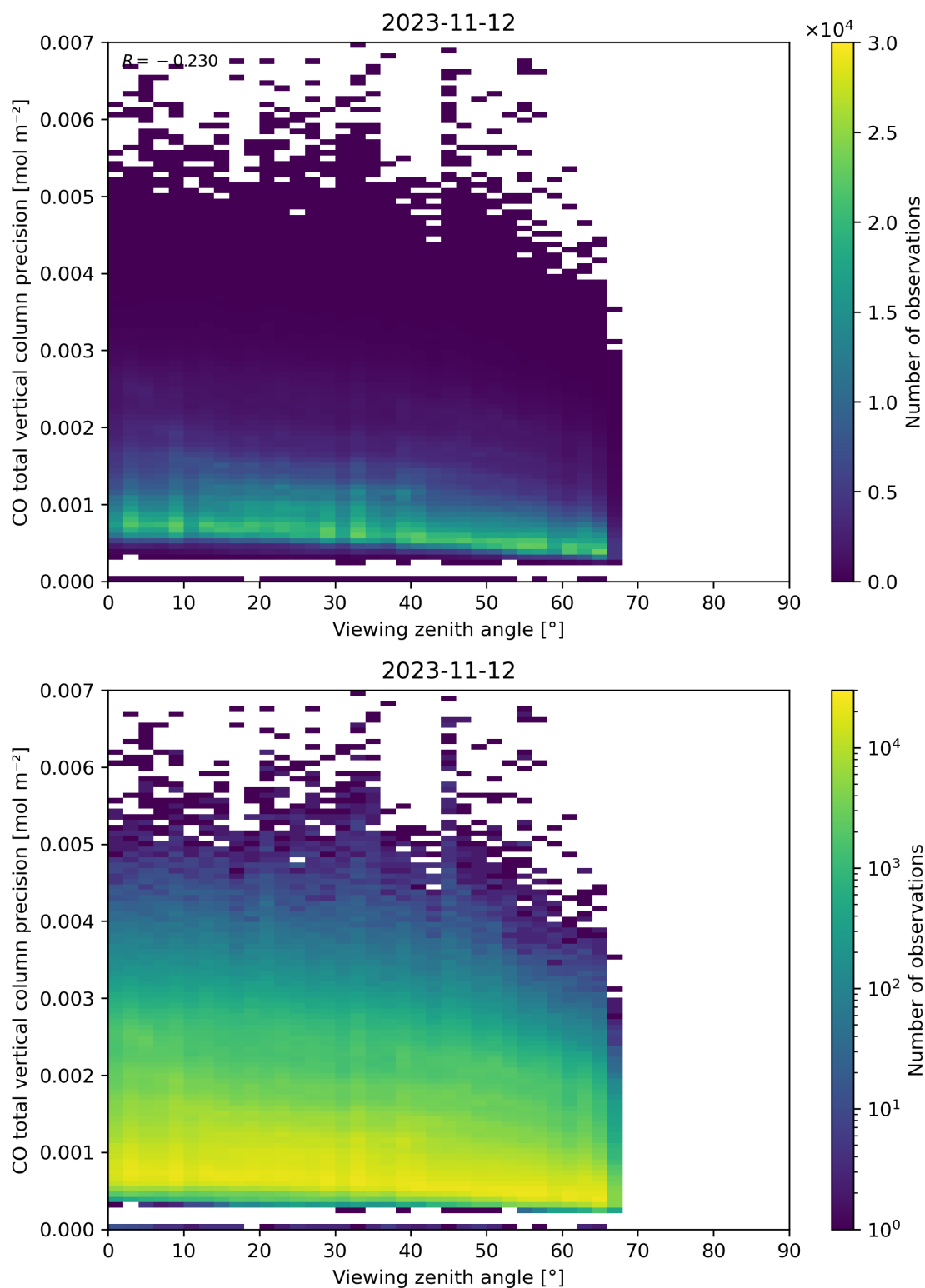
Figure 71: Scatter density plot of “Viewing zenith angle” against “CO total vertical column precision” for 2023-11-12 to 2023-11-13.
