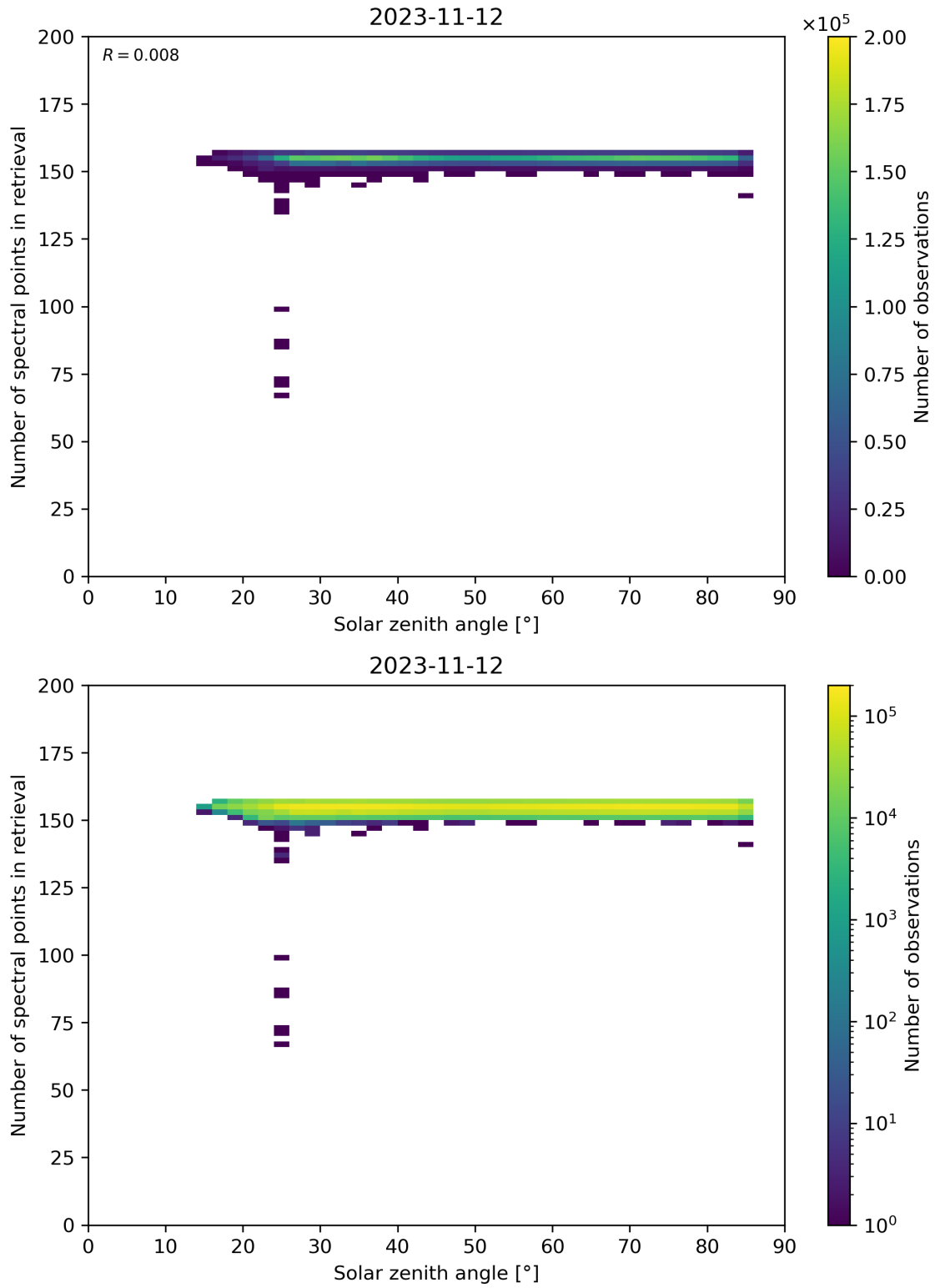
Figure 68: Scatter density plot of “Solar zenith angle” against “Number of spectral points in retrieval” for 2023-11-12 to 2023-11-13.
