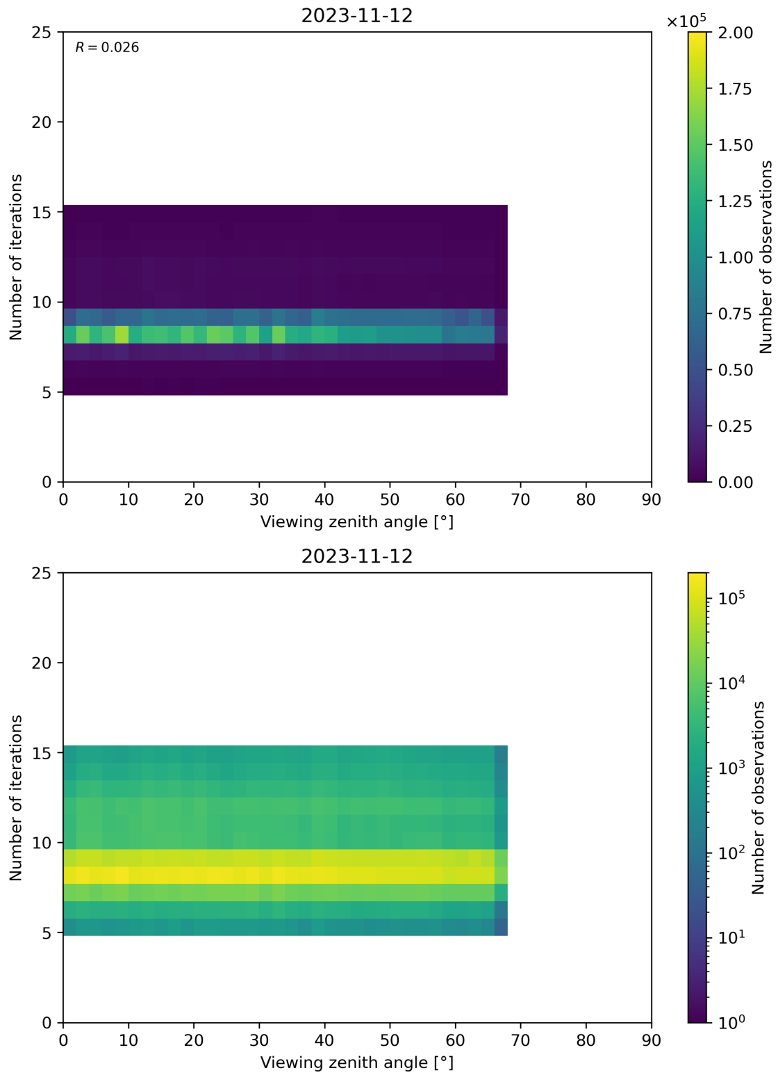
Figure 75: Scatter density plot of “Viewing zenith angle” against “Number of iterations” for 2023-11-12 to 2023-11-13.
