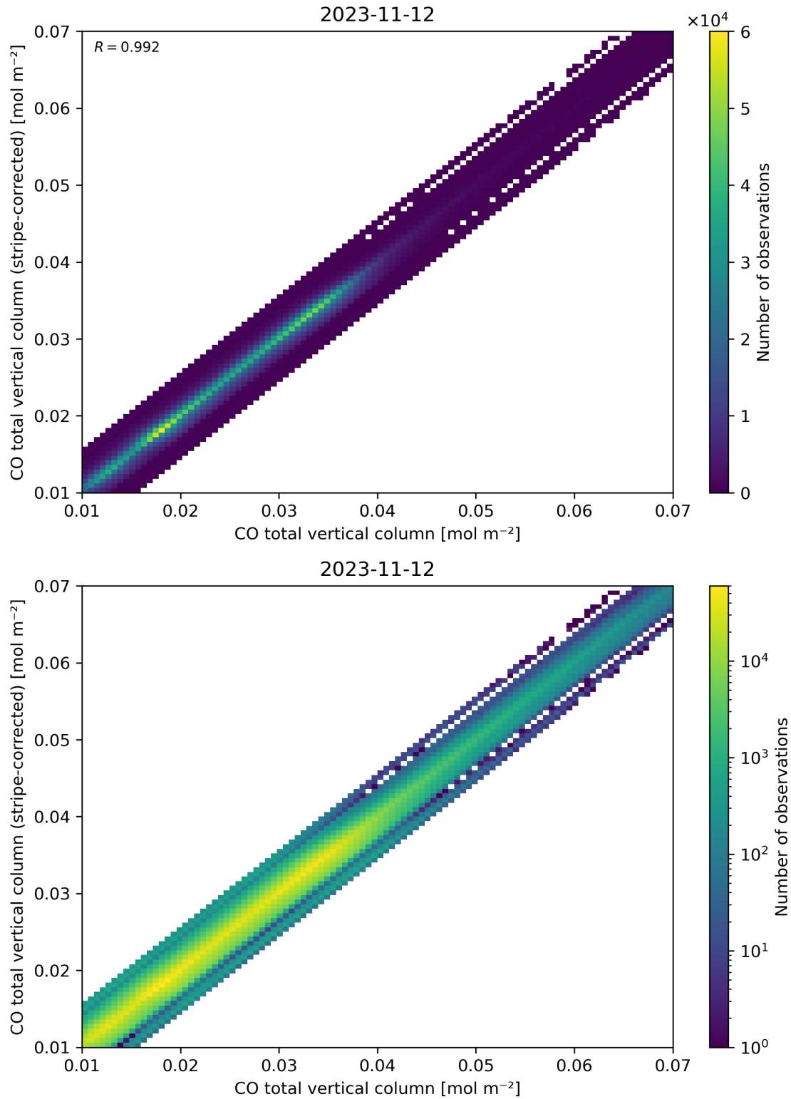
Figure 33: Scatter density plot of “CO total vertical column” against “CO total vertical column (stripe-corrected)” for 2023-11-12 to 2023-11-13.
