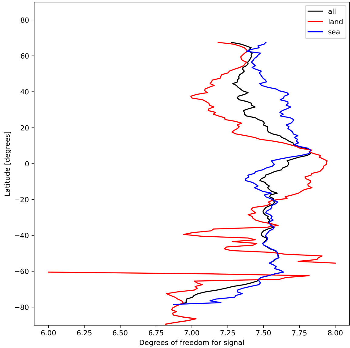
Figure 15: Zonal average of “Degrees of freedom for signal” for 2023-11-12 to 2023-11-13.
