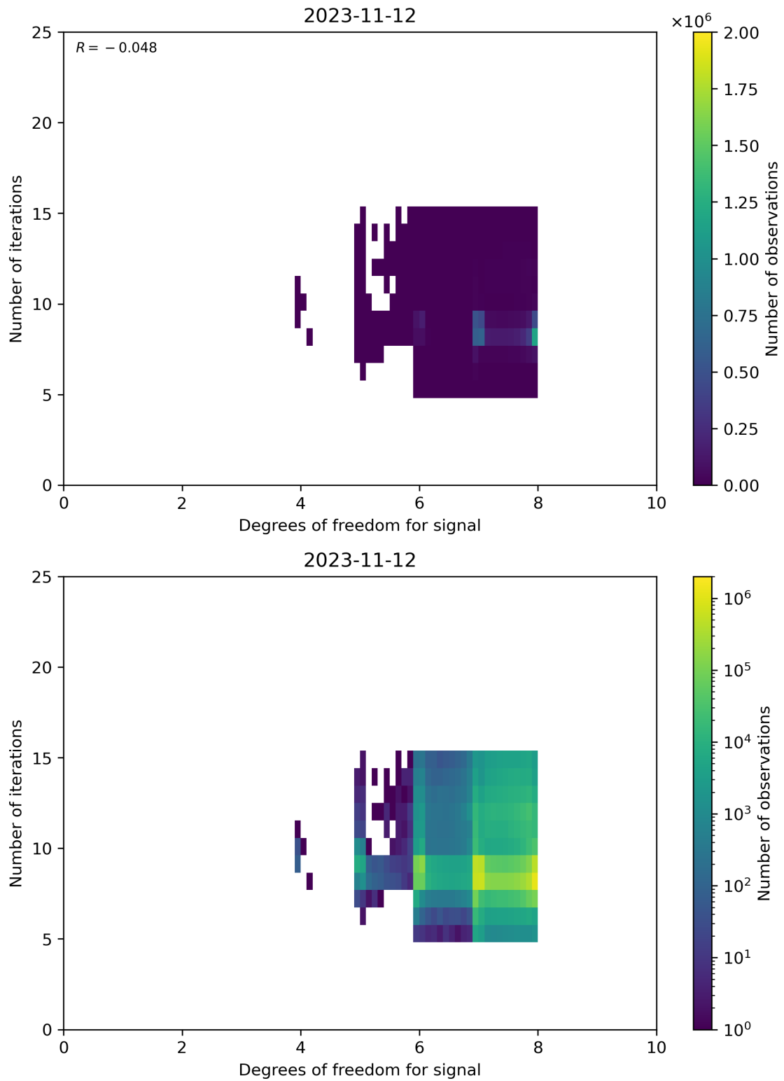
Figure 50: Scatter density plot of “Degrees of freedom for signal” against “Number of iterations” for 2023-11-12 to 2023-11-13.
