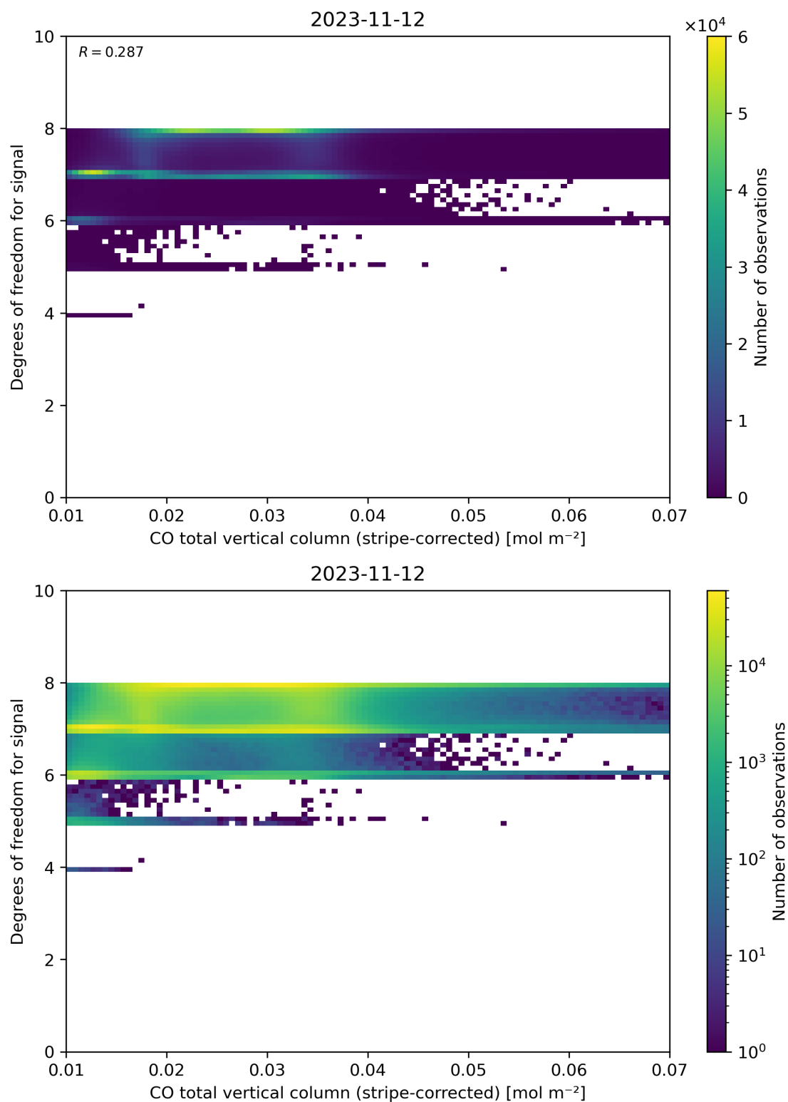
Figure 38: Scatter density plot of “CO total vertical column (stripe-corrected)” against “Degrees of freedom for signal” for 2023-11-12 to 2023-11-13.
