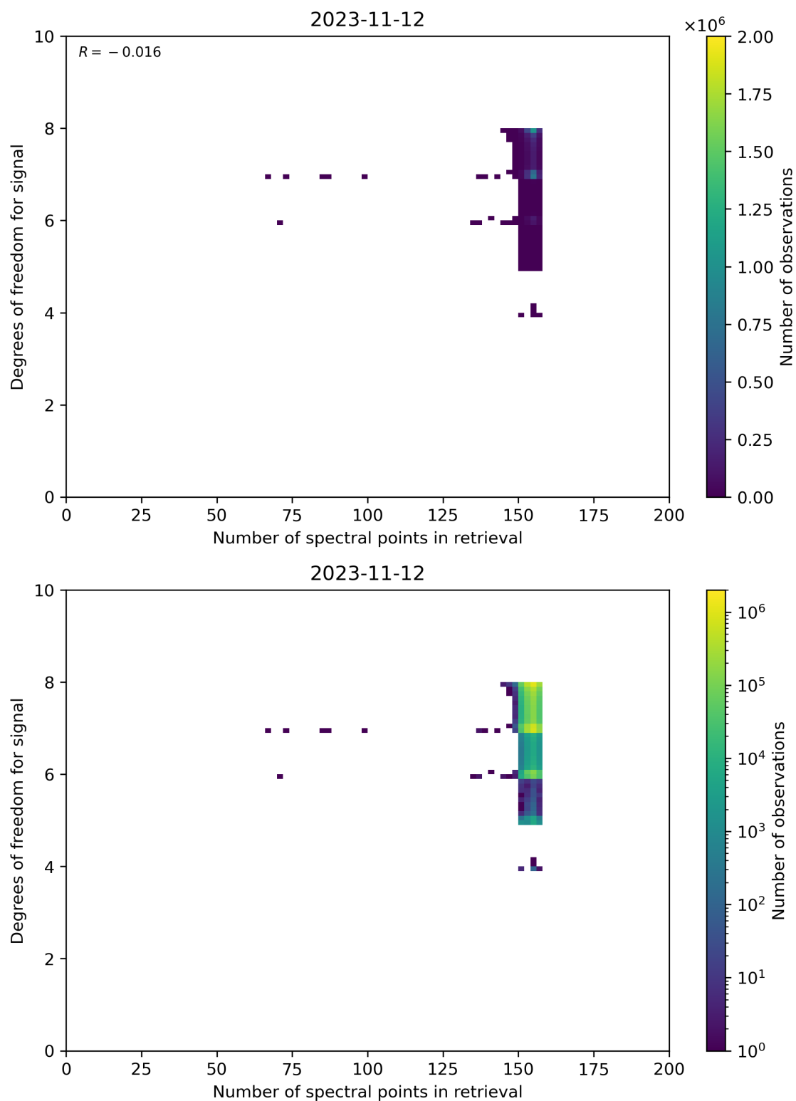
Figure 59: Scatter density plot of “Number of spectral points in retrieval” against “Degrees of freedom for signal” for 2023-11-12 to 2023-11-13.
