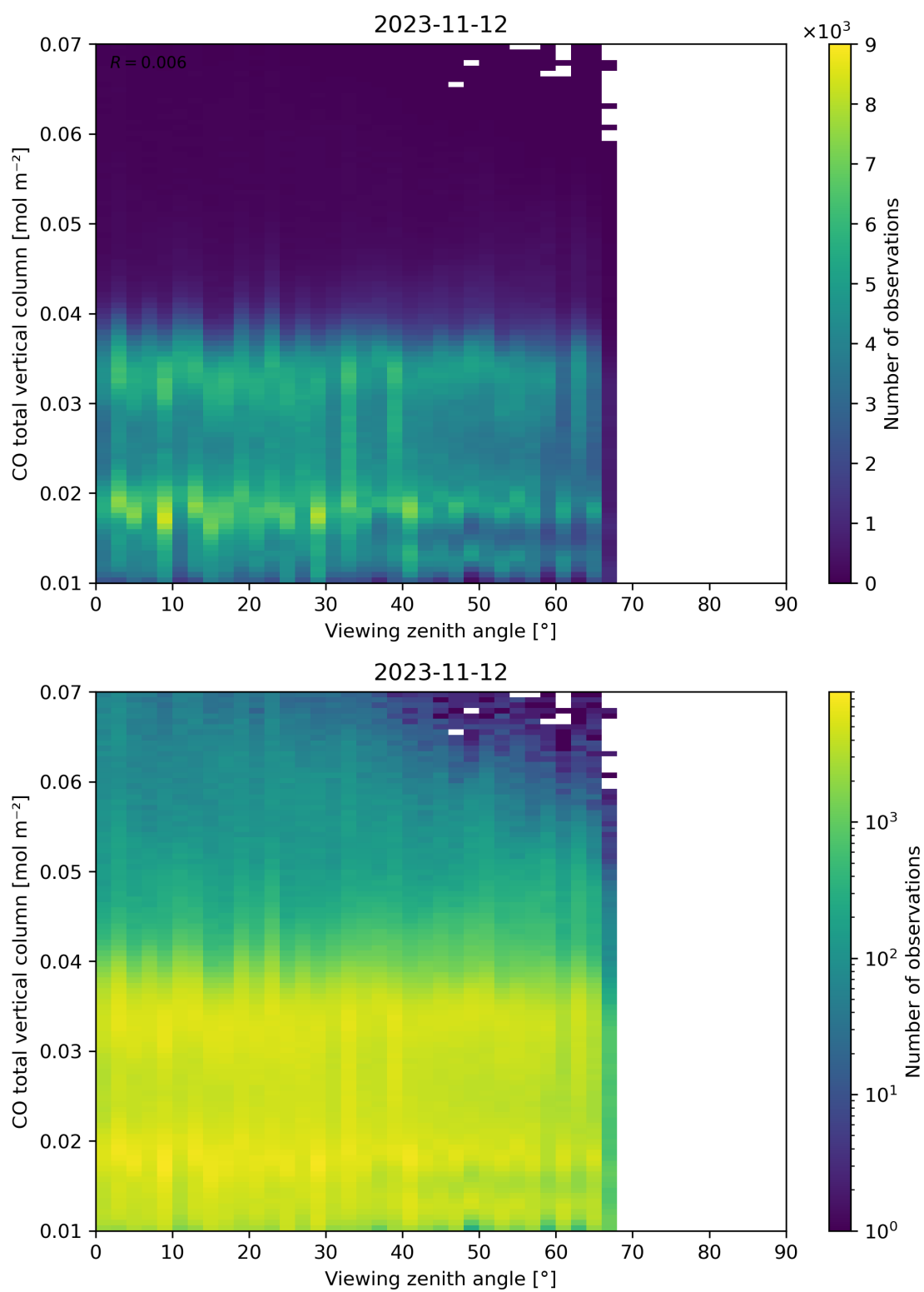
Figure 69: Scatter density plot of “Viewing zenith angle” against “CO total vertical column” for 2023-11-12 to 2023-11-13.
