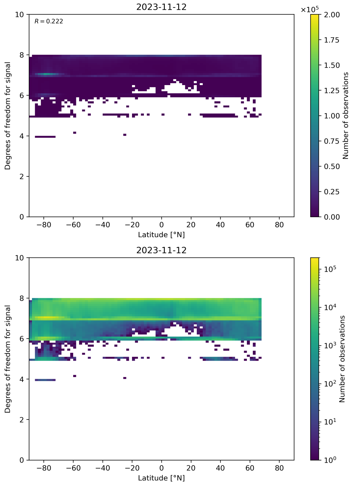
Figure 55: Scatter density plot of “Latitude” against “Degrees of freedom for signal” for 2023-11-12 to 2023-11-13.
