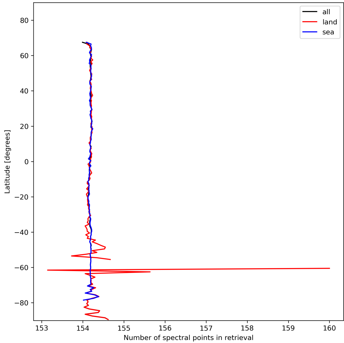
Figure 13: Zonal average of “Number of spectral points in retrieval” for 2023-11-12 to 2023-11-13.
