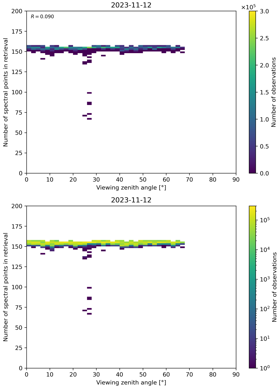
Figure 76: Scatter density plot of “Viewing zenith angle” against “Number of spectral points in retrieval” for 2023-11-12 to 2023-11-13.
