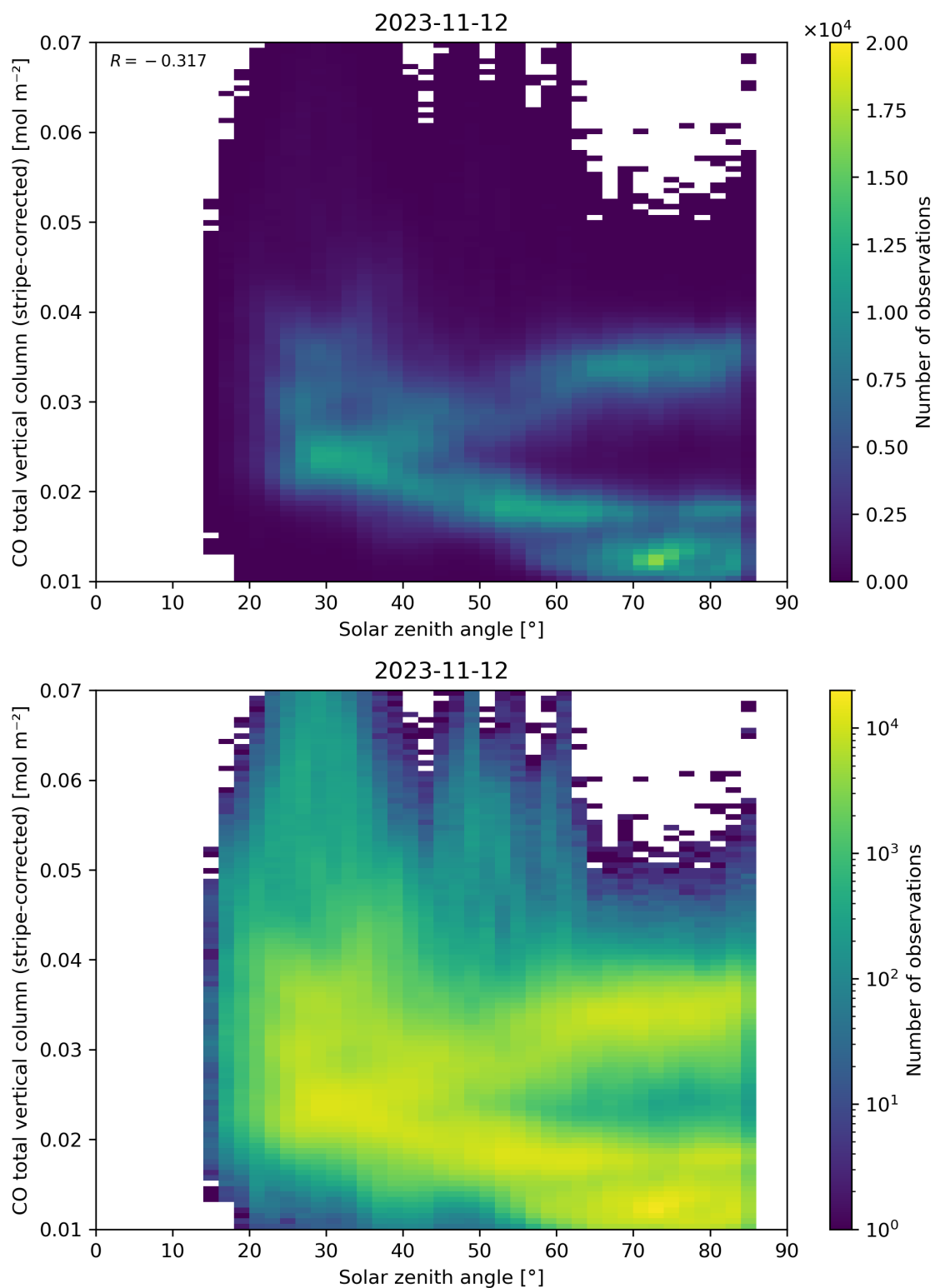
Figure 62: Scatter density plot of “Solar zenith angle” against “CO total vertical column (stripe-corrected)” for 2023-11-12 to 2023-11-13.
