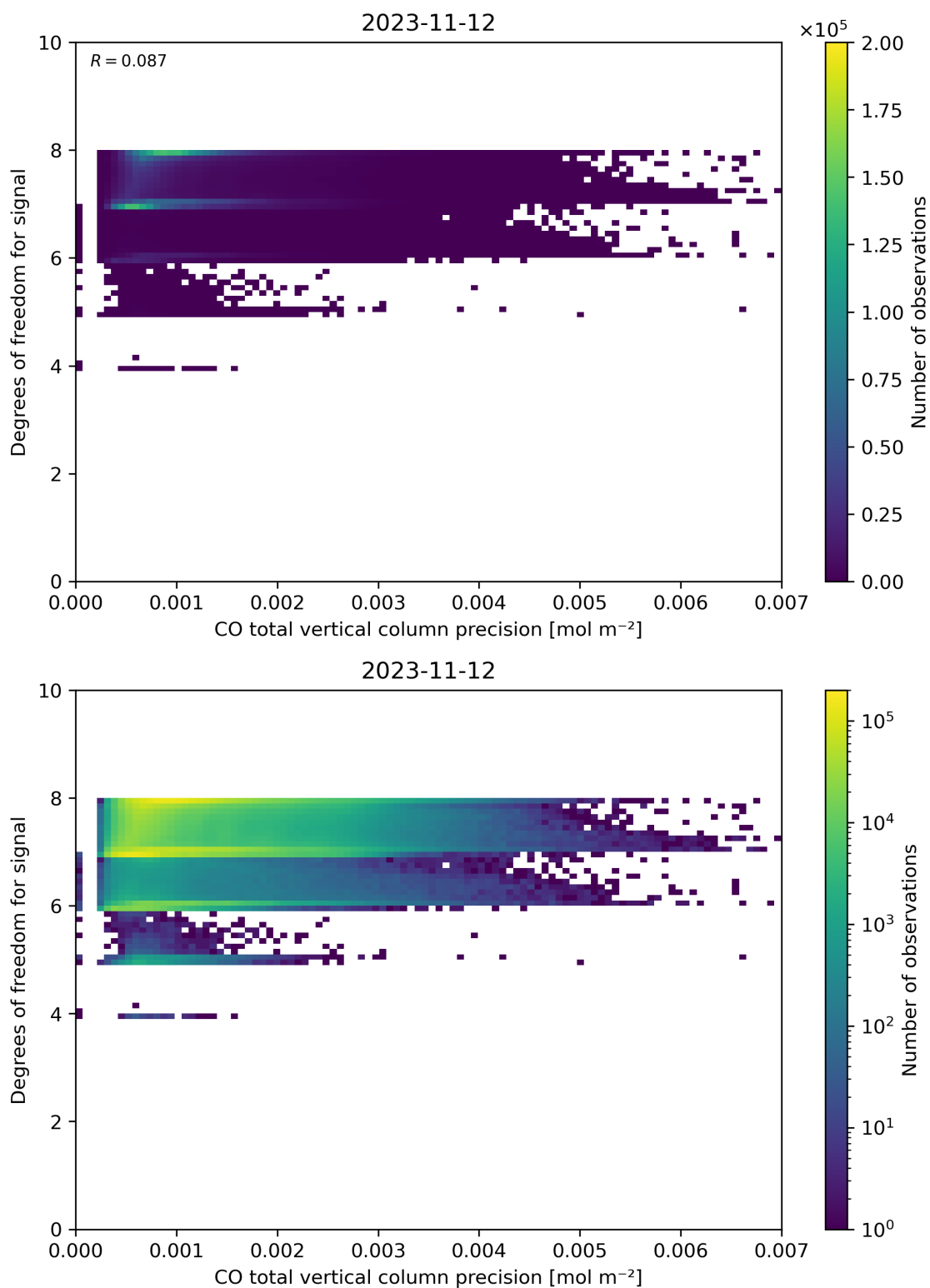
Figure 45: Scatter density plot of “CO total vertical column precision” against “Degrees of freedom for signal” for 2023-11-12 to 2023-11-13.
