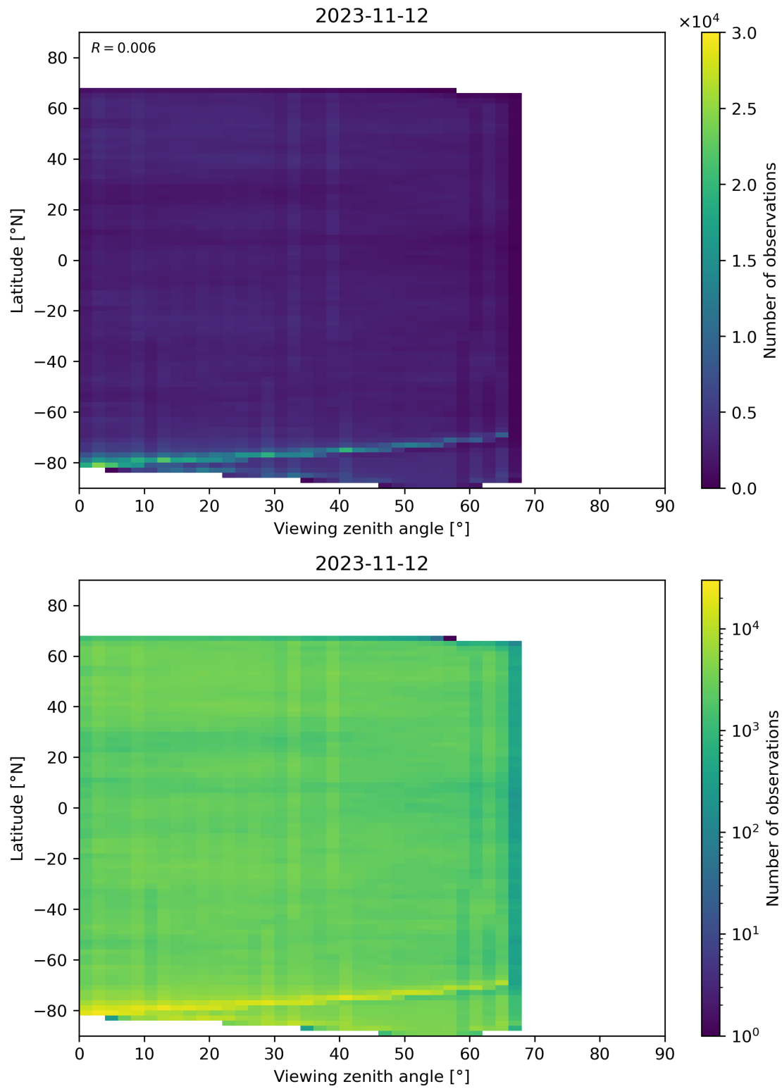
Figure 74: Scatter density plot of “Viewing zenith angle” against “Latitude” for 2023-11-12 to 2023-11-13.
