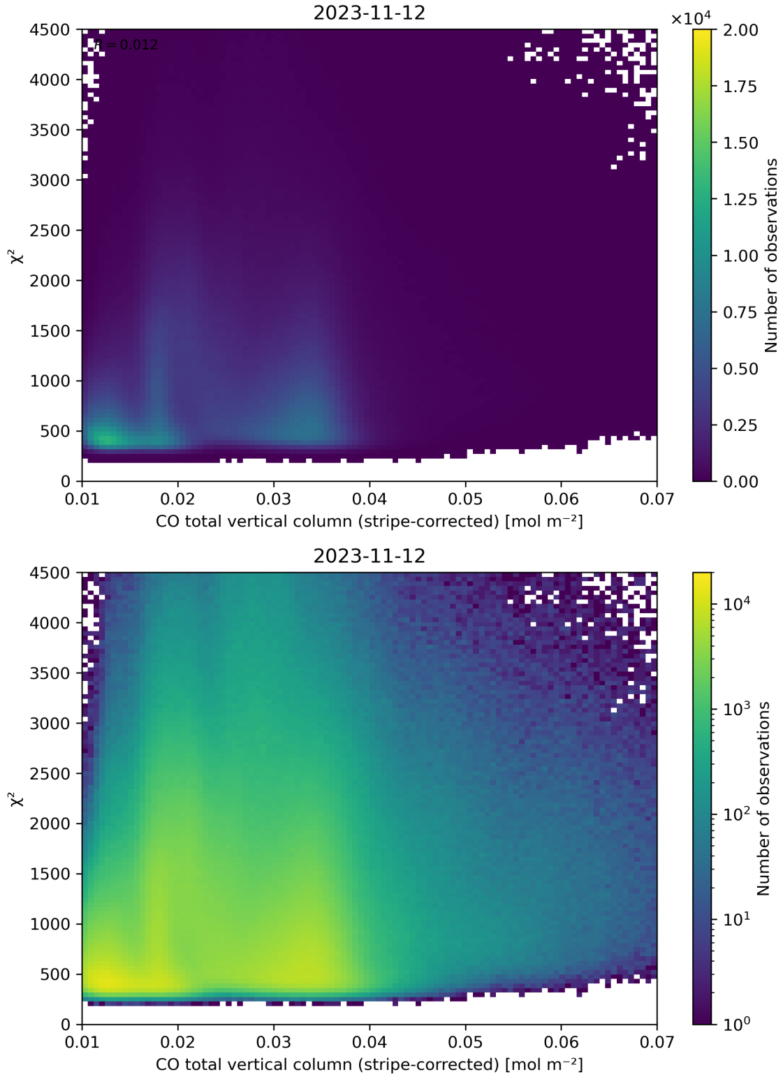
Figure 37: Scatter density plot of “CO total vertical column (stripe-corrected)” against “ \chi^2 ” for 2023-11-12 to 2023-11-13.
