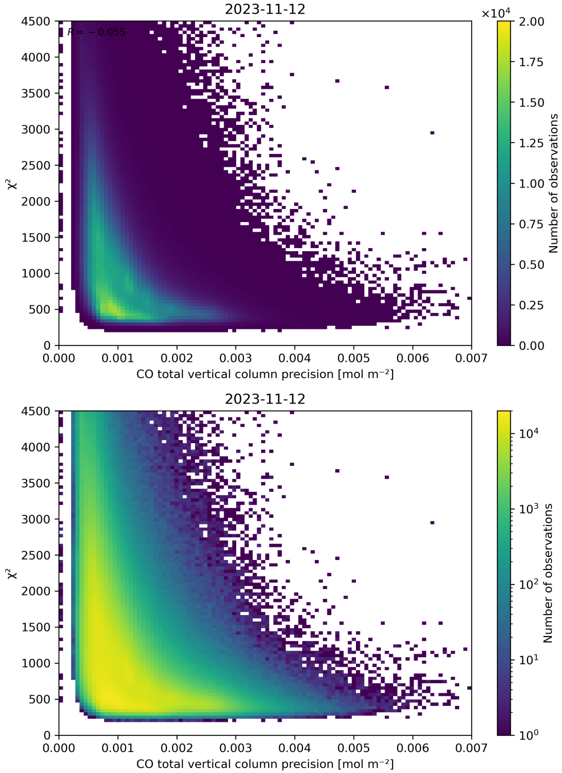
Figure 44: Scatter density plot of “CO total vertical column precision” against “ \chi^2 ” for 2023-11-12 to 2023-11-13.
