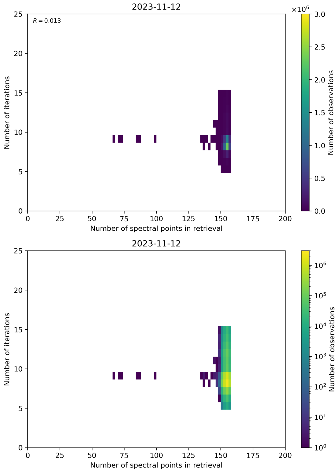
Figure 60: Scatter density plot of “Number of spectral points in retrieval” against “Number of iterations” for 2023-11-12 to 2023-11-13.
