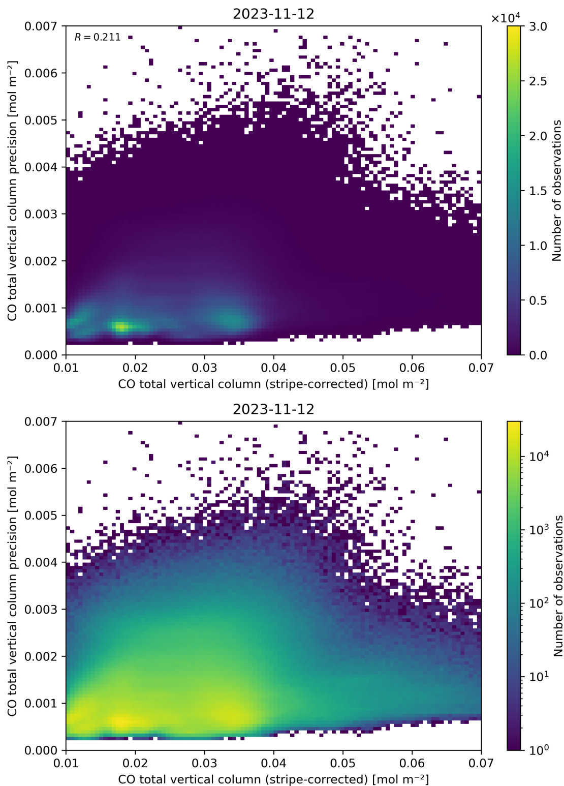
Figure 36: Scatter density plot of “CO total vertical column (stripe-corrected)” against “CO total vertical column precision” for 2023-11-12 to 2023-11-13.
