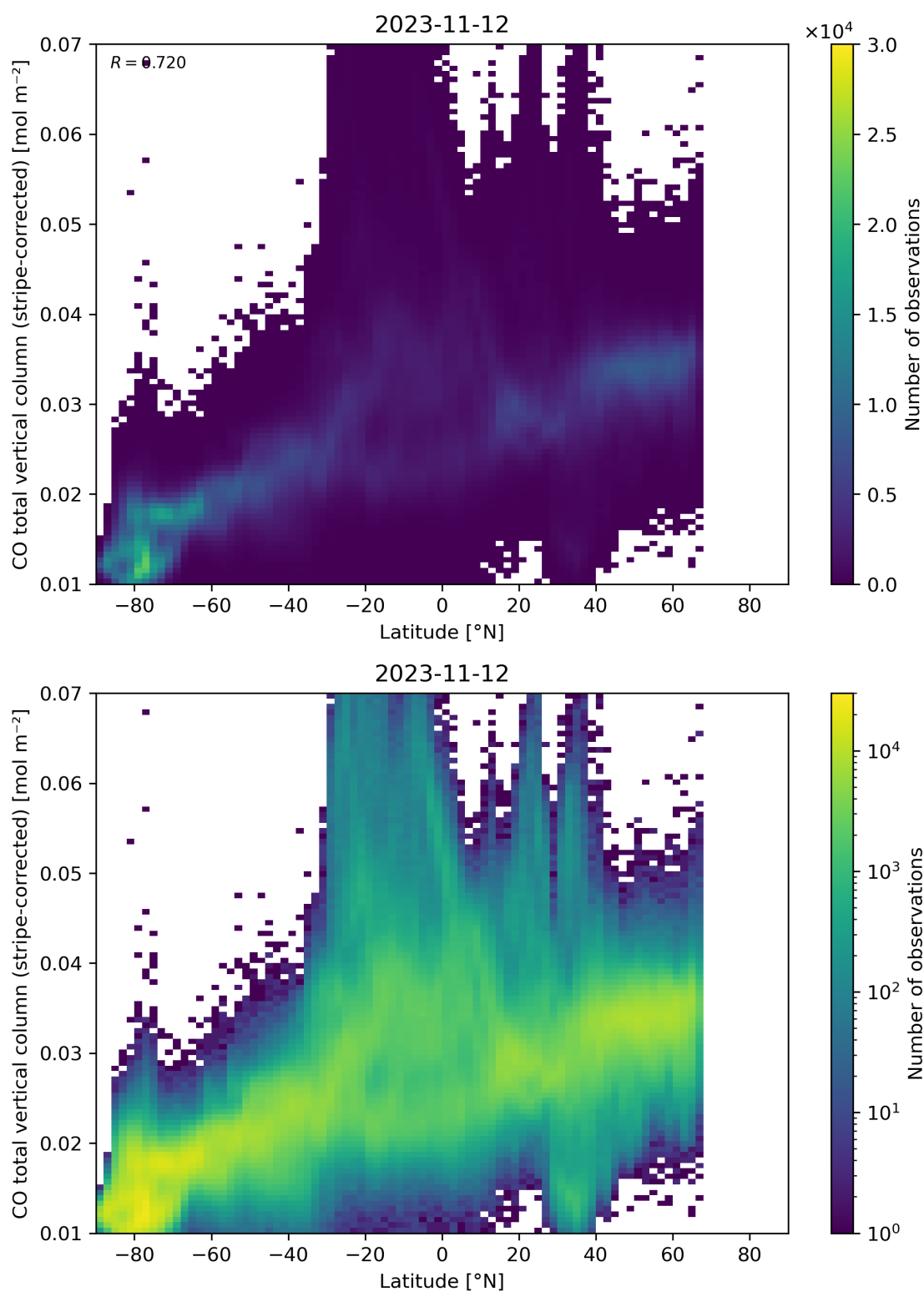
Figure 52: Scatter density plot of “Latitude” against “CO total vertical column (stripe-corrected)” for 2023-11-12 to 2023-11-13.
