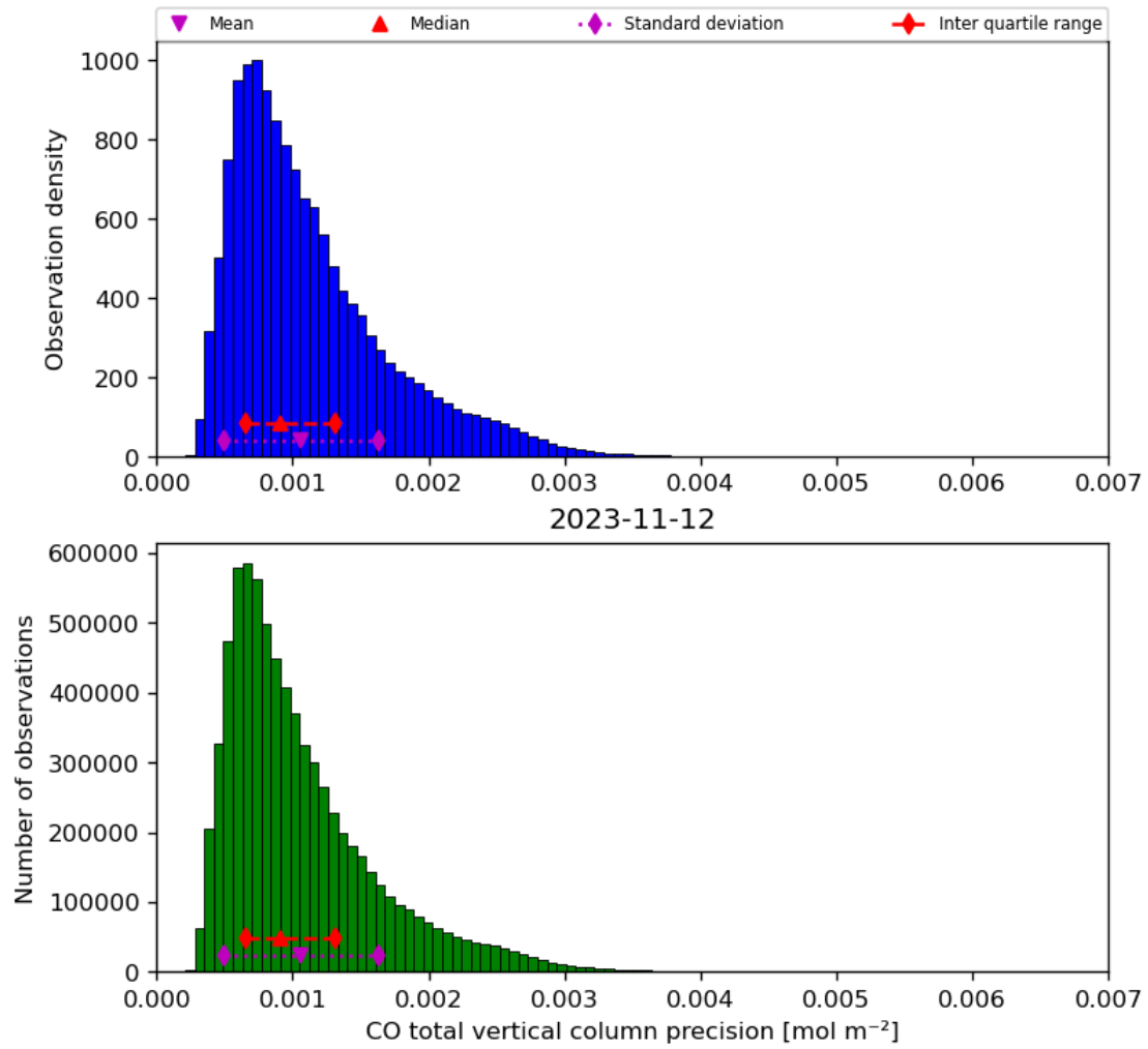
Figure 20: Histogram of “CO total vertical column precision” for 2023-11-12 to 2023-11-13
