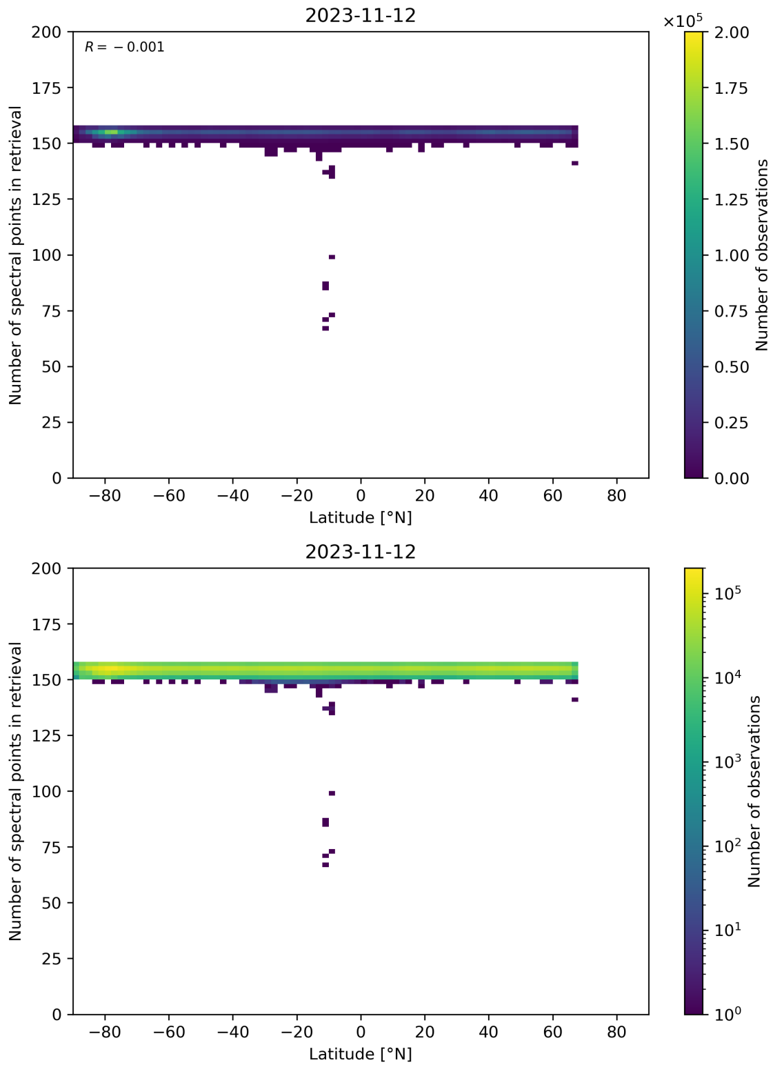
Figure 57: Scatter density plot of “Latitude” against “Number of spectral points in retrieval” for 2023-11-12 to 2023-11-13.
