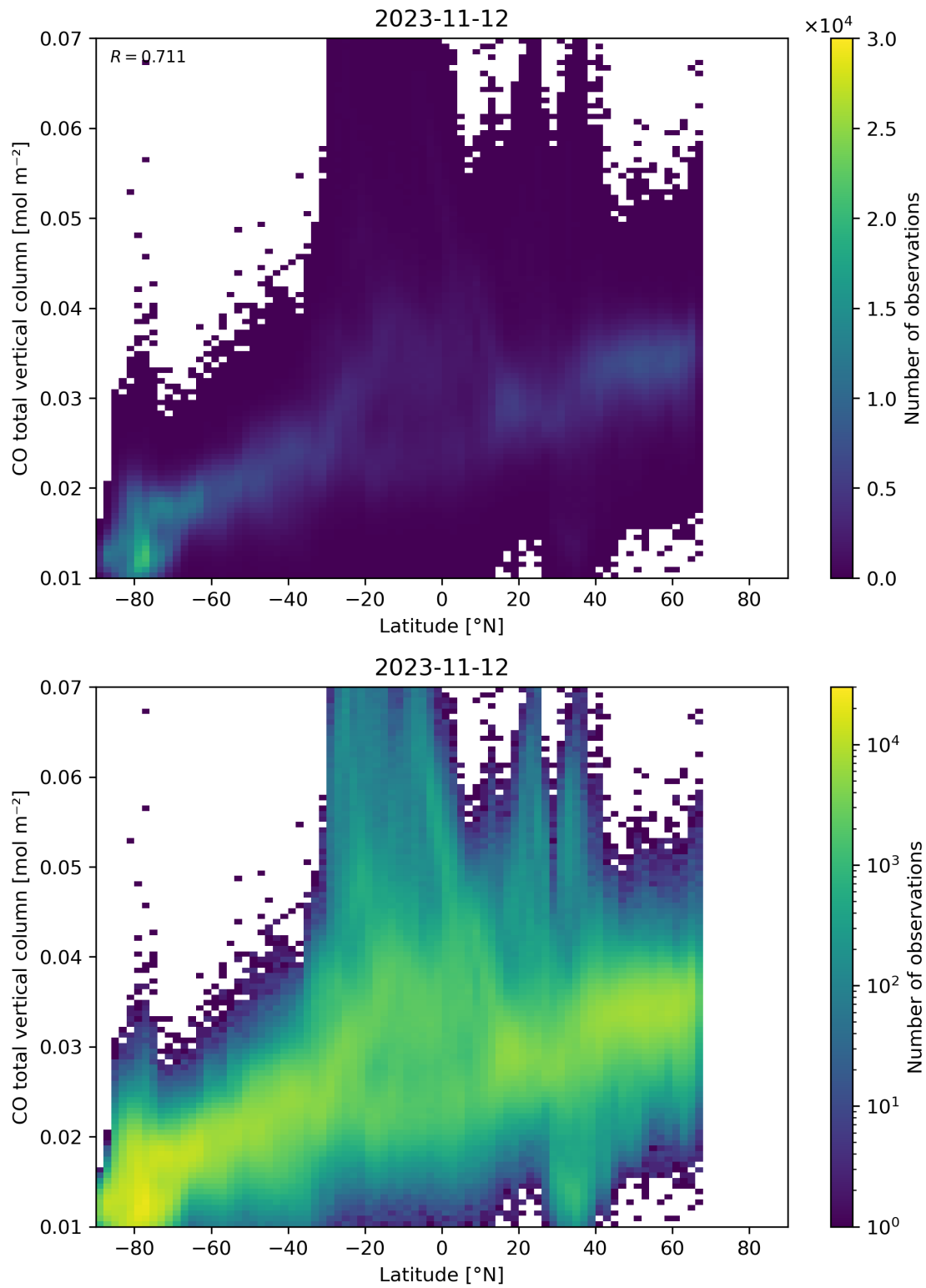
Figure 51: Scatter density plot of “Latitude” against “CO total vertical column” for 2023-11-12 to 2023-11-13.
