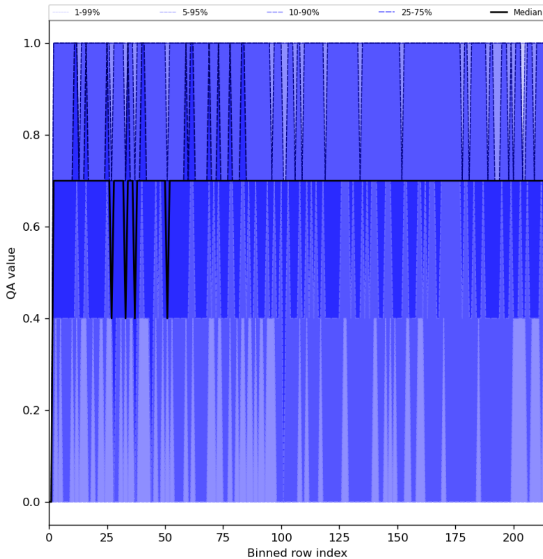
Figure 25: Along track statistics of “QA value” for 2023-11-12 to 2023-11-13
