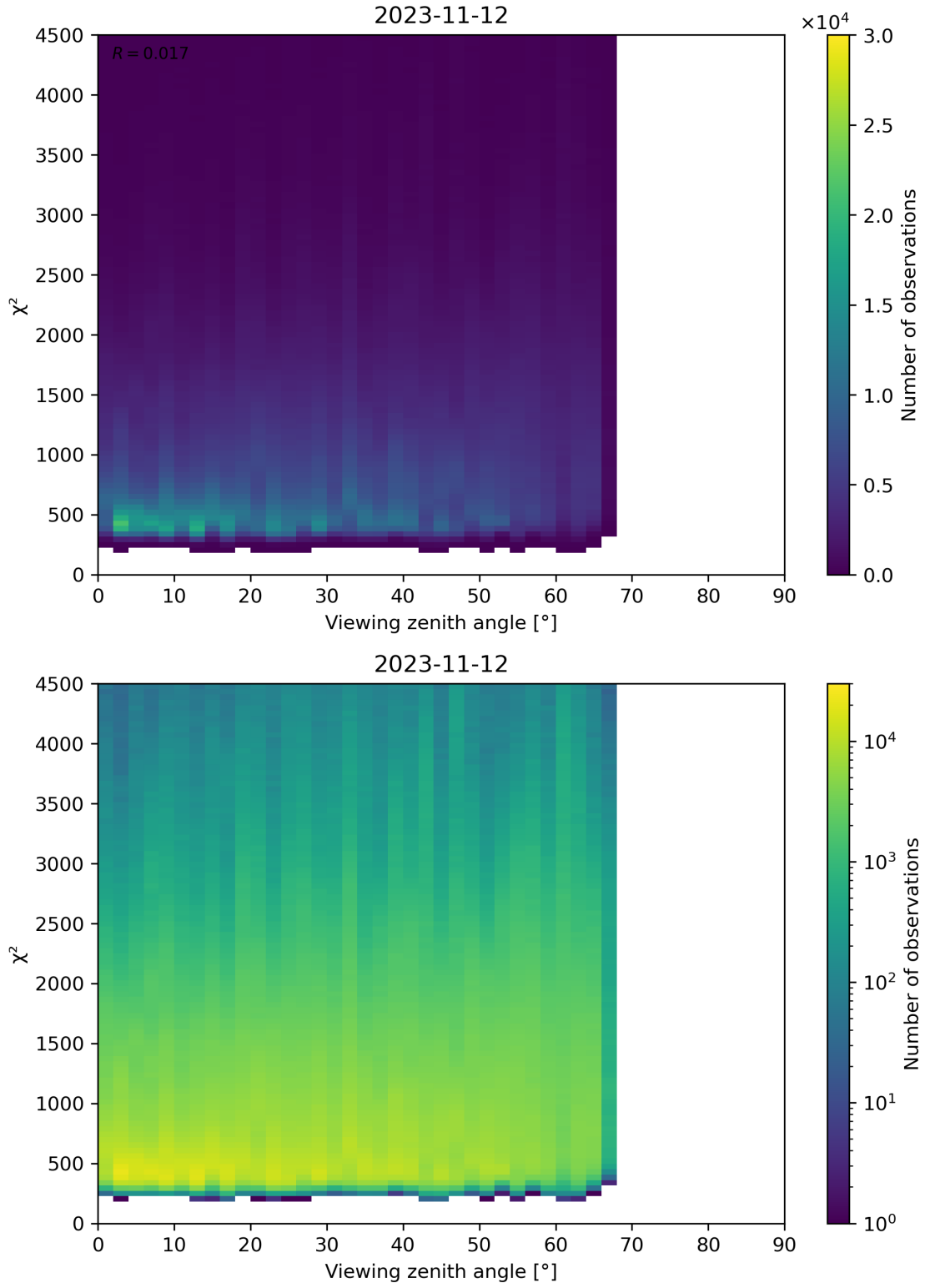
Figure 72: Scatter density plot of “Viewing zenith angle” against “ \chi^2 ” for 2023-11-12 to 2023-11-13.
