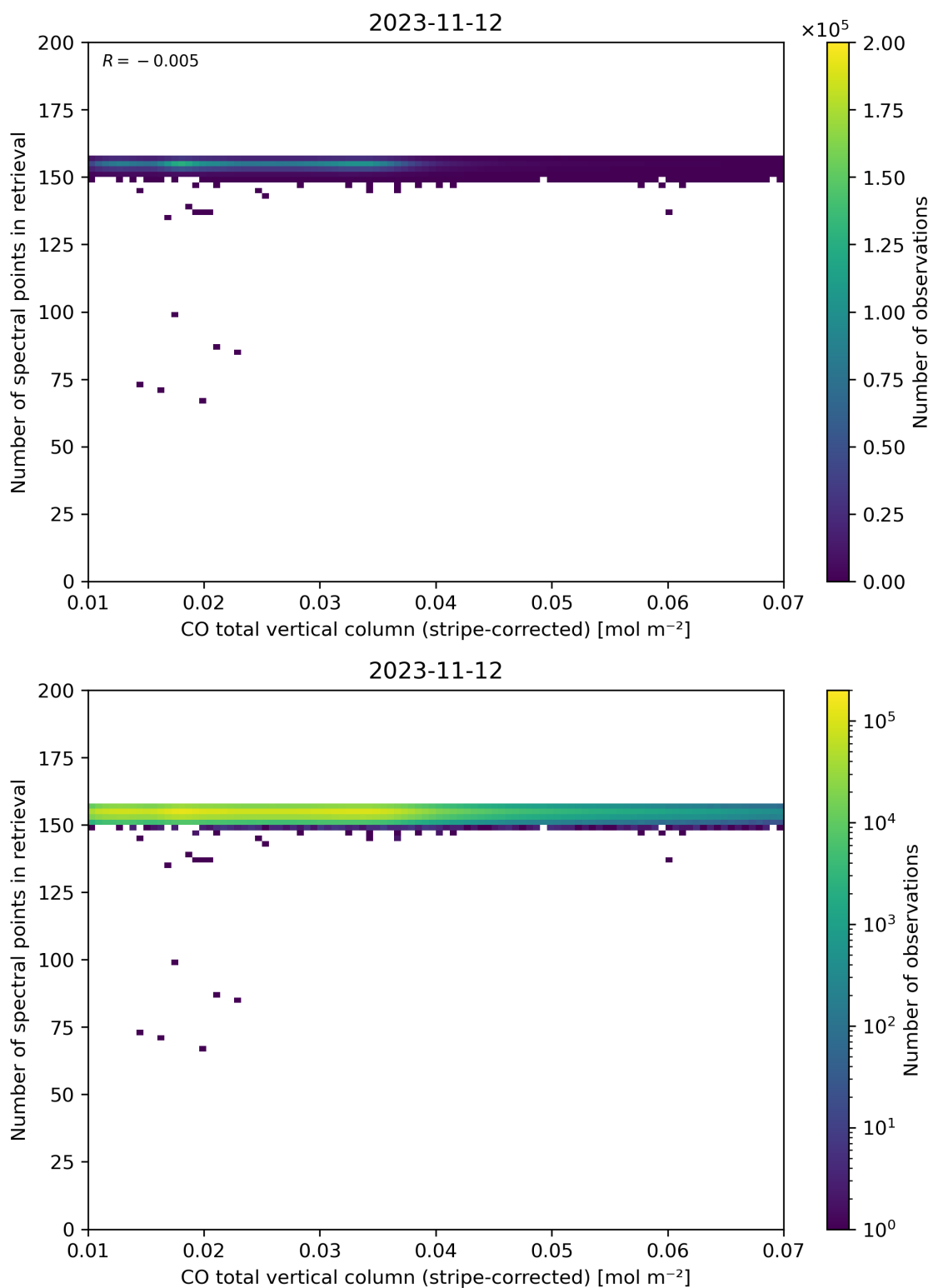
Figure 40: Scatter density plot of “CO total vertical column (stripe-corrected)” against “Number of spectral points in retrieval” for 2023-11-12 to 2023-11-13.
