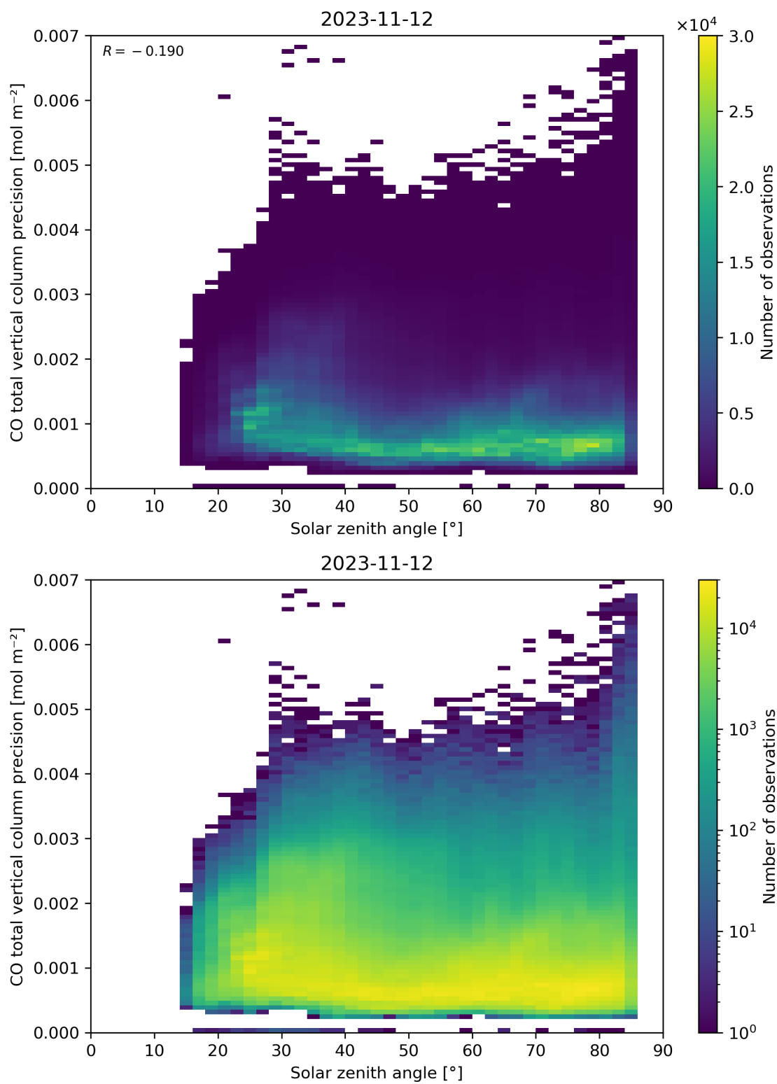
Figure 63: Scatter density plot of “Solar zenith angle” against “CO total vertical column precision” for 2023-11-12 to 2023-11-13.
