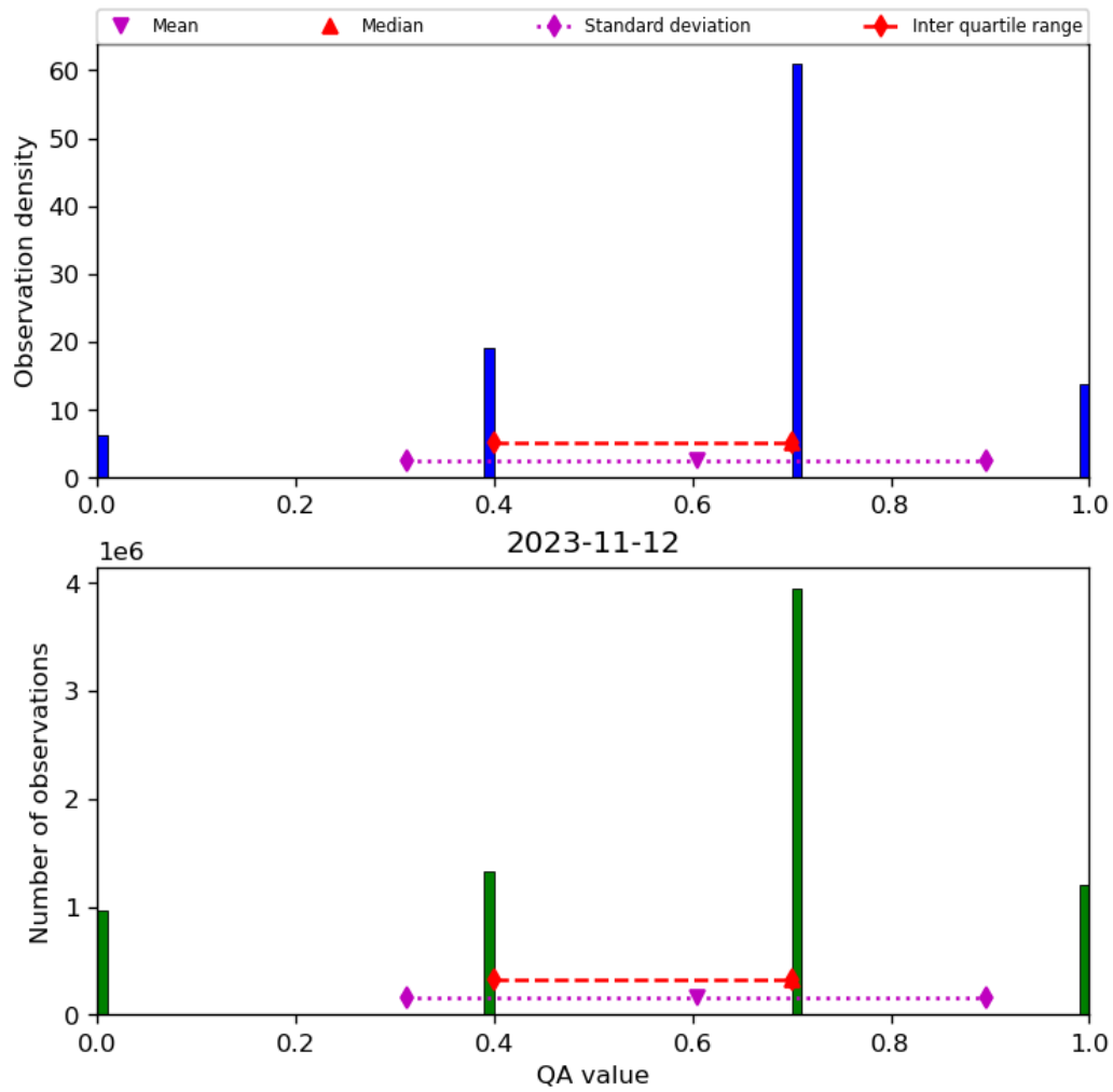
Figure 17: Histogram of “QA value” for 2023-11-12 to 2023-11-13
