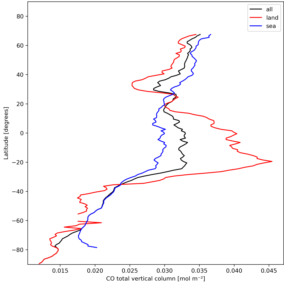
Figure 10: Zonal average of “CO total vertical column” for 2023-11-12 to 2023-11-13.
