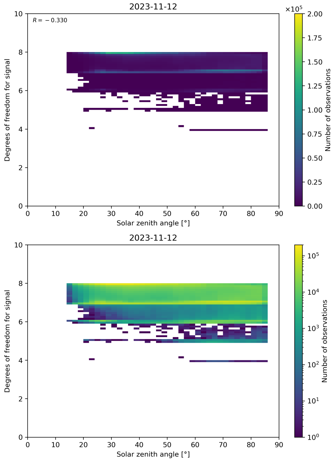
Figure 65: Scatter density plot of “Solar zenith angle” against “Degrees of freedom for signal” for 2023-11-12 to 2023-11-13.
