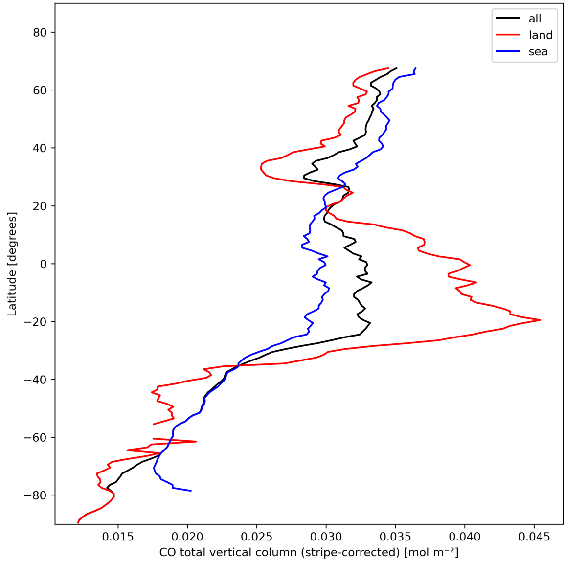
Figure 11: Zonal average of “CO total vertical column (stripe-corrected)” for 2023-11-12 to 2023-11-13.
