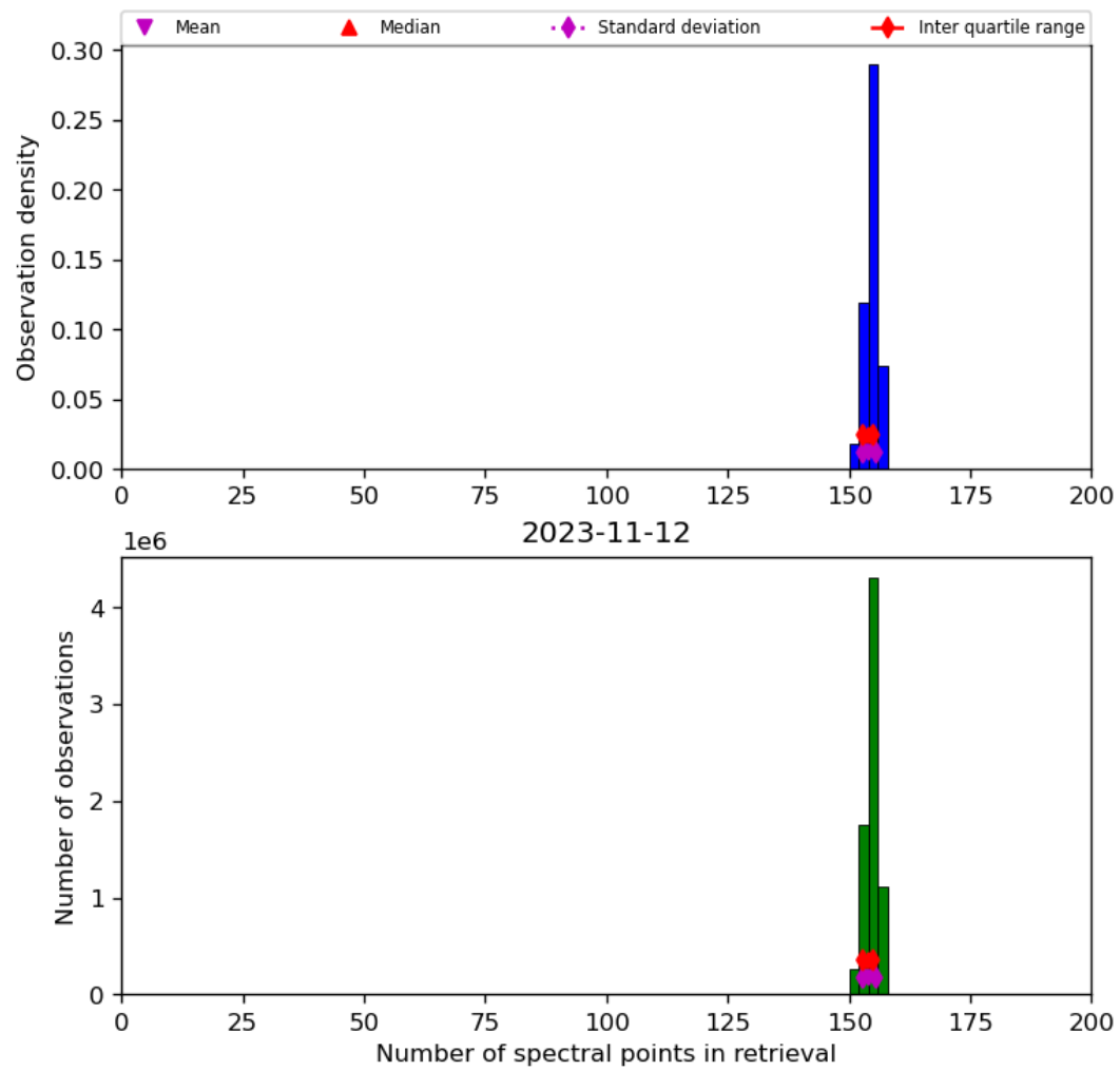
Figure 21: Histogram of “Number of spectral points in retrieval” for 2023-11-12 to 2023-11-13
