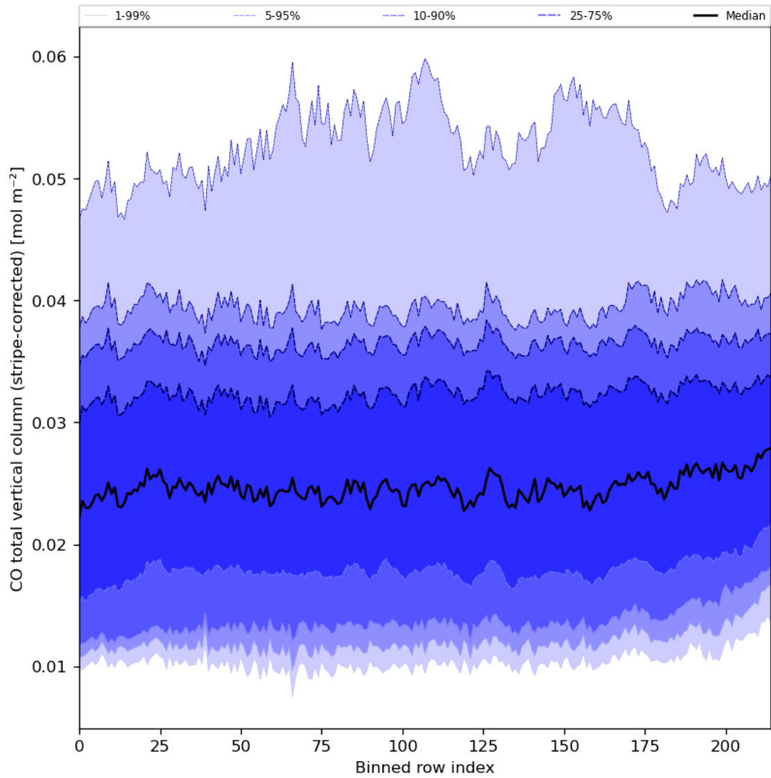
Figure 27: Along track statistics of “CO total vertical column (stripe-corrected)” for 2023-11-12 to 2023-11-13
