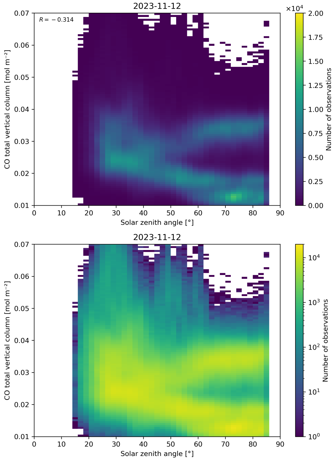
Figure 61: Scatter density plot of “Solar zenith angle” against “CO total vertical column” for 2023-11-12 to 2023-11-13.
