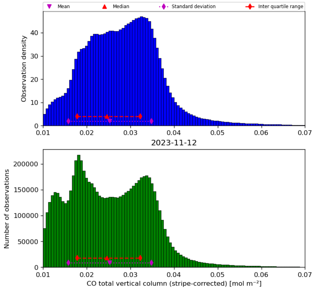
Figure 19: Histogram of “CO total vertical column (stripe-corrected)” for 2023-11-12 to 2023-11-13
