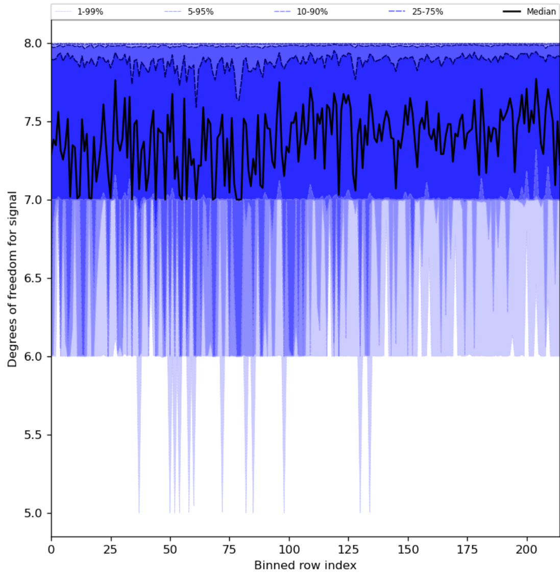
Figure 31: Along track statistics of “Degrees of freedom for signal” for 2023-11-12 to 2023-11-13
