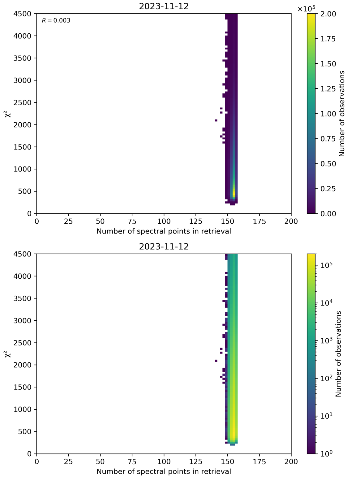
Figure 58: Scatter density plot of “Number of spectral points in retrieval” against “ \chi^2 ” for 2023-11-12 to 2023-11-13.
