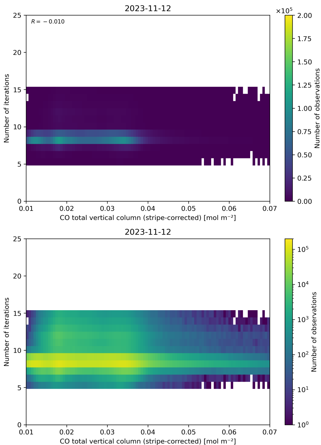
Figure 39: Scatter density plot of “CO total vertical column (stripe-corrected)” against “Number of iterations” for 2023-11-12 to 2023-11-13.
