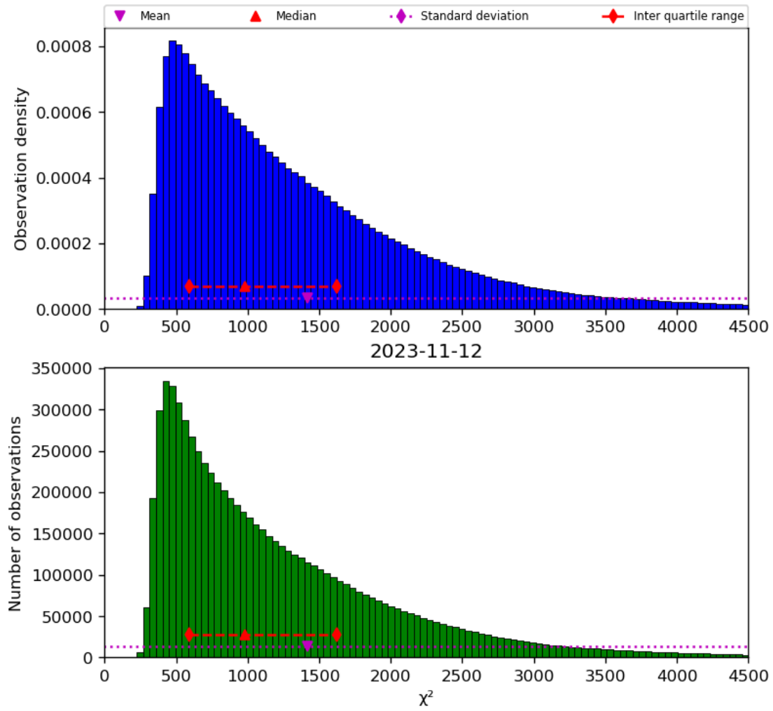
Figure 22: Histogram of “ \chi^2 ” for 2023-11-12 to 2023-11-13
