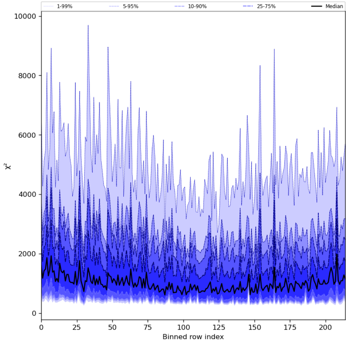
Figure 30: Along track statistics of “ \chi^2 ” for 2023-11-12 to 2023-11-13
