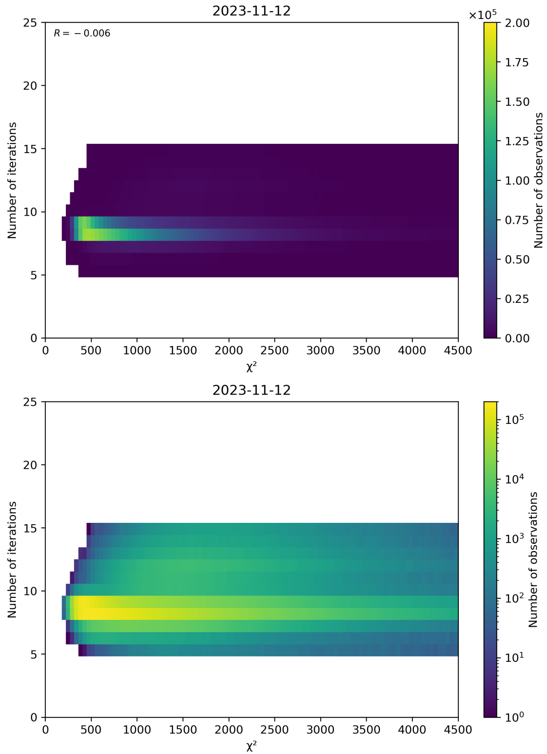
Figure 49: Scatter density plot of “ \chi^2 ” against “Number of iterations” for 2023-11-12 to 2023-11-13.
