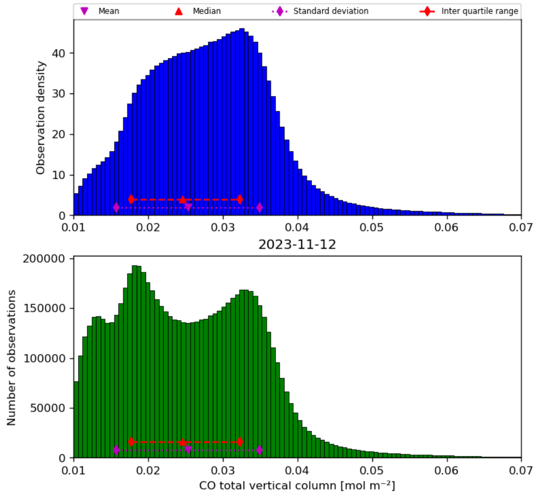
Figure 18: Histogram of “CO total vertical column” for 2023-11-12 to 2023-11-13
