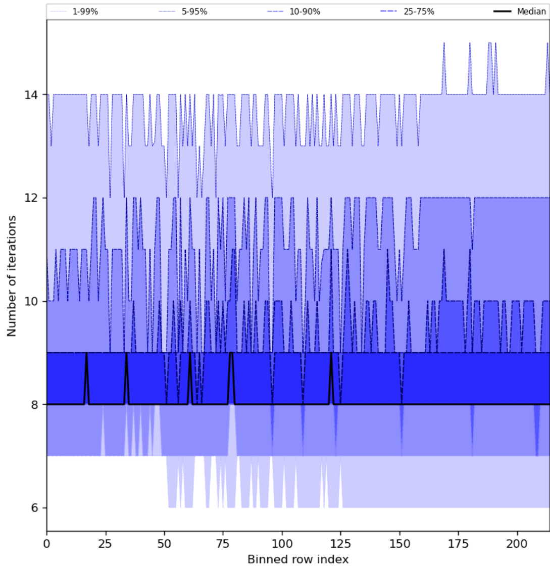
Figure 32: Along track statistics of “Number of iterations” for 2023-11-12 to 2023-11-13
