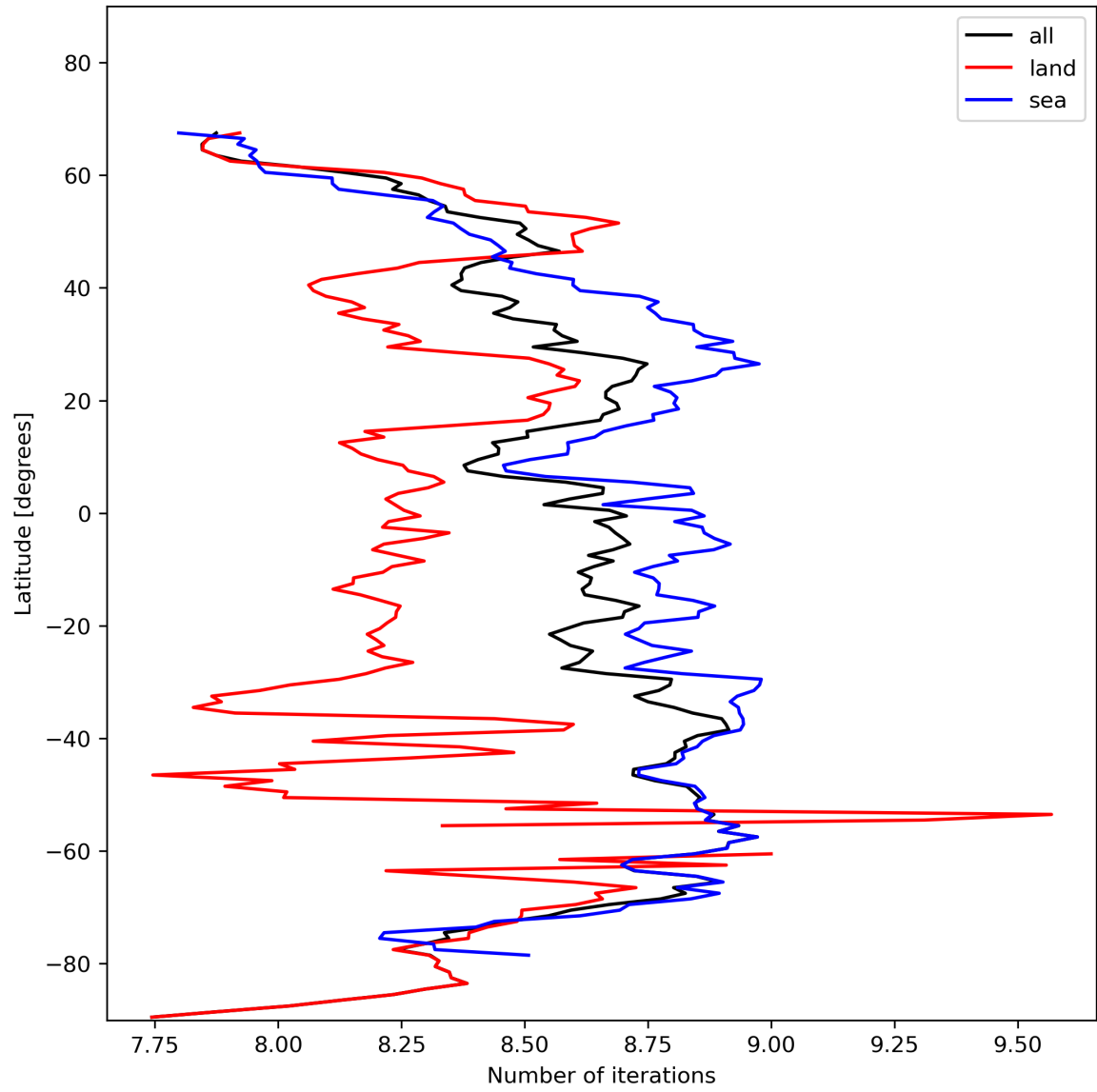
Figure 16: Zonal average of “Number of iterations” for 2023-11-12 to 2023-11-13.
