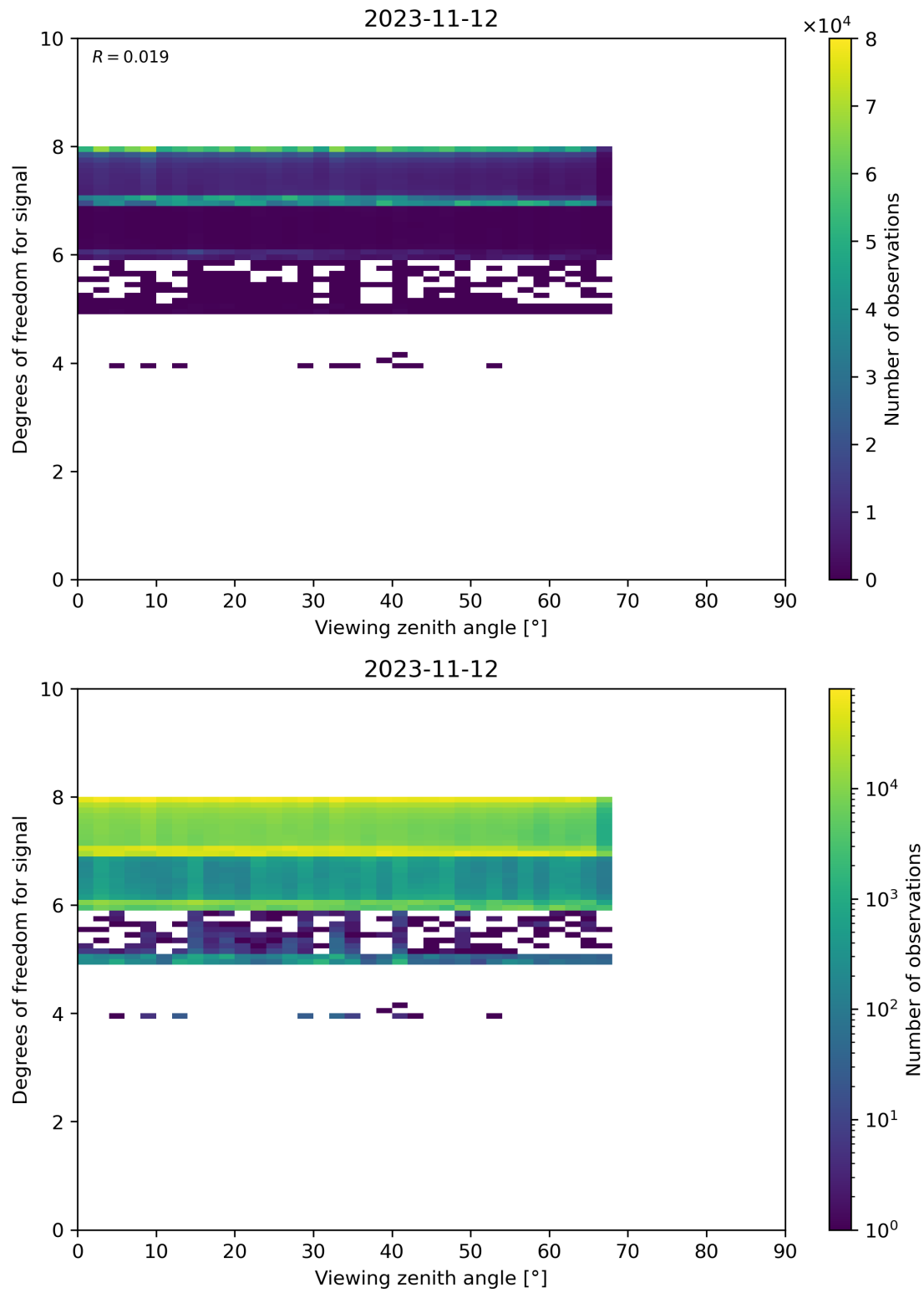
Figure 73: Scatter density plot of “Viewing zenith angle” against “Degrees of freedom for signal” for 2023-11-12 to 2023-11-13.
