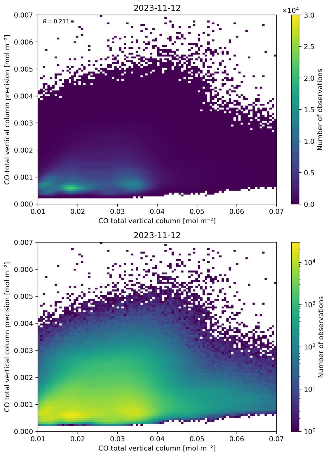
Figure 34: Scatter density plot of “CO total vertical column” against “CO total vertical column precision” for 2023-11-12 to 2023-11-13.
