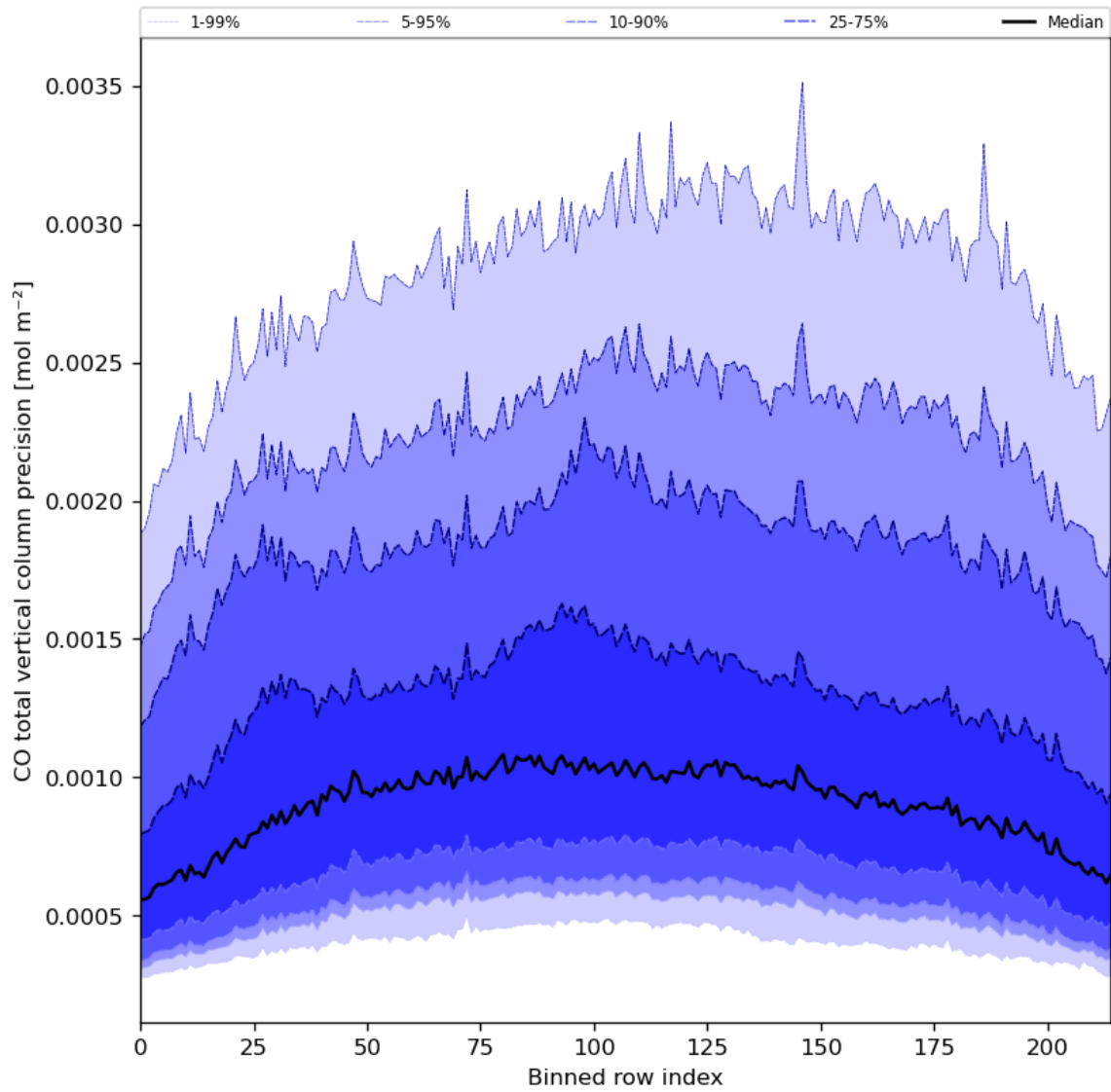
Figure 28: Along track statistics of “CO total vertical column precision” for 2023-11-12 to 2023-11-13
