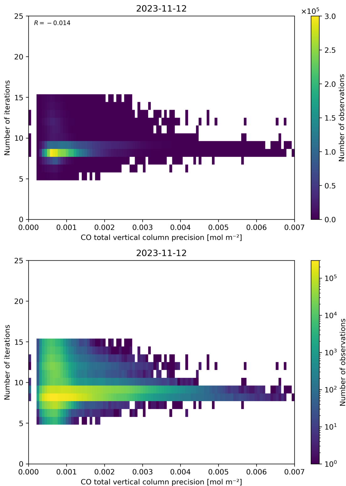
Figure 46: Scatter density plot of “CO total vertical column precision” against “Number of iterations” for 2023-11-12 to 2023-11-13.
