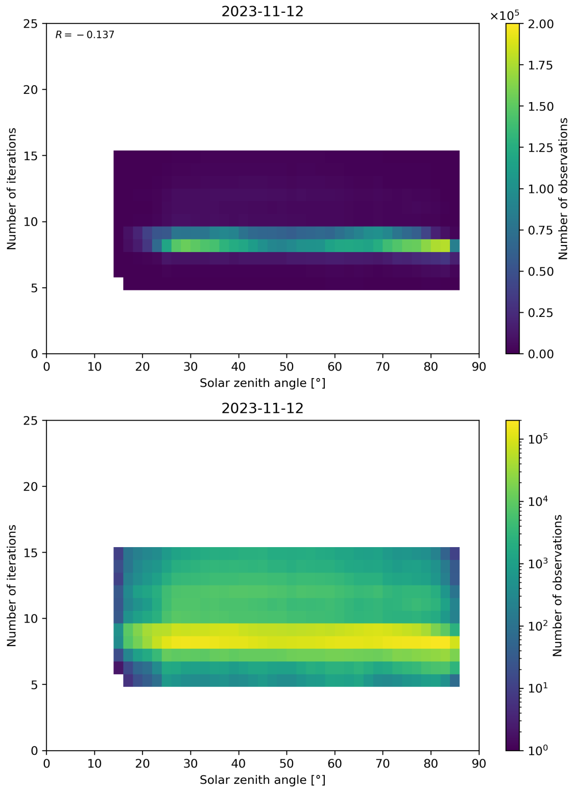
Figure 67: Scatter density plot of “Solar zenith angle” against “Number of iterations” for 2023-11-12 to 2023-11-13.
