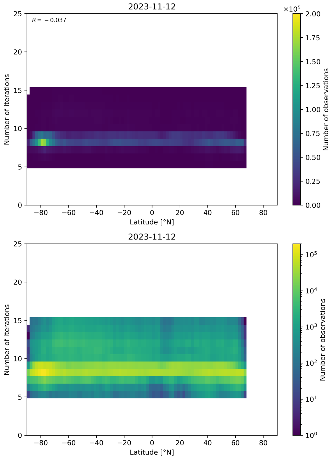
Figure 56: Scatter density plot of “Latitude” against “Number of iterations” for 2023-11-12 to 2023-11-13.
