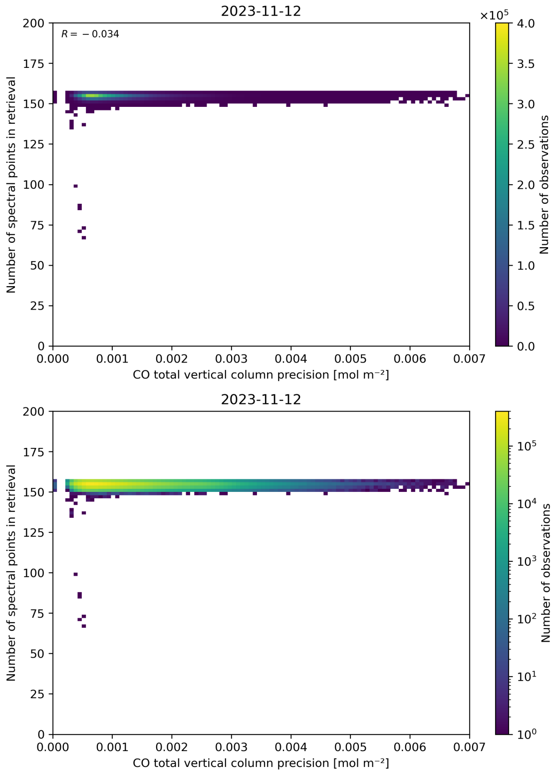
Figure 47: Scatter density plot of “CO total vertical column precision” against “Number of spectral points in retrieval” for 2023-11-12 to 2023-11-13.
