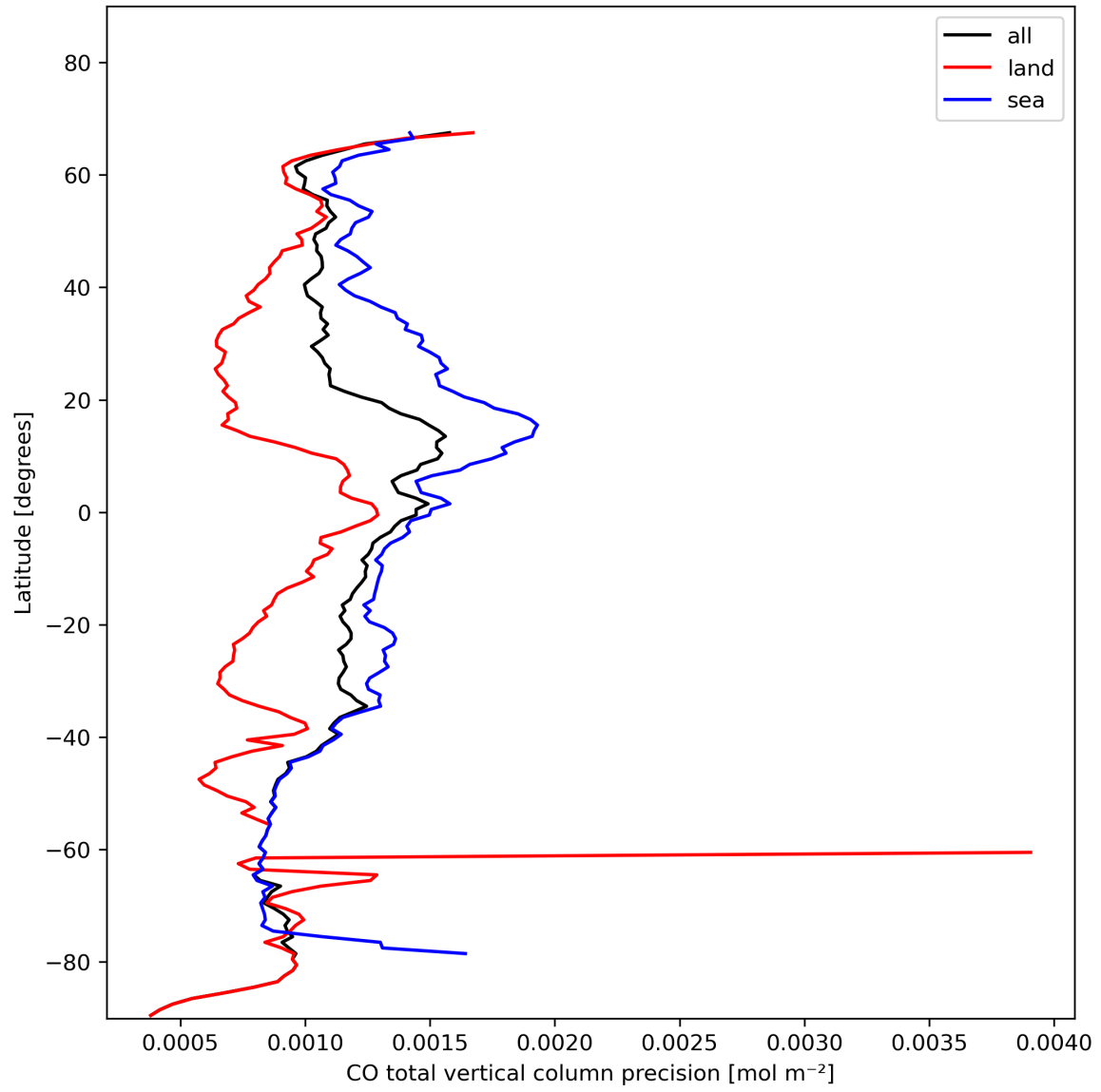
Figure 12: Zonal average of “CO total vertical column precision” for 2023-11-12 to 2023-11-13.
