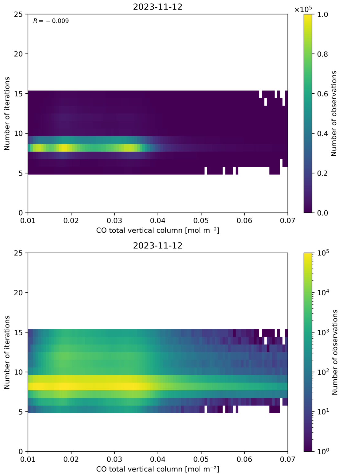
Figure 42: Scatter density plot of “CO total vertical column” against “Number of iterations” for 2023-11-12 to 2023-11-13.
