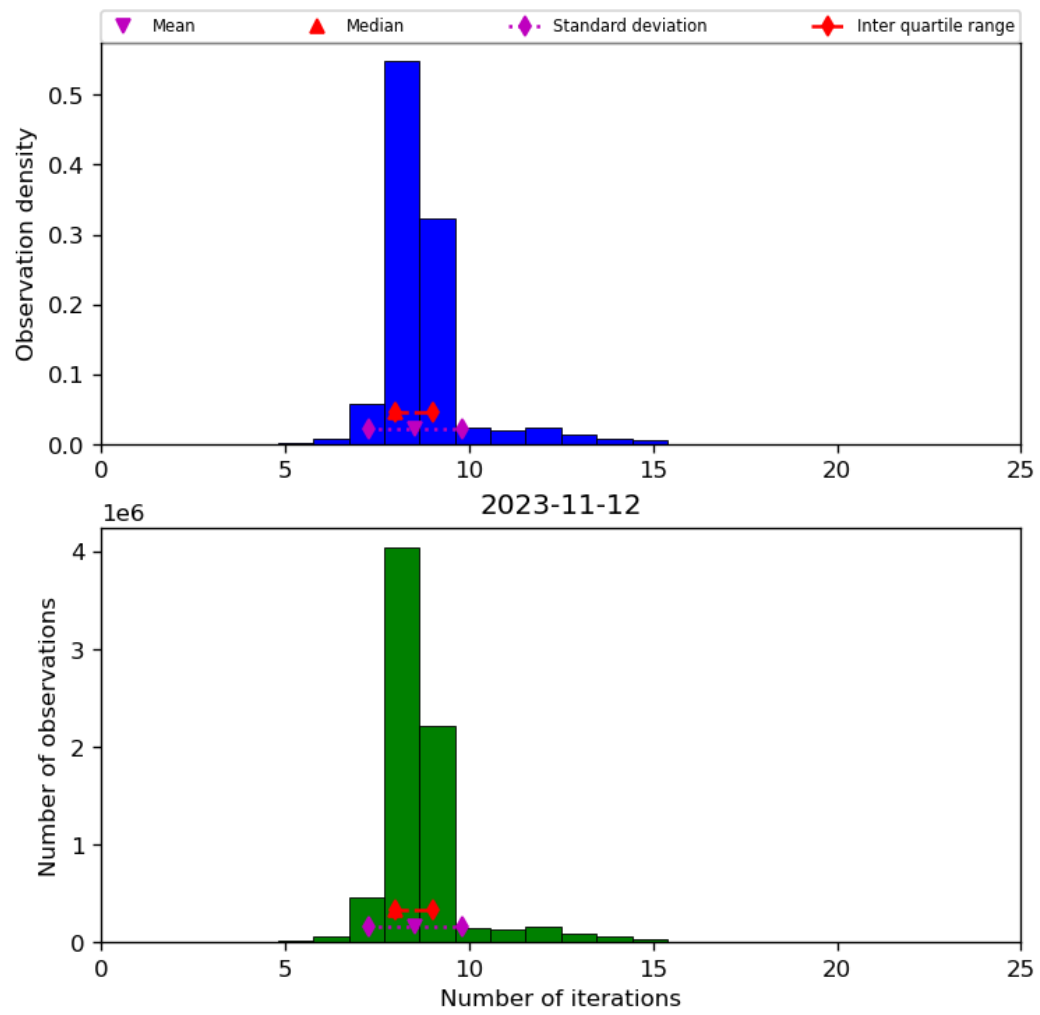
Figure 24: Histogram of “Number of iterations” for 2023-11-12 to 2023-11-13
