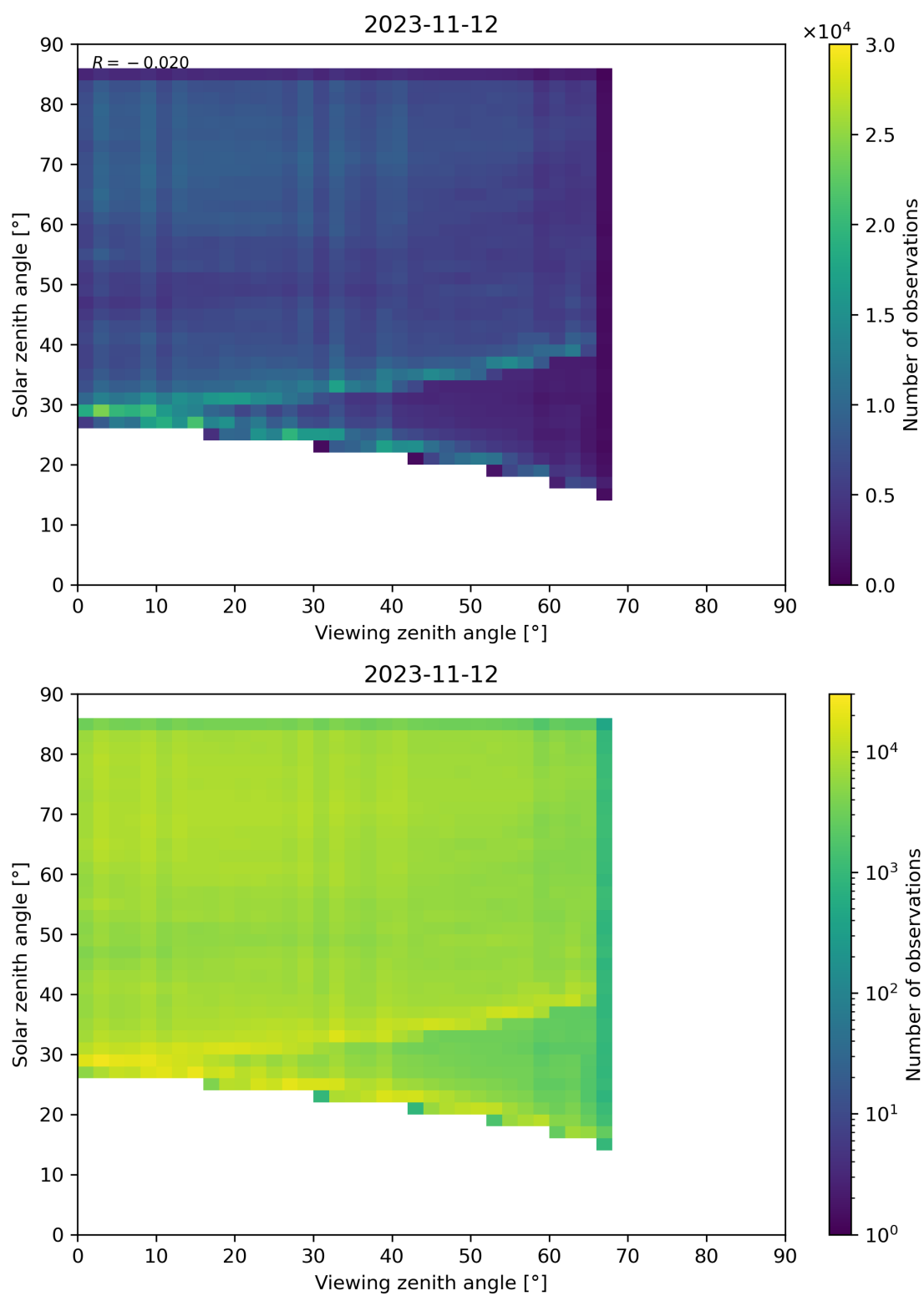
Figure 77: Scatter density plot of “Viewing zenith angle” against “Solar zenith angle” for 2023-11-12 to 2023-11-13.
