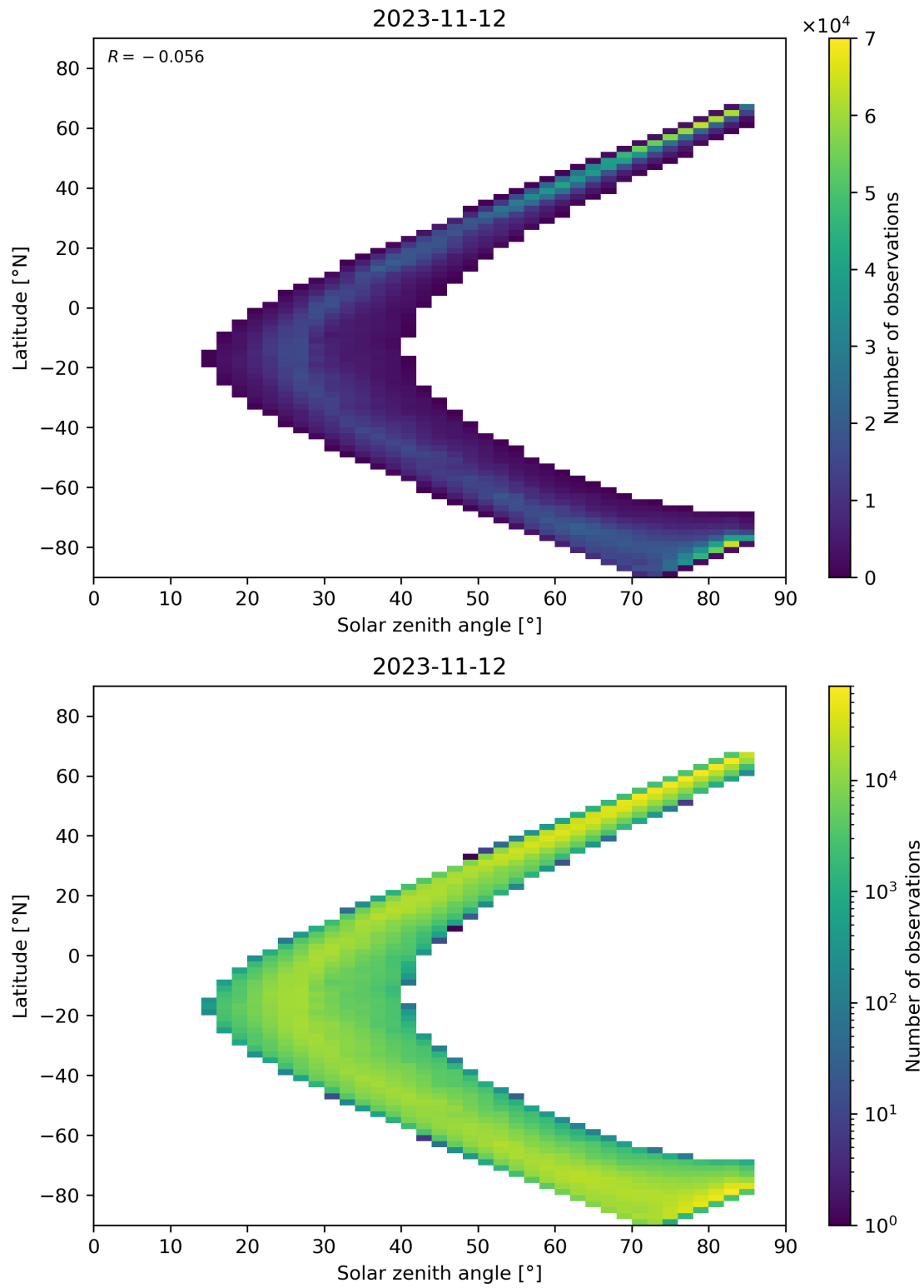
Figure 66: Scatter density plot of “Solar zenith angle” against “Latitude” for 2023-11-12 to 2023-11-13.
