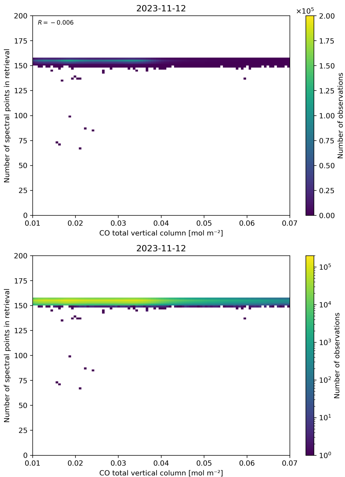
Figure 43: Scatter density plot of “CO total vertical column” against “Number of spectral points in retrieval” for 2023-11-12 to 2023-11-13.
