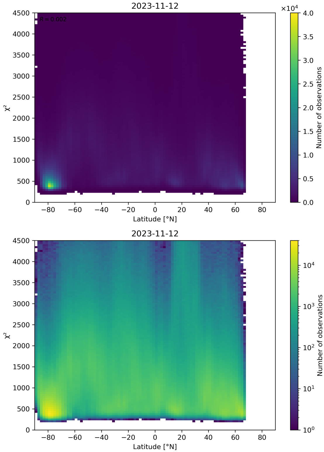
Figure 54: Scatter density plot of “Latitude” against “ \chi^2 ” for 2023-11-12 to 2023-11-13.
