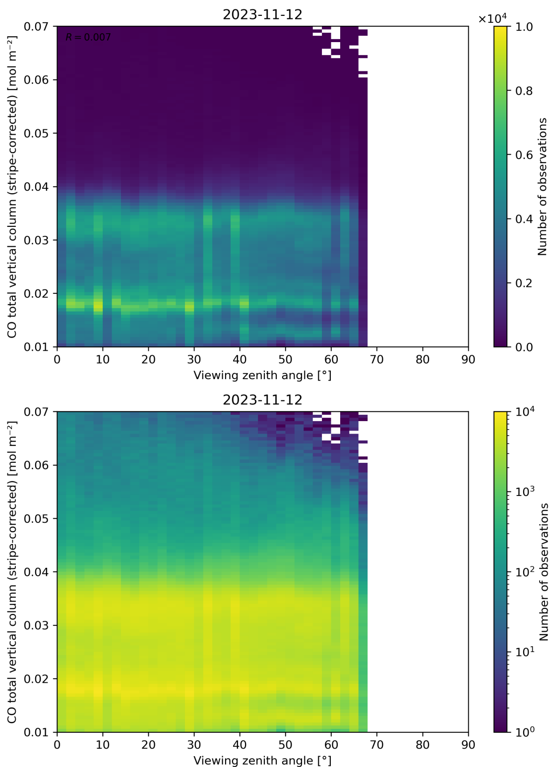
Figure 70: Scatter density plot of “Viewing zenith angle” against “CO total vertical column (stripe-corrected)” for 2023-11-12 to 2023-11-13.
