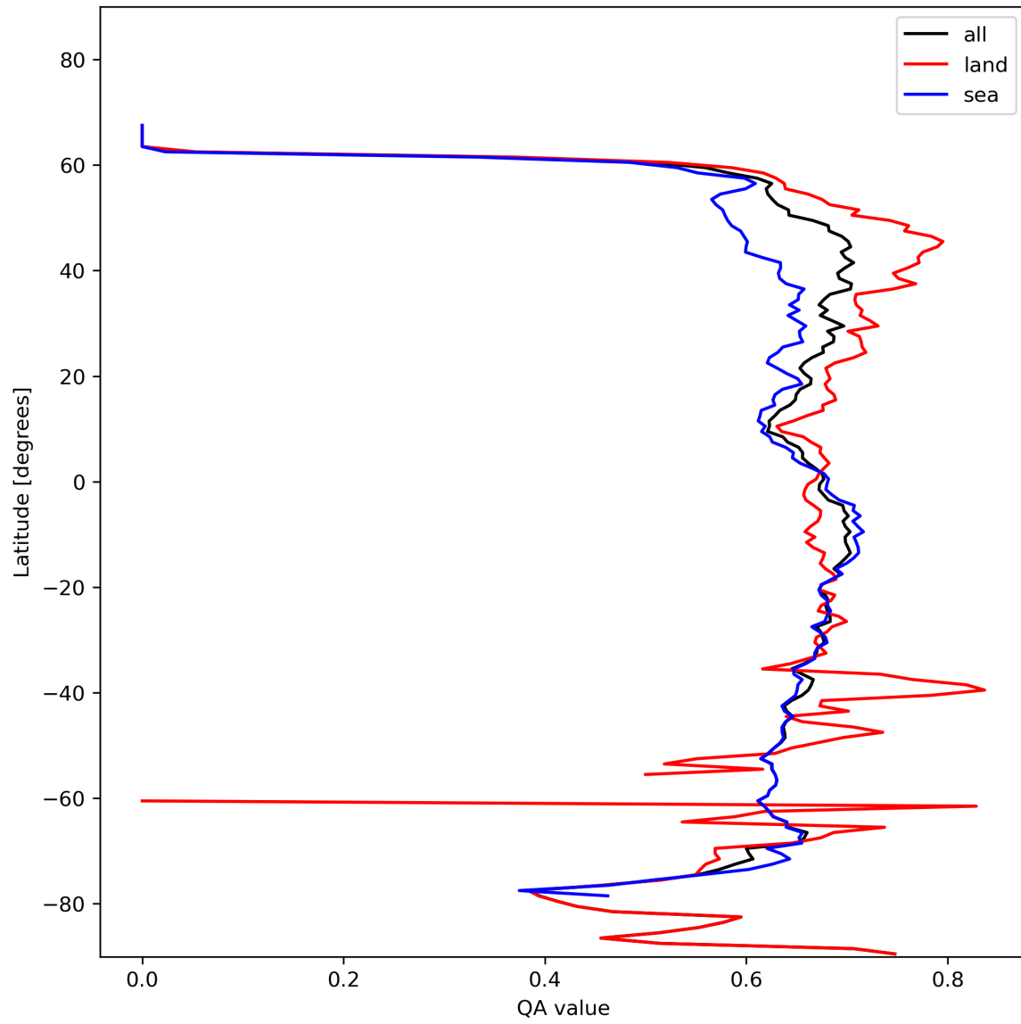
Figure 9: Zonal average of “QA value” for 2023-11-12 to 2023-11-13.
