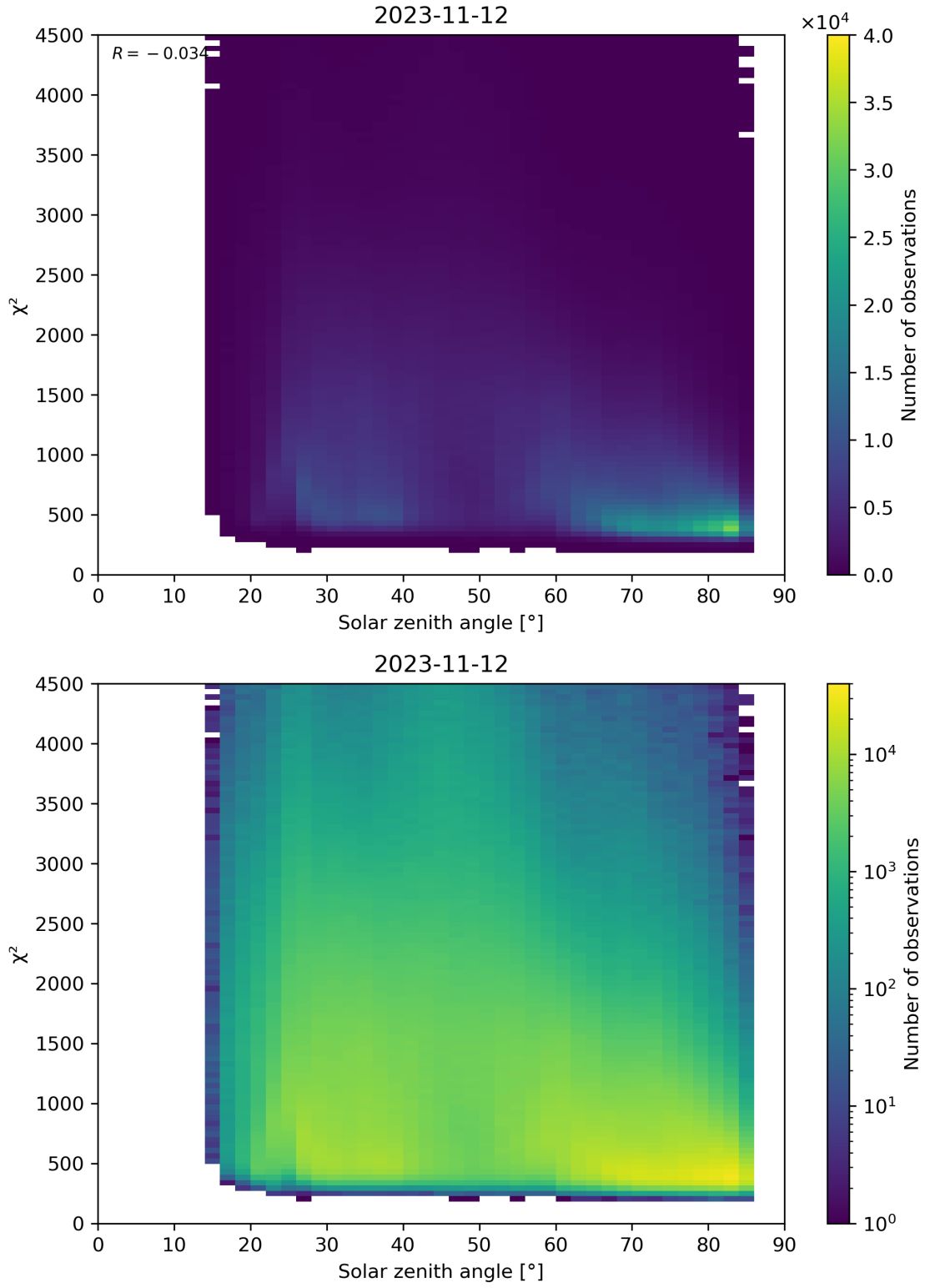
Figure 64: Scatter density plot of “Solar zenith angle” against “ \chi^2 ” for 2023-11-12 to 2023-11-13.
