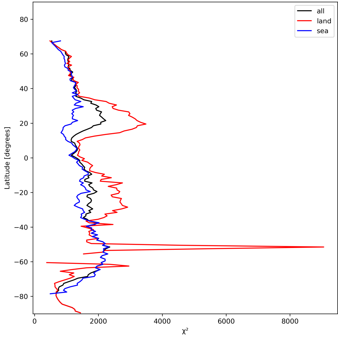
Figure 14: Zonal average of “ \chi^2 ” for 2023-11-12 to 2023-11-13.
