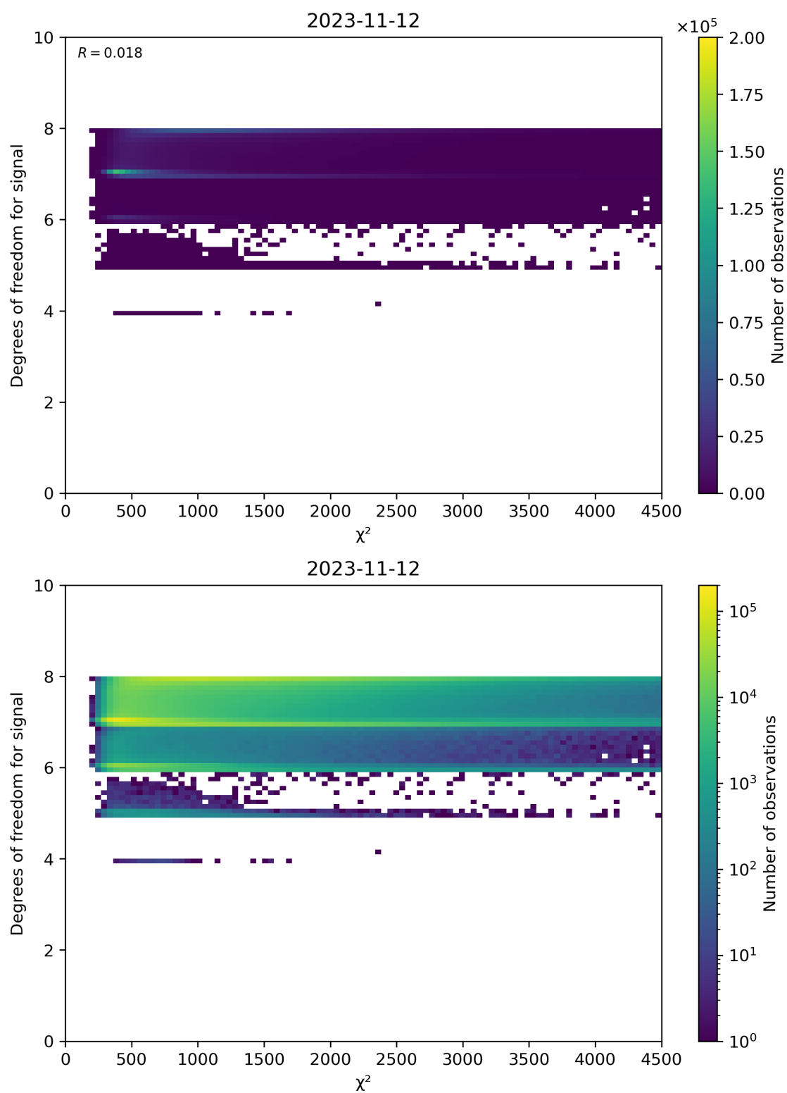
Figure 48: Scatter density plot of " \chi^2 " against "Degrees of freedom for signal" for 2023-11-12 to 2023-11-13.
