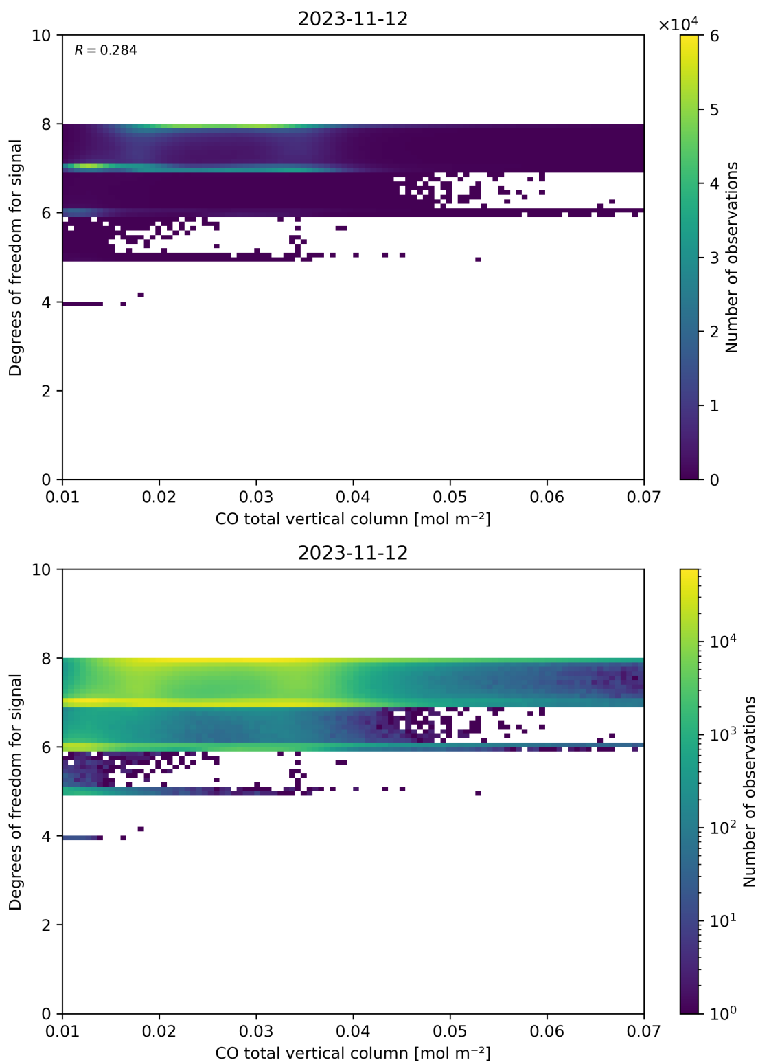
Figure 41: Scatter density plot of “CO total vertical column” against “Degrees of freedom for signal” for 2023-11-12 to 2023-11-13.
