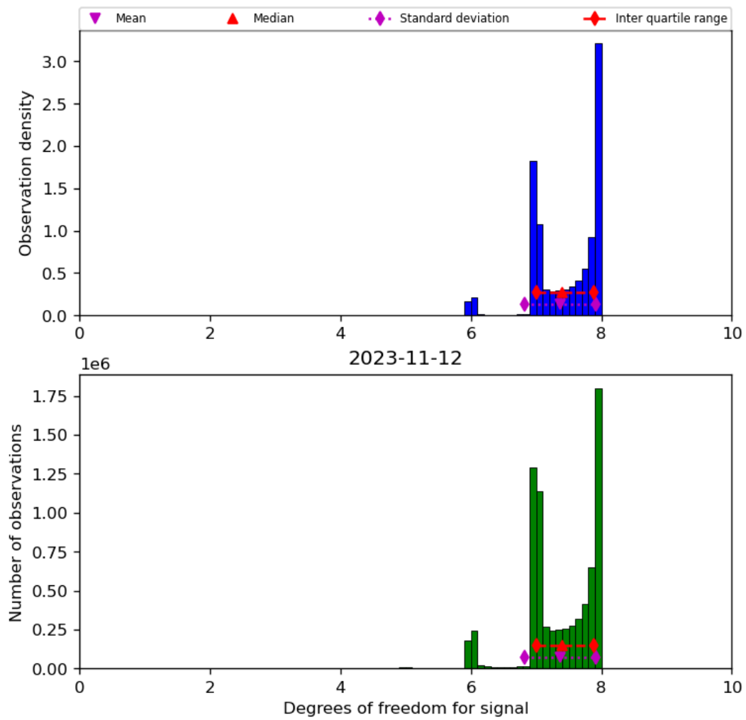
Figure 23: Histogram of “Degrees of freedom for signal” for 2023-11-12 to 2023-11-13
