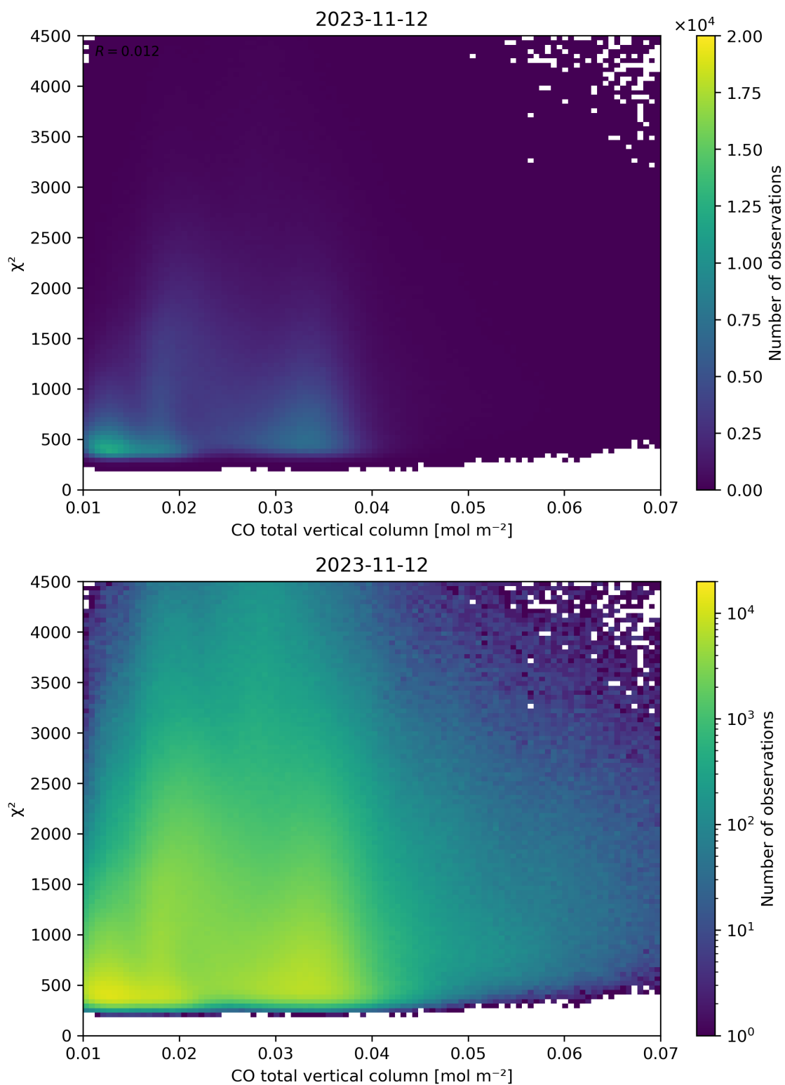
Figure 35: Scatter density plot of “CO total vertical column” against “ \chi^2 ” for 2023-11-12 to 2023-11-13.
