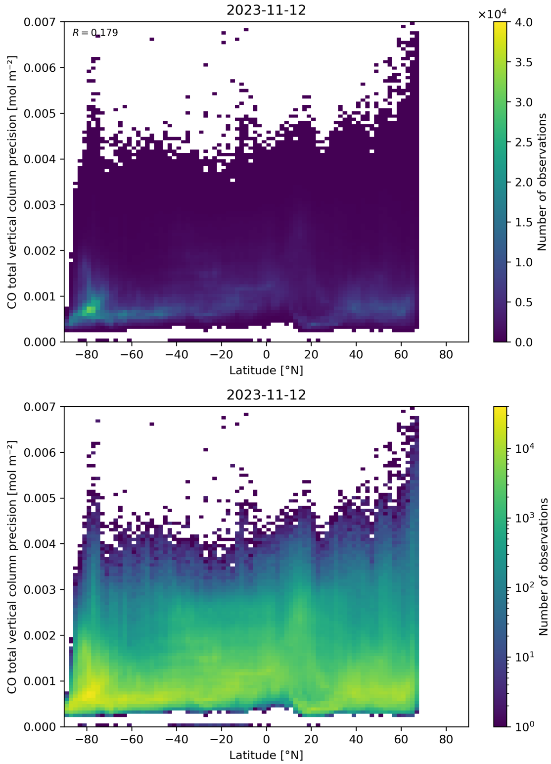
Figure 53: Scatter density plot of “Latitude” against “CO total vertical column precision” for 2023-11-12 to 2023-11-13.
