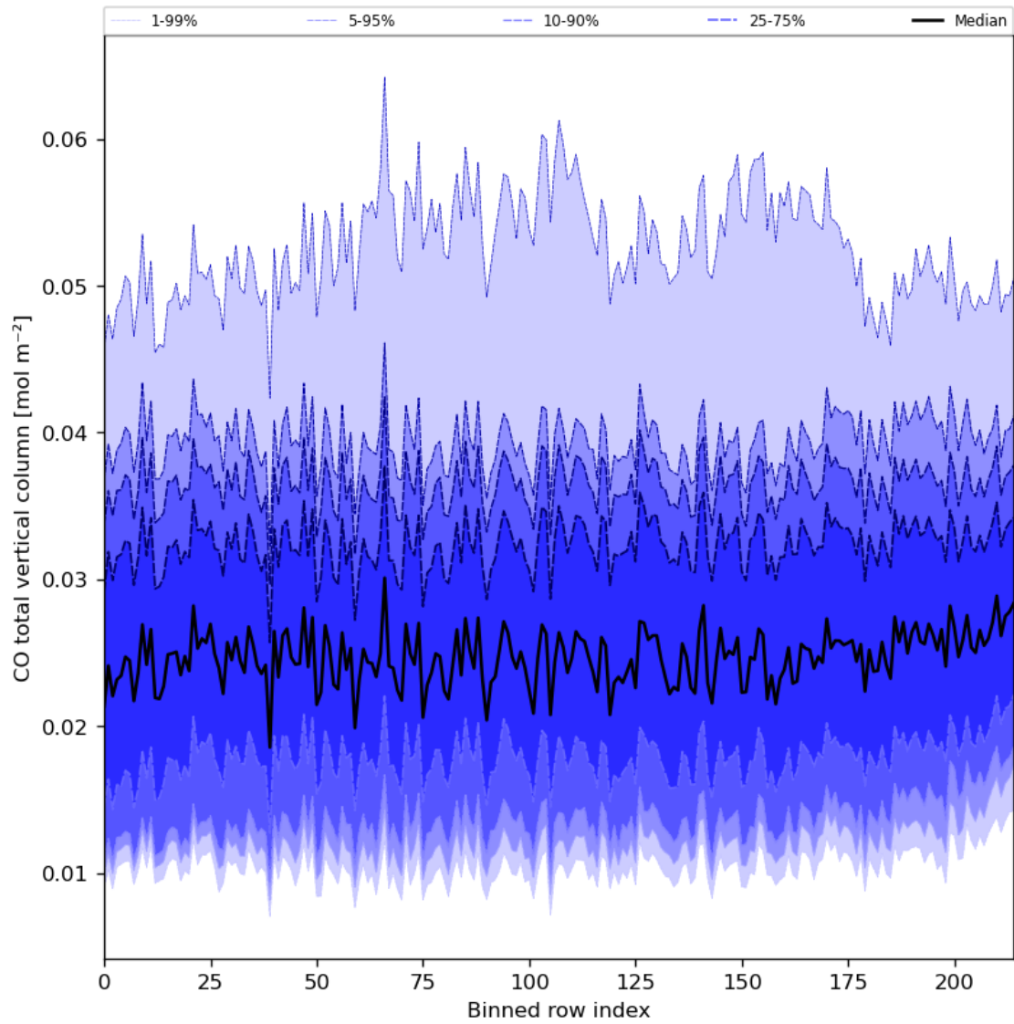
Figure 26: Along track statistics of “CO total vertical column” for 2023-11-12 to 2023-11-13
