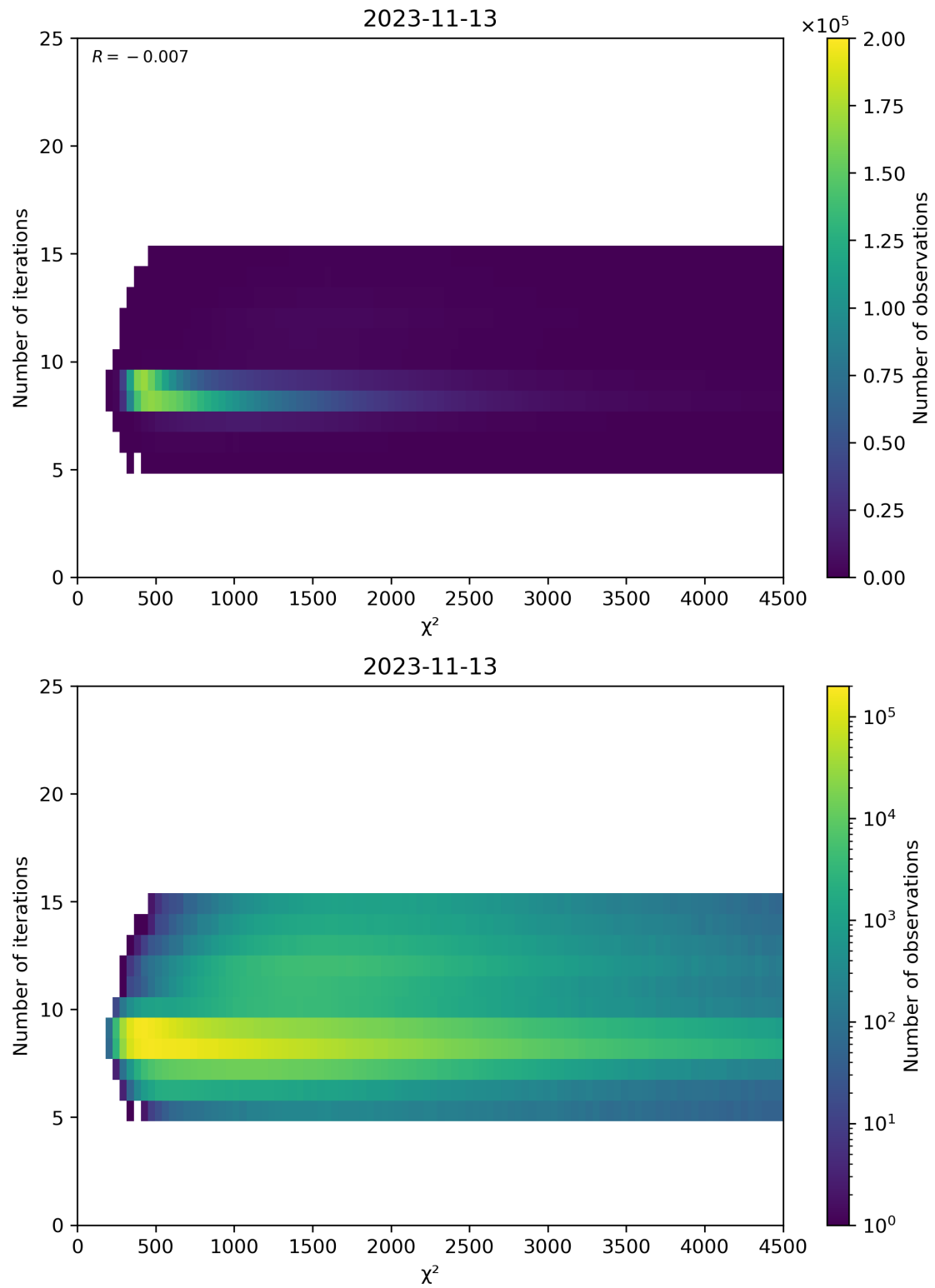
Figure 49: Scatter density plot of “ \chi^2 ” against “Number of iterations” for 2023-11-13 to 2023-11-14.
