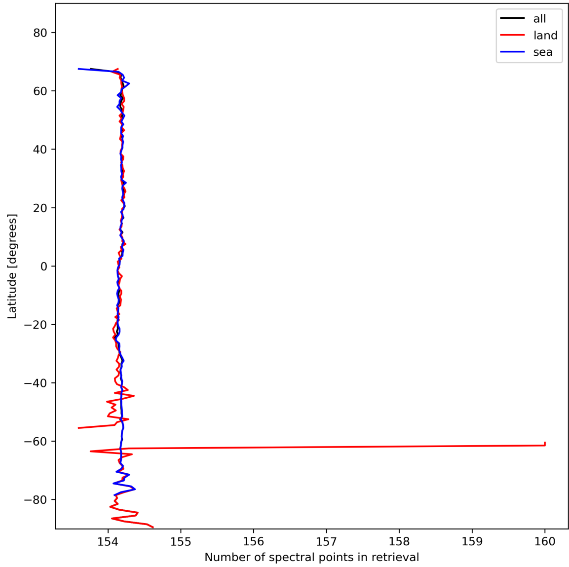
Figure 13: Zonal average of “Number of spectral points in retrieval” for 2023-11-13 to 2023-11-14.
