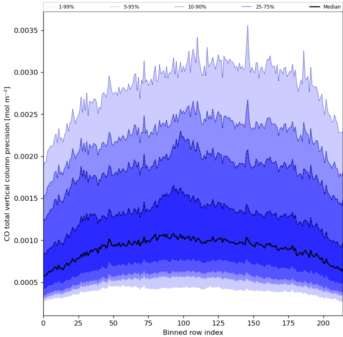
Figure 28: Along track statistics of “CO total vertical column precision” for 2023-11-13 to 2023-11-14
