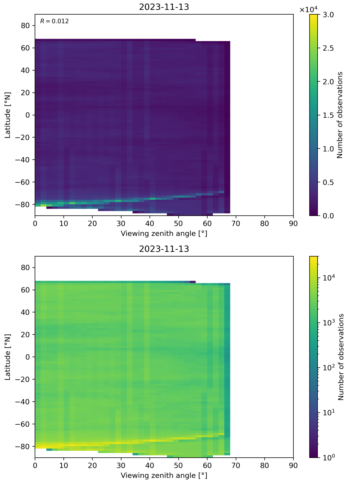
Figure 74: Scatter density plot of “Viewing zenith angle” against “Latitude” for 2023-11-13 to 2023-11-14.
