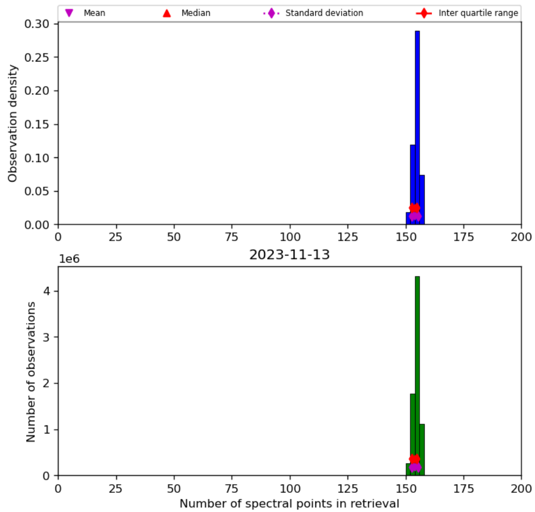
Figure 21: Histogram of “Number of spectral points in retrieval” for 2023-11-13 to 2023-11-14
