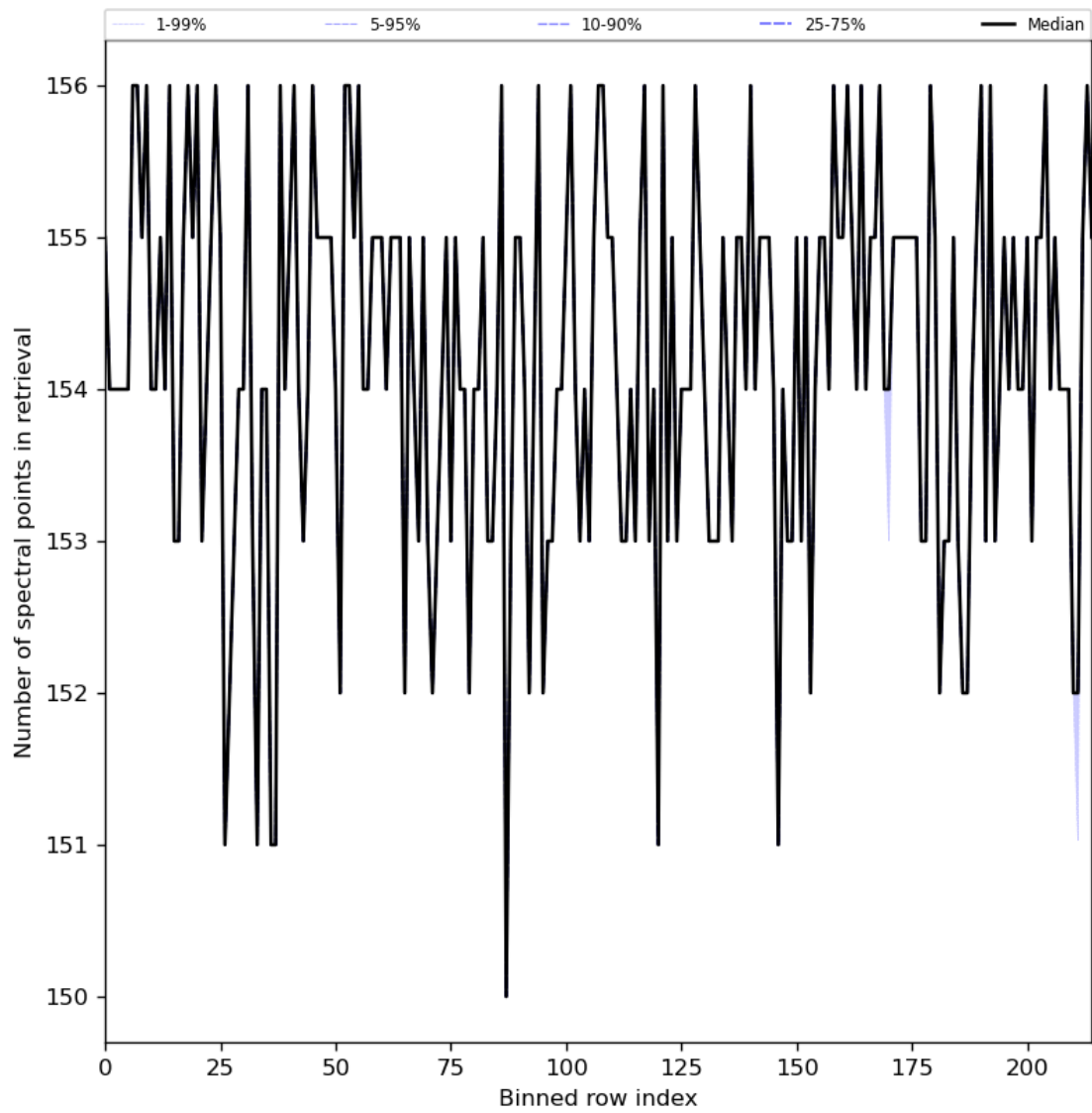
Figure 29: Along track statistics of “Number of spectral points in retrieval” for 2023-11-13 to 2023-11-14
