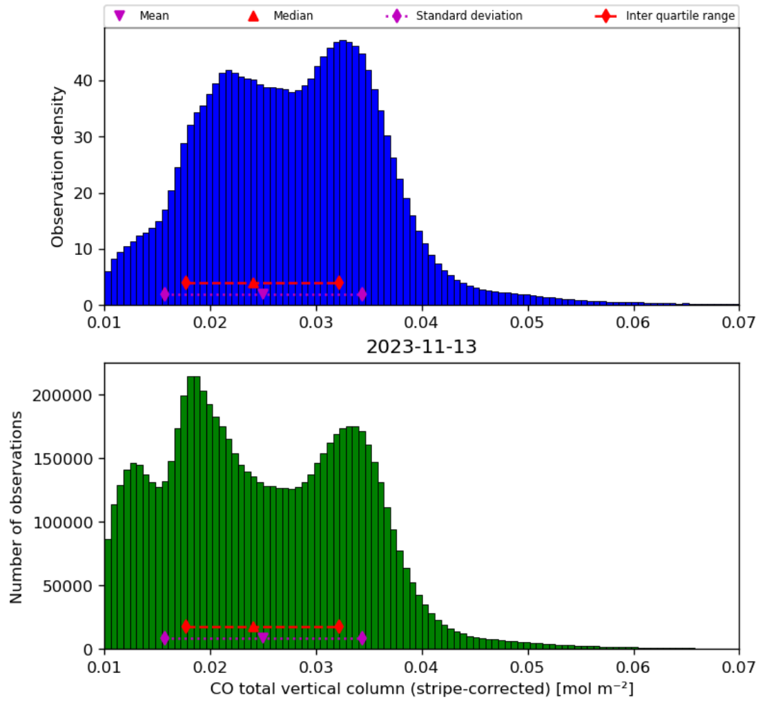
Figure 19: Histogram of “CO total vertical column (stripe-corrected)” for 2023-11-13 to 2023-11-14
