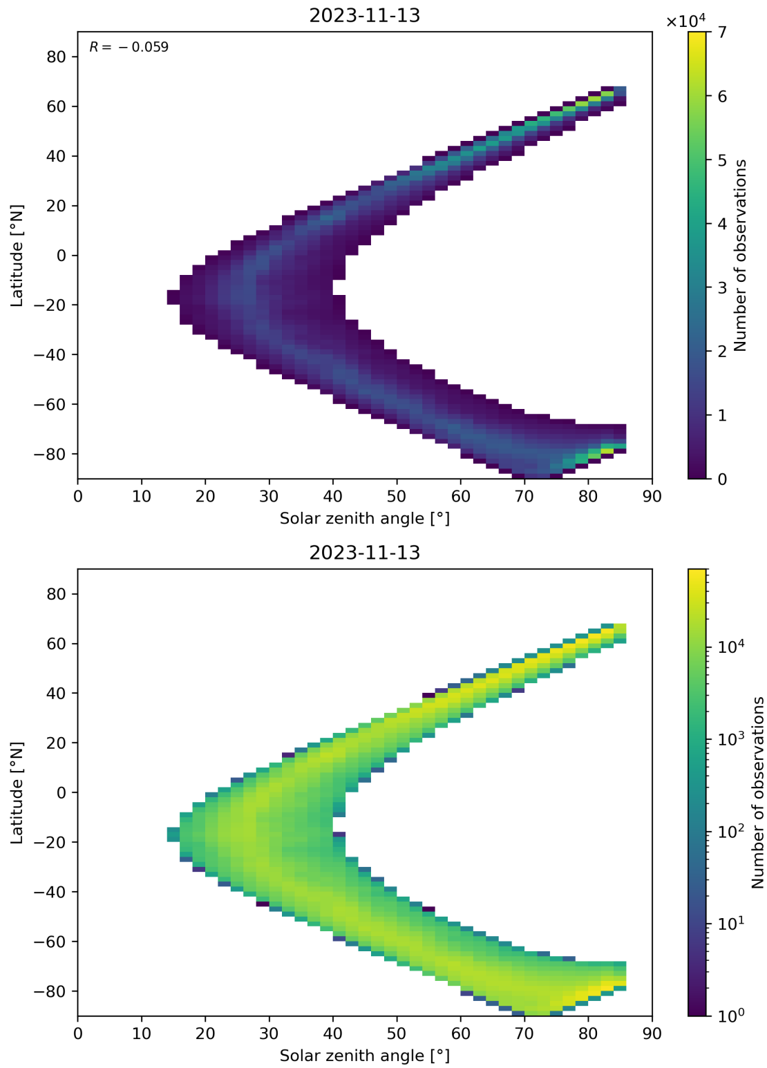
Figure 66: Scatter density plot of “Solar zenith angle” against “Latitude” for 2023-11-13 to 2023-11-14.
