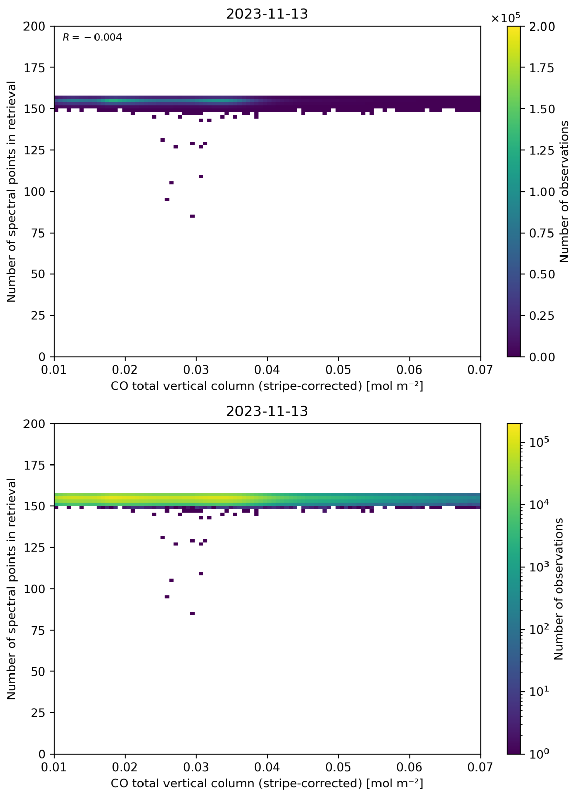
Figure 40: Scatter density plot of “CO total vertical column (stripe-corrected)” against “Number of spectral points in retrieval” for 2023-11-13 to 2023-11-14.
