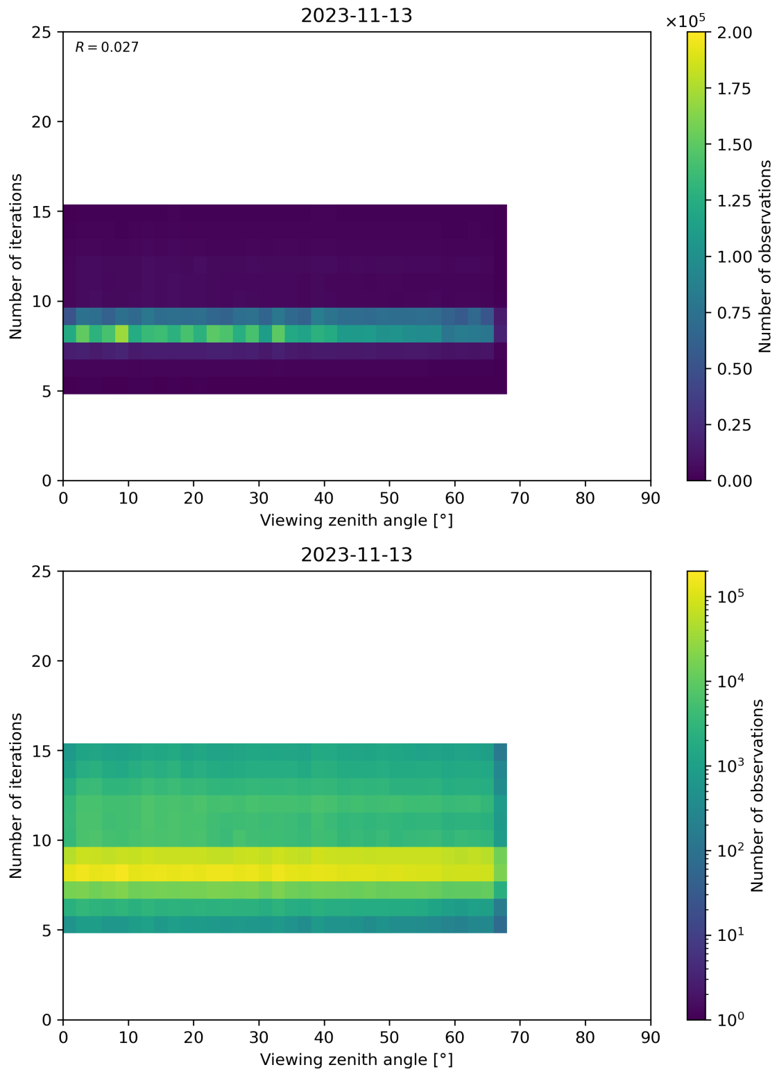
Figure 75: Scatter density plot of “Viewing zenith angle” against “Number of iterations” for 2023-11-13 to 2023-11-14.
