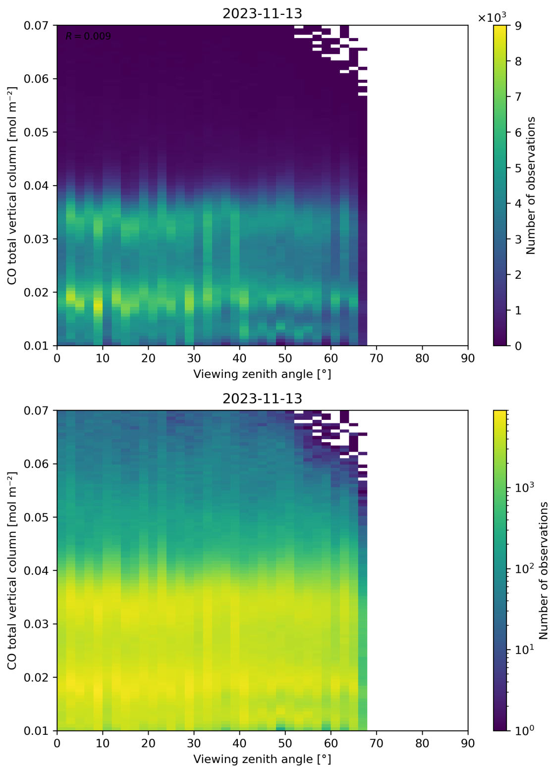
Figure 69: Scatter density plot of “Viewing zenith angle” against “CO total vertical column” for 2023-11-13 to 2023-11-14.
