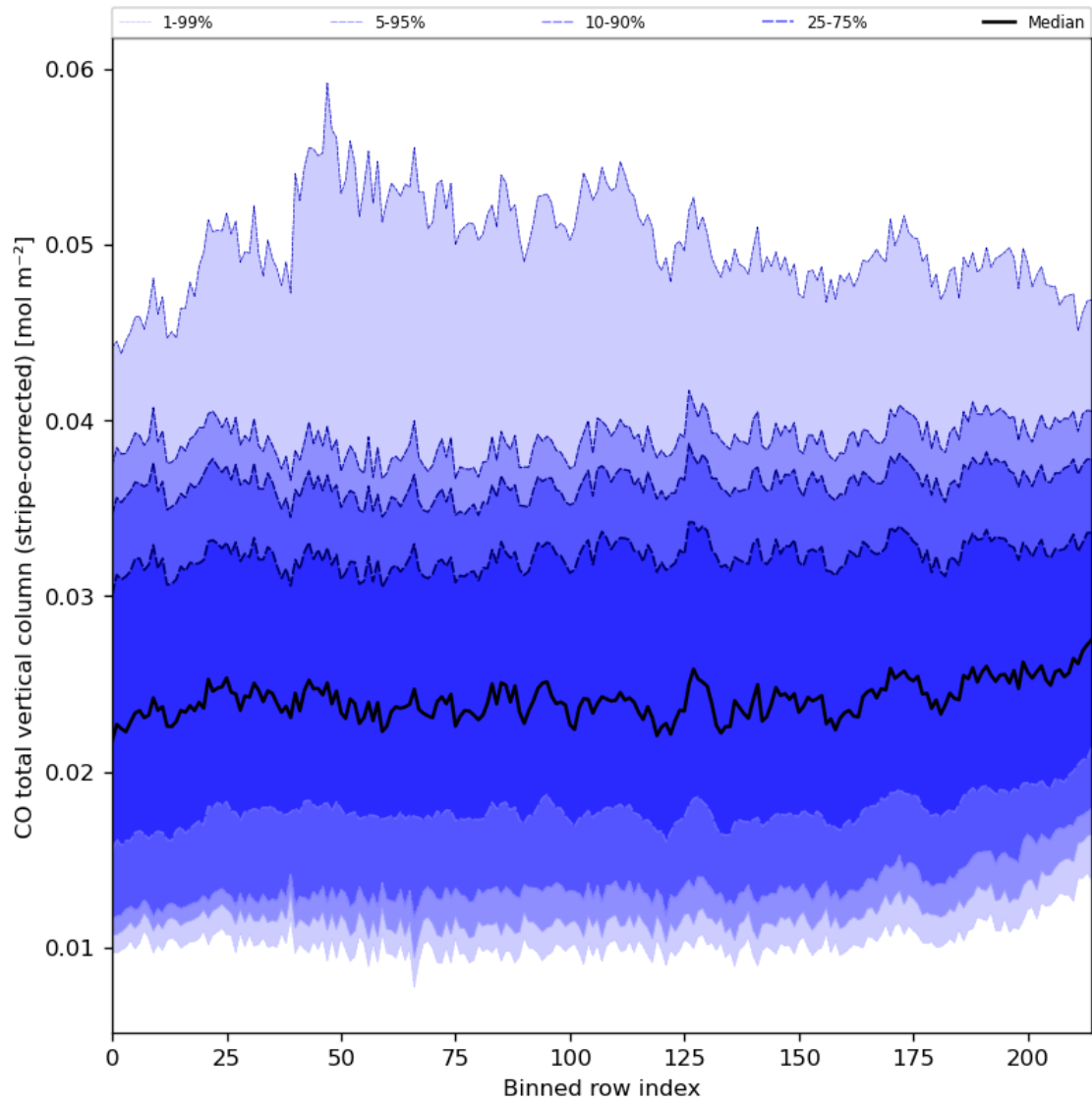
Figure 27: Along track statistics of “CO total vertical column (stripe-corrected)” for 2023-11-13 to 2023-11-14
