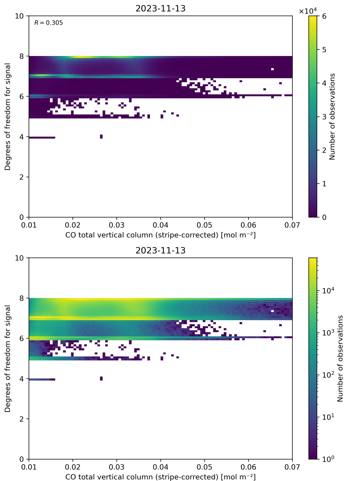
Figure 38: Scatter density plot of “CO total vertical column (stripe-corrected)” against “Degrees of freedom for signal” for 2023-11-13 to 2023-11-14.
