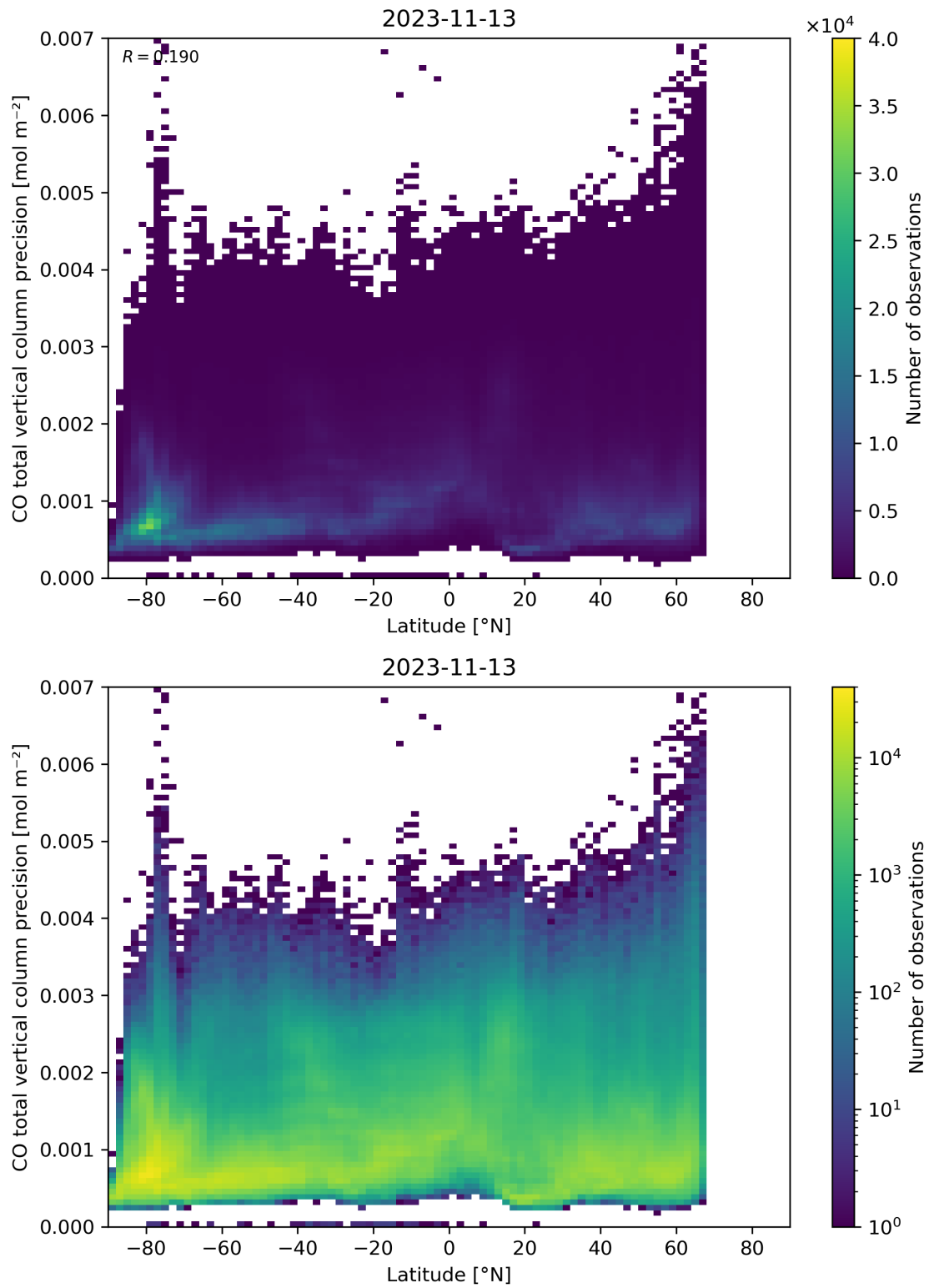
Figure 53: Scatter density plot of “Latitude” against “CO total vertical column precision” for 2023-11-13 to 2023-11-14.
