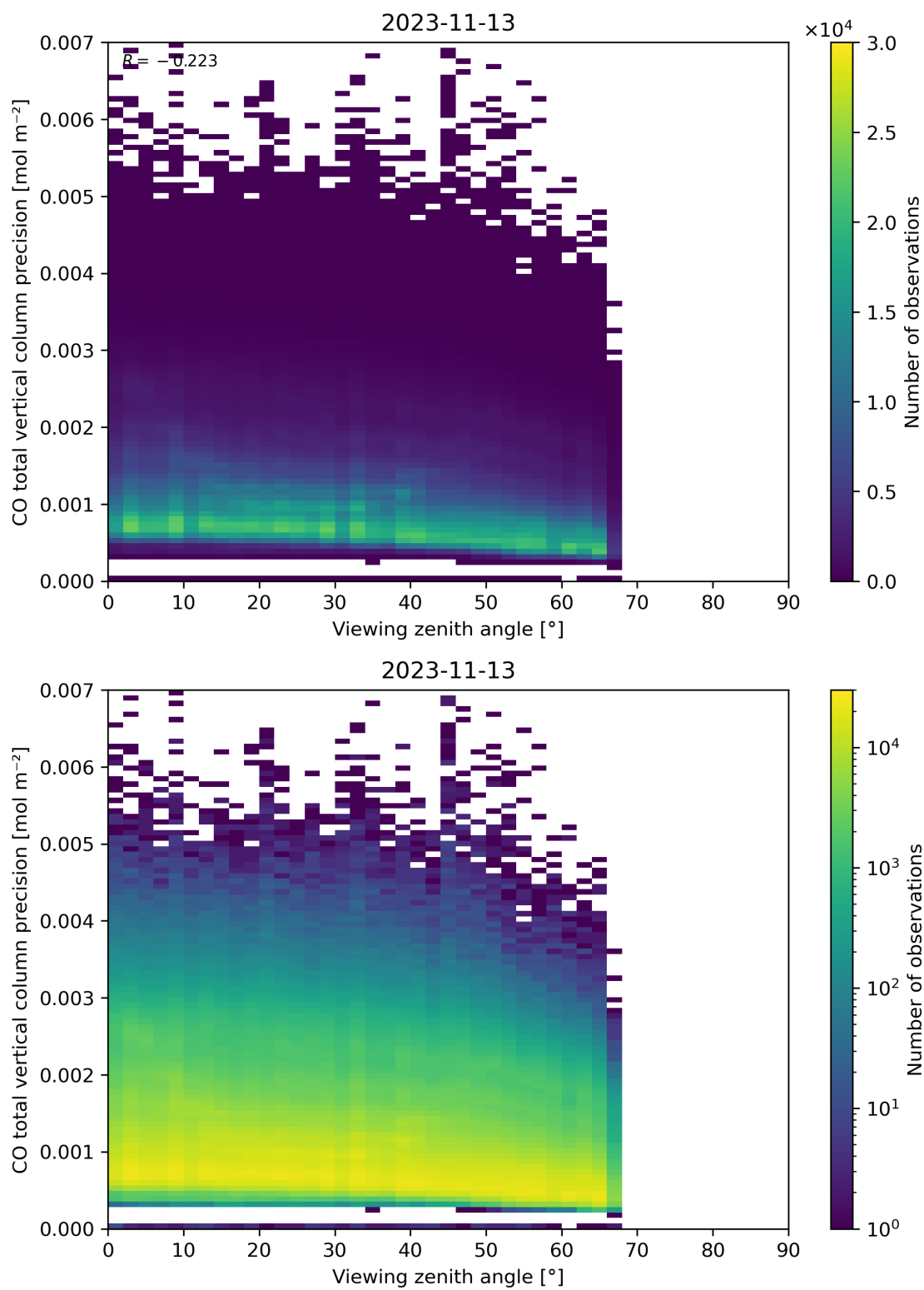
Figure 71: Scatter density plot of “Viewing zenith angle” against “CO total vertical column precision” for 2023-11-13 to 2023-11-14.
