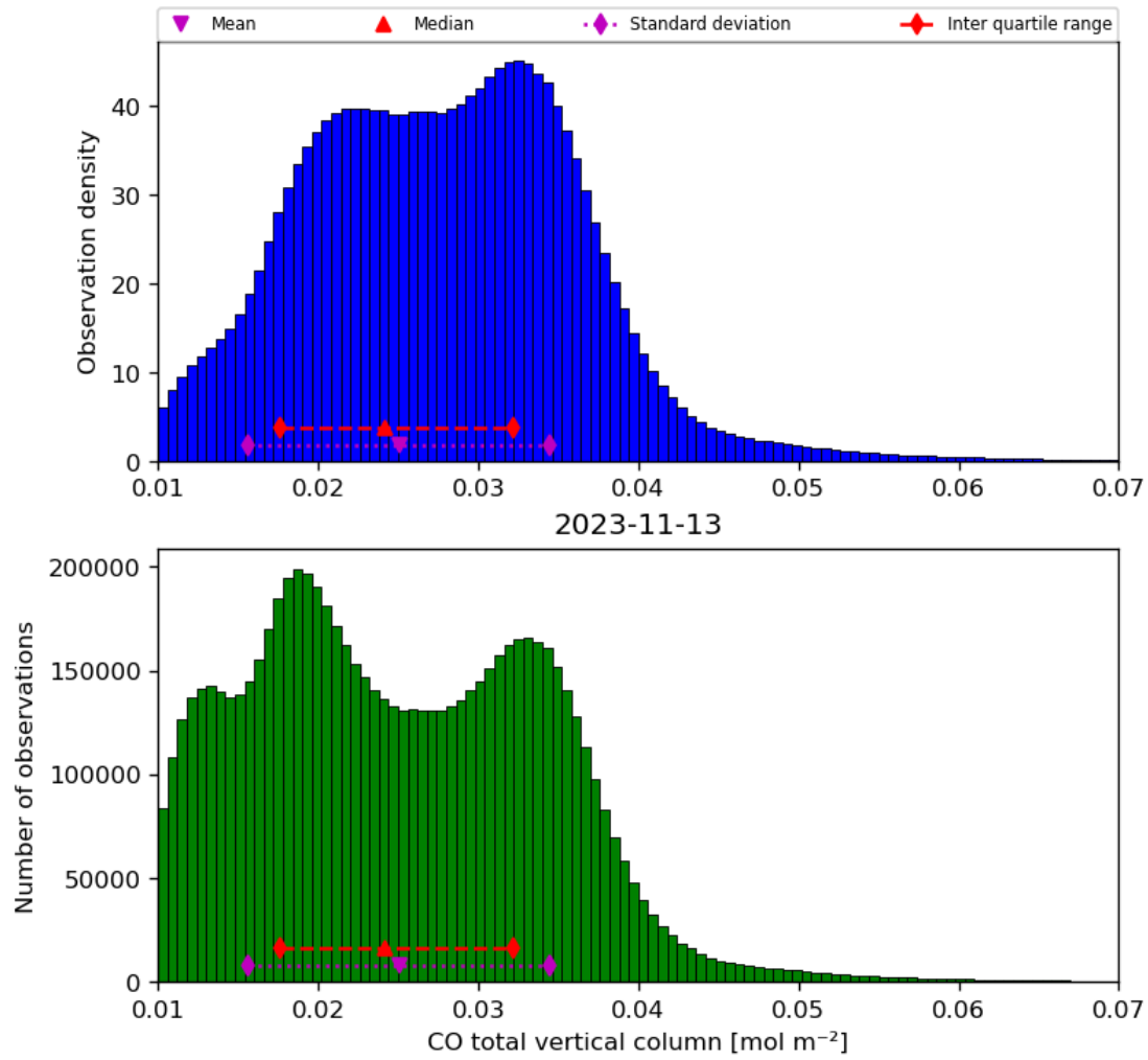
Figure 18: Histogram of “CO total vertical column” for 2023-11-13 to 2023-11-14
