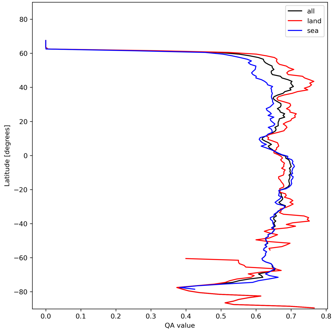
Figure 9: Zonal average of “QA value” for 2023-11-13 to 2023-11-14.
