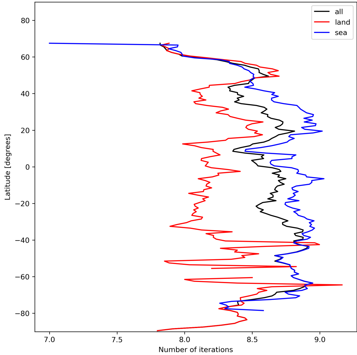
Figure 16: Zonal average of “Number of iterations” for 2023-11-13 to 2023-11-14.
