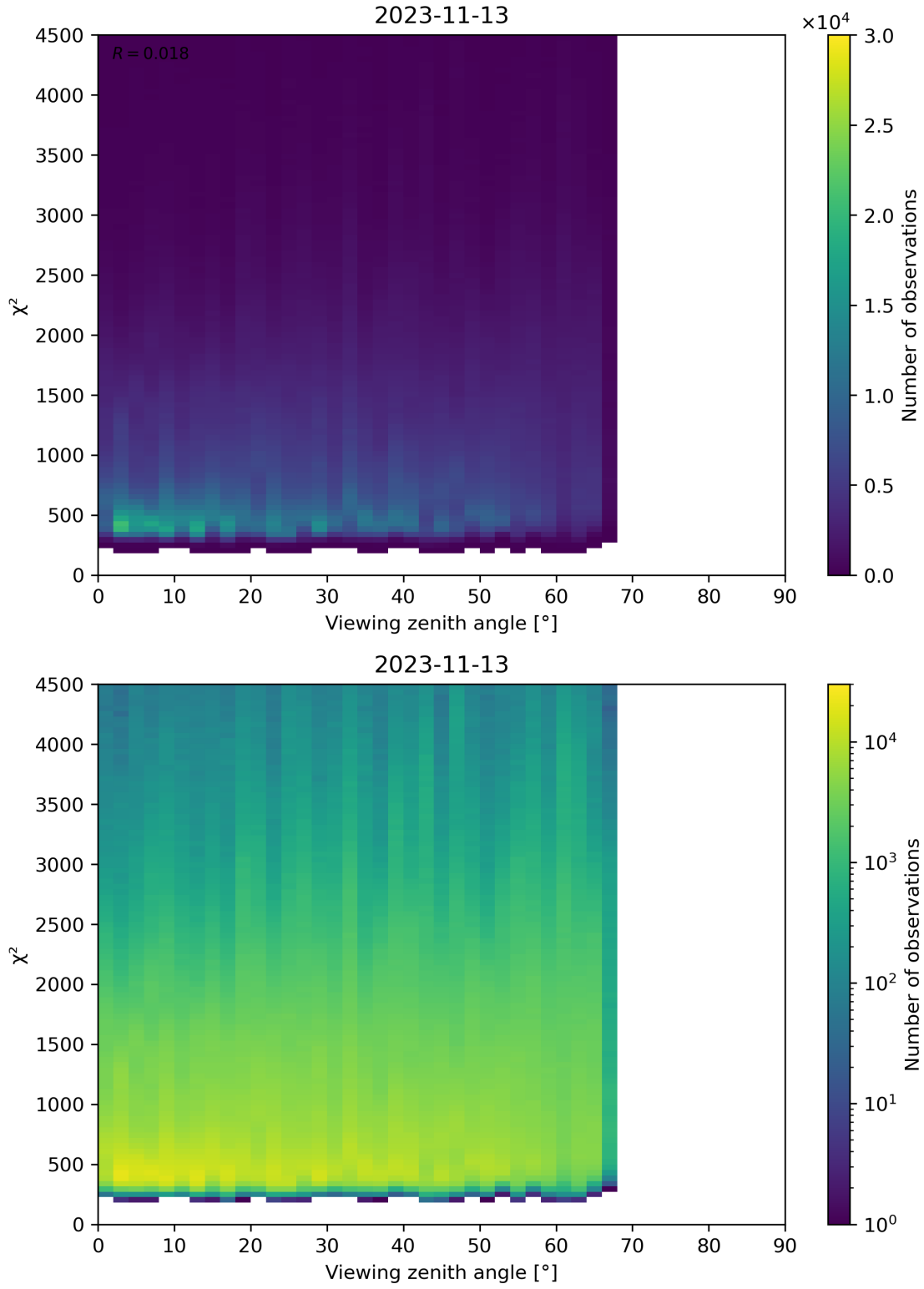
Figure 72: Scatter density plot of “Viewing zenith angle” against “ \chi^2 ” for 2023-11-13 to 2023-11-14.
