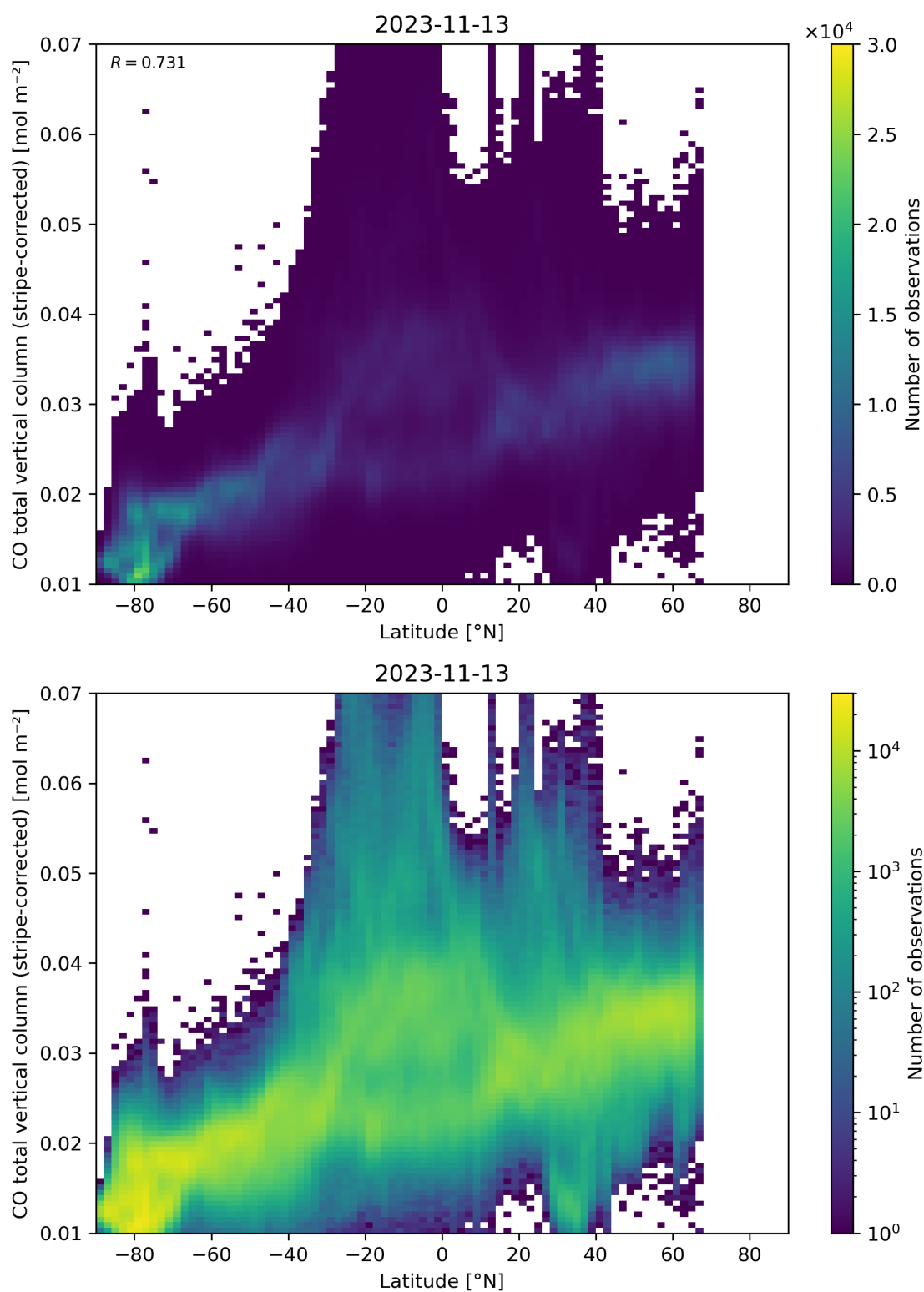
Figure 52: Scatter density plot of “Latitude” against “CO total vertical column (stripe-corrected)” for 2023-11-13 to 2023-11-14.
