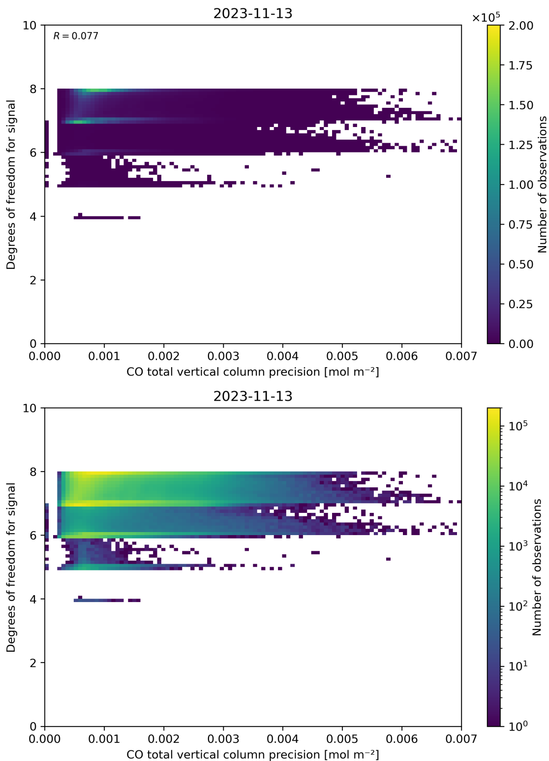
Figure 45: Scatter density plot of “CO total vertical column precision” against “Degrees of freedom for signal” for 2023-11-13 to 2023-11-14.
