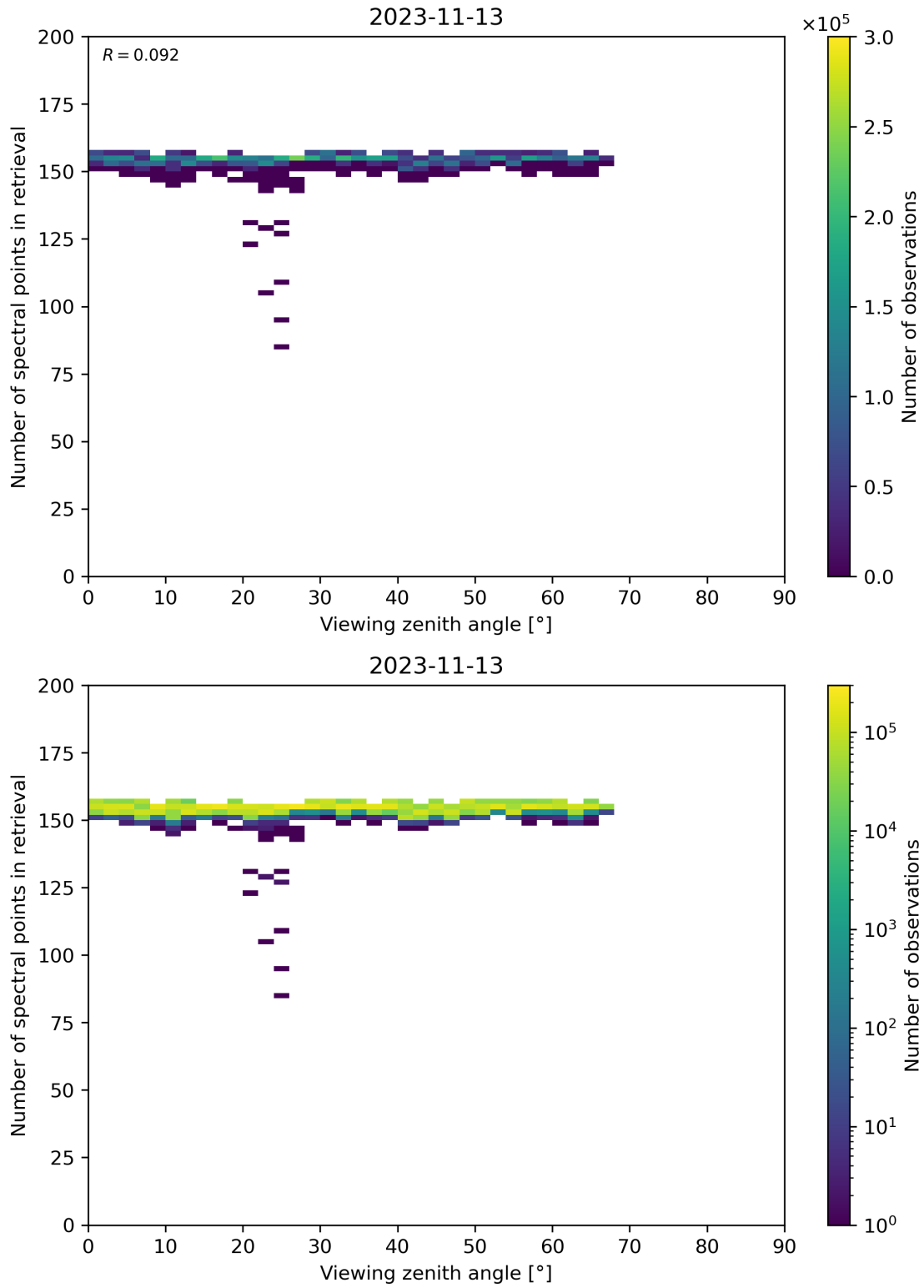
Figure 76: Scatter density plot of “Viewing zenith angle” against “Number of spectral points in retrieval” for 2023-11-13 to 2023-11-14.
