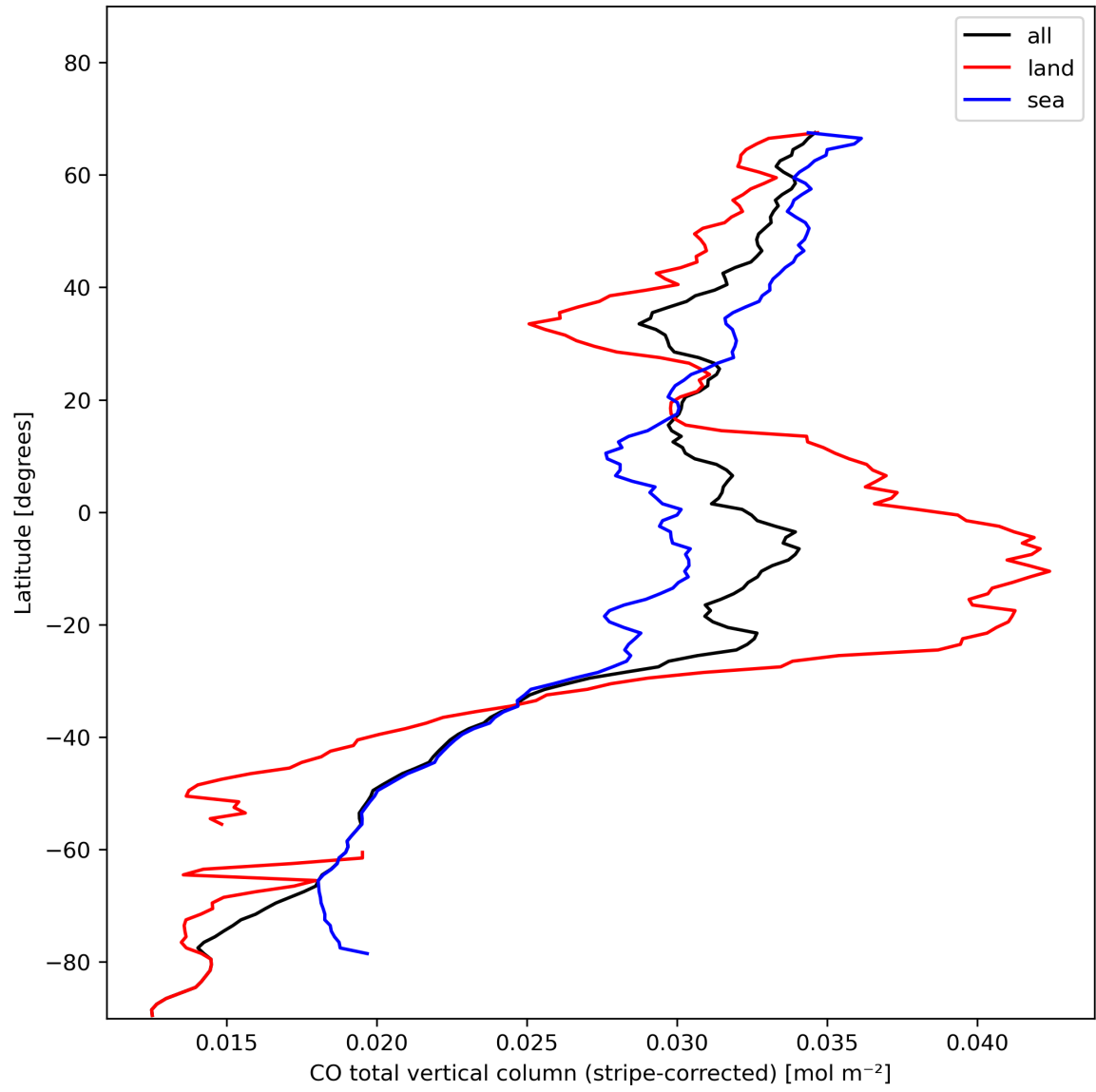
Figure 11: Zonal average of “CO total vertical column (stripe-corrected)” for 2023-11-13 to 2023-11-14.
