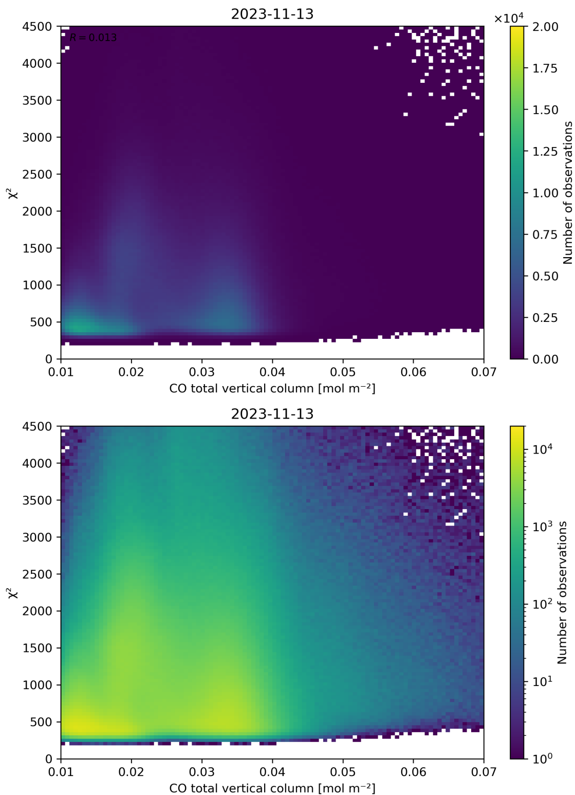
Figure 35: Scatter density plot of “CO total vertical column” against “ \chi^2 ” for 2023-11-13 to 2023-11-14.
