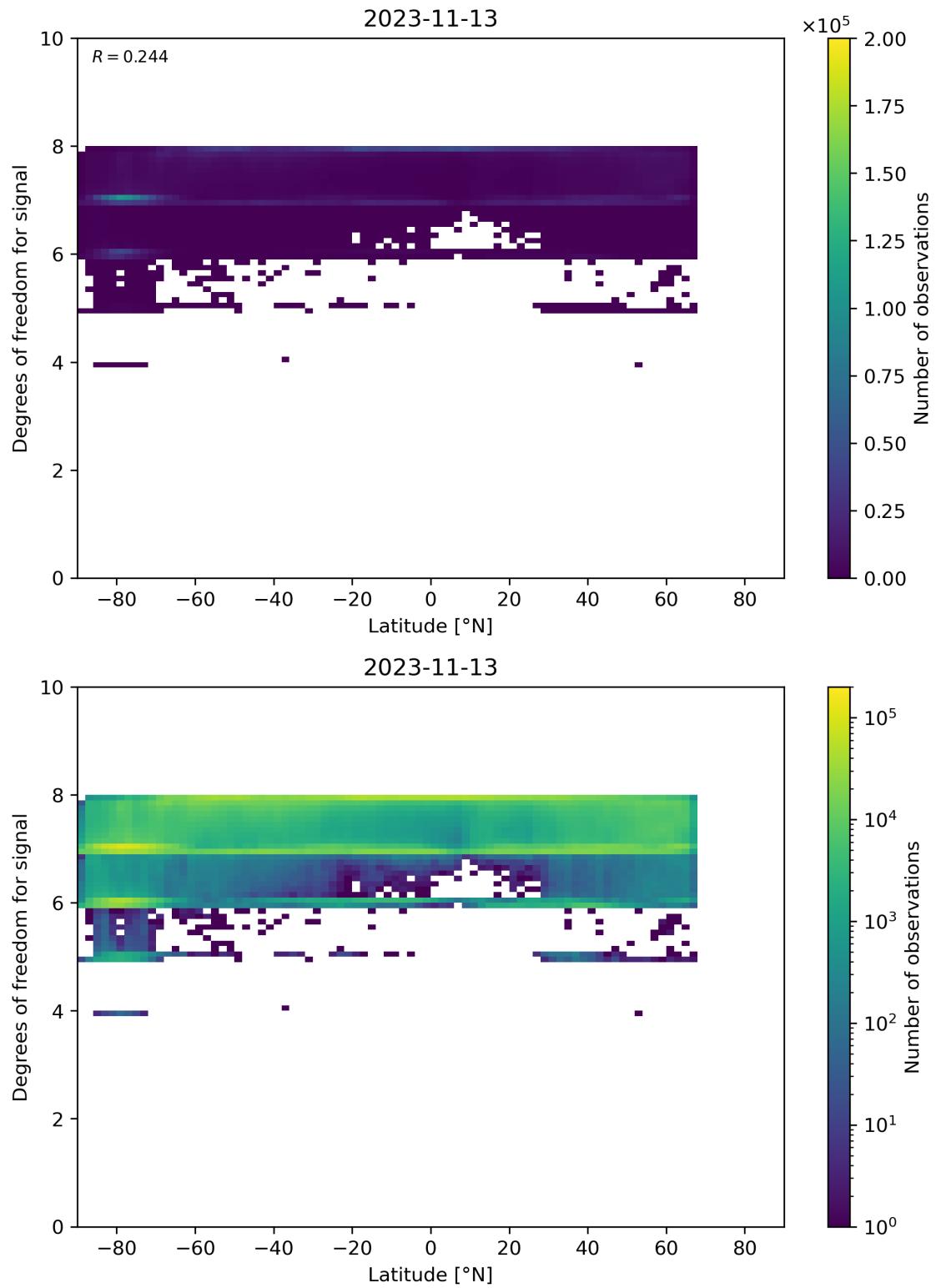
Figure 55: Scatter density plot of “Latitude” against “Degrees of freedom for signal” for 2023-11-13 to 2023-11-14.
