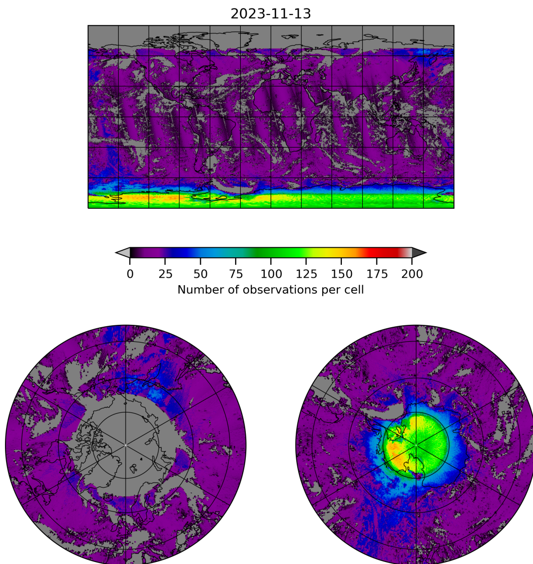
Figure 8: Map of the number of observations for 2023-11-13 to 2023-11-14
