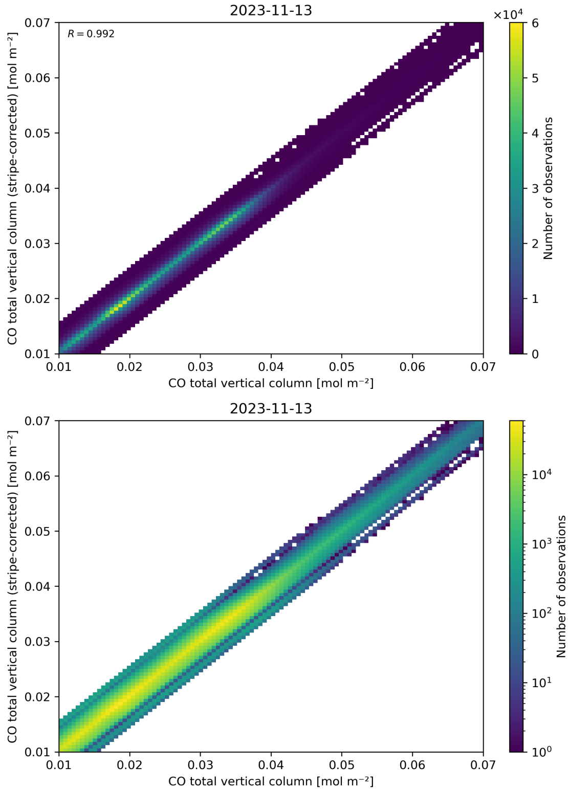
Figure 33: Scatter density plot of “CO total vertical column” against “CO total vertical column (stripe-corrected)” for 2023-11-13 to 2023-11-14.
