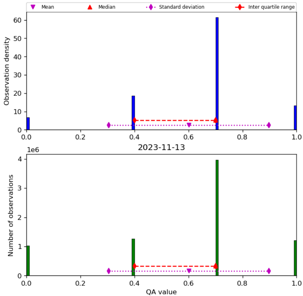
Figure 17: Histogram of “QA value” for 2023-11-13 to 2023-11-14
