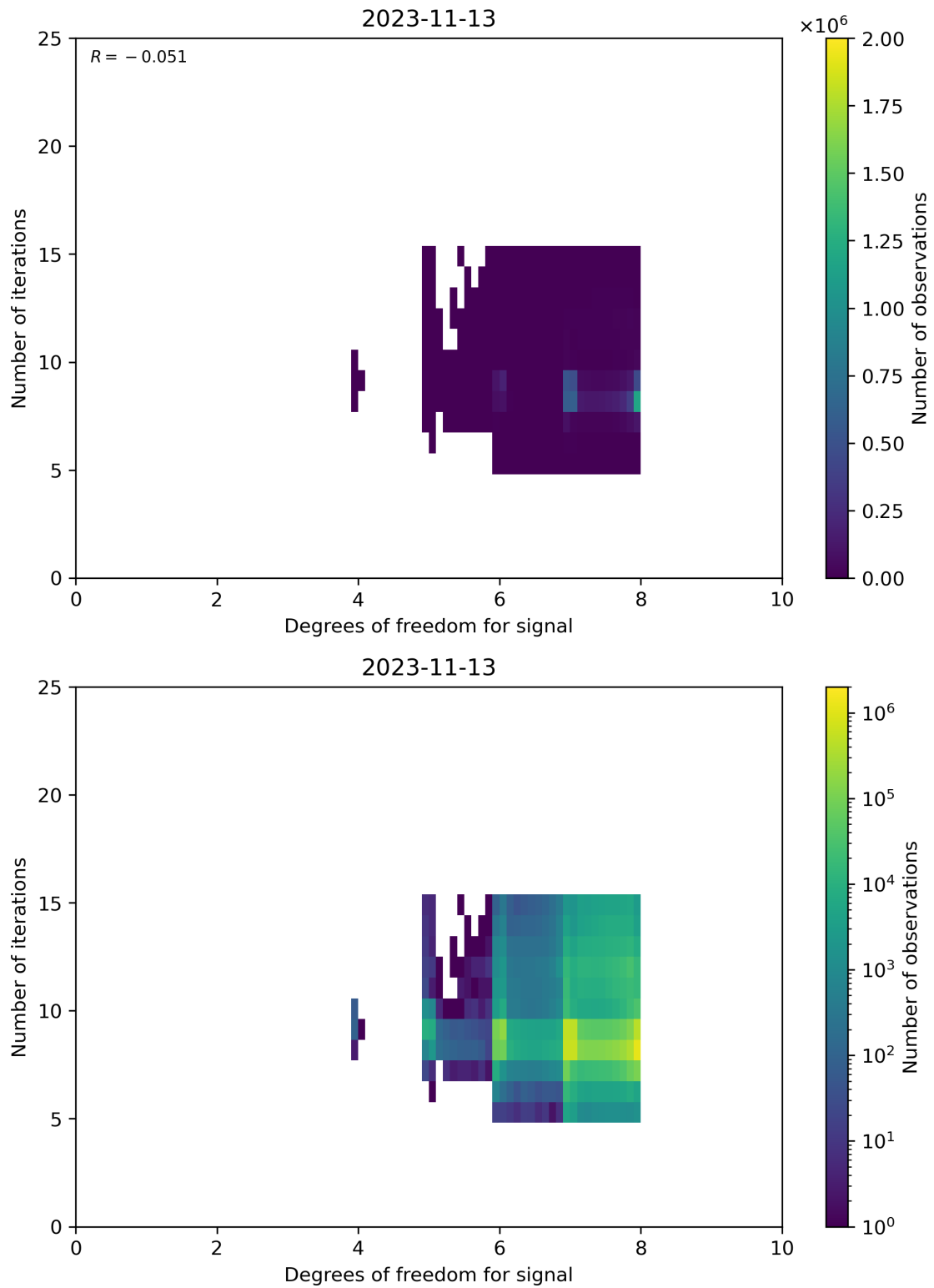
Figure 50: Scatter density plot of “Degrees of freedom for signal” against “Number of iterations” for 2023-11-13 to 2023-11-14.
