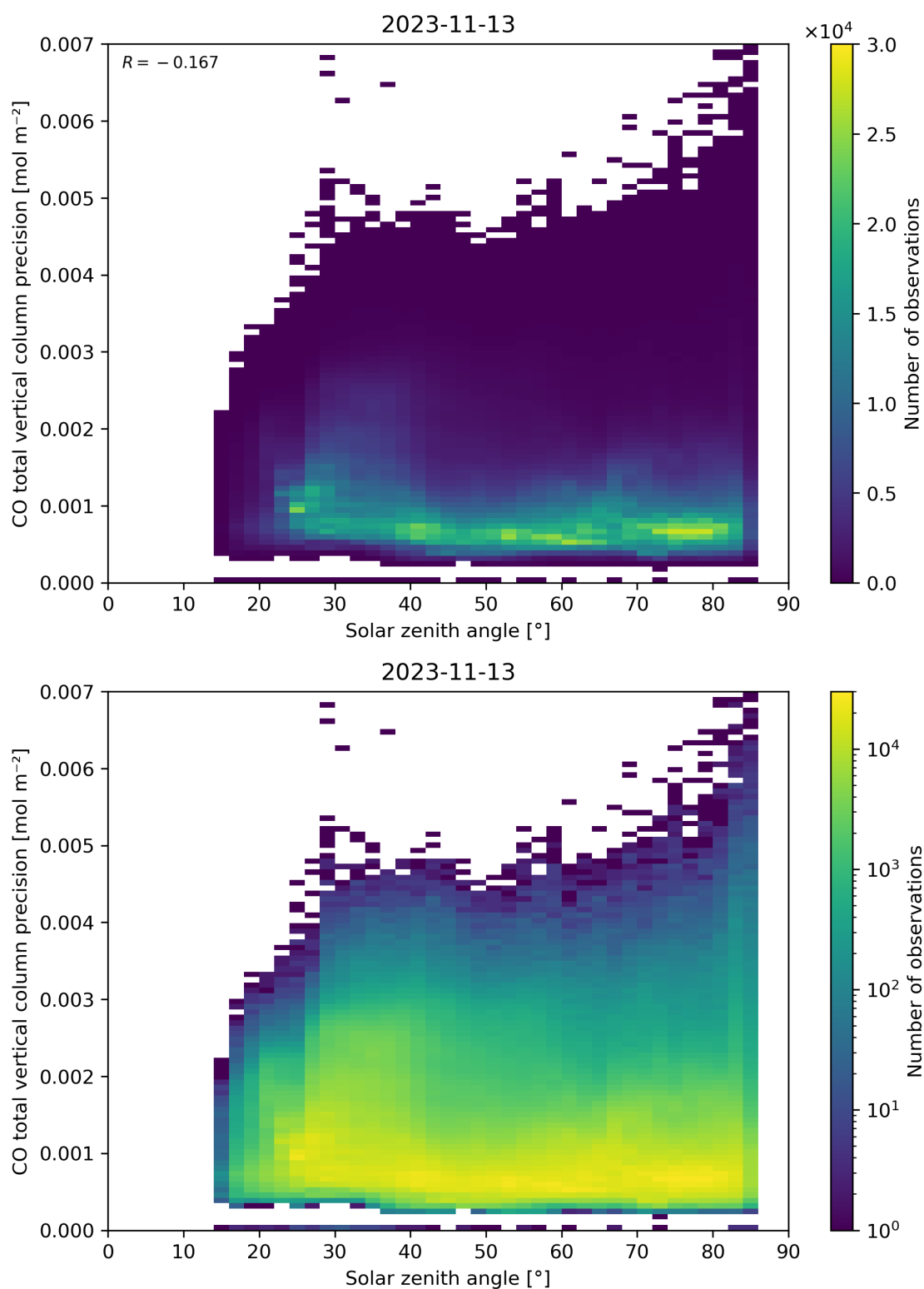
Figure 63: Scatter density plot of “Solar zenith angle” against “CO total vertical column precision” for 2023-11-13 to 2023-11-14.
