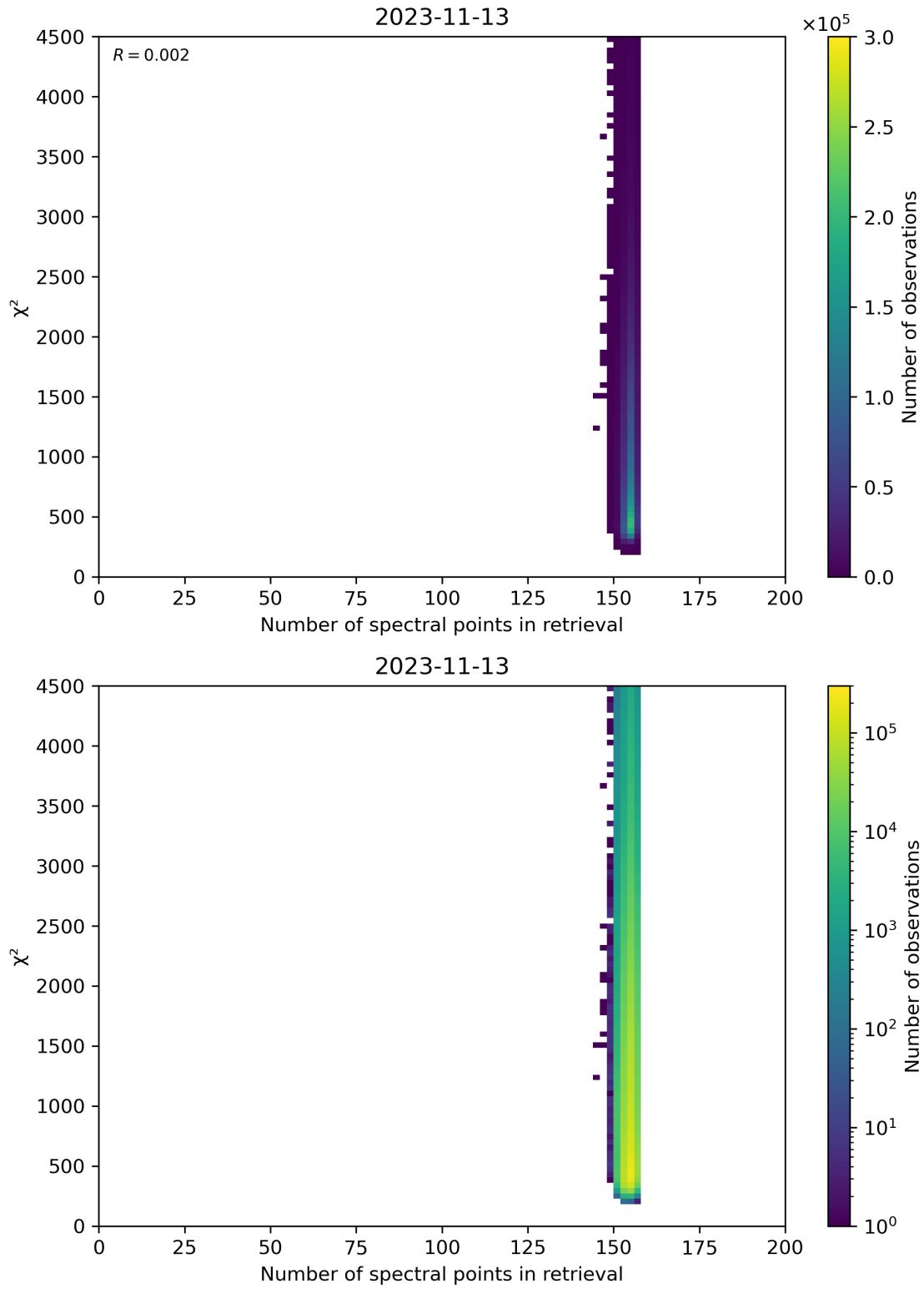
Figure 58: Scatter density plot of “Number of spectral points in retrieval” against “ \chi^2 ” for 2023-11-13 to 2023-11-14.
