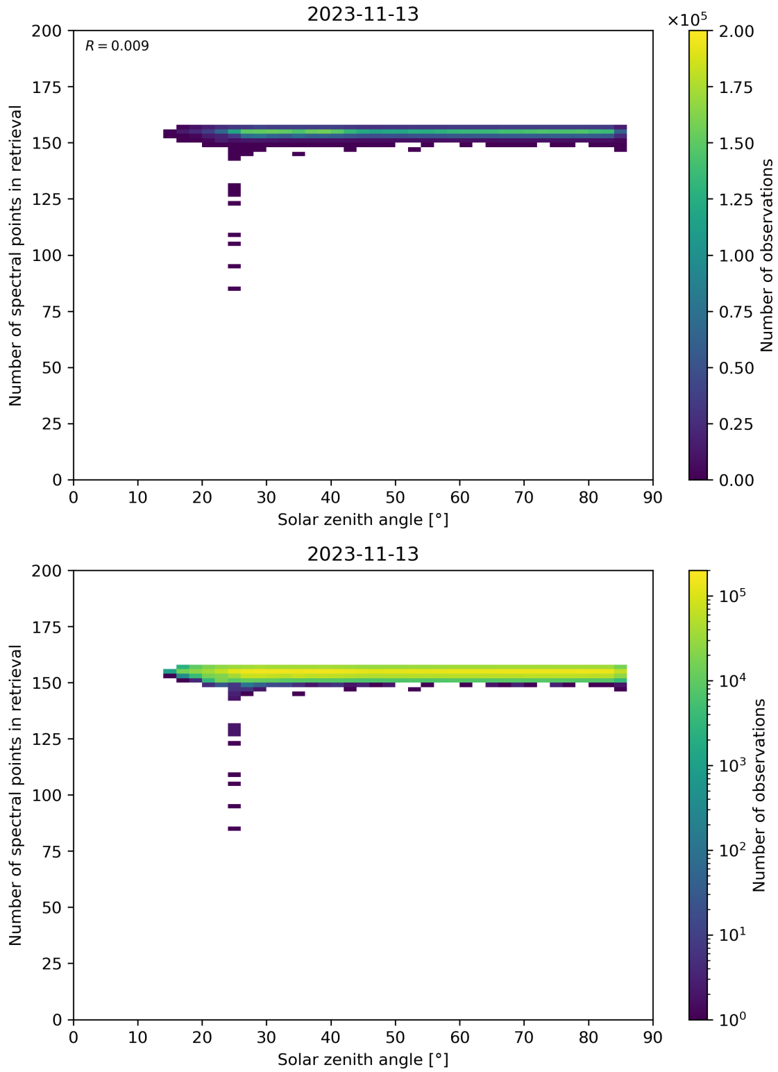
Figure 68: Scatter density plot of “Solar zenith angle” against “Number of spectral points in retrieval” for 2023-11-13 to 2023-11-14.
