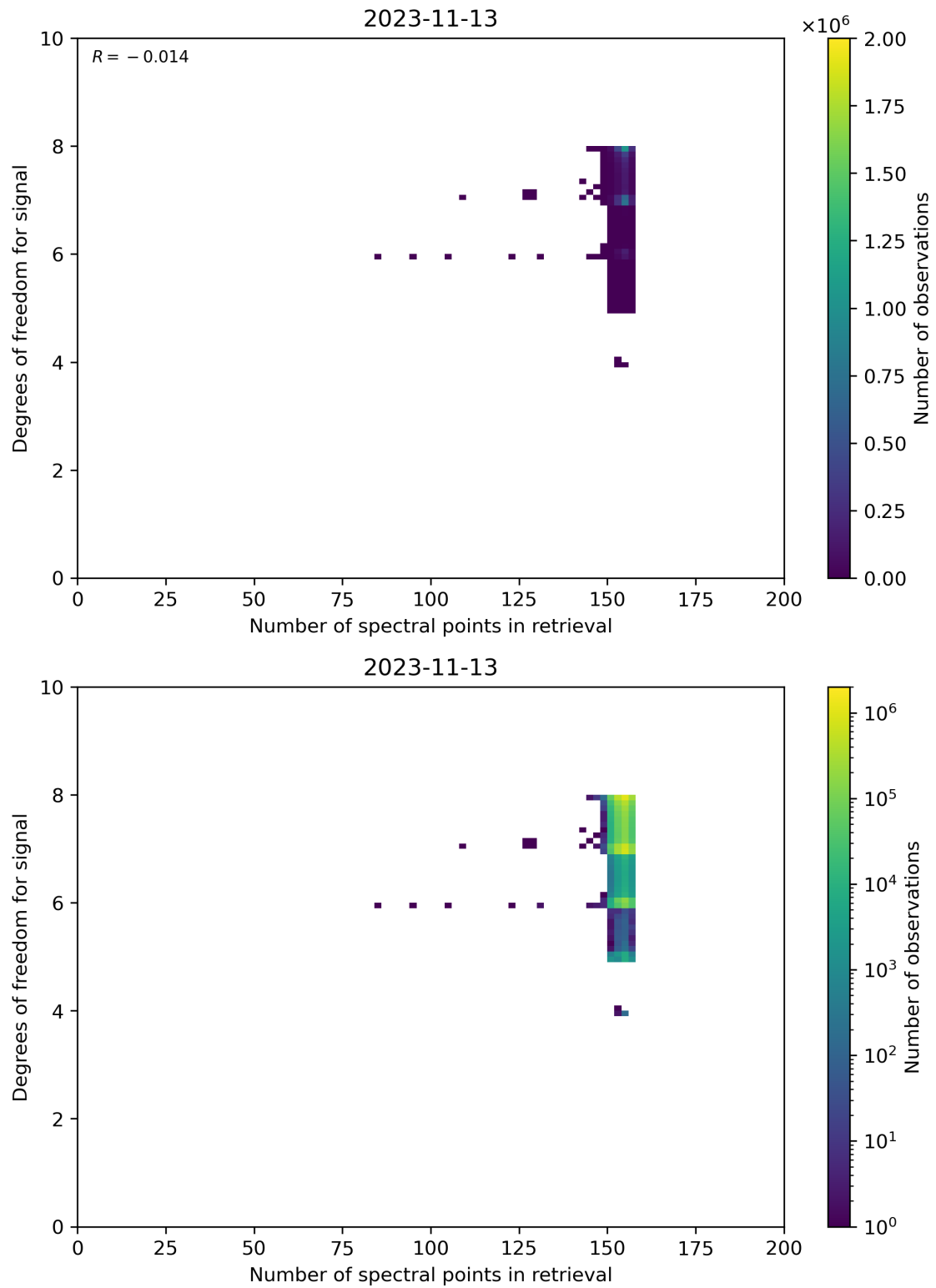
Figure 59: Scatter density plot of “Number of spectral points in retrieval” against “Degrees of freedom for signal” for 2023-11-13 to 2023-11-14.
