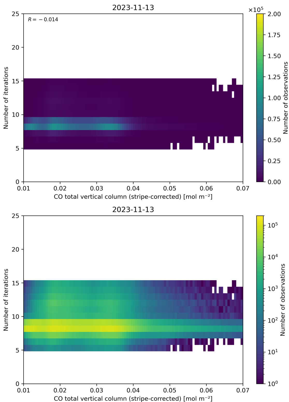
Figure 39: Scatter density plot of “CO total vertical column (stripe-corrected)” against “Number of iterations” for 2023-11-13 to 2023-11-14.
