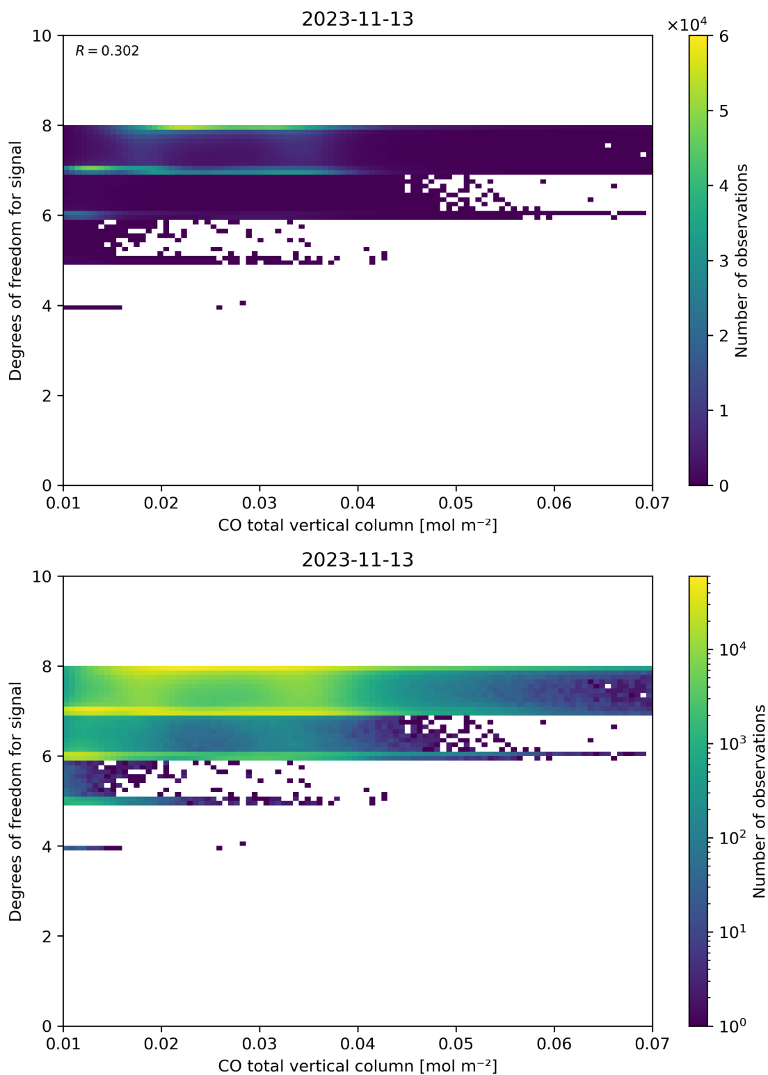
Figure 41: Scatter density plot of “CO total vertical column” against “Degrees of freedom for signal” for 2023-11-13 to 2023-11-14.
