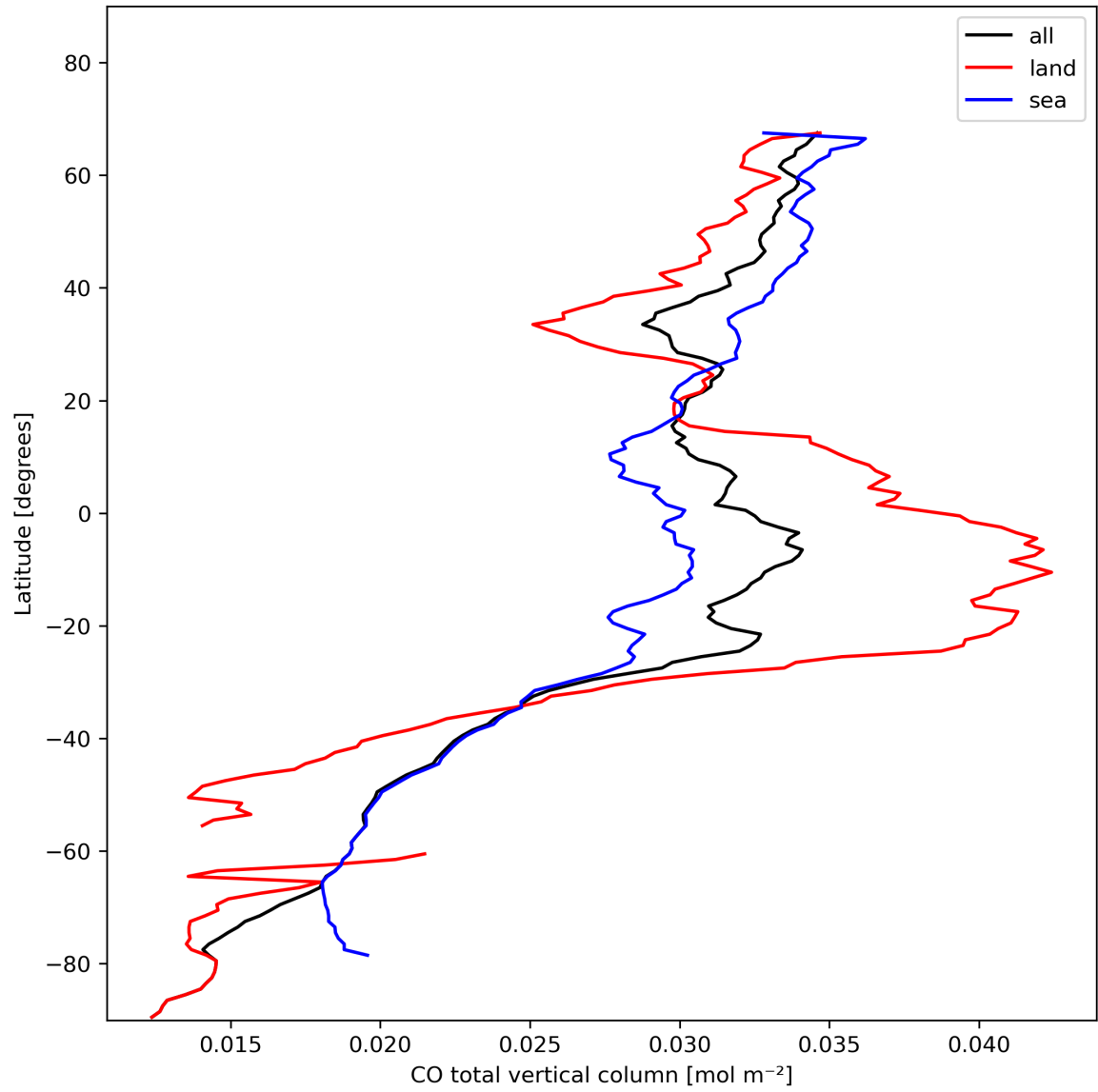
Figure 10: Zonal average of “CO total vertical column” for 2023-11-13 to 2023-11-14.
