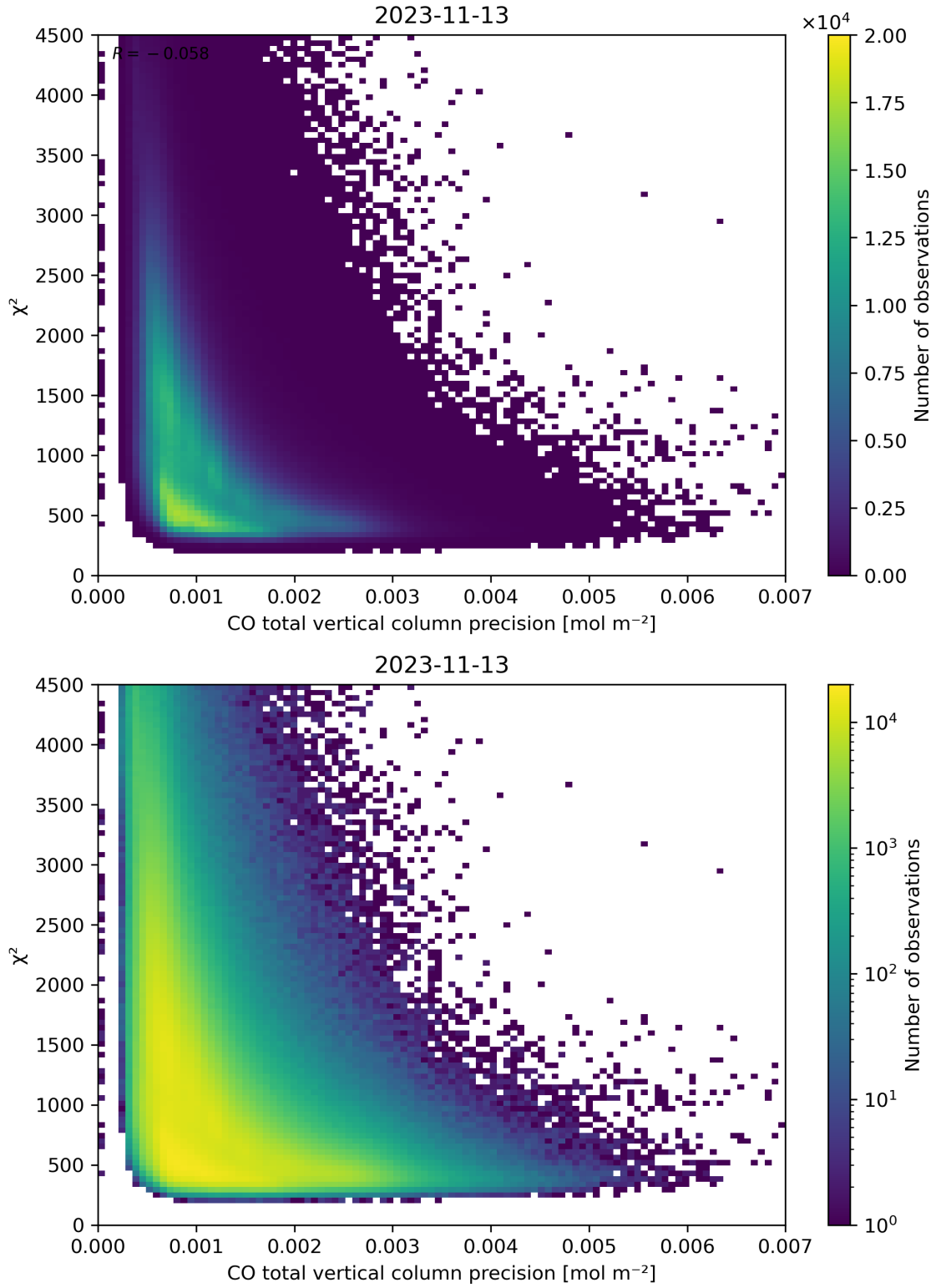
Figure 44: Scatter density plot of “CO total vertical column precision” against “ \chi^2 ” for 2023-11-13 to 2023-11-14.
