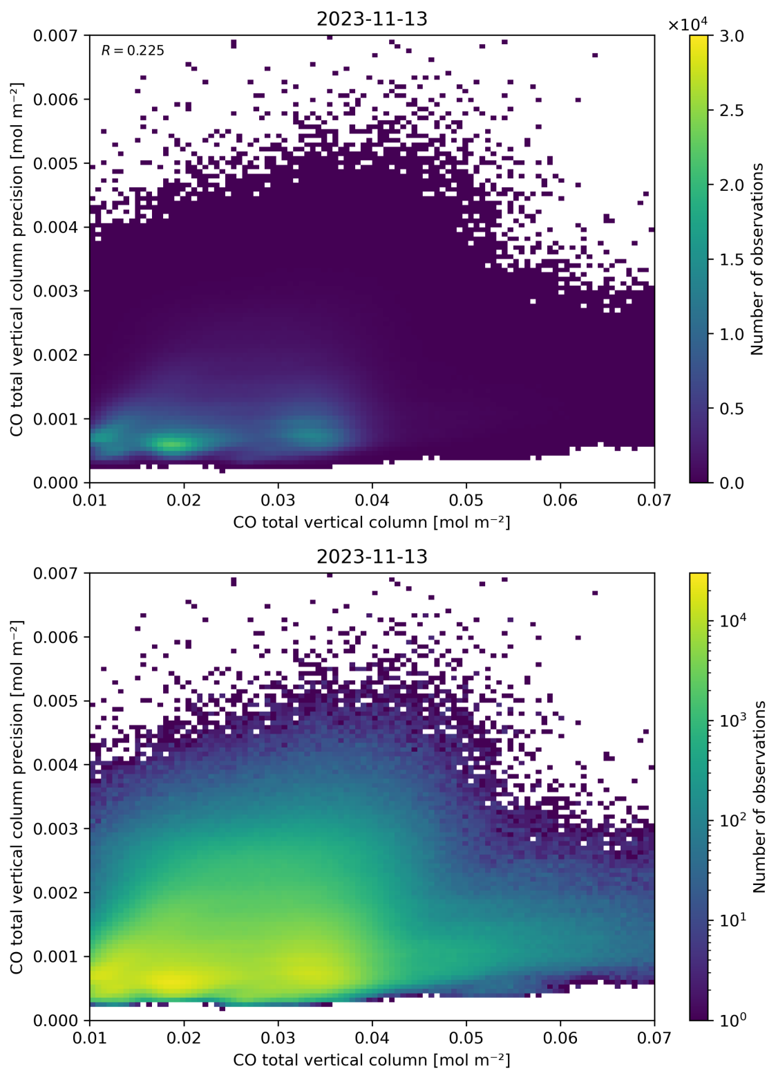
Figure 34: Scatter density plot of “CO total vertical column” against “CO total vertical column precision” for 2023-11-13 to 2023-11-14.
