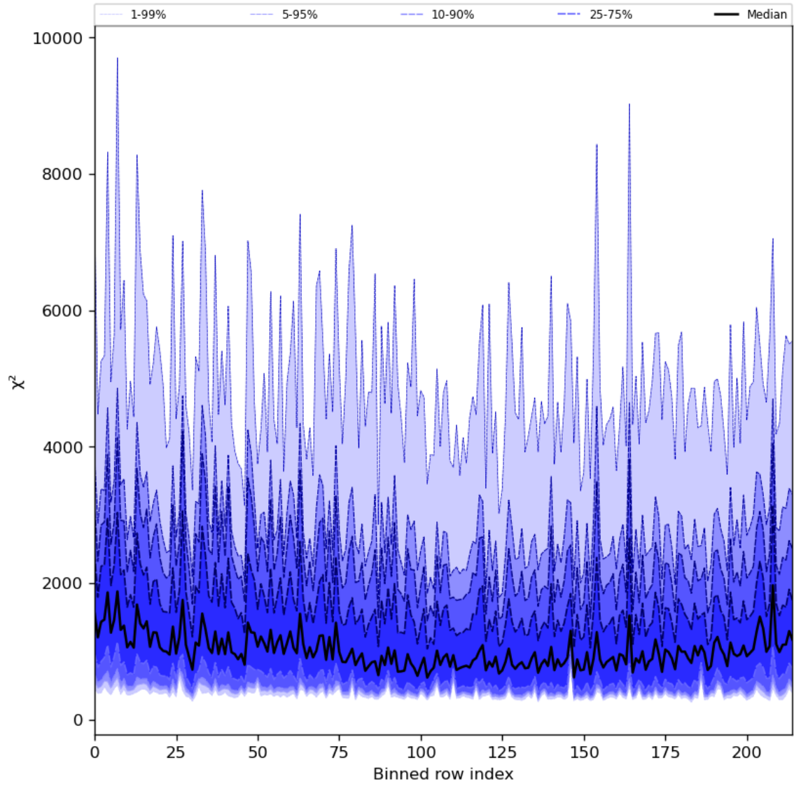
Figure 30: Along track statistics of “ \chi^2 ” for 2023-11-13 to 2023-11-14
