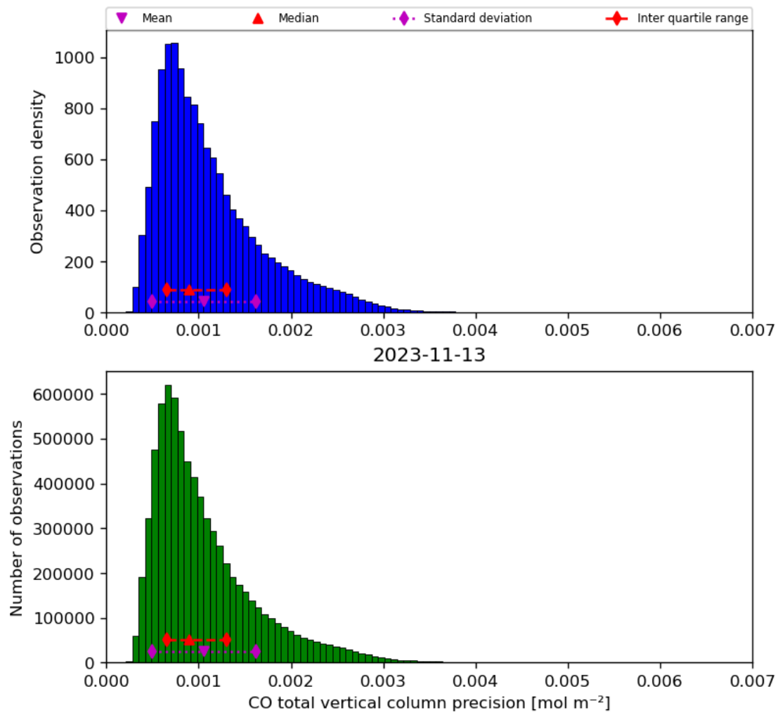
Figure 20: Histogram of “CO total vertical column precision” for 2023-11-13 to 2023-11-14
