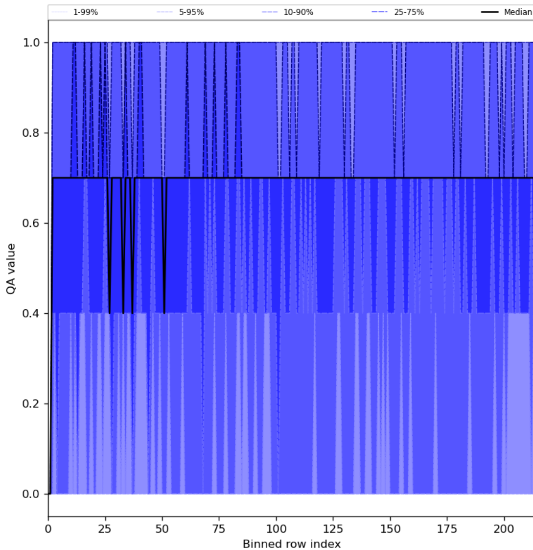
Figure 25: Along track statistics of “QA value” for 2023-11-13 to 2023-11-14
