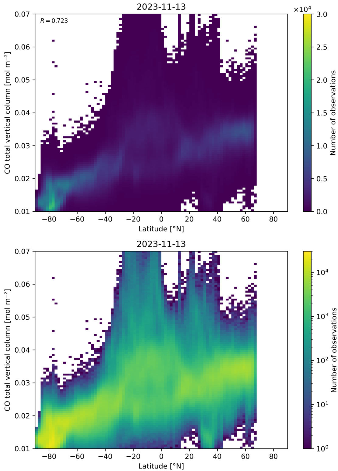
Figure 51: Scatter density plot of “Latitude” against “CO total vertical column” for 2023-11-13 to 2023-11-14.
