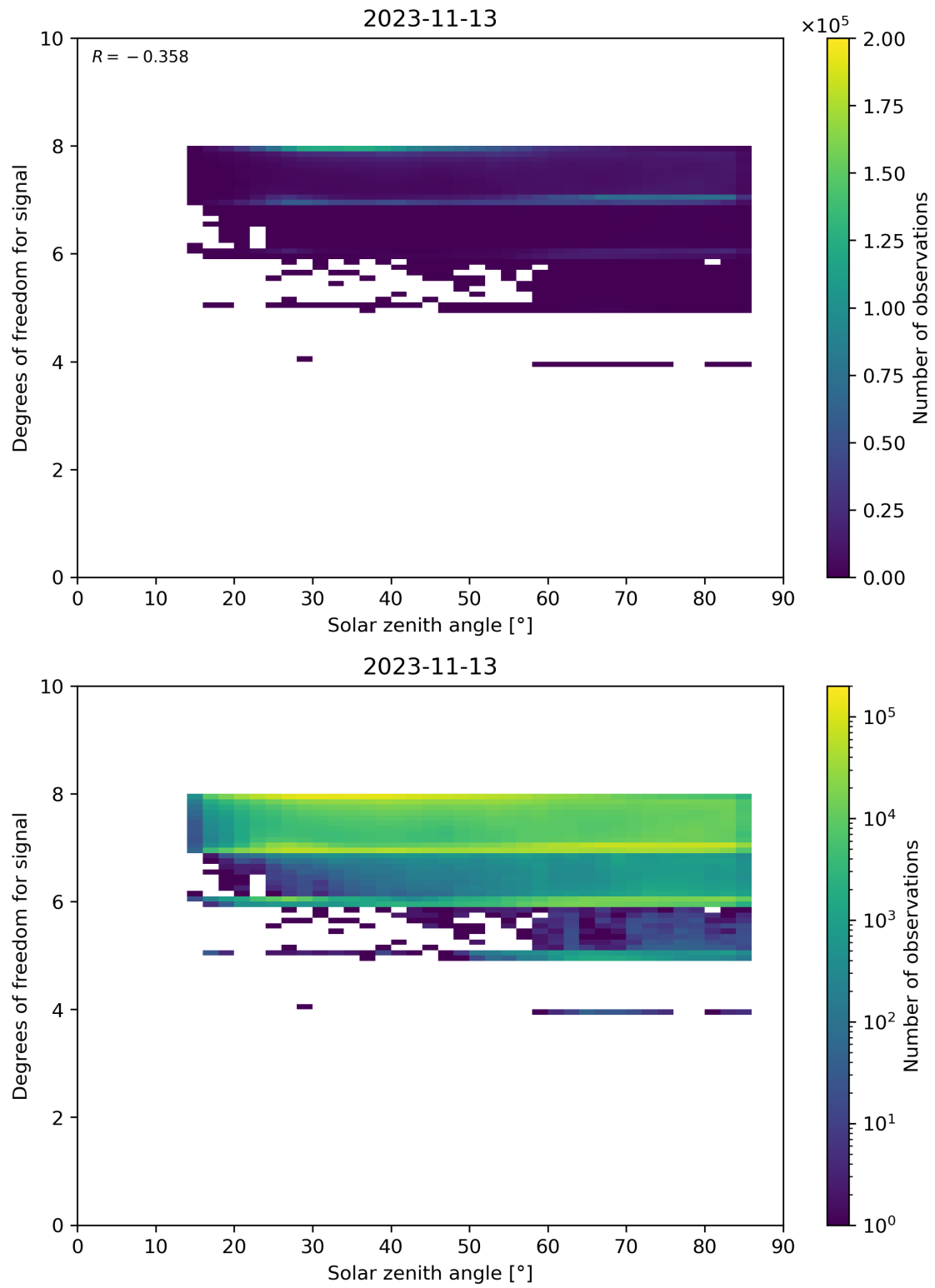
Figure 65: Scatter density plot of “Solar zenith angle” against “Degrees of freedom for signal” for 2023-11-13 to 2023-11-14.
