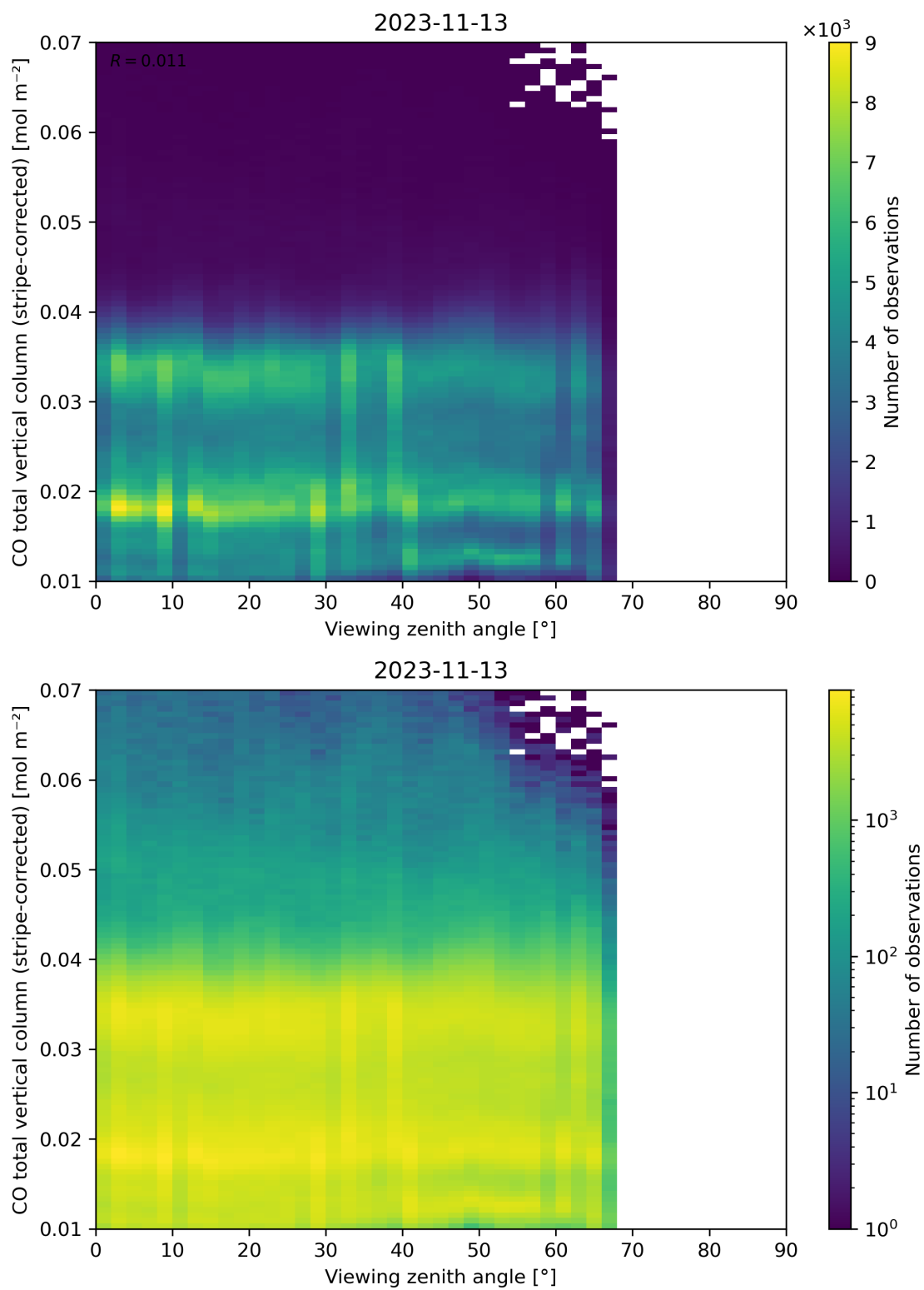
Figure 70: Scatter density plot of “Viewing zenith angle” against “CO total vertical column (stripe-corrected)” for 2023-11-13 to 2023-11-14.
