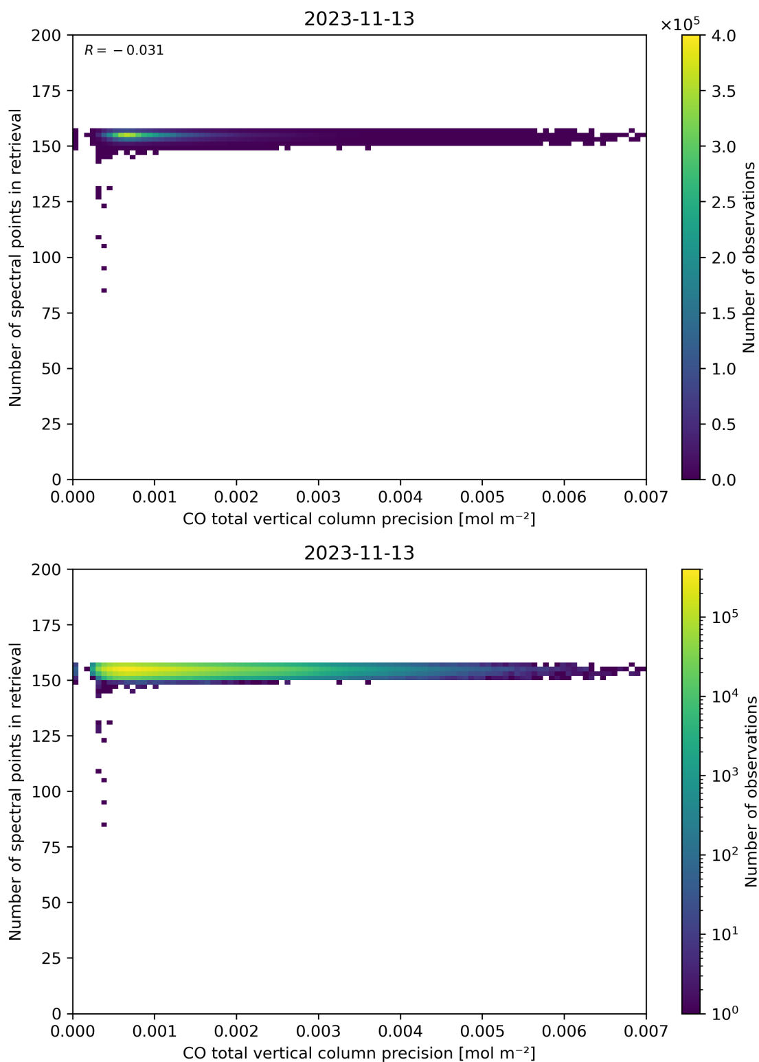
Figure 47: Scatter density plot of “CO total vertical column precision” against “Number of spectral points in retrieval” for 2023-11-13 to 2023-11-14.
