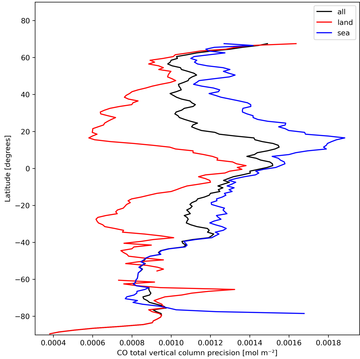
Figure 12: Zonal average of “CO total vertical column precision” for 2023-11-13 to 2023-11-14.
