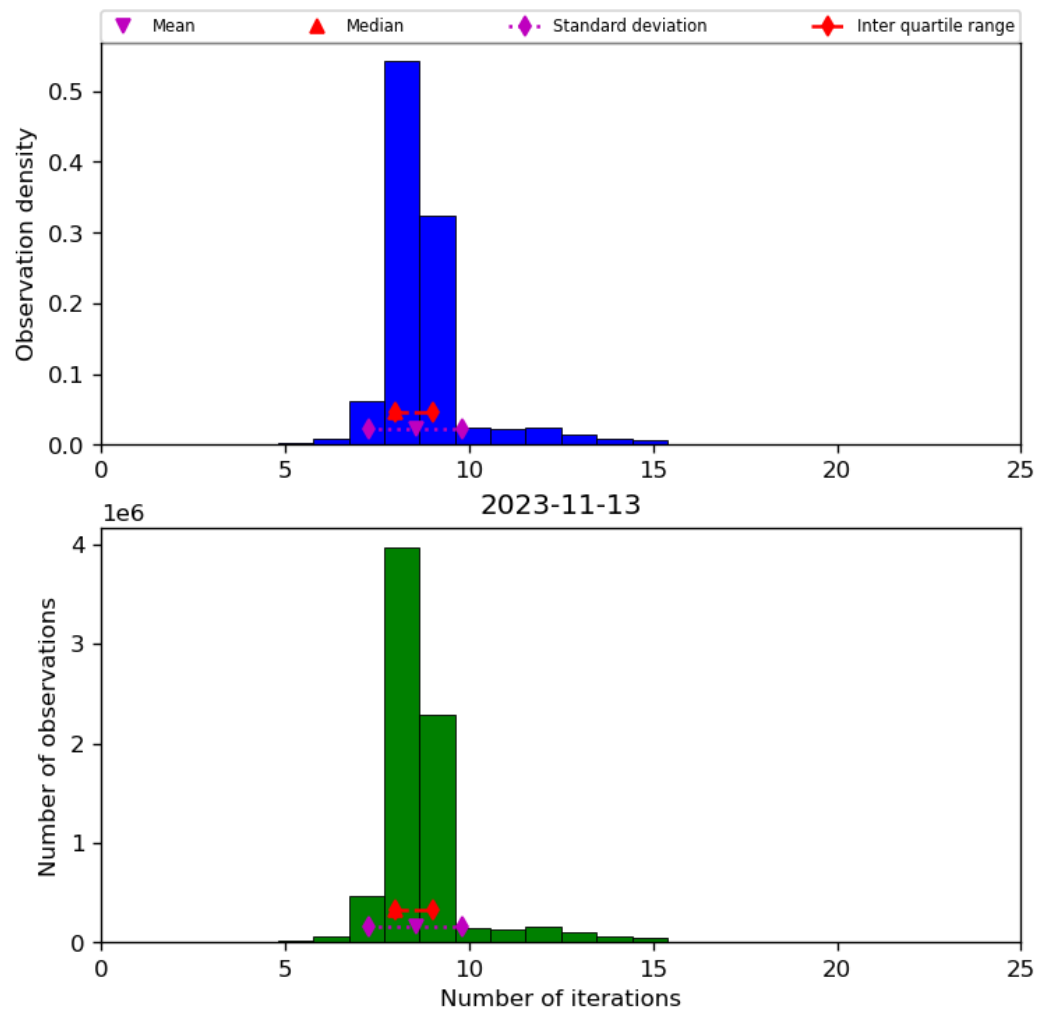
Figure 24: Histogram of “Number of iterations” for 2023-11-13 to 2023-11-14
