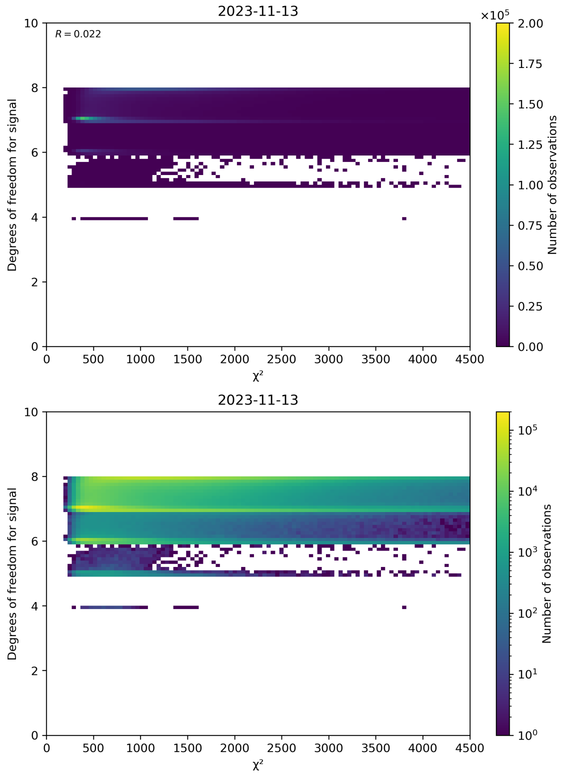
Figure 48: Scatter density plot of “ \chi^2 ” against “Degrees of freedom for signal” for 2023-11-13 to 2023-11-14.
