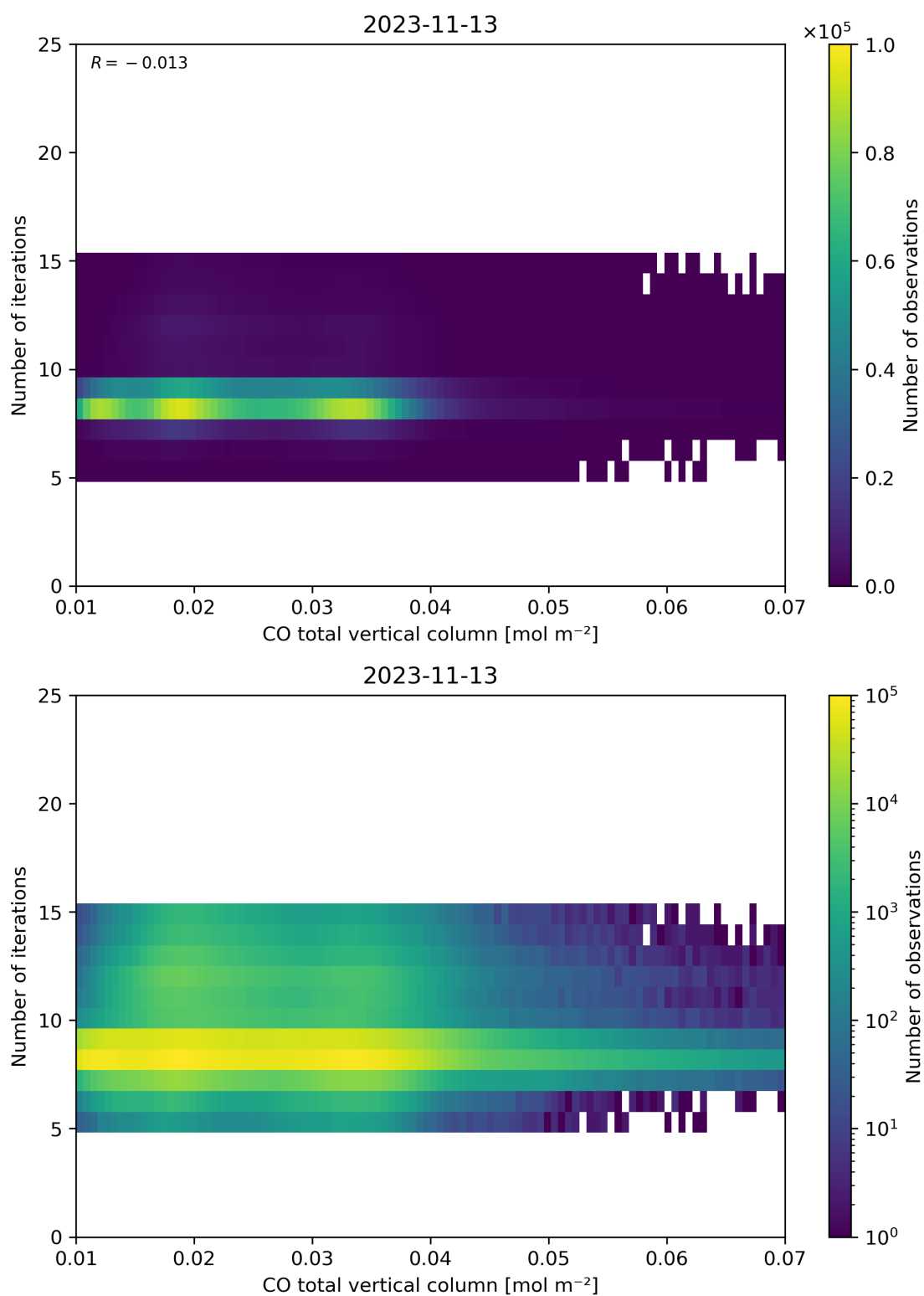
Figure 42: Scatter density plot of “CO total vertical column” against “Number of iterations” for 2023-11-13 to 2023-11-14.
