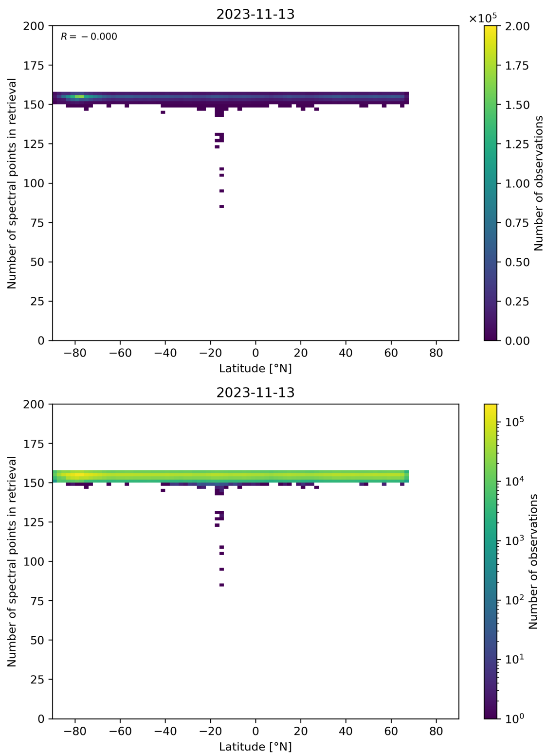
Figure 57: Scatter density plot of “Latitude” against “Number of spectral points in retrieval” for 2023-11-13 to 2023-11-14.
