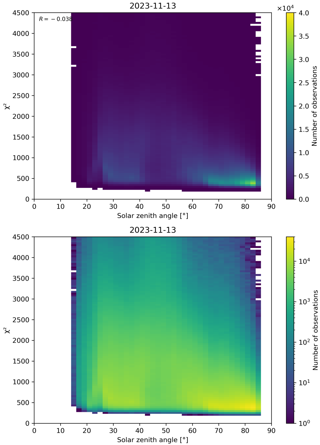
Figure 64: Scatter density plot of “Solar zenith angle” against “ \chi^2 ” for 2023-11-13 to 2023-11-14.
