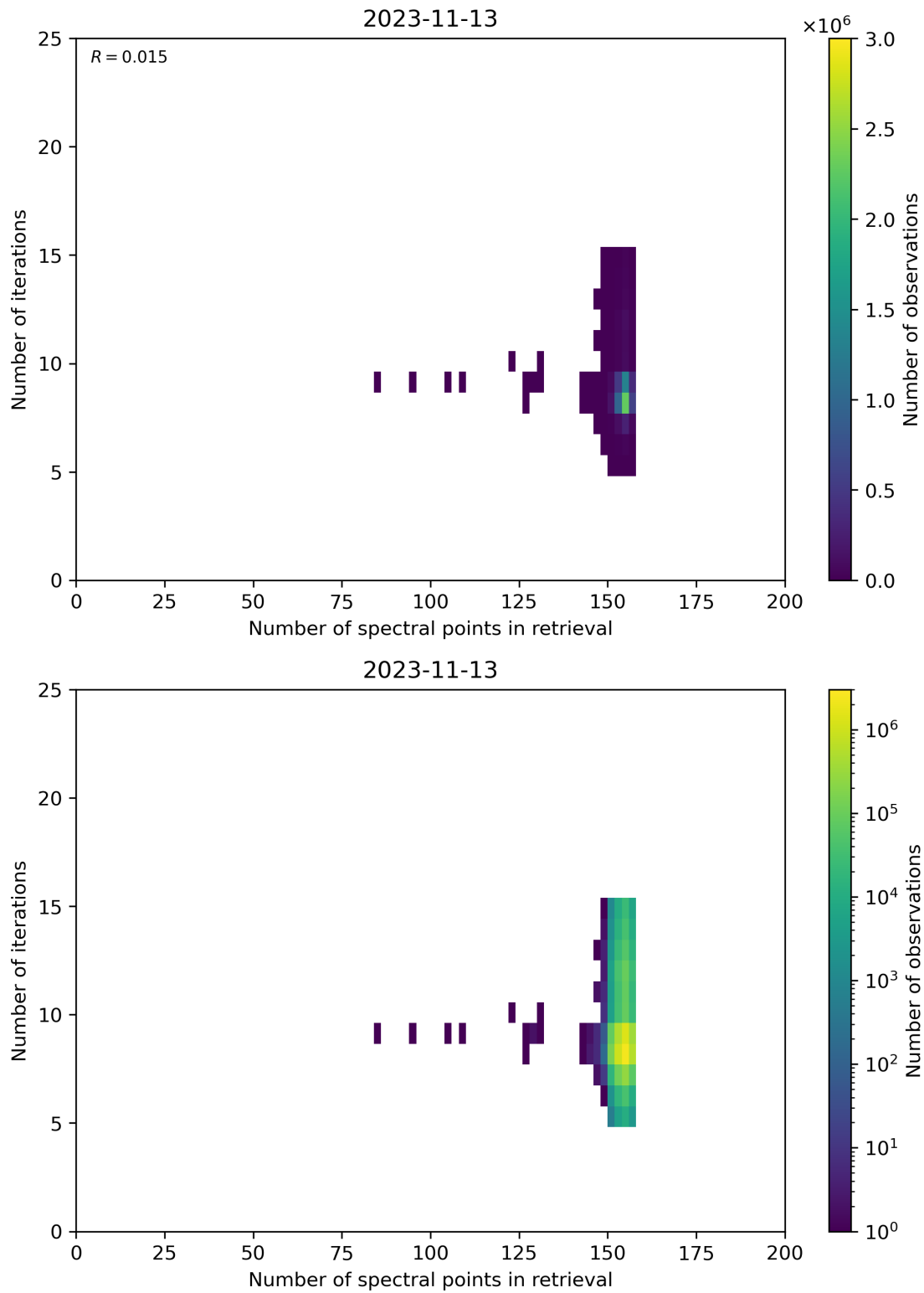
Figure 60: Scatter density plot of “Number of spectral points in retrieval” against “Number of iterations” for 2023-11-13 to 2023-11-14.
