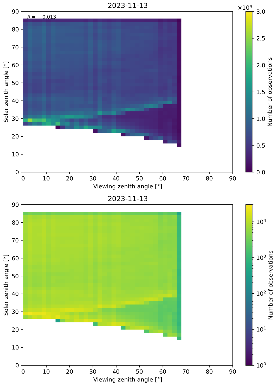
Figure 77: Scatter density plot of “Viewing zenith angle” against “Solar zenith angle” for 2023-11-13 to 2023-11-14.
