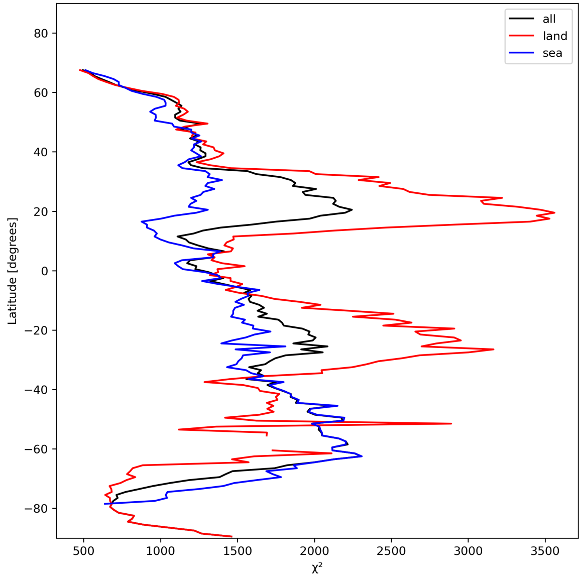
Figure 14: Zonal average of “ \chi^2 ” for 2023-11-13 to 2023-11-14.
