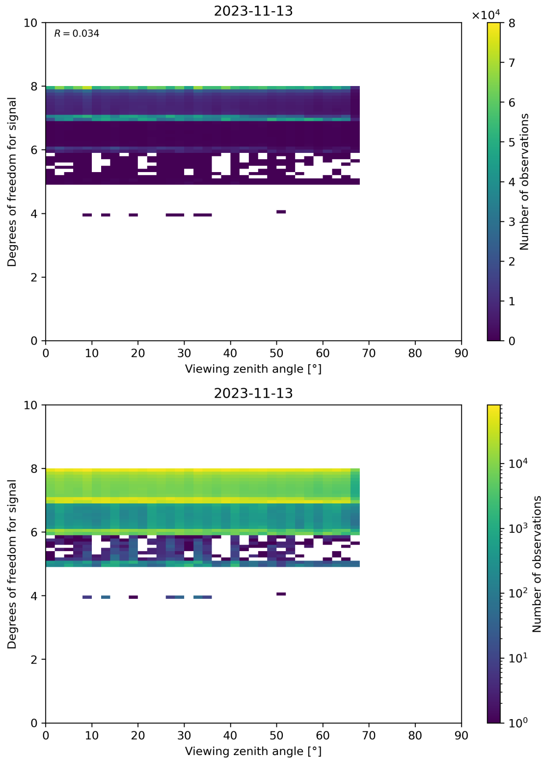
Figure 73: Scatter density plot of “Viewing zenith angle” against “Degrees of freedom for signal” for 2023-11-13 to 2023-11-14.
