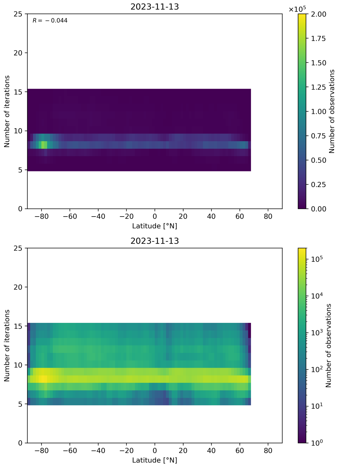
Figure 56: Scatter density plot of “Latitude” against “Number of iterations” for 2023-11-13 to 2023-11-14.
