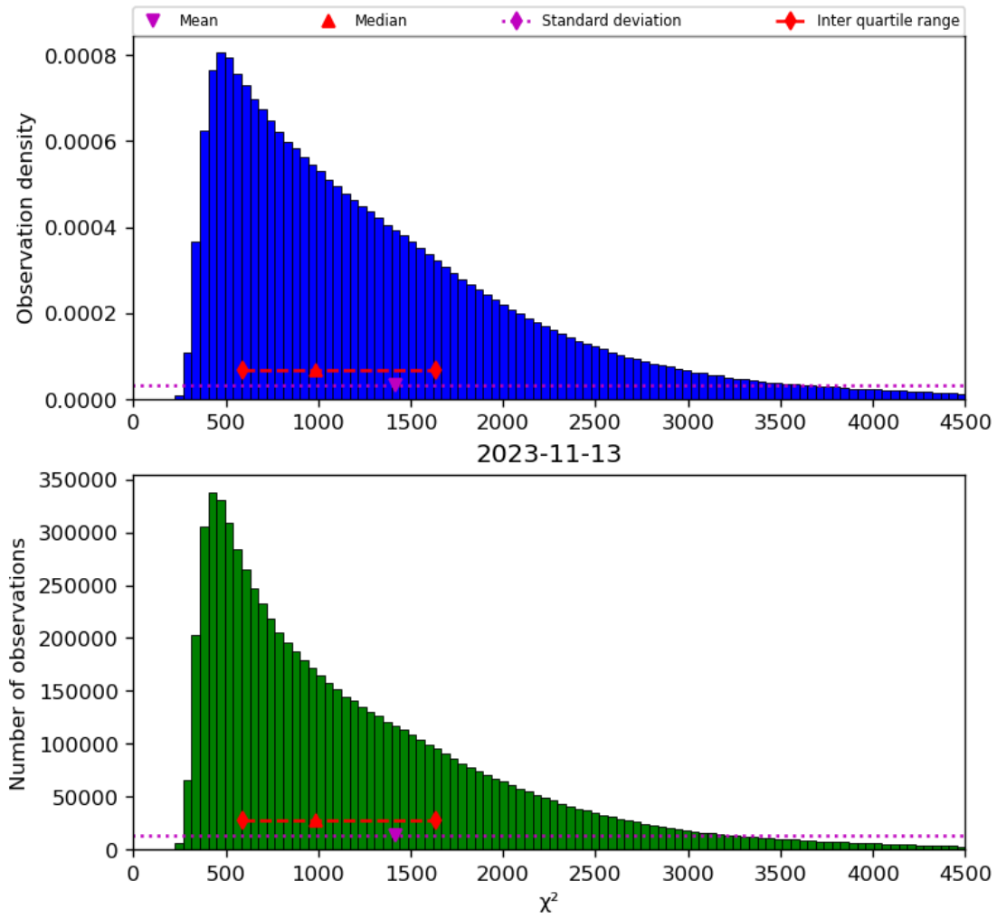
Figure 22: Histogram of “ \chi^2 ” for 2023-11-13 to 2023-11-14
