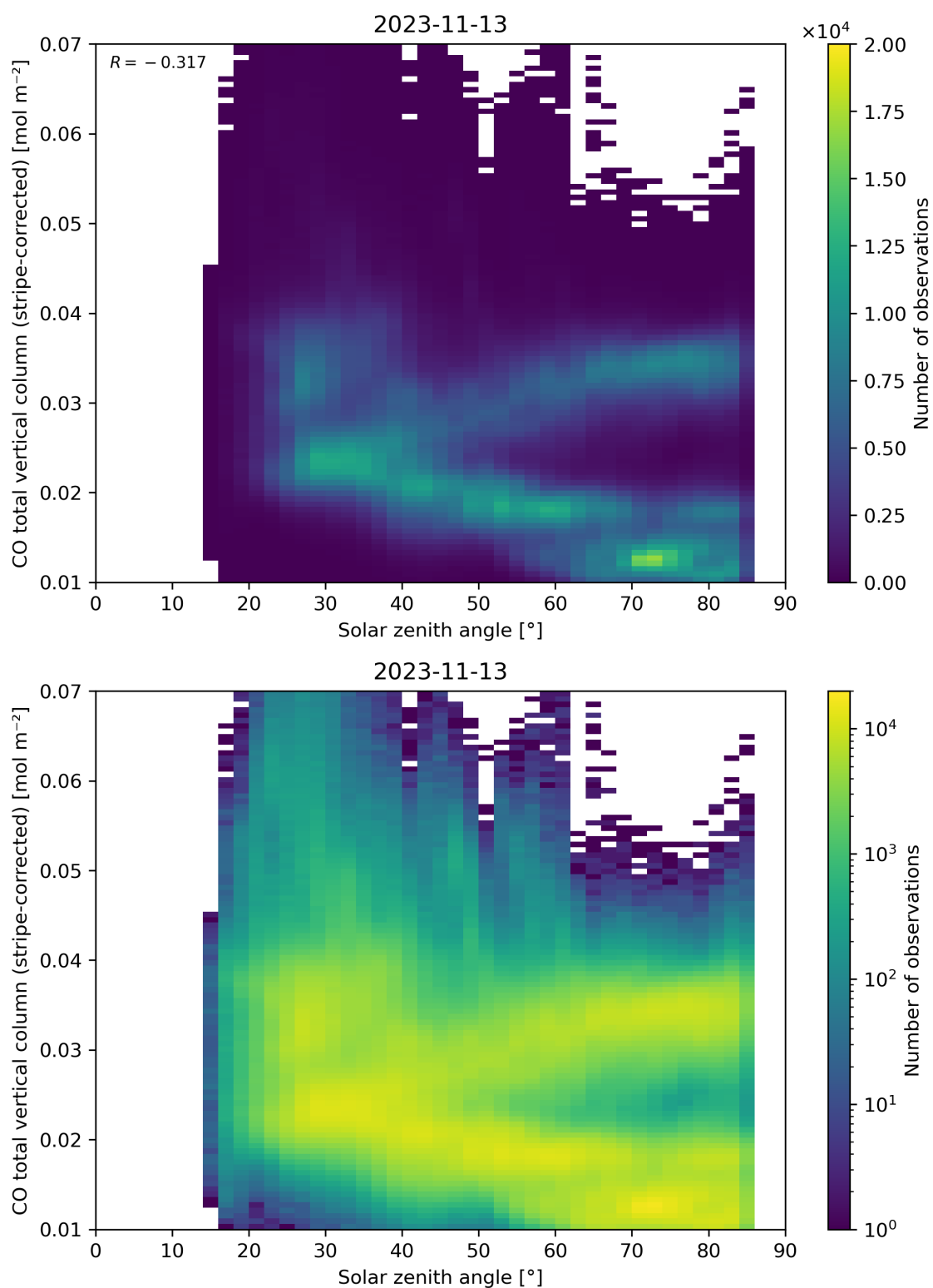
Figure 62: Scatter density plot of “Solar zenith angle” against “CO total vertical column (stripe-corrected)” for 2023-11-13 to 2023-11-14.
