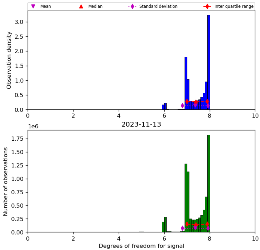
Figure 23: Histogram of “Degrees of freedom for signal” for 2023-11-13 to 2023-11-14
