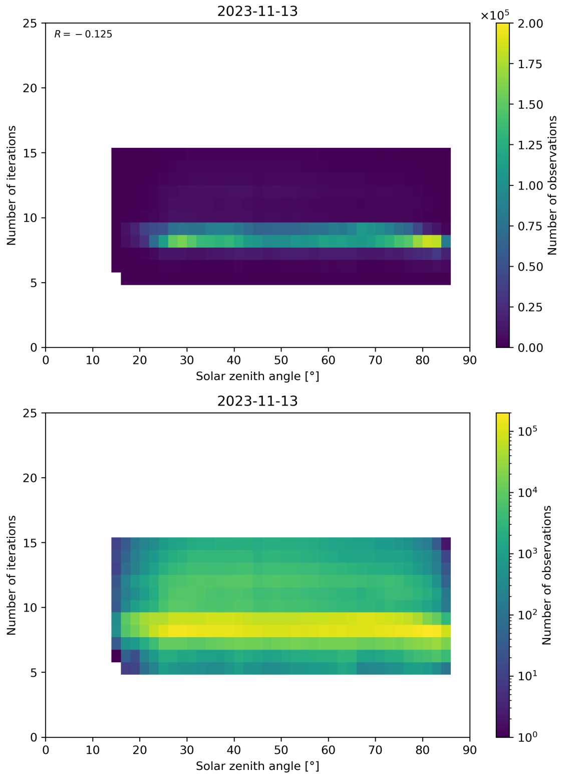
Figure 67: Scatter density plot of “Solar zenith angle” against “Number of iterations” for 2023-11-13 to 2023-11-14.
