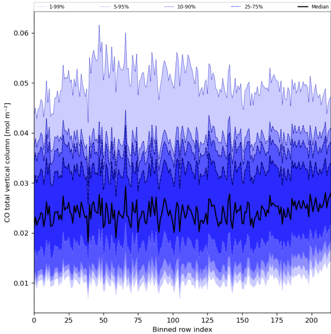
Figure 26: Along track statistics of “CO total vertical column” for 2023-11-13 to 2023-11-14
