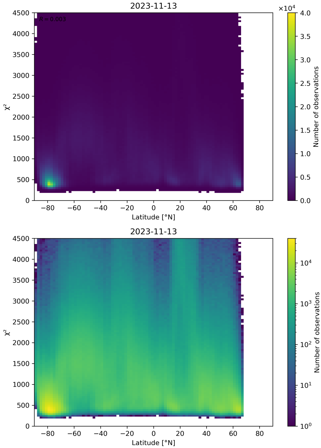
Figure 54: Scatter density plot of “Latitude” against “ \chi^2 ” for 2023-11-13 to 2023-11-14.
