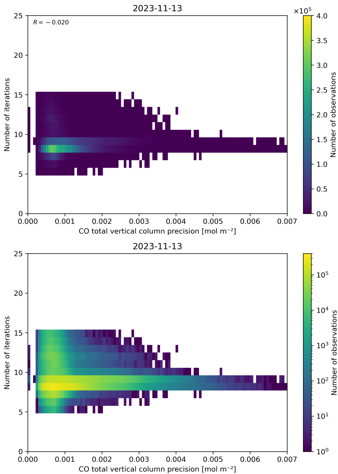
Figure 46: Scatter density plot of “CO total vertical column precision” against “Number of iterations” for 2023-11-13 to 2023-11-14.
