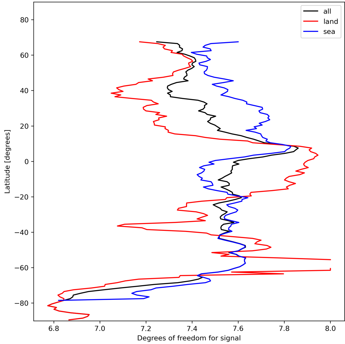
Figure 15: Zonal average of “Degrees of freedom for signal” for 2023-11-13 to 2023-11-14.
