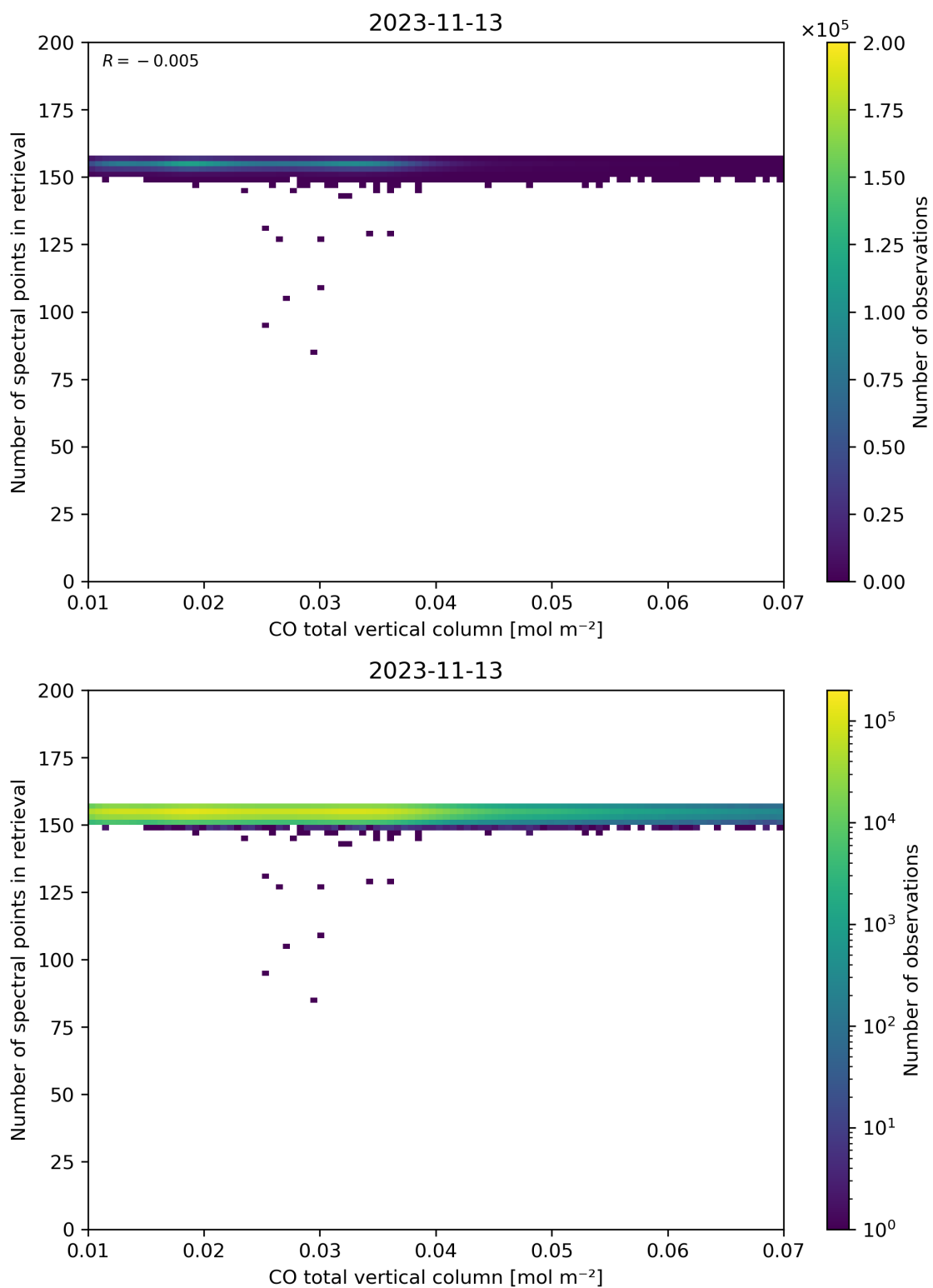
Figure 43: Scatter density plot of “CO total vertical column” against “Number of spectral points in retrieval” for 2023-11-13 to 2023-11-14.
