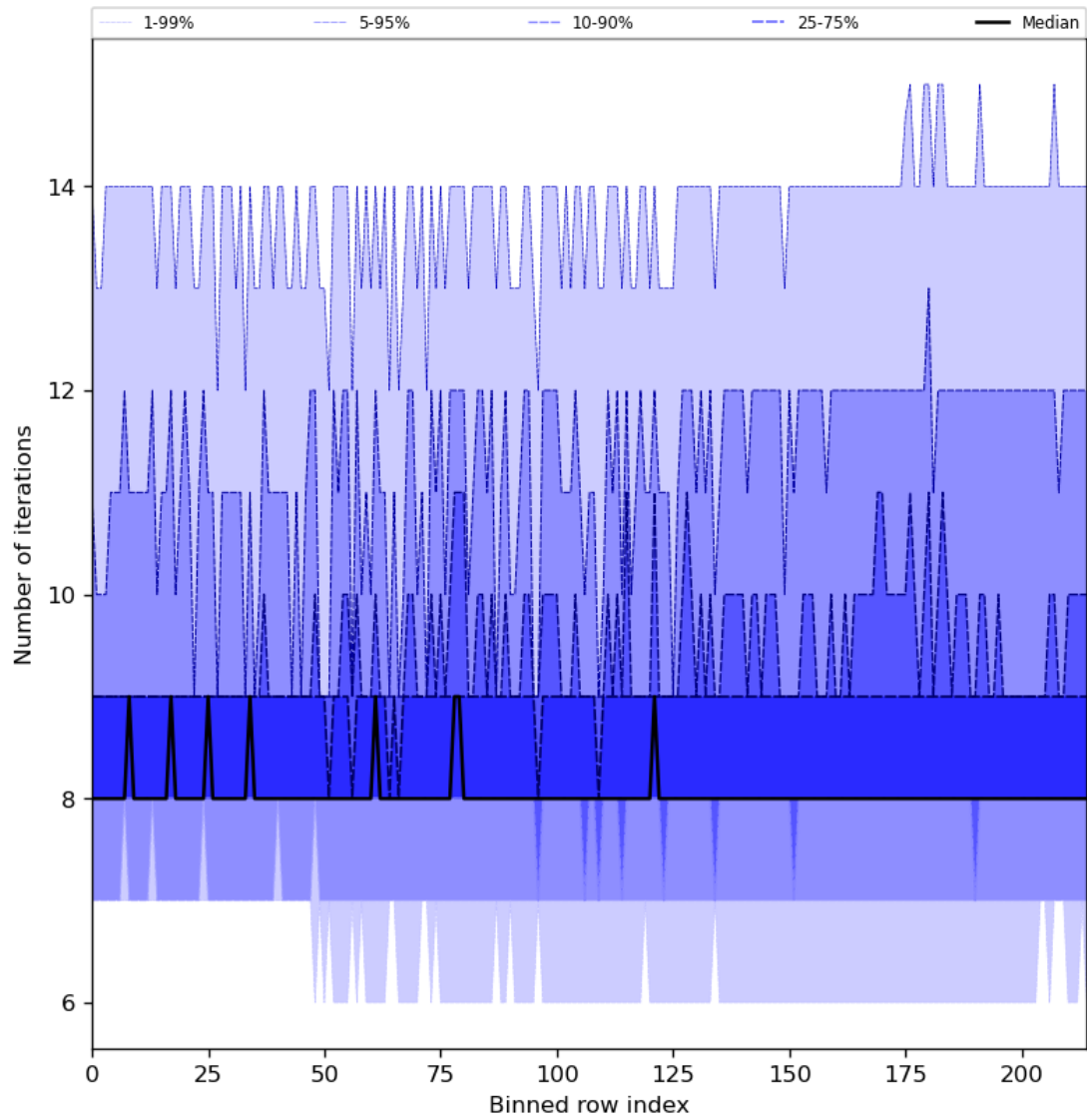
Figure 32: Along track statistics of “Number of iterations” for 2023-11-13 to 2023-11-14
