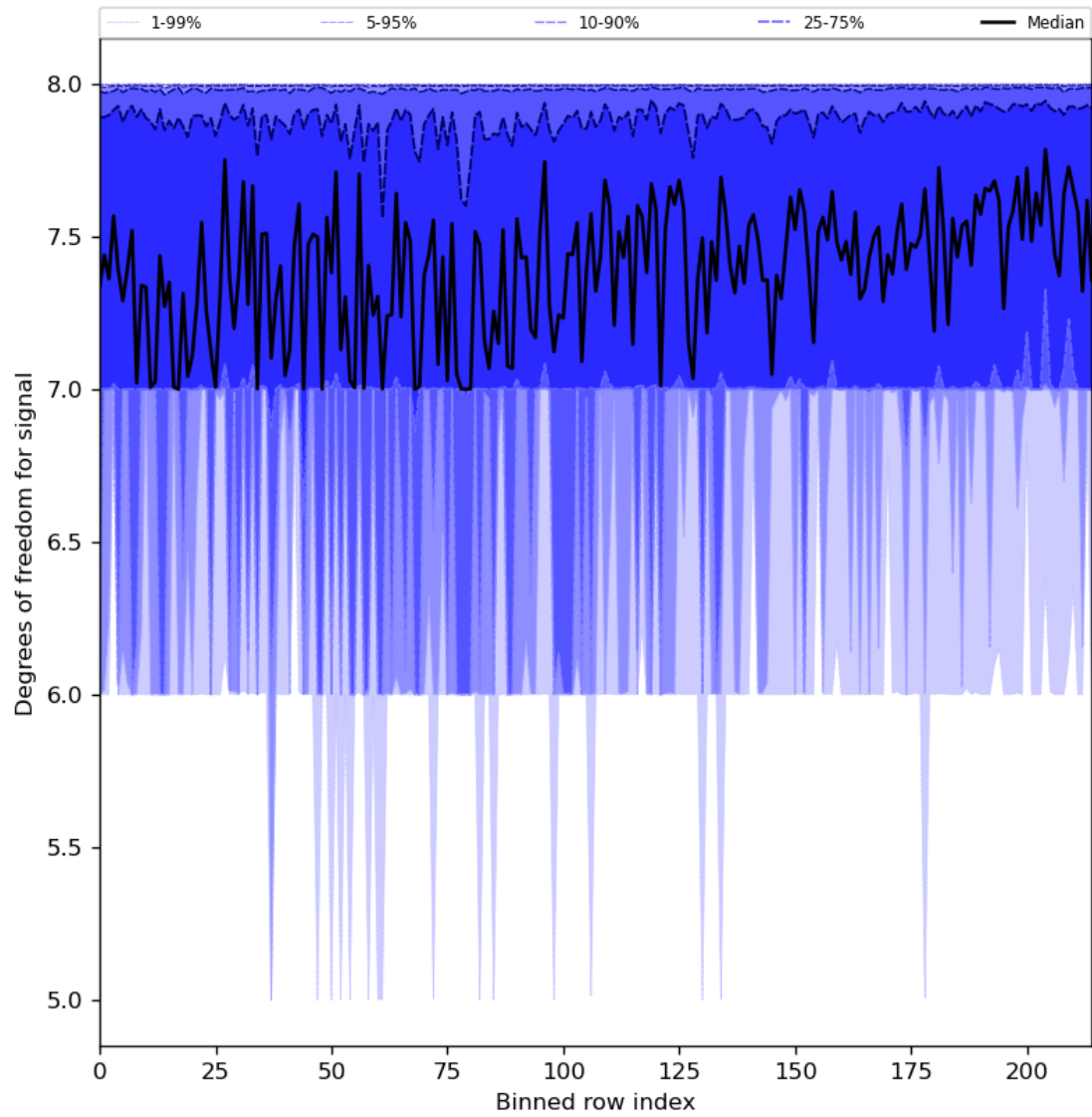
Figure 31: Along track statistics of “Degrees of freedom for signal” for 2023-11-13 to 2023-11-14
