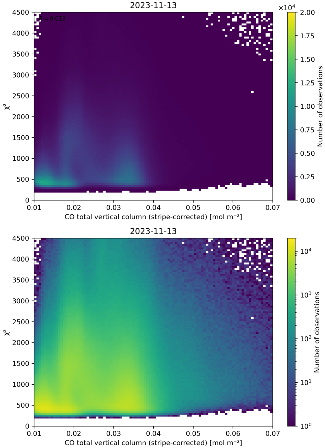
Figure 37: Scatter density plot of “CO total vertical column (stripe-corrected)” against “ \chi^2 ” for 2023-11-13 to 2023-11-14.
