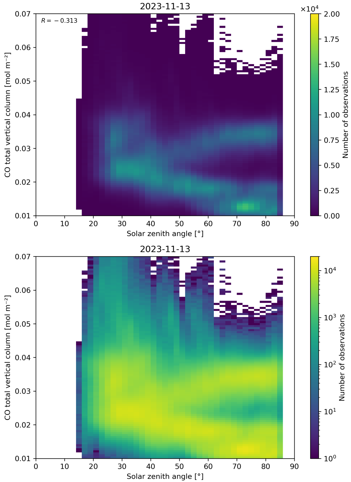
Figure 61: Scatter density plot of “Solar zenith angle” against “CO total vertical column” for 2023-11-13 to 2023-11-14.
