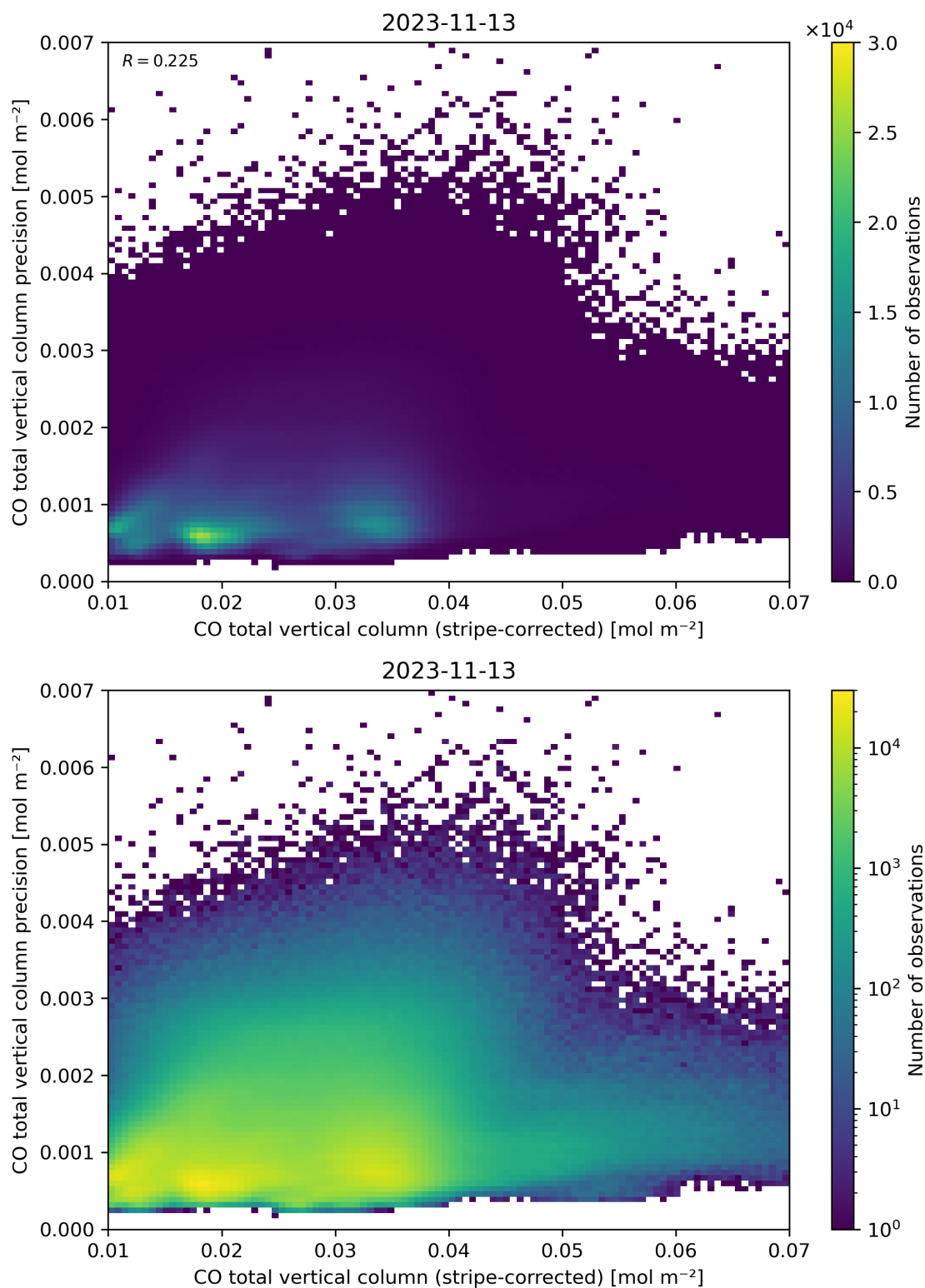
Figure 36: Scatter density plot of “CO total vertical column (stripe-corrected)” against “CO total vertical column precision” for 2023-11-13 to 2023-11-14.
