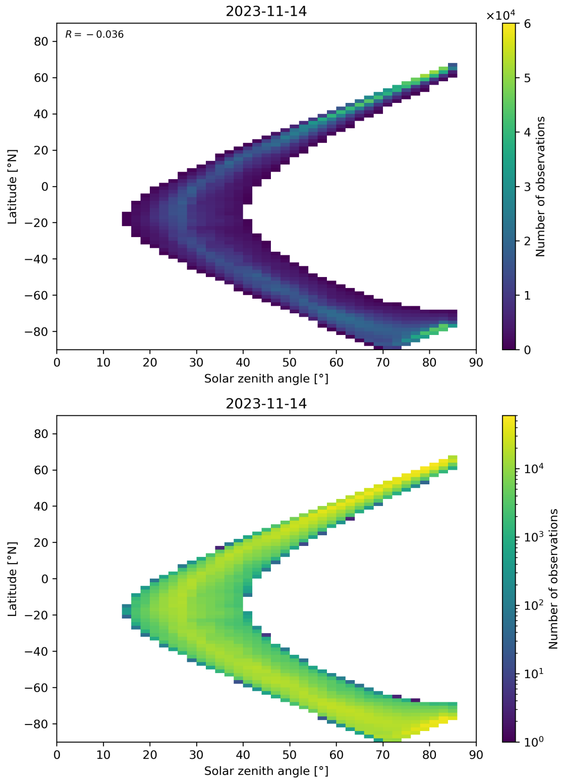
Figure 66: Scatter density plot of “Solar zenith angle” against “Latitude” for 2023-11-13 to 2023-11-15.
