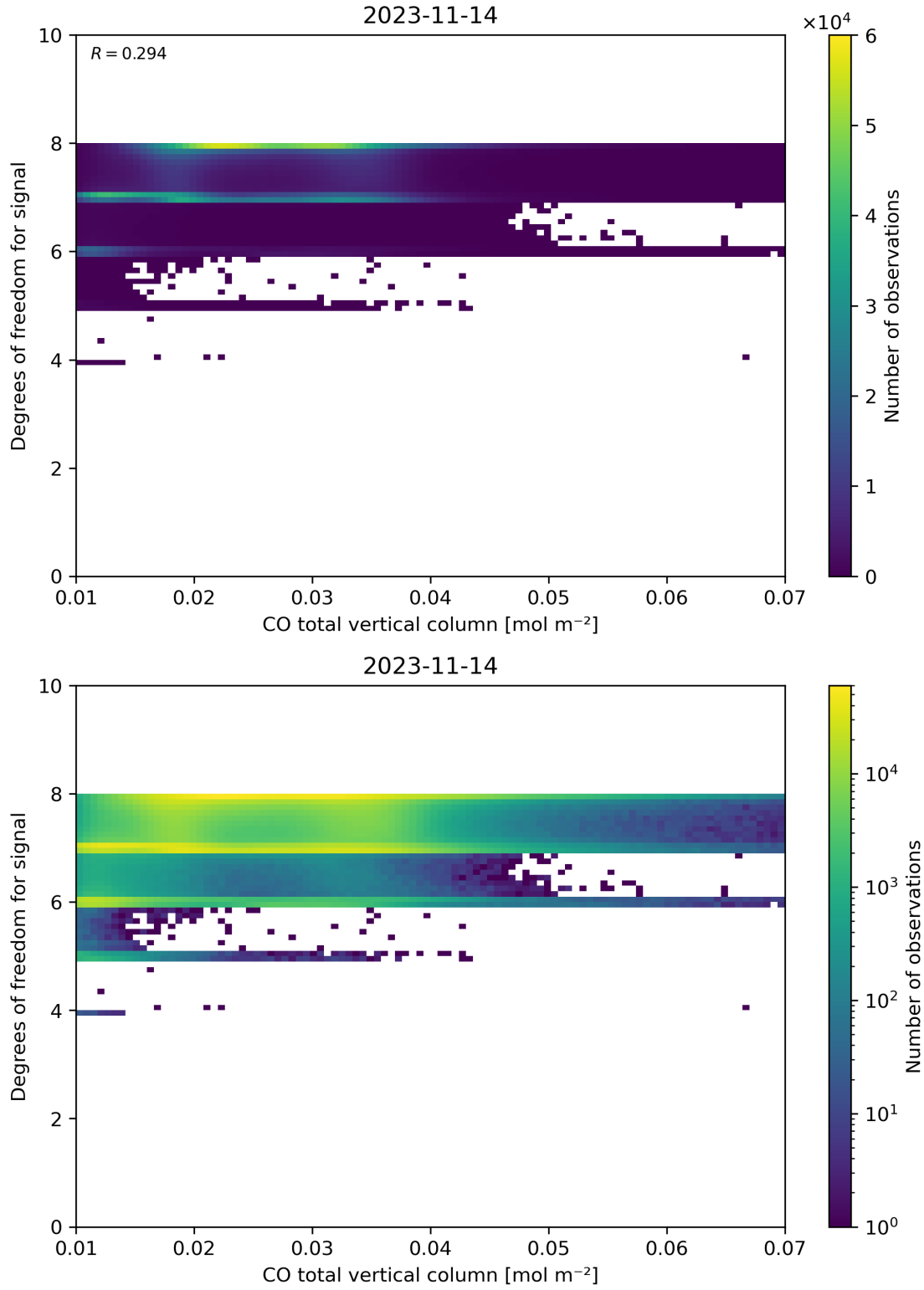
Figure 41: Scatter density plot of “CO total vertical column” against “Degrees of freedom for signal” for 2023-11-13 to 2023-11-15.
