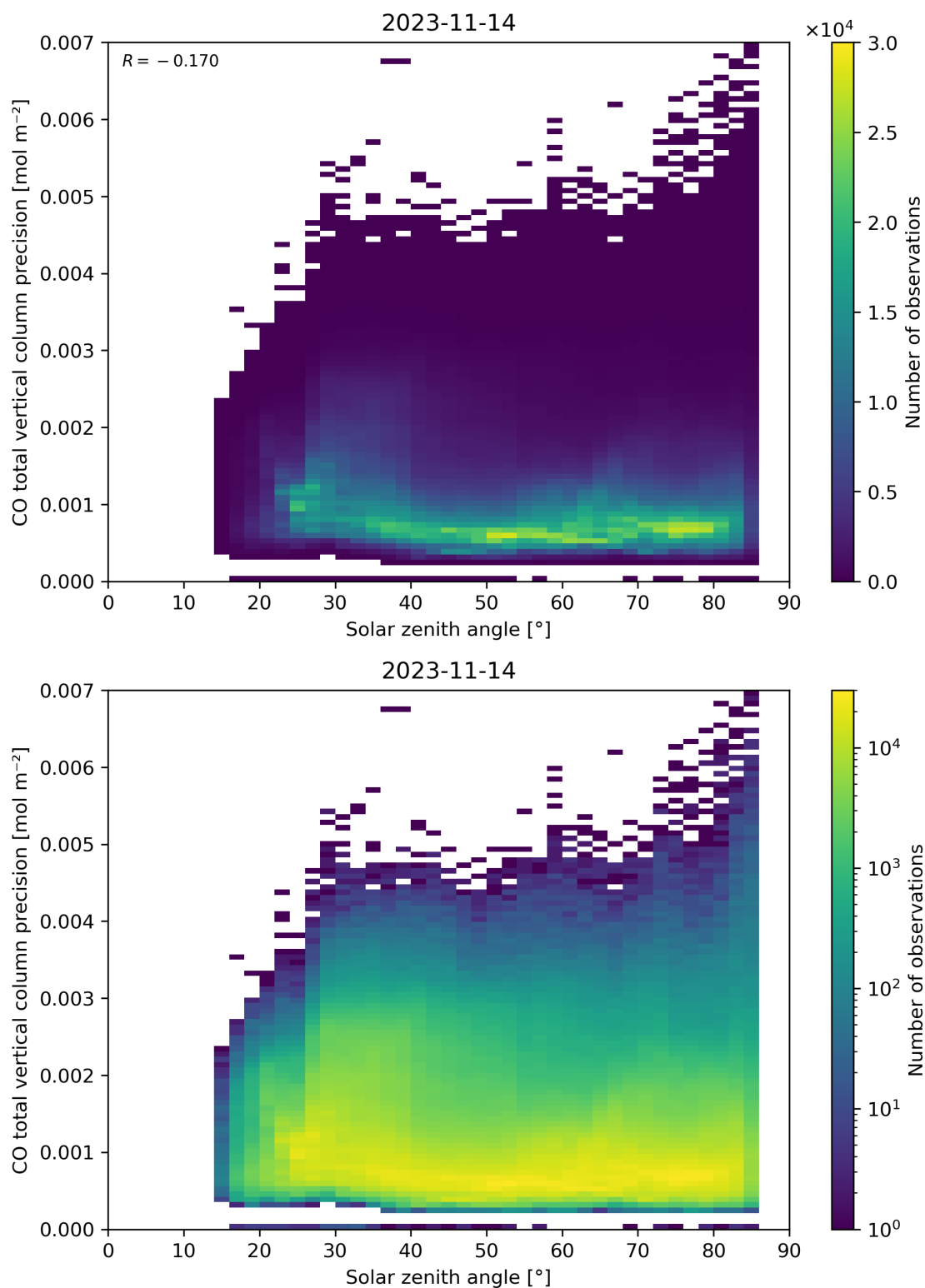
Figure 63: Scatter density plot of “Solar zenith angle” against “CO total vertical column precision” for 2023-11-13 to 2023-11-15.
