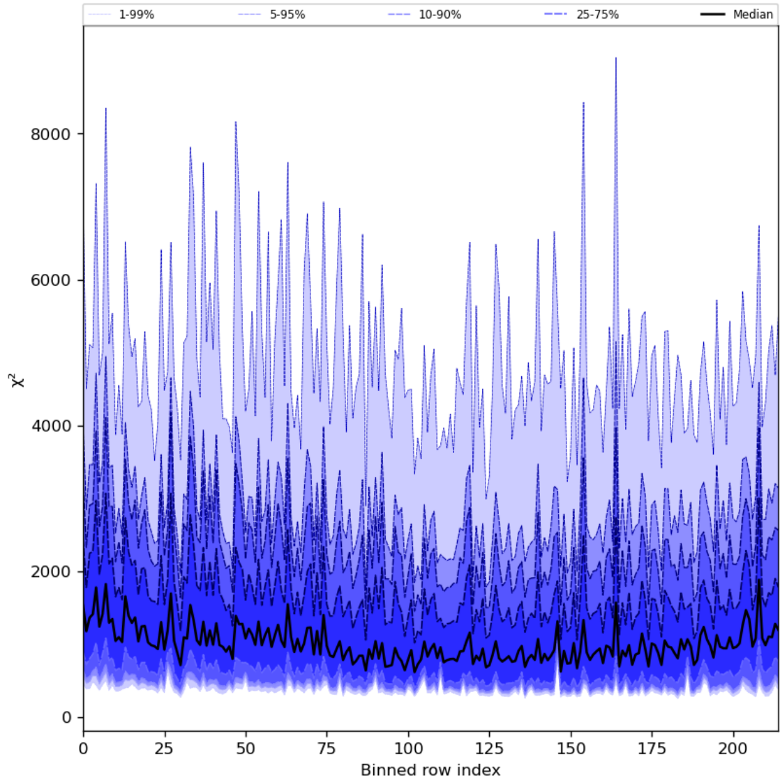
Figure 30: Along track statistics of “ \chi^2 ” for 2023-11-13 to 2023-11-15
