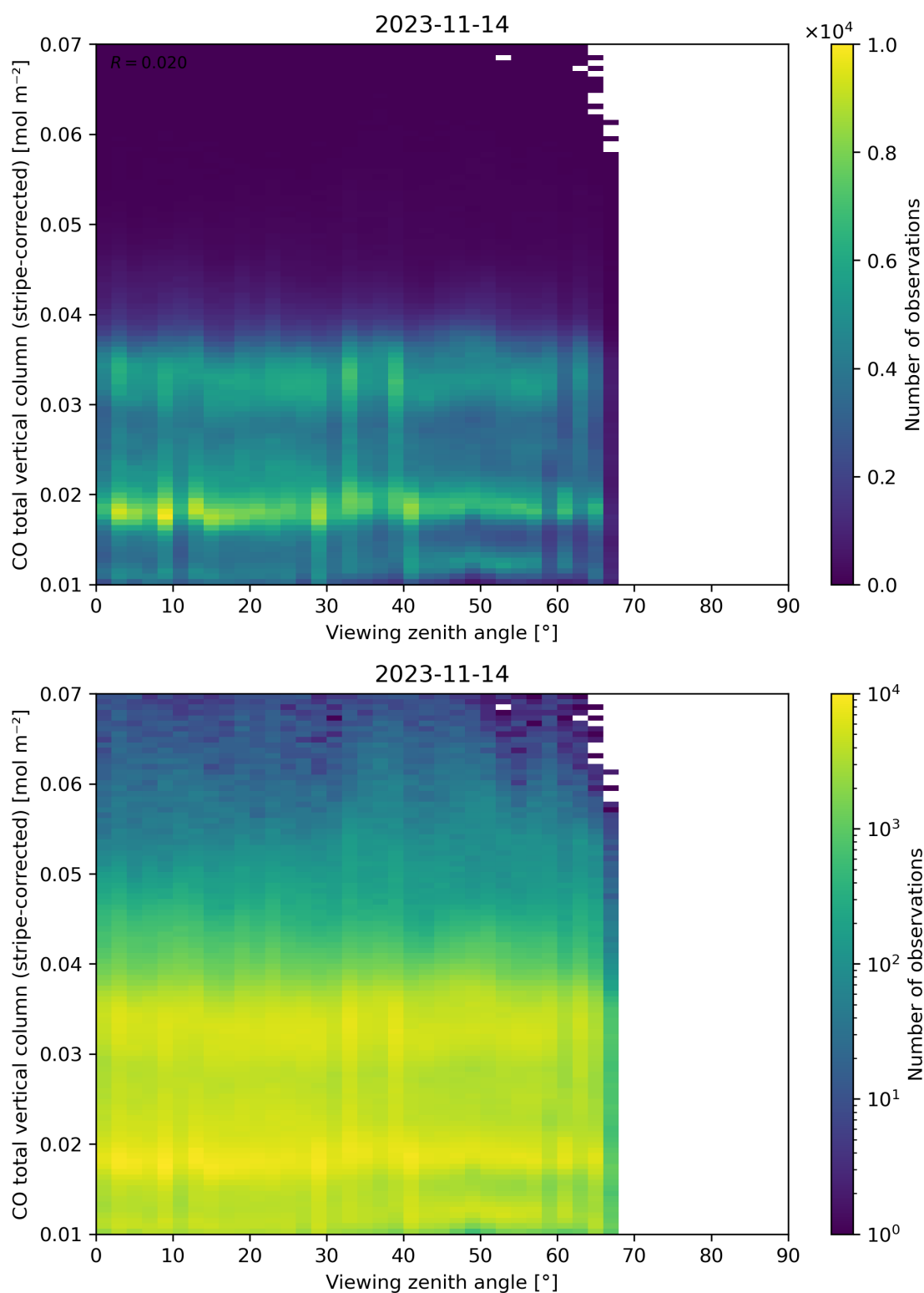
Figure 70: Scatter density plot of “Viewing zenith angle” against “CO total vertical column (stripe-corrected)” for 2023-11-13 to 2023-11-15.
