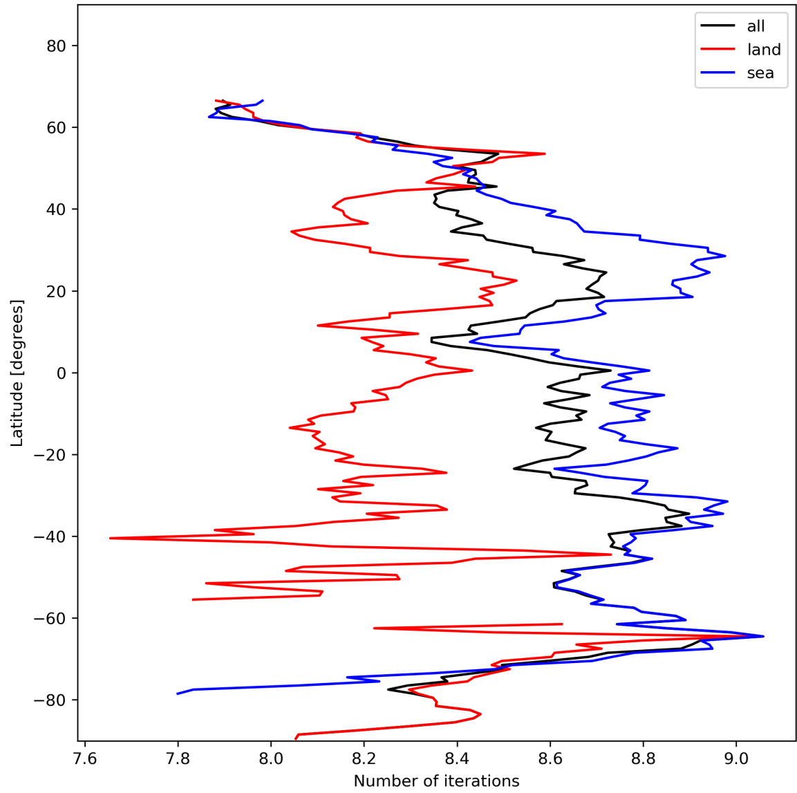
Figure 16: Zonal average of “Number of iterations” for 2023-11-13 to 2023-11-15.
