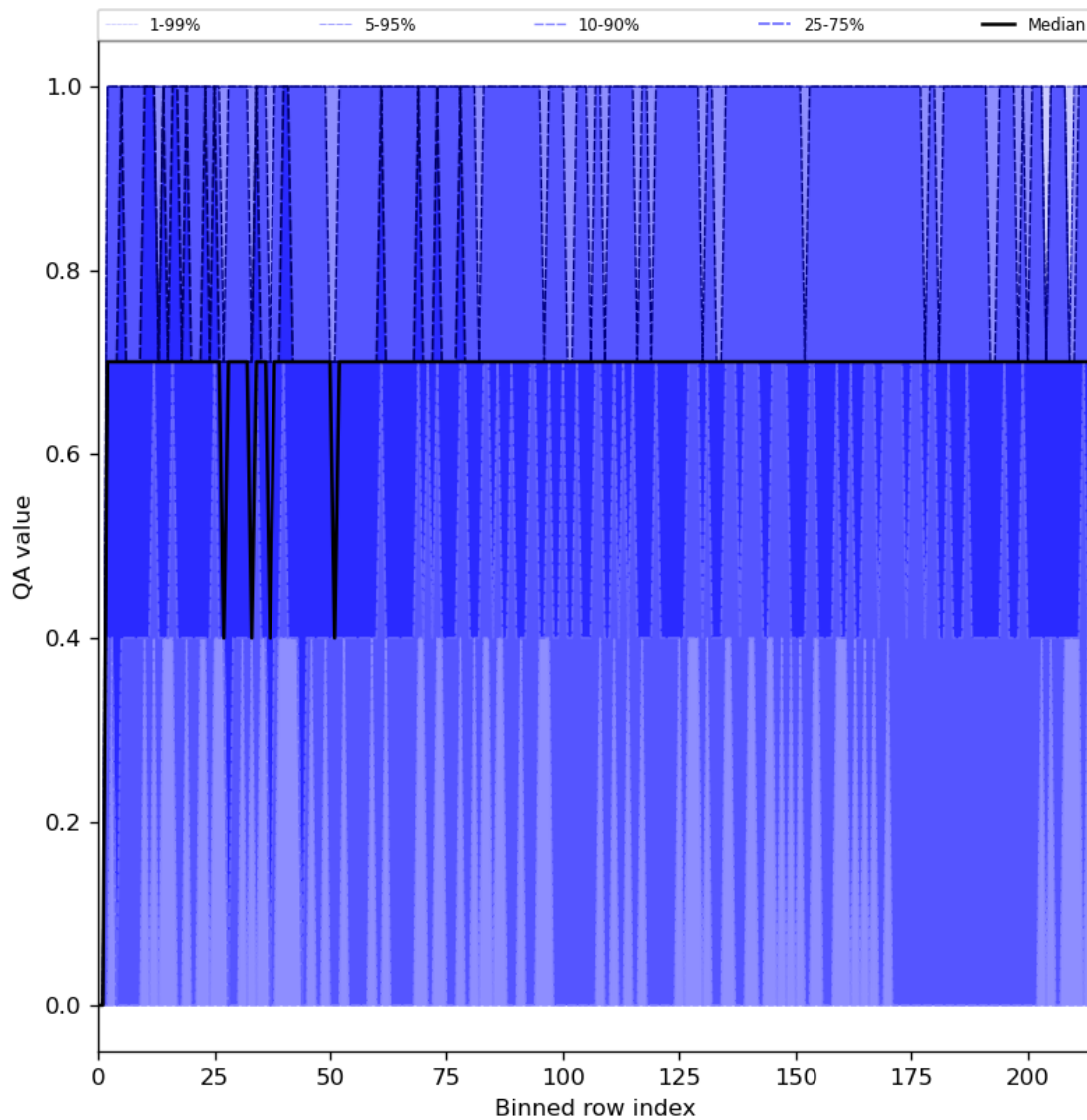
Figure 25: Along track statistics of “QA value” for 2023-11-13 to 2023-11-15
