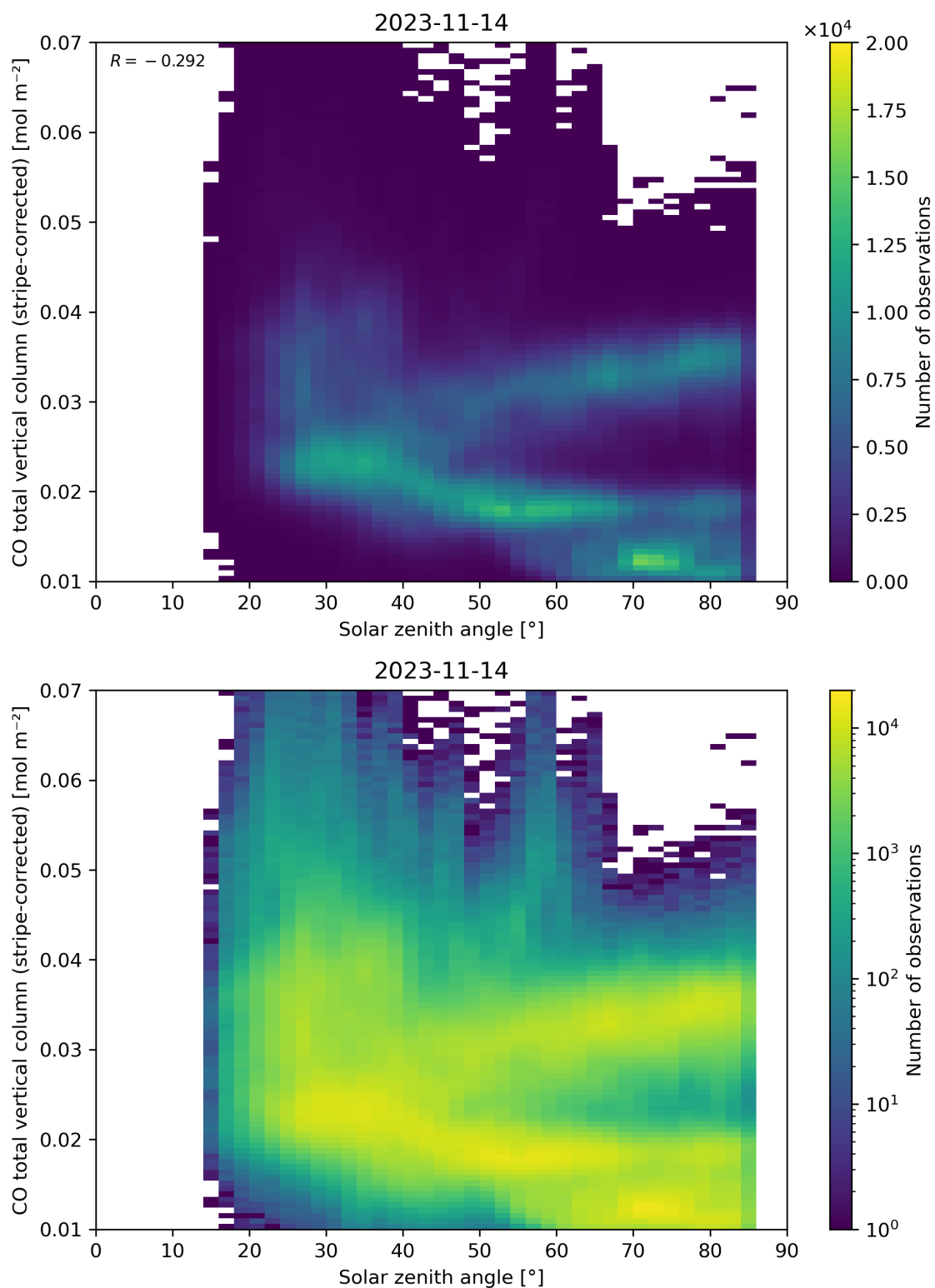
Figure 62: Scatter density plot of “Solar zenith angle” against “CO total vertical column (stripe-corrected)” for 2023-11-13 to 2023-11-15.
