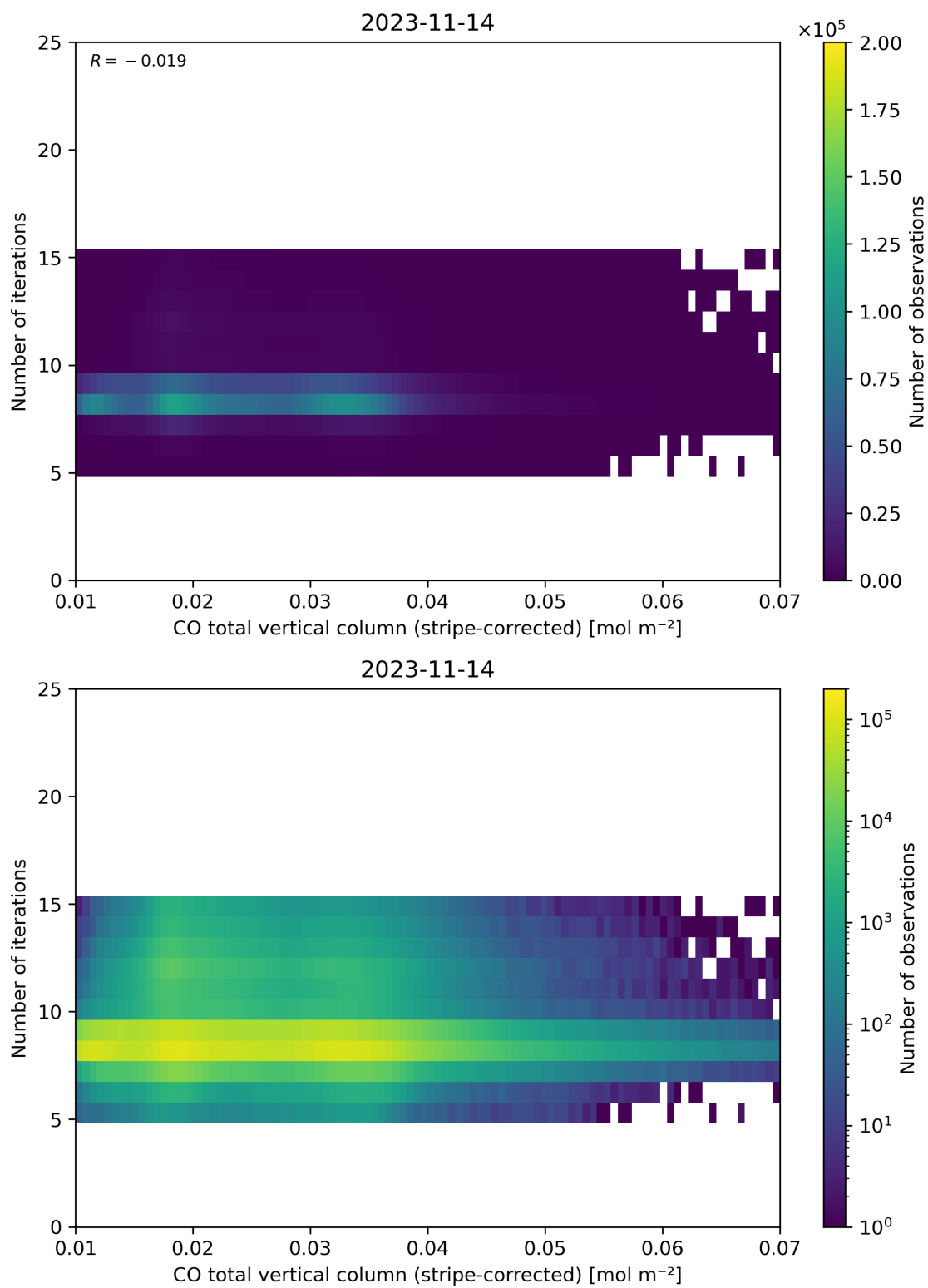
Figure 39: Scatter density plot of “CO total vertical column (stripe-corrected)” against “Number of iterations” for 2023-11-13 to 2023-11-15.
