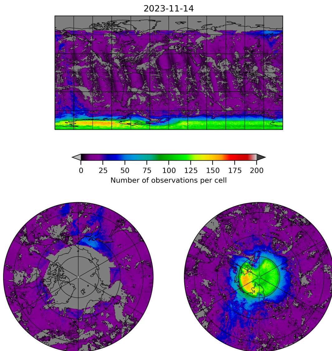
Figure 8: Map of the number of observations for 2023-11-13 to 2023-11-15
