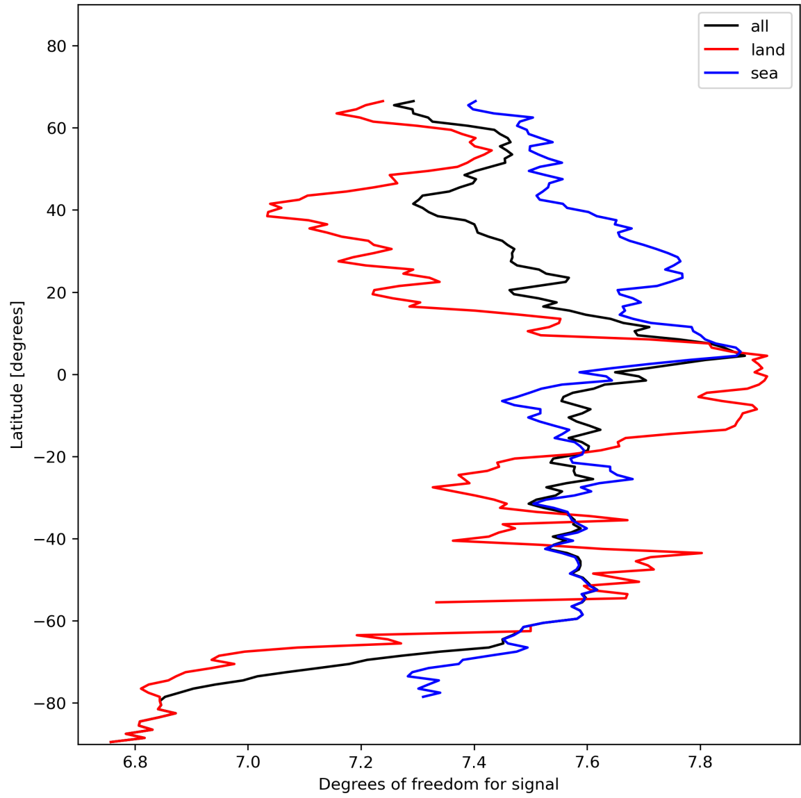
Figure 15: Zonal average of “Degrees of freedom for signal” for 2023-11-13 to 2023-11-15.
