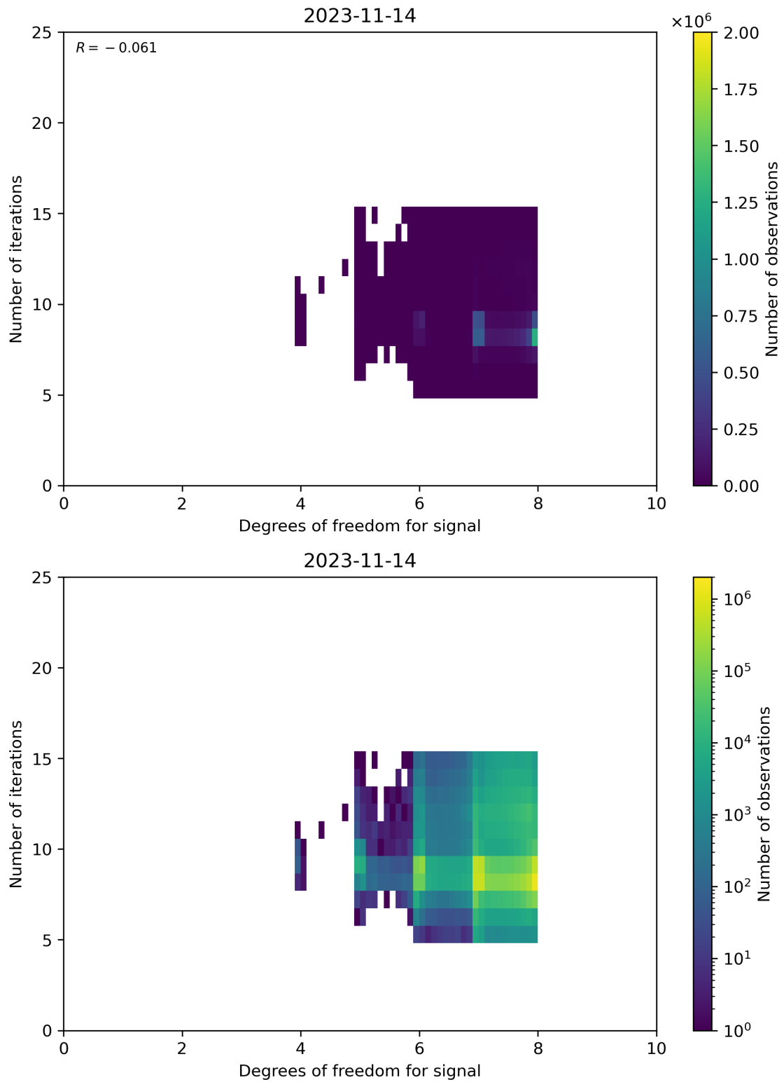
Figure 50: Scatter density plot of “Degrees of freedom for signal” against “Number of iterations” for 2023-11-13 to 2023-11-15.
