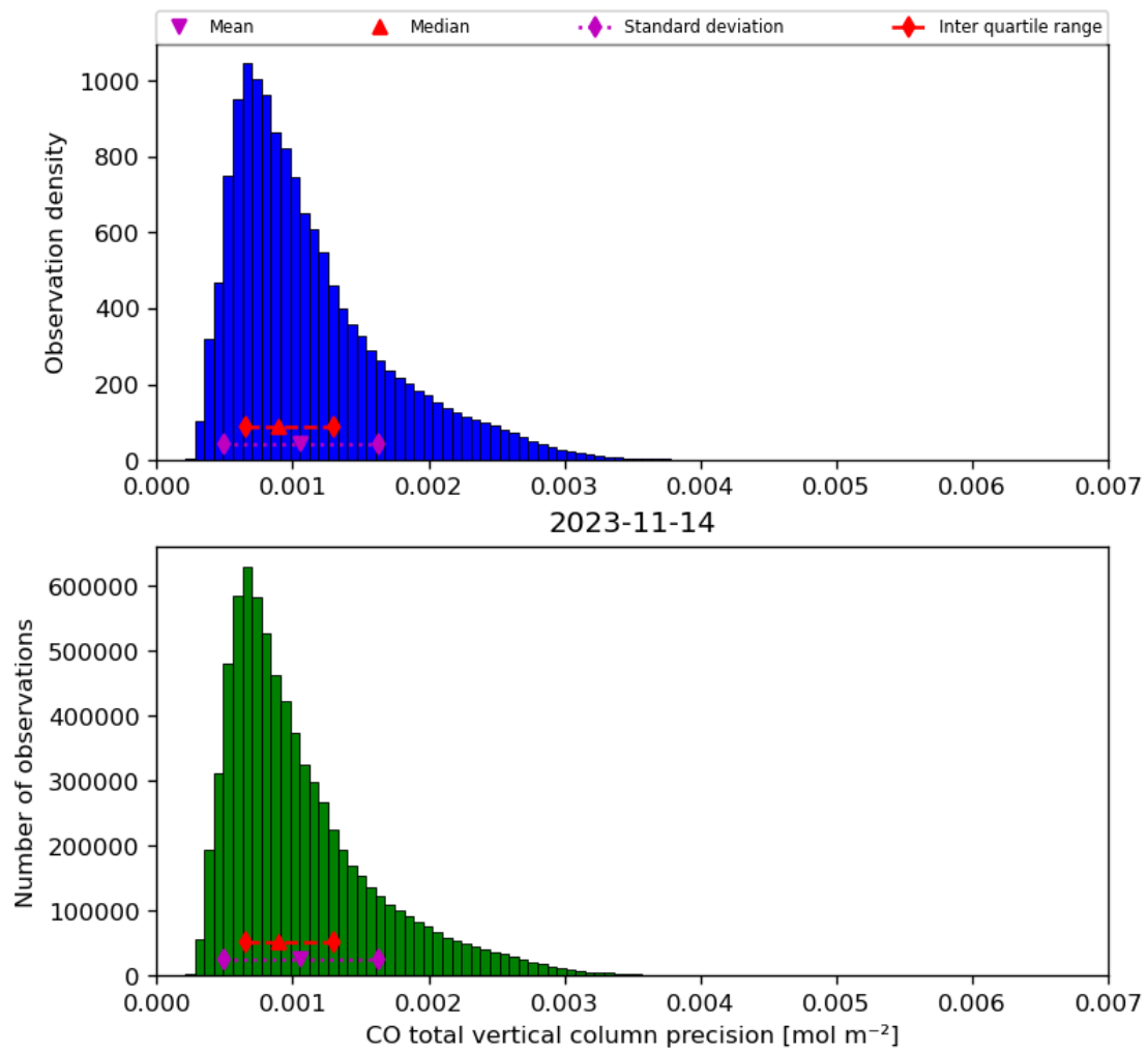
Figure 20: Histogram of “CO total vertical column precision” for 2023-11-13 to 2023-11-15
