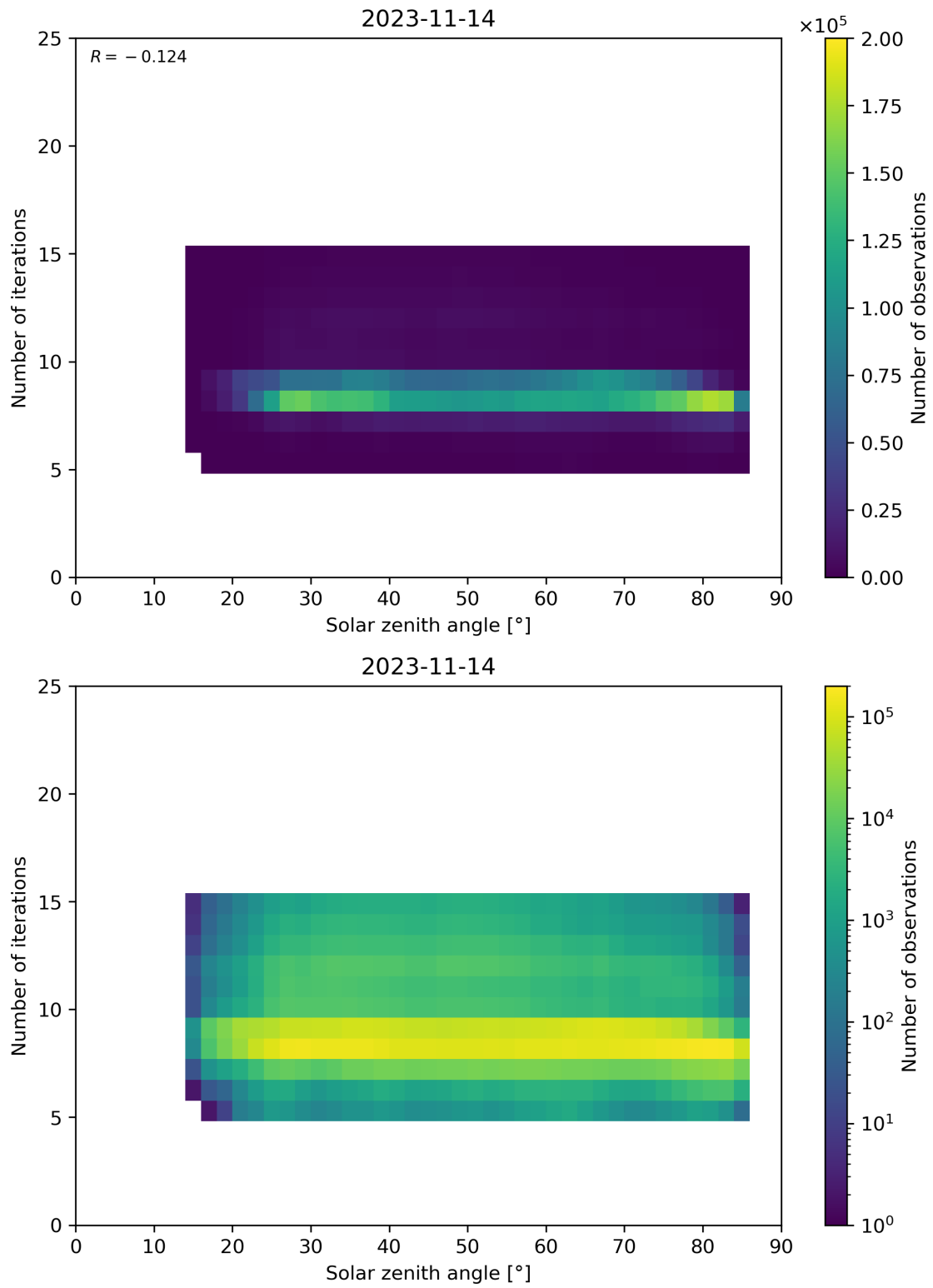
Figure 67: Scatter density plot of “Solar zenith angle” against “Number of iterations” for 2023-11-13 to 2023-11-15.
