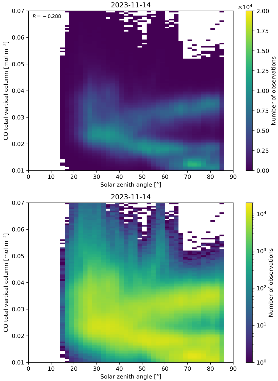
Figure 61: Scatter density plot of “Solar zenith angle” against “CO total vertical column” for 2023-11-13 to 2023-11-15.
