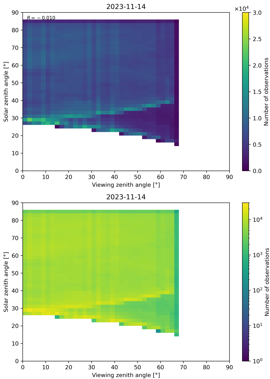
Figure 77: Scatter density plot of “Viewing zenith angle” against “Solar zenith angle” for 2023-11-13 to 2023-11-15.
