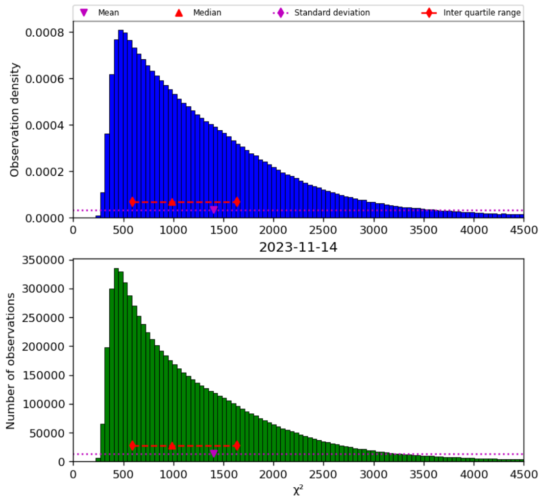
Figure 22: Histogram of “ \chi^2 ” for 2023-11-13 to 2023-11-15
