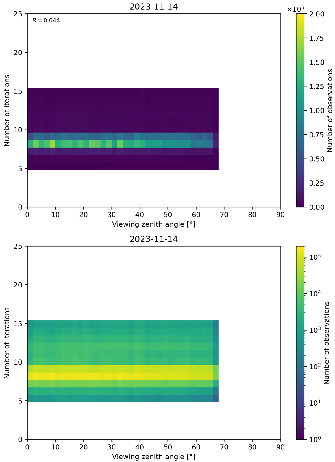
Figure 75: Scatter density plot of “Viewing zenith angle” against “Number of iterations” for 2023-11-13 to 2023-11-15.
