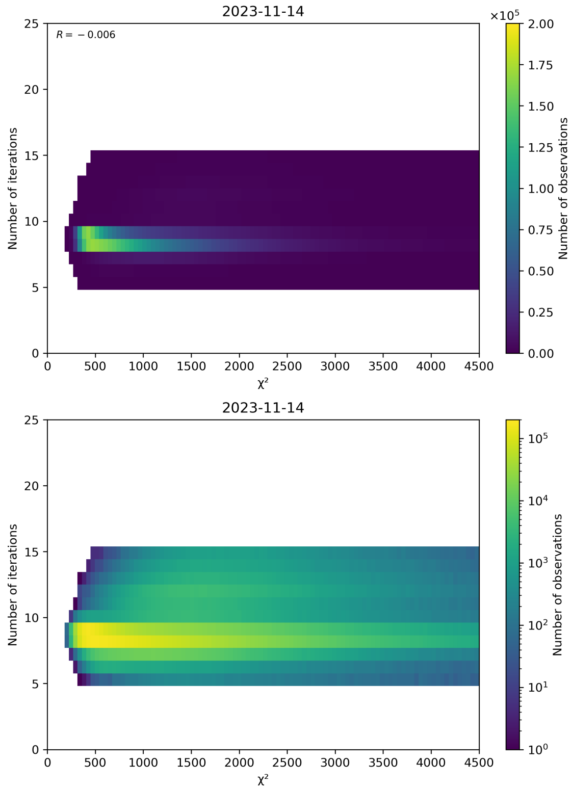
Figure 49: Scatter density plot of “ \chi^2 ” against “Number of iterations” for 2023-11-13 to 2023-11-15.
