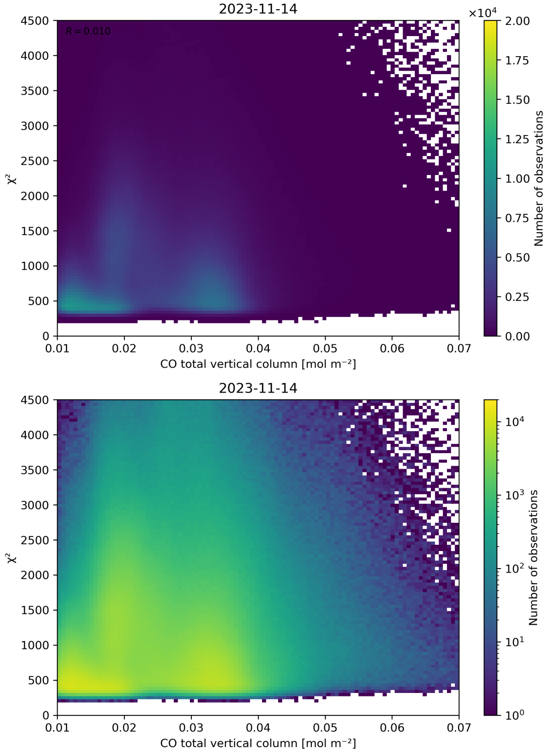
Figure 35: Scatter density plot of “CO total vertical column” against “ \chi^2 ” for 2023-11-13 to 2023-11-15.
