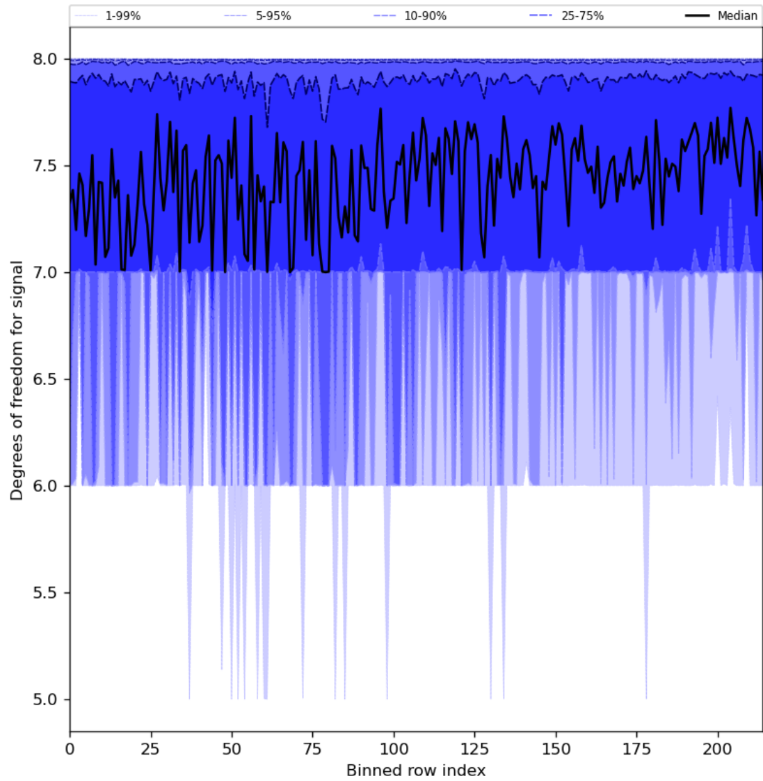
Figure 31: Along track statistics of “Degrees of freedom for signal” for 2023-11-13 to 2023-11-15
