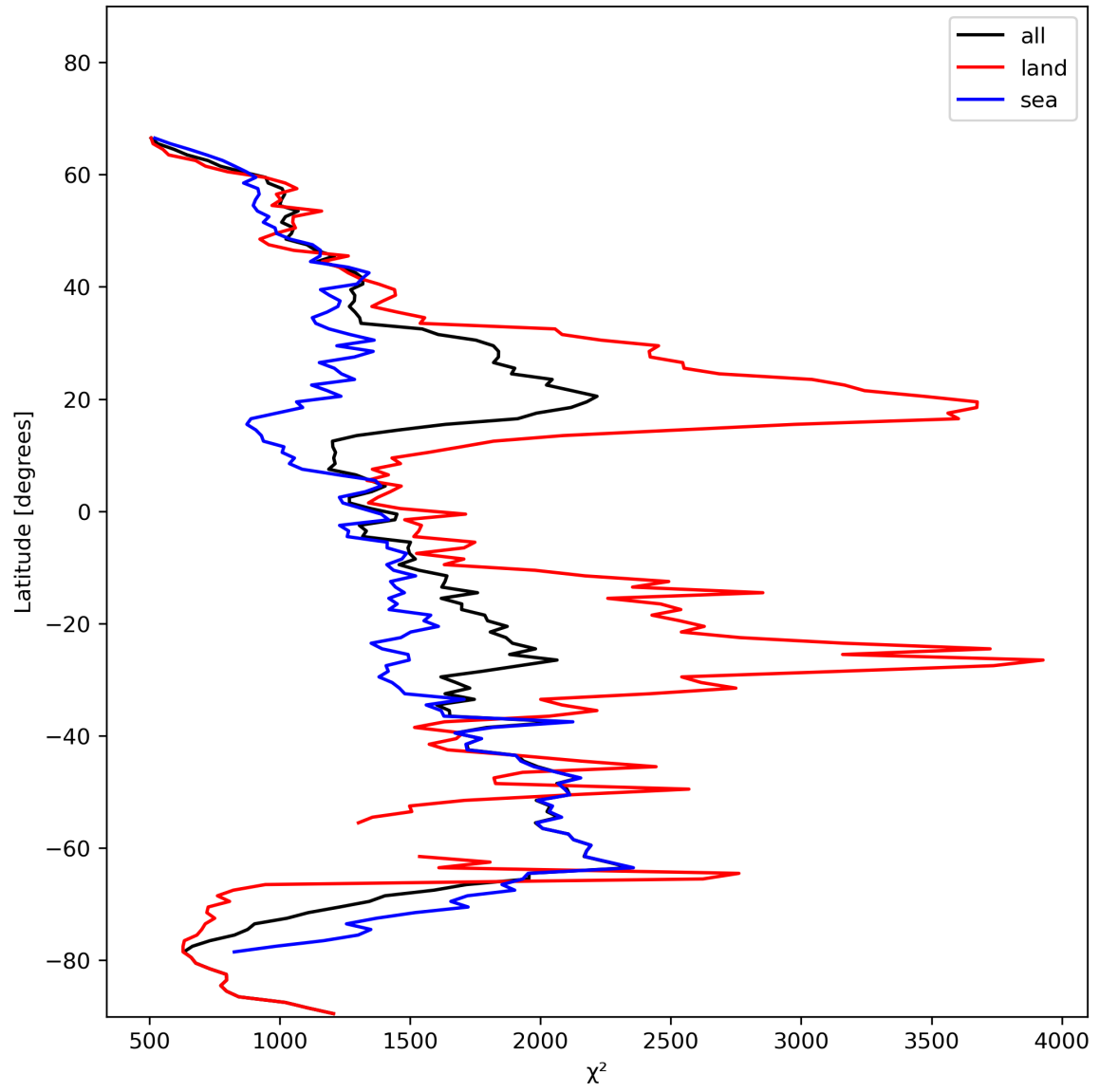
Figure 14: Zonal average of “ \chi^2 ” for 2023-11-13 to 2023-11-15.
