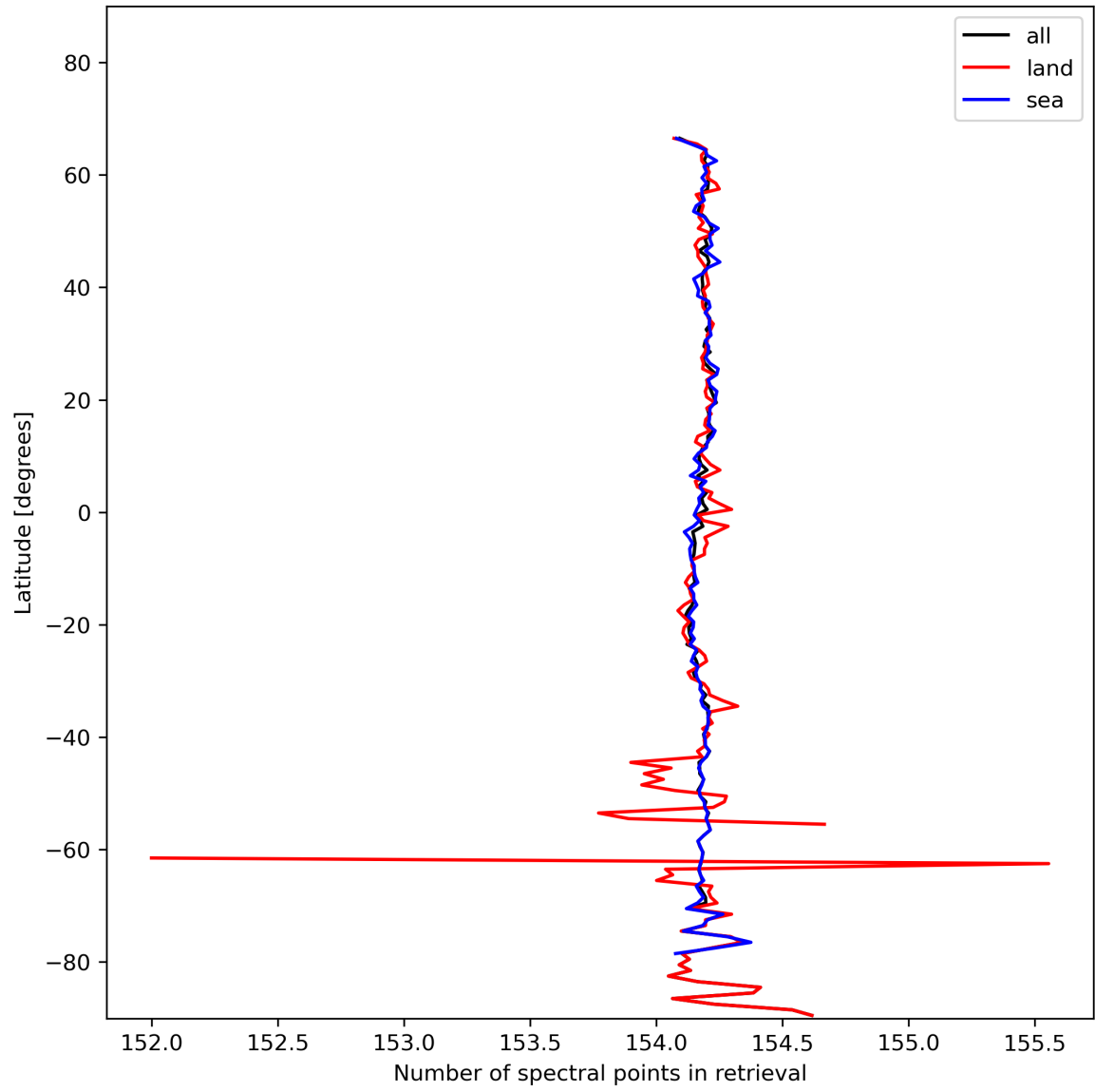
Figure 13: Zonal average of “Number of spectral points in retrieval” for 2023-11-13 to 2023-11-15.
