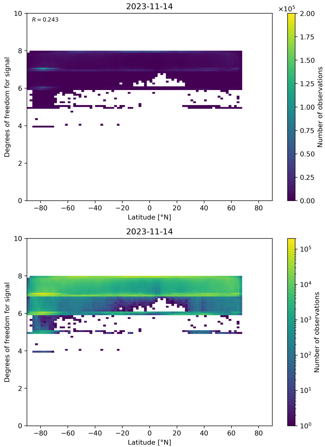
Figure 55: Scatter density plot of “Latitude” against “Degrees of freedom for signal” for 2023-11-13 to 2023-11-15.
