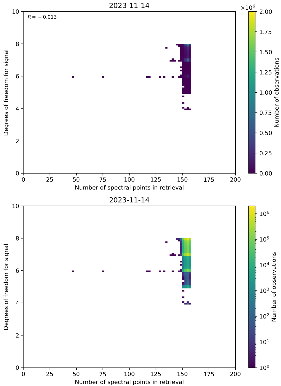
Figure 59: Scatter density plot of “Number of spectral points in retrieval” against “Degrees of freedom for signal” for 2023-11-13 to 2023-11-15.
