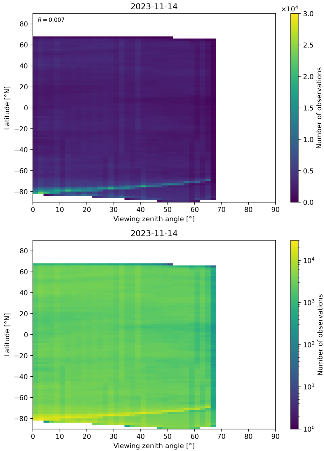
Figure 74: Scatter density plot of “Viewing zenith angle” against “Latitude” for 2023-11-13 to 2023-11-15.
