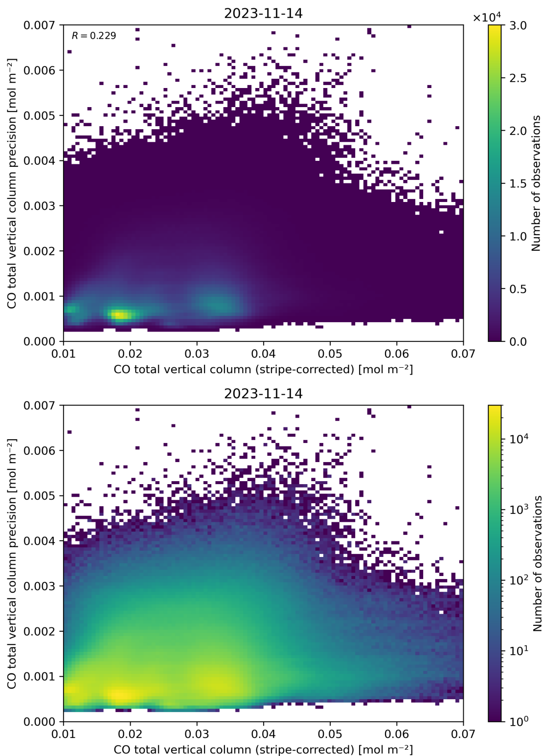
Figure 36: Scatter density plot of “CO total vertical column (stripe-corrected)” against “CO total vertical column precision” for 2023-11-13 to 2023-11-15.
