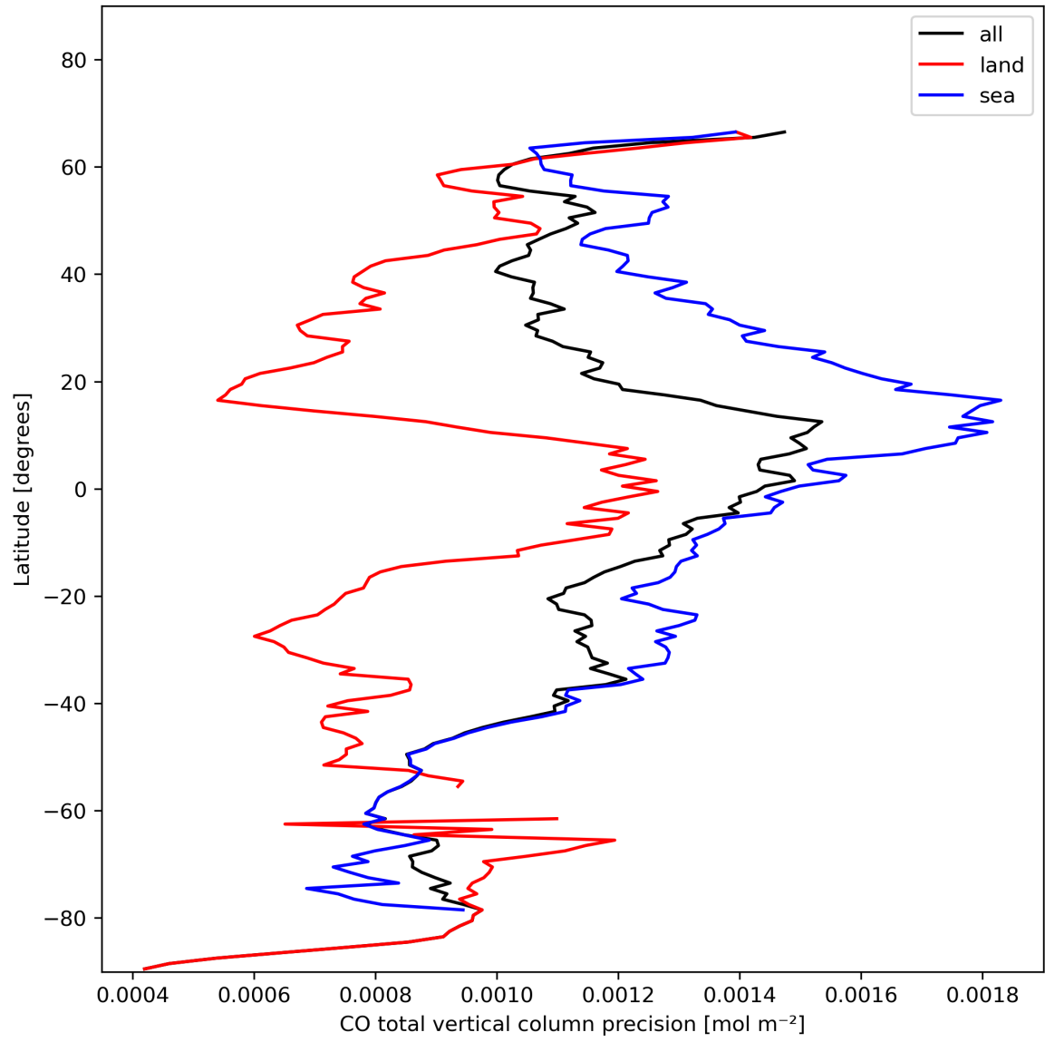
Figure 12: Zonal average of “CO total vertical column precision” for 2023-11-13 to 2023-11-15.
