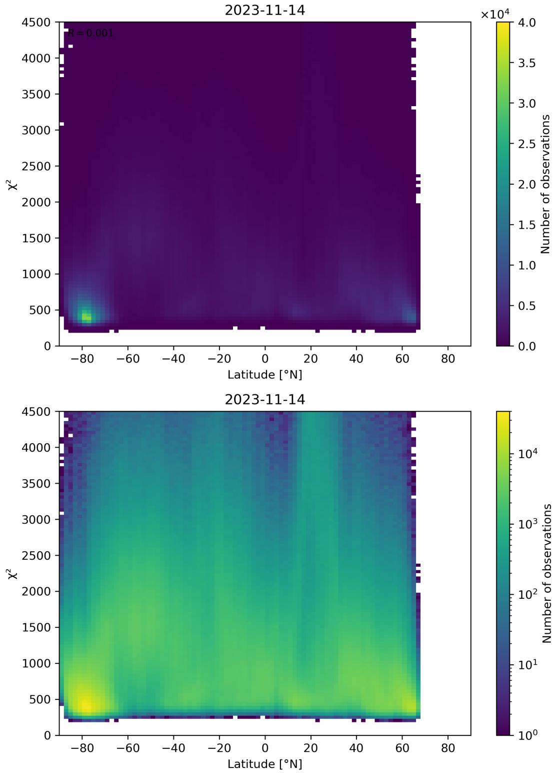
Figure 54: Scatter density plot of “Latitude” against “ \chi^2 ” for 2023-11-13 to 2023-11-15.
