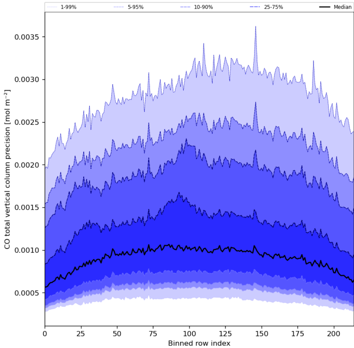
Figure 28: Along track statistics of “CO total vertical column precision” for 2023-11-13 to 2023-11-15
