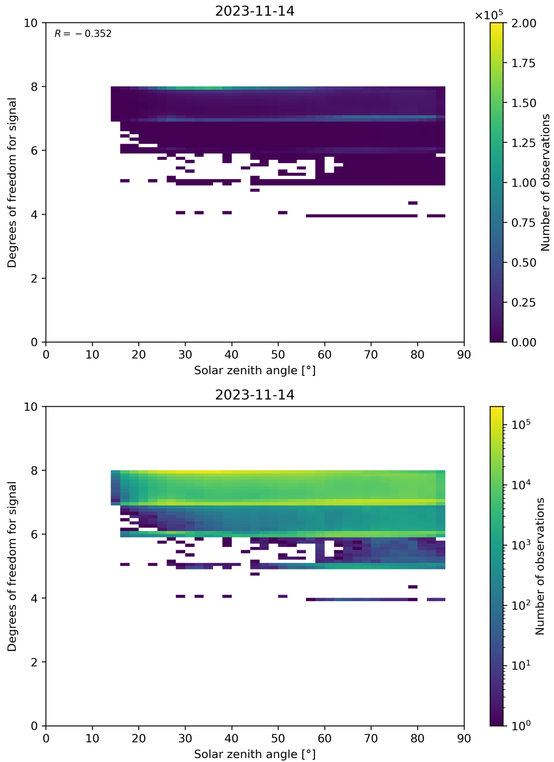
Figure 65: Scatter density plot of “Solar zenith angle” against “Degrees of freedom for signal” for 2023-11-13 to 2023-11-15.
