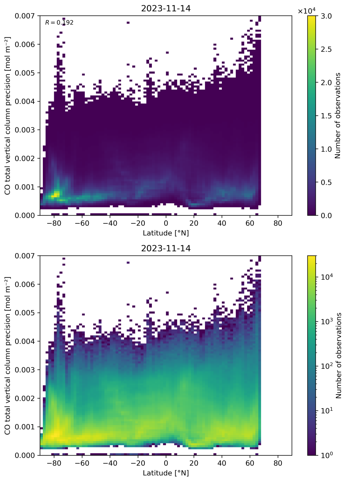
Figure 53: Scatter density plot of “Latitude” against “CO total vertical column precision” for 2023-11-13 to 2023-11-15.
