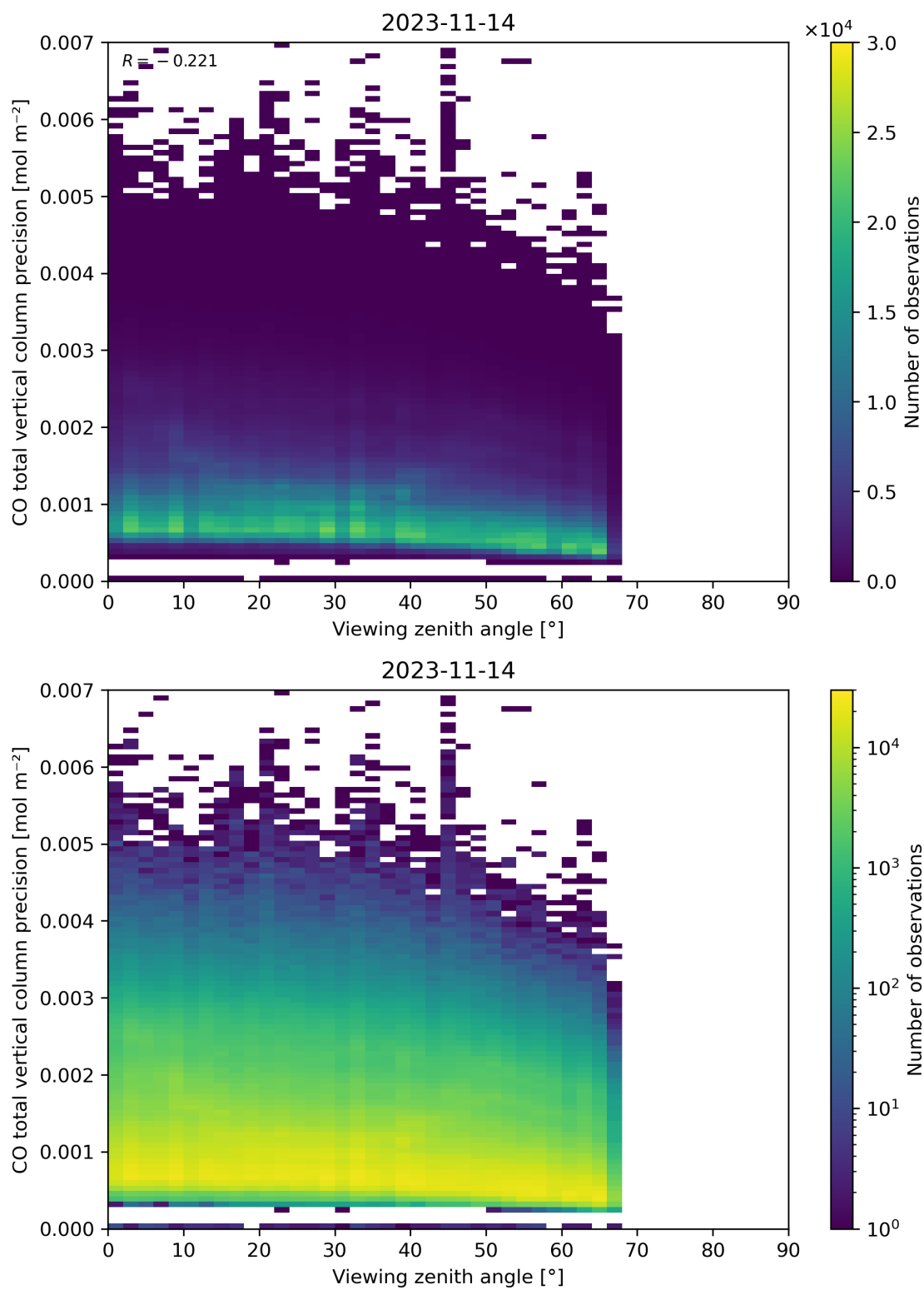
Figure 71: Scatter density plot of “Viewing zenith angle” against “CO total vertical column precision” for 2023-11-13 to 2023-11-15.
