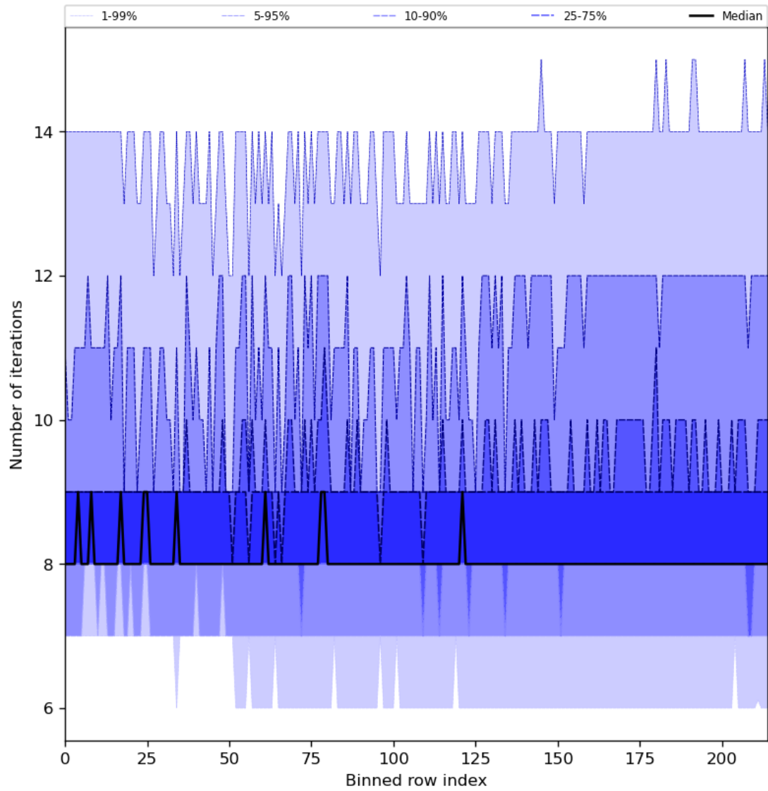
Figure 32: Along track statistics of “Number of iterations” for 2023-11-13 to 2023-11-15
