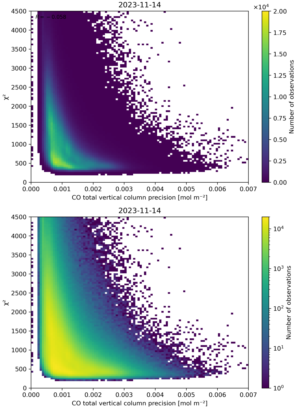
Figure 44: Scatter density plot of “CO total vertical column precision” against “ \chi^2 ” for 2023-11-13 to 2023-11-15.
