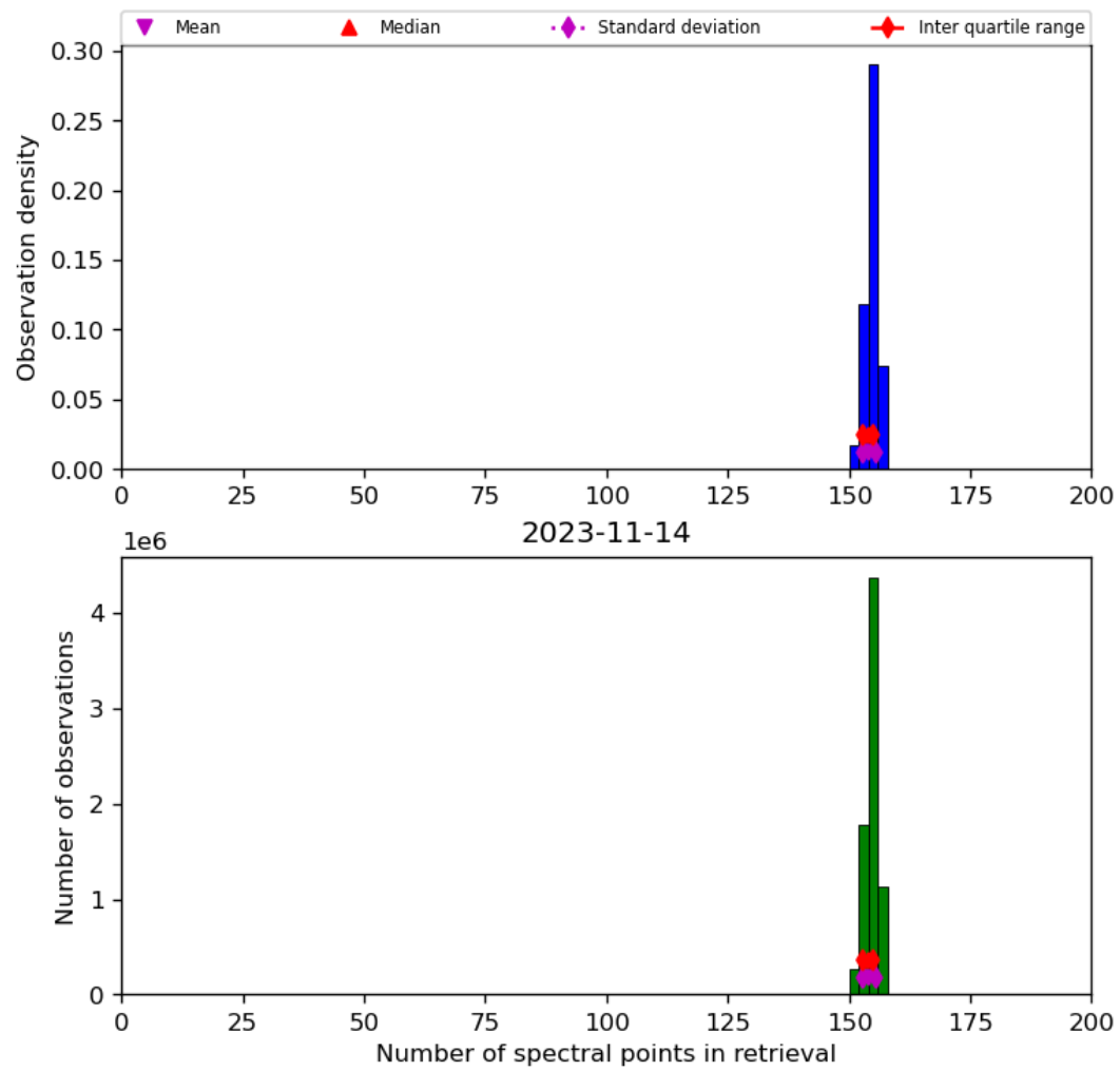
Figure 21: Histogram of “Number of spectral points in retrieval” for 2023-11-13 to 2023-11-15
