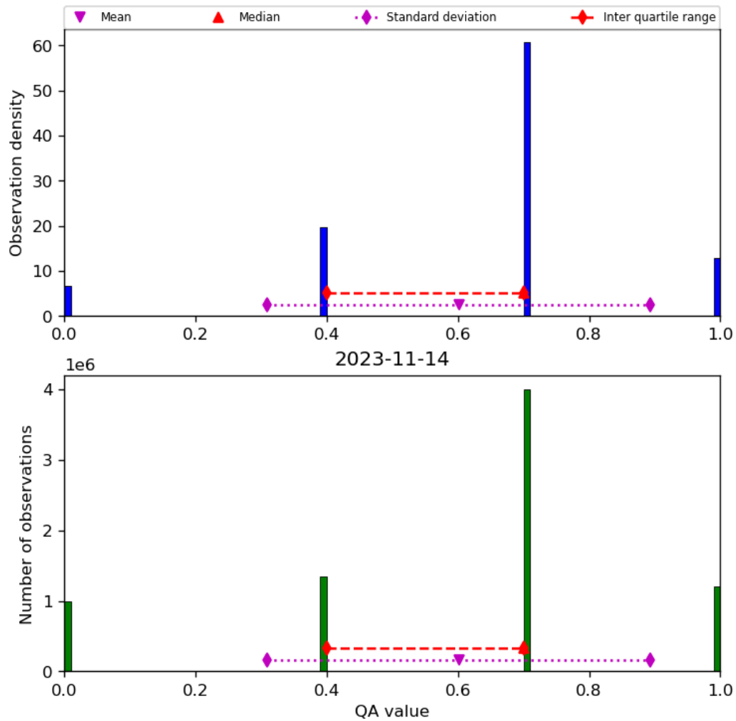
Figure 17: Histogram of “QA value” for 2023-11-13 to 2023-11-15
