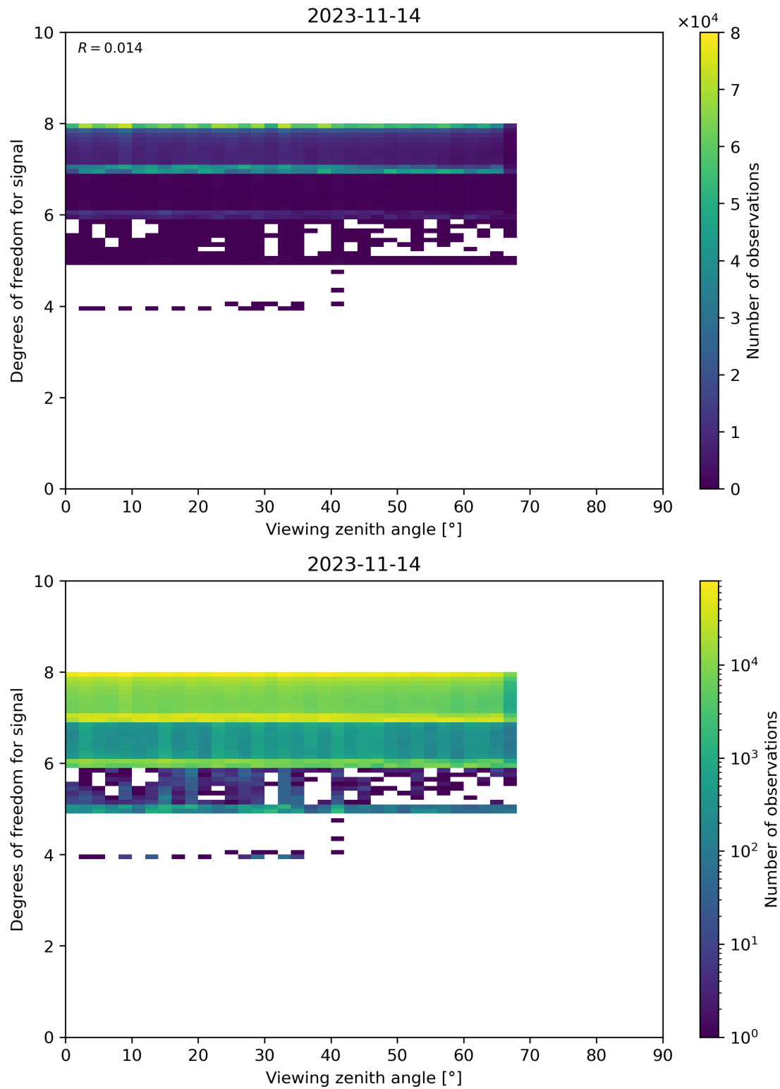
Figure 73: Scatter density plot of “Viewing zenith angle” against “Degrees of freedom for signal” for 2023-11-13 to 2023-11-15.
