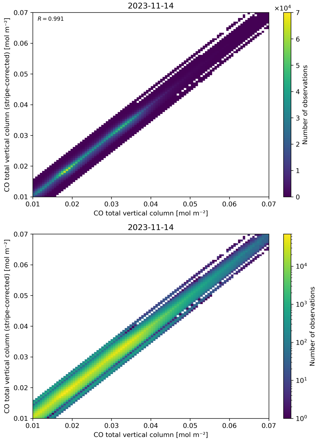
Figure 33: Scatter density plot of “CO total vertical column” against “CO total vertical column (stripe-corrected)” for 2023-11-13 to 2023-11-15.
