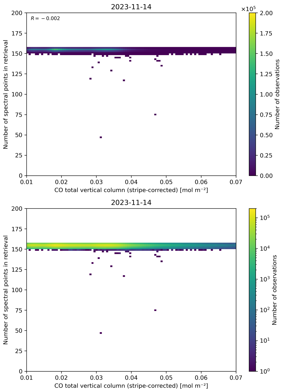
Figure 40: Scatter density plot of “CO total vertical column (stripe-corrected)” against “Number of spectral points in retrieval” for 2023-11-13 to 2023-11-15.
