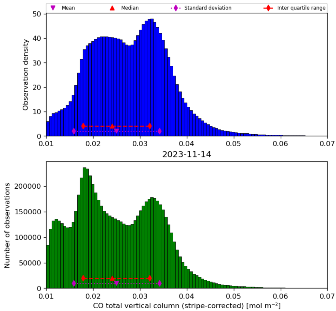
Figure 19: Histogram of “CO total vertical column (stripe-corrected)” for 2023-11-13 to 2023-11-15
