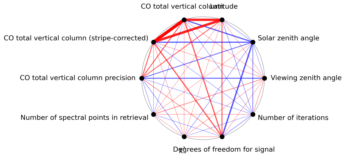
Figure 1: Map of correlation graph for 2023-11-13 to 2023-11-15.
