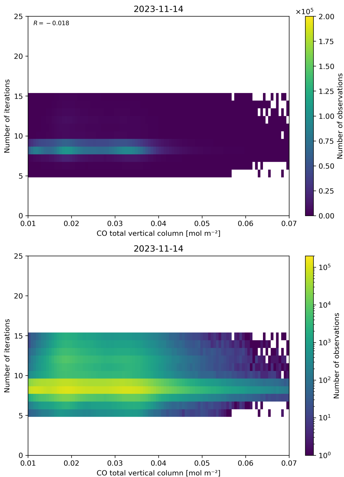
Figure 42: Scatter density plot of “CO total vertical column” against “Number of iterations” for 2023-11-13 to 2023-11-15.
