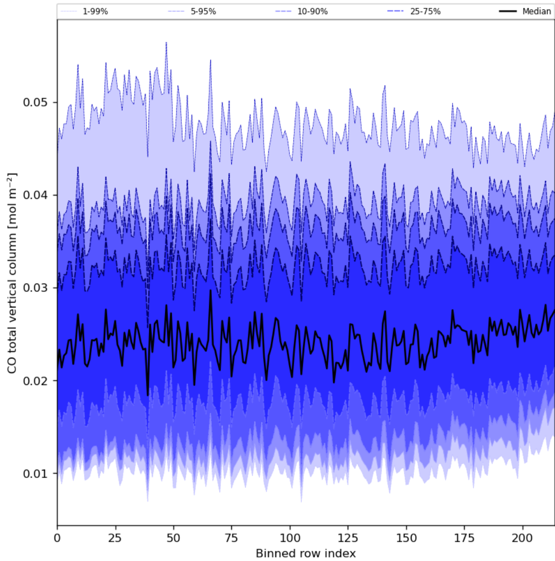
Figure 26: Along track statistics of “CO total vertical column” for 2023-11-13 to 2023-11-15
