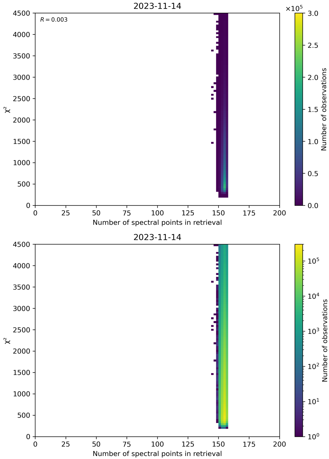
Figure 58: Scatter density plot of “Number of spectral points in retrieval” against “ \chi^2 ” for 2023-11-13 to 2023-11-15.
