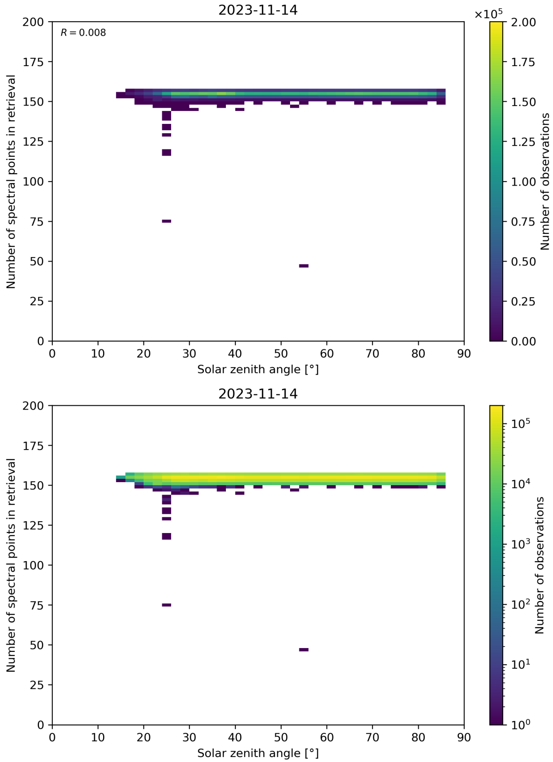
Figure 68: Scatter density plot of “Solar zenith angle” against “Number of spectral points in retrieval” for 2023-11-13 to 2023-11-15.
