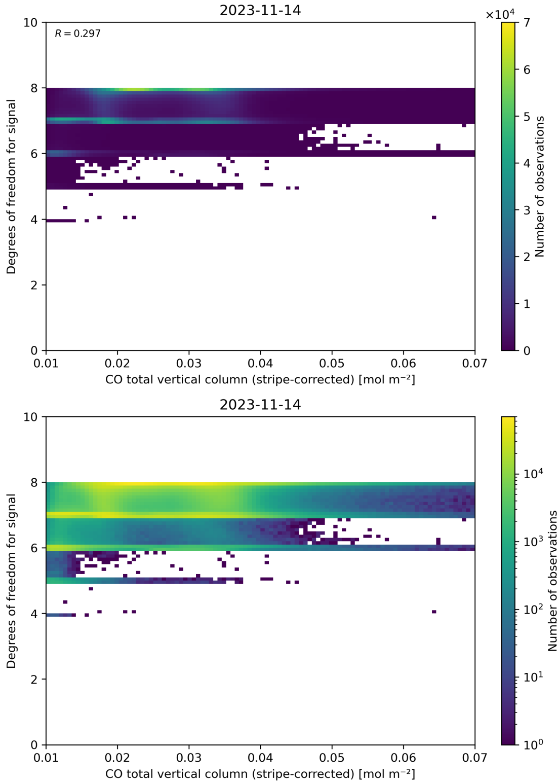
Figure 38: Scatter density plot of “CO total vertical column (stripe-corrected)” against “Degrees of freedom for signal” for 2023-11-13 to 2023-11-15.
