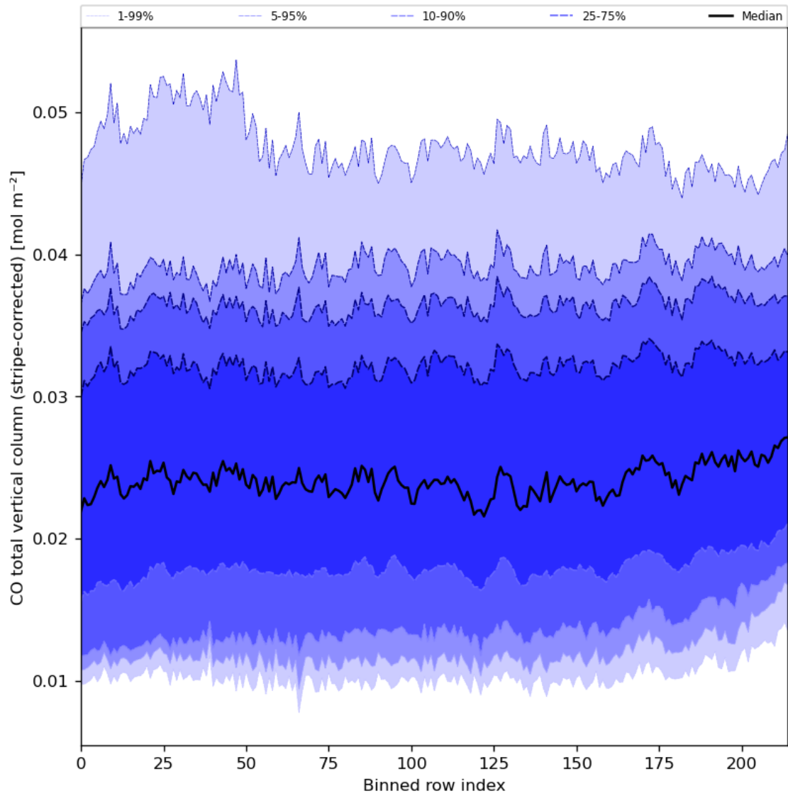
Figure 27: Along track statistics of “CO total vertical column (stripe-corrected)” for 2023-11-13 to 2023-11-15
