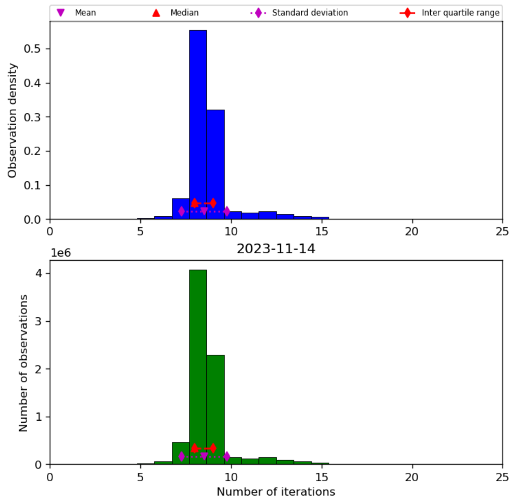
Figure 24: Histogram of “Number of iterations” for 2023-11-13 to 2023-11-15
