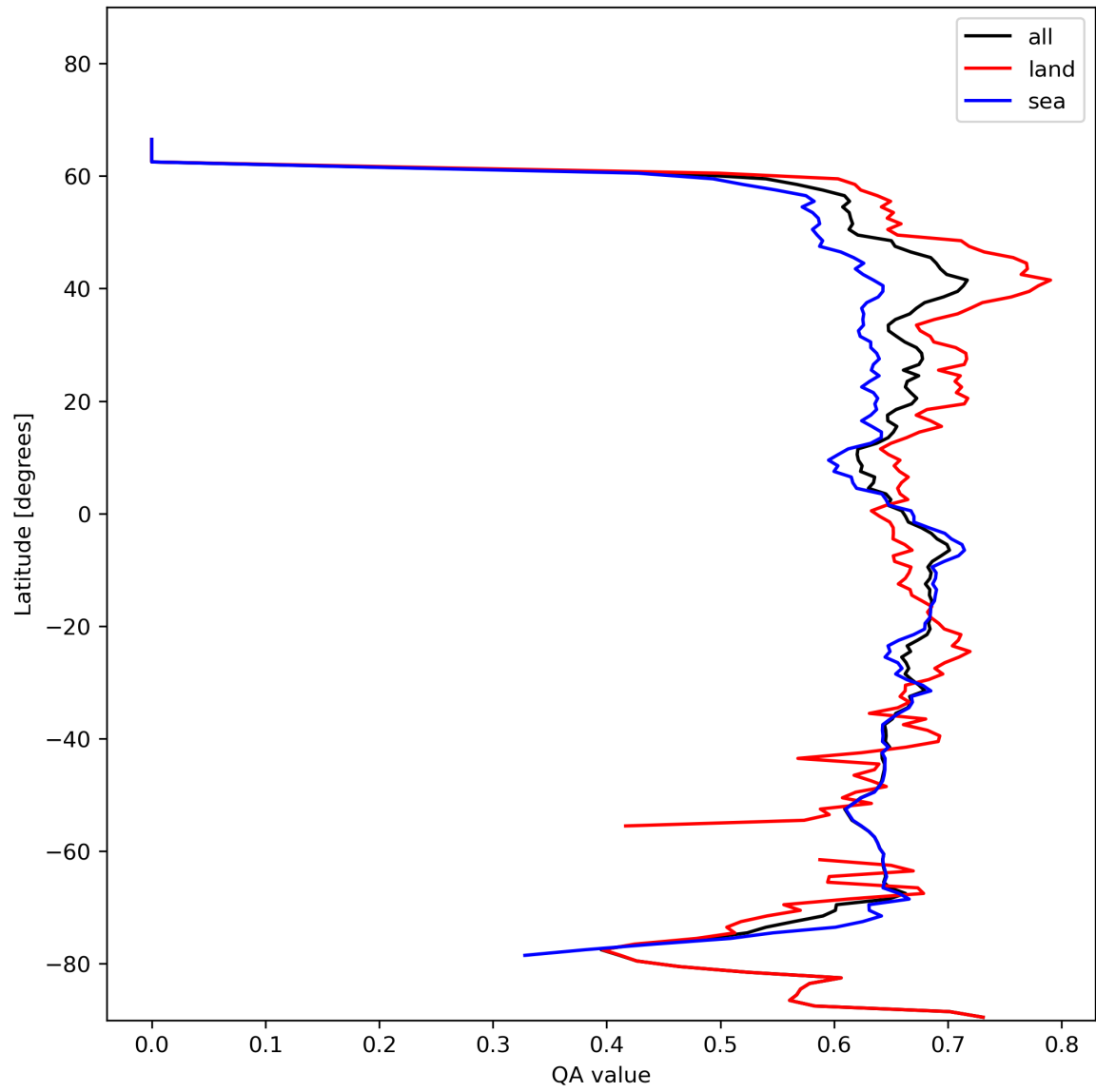
Figure 9: Zonal average of “QA value” for 2023-11-13 to 2023-11-15.
