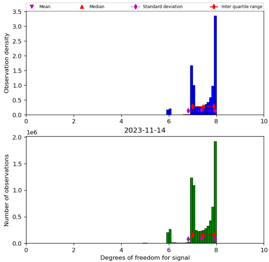
Figure 23: Histogram of “Degrees of freedom for signal” for 2023-11-13 to 2023-11-15
