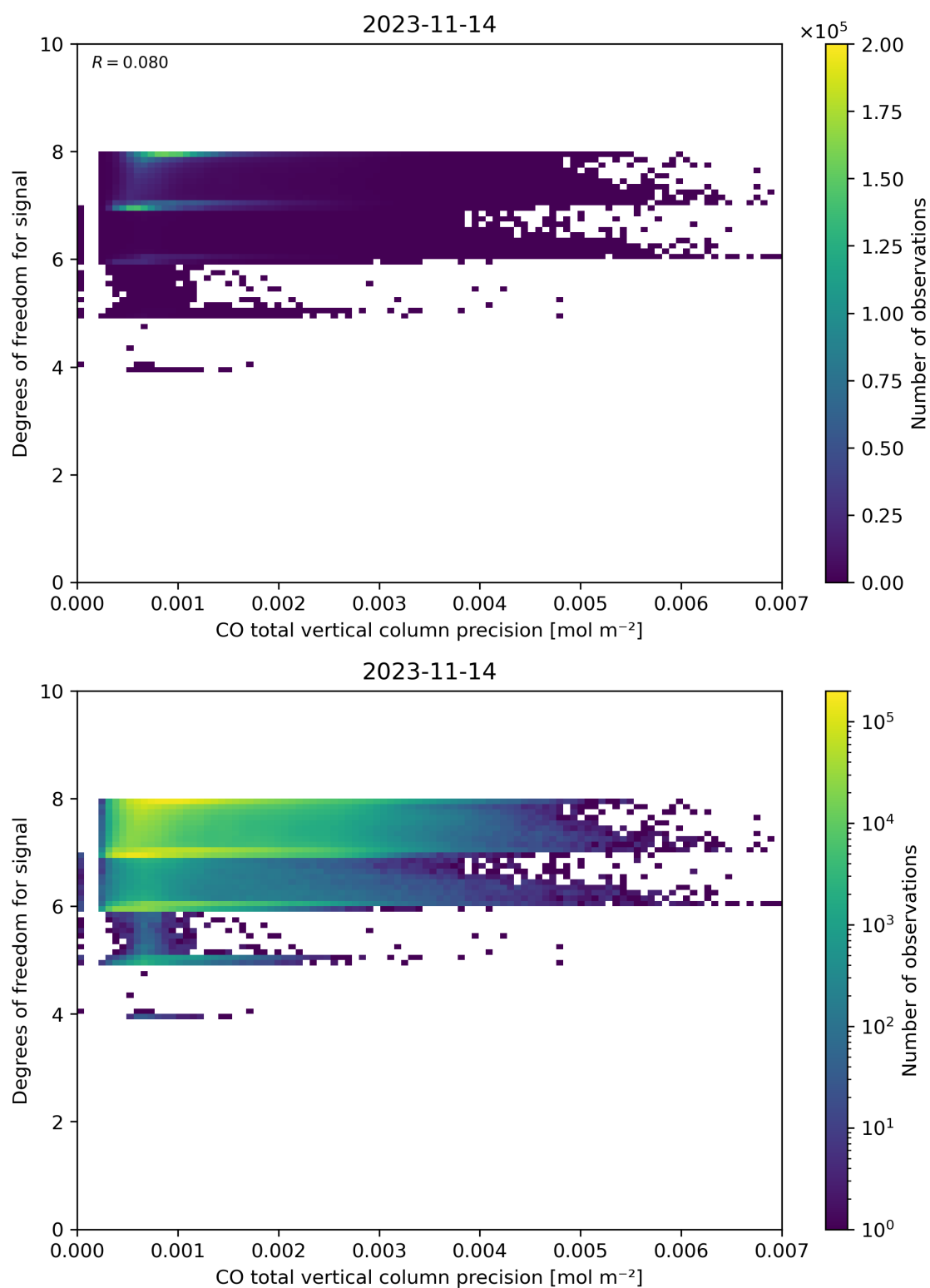
Figure 45: Scatter density plot of “CO total vertical column precision” against “Degrees of freedom for signal” for 2023-11-13 to 2023-11-15.
