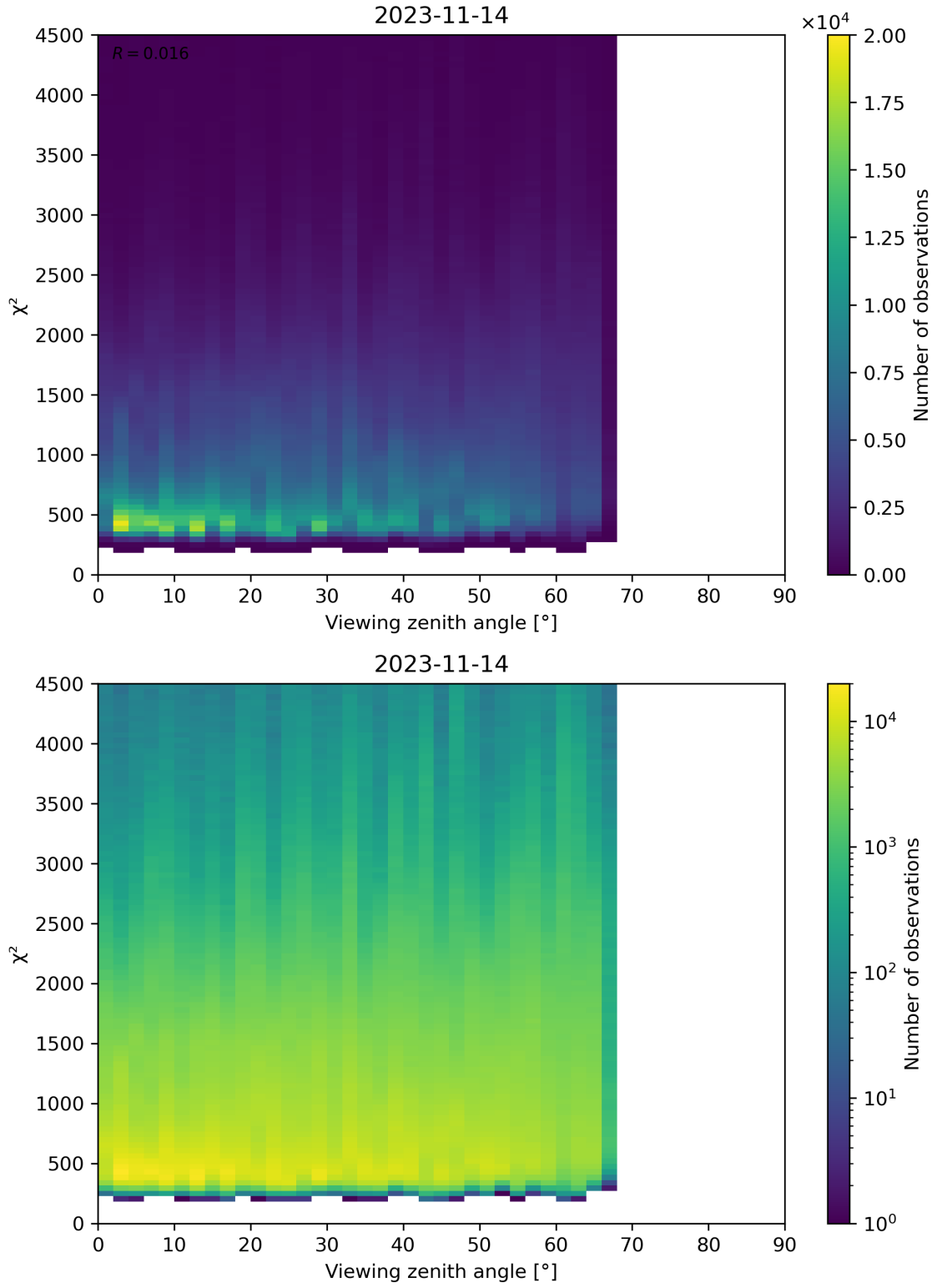
Figure 72: Scatter density plot of “Viewing zenith angle” against “ \chi^2 ” for 2023-11-13 to 2023-11-15.
