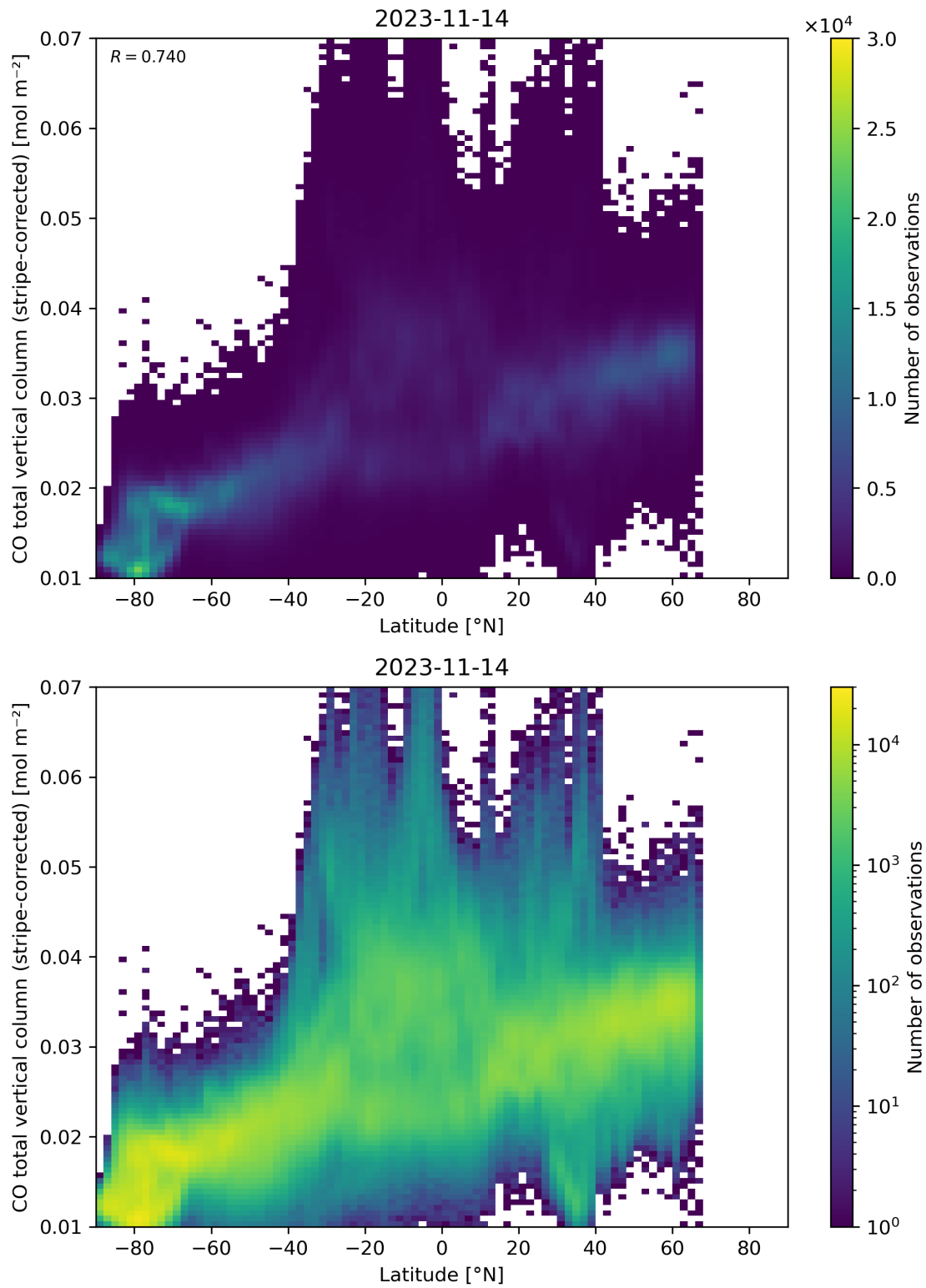
Figure 52: Scatter density plot of “Latitude” against “CO total vertical column (stripe-corrected)” for 2023-11-13 to 2023-11-15.
