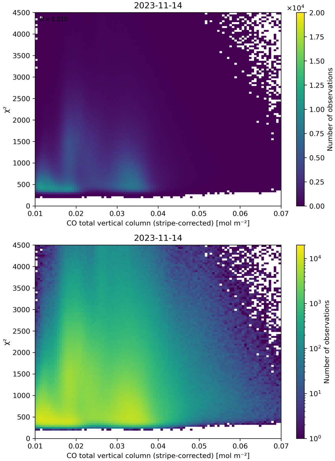
Figure 37: Scatter density plot of “CO total vertical column (stripe-corrected)” against “ \chi^2 ” for 2023-11-13 to 2023-11-15.
