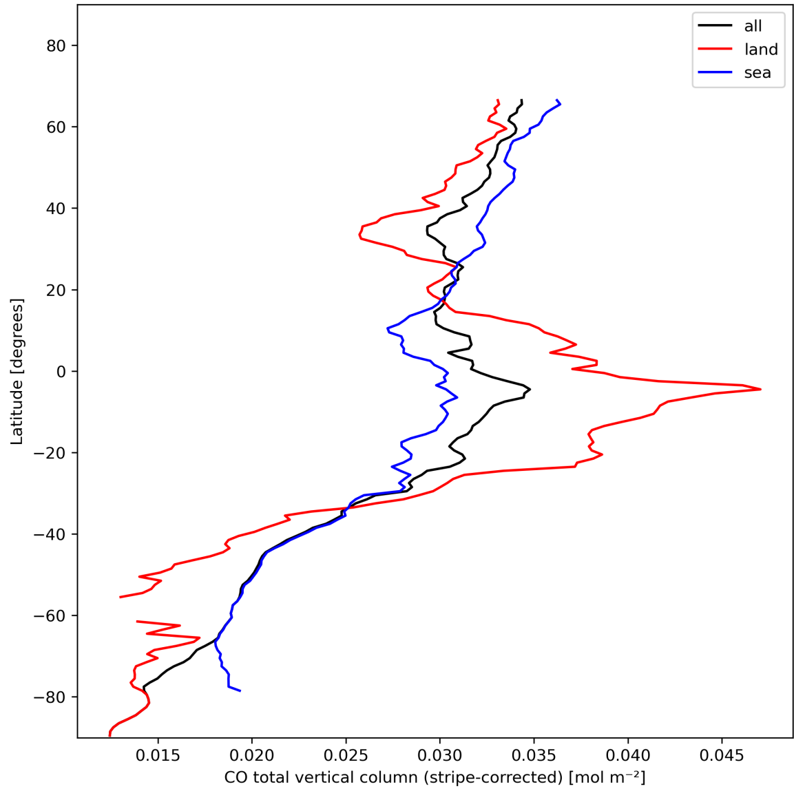
Figure 11: Zonal average of “CO total vertical column (stripe-corrected)” for 2023-11-13 to 2023-11-15.
