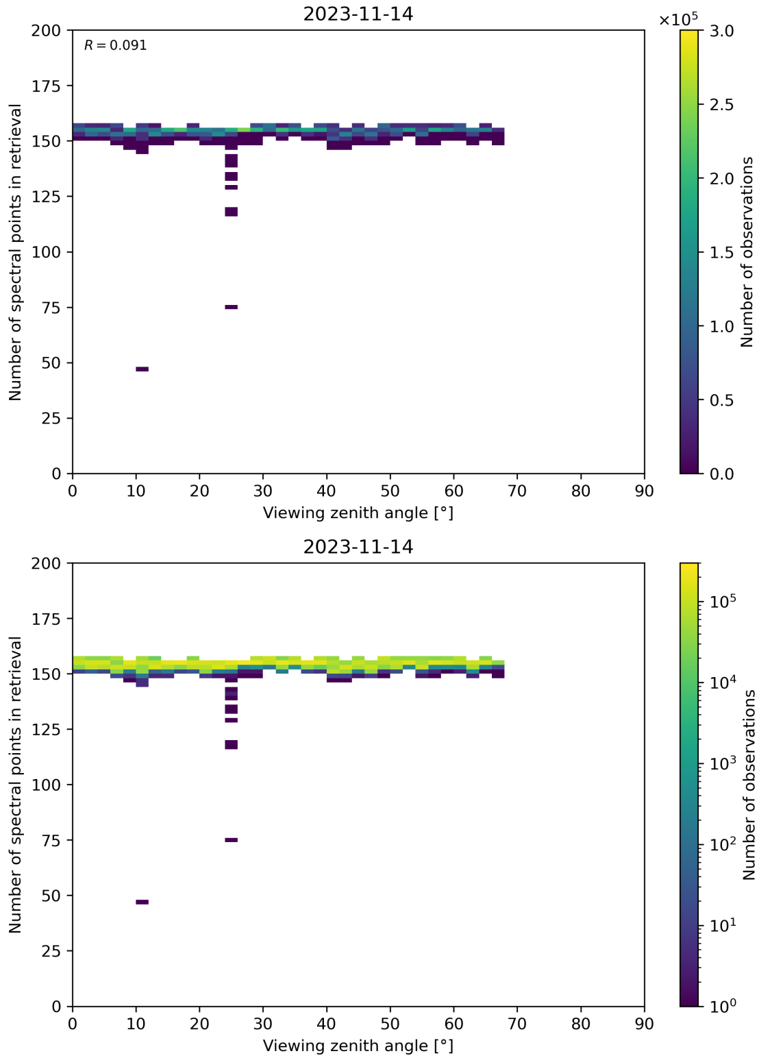
Figure 76: Scatter density plot of “Viewing zenith angle” against “Number of spectral points in retrieval” for 2023-11-13 to 2023-11-15.
