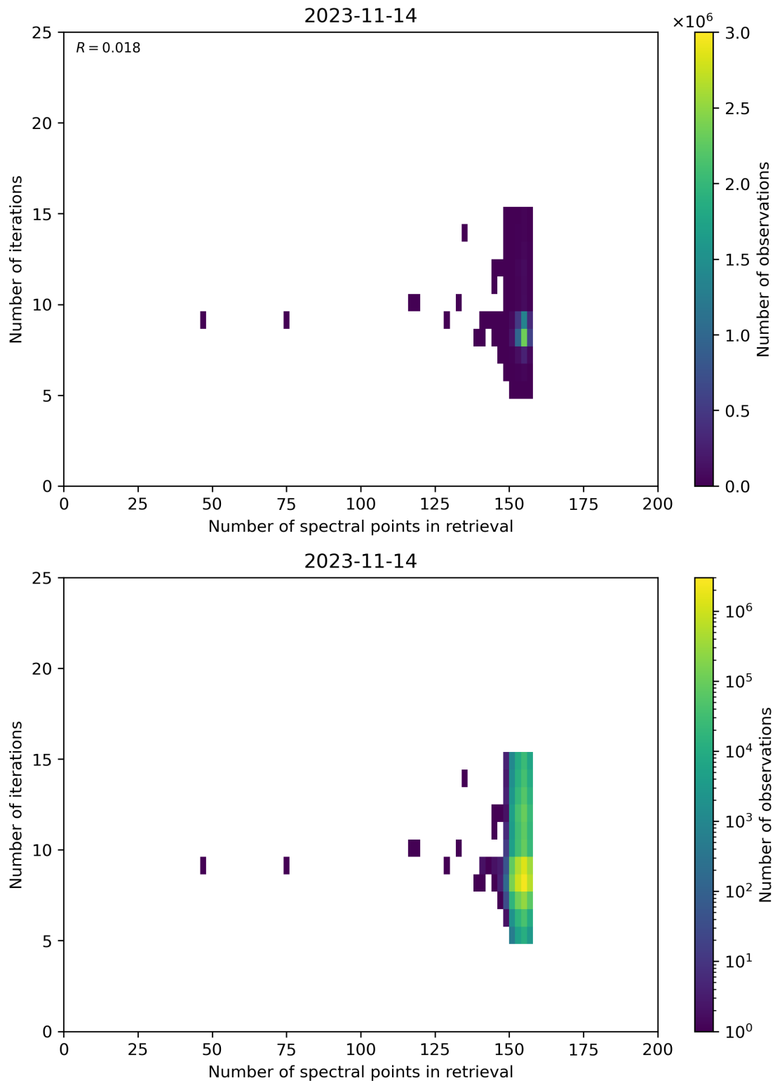
Figure 60: Scatter density plot of “Number of spectral points in retrieval” against “Number of iterations” for 2023-11-13 to 2023-11-15.
