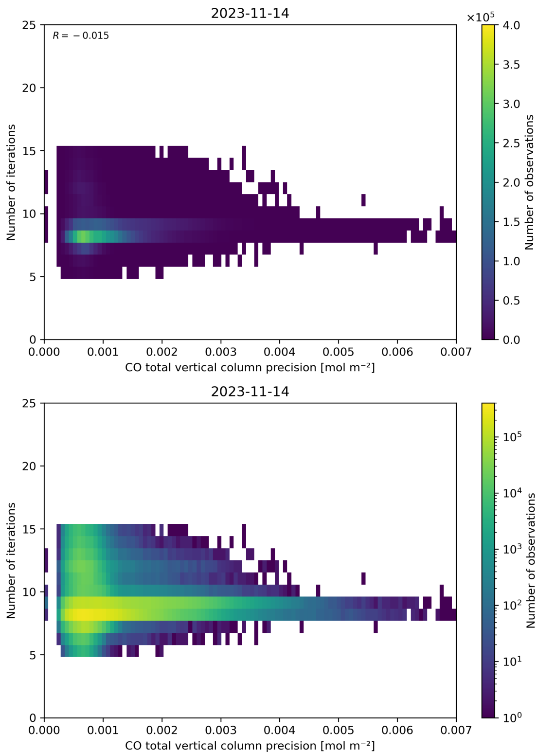
Figure 46: Scatter density plot of “CO total vertical column precision” against “Number of iterations” for 2023-11-13 to 2023-11-15.
