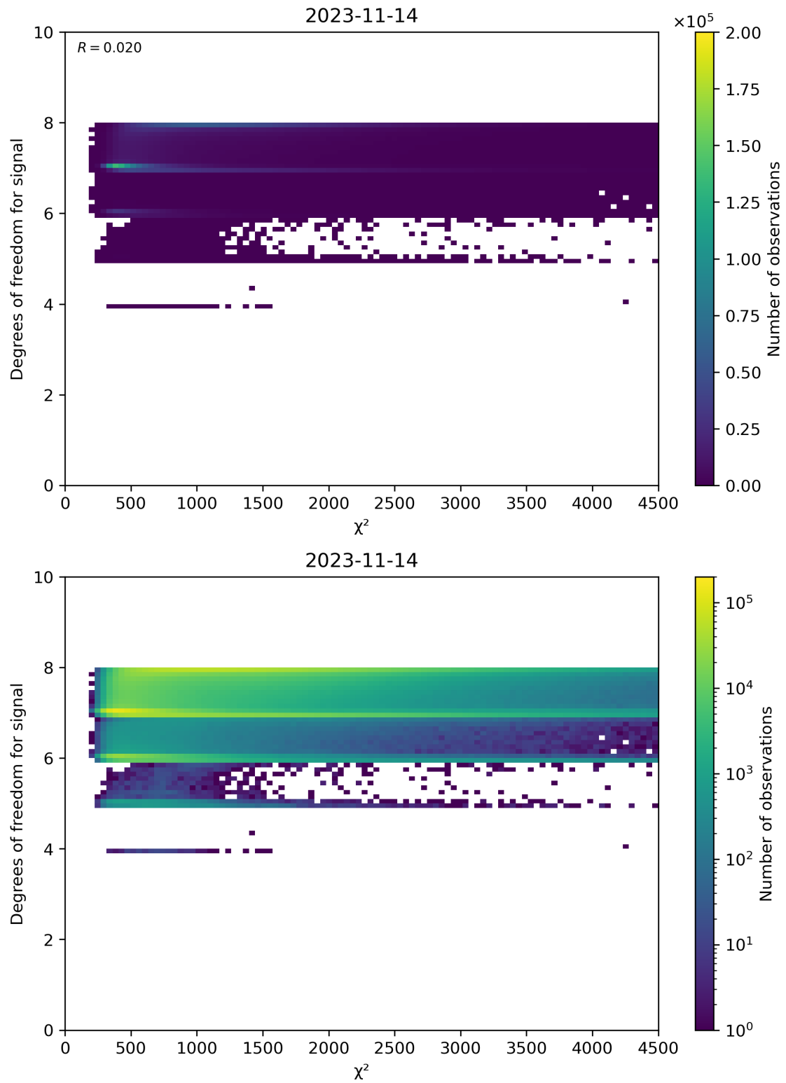
Figure 48: Scatter density plot of “ \chi^2 ” against “Degrees of freedom for signal” for 2023-11-13 to 2023-11-15.
