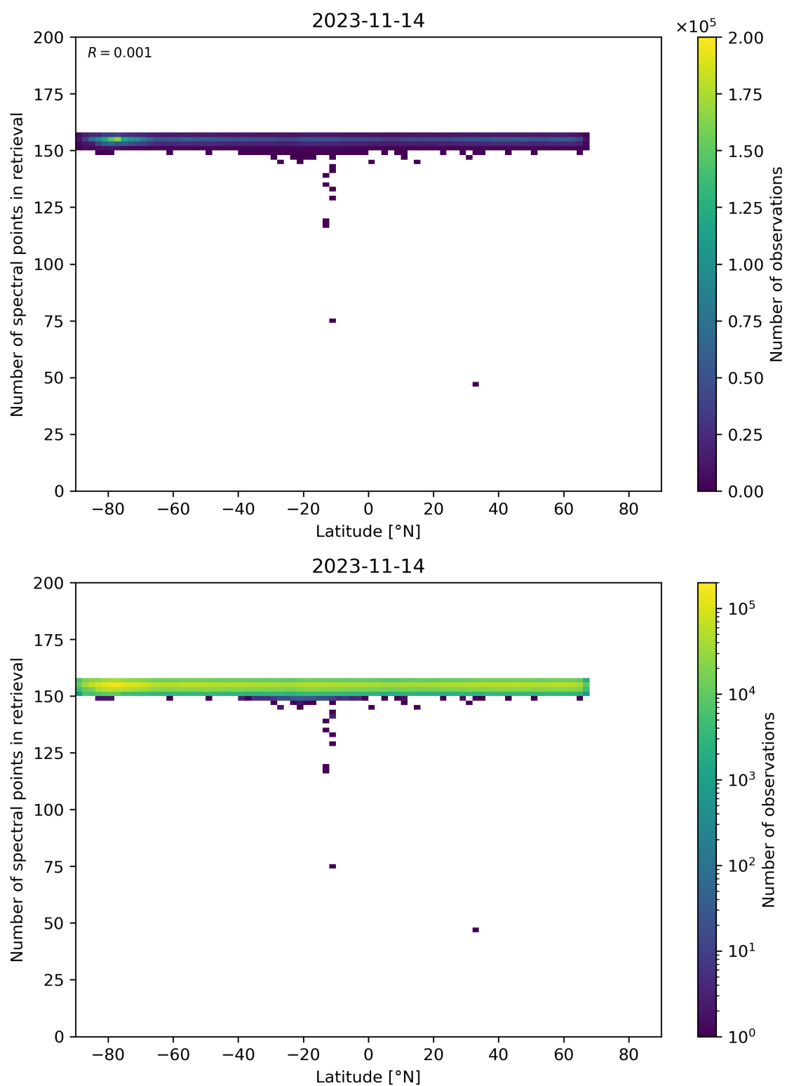
Figure 57: Scatter density plot of “Latitude” against “Number of spectral points in retrieval” for 2023-11-13 to 2023-11-15.
