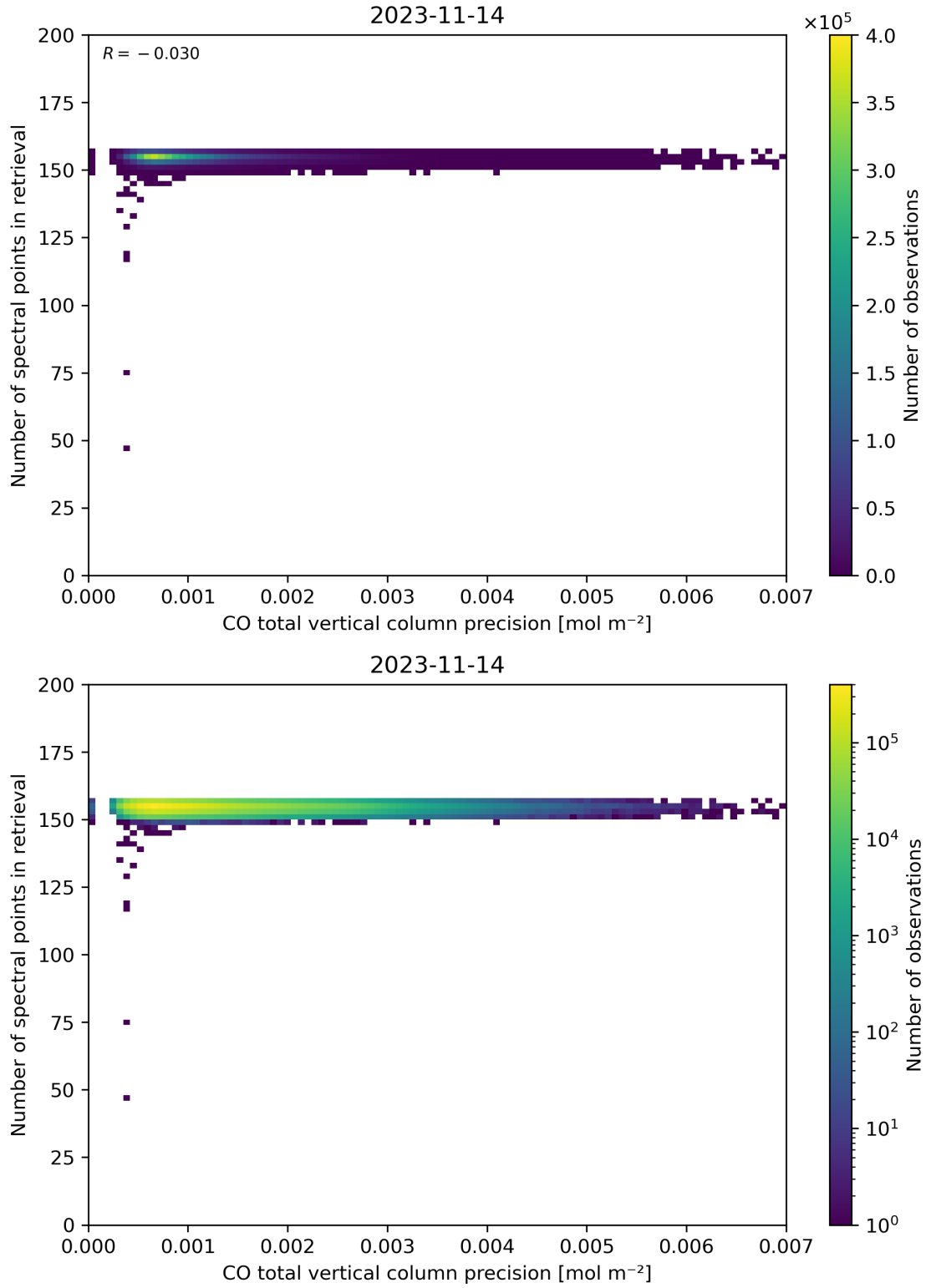
Figure 47: Scatter density plot of “CO total vertical column precision” against “Number of spectral points in retrieval” for 2023-11-13 to 2023-11-15.
