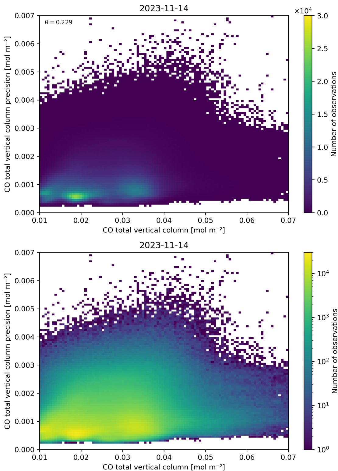
Figure 34: Scatter density plot of “CO total vertical column” against “CO total vertical column precision” for 2023-11-13 to 2023-11-15.
