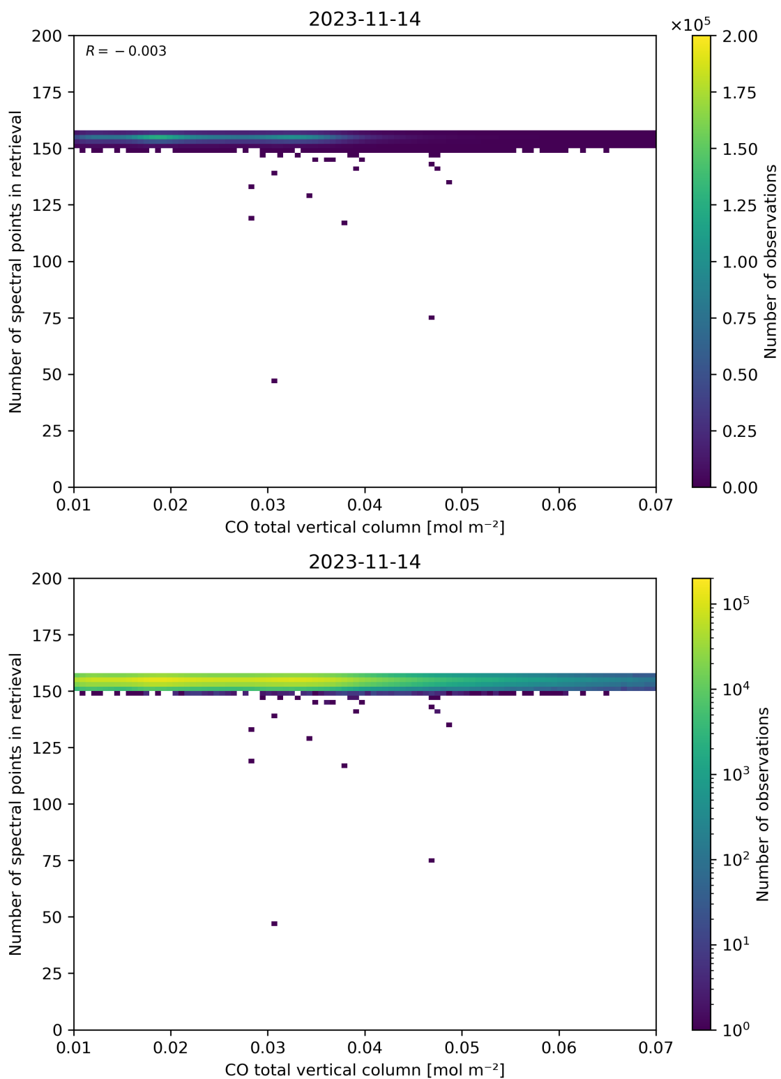
Figure 43: Scatter density plot of “CO total vertical column” against “Number of spectral points in retrieval” for 2023-11-13 to 2023-11-15.
