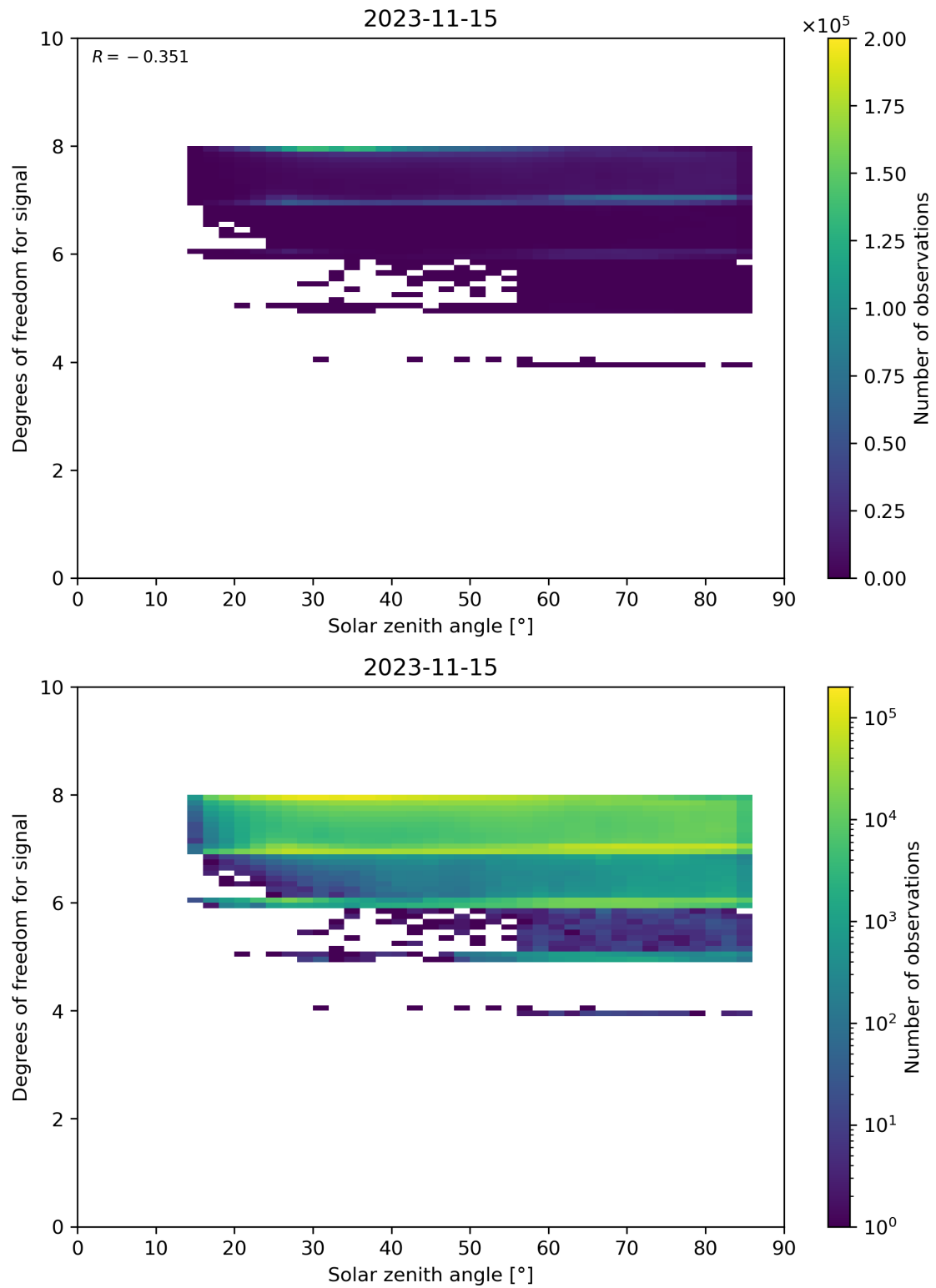
Figure 65: Scatter density plot of “Solar zenith angle” against “Degrees of freedom for signal” for 2023-11-14 to 2023-11-16.
