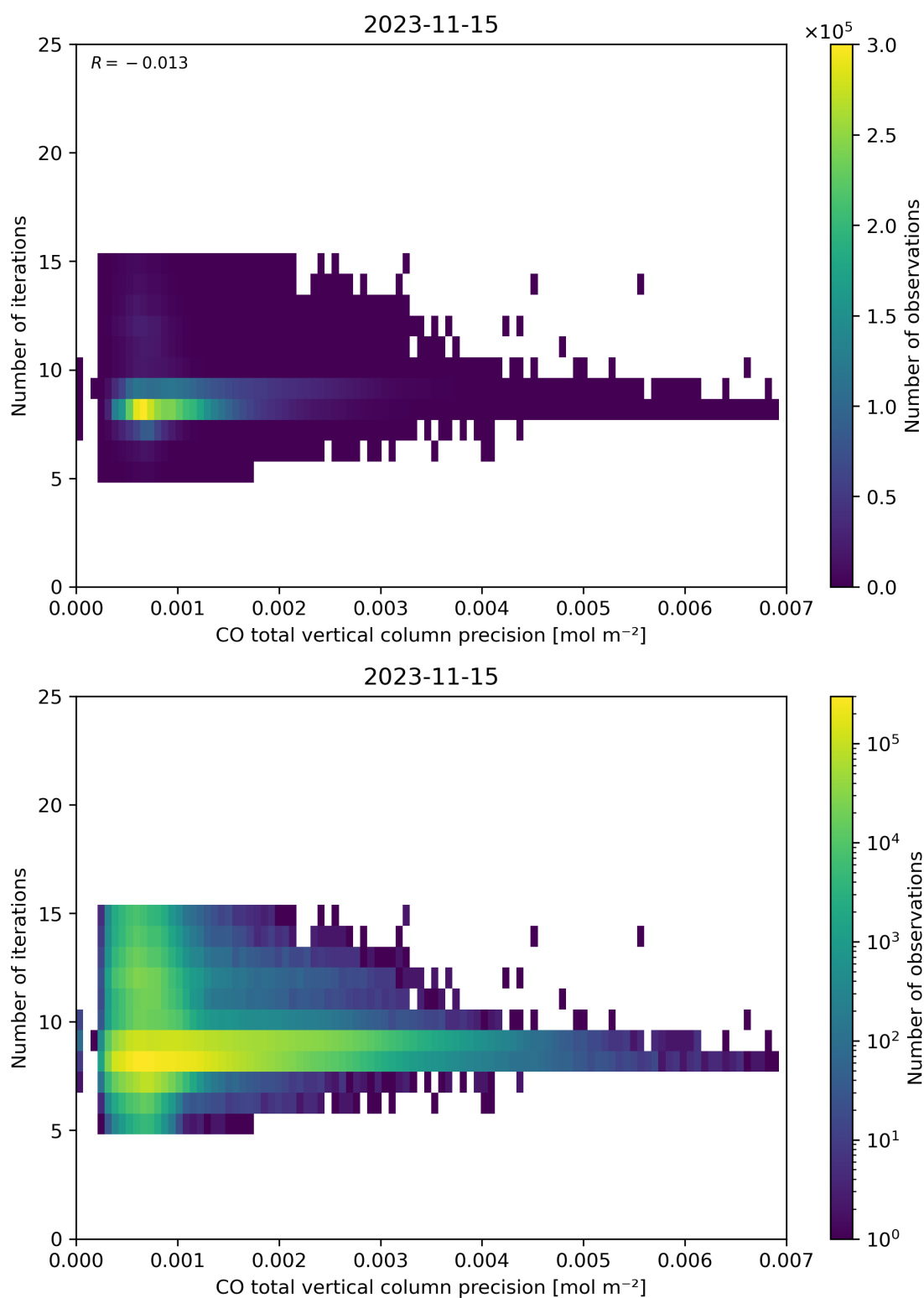
Figure 46: Scatter density plot of “CO total vertical column precision” against “Number of iterations” for 2023-11-14 to 2023-11-16.
