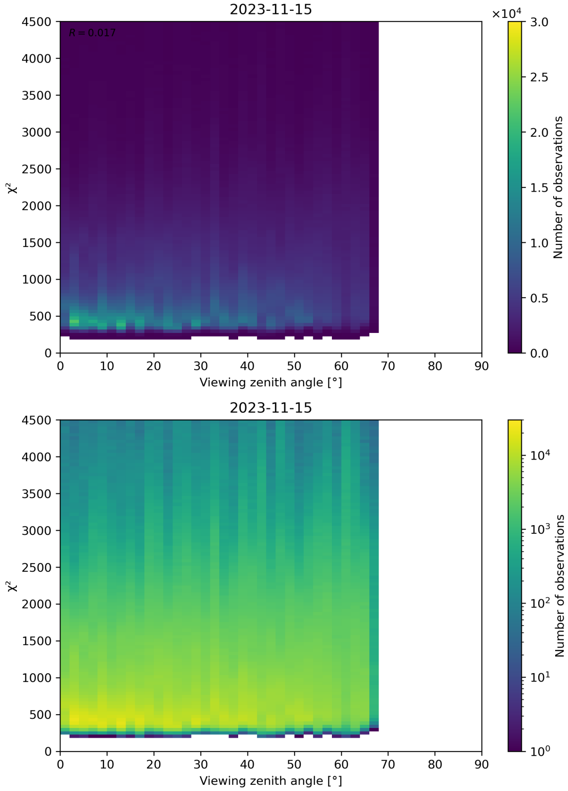
Figure 72: Scatter density plot of “Viewing zenith angle” against “ \chi^2 ” for 2023-11-14 to 2023-11-16.
