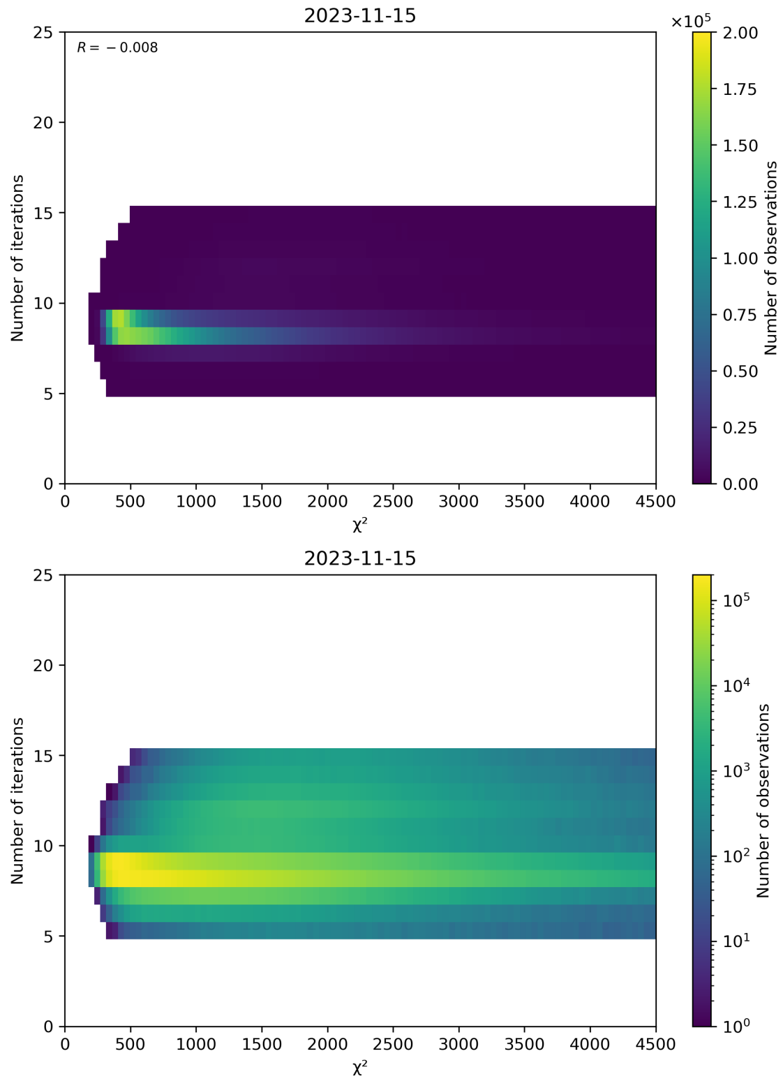
Figure 49: Scatter density plot of “ \chi^2 ” against “Number of iterations” for 2023-11-14 to 2023-11-16.
