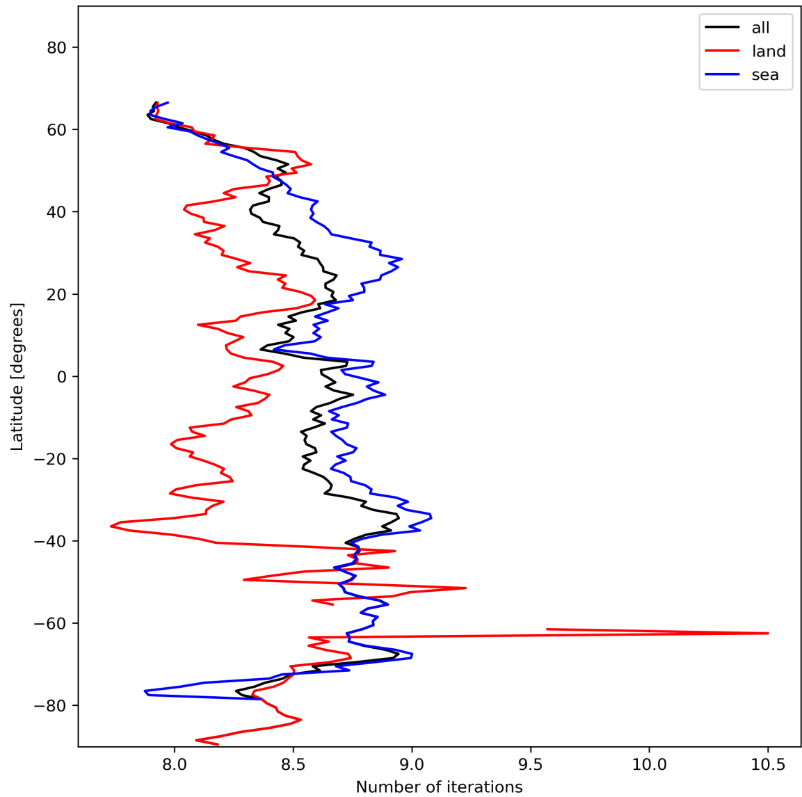
Figure 16: Zonal average of “Number of iterations” for 2023-11-14 to 2023-11-16.
