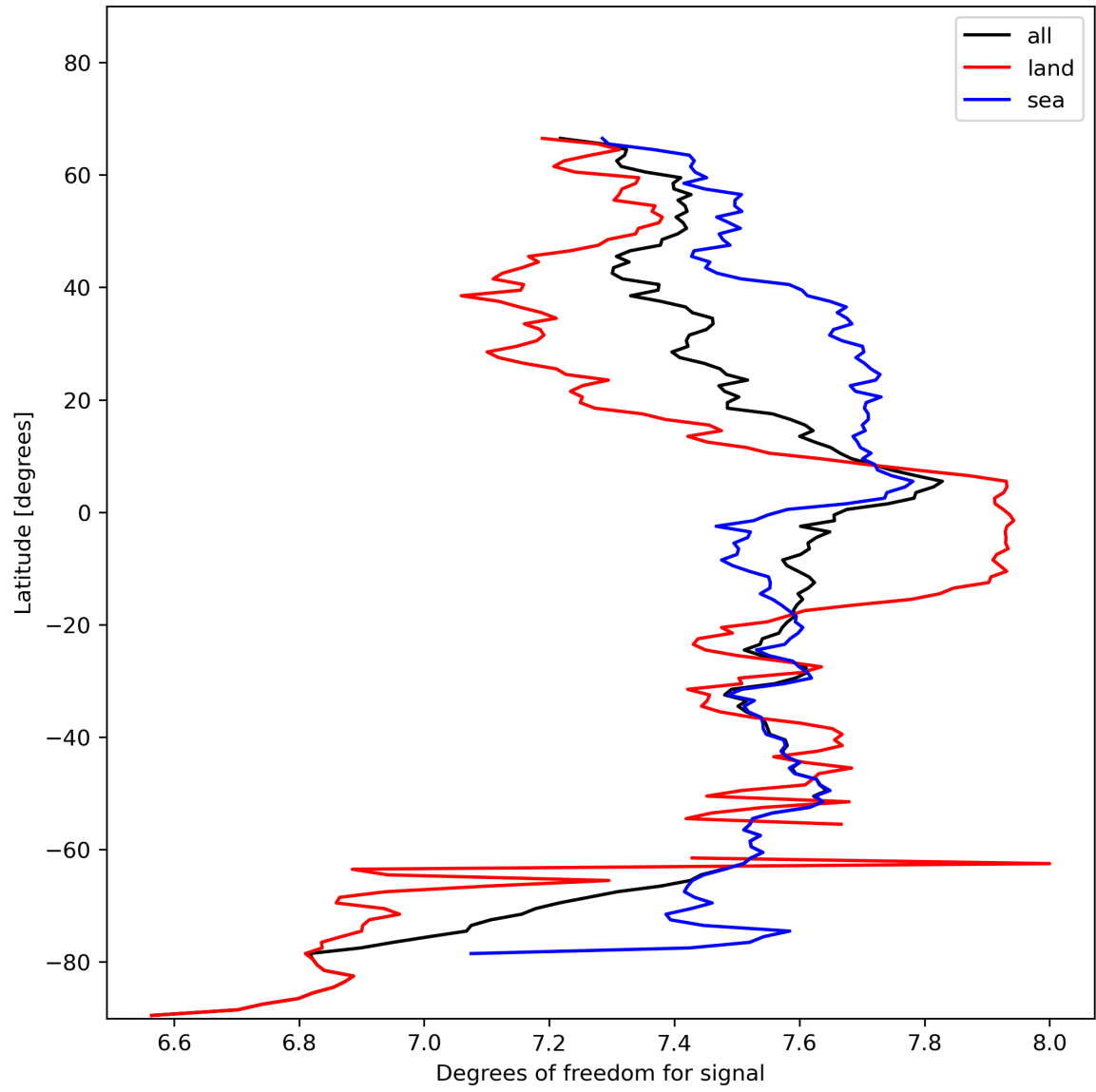
Figure 15: Zonal average of “Degrees of freedom for signal” for 2023-11-14 to 2023-11-16.
