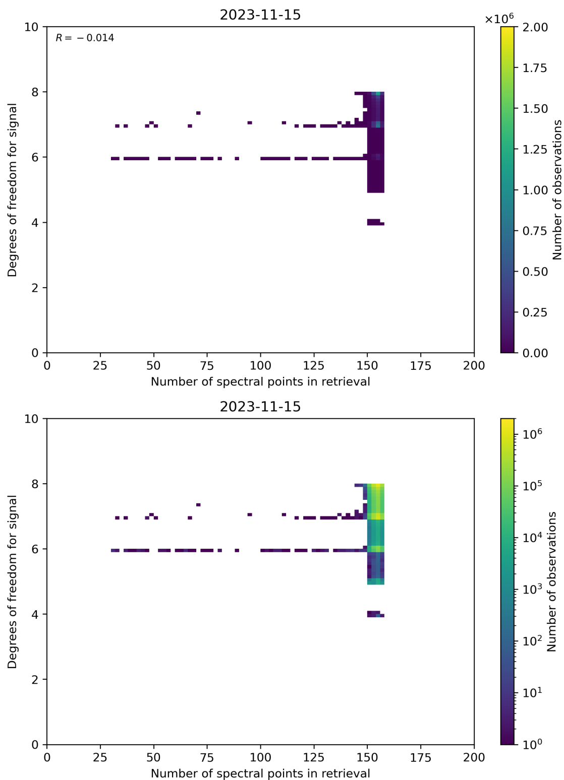
Figure 59: Scatter density plot of “Number of spectral points in retrieval” against “Degrees of freedom for signal” for 2023-11-14 to 2023-11-16.
