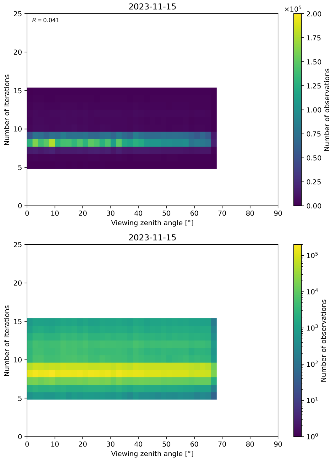
Figure 75: Scatter density plot of “Viewing zenith angle” against “Number of iterations” for 2023-11-14 to 2023-11-16.
