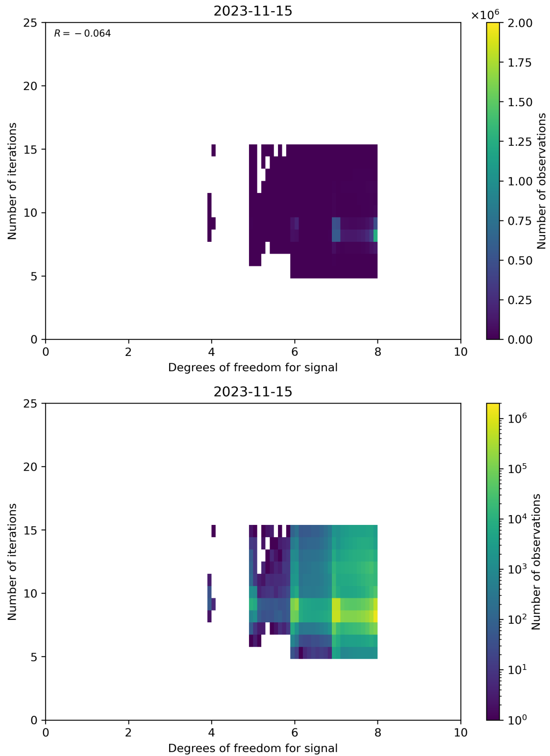
Figure 50: Scatter density plot of “Degrees of freedom for signal” against “Number of iterations” for 2023-11-14 to 2023-11-16.
