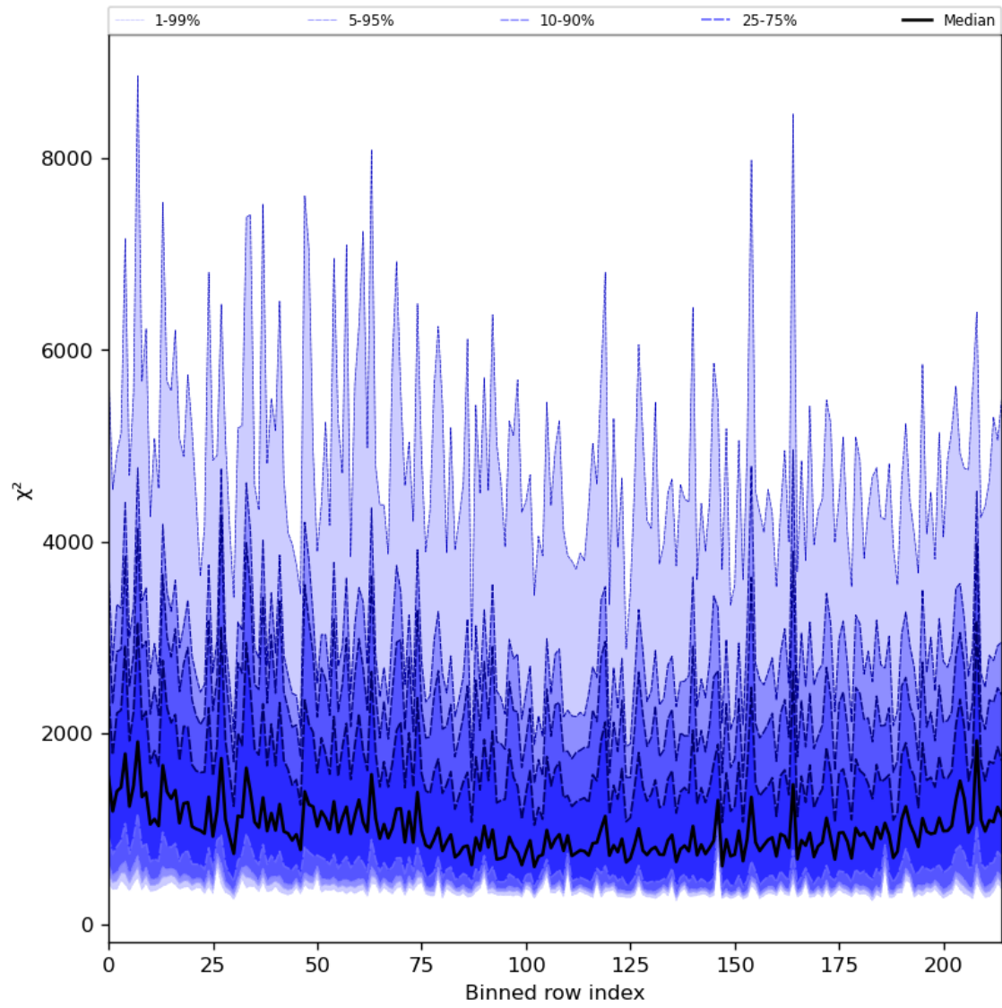
Figure 30: Along track statistics of “ \chi^2 ” for 2023-11-14 to 2023-11-16
