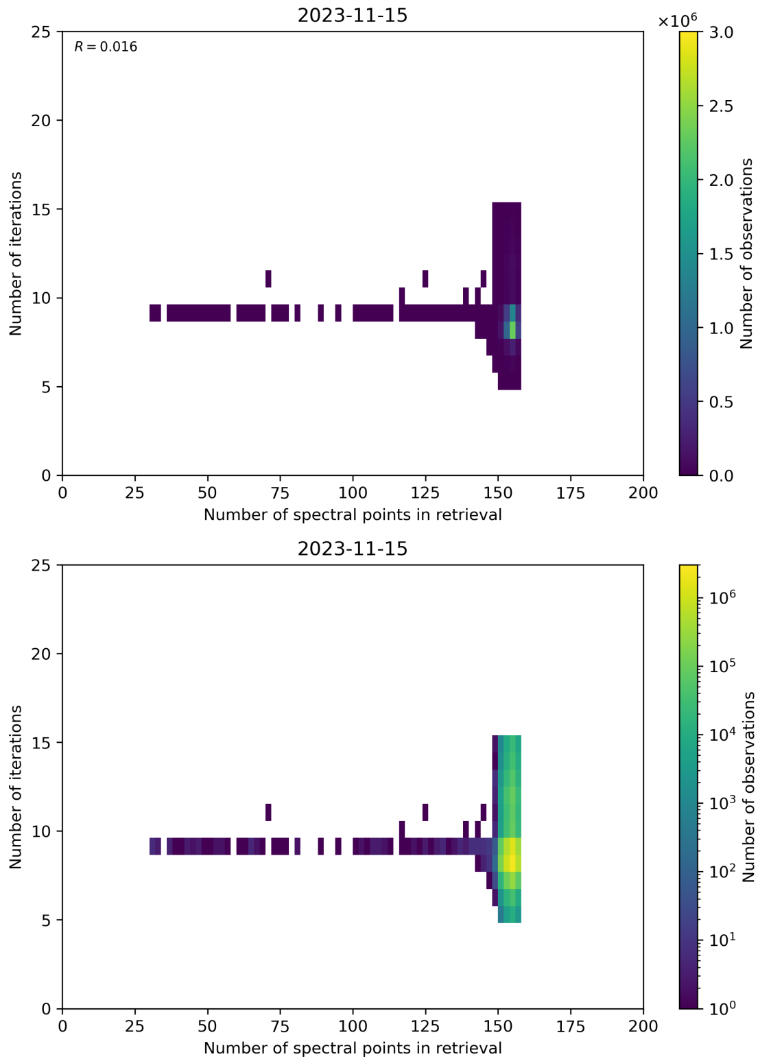
Figure 60: Scatter density plot of “Number of spectral points in retrieval” against “Number of iterations” for 2023-11-14 to 2023-11-16.
