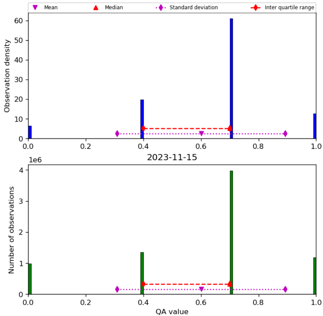
Figure 17: Histogram of “QA value” for 2023-11-14 to 2023-11-16
