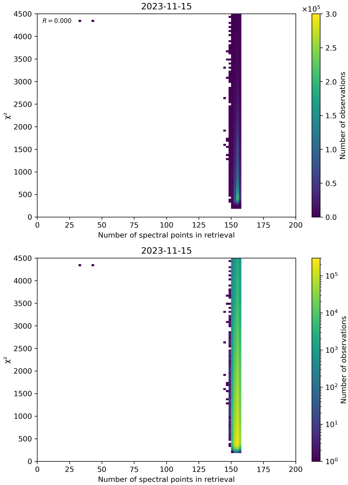
Figure 58: Scatter density plot of “Number of spectral points in retrieval” against “ \chi^2 ” for 2023-11-14 to 2023-11-16.
