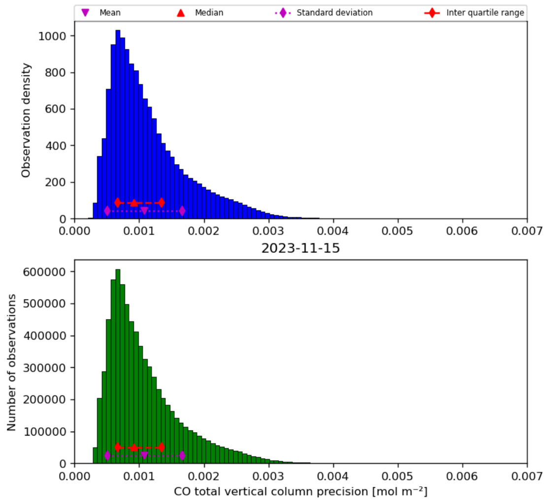
Figure 20: Histogram of “CO total vertical column precision” for 2023-11-14 to 2023-11-16
