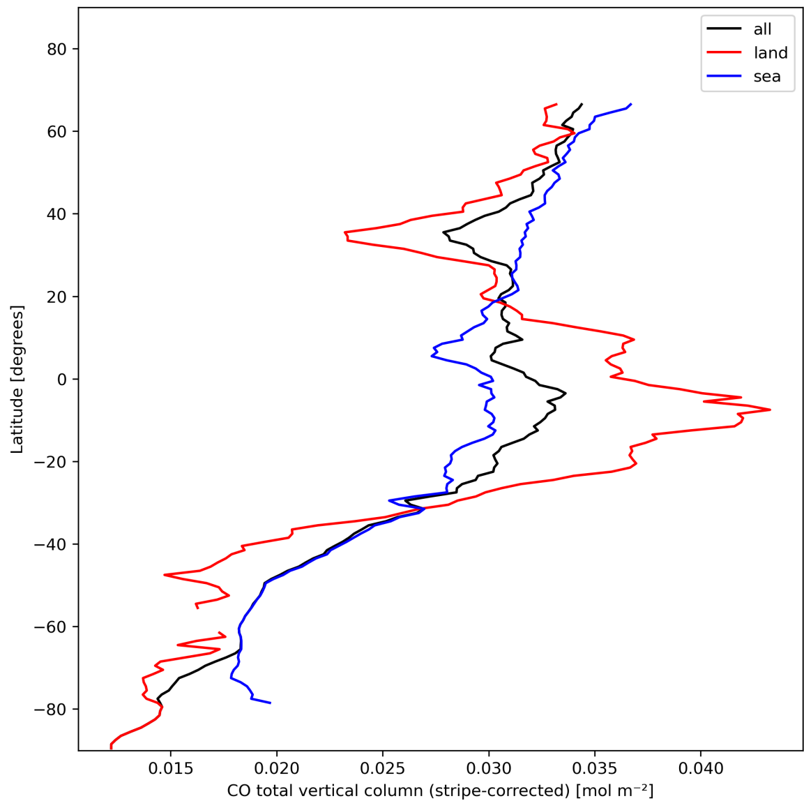
Figure 11: Zonal average of “CO total vertical column (stripe-corrected)” for 2023-11-14 to 2023-11-16.
