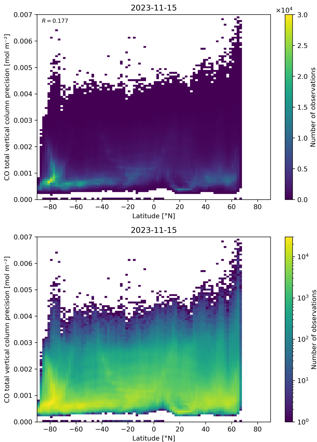
Figure 53: Scatter density plot of “Latitude” against “CO total vertical column precision” for 2023-11-14 to 2023-11-16.
