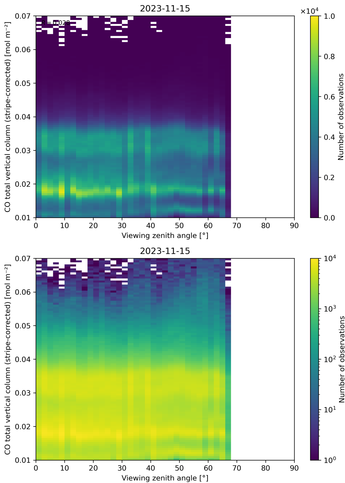
Figure 70: Scatter density plot of “Viewing zenith angle” against “CO total vertical column (stripe-corrected)” for 2023-11-14 to 2023-11-16.
