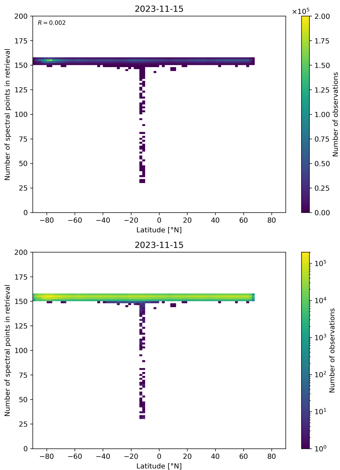
Figure 57: Scatter density plot of “Latitude” against “Number of spectral points in retrieval” for 2023-11-14 to 2023-11-16.
