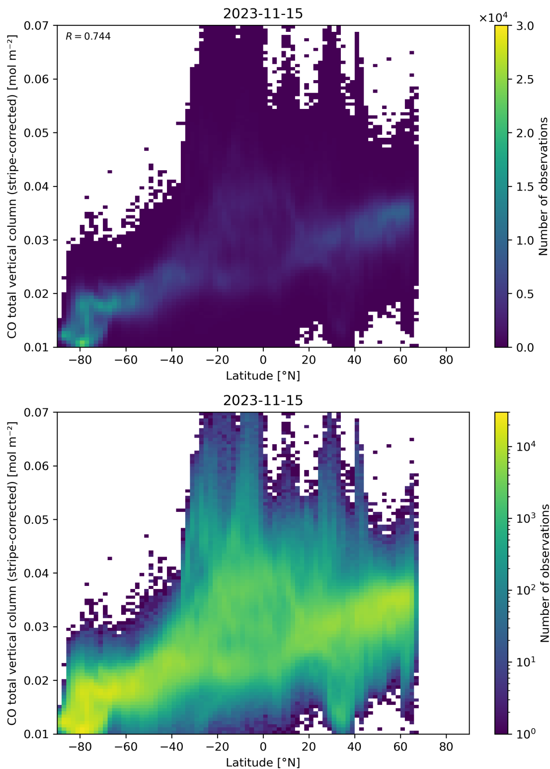
Figure 52: Scatter density plot of “Latitude” against “CO total vertical column (stripe-corrected)” for 2023-11-14 to 2023-11-16.
