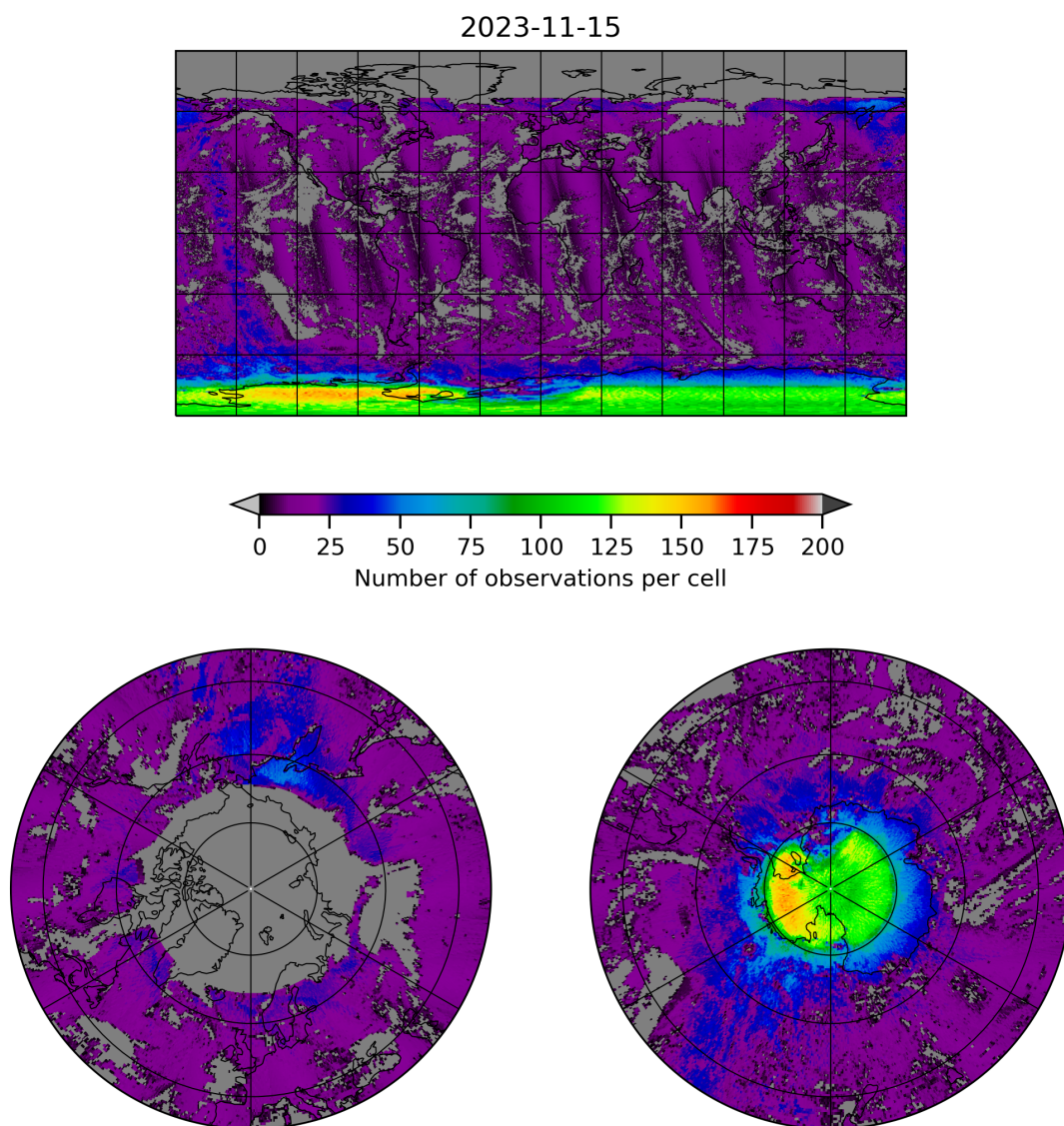
Figure 8: Map of the number of observations for 2023-11-14 to 2023-11-16
