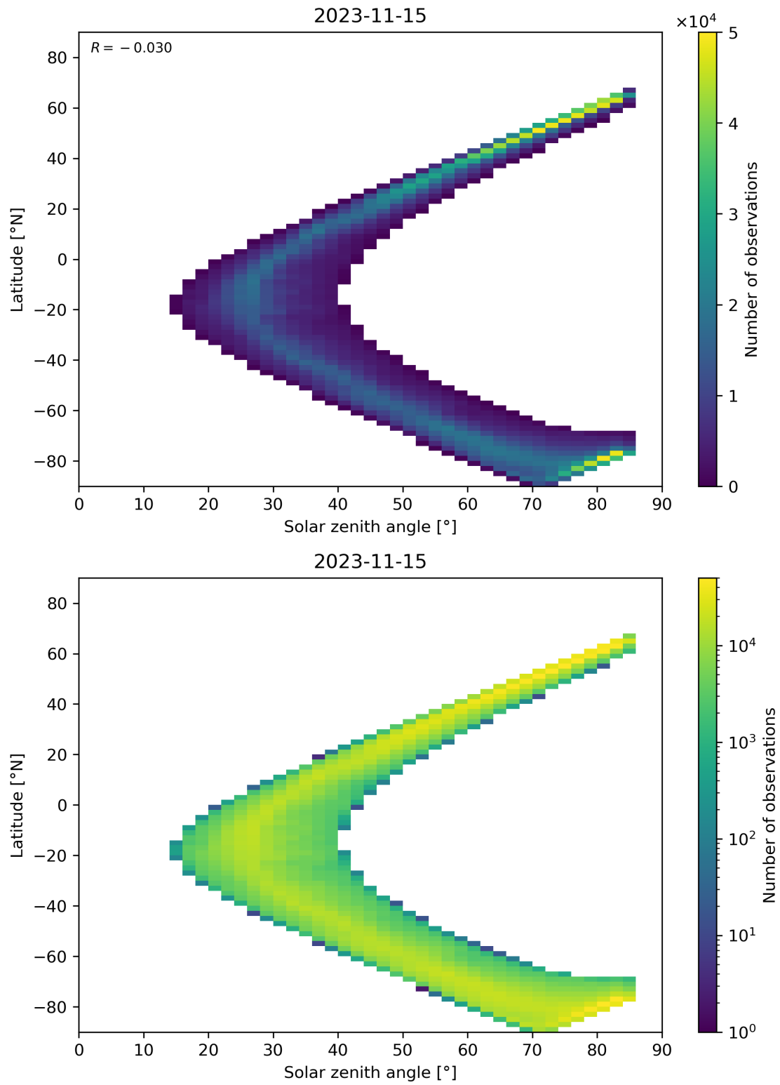
Figure 66: Scatter density plot of “Solar zenith angle” against “Latitude” for 2023-11-14 to 2023-11-16.
