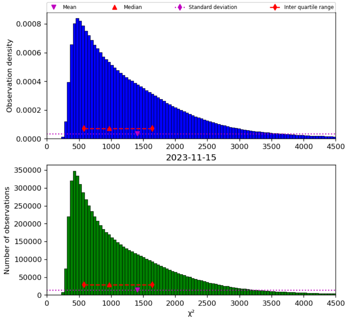
Figure 22: Histogram of “ \chi^2 ” for 2023-11-14 to 2023-11-16
