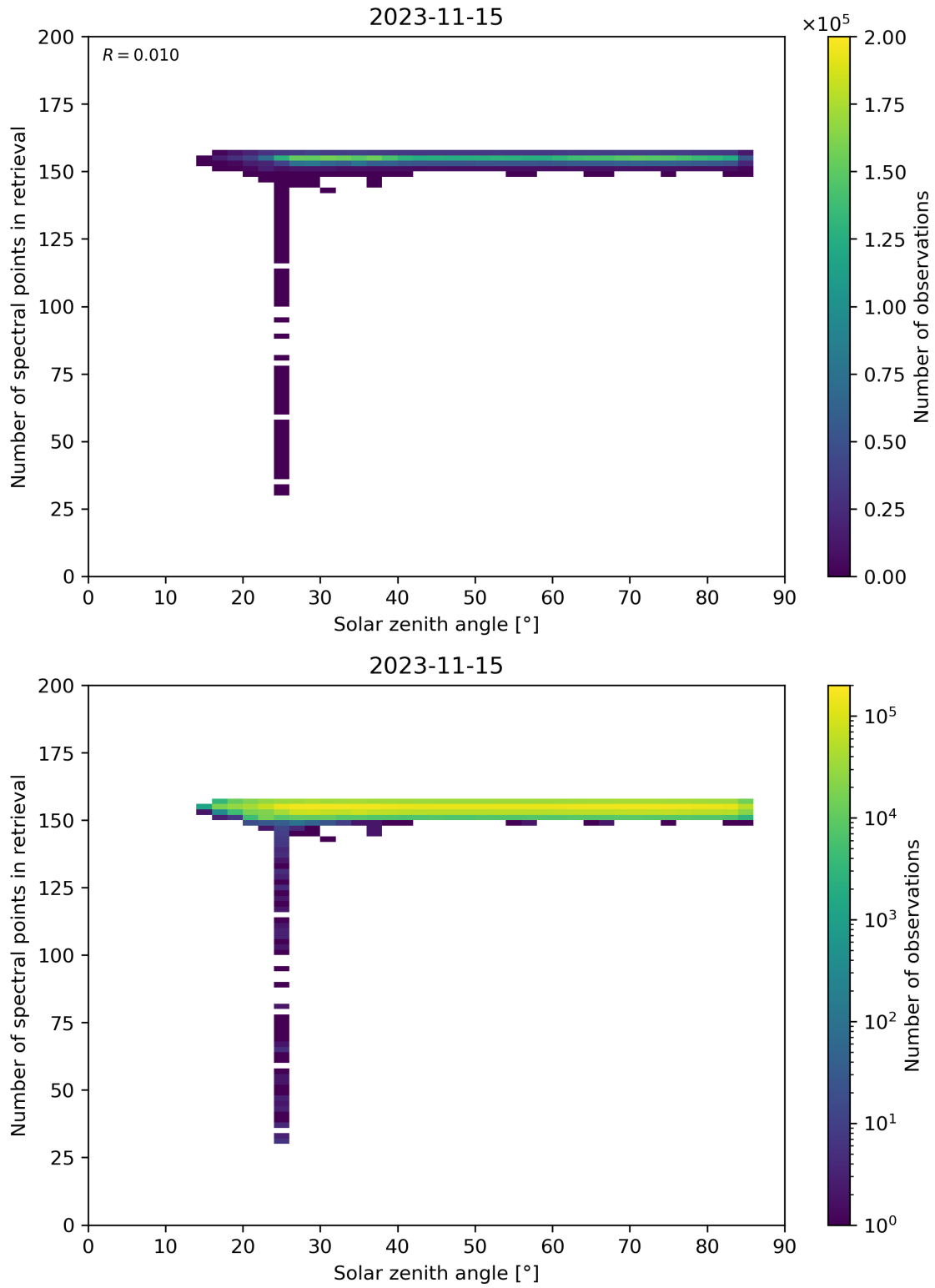
Figure 68: Scatter density plot of “Solar zenith angle” against “Number of spectral points in retrieval” for 2023-11-14 to 2023-11-16.
