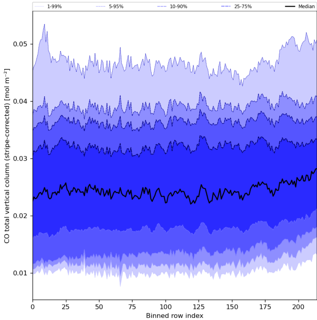
Figure 27: Along track statistics of “CO total vertical column (stripe-corrected)” for 2023-11-14 to 2023-11-16
