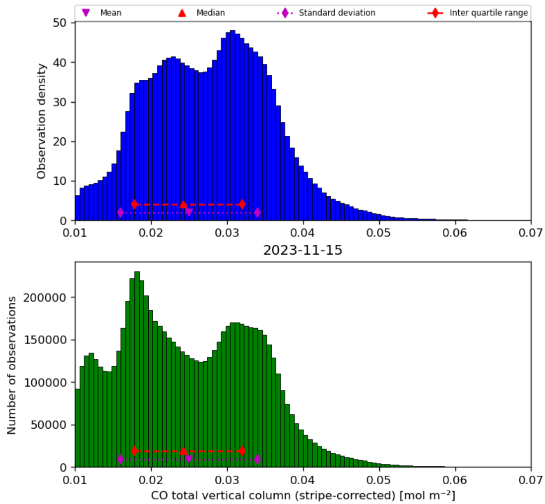
Figure 19: Histogram of “CO total vertical column (stripe-corrected)” for 2023-11-14 to 2023-11-16
