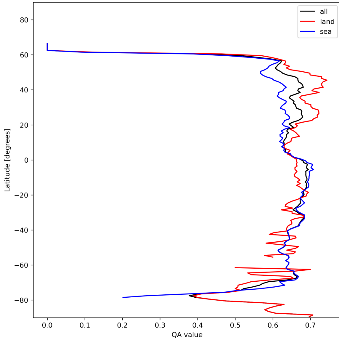
Figure 9: Zonal average of “QA value” for 2023-11-14 to 2023-11-16.
