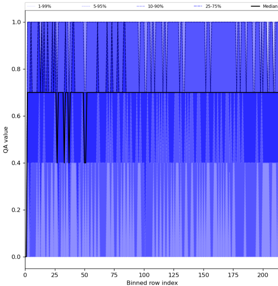
Figure 25: Along track statistics of “QA value” for 2023-11-14 to 2023-11-16
