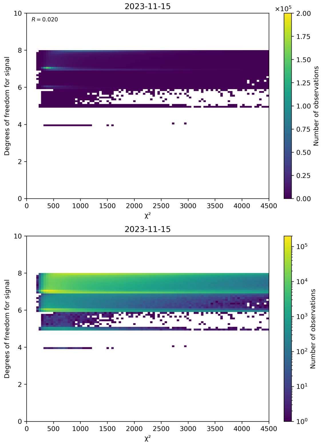
Figure 48: Scatter density plot of “ \chi^2 ” against “Degrees of freedom for signal” for 2023-11-14 to 2023-11-16.
