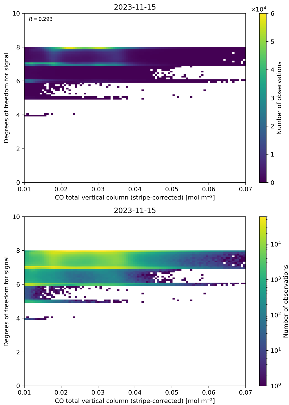
Figure 38: Scatter density plot of “CO total vertical column (stripe-corrected)” against “Degrees of freedom for signal” for 2023-11-14 to 2023-11-16.
