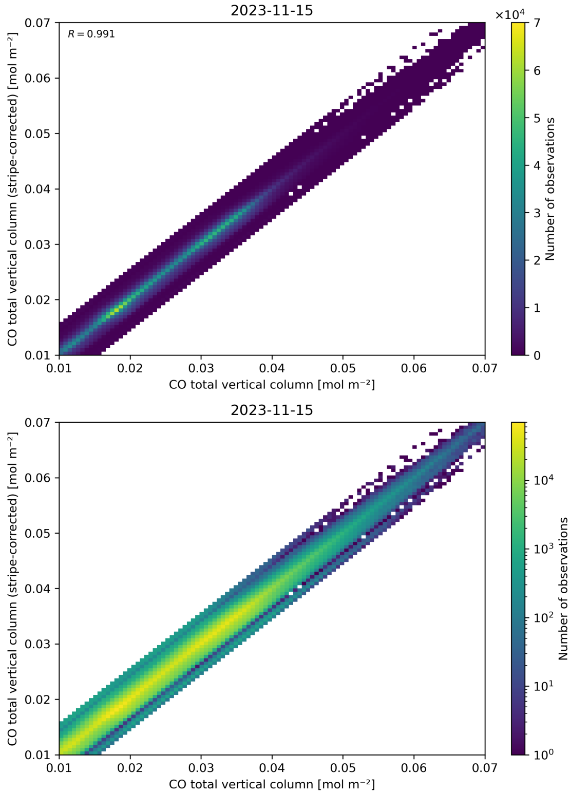
Figure 33: Scatter density plot of “CO total vertical column” against “CO total vertical column (stripe-corrected)” for 2023-11-14 to 2023-11-16.
