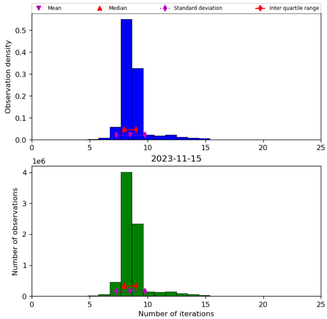
Figure 24: Histogram of “Number of iterations” for 2023-11-14 to 2023-11-16
