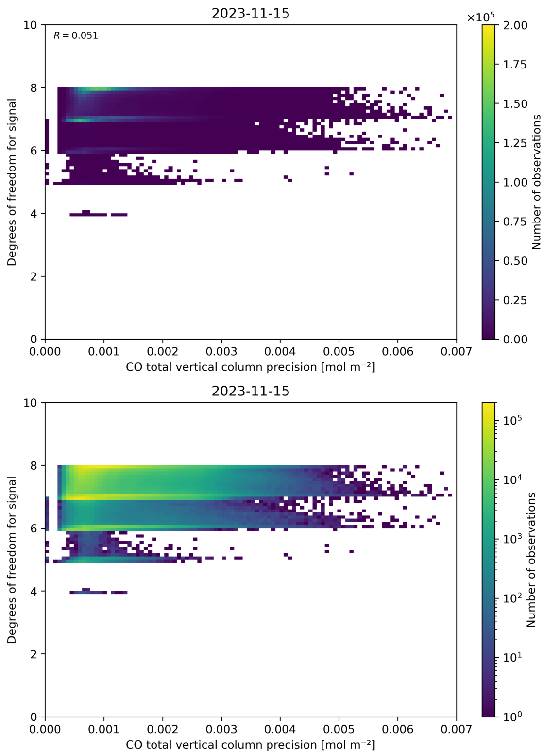
Figure 45: Scatter density plot of “CO total vertical column precision” against “Degrees of freedom for signal” for 2023-11-14 to 2023-11-16.
