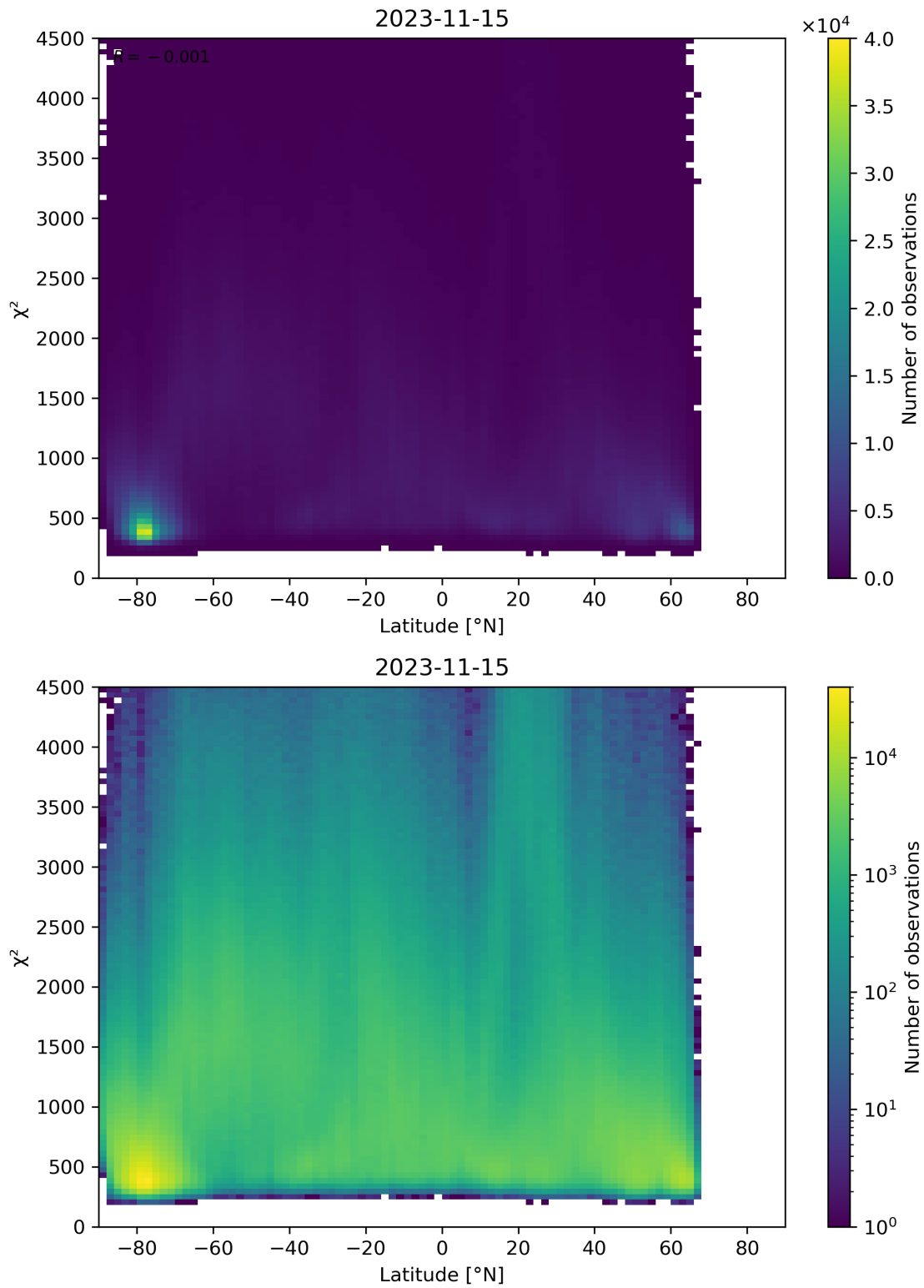
Figure 54: Scatter density plot of “Latitude” against “ \chi^2 ” for 2023-11-14 to 2023-11-16.
