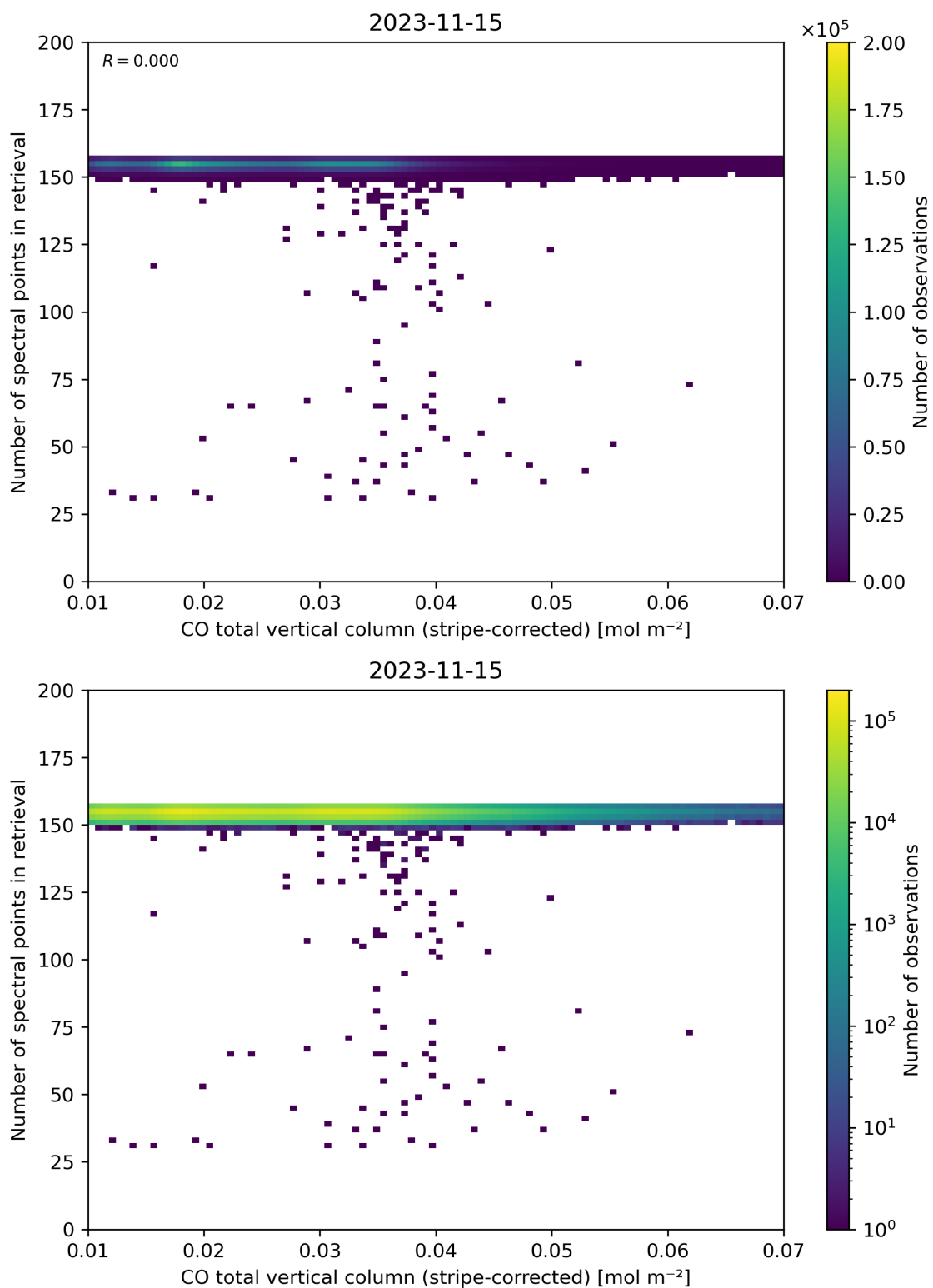
Figure 40: Scatter density plot of “CO total vertical column (stripe-corrected)” against “Number of spectral points in retrieval” for 2023-11-14 to 2023-11-16.
