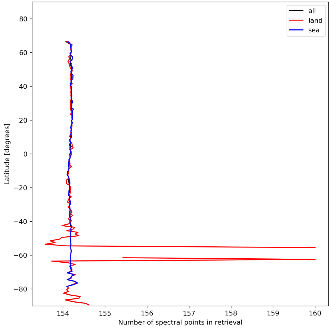
Figure 13: Zonal average of “Number of spectral points in retrieval” for 2023-11-14 to 2023-11-16.
