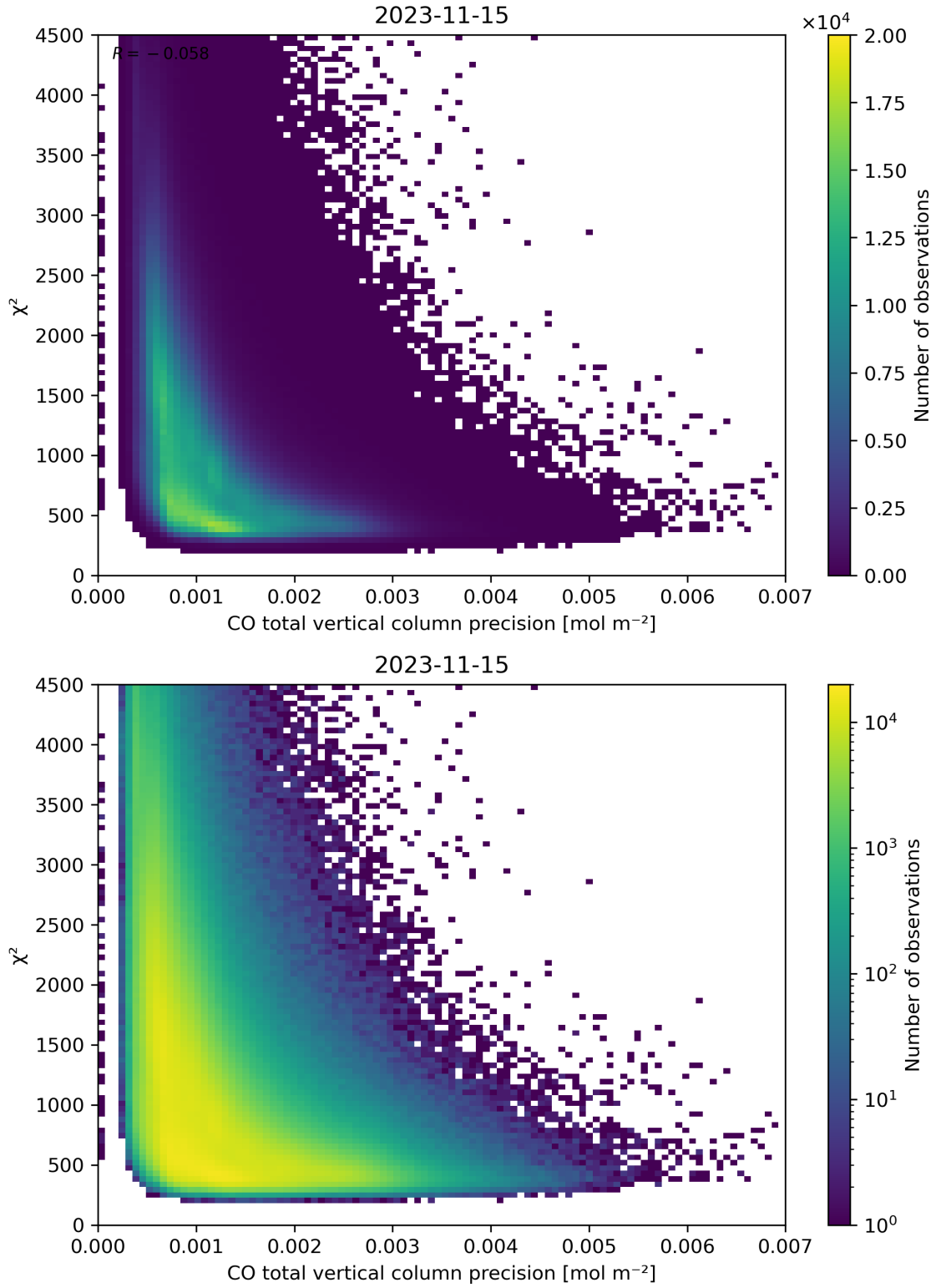
Figure 44: Scatter density plot of “CO total vertical column precision” against “ \chi^2 ” for 2023-11-14 to 2023-11-16.
