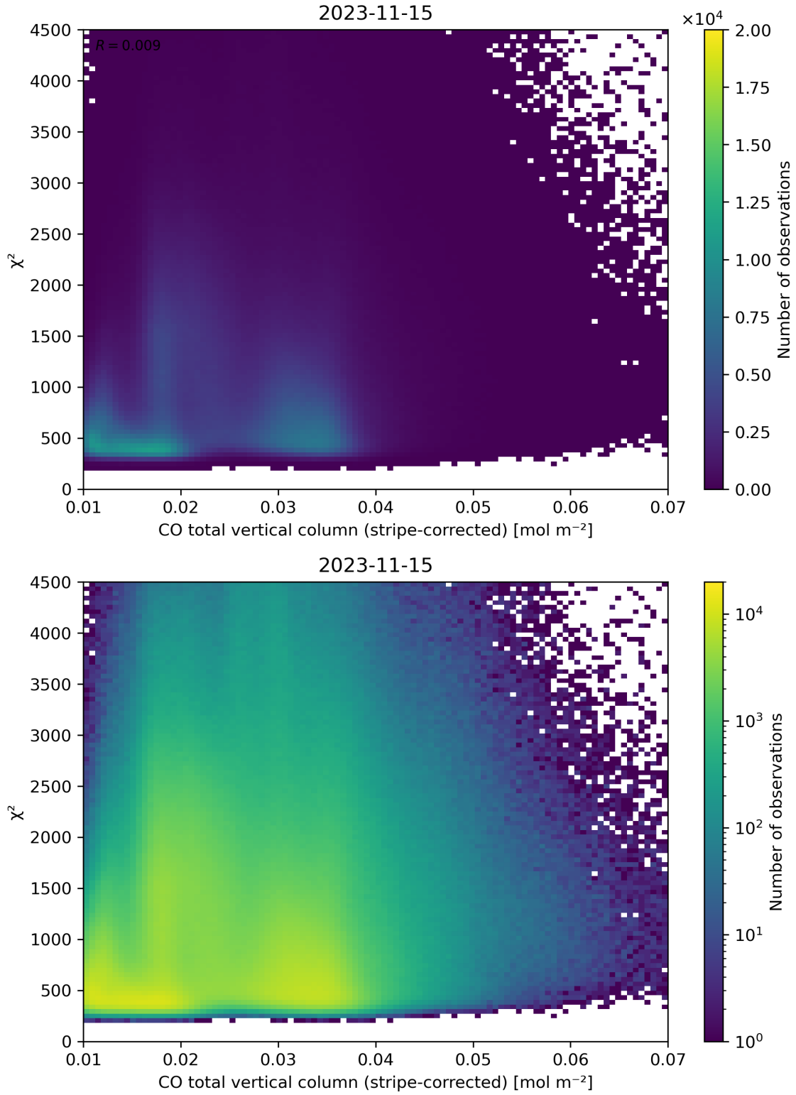
Figure 37: Scatter density plot of “CO total vertical column (stripe-corrected)” against “ \chi^2 ” for 2023-11-14 to 2023-11-16.
