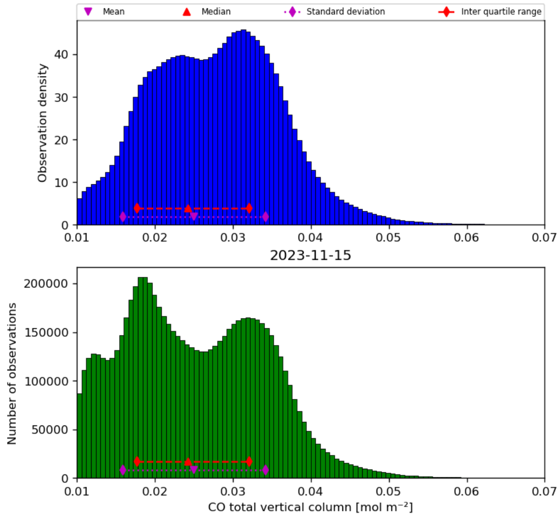
Figure 18: Histogram of “CO total vertical column” for 2023-11-14 to 2023-11-16
