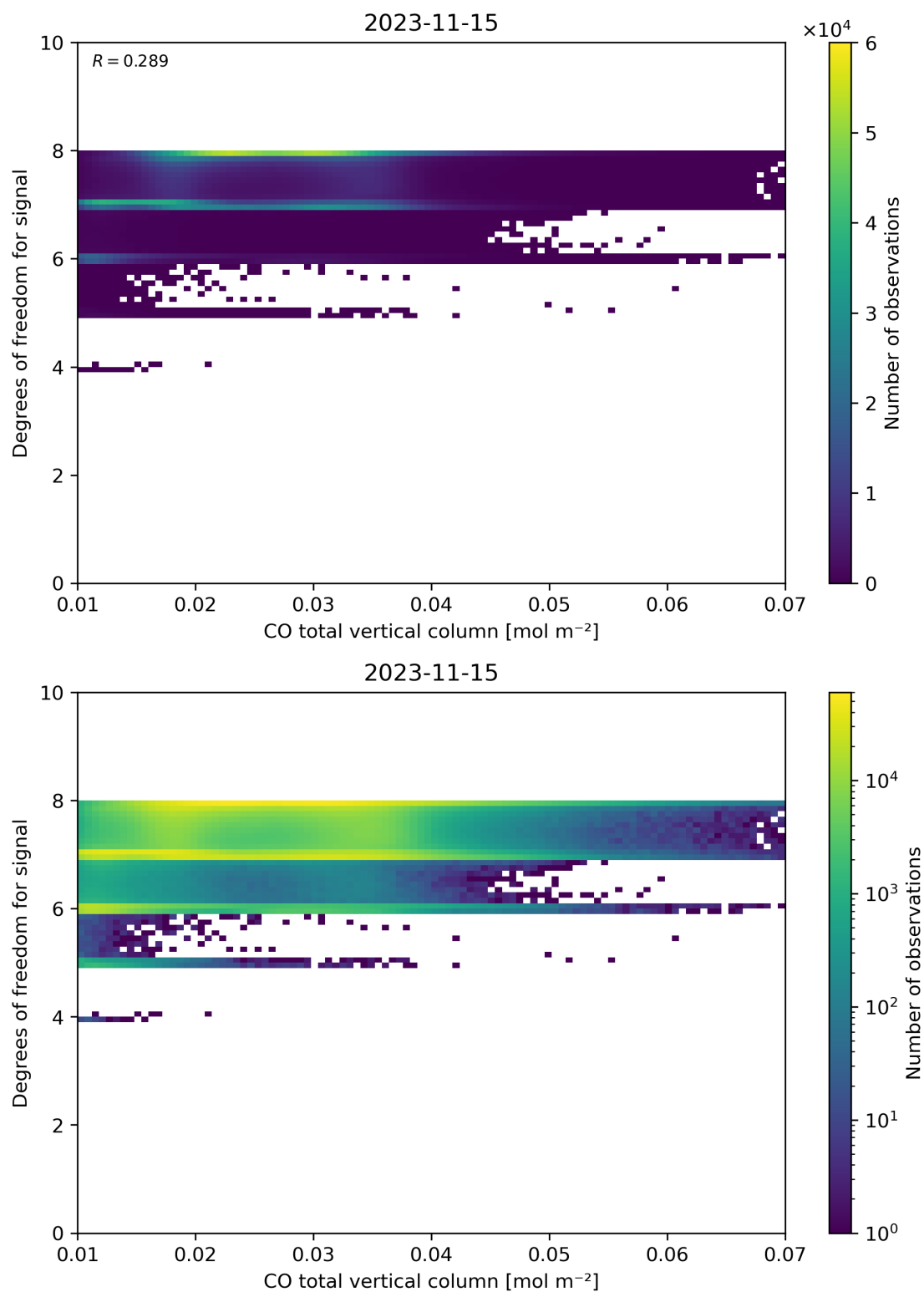
Figure 41: Scatter density plot of “CO total vertical column” against “Degrees of freedom for signal” for 2023-11-14 to 2023-11-16.
