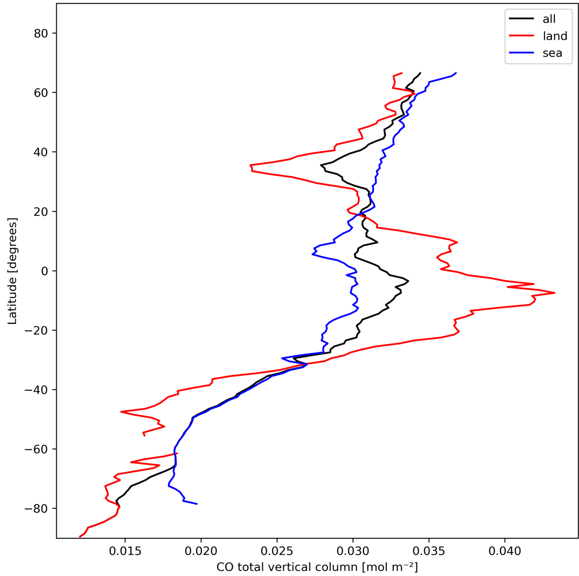
Figure 10: Zonal average of “CO total vertical column” for 2023-11-14 to 2023-11-16.
