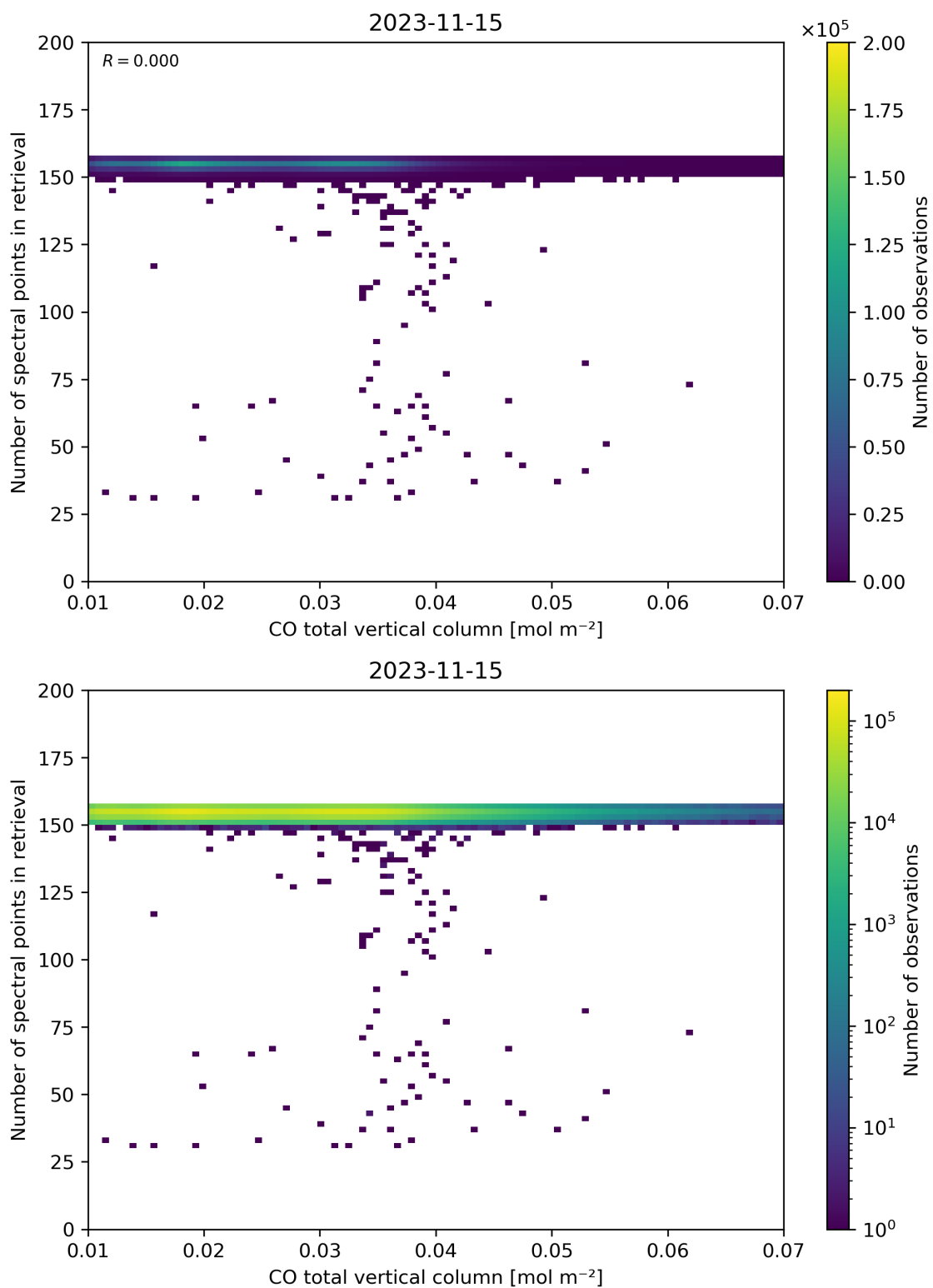
Figure 43: Scatter density plot of “CO total vertical column” against “Number of spectral points in retrieval” for 2023-11-14 to 2023-11-16.
