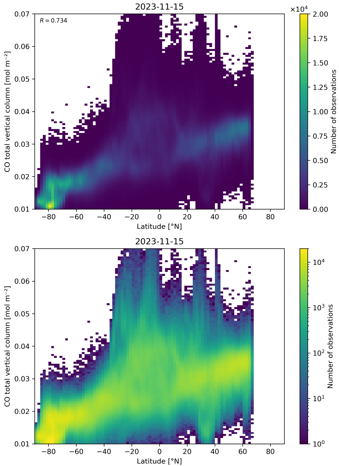
Figure 51: Scatter density plot of “Latitude” against “CO total vertical column” for 2023-11-14 to 2023-11-16.
