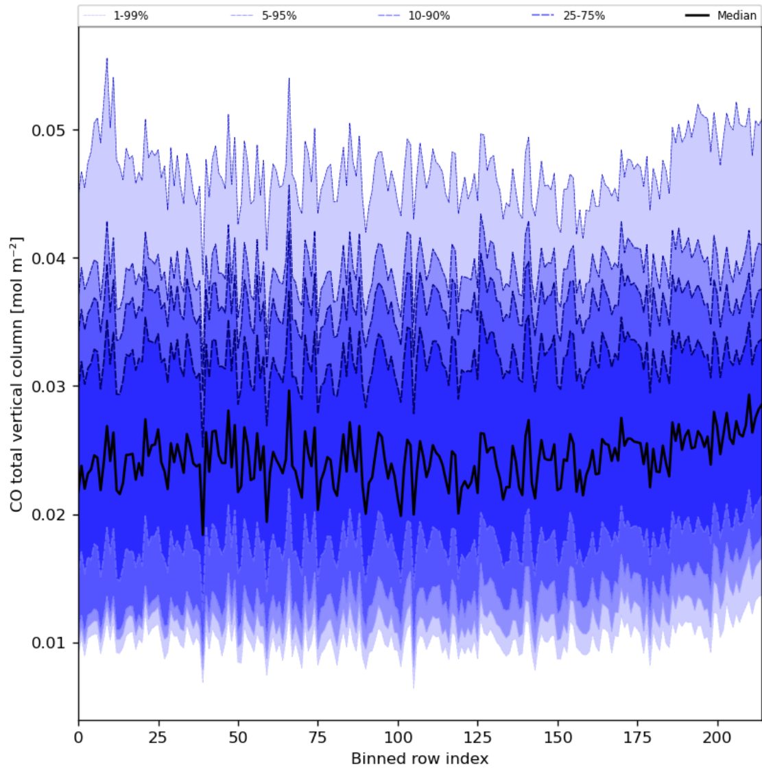
Figure 26: Along track statistics of “CO total vertical column” for 2023-11-14 to 2023-11-16
