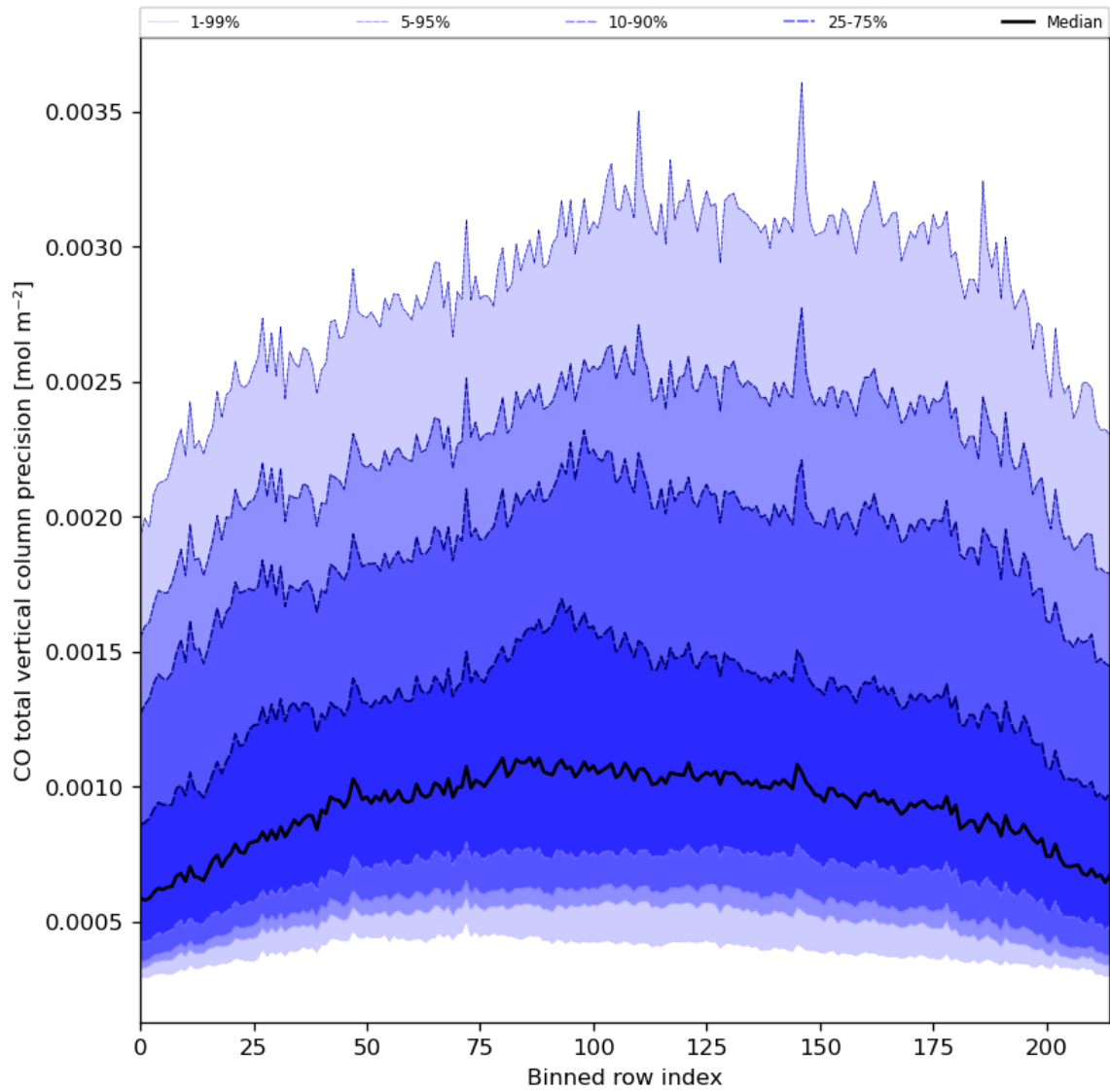
Figure 28: Along track statistics of “CO total vertical column precision” for 2023-11-14 to 2023-11-16
