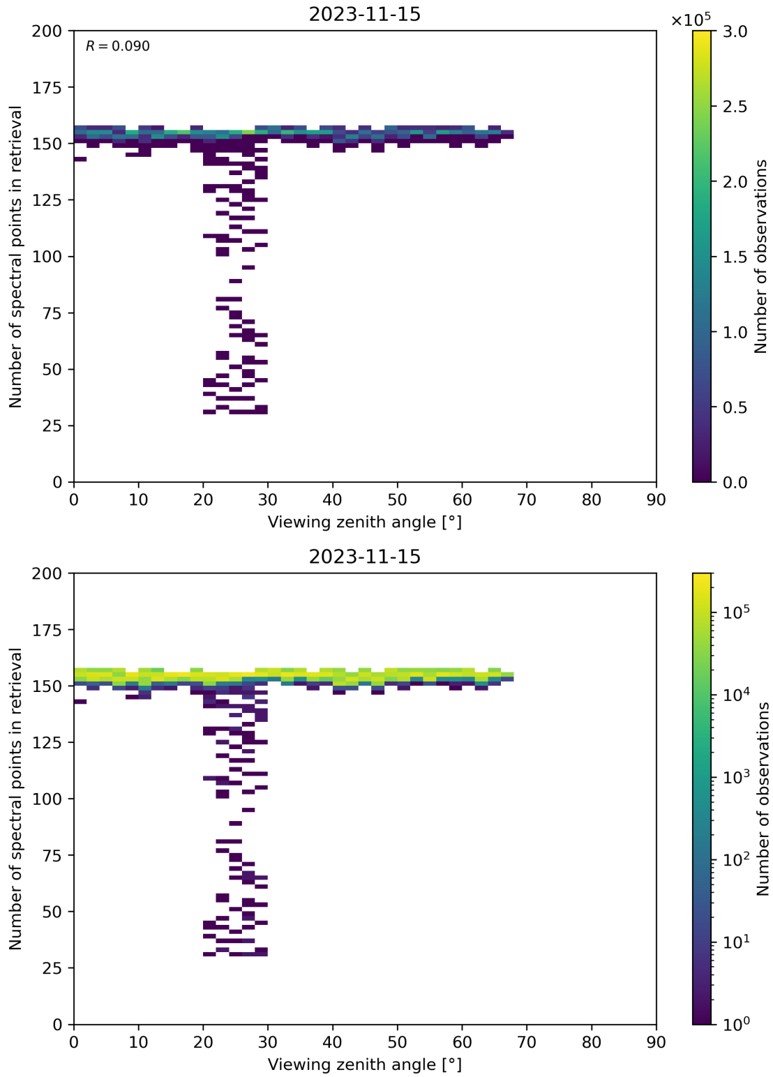
Figure 76: Scatter density plot of “Viewing zenith angle” against “Number of spectral points in retrieval” for 2023-11-14 to 2023-11-16.
