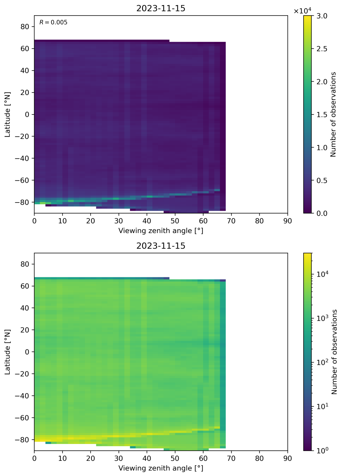
Figure 74: Scatter density plot of “Viewing zenith angle” against “Latitude” for 2023-11-14 to 2023-11-16.
