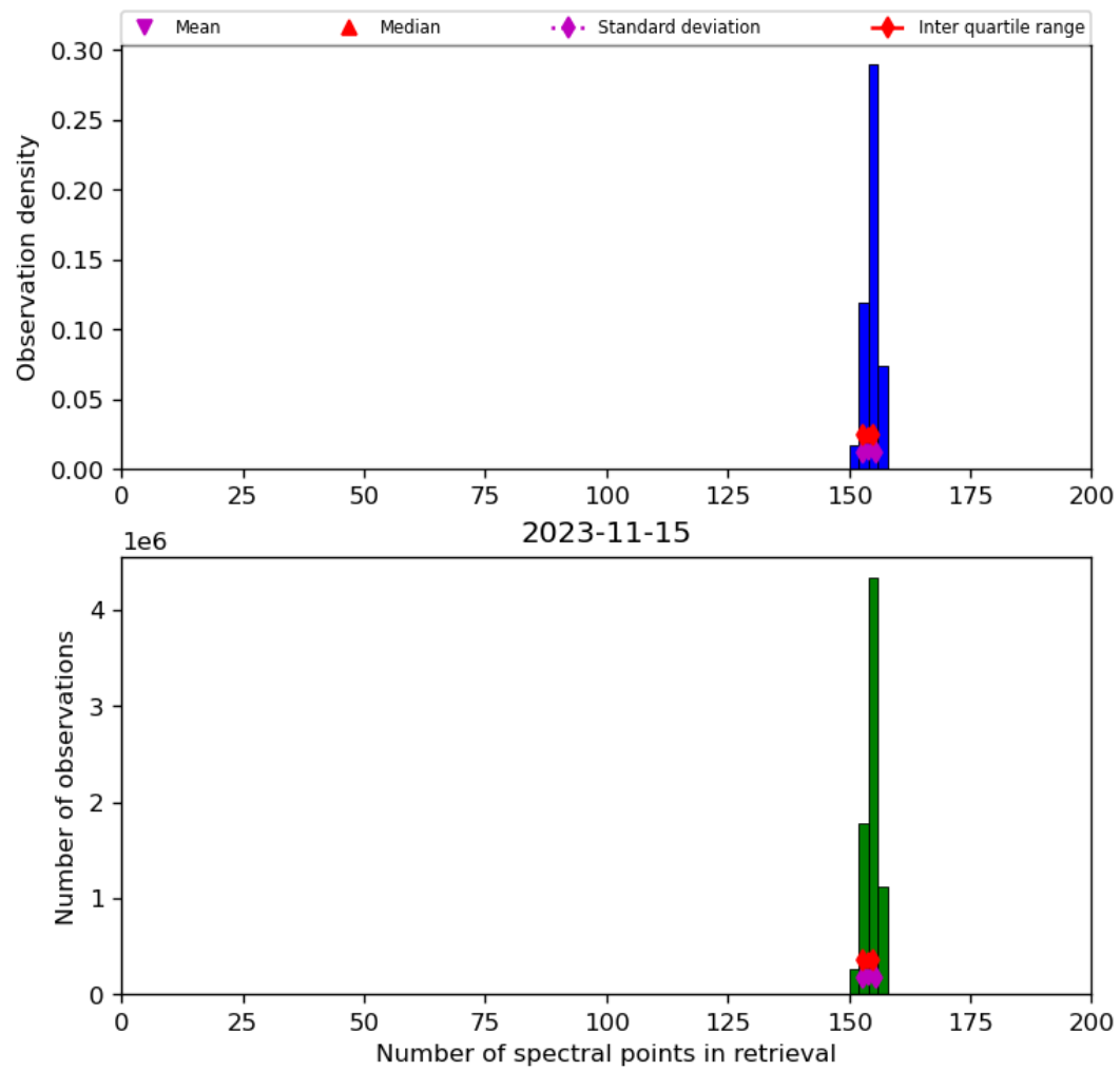
Figure 21: Histogram of “Number of spectral points in retrieval” for 2023-11-14 to 2023-11-16
