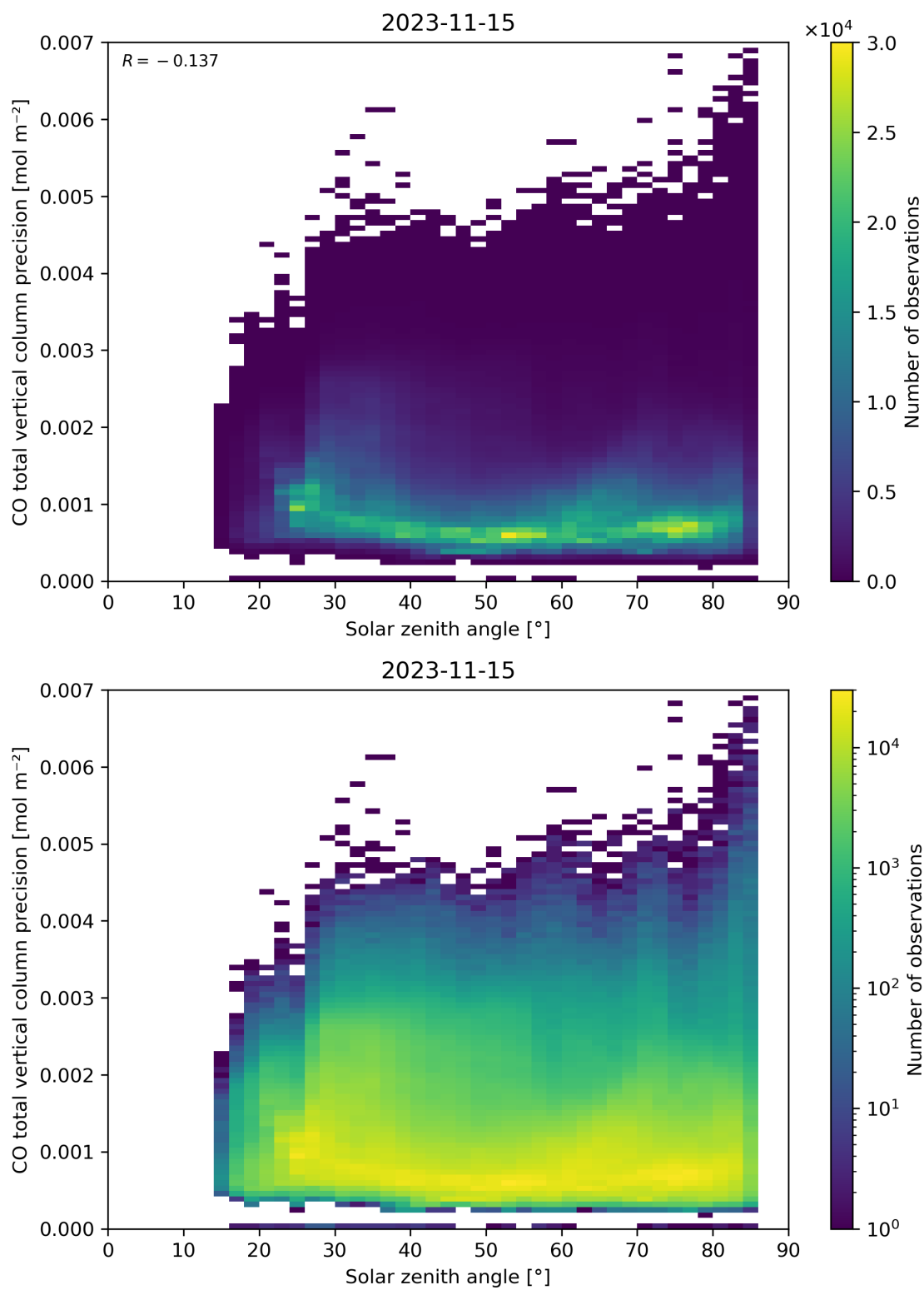
Figure 63: Scatter density plot of “Solar zenith angle” against “CO total vertical column precision” for 2023-11-14 to 2023-11-16.
