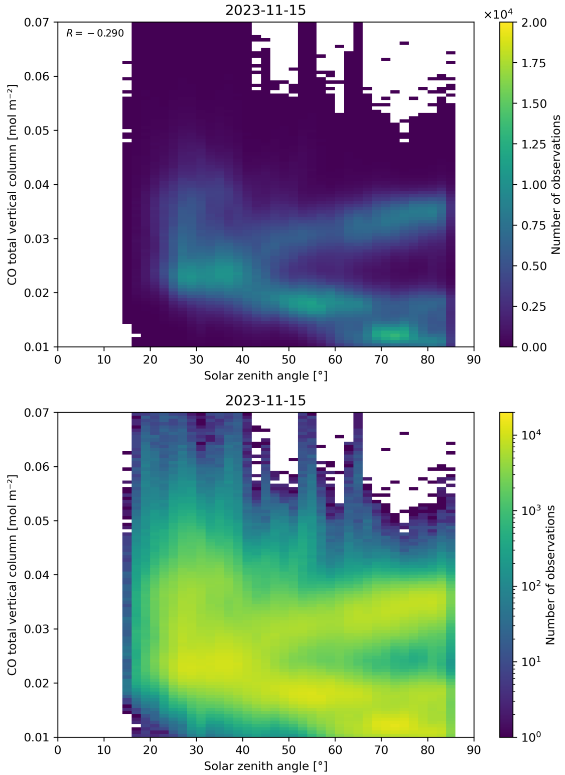
Figure 61: Scatter density plot of “Solar zenith angle” against “CO total vertical column” for 2023-11-14 to 2023-11-16.
