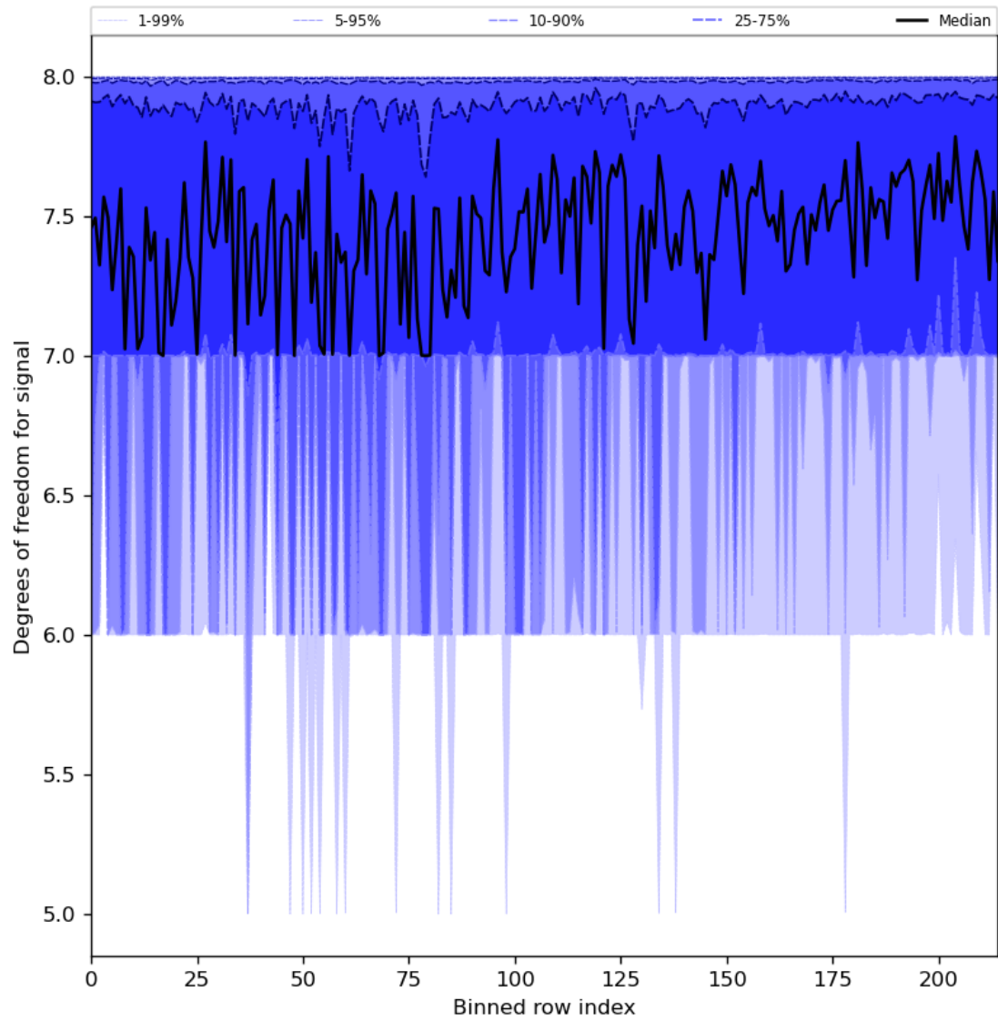
Figure 31: Along track statistics of “Degrees of freedom for signal” for 2023-11-14 to 2023-11-16
