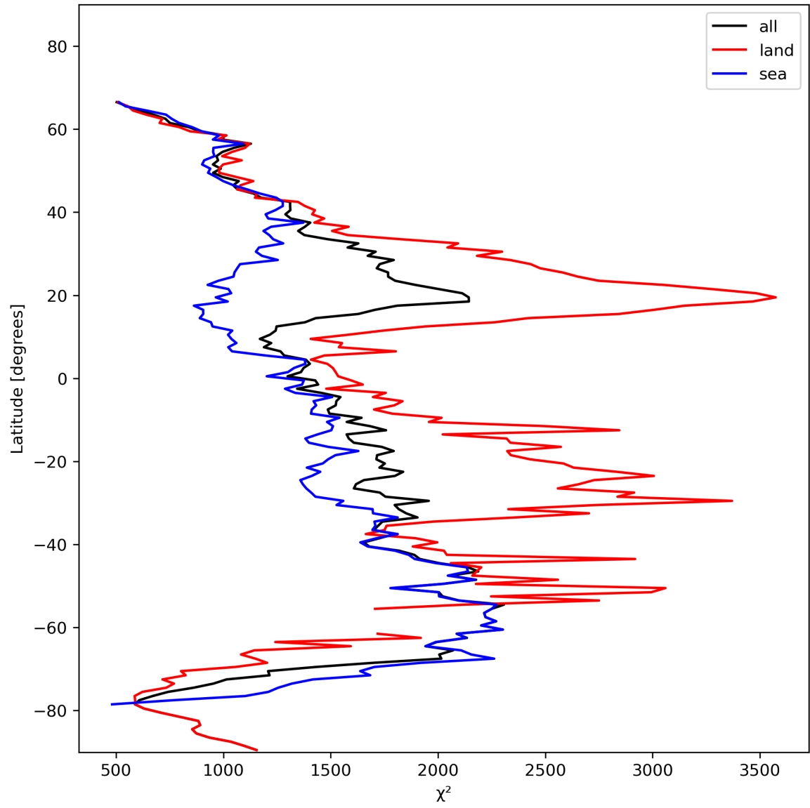
Figure 14: Zonal average of “ \chi^2 ” for 2023-11-14 to 2023-11-16.
