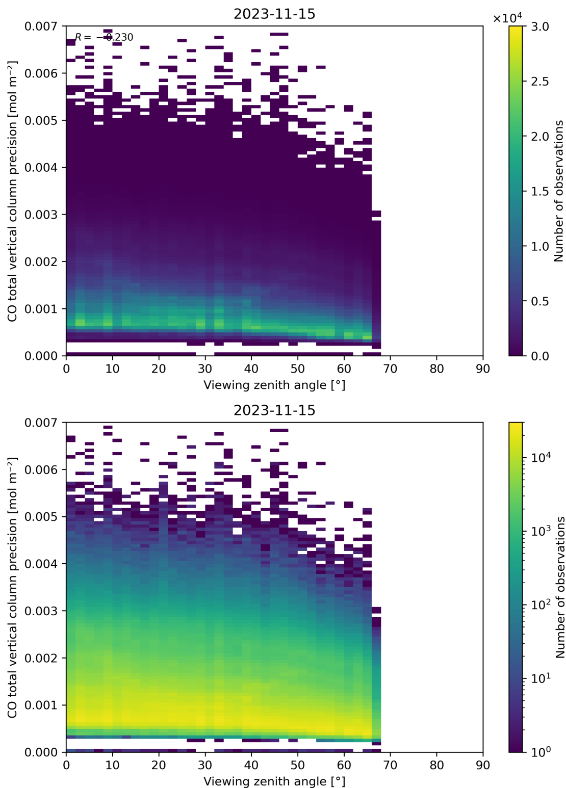
Figure 71: Scatter density plot of “Viewing zenith angle” against “CO total vertical column precision” for 2023-11-14 to 2023-11-16.
