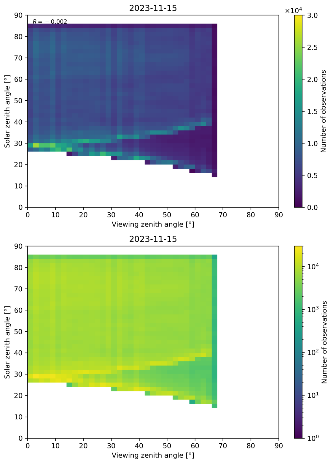
Figure 77: Scatter density plot of “Viewing zenith angle” against “Solar zenith angle” for 2023-11-14 to 2023-11-16.
