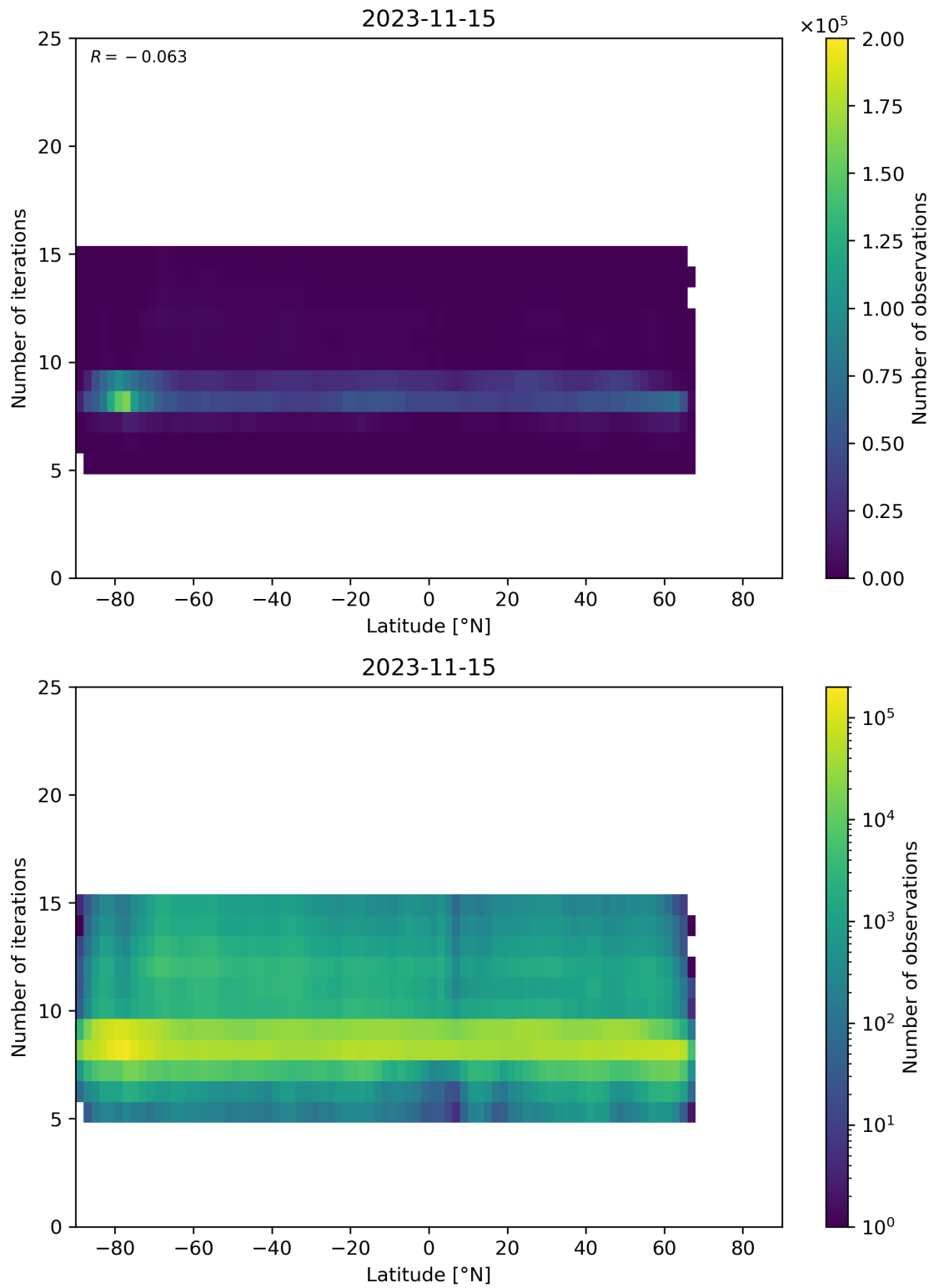
Figure 56: Scatter density plot of “Latitude” against “Number of iterations” for 2023-11-14 to 2023-11-16.
