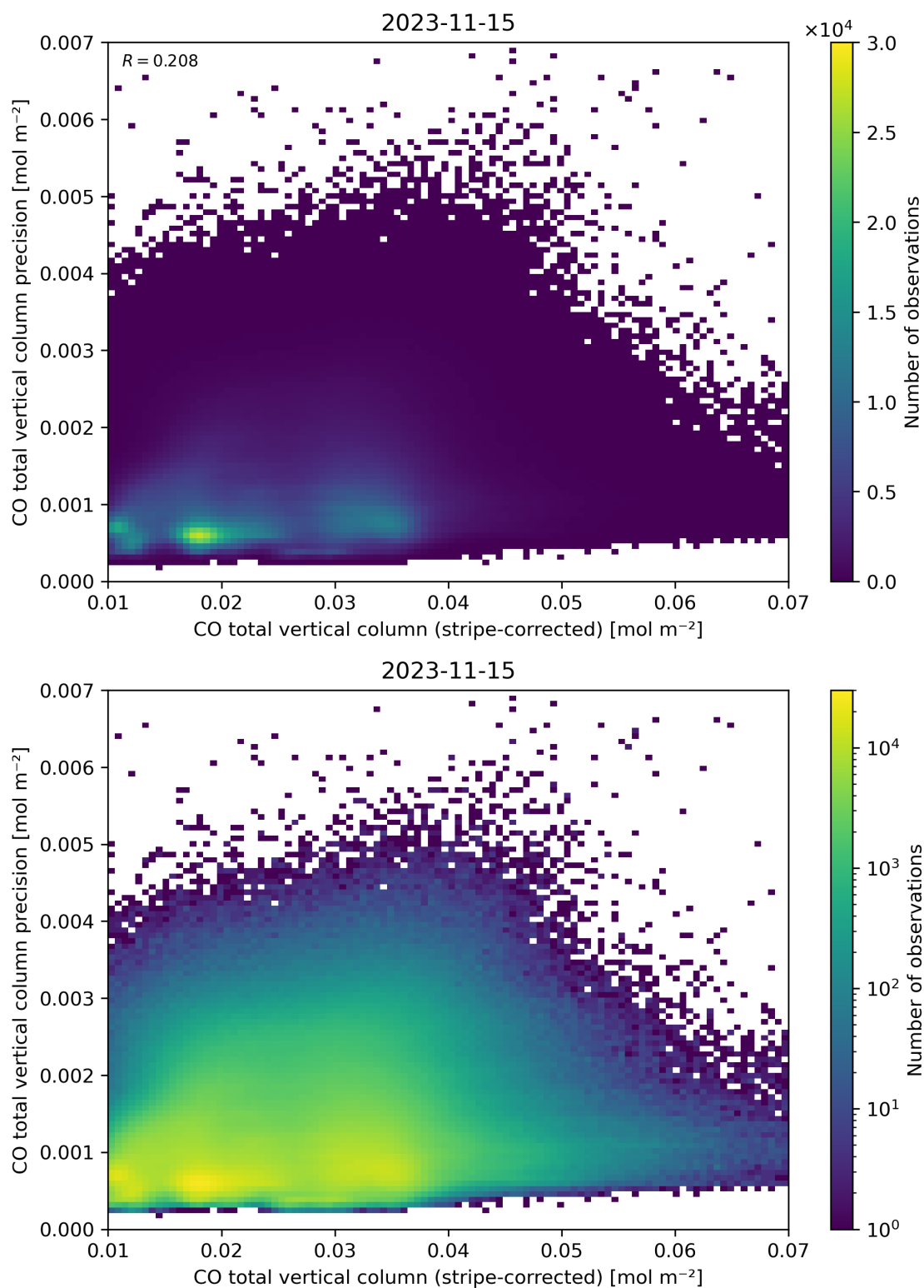
Figure 36: Scatter density plot of “CO total vertical column (stripe-corrected)” against “CO total vertical column precision” for 2023-11-14 to 2023-11-16.
