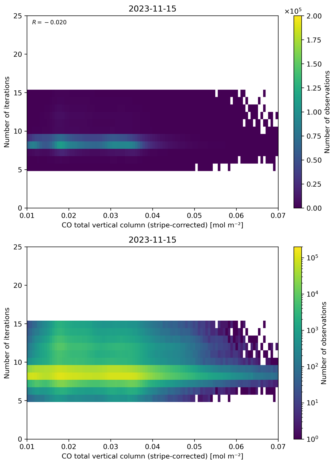
Figure 39: Scatter density plot of “CO total vertical column (stripe-corrected)” against “Number of iterations” for 2023-11-14 to 2023-11-16.
