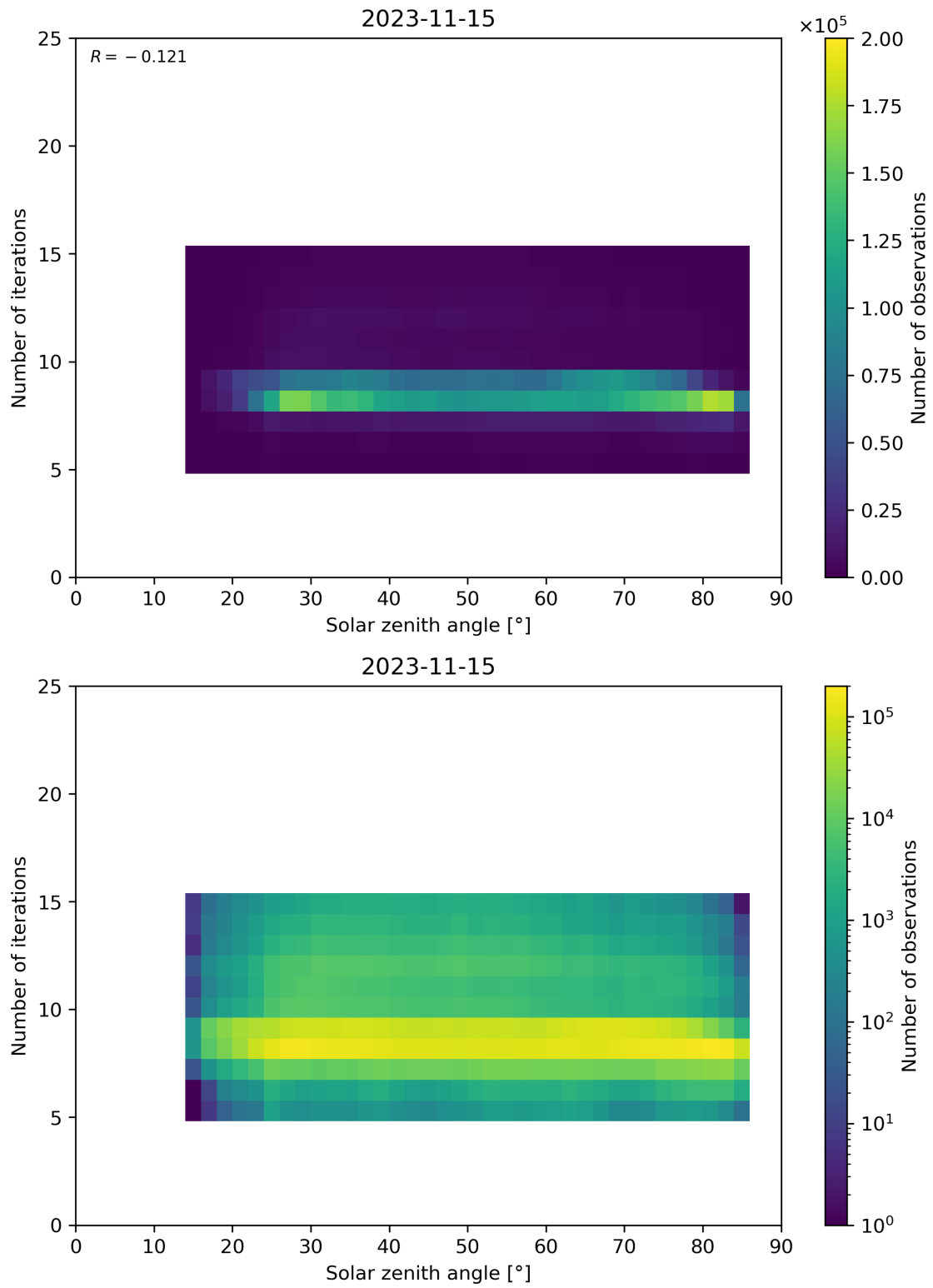
Figure 67: Scatter density plot of “Solar zenith angle” against “Number of iterations” for 2023-11-14 to 2023-11-16.
