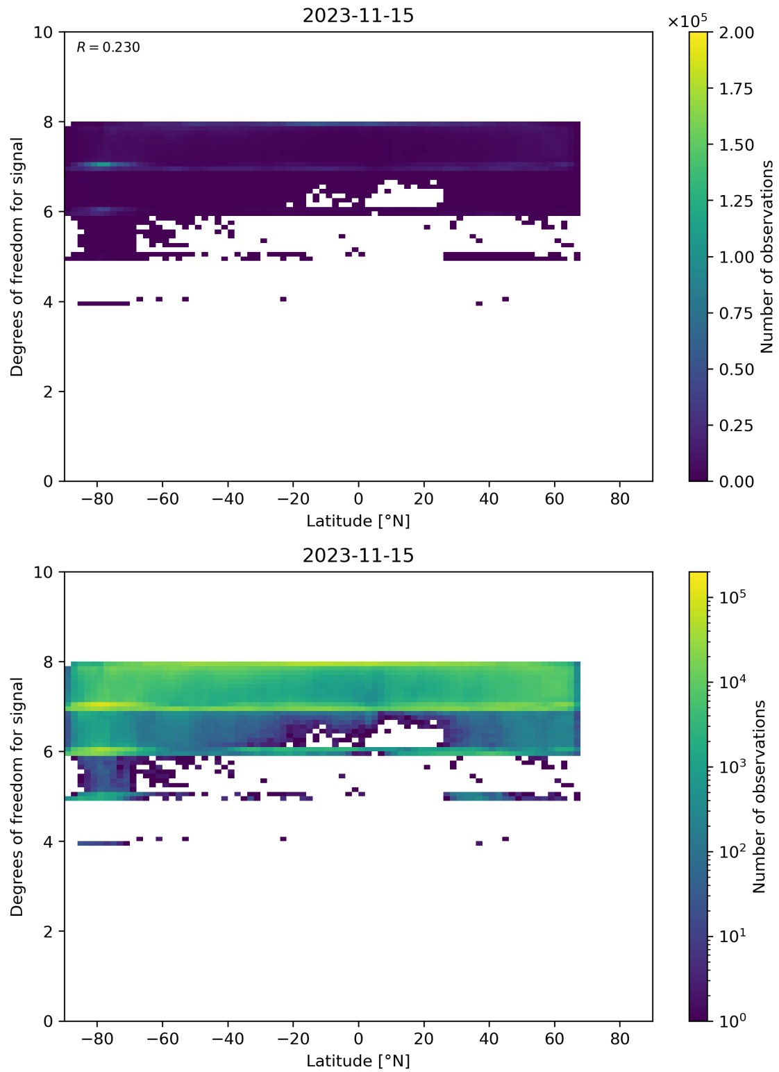
Figure 55: Scatter density plot of “Latitude” against “Degrees of freedom for signal” for 2023-11-14 to 2023-11-16.
