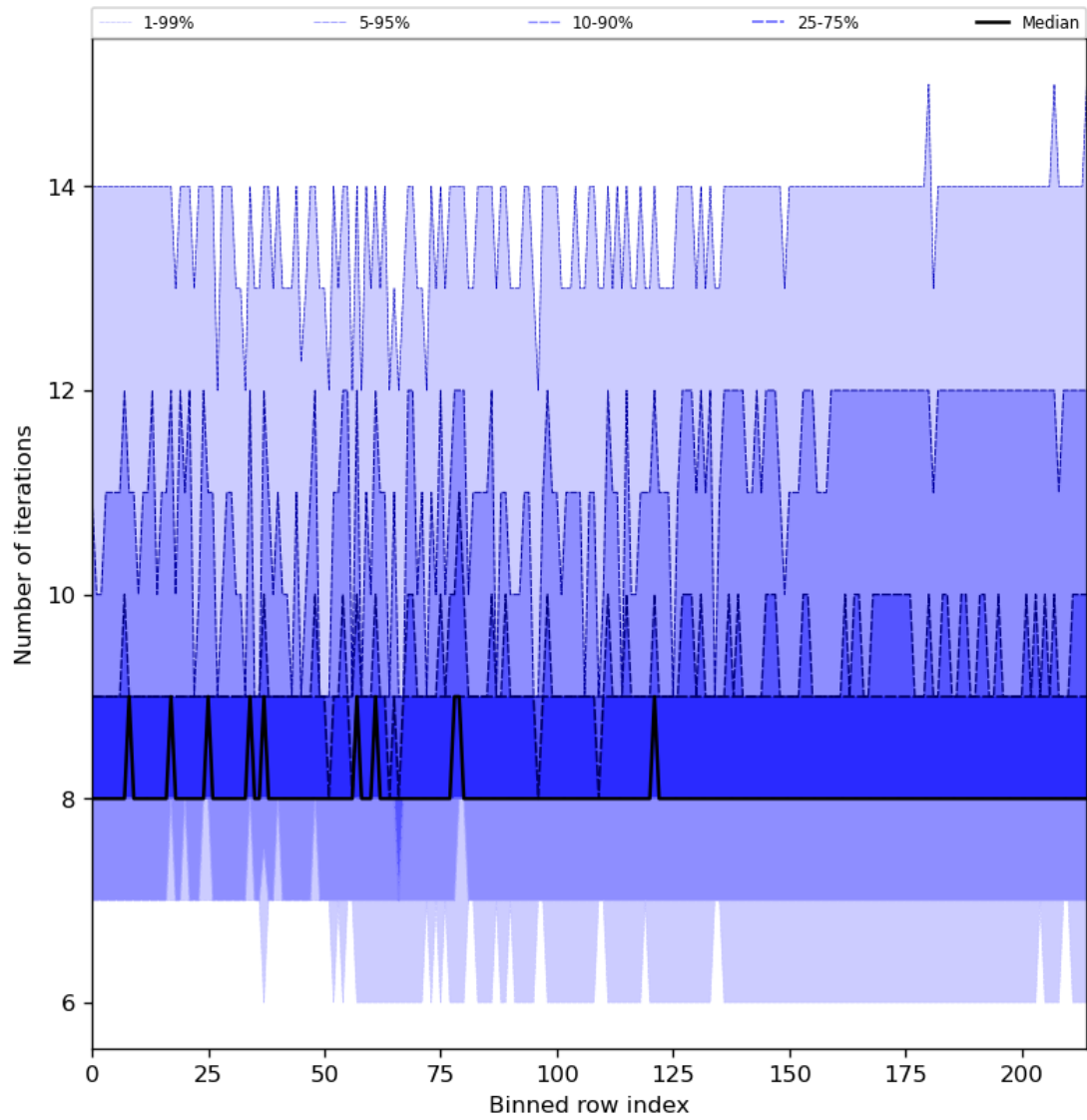
Figure 32: Along track statistics of “Number of iterations” for 2023-11-14 to 2023-11-16
