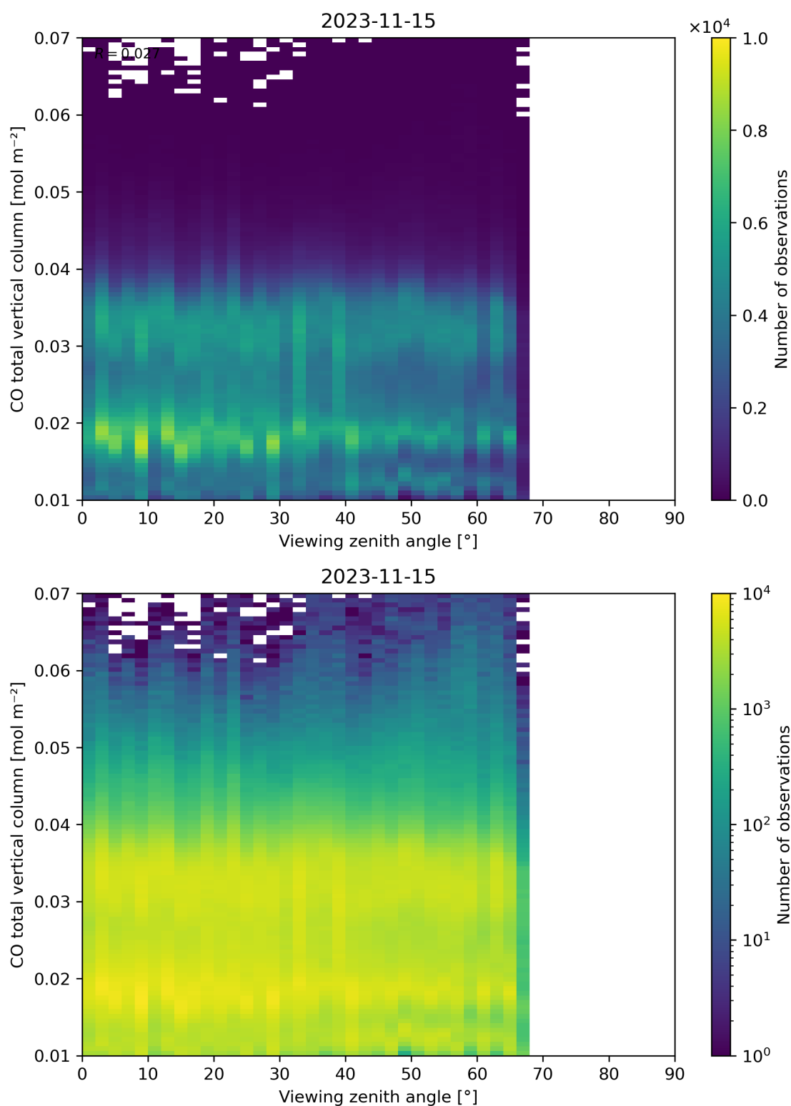
Figure 69: Scatter density plot of “Viewing zenith angle” against “CO total vertical column” for 2023-11-14 to 2023-11-16.
