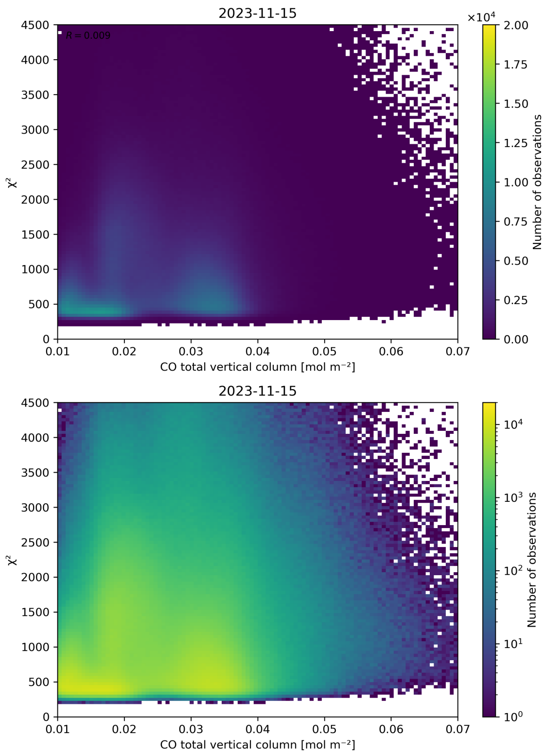
Figure 35: Scatter density plot of “CO total vertical column” against “ \chi^2 ” for 2023-11-14 to 2023-11-16.
