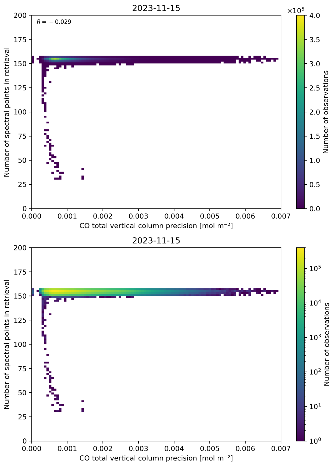
Figure 47: Scatter density plot of “CO total vertical column precision” against “Number of spectral points in retrieval” for 2023-11-14 to 2023-11-16.
