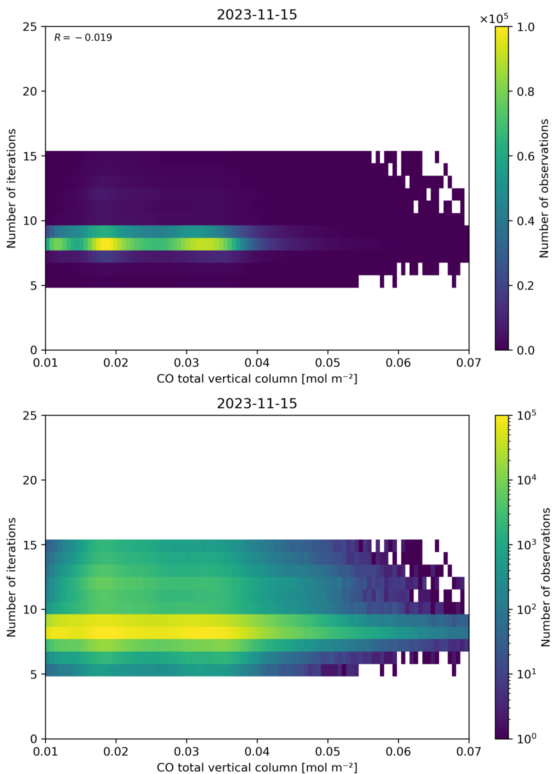
Figure 42: Scatter density plot of “CO total vertical column” against “Number of iterations” for 2023-11-14 to 2023-11-16.
