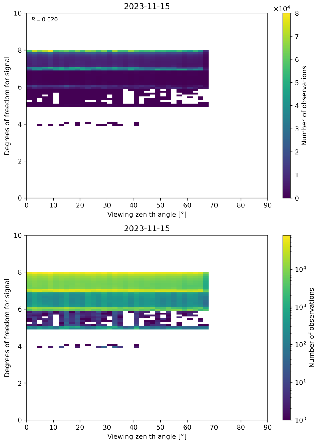
Figure 73: Scatter density plot of “Viewing zenith angle” against “Degrees of freedom for signal” for 2023-11-14 to 2023-11-16.
