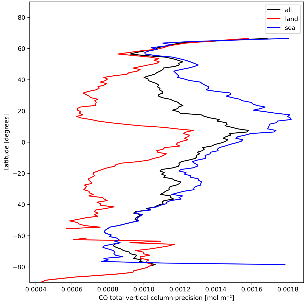
Figure 12: Zonal average of “CO total vertical column precision” for 2023-11-14 to 2023-11-16.
