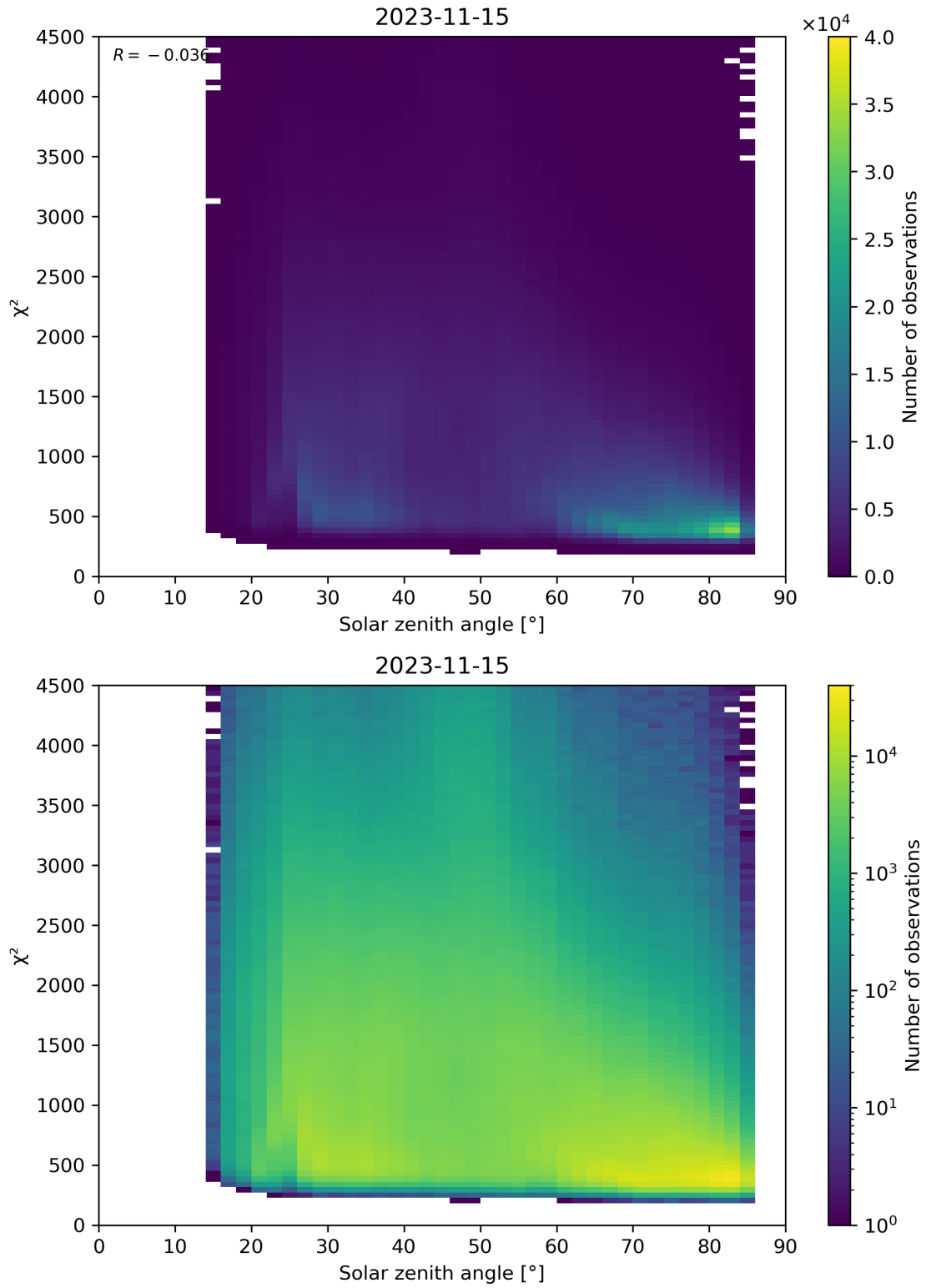
Figure 64: Scatter density plot of “Solar zenith angle” against “ \chi^2 ” for 2023-11-14 to 2023-11-16.
