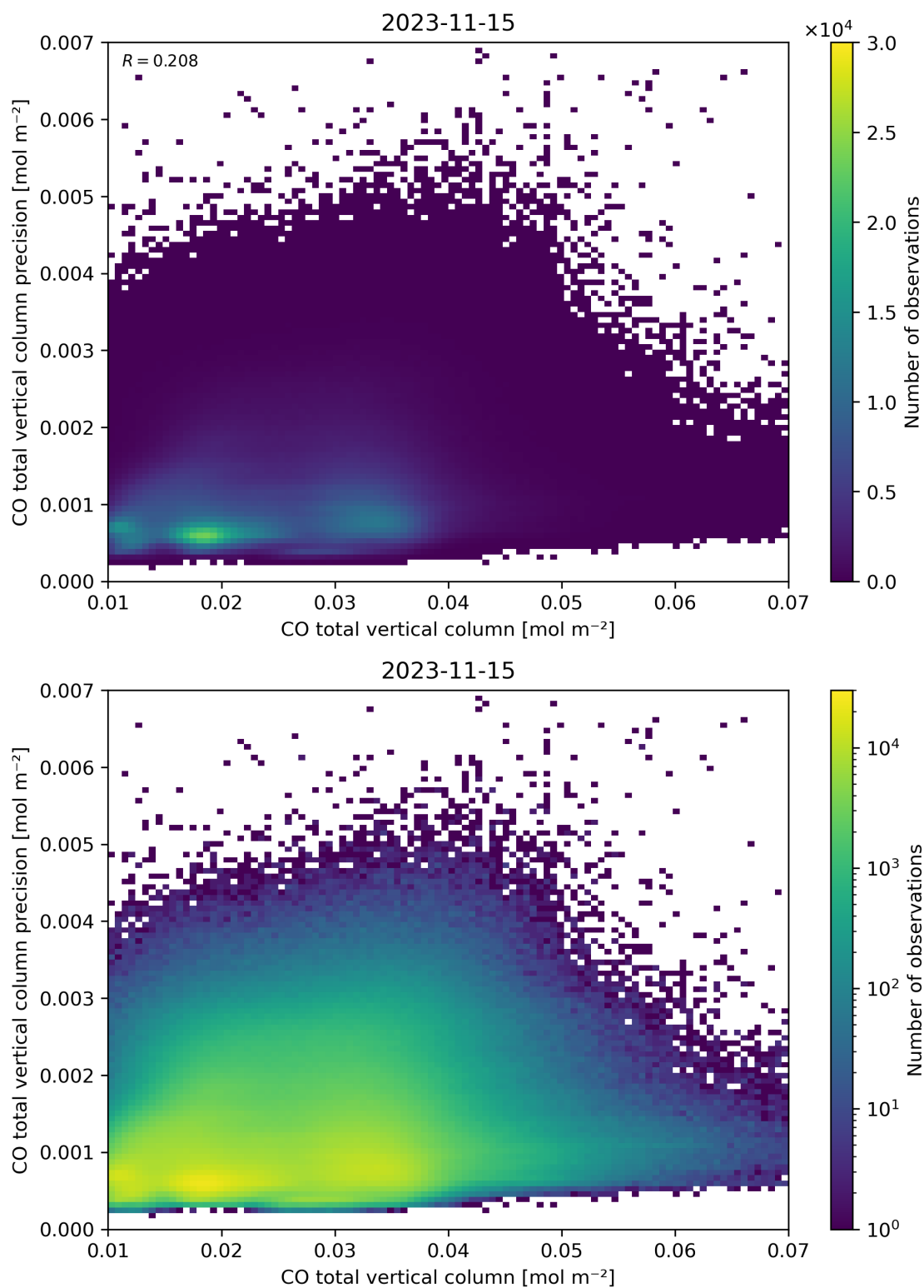
Figure 34: Scatter density plot of “CO total vertical column” against “CO total vertical column precision” for 2023-11-14 to 2023-11-16.
