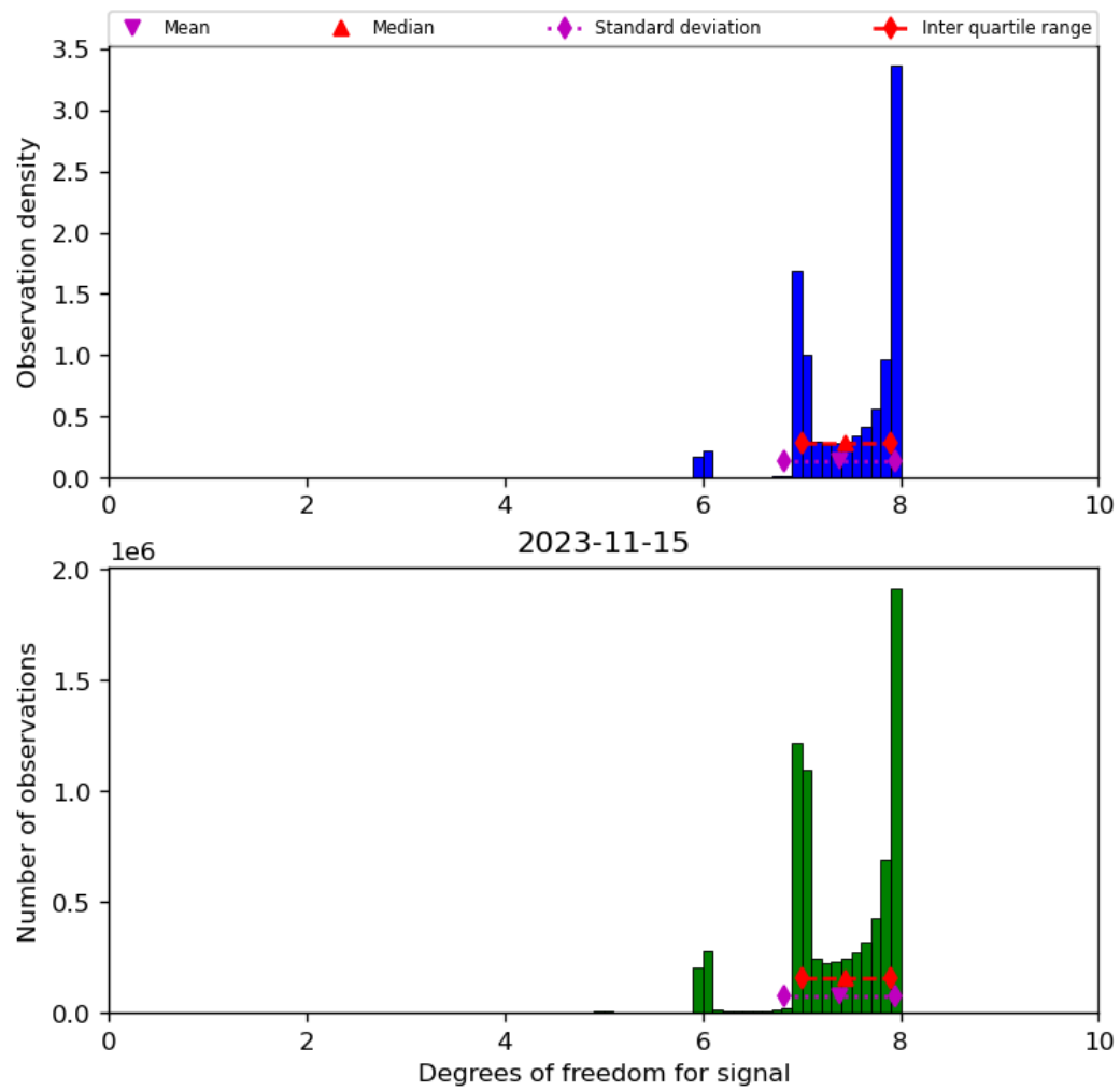
Figure 23: Histogram of “Degrees of freedom for signal” for 2023-11-14 to 2023-11-16
