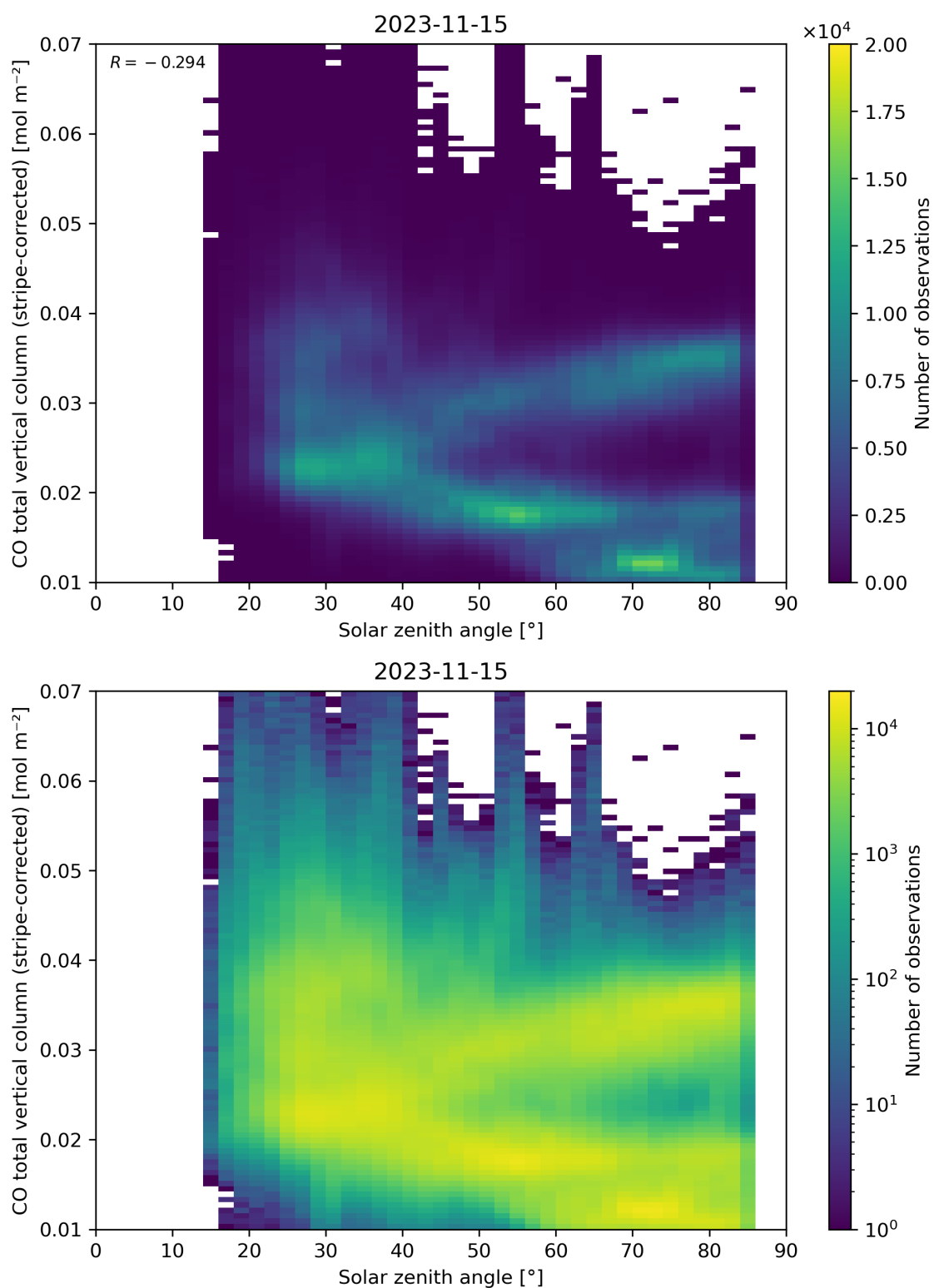
Figure 62: Scatter density plot of “Solar zenith angle” against “CO total vertical column (stripe-corrected)” for 2023-11-14 to 2023-11-16.
