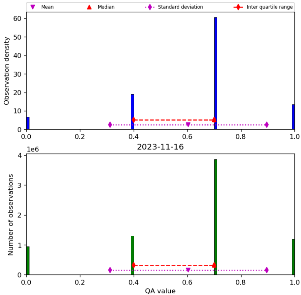
Figure 17: Histogram of “QA value” for 2023-11-15 to 2023-11-17
