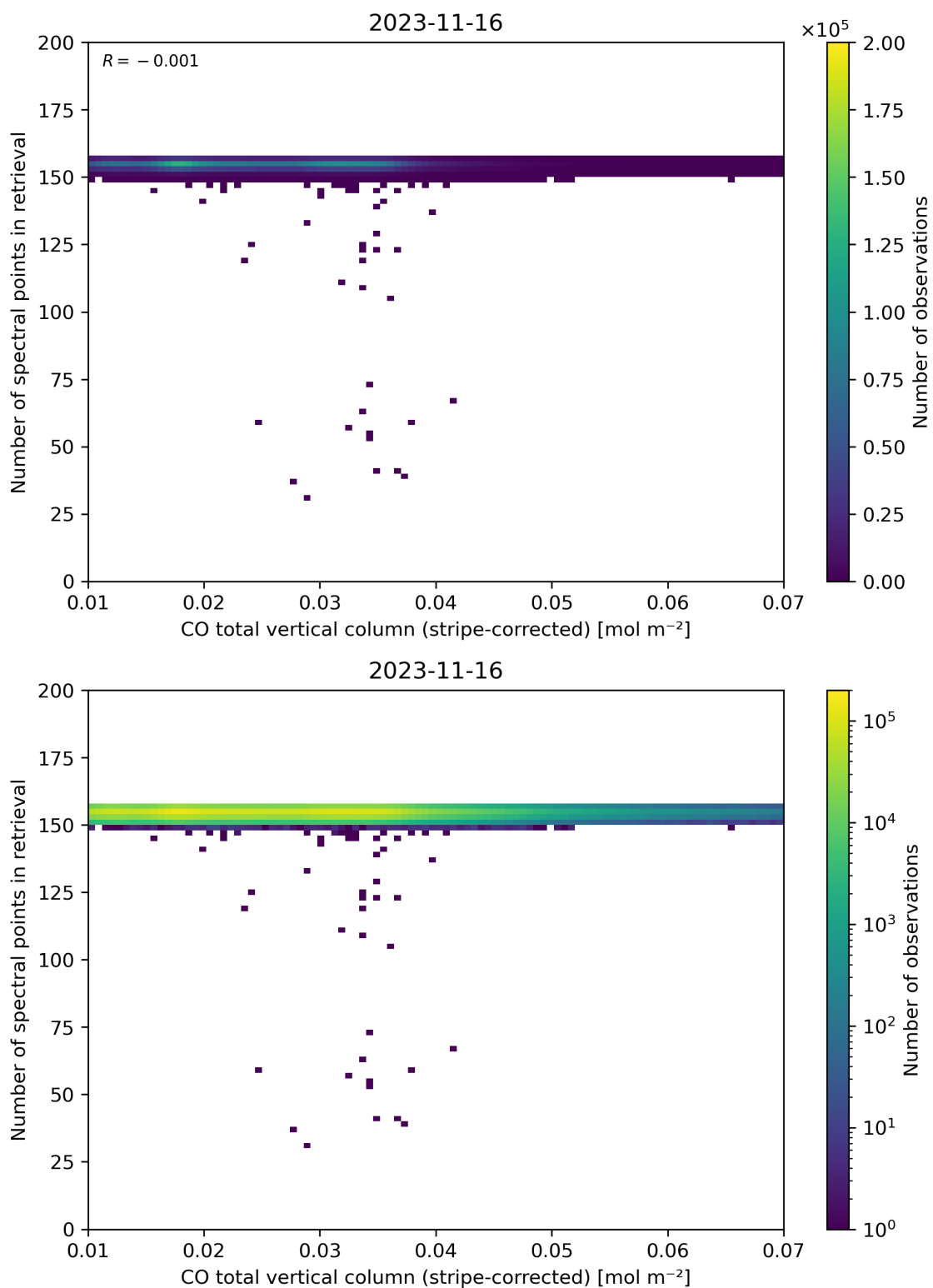
Figure 40: Scatter density plot of “CO total vertical column (stripe-corrected)” against “Number of spectral points in retrieval” for 2023-11-15 to 2023-11-17.
