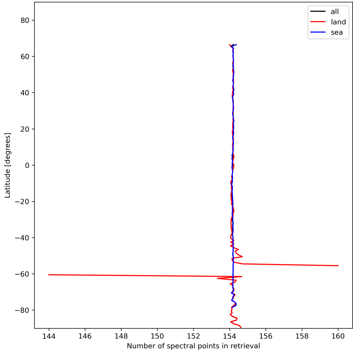
Figure 13: Zonal average of “Number of spectral points in retrieval” for 2023-11-15 to 2023-11-17.
