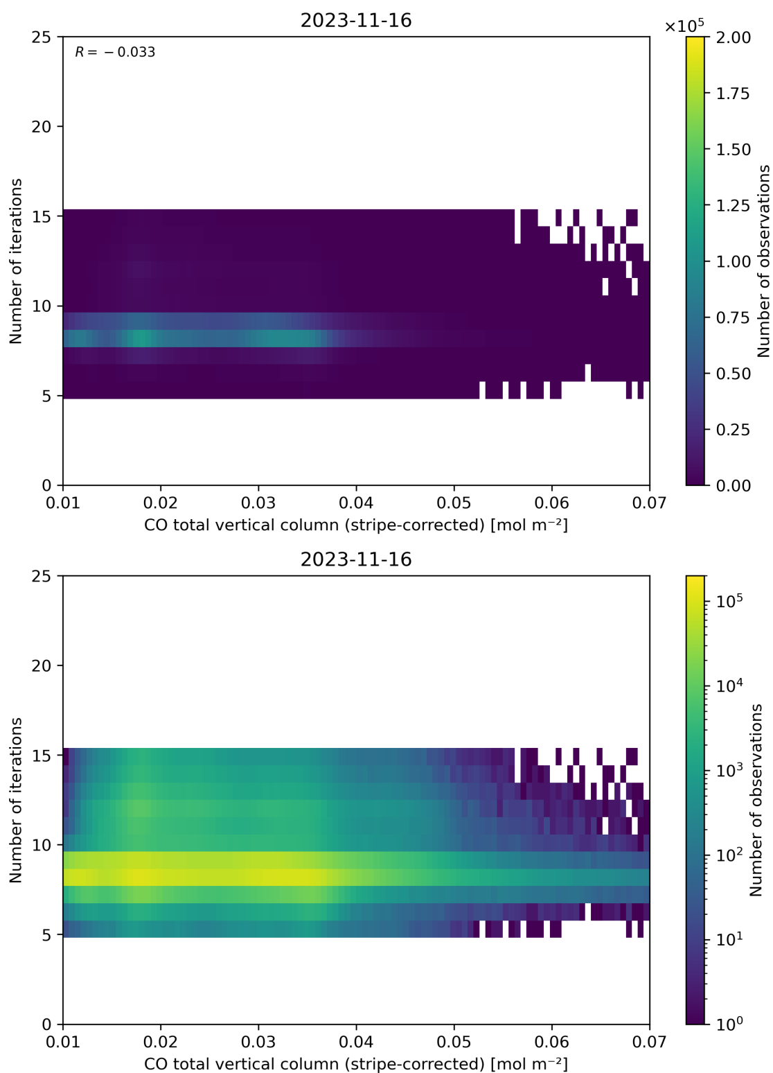
Figure 39: Scatter density plot of “CO total vertical column (stripe-corrected)” against “Number of iterations” for 2023-11-15 to 2023-11-17.
