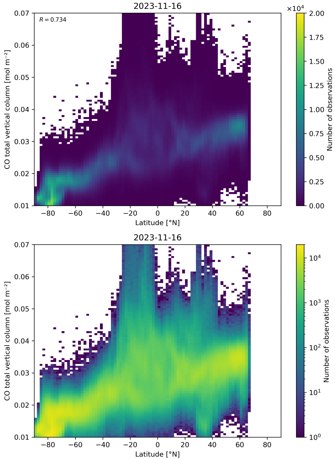
Figure 51: Scatter density plot of “Latitude” against “CO total vertical column” for 2023-11-15 to 2023-11-17.
