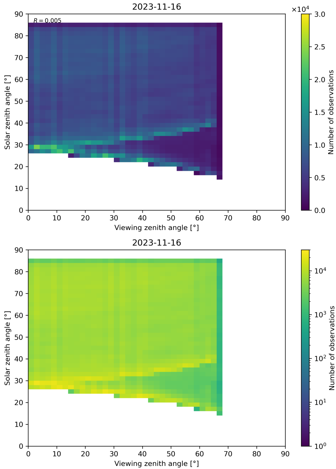
Figure 77: Scatter density plot of “Viewing zenith angle” against “Solar zenith angle” for 2023-11-15 to 2023-11-17.
