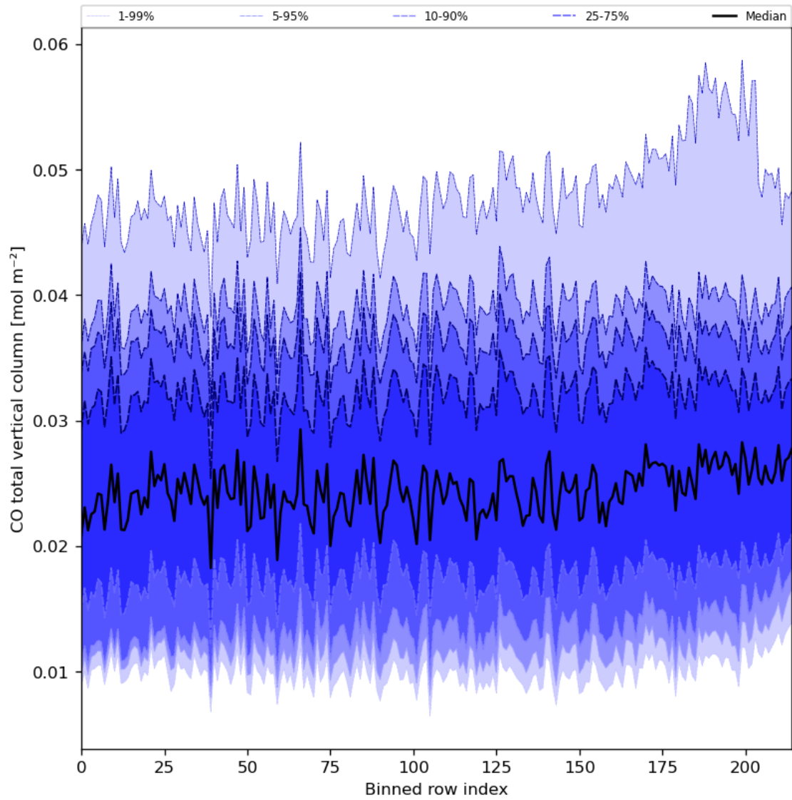
Figure 26: Along track statistics of “CO total vertical column” for 2023-11-15 to 2023-11-17
