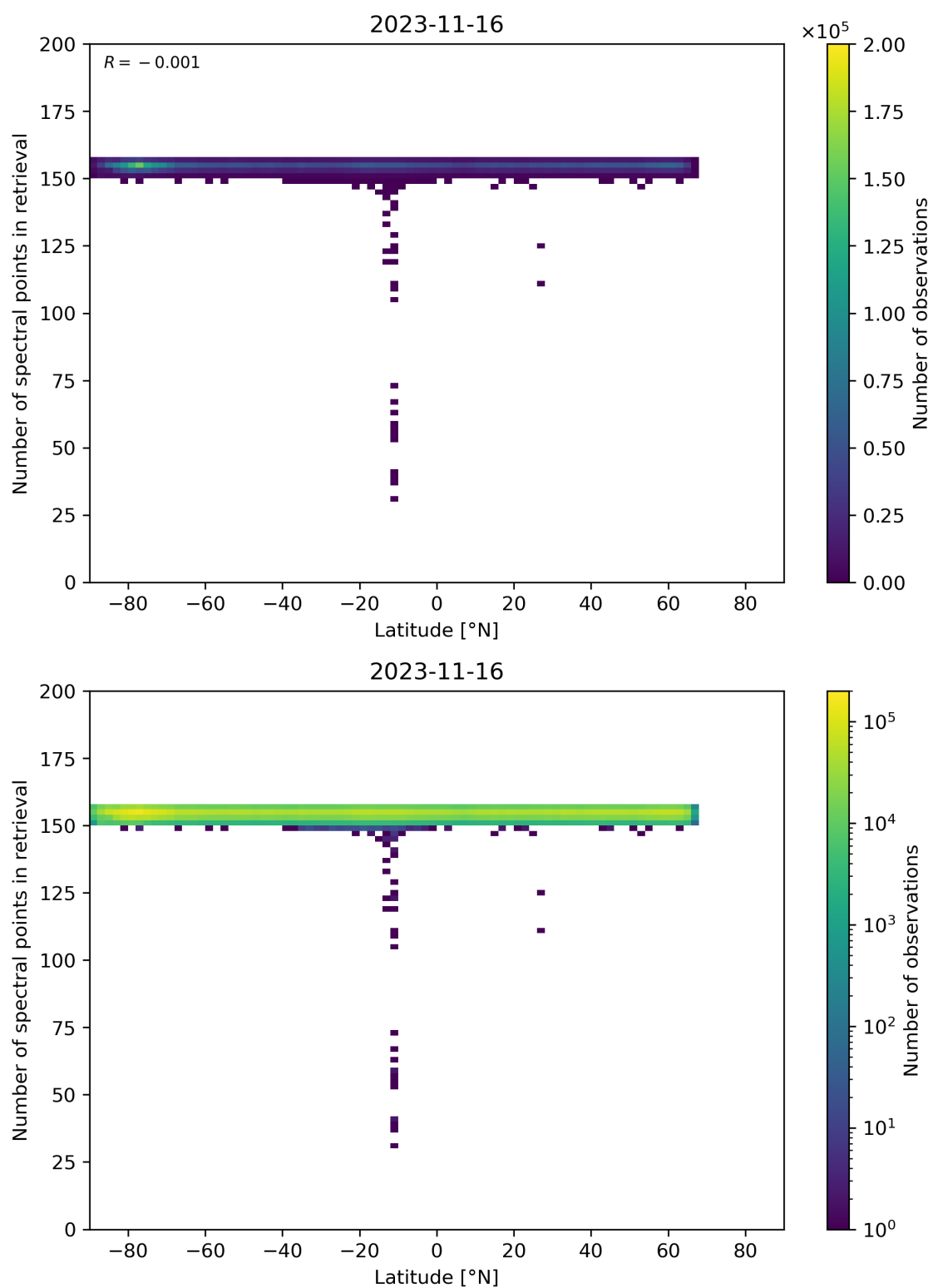
Figure 57: Scatter density plot of “Latitude” against “Number of spectral points in retrieval” for 2023-11-15 to 2023-11-17.
