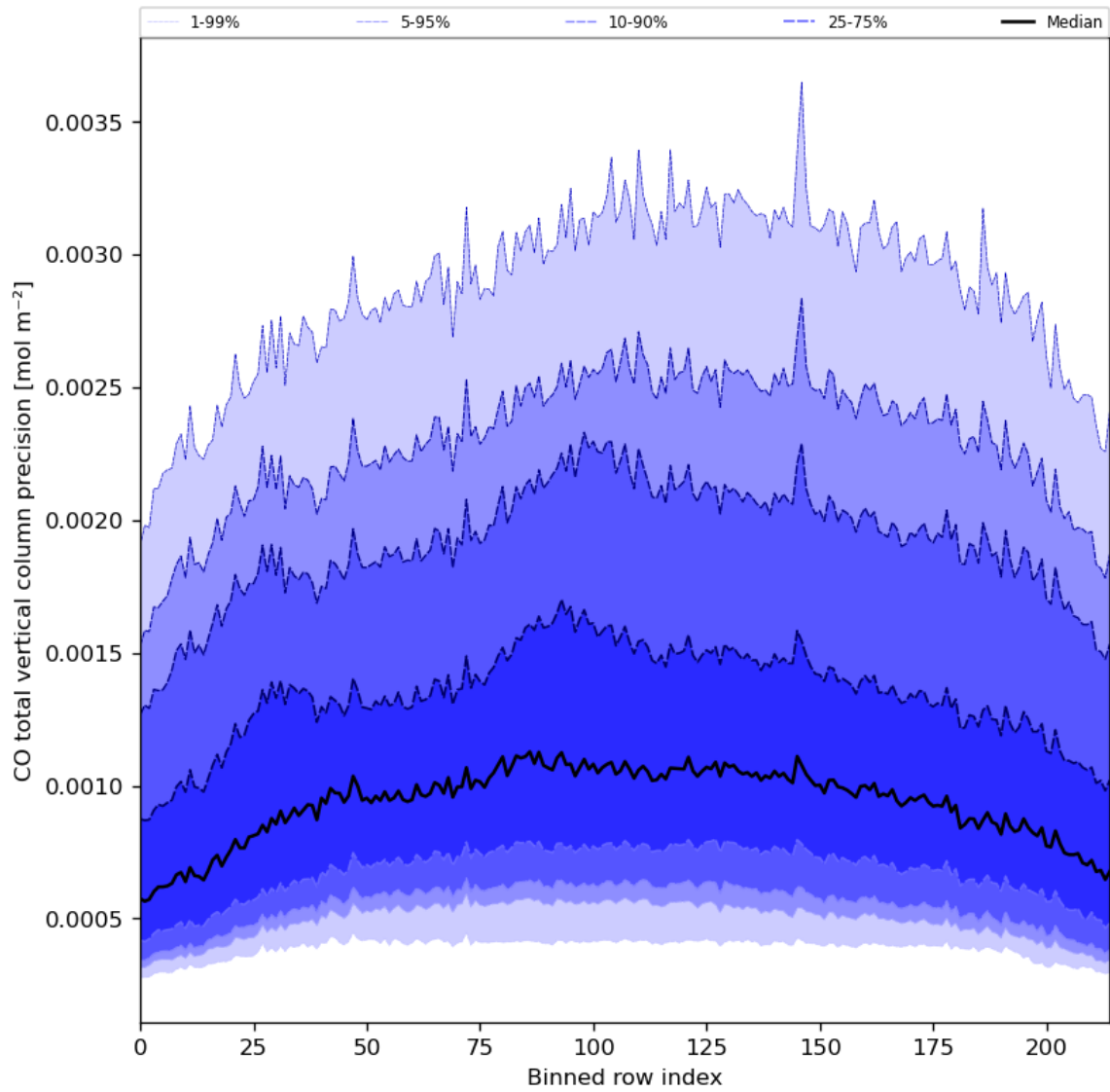
Figure 28: Along track statistics of “CO total vertical column precision” for 2023-11-15 to 2023-11-17
