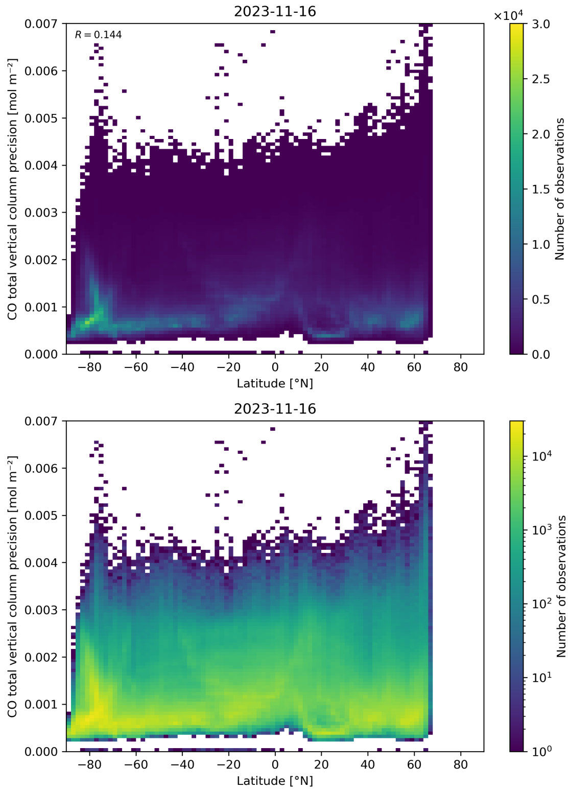
Figure 53: Scatter density plot of “Latitude” against “CO total vertical column precision” for 2023-11-15 to 2023-11-17.
