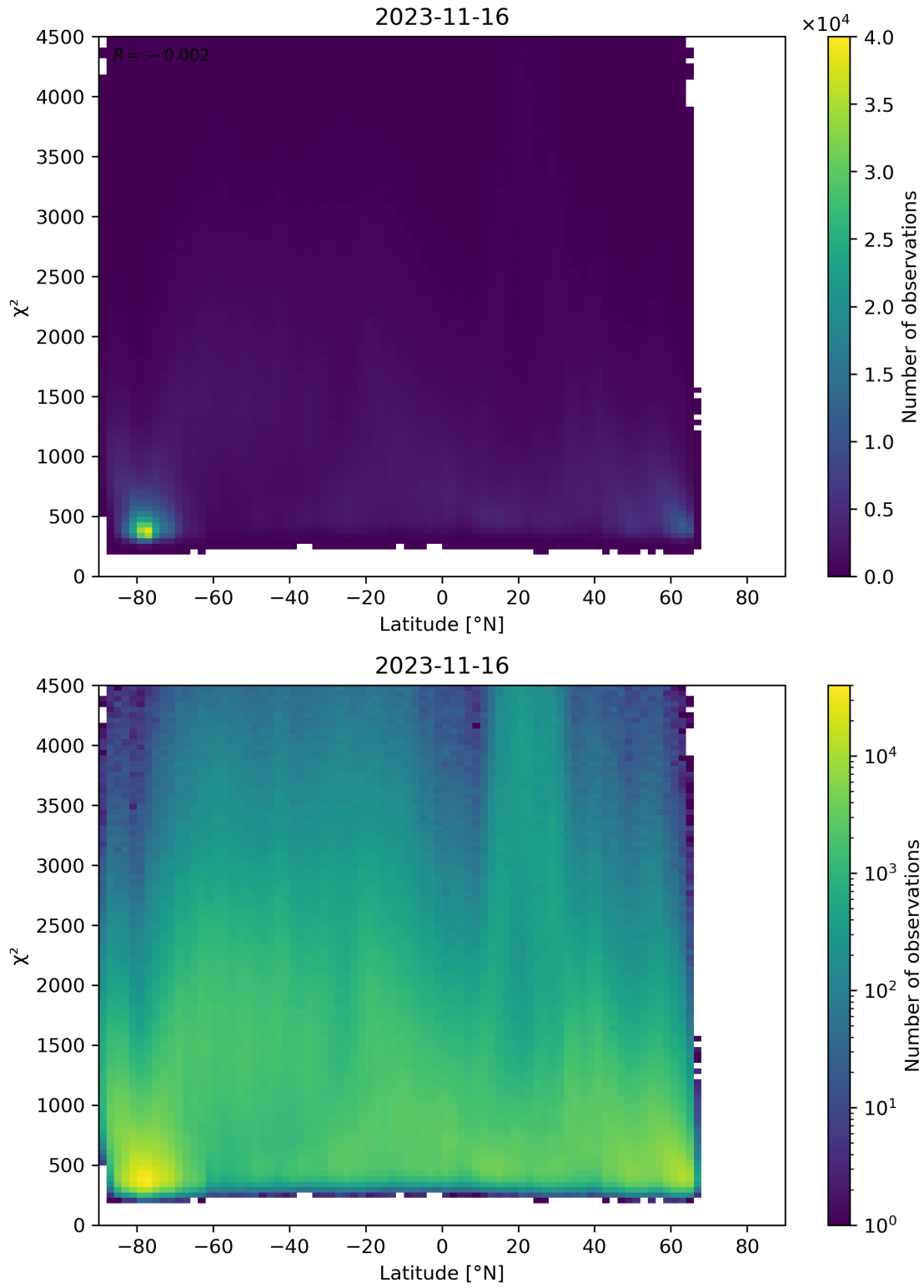
Figure 54: Scatter density plot of “Latitude” against “ \chi^2 ” for 2023-11-15 to 2023-11-17.
