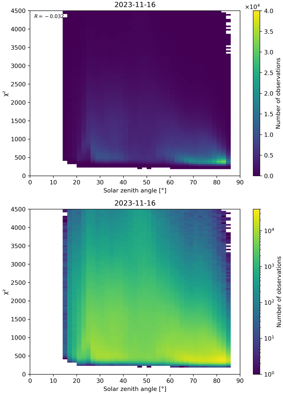
Figure 64: Scatter density plot of “Solar zenith angle” against “ \chi^2 ” for 2023-11-15 to 2023-11-17.
