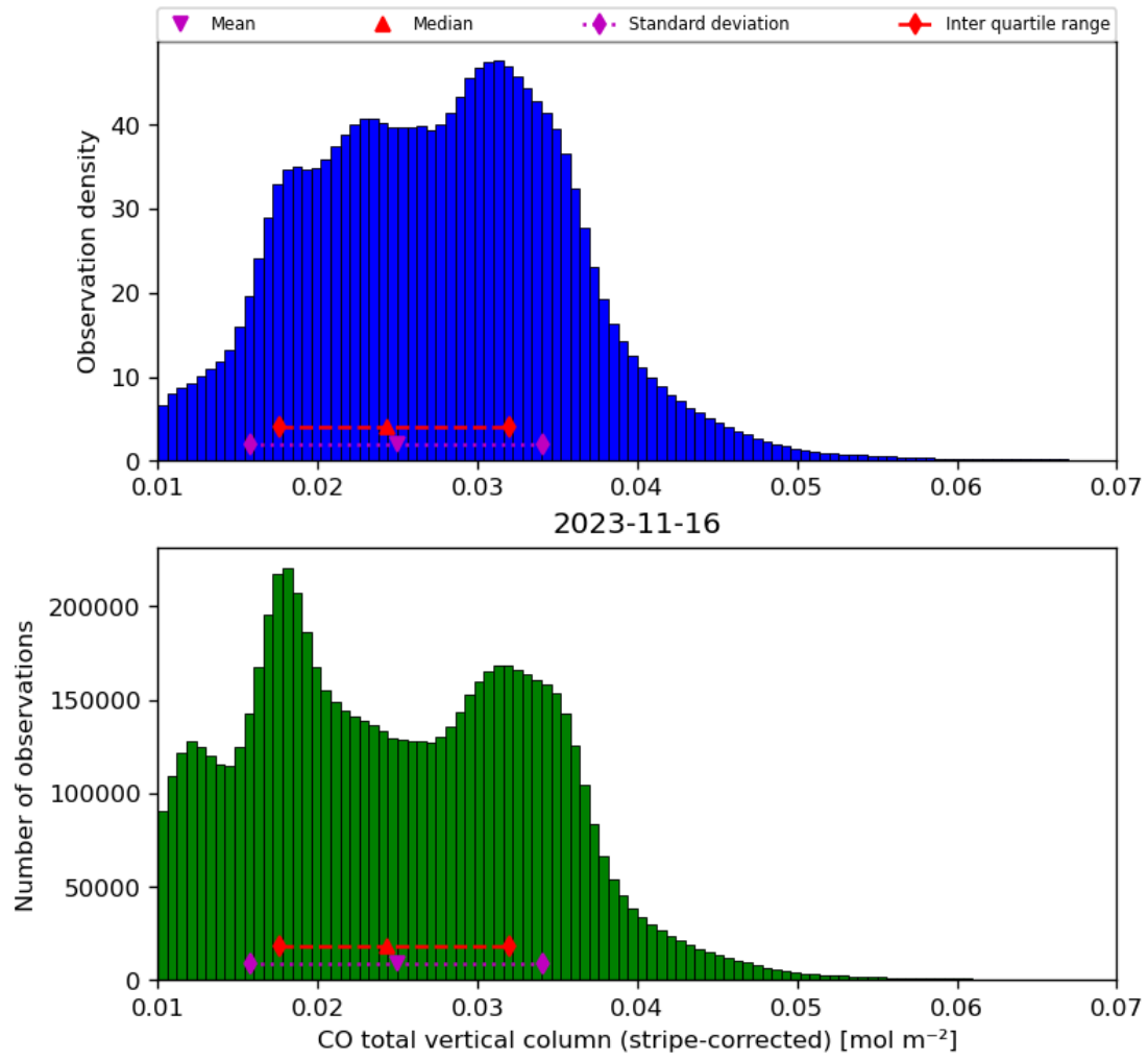
Figure 19: Histogram of “CO total vertical column (stripe-corrected)” for 2023-11-15 to 2023-11-17
