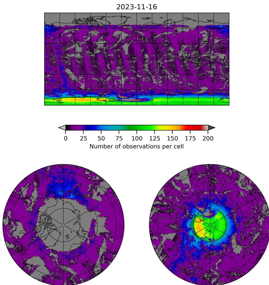
Figure 8: Map of the number of observations for 2023-11-15 to 2023-11-17
