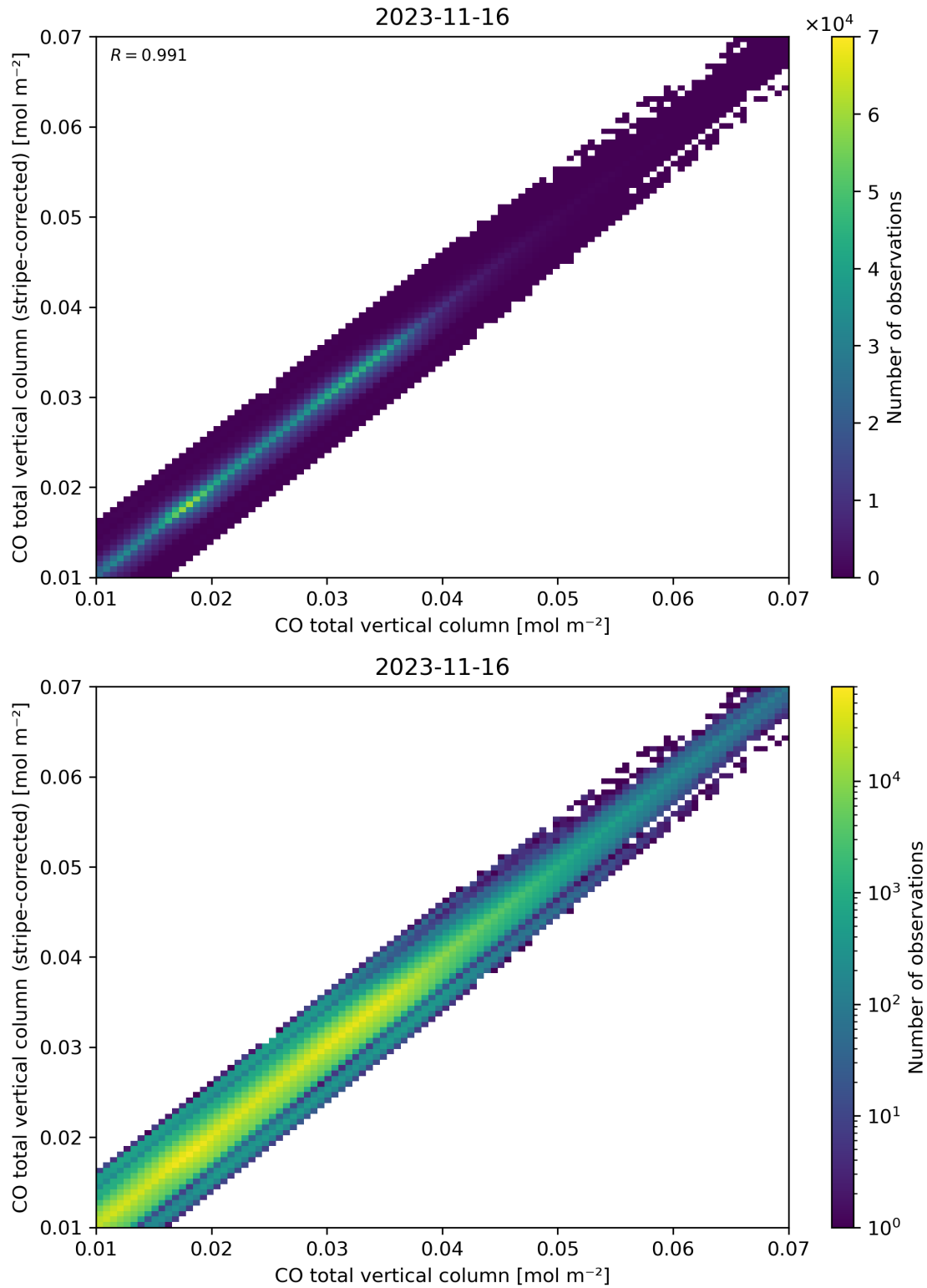
Figure 33: Scatter density plot of “CO total vertical column” against “CO total vertical column (stripe-corrected)” for 2023-11-15 to 2023-11-17.
