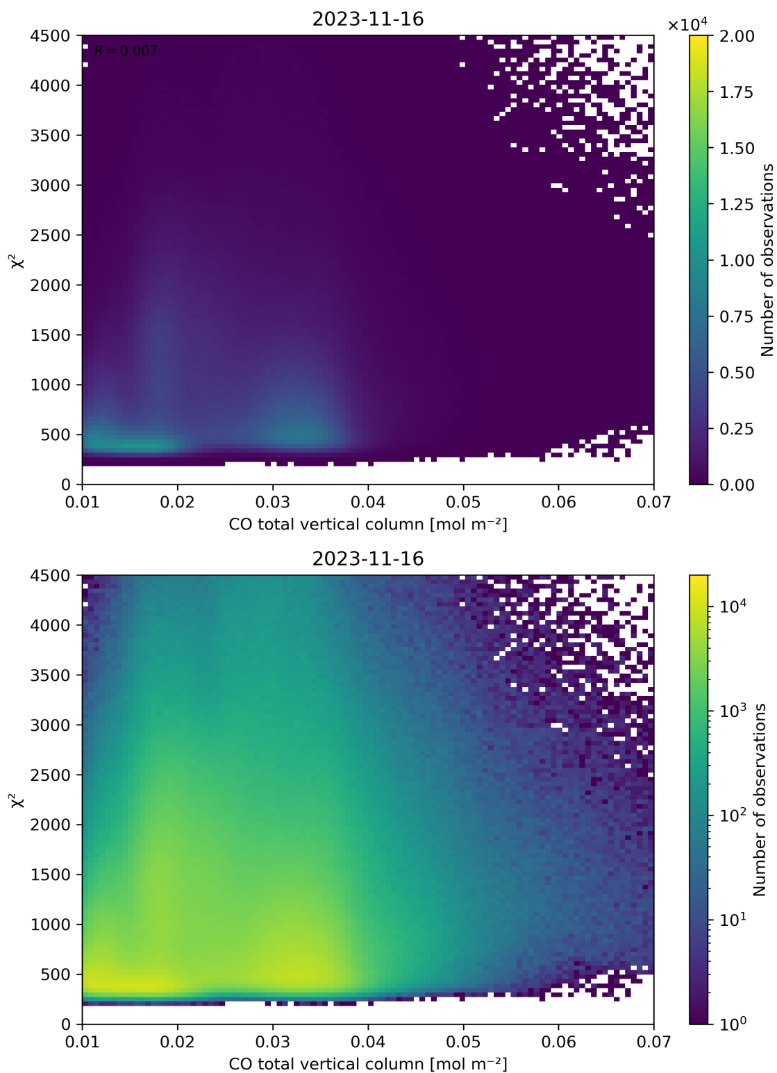
Figure 35: Scatter density plot of “CO total vertical column” against “ \chi^2 ” for 2023-11-15 to 2023-11-17.
