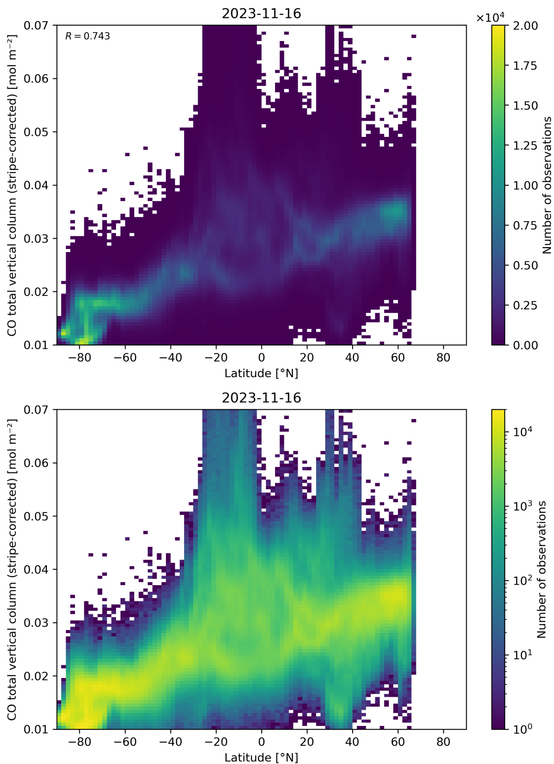
Figure 52: Scatter density plot of “Latitude” against “CO total vertical column (stripe-corrected)” for 2023-11-15 to 2023-11-17.
