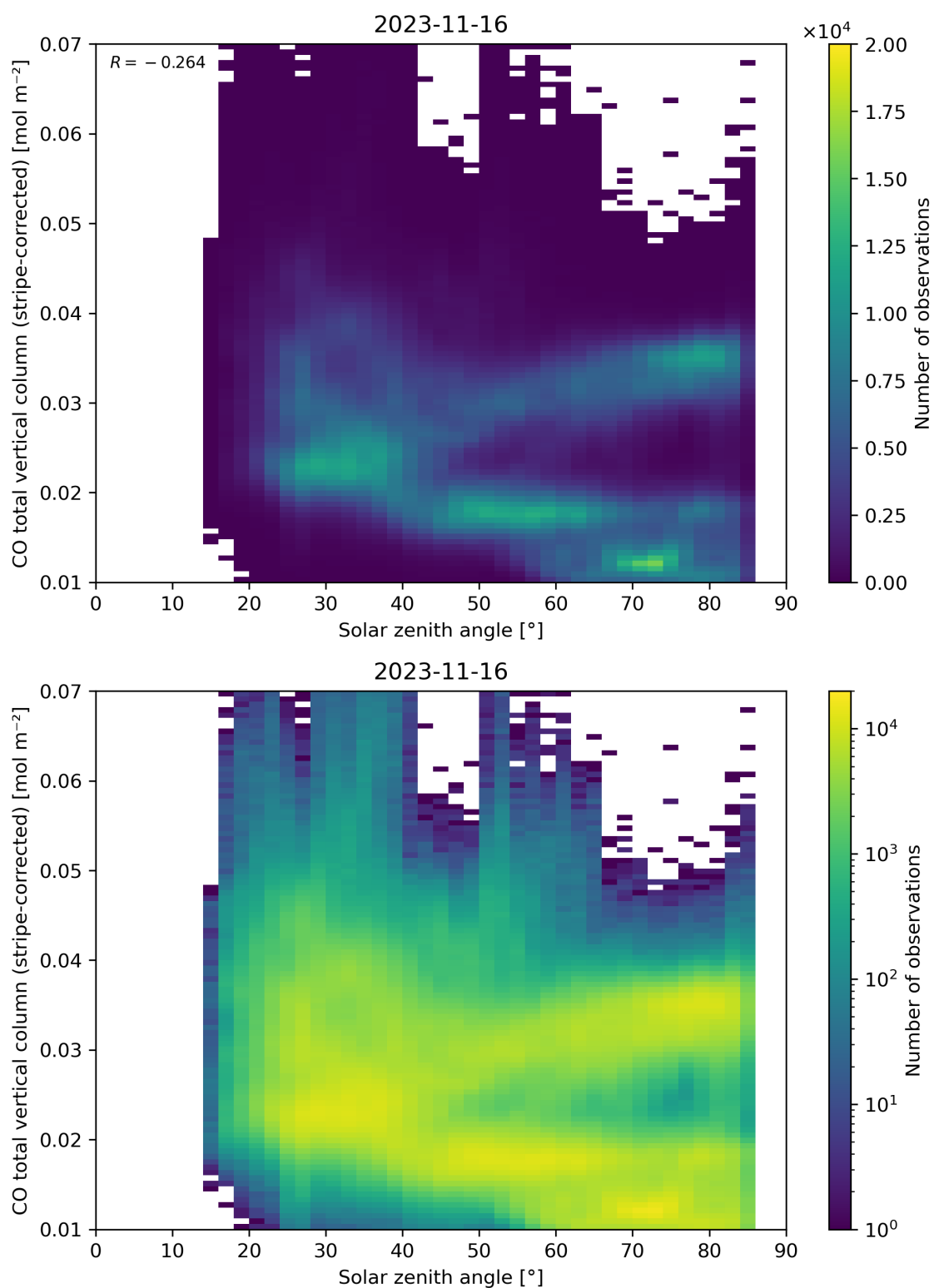
Figure 62: Scatter density plot of “Solar zenith angle” against “CO total vertical column (stripe-corrected)” for 2023-11-15 to 2023-11-17.
