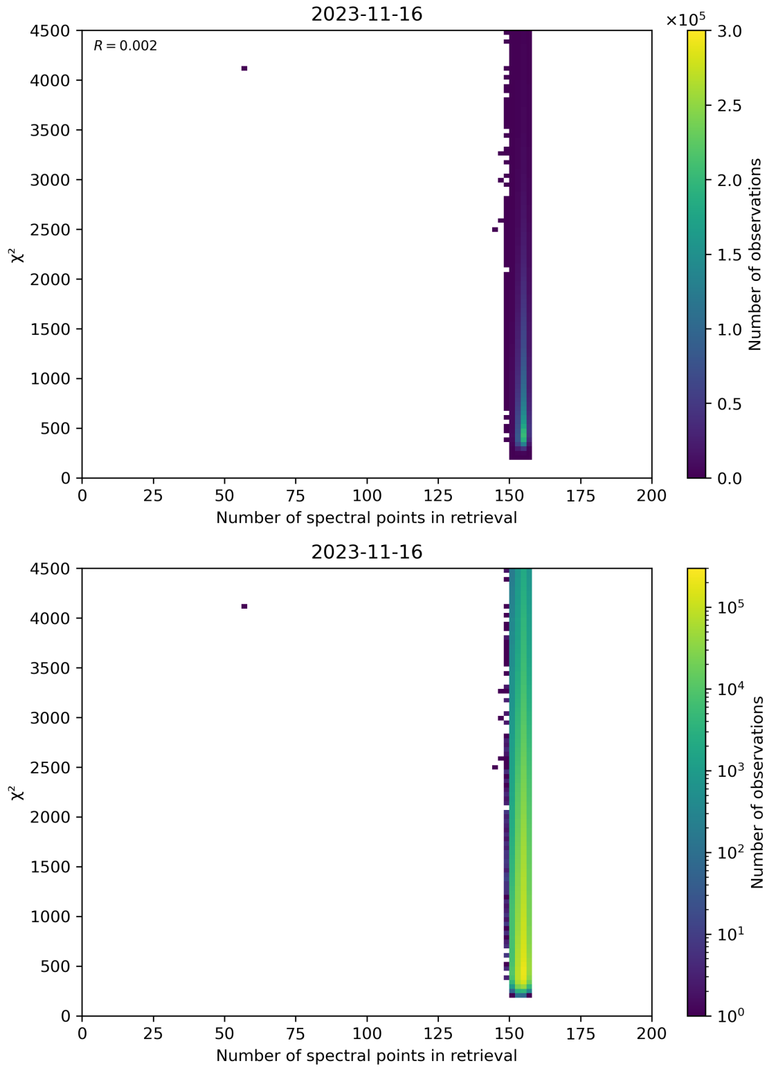
Figure 58: Scatter density plot of “Number of spectral points in retrieval” against “ \chi^2 ” for 2023-11-15 to 2023-11-17.
