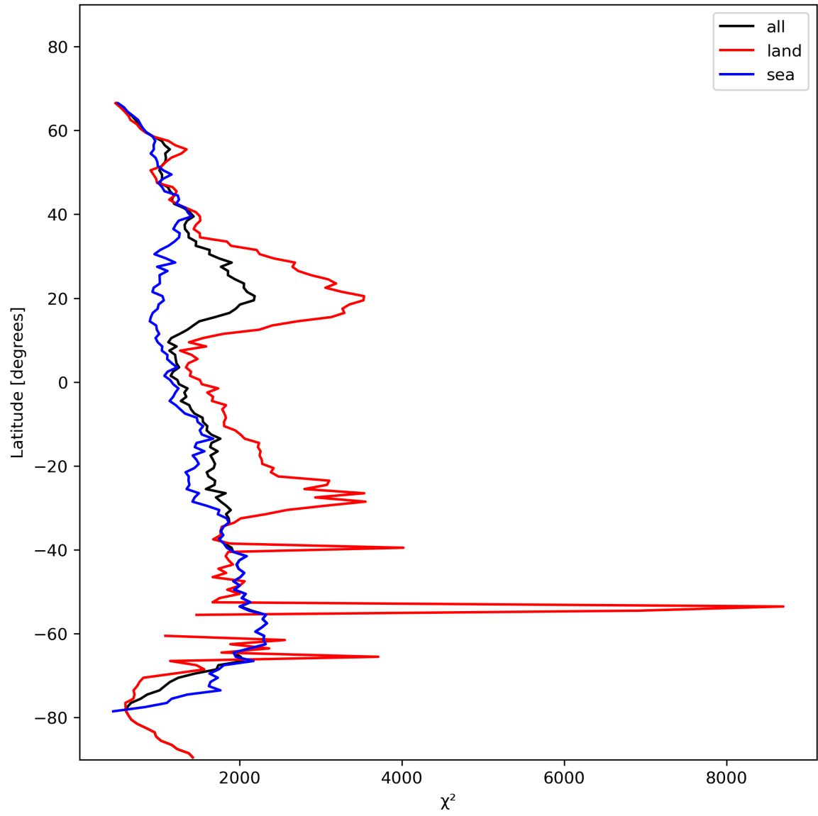
Figure 14: Zonal average of “ \chi^2 ” for 2023-11-15 to 2023-11-17.
