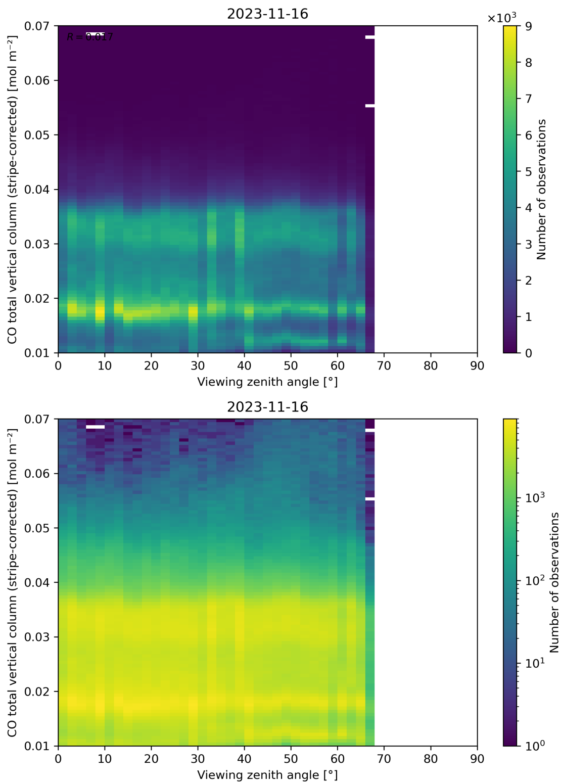
Figure 70: Scatter density plot of “Viewing zenith angle” against “CO total vertical column (stripe-corrected)” for 2023-11-15 to 2023-11-17.
