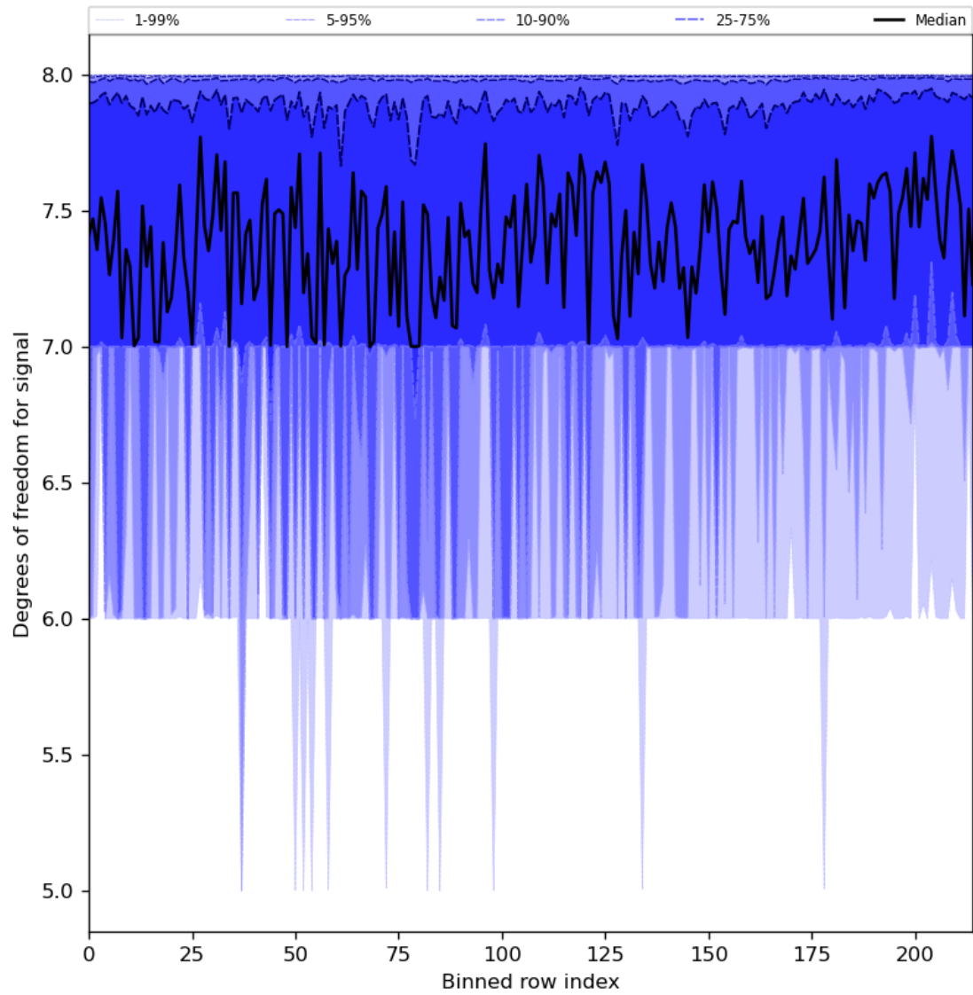
Figure 31: Along track statistics of “Degrees of freedom for signal” for 2023-11-15 to 2023-11-17
