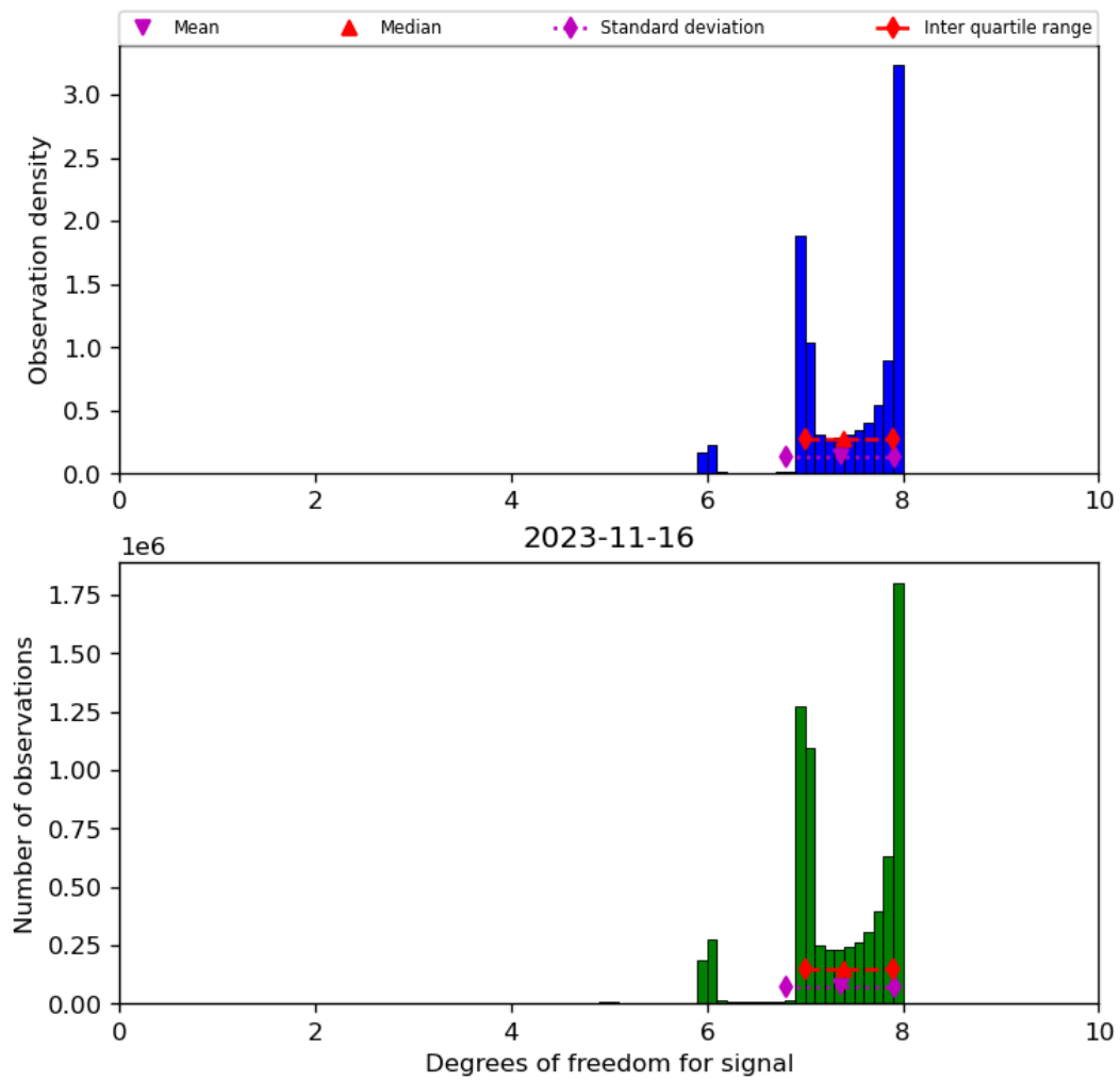
Figure 23: Histogram of “Degrees of freedom for signal” for 2023-11-15 to 2023-11-17
