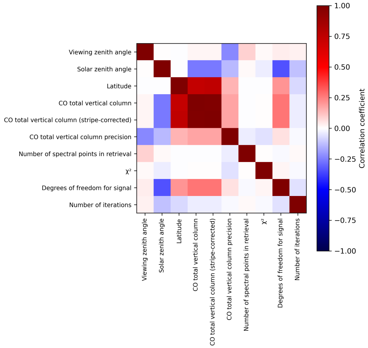
Figure 2: Map of correlation matrix for 2023-11-15 to 2023-11-17.
