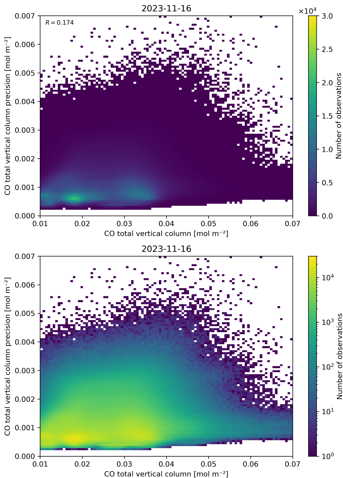
Figure 34: Scatter density plot of “CO total vertical column” against “CO total vertical column precision” for 2023-11-15 to 2023-11-17.
