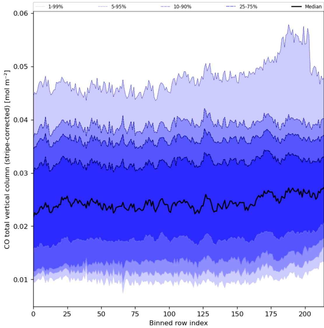
Figure 27: Along track statistics of “CO total vertical column (stripe-corrected)” for 2023-11-15 to 2023-11-17
