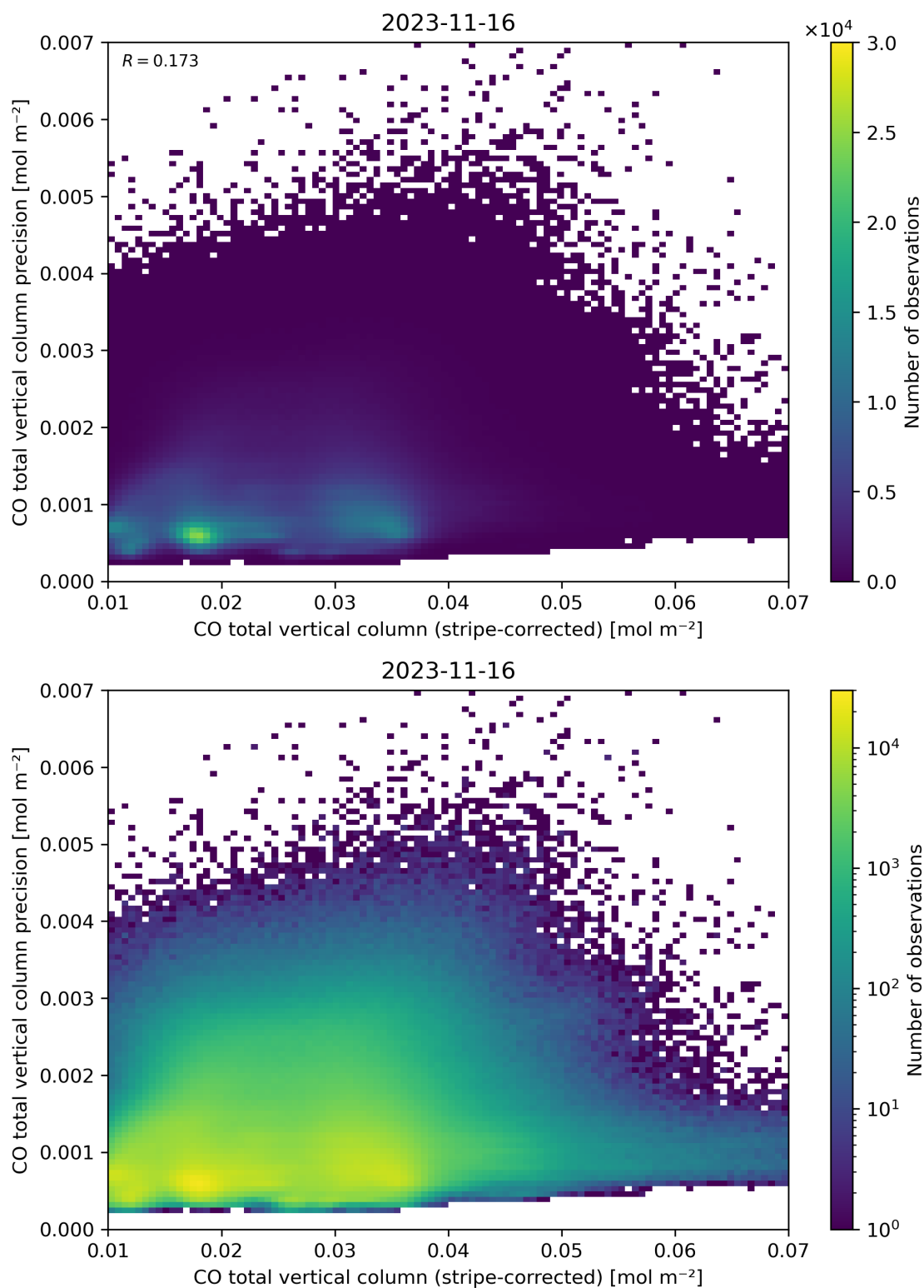
Figure 36: Scatter density plot of “CO total vertical column (stripe-corrected)” against “CO total vertical column precision” for 2023-11-15 to 2023-11-17.
