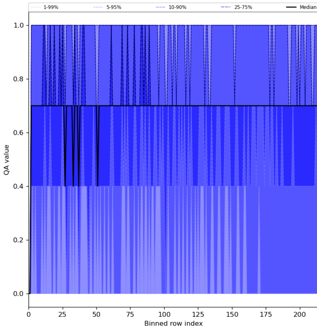
Figure 25: Along track statistics of “QA value” for 2023-11-15 to 2023-11-17
