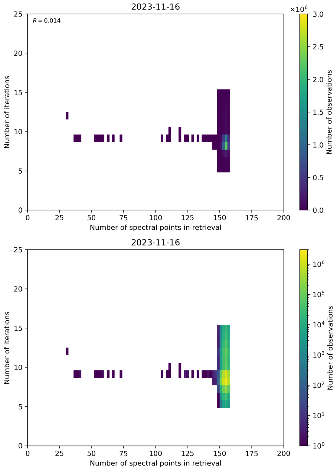
Figure 60: Scatter density plot of “Number of spectral points in retrieval” against “Number of iterations” for 2023-11-15 to 2023-11-17.
