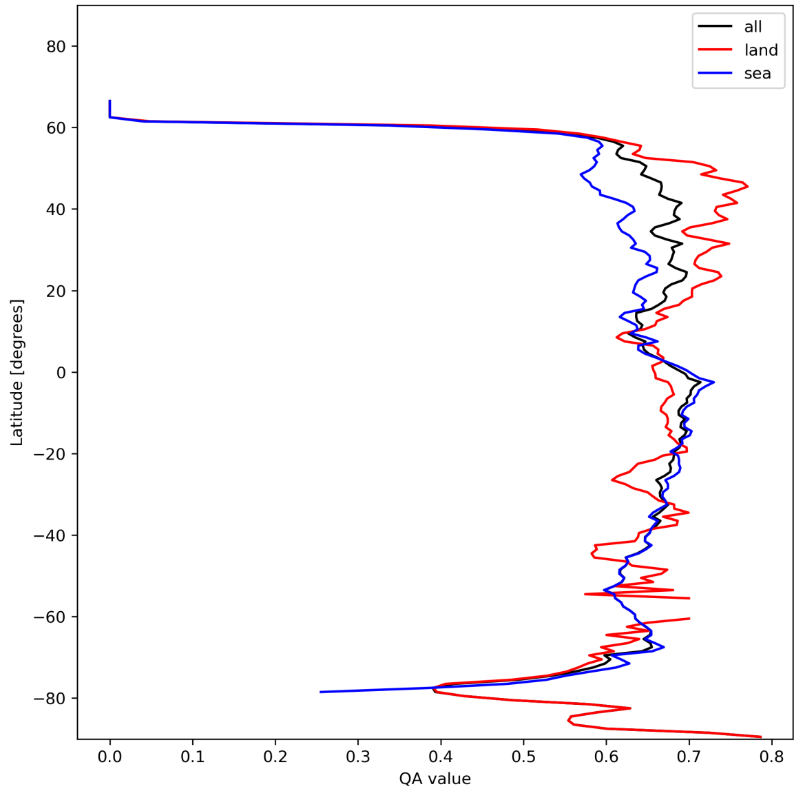
Figure 9: Zonal average of “QA value” for 2023-11-15 to 2023-11-17.
