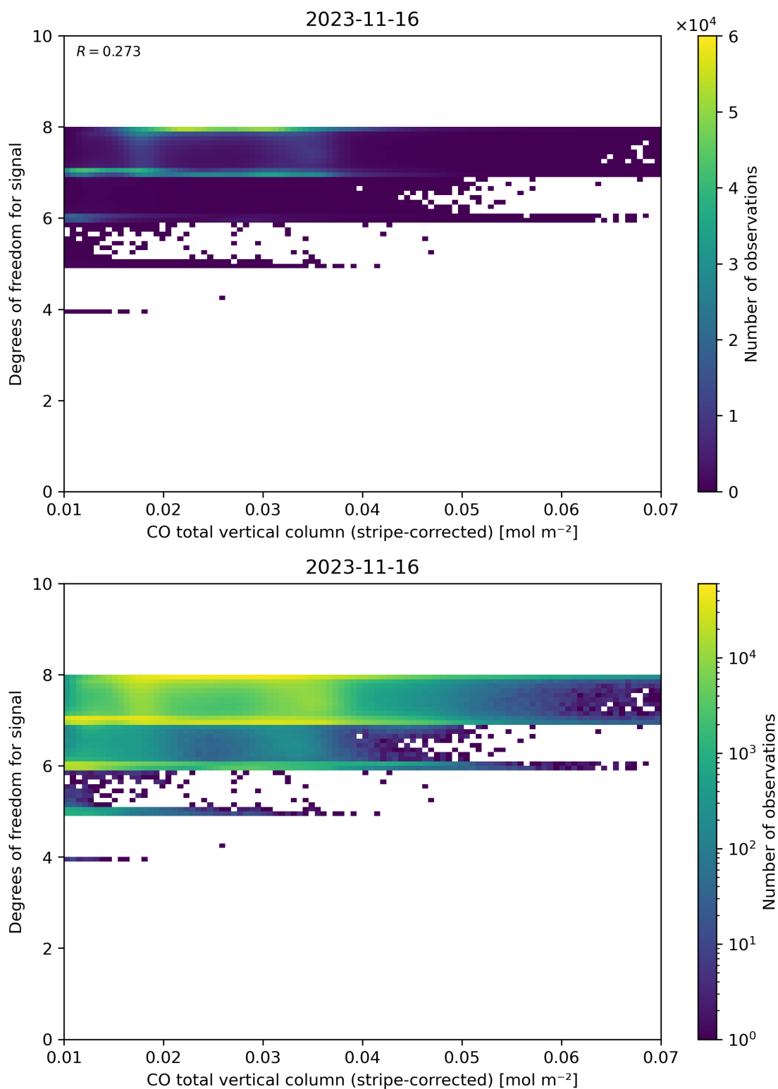
Figure 38: Scatter density plot of “CO total vertical column (stripe-corrected)” against “Degrees of freedom for signal” for 2023-11-15 to 2023-11-17.
