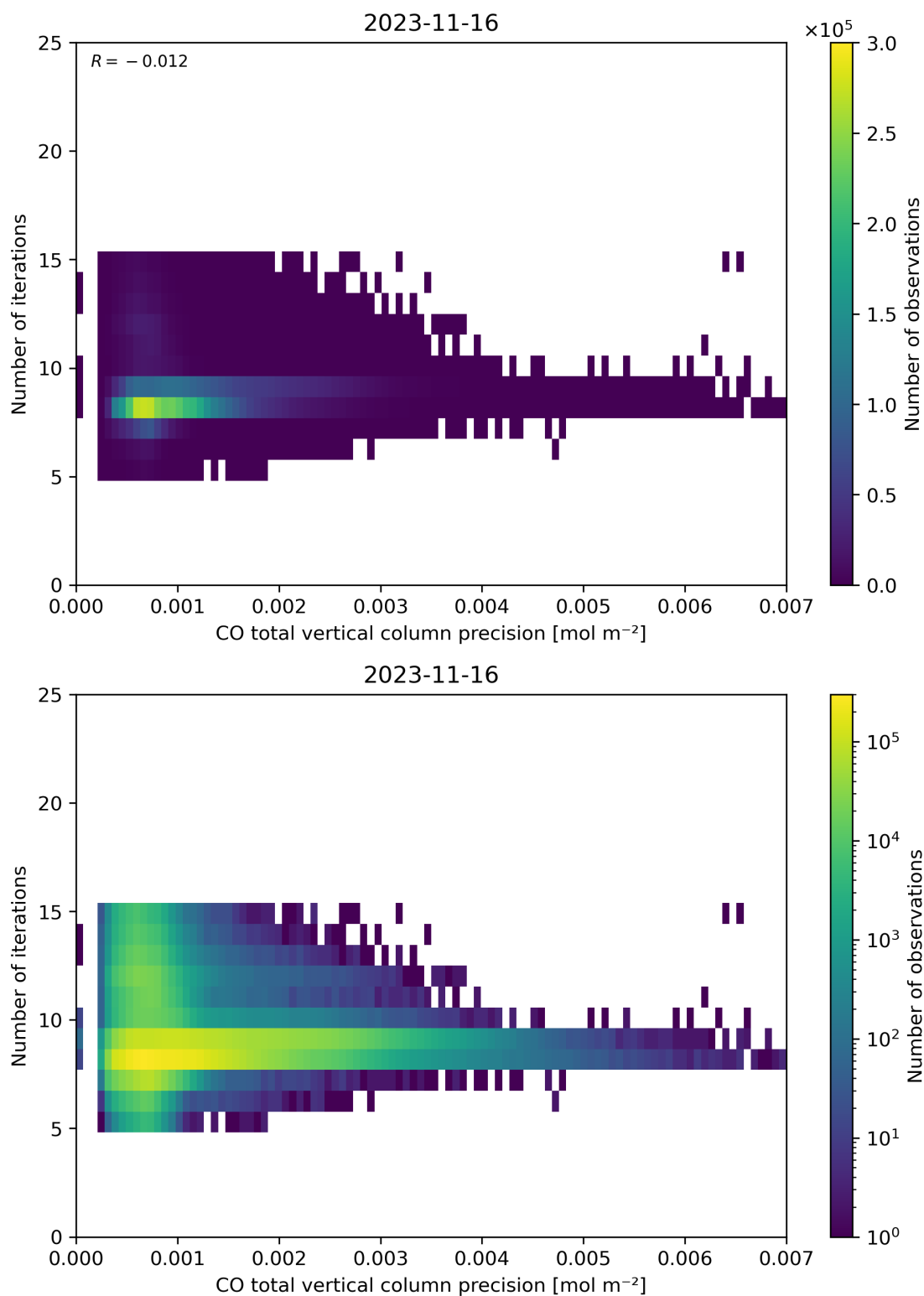
Figure 46: Scatter density plot of “CO total vertical column precision” against “Number of iterations” for 2023-11-15 to 2023-11-17.
