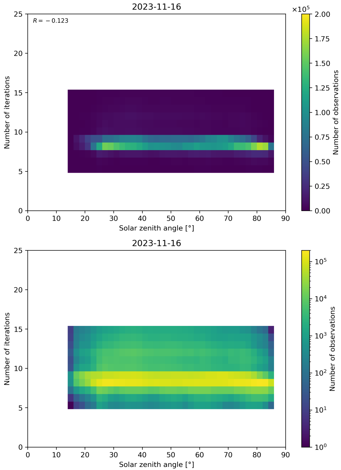
Figure 67: Scatter density plot of “Solar zenith angle” against “Number of iterations” for 2023-11-15 to 2023-11-17.
