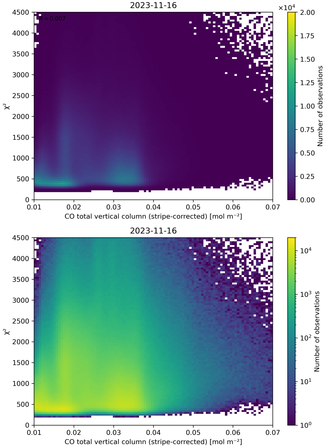
Figure 37: Scatter density plot of “CO total vertical column (stripe-corrected)” against “ \chi^2 ” for 2023-11-15 to 2023-11-17.
