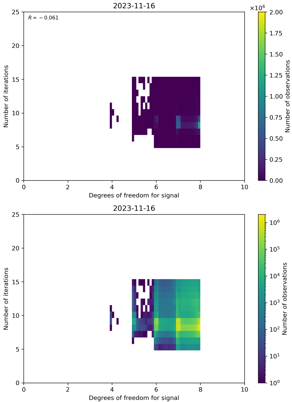
Figure 50: Scatter density plot of “Degrees of freedom for signal” against “Number of iterations” for 2023-11-15 to 2023-11-17.
