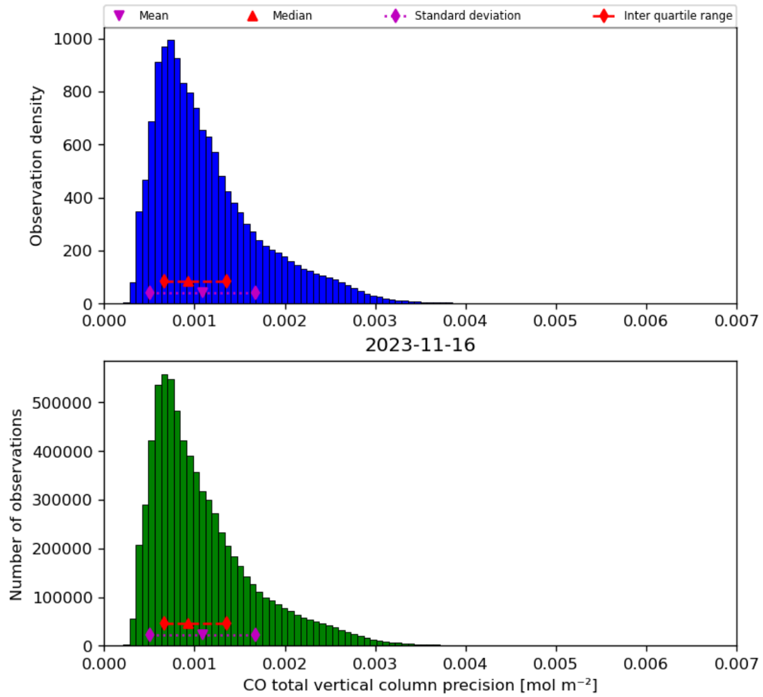
Figure 20: Histogram of “CO total vertical column precision” for 2023-11-15 to 2023-11-17
