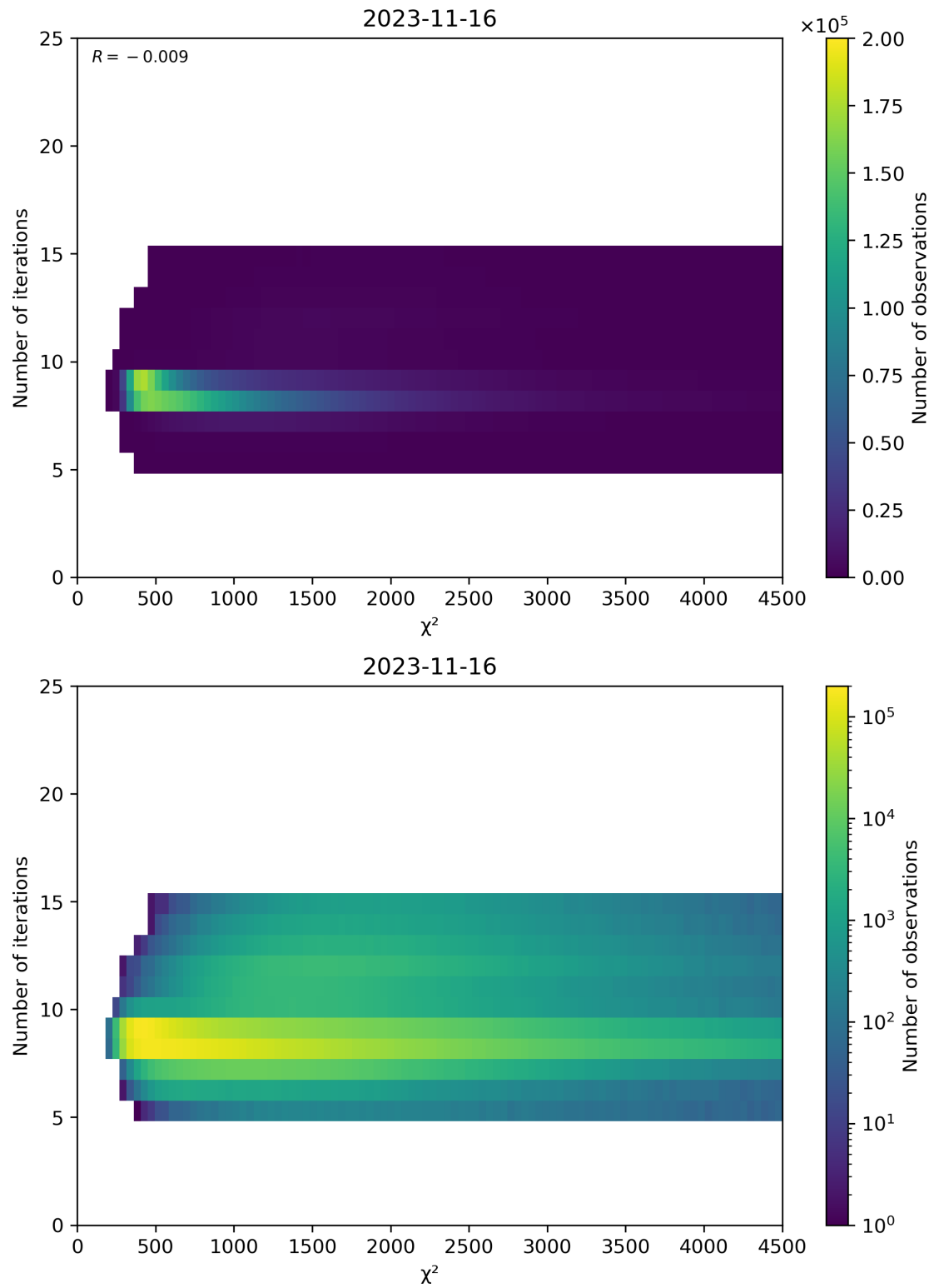
Figure 49: Scatter density plot of “ \chi^2 ” against “Number of iterations” for 2023-11-15 to 2023-11-17.
