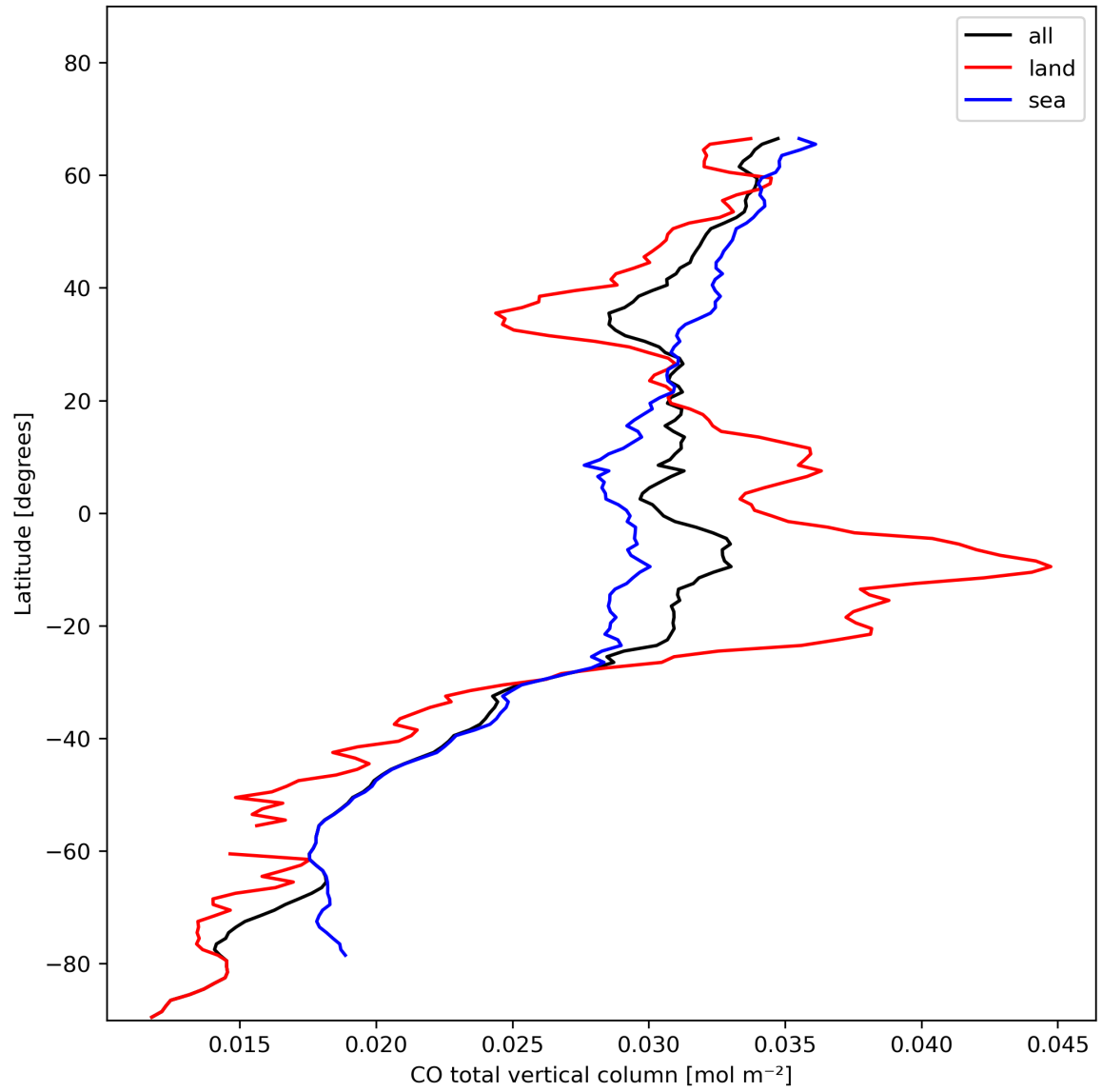
Figure 10: Zonal average of “CO total vertical column” for 2023-11-15 to 2023-11-17.
