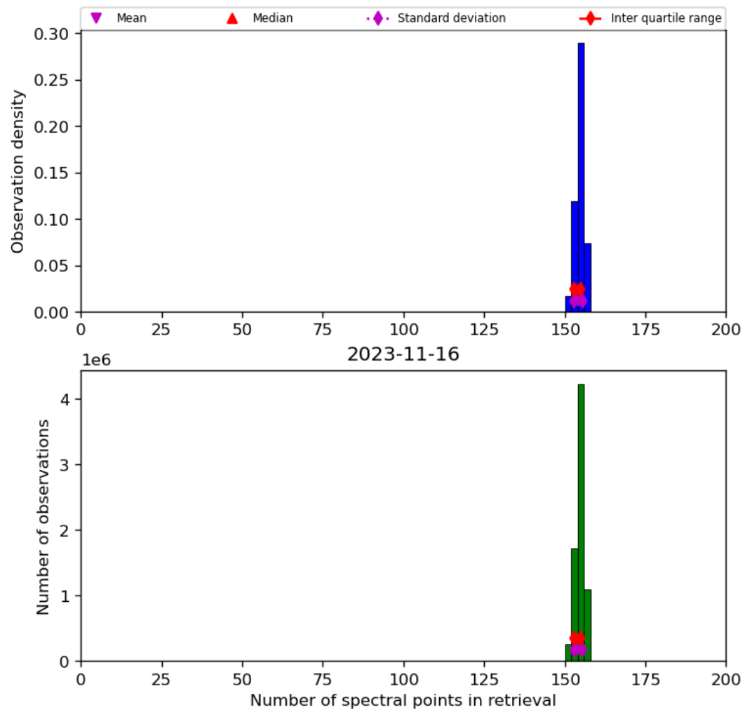
Figure 21: Histogram of “Number of spectral points in retrieval” for 2023-11-15 to 2023-11-17
