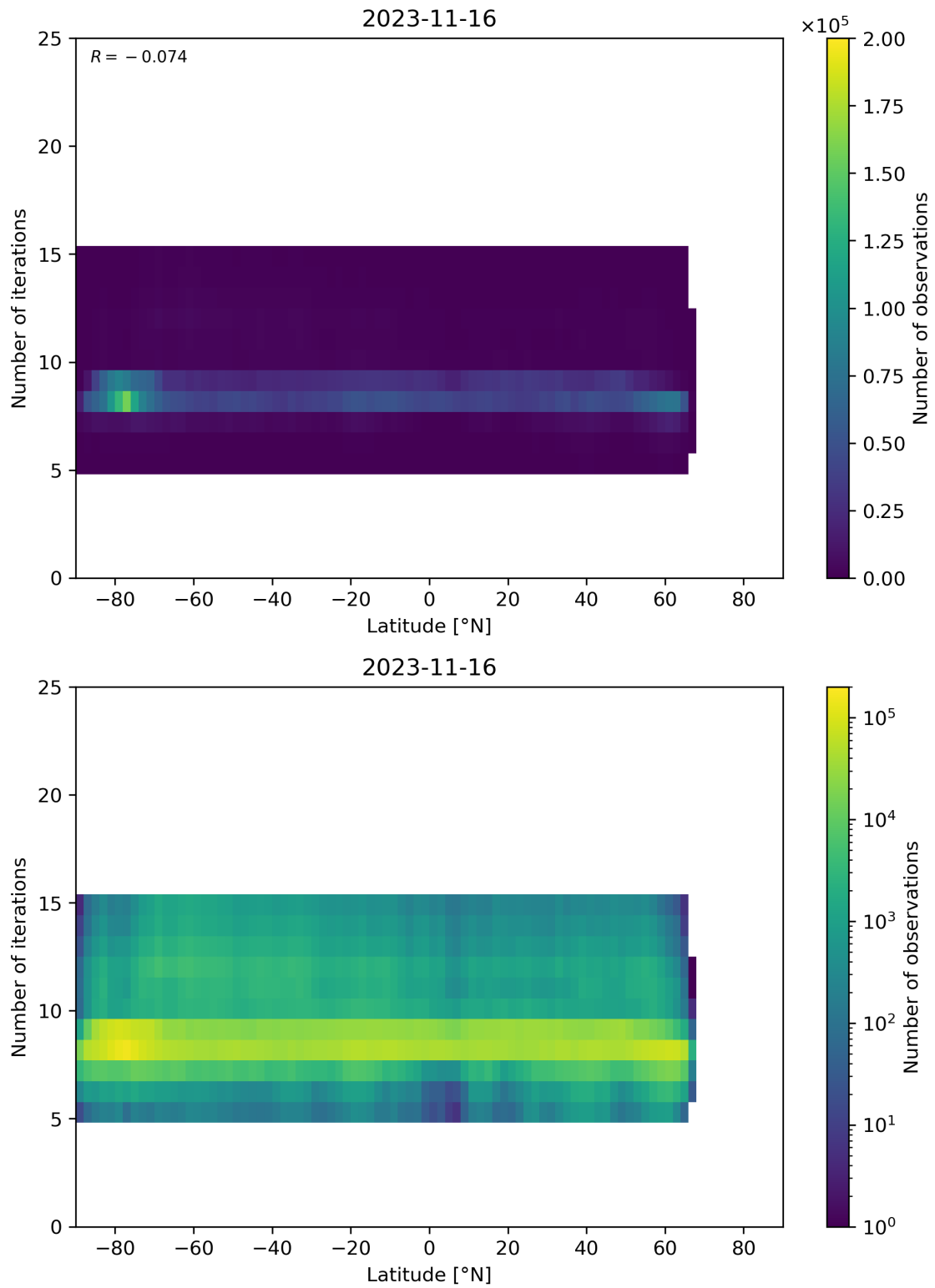
Figure 56: Scatter density plot of “Latitude” against “Number of iterations” for 2023-11-15 to 2023-11-17.
