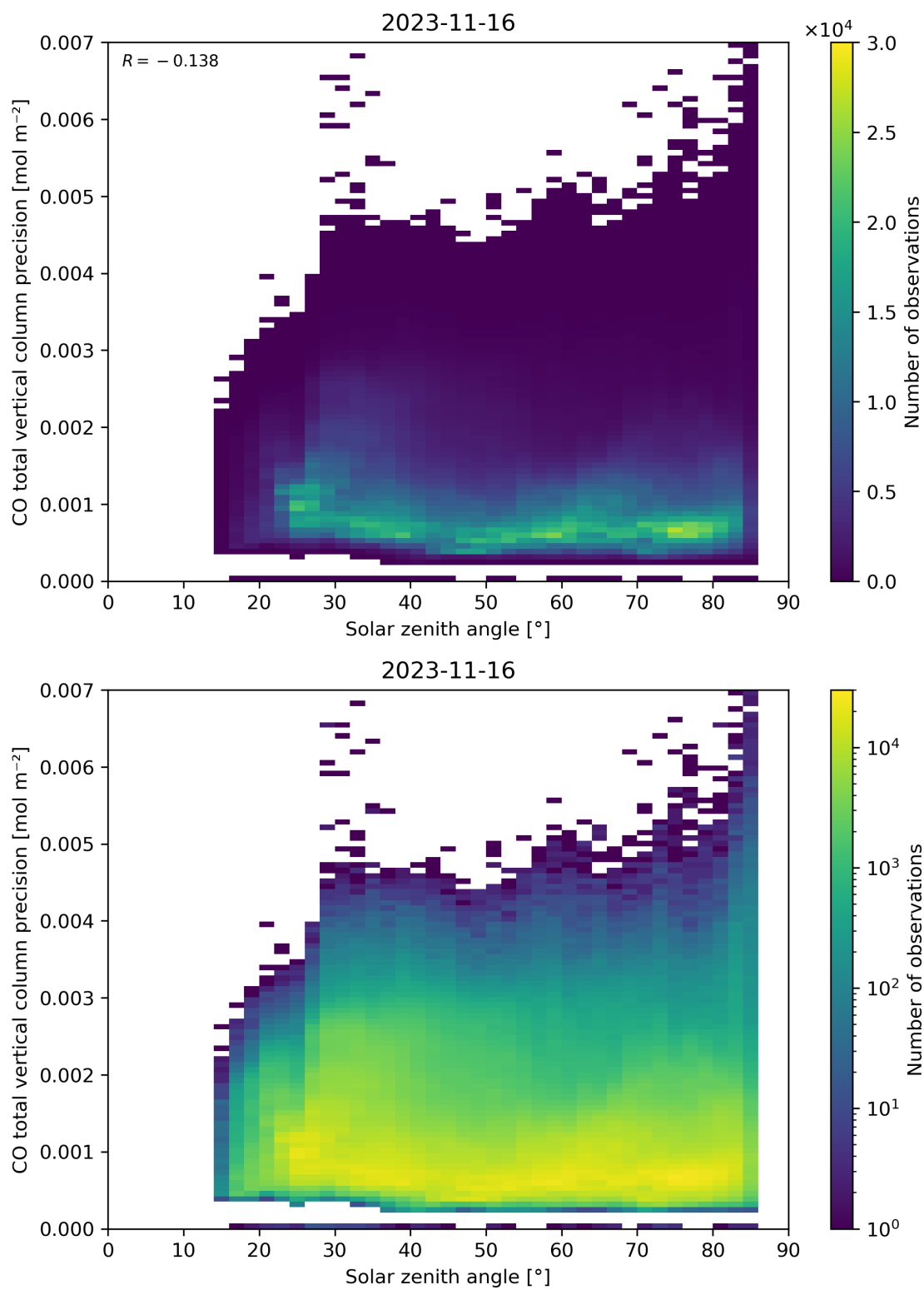
Figure 63: Scatter density plot of “Solar zenith angle” against “CO total vertical column precision” for 2023-11-15 to 2023-11-17.
