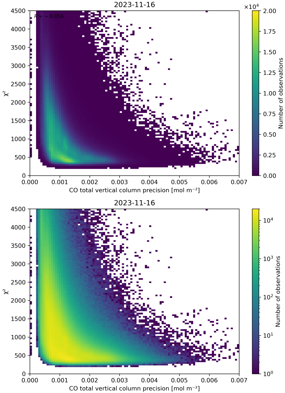
Figure 44: Scatter density plot of “CO total vertical column precision” against “ \chi^2 ” for 2023-11-15 to 2023-11-17.
