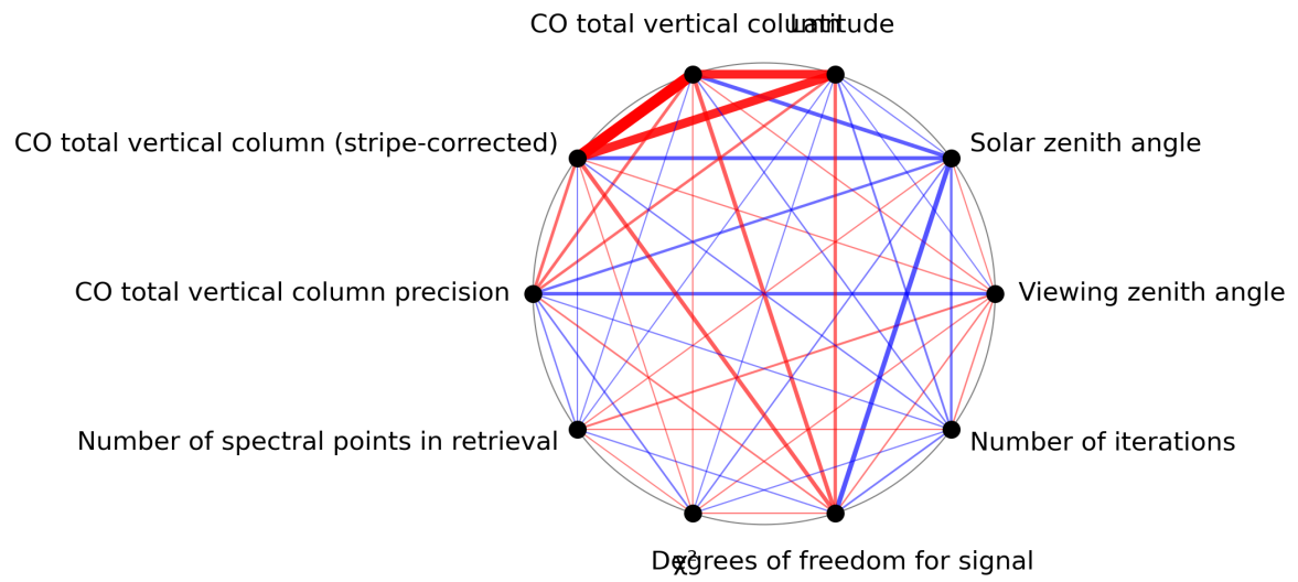
Figure 1: Map of correlation graph for 2023-11-15 to 2023-11-17.
