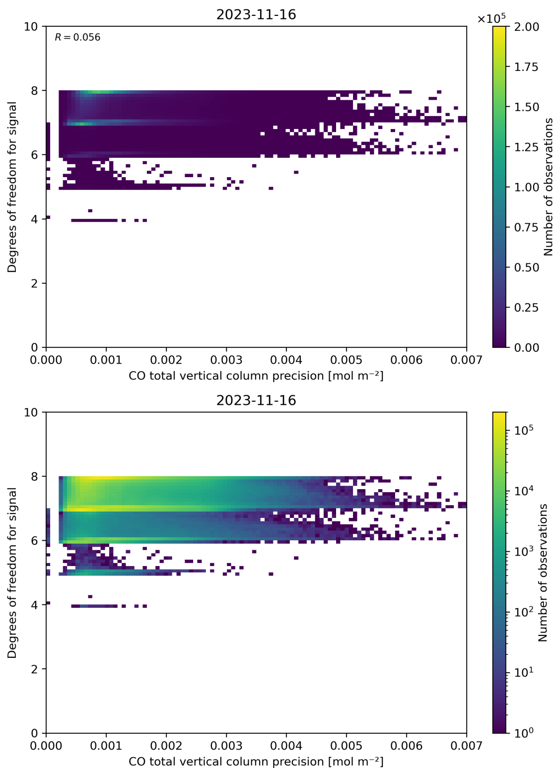
Figure 45: Scatter density plot of “CO total vertical column precision” against “Degrees of freedom for signal” for 2023-11-15 to 2023-11-17.
