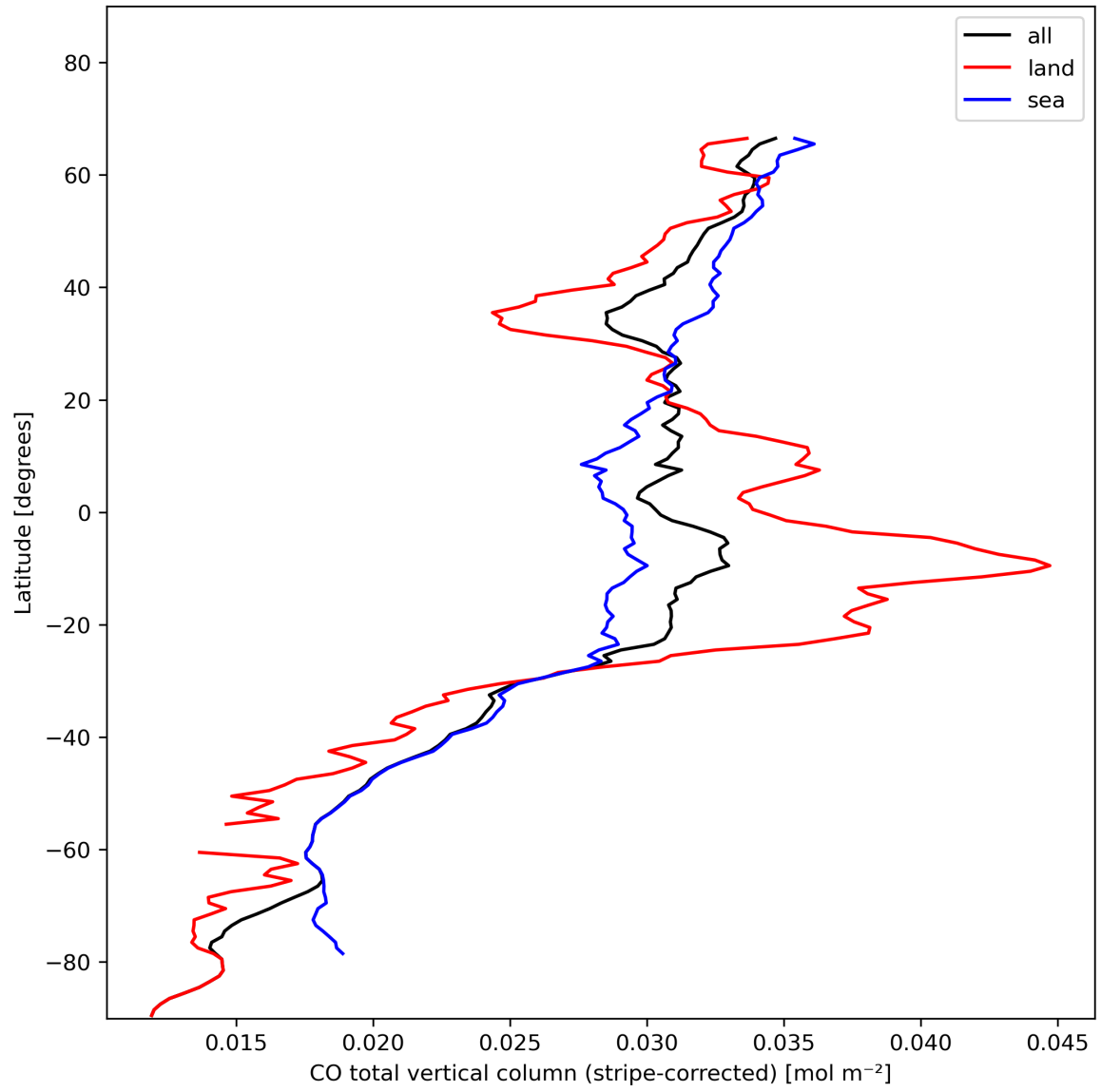
Figure 11: Zonal average of “CO total vertical column (stripe-corrected)” for 2023-11-15 to 2023-11-17.
