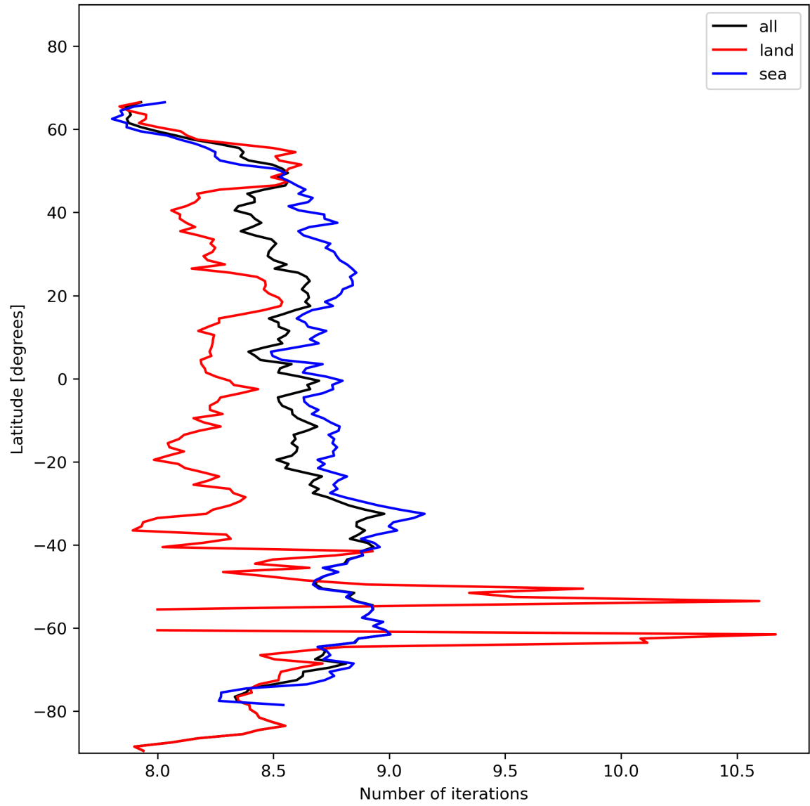
Figure 16: Zonal average of “Number of iterations” for 2023-11-15 to 2023-11-17.
