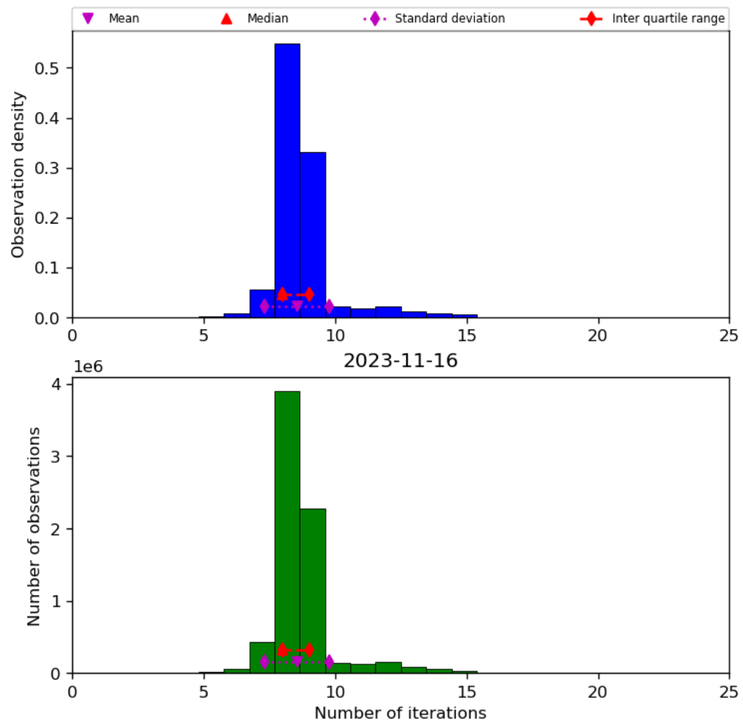
Figure 24: Histogram of “Number of iterations” for 2023-11-15 to 2023-11-17
