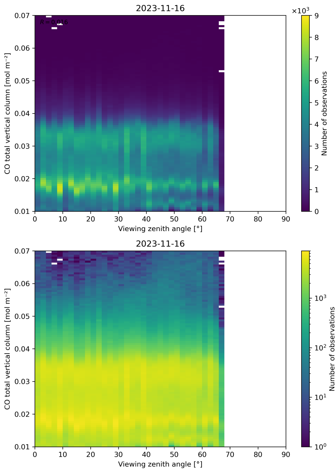
Figure 69: Scatter density plot of “Viewing zenith angle” against “CO total vertical column” for 2023-11-15 to 2023-11-17.
