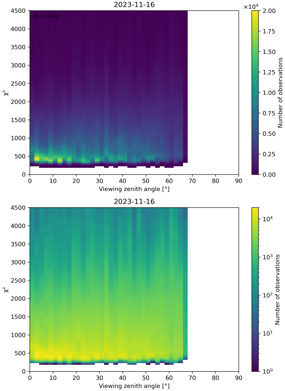
Figure 72: Scatter density plot of “Viewing zenith angle” against “ \chi^2 ” for 2023-11-15 to 2023-11-17.
