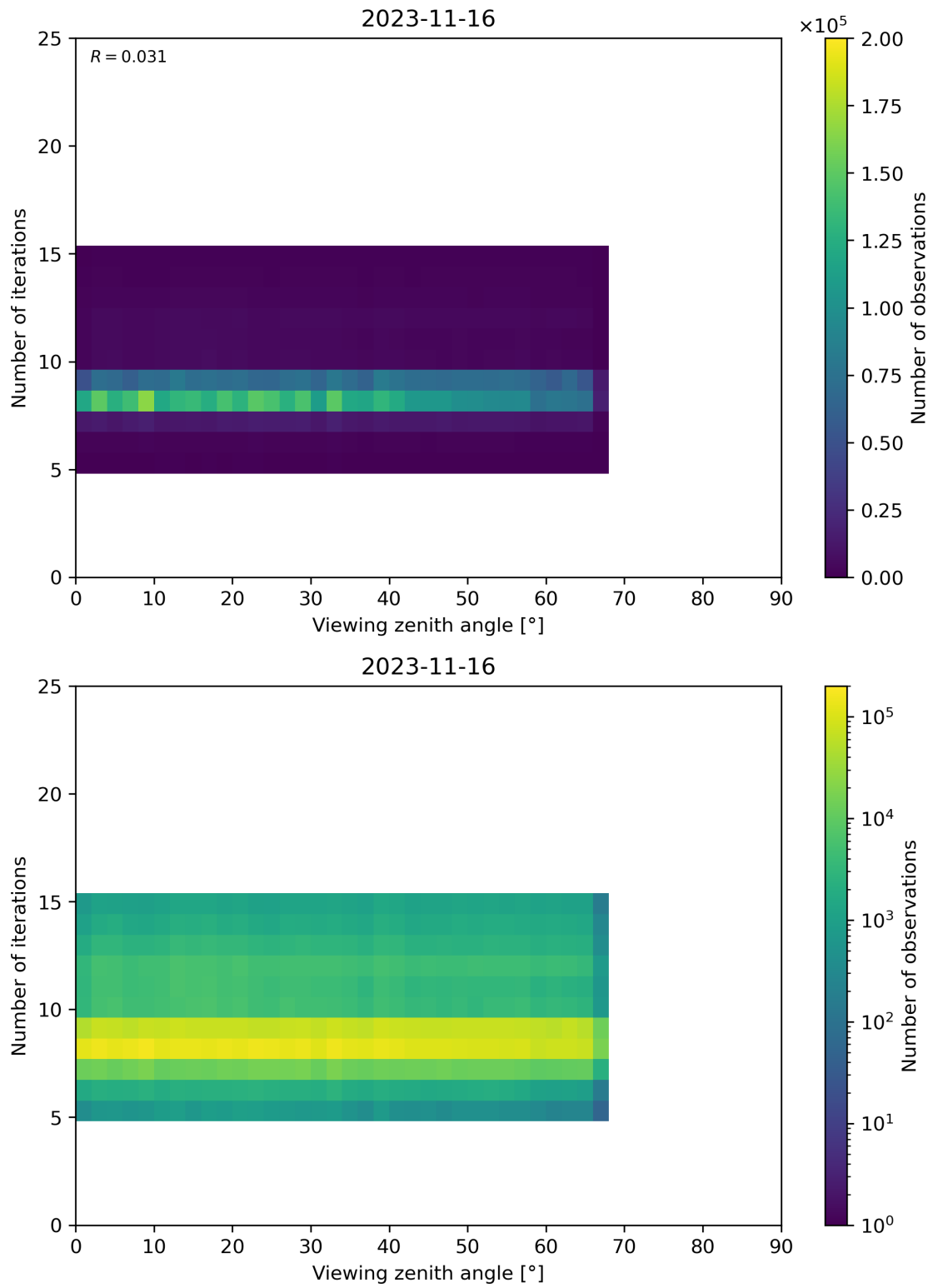
Figure 75: Scatter density plot of “Viewing zenith angle” against “Number of iterations” for 2023-11-15 to 2023-11-17.
