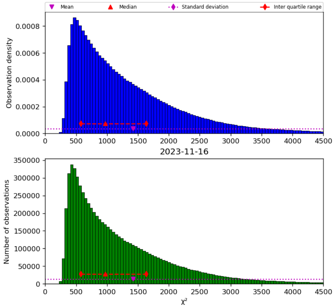
Figure 22: Histogram of “ \chi^2 ” for 2023-11-15 to 2023-11-17
