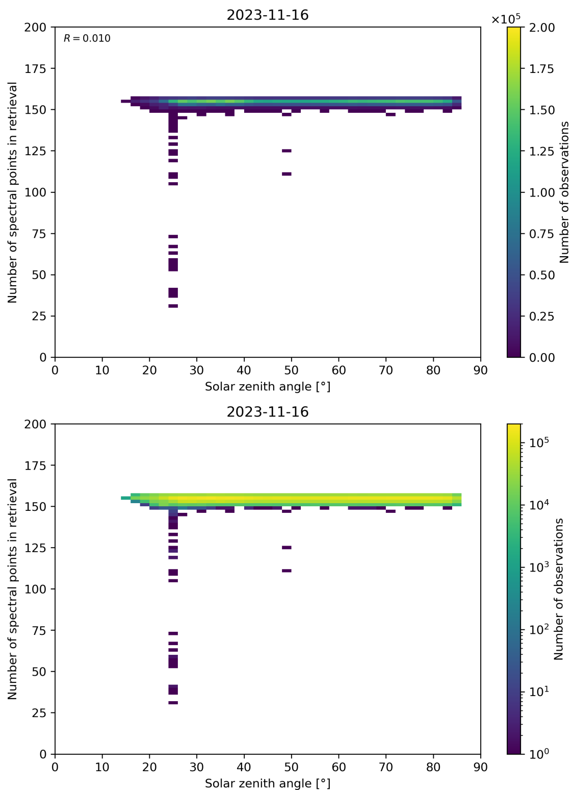
Figure 68: Scatter density plot of “Solar zenith angle” against “Number of spectral points in retrieval” for 2023-11-15 to 2023-11-17.
