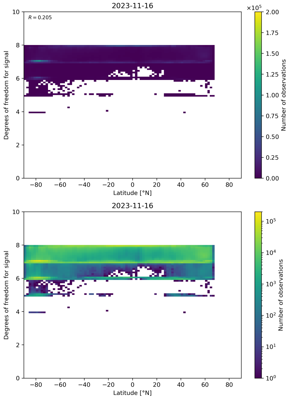
Figure 55: Scatter density plot of “Latitude” against “Degrees of freedom for signal” for 2023-11-15 to 2023-11-17.
