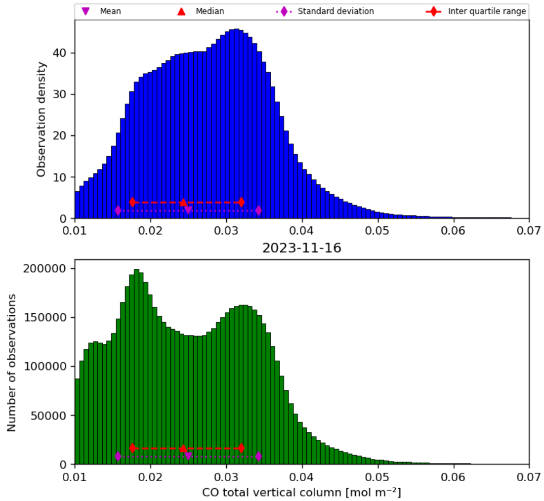
Figure 18: Histogram of “CO total vertical column” for 2023-11-15 to 2023-11-17
