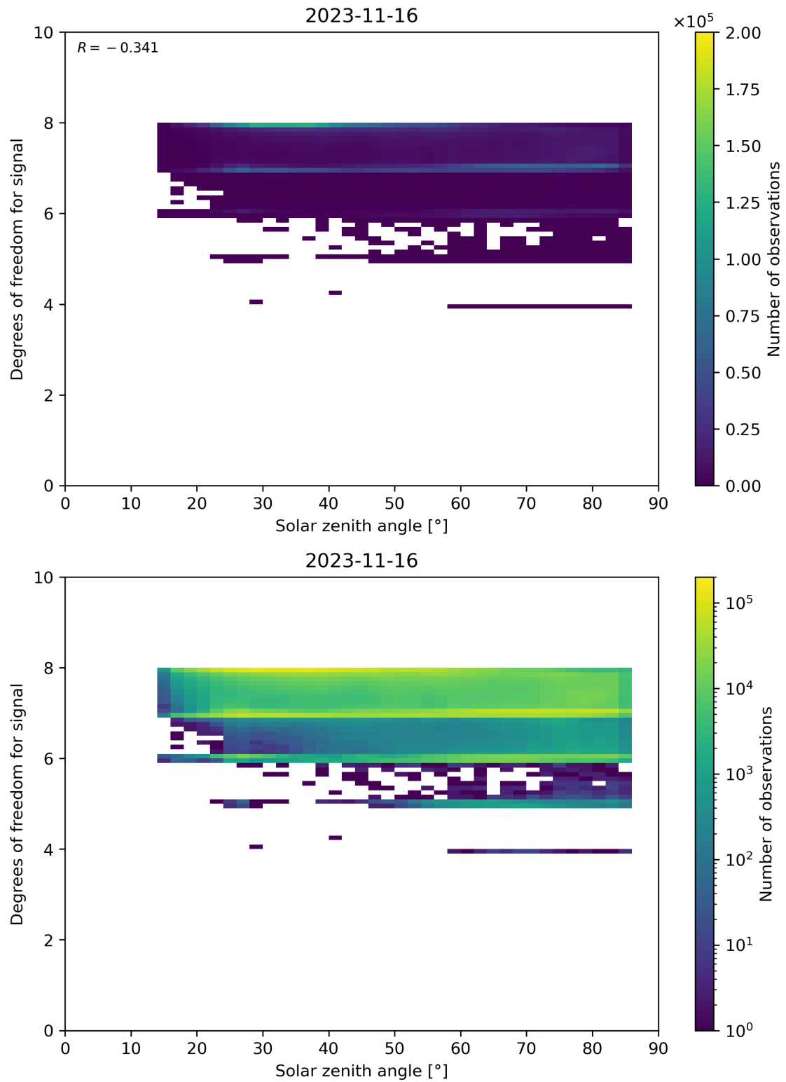
Figure 65: Scatter density plot of “Solar zenith angle” against “Degrees of freedom for signal” for 2023-11-15 to 2023-11-17.
