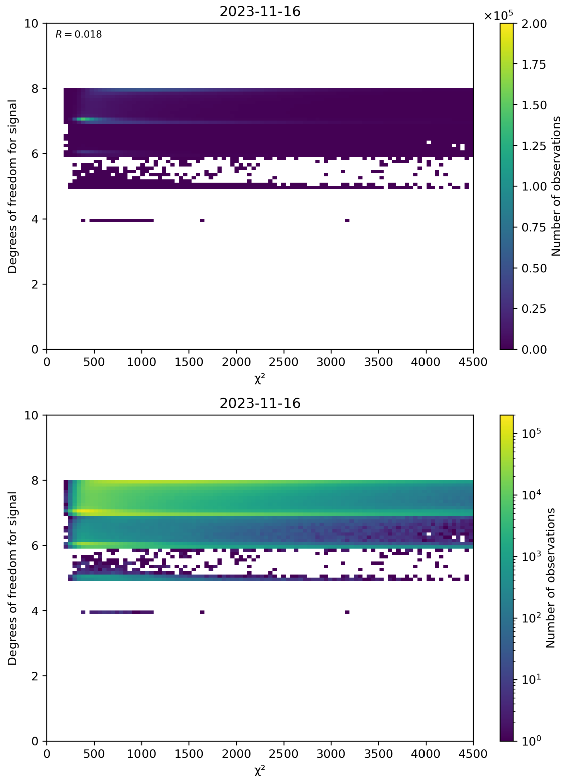
Figure 48: Scatter density plot of “ \chi^2 ” against “Degrees of freedom for signal” for 2023-11-15 to 2023-11-17.
