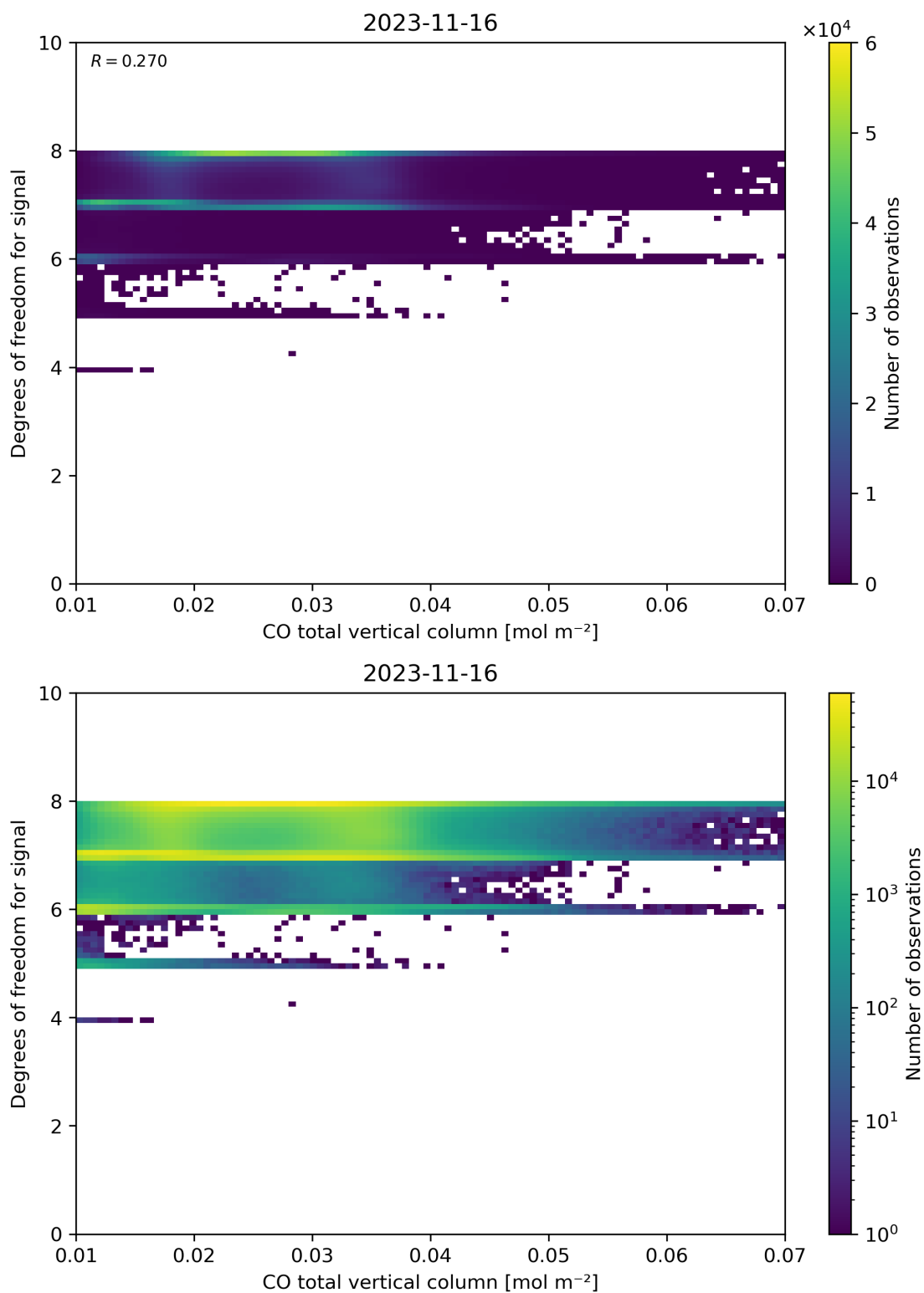
Figure 41: Scatter density plot of “CO total vertical column” against “Degrees of freedom for signal” for 2023-11-15 to 2023-11-17.
