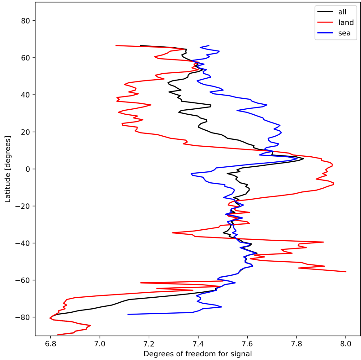
Figure 15: Zonal average of “Degrees of freedom for signal” for 2023-11-15 to 2023-11-17.
