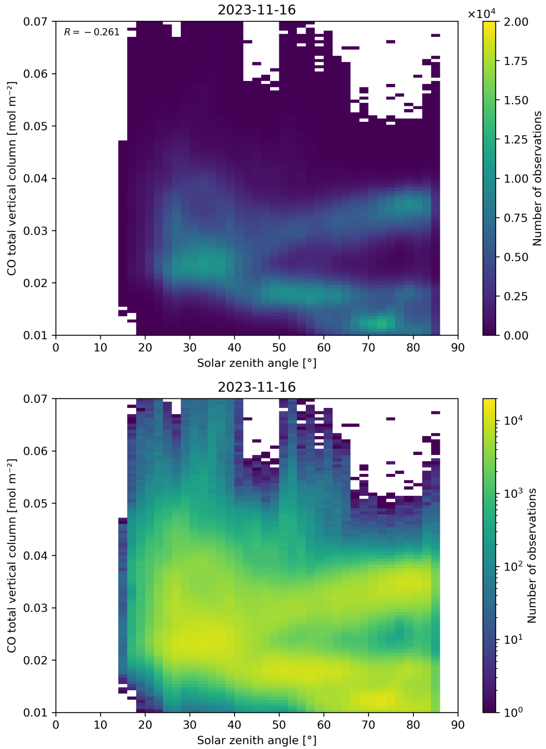
Figure 61: Scatter density plot of “Solar zenith angle” against “CO total vertical column” for 2023-11-15 to 2023-11-17.
