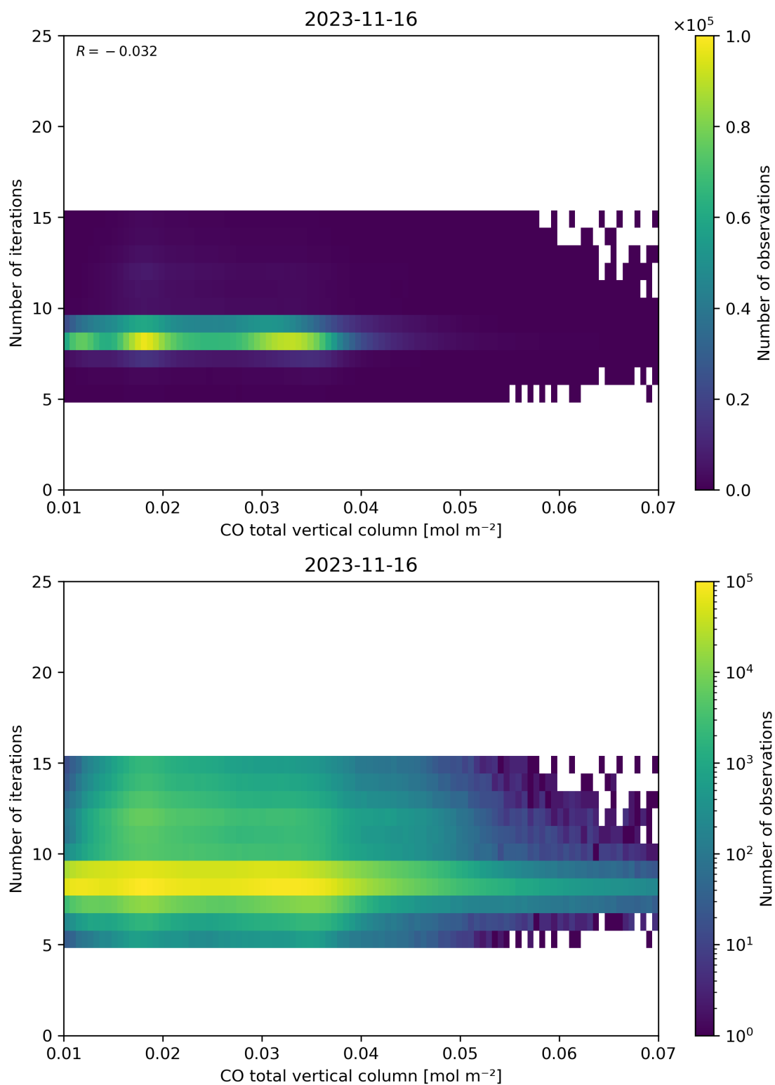
Figure 42: Scatter density plot of “CO total vertical column” against “Number of iterations” for 2023-11-15 to 2023-11-17.
