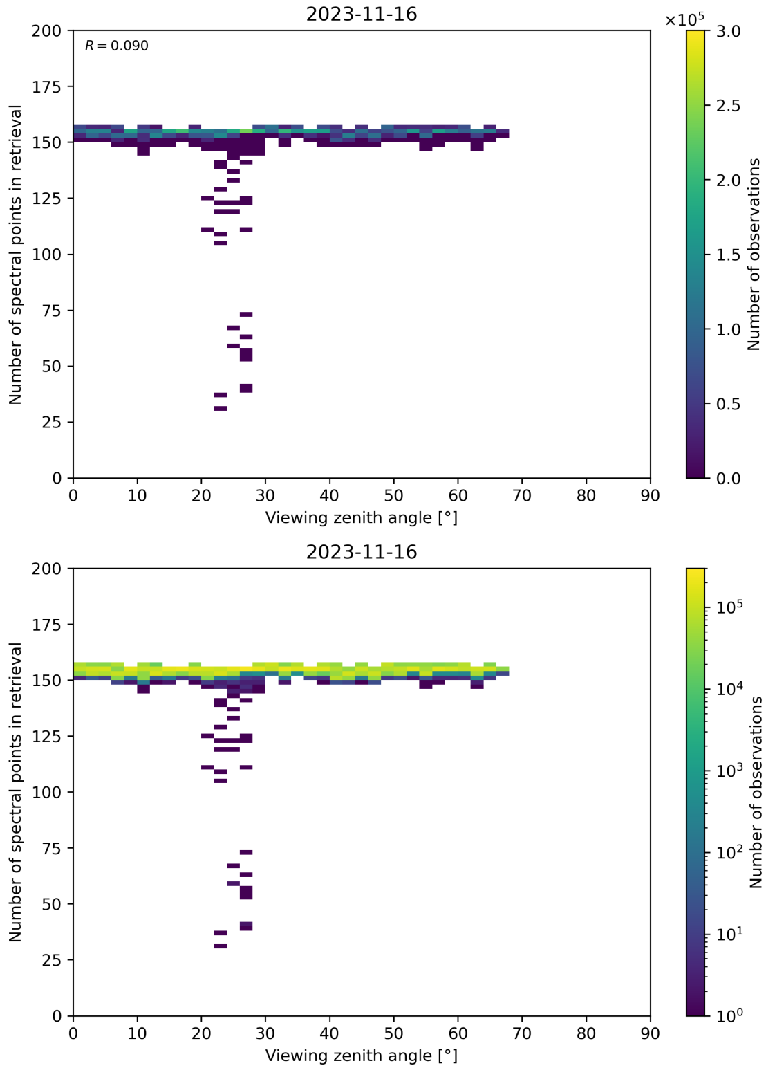
Figure 76: Scatter density plot of “Viewing zenith angle” against “Number of spectral points in retrieval” for 2023-11-15 to 2023-11-17.
