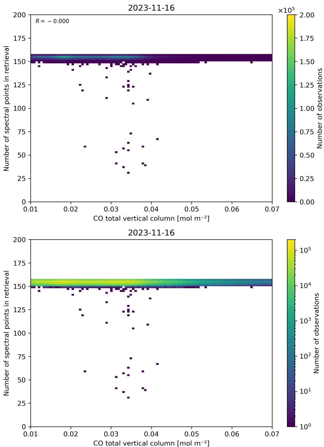
Figure 43: Scatter density plot of “CO total vertical column” against “Number of spectral points in retrieval” for 2023-11-15 to 2023-11-17.
