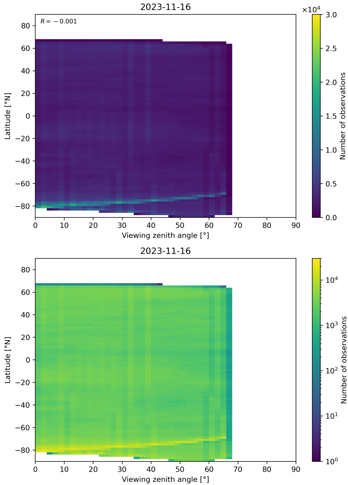
Figure 74: Scatter density plot of “Viewing zenith angle” against “Latitude” for 2023-11-15 to 2023-11-17.
