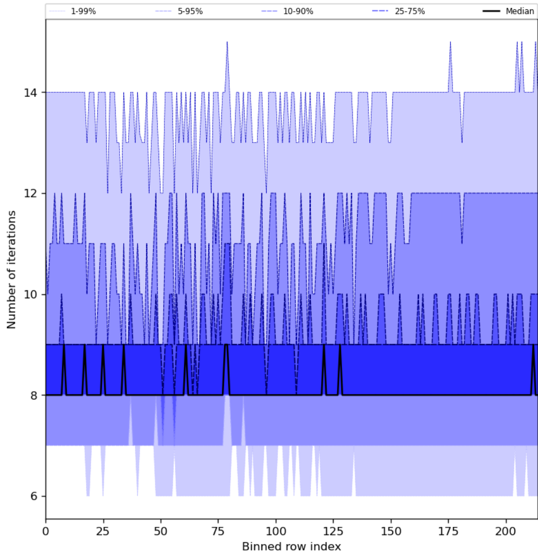
Figure 32: Along track statistics of “Number of iterations” for 2023-11-15 to 2023-11-17
