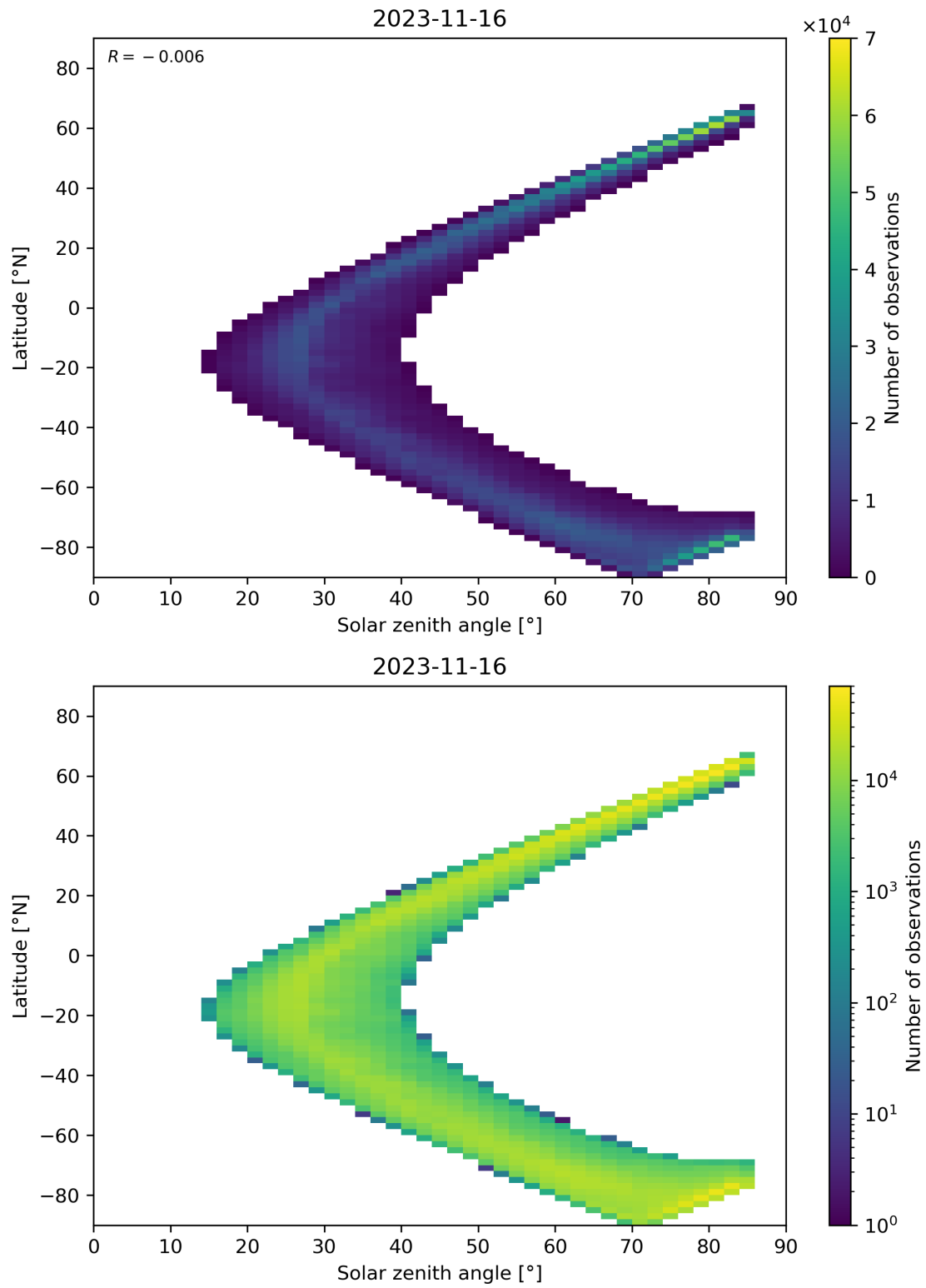
Figure 66: Scatter density plot of “Solar zenith angle” against “Latitude” for 2023-11-15 to 2023-11-17.
