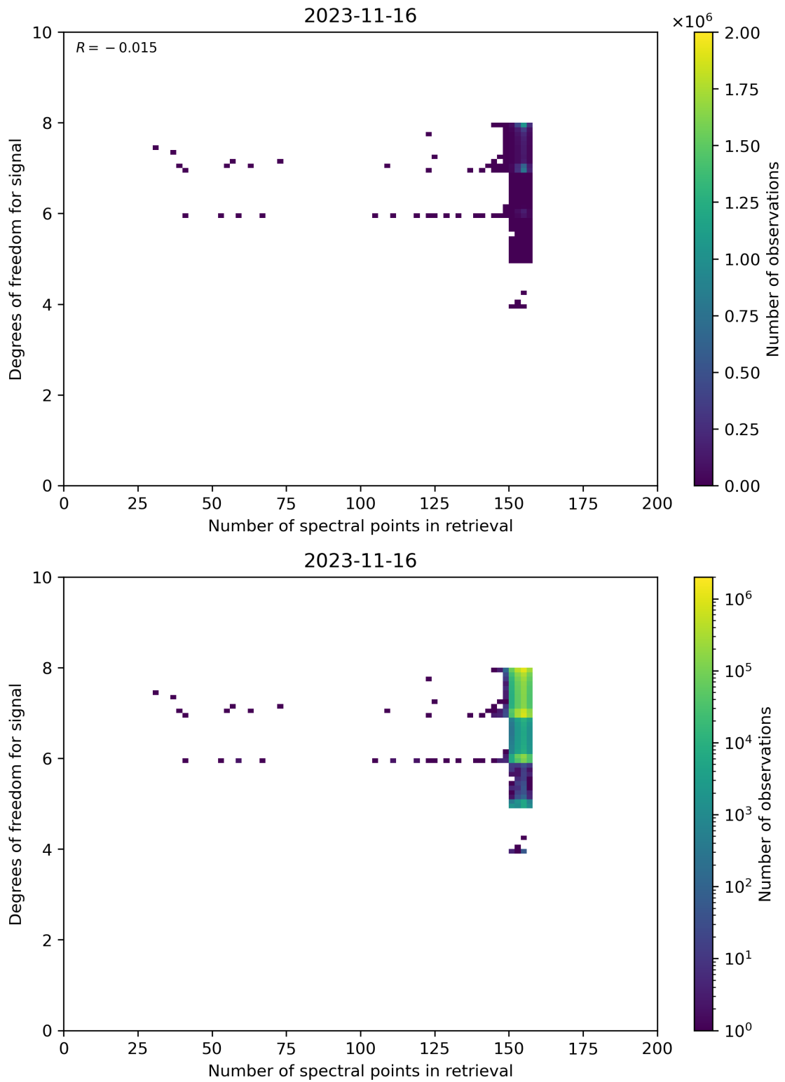
Figure 59: Scatter density plot of “Number of spectral points in retrieval” against “Degrees of freedom for signal” for 2023-11-15 to 2023-11-17.
