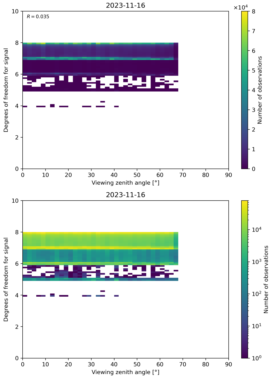
Figure 73: Scatter density plot of “Viewing zenith angle” against “Degrees of freedom for signal” for 2023-11-15 to 2023-11-17.
