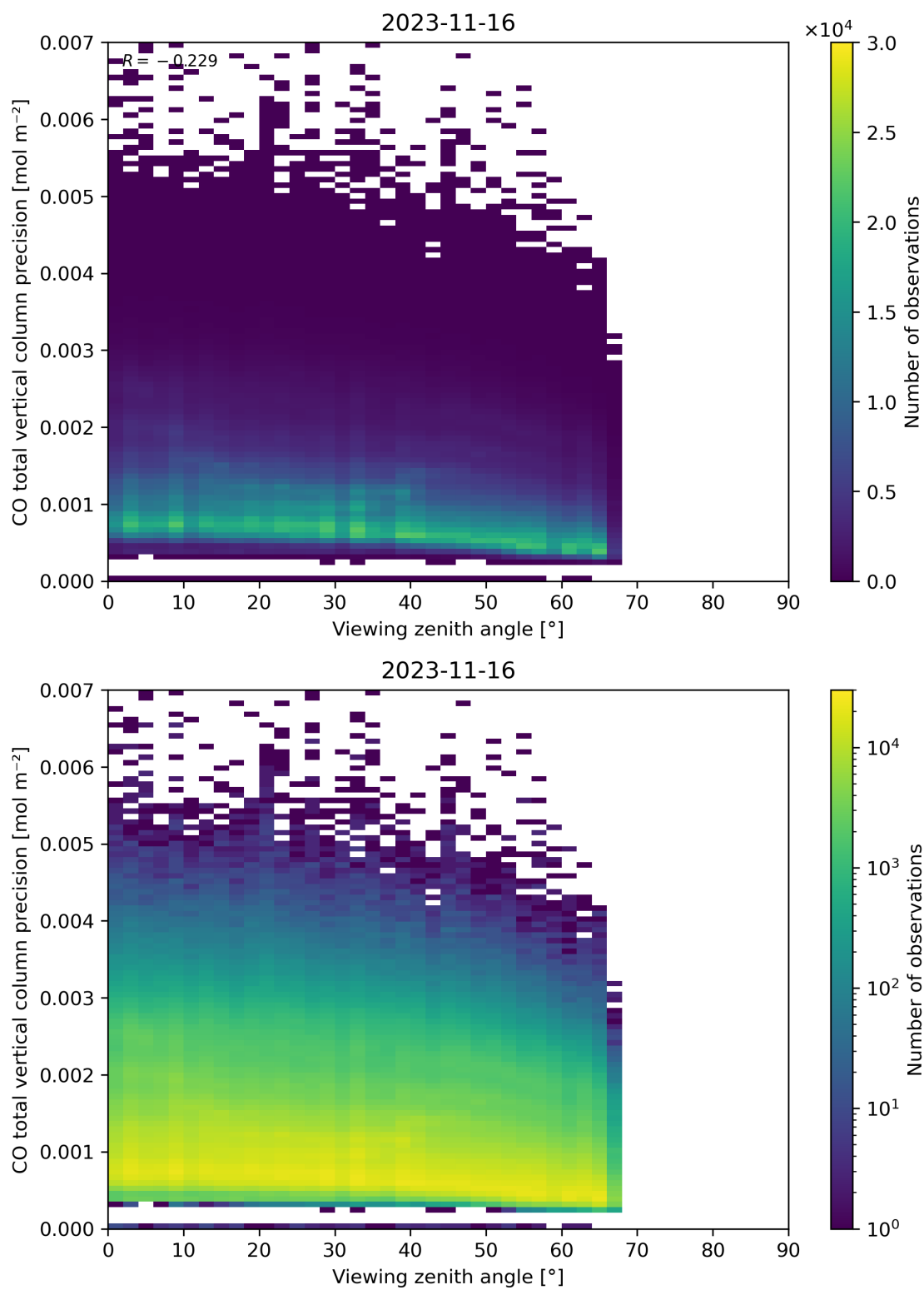
Figure 71: Scatter density plot of “Viewing zenith angle” against “CO total vertical column precision” for 2023-11-15 to 2023-11-17.
