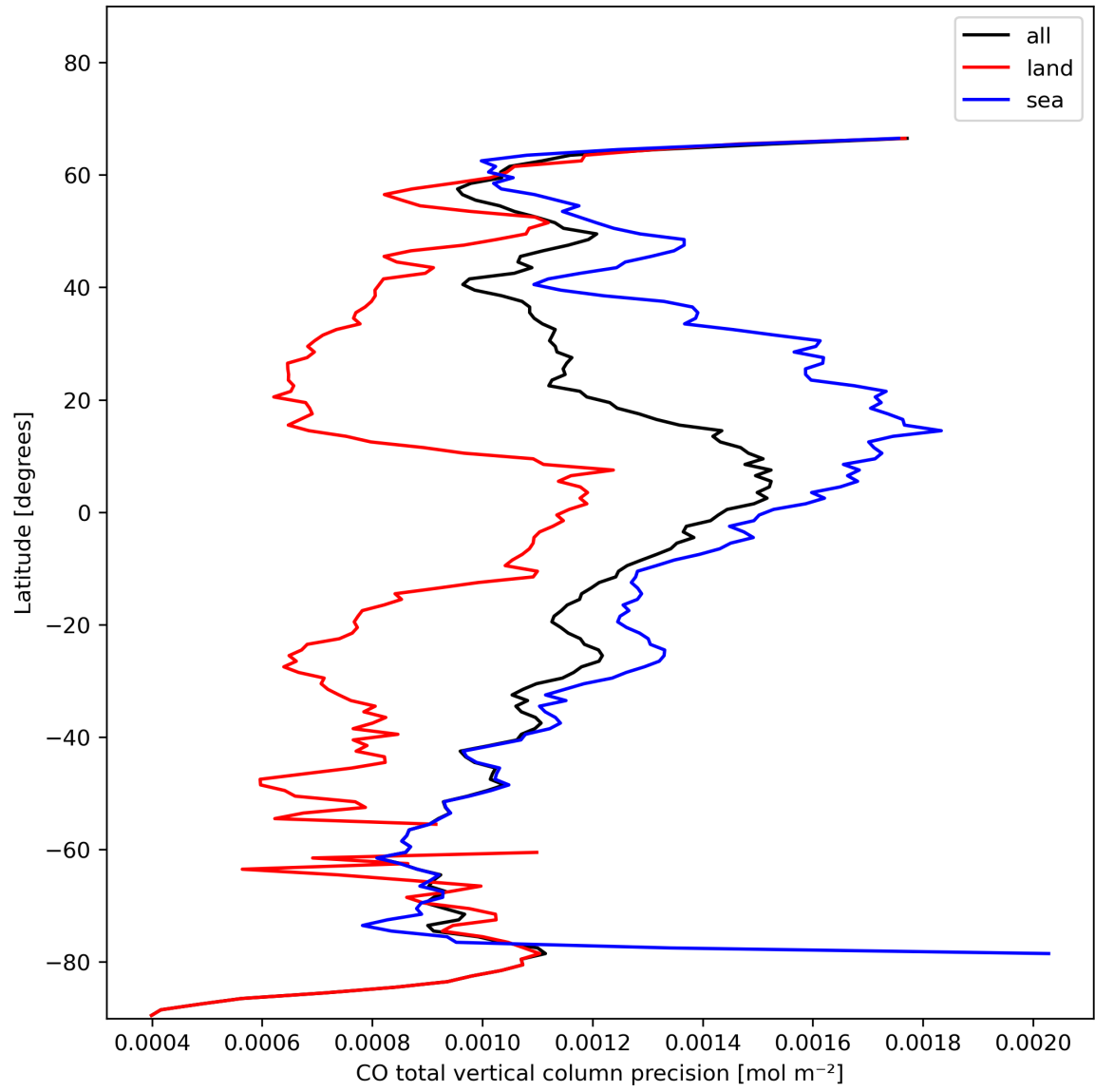
Figure 12: Zonal average of “CO total vertical column precision” for 2023-11-15 to 2023-11-17.
