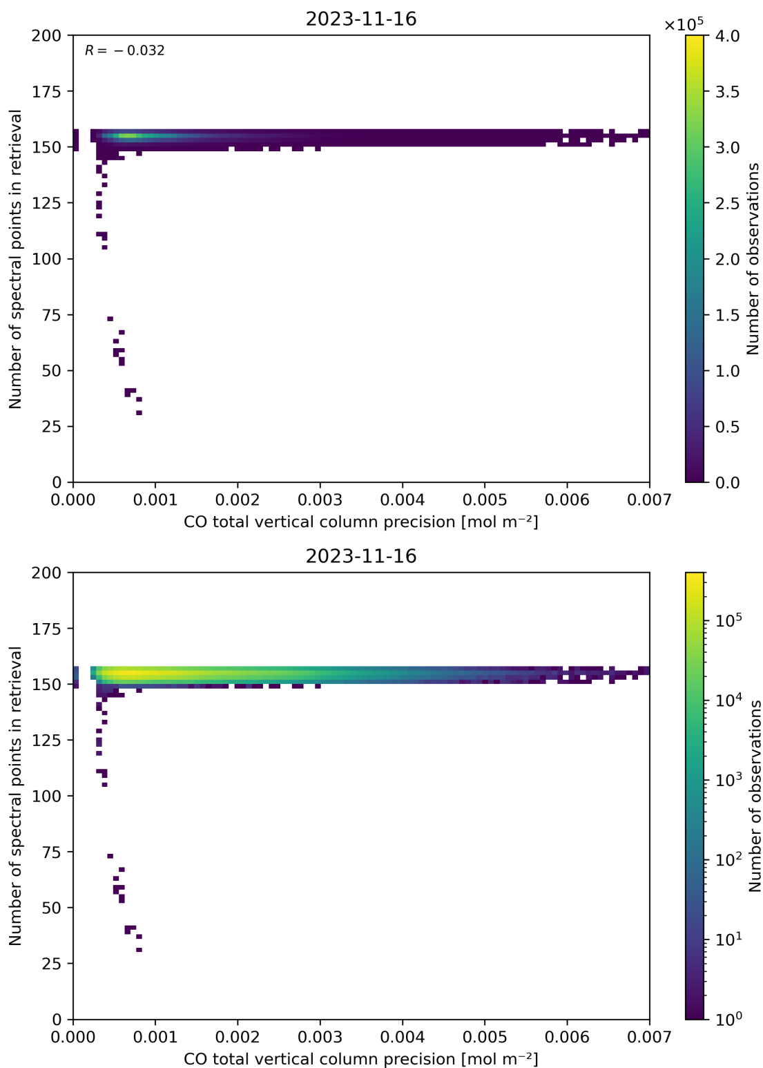
Figure 47: Scatter density plot of “CO total vertical column precision” against “Number of spectral points in retrieval” for 2023-11-15 to 2023-11-17.
