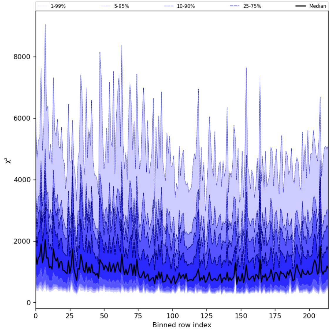
Figure 30: Along track statistics of “ \chi^2 ” for 2023-11-15 to 2023-11-17
