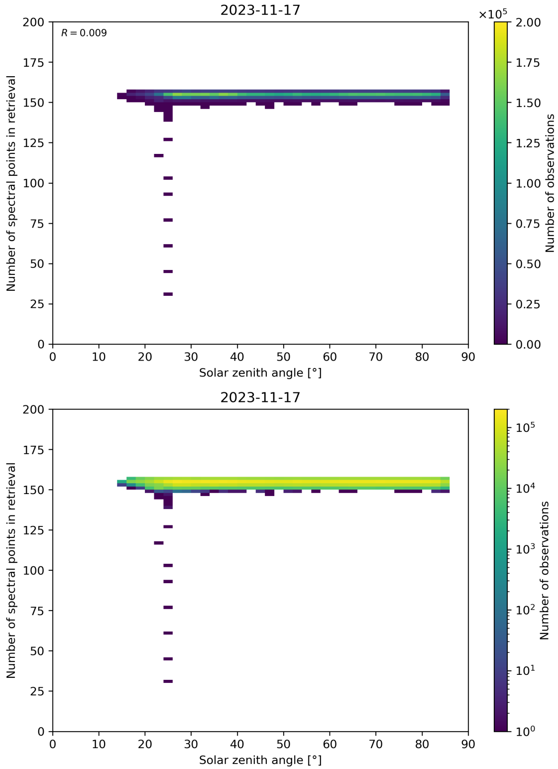
Figure 68: Scatter density plot of “Solar zenith angle” against “Number of spectral points in retrieval” for 2023-11-16 to 2023-11-18.
