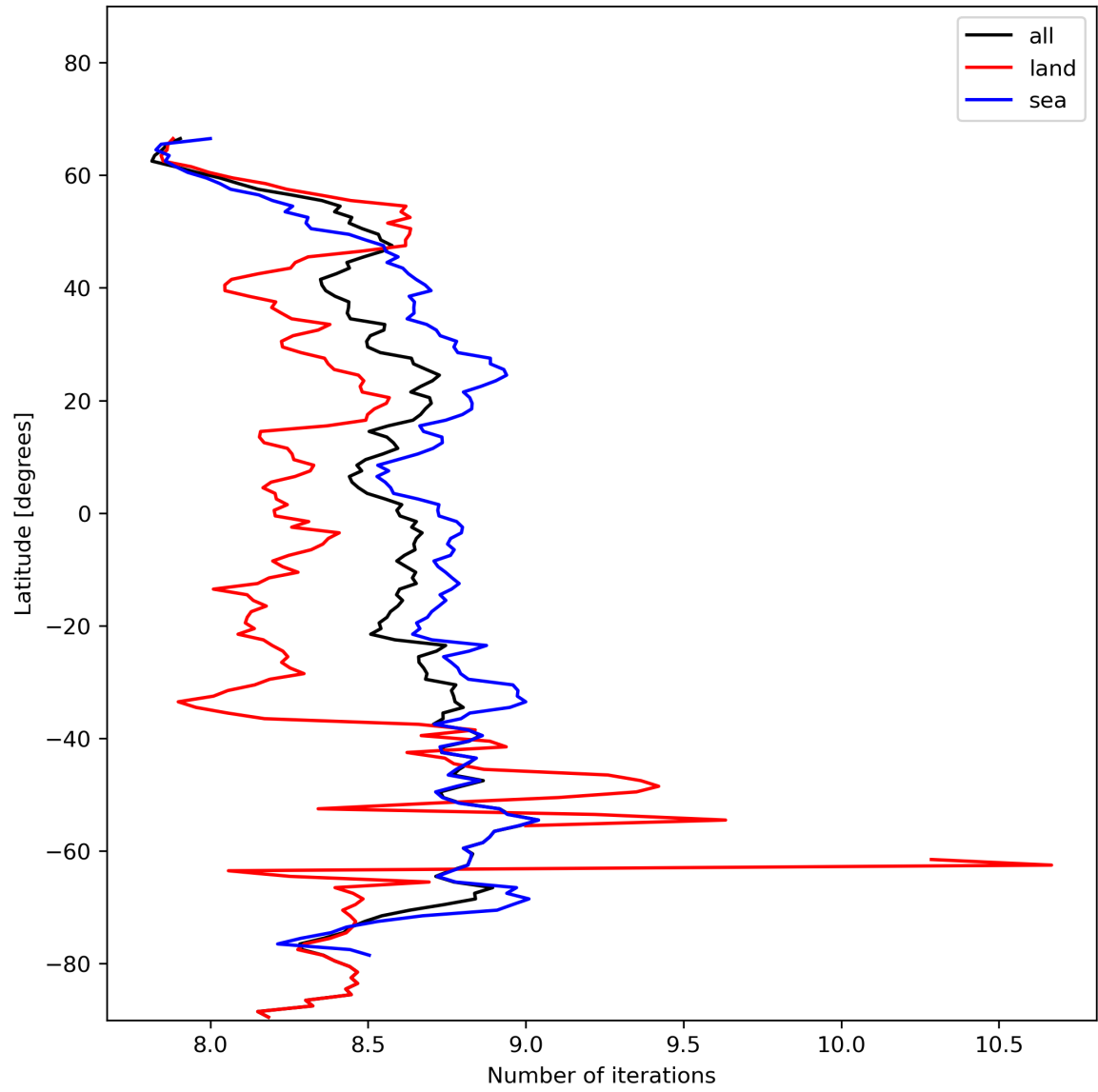
Figure 16: Zonal average of “Number of iterations” for 2023-11-16 to 2023-11-18.
