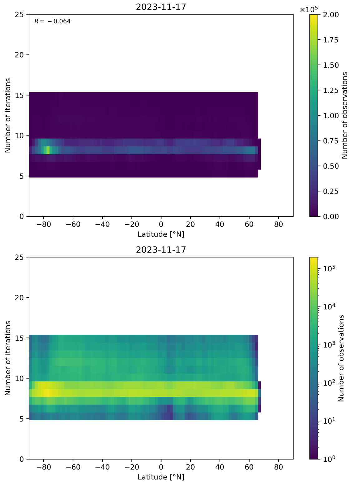
Figure 56: Scatter density plot of “Latitude” against “Number of iterations” for 2023-11-16 to 2023-11-18.
