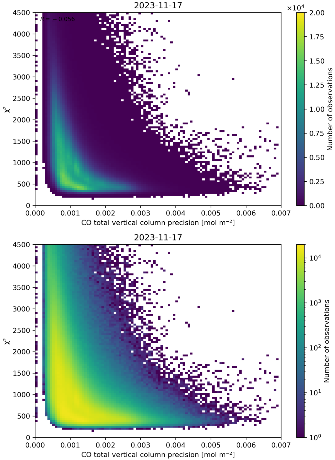
Figure 44: Scatter density plot of “CO total vertical column precision” against “ \chi^2 ” for 2023-11-16 to 2023-11-18.
