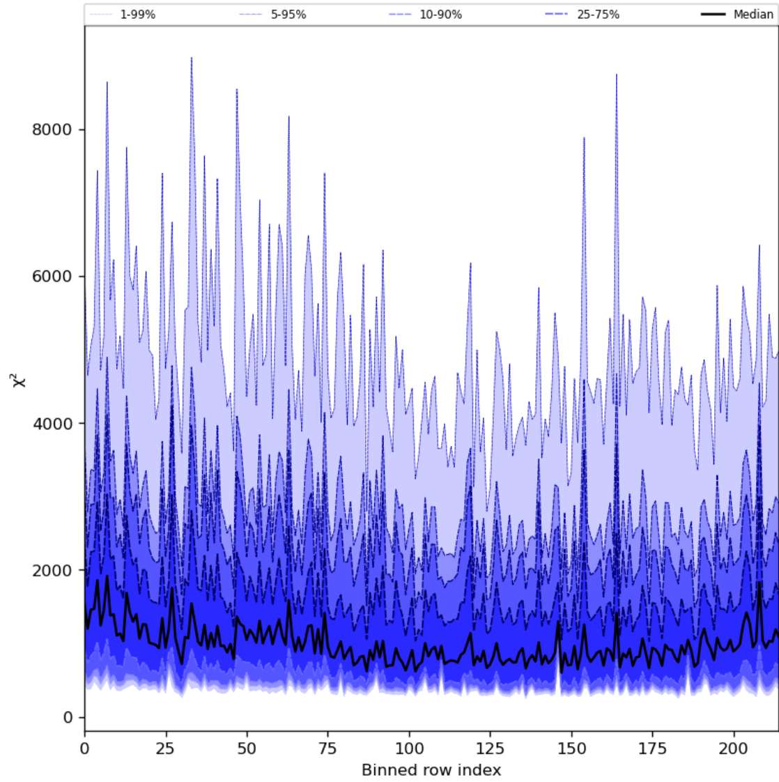
Figure 30: Along track statistics of “ \chi^2 ” for 2023-11-16 to 2023-11-18
