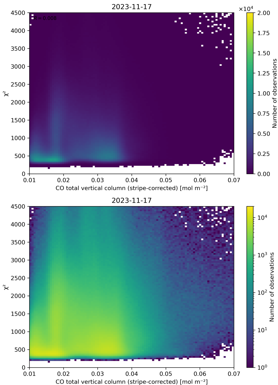
Figure 37: Scatter density plot of “CO total vertical column (stripe-corrected)” against “ \chi^2 ” for 2023-11-16 to 2023-11-18.
