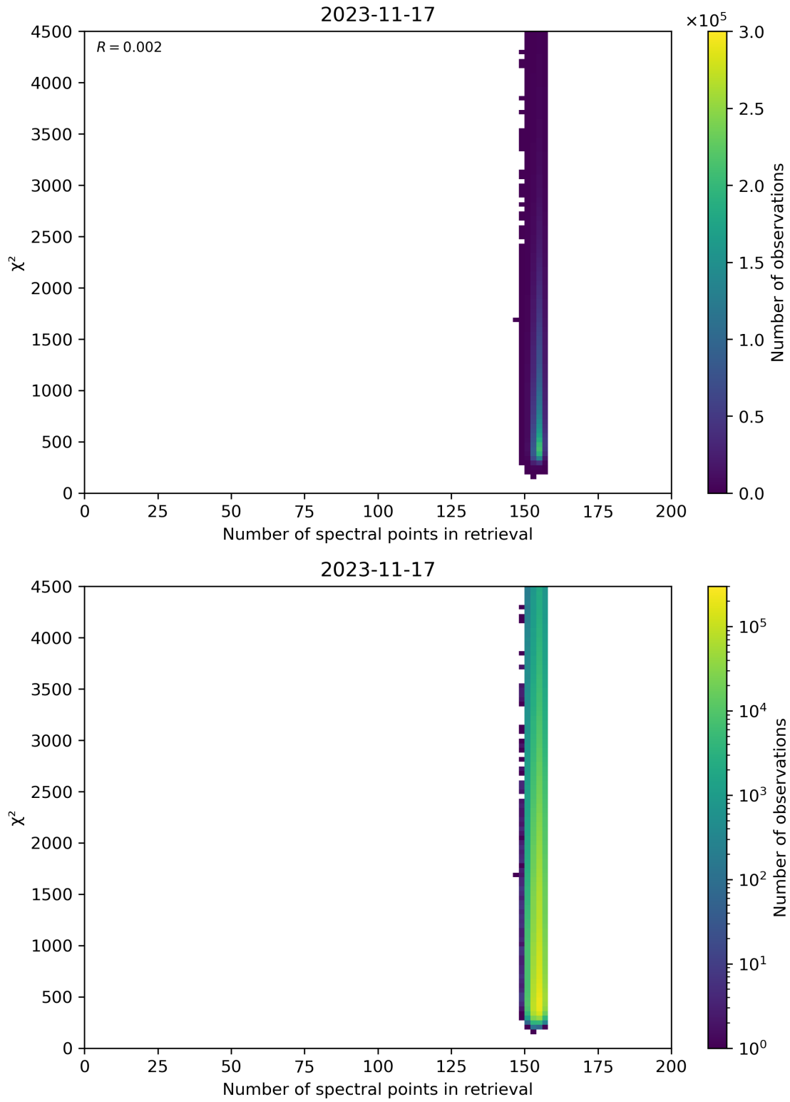
Figure 58: Scatter density plot of “Number of spectral points in retrieval” against “ \chi^2 ” for 2023-11-16 to 2023-11-18.
