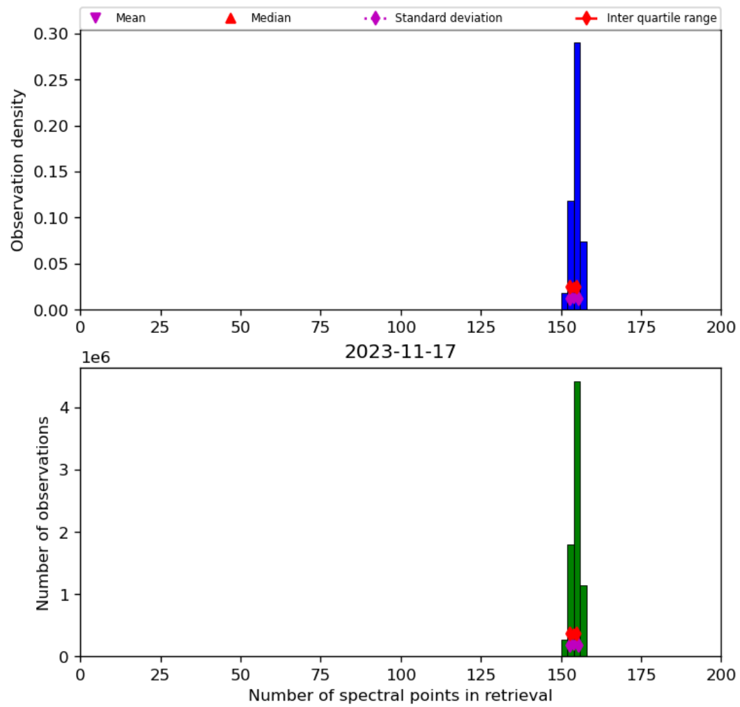
Figure 21: Histogram of “Number of spectral points in retrieval” for 2023-11-16 to 2023-11-18
