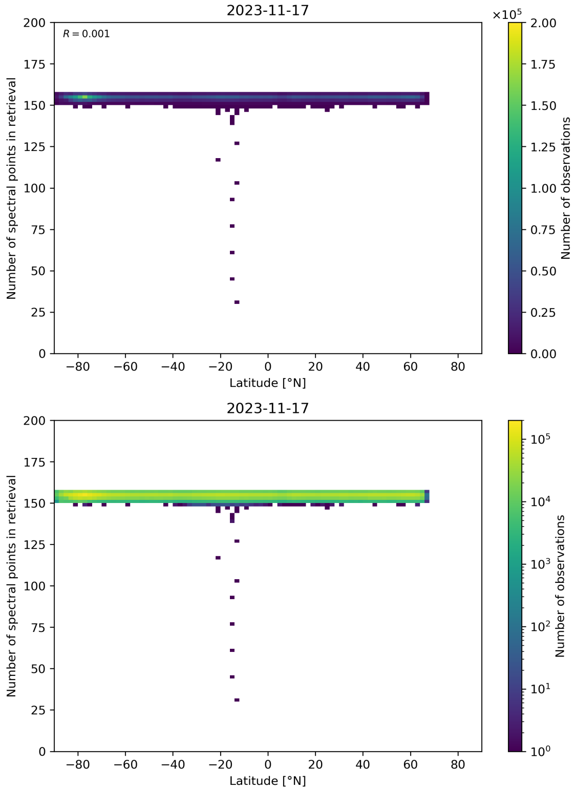
Figure 57: Scatter density plot of “Latitude” against “Number of spectral points in retrieval” for 2023-11-16 to 2023-11-18.
