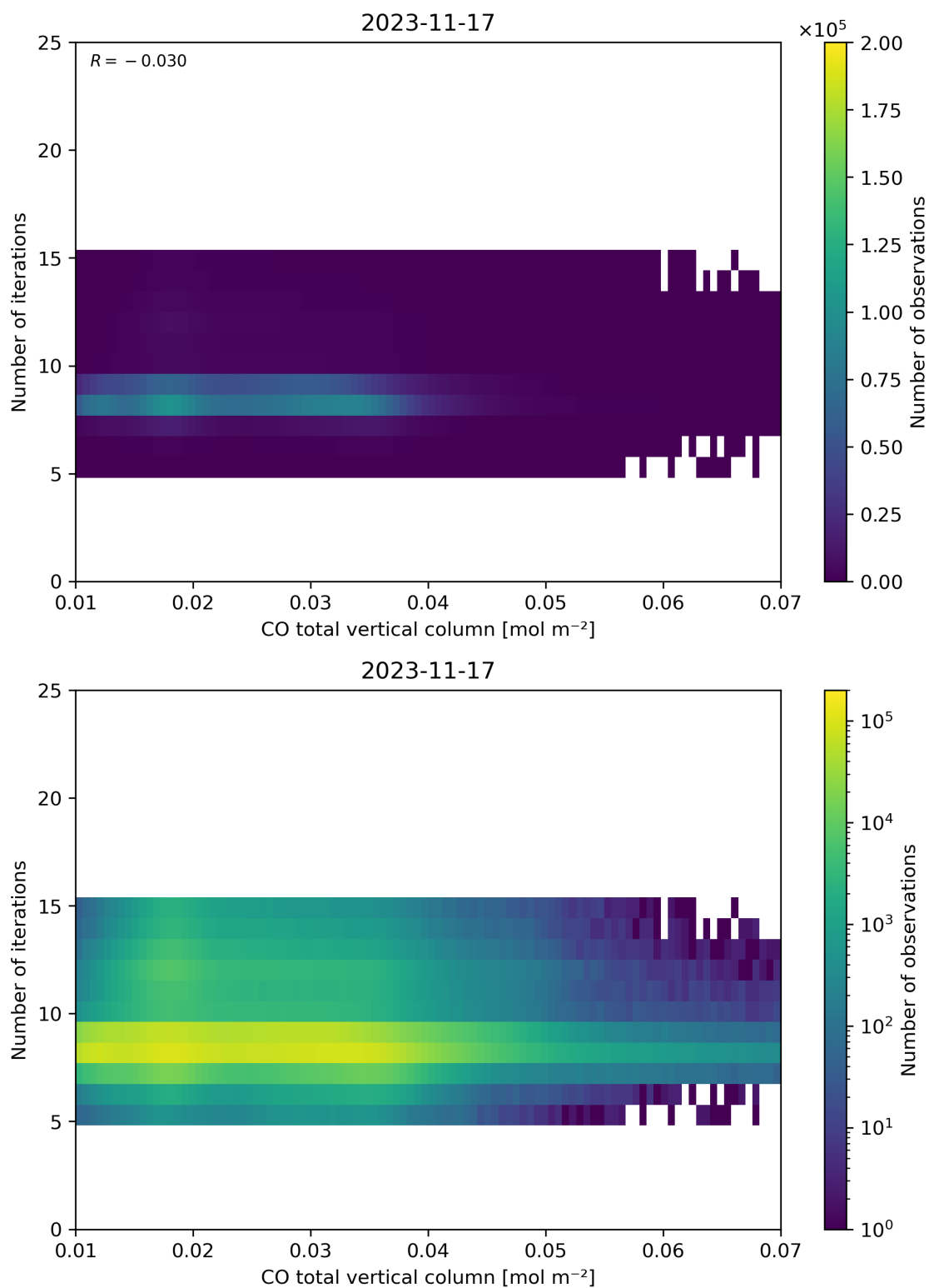
Figure 42: Scatter density plot of “CO total vertical column” against “Number of iterations” for 2023-11-16 to 2023-11-18.
