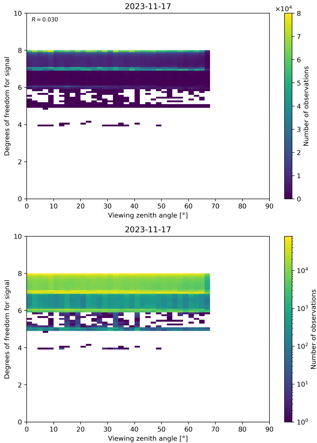
Figure 73: Scatter density plot of “Viewing zenith angle” against “Degrees of freedom for signal” for 2023-11-16 to 2023-11-18.
