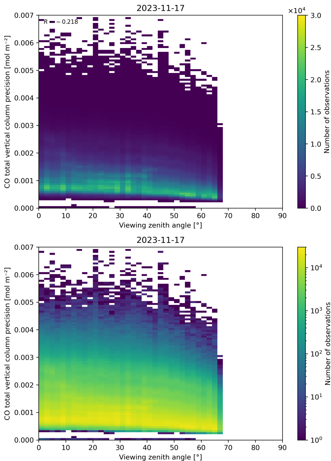
Figure 71: Scatter density plot of “Viewing zenith angle” against “CO total vertical column precision” for 2023-11-16 to 2023-11-18.
