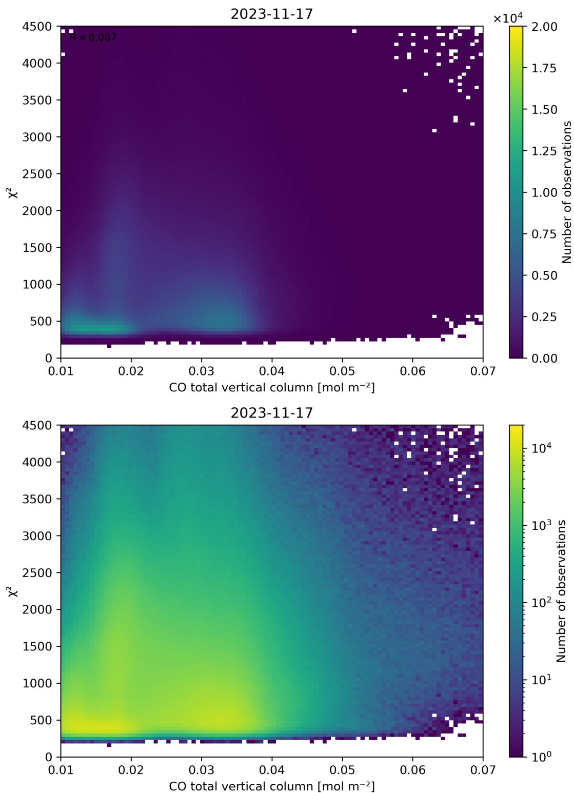
Figure 35: Scatter density plot of “CO total vertical column” against “ \chi^2 ” for 2023-11-16 to 2023-11-18.
