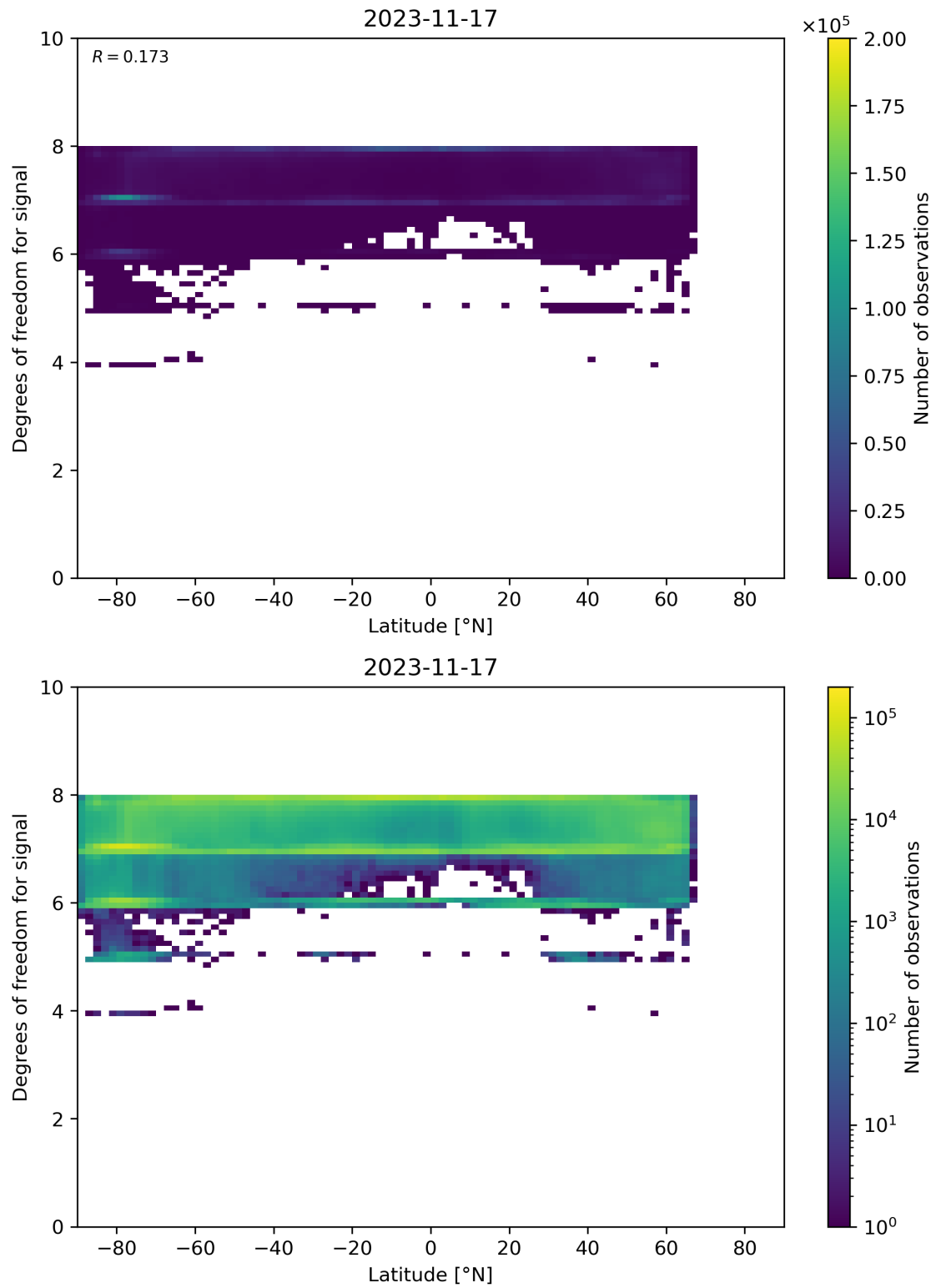
Figure 55: Scatter density plot of “Latitude” against “Degrees of freedom for signal” for 2023-11-16 to 2023-11-18.
