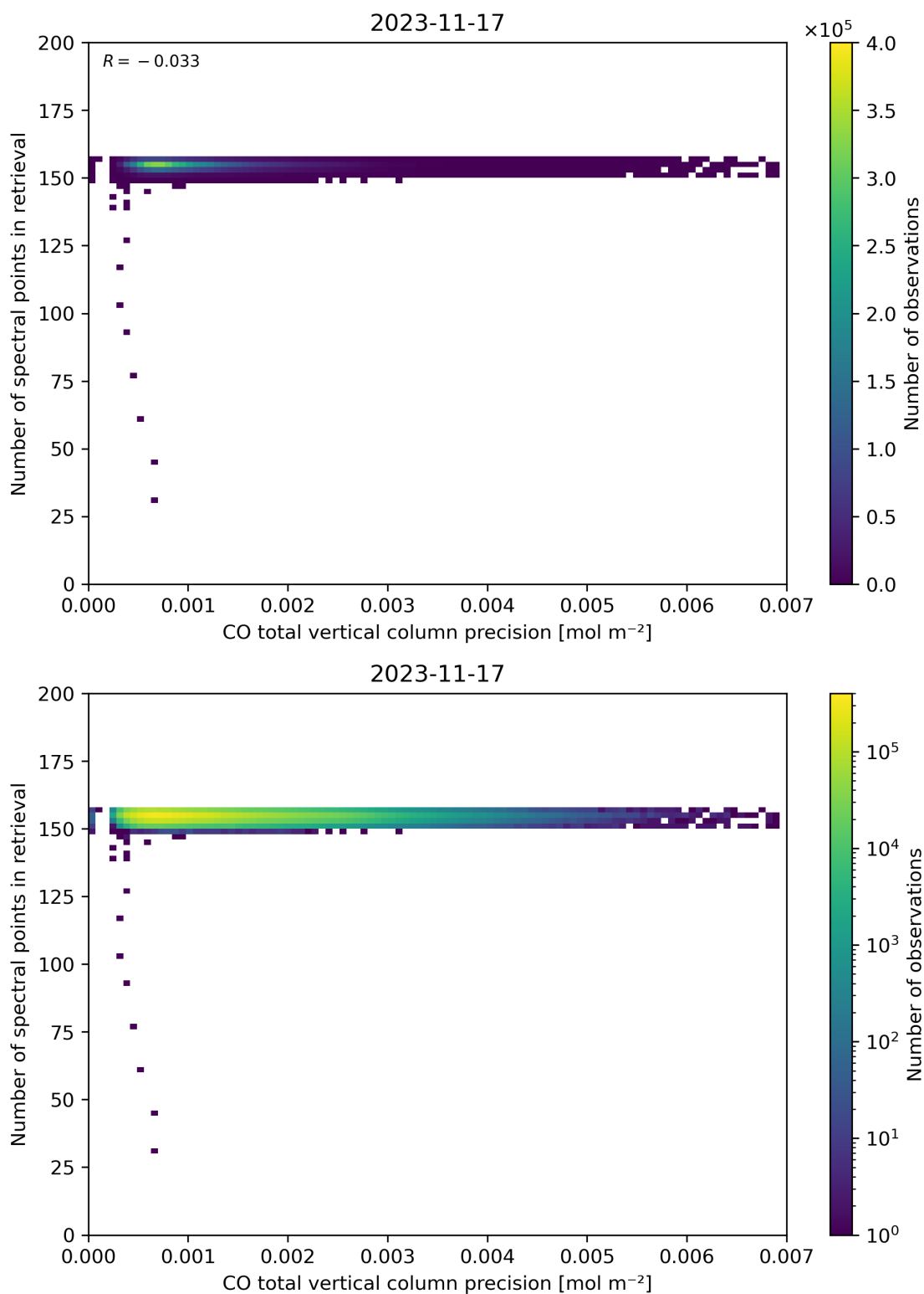
Figure 47: Scatter density plot of “CO total vertical column precision” against “Number of spectral points in retrieval” for 2023-11-16 to 2023-11-18.
