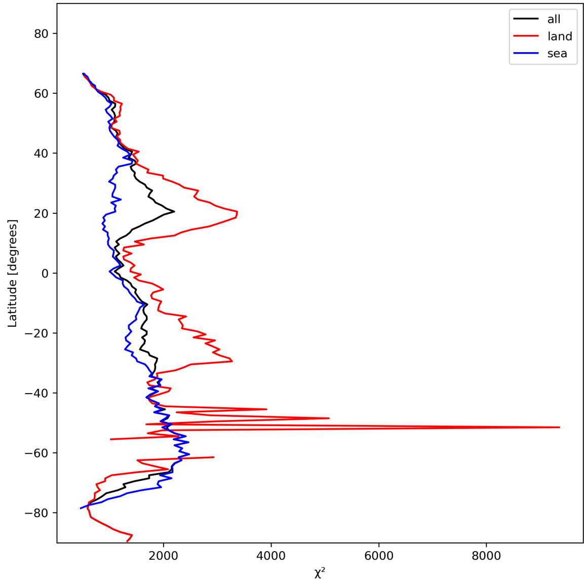
Figure 14: Zonal average of “ \chi^2 ” for 2023-11-16 to 2023-11-18.
