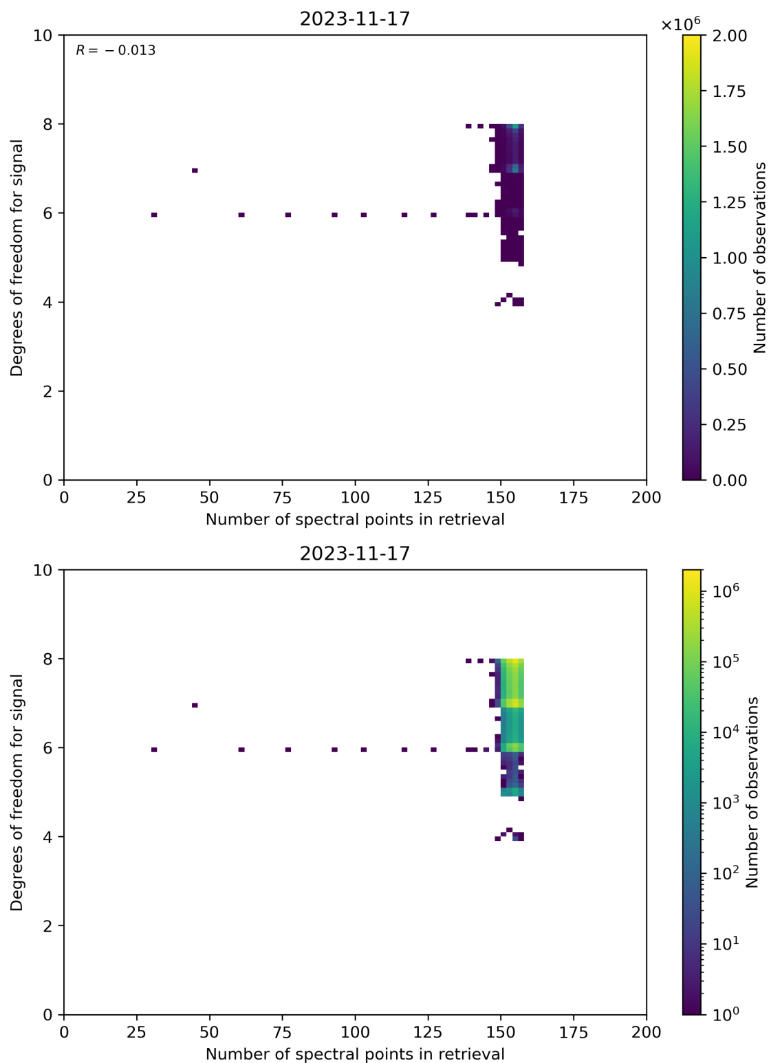
Figure 59: Scatter density plot of “Number of spectral points in retrieval” against “Degrees of freedom for signal” for 2023-11-16 to 2023-11-18.
