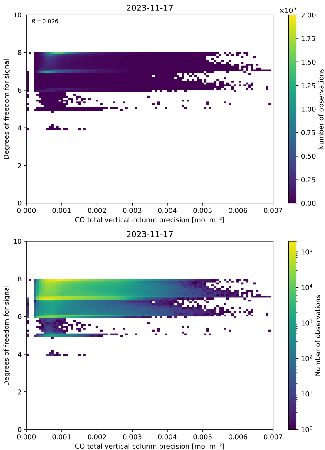
Figure 45: Scatter density plot of “CO total vertical column precision” against “Degrees of freedom for signal” for 2023-11-16 to 2023-11-18.
