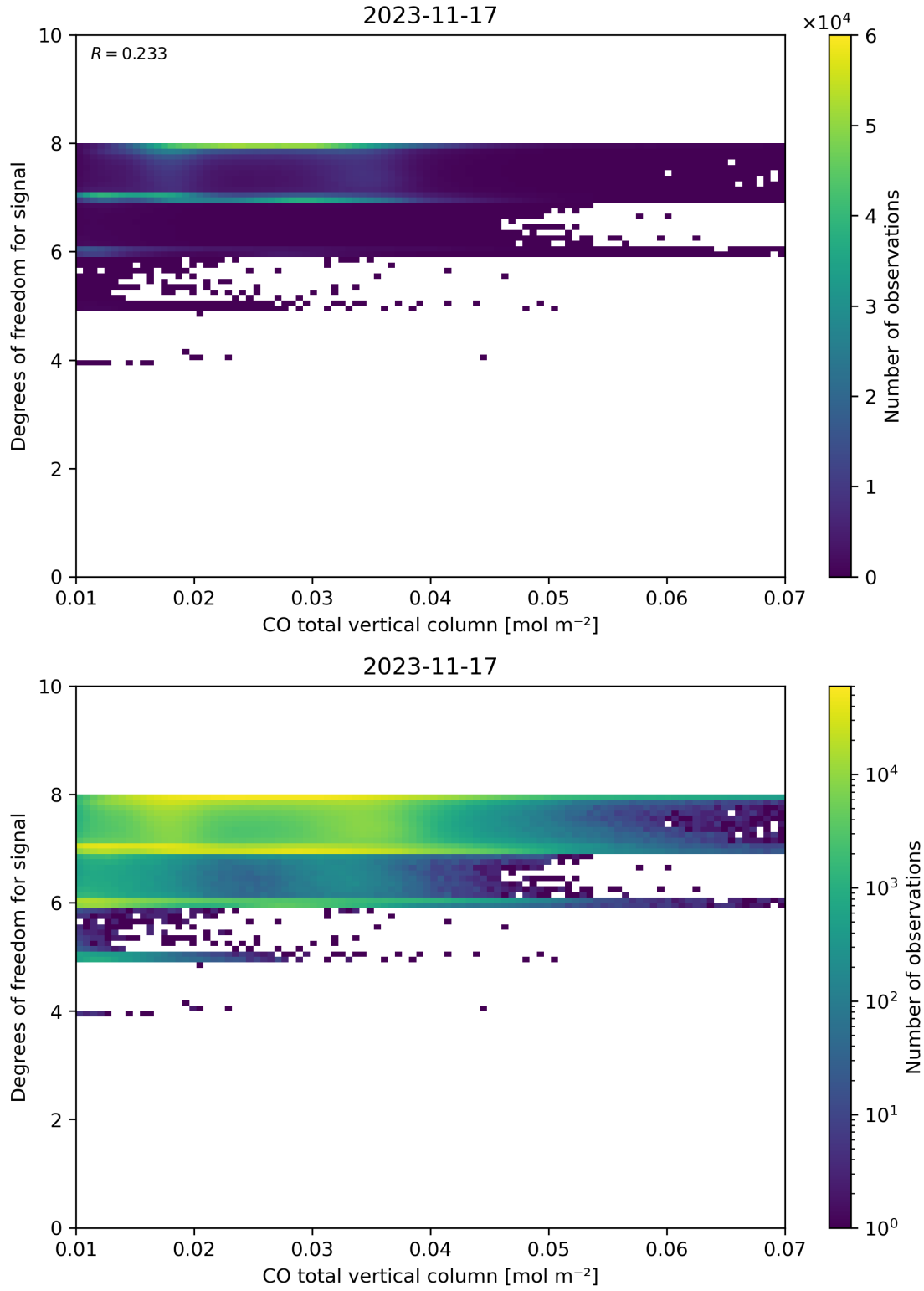
Figure 41: Scatter density plot of “CO total vertical column” against “Degrees of freedom for signal” for 2023-11-16 to 2023-11-18.
