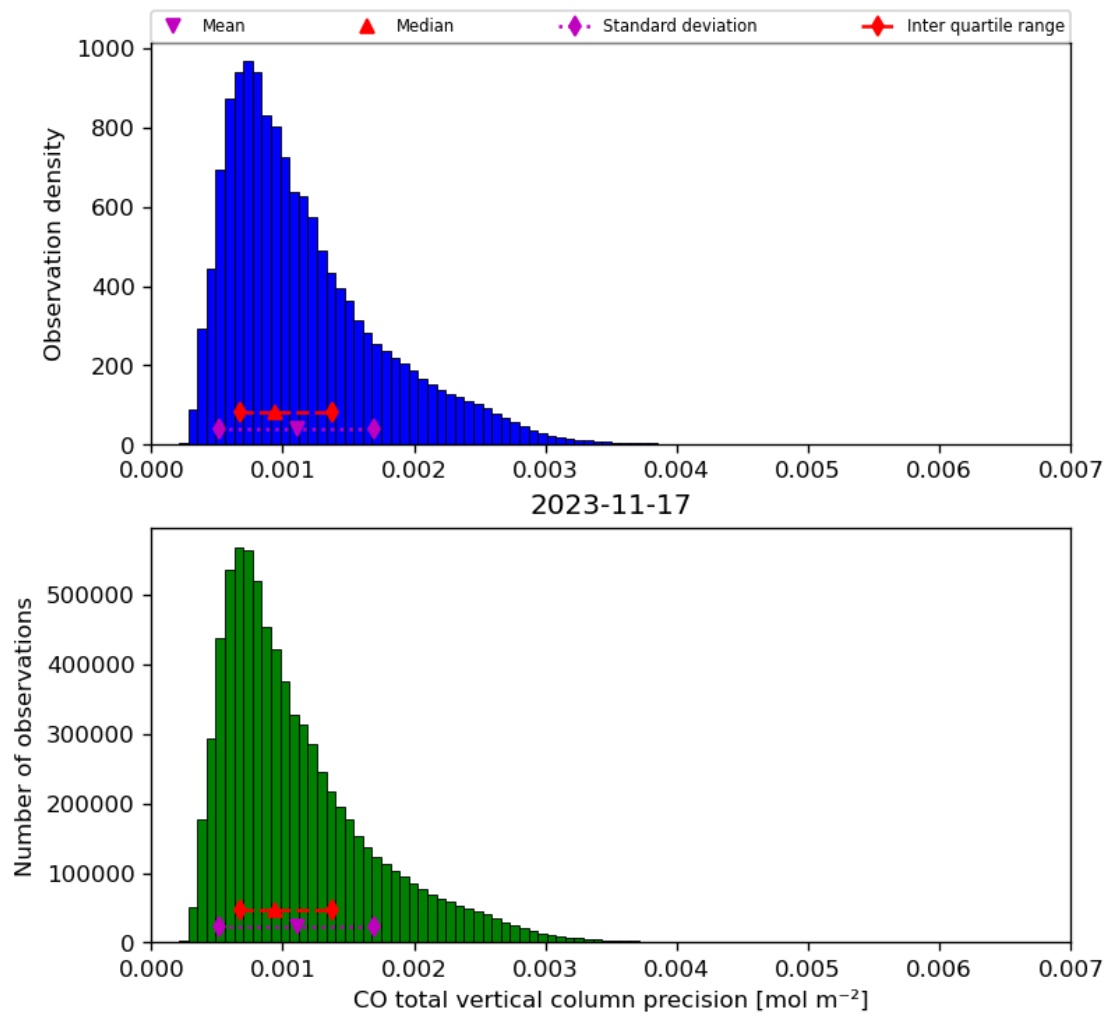
Figure 20: Histogram of “CO total vertical column precision” for 2023-11-16 to 2023-11-18
