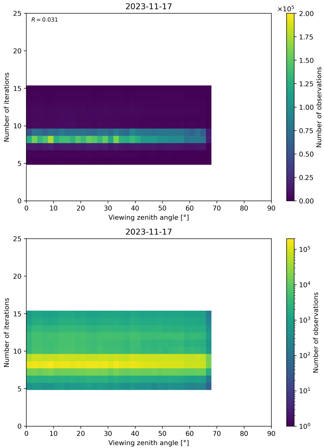
Figure 75: Scatter density plot of “Viewing zenith angle” against “Number of iterations” for 2023-11-16 to 2023-11-18.
