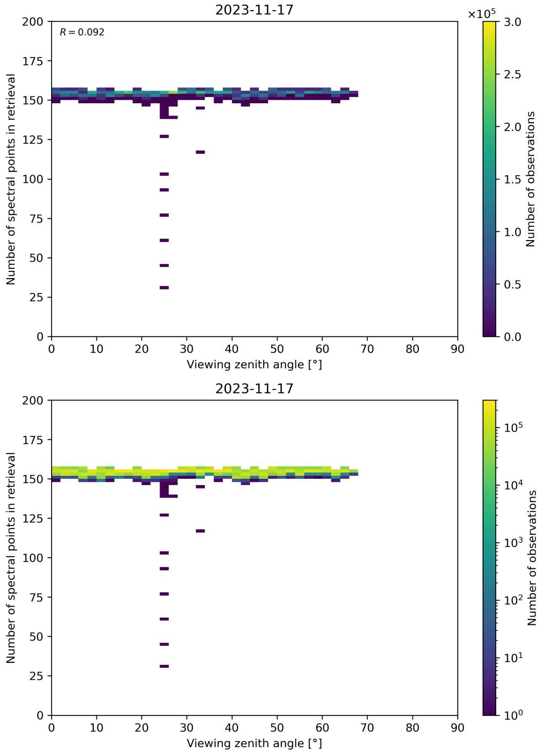
Figure 76: Scatter density plot of “Viewing zenith angle” against “Number of spectral points in retrieval” for 2023-11-16 to 2023-11-18.
