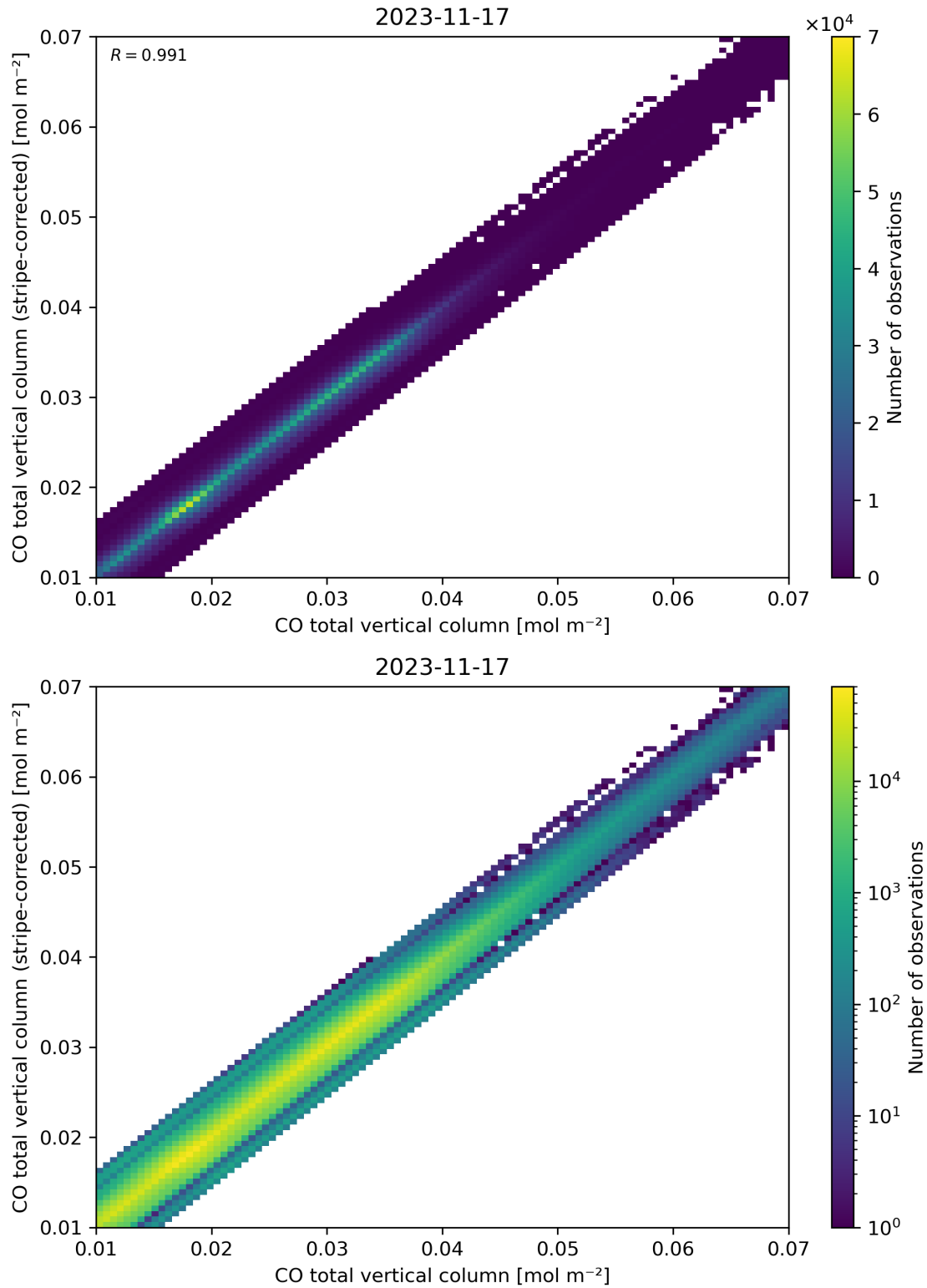
Figure 33: Scatter density plot of “CO total vertical column” against “CO total vertical column (stripe-corrected)” for 2023-11-16 to 2023-11-18.
