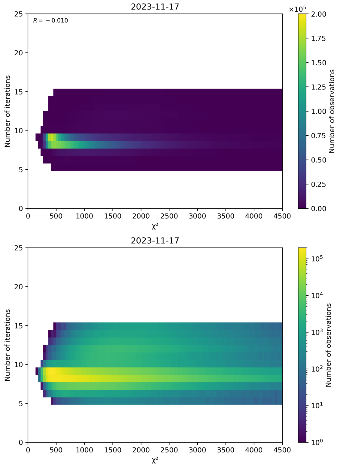
Figure 49: Scatter density plot of “ \chi^2 ” against “Number of iterations” for 2023-11-16 to 2023-11-18.
