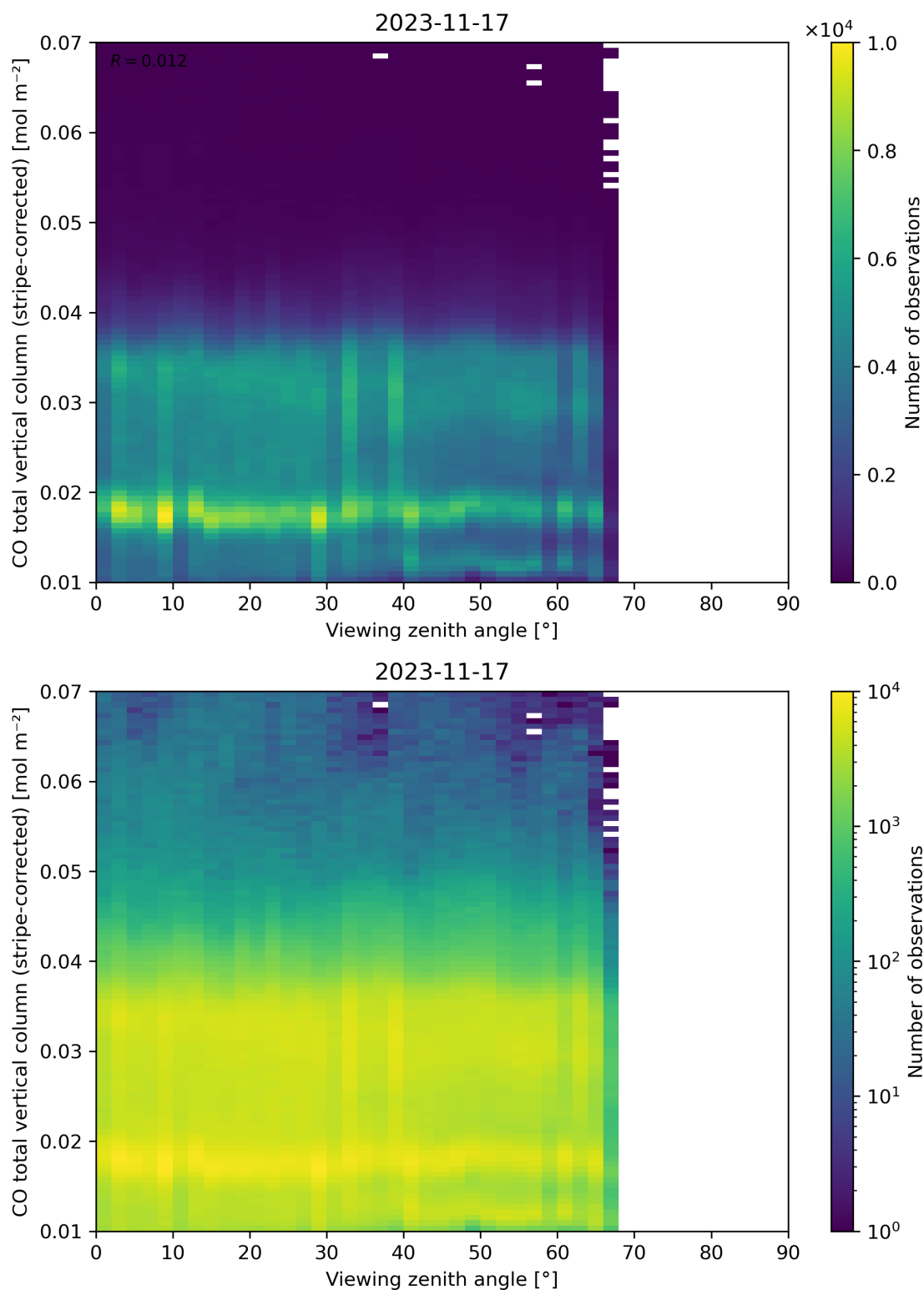
Figure 70: Scatter density plot of “Viewing zenith angle” against “CO total vertical column (stripe-corrected)” for 2023-11-16 to 2023-11-18.
