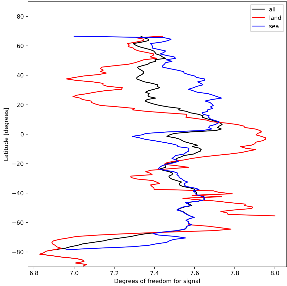
Figure 15: Zonal average of “Degrees of freedom for signal” for 2023-11-16 to 2023-11-18.
