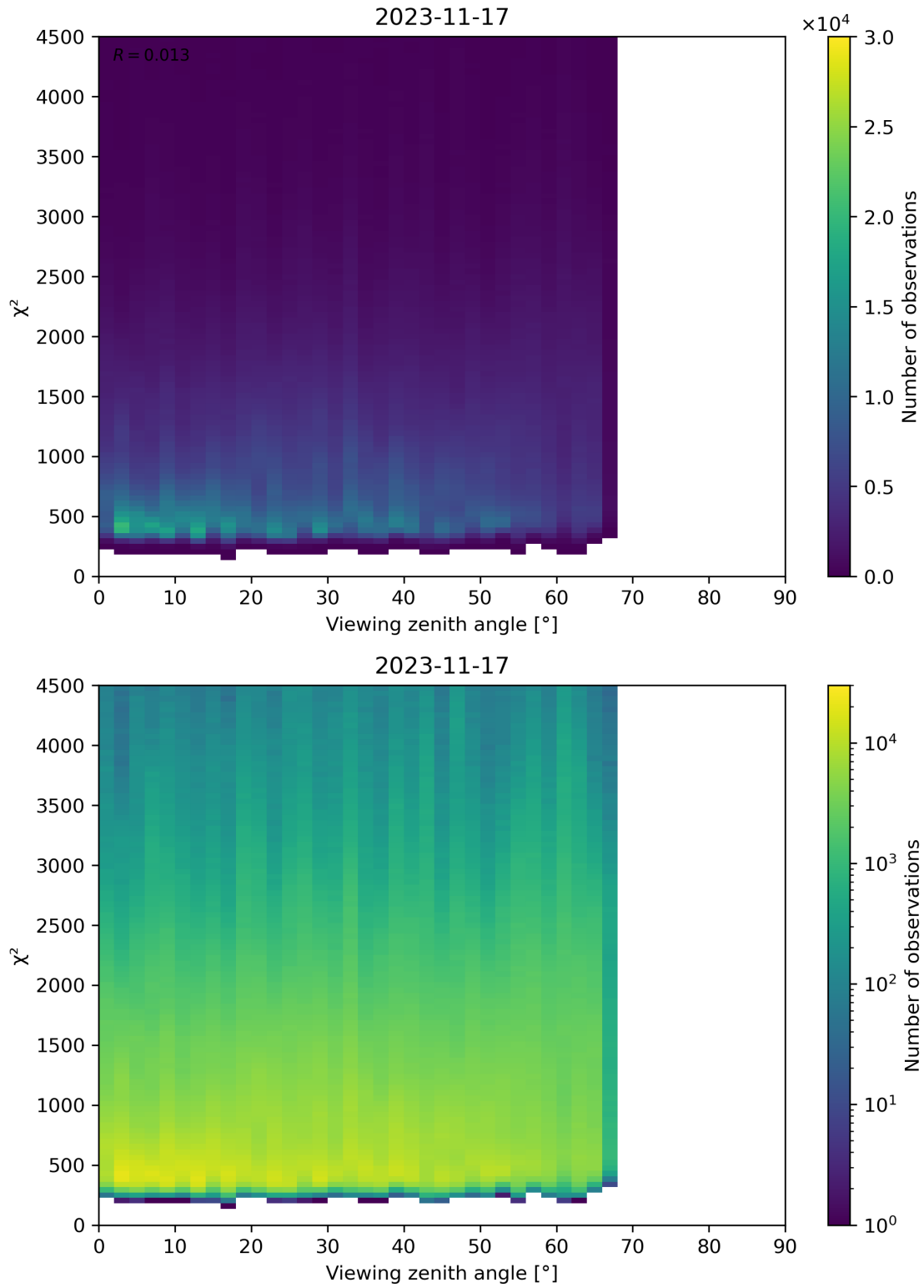
Figure 72: Scatter density plot of “Viewing zenith angle” against “ \chi^2 ” for 2023-11-16 to 2023-11-18.
