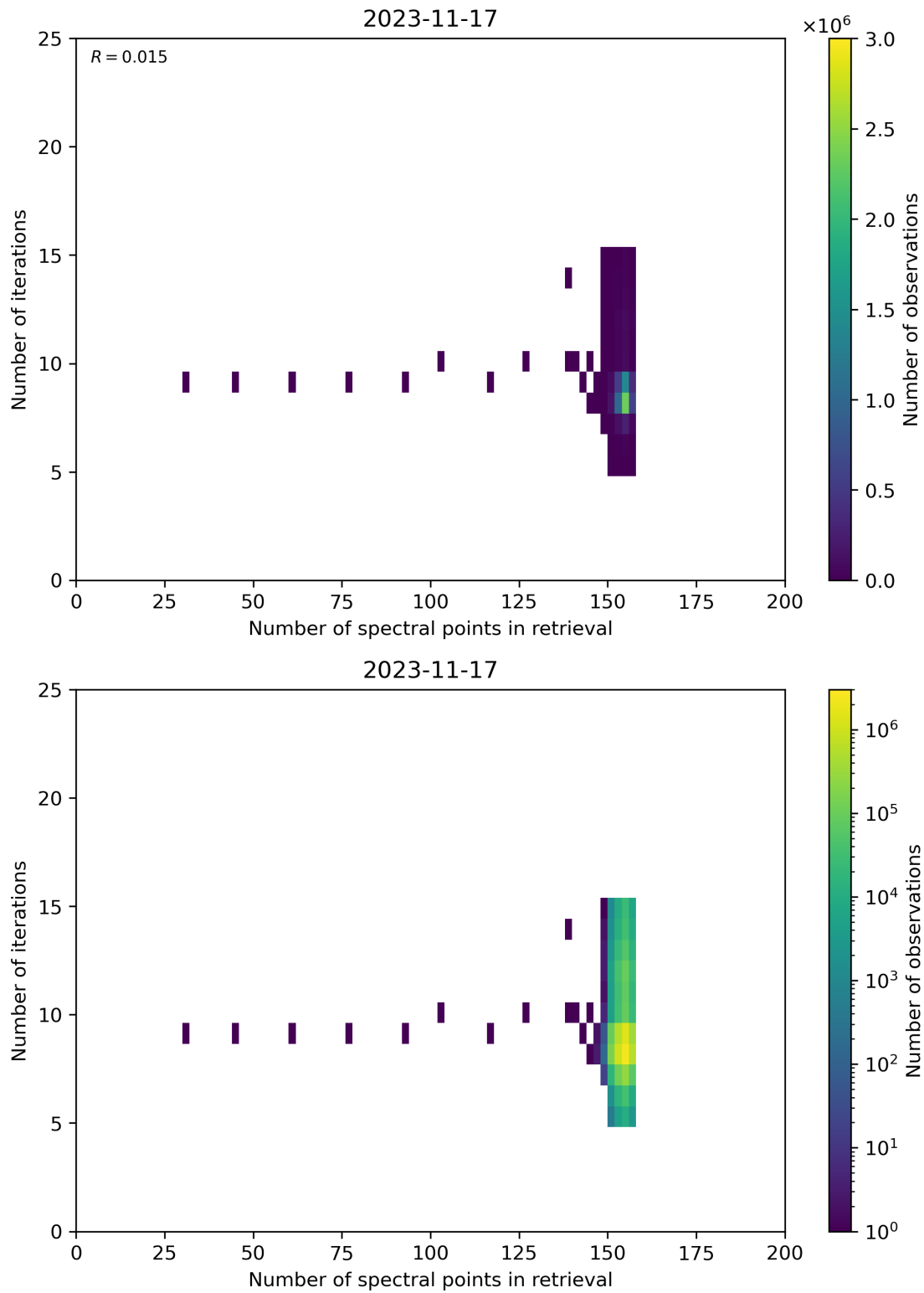
Figure 60: Scatter density plot of “Number of spectral points in retrieval” against “Number of iterations” for 2023-11-16 to 2023-11-18.
