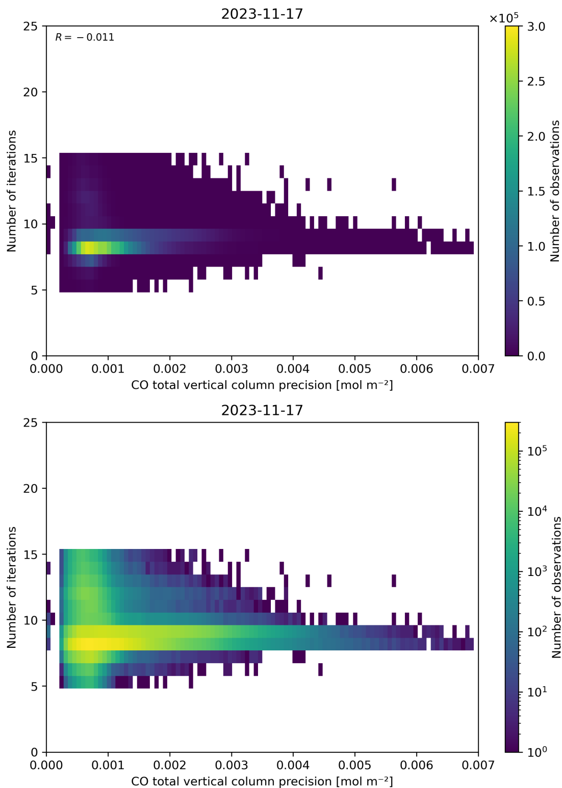
Figure 46: Scatter density plot of “CO total vertical column precision” against “Number of iterations” for 2023-11-16 to 2023-11-18.
