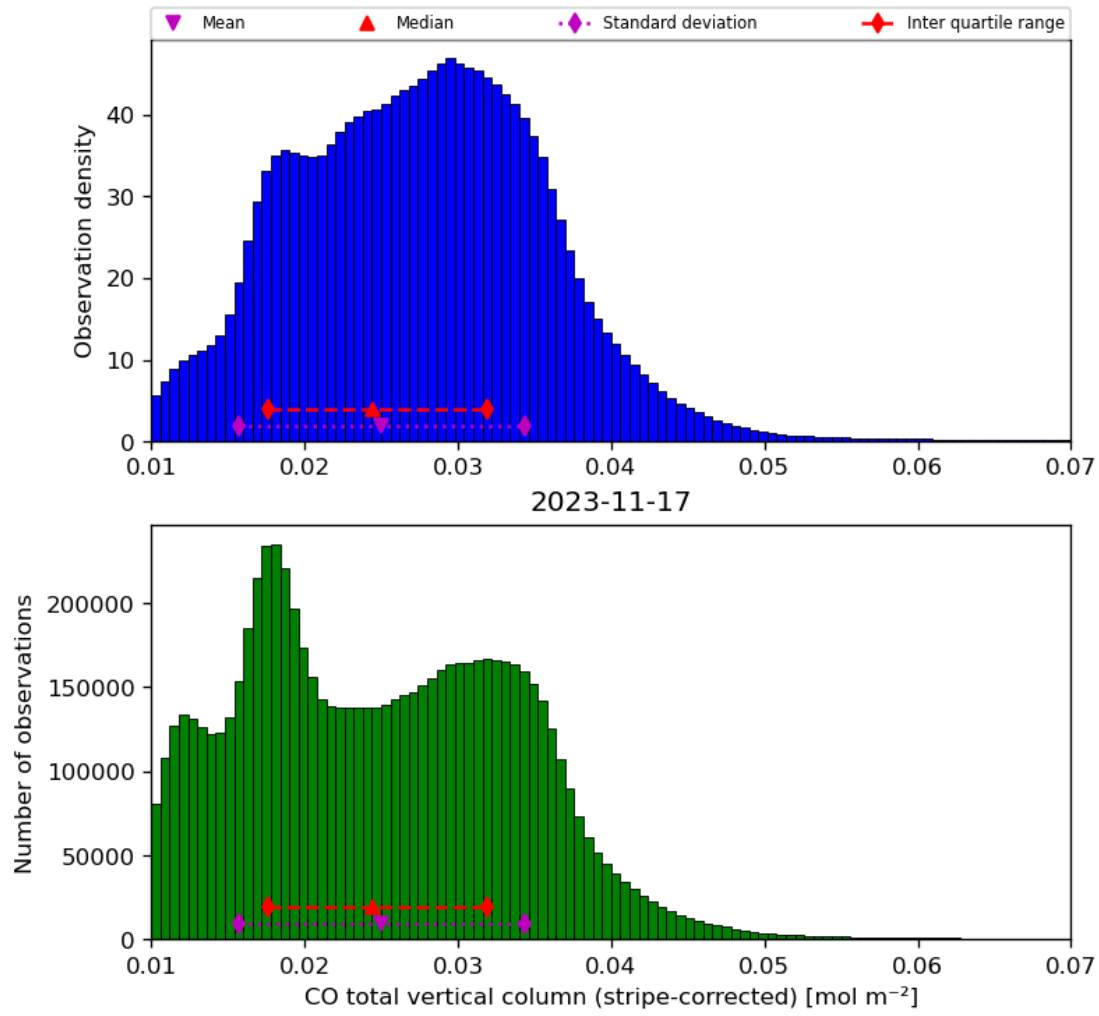
Figure 19: Histogram of “CO total vertical column (stripe-corrected)” for 2023-11-16 to 2023-11-18
