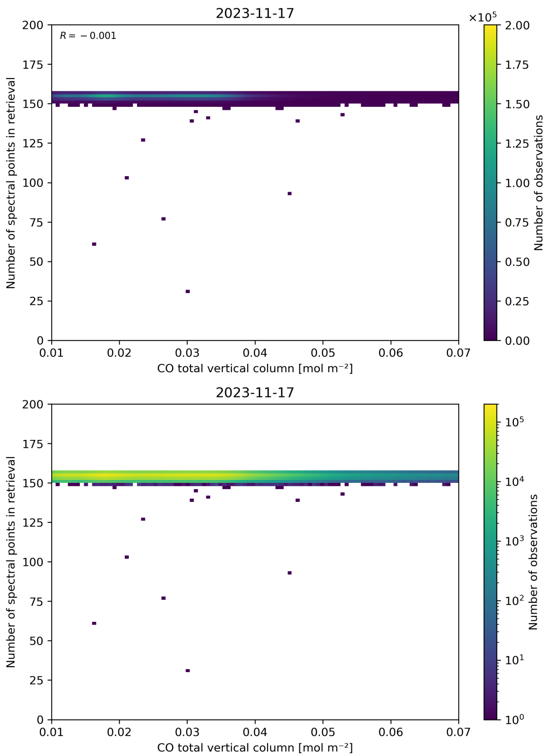
Figure 43: Scatter density plot of “CO total vertical column” against “Number of spectral points in retrieval” for 2023-11-16 to 2023-11-18.
