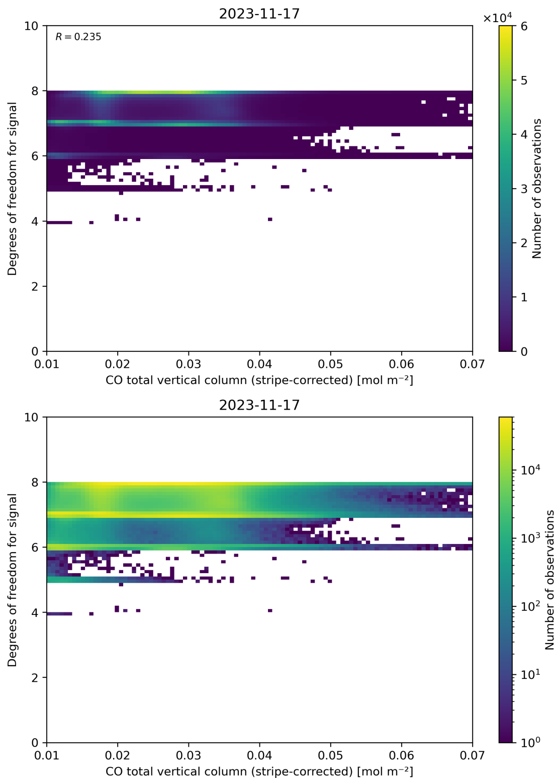
Figure 38: Scatter density plot of “CO total vertical column (stripe-corrected)” against “Degrees of freedom for signal” for 2023-11-16 to 2023-11-18.
