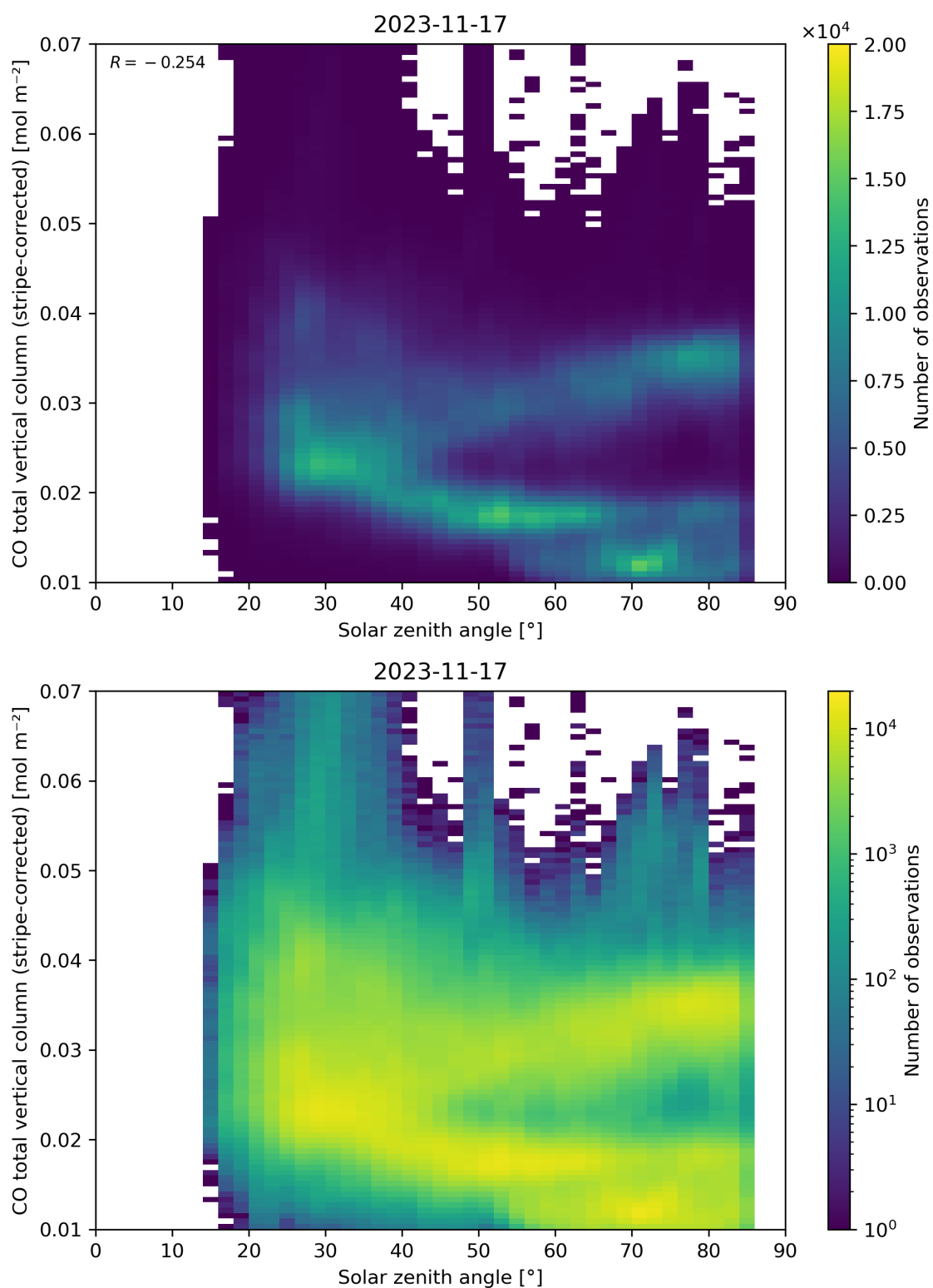
Figure 62: Scatter density plot of “Solar zenith angle” against “CO total vertical column (stripe-corrected)” for 2023-11-16 to 2023-11-18.
