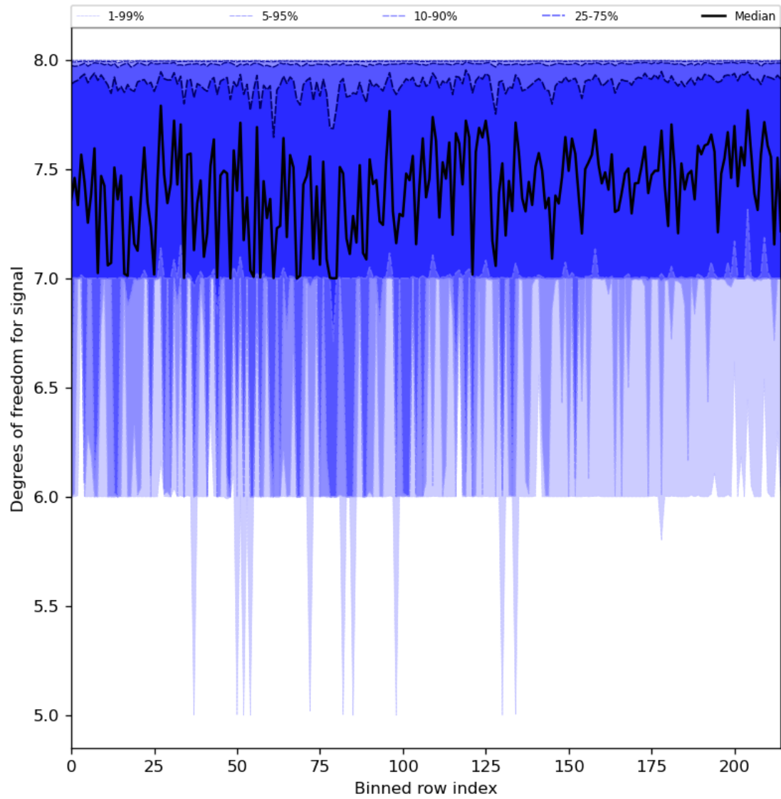
Figure 31: Along track statistics of “Degrees of freedom for signal” for 2023-11-16 to 2023-11-18
