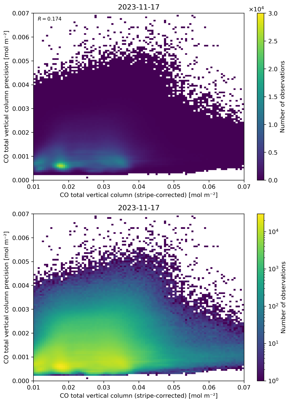
Figure 36: Scatter density plot of “CO total vertical column (stripe-corrected)” against “CO total vertical column precision” for 2023-11-16 to 2023-11-18.
