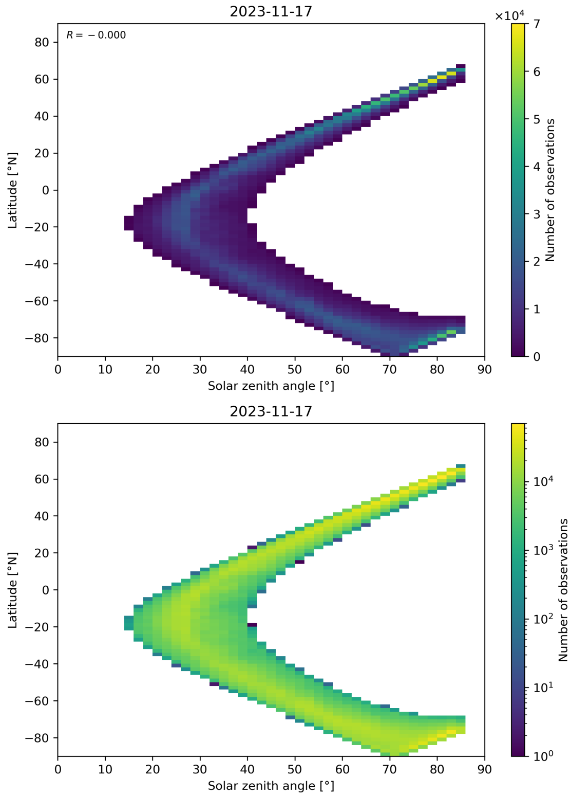
Figure 66: Scatter density plot of “Solar zenith angle” against “Latitude” for 2023-11-16 to 2023-11-18.
