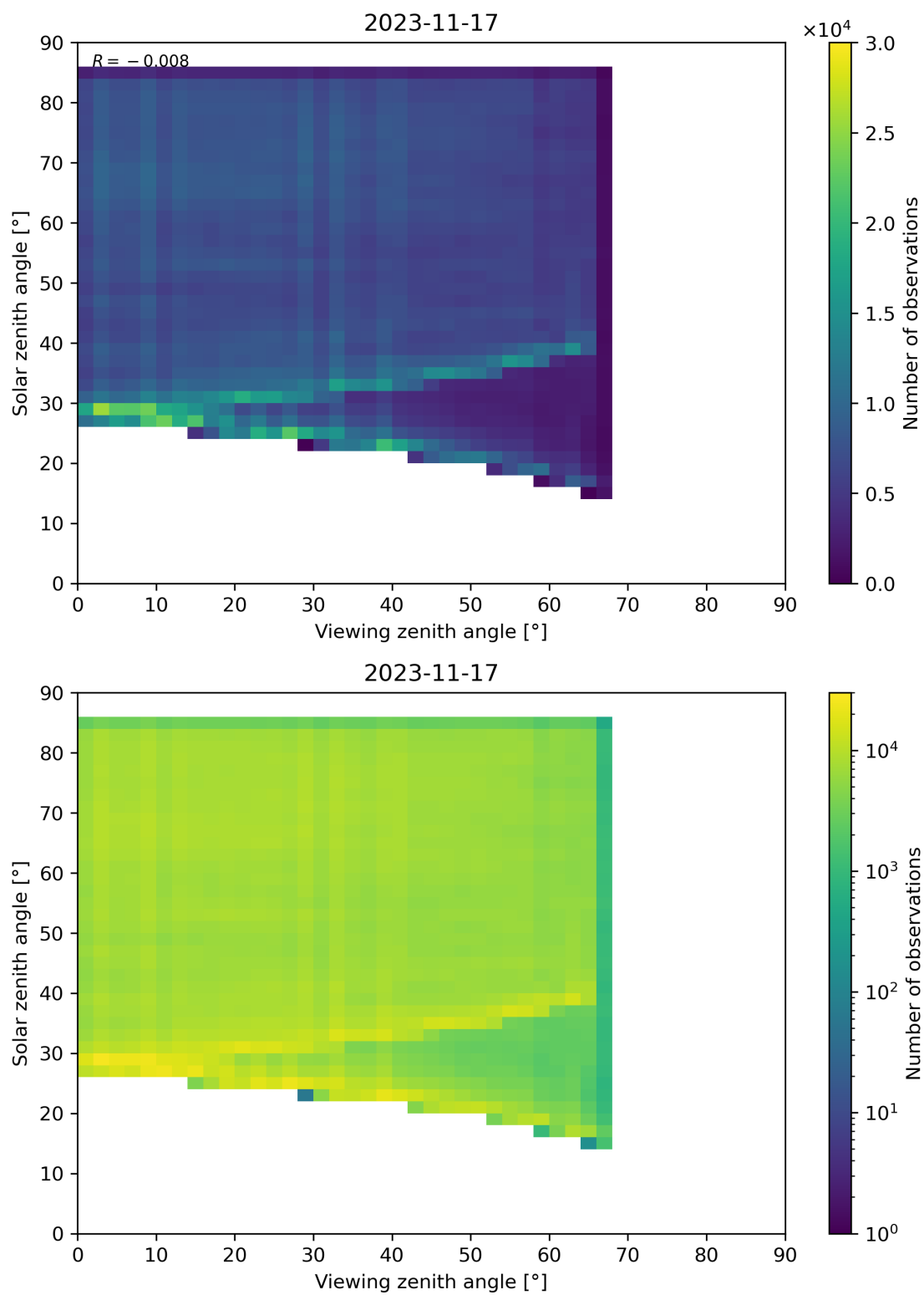
Figure 77: Scatter density plot of “Viewing zenith angle” against “Solar zenith angle” for 2023-11-16 to 2023-11-18.
