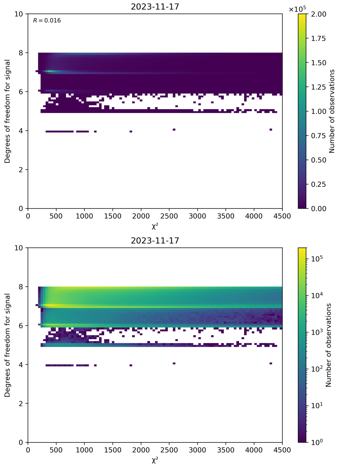
Figure 48: Scatter density plot of “ \chi^2 ” against “Degrees of freedom for signal” for 2023-11-16 to 2023-11-18.
