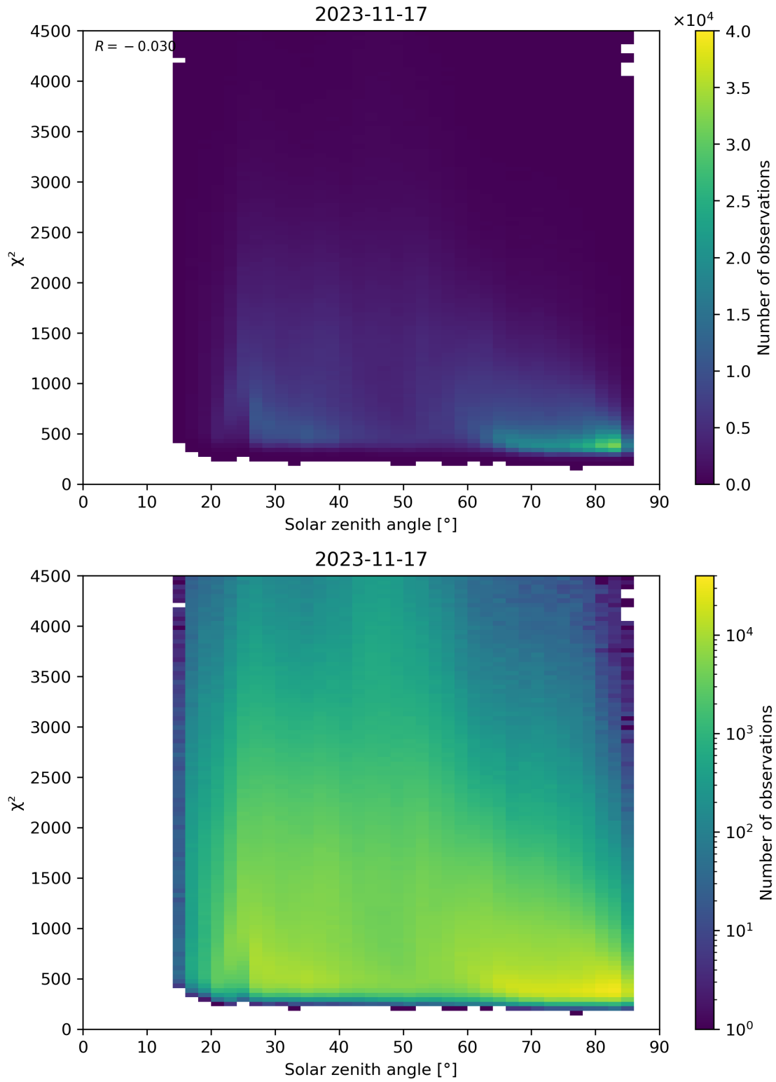
Figure 64: Scatter density plot of “Solar zenith angle” against “ \chi^2 ” for 2023-11-16 to 2023-11-18.
