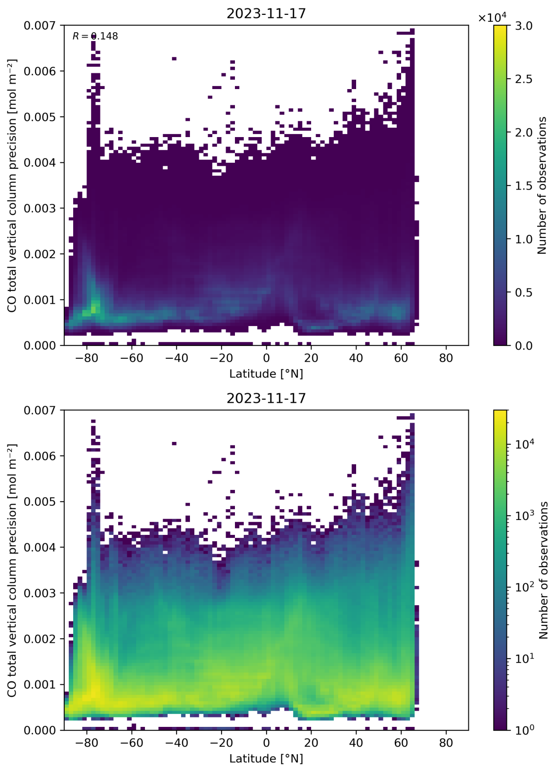
Figure 53: Scatter density plot of “Latitude” against “CO total vertical column precision” for 2023-11-16 to 2023-11-18.
