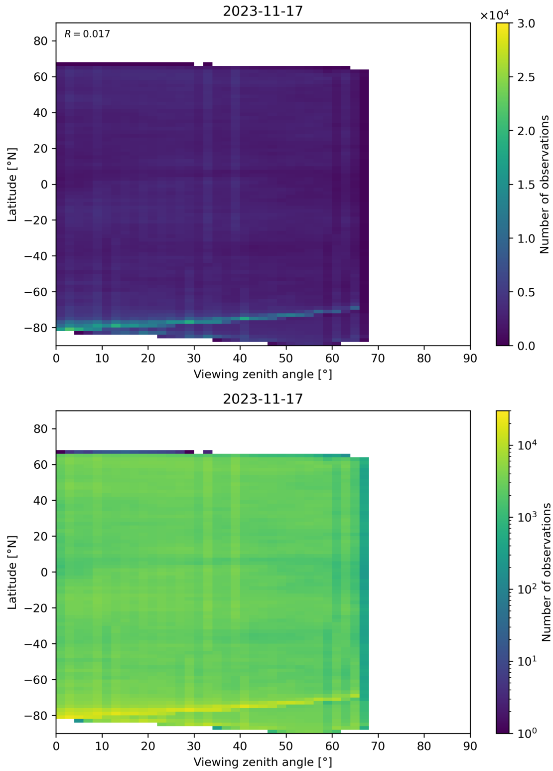
Figure 74: Scatter density plot of “Viewing zenith angle” against “Latitude” for 2023-11-16 to 2023-11-18.
