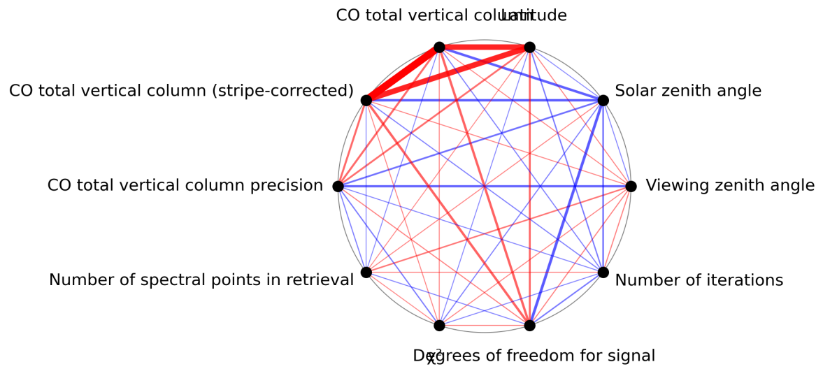
Figure 1: Map of correlation graph for 2023-11-16 to 2023-11-18.
