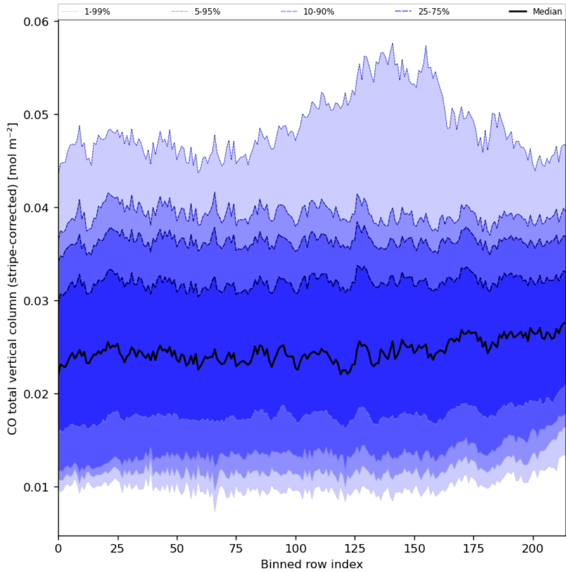
Figure 27: Along track statistics of “CO total vertical column (stripe-corrected)” for 2023-11-16 to 2023-11-18
