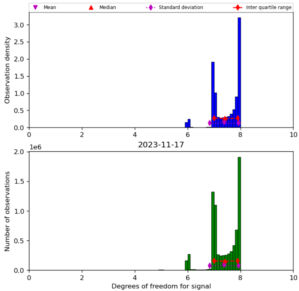
Figure 23: Histogram of “Degrees of freedom for signal” for 2023-11-16 to 2023-11-18
