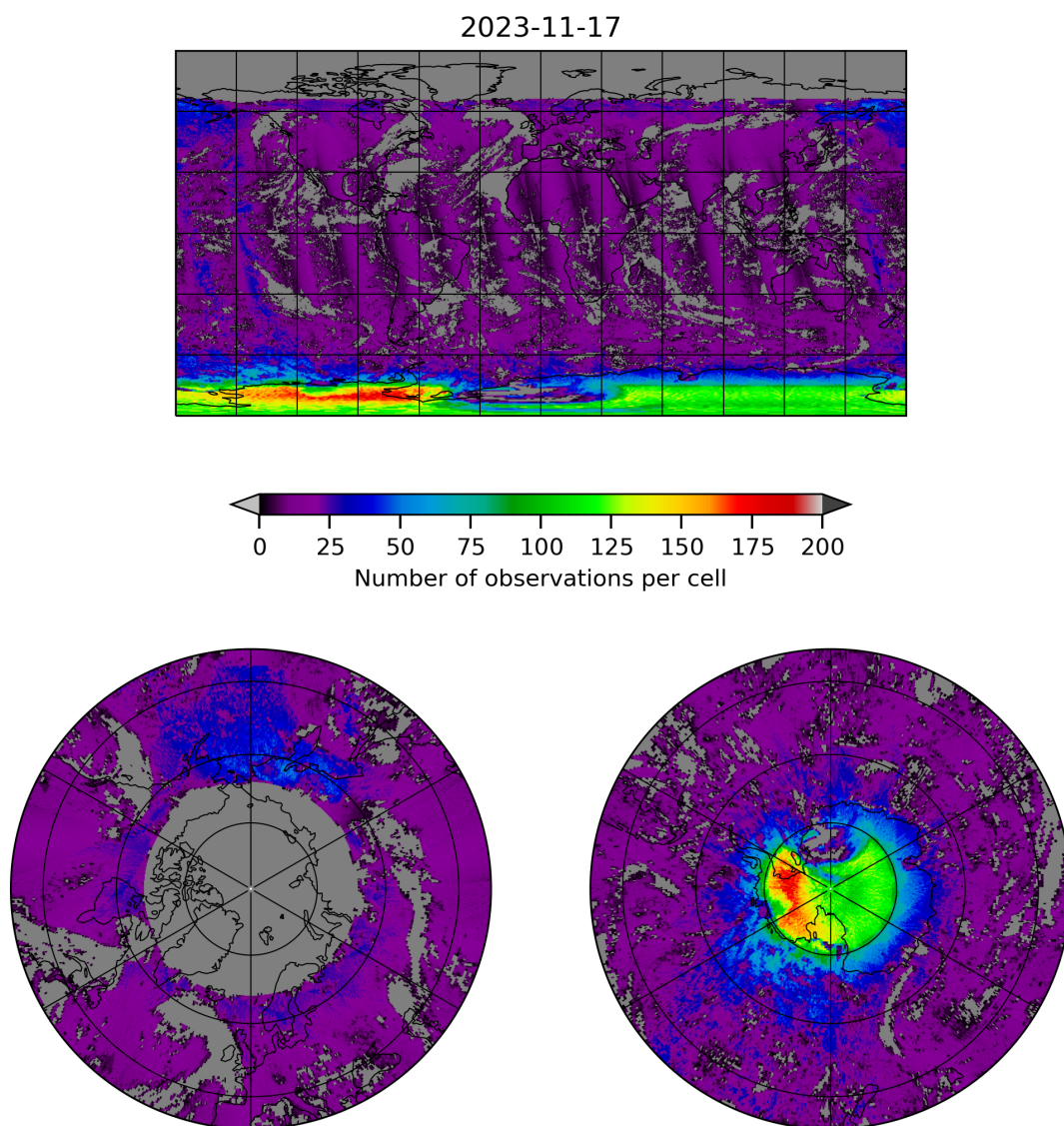
Figure 8: Map of the number of observations for 2023-11-16 to 2023-11-18
