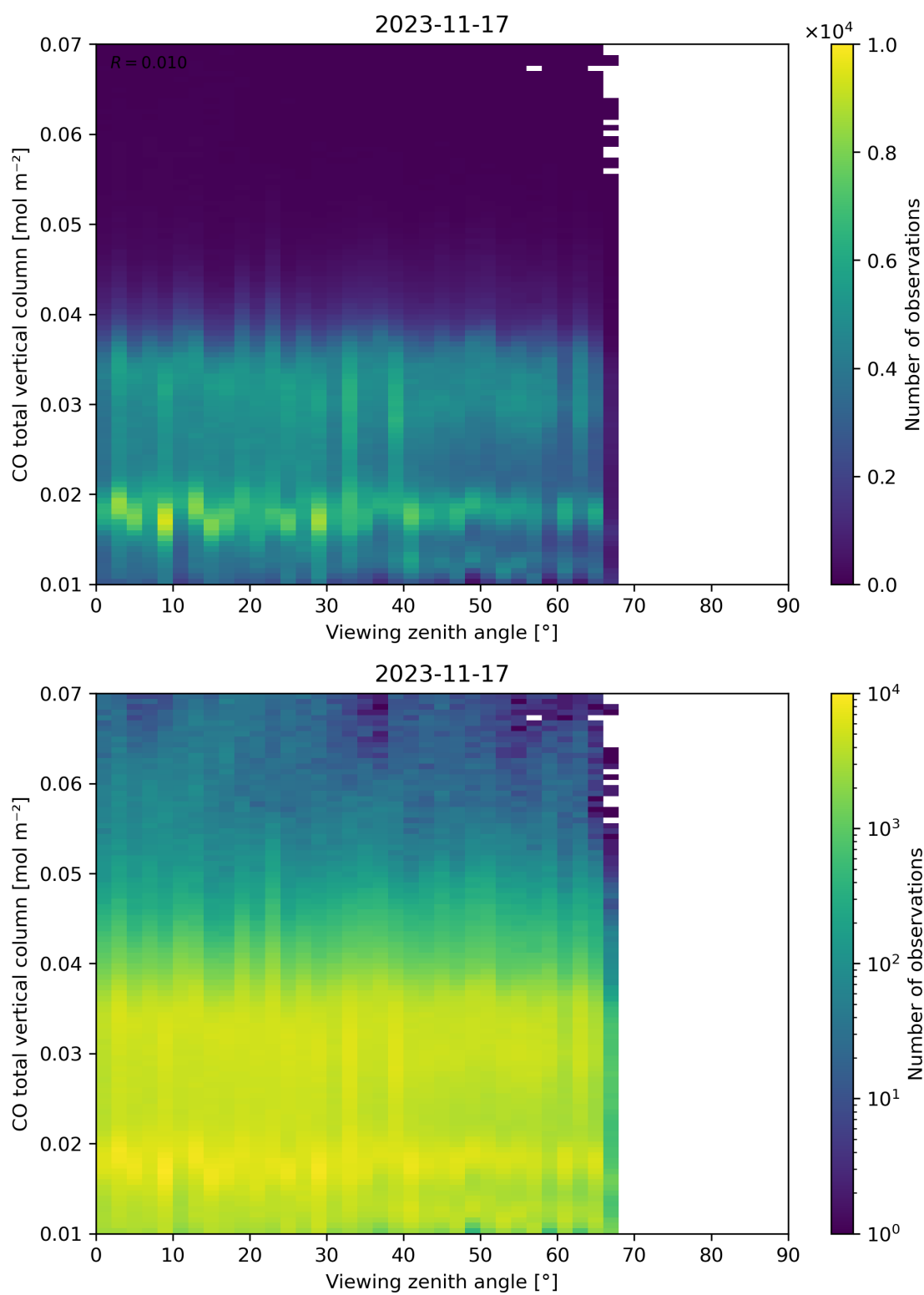
Figure 69: Scatter density plot of “Viewing zenith angle” against “CO total vertical column” for 2023-11-16 to 2023-11-18.
