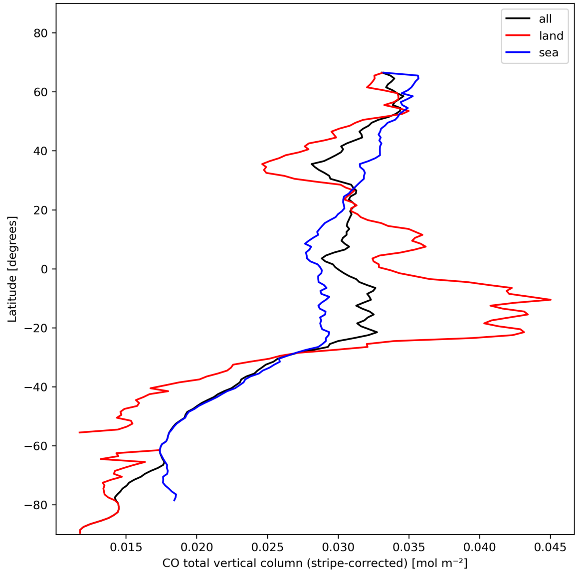
Figure 11: Zonal average of “CO total vertical column (stripe-corrected)” for 2023-11-16 to 2023-11-18.
