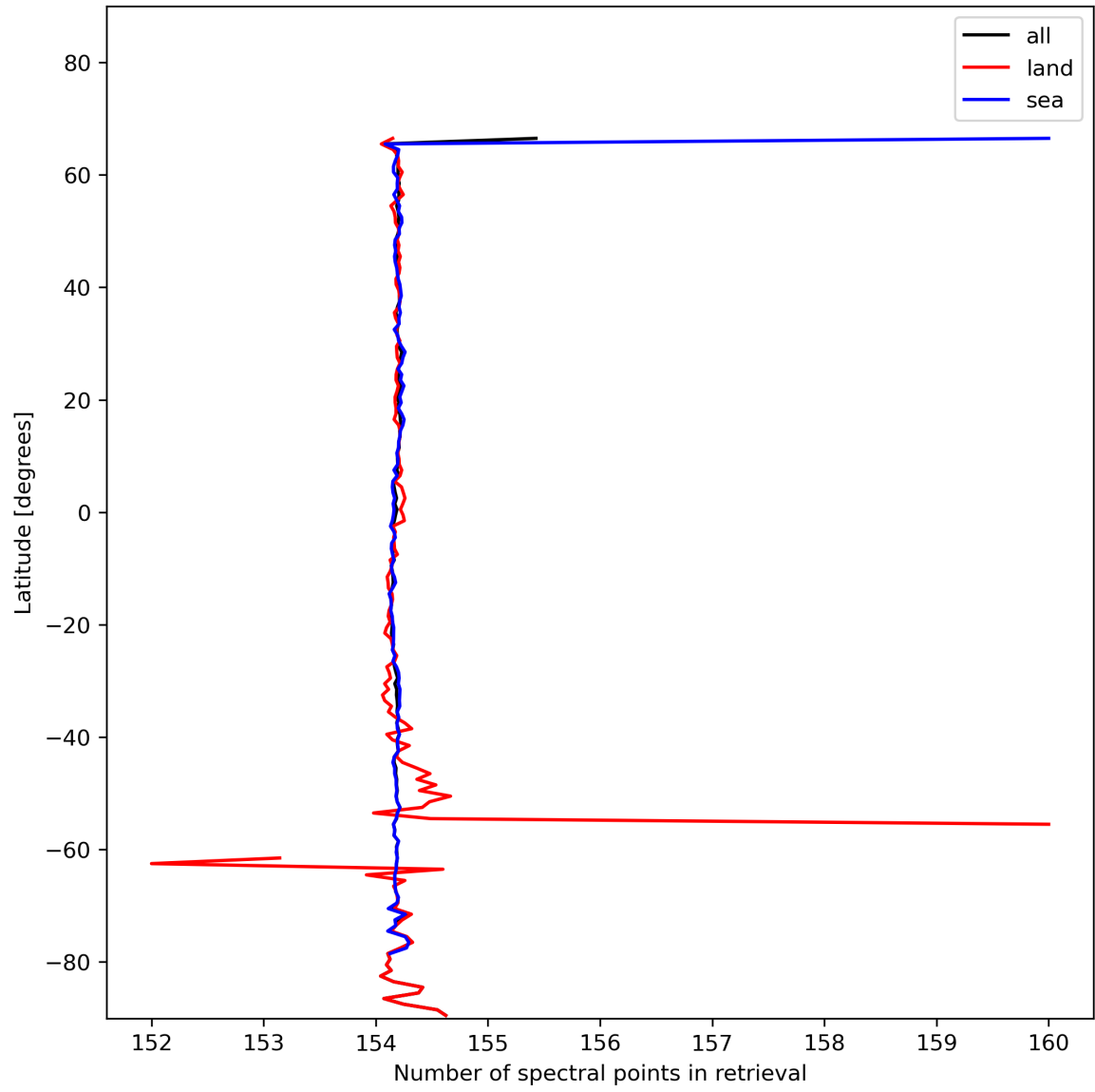
Figure 13: Zonal average of “Number of spectral points in retrieval” for 2023-11-16 to 2023-11-18.
