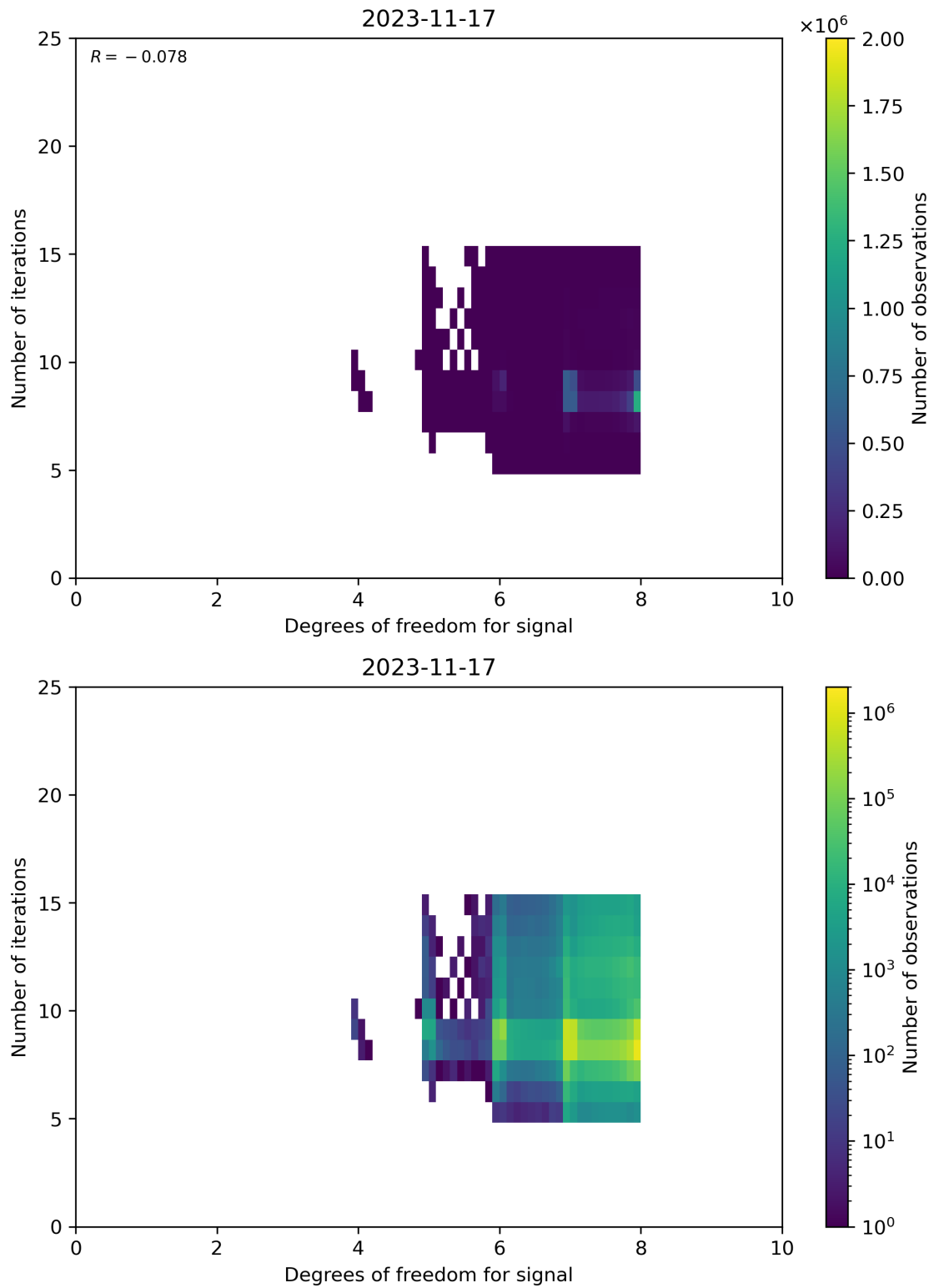
Figure 50: Scatter density plot of “Degrees of freedom for signal” against “Number of iterations” for 2023-11-16 to 2023-11-18.
