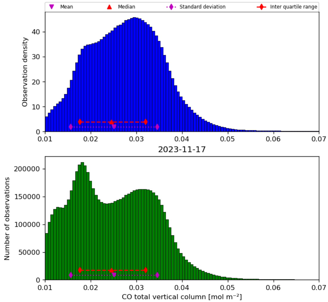
Figure 18: Histogram of “CO total vertical column” for 2023-11-16 to 2023-11-18
