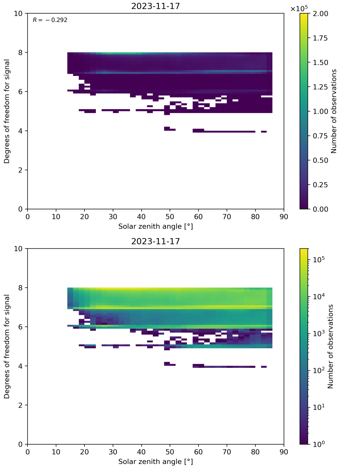
Figure 65: Scatter density plot of “Solar zenith angle” against “Degrees of freedom for signal” for 2023-11-16 to 2023-11-18.
