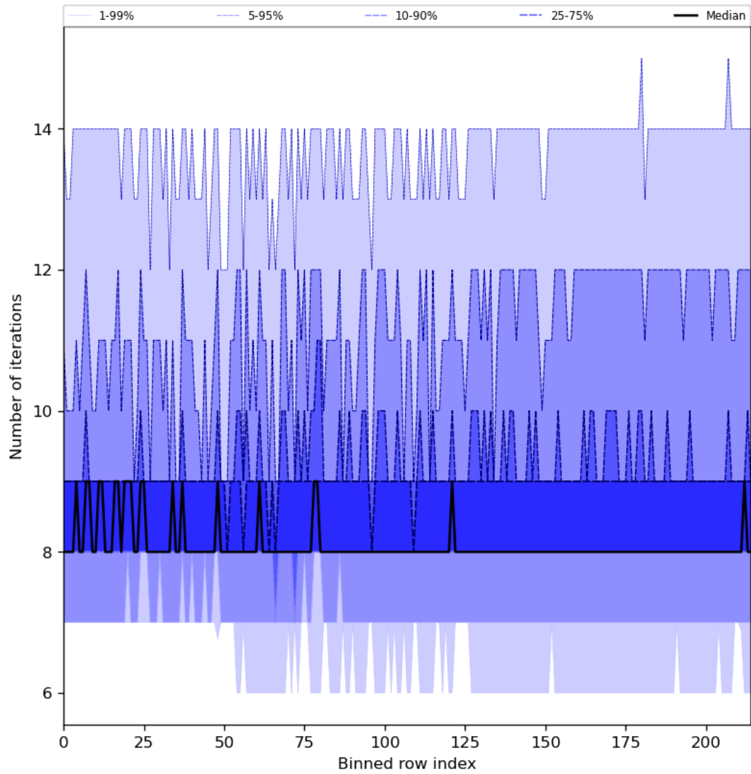
Figure 32: Along track statistics of “Number of iterations” for 2023-11-16 to 2023-11-18
