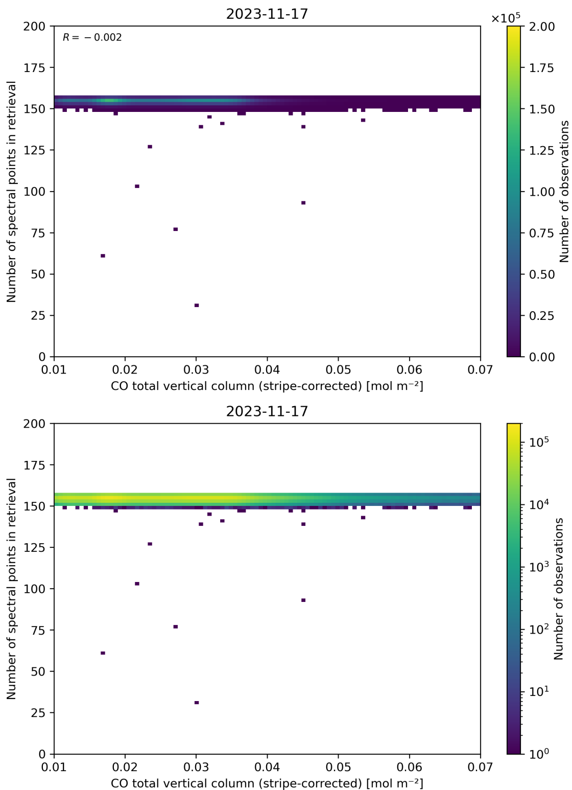
Figure 40: Scatter density plot of “CO total vertical column (stripe-corrected)” against “Number of spectral points in retrieval” for 2023-11-16 to 2023-11-18.
