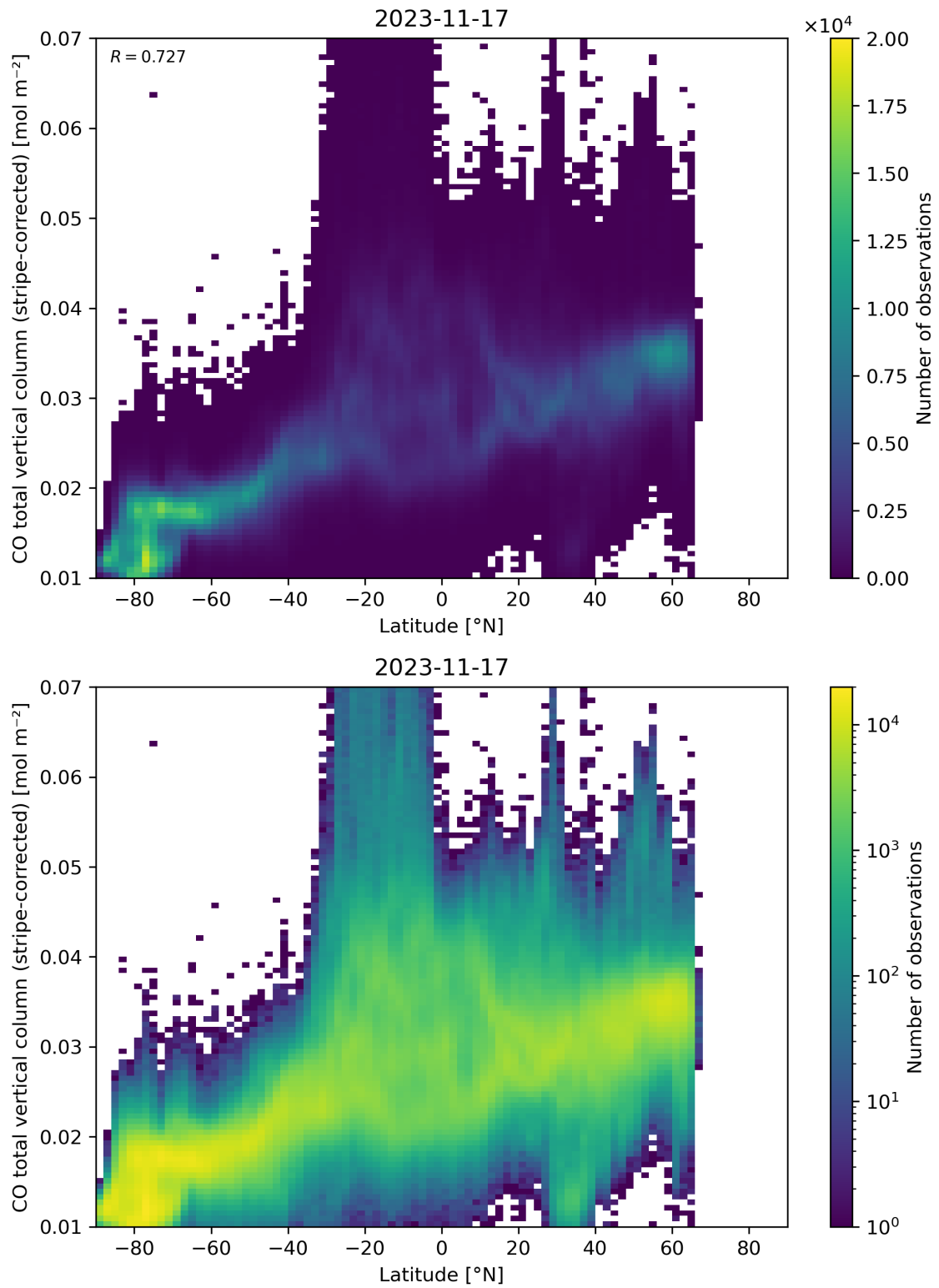
Figure 52: Scatter density plot of “Latitude” against “CO total vertical column (stripe-corrected)” for 2023-11-16 to 2023-11-18.
