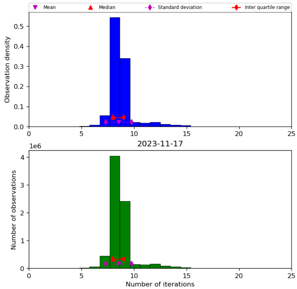
Figure 24: Histogram of “Number of iterations” for 2023-11-16 to 2023-11-18
