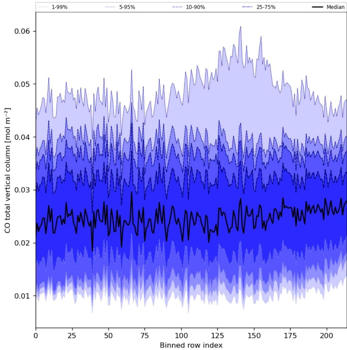
Figure 26: Along track statistics of “CO total vertical column” for 2023-11-16 to 2023-11-18
