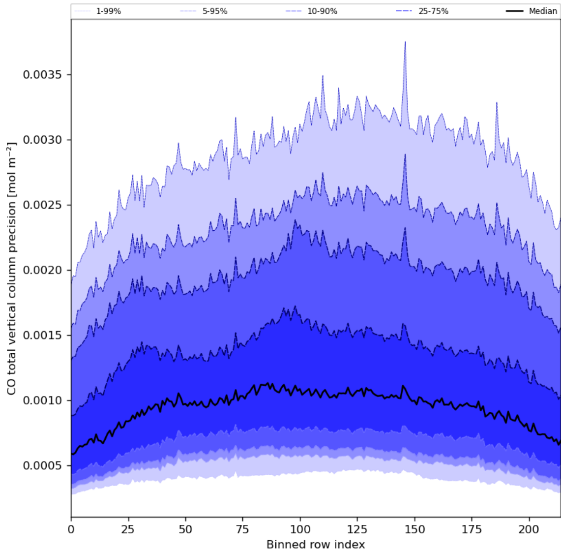
Figure 28: Along track statistics of “CO total vertical column precision” for 2023-11-16 to 2023-11-18
