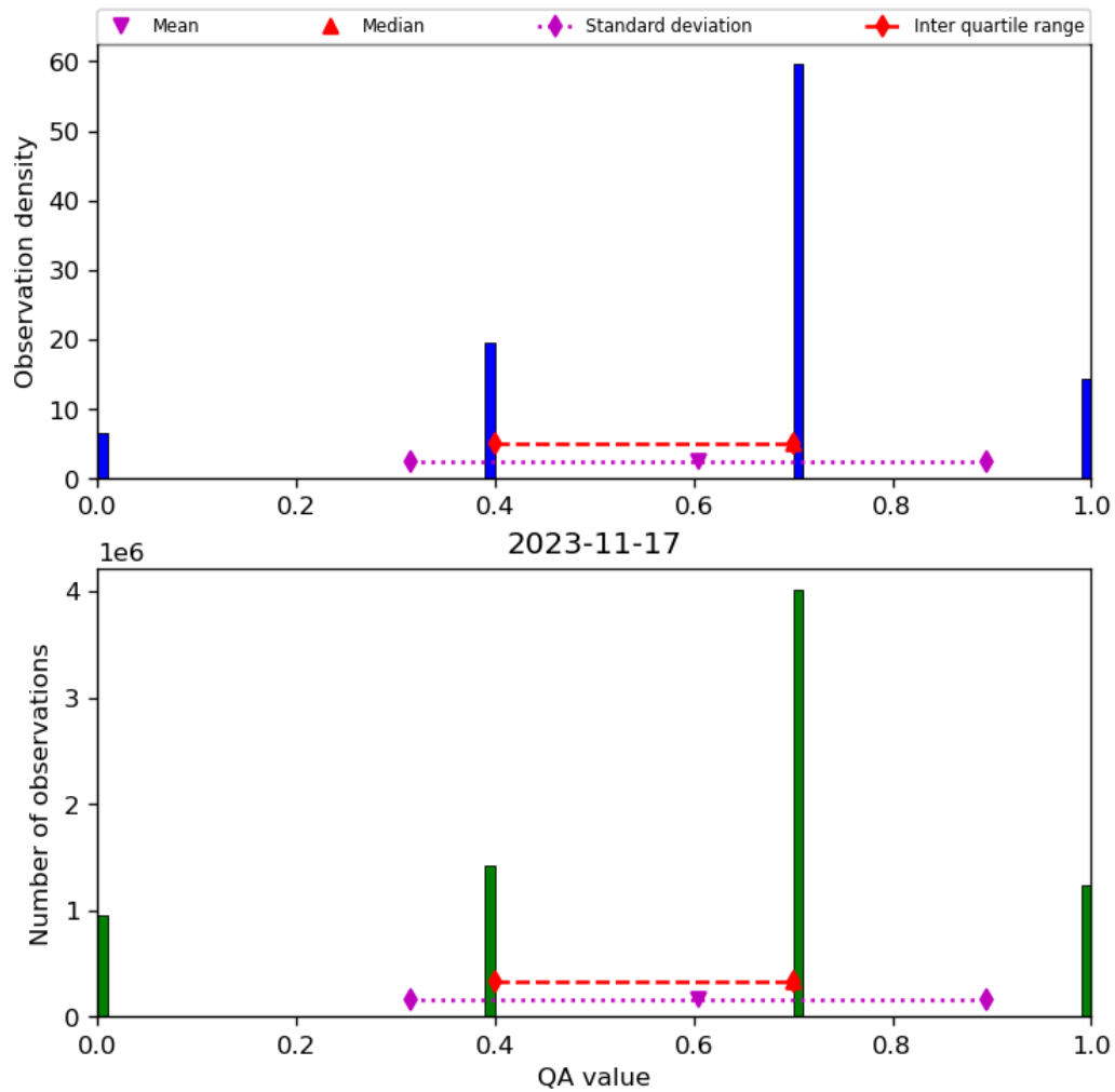
Figure 17: Histogram of “QA value” for 2023-11-16 to 2023-11-18
