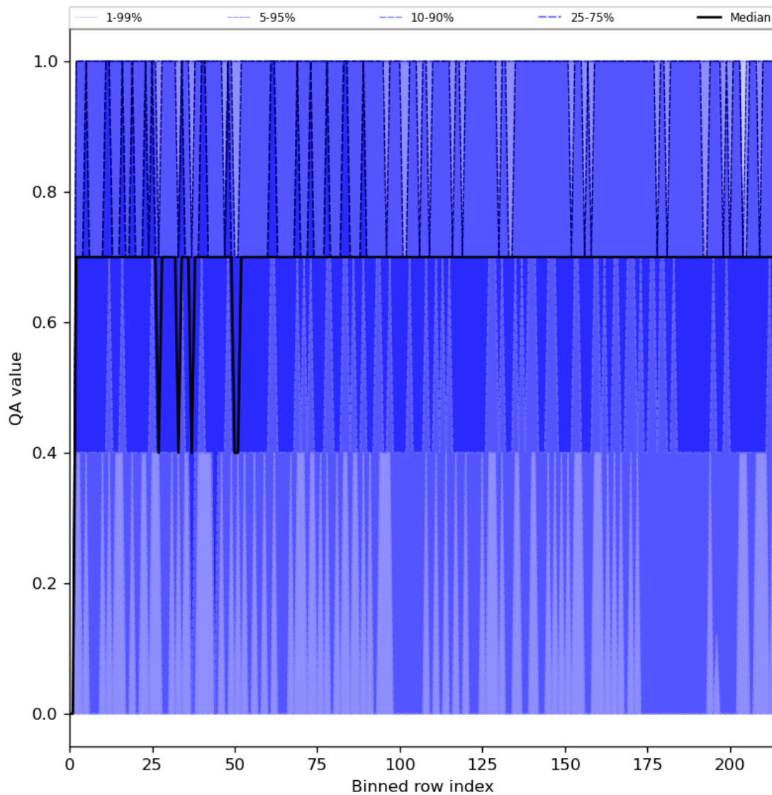
Figure 25: Along track statistics of “QA value” for 2023-11-16 to 2023-11-18
