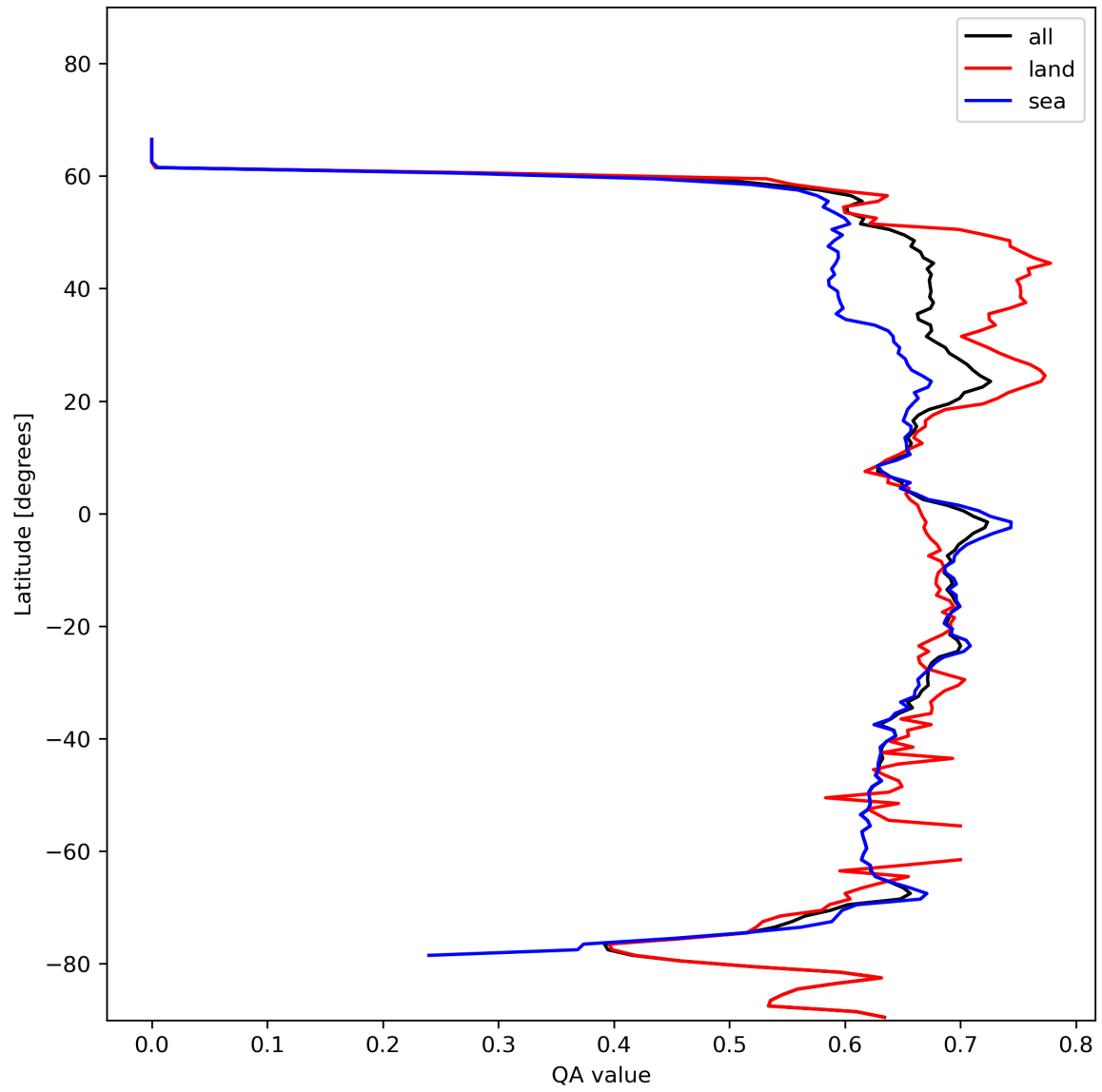
Figure 9: Zonal average of “QA value” for 2023-11-16 to 2023-11-18.
