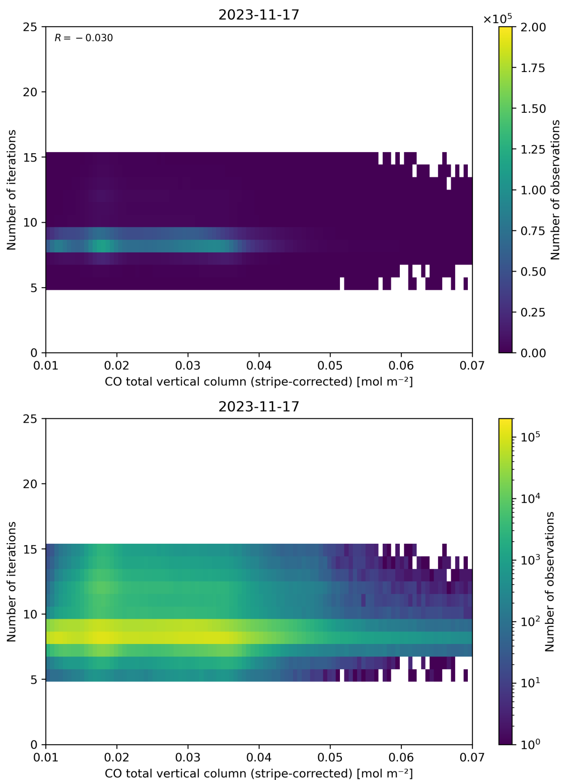
Figure 39: Scatter density plot of “CO total vertical column (stripe-corrected)” against “Number of iterations” for 2023-11-16 to 2023-11-18.
