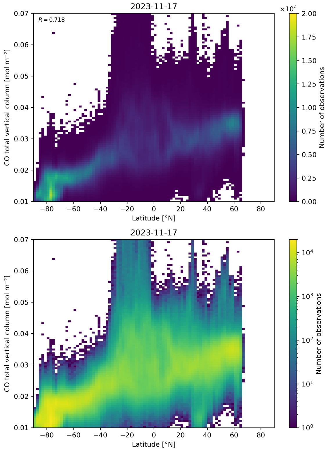
Figure 51: Scatter density plot of “Latitude” against “CO total vertical column” for 2023-11-16 to 2023-11-18.
