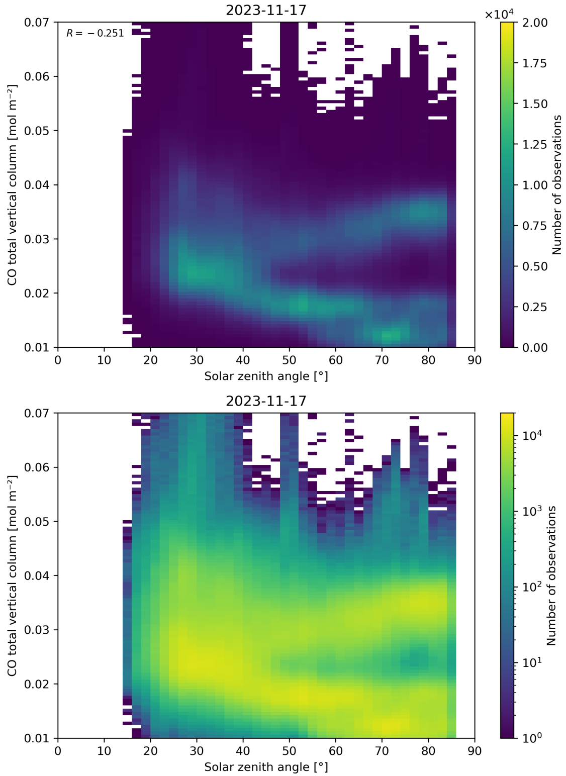
Figure 61: Scatter density plot of “Solar zenith angle” against “CO total vertical column” for 2023-11-16 to 2023-11-18.
