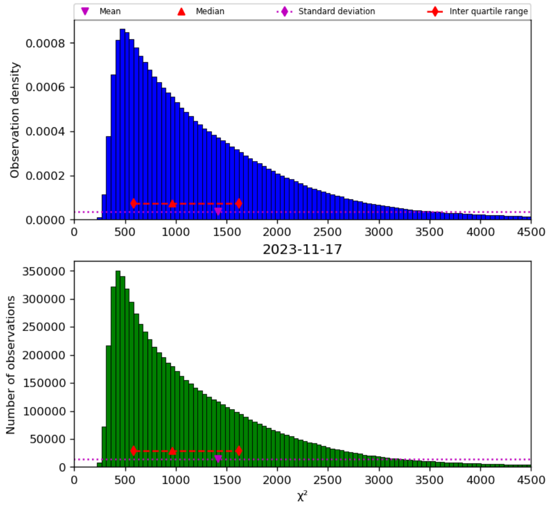
Figure 22: Histogram of “ \chi^2 ” for 2023-11-16 to 2023-11-18
