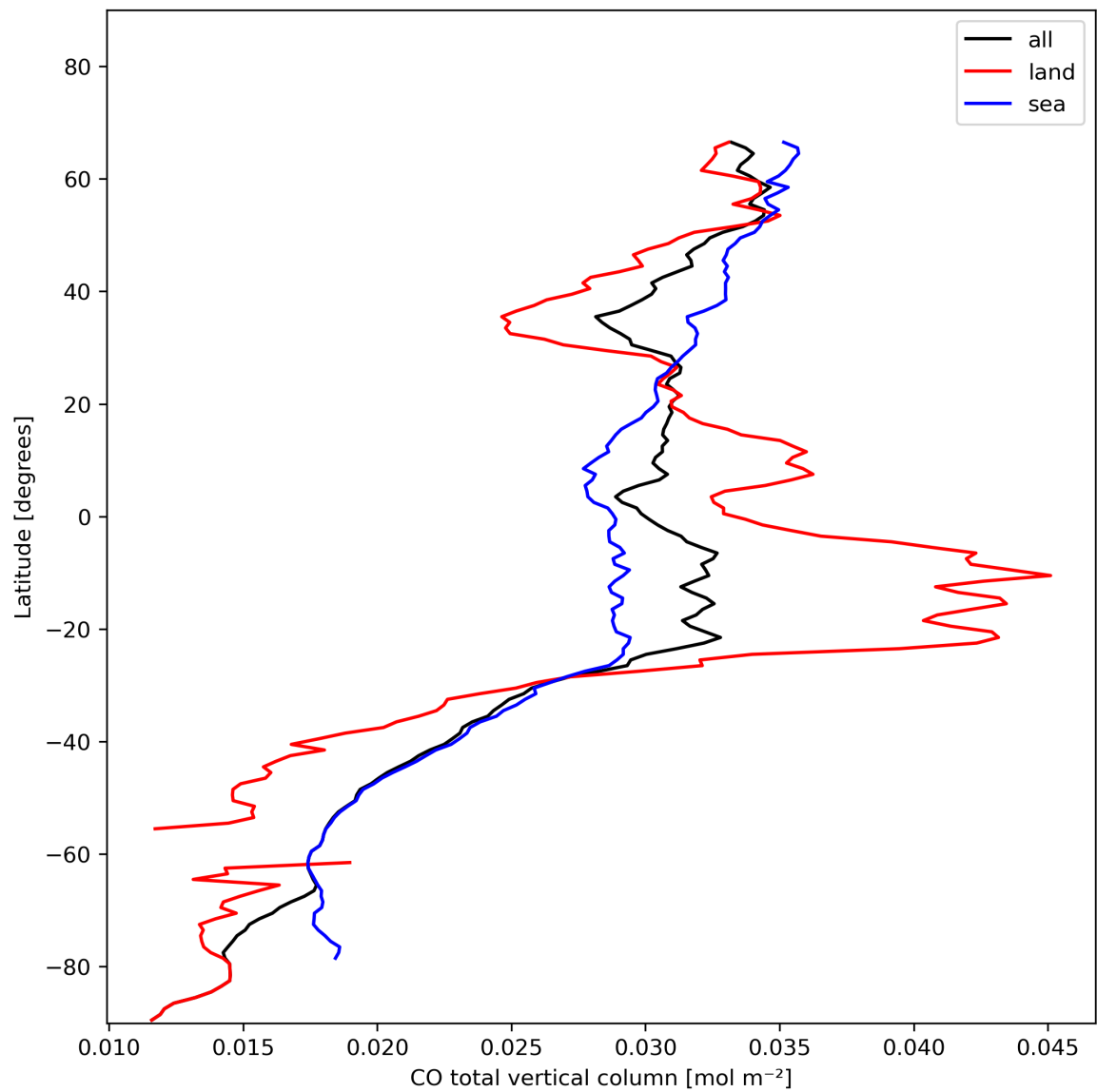
Figure 10: Zonal average of “CO total vertical column” for 2023-11-16 to 2023-11-18.
