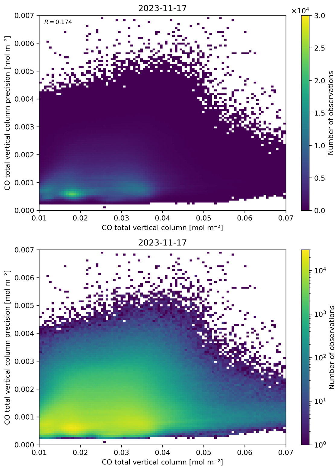
Figure 34: Scatter density plot of “CO total vertical column” against “CO total vertical column precision” for 2023-11-16 to 2023-11-18.
