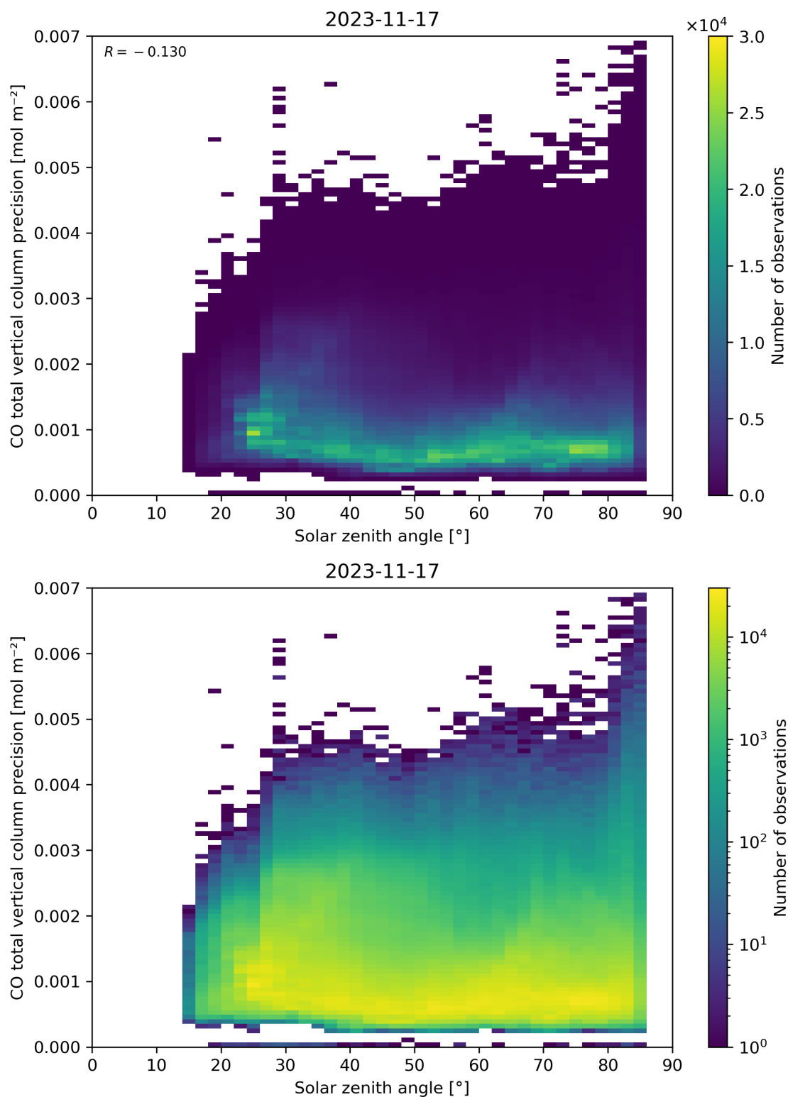
Figure 63: Scatter density plot of “Solar zenith angle” against “CO total vertical column precision” for 2023-11-16 to 2023-11-18.
