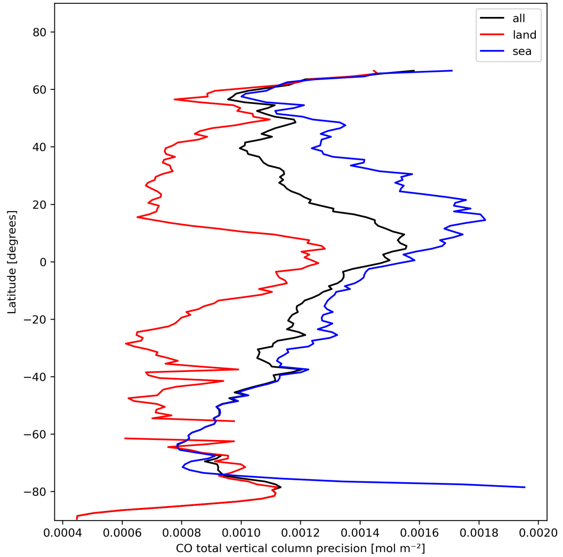
Figure 12: Zonal average of “CO total vertical column precision” for 2023-11-16 to 2023-11-18.
