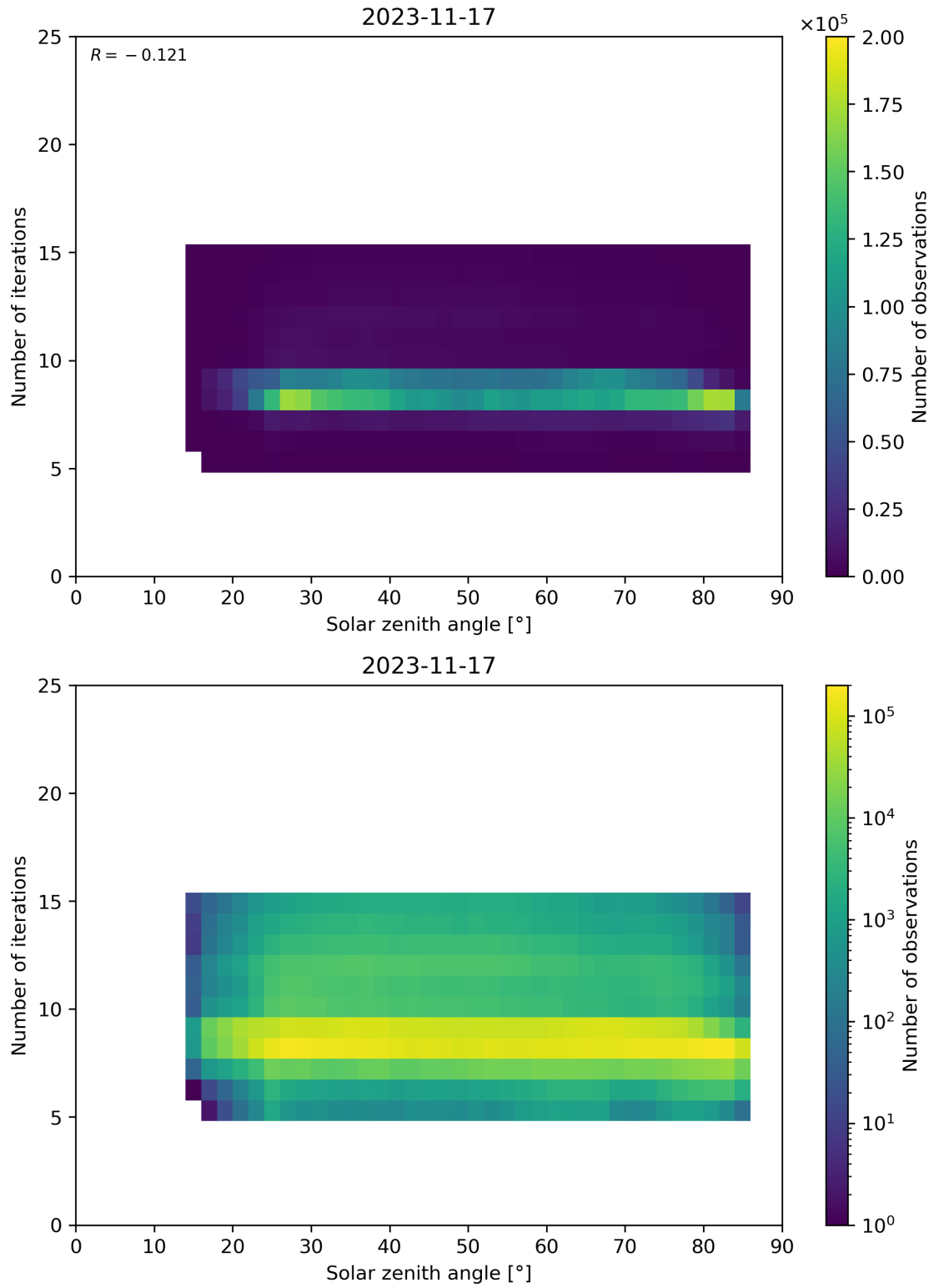
Figure 67: Scatter density plot of “Solar zenith angle” against “Number of iterations” for 2023-11-16 to 2023-11-18.
