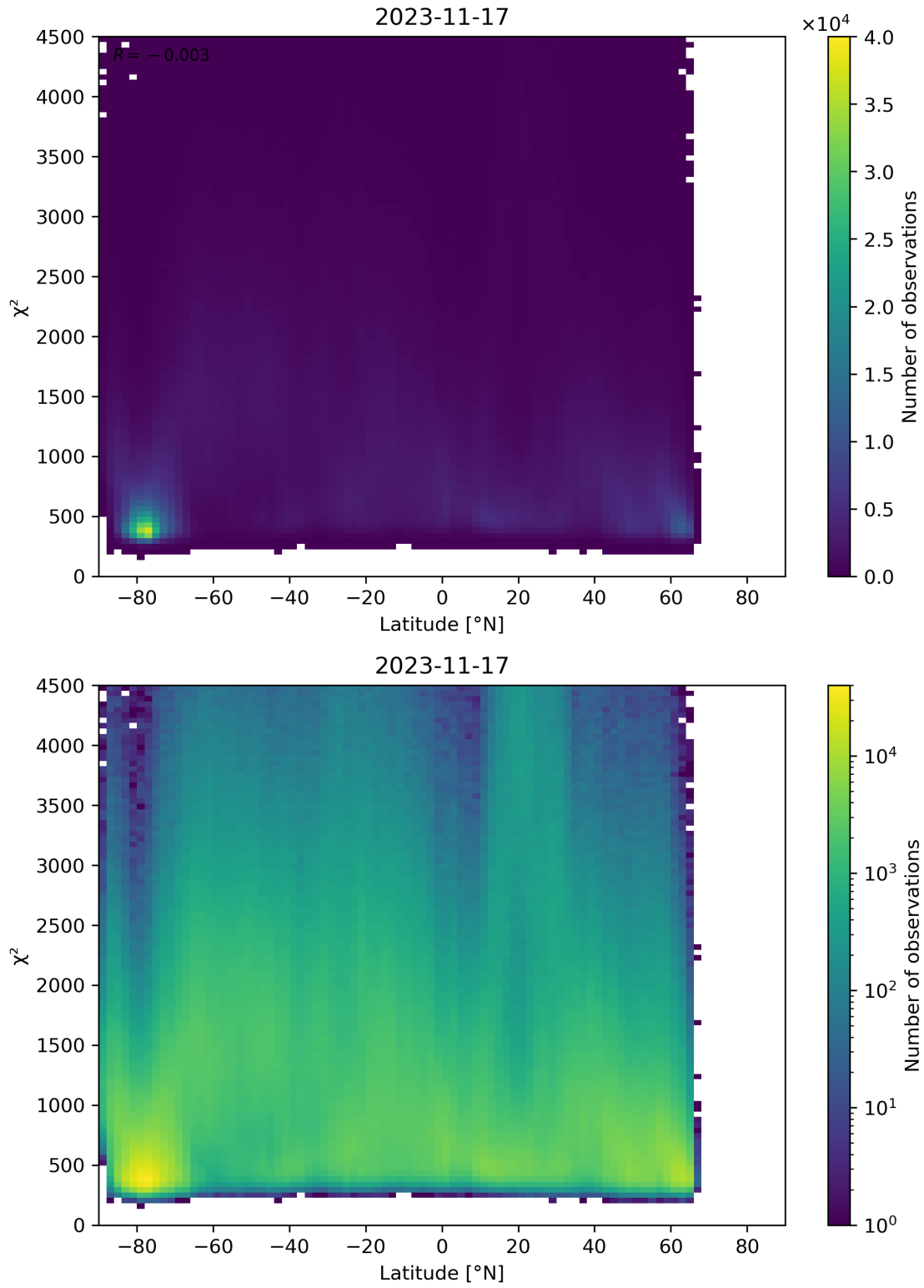
Figure 54: Scatter density plot of “Latitude” against “ \chi^2 ” for 2023-11-16 to 2023-11-18.
