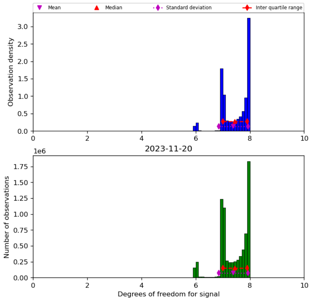
Figure 23: Histogram of “Degrees of freedom for signal” for 2023-11-19 to 2023-11-21
