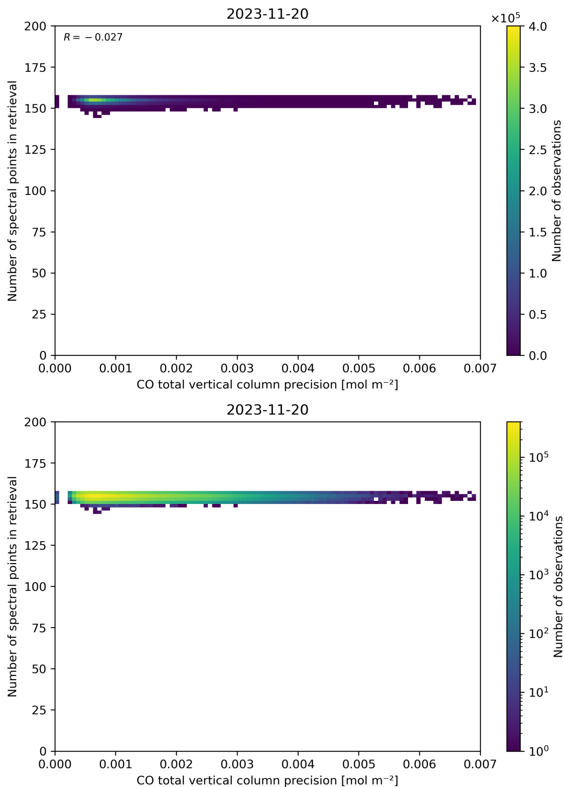
Figure 47: Scatter density plot of “CO total vertical column precision” against “Number of spectral points in retrieval” for 2023-11-19 to 2023-11-21.
