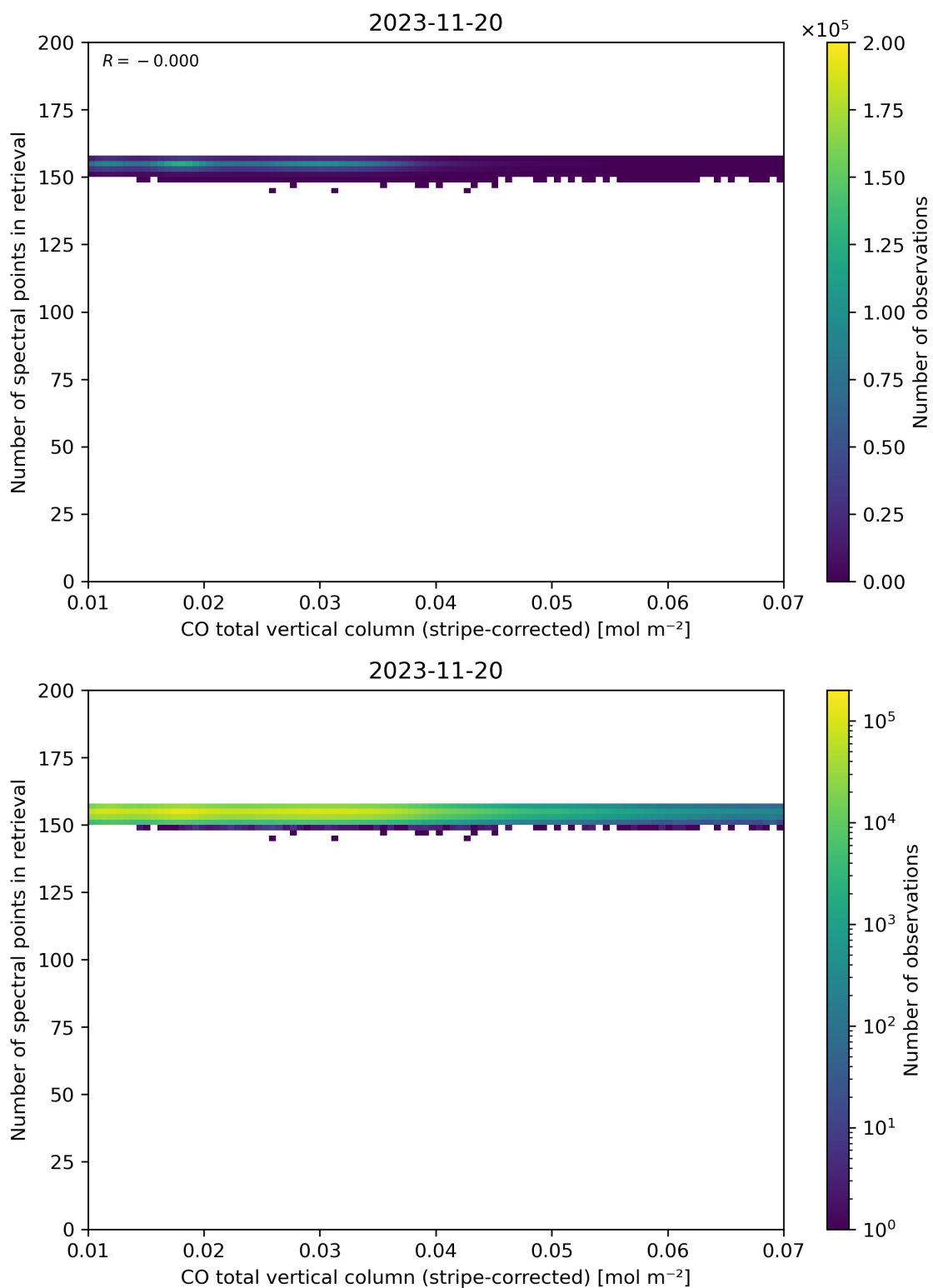
Figure 40: Scatter density plot of “CO total vertical column (stripe-corrected)” against “Number of spectral points in retrieval” for 2023-11-19 to 2023-11-21.
