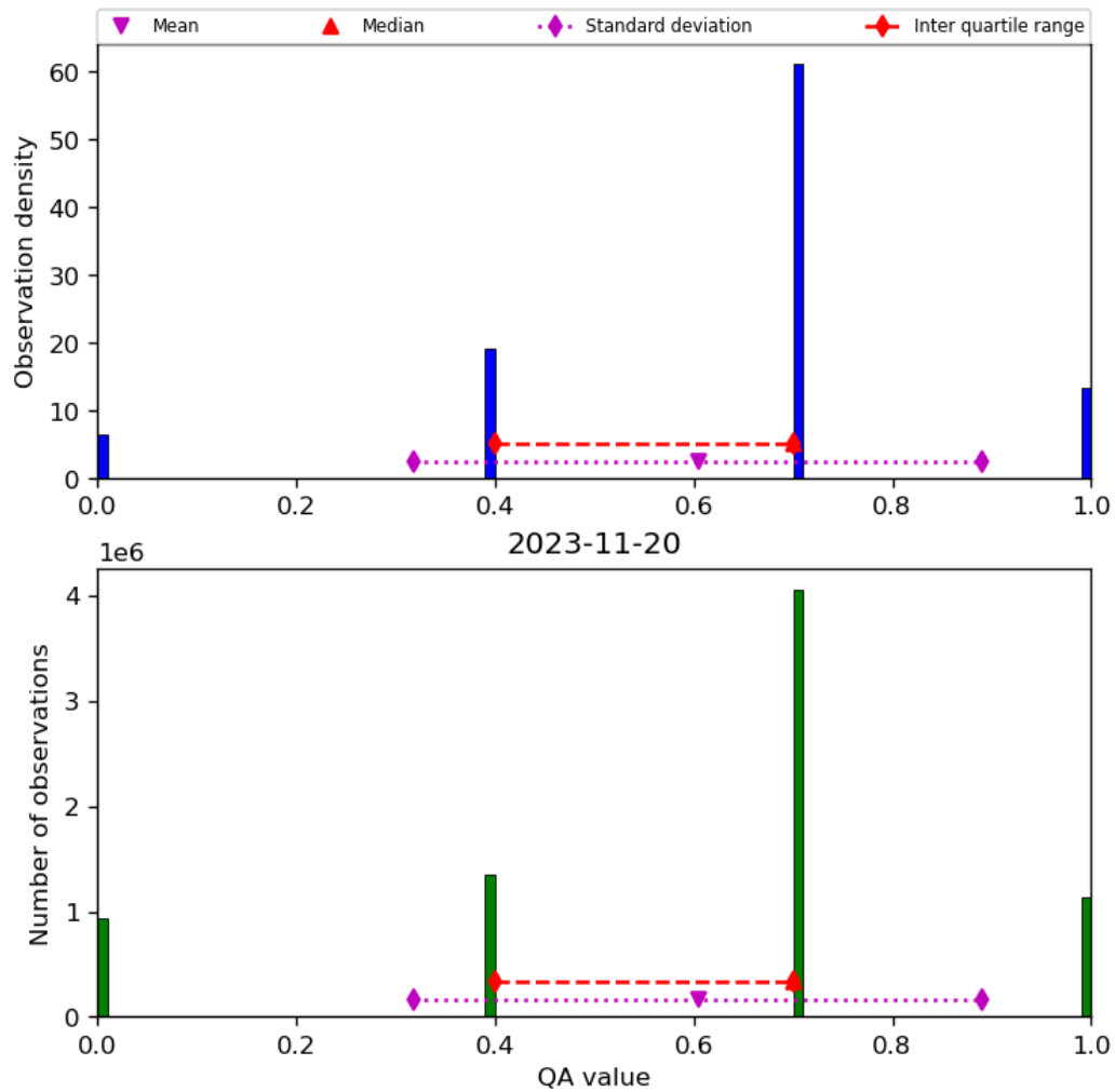
Figure 17: Histogram of “QA value” for 2023-11-19 to 2023-11-21
