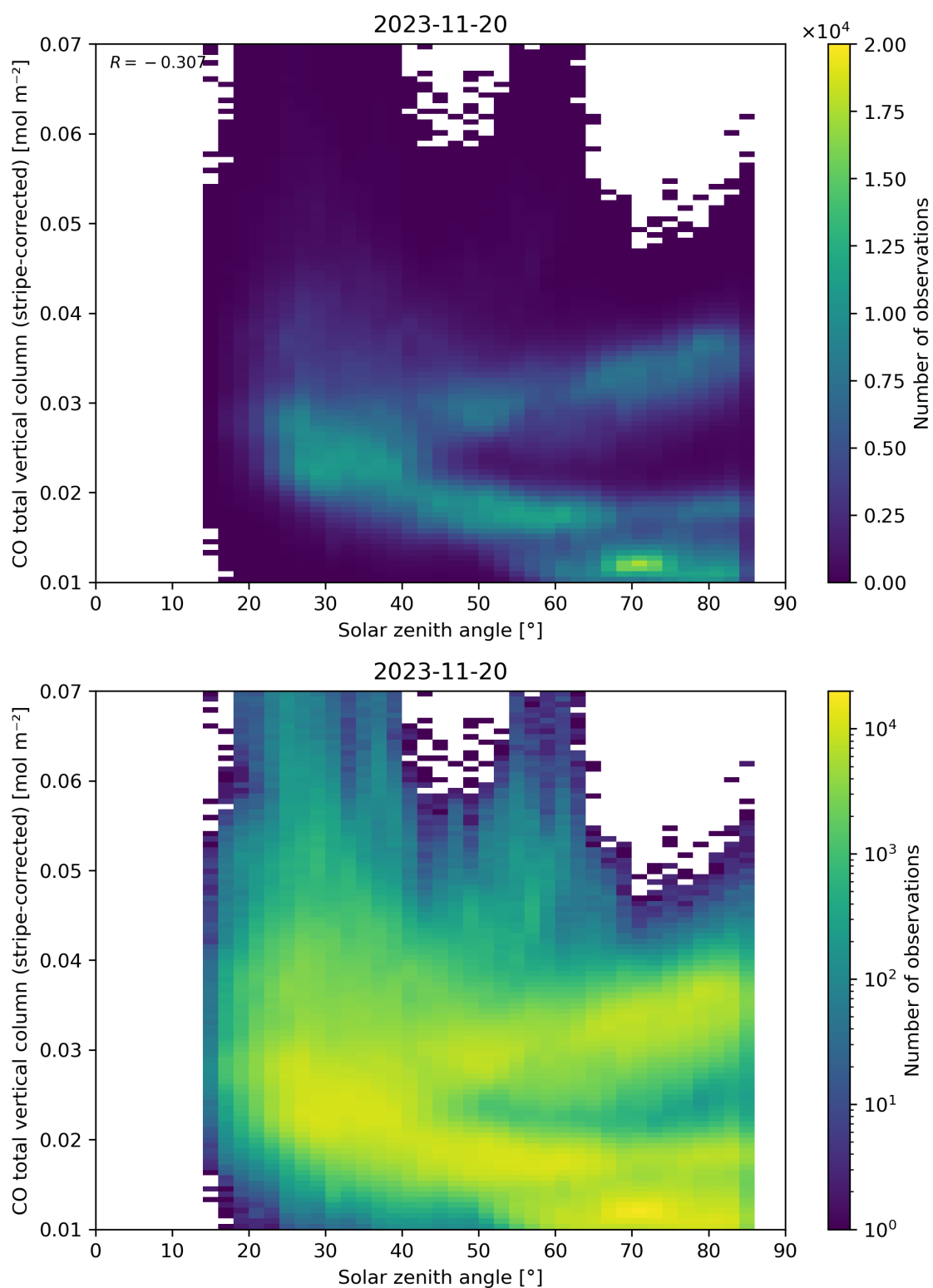
Figure 62: Scatter density plot of “Solar zenith angle” against “CO total vertical column (stripe-corrected)” for 2023-11-19 to 2023-11-21.
