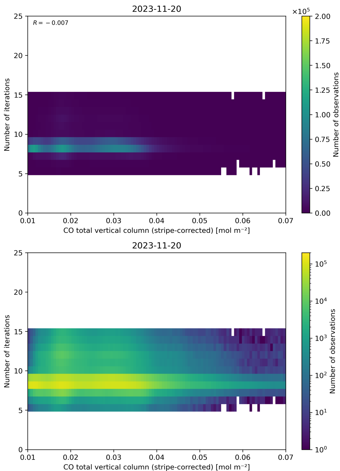
Figure 39: Scatter density plot of “CO total vertical column (stripe-corrected)” against “Number of iterations” for 2023-11-19 to 2023-11-21.
