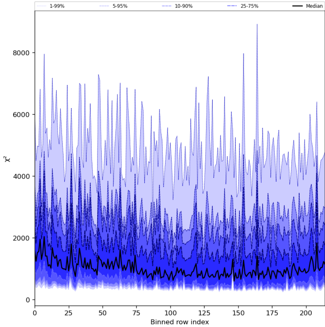
Figure 30: Along track statistics of “ \chi^2 ” for 2023-11-19 to 2023-11-21
