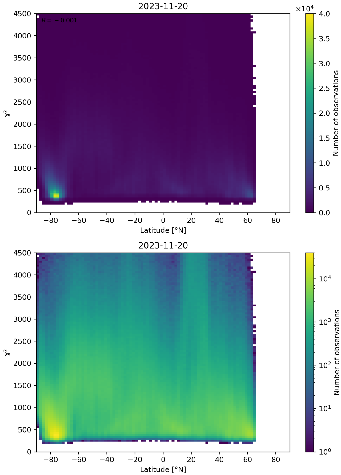
Figure 54: Scatter density plot of “Latitude” against “ \chi^2 ” for 2023-11-19 to 2023-11-21.
