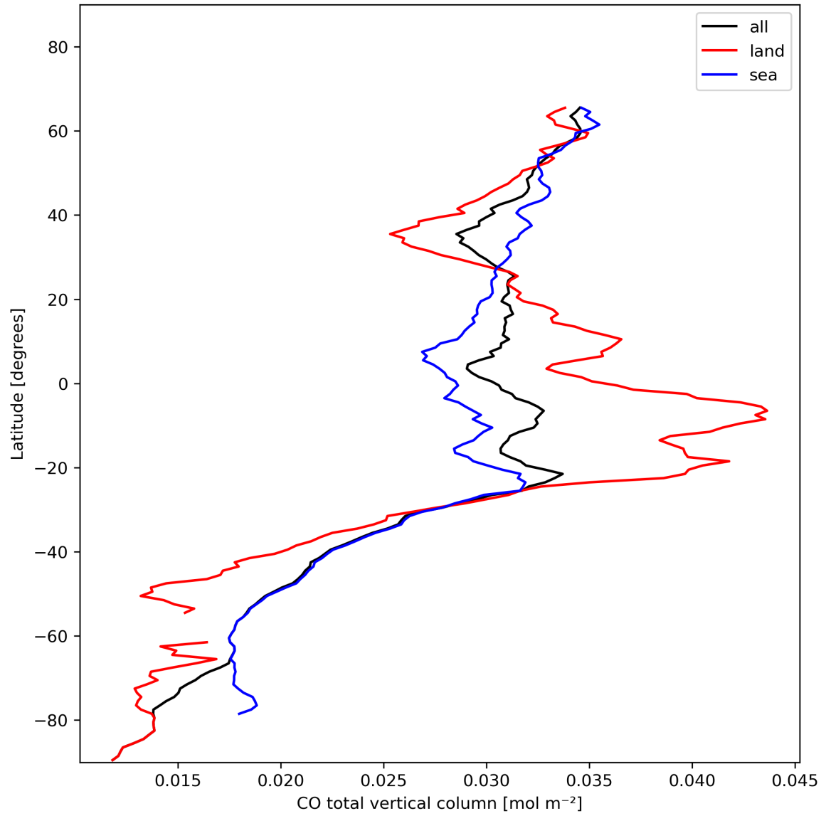
Figure 10: Zonal average of “CO total vertical column” for 2023-11-19 to 2023-11-21.
