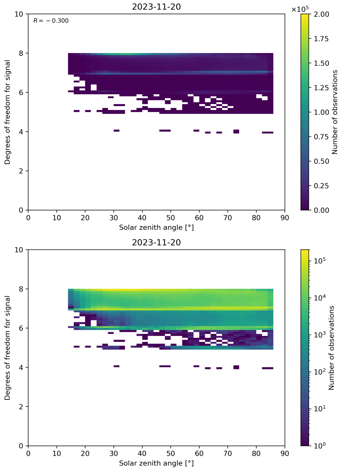
Figure 65: Scatter density plot of “Solar zenith angle” against “Degrees of freedom for signal” for 2023-11-19 to 2023-11-21.
