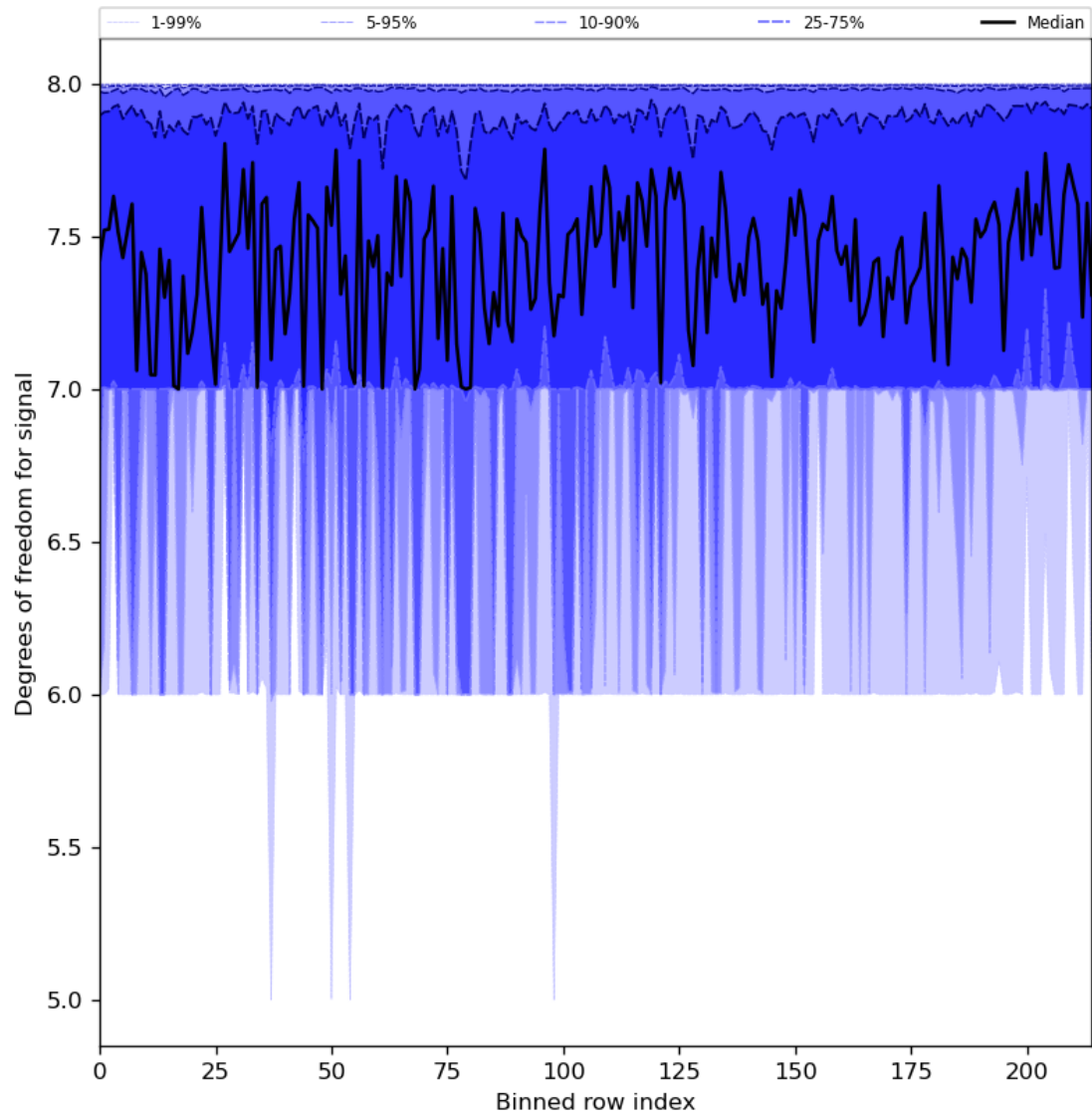
Figure 31: Along track statistics of “Degrees of freedom for signal” for 2023-11-19 to 2023-11-21
