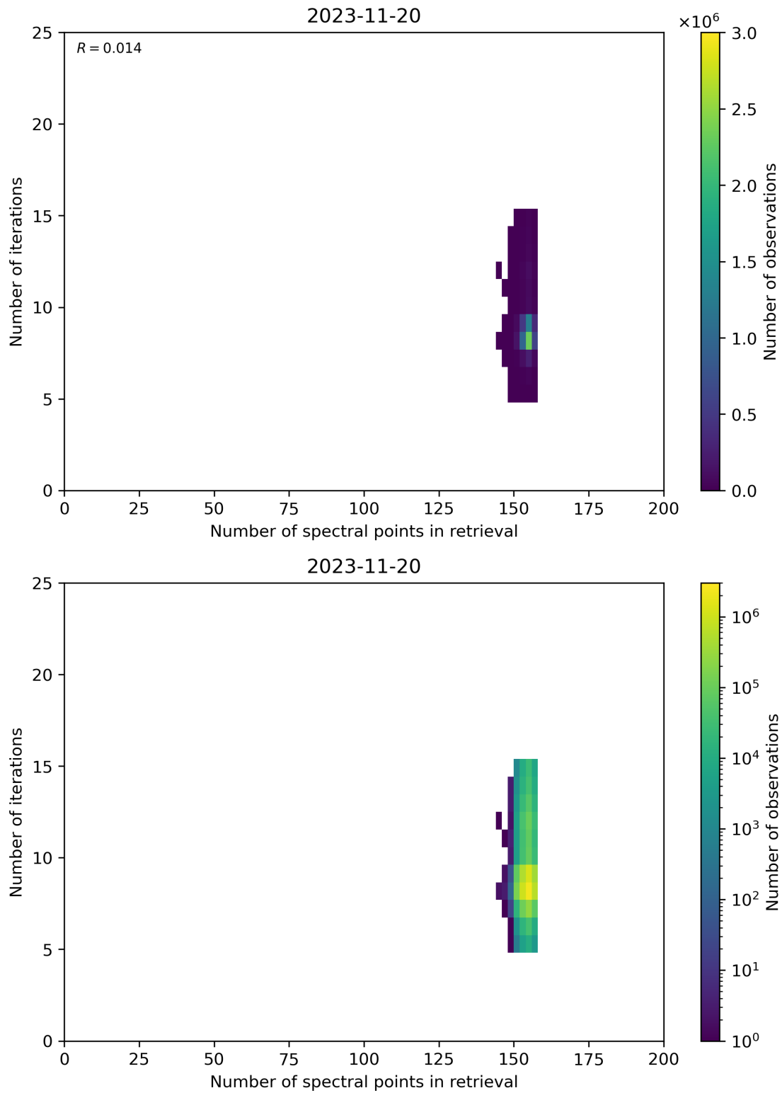
Figure 60: Scatter density plot of “Number of spectral points in retrieval” against “Number of iterations” for 2023-11-19 to 2023-11-21.
