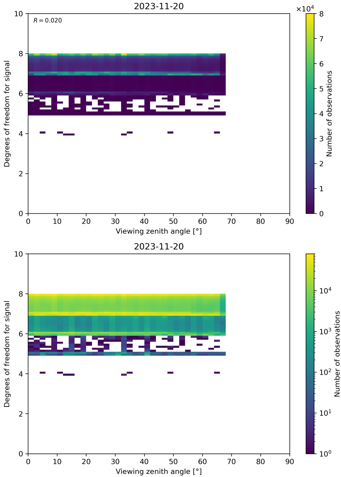
Figure 73: Scatter density plot of “Viewing zenith angle” against “Degrees of freedom for signal” for 2023-11-19 to 2023-11-21.
