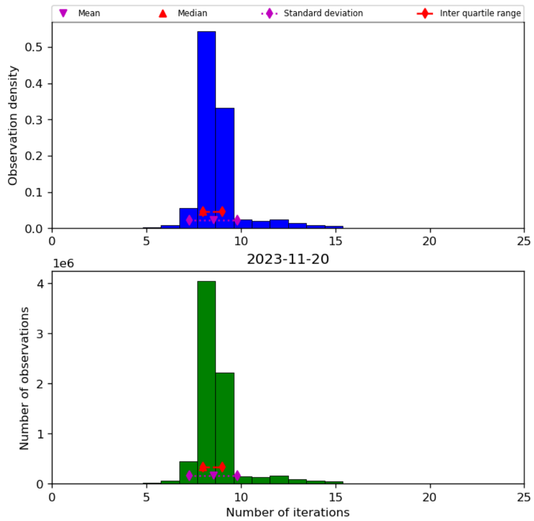
Figure 24: Histogram of “Number of iterations” for 2023-11-19 to 2023-11-21
