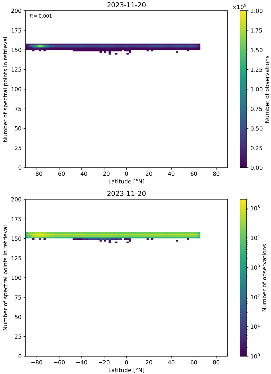
Figure 57: Scatter density plot of “Latitude” against “Number of spectral points in retrieval” for 2023-11-19 to 2023-11-21.
