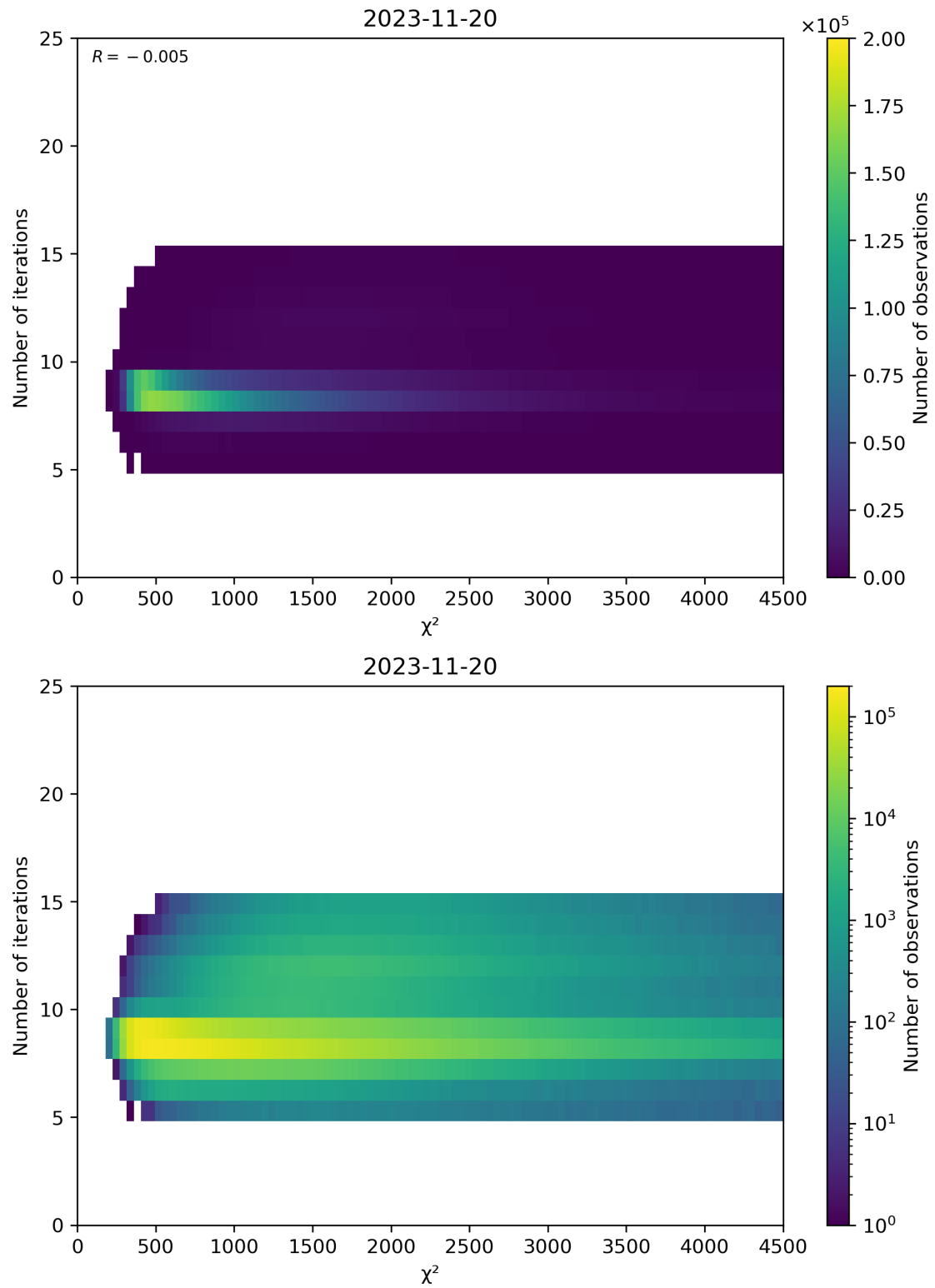
Figure 49: Scatter density plot of “ \chi^2 ” against “Number of iterations” for 2023-11-19 to 2023-11-21.
