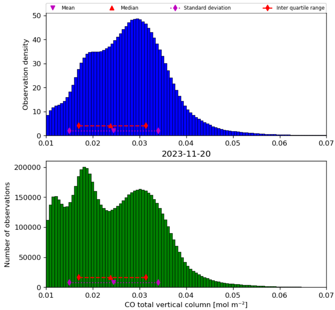
Figure 18: Histogram of “CO total vertical column” for 2023-11-19 to 2023-11-21
