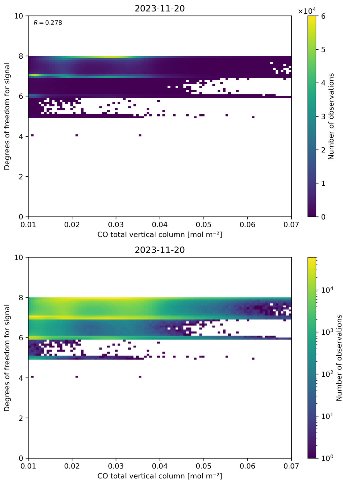
Figure 41: Scatter density plot of “CO total vertical column” against “Degrees of freedom for signal” for 2023-11-19 to 2023-11-21.
