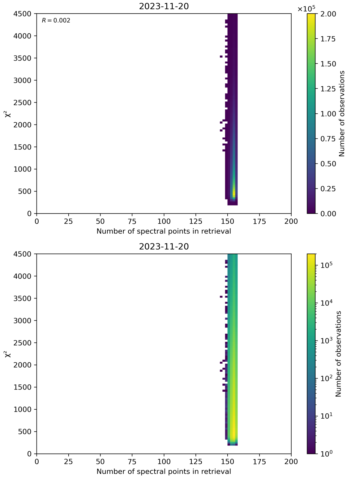
Figure 58: Scatter density plot of “Number of spectral points in retrieval” against “ \chi^2 ” for 2023-11-19 to 2023-11-21.
