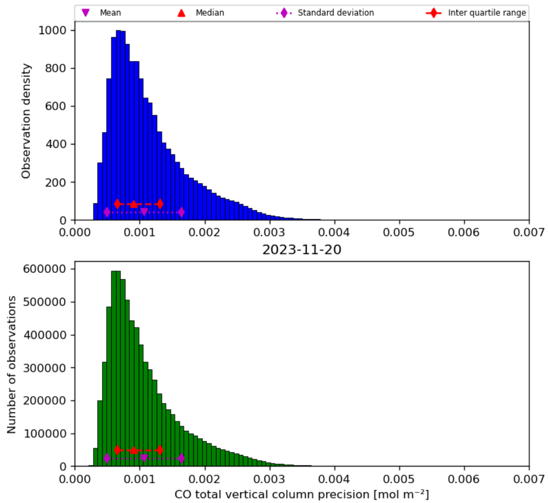
Figure 20: Histogram of “CO total vertical column precision” for 2023-11-19 to 2023-11-21
