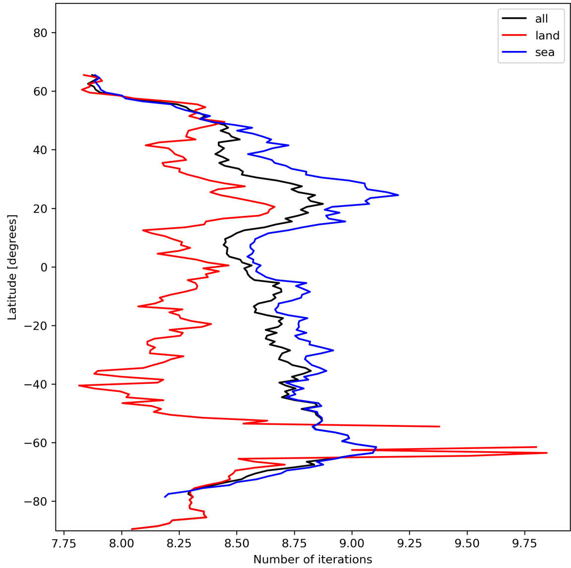
Figure 16: Zonal average of “Number of iterations” for 2023-11-19 to 2023-11-21.
