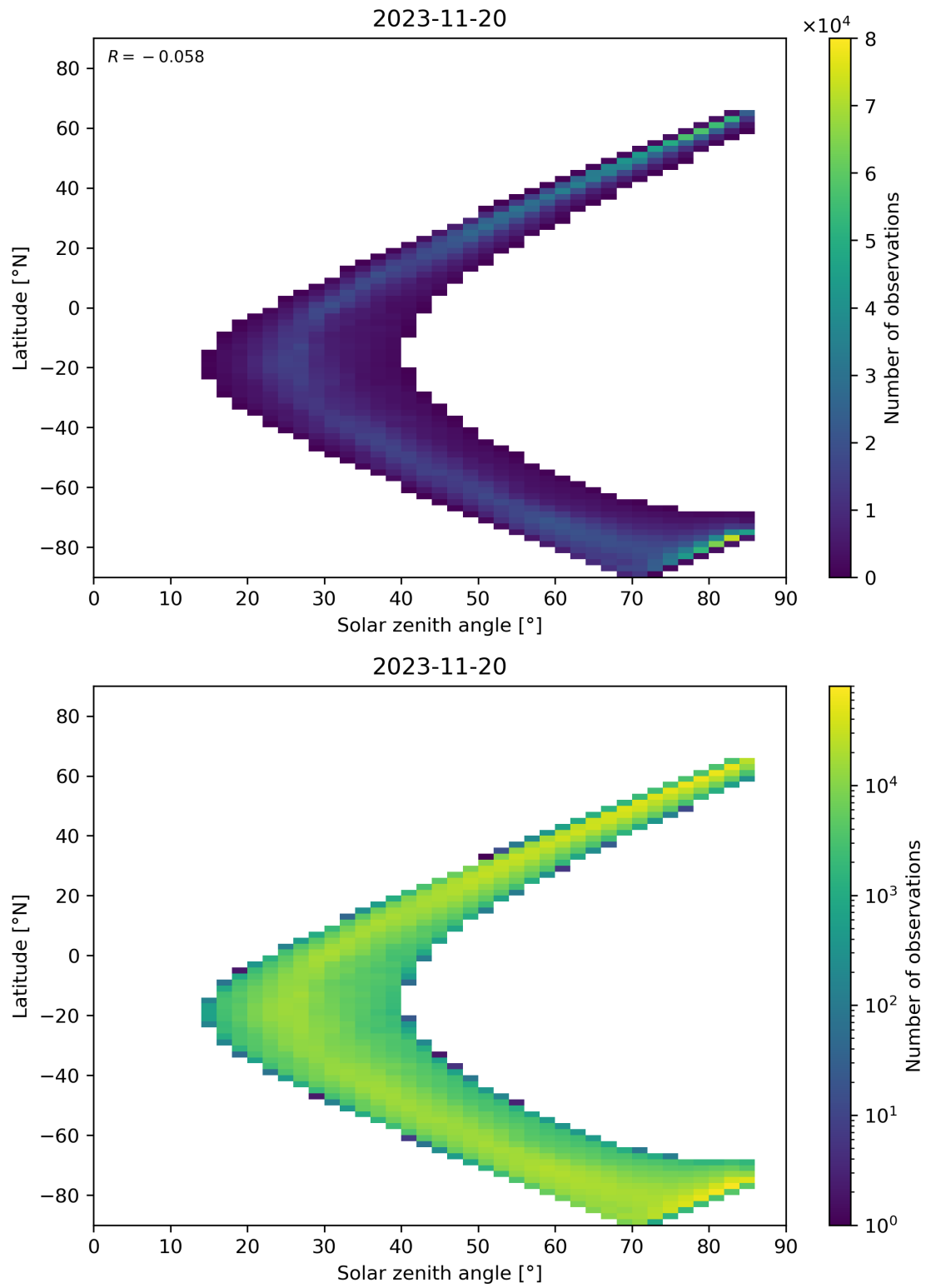
Figure 66: Scatter density plot of “Solar zenith angle” against “Latitude” for 2023-11-19 to 2023-11-21.
