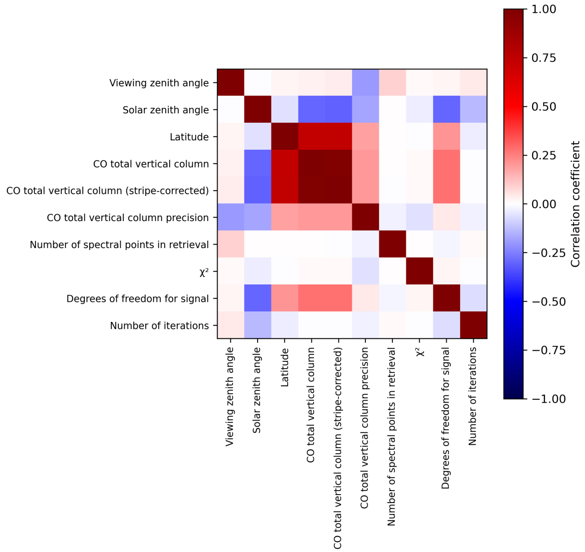
Figure 2: Map of correlation matrix for 2023-11-19 to 2023-11-21.
