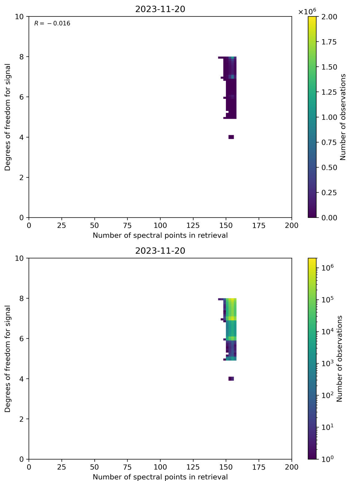
Figure 59: Scatter density plot of “Number of spectral points in retrieval” against “Degrees of freedom for signal” for 2023-11-19 to 2023-11-21.
