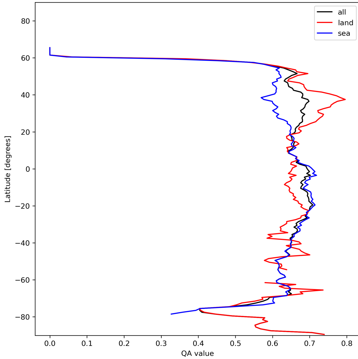
Figure 9: Zonal average of “QA value” for 2023-11-19 to 2023-11-21.
