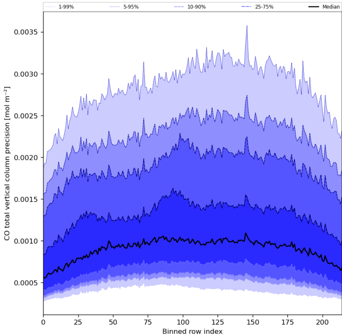
Figure 28: Along track statistics of “CO total vertical column precision” for 2023-11-19 to 2023-11-21
