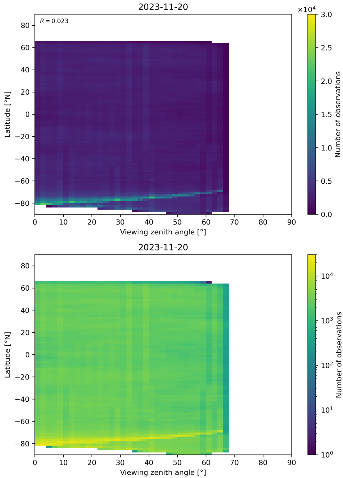
Figure 74: Scatter density plot of “Viewing zenith angle” against “Latitude” for 2023-11-19 to 2023-11-21.
