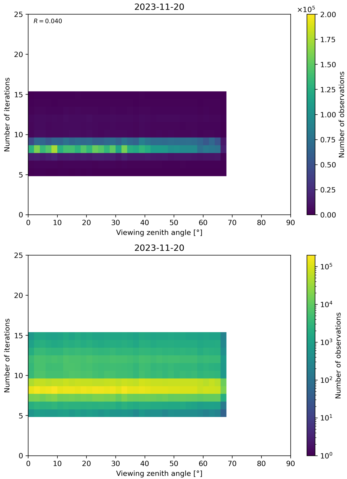
Figure 75: Scatter density plot of “Viewing zenith angle” against “Number of iterations” for 2023-11-19 to 2023-11-21.
