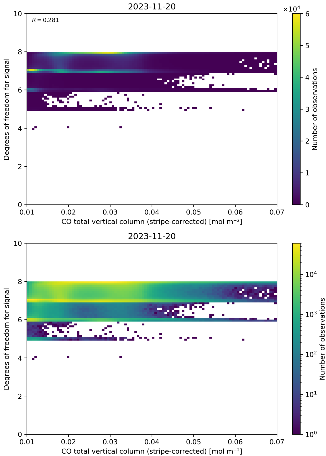
Figure 38: Scatter density plot of “CO total vertical column (stripe-corrected)” against “Degrees of freedom for signal” for 2023-11-19 to 2023-11-21.
