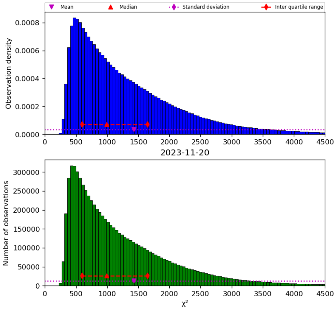
Figure 22: Histogram of “ \chi^2 ” for 2023-11-19 to 2023-11-21
