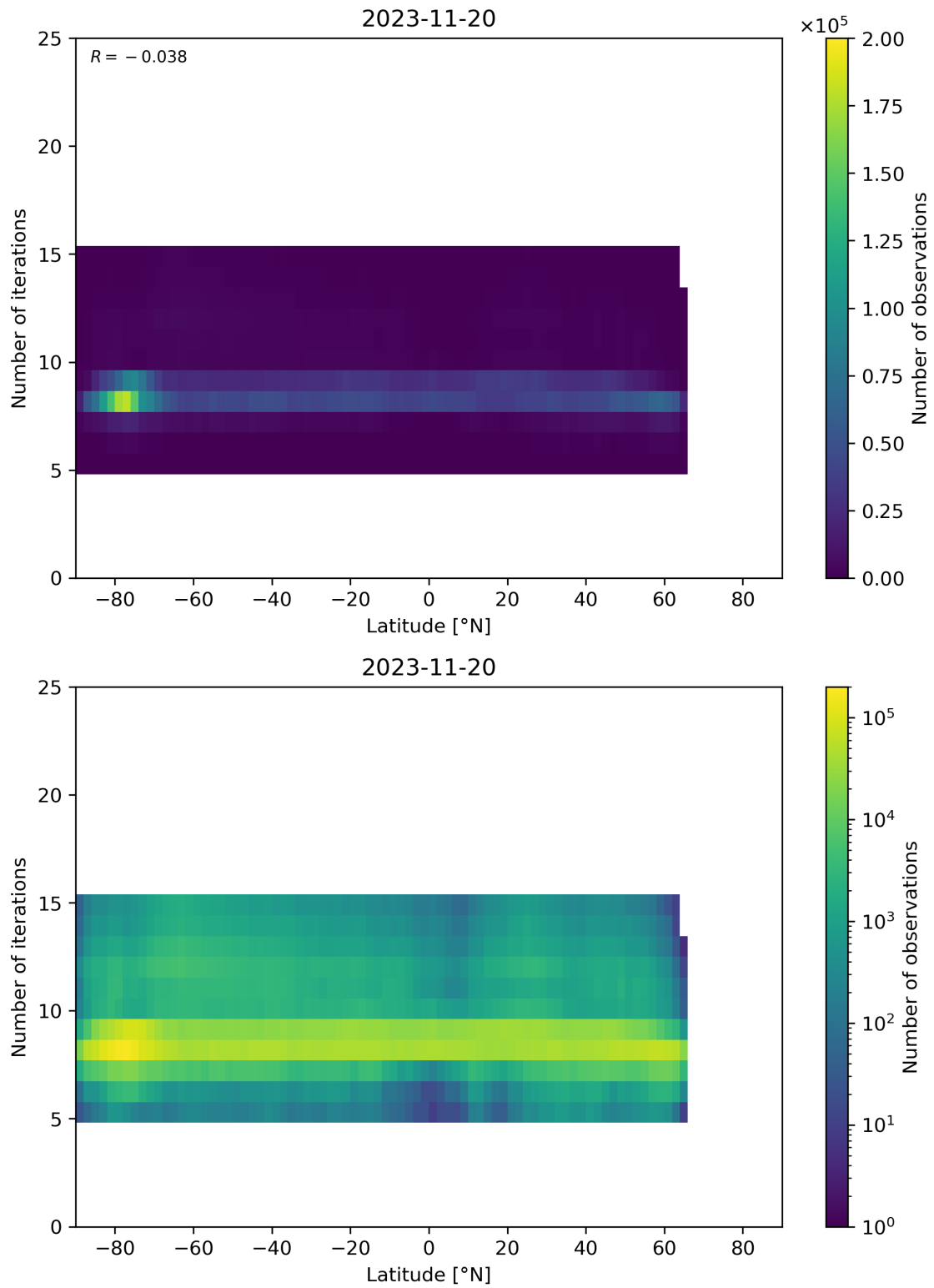
Figure 56: Scatter density plot of “Latitude” against “Number of iterations” for 2023-11-19 to 2023-11-21.
