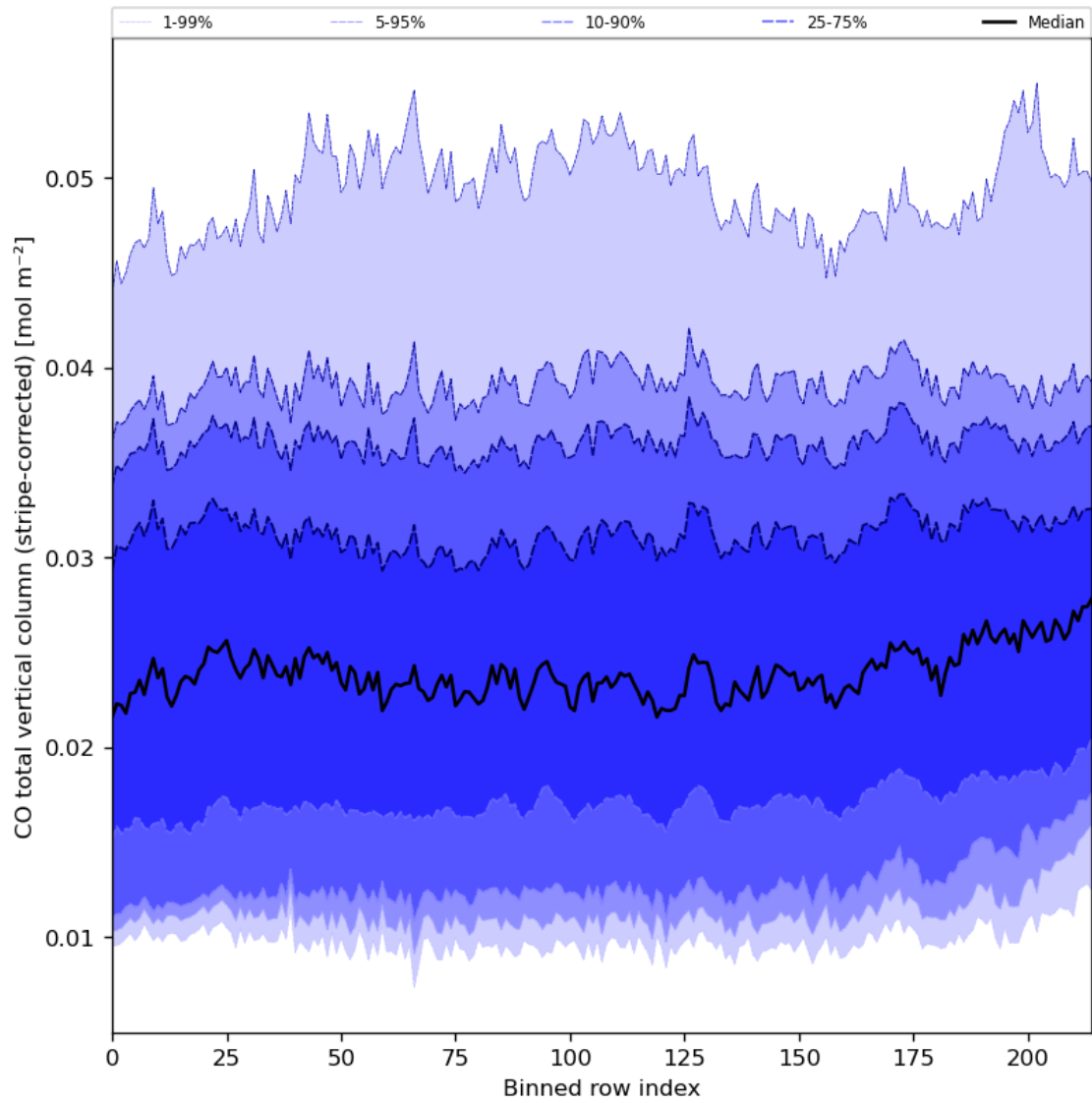
Figure 27: Along track statistics of “CO total vertical column (stripe-corrected)” for 2023-11-19 to 2023-11-21
