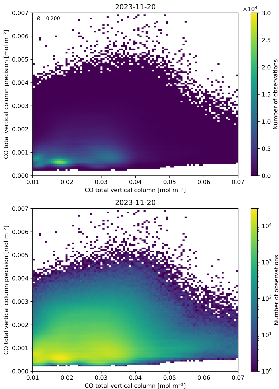
Figure 34: Scatter density plot of “CO total vertical column” against “CO total vertical column precision” for 2023-11-19 to 2023-11-21.
