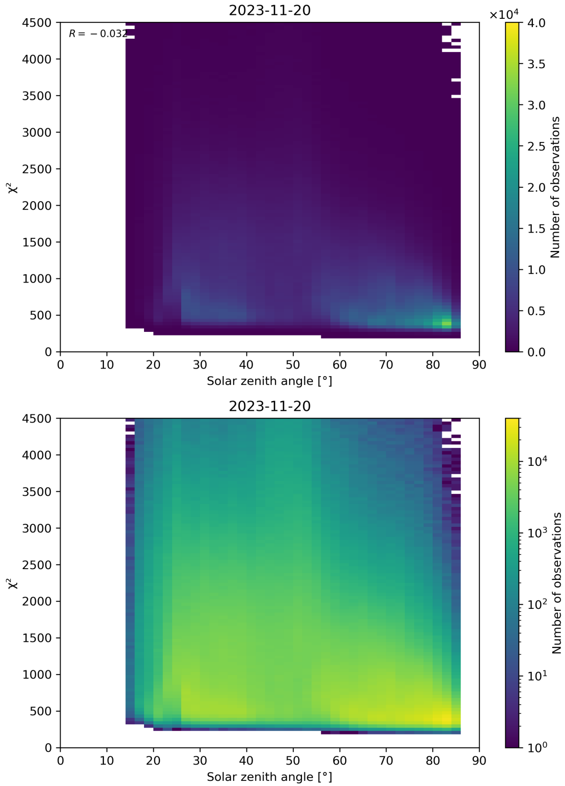
Figure 64: Scatter density plot of “Solar zenith angle” against “ \chi^2 ” for 2023-11-19 to 2023-11-21.
