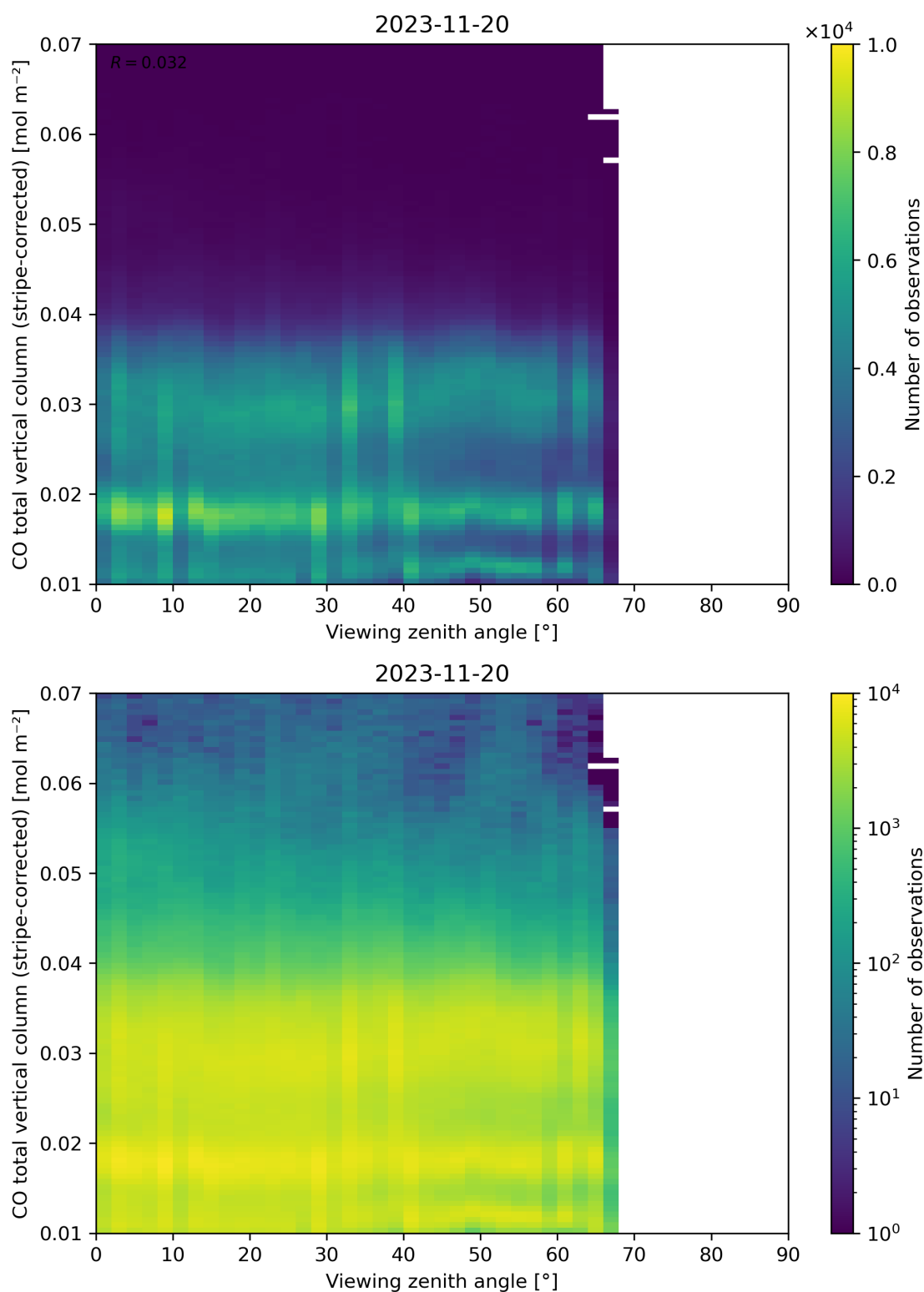
Figure 70: Scatter density plot of “Viewing zenith angle” against “CO total vertical column (stripe-corrected)” for 2023-11-19 to 2023-11-21.
