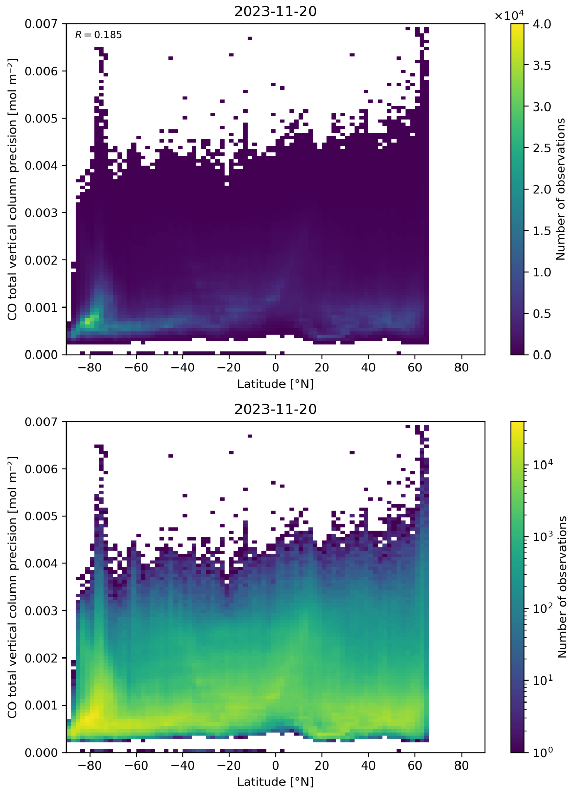
Figure 53: Scatter density plot of “Latitude” against “CO total vertical column precision” for 2023-11-19 to 2023-11-21.
