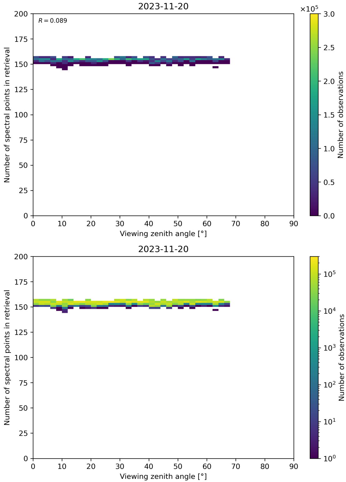
Figure 76: Scatter density plot of “Viewing zenith angle” against “Number of spectral points in retrieval” for 2023-11-19 to 2023-11-21.
