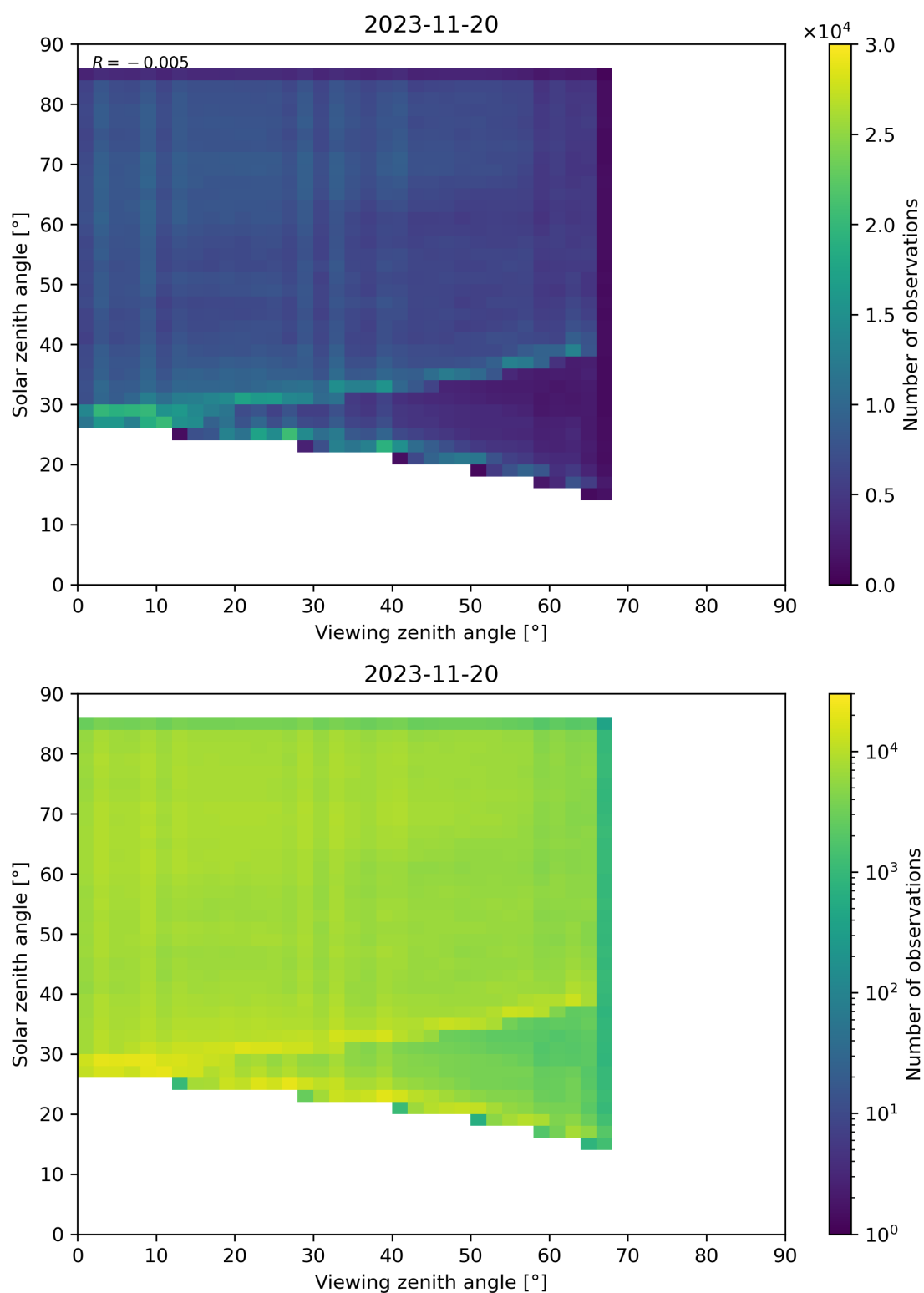
Figure 77: Scatter density plot of “Viewing zenith angle” against “Solar zenith angle” for 2023-11-19 to 2023-11-21.
