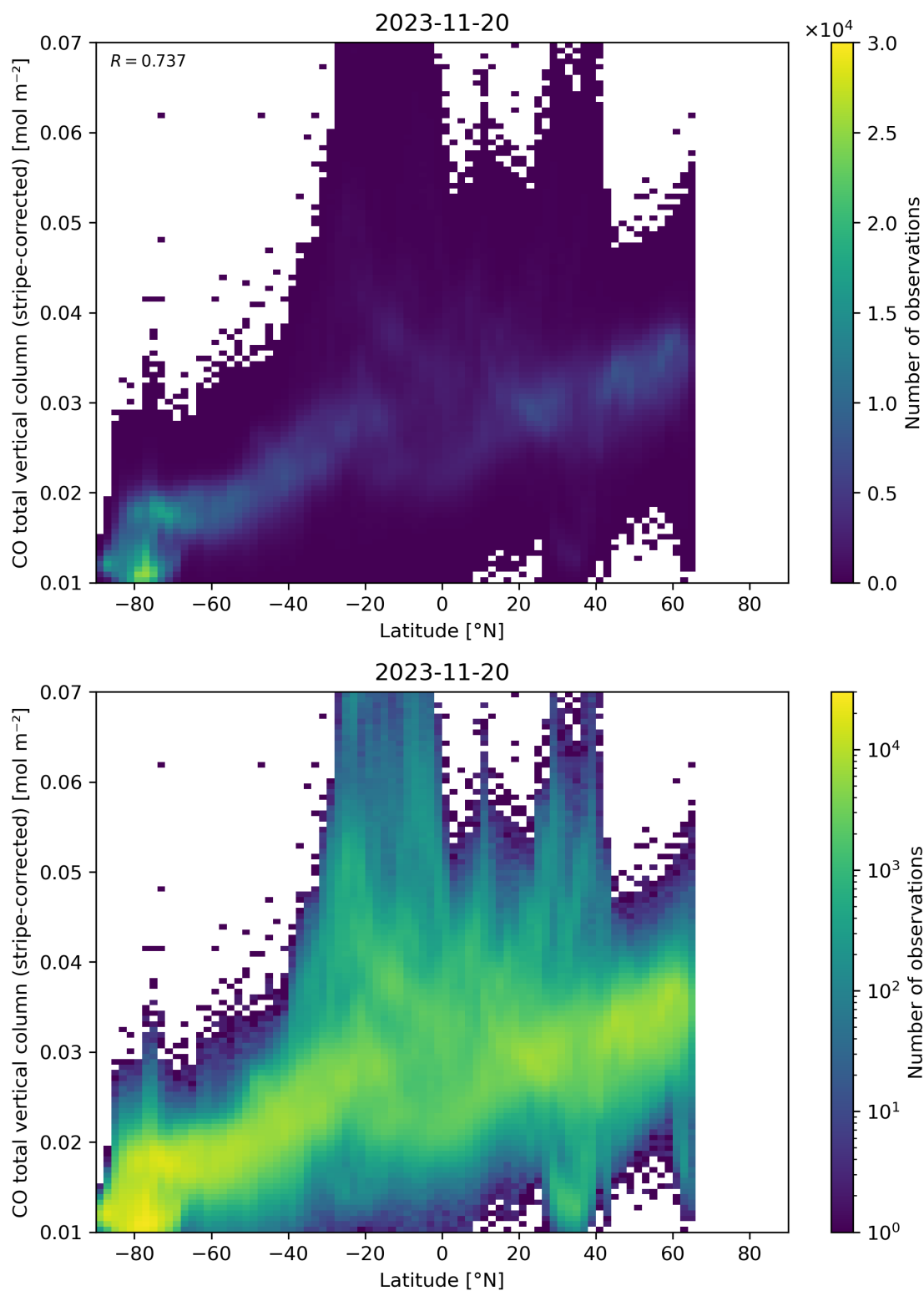
Figure 52: Scatter density plot of “Latitude” against “CO total vertical column (stripe-corrected)” for 2023-11-19 to 2023-11-21.
