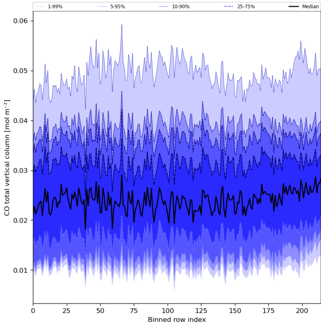
Figure 26: Along track statistics of “CO total vertical column” for 2023-11-19 to 2023-11-21
