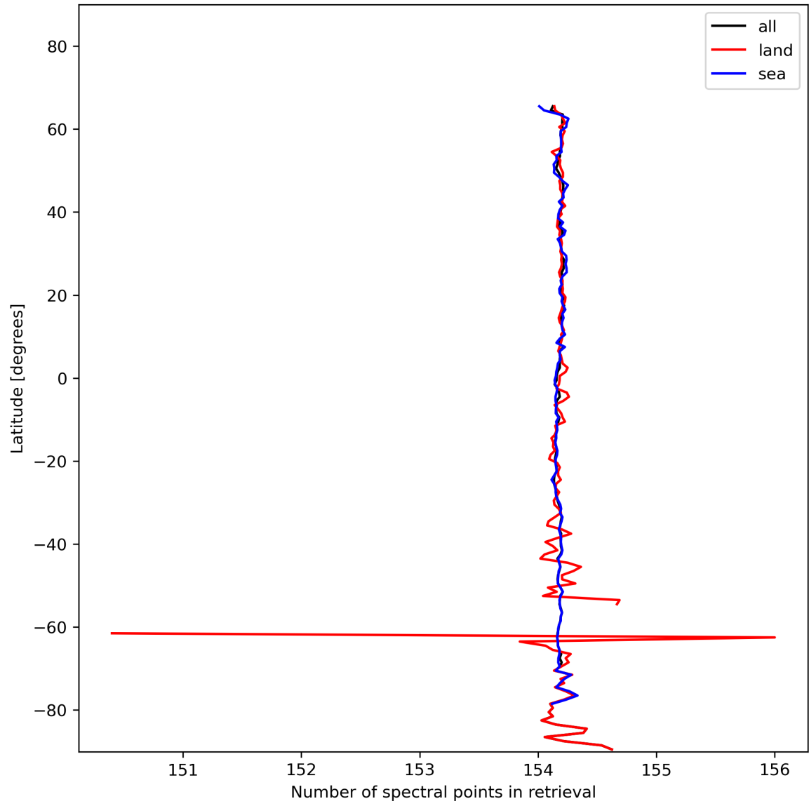
Figure 13: Zonal average of “Number of spectral points in retrieval” for 2023-11-19 to 2023-11-21.
