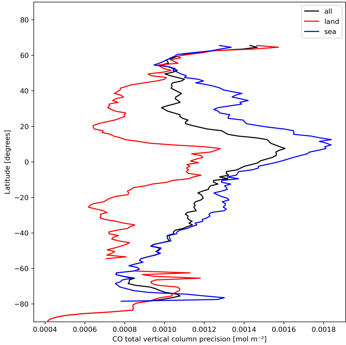
Figure 12: Zonal average of “CO total vertical column precision” for 2023-11-19 to 2023-11-21.
