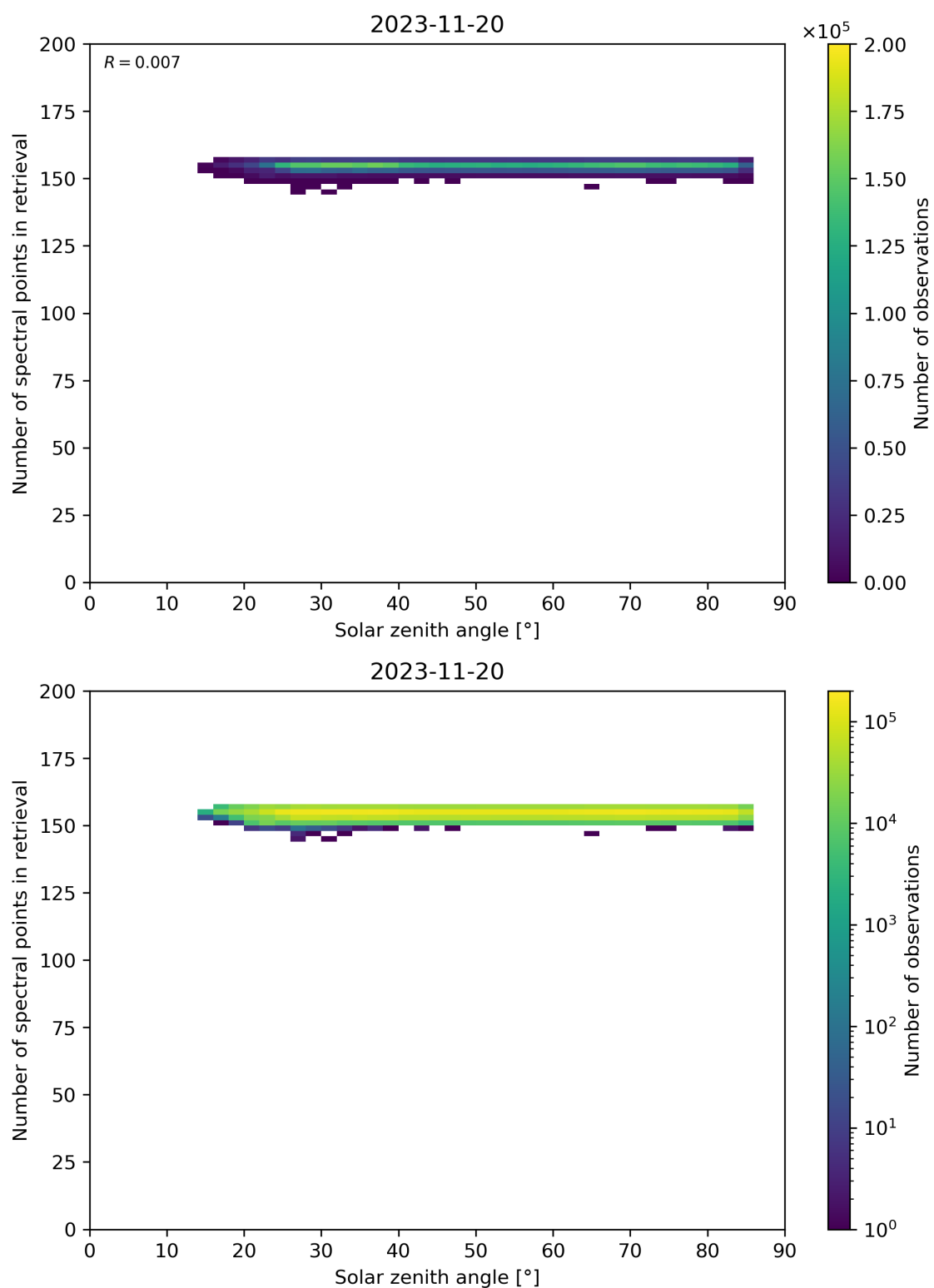
Figure 68: Scatter density plot of “Solar zenith angle” against “Number of spectral points in retrieval” for 2023-11-19 to 2023-11-21.
