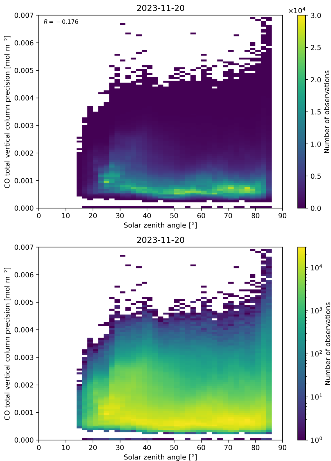
Figure 63: Scatter density plot of “Solar zenith angle” against “CO total vertical column precision” for 2023-11-19 to 2023-11-21.
