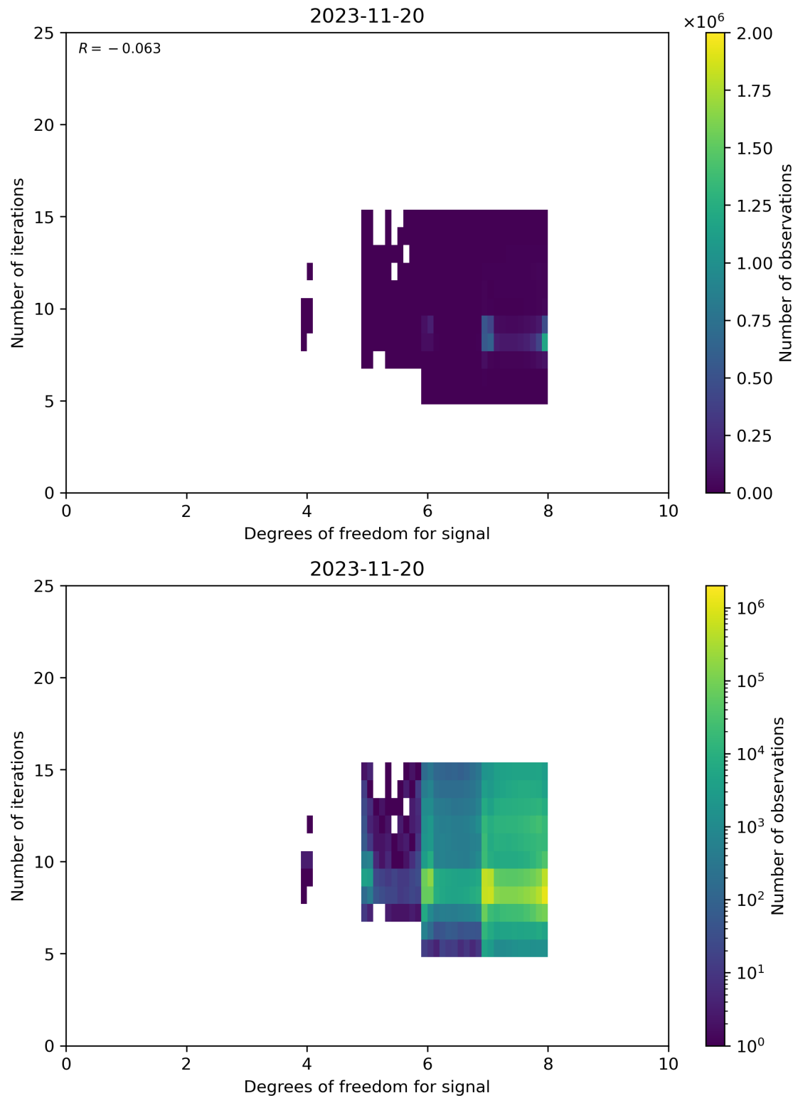
Figure 50: Scatter density plot of “Degrees of freedom for signal” against “Number of iterations” for 2023-11-19 to 2023-11-21.
