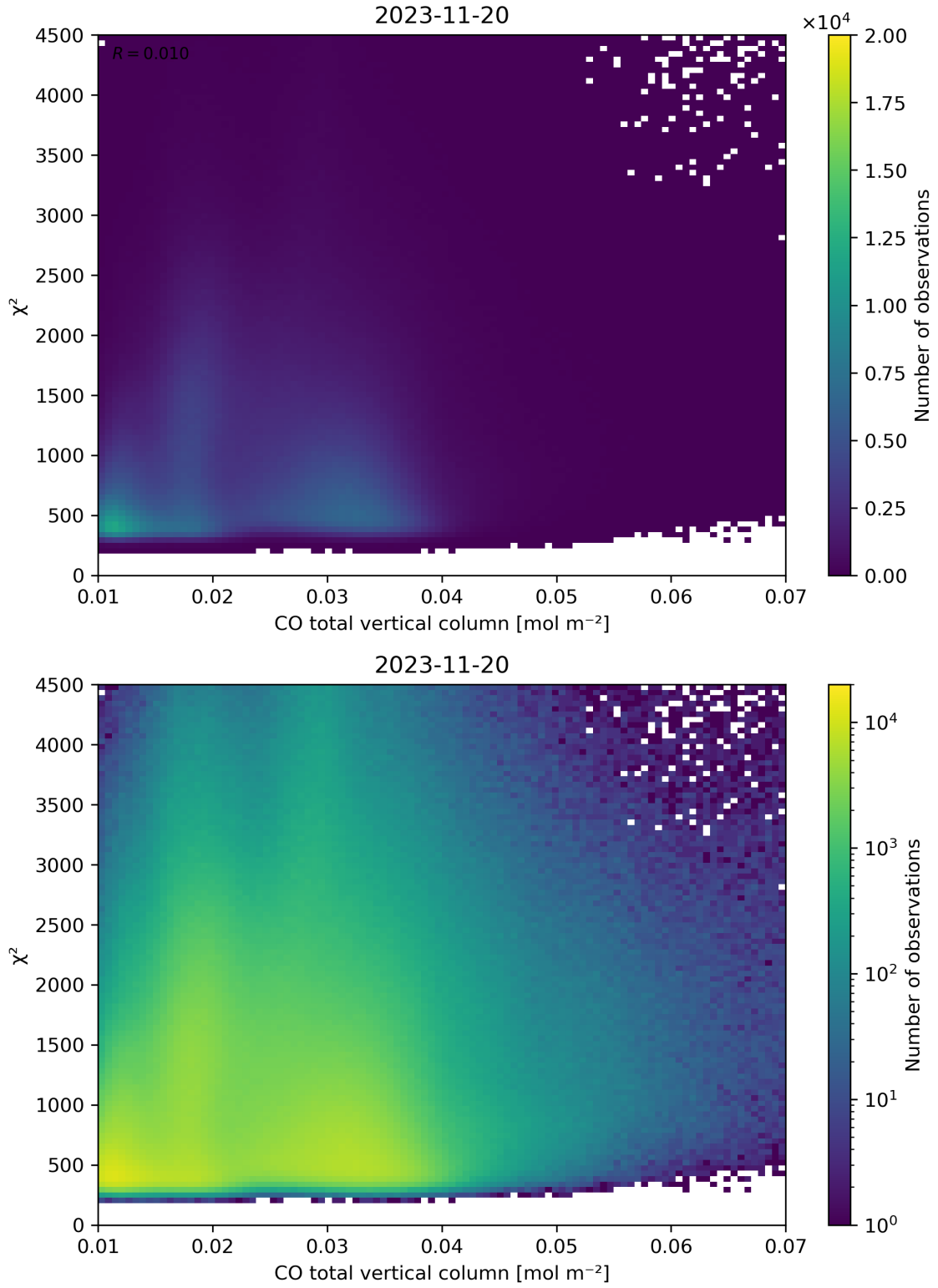
Figure 35: Scatter density plot of “CO total vertical column” against “ \chi^2 ” for 2023-11-19 to 2023-11-21.
