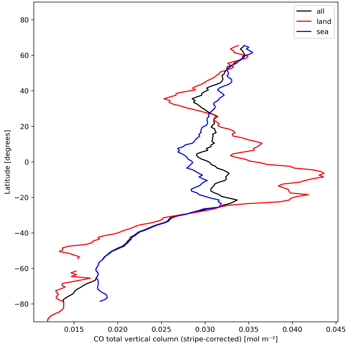
Figure 11: Zonal average of “CO total vertical column (stripe-corrected)” for 2023-11-19 to 2023-11-21.
