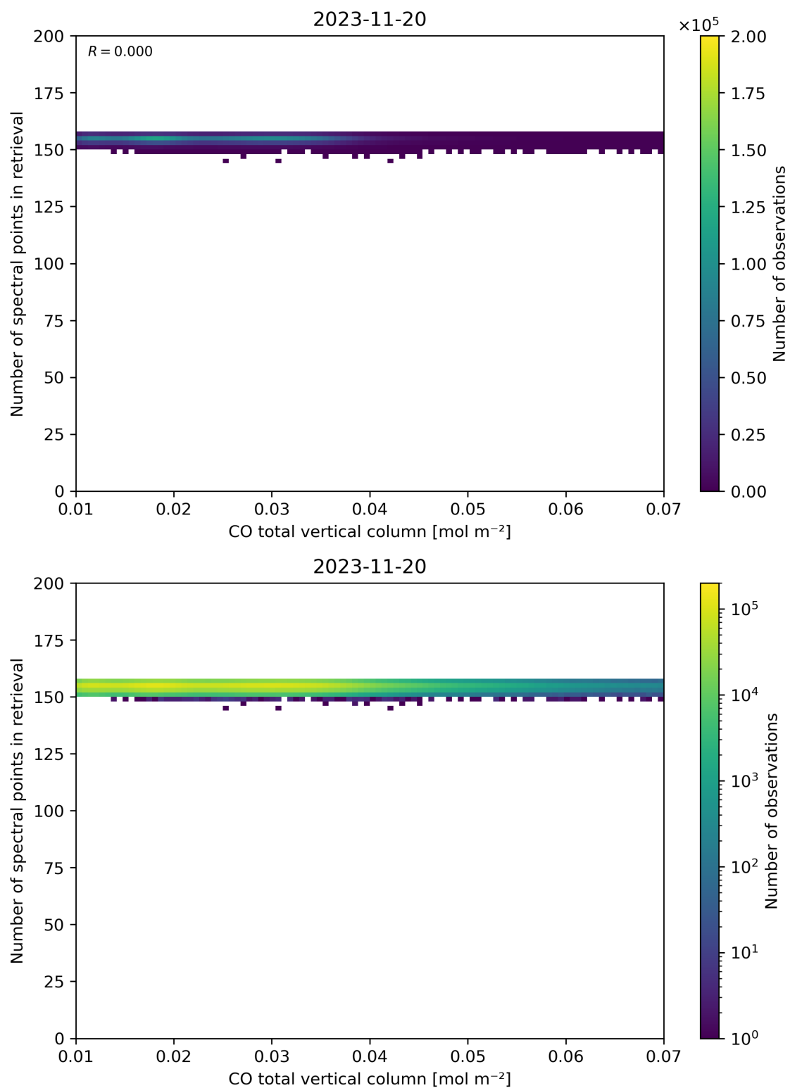
Figure 43: Scatter density plot of “CO total vertical column” against “Number of spectral points in retrieval” for 2023-11-19 to 2023-11-21.
