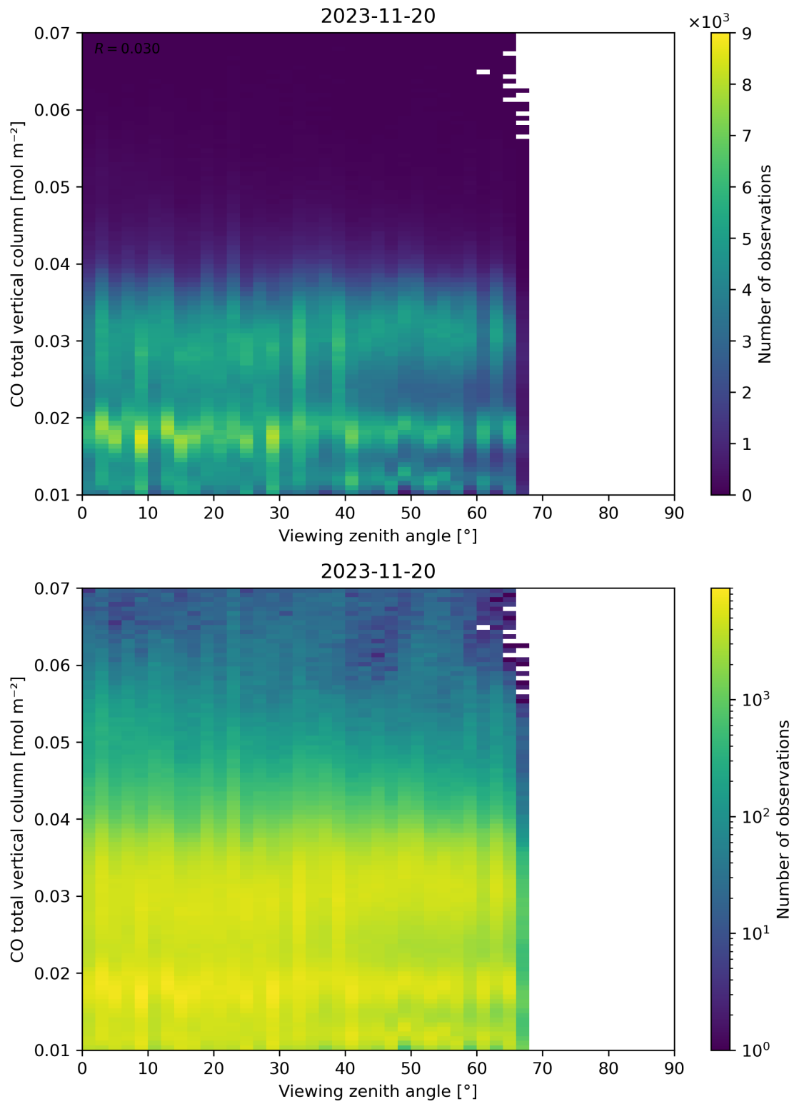
Figure 69: Scatter density plot of “Viewing zenith angle” against “CO total vertical column” for 2023-11-19 to 2023-11-21.
