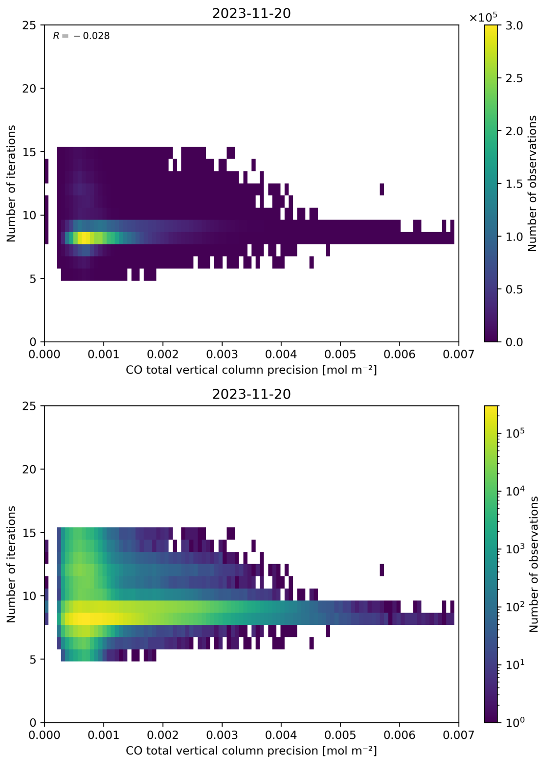
Figure 46: Scatter density plot of “CO total vertical column precision” against “Number of iterations” for 2023-11-19 to 2023-11-21.
