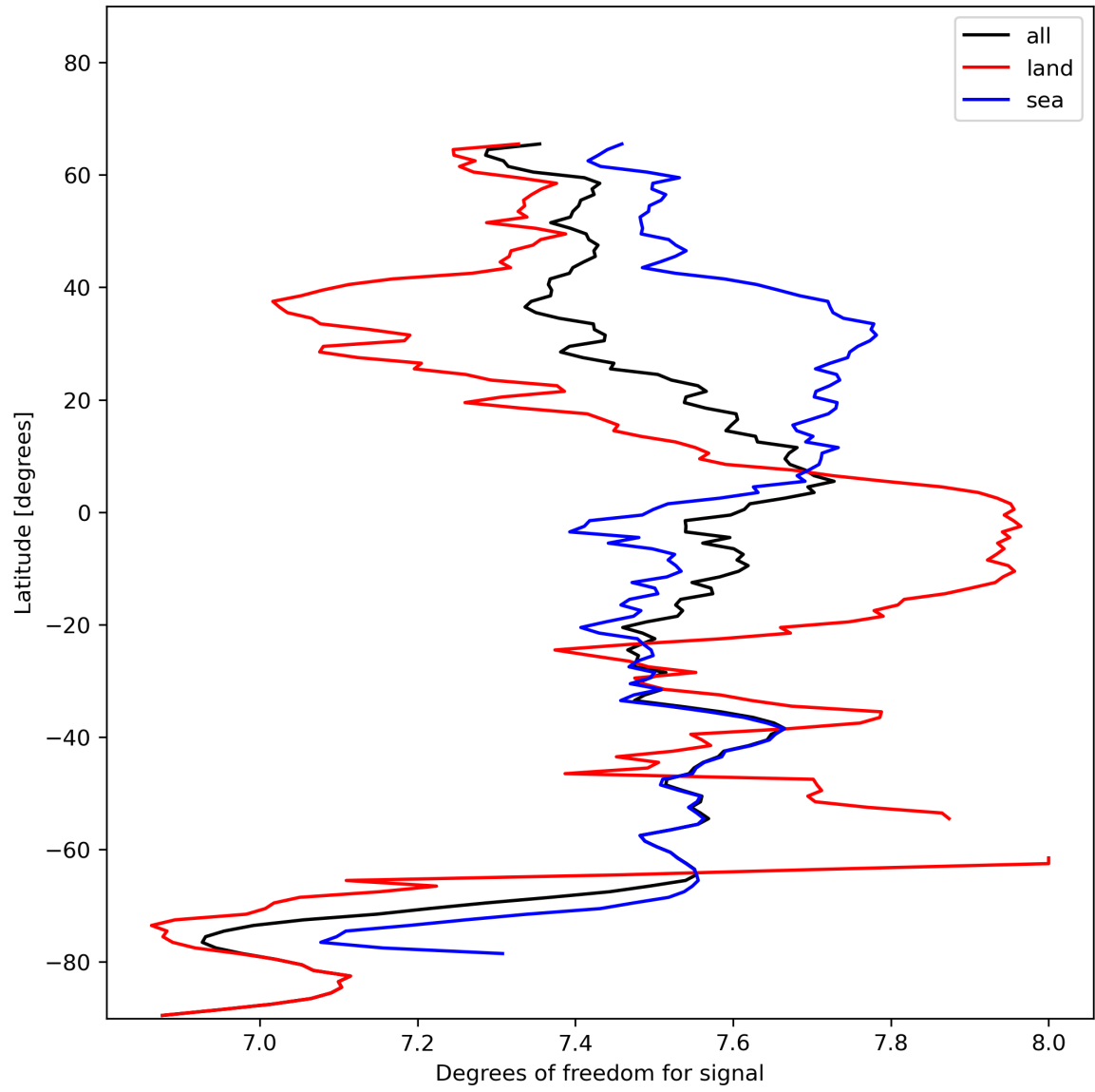
Figure 15: Zonal average of “Degrees of freedom for signal” for 2023-11-19 to 2023-11-21.
