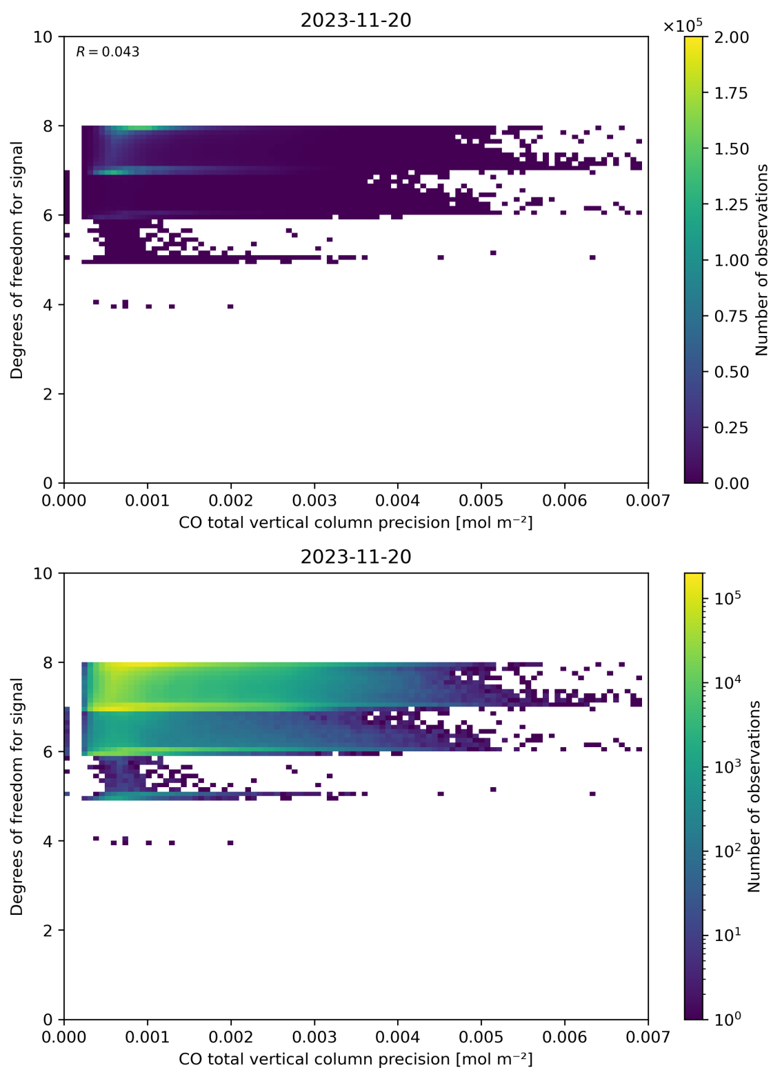
Figure 45: Scatter density plot of “CO total vertical column precision” against “Degrees of freedom for signal” for 2023-11-19 to 2023-11-21.
