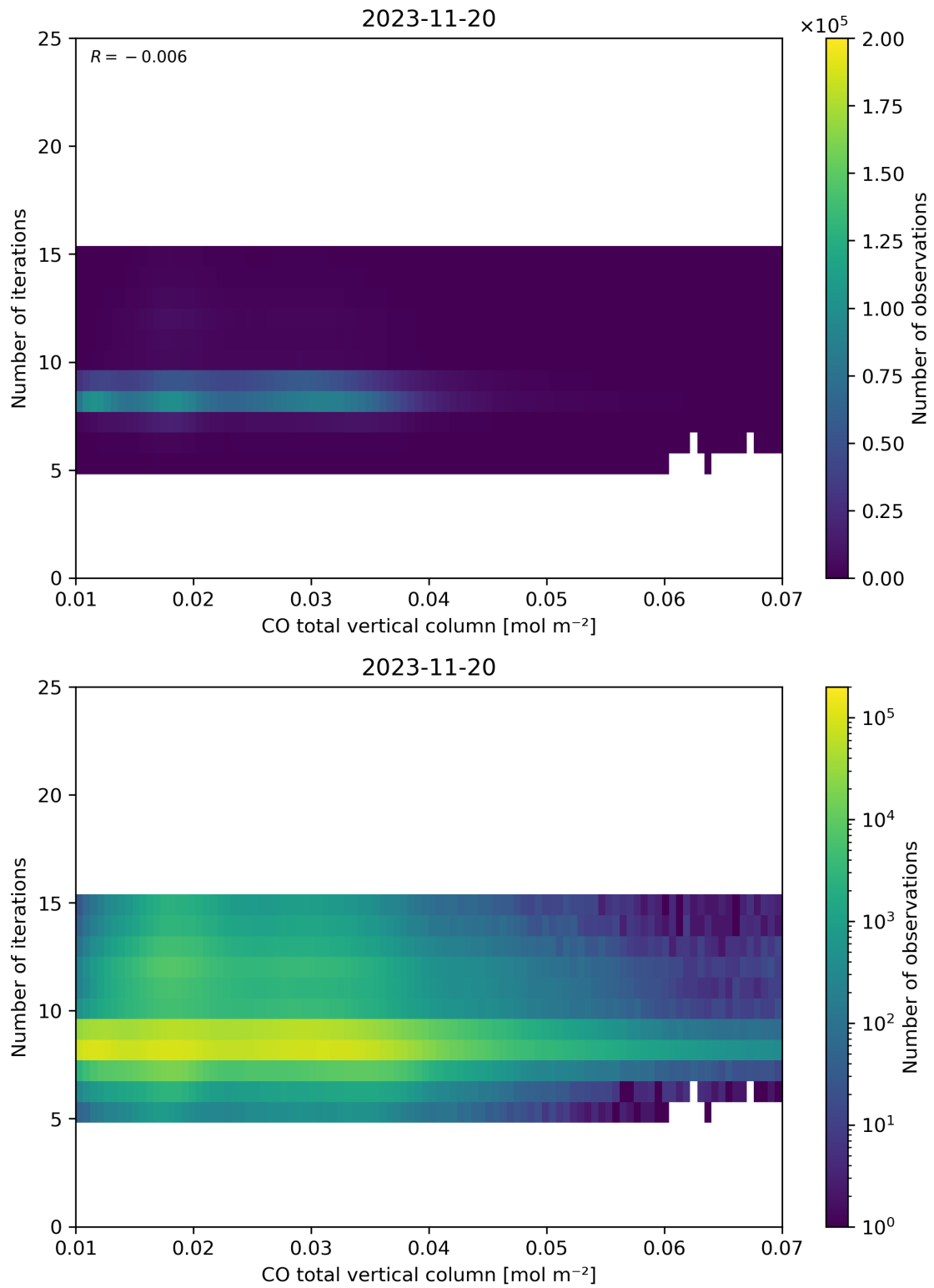
Figure 42: Scatter density plot of “CO total vertical column” against “Number of iterations” for 2023-11-19 to 2023-11-21.
