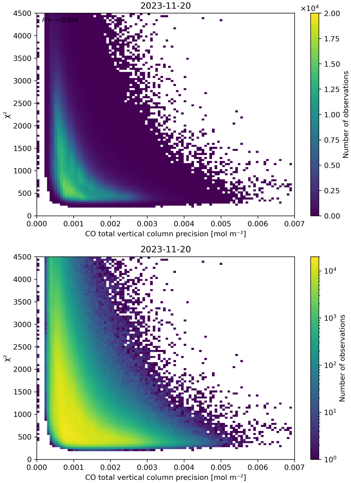
Figure 44: Scatter density plot of “CO total vertical column precision” against “ \chi^2 ” for 2023-11-19 to 2023-11-21.
