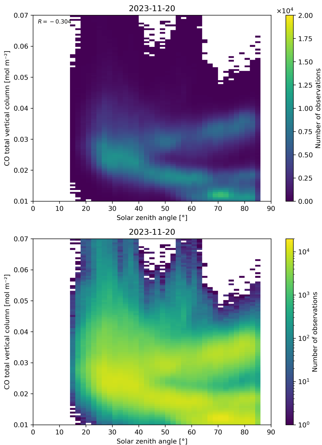
Figure 61: Scatter density plot of “Solar zenith angle” against “CO total vertical column” for 2023-11-19 to 2023-11-21.
