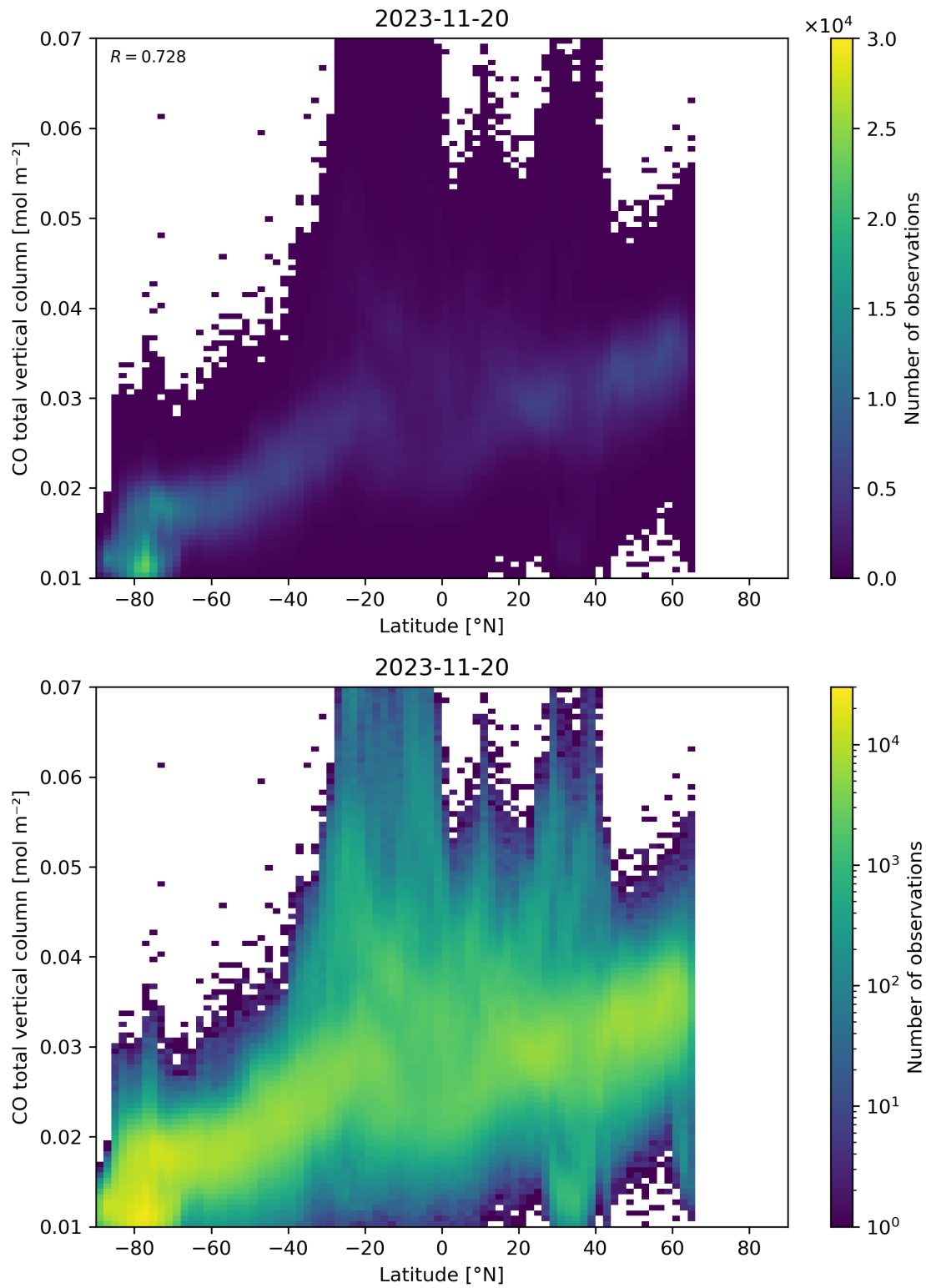
Figure 51: Scatter density plot of “Latitude” against “CO total vertical column” for 2023-11-19 to 2023-11-21.
