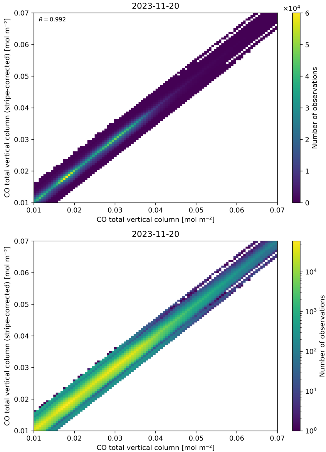
Figure 33: Scatter density plot of “CO total vertical column” against “CO total vertical column (stripe-corrected)” for 2023-11-19 to 2023-11-21.
