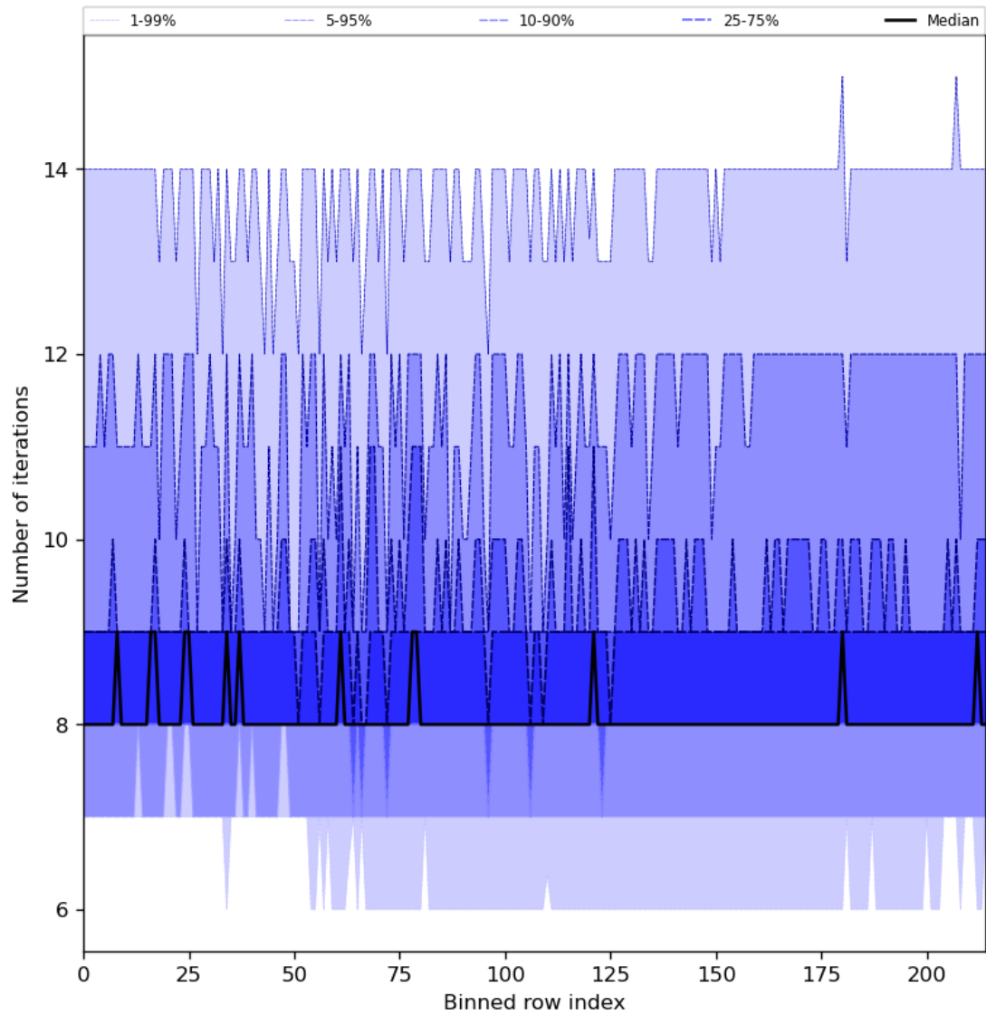
Figure 32: Along track statistics of “Number of iterations” for 2023-11-19 to 2023-11-21
