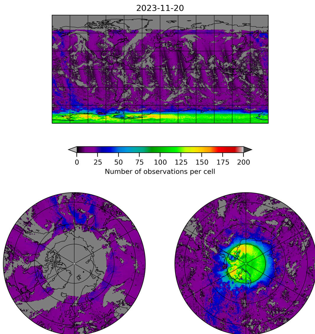
Figure 8: Map of the number of observations for 2023-11-19 to 2023-11-21
