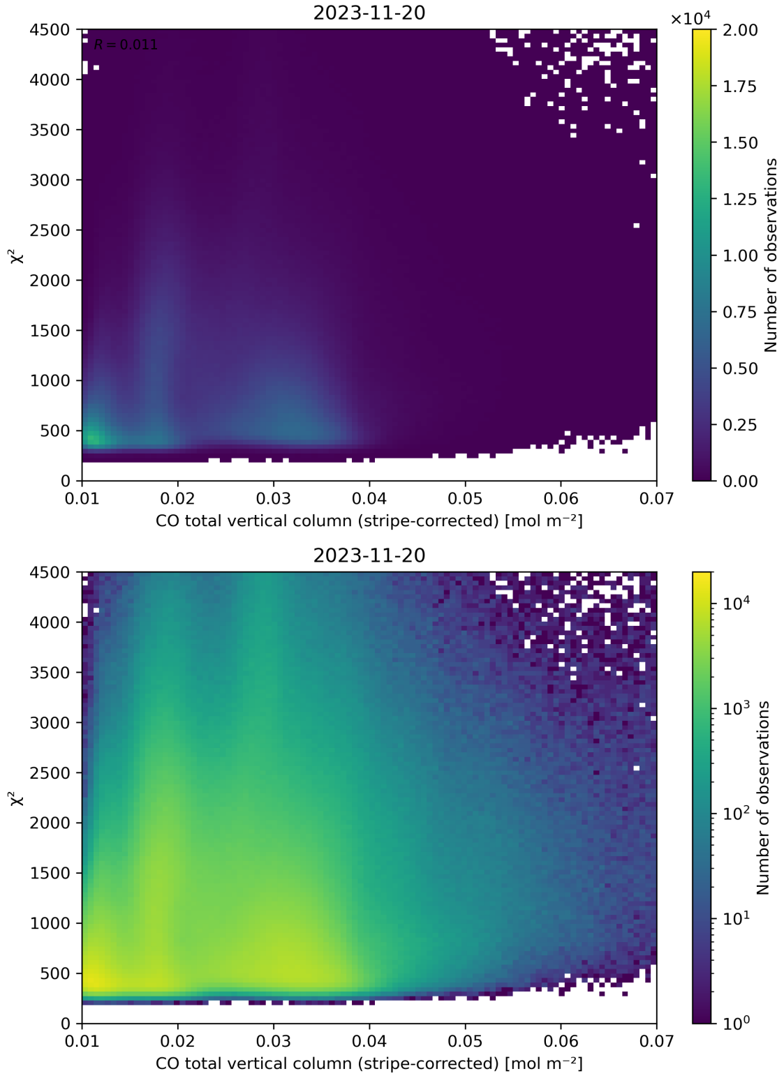
Figure 37: Scatter density plot of “CO total vertical column (stripe-corrected)” against “ \chi^2 ” for 2023-11-19 to 2023-11-21.
