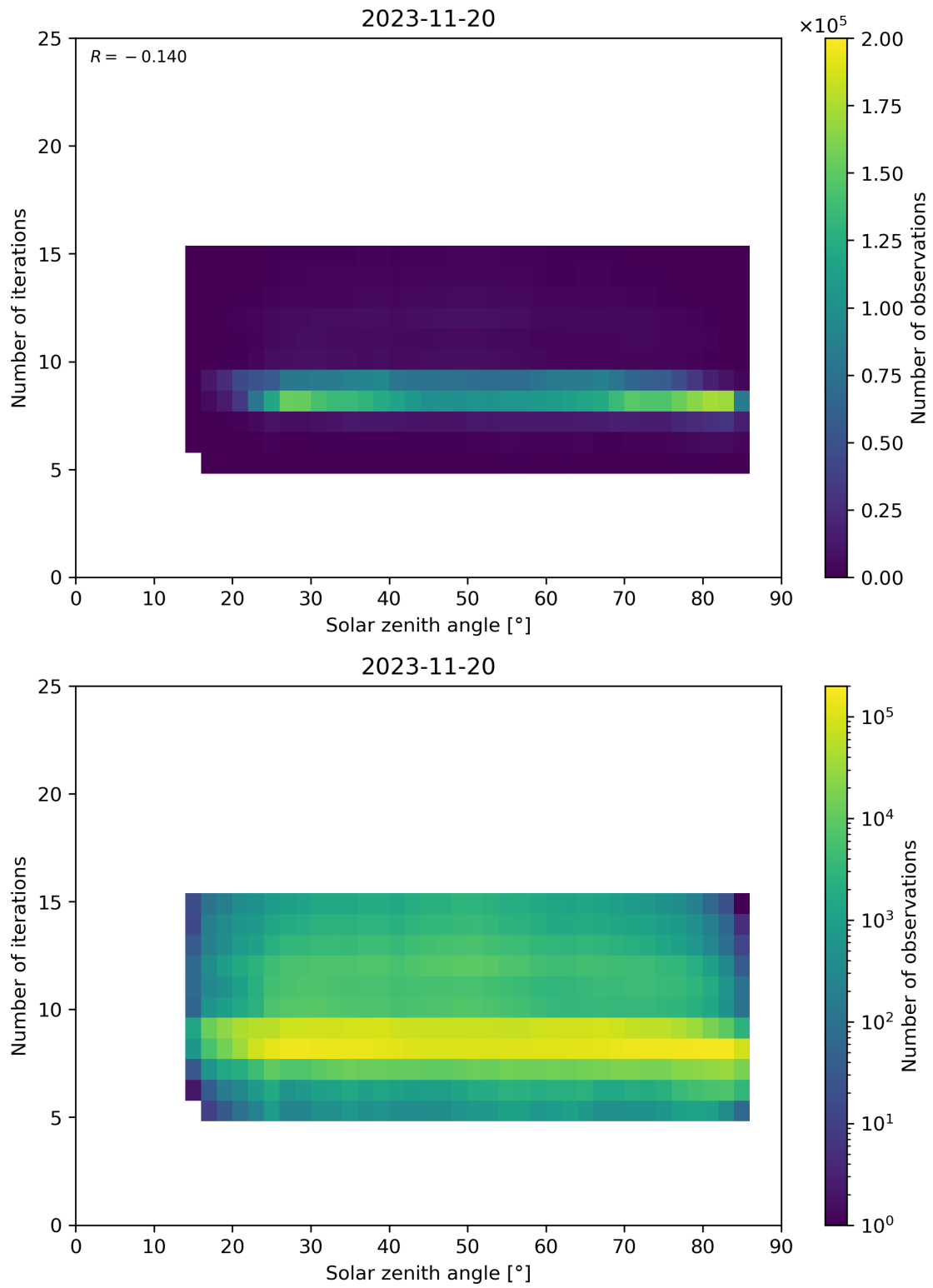
Figure 67: Scatter density plot of “Solar zenith angle” against “Number of iterations” for 2023-11-19 to 2023-11-21.
