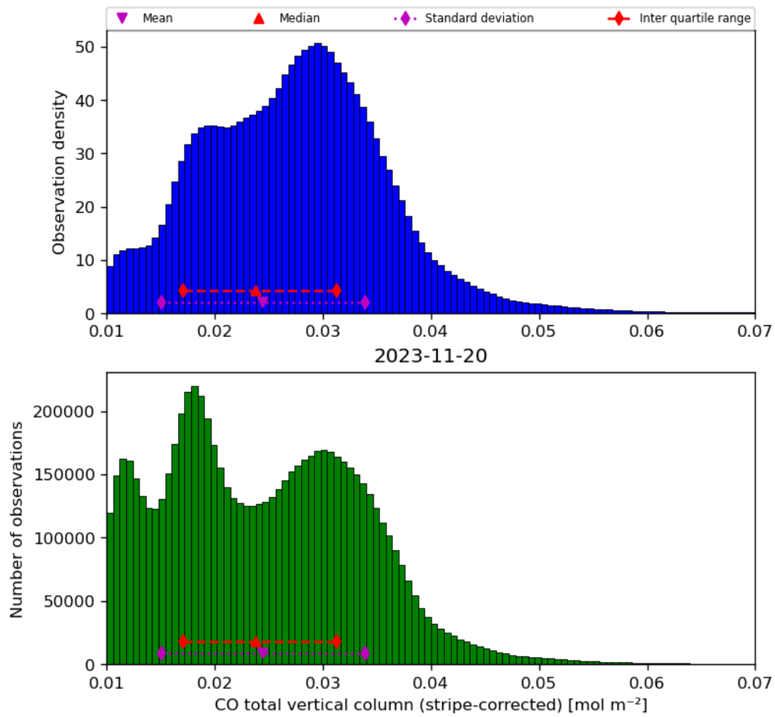
Figure 19: Histogram of “CO total vertical column (stripe-corrected)” for 2023-11-19 to 2023-11-21
