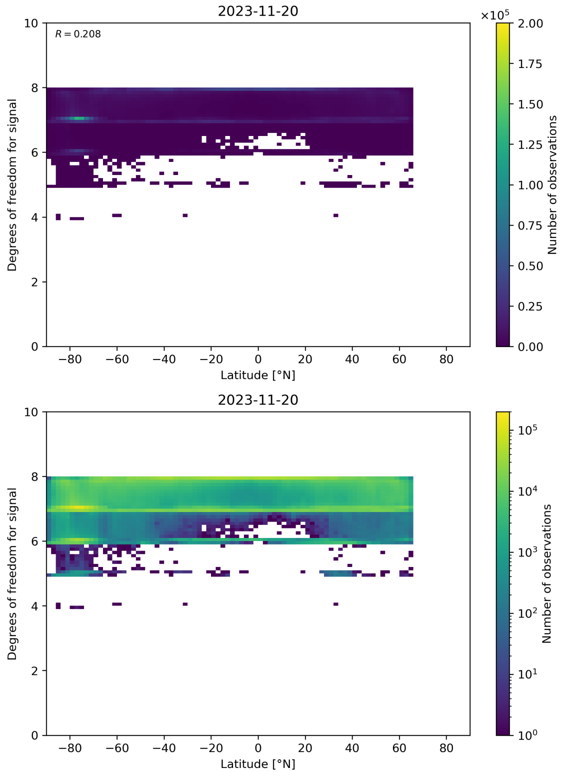
Figure 55: Scatter density plot of “Latitude” against “Degrees of freedom for signal” for 2023-11-19 to 2023-11-21.
