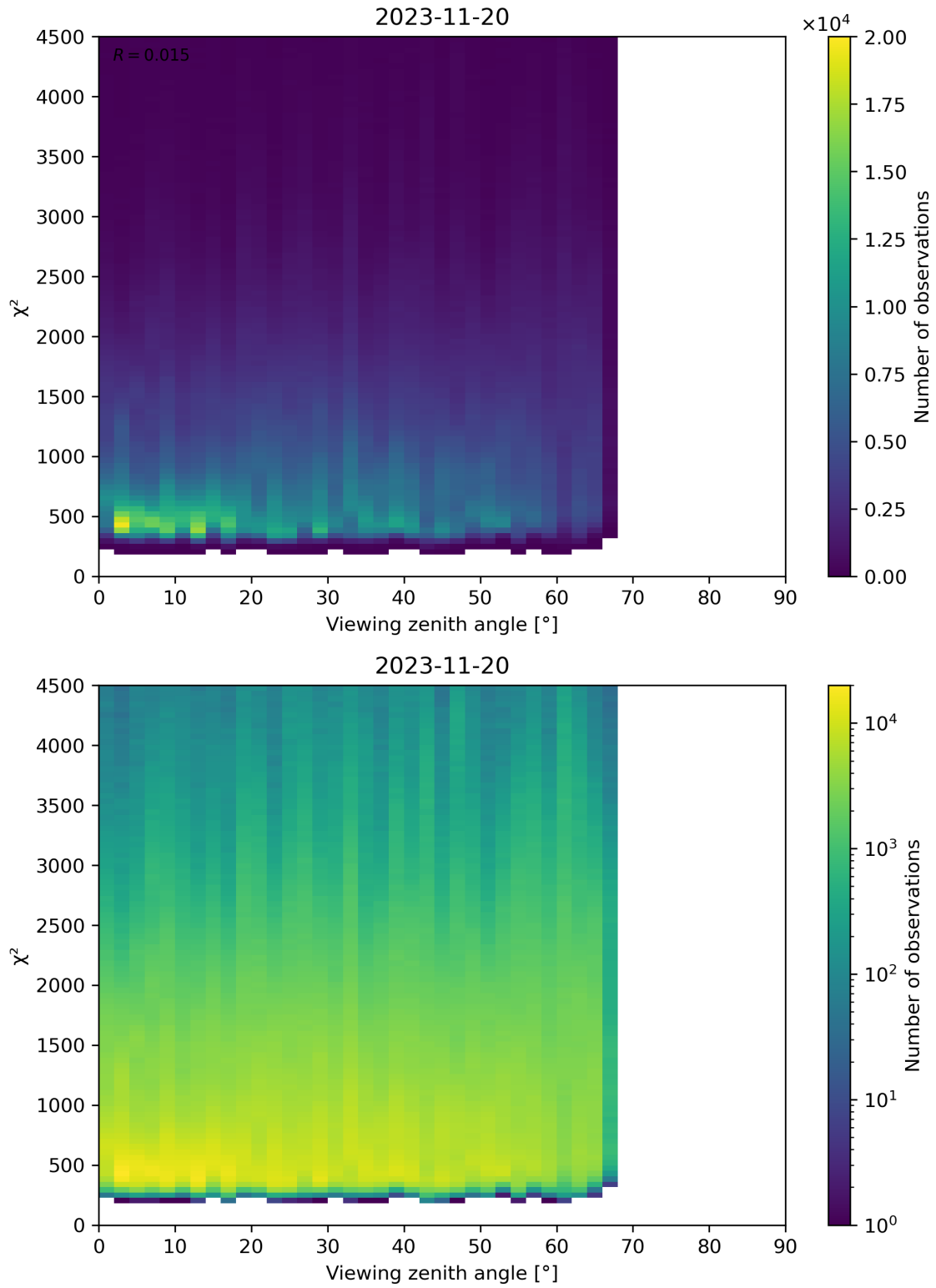
Figure 72: Scatter density plot of “Viewing zenith angle” against “ \chi^2 ” for 2023-11-19 to 2023-11-21.
