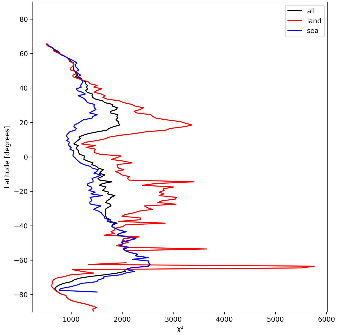
Figure 14: Zonal average of “ \chi^2 ” for 2023-11-19 to 2023-11-21.
