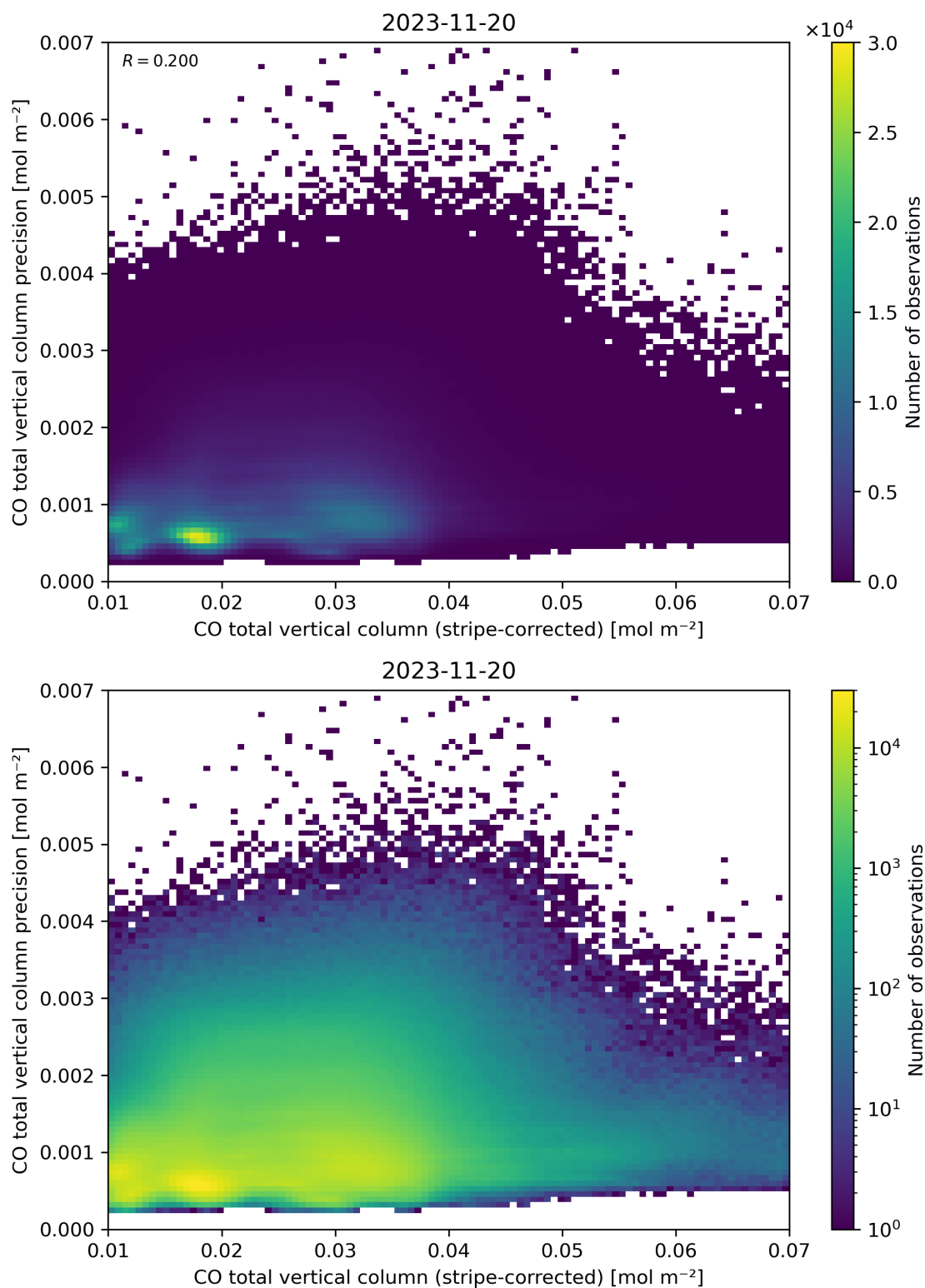
Figure 36: Scatter density plot of “CO total vertical column (stripe-corrected)” against “CO total vertical column precision” for 2023-11-19 to 2023-11-21.
