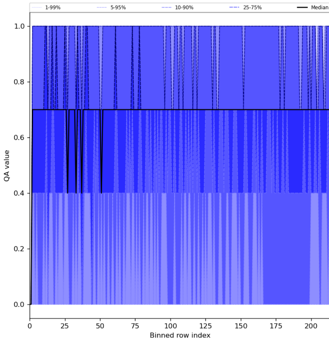
Figure 25: Along track statistics of “QA value” for 2023-11-19 to 2023-11-21
