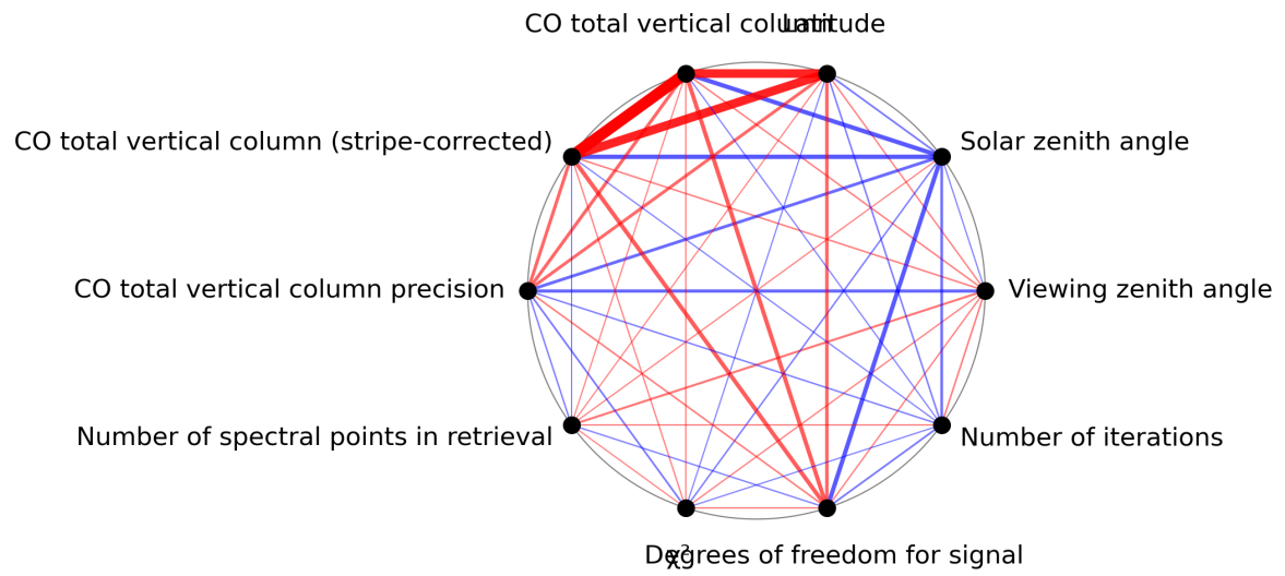
Figure 1: Map of correlation graph for 2023-11-19 to 2023-11-21.
