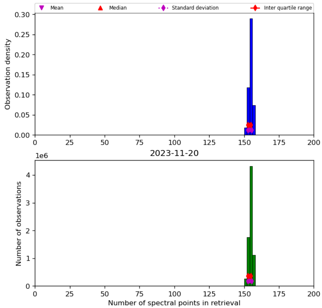
Figure 21: Histogram of “Number of spectral points in retrieval” for 2023-11-19 to 2023-11-21
