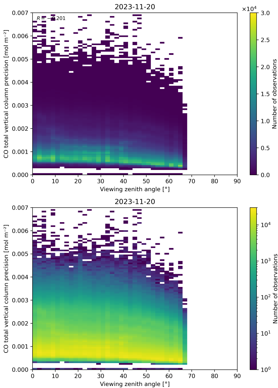
Figure 71: Scatter density plot of “Viewing zenith angle” against “CO total vertical column precision” for 2023-11-19 to 2023-11-21.
