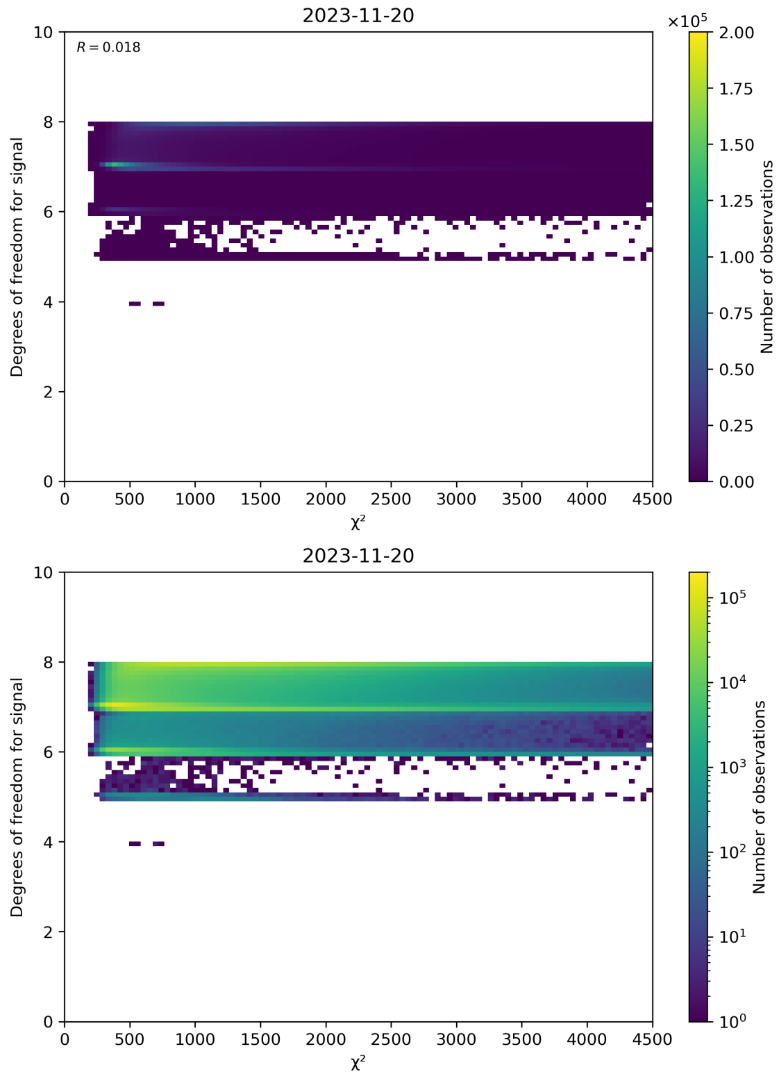
Figure 48: Scatter density plot of “ \chi^2 ” against “Degrees of freedom for signal” for 2023-11-19 to 2023-11-21.
