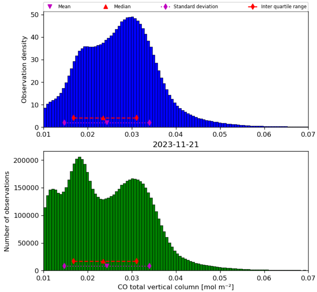
Figure 18: Histogram of “CO total vertical column” for 2023-11-20 to 2023-11-22
