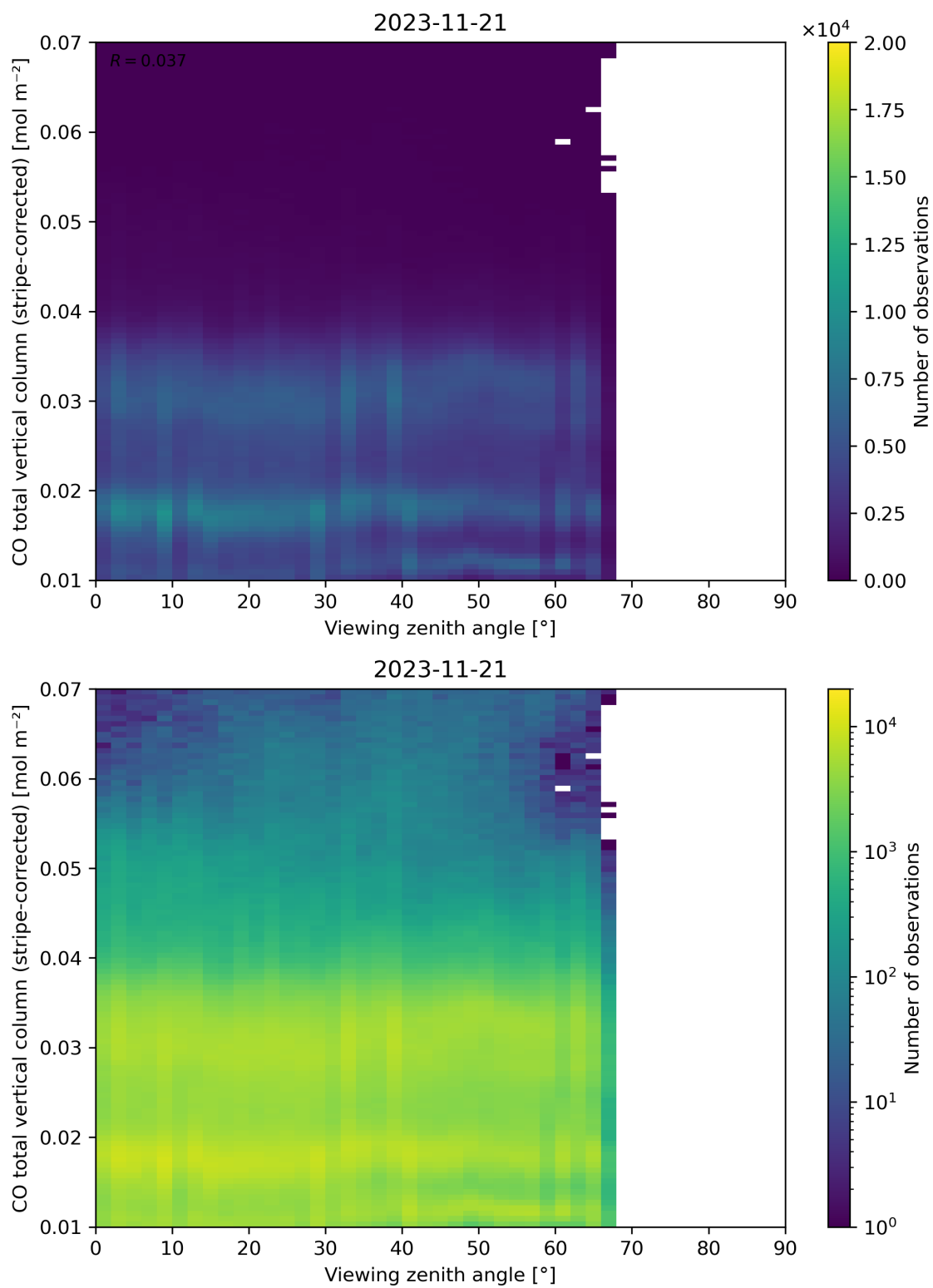
Figure 70: Scatter density plot of “Viewing zenith angle” against “CO total vertical column (stripe-corrected)” for 2023-11-20 to 2023-11-22.
