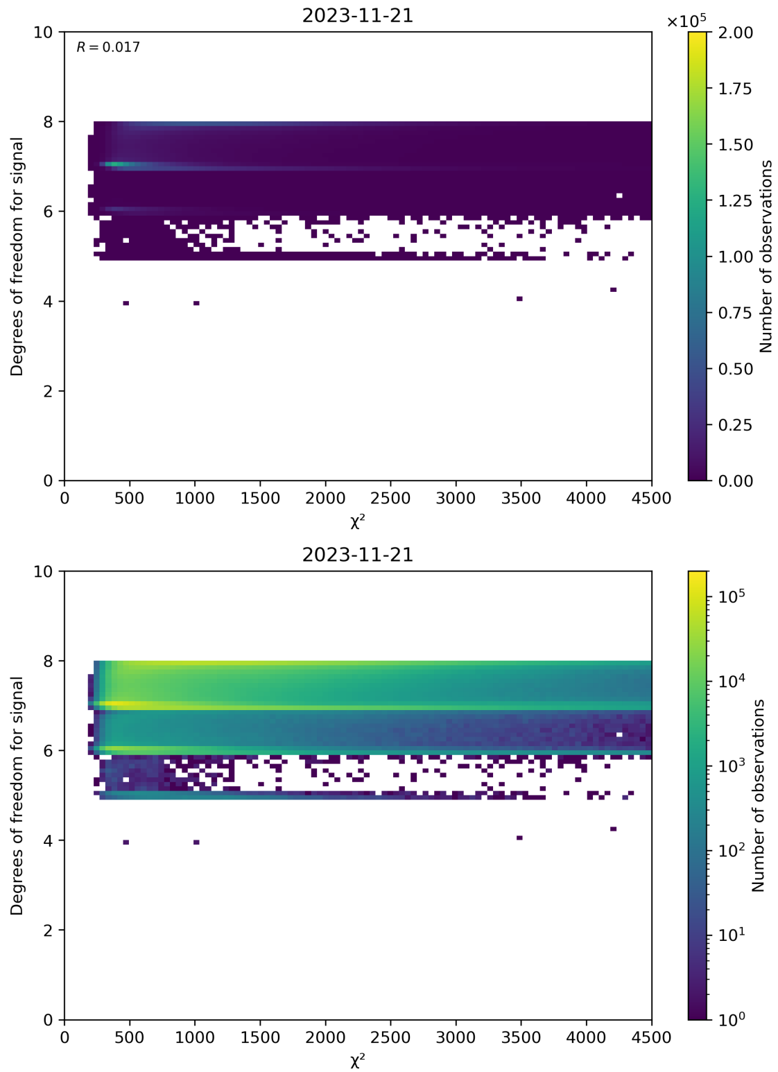
Figure 48: Scatter density plot of “ \chi^2 ” against “Degrees of freedom for signal” for 2023-11-20 to 2023-11-22.
