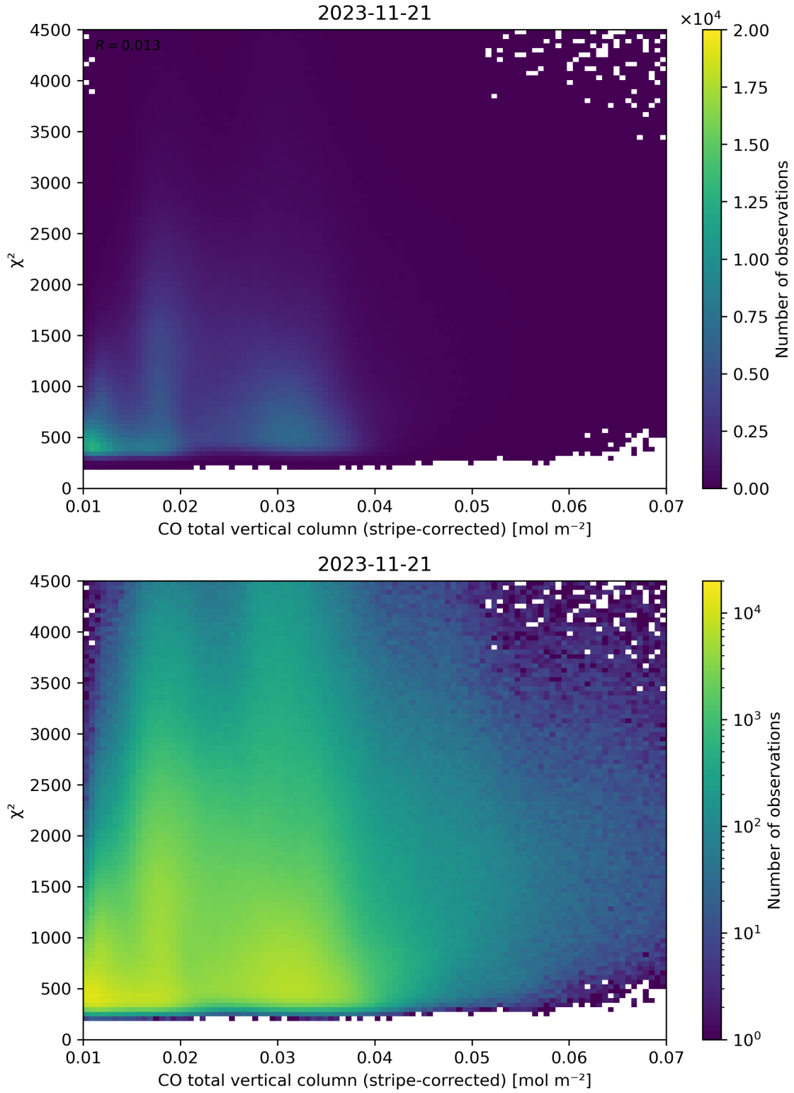
Figure 37: Scatter density plot of “CO total vertical column (stripe-corrected)” against “ \chi^2 ” for 2023-11-20 to 2023-11-22.
