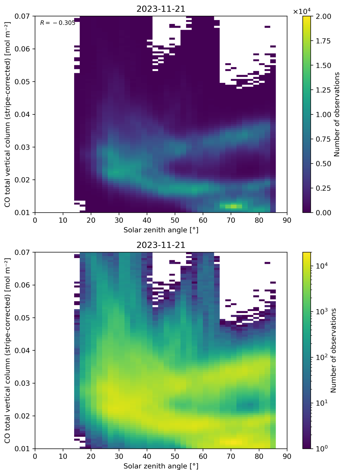
Figure 62: Scatter density plot of “Solar zenith angle” against “CO total vertical column (stripe-corrected)” for 2023-11-20 to 2023-11-22.
