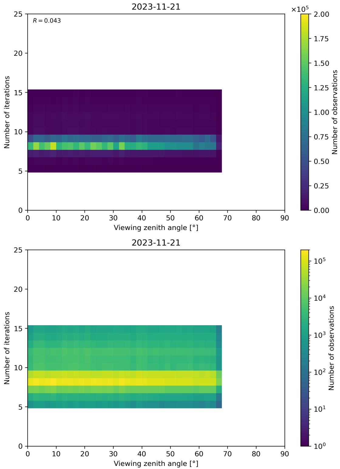
Figure 75: Scatter density plot of “Viewing zenith angle” against “Number of iterations” for 2023-11-20 to 2023-11-22.
