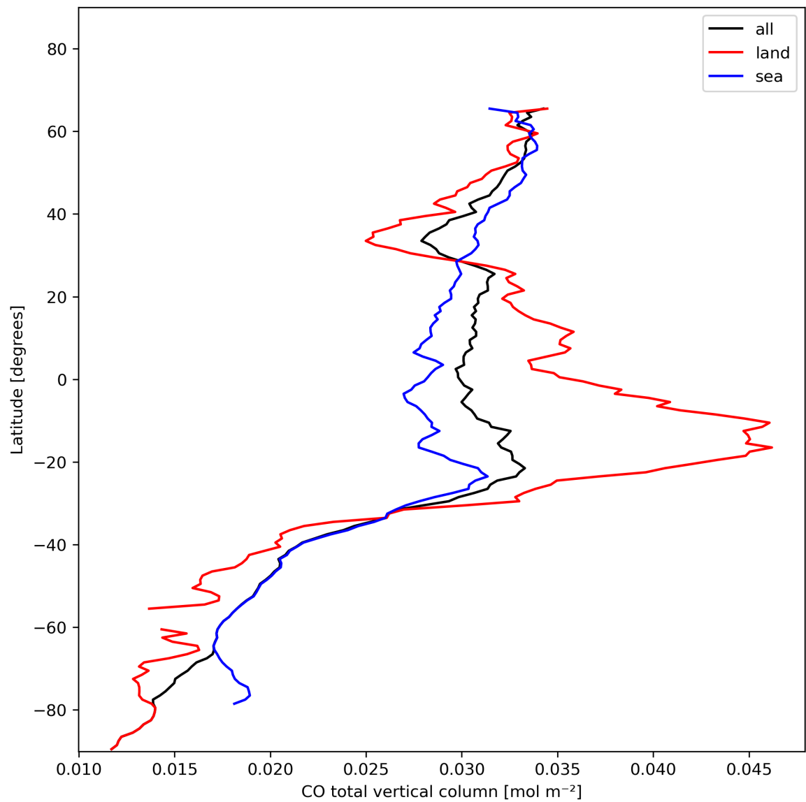
Figure 10: Zonal average of “CO total vertical column” for 2023-11-20 to 2023-11-22.
