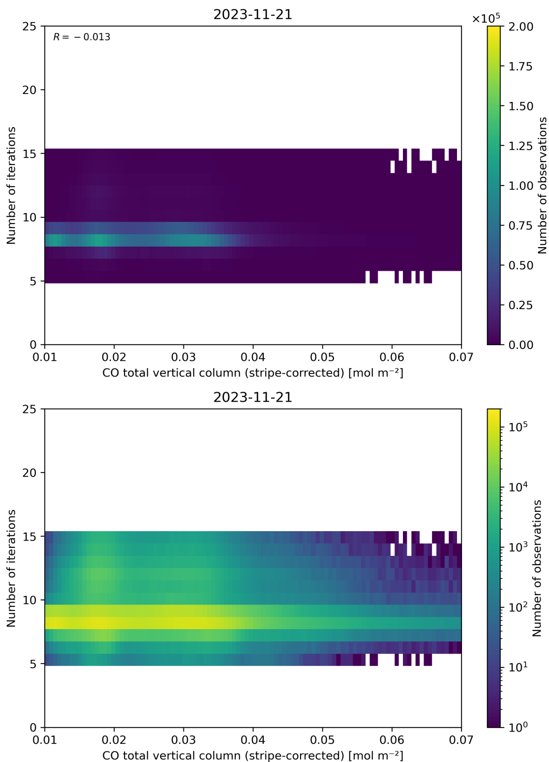
Figure 39: Scatter density plot of “CO total vertical column (stripe-corrected)” against “Number of iterations” for 2023-11-20 to 2023-11-22.
