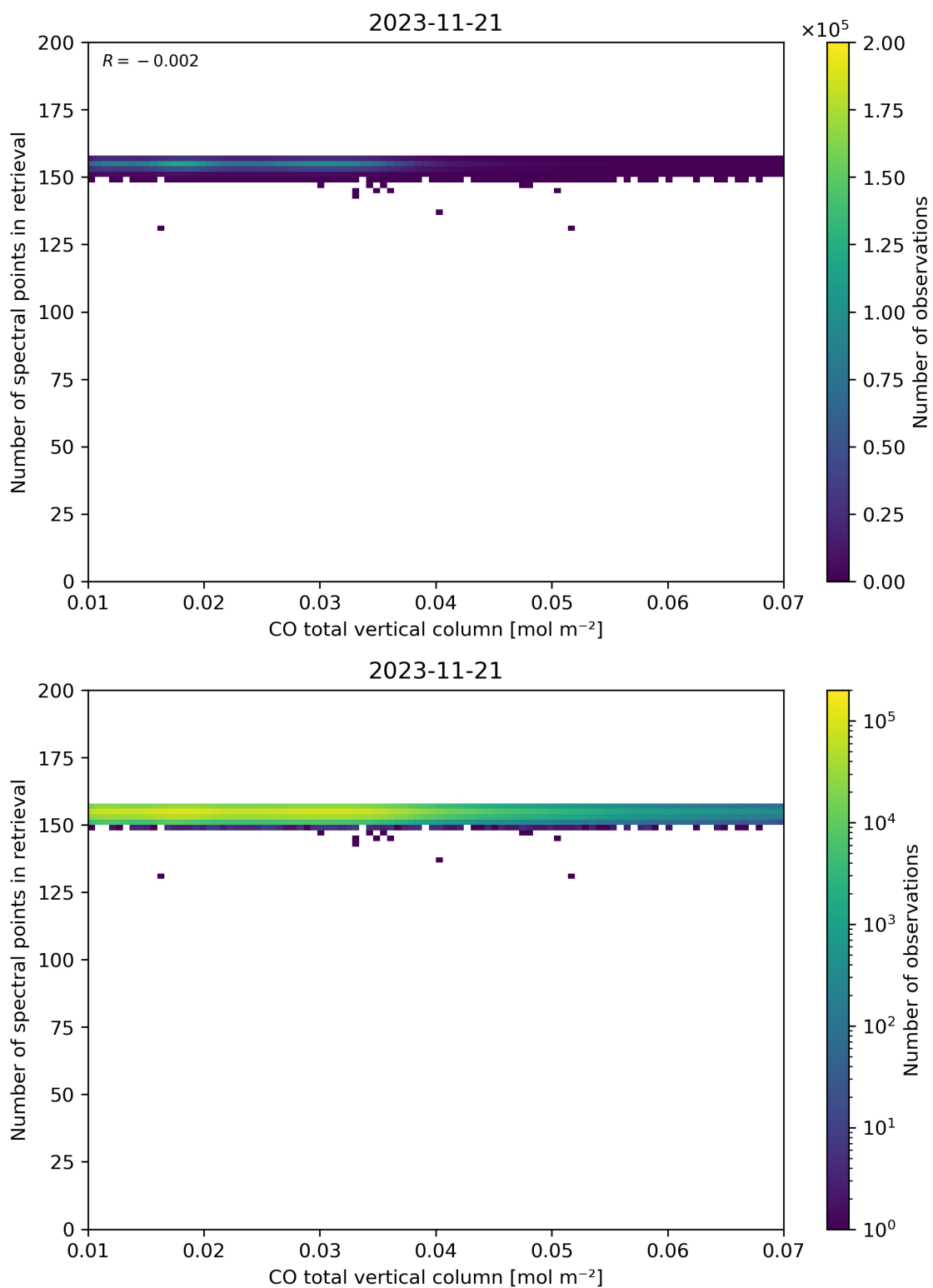
Figure 43: Scatter density plot of “CO total vertical column” against “Number of spectral points in retrieval” for 2023-11-20 to 2023-11-22.
