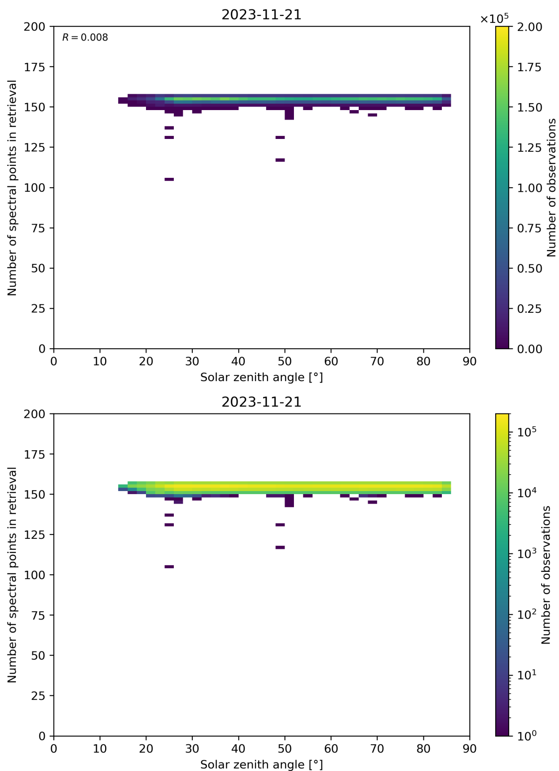
Figure 68: Scatter density plot of “Solar zenith angle” against “Number of spectral points in retrieval” for 2023-11-20 to 2023-11-22.
