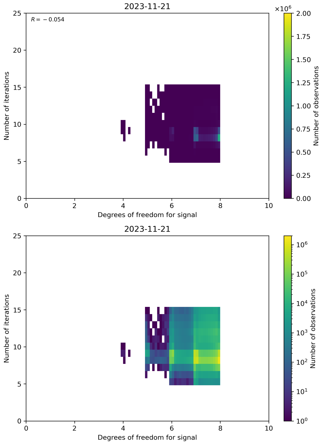
Figure 50: Scatter density plot of “Degrees of freedom for signal” against “Number of iterations” for 2023-11-20 to 2023-11-22.
