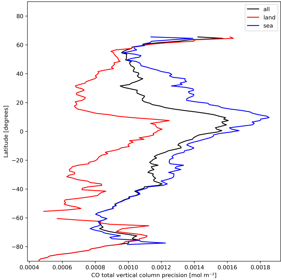
Figure 12: Zonal average of “CO total vertical column precision” for 2023-11-20 to 2023-11-22.
