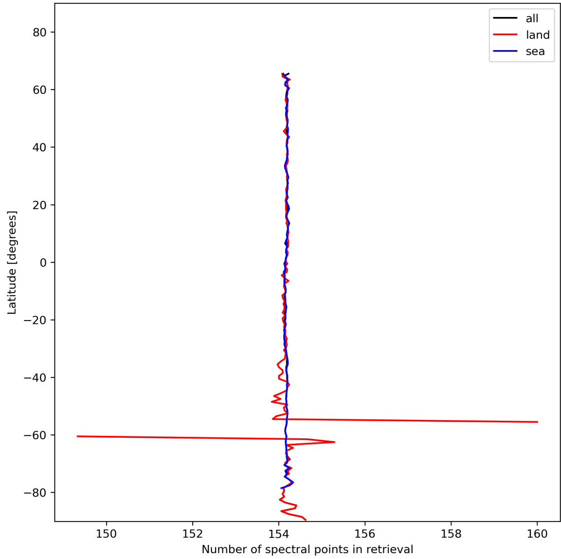
Figure 13: Zonal average of “Number of spectral points in retrieval” for 2023-11-20 to 2023-11-22.
