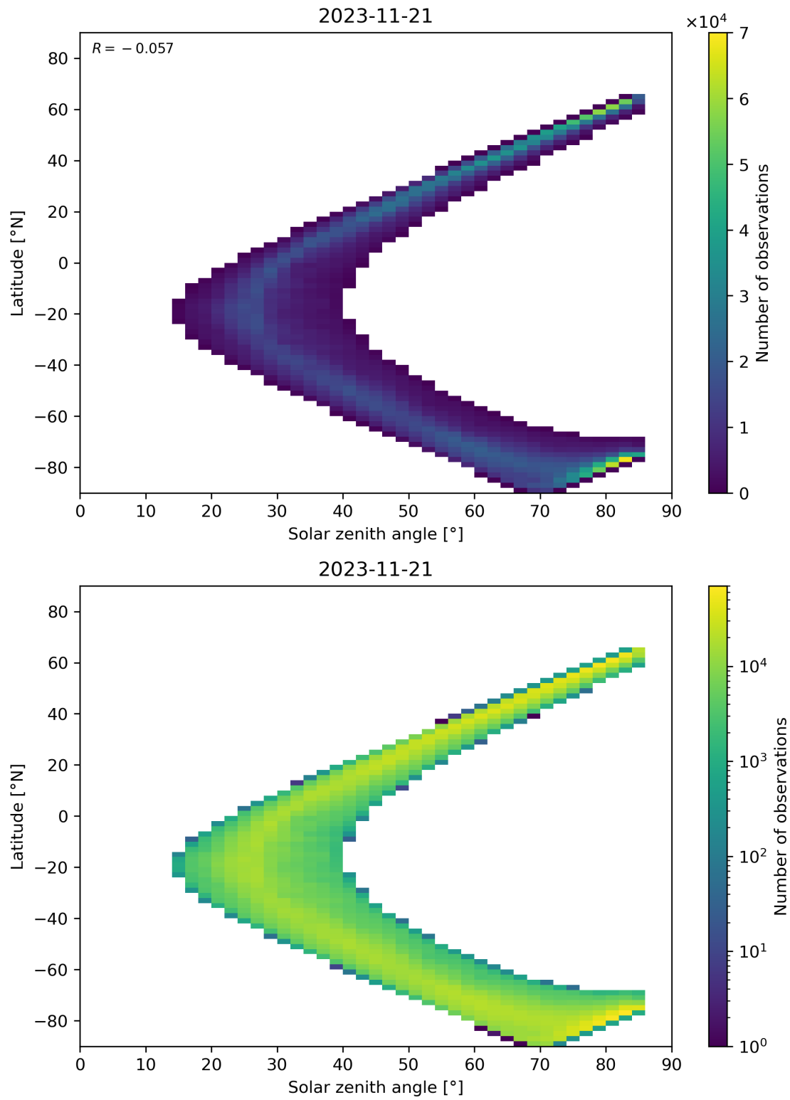
Figure 66: Scatter density plot of “Solar zenith angle” against “Latitude” for 2023-11-20 to 2023-11-22.
