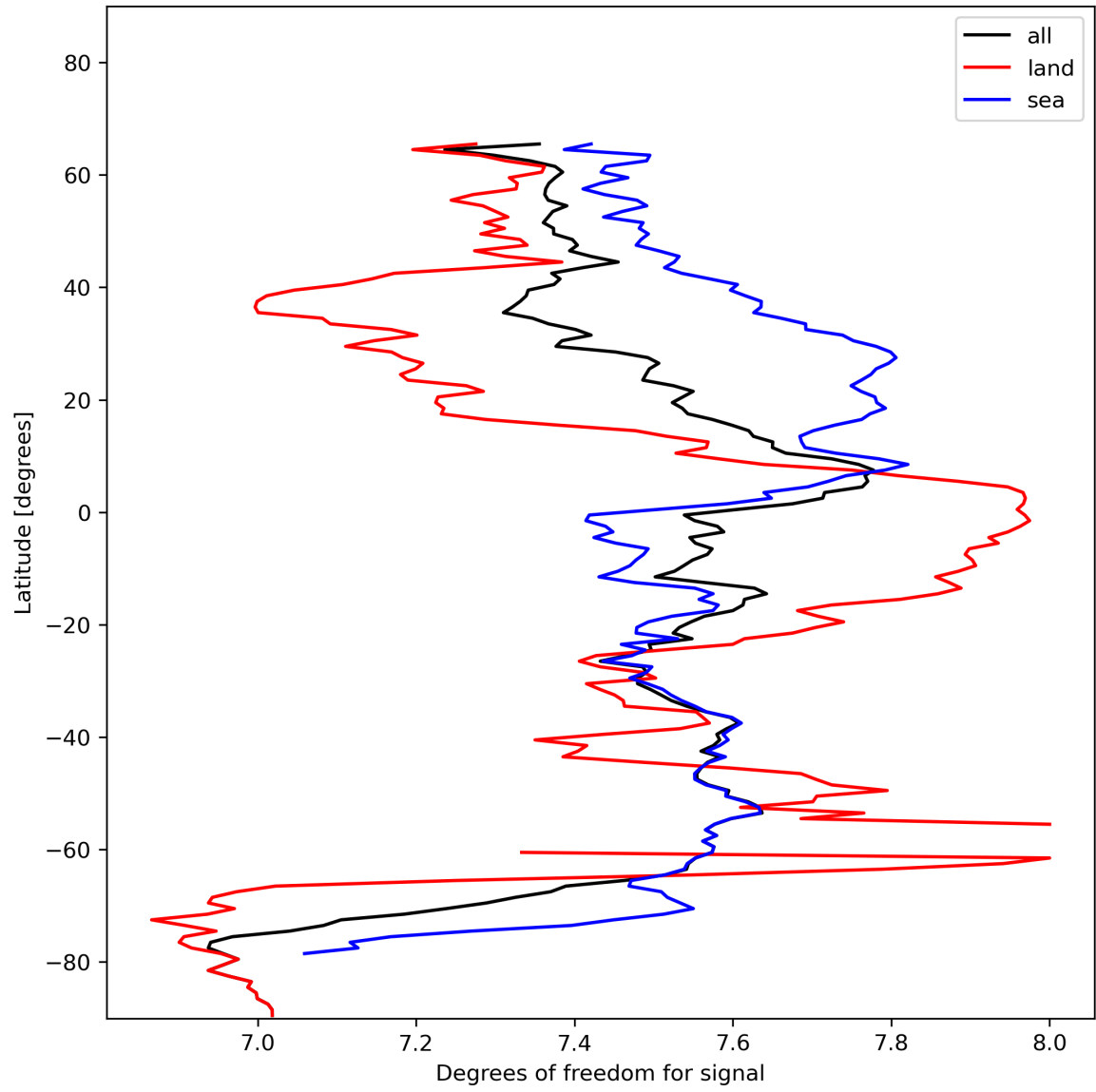
Figure 15: Zonal average of “Degrees of freedom for signal” for 2023-11-20 to 2023-11-22.
