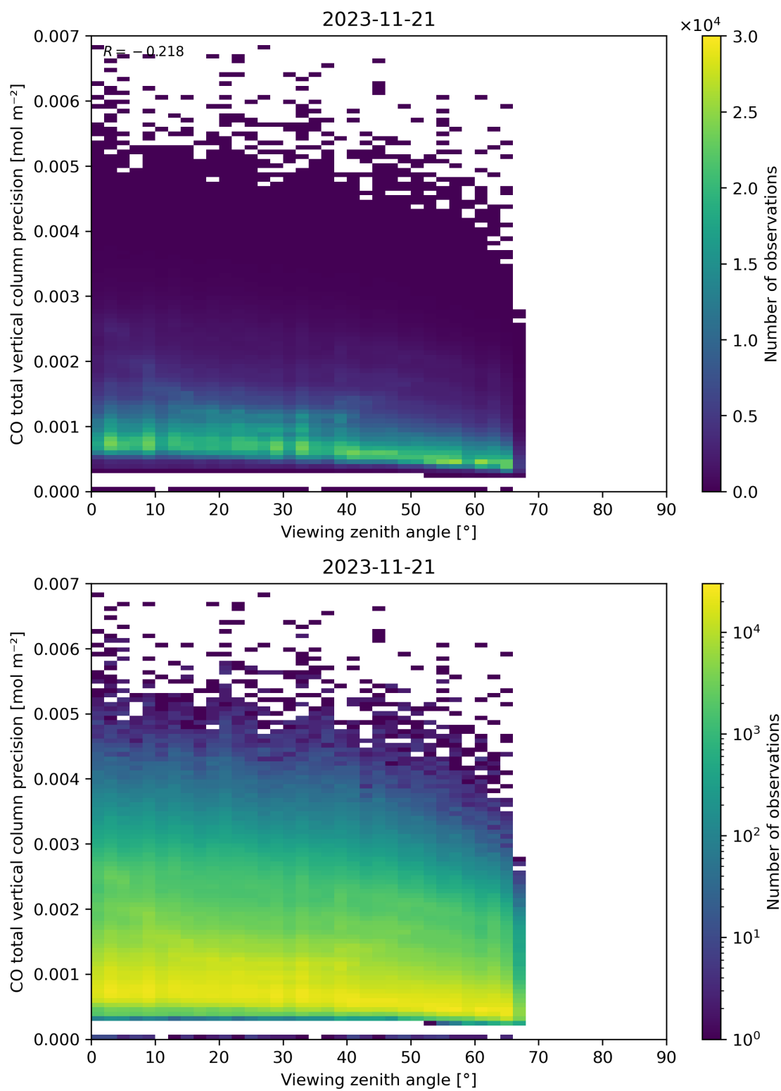
Figure 71: Scatter density plot of “Viewing zenith angle” against “CO total vertical column precision” for 2023-11-20 to 2023-11-22.
