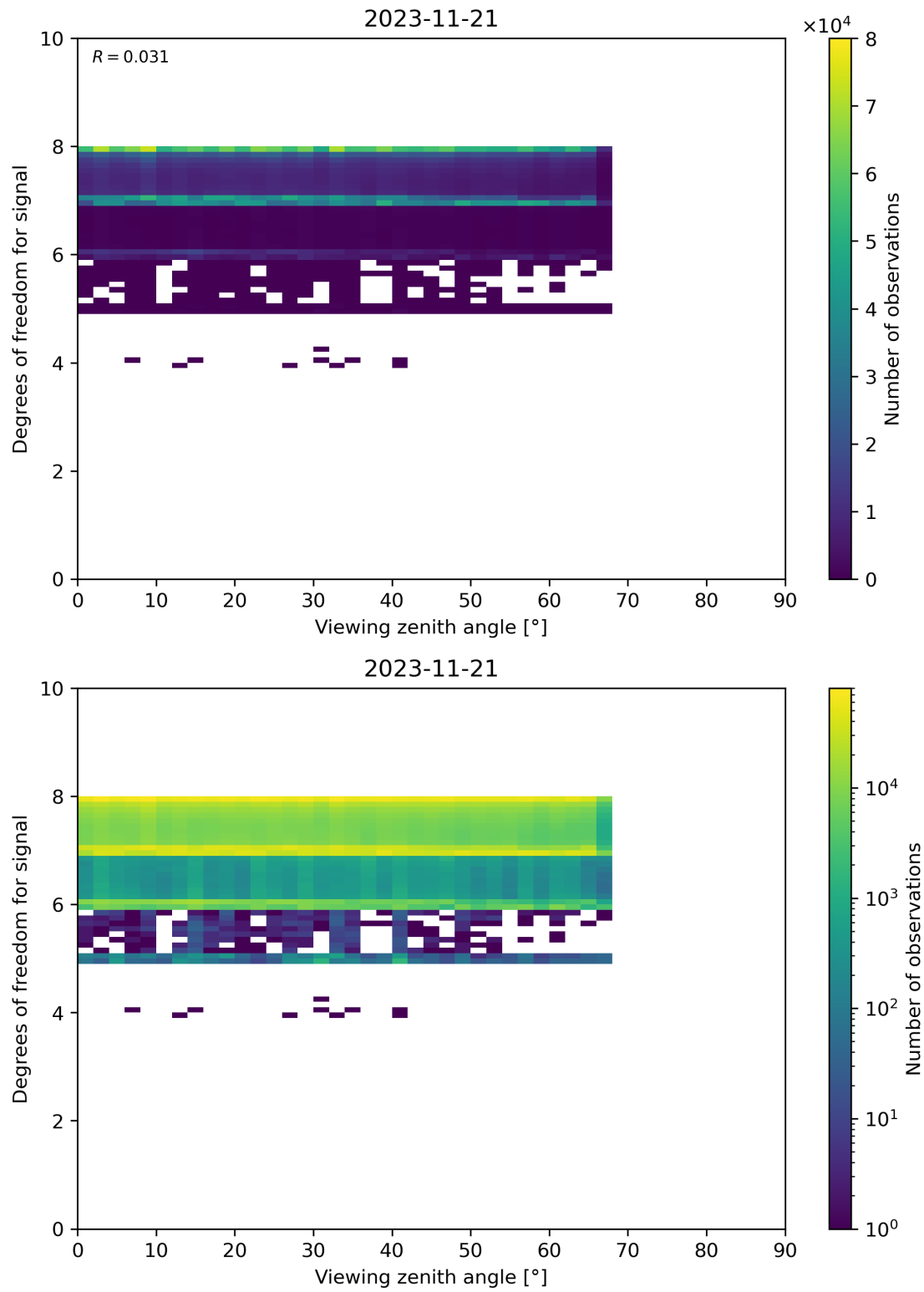
Figure 73: Scatter density plot of “Viewing zenith angle” against “Degrees of freedom for signal” for 2023-11-20 to 2023-11-22.
