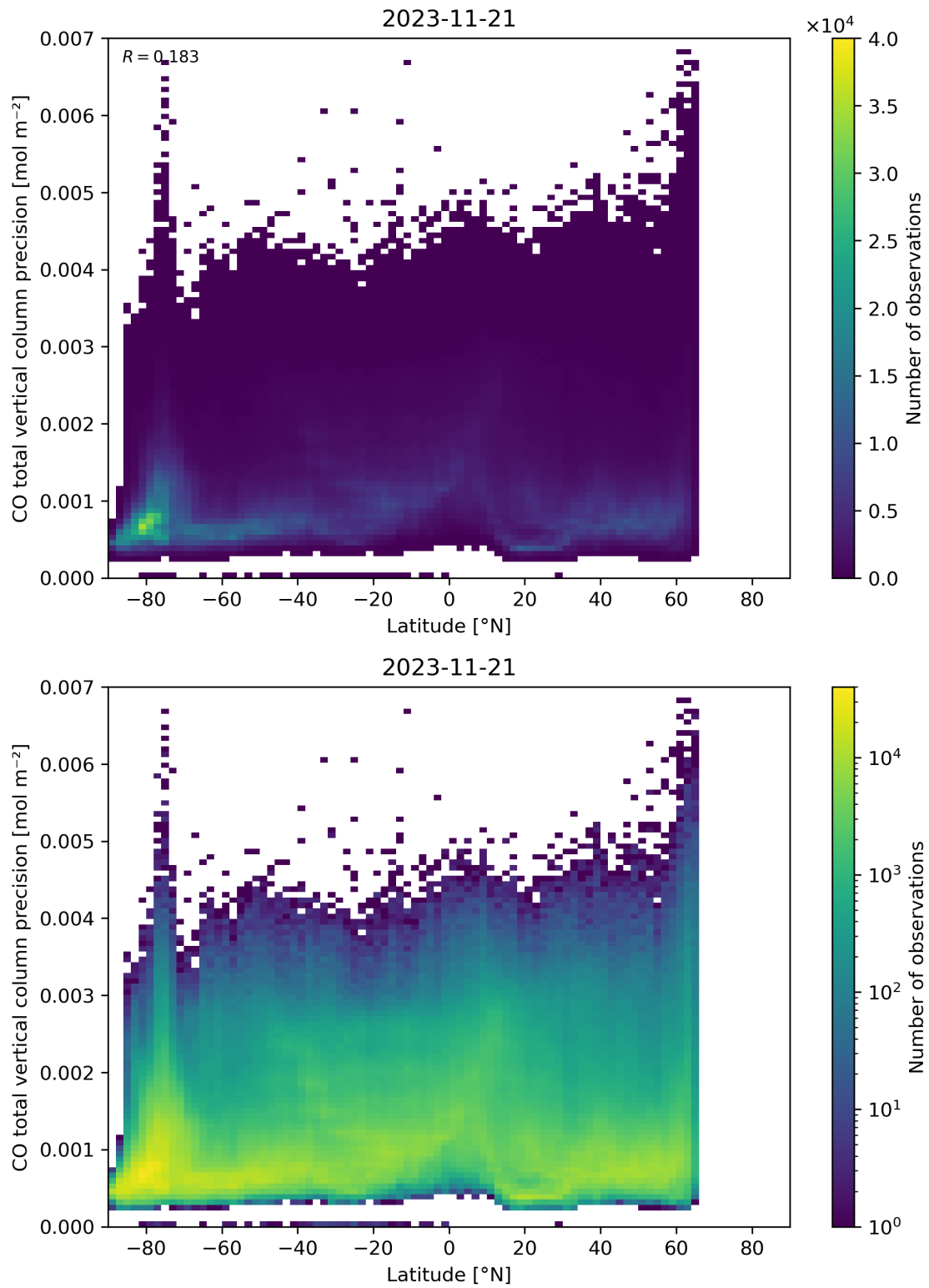
Figure 53: Scatter density plot of “Latitude” against “CO total vertical column precision” for 2023-11-20 to 2023-11-22.
