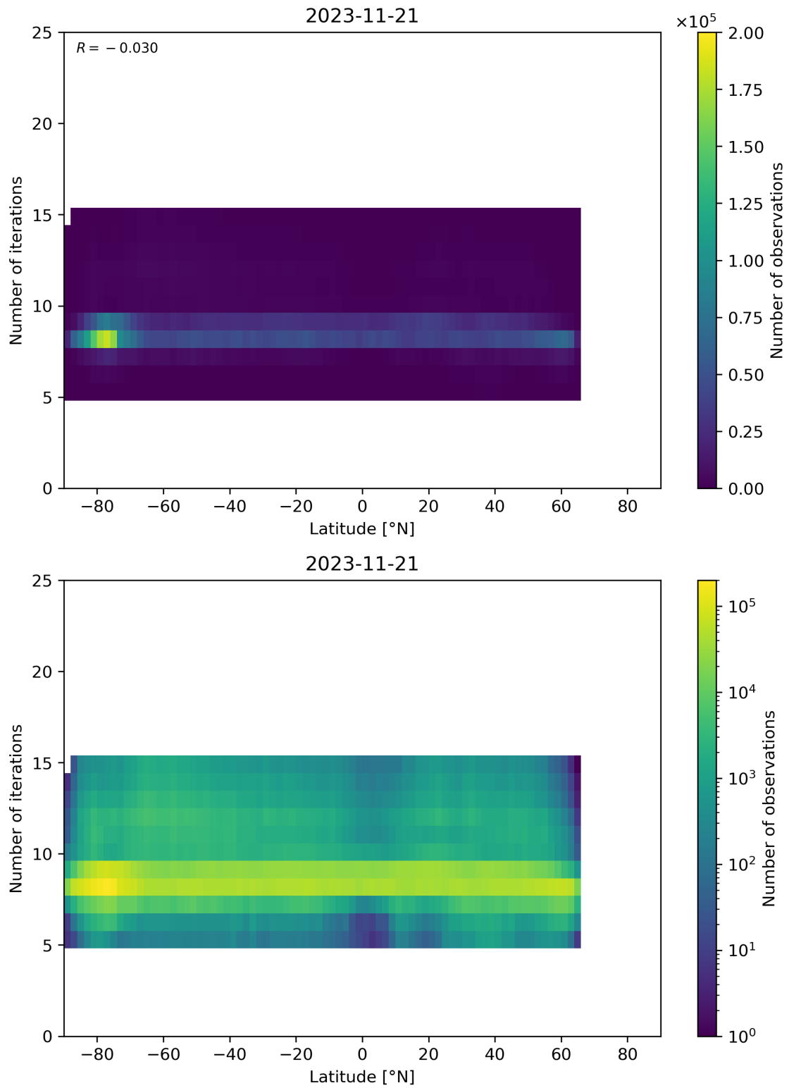
Figure 56: Scatter density plot of “Latitude” against “Number of iterations” for 2023-11-20 to 2023-11-22.
