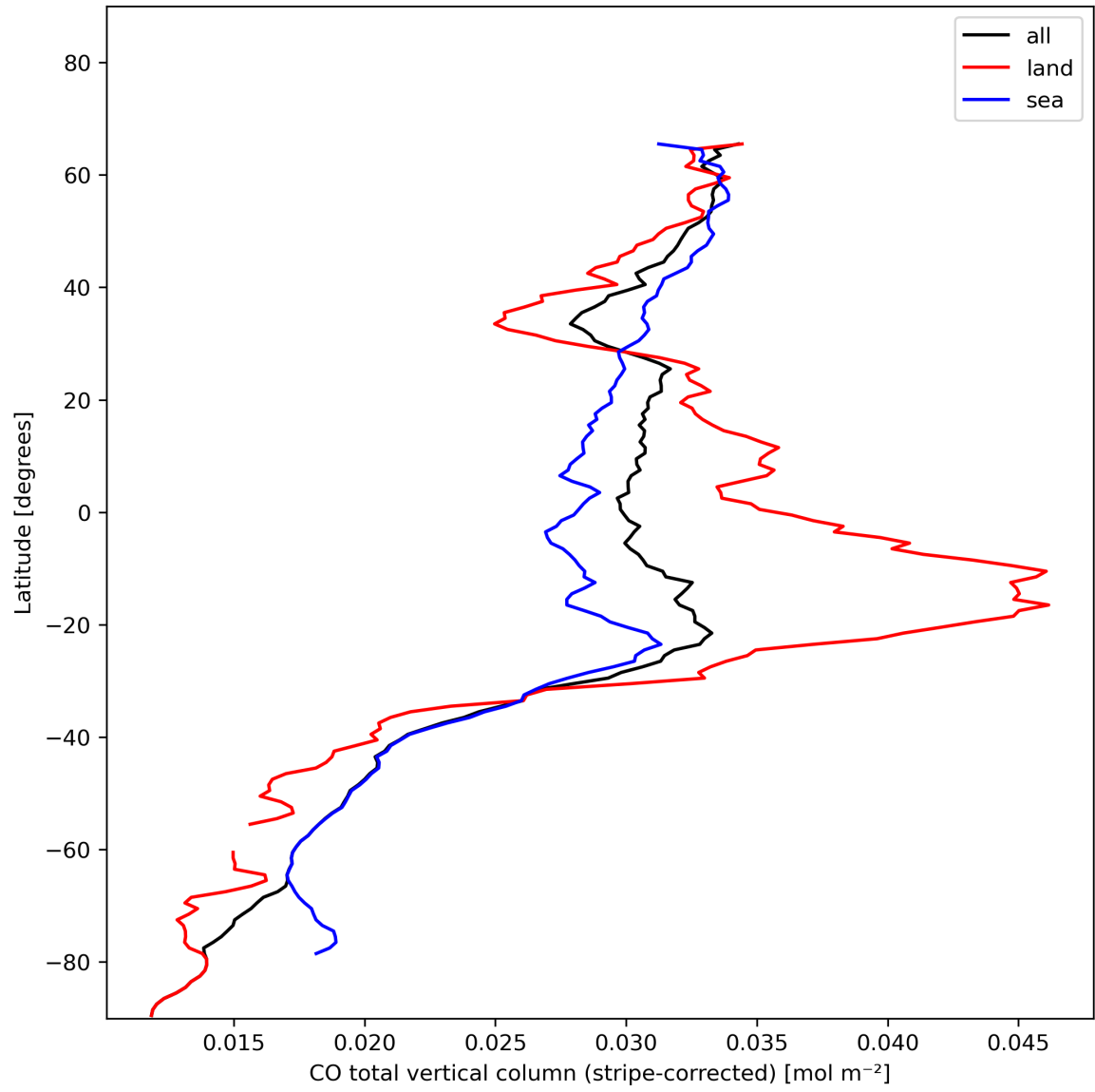
Figure 11: Zonal average of “CO total vertical column (stripe-corrected)” for 2023-11-20 to 2023-11-22.
