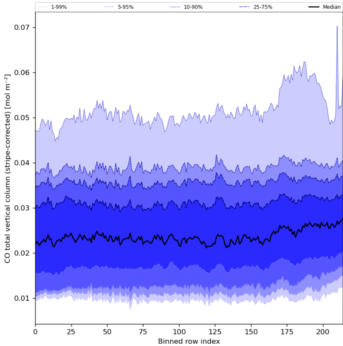
Figure 27: Along track statistics of “CO total vertical column (stripe-corrected)” for 2023-11-20 to 2023-11-22
