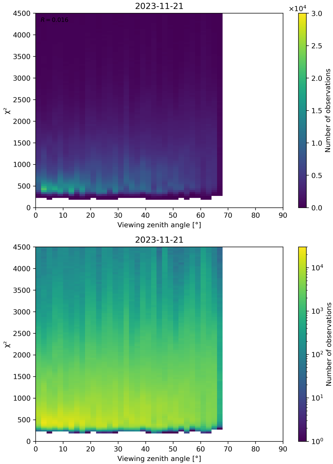
Figure 72: Scatter density plot of “Viewing zenith angle” against “ \chi^2 ” for 2023-11-20 to 2023-11-22.
