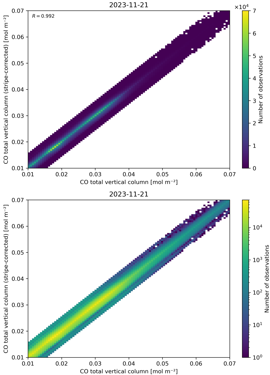
Figure 33: Scatter density plot of “CO total vertical column” against “CO total vertical column (stripe-corrected)” for 2023-11-20 to 2023-11-22.
