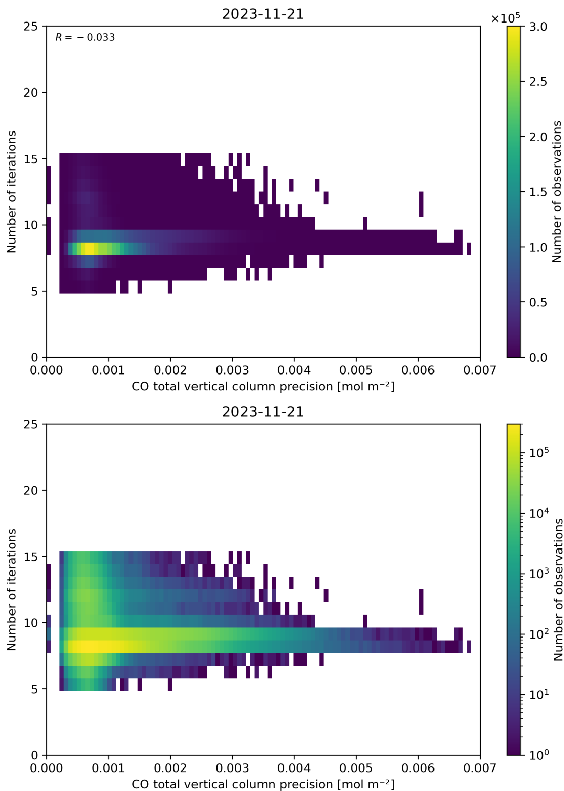
Figure 46: Scatter density plot of “CO total vertical column precision” against “Number of iterations” for 2023-11-20 to 2023-11-22.
