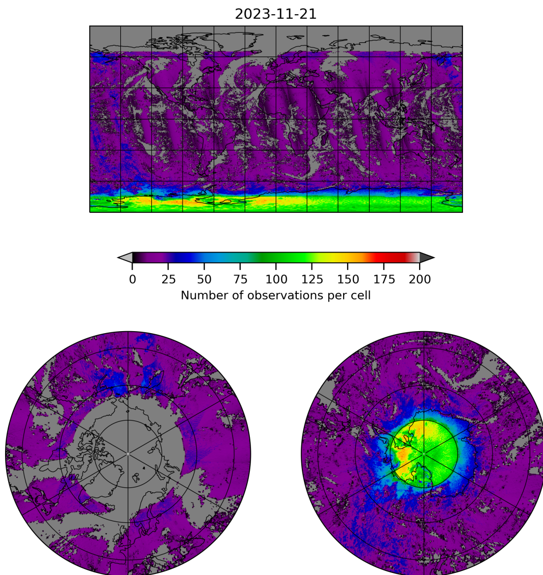
Figure 8: Map of the number of observations for 2023-11-20 to 2023-11-22
