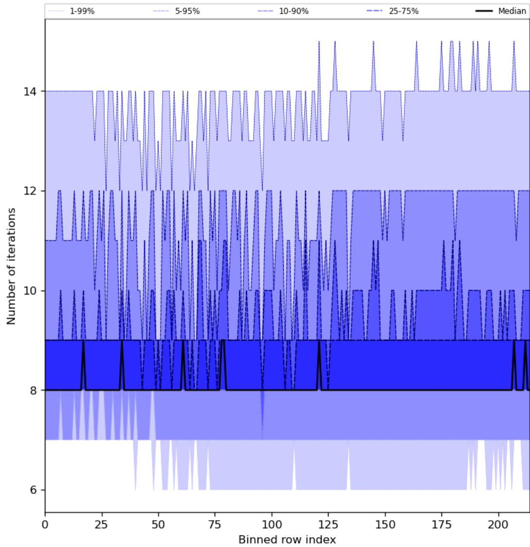
Figure 32: Along track statistics of “Number of iterations” for 2023-11-20 to 2023-11-22
