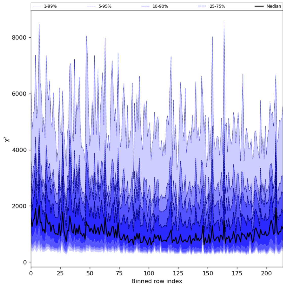
Figure 30: Along track statistics of “ \chi^2 ” for 2023-11-20 to 2023-11-22
