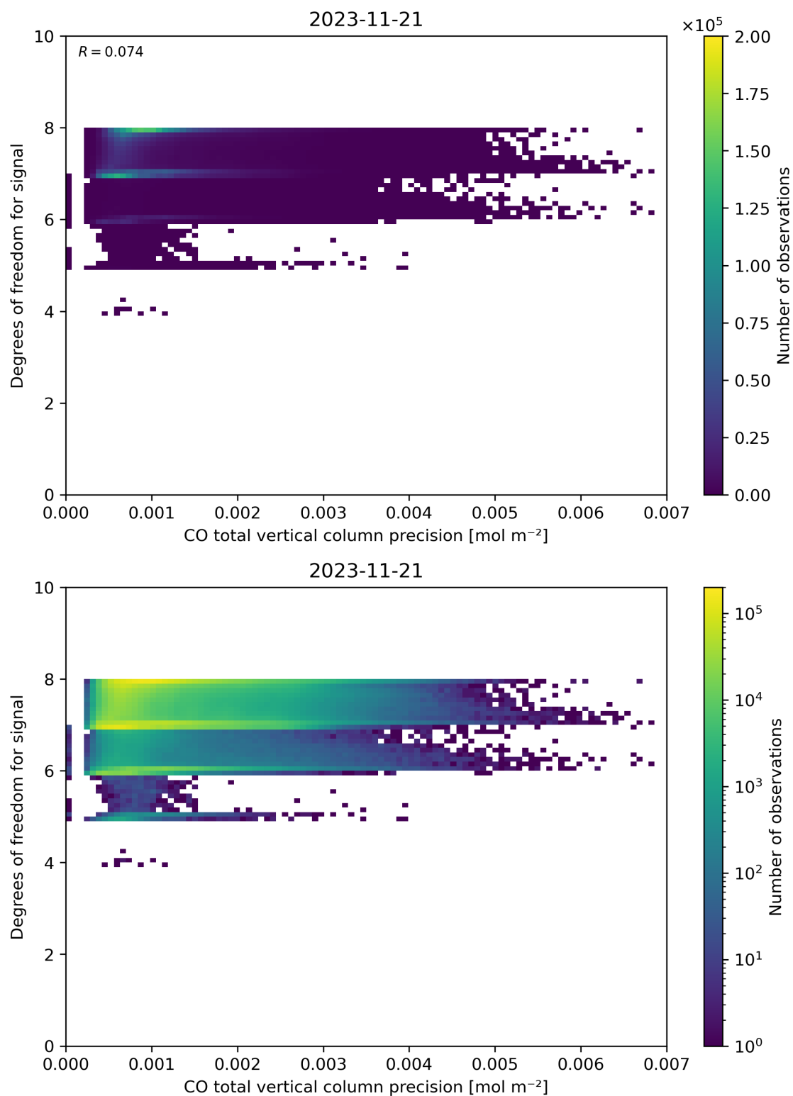
Figure 45: Scatter density plot of “CO total vertical column precision” against “Degrees of freedom for signal” for 2023-11-20 to 2023-11-22.
