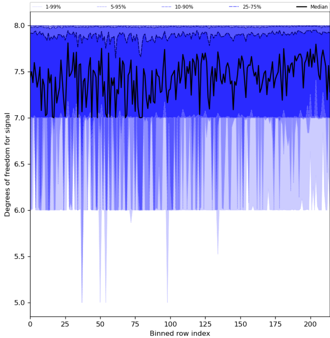
Figure 31: Along track statistics of “Degrees of freedom for signal” for 2023-11-20 to 2023-11-22
