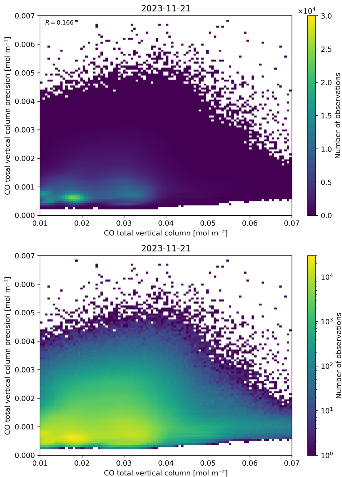
Figure 34: Scatter density plot of “CO total vertical column” against “CO total vertical column precision” for 2023-11-20 to 2023-11-22.
