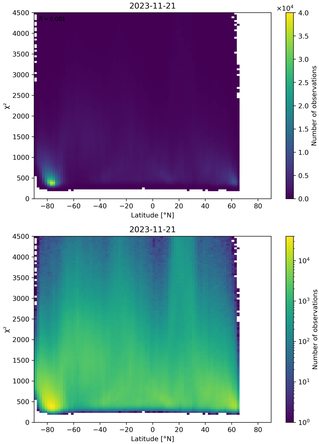
Figure 54: Scatter density plot of “Latitude” against “ \chi^2 ” for 2023-11-20 to 2023-11-22.
