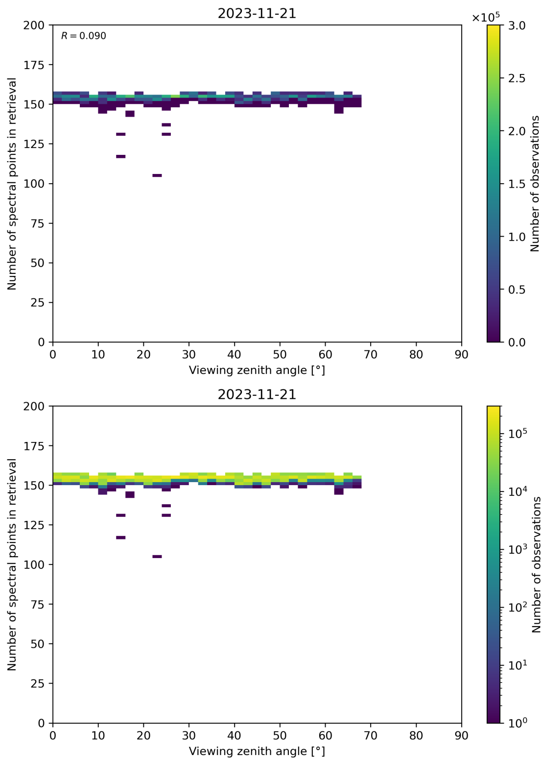
Figure 76: Scatter density plot of “Viewing zenith angle” against “Number of spectral points in retrieval” for 2023-11-20 to 2023-11-22.
