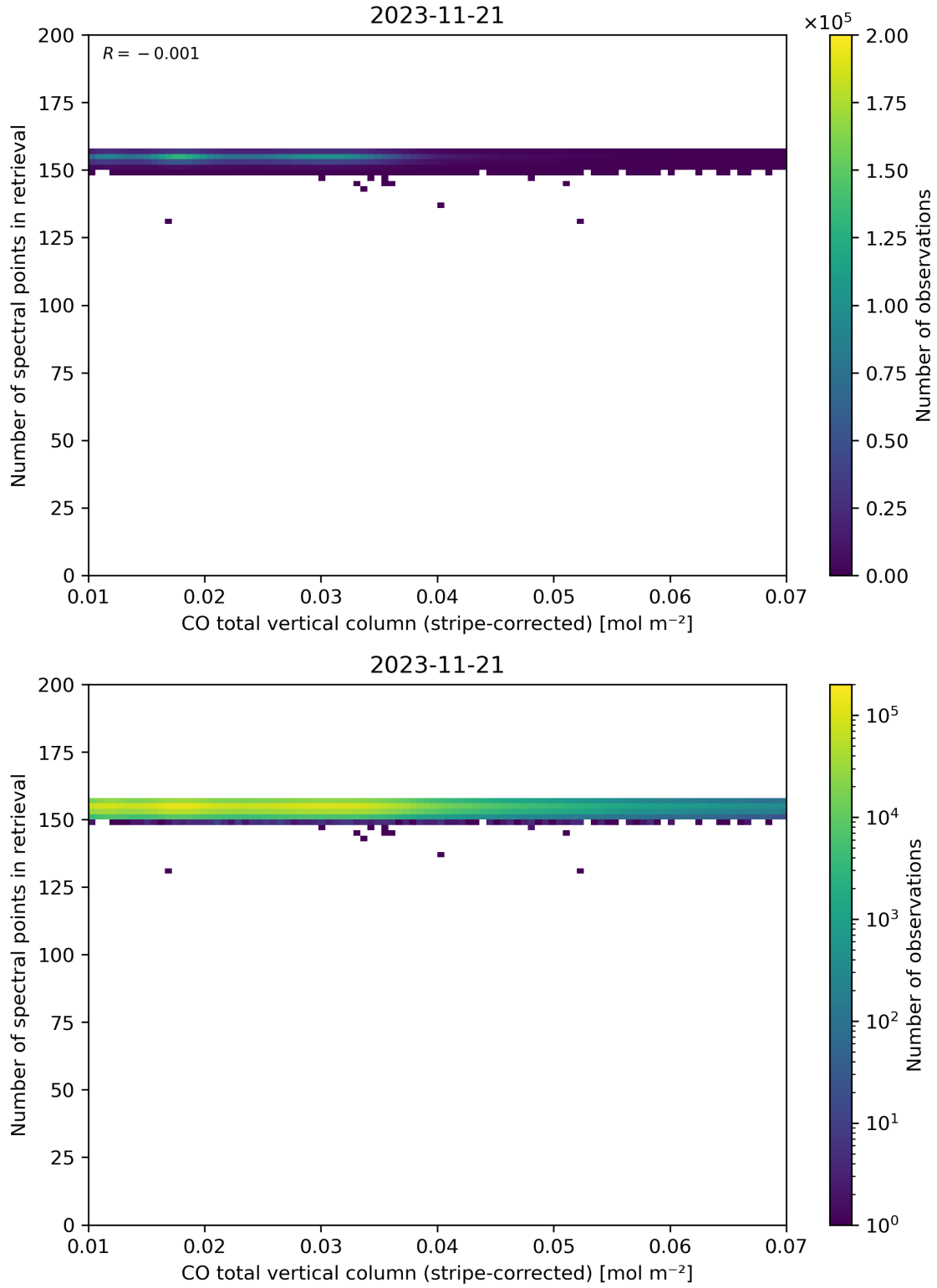
Figure 40: Scatter density plot of “CO total vertical column (stripe-corrected)” against “Number of spectral points in retrieval” for 2023-11-20 to 2023-11-22.
