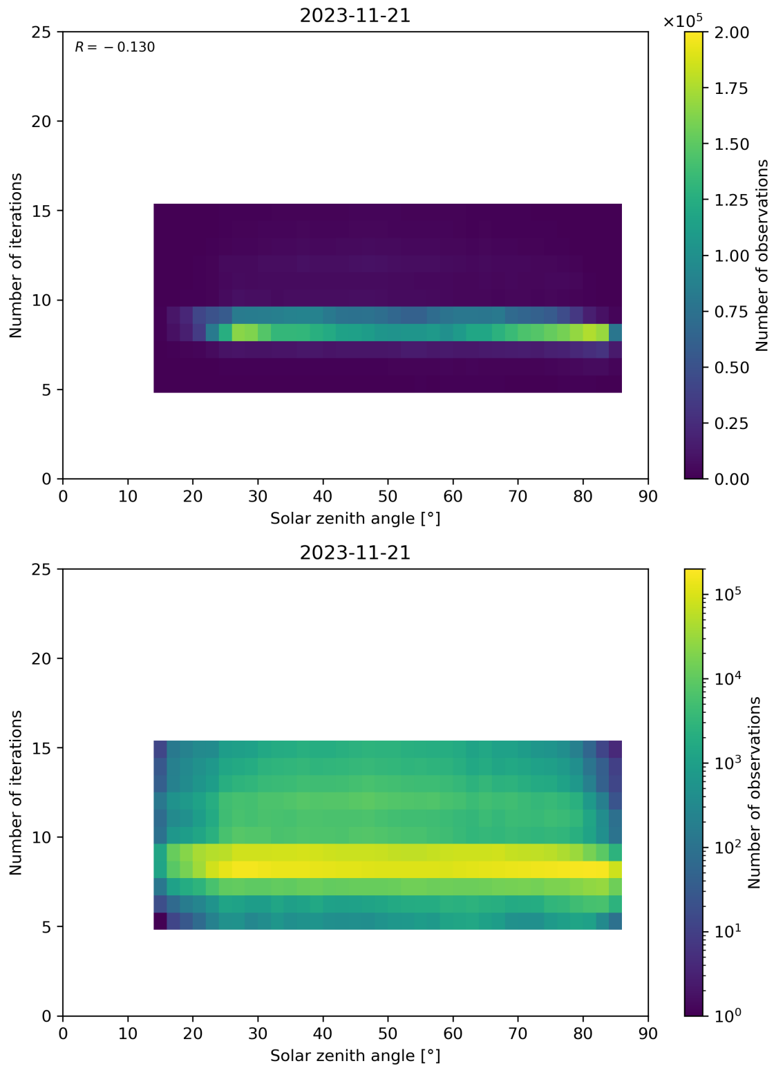
Figure 67: Scatter density plot of “Solar zenith angle” against “Number of iterations” for 2023-11-20 to 2023-11-22.
