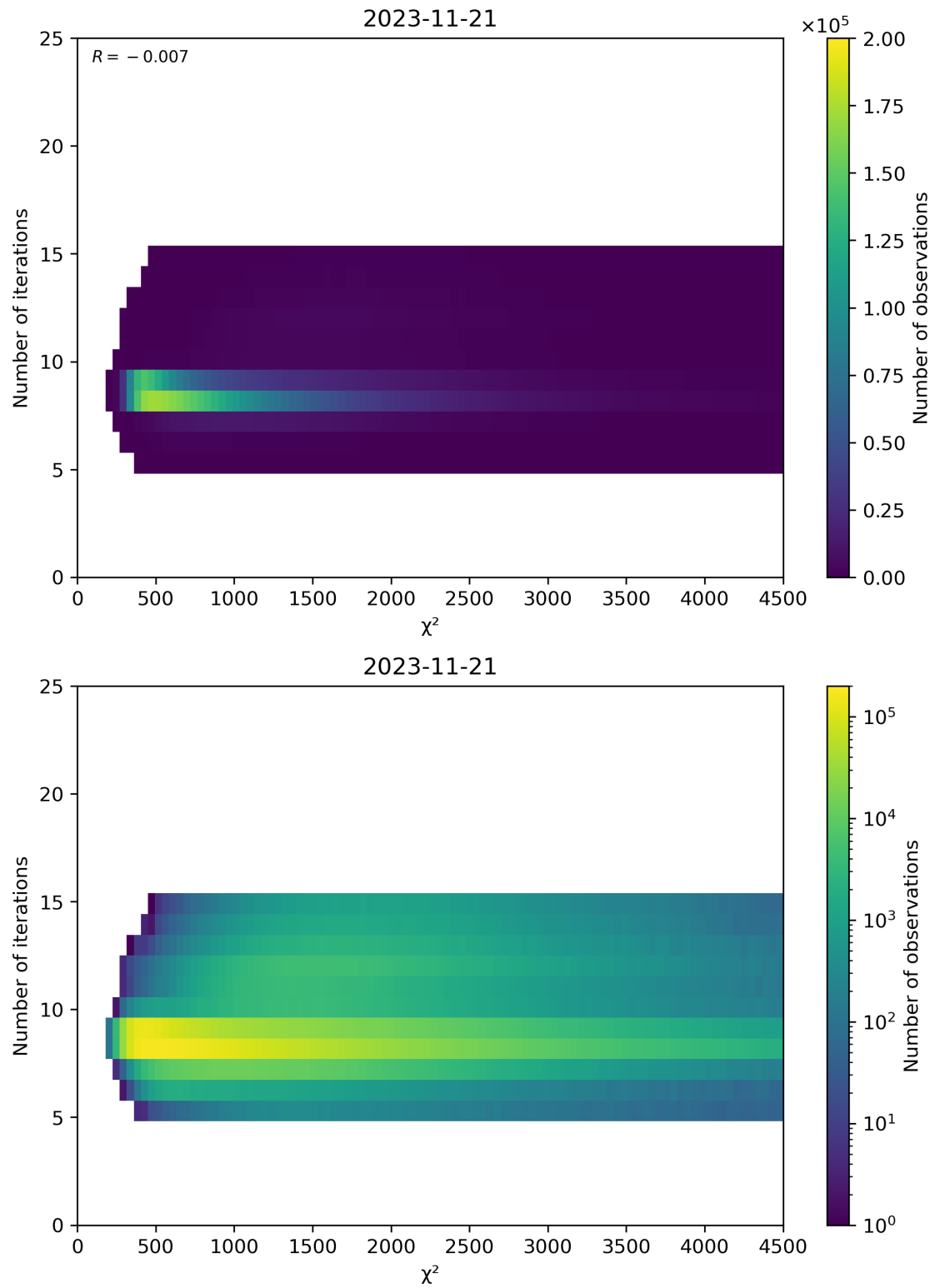
Figure 49: Scatter density plot of “ \chi^2 ” against “Number of iterations” for 2023-11-20 to 2023-11-22.
