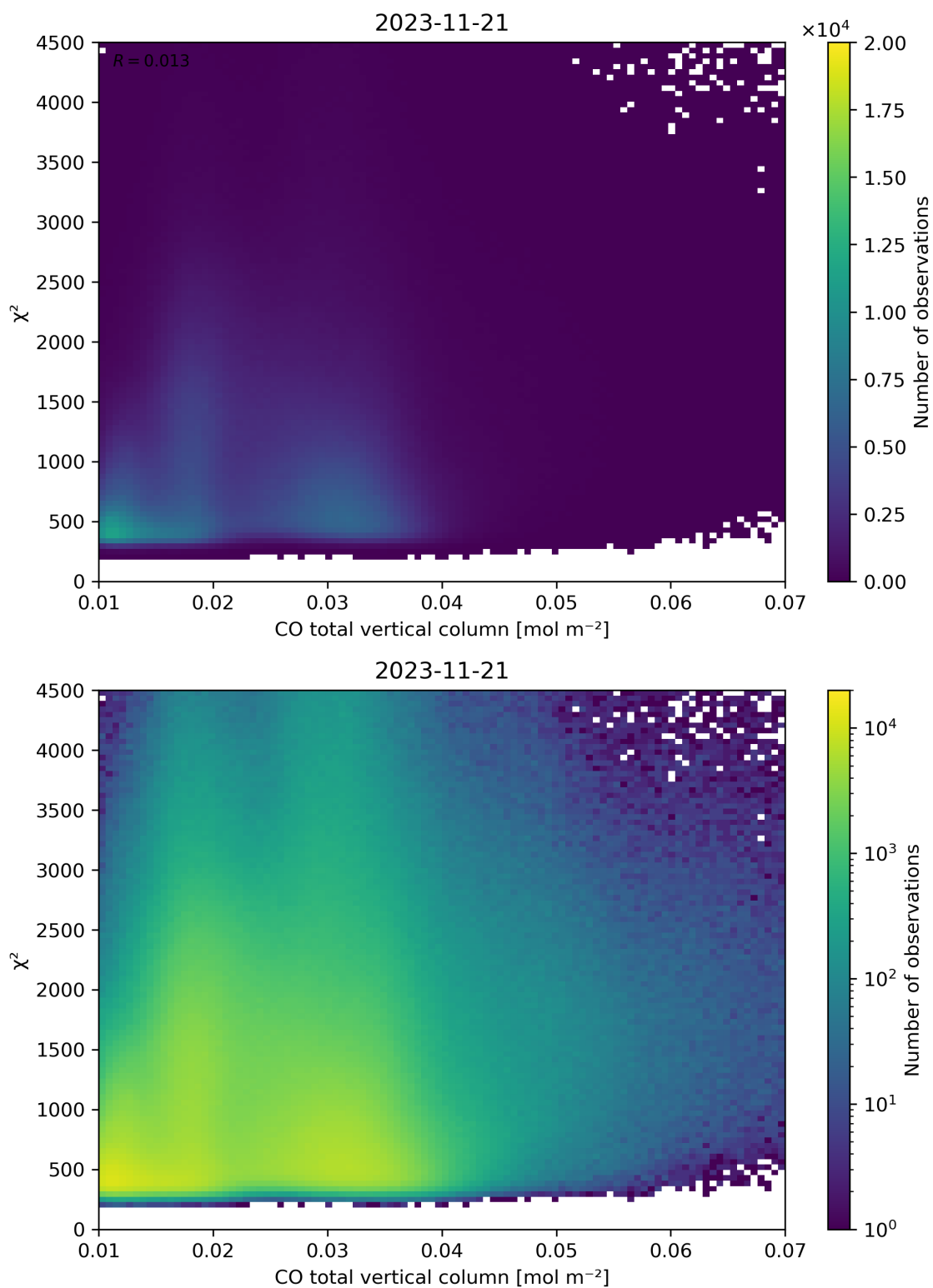
Figure 35: Scatter density plot of “CO total vertical column” against “ \chi^2 ” for 2023-11-20 to 2023-11-22.
