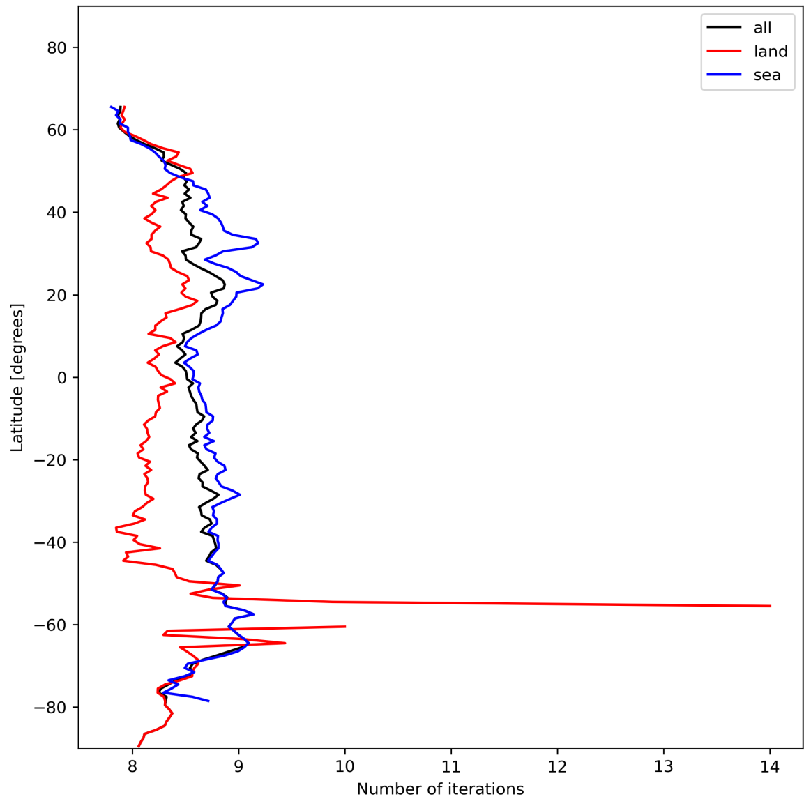
Figure 16: Zonal average of “Number of iterations” for 2023-11-20 to 2023-11-22.
