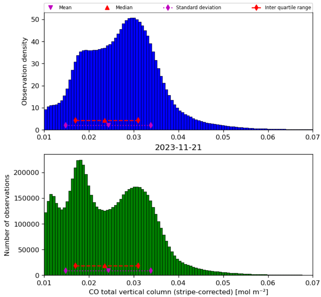
Figure 19: Histogram of “CO total vertical column (stripe-corrected)” for 2023-11-20 to 2023-11-22
