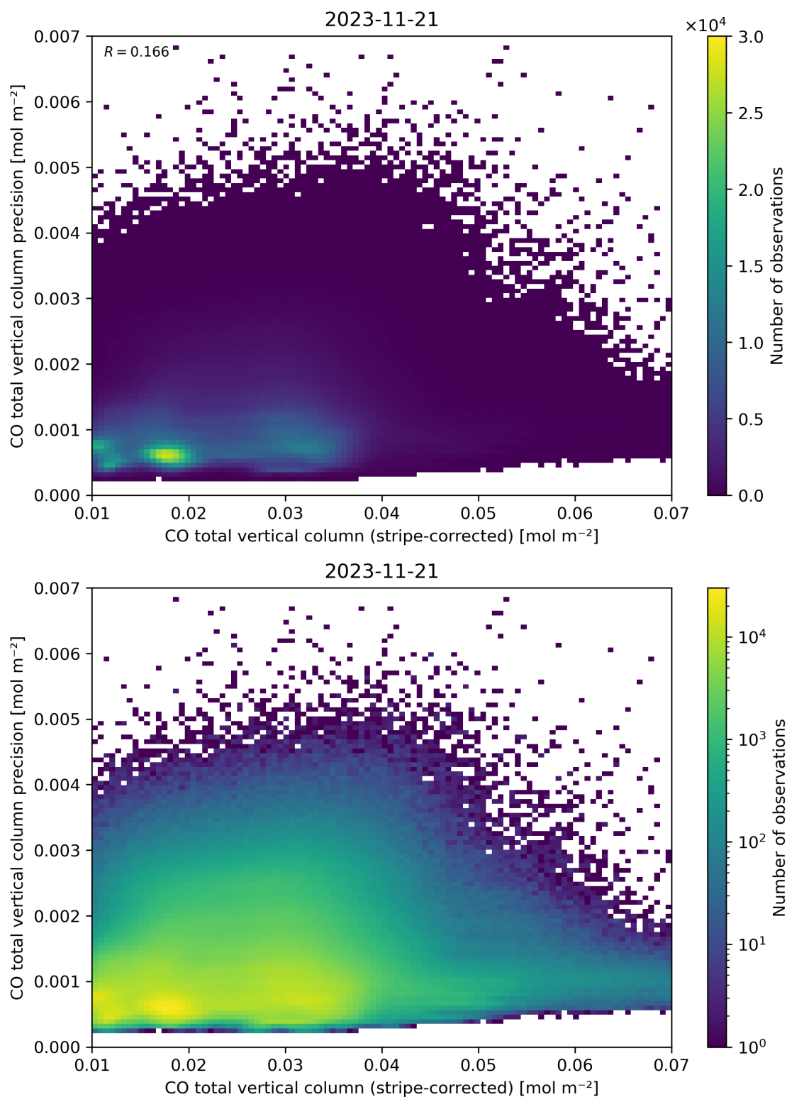
Figure 36: Scatter density plot of “CO total vertical column (stripe-corrected)” against “CO total vertical column precision” for 2023-11-20 to 2023-11-22.
