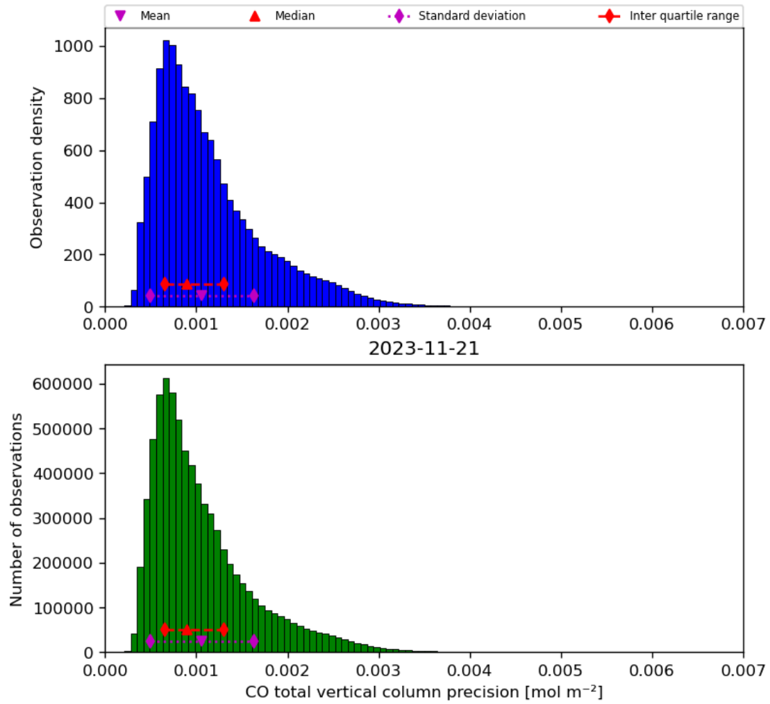
Figure 20: Histogram of “CO total vertical column precision” for 2023-11-20 to 2023-11-22
