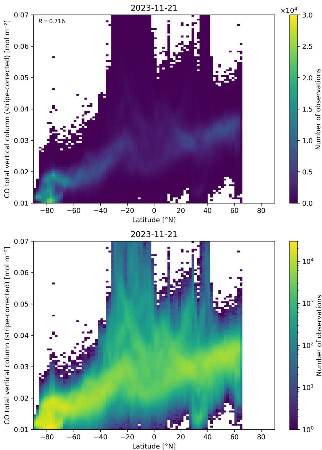
Figure 52: Scatter density plot of “Latitude” against “CO total vertical column (stripe-corrected)” for 2023-11-20 to 2023-11-22.
