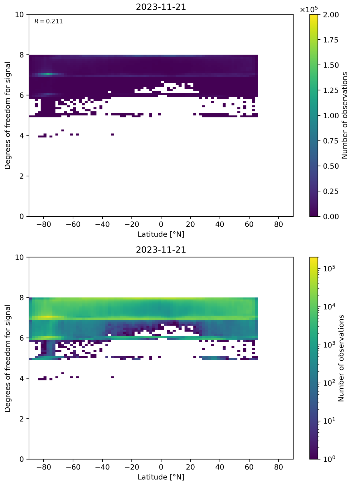
Figure 55: Scatter density plot of “Latitude” against “Degrees of freedom for signal” for 2023-11-20 to 2023-11-22.
