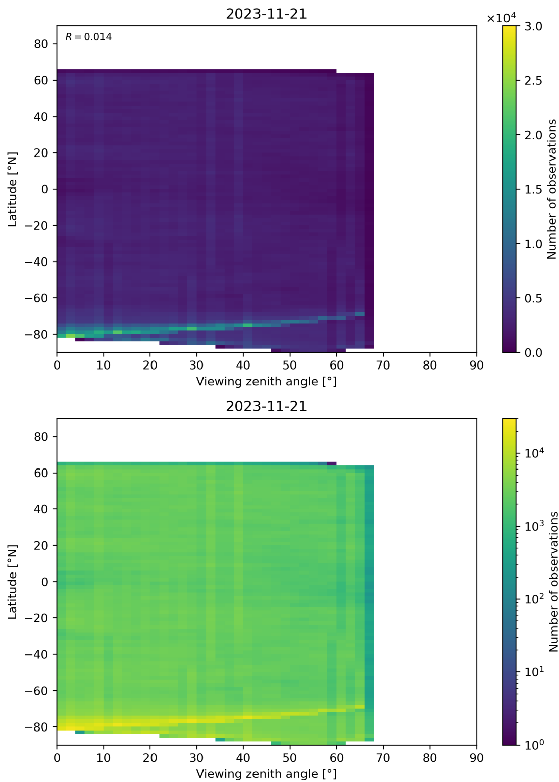
Figure 74: Scatter density plot of “Viewing zenith angle” against “Latitude” for 2023-11-20 to 2023-11-22.
