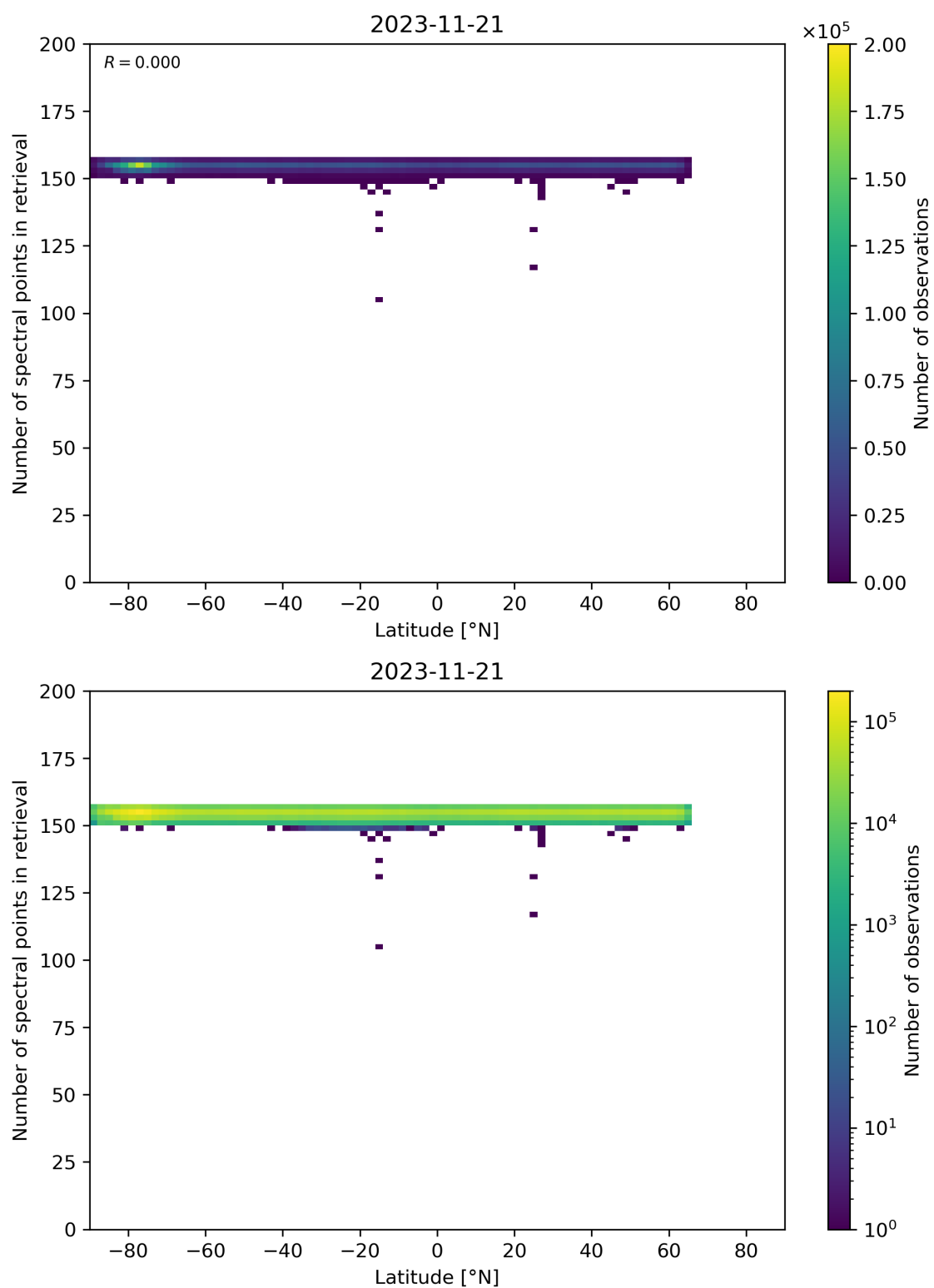
Figure 57: Scatter density plot of “Latitude” against “Number of spectral points in retrieval” for 2023-11-20 to 2023-11-22.
