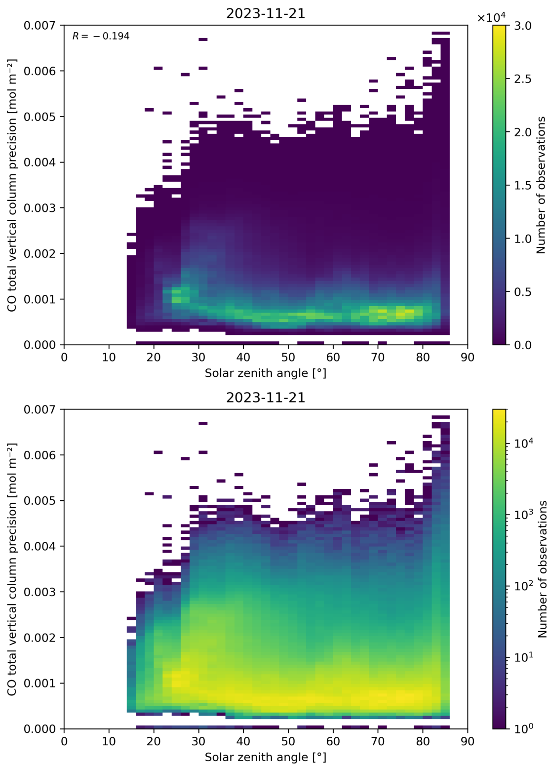
Figure 63: Scatter density plot of “Solar zenith angle” against “CO total vertical column precision” for 2023-11-20 to 2023-11-22.
