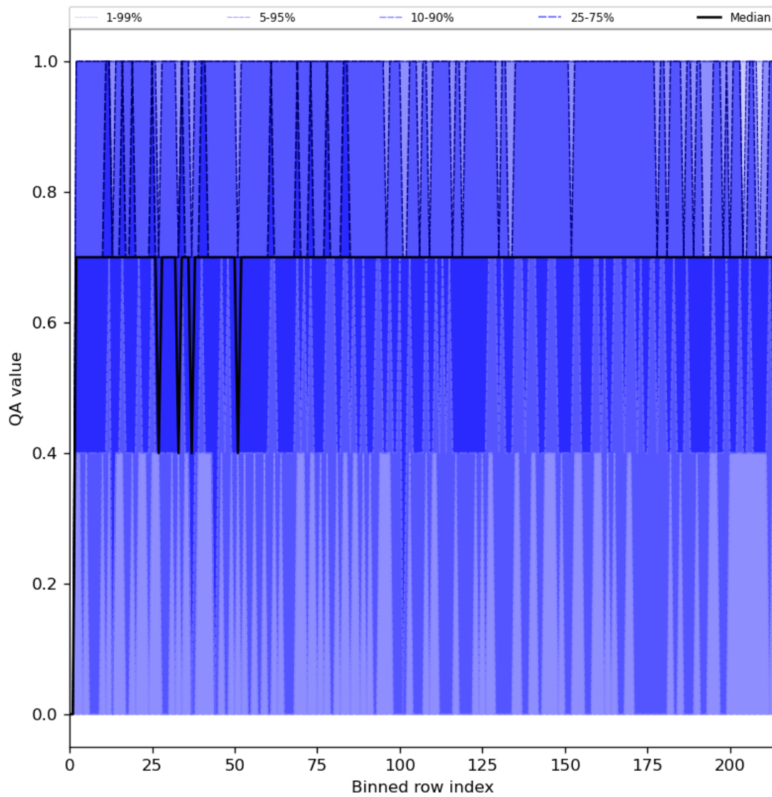
Figure 25: Along track statistics of “QA value” for 2023-11-20 to 2023-11-22
