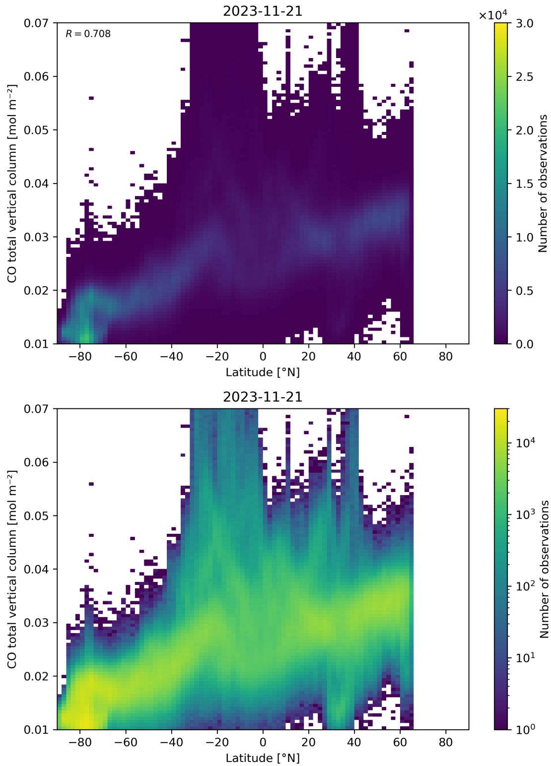
Figure 51: Scatter density plot of “Latitude” against “CO total vertical column” for 2023-11-20 to 2023-11-22.
