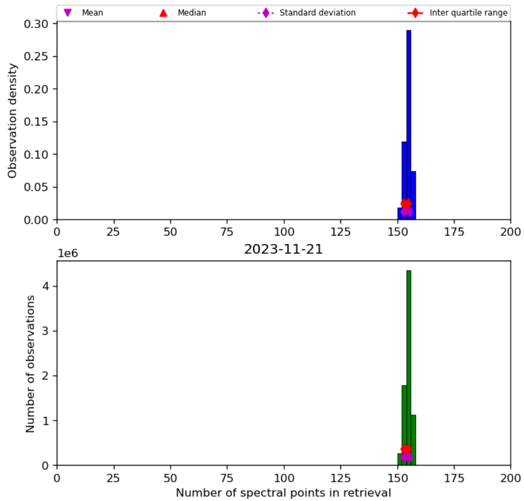
Figure 21: Histogram of “Number of spectral points in retrieval” for 2023-11-20 to 2023-11-22
