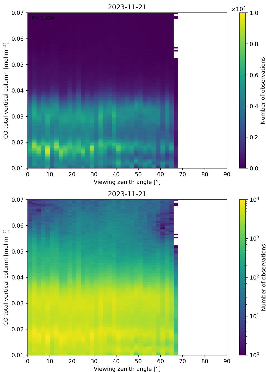
Figure 69: Scatter density plot of “Viewing zenith angle” against “CO total vertical column” for 2023-11-20 to 2023-11-22.
