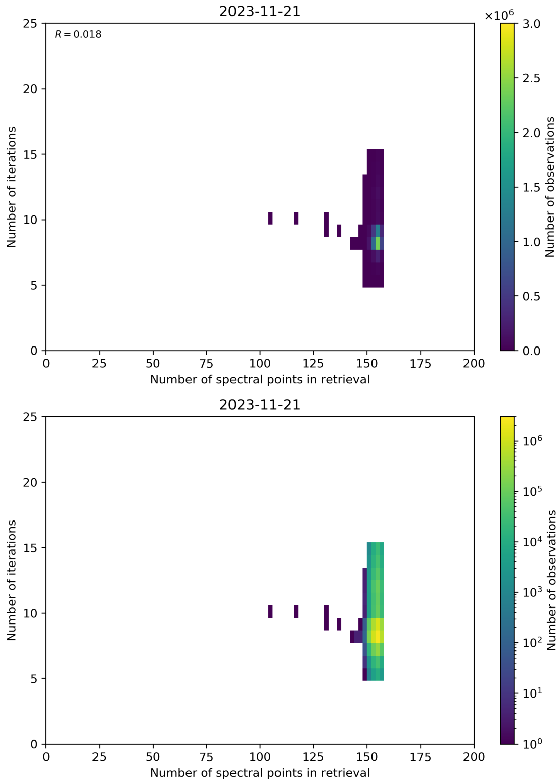
Figure 60: Scatter density plot of “Number of spectral points in retrieval” against “Number of iterations” for 2023-11-20 to 2023-11-22.
