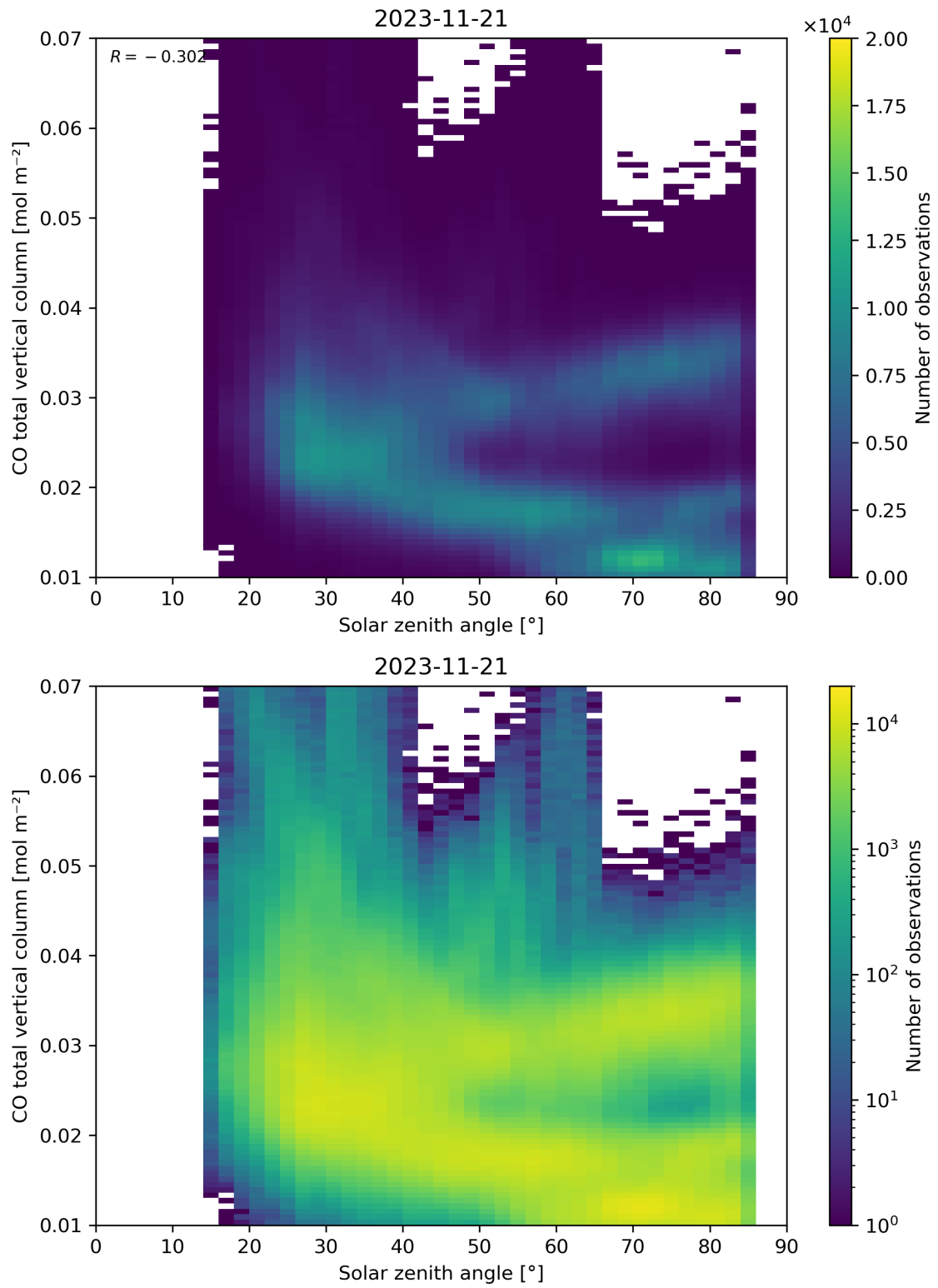
Figure 61: Scatter density plot of “Solar zenith angle” against “CO total vertical column” for 2023-11-20 to 2023-11-22.
