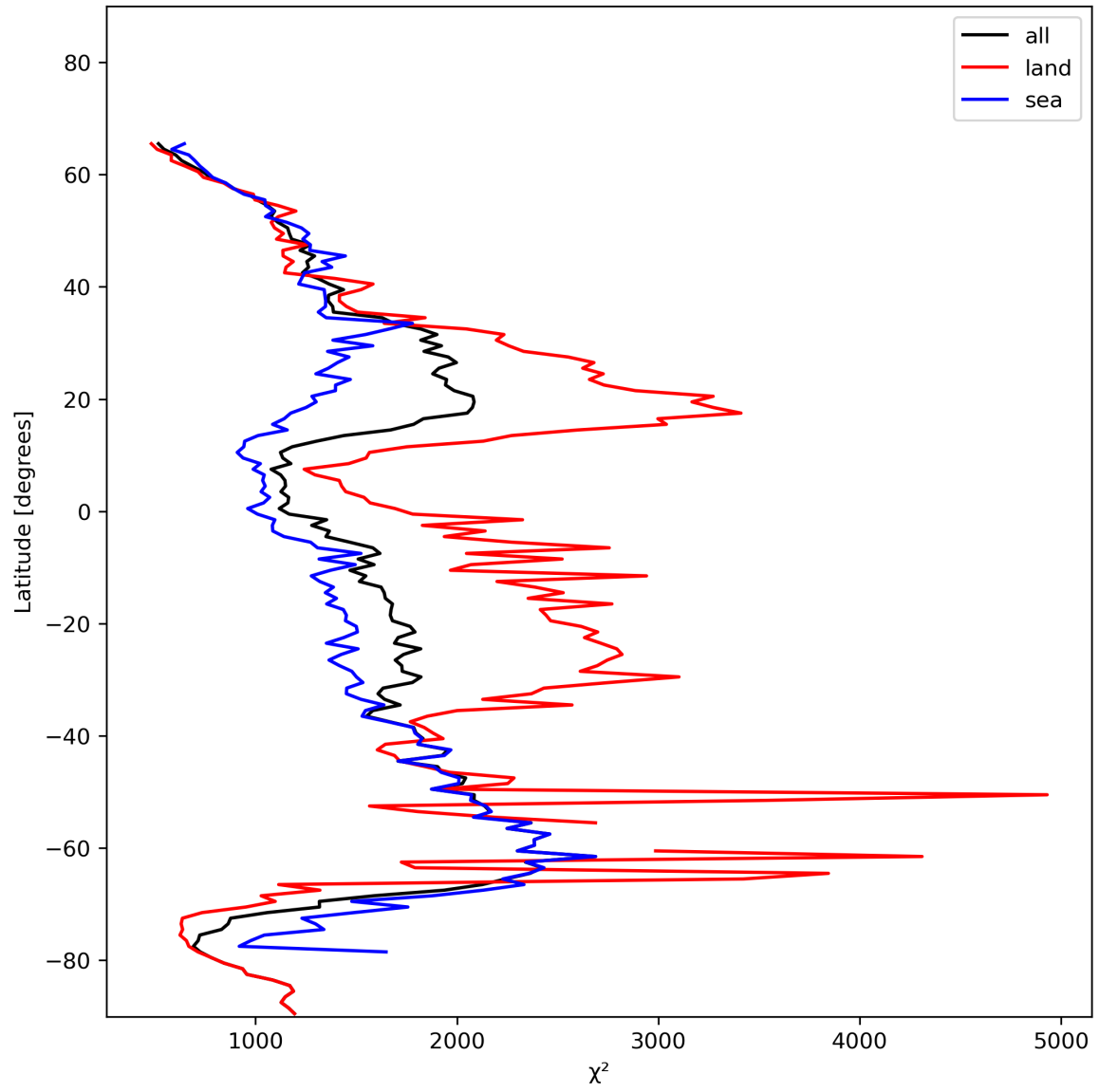
Figure 14: Zonal average of “ \chi^2 ” for 2023-11-20 to 2023-11-22.
