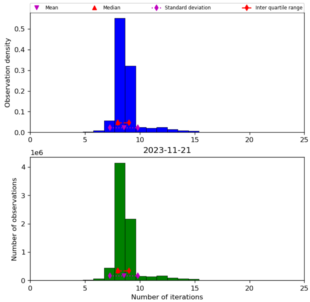
Figure 24: Histogram of “Number of iterations” for 2023-11-20 to 2023-11-22
