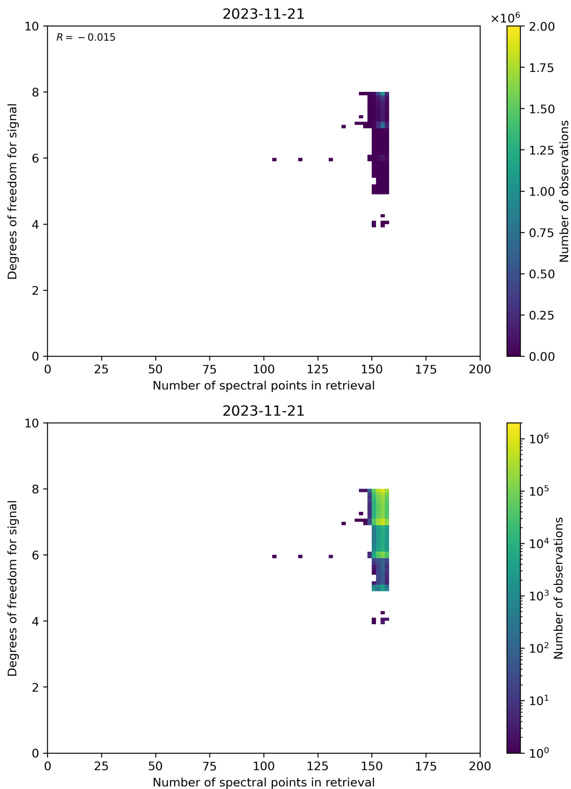
Figure 59: Scatter density plot of “Number of spectral points in retrieval” against “Degrees of freedom for signal” for 2023-11-20 to 2023-11-22.
