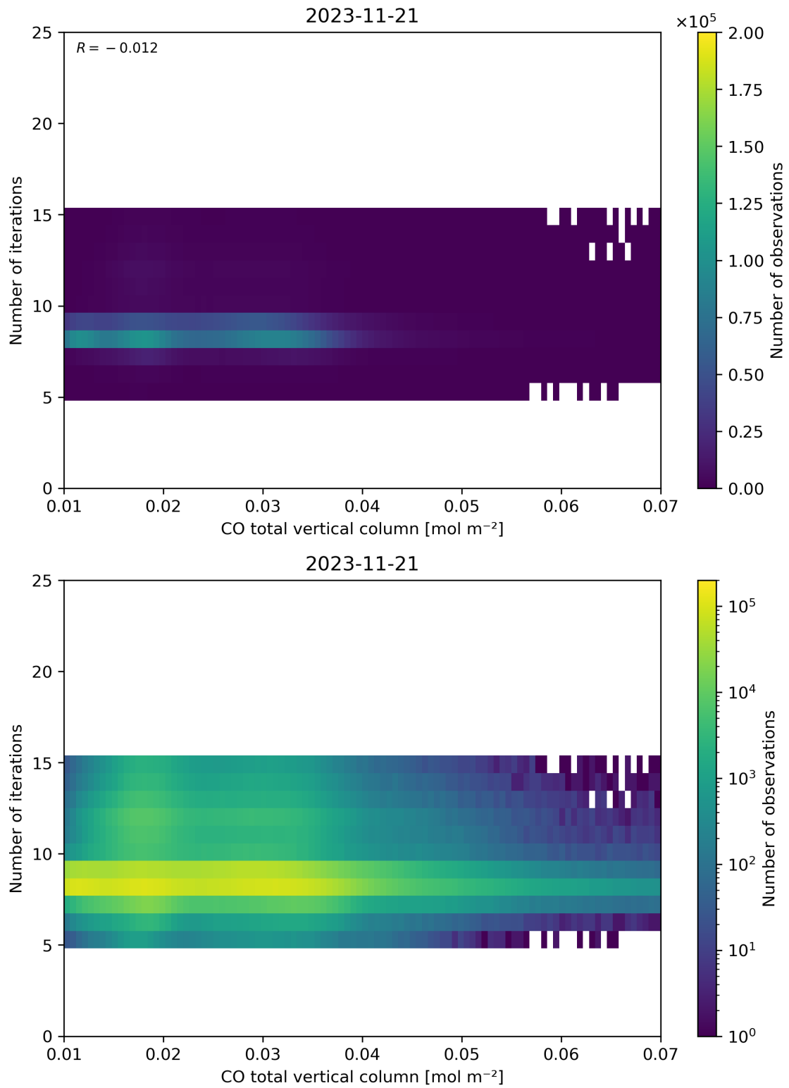
Figure 42: Scatter density plot of “CO total vertical column” against “Number of iterations” for 2023-11-20 to 2023-11-22.
