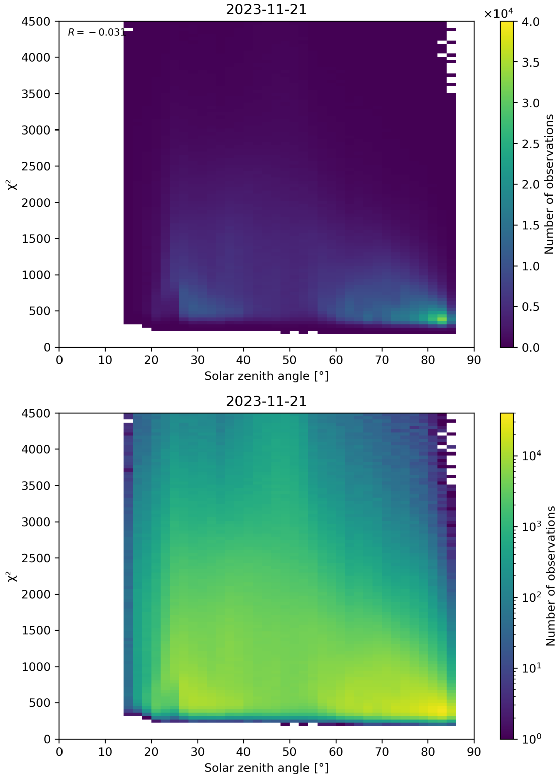
Figure 64: Scatter density plot of “Solar zenith angle” against “ \chi^2 ” for 2023-11-20 to 2023-11-22.
