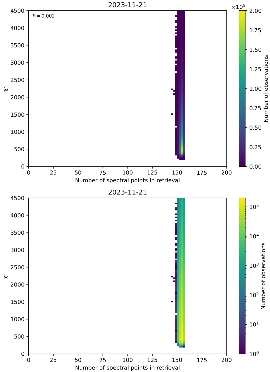
Figure 58: Scatter density plot of “Number of spectral points in retrieval” against “ \chi^2 ” for 2023-11-20 to 2023-11-22.
