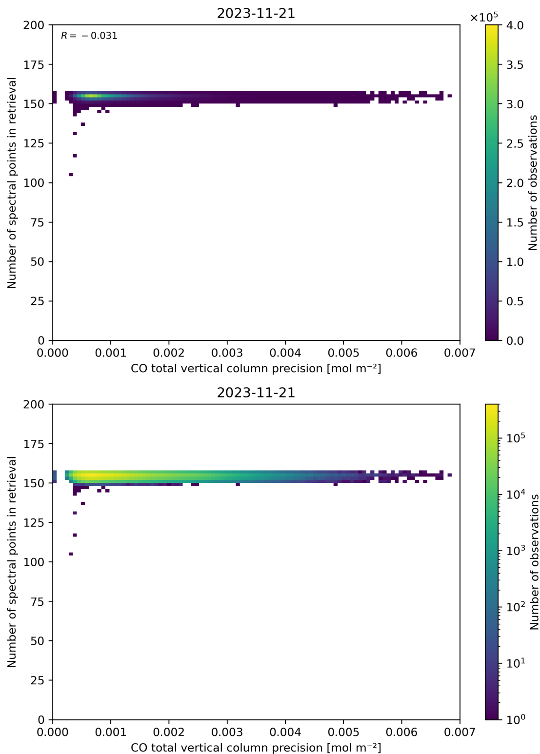
Figure 47: Scatter density plot of “CO total vertical column precision” against “Number of spectral points in retrieval” for 2023-11-20 to 2023-11-22.
