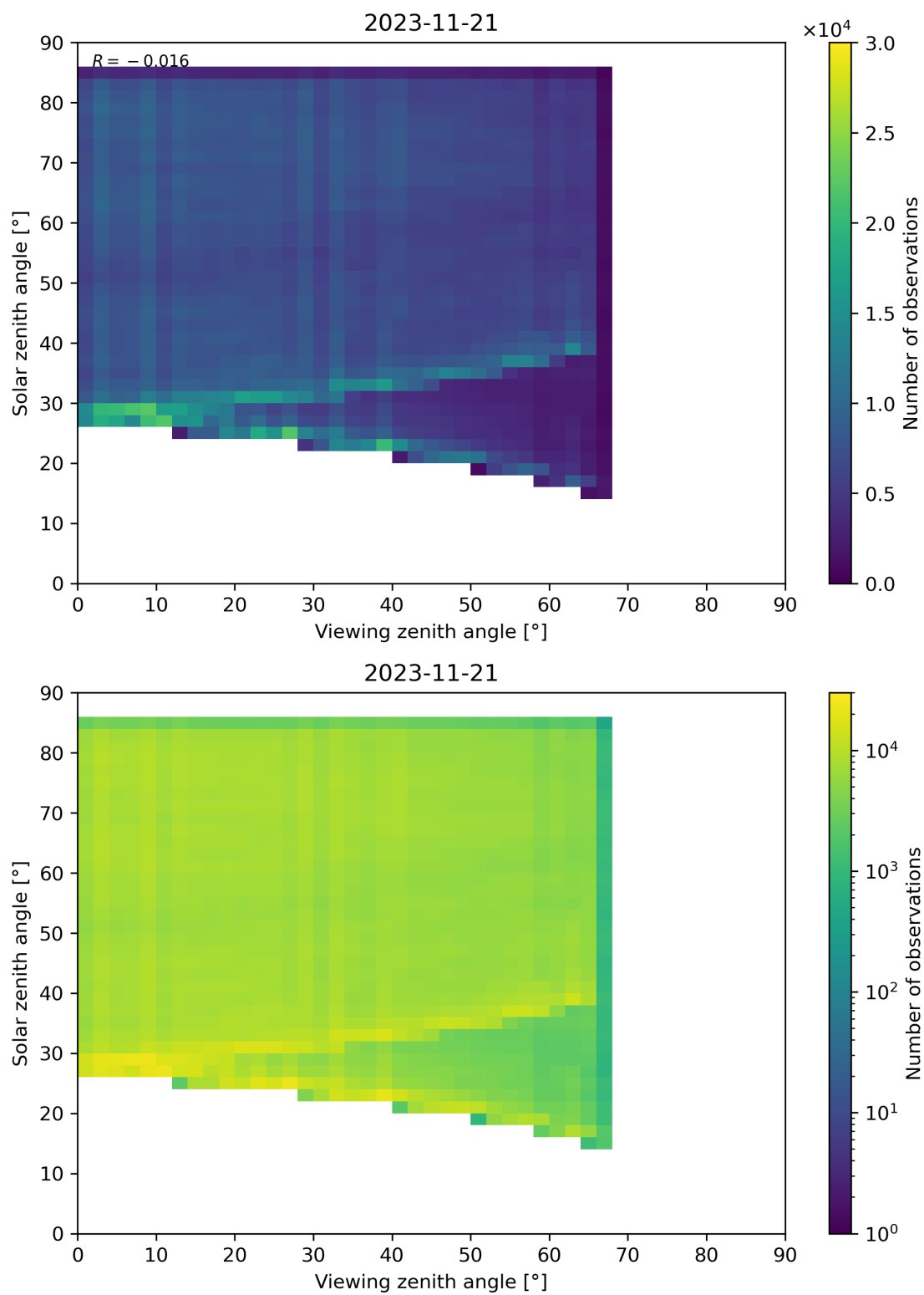
Figure 77: Scatter density plot of “Viewing zenith angle” against “Solar zenith angle” for 2023-11-20 to 2023-11-22.
