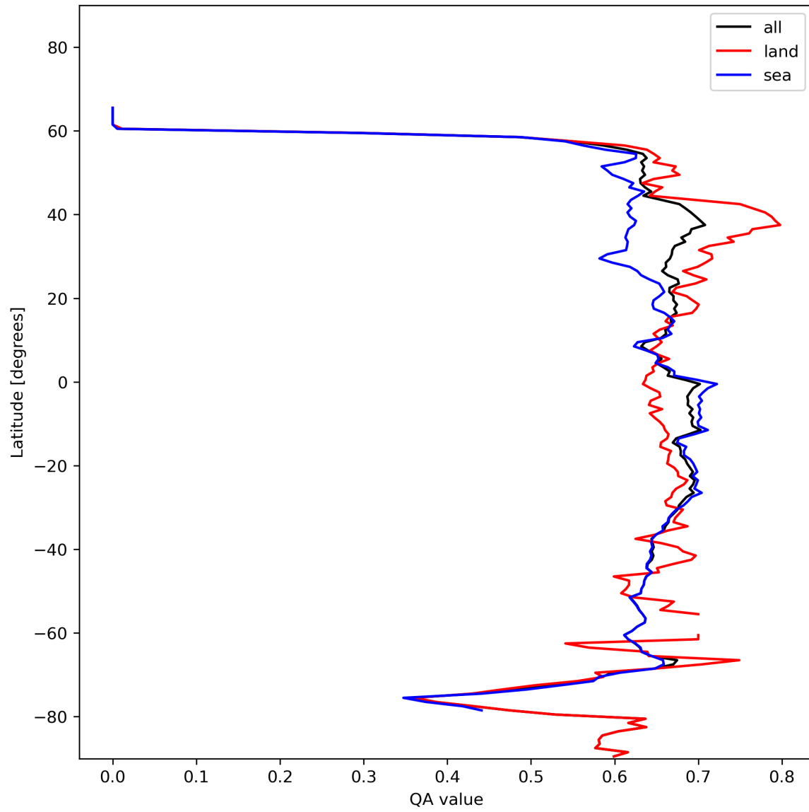
Figure 9: Zonal average of “QA value” for 2023-11-20 to 2023-11-22.
