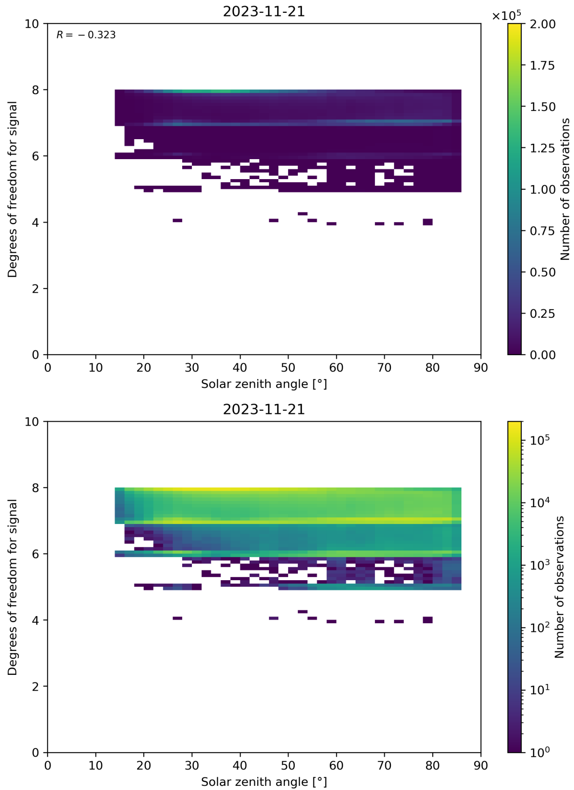
Figure 65: Scatter density plot of “Solar zenith angle” against “Degrees of freedom for signal” for 2023-11-20 to 2023-11-22.
