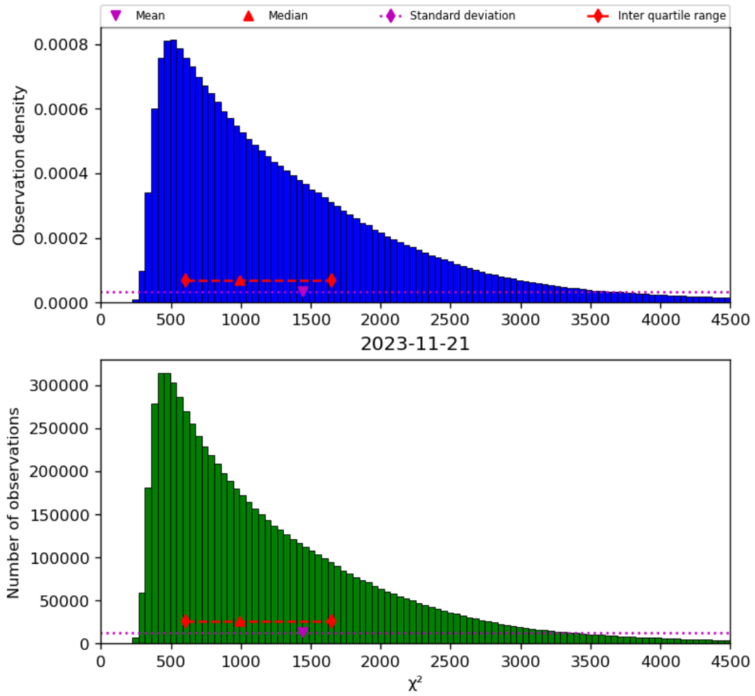
Figure 22: Histogram of “ \chi^2 ” for 2023-11-20 to 2023-11-22
