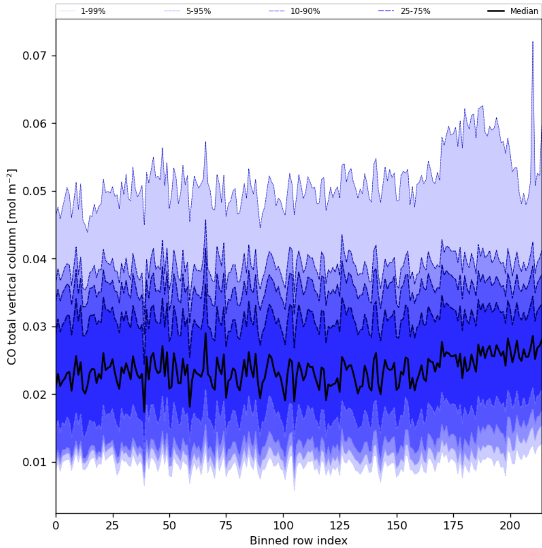
Figure 26: Along track statistics of “CO total vertical column” for 2023-11-20 to 2023-11-22
