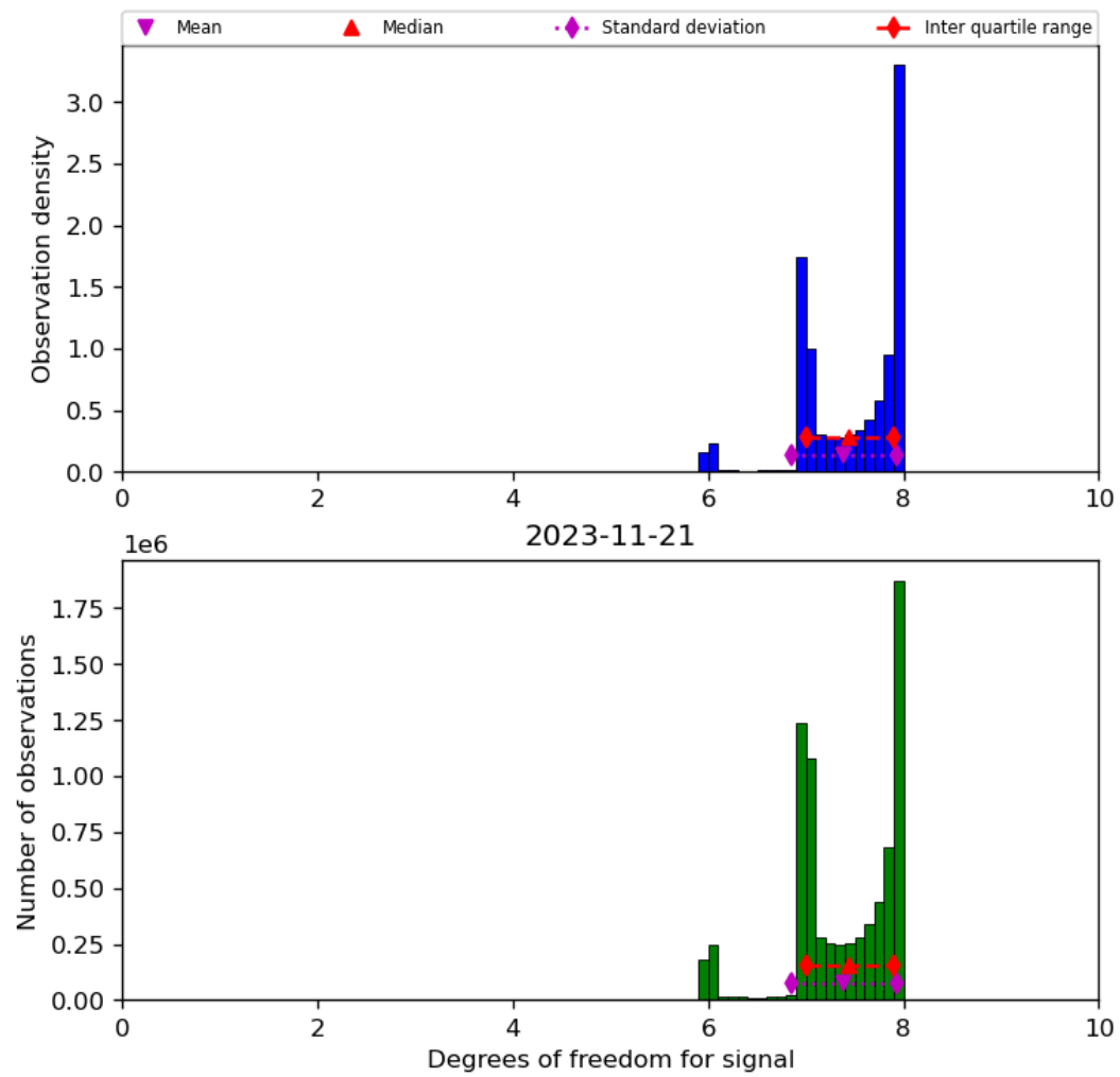
Figure 23: Histogram of “Degrees of freedom for signal” for 2023-11-20 to 2023-11-22
