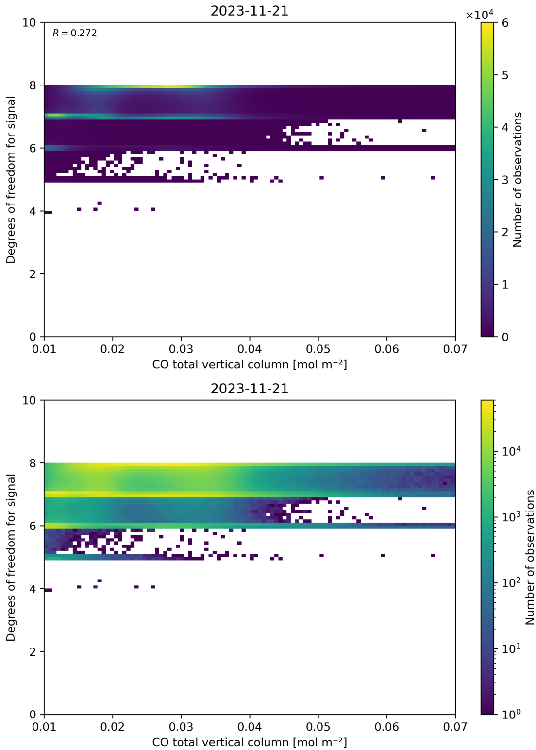
Figure 41: Scatter density plot of “CO total vertical column” against “Degrees of freedom for signal” for 2023-11-20 to 2023-11-22.
