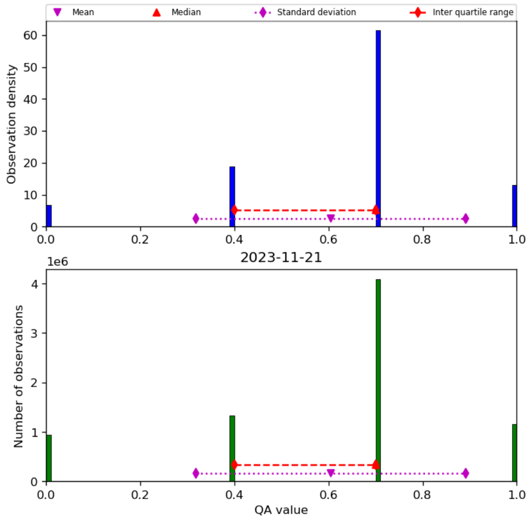
Figure 17: Histogram of “QA value” for 2023-11-20 to 2023-11-22
