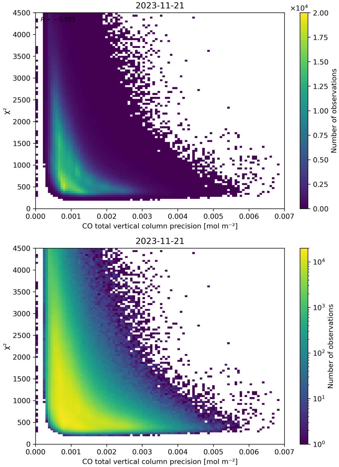
Figure 44: Scatter density plot of “CO total vertical column precision” against “ \chi^2 ” for 2023-11-20 to 2023-11-22.
