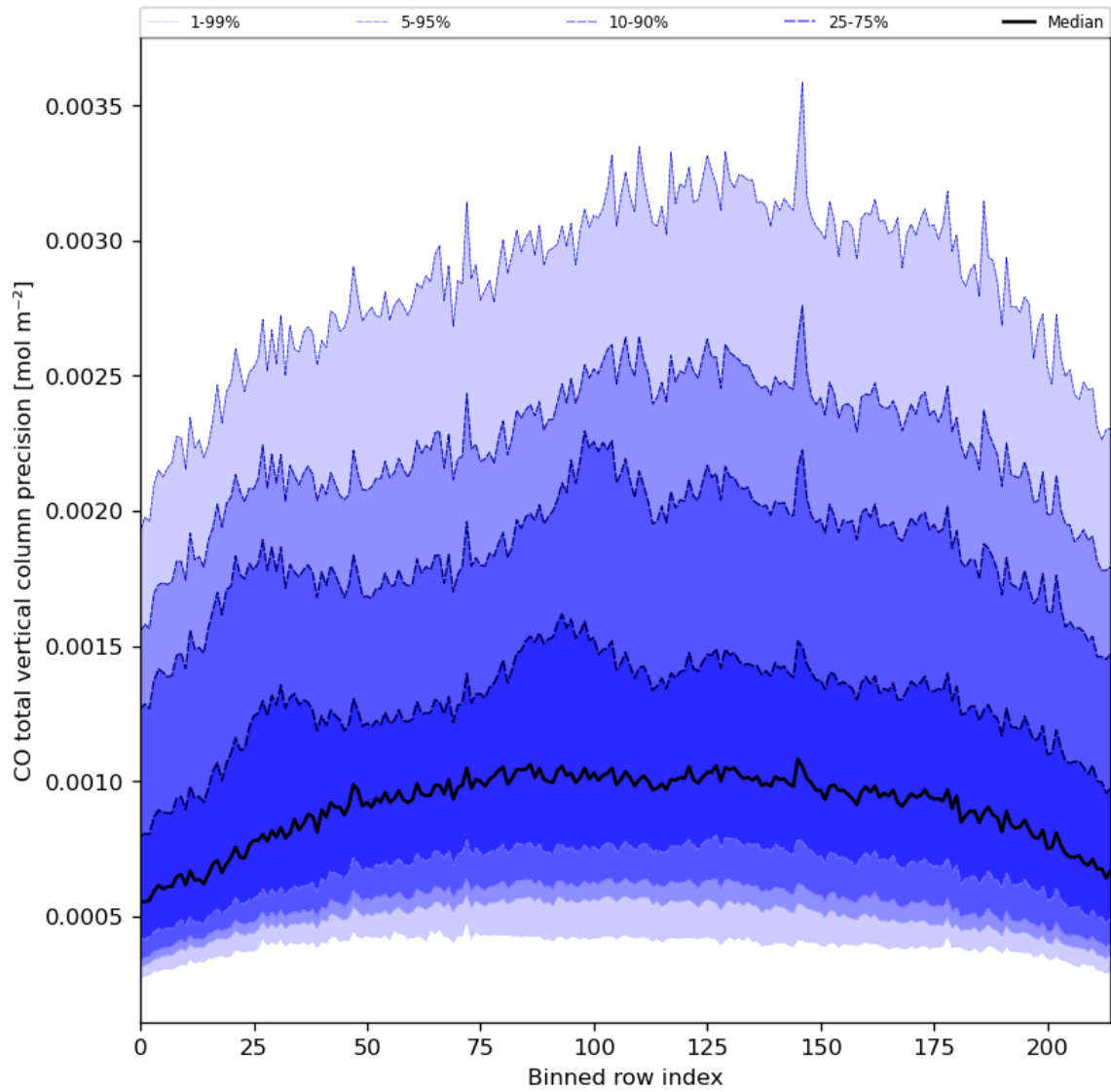
Figure 28: Along track statistics of “CO total vertical column precision” for 2023-11-20 to 2023-11-22
