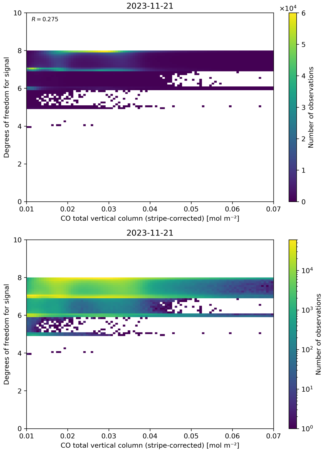
Figure 38: Scatter density plot of “CO total vertical column (stripe-corrected)” against “Degrees of freedom for signal” for 2023-11-20 to 2023-11-22.
