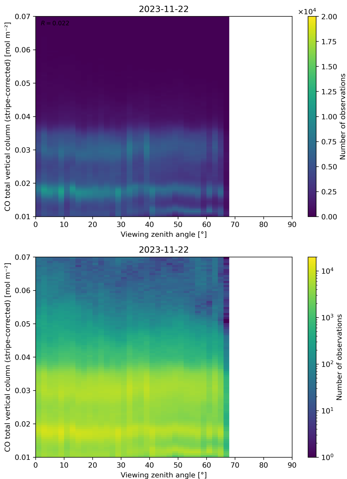
Figure 70: Scatter density plot of “Viewing zenith angle” against “CO total vertical column (stripe-corrected)” for 2023-11-21 to 2023-11-23.
