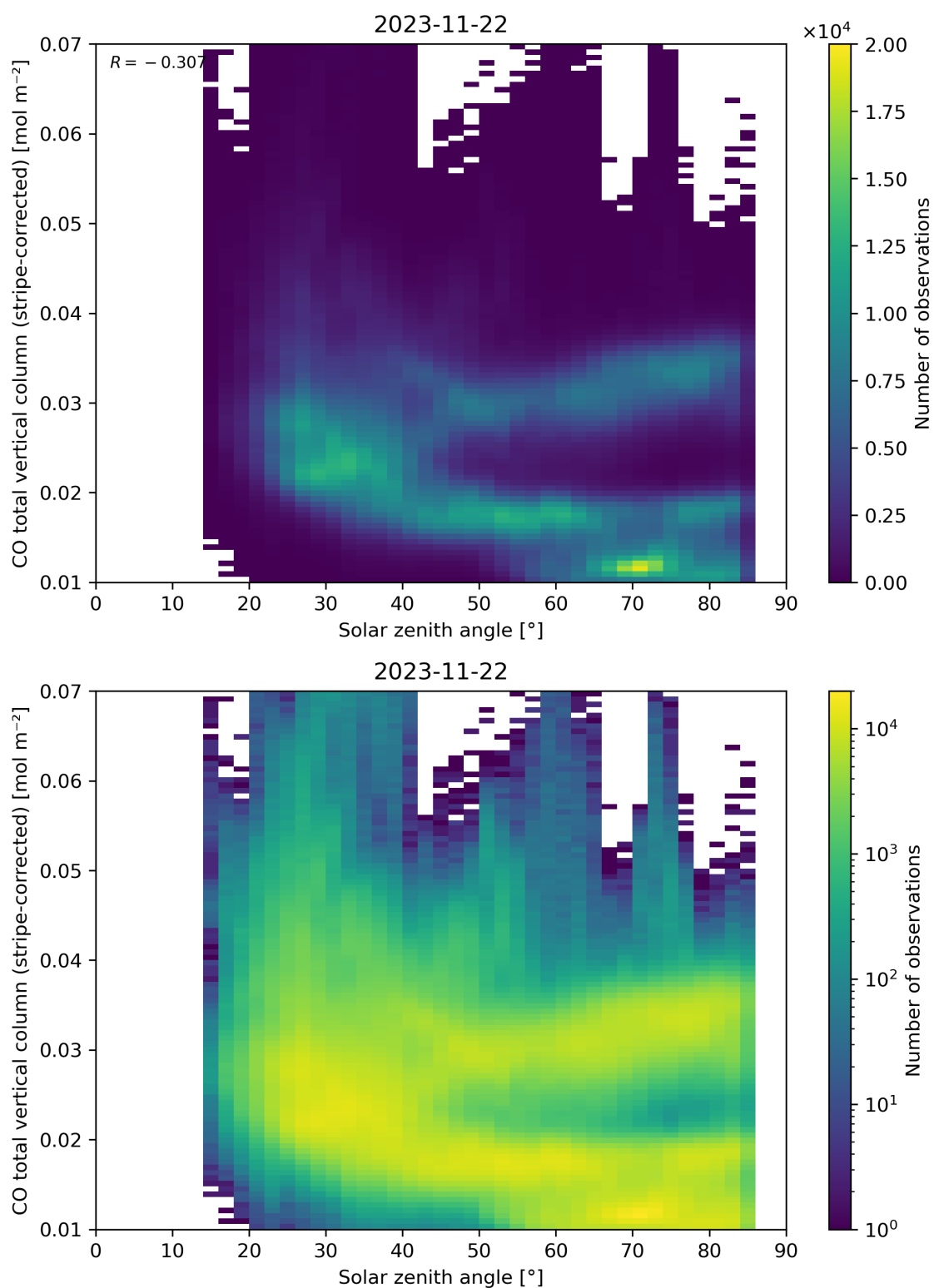
Figure 62: Scatter density plot of “Solar zenith angle” against “CO total vertical column (stripe-corrected)” for 2023-11-21 to 2023-11-23.
