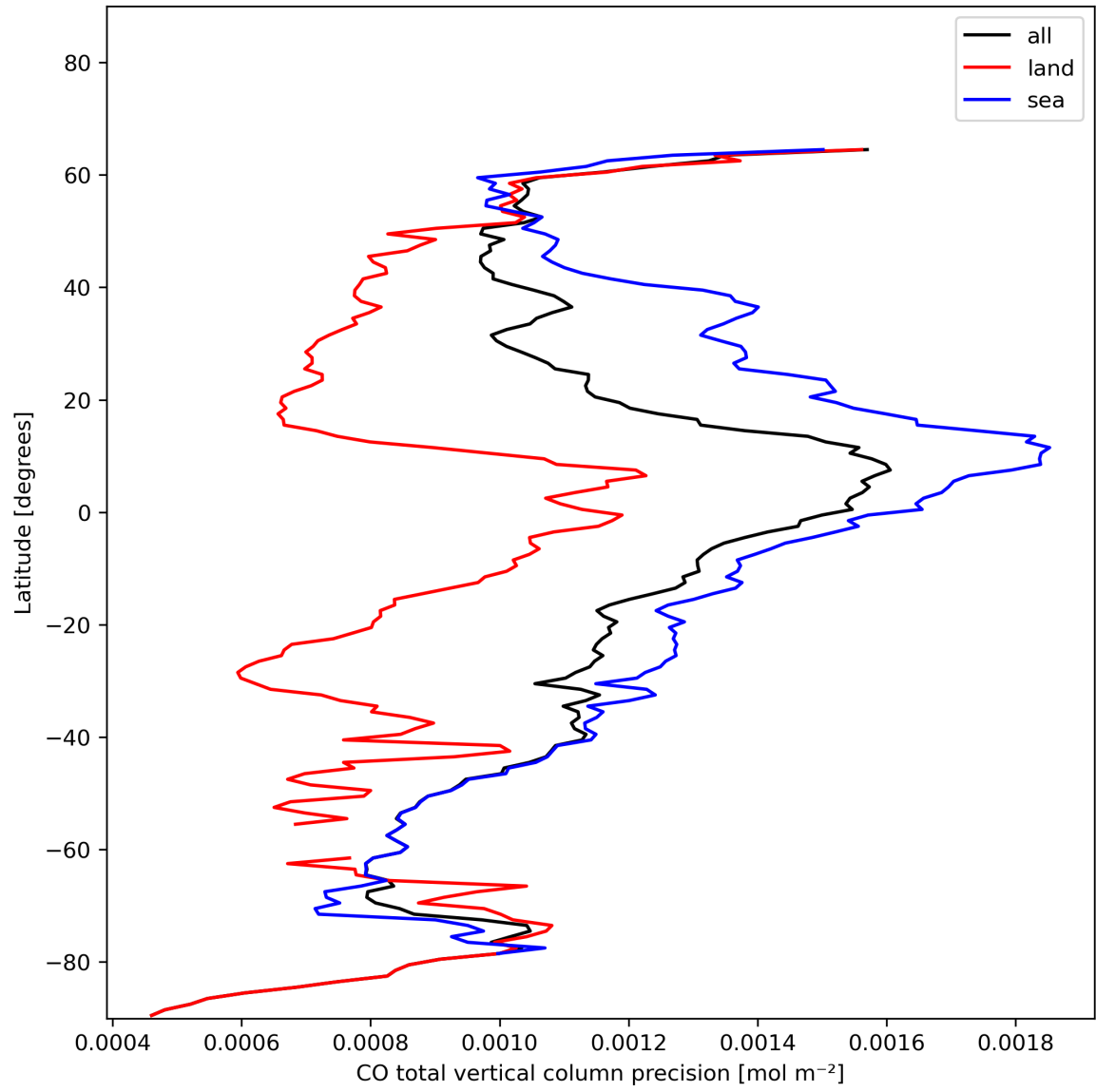
Figure 12: Zonal average of “CO total vertical column precision” for 2023-11-21 to 2023-11-23.
