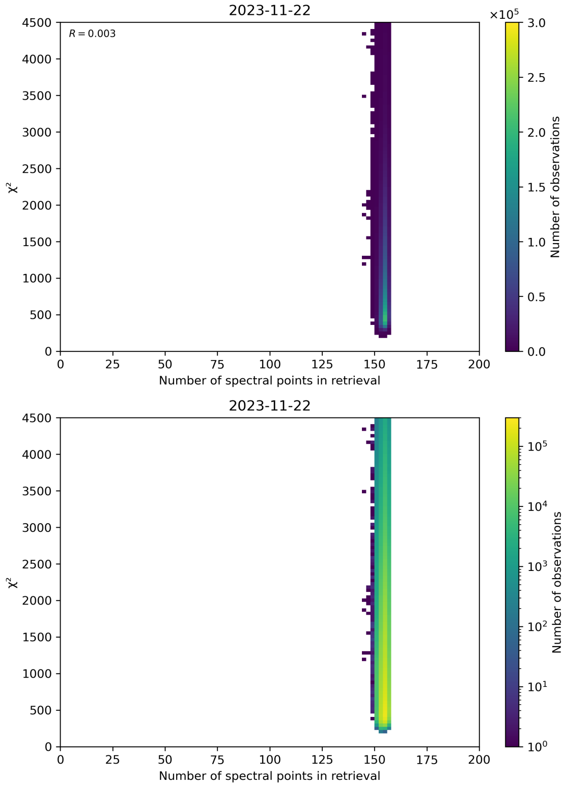
Figure 58: Scatter density plot of “Number of spectral points in retrieval” against “ \chi^2 ” for 2023-11-21 to 2023-11-23.
