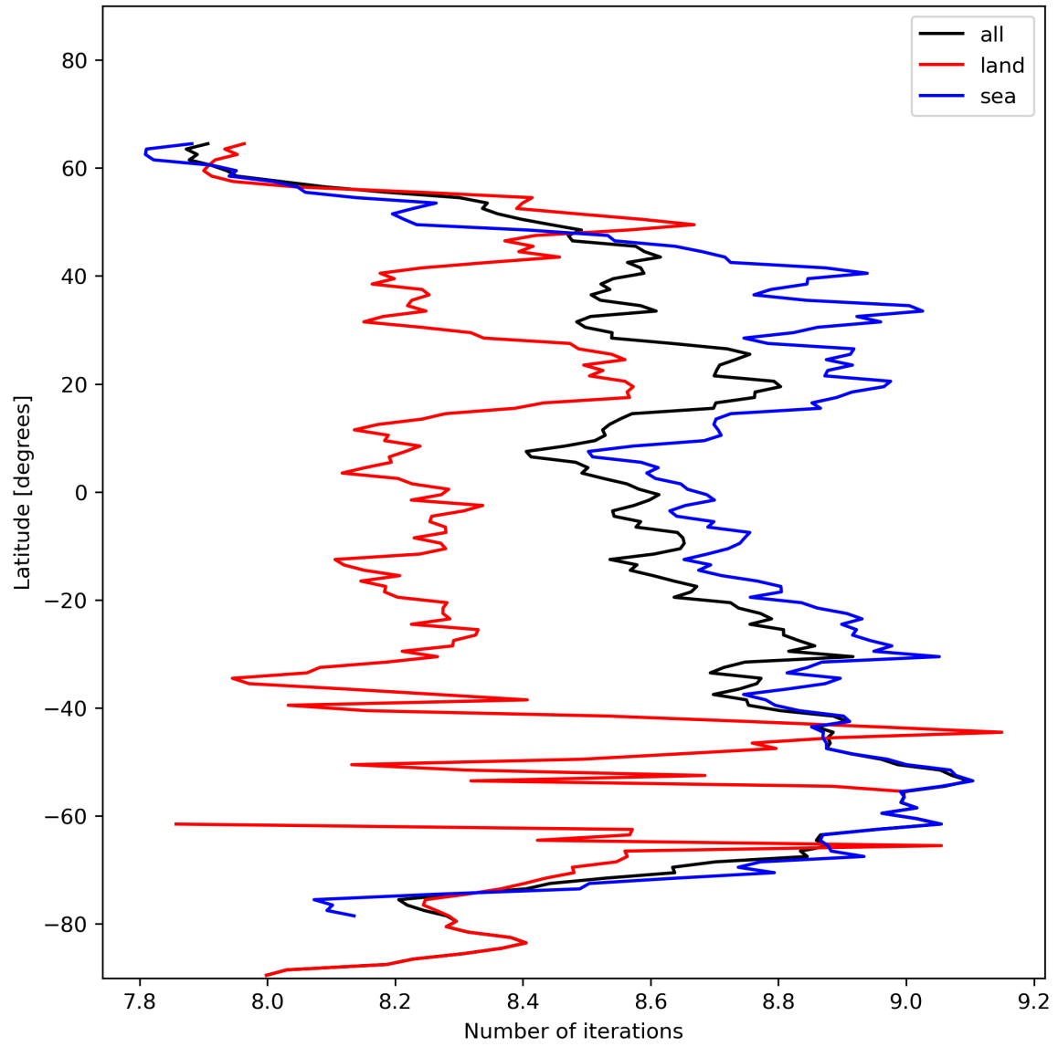
Figure 16: Zonal average of “Number of iterations” for 2023-11-21 to 2023-11-23.
