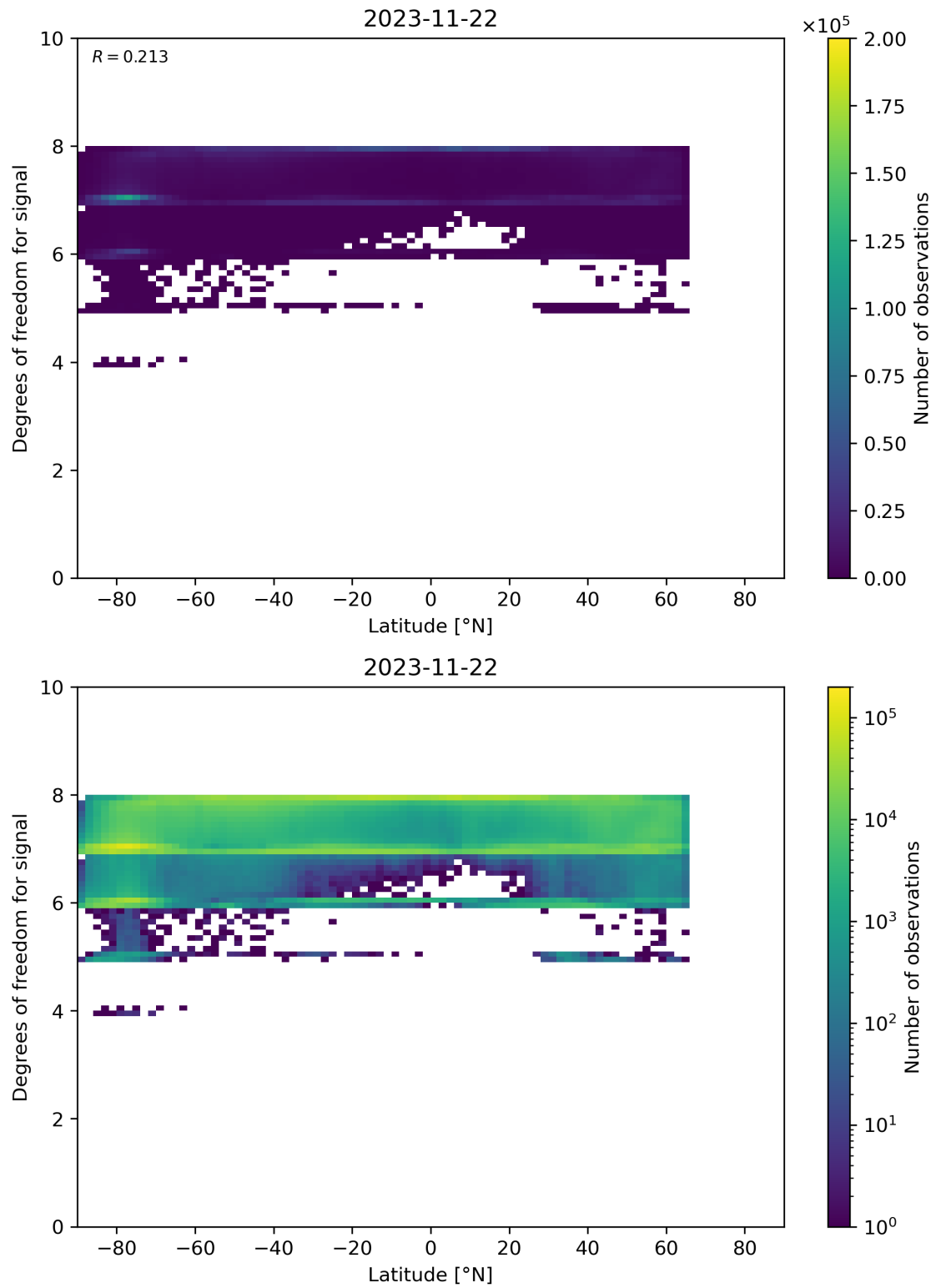
Figure 55: Scatter density plot of “Latitude” against “Degrees of freedom for signal” for 2023-11-21 to 2023-11-23.
