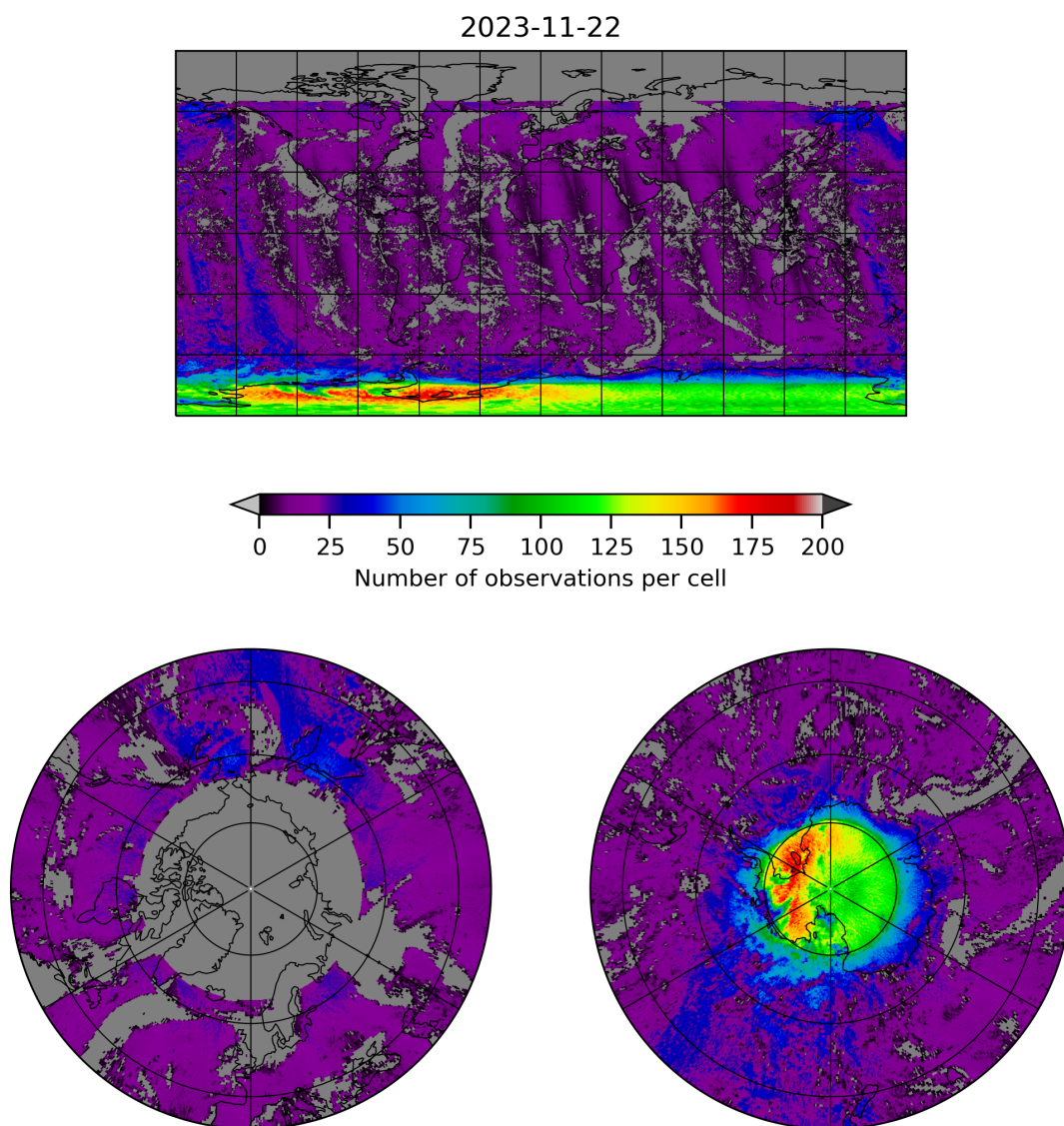
Figure 8: Map of the number of observations for 2023-11-21 to 2023-11-23
