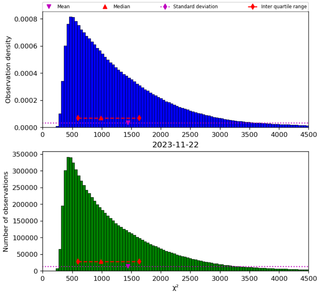
Figure 22: Histogram of “ \chi^2 ” for 2023-11-21 to 2023-11-23
