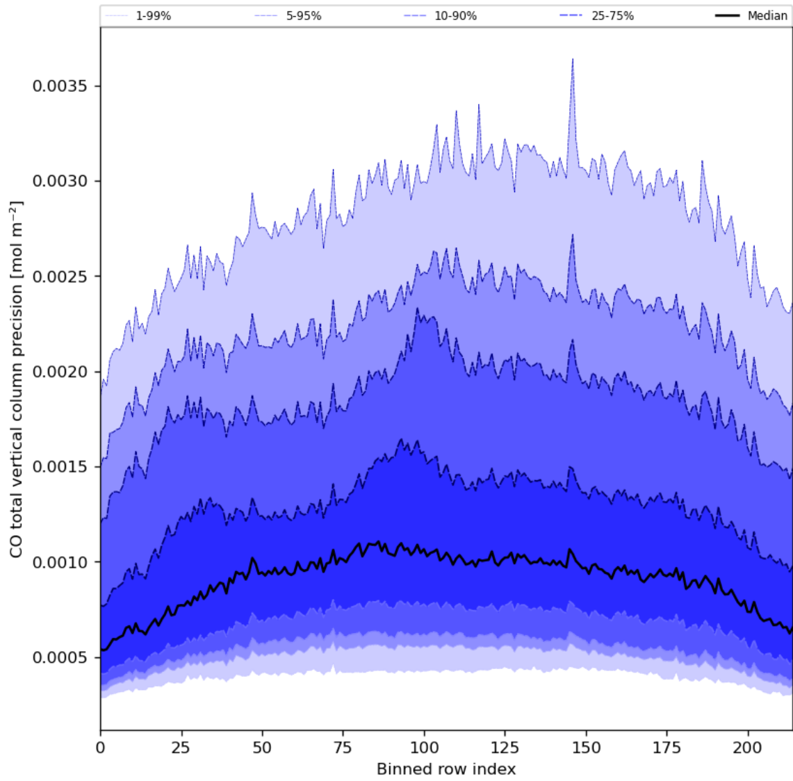
Figure 28: Along track statistics of “CO total vertical column precision” for 2023-11-21 to 2023-11-23
