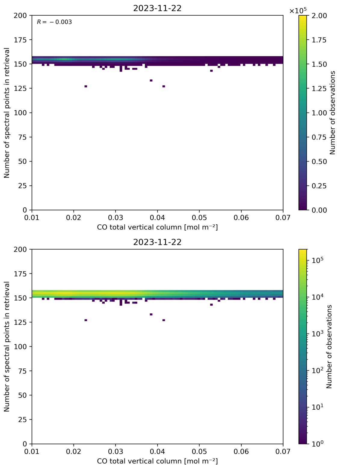
Figure 43: Scatter density plot of “CO total vertical column” against “Number of spectral points in retrieval” for 2023-11-21 to 2023-11-23.
