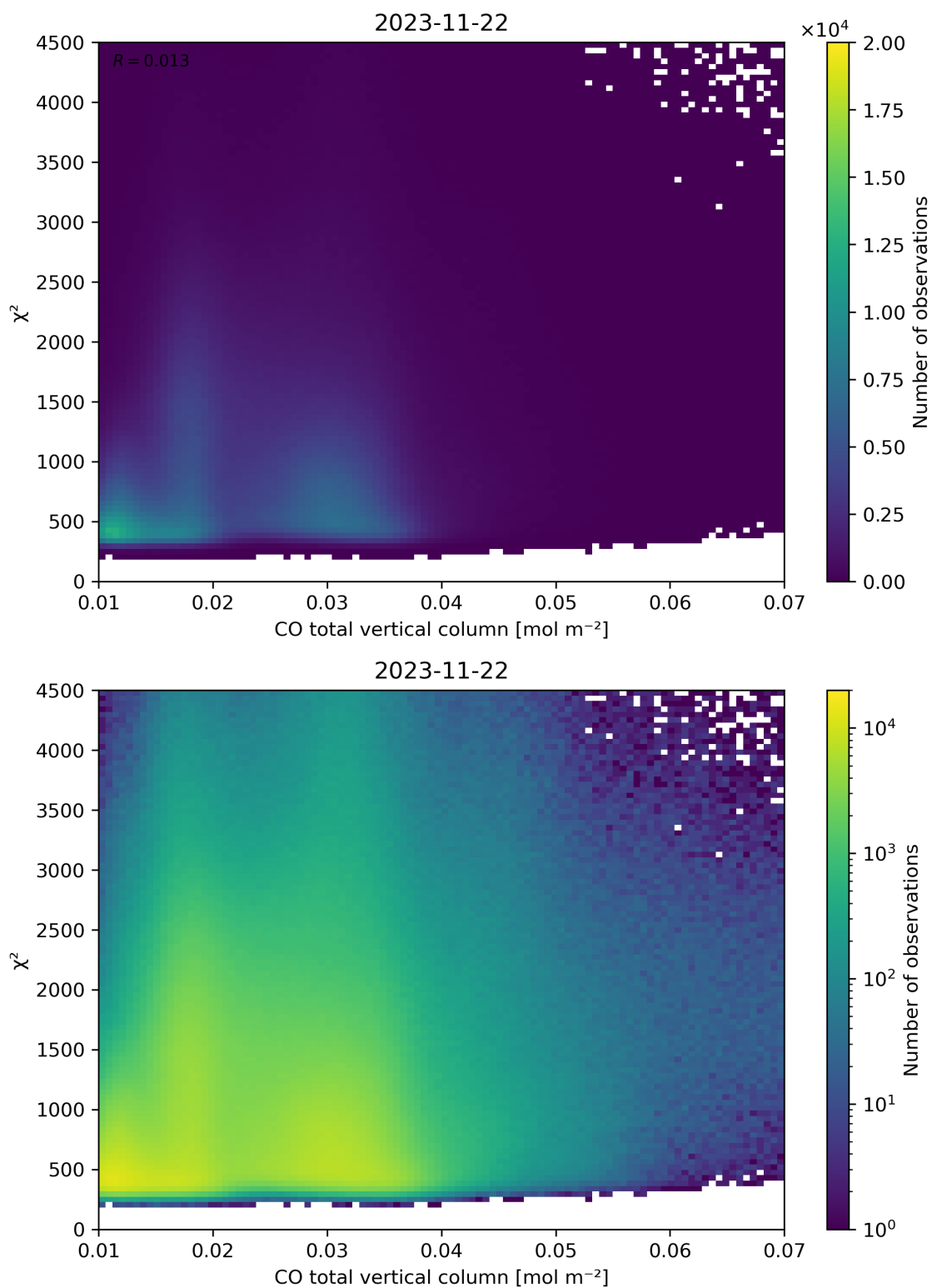
Figure 35: Scatter density plot of “CO total vertical column” against “ \chi^2 ” for 2023-11-21 to 2023-11-23.
