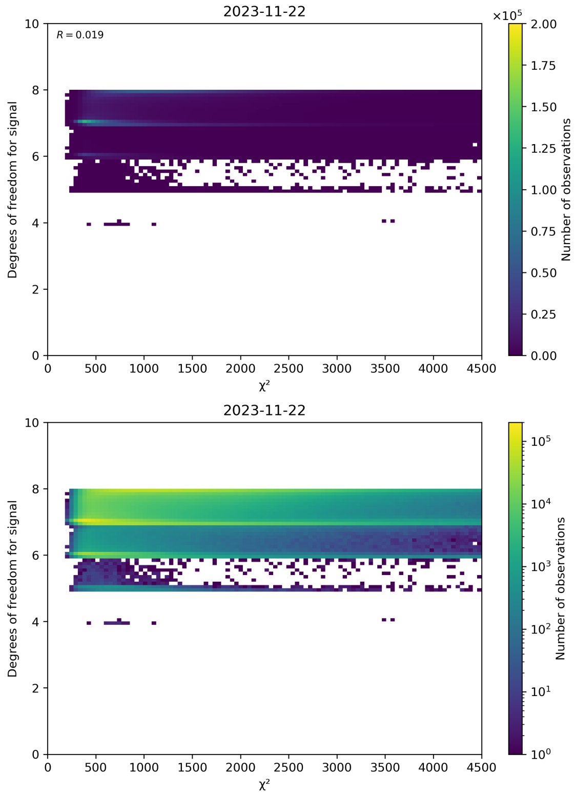
Figure 48: Scatter density plot of “ \chi^2 ” against “Degrees of freedom for signal” for 2023-11-21 to 2023-11-23.
