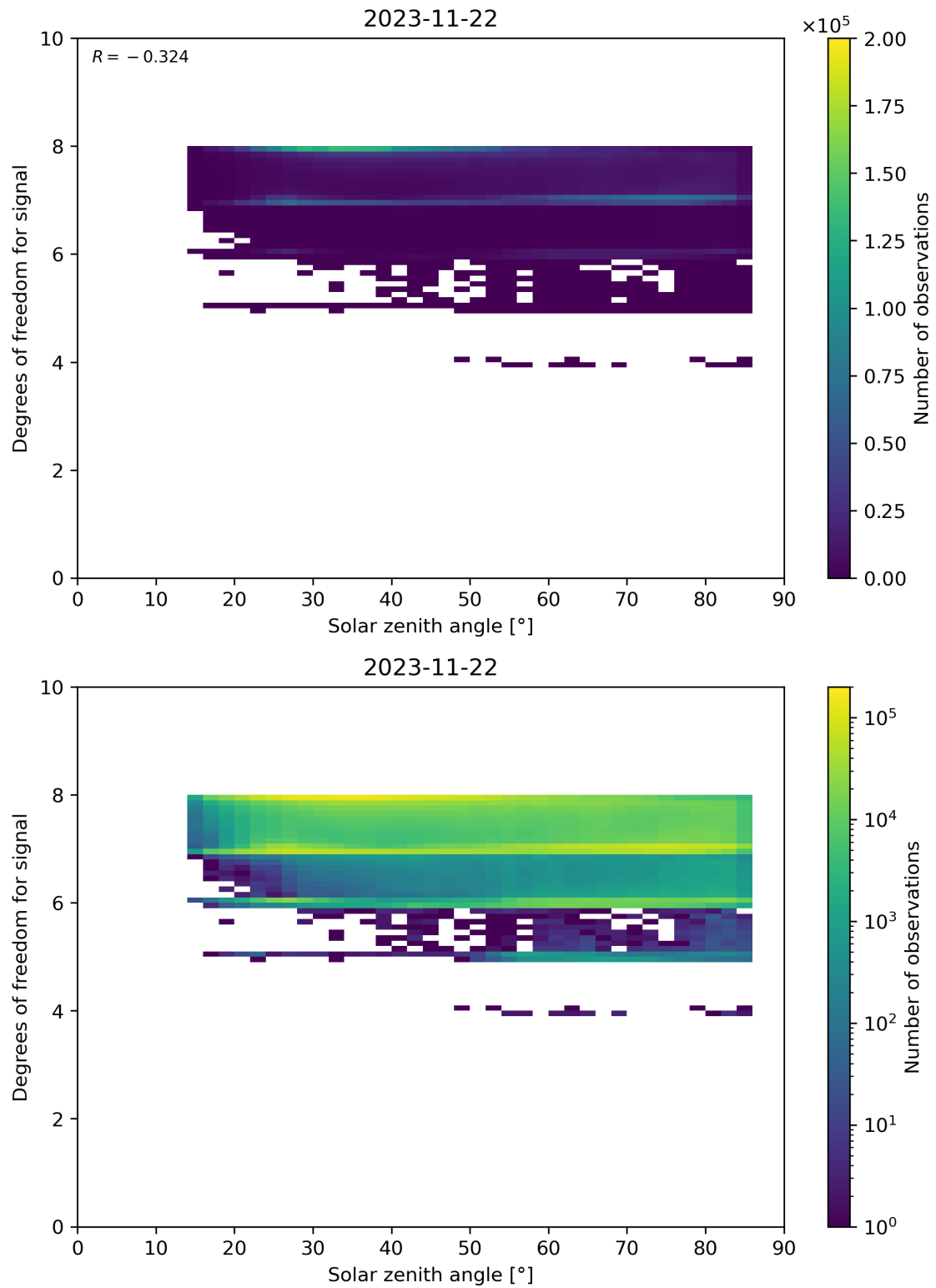
Figure 65: Scatter density plot of “Solar zenith angle” against “Degrees of freedom for signal” for 2023-11-21 to 2023-11-23.
