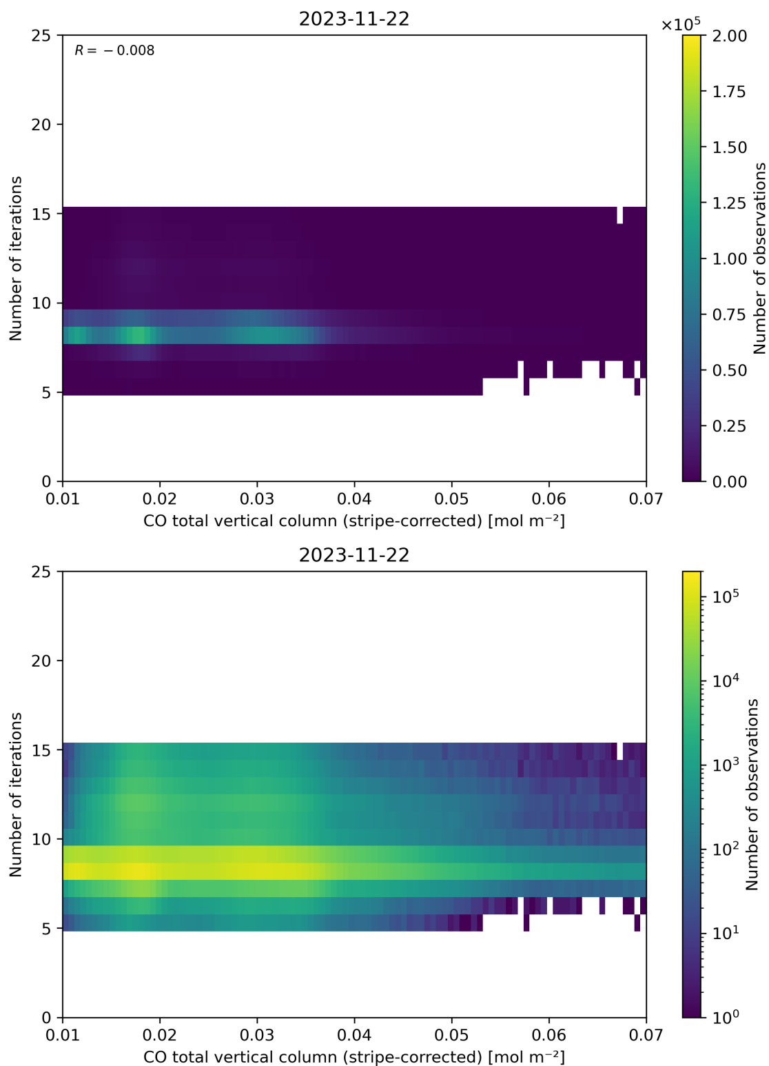
Figure 39: Scatter density plot of “CO total vertical column (stripe-corrected)” against “Number of iterations” for 2023-11-21 to 2023-11-23.
