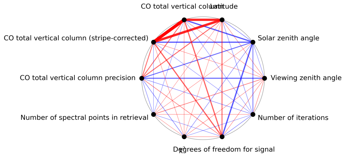
Figure 1: Map of correlation graph for 2023-11-21 to 2023-11-23.
