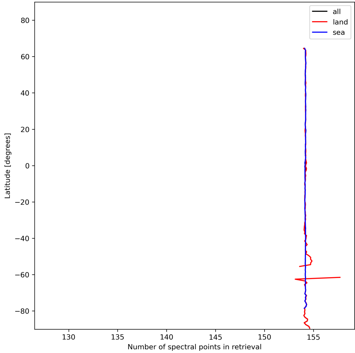
Figure 13: Zonal average of “Number of spectral points in retrieval” for 2023-11-21 to 2023-11-23.
