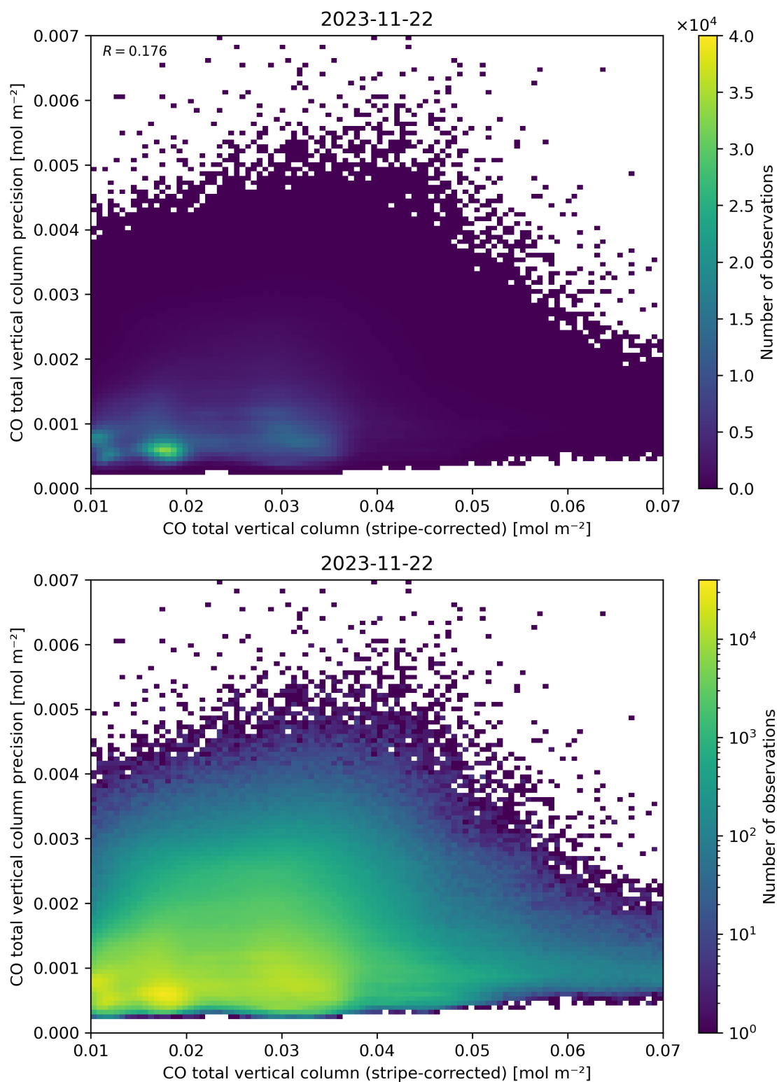
Figure 36: Scatter density plot of “CO total vertical column (stripe-corrected)” against “CO total vertical column precision” for 2023-11-21 to 2023-11-23.
