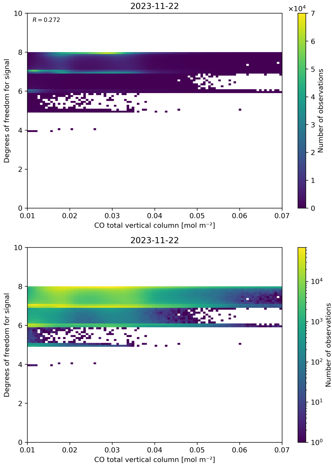
Figure 41: Scatter density plot of “CO total vertical column” against “Degrees of freedom for signal” for 2023-11-21 to 2023-11-23.
