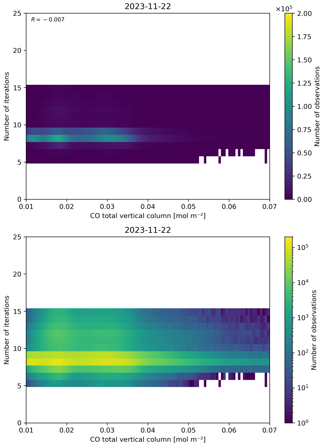
Figure 42: Scatter density plot of “CO total vertical column” against “Number of iterations” for 2023-11-21 to 2023-11-23.
