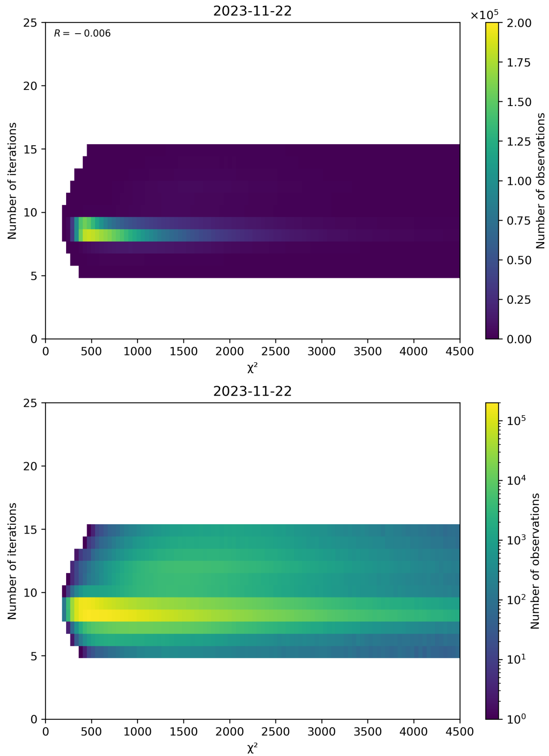
Figure 49: Scatter density plot of “ \chi^2 ” against “Number of iterations” for 2023-11-21 to 2023-11-23.
