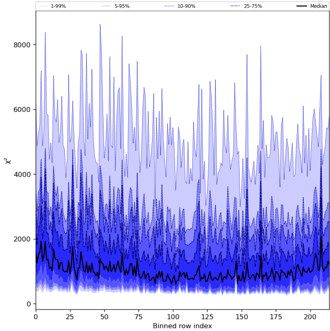
Figure 30: Along track statistics of “ \chi^2 ” for 2023-11-21 to 2023-11-23
