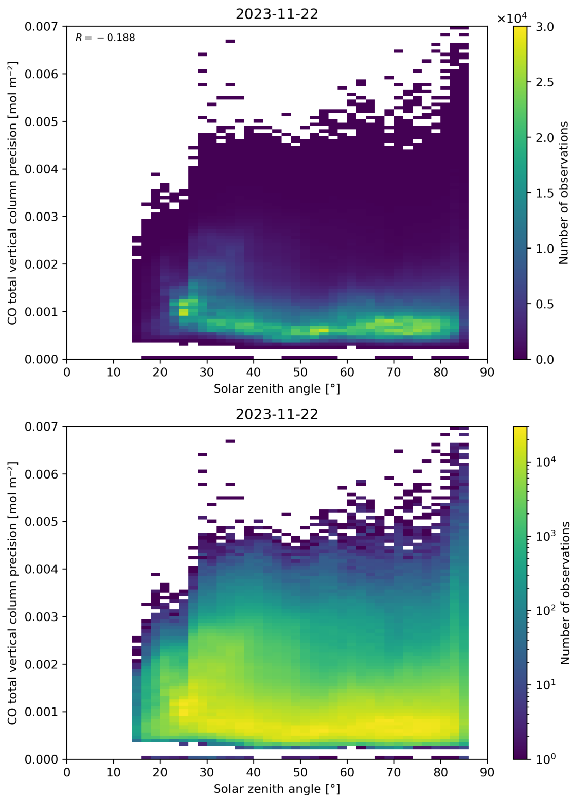
Figure 63: Scatter density plot of “Solar zenith angle” against “CO total vertical column precision” for 2023-11-21 to 2023-11-23.
