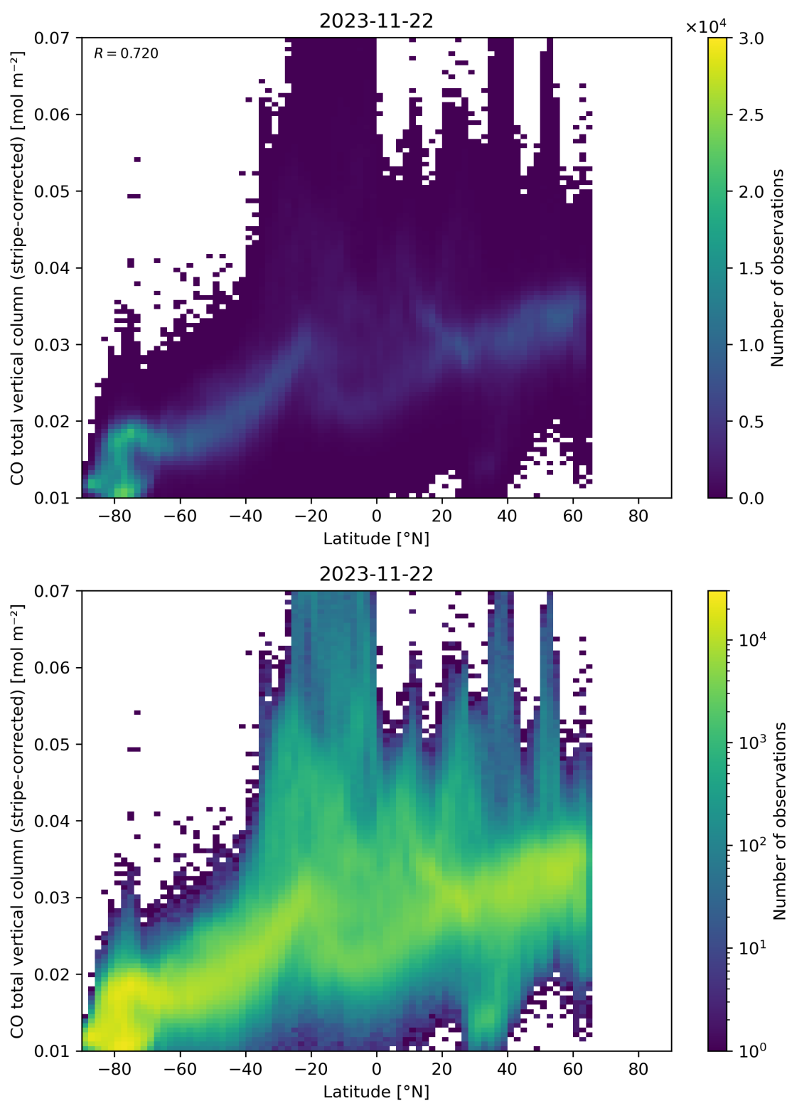
Figure 52: Scatter density plot of “Latitude” against “CO total vertical column (stripe-corrected)” for 2023-11-21 to 2023-11-23.
