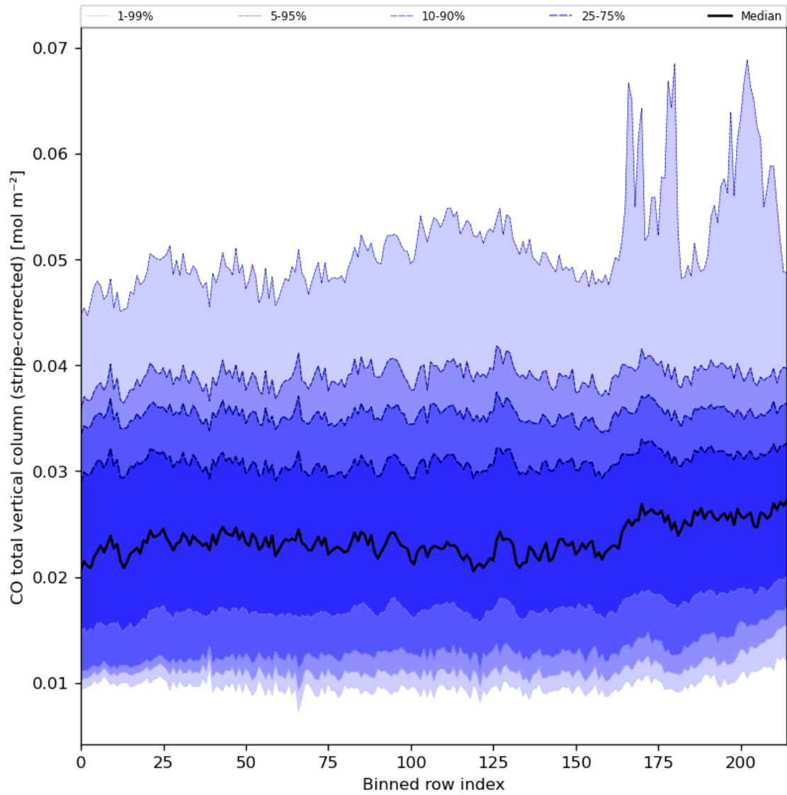
Figure 27: Along track statistics of “CO total vertical column (stripe-corrected)” for 2023-11-21 to 2023-11-23
