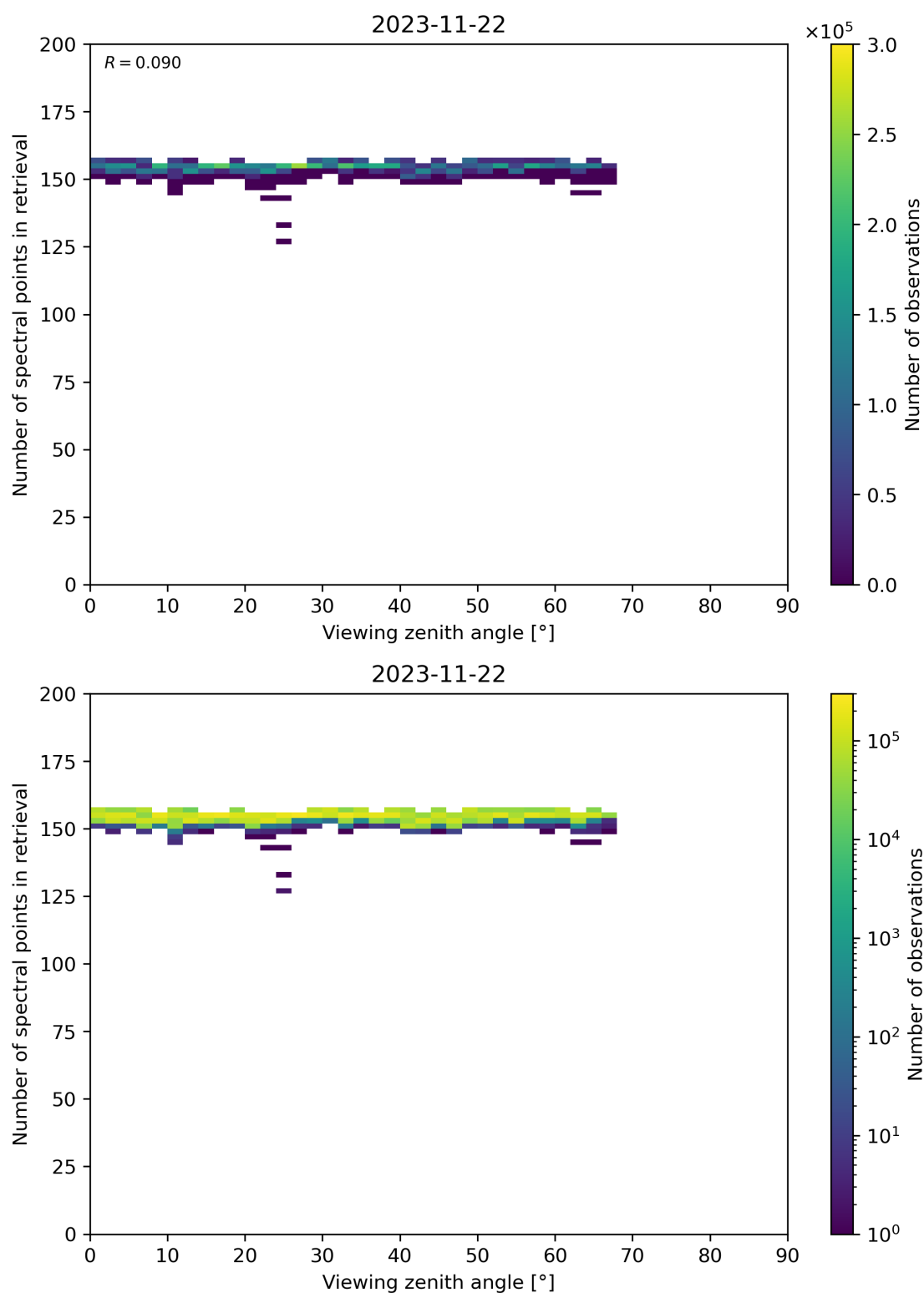
Figure 76: Scatter density plot of “Viewing zenith angle” against “Number of spectral points in retrieval” for 2023-11-21 to 2023-11-23.
