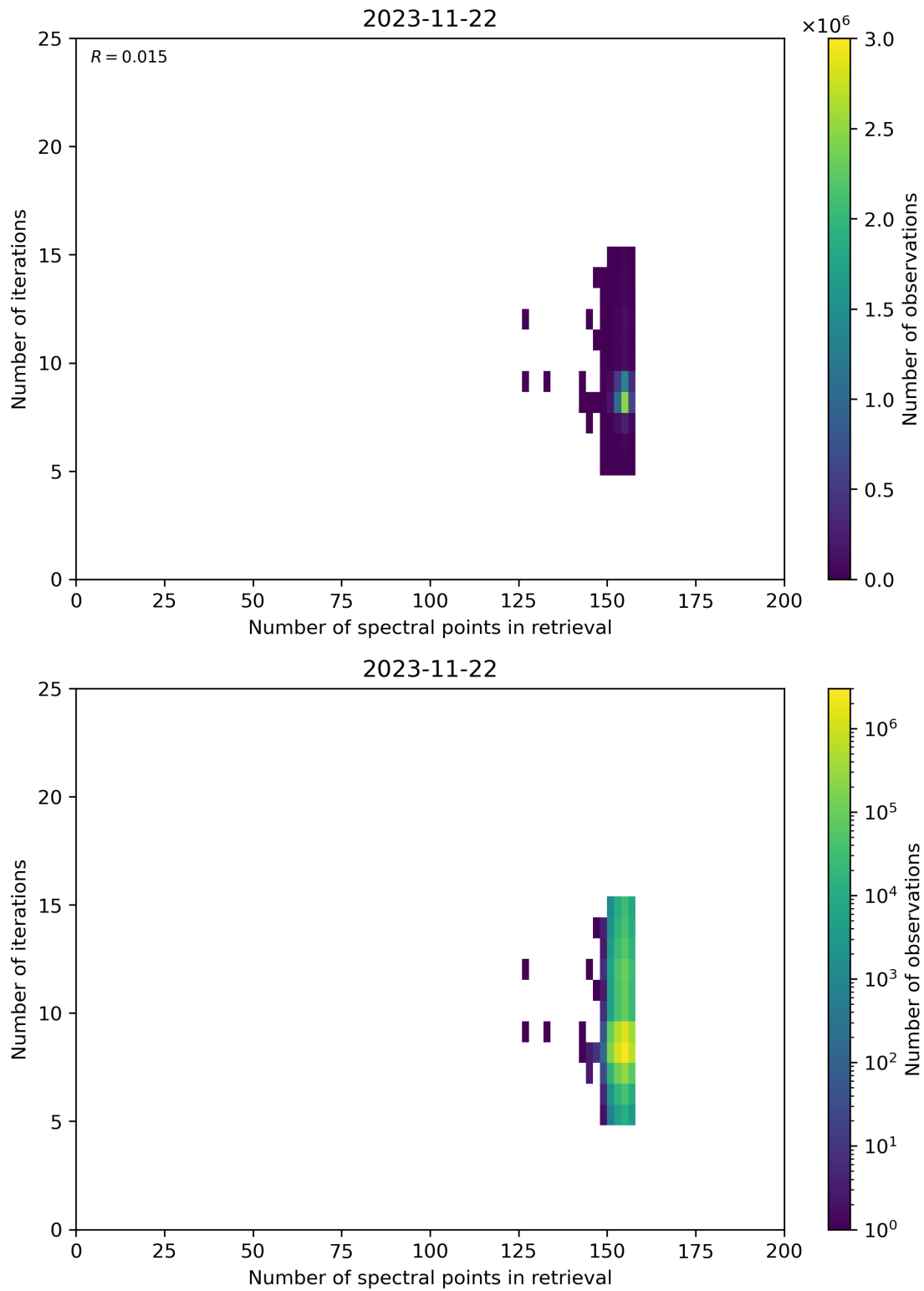
Figure 60: Scatter density plot of “Number of spectral points in retrieval” against “Number of iterations” for 2023-11-21 to 2023-11-23.
