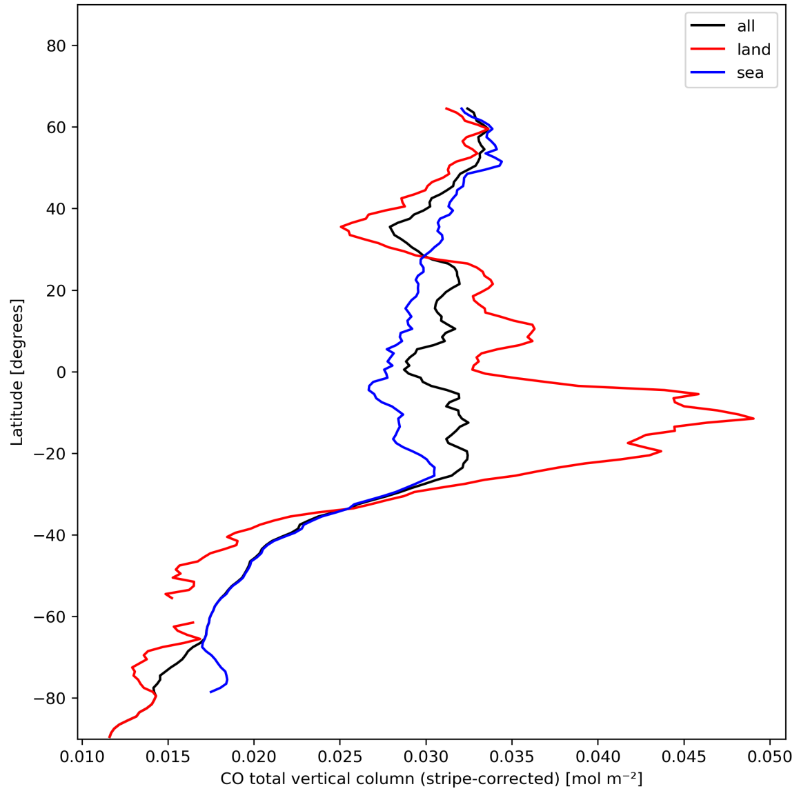
Figure 11: Zonal average of “CO total vertical column (stripe-corrected)” for 2023-11-21 to 2023-11-23.
