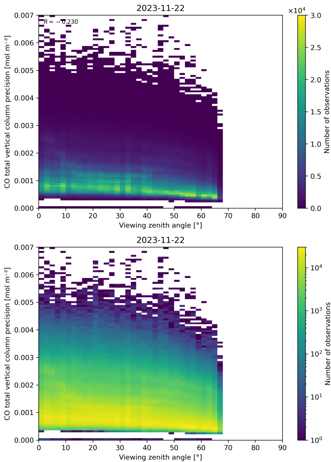
Figure 71: Scatter density plot of “Viewing zenith angle” against “CO total vertical column precision” for 2023-11-21 to 2023-11-23.
