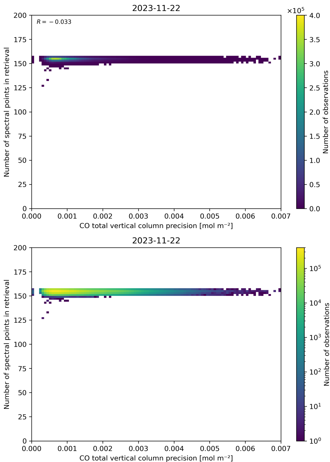
Figure 47: Scatter density plot of “CO total vertical column precision” against “Number of spectral points in retrieval” for 2023-11-21 to 2023-11-23.
