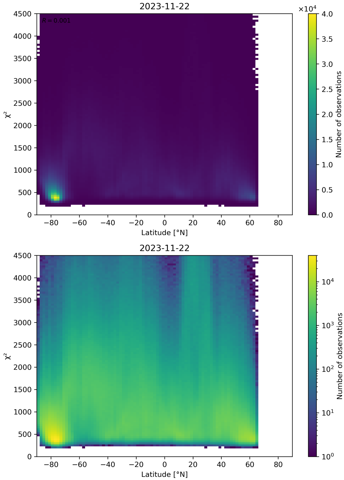
Figure 54: Scatter density plot of “Latitude” against “ \chi^2 ” for 2023-11-21 to 2023-11-23.
