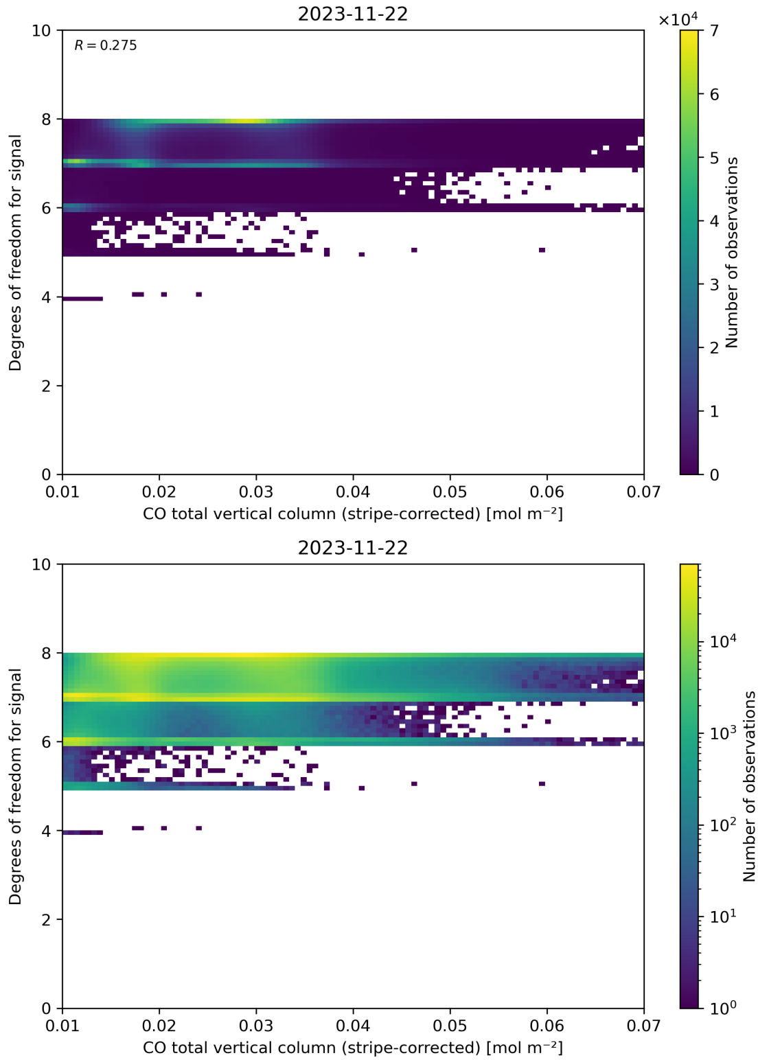
Figure 38: Scatter density plot of “CO total vertical column (stripe-corrected)” against “Degrees of freedom for signal” for 2023-11-21 to 2023-11-23.
