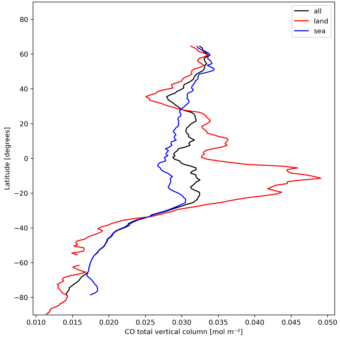
Figure 10: Zonal average of “CO total vertical column” for 2023-11-21 to 2023-11-23.
