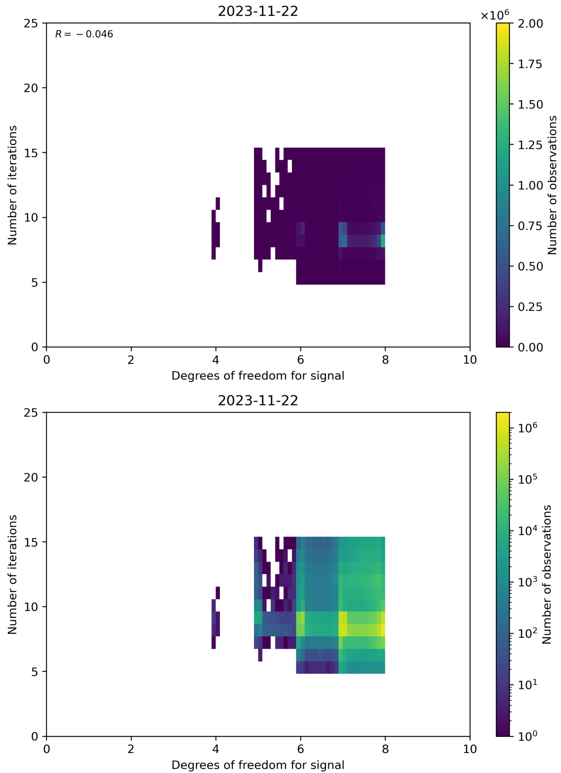
Figure 50: Scatter density plot of “Degrees of freedom for signal” against “Number of iterations” for 2023-11-21 to 2023-11-23.
