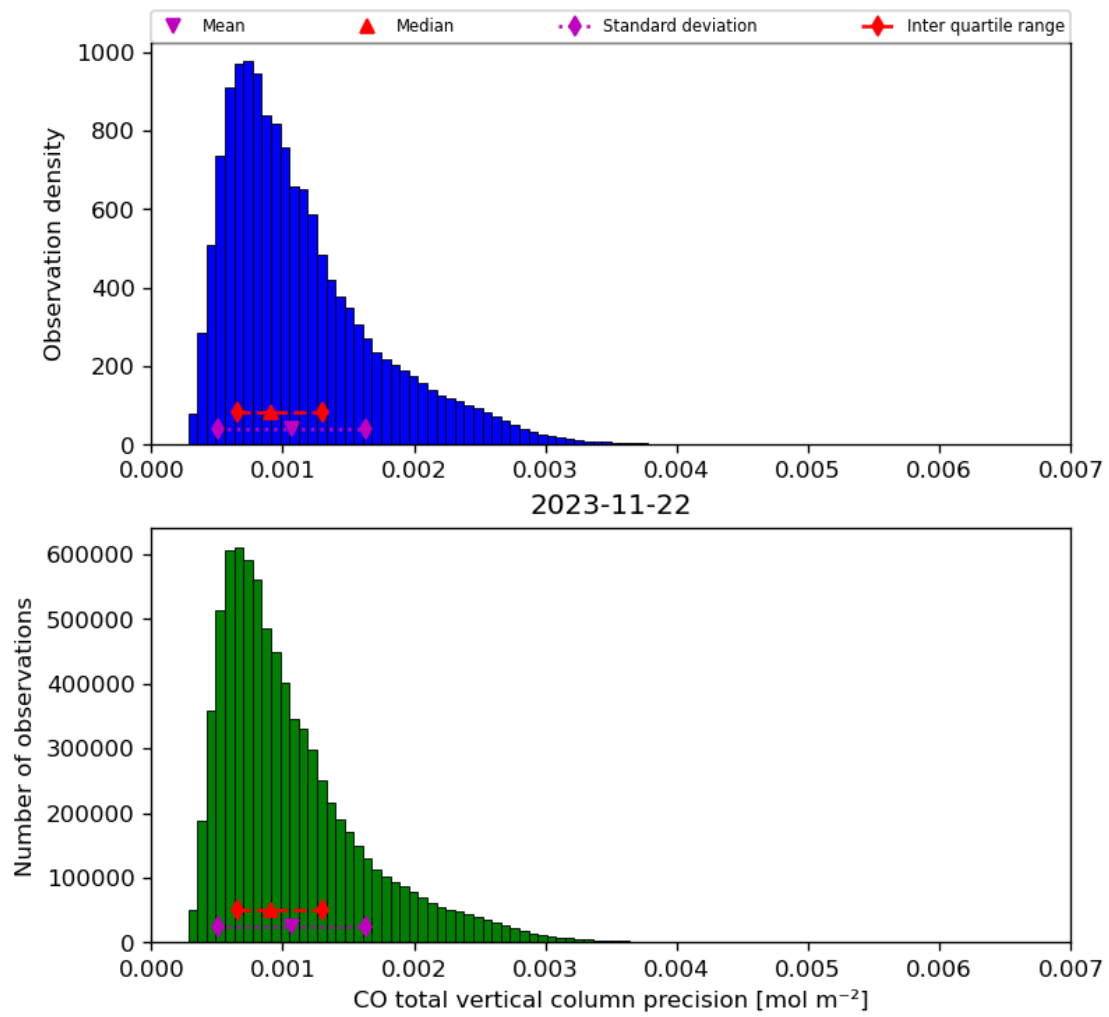
Figure 20: Histogram of “CO total vertical column precision” for 2023-11-21 to 2023-11-23
