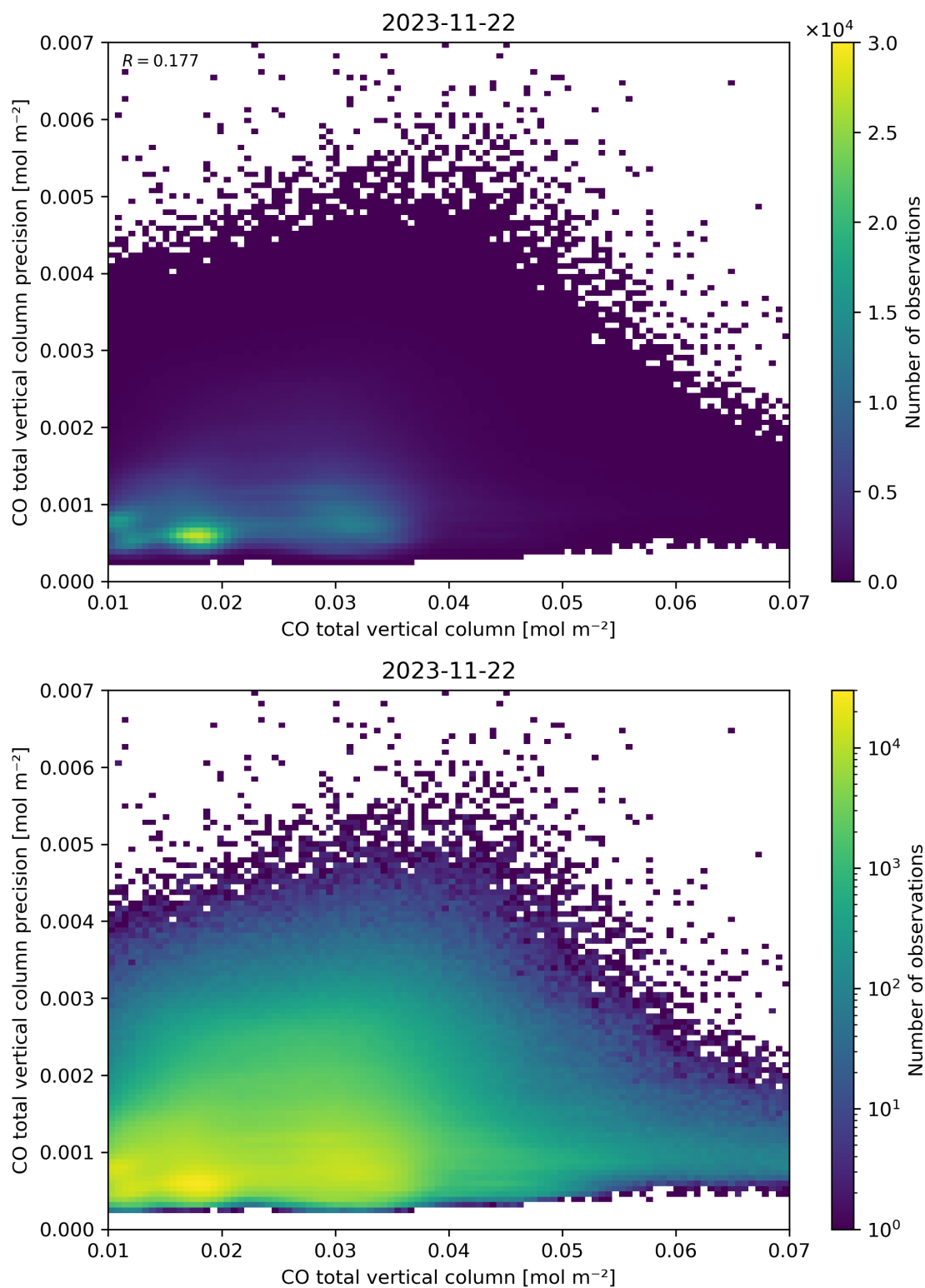
Figure 34: Scatter density plot of “CO total vertical column” against “CO total vertical column precision” for 2023-11-21 to 2023-11-23.
