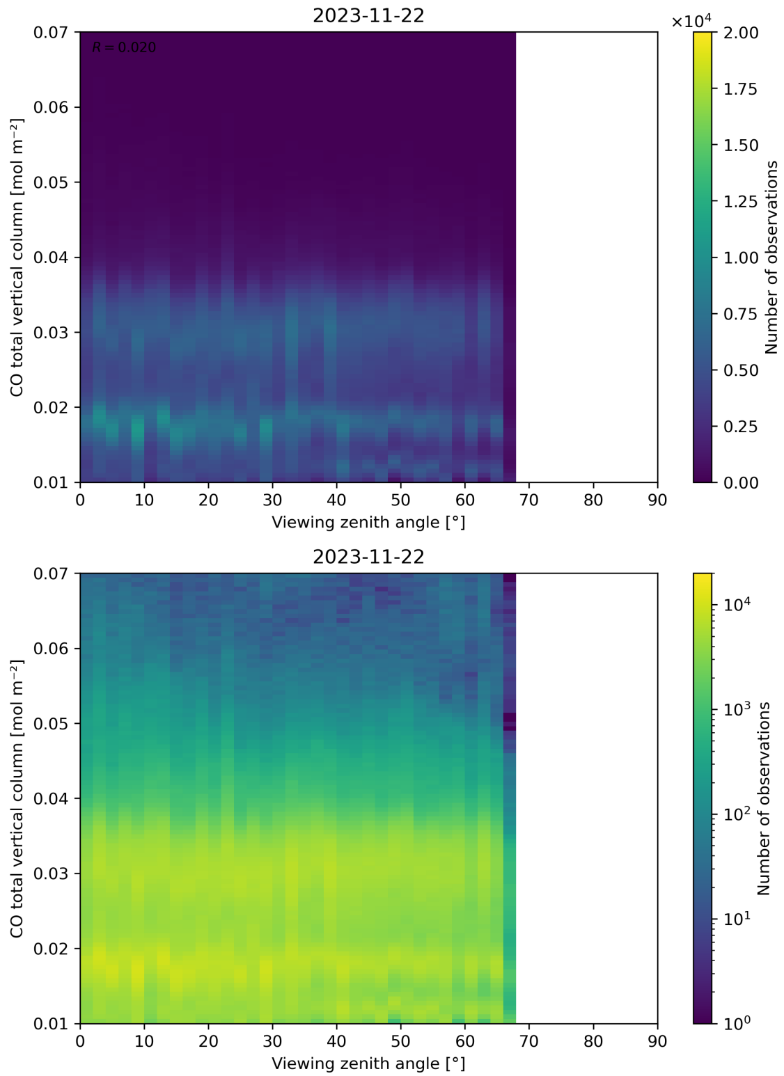
Figure 69: Scatter density plot of “Viewing zenith angle” against “CO total vertical column” for 2023-11-21 to 2023-11-23.
