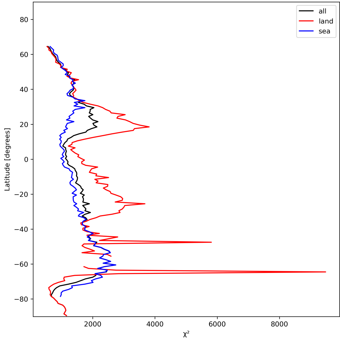
Figure 14: Zonal average of “ \chi^2 ” for 2023-11-21 to 2023-11-23.
