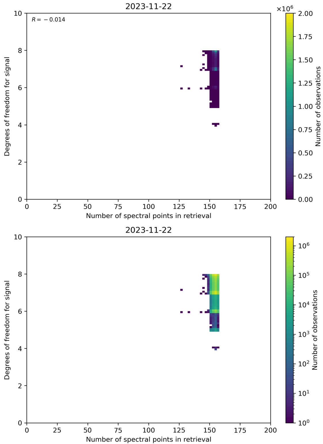
Figure 59: Scatter density plot of “Number of spectral points in retrieval” against “Degrees of freedom for signal” for 2023-11-21 to 2023-11-23.
