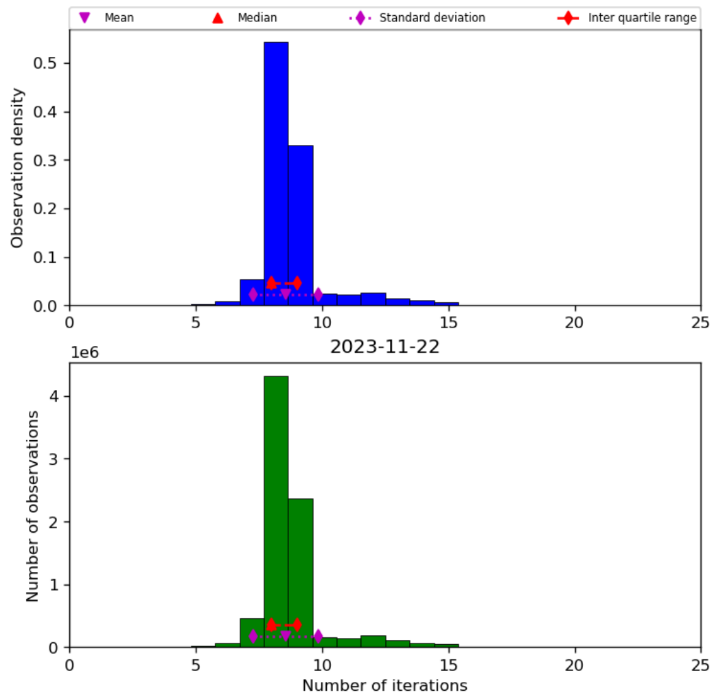
Figure 24: Histogram of “Number of iterations” for 2023-11-21 to 2023-11-23
