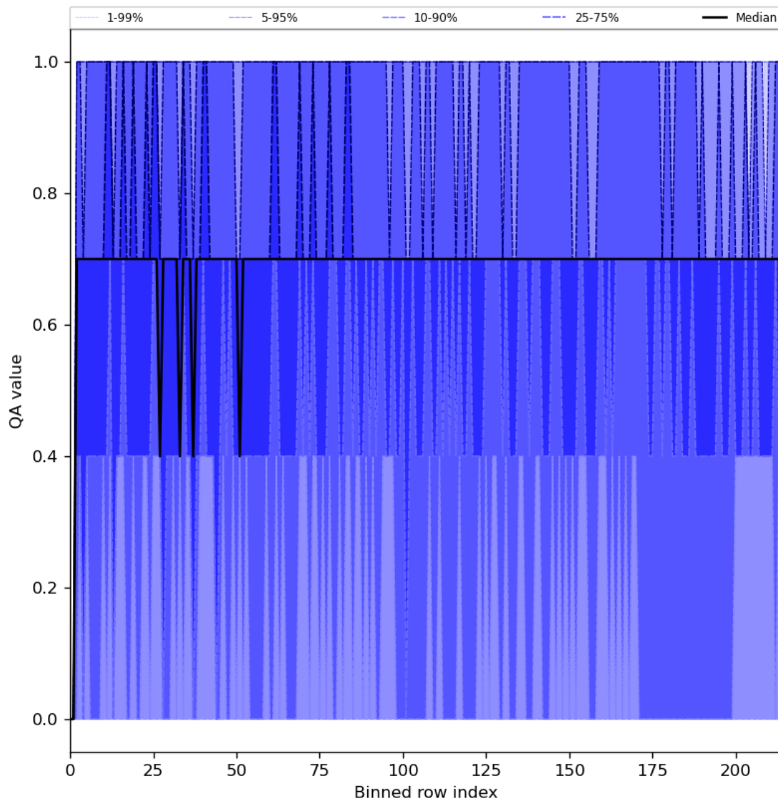
Figure 25: Along track statistics of “QA value” for 2023-11-21 to 2023-11-23
