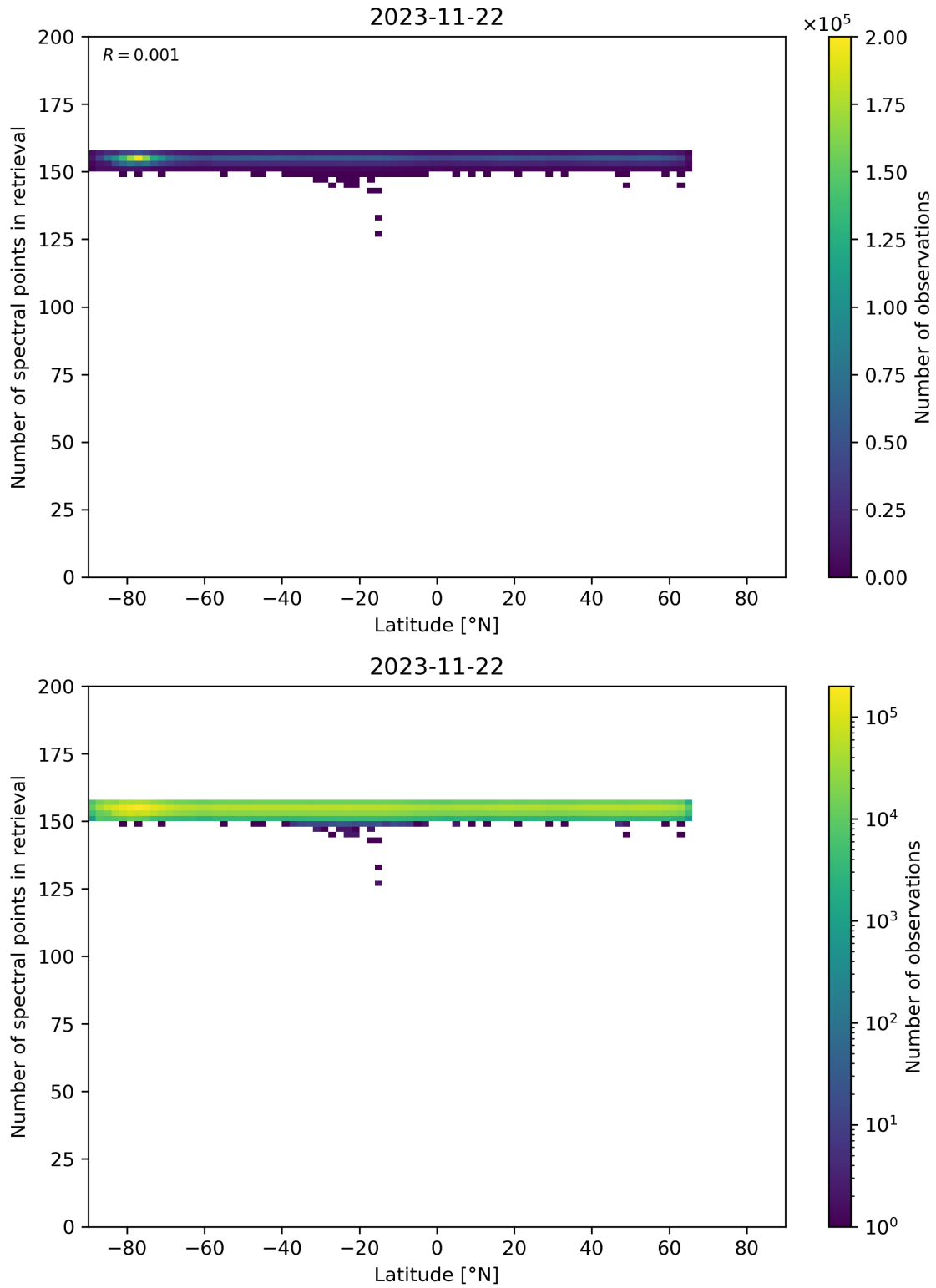
Figure 57: Scatter density plot of “Latitude” against “Number of spectral points in retrieval” for 2023-11-21 to 2023-11-23.
