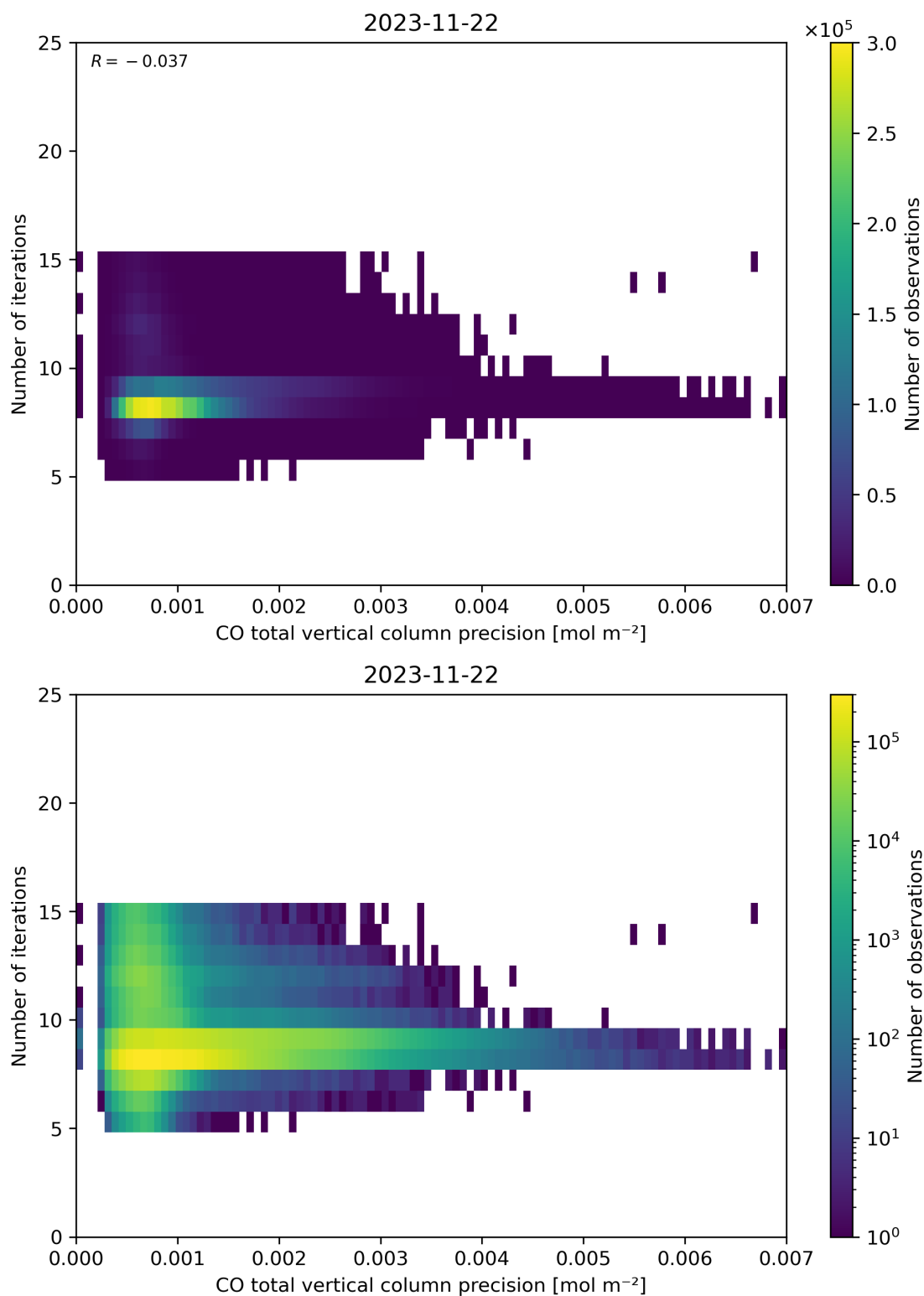
Figure 46: Scatter density plot of “CO total vertical column precision” against “Number of iterations” for 2023-11-21 to 2023-11-23.
