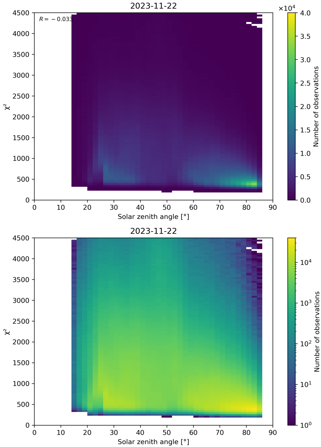
Figure 64: Scatter density plot of “Solar zenith angle” against “ \chi^2 ” for 2023-11-21 to 2023-11-23.
