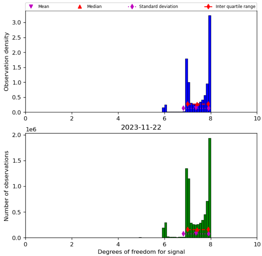
Figure 23: Histogram of “Degrees of freedom for signal” for 2023-11-21 to 2023-11-23
