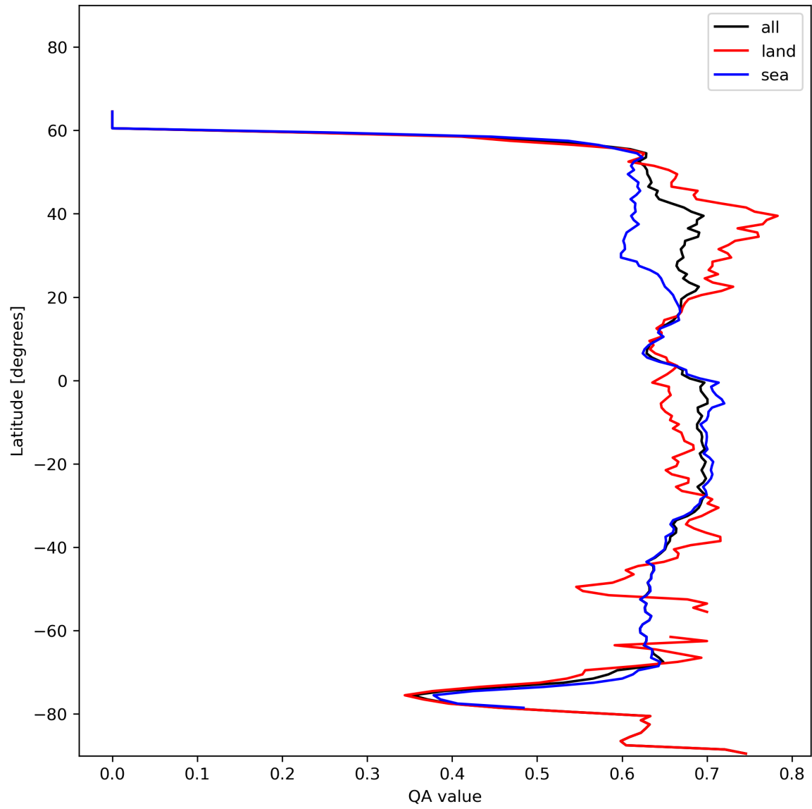
Figure 9: Zonal average of “QA value” for 2023-11-21 to 2023-11-23.
