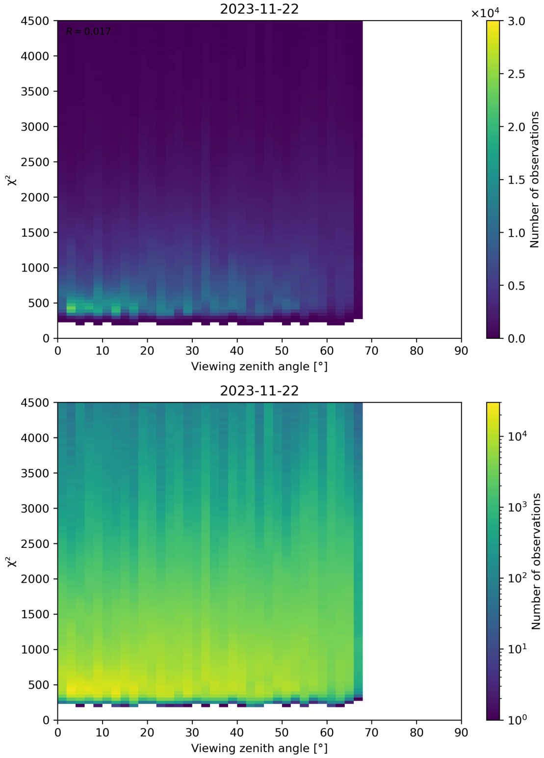
Figure 72: Scatter density plot of “Viewing zenith angle” against “ \chi^2 ” for 2023-11-21 to 2023-11-23.
