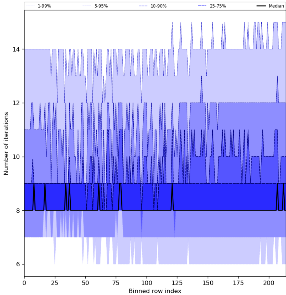
Figure 32: Along track statistics of “Number of iterations” for 2023-11-21 to 2023-11-23
