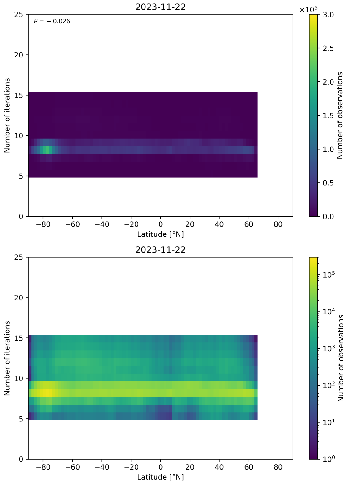
Figure 56: Scatter density plot of “Latitude” against “Number of iterations” for 2023-11-21 to 2023-11-23.
