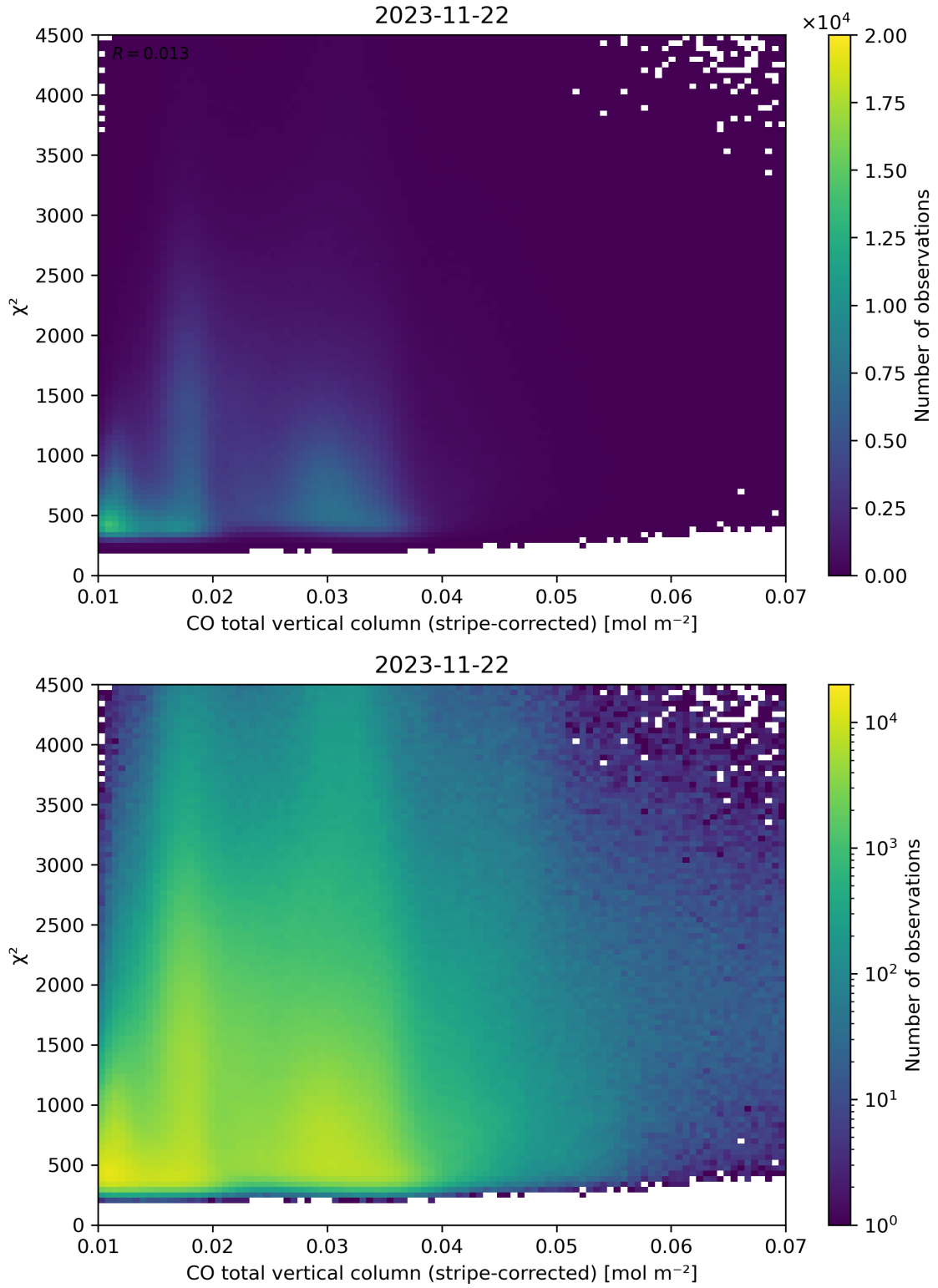
Figure 37: Scatter density plot of “CO total vertical column (stripe-corrected)” against “ \chi^2 ” for 2023-11-21 to 2023-11-23.
