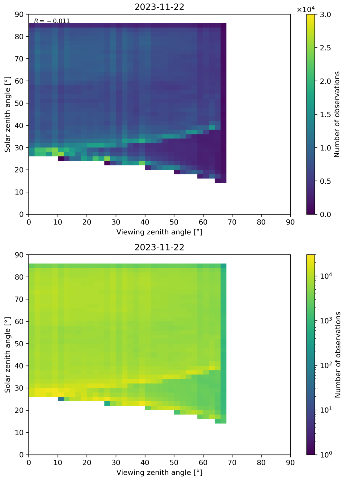
Figure 77: Scatter density plot of “Viewing zenith angle” against “Solar zenith angle” for 2023-11-21 to 2023-11-23.
