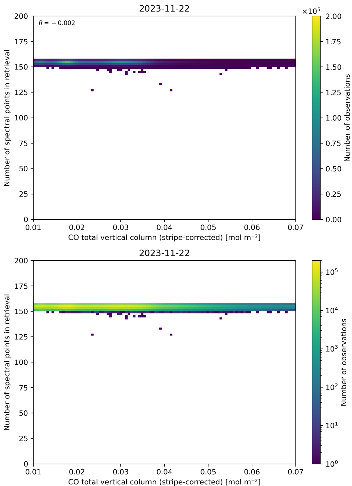
Figure 40: Scatter density plot of “CO total vertical column (stripe-corrected)” against “Number of spectral points in retrieval” for 2023-11-21 to 2023-11-23.
