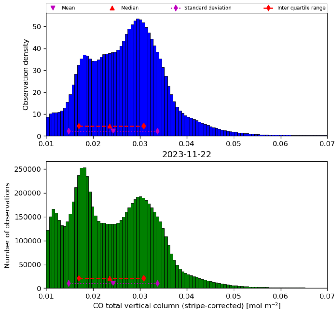
Figure 19: Histogram of “CO total vertical column (stripe-corrected)” for 2023-11-21 to 2023-11-23
