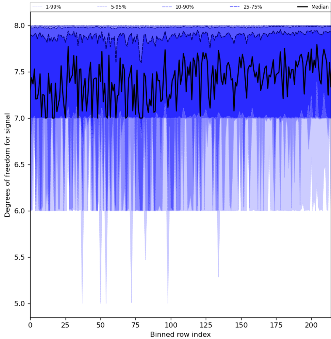
Figure 31: Along track statistics of “Degrees of freedom for signal” for 2023-11-21 to 2023-11-23
