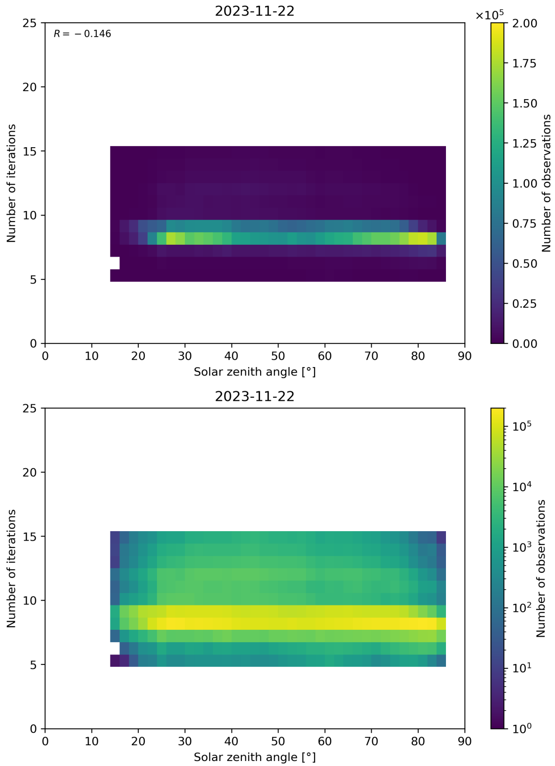
Figure 67: Scatter density plot of “Solar zenith angle” against “Number of iterations” for 2023-11-21 to 2023-11-23.
