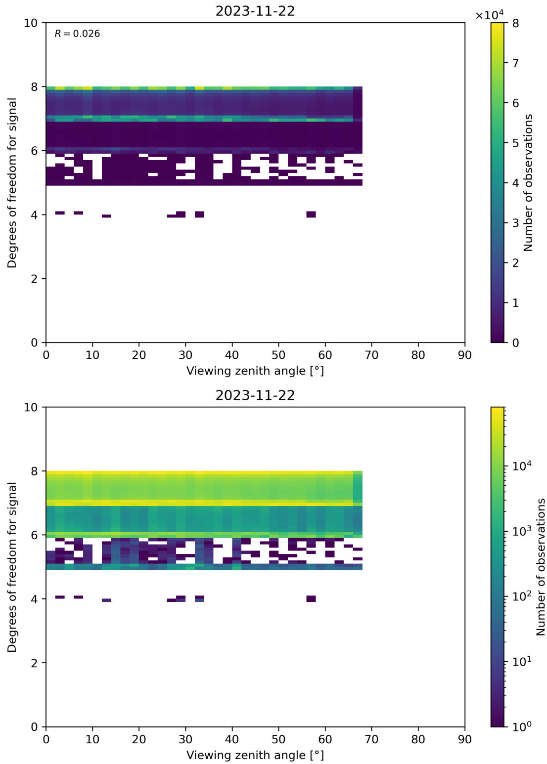
Figure 73: Scatter density plot of “Viewing zenith angle” against “Degrees of freedom for signal” for 2023-11-21 to 2023-11-23.
