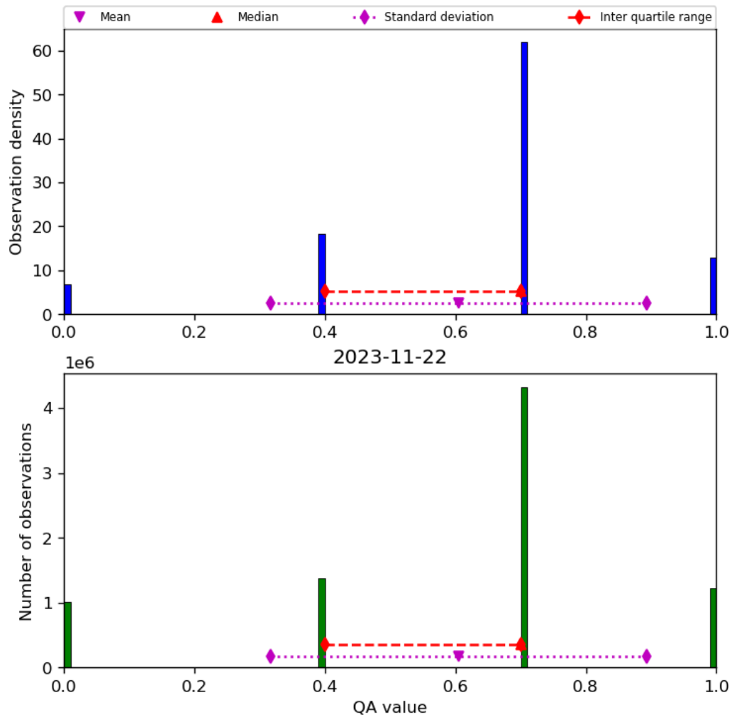
Figure 17: Histogram of “QA value” for 2023-11-21 to 2023-11-23
