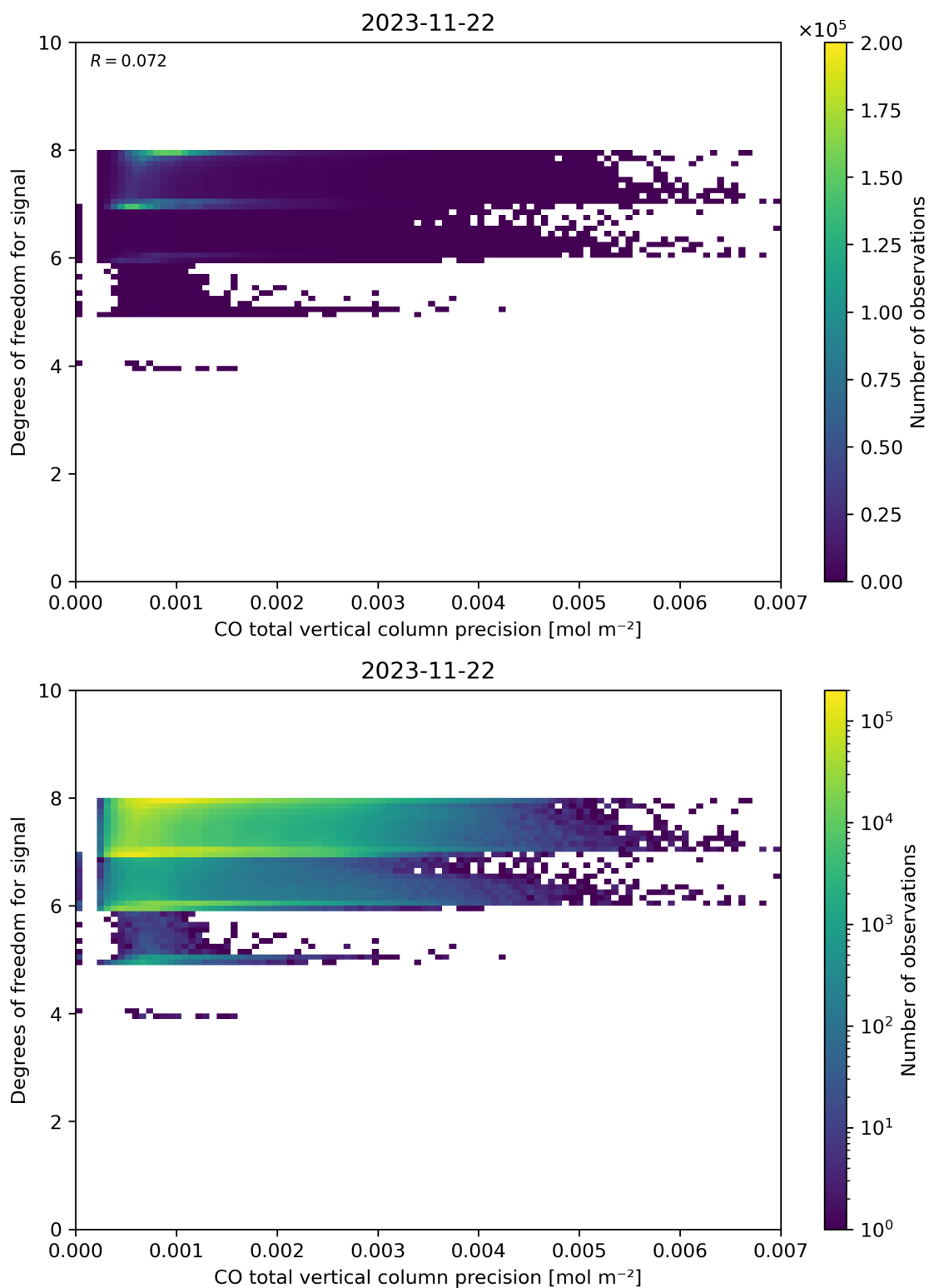
Figure 45: Scatter density plot of “CO total vertical column precision” against “Degrees of freedom for signal” for 2023-11-21 to 2023-11-23.
