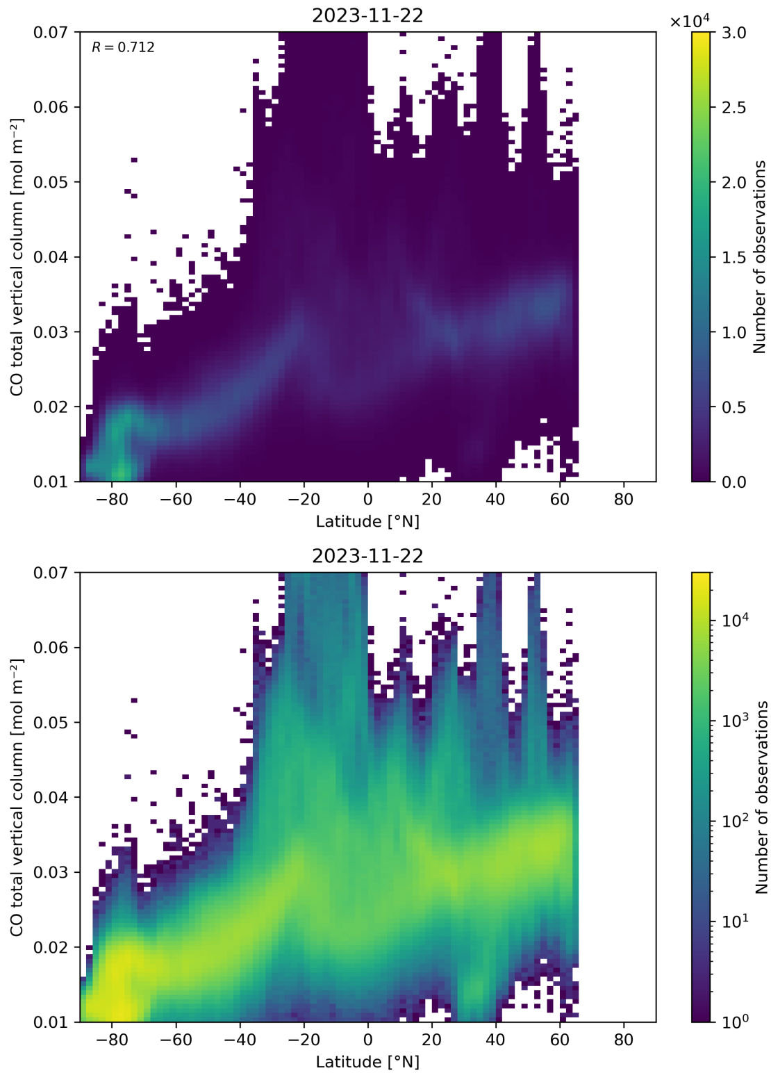
Figure 51: Scatter density plot of “Latitude” against “CO total vertical column” for 2023-11-21 to 2023-11-23.
