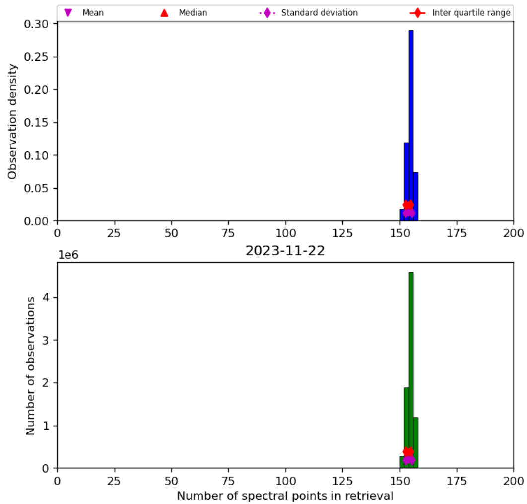
Figure 21: Histogram of “Number of spectral points in retrieval” for 2023-11-21 to 2023-11-23
