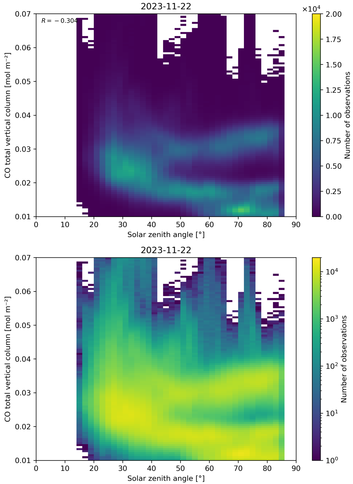
Figure 61: Scatter density plot of “Solar zenith angle” against “CO total vertical column” for 2023-11-21 to 2023-11-23.
