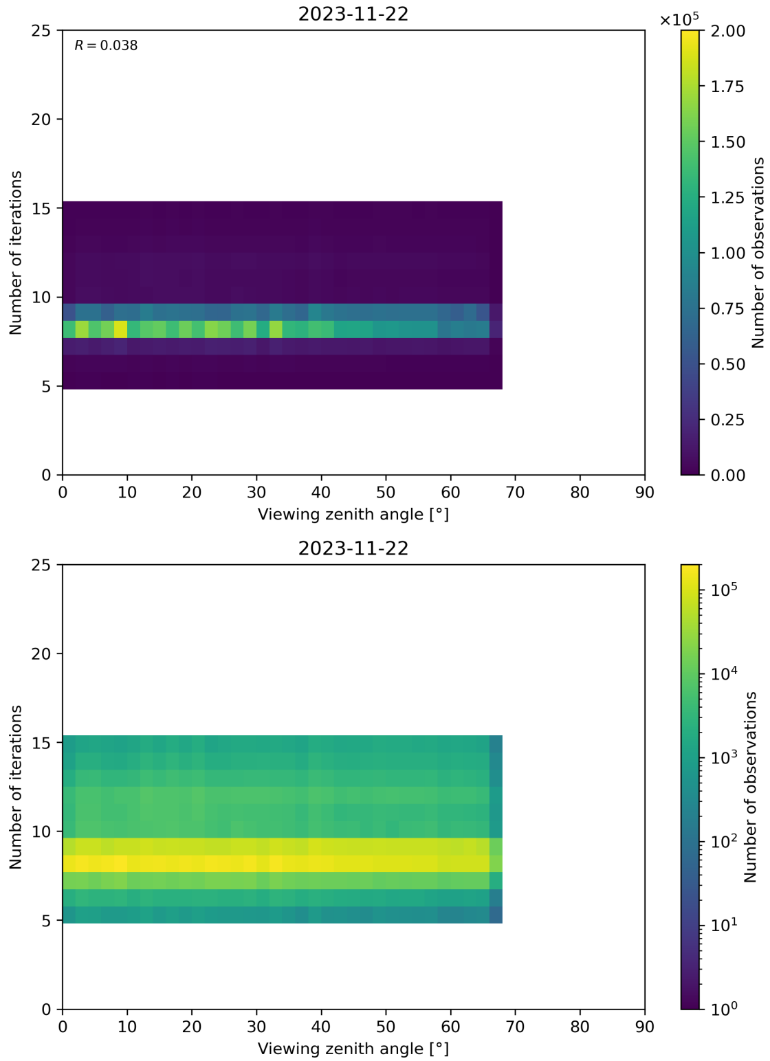
Figure 75: Scatter density plot of “Viewing zenith angle” against “Number of iterations” for 2023-11-21 to 2023-11-23.
