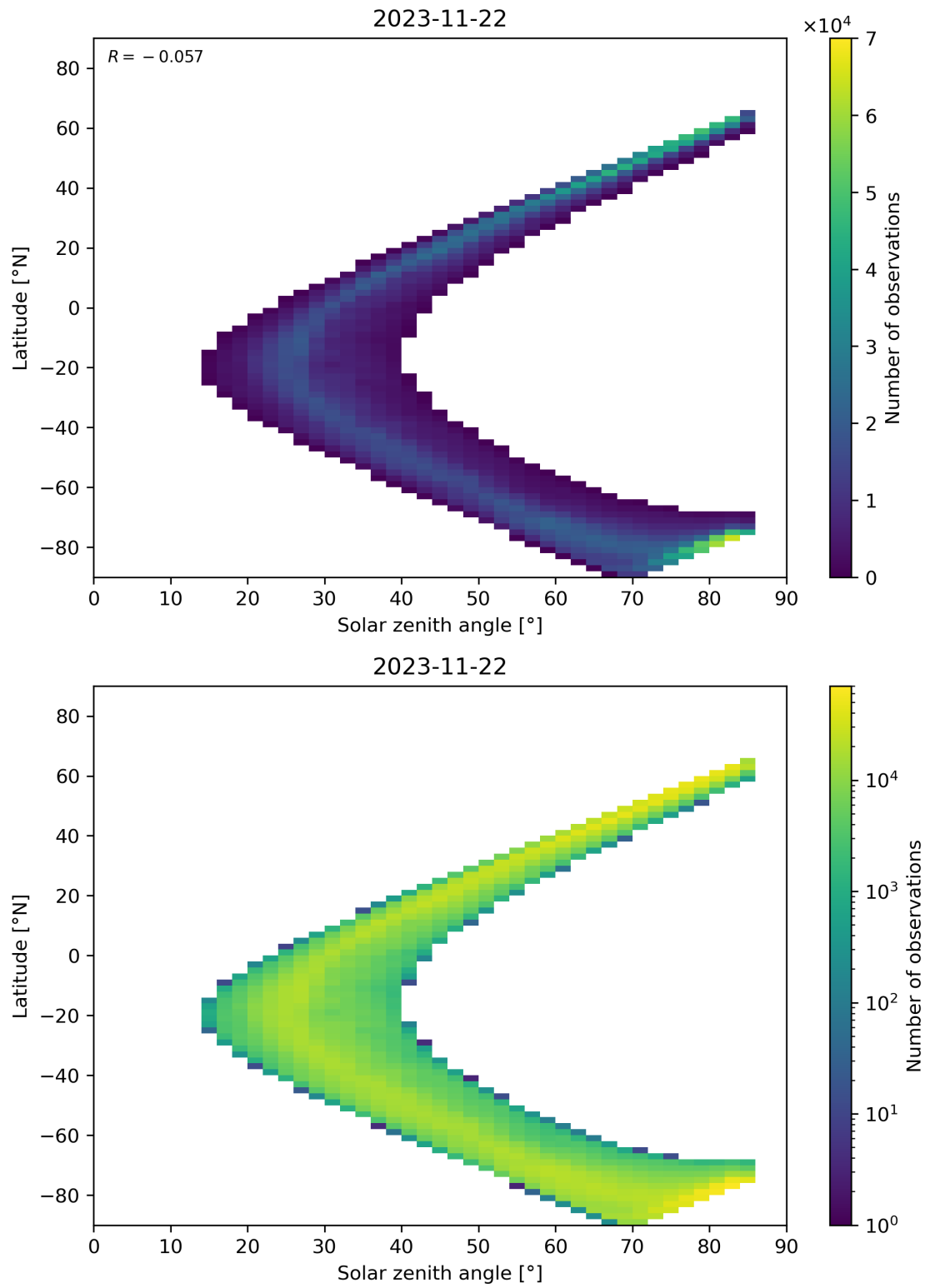
Figure 66: Scatter density plot of “Solar zenith angle” against “Latitude” for 2023-11-21 to 2023-11-23.
