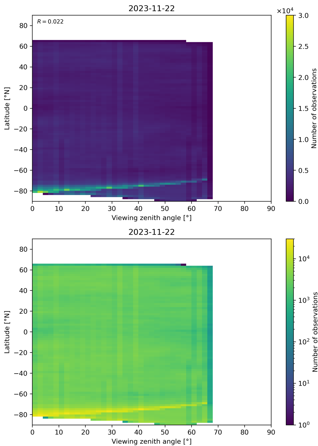
Figure 74: Scatter density plot of “Viewing zenith angle” against “Latitude” for 2023-11-21 to 2023-11-23.
