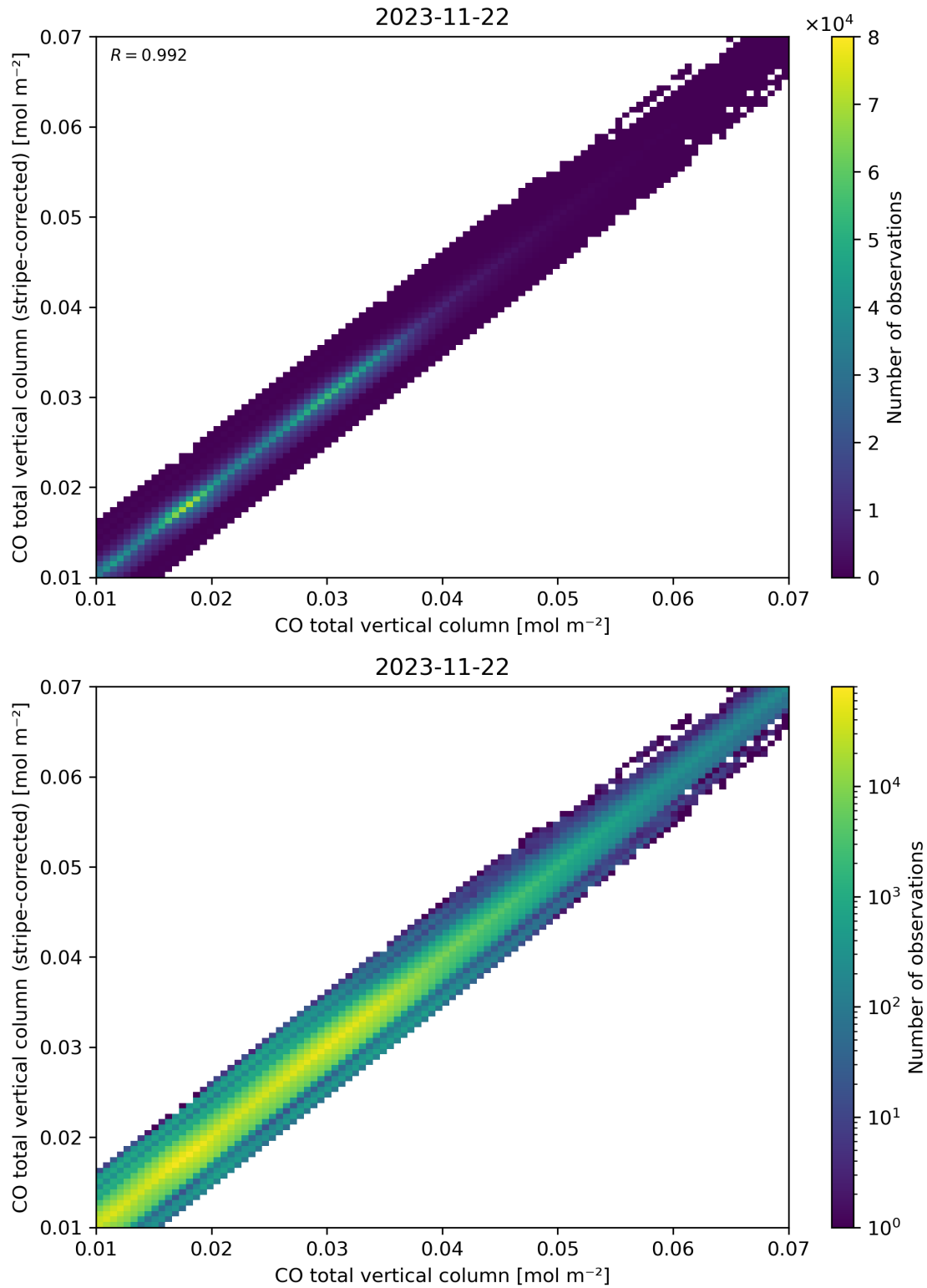
Figure 33: Scatter density plot of “CO total vertical column” against “CO total vertical column (stripe-corrected)” for 2023-11-21 to 2023-11-23.
