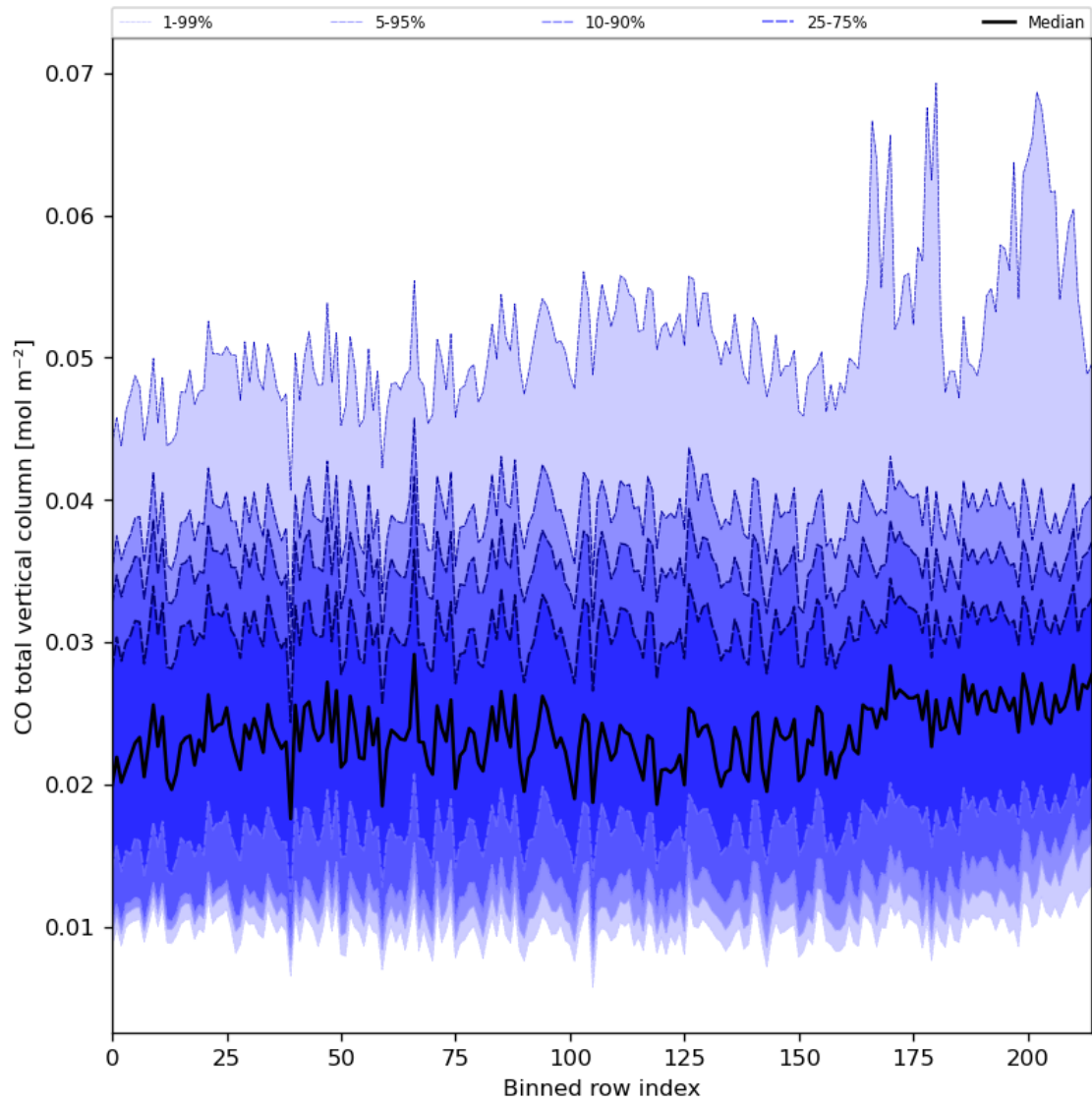
Figure 26: Along track statistics of “CO total vertical column” for 2023-11-21 to 2023-11-23
