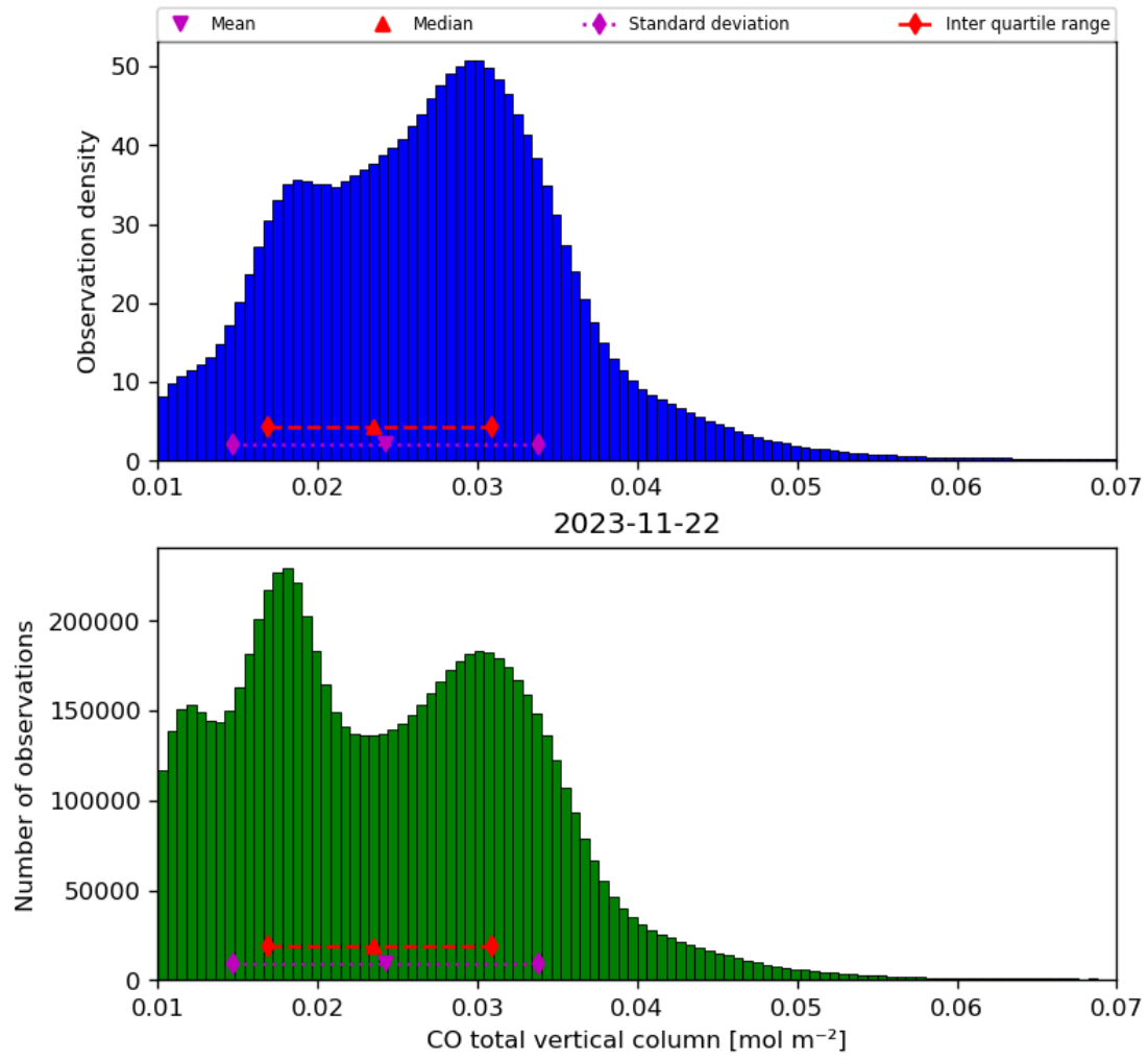
Figure 18: Histogram of “CO total vertical column” for 2023-11-21 to 2023-11-23
