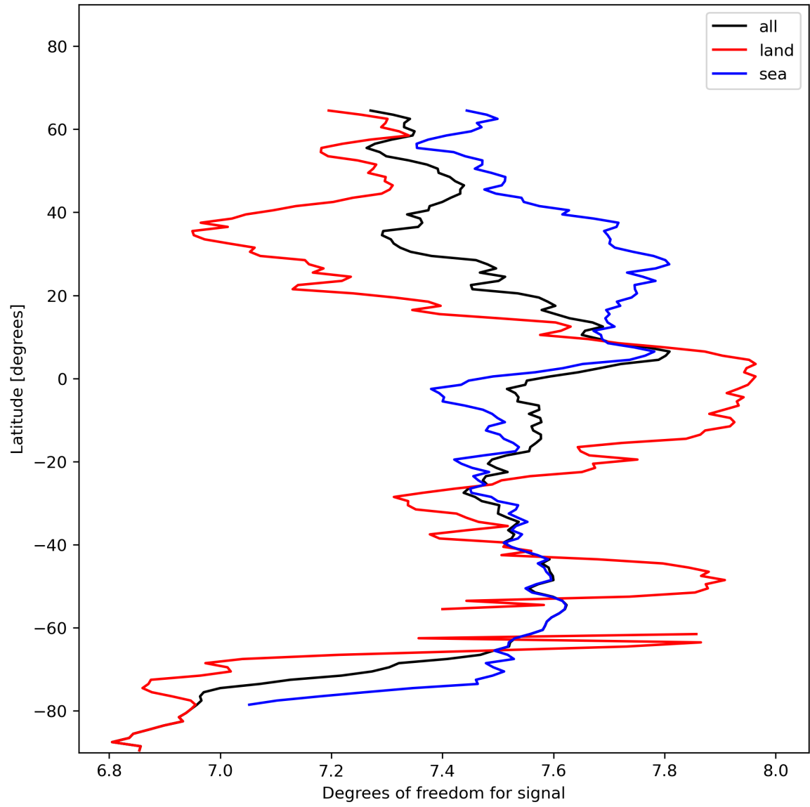
Figure 15: Zonal average of “Degrees of freedom for signal” for 2023-11-21 to 2023-11-23.
