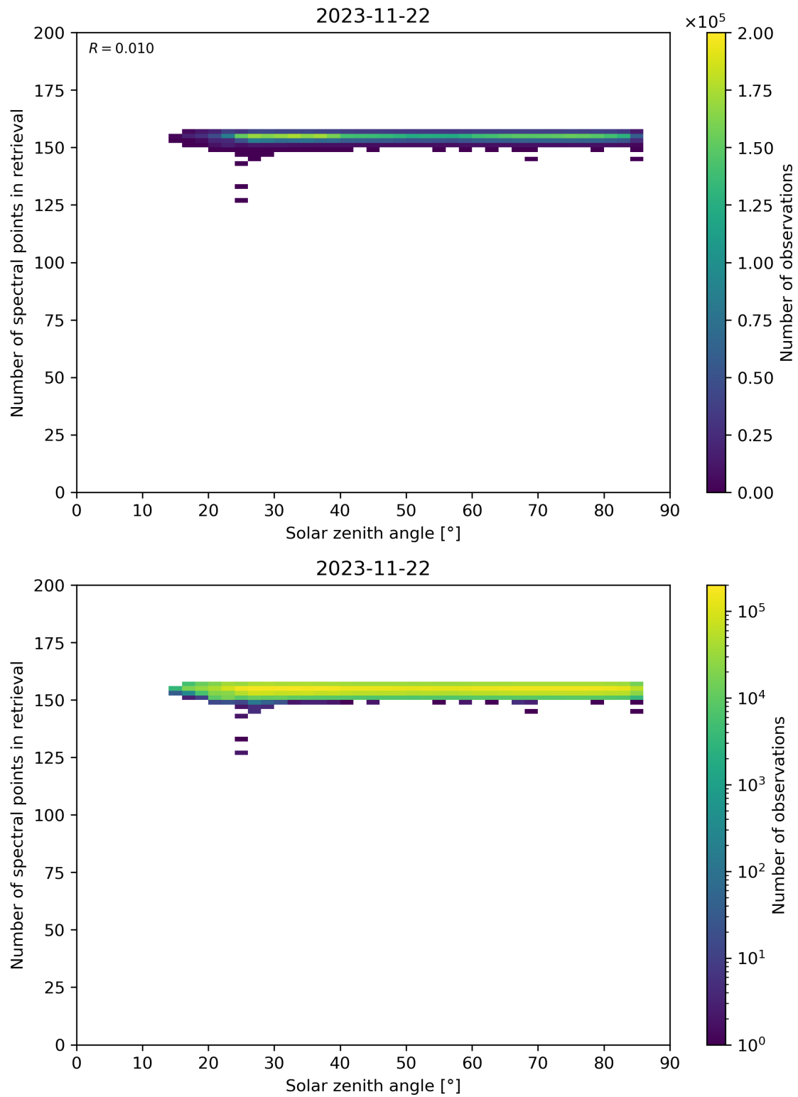
Figure 68: Scatter density plot of “Solar zenith angle” against “Number of spectral points in retrieval” for 2023-11-21 to 2023-11-23.
