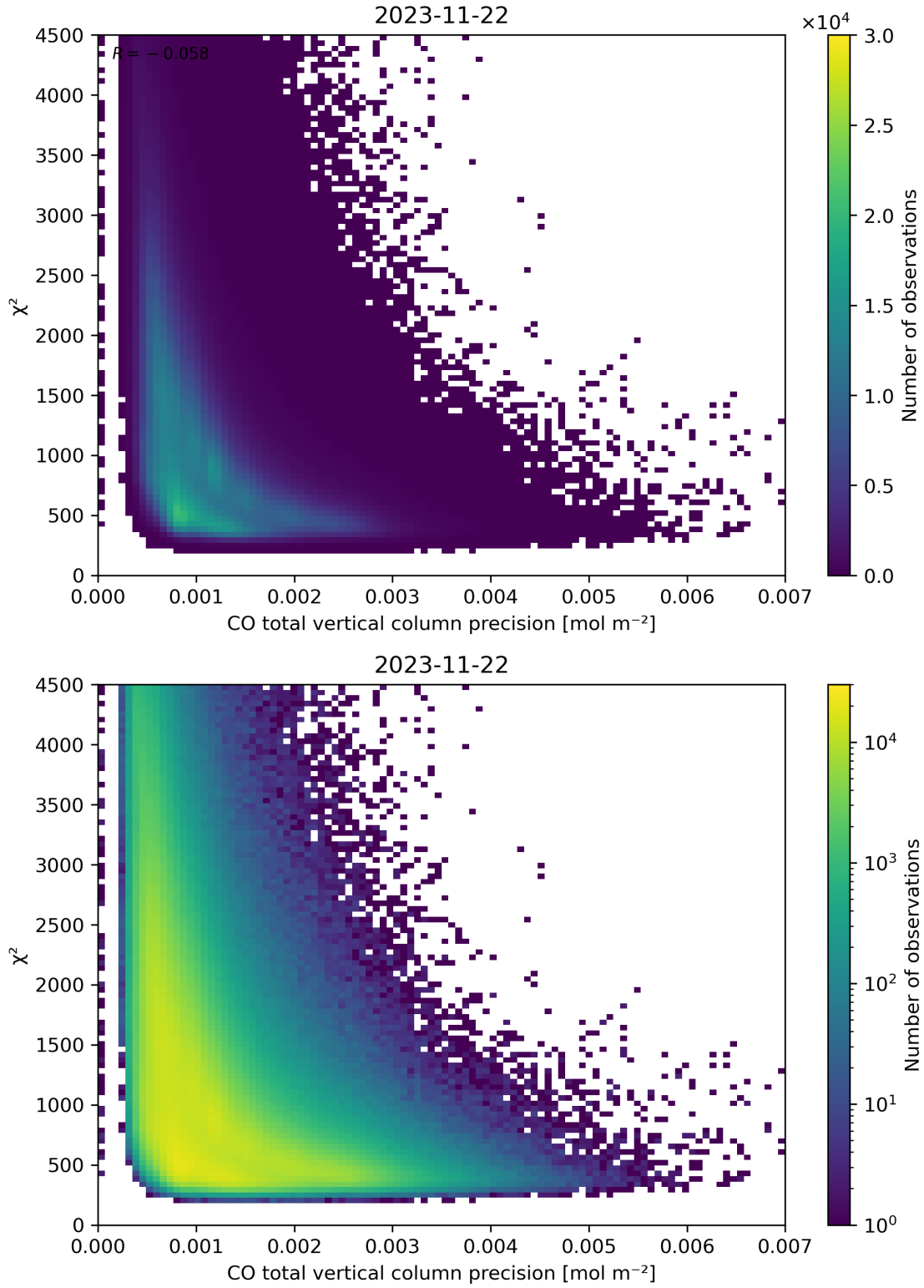
Figure 44: Scatter density plot of “CO total vertical column precision” against “ \chi^2 ” for 2023-11-21 to 2023-11-23.
