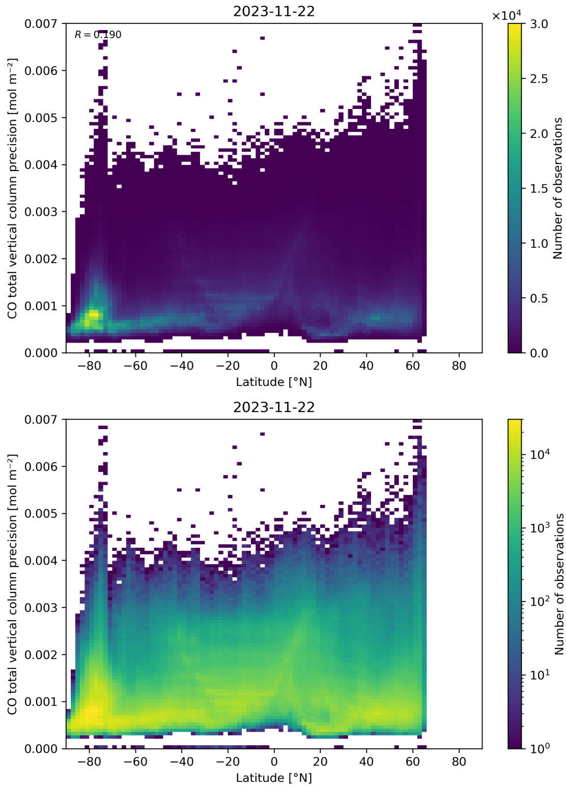
Figure 53: Scatter density plot of “Latitude” against “CO total vertical column precision” for 2023-11-21 to 2023-11-23.
