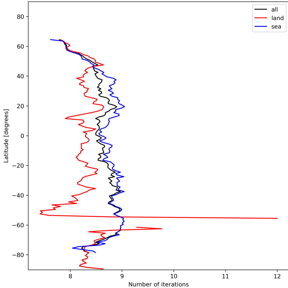
Figure 16: Zonal average of “Number of iterations” for 2023-11-23 to 2023-11-25.
