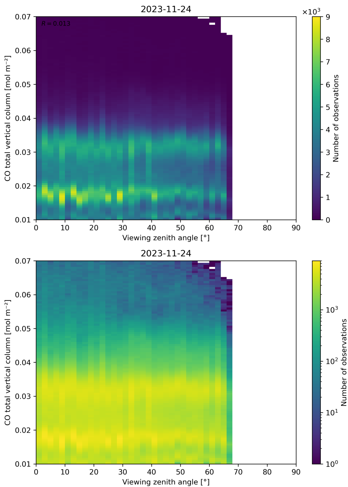
Figure 69: Scatter density plot of “Viewing zenith angle” against “CO total vertical column” for 2023-11-23 to 2023-11-25.
