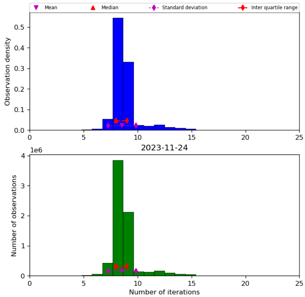
Figure 24: Histogram of “Number of iterations” for 2023-11-23 to 2023-11-25
