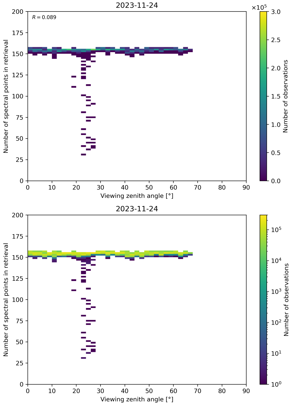
Figure 76: Scatter density plot of “Viewing zenith angle” against “Number of spectral points in retrieval” for 2023-11-23 to 2023-11-25.
