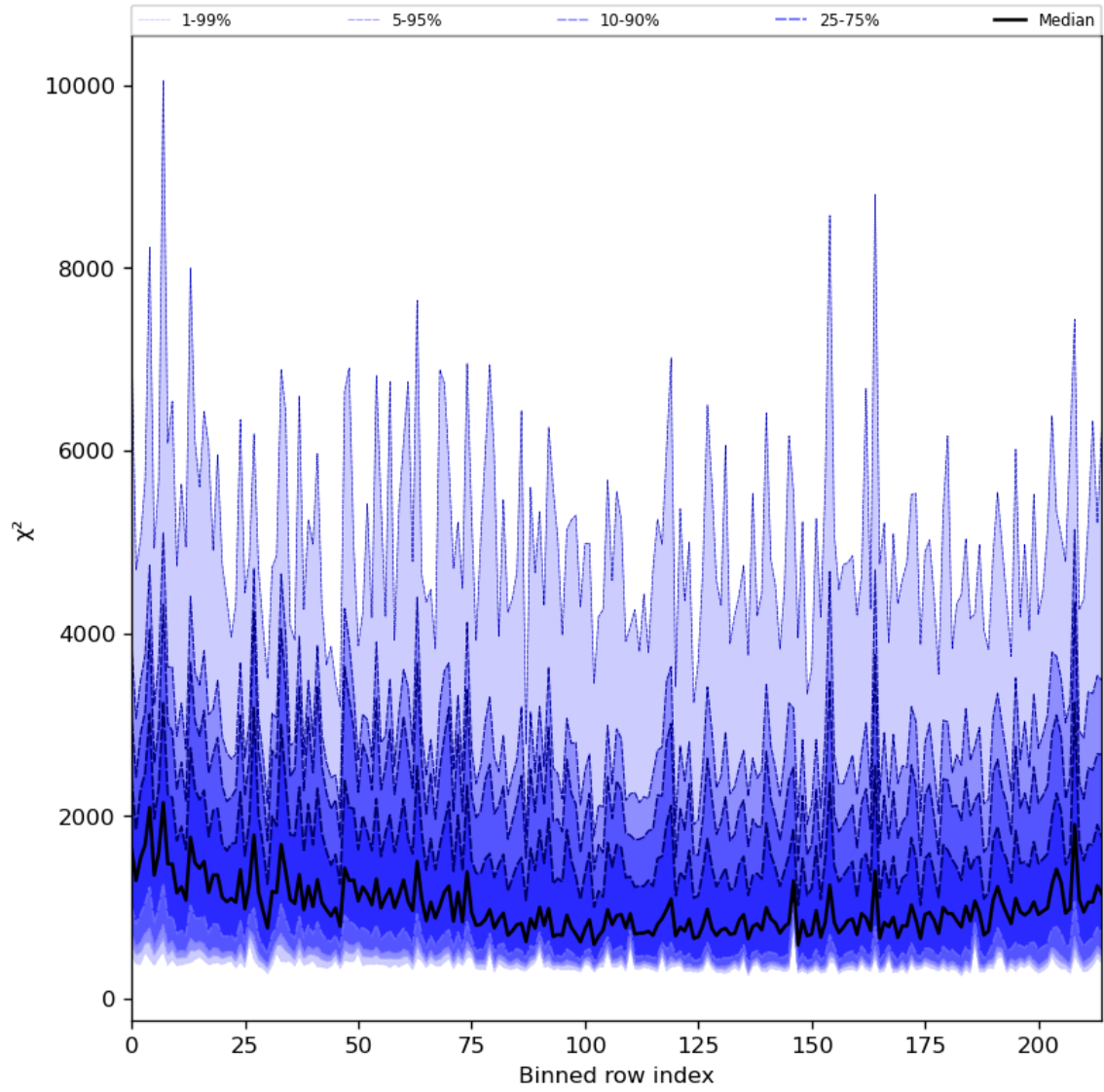
Figure 30: Along track statistics of “ \chi^2 ” for 2023-11-23 to 2023-11-25
