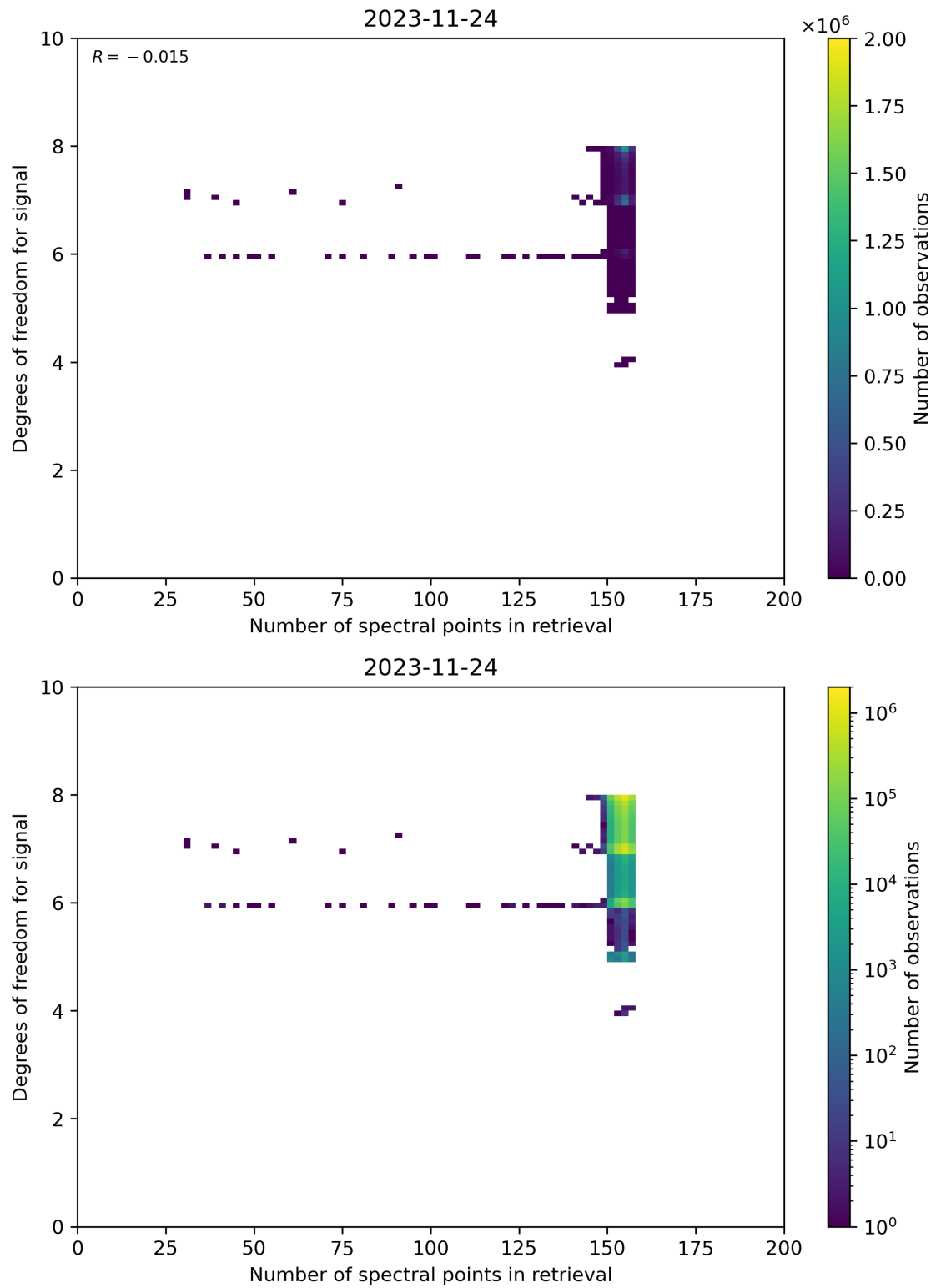
Figure 59: Scatter density plot of “Number of spectral points in retrieval” against “Degrees of freedom for signal” for 2023-11-23 to 2023-11-25.
