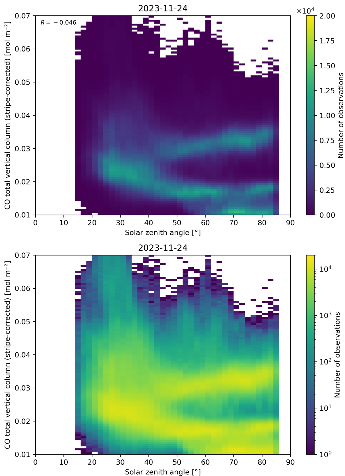
Figure 62: Scatter density plot of “Solar zenith angle” against “CO total vertical column (stripe-corrected)” for 2023-11-23 to 2023-11-25.
