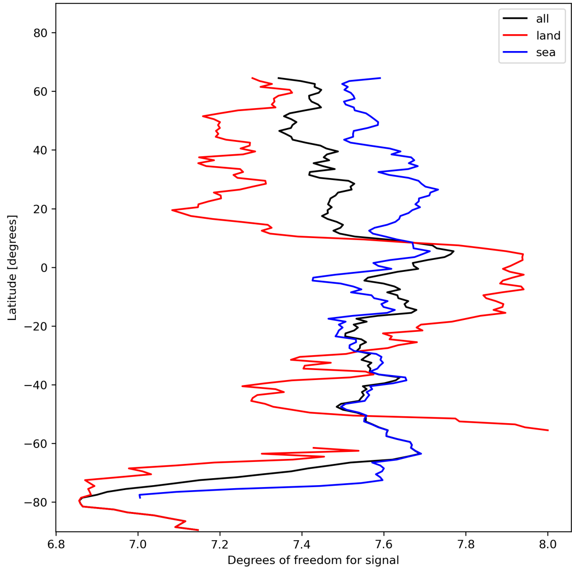
Figure 15: Zonal average of “Degrees of freedom for signal” for 2023-11-23 to 2023-11-25.
