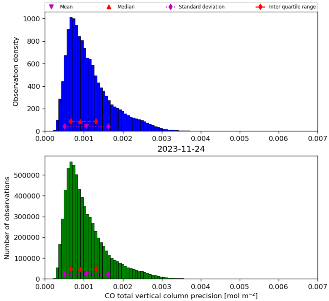
Figure 20: Histogram of “CO total vertical column precision” for 2023-11-23 to 2023-11-25
