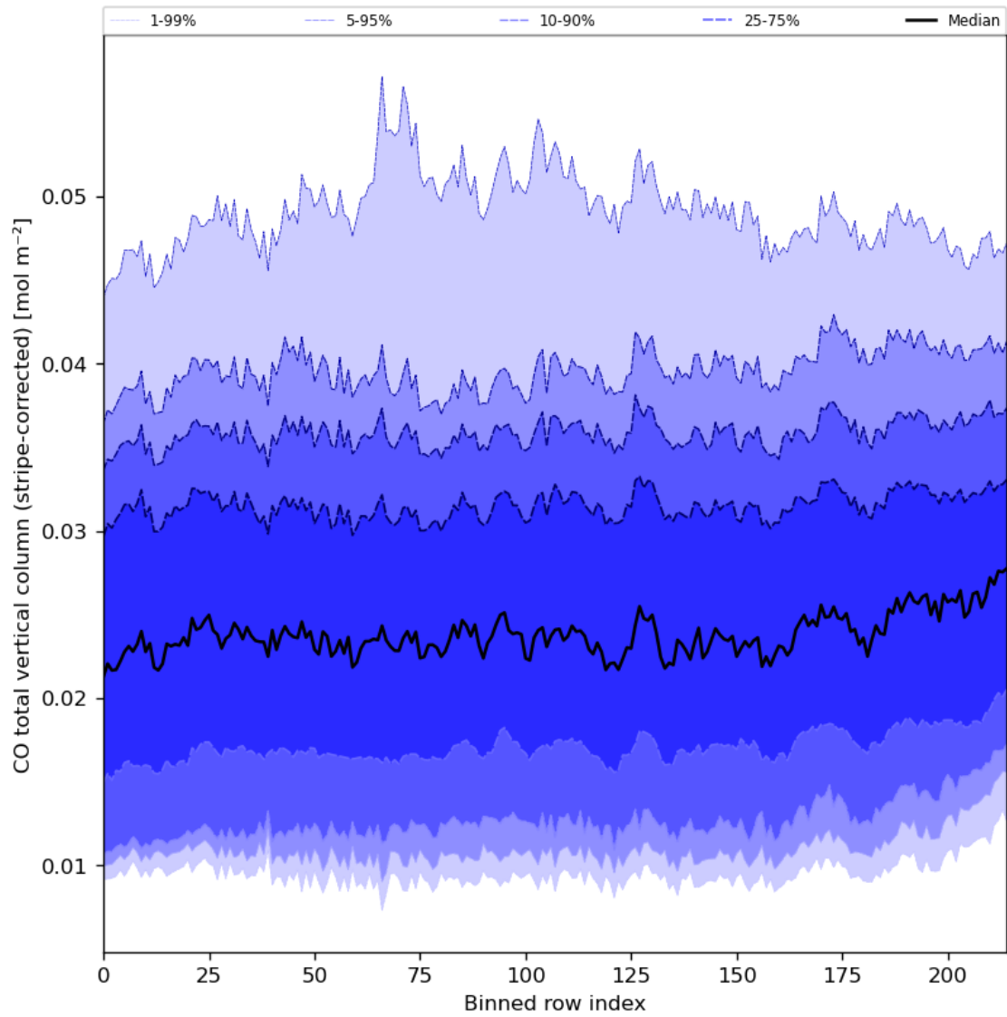
Figure 27: Along track statistics of “CO total vertical column (stripe-corrected)” for 2023-11-23 to 2023-11-25
