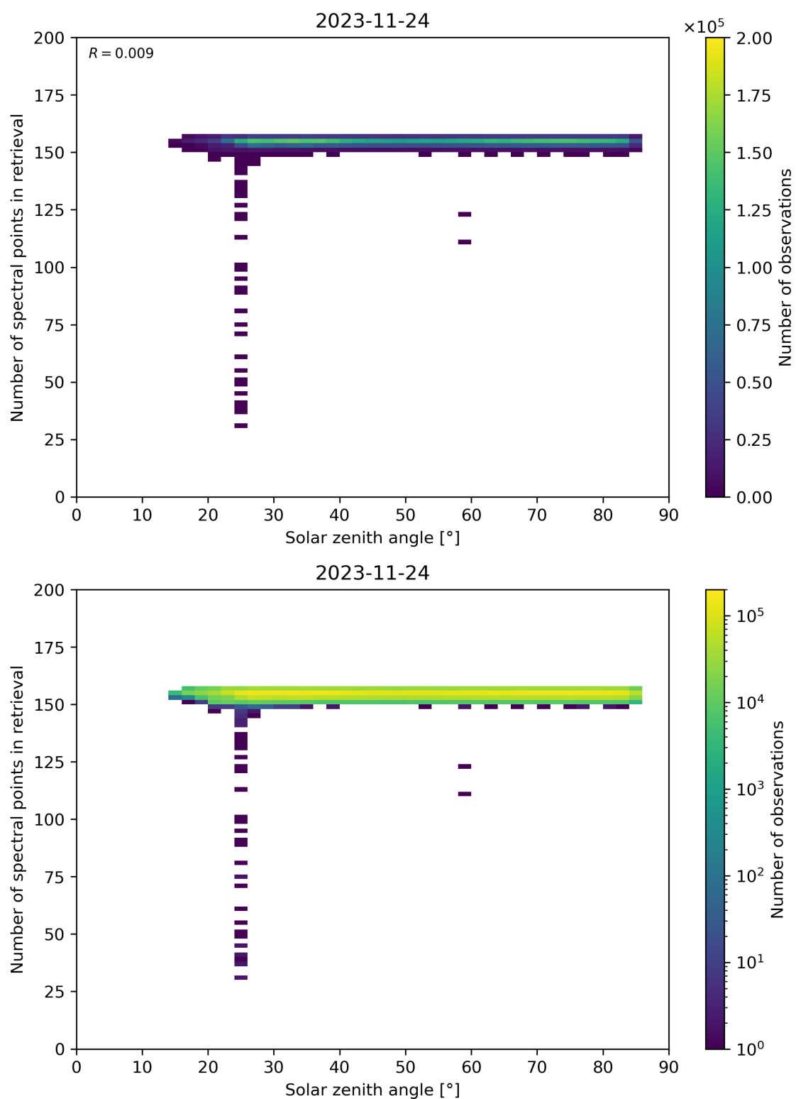
Figure 68: Scatter density plot of “Solar zenith angle” against “Number of spectral points in retrieval” for 2023-11-23 to 2023-11-25.
