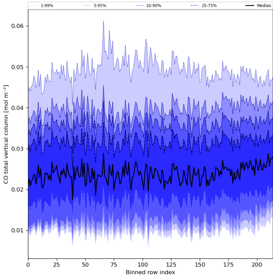
Figure 26: Along track statistics of “CO total vertical column” for 2023-11-23 to 2023-11-25
