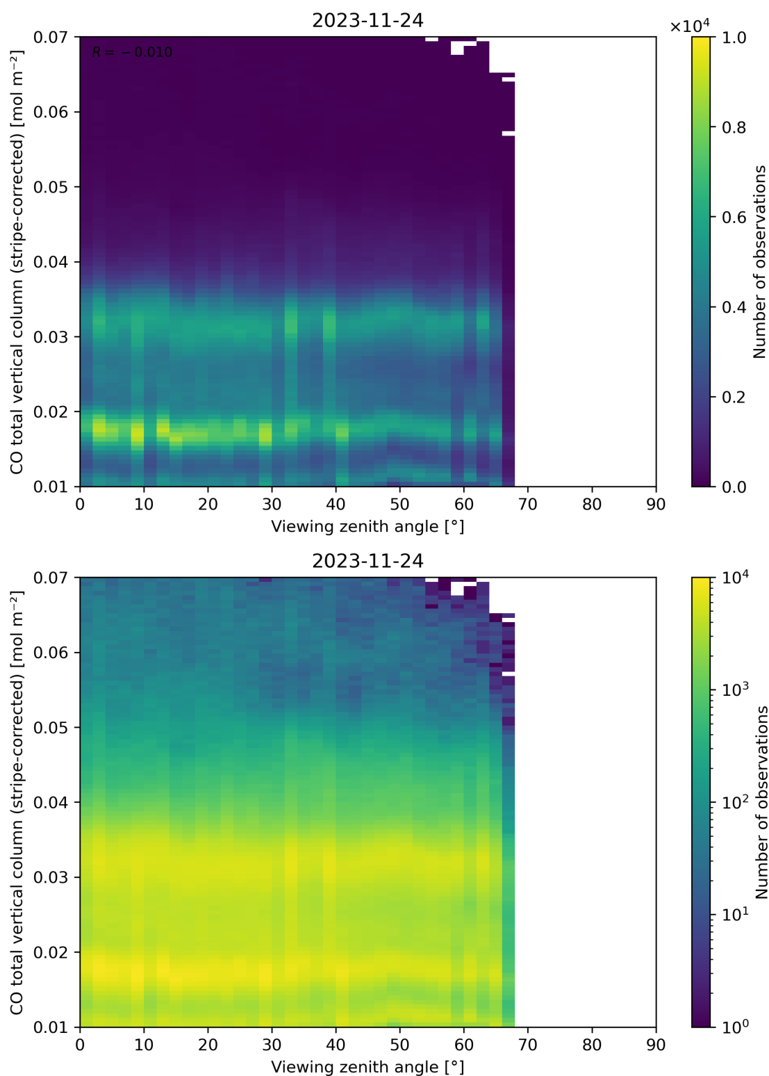
Figure 70: Scatter density plot of “Viewing zenith angle” against “CO total vertical column (stripe-corrected)” for 2023-11-23 to 2023-11-25.
