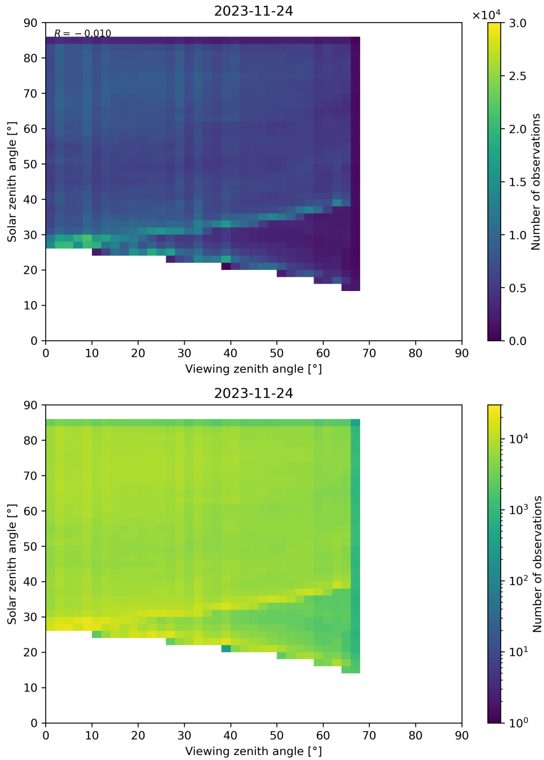
Figure 77: Scatter density plot of “Viewing zenith angle” against “Solar zenith angle” for 2023-11-23 to 2023-11-25.
