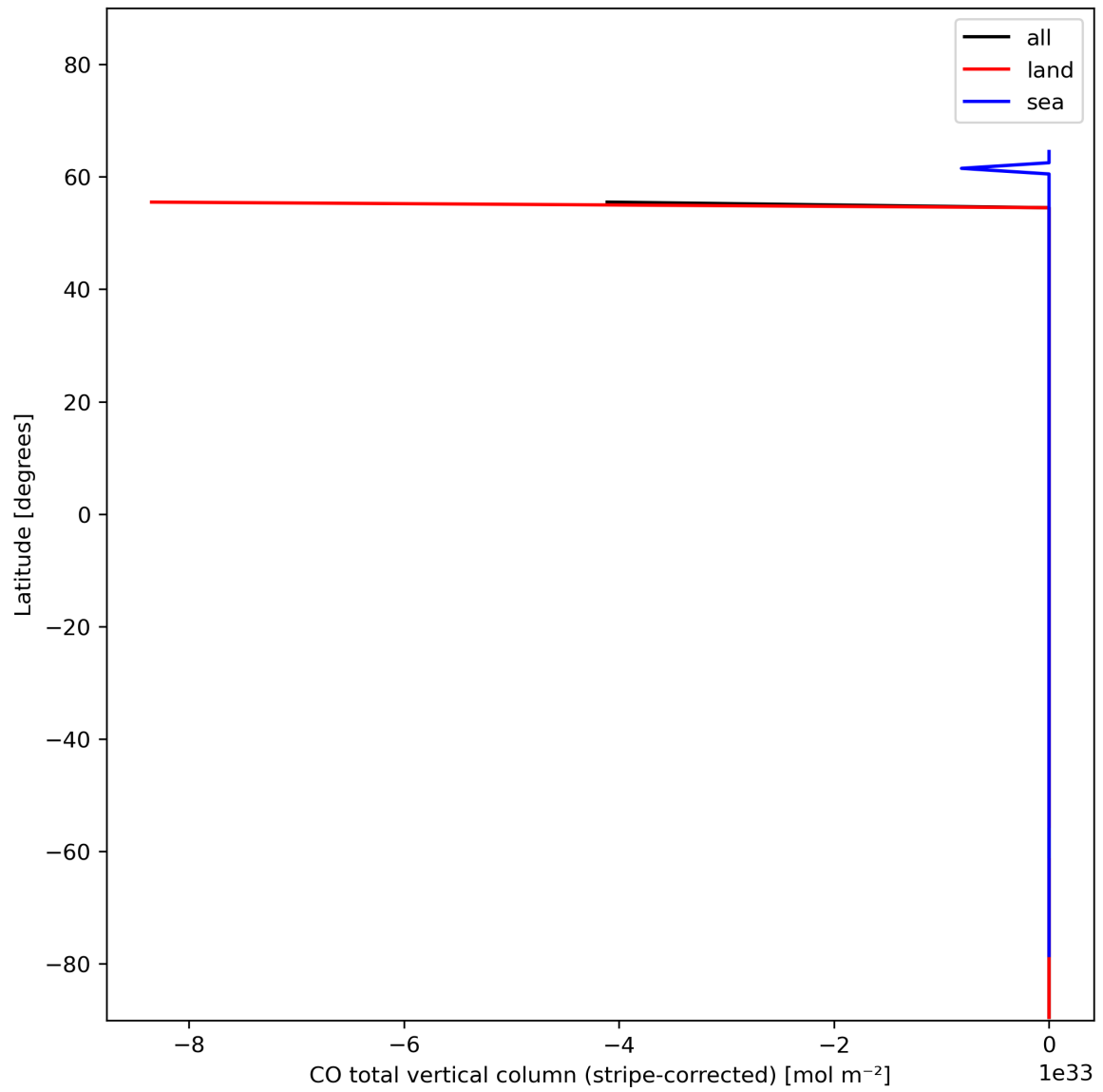
Figure 11: Zonal average of “CO total vertical column (stripe-corrected)” for 2023-11-23 to 2023-11-25.
