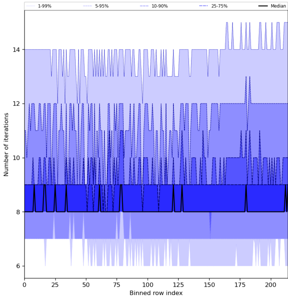
Figure 32: Along track statistics of “Number of iterations” for 2023-11-23 to 2023-11-25
