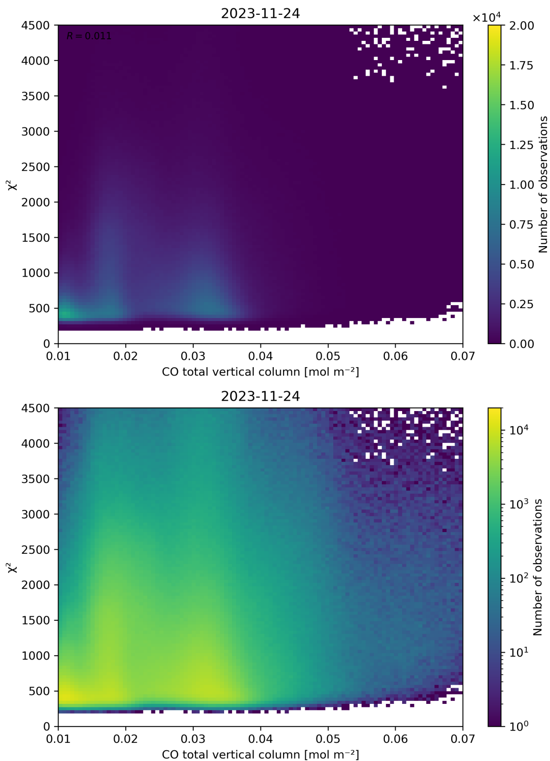
Figure 35: Scatter density plot of “CO total vertical column” against “ \chi^2 ” for 2023-11-23 to 2023-11-25.
