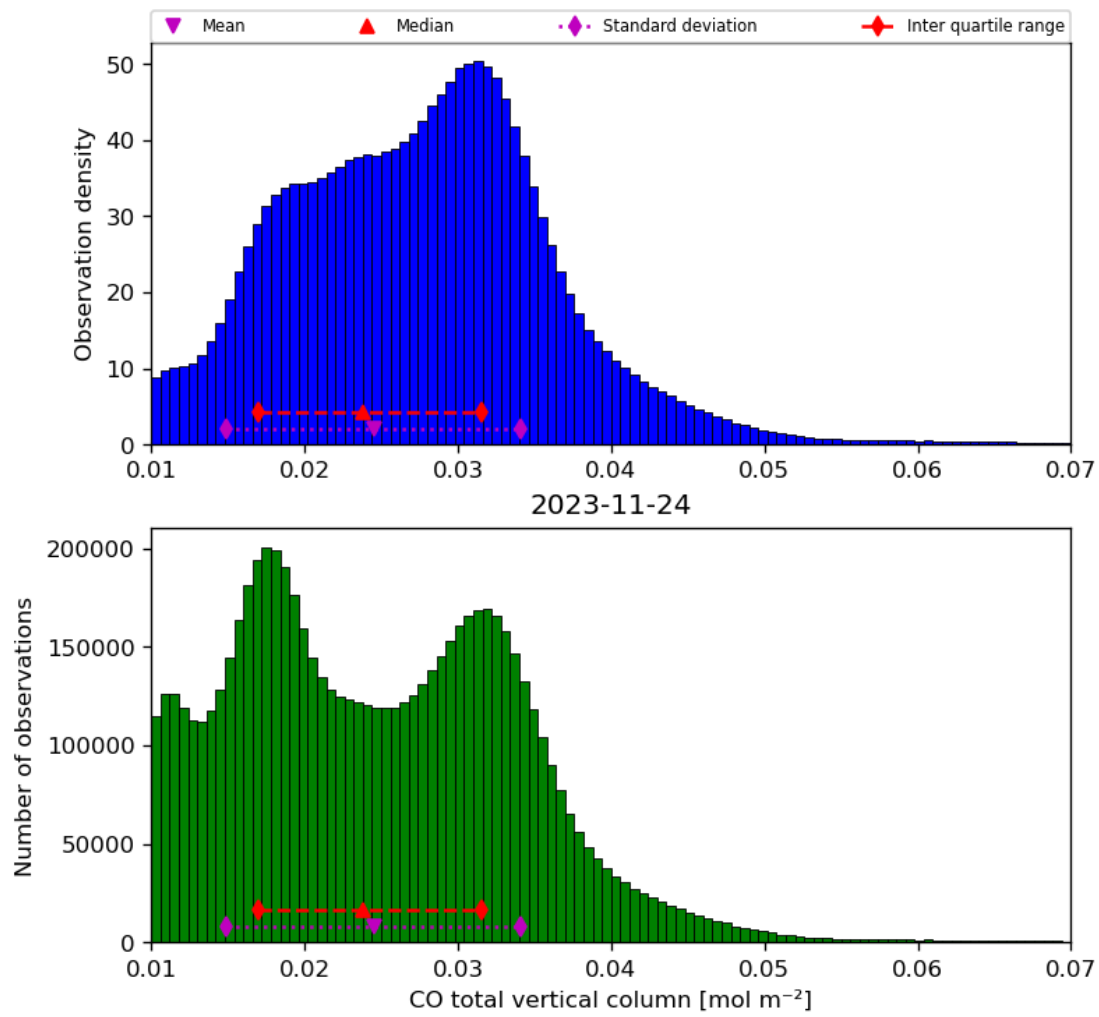
Figure 18: Histogram of “CO total vertical column” for 2023-11-23 to 2023-11-25
