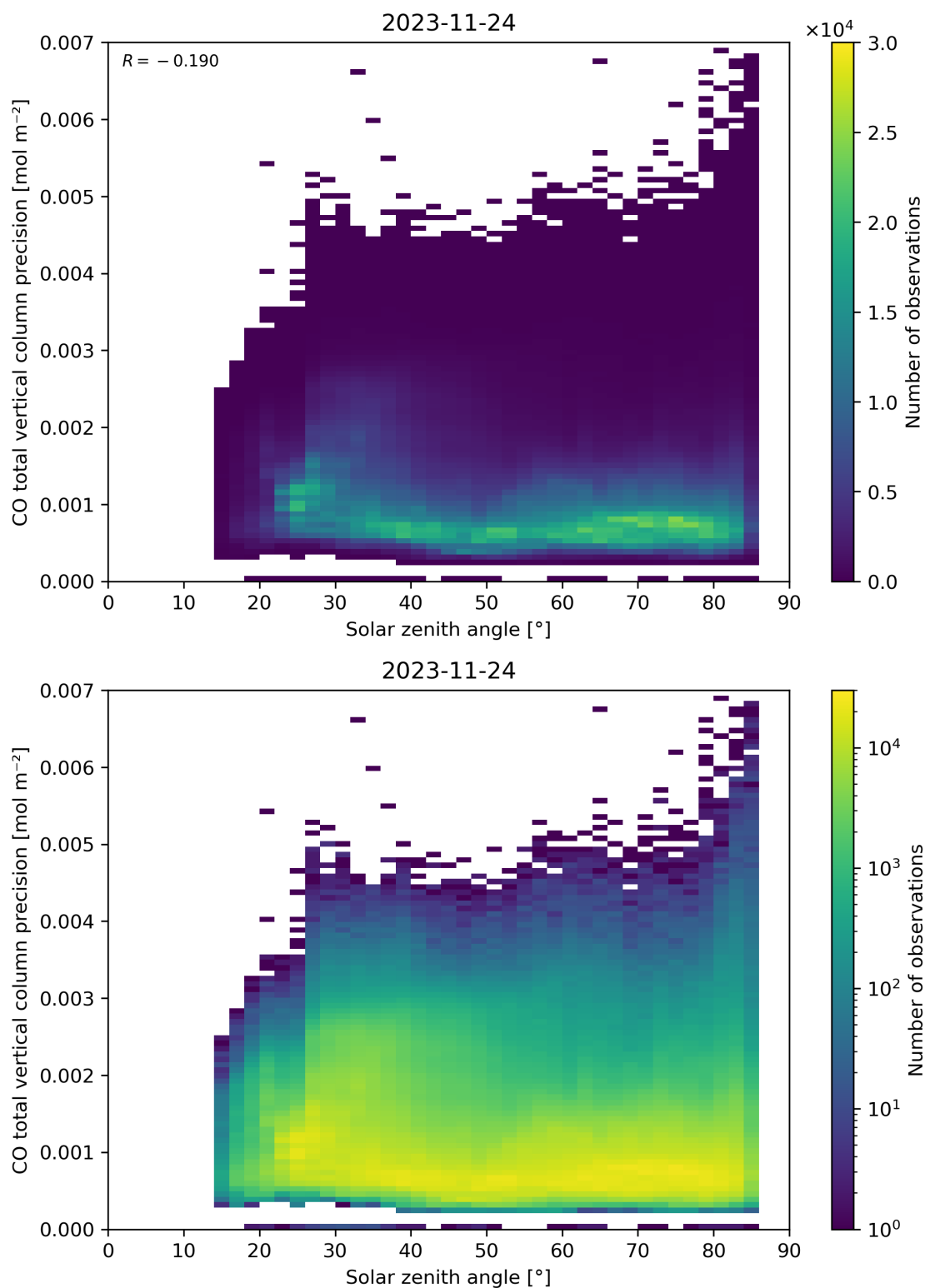
Figure 63: Scatter density plot of “Solar zenith angle” against “CO total vertical column precision” for 2023-11-23 to 2023-11-25.
