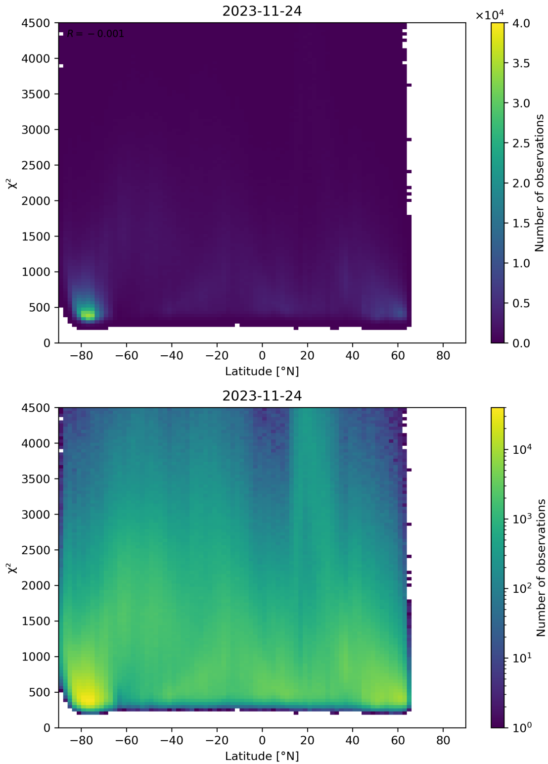
Figure 54: Scatter density plot of “Latitude” against “ \chi^2 ” for 2023-11-23 to 2023-11-25.
