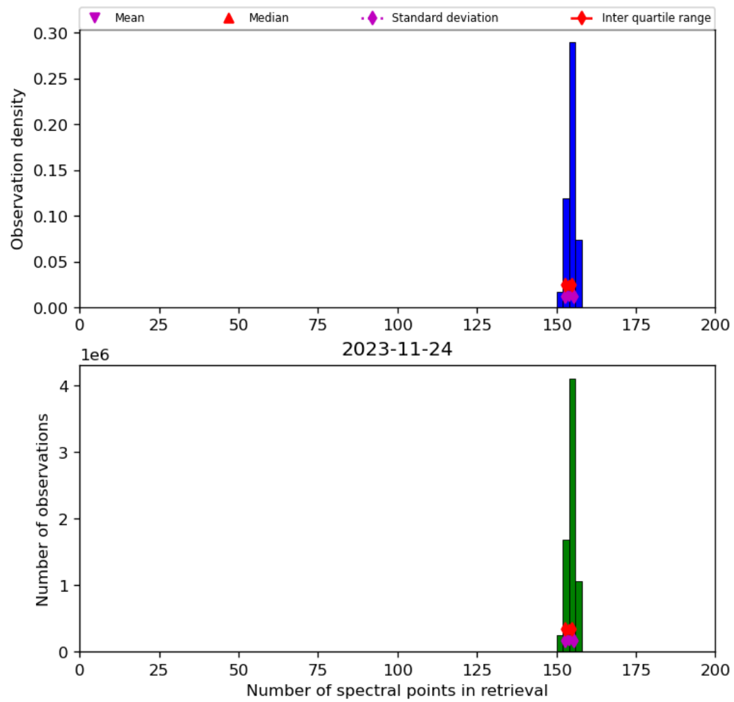
Figure 21: Histogram of “Number of spectral points in retrieval” for 2023-11-23 to 2023-11-25
