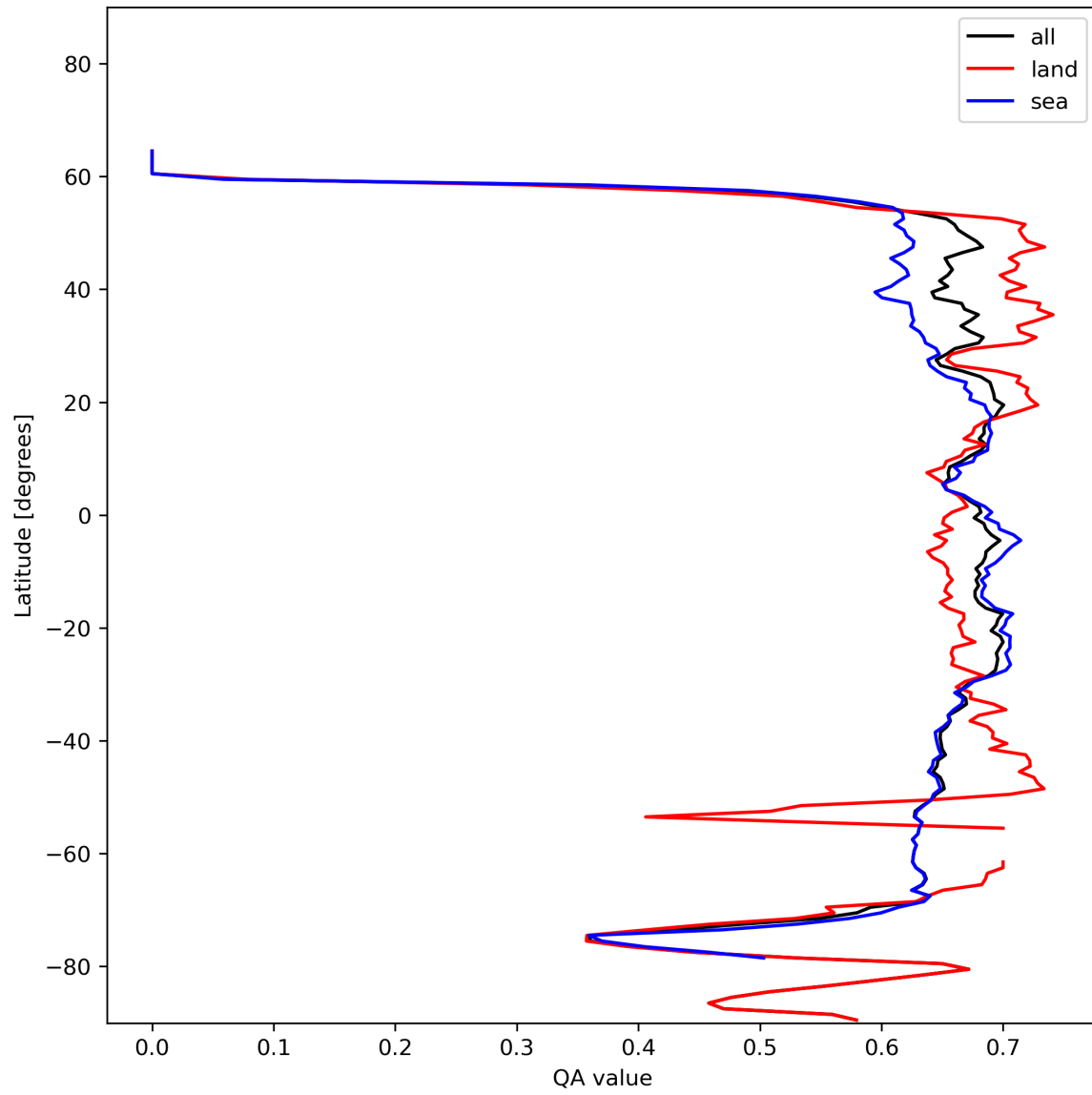
Figure 9: Zonal average of “QA value” for 2023-11-23 to 2023-11-25.
