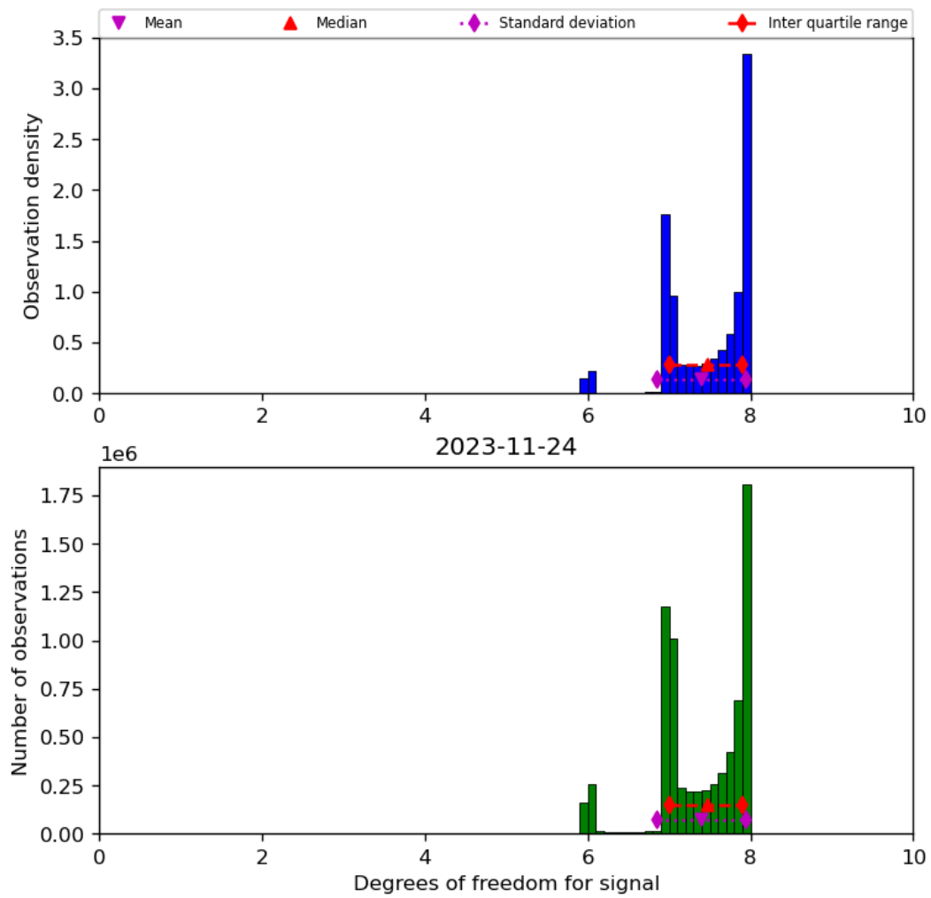
Figure 23: Histogram of “Degrees of freedom for signal” for 2023-11-23 to 2023-11-25
