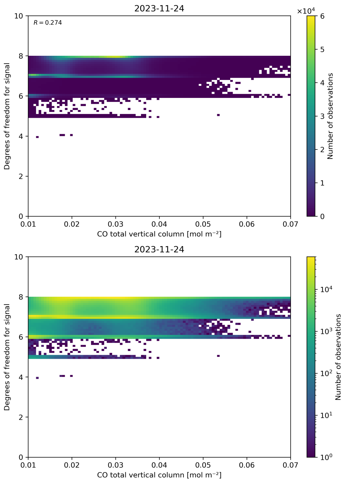
Figure 41: Scatter density plot of “CO total vertical column” against “Degrees of freedom for signal” for 2023-11-23 to 2023-11-25.
