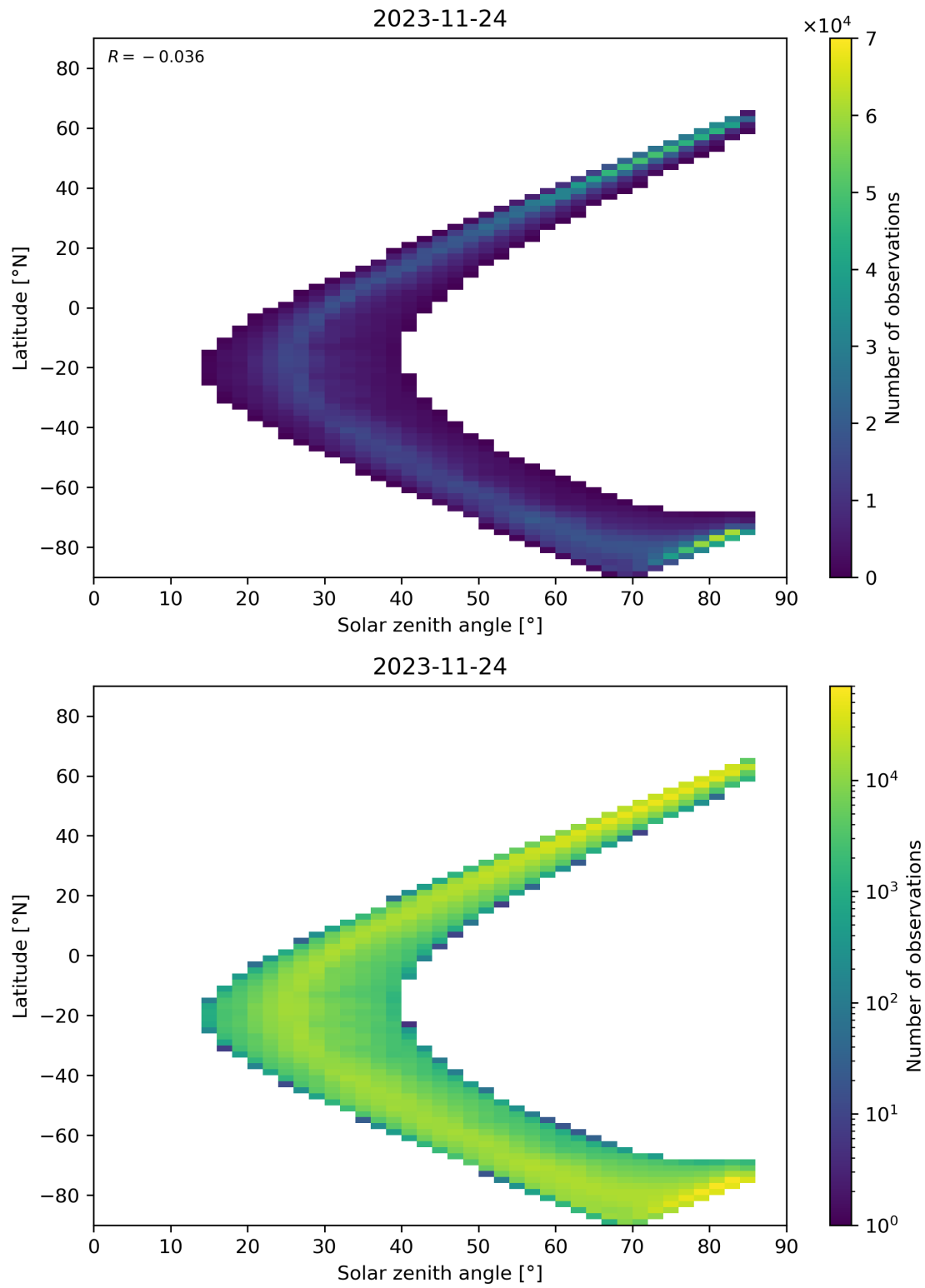
Figure 66: Scatter density plot of “Solar zenith angle” against “Latitude” for 2023-11-23 to 2023-11-25.
