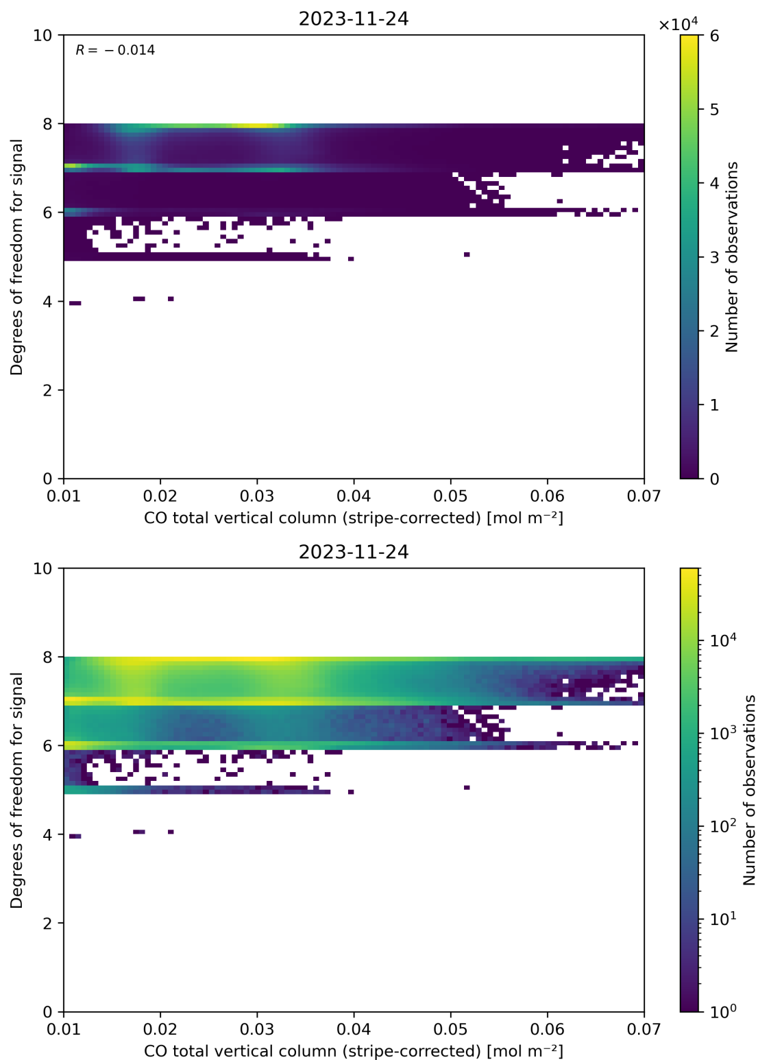
Figure 38: Scatter density plot of “CO total vertical column (stripe-corrected)” against “Degrees of freedom for signal” for 2023-11-23 to 2023-11-25.
