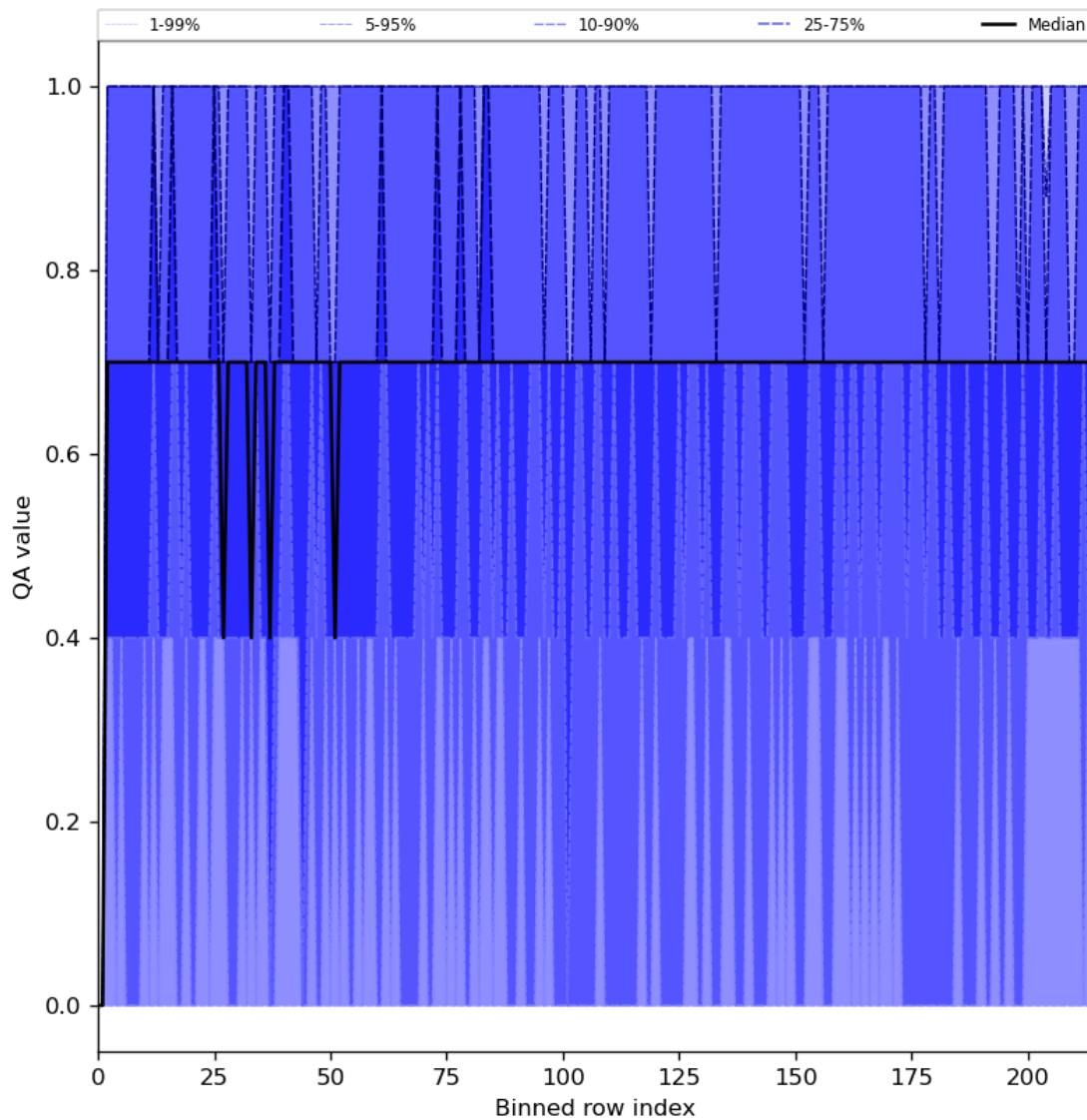
Figure 25: Along track statistics of “QA value” for 2023-11-23 to 2023-11-25
