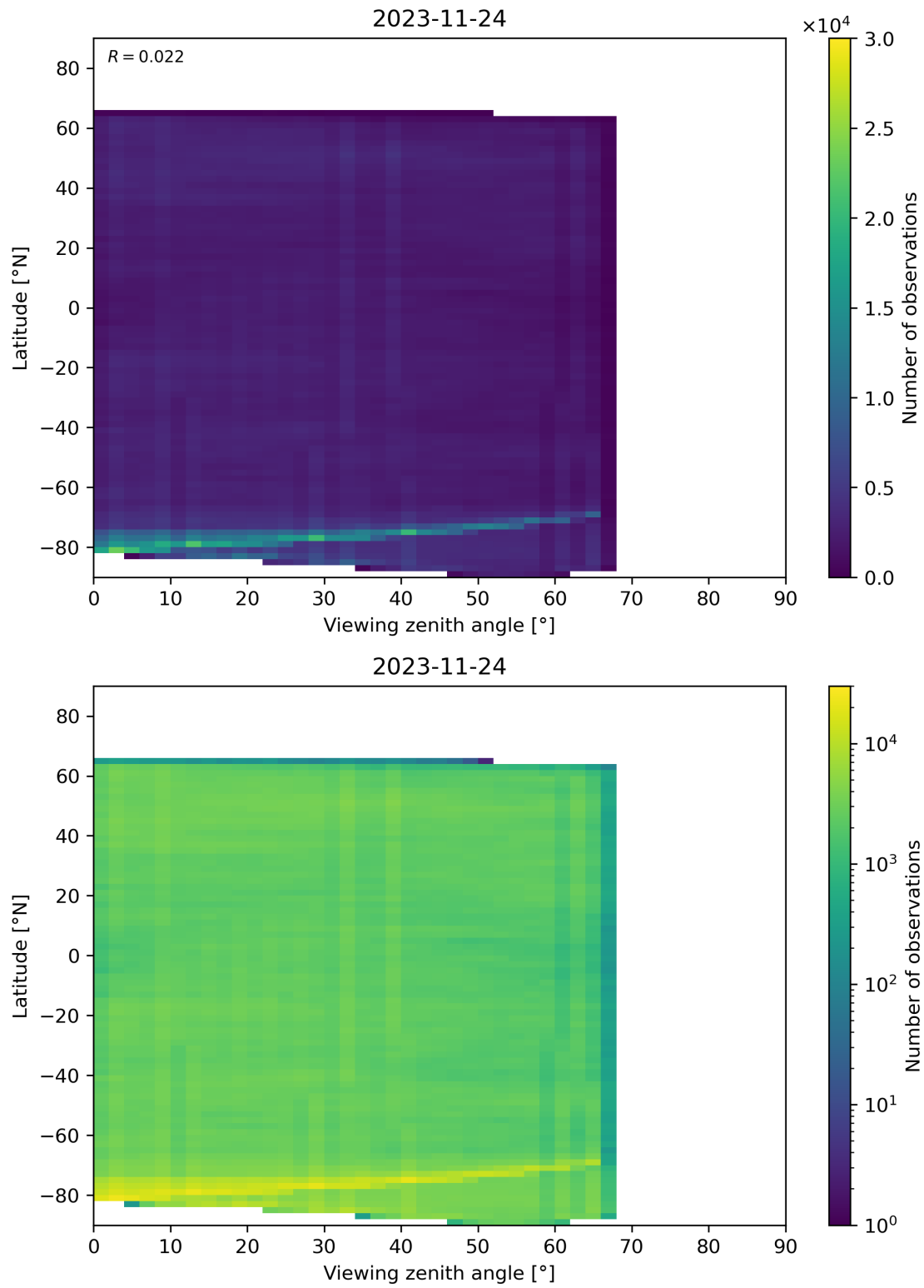
Figure 74: Scatter density plot of “Viewing zenith angle” against “Latitude” for 2023-11-23 to 2023-11-25.
