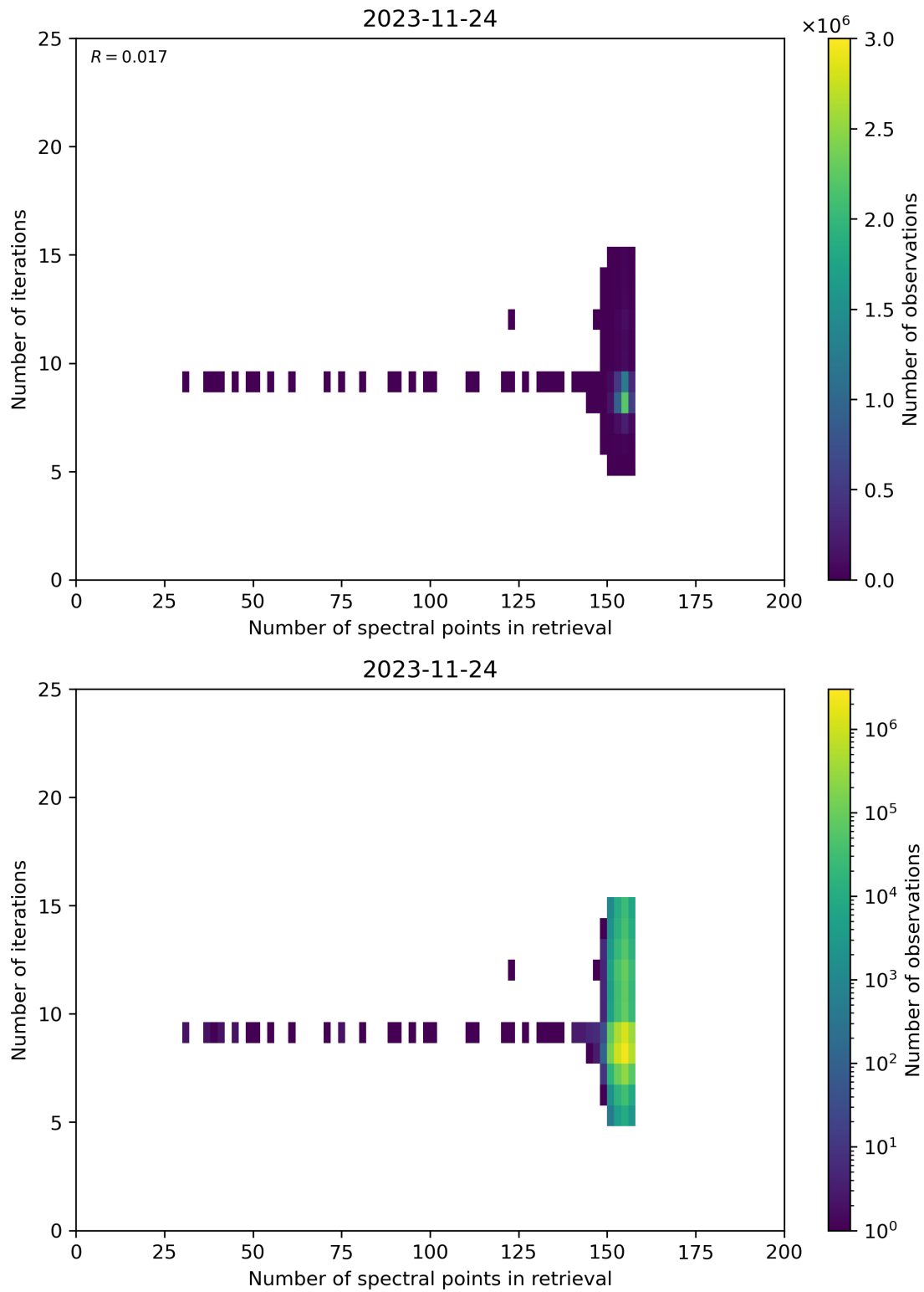
Figure 60: Scatter density plot of “Number of spectral points in retrieval” against “Number of iterations” for 2023-11-23 to 2023-11-25.
