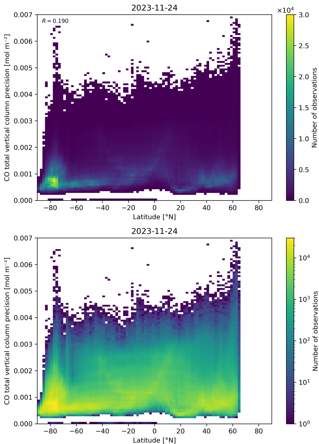
Figure 53: Scatter density plot of “Latitude” against “CO total vertical column precision” for 2023-11-23 to 2023-11-25.
