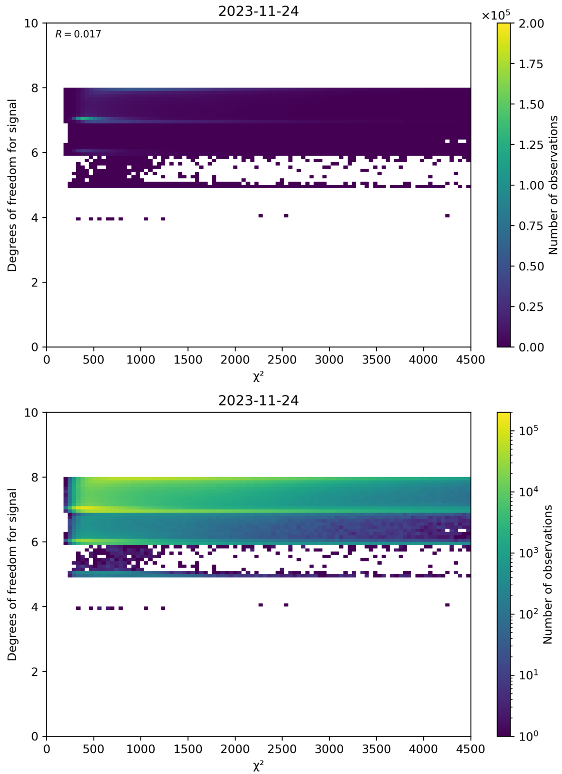
Figure 48: Scatter density plot of “ \chi^2 ” against “Degrees of freedom for signal” for 2023-11-23 to 2023-11-25.
