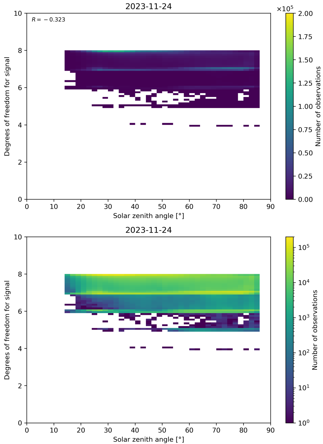
Figure 65: Scatter density plot of “Solar zenith angle” against “Degrees of freedom for signal” for 2023-11-23 to 2023-11-25.
