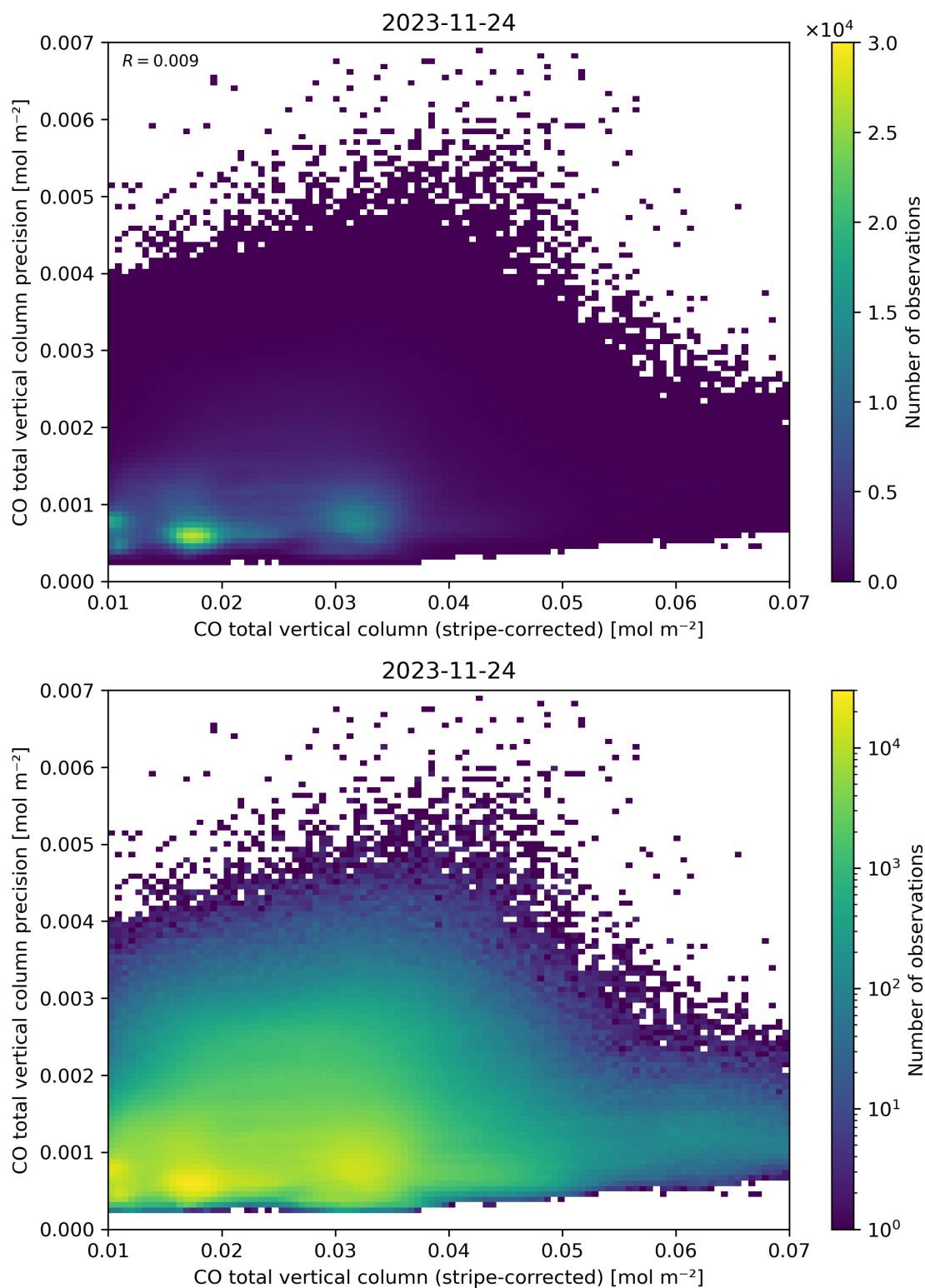
Figure 36: Scatter density plot of “CO total vertical column (stripe-corrected)” against “CO total vertical column precision” for 2023-11-23 to 2023-11-25.
