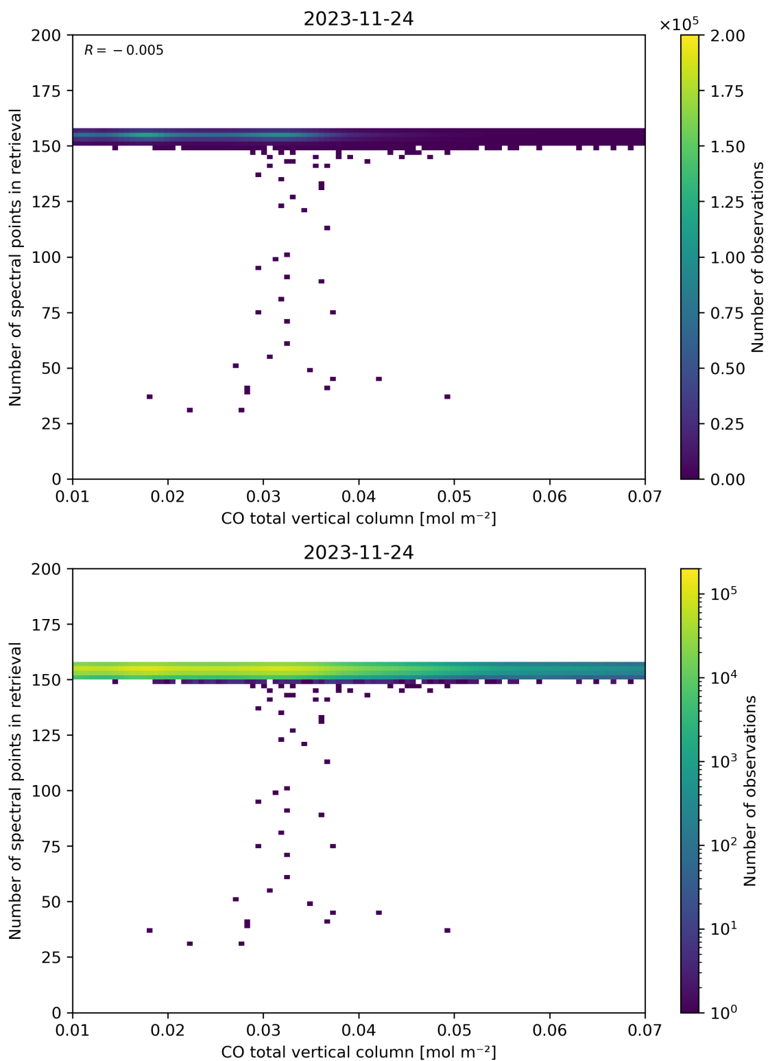
Figure 43: Scatter density plot of “CO total vertical column” against “Number of spectral points in retrieval” for 2023-11-23 to 2023-11-25.
