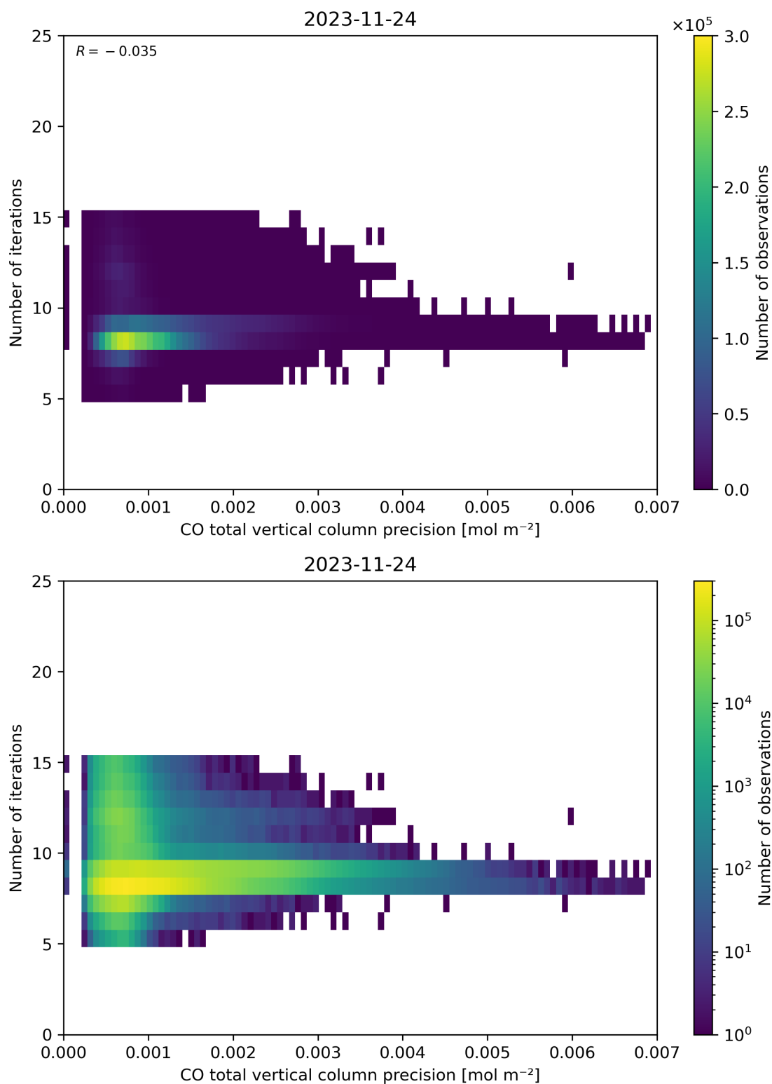
Figure 46: Scatter density plot of “CO total vertical column precision” against “Number of iterations” for 2023-11-23 to 2023-11-25.
