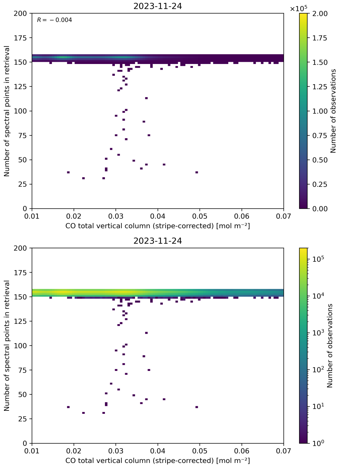
Figure 40: Scatter density plot of “CO total vertical column (stripe-corrected)” against “Number of spectral points in retrieval” for 2023-11-23 to 2023-11-25.
