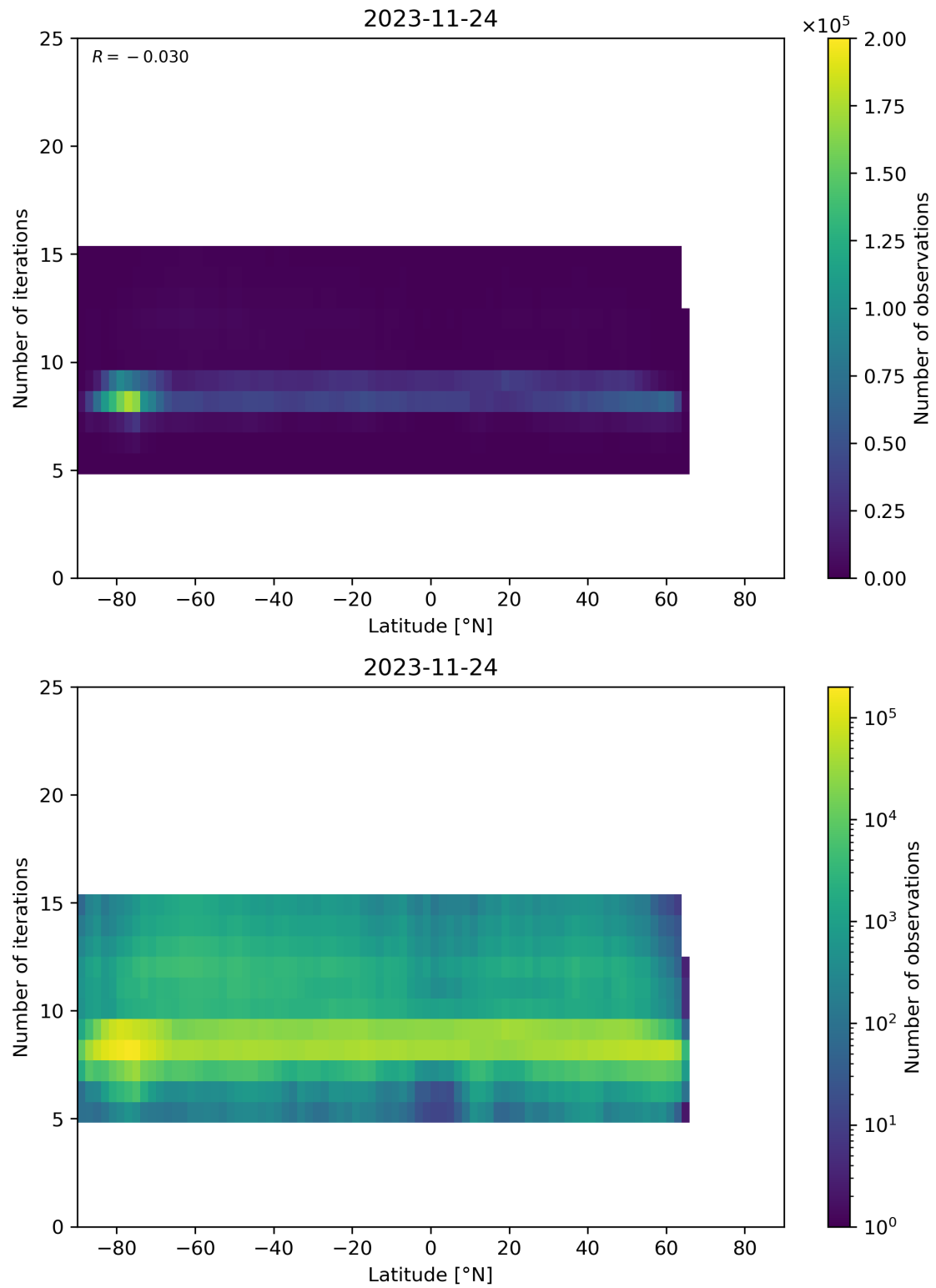
Figure 56: Scatter density plot of “Latitude” against “Number of iterations” for 2023-11-23 to 2023-11-25.
