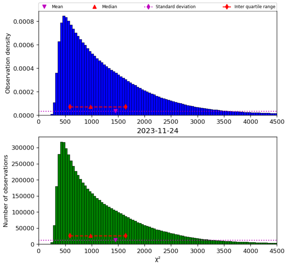
Figure 22: Histogram of “ \chi^2 ” for 2023-11-23 to 2023-11-25
