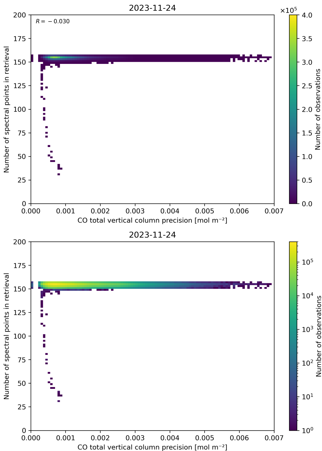
Figure 47: Scatter density plot of “CO total vertical column precision” against “Number of spectral points in retrieval” for 2023-11-23 to 2023-11-25.
