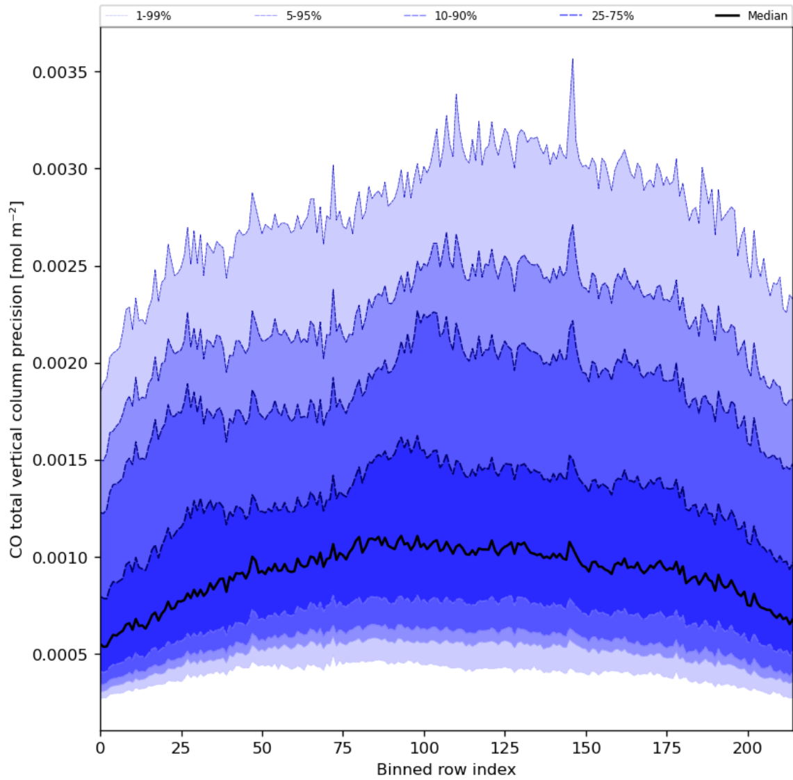
Figure 28: Along track statistics of “CO total vertical column precision” for 2023-11-23 to 2023-11-25
