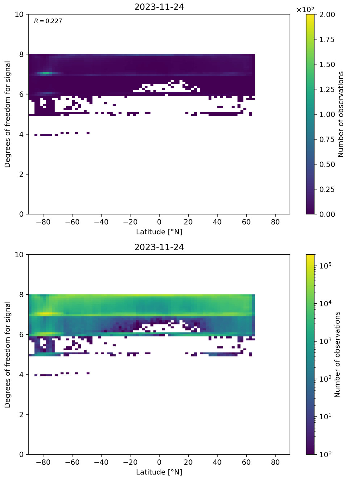
Figure 55: Scatter density plot of “Latitude” against “Degrees of freedom for signal” for 2023-11-23 to 2023-11-25.
