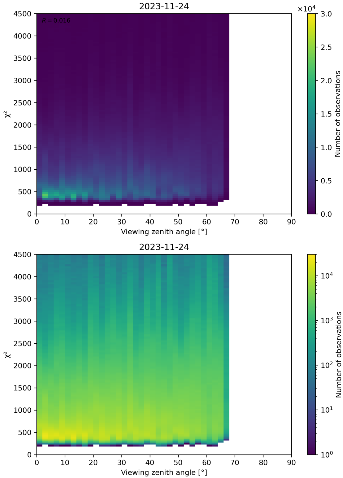
Figure 72: Scatter density plot of “Viewing zenith angle” against “ \chi^2 ” for 2023-11-23 to 2023-11-25.
