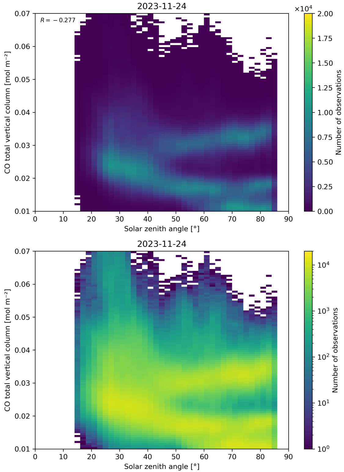
Figure 61: Scatter density plot of “Solar zenith angle” against “CO total vertical column” for 2023-11-23 to 2023-11-25.
