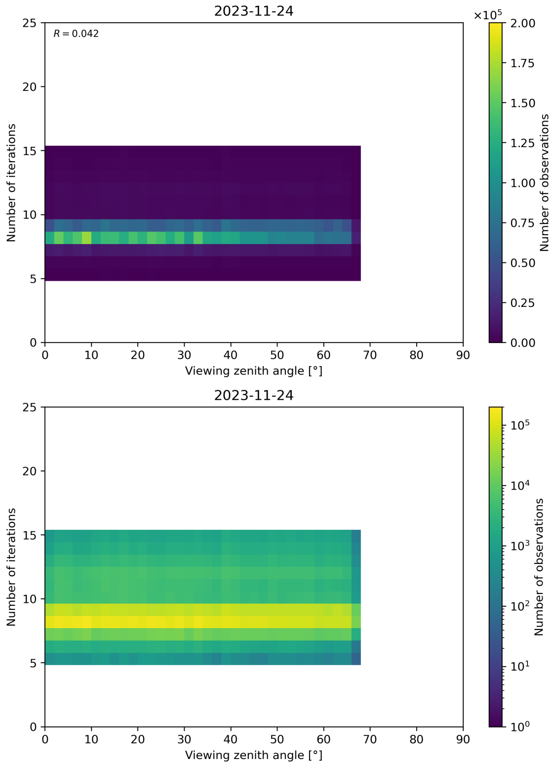
Figure 75: Scatter density plot of “Viewing zenith angle” against “Number of iterations” for 2023-11-23 to 2023-11-25.
