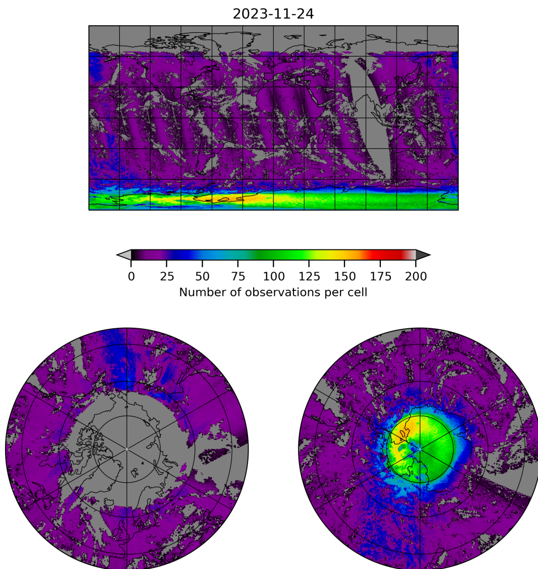
Figure 8: Map of the number of observations for 2023-11-23 to 2023-11-25
