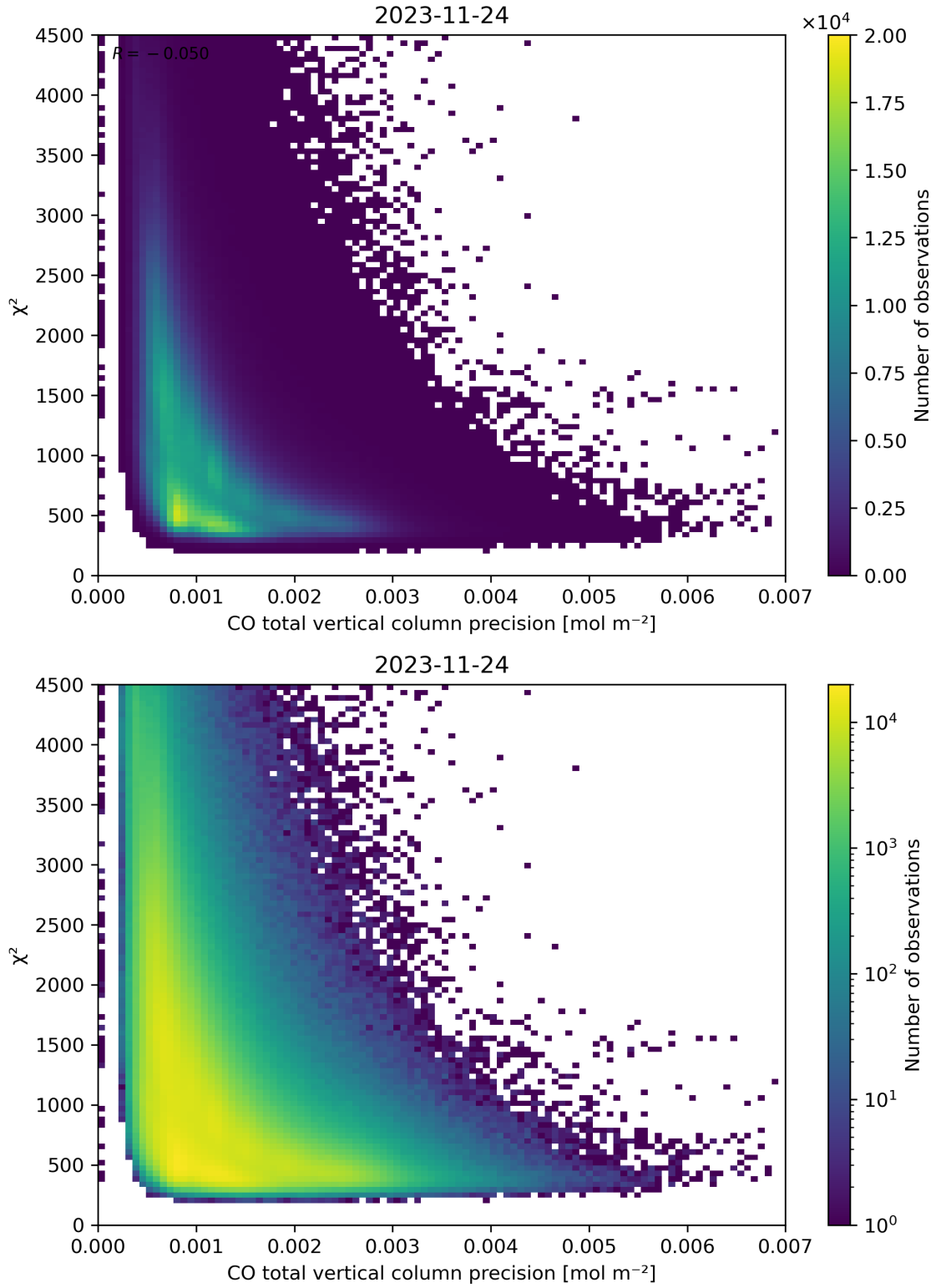
Figure 44: Scatter density plot of “CO total vertical column precision” against “ \chi^2 ” for 2023-11-23 to 2023-11-25.
