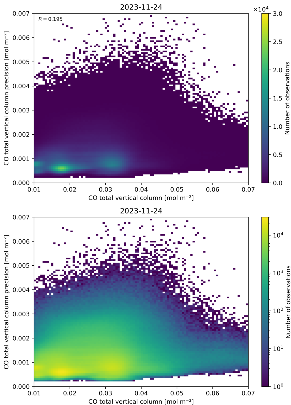
Figure 34: Scatter density plot of “CO total vertical column” against “CO total vertical column precision” for 2023-11-23 to 2023-11-25.
