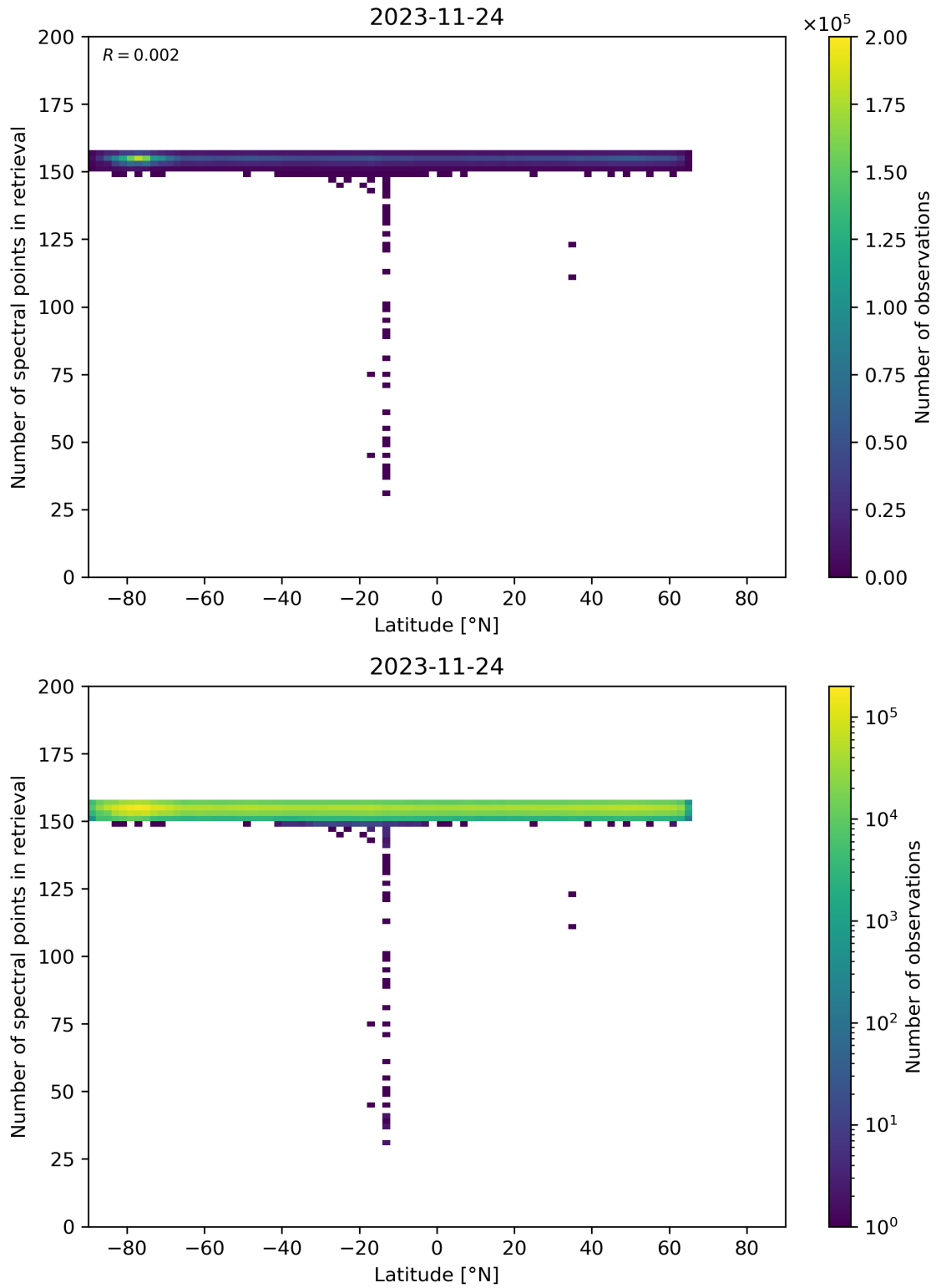
Figure 57: Scatter density plot of “Latitude” against “Number of spectral points in retrieval” for 2023-11-23 to 2023-11-25.
