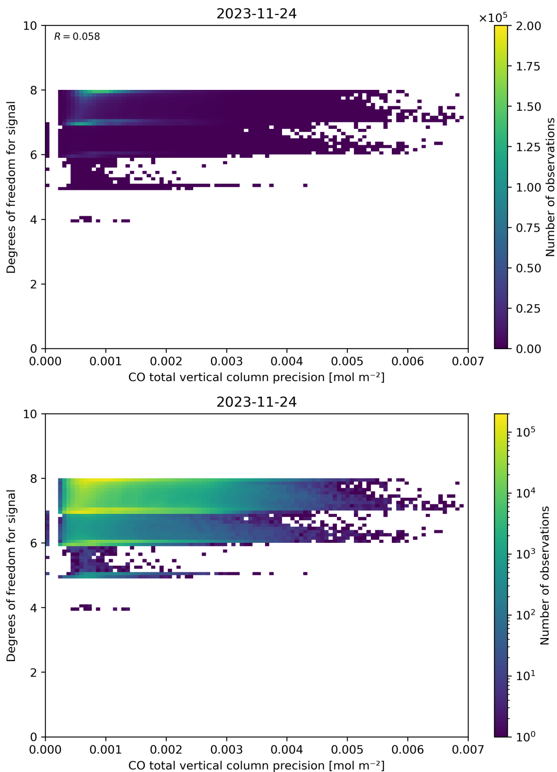
Figure 45: Scatter density plot of “CO total vertical column precision” against “Degrees of freedom for signal” for 2023-11-23 to 2023-11-25.
