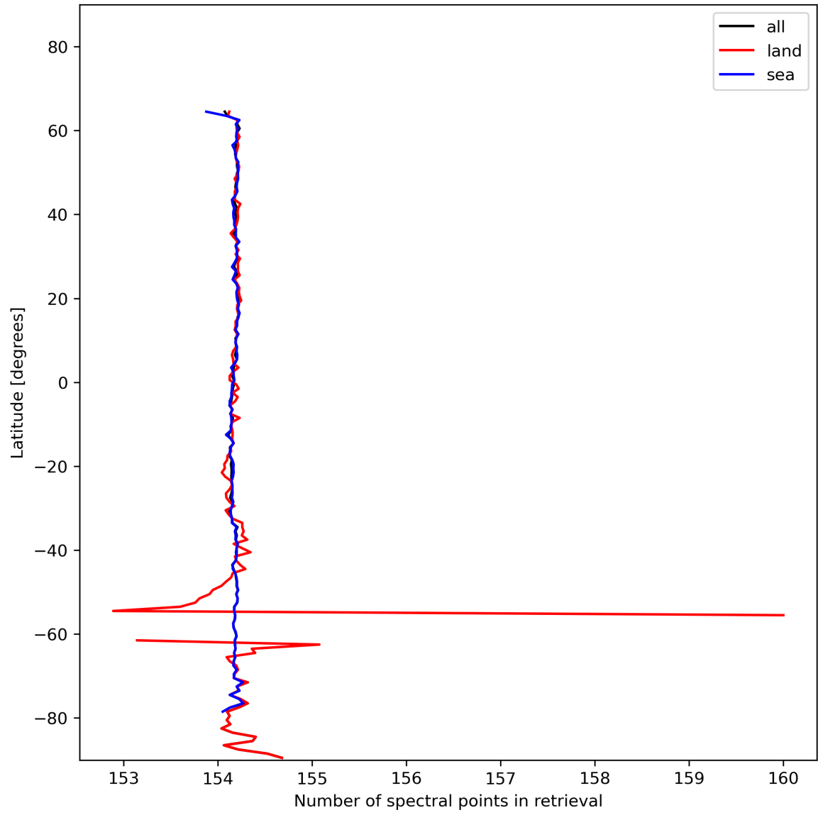
Figure 13: Zonal average of “Number of spectral points in retrieval” for 2023-11-23 to 2023-11-25.
