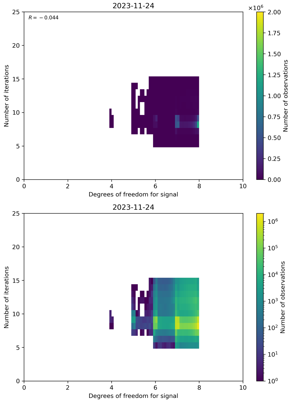
Figure 50: Scatter density plot of “Degrees of freedom for signal” against “Number of iterations” for 2023-11-23 to 2023-11-25.
