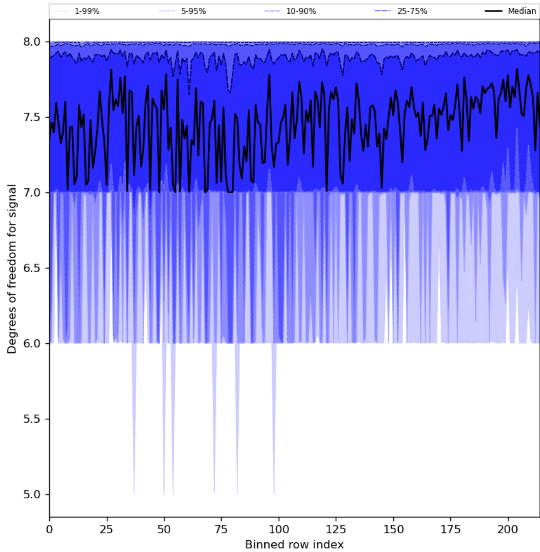
Figure 31: Along track statistics of “Degrees of freedom for signal” for 2023-11-23 to 2023-11-25
