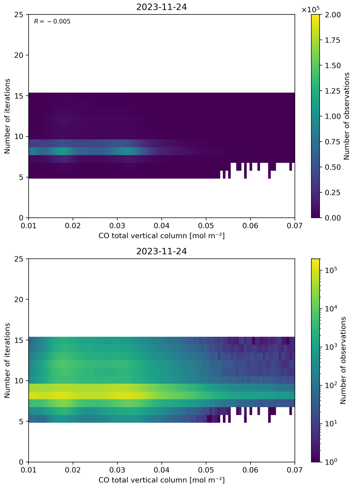
Figure 42: Scatter density plot of “CO total vertical column” against “Number of iterations” for 2023-11-23 to 2023-11-25.
