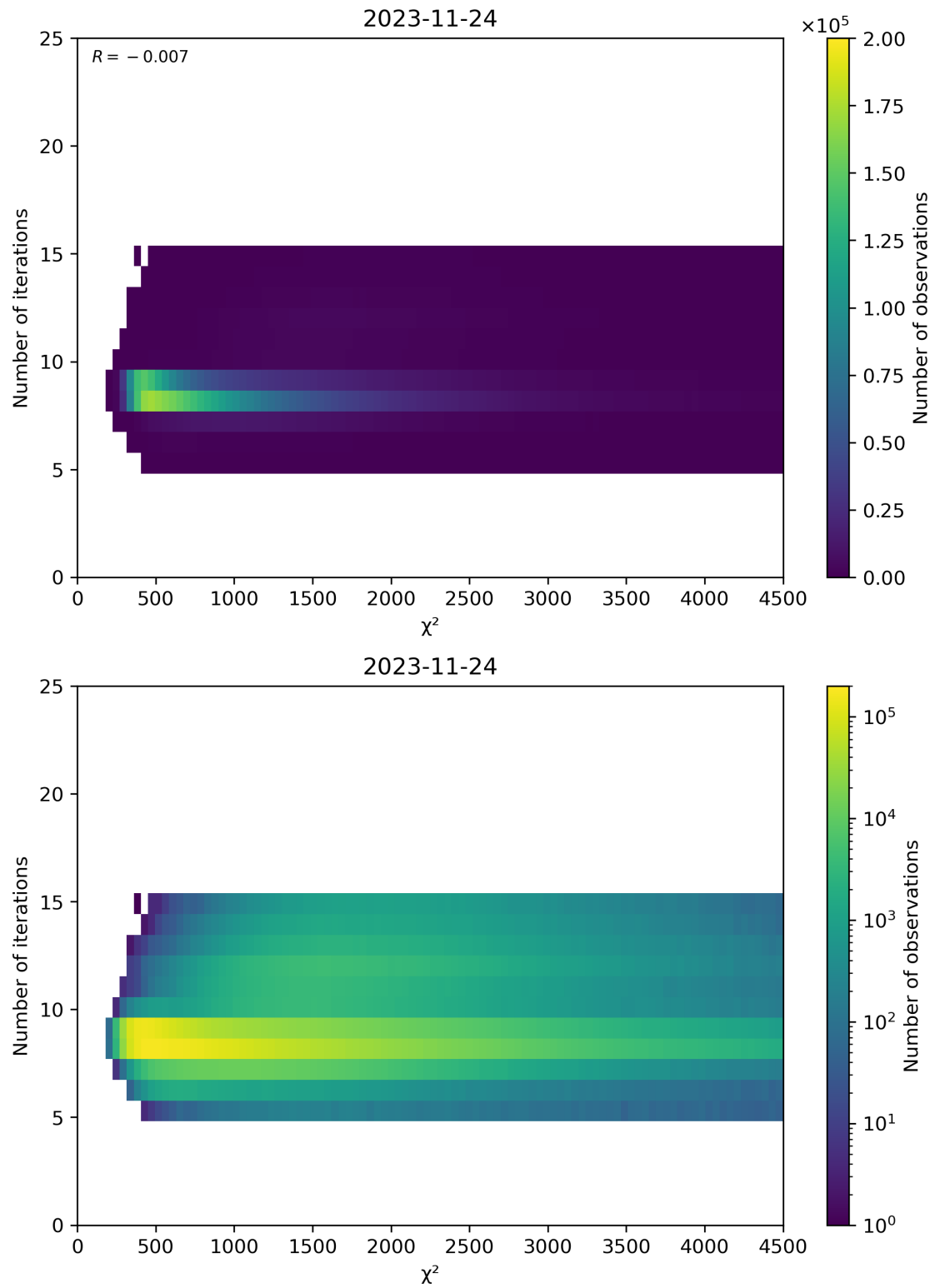
Figure 49: Scatter density plot of “ \chi^2 ” against “Number of iterations” for 2023-11-23 to 2023-11-25.
