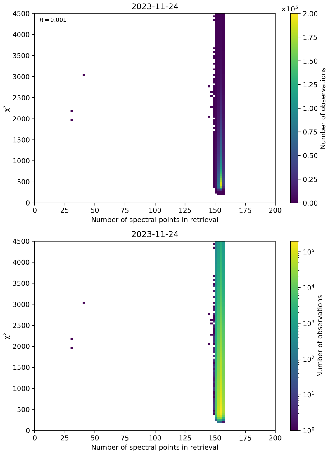
Figure 58: Scatter density plot of “Number of spectral points in retrieval” against “ \chi^2 ” for 2023-11-23 to 2023-11-25.
