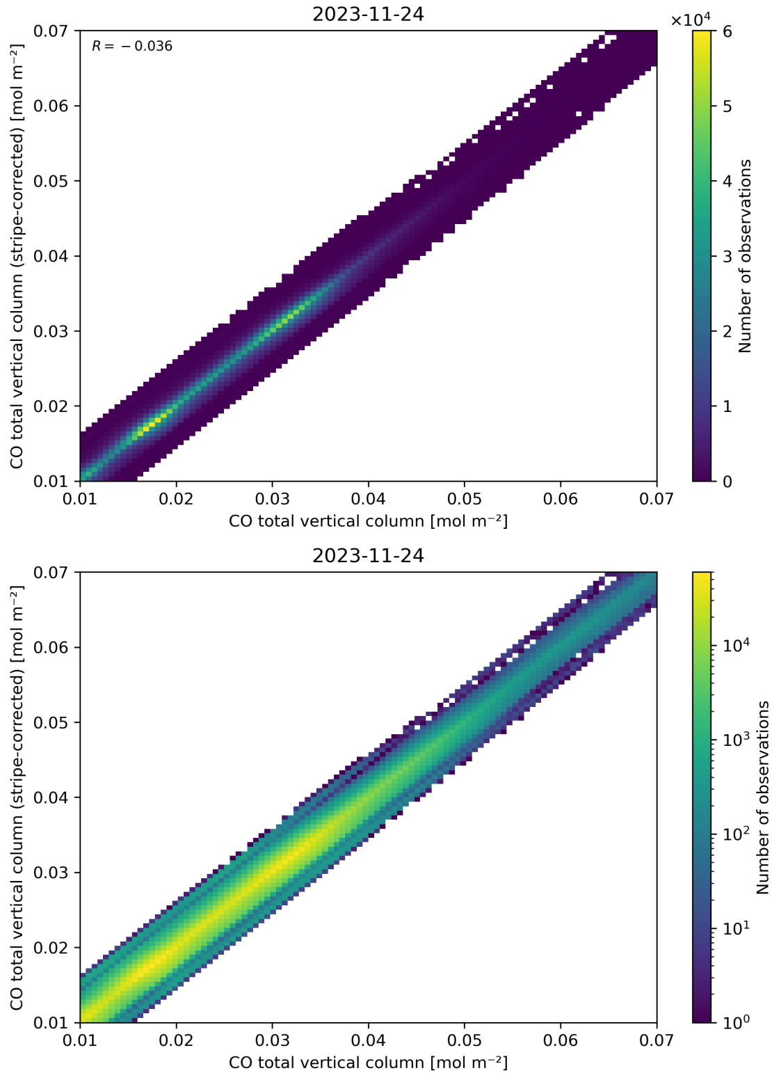
Figure 33: Scatter density plot of “CO total vertical column” against “CO total vertical column (stripe-corrected)” for 2023-11-23 to 2023-11-25.
