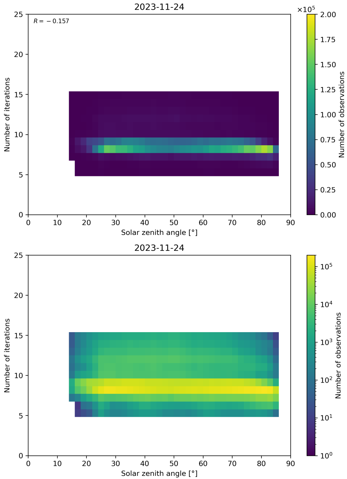
Figure 67: Scatter density plot of “Solar zenith angle” against “Number of iterations” for 2023-11-23 to 2023-11-25.
