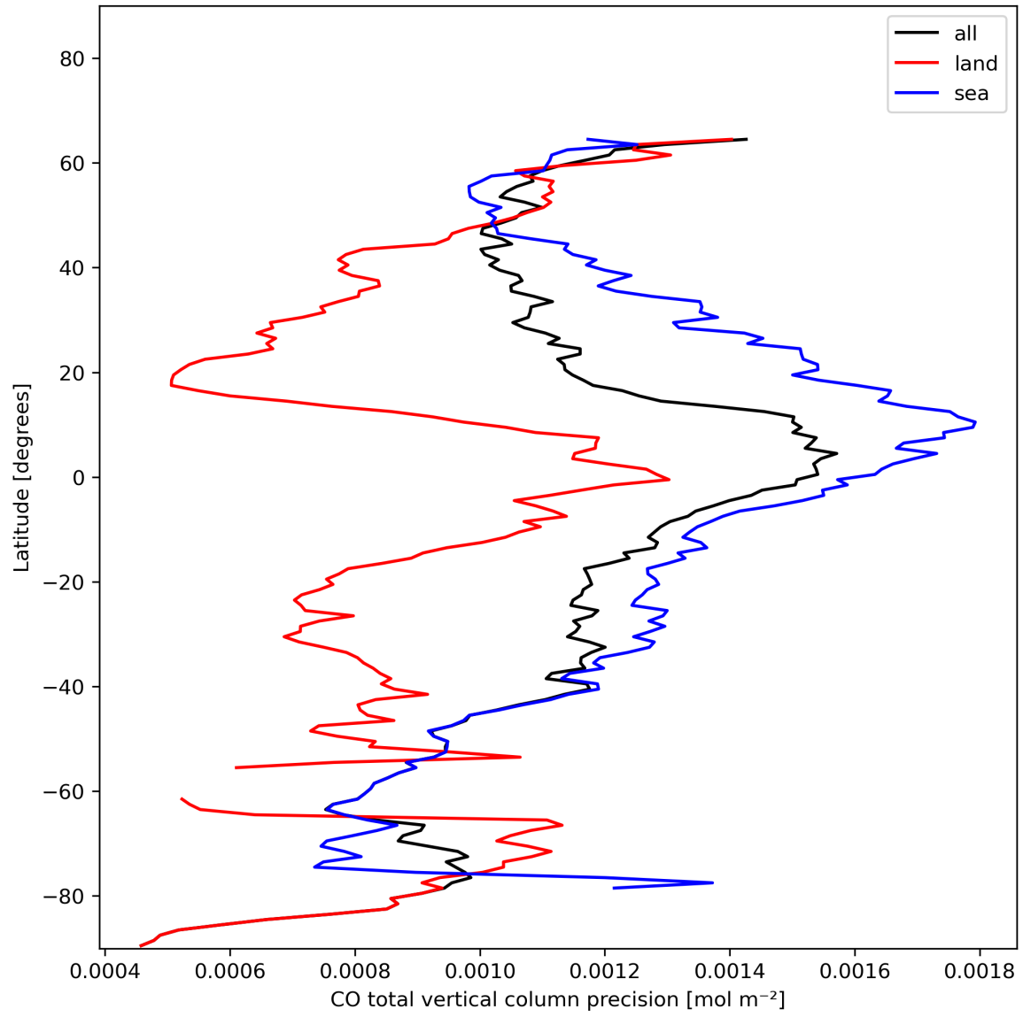
Figure 12: Zonal average of “CO total vertical column precision” for 2023-11-23 to 2023-11-25.
