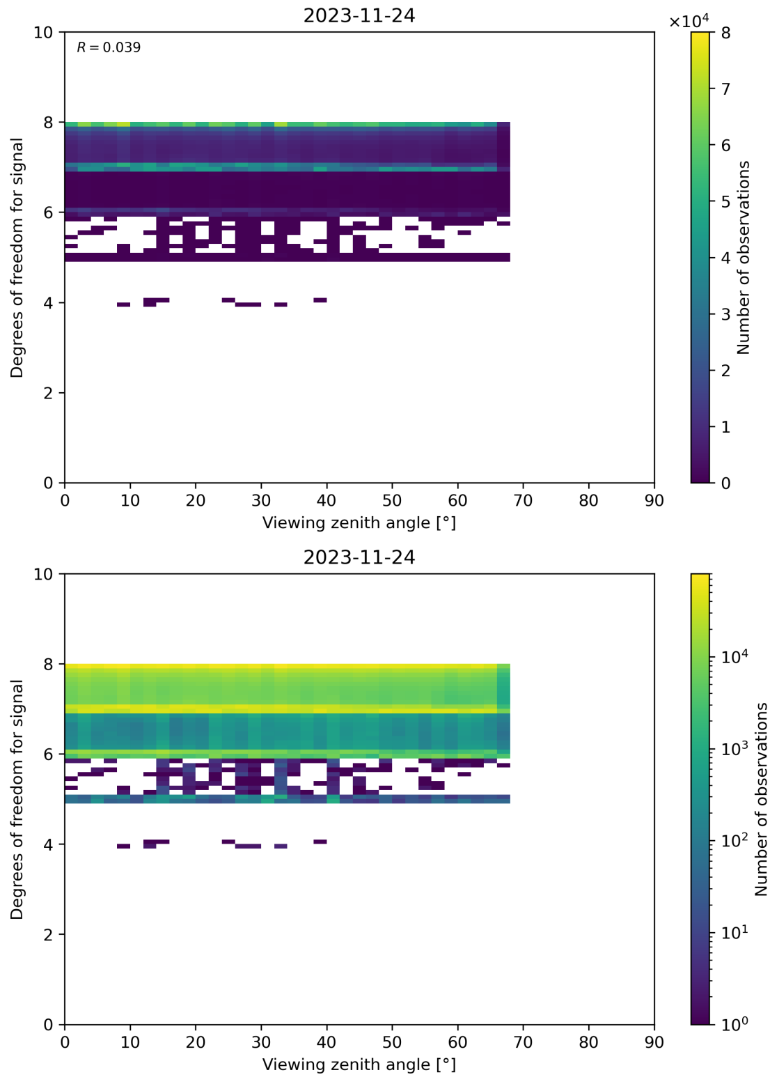
Figure 73: Scatter density plot of “Viewing zenith angle” against “Degrees of freedom for signal” for 2023-11-23 to 2023-11-25.
