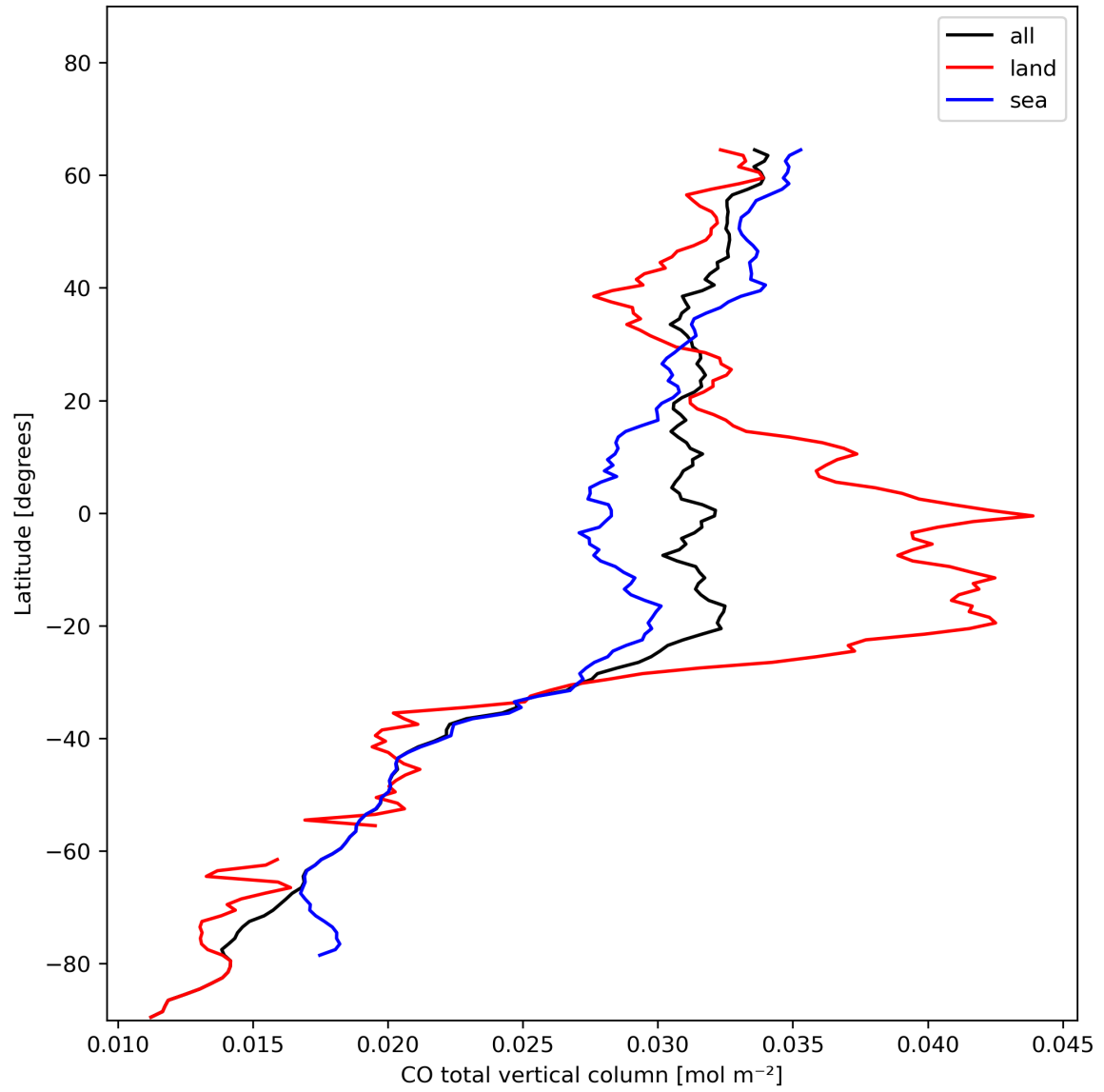
Figure 10: Zonal average of “CO total vertical column” for 2023-11-23 to 2023-11-25.
