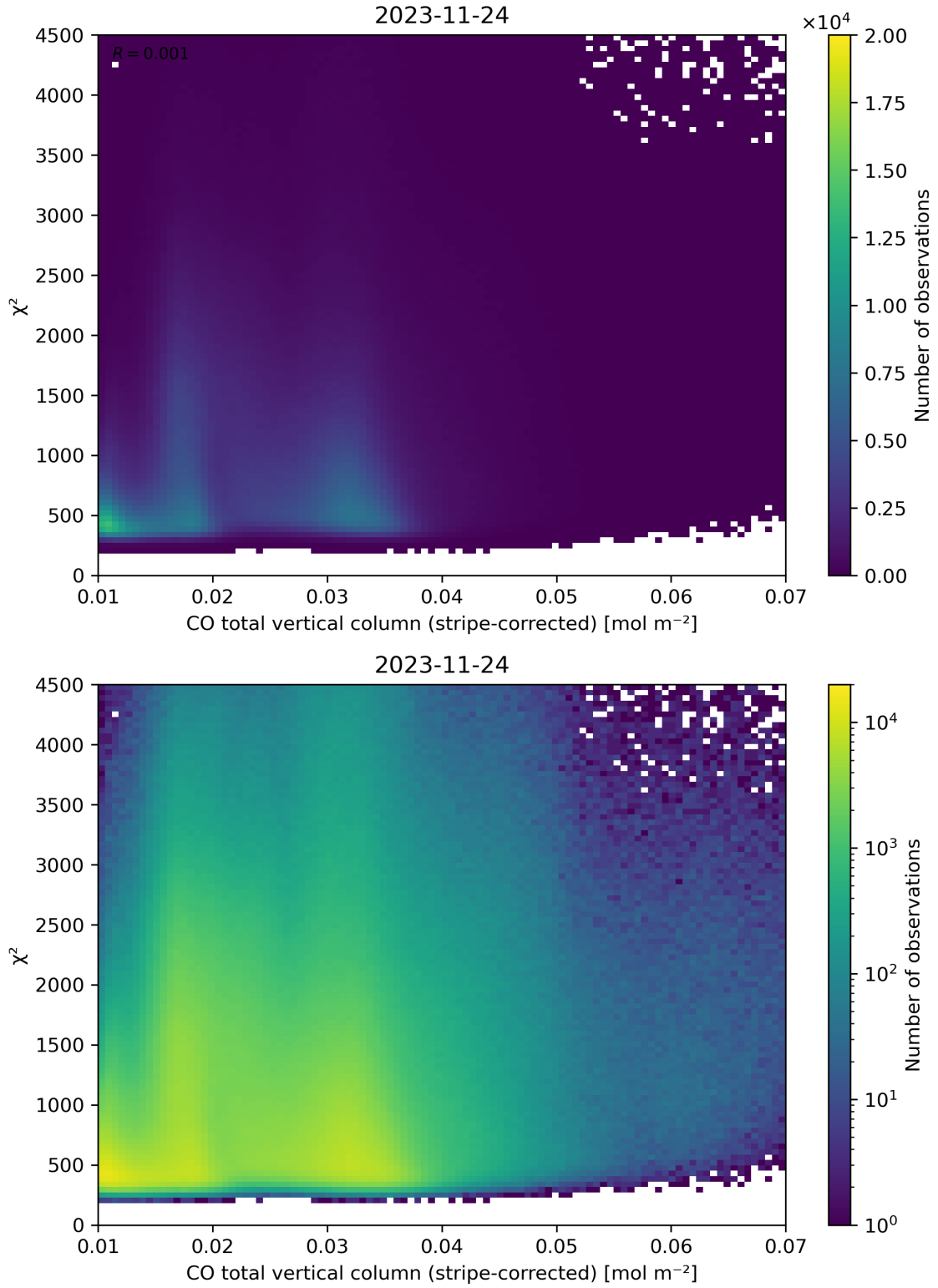
Figure 37: Scatter density plot of “CO total vertical column (stripe-corrected)” against “ \chi^2 ” for 2023-11-23 to 2023-11-25.
