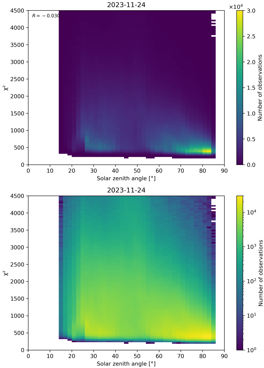
Figure 64: Scatter density plot of “Solar zenith angle” against “ \chi^2 ” for 2023-11-23 to 2023-11-25.
