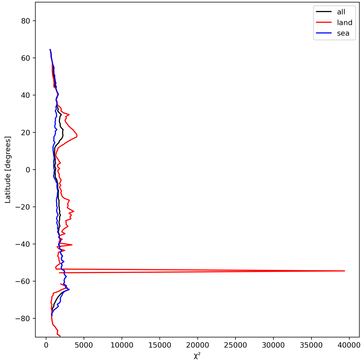
Figure 14: Zonal average of “ \chi^2 ” for 2023-11-23 to 2023-11-25.
