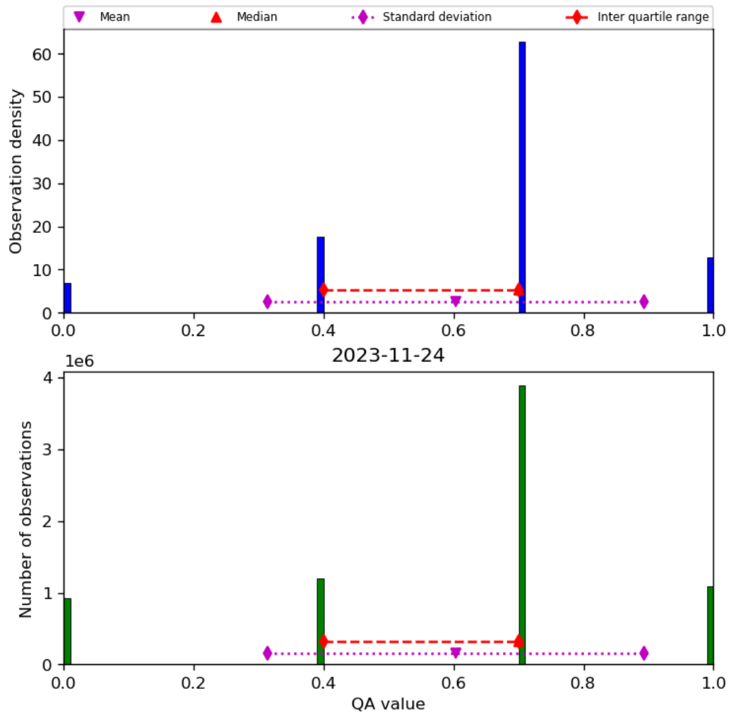
Figure 17: Histogram of “QA value” for 2023-11-23 to 2023-11-25
