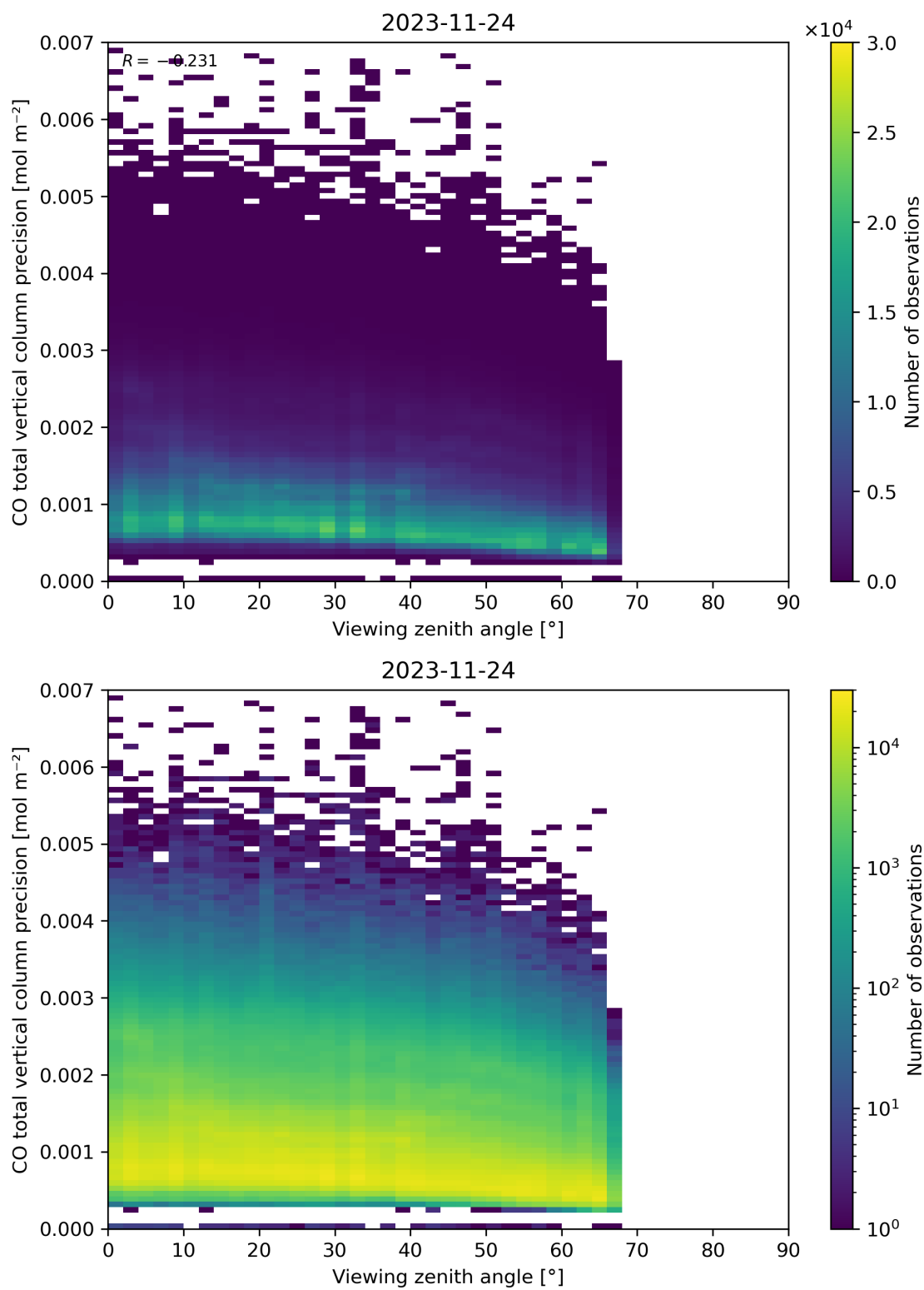
Figure 71: Scatter density plot of “Viewing zenith angle” against “CO total vertical column precision” for 2023-11-23 to 2023-11-25.
