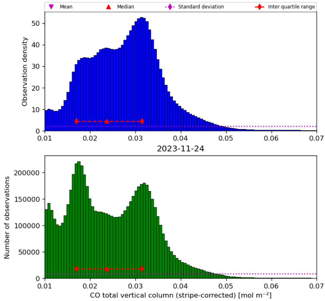
Figure 19: Histogram of “CO total vertical column (stripe-corrected)” for 2023-11-23 to 2023-11-25
