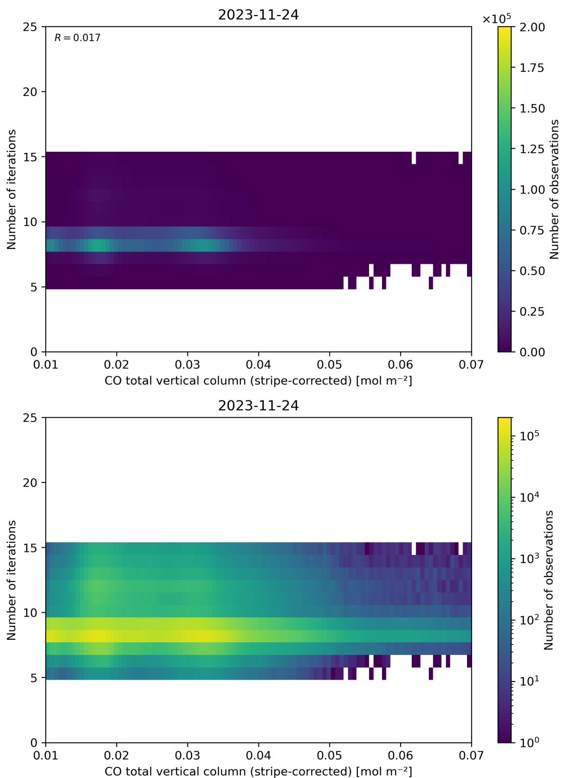
Figure 39: Scatter density plot of “CO total vertical column (stripe-corrected)” against “Number of iterations” for 2023-11-23 to 2023-11-25.
