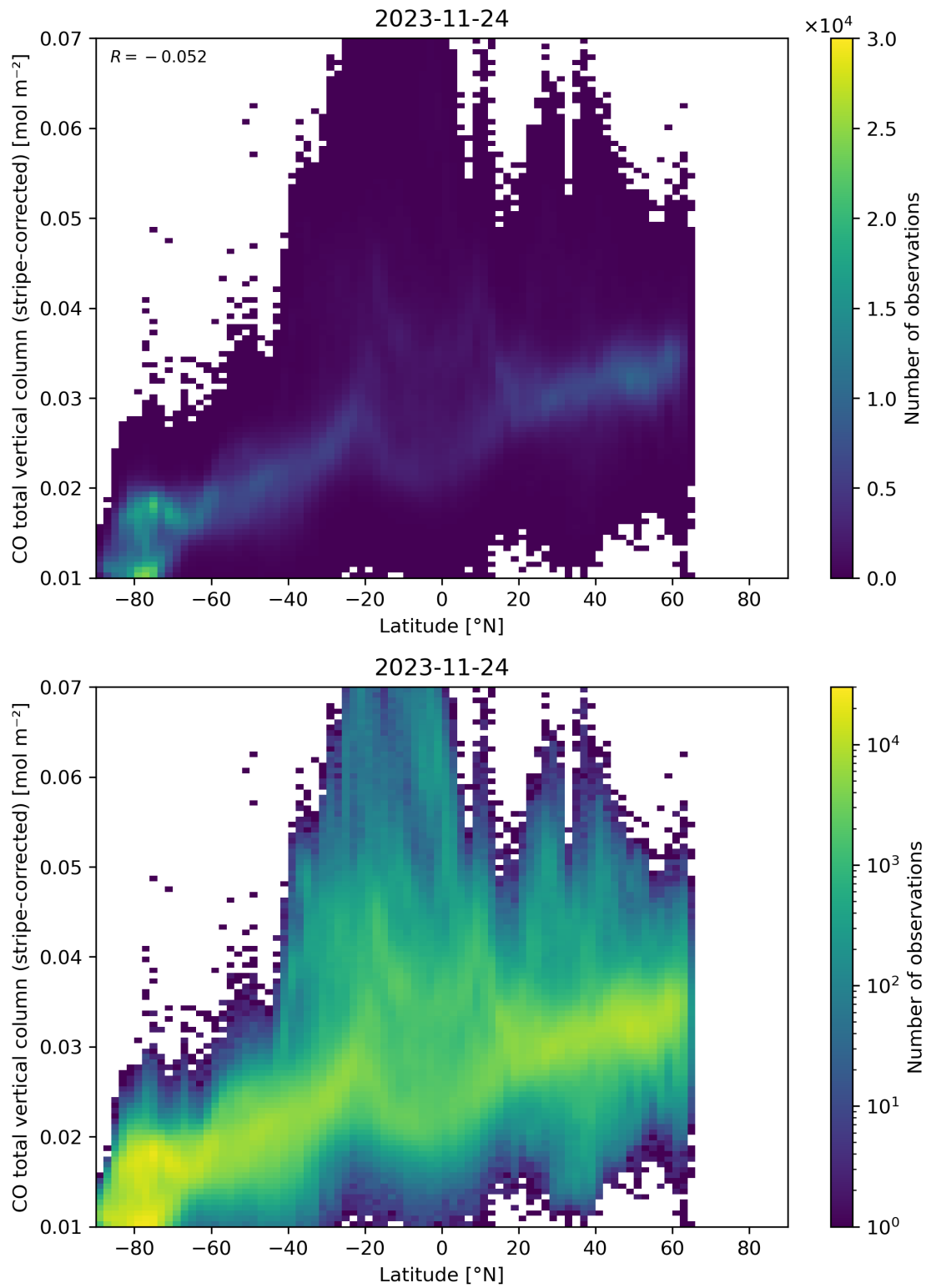
Figure 52: Scatter density plot of “Latitude” against “CO total vertical column (stripe-corrected)” for 2023-11-23 to 2023-11-25.
