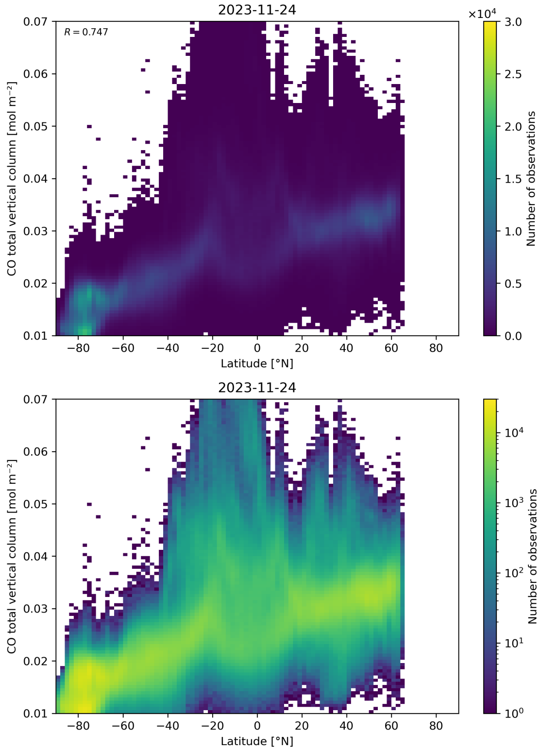
Figure 51: Scatter density plot of “Latitude” against “CO total vertical column” for 2023-11-23 to 2023-11-25.
