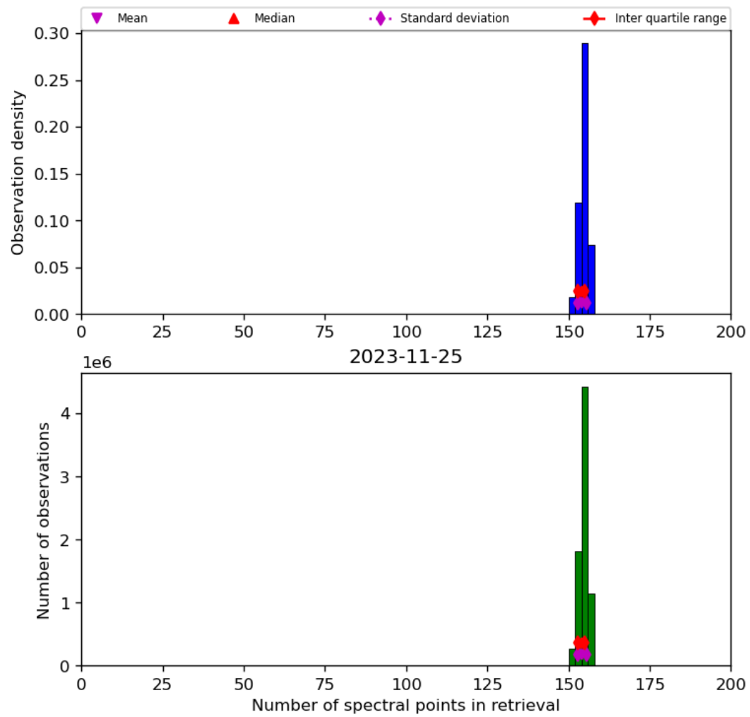
Figure 21: Histogram of “Number of spectral points in retrieval” for 2023-11-24 to 2023-11-26
