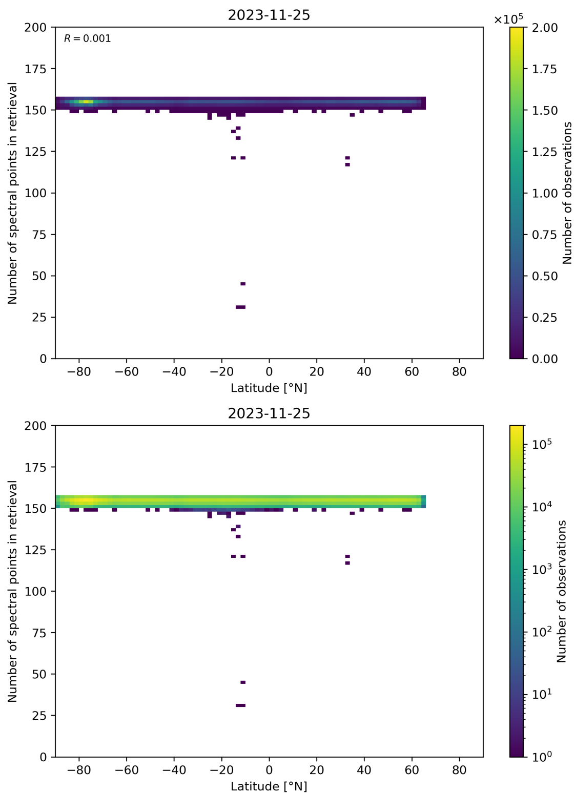
Figure 57: Scatter density plot of “Latitude” against “Number of spectral points in retrieval” for 2023-11-24 to 2023-11-26.
