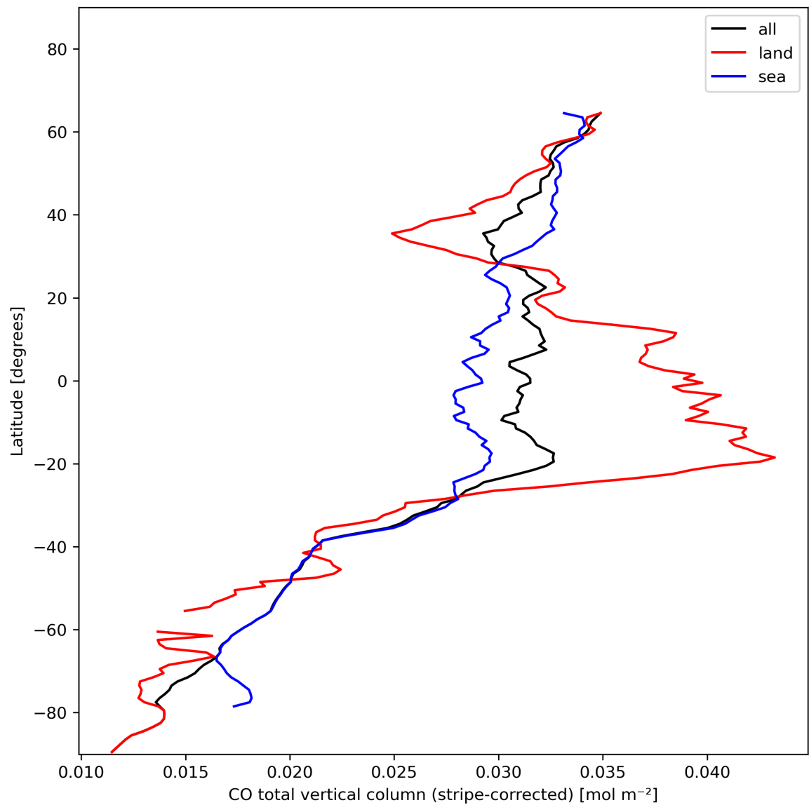
Figure 11: Zonal average of “CO total vertical column (stripe-corrected)” for 2023-11-24 to 2023-11-26.
