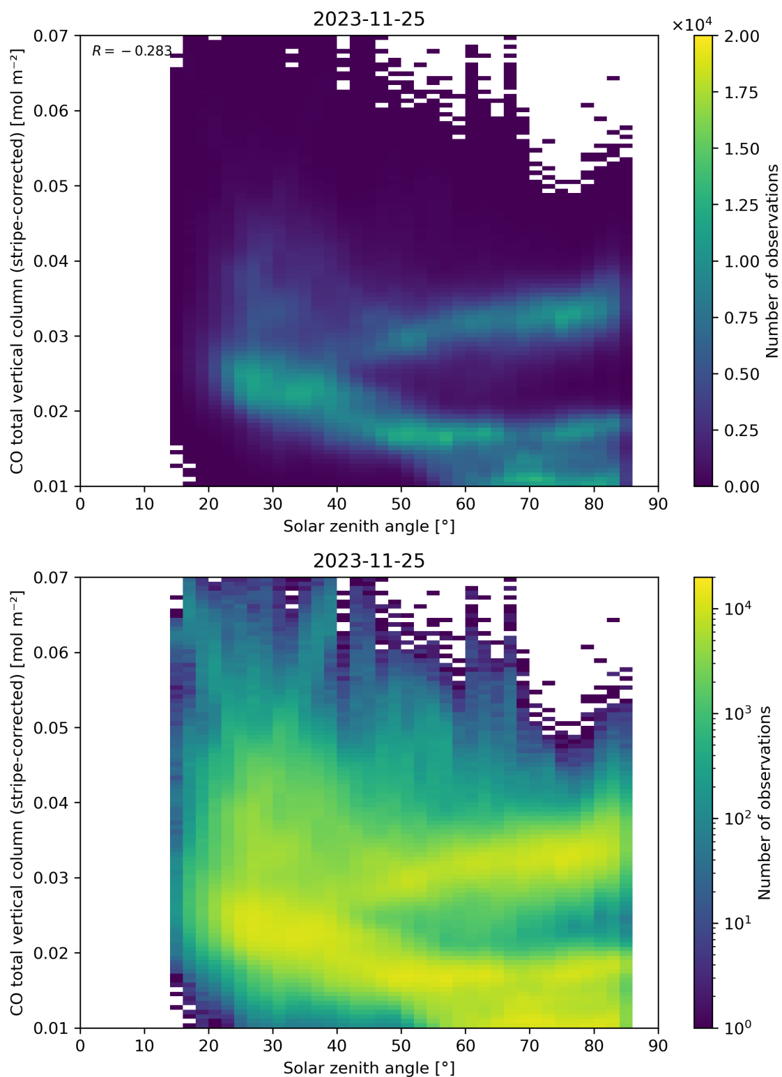
Figure 62: Scatter density plot of “Solar zenith angle” against “CO total vertical column (stripe-corrected)” for 2023-11-24 to 2023-11-26.
