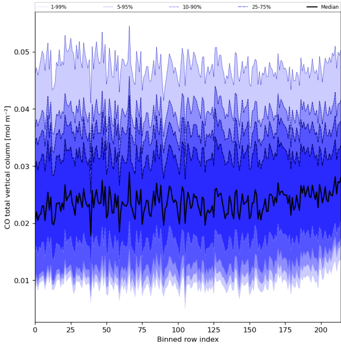
Figure 26: Along track statistics of “CO total vertical column” for 2023-11-24 to 2023-11-26
