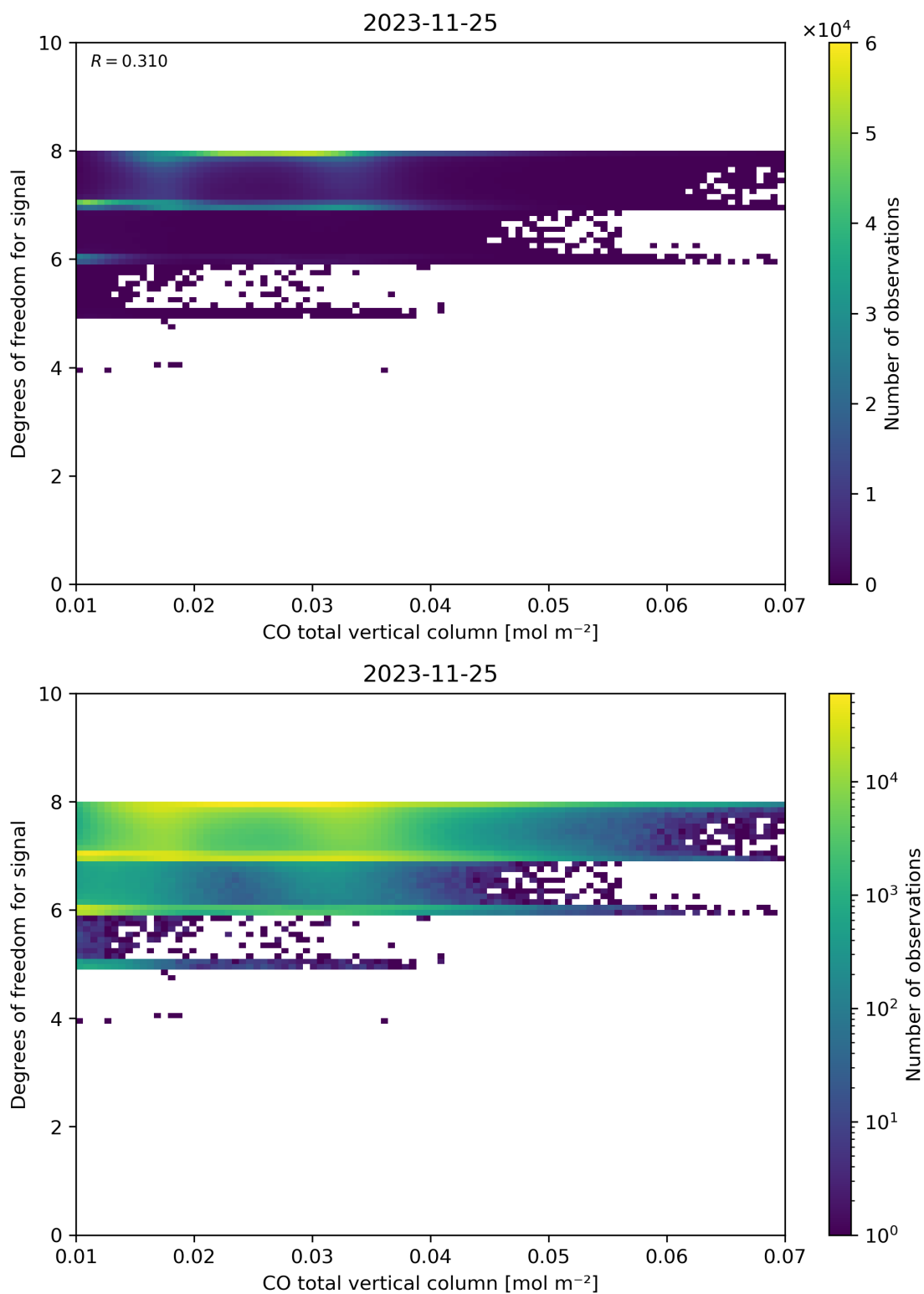
Figure 41: Scatter density plot of “CO total vertical column” against “Degrees of freedom for signal” for 2023-11-24 to 2023-11-26.
