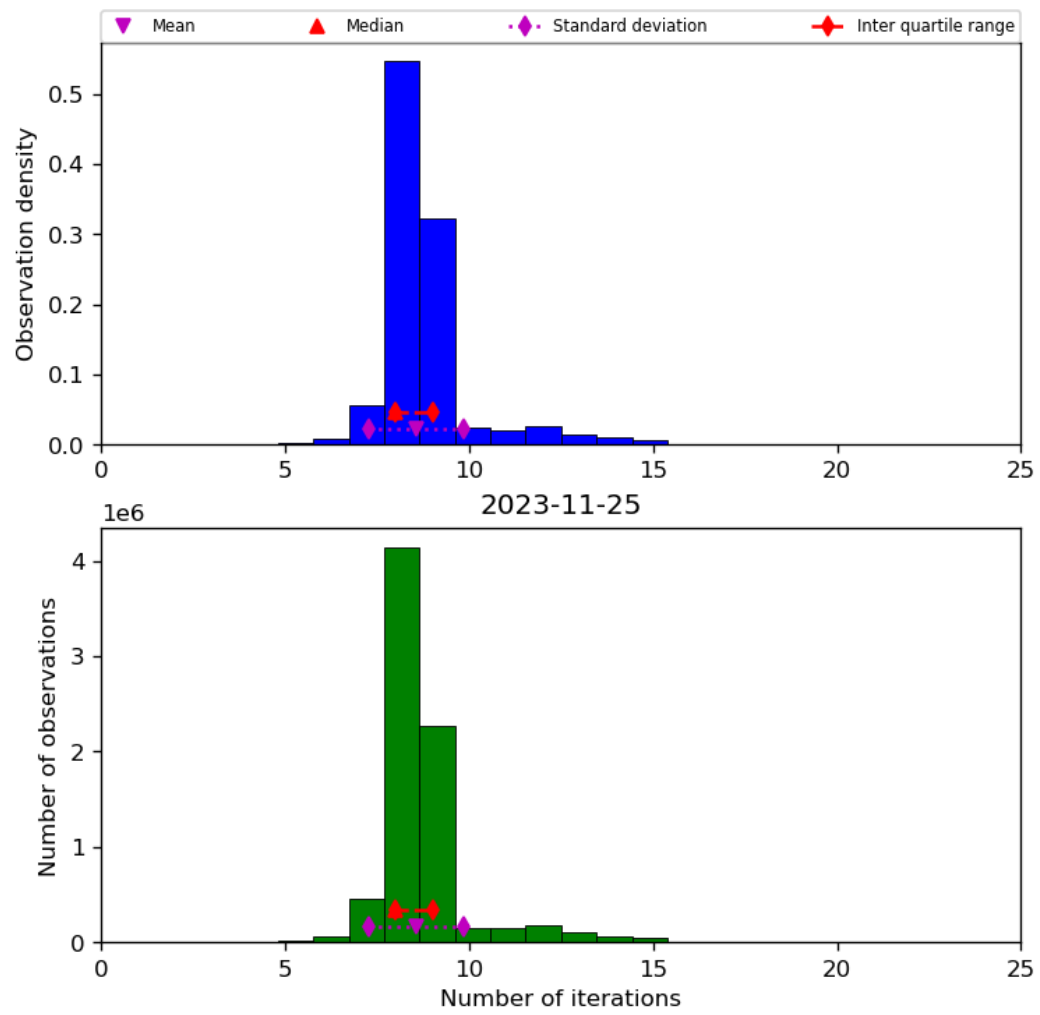
Figure 24: Histogram of “Number of iterations” for 2023-11-24 to 2023-11-26
