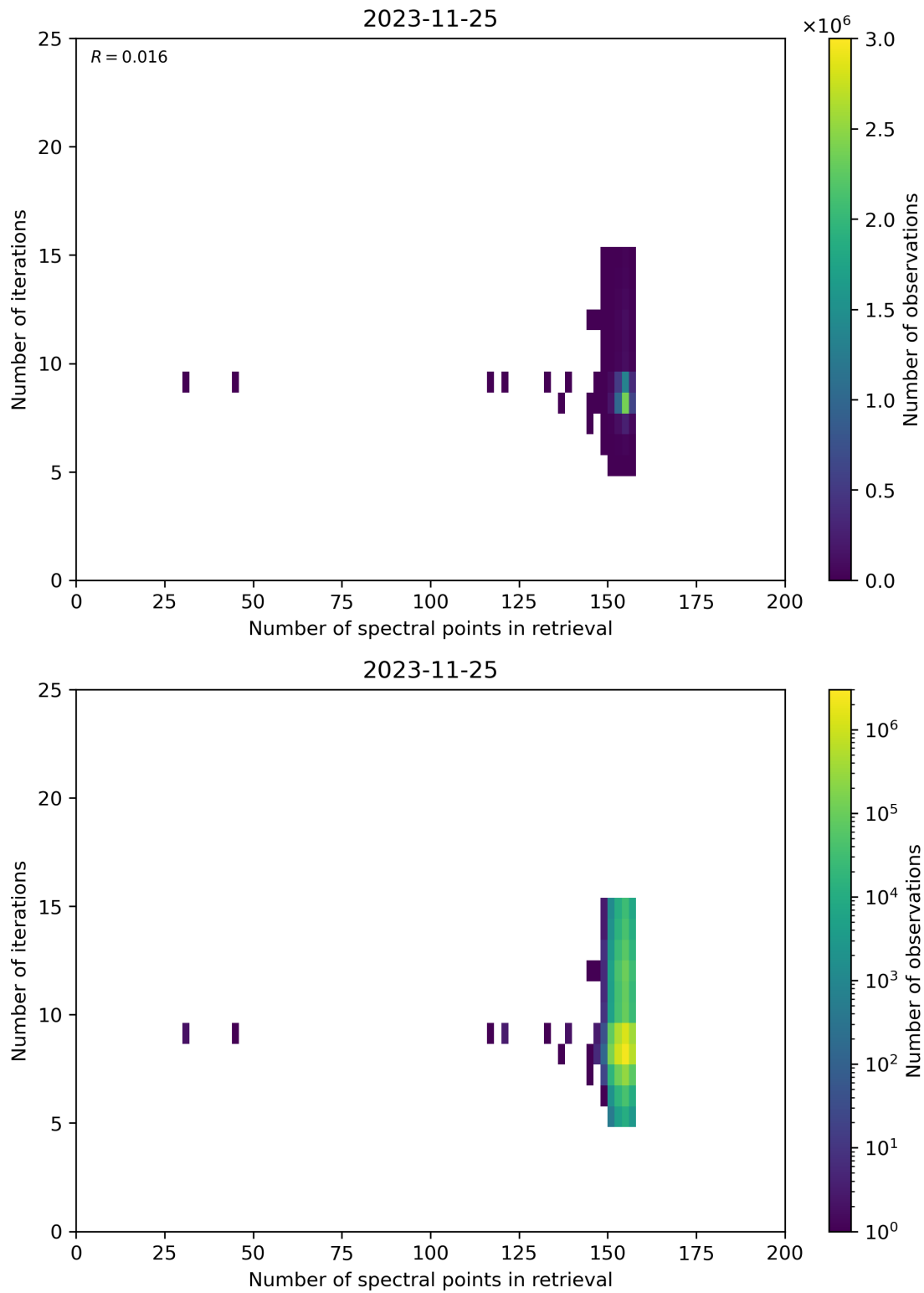
Figure 60: Scatter density plot of “Number of spectral points in retrieval” against “Number of iterations” for 2023-11-24 to 2023-11-26.
