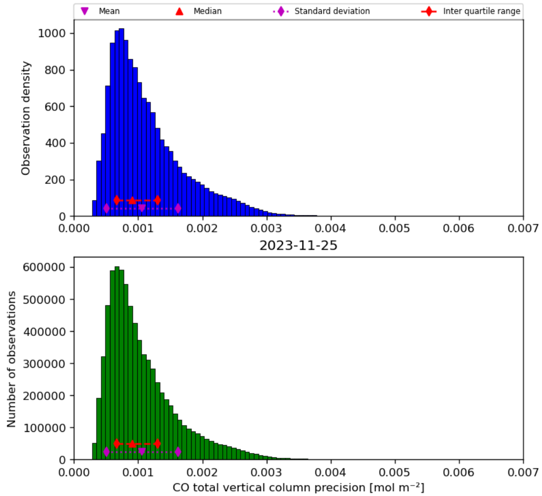
Figure 20: Histogram of “CO total vertical column precision” for 2023-11-24 to 2023-11-26
