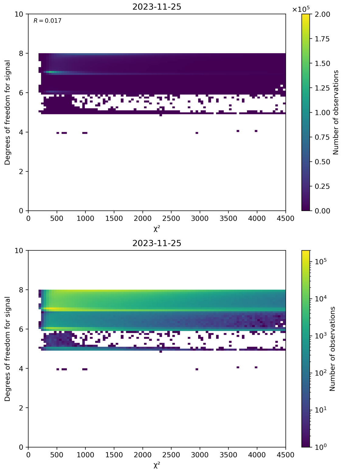
Figure 48: Scatter density plot of “ \chi^2 ” against “Degrees of freedom for signal” for 2023-11-24 to 2023-11-26.
