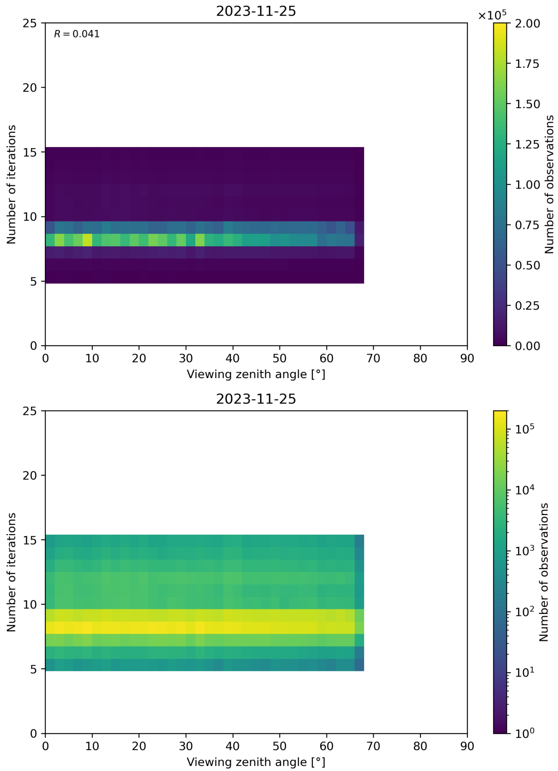
Figure 75: Scatter density plot of “Viewing zenith angle” against “Number of iterations” for 2023-11-24 to 2023-11-26.
