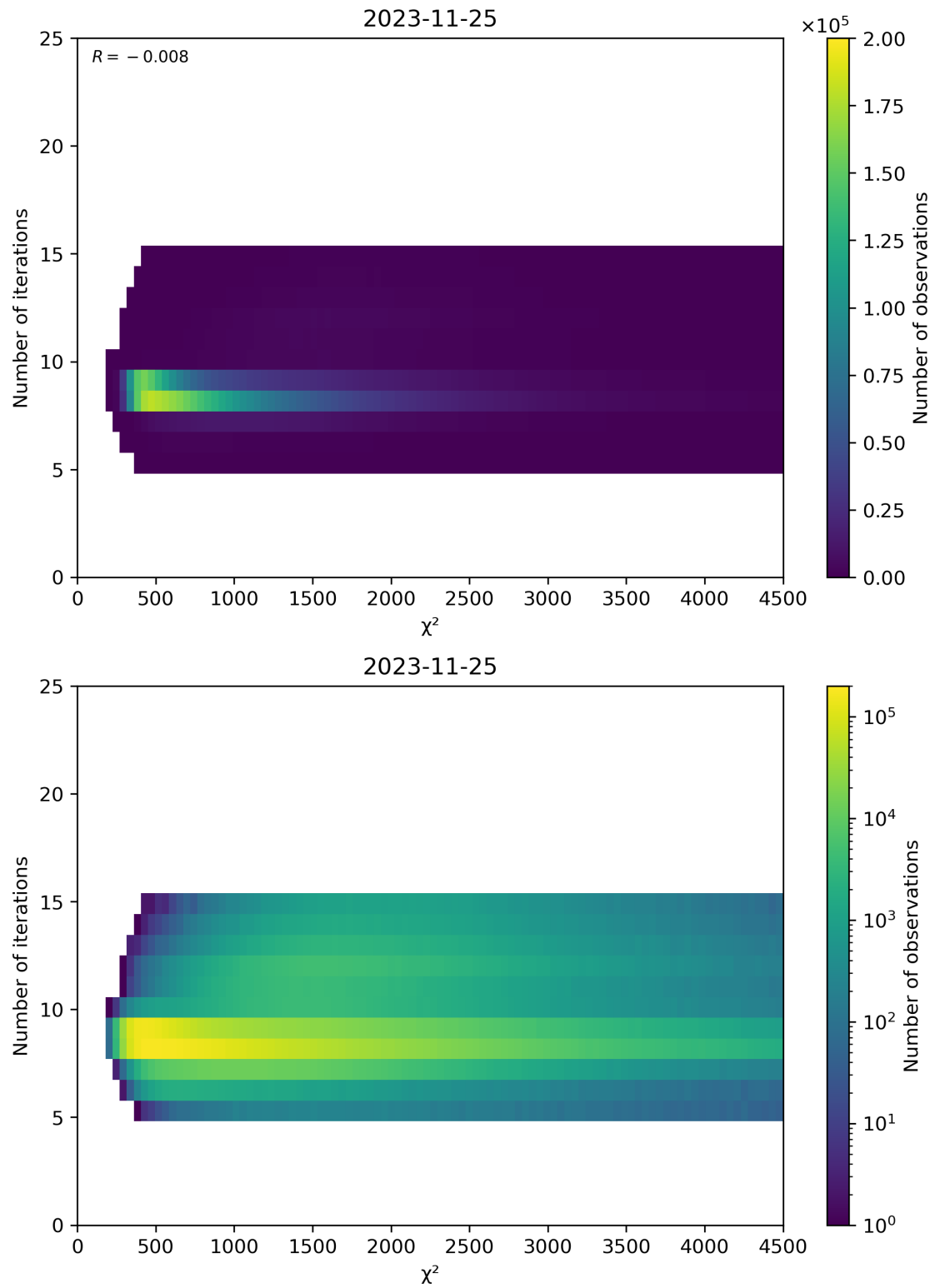
Figure 49: Scatter density plot of “ \chi^2 ” against “Number of iterations” for 2023-11-24 to 2023-11-26.
