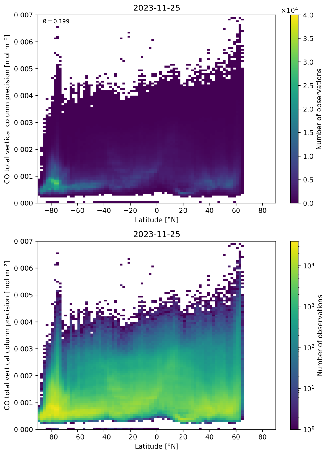
Figure 53: Scatter density plot of “Latitude” against “CO total vertical column precision” for 2023-11-24 to 2023-11-26.
