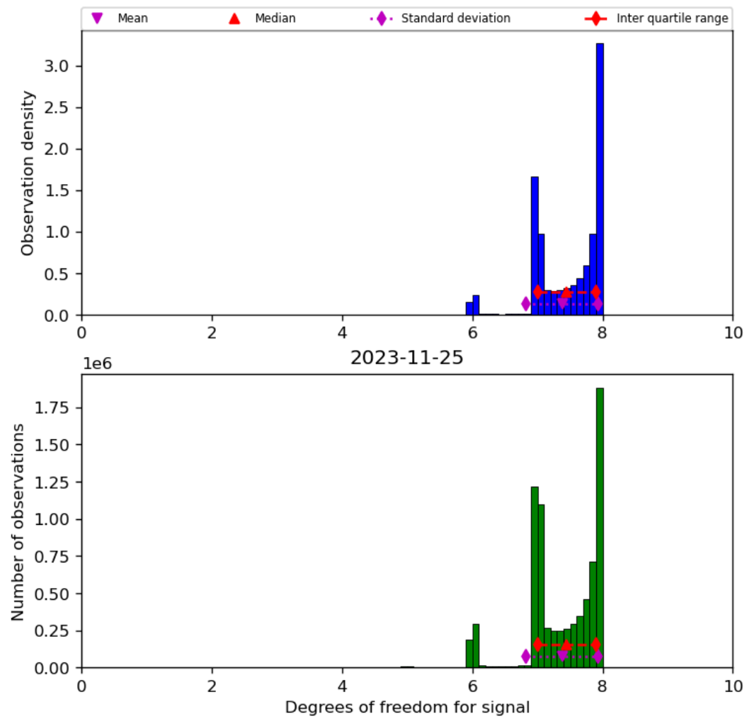
Figure 23: Histogram of “Degrees of freedom for signal” for 2023-11-24 to 2023-11-26
