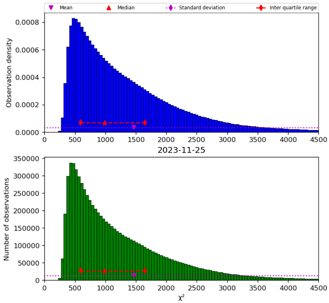
Figure 22: Histogram of “ \chi^2 ” for 2023-11-24 to 2023-11-26
