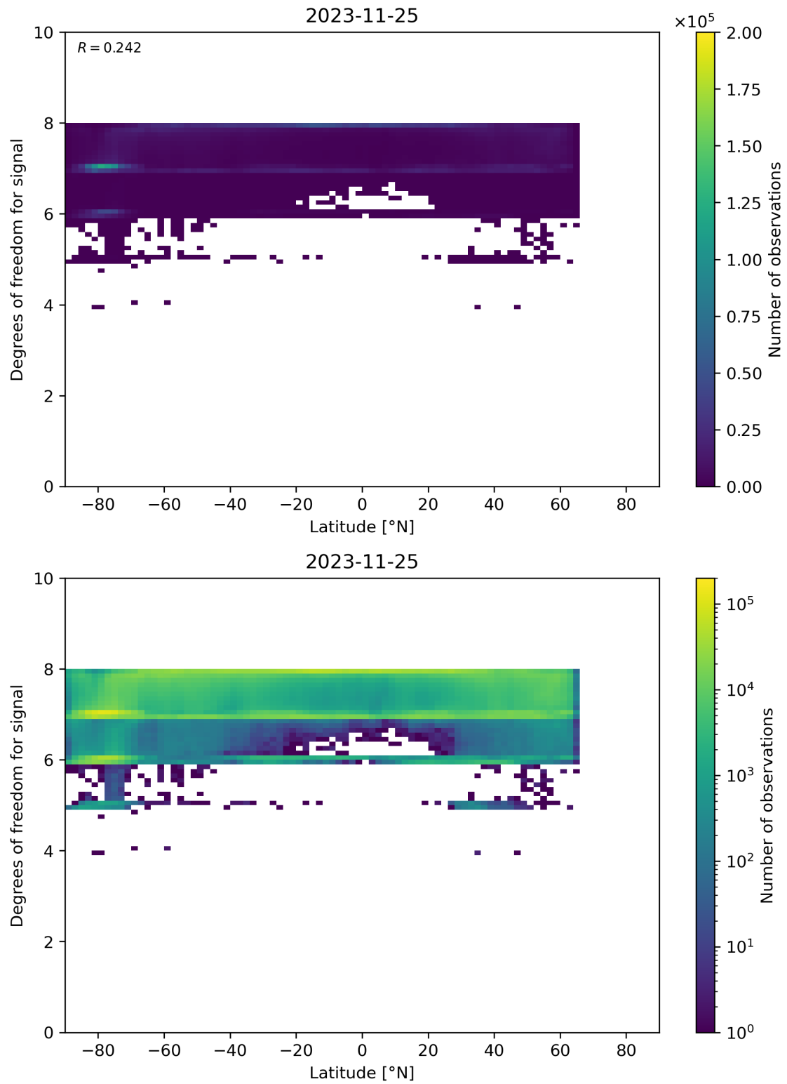
Figure 55: Scatter density plot of “Latitude” against “Degrees of freedom for signal” for 2023-11-24 to 2023-11-26.
