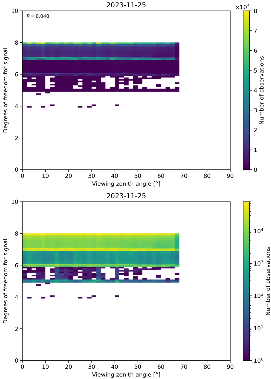
Figure 73: Scatter density plot of “Viewing zenith angle” against “Degrees of freedom for signal” for 2023-11-24 to 2023-11-26.
