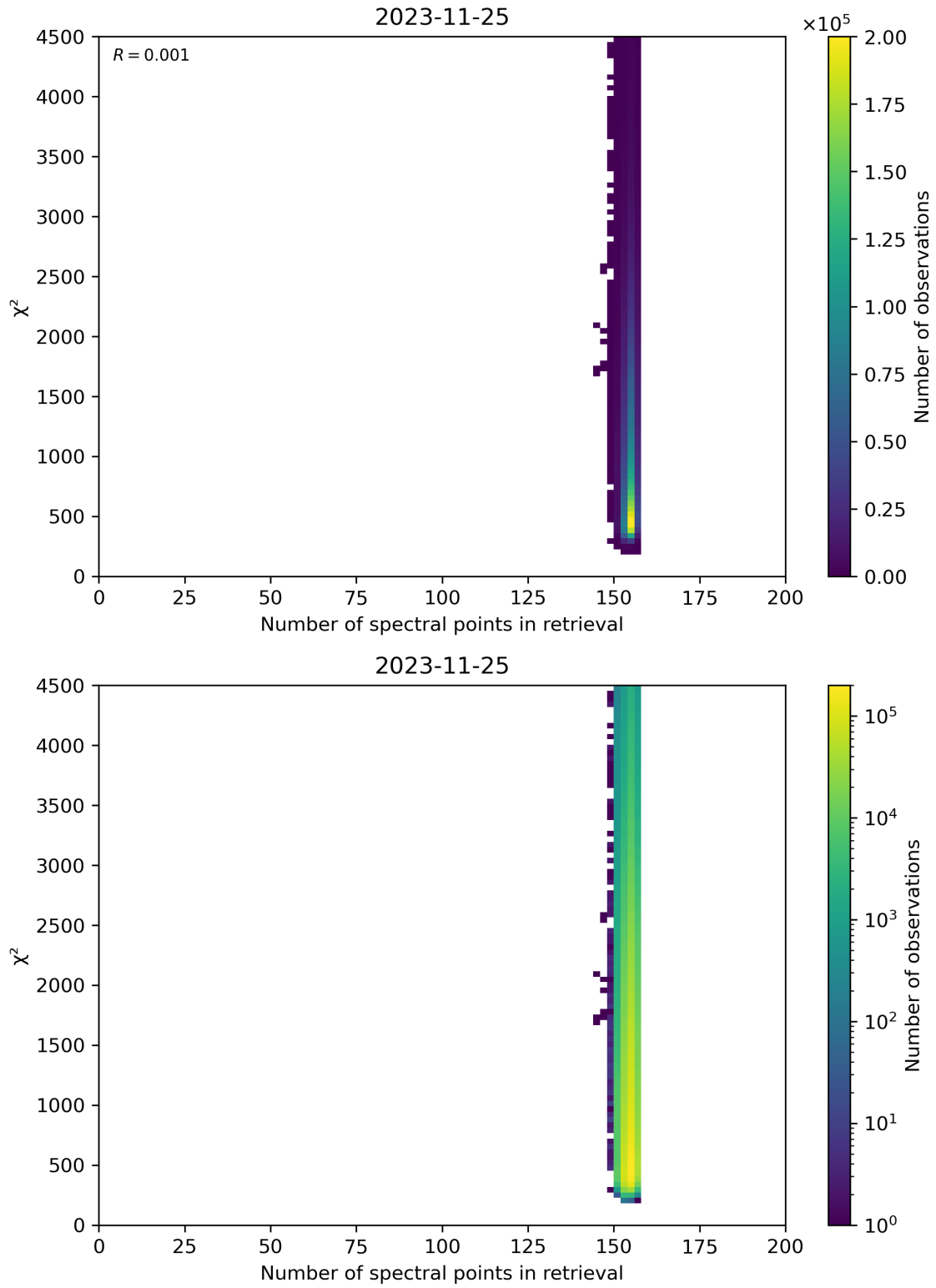
Figure 58: Scatter density plot of “Number of spectral points in retrieval” against “ \chi^2 ” for 2023-11-24 to 2023-11-26.
