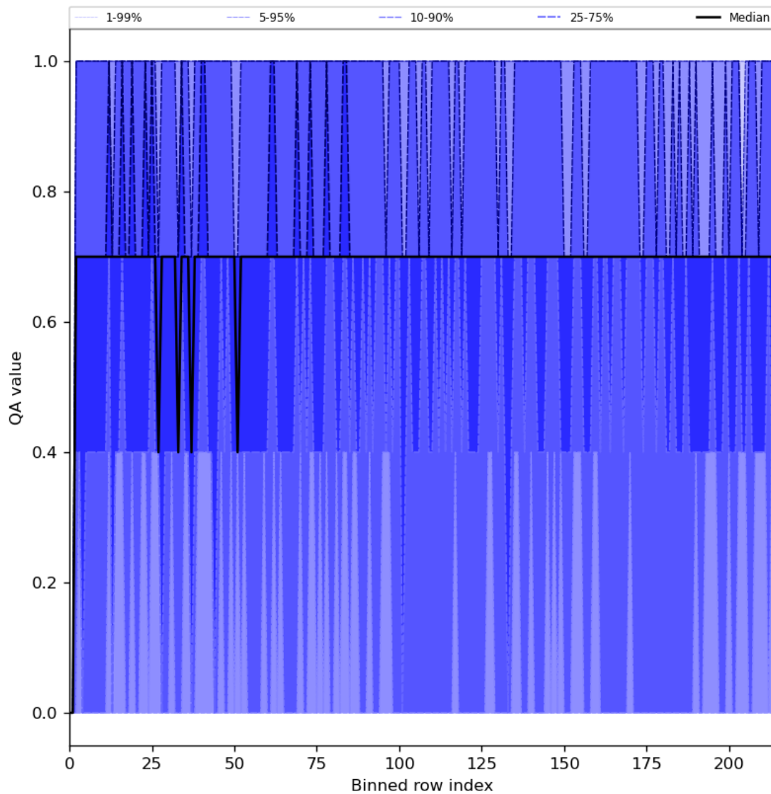
Figure 25: Along track statistics of “QA value” for 2023-11-24 to 2023-11-26
