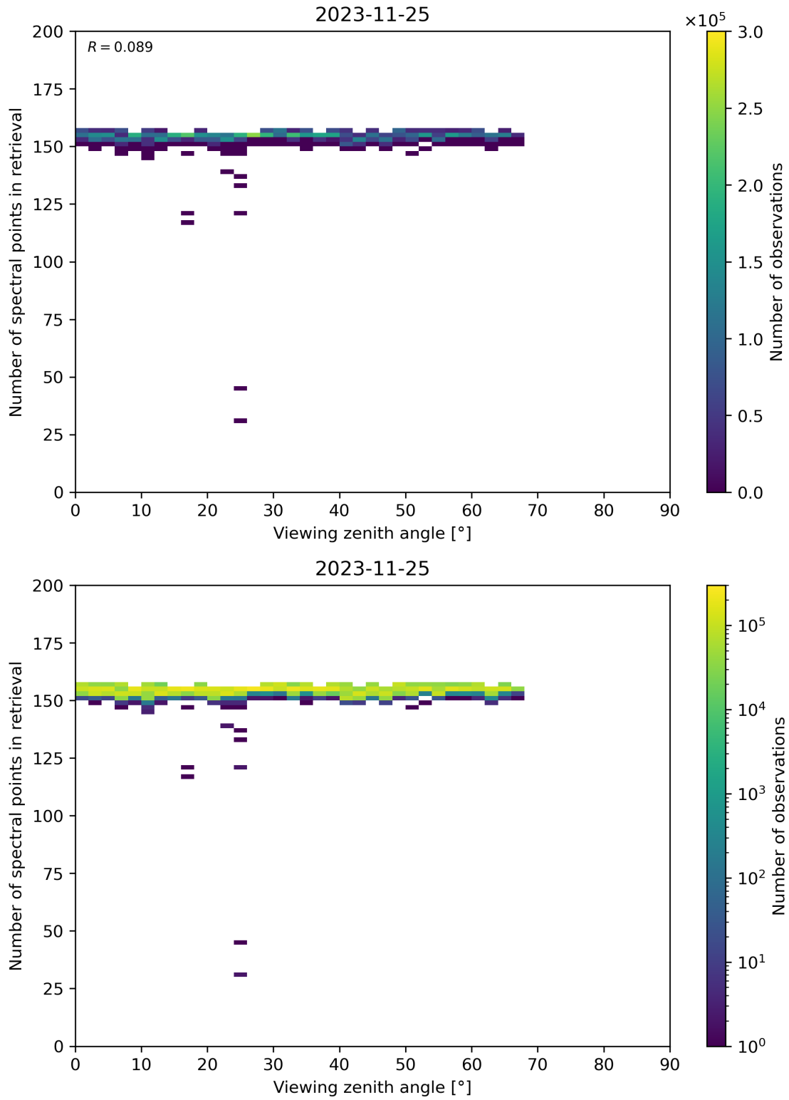
Figure 76: Scatter density plot of “Viewing zenith angle” against “Number of spectral points in retrieval” for 2023-11-24 to 2023-11-26.
