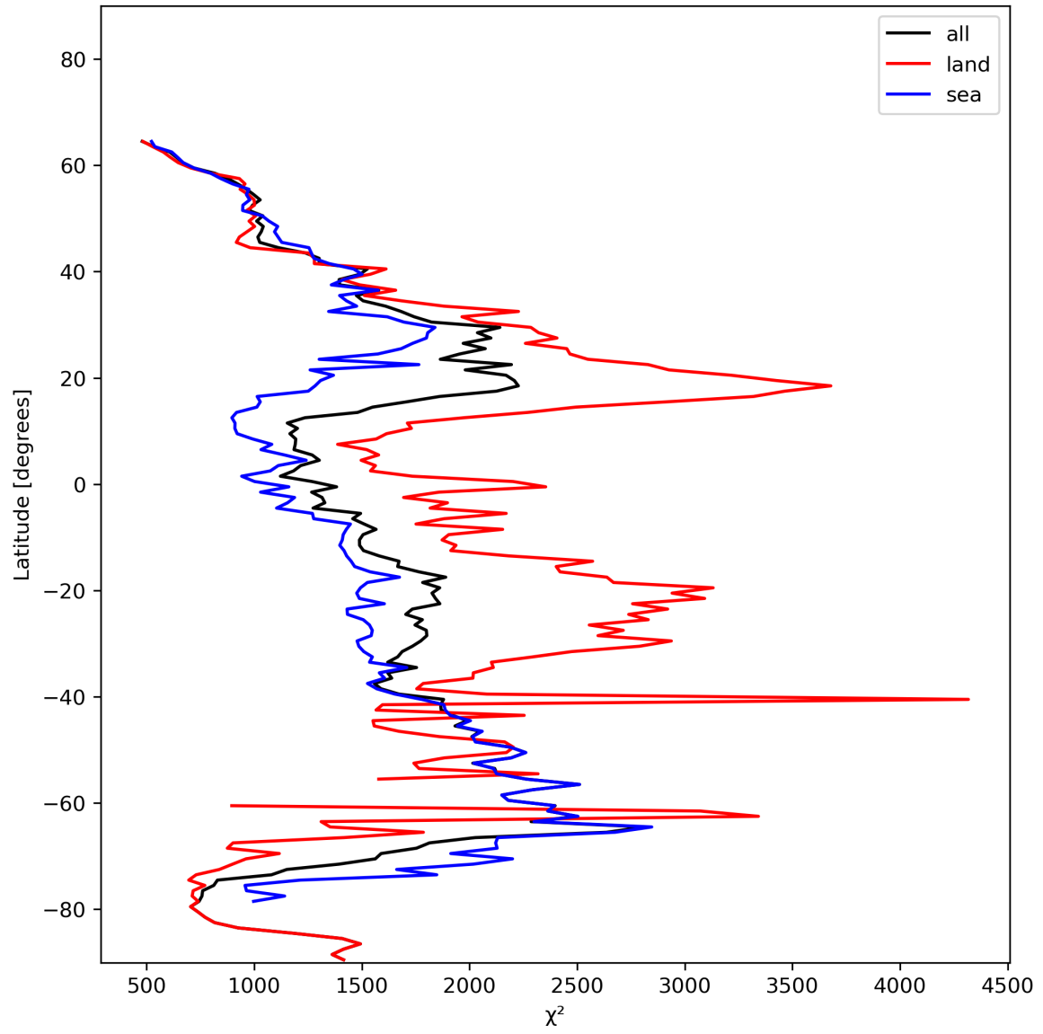
Figure 14: Zonal average of “ \chi^2 ” for 2023-11-24 to 2023-11-26.
