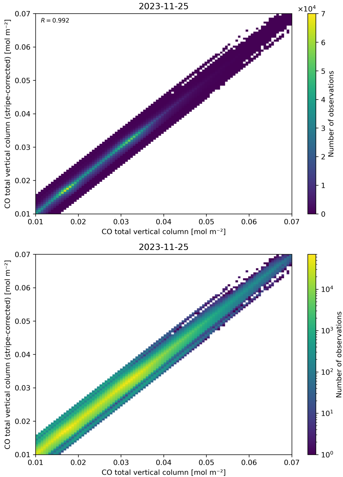
Figure 33: Scatter density plot of “CO total vertical column” against “CO total vertical column (stripe-corrected)” for 2023-11-24 to 2023-11-26.
