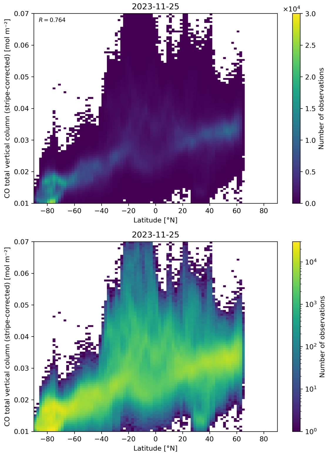
Figure 52: Scatter density plot of “Latitude” against “CO total vertical column (stripe-corrected)” for 2023-11-24 to 2023-11-26.
