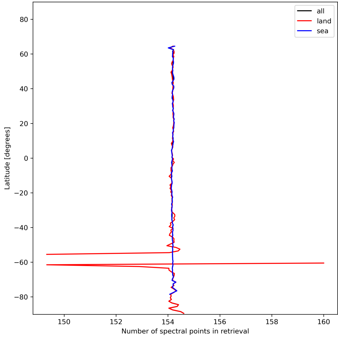
Figure 13: Zonal average of “Number of spectral points in retrieval” for 2023-11-24 to 2023-11-26.
