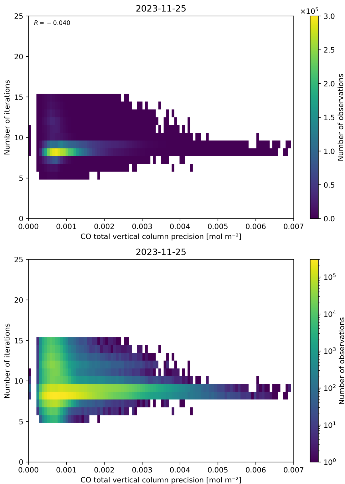
Figure 46: Scatter density plot of “CO total vertical column precision” against “Number of iterations” for 2023-11-24 to 2023-11-26.
