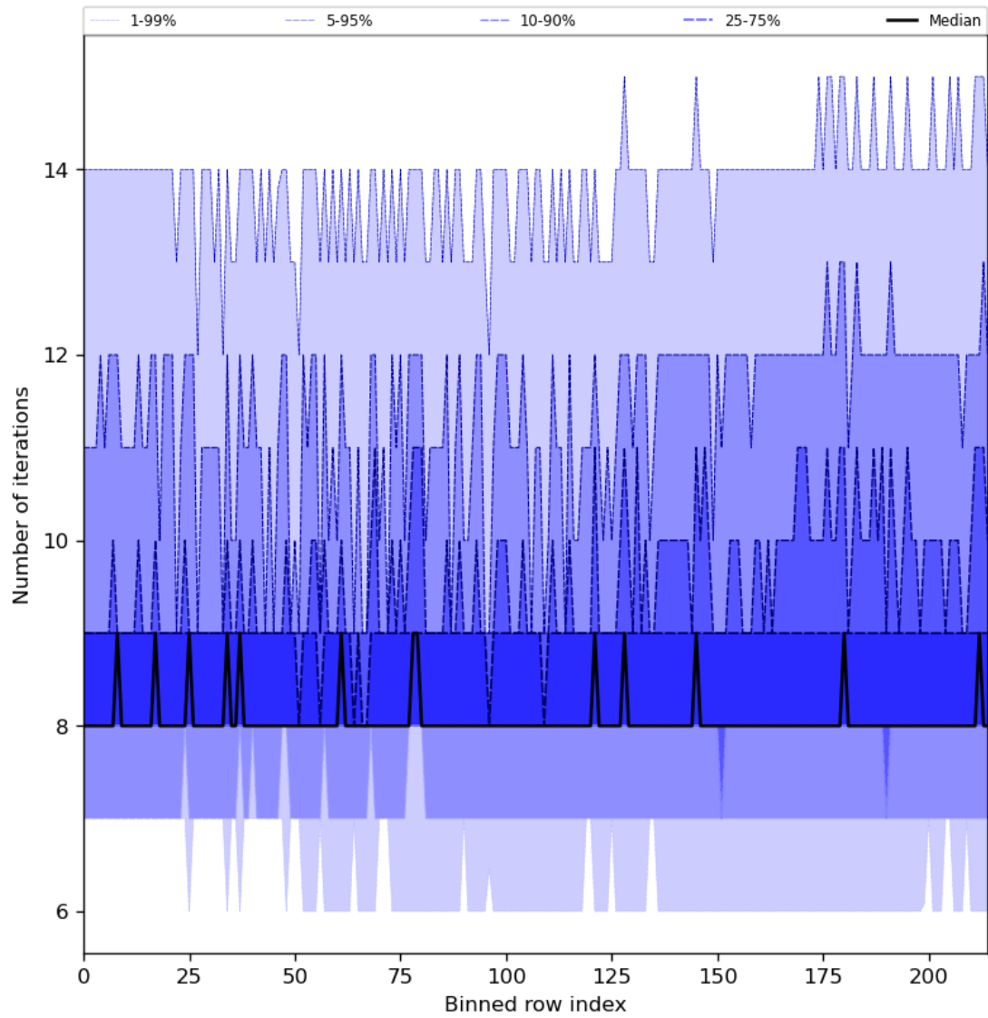
Figure 32: Along track statistics of “Number of iterations” for 2023-11-24 to 2023-11-26
