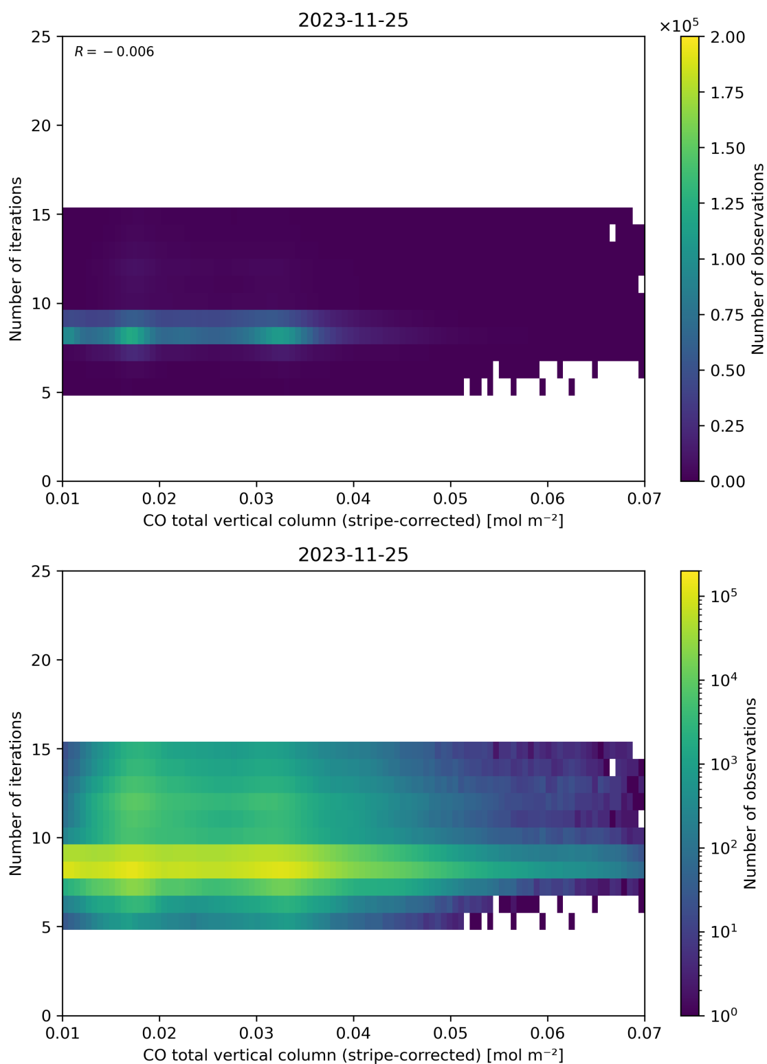
Figure 39: Scatter density plot of “CO total vertical column (stripe-corrected)” against “Number of iterations” for 2023-11-24 to 2023-11-26.
