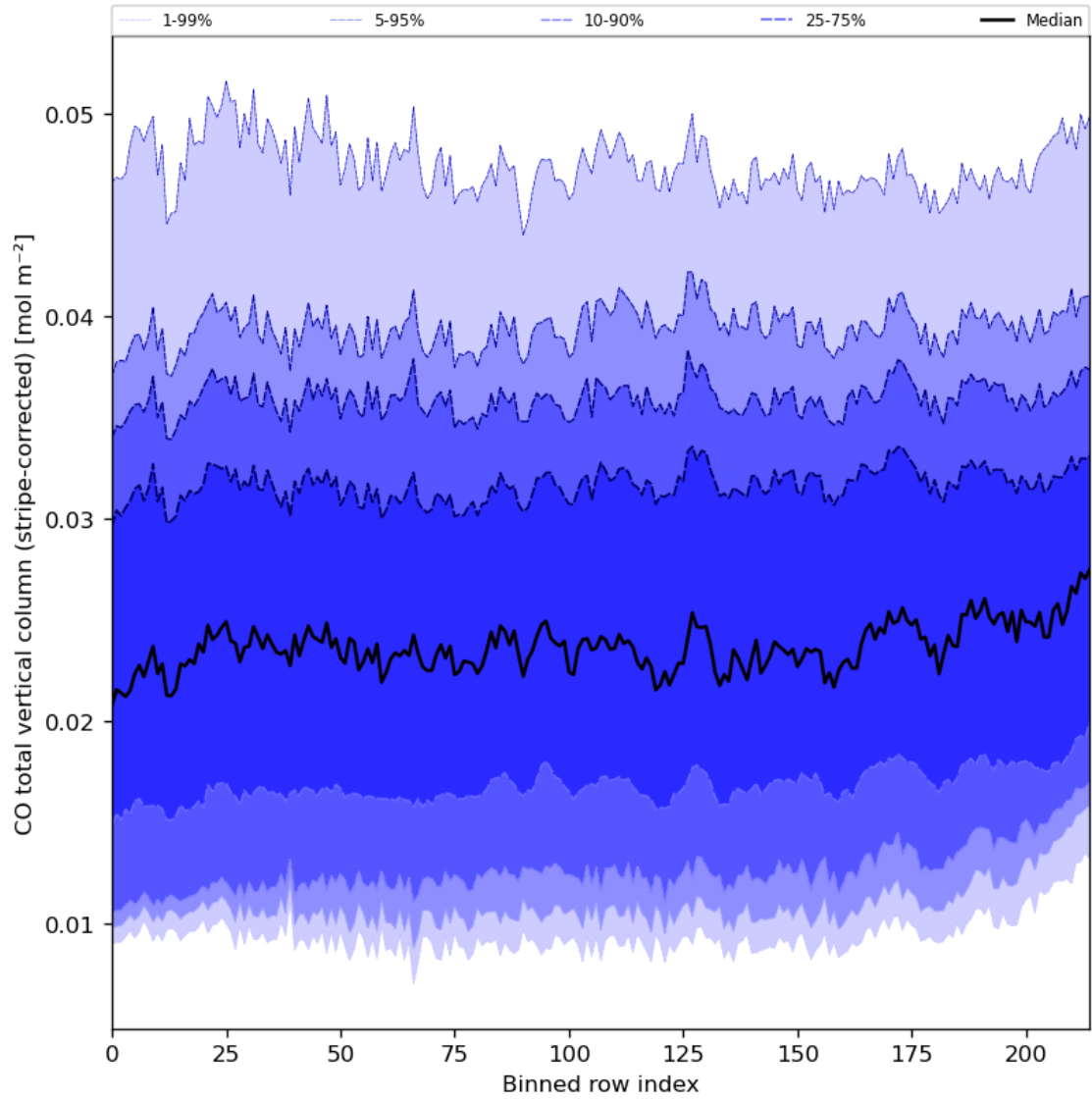
Figure 27: Along track statistics of “CO total vertical column (stripe-corrected)” for 2023-11-24 to 2023-11-26
