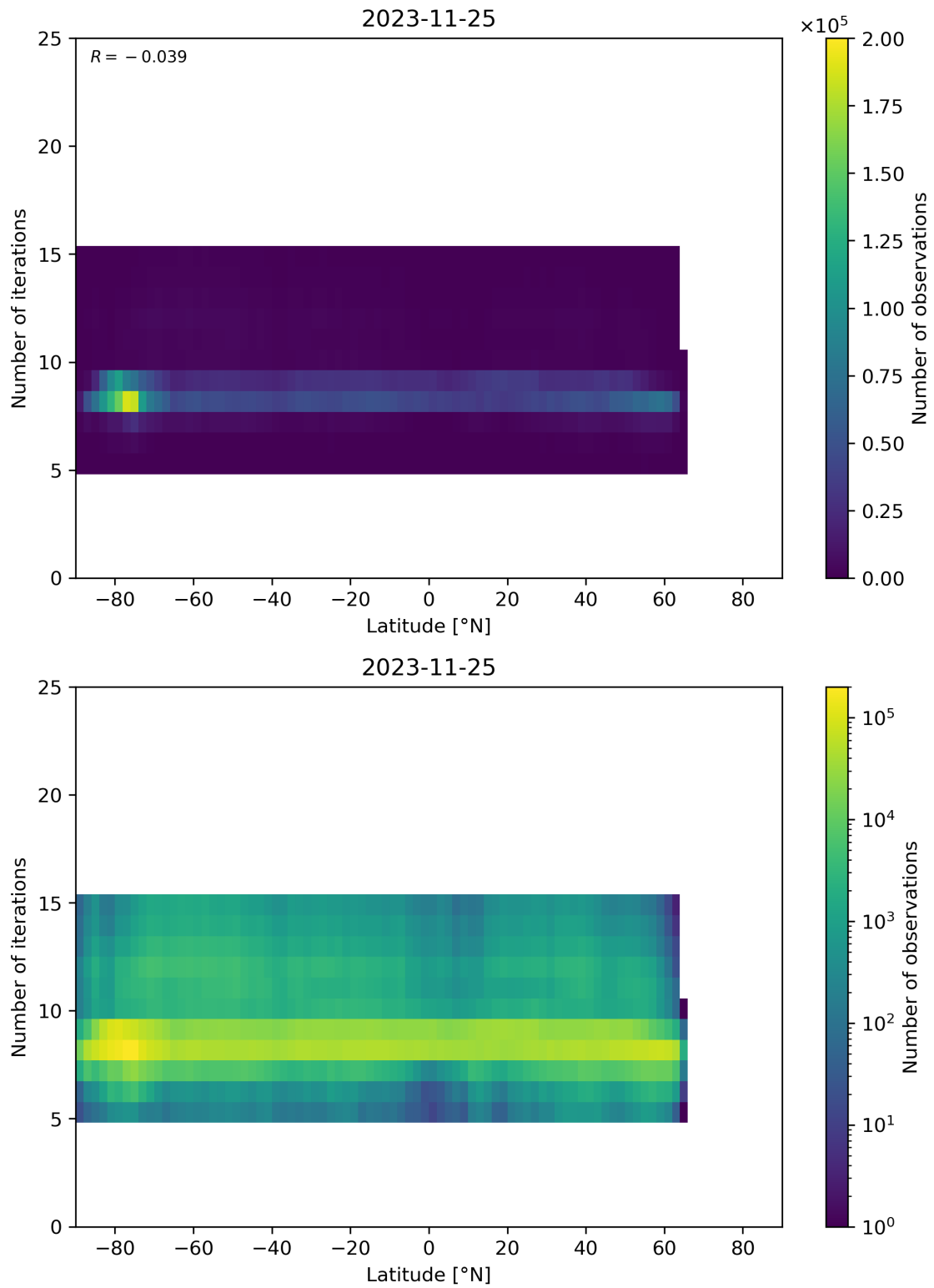
Figure 56: Scatter density plot of “Latitude” against “Number of iterations” for 2023-11-24 to 2023-11-26.
