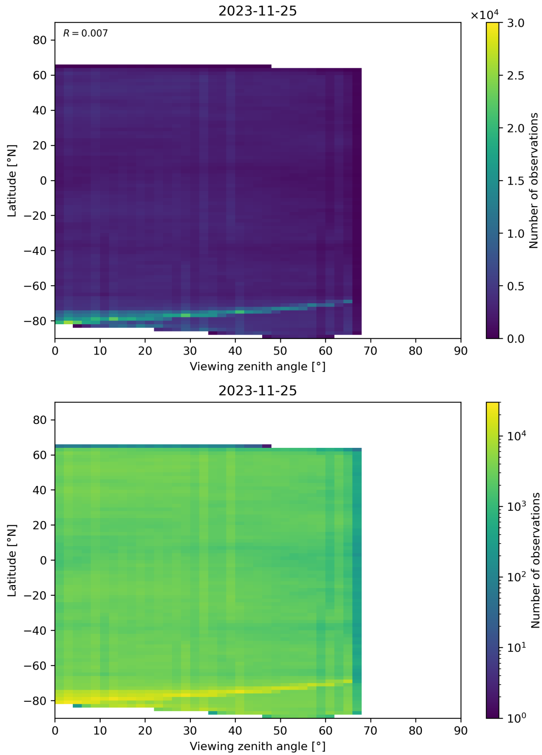
Figure 74: Scatter density plot of “Viewing zenith angle” against “Latitude” for 2023-11-24 to 2023-11-26.
