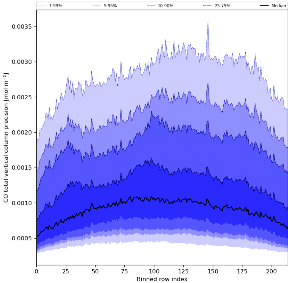
Figure 28: Along track statistics of “CO total vertical column precision” for 2023-11-24 to 2023-11-26
