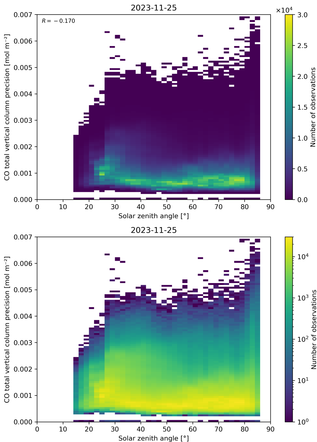
Figure 63: Scatter density plot of “Solar zenith angle” against “CO total vertical column precision” for 2023-11-24 to 2023-11-26.
