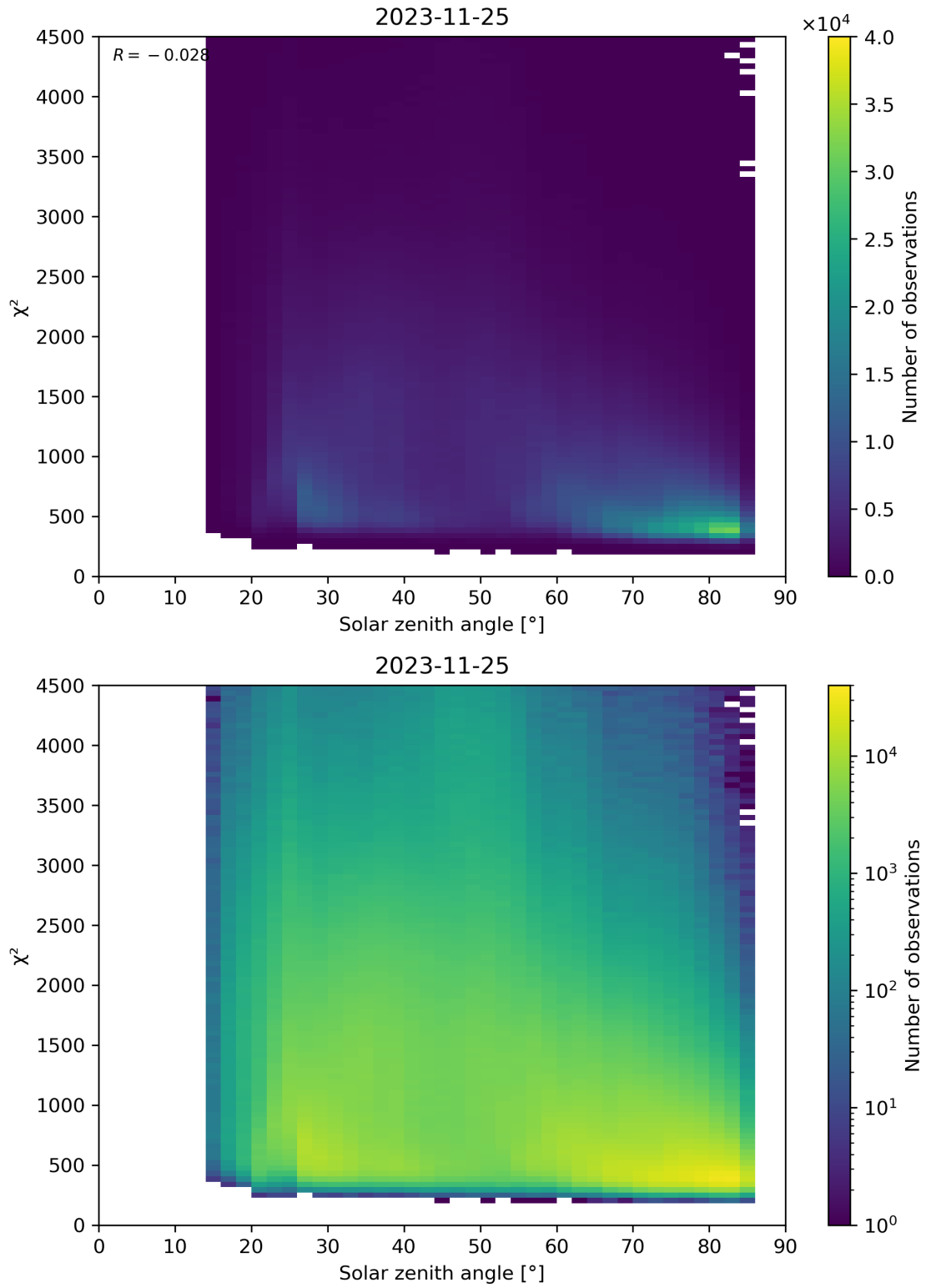
Figure 64: Scatter density plot of “Solar zenith angle” against “ \chi^2 ” for 2023-11-24 to 2023-11-26.
