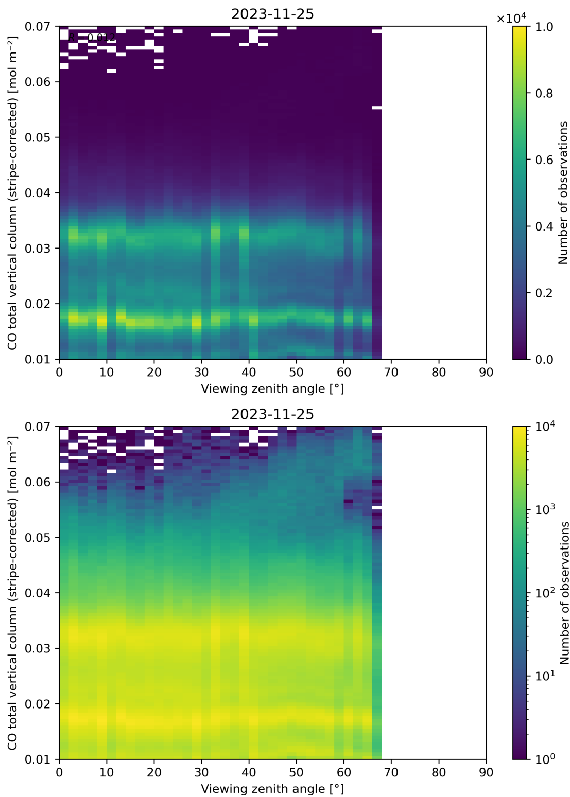
Figure 70: Scatter density plot of “Viewing zenith angle” against “CO total vertical column (stripe-corrected)” for 2023-11-24 to 2023-11-26.
