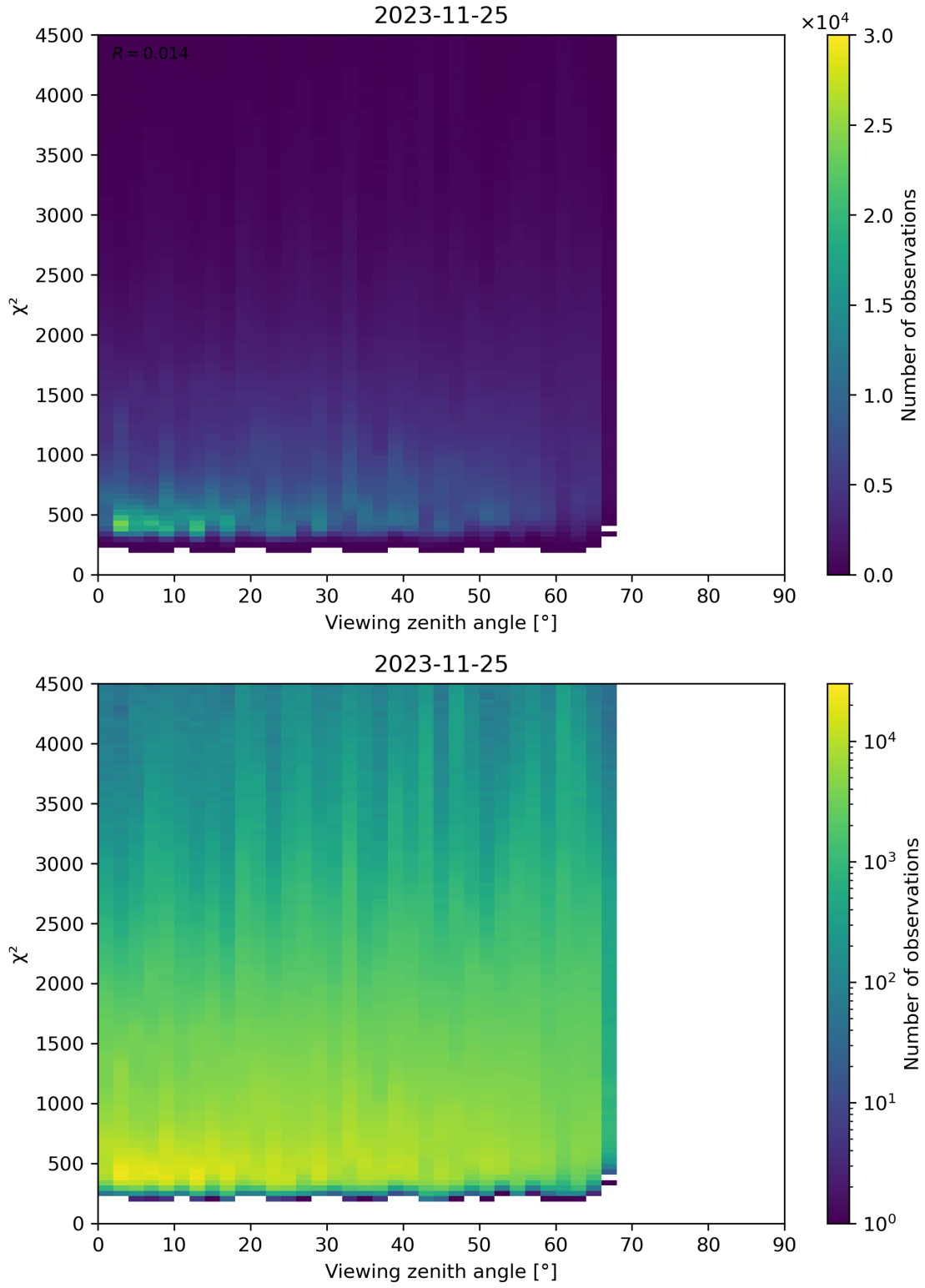
Figure 72: Scatter density plot of “Viewing zenith angle” against “ \chi^2 ” for 2023-11-24 to 2023-11-26.
