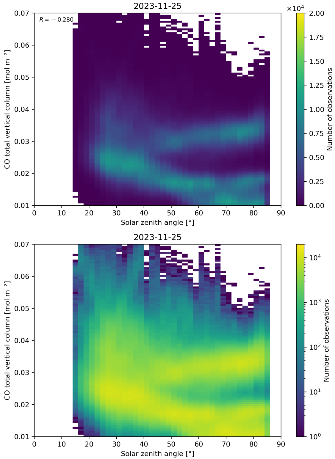
Figure 61: Scatter density plot of “Solar zenith angle” against “CO total vertical column” for 2023-11-24 to 2023-11-26.
