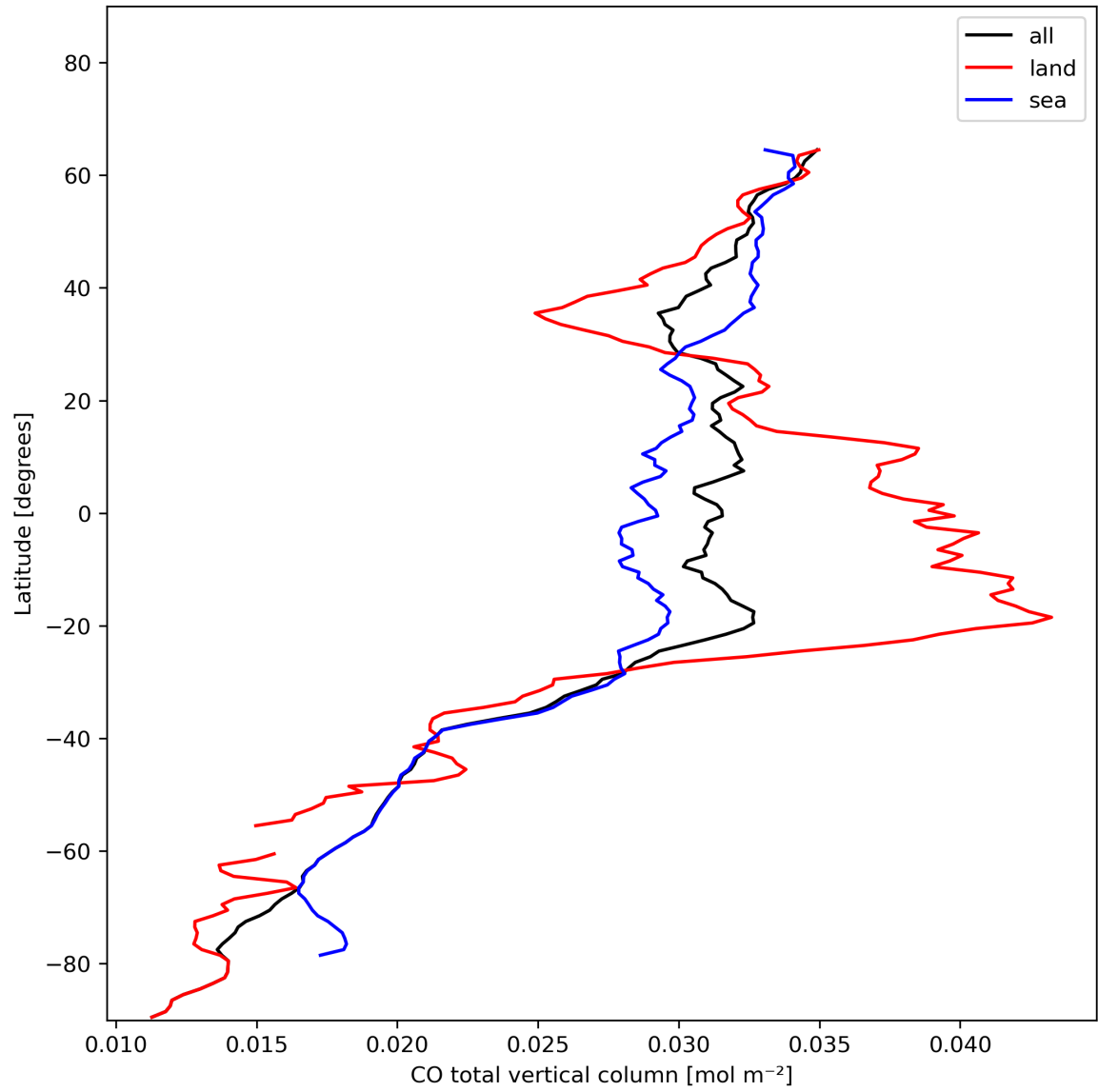
Figure 10: Zonal average of “CO total vertical column” for 2023-11-24 to 2023-11-26.
