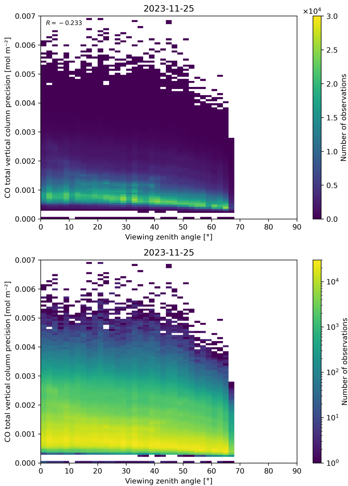
Figure 71: Scatter density plot of “Viewing zenith angle” against “CO total vertical column precision” for 2023-11-24 to 2023-11-26.
