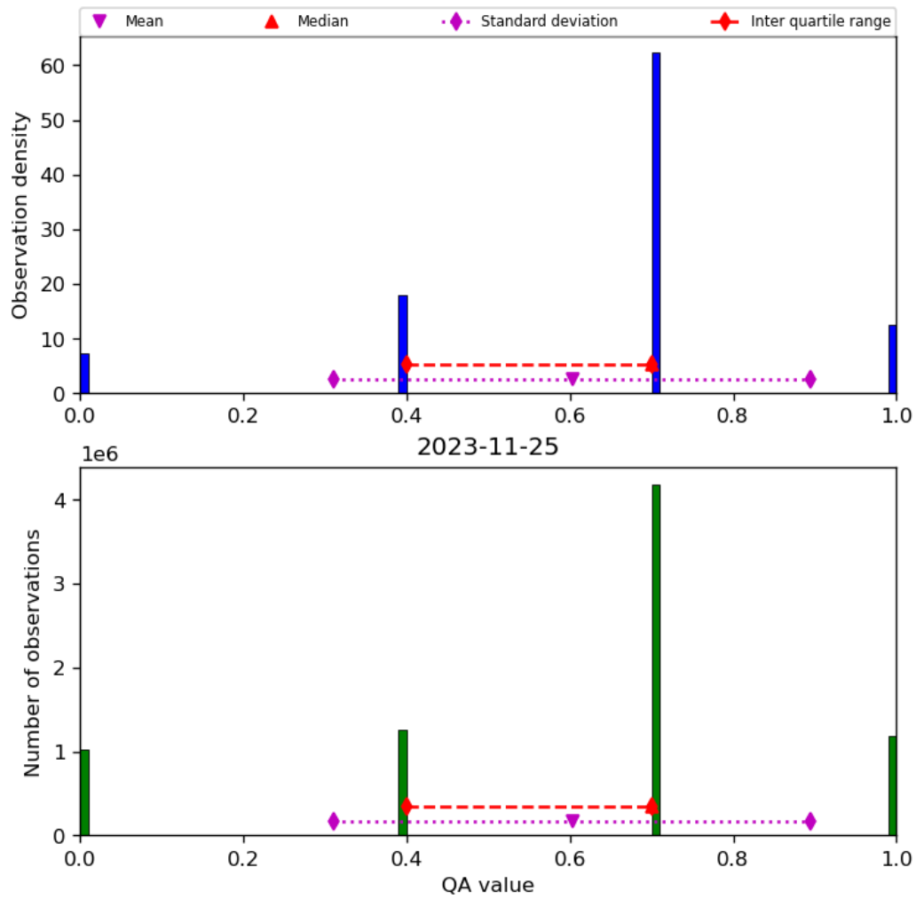
Figure 17: Histogram of “QA value” for 2023-11-24 to 2023-11-26
