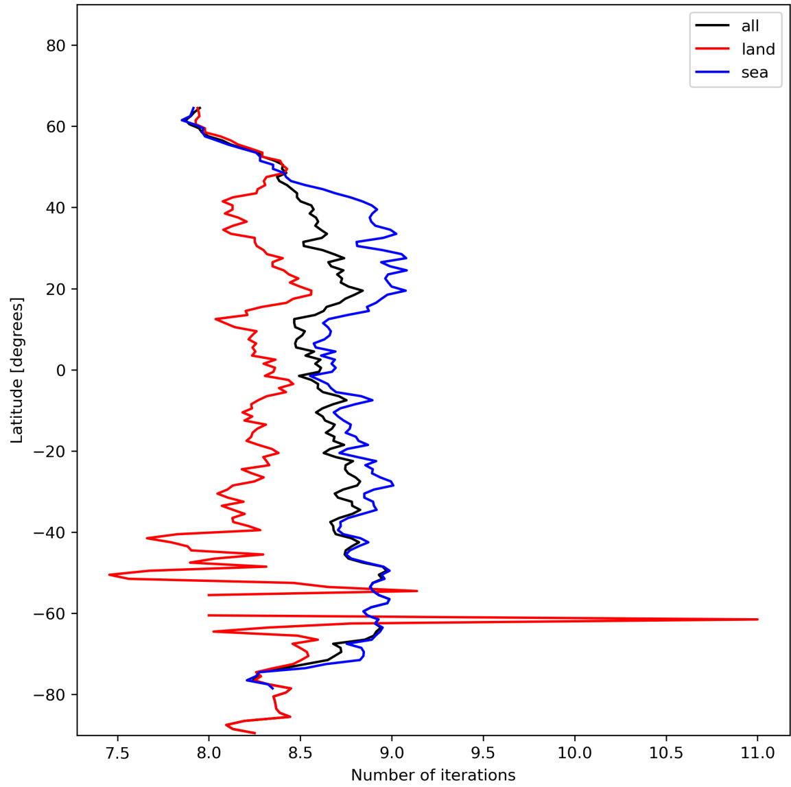
Figure 16: Zonal average of “Number of iterations” for 2023-11-24 to 2023-11-26.
