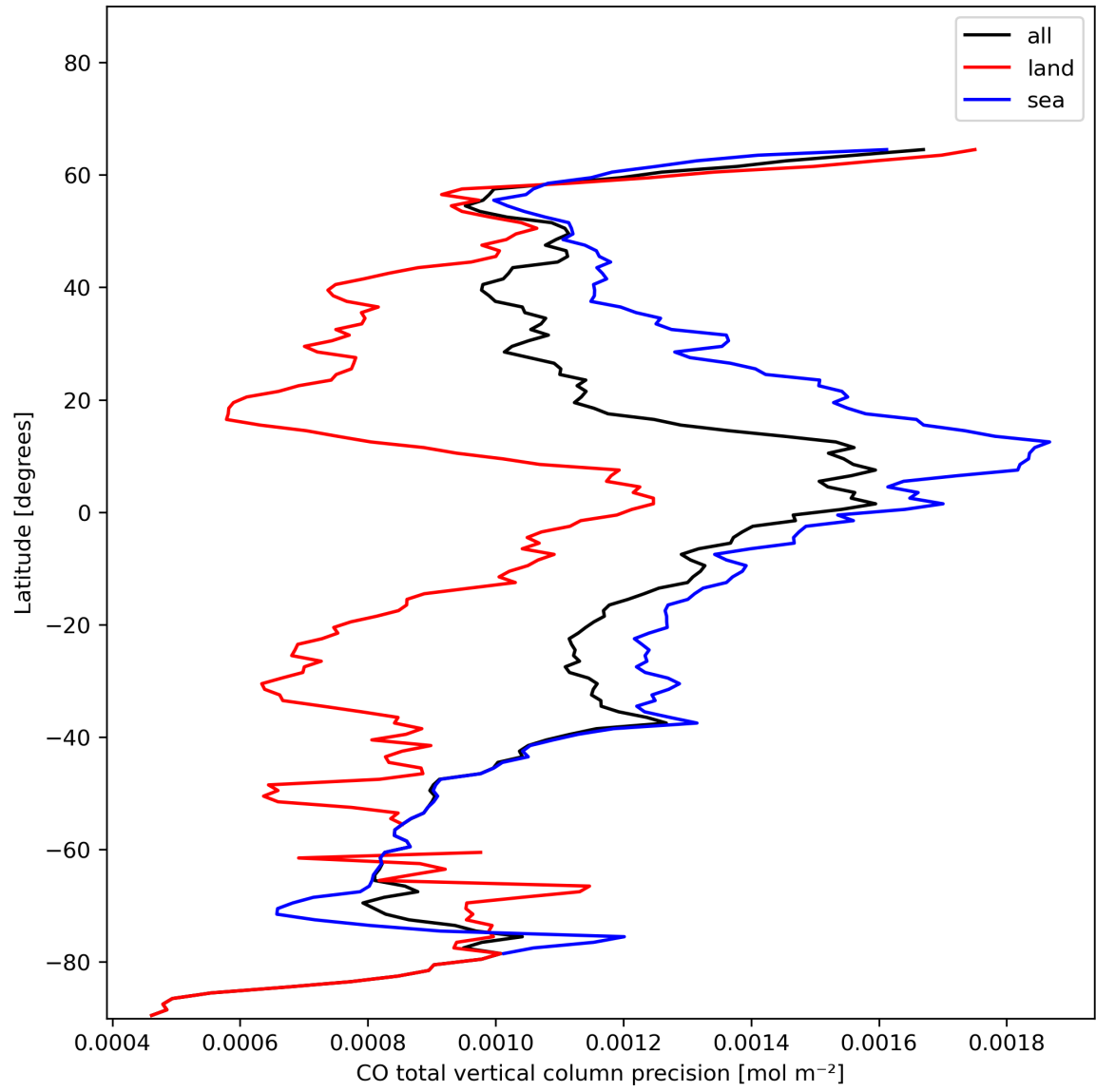
Figure 12: Zonal average of “CO total vertical column precision” for 2023-11-24 to 2023-11-26.
