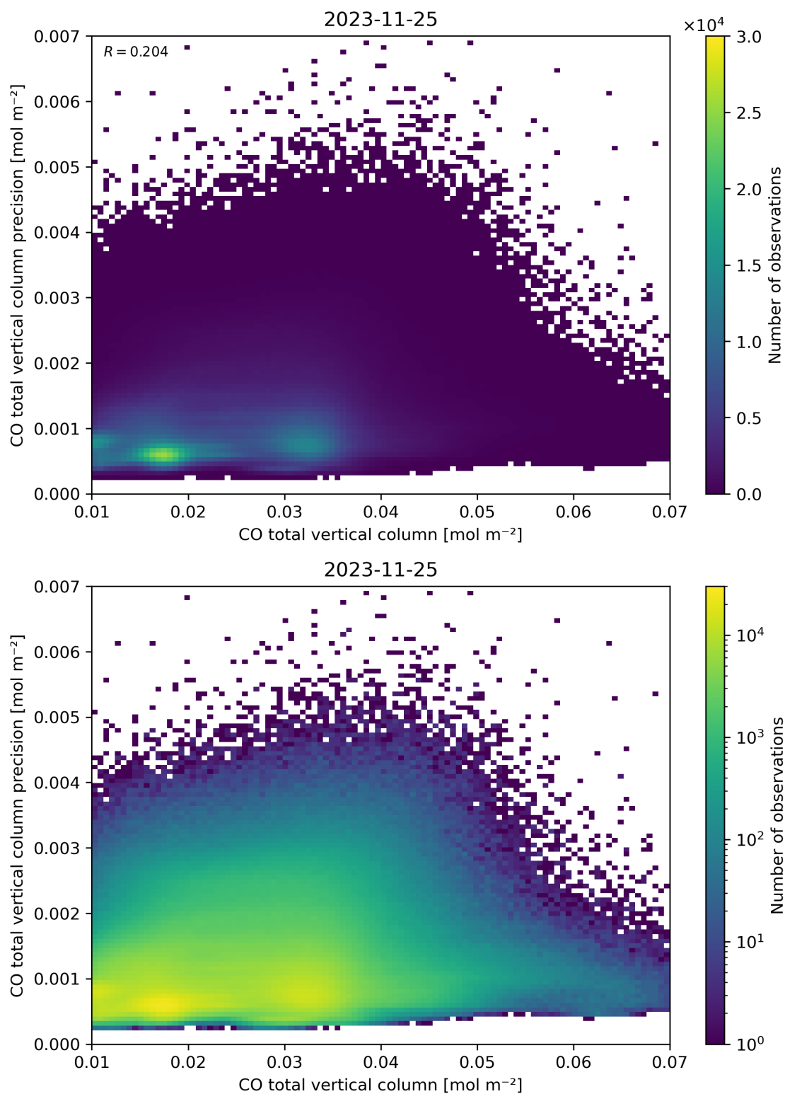
Figure 34: Scatter density plot of “CO total vertical column” against “CO total vertical column precision” for 2023-11-24 to 2023-11-26.
