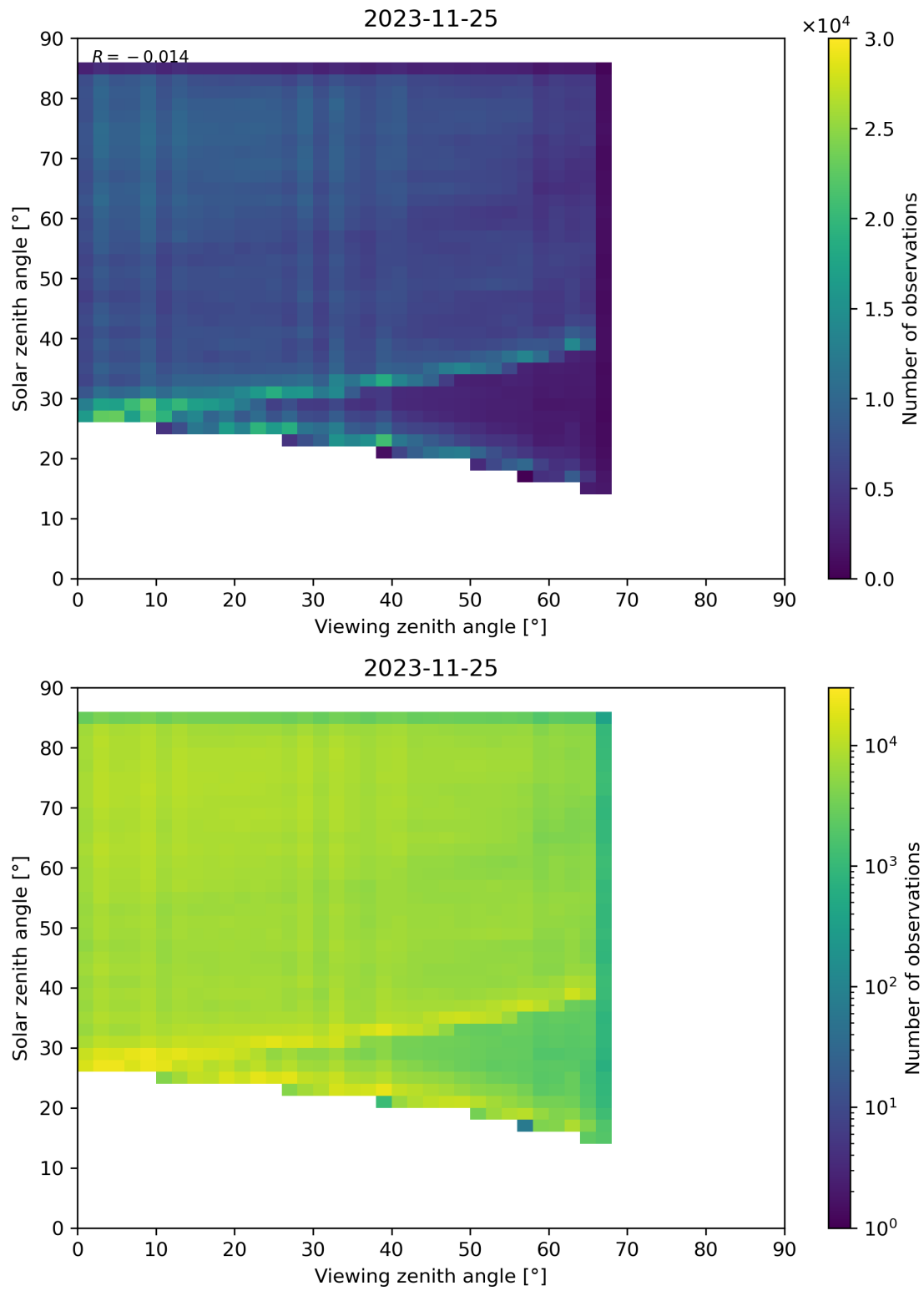
Figure 77: Scatter density plot of “Viewing zenith angle” against “Solar zenith angle” for 2023-11-24 to 2023-11-26.
