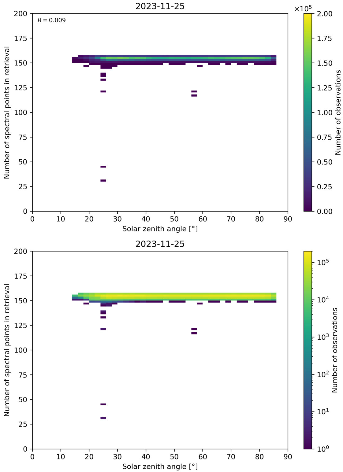
Figure 68: Scatter density plot of “Solar zenith angle” against “Number of spectral points in retrieval” for 2023-11-24 to 2023-11-26.
