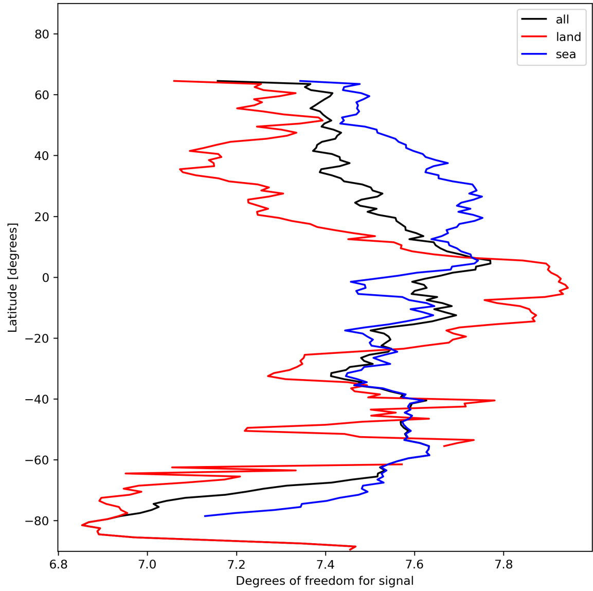
Figure 15: Zonal average of “Degrees of freedom for signal” for 2023-11-25 to 2023-11-27.
