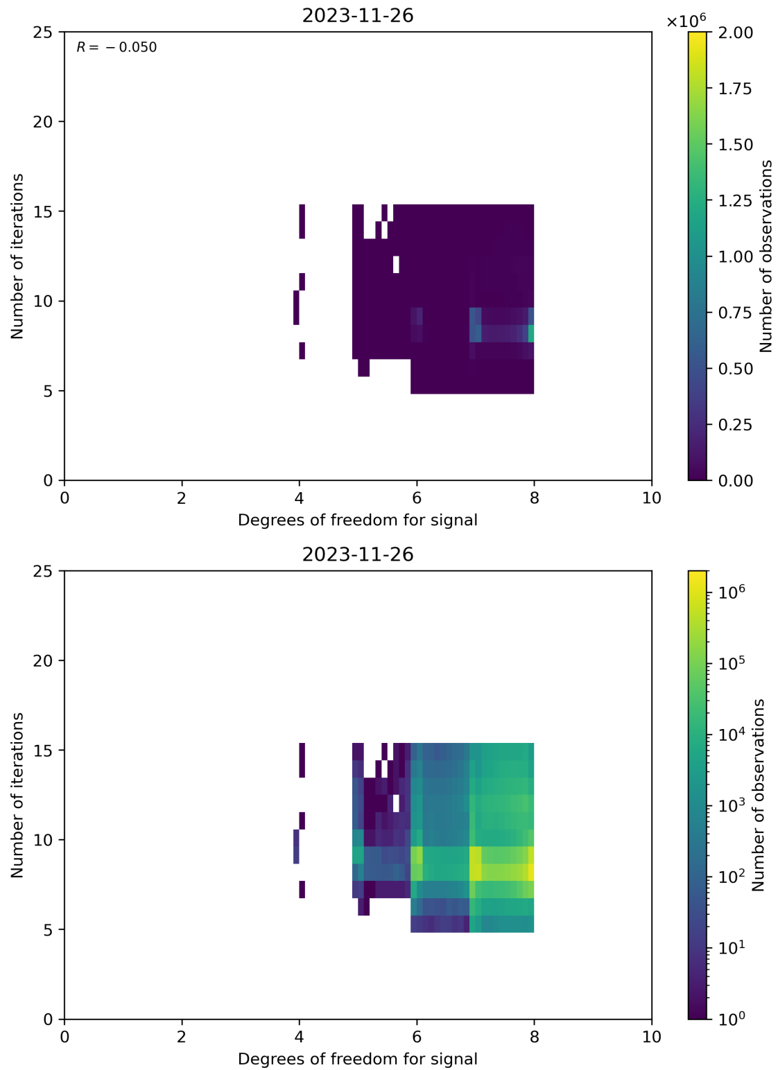
Figure 50: Scatter density plot of “Degrees of freedom for signal” against “Number of iterations” for 2023-11-25 to 2023-11-27.
