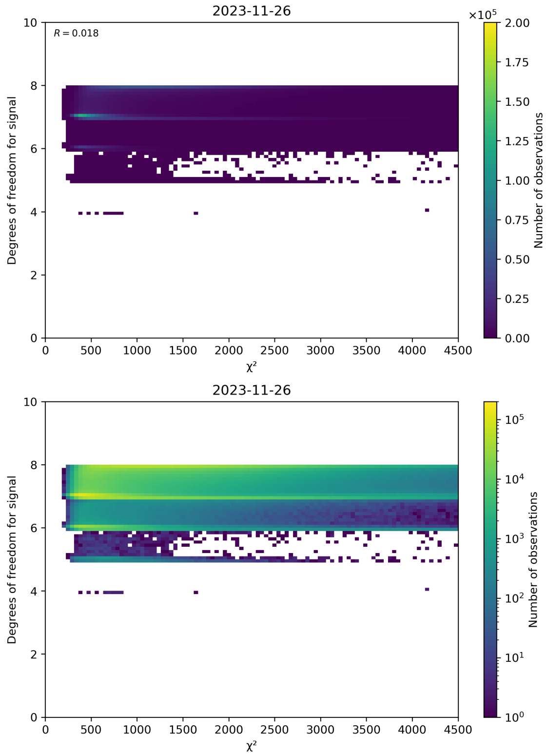
Figure 48: Scatter density plot of “ \chi^2 ” against “Degrees of freedom for signal” for 2023-11-25 to 2023-11-27.
