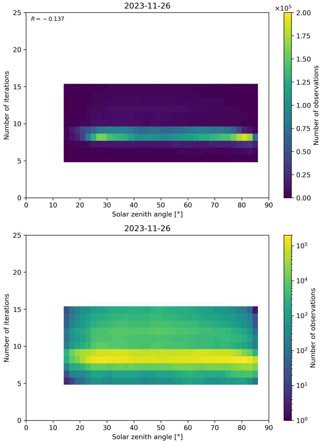
Figure 67: Scatter density plot of “Solar zenith angle” against “Number of iterations” for 2023-11-25 to 2023-11-27.
