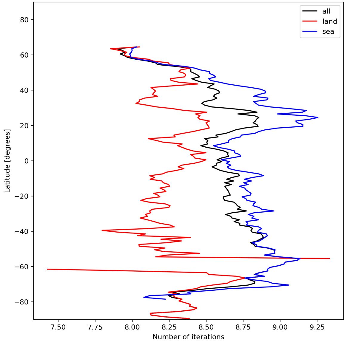
Figure 16: Zonal average of “Number of iterations” for 2023-11-25 to 2023-11-27.
