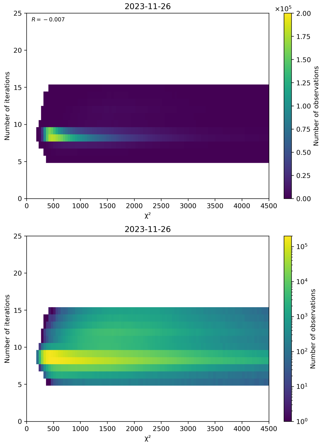
Figure 49: Scatter density plot of “ \chi^2 ” against “Number of iterations” for 2023-11-25 to 2023-11-27.
