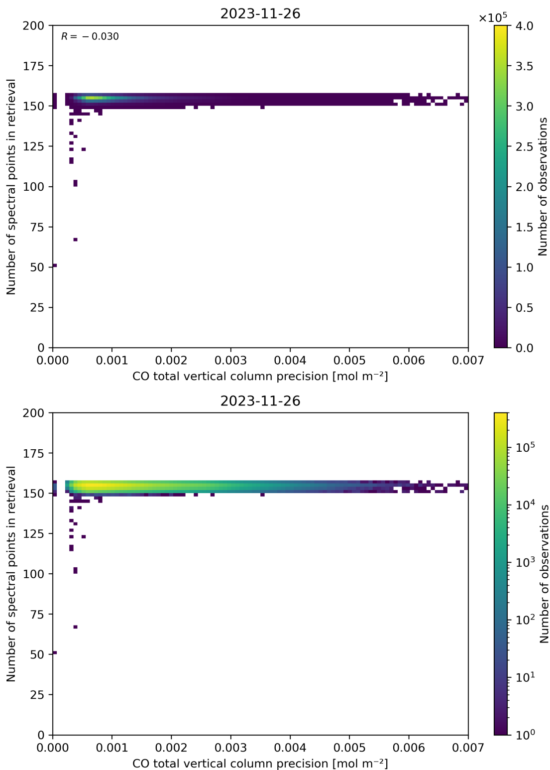
Figure 47: Scatter density plot of “CO total vertical column precision” against “Number of spectral points in retrieval” for 2023-11-25 to 2023-11-27.
