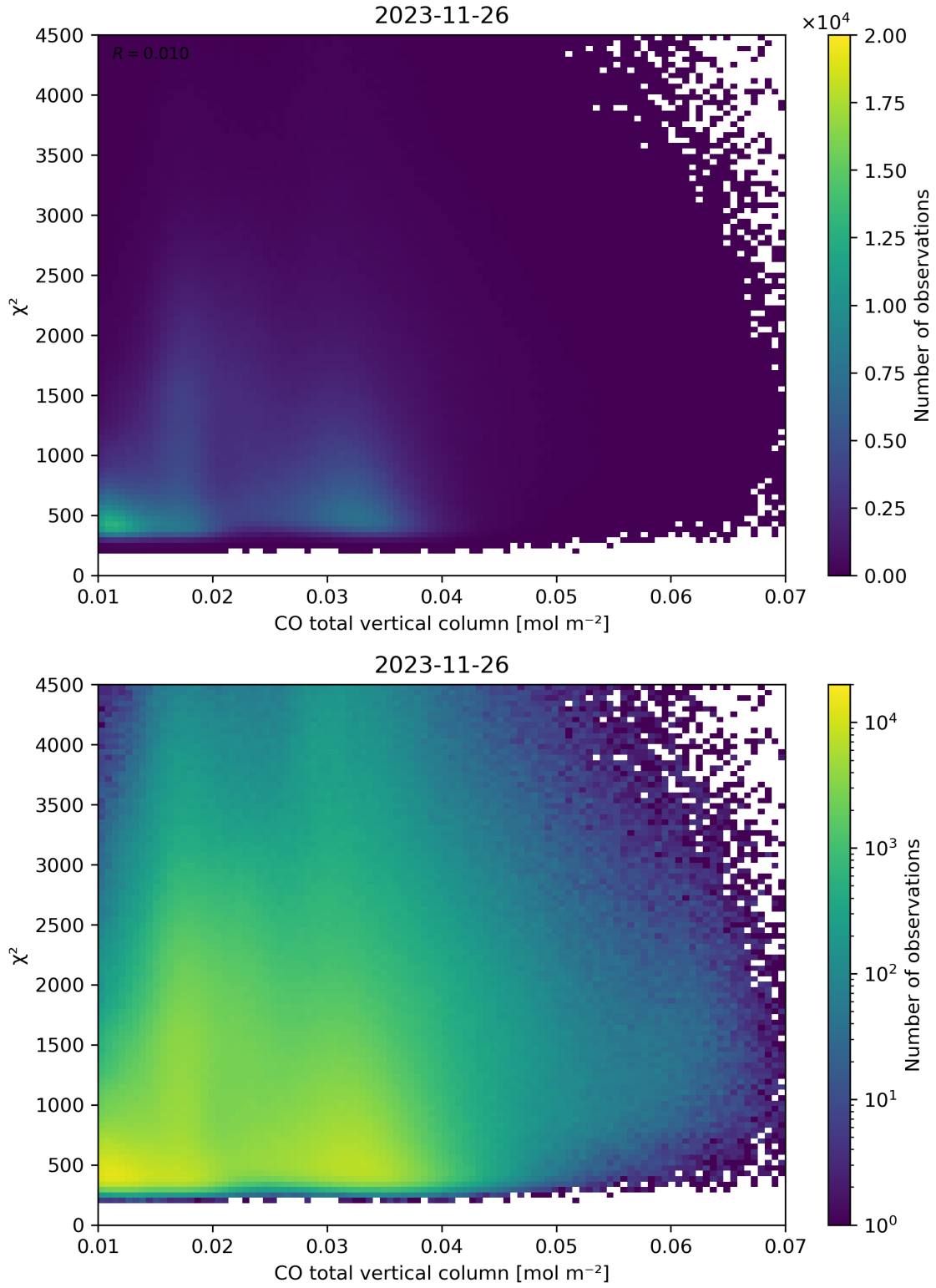
Figure 35: Scatter density plot of “CO total vertical column” against “ \chi^2 ” for 2023-11-25 to 2023-11-27.
