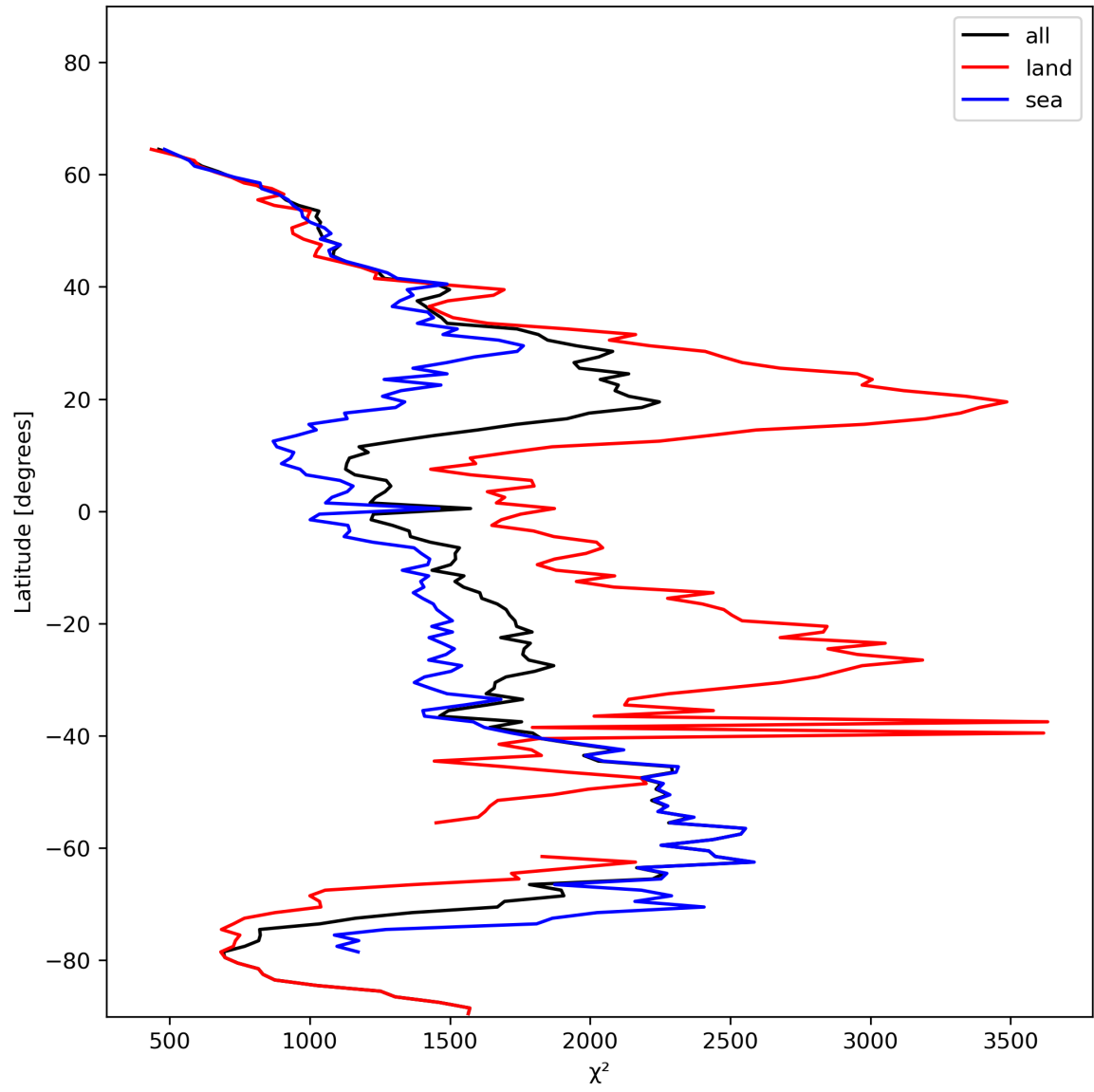
Figure 14: Zonal average of “ \chi^2 ” for 2023-11-25 to 2023-11-27.
