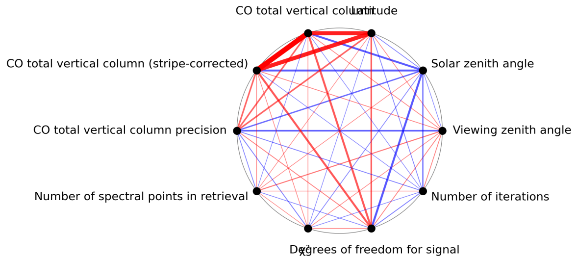
Figure 1: Map of correlation graph for 2023-11-25 to 2023-11-27.
