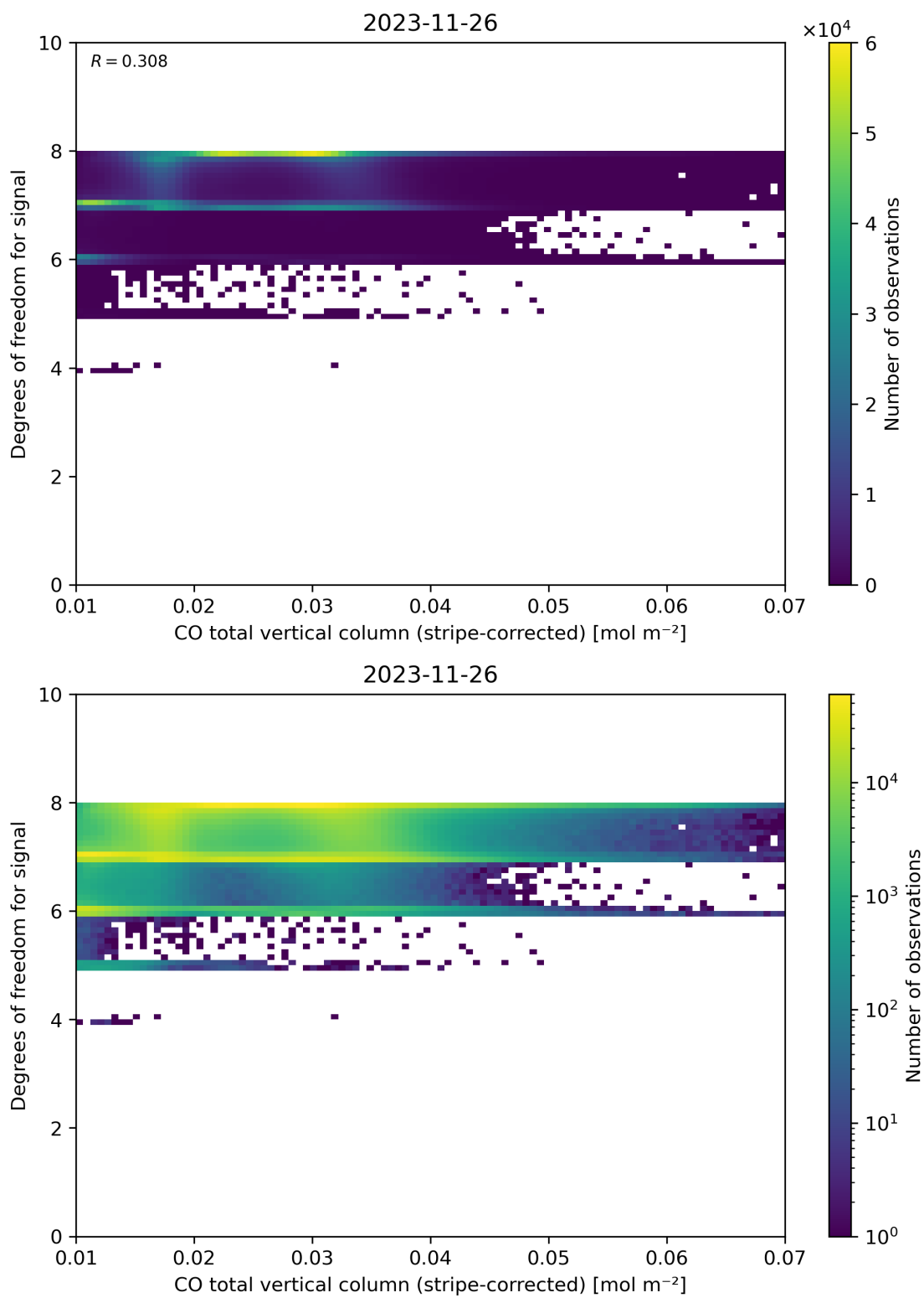
Figure 38: Scatter density plot of “CO total vertical column (stripe-corrected)” against “Degrees of freedom for signal” for 2023-11-25 to 2023-11-27.
