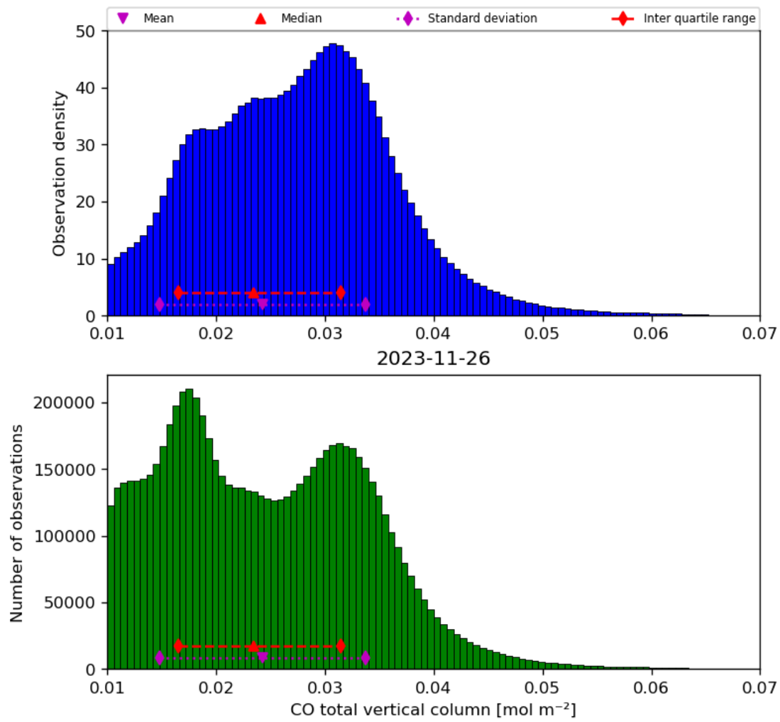
Figure 18: Histogram of “CO total vertical column” for 2023-11-25 to 2023-11-27
