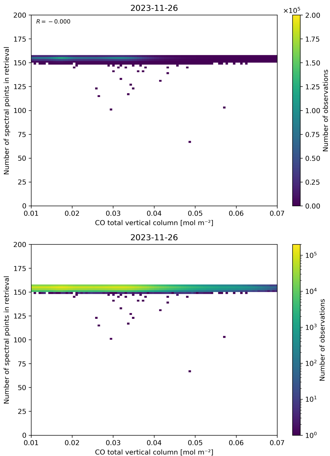
Figure 43: Scatter density plot of “CO total vertical column” against “Number of spectral points in retrieval” for 2023-11-25 to 2023-11-27.
