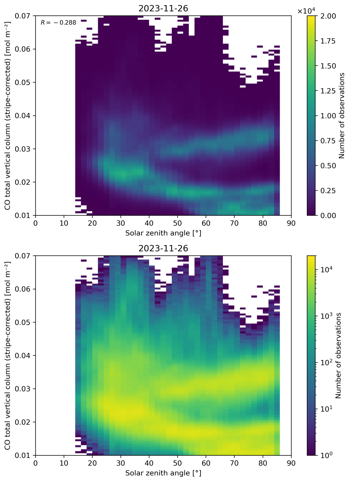
Figure 62: Scatter density plot of “Solar zenith angle” against “CO total vertical column (stripe-corrected)” for 2023-11-25 to 2023-11-27.
