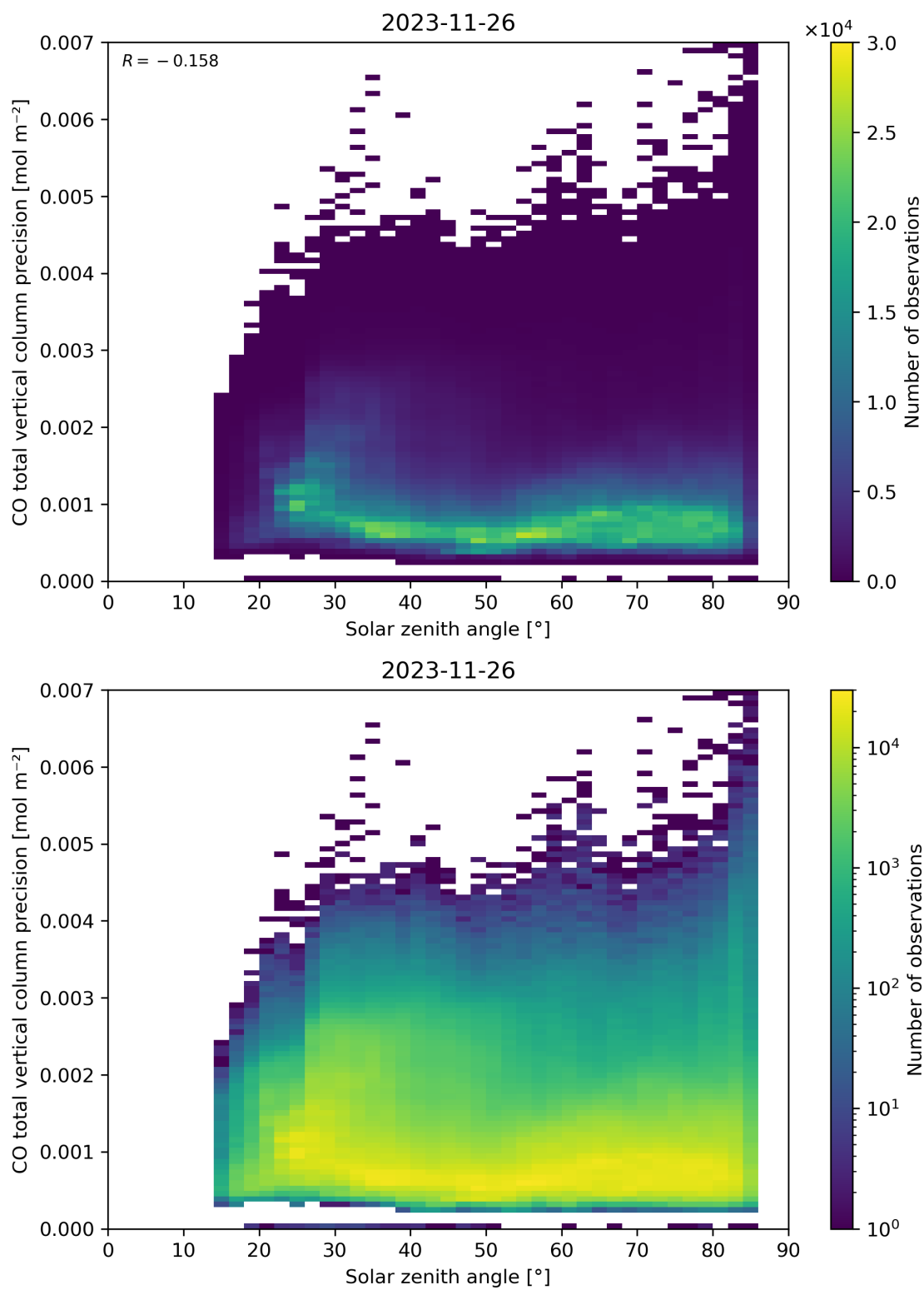
Figure 63: Scatter density plot of “Solar zenith angle” against “CO total vertical column precision” for 2023-11-25 to 2023-11-27.
