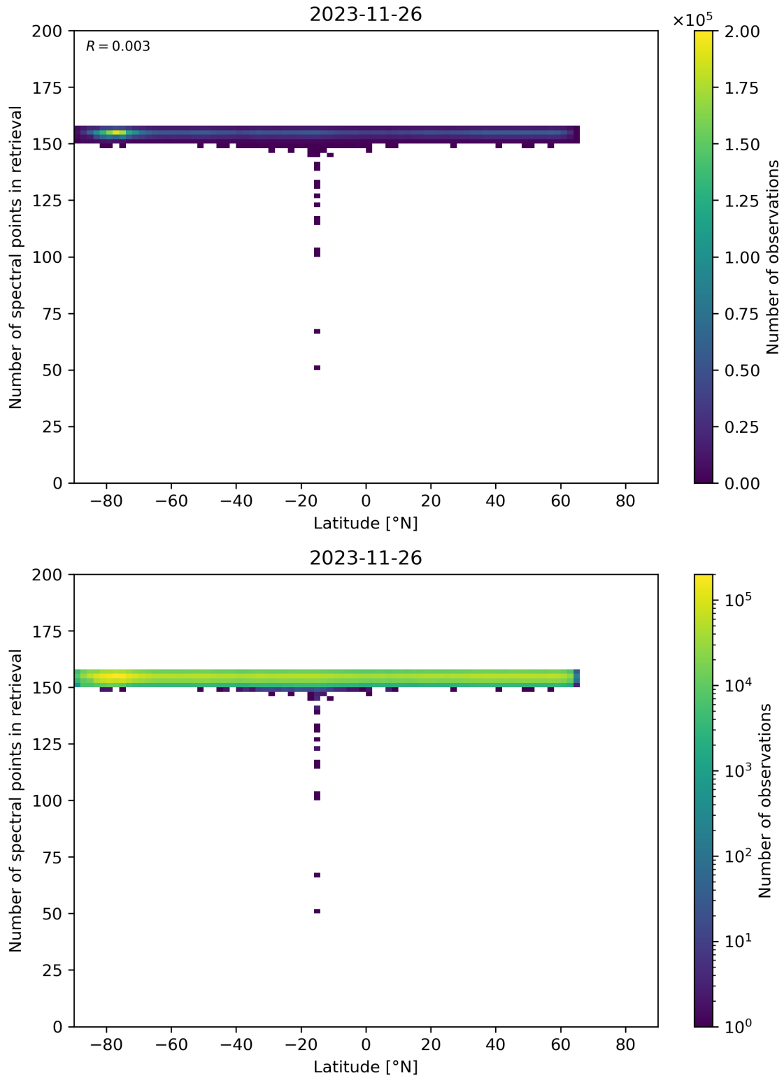
Figure 57: Scatter density plot of “Latitude” against “Number of spectral points in retrieval” for 2023-11-25 to 2023-11-27.
