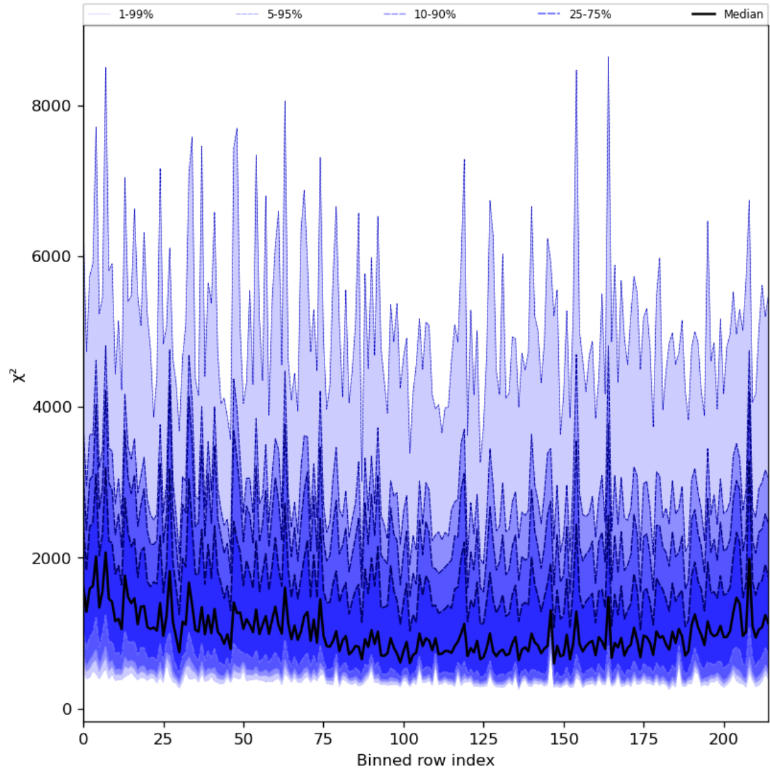
Figure 30: Along track statistics of “ \chi^2 ” for 2023-11-25 to 2023-11-27
