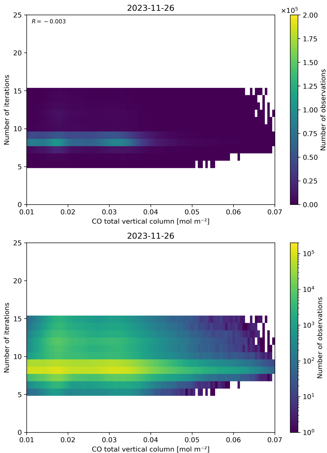
Figure 42: Scatter density plot of “CO total vertical column” against “Number of iterations” for 2023-11-25 to 2023-11-27.
