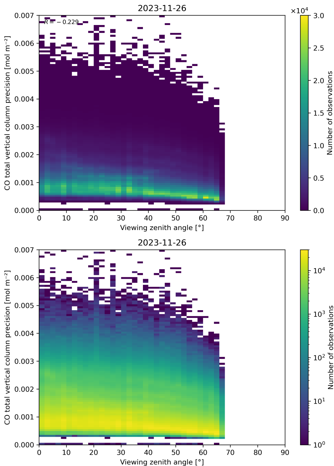
Figure 71: Scatter density plot of “Viewing zenith angle” against “CO total vertical column precision” for 2023-11-25 to 2023-11-27.
