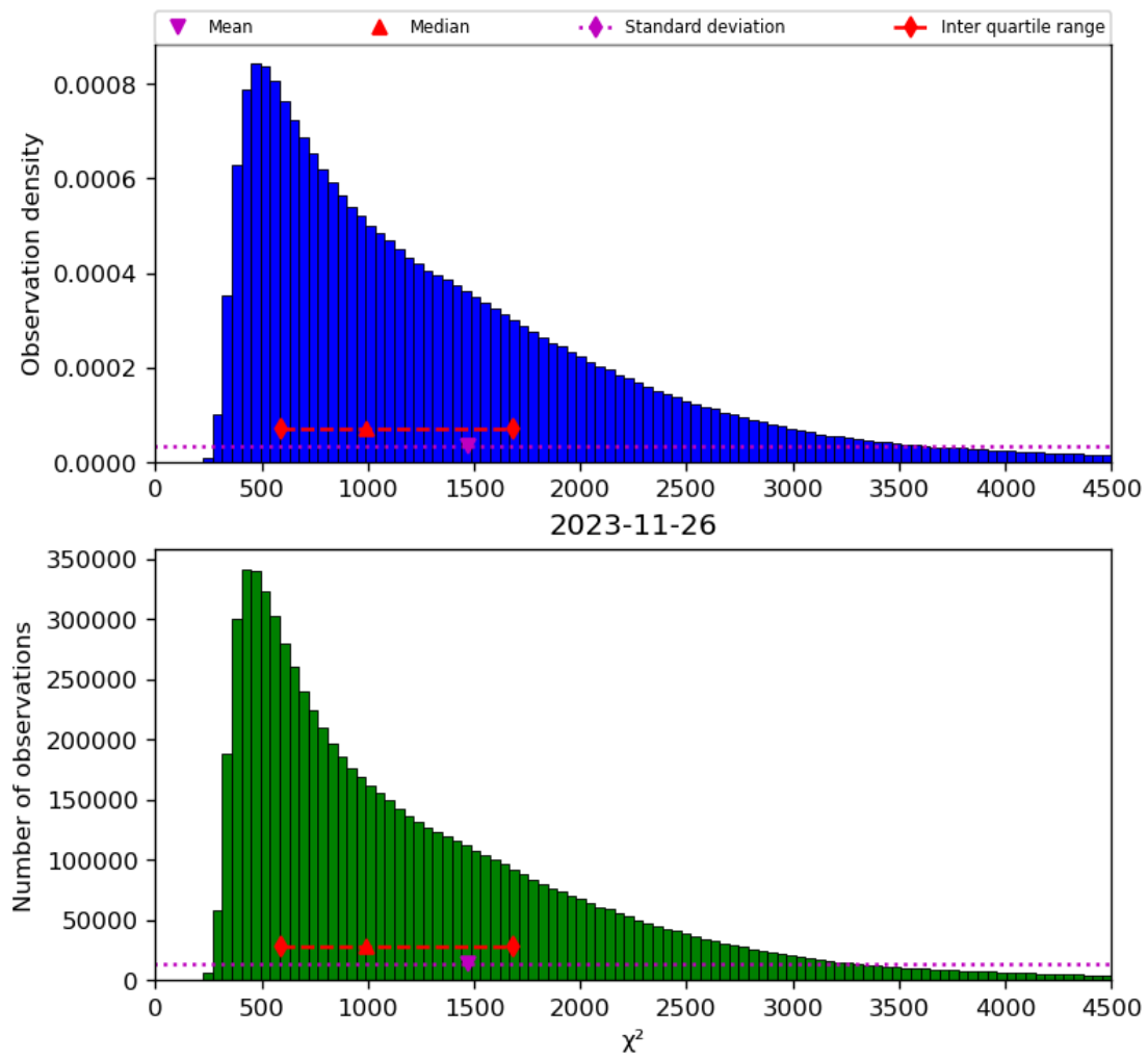
Figure 22: Histogram of “ \chi^2 ” for 2023-11-25 to 2023-11-27
