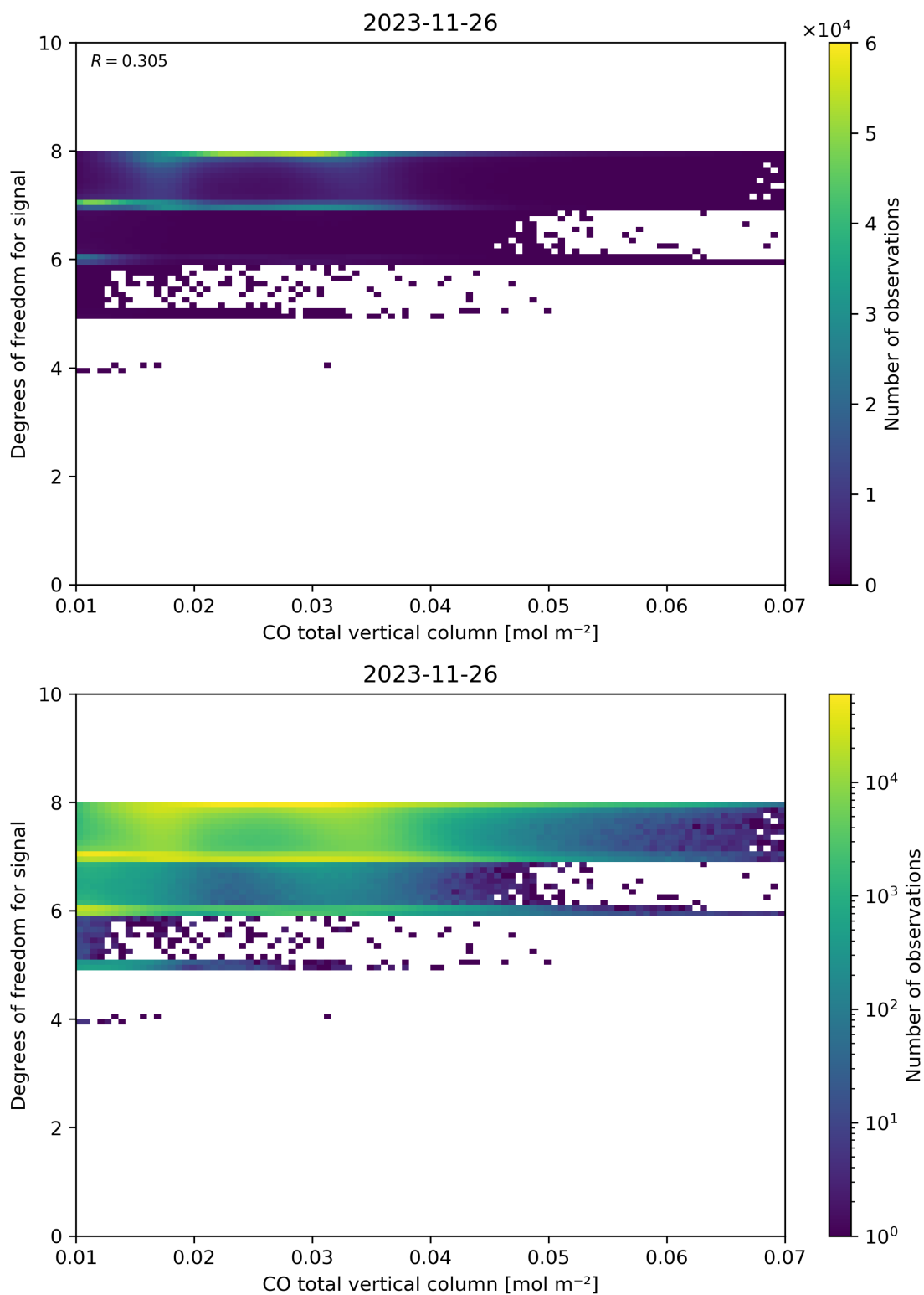
Figure 41: Scatter density plot of “CO total vertical column” against “Degrees of freedom for signal” for 2023-11-25 to 2023-11-27.
