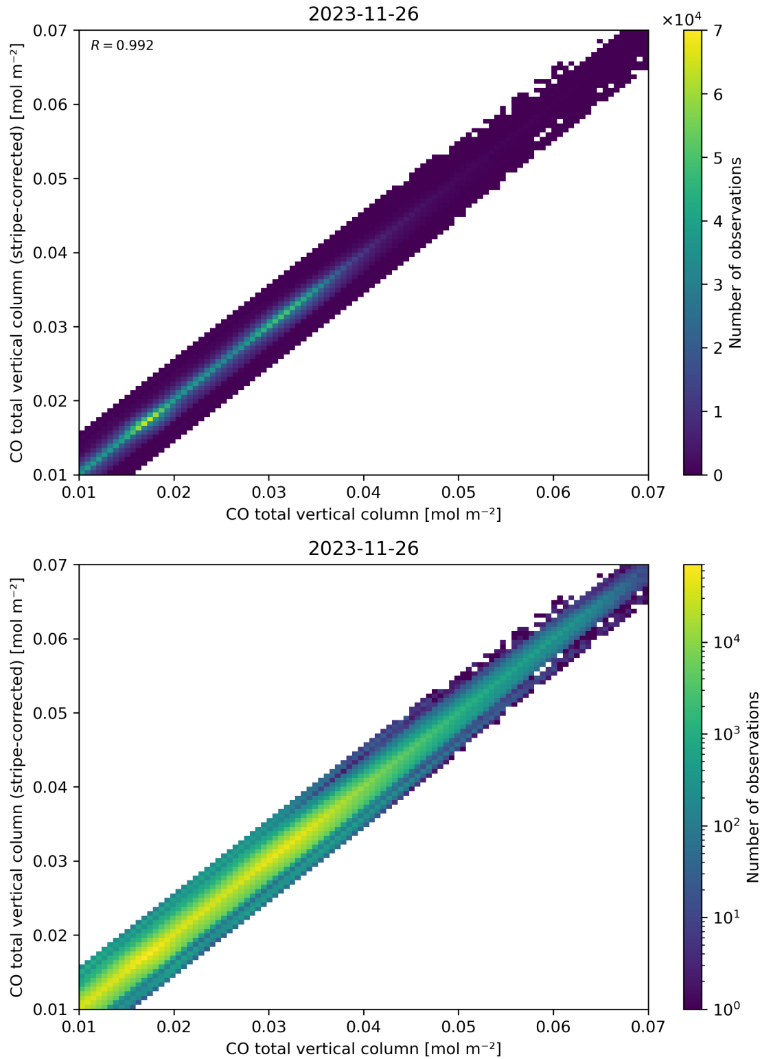
Figure 33: Scatter density plot of “CO total vertical column” against “CO total vertical column (stripe-corrected)” for 2023-11-25 to 2023-11-27.
