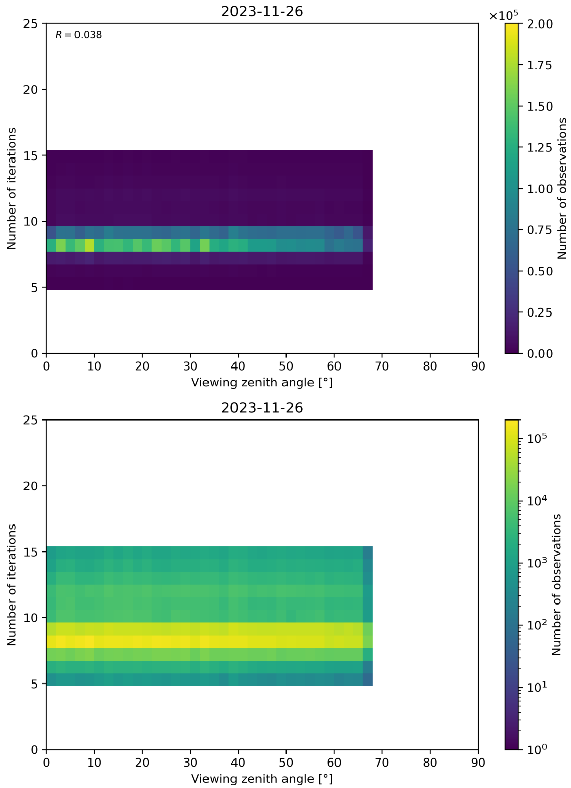
Figure 75: Scatter density plot of “Viewing zenith angle” against “Number of iterations” for 2023-11-25 to 2023-11-27.
