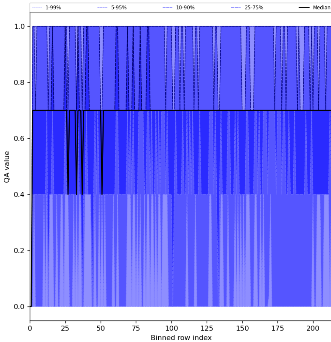
Figure 25: Along track statistics of “QA value” for 2023-11-25 to 2023-11-27
