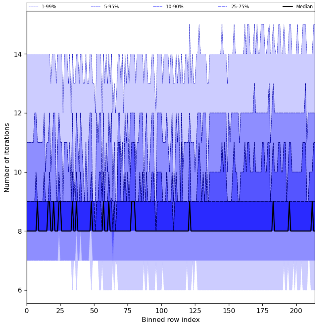
Figure 32: Along track statistics of “Number of iterations” for 2023-11-25 to 2023-11-27
