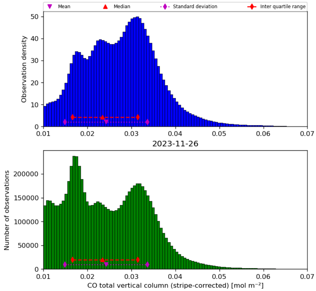
Figure 19: Histogram of “CO total vertical column (stripe-corrected)” for 2023-11-25 to 2023-11-27
