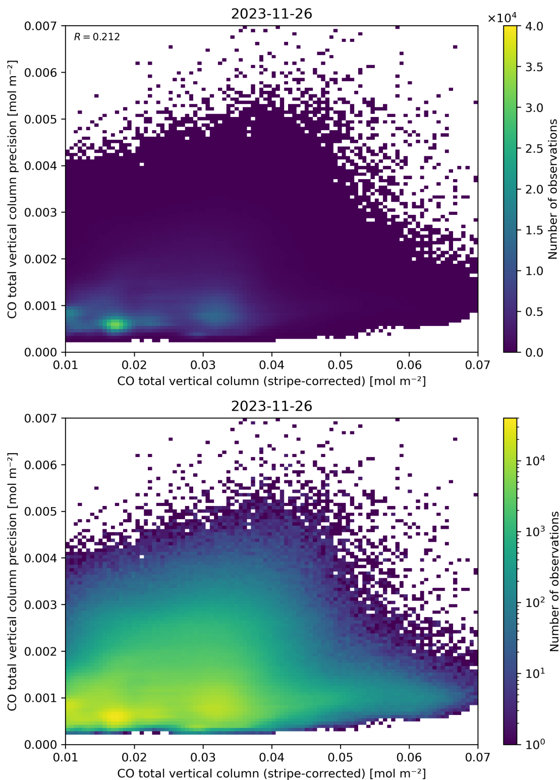
Figure 36: Scatter density plot of “CO total vertical column (stripe-corrected)” against “CO total vertical column precision” for 2023-11-25 to 2023-11-27.
