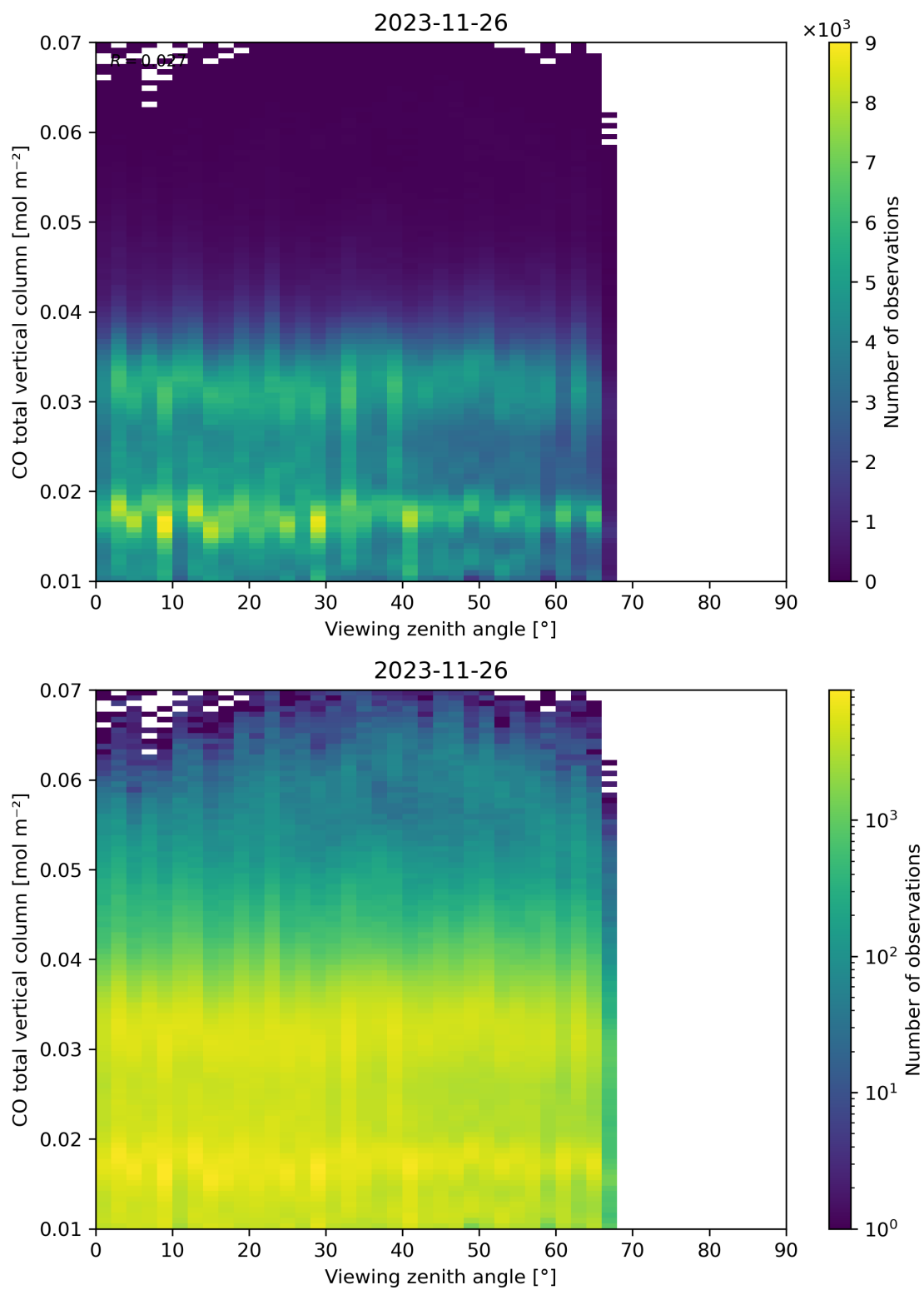
Figure 69: Scatter density plot of “Viewing zenith angle” against “CO total vertical column” for 2023-11-25 to 2023-11-27.
