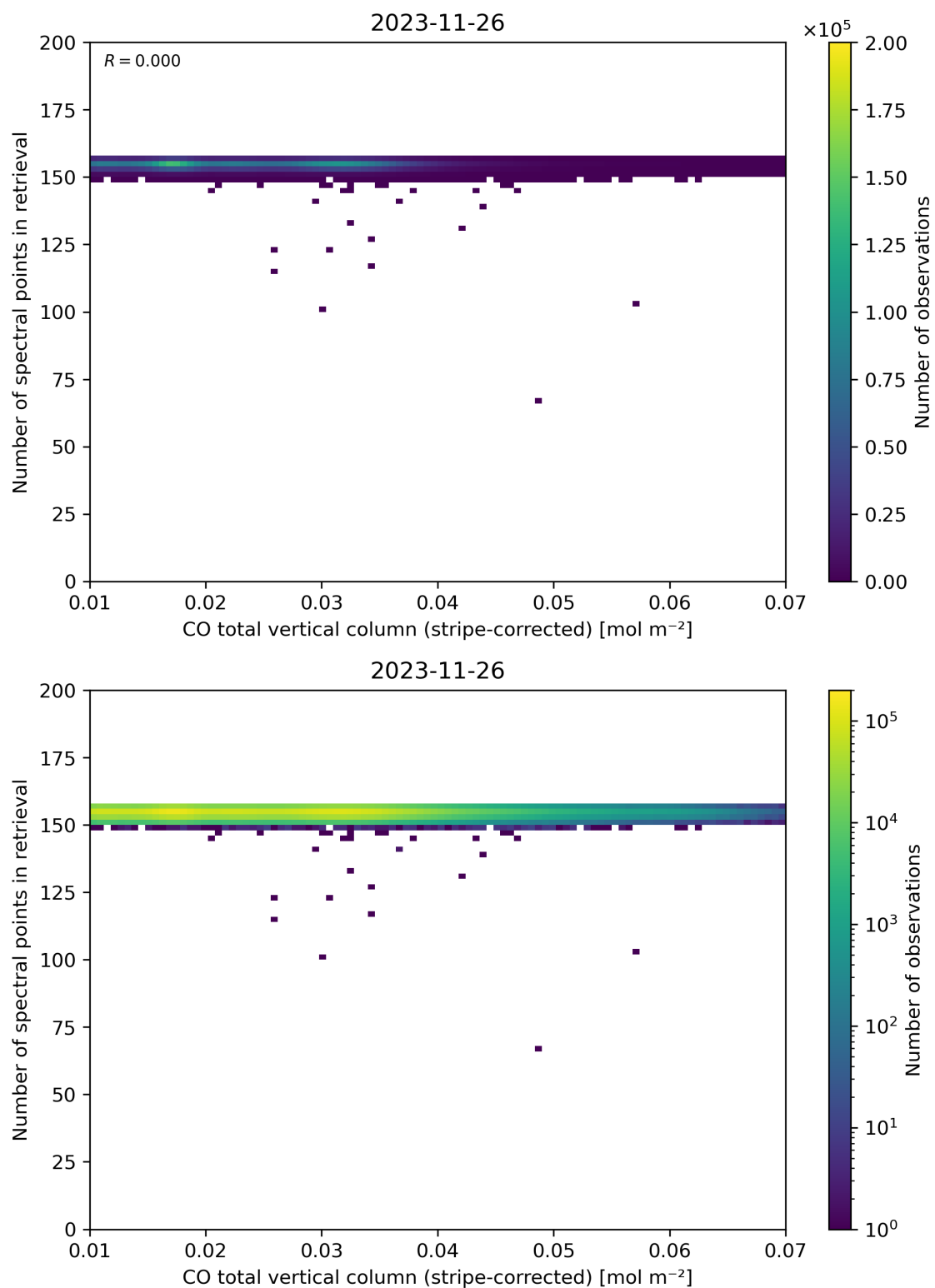
Figure 40: Scatter density plot of “CO total vertical column (stripe-corrected)” against “Number of spectral points in retrieval” for 2023-11-25 to 2023-11-27.
