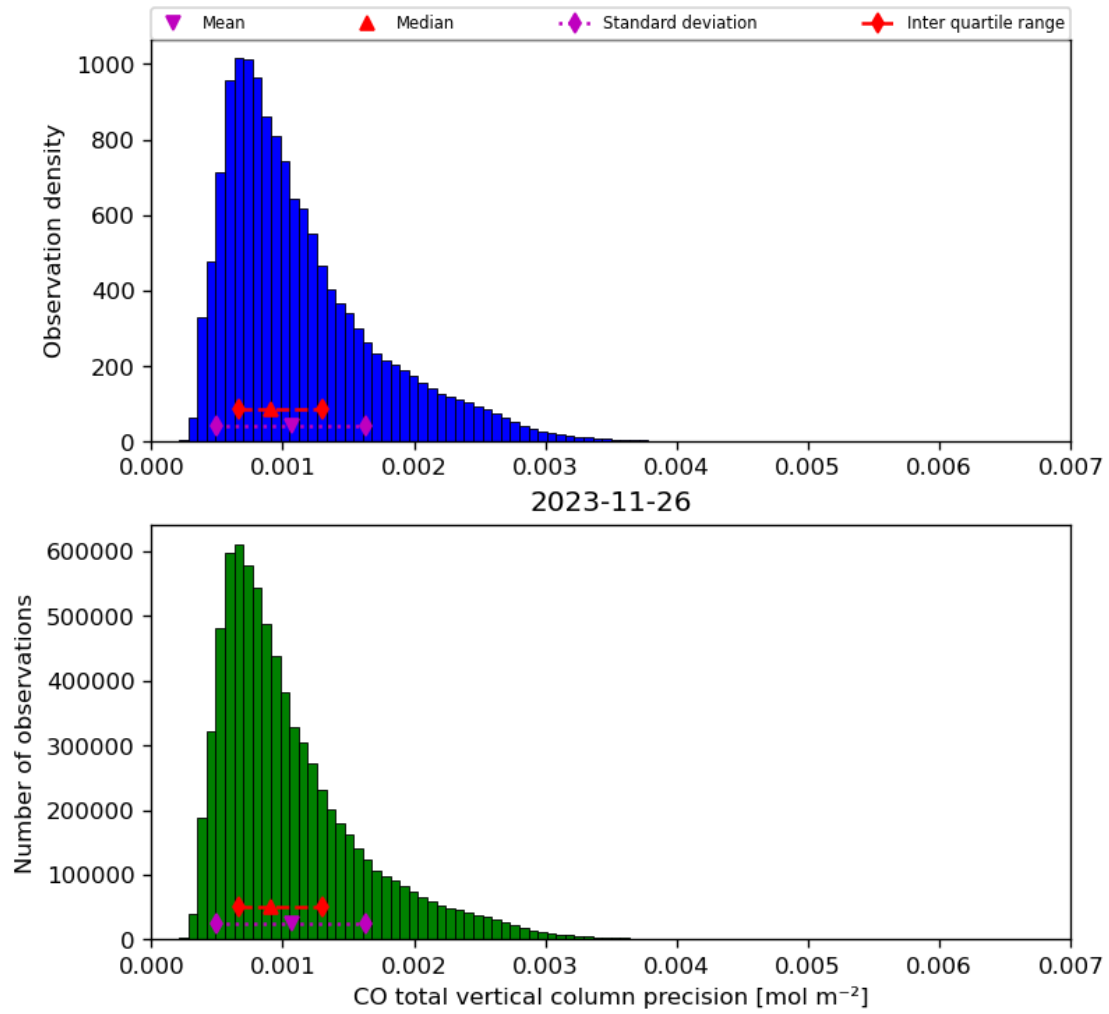
Figure 20: Histogram of “CO total vertical column precision” for 2023-11-25 to 2023-11-27
