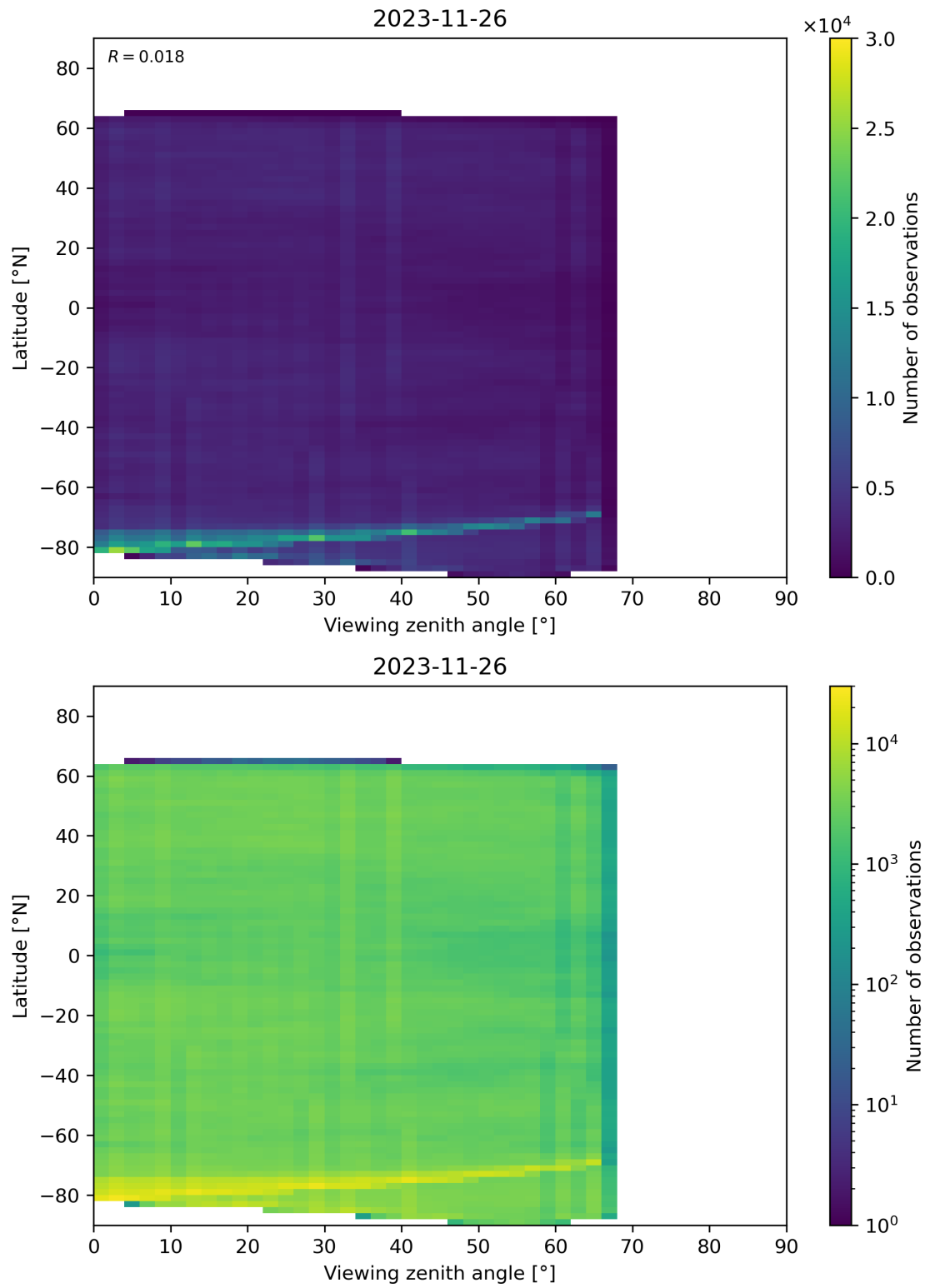
Figure 74: Scatter density plot of “Viewing zenith angle” against “Latitude” for 2023-11-25 to 2023-11-27.
