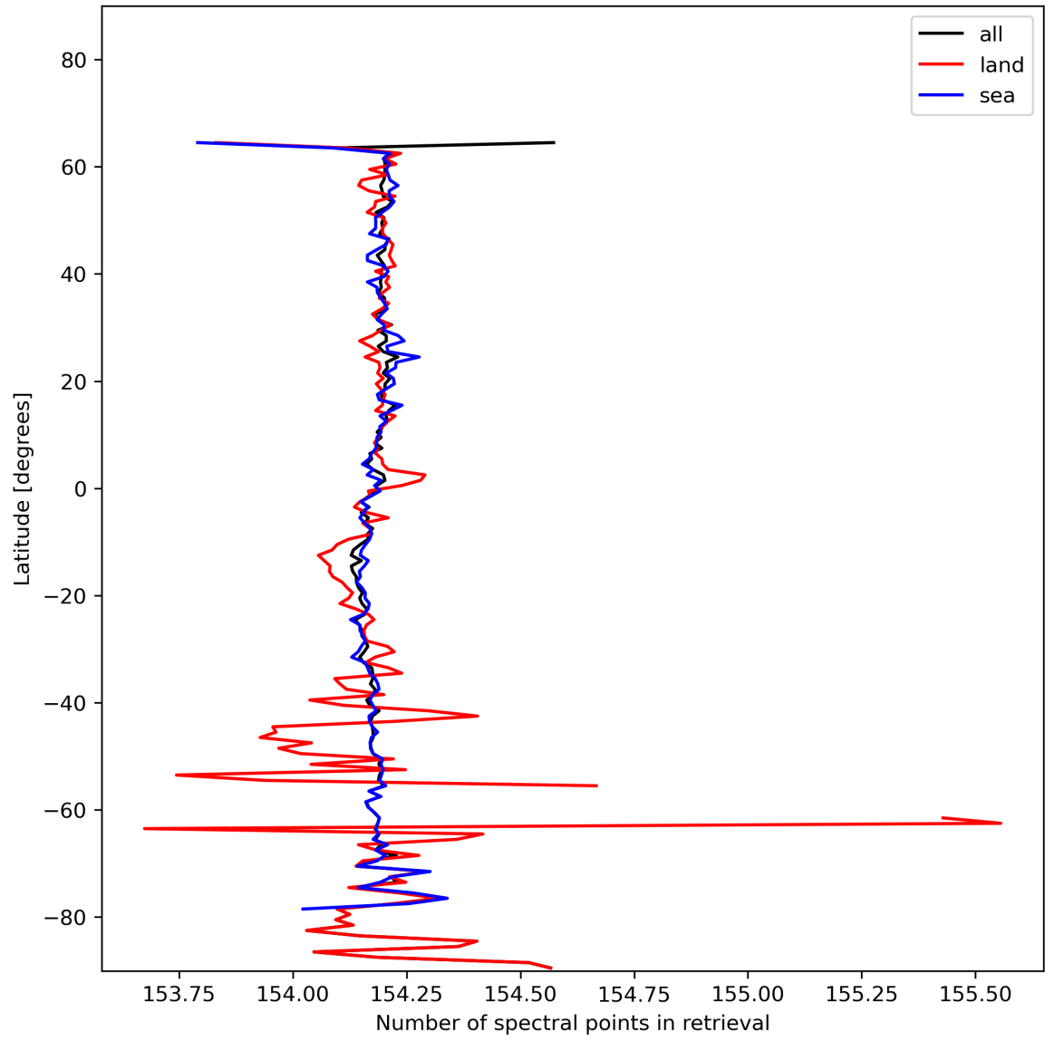
Figure 13: Zonal average of “Number of spectral points in retrieval” for 2023-11-25 to 2023-11-27.
