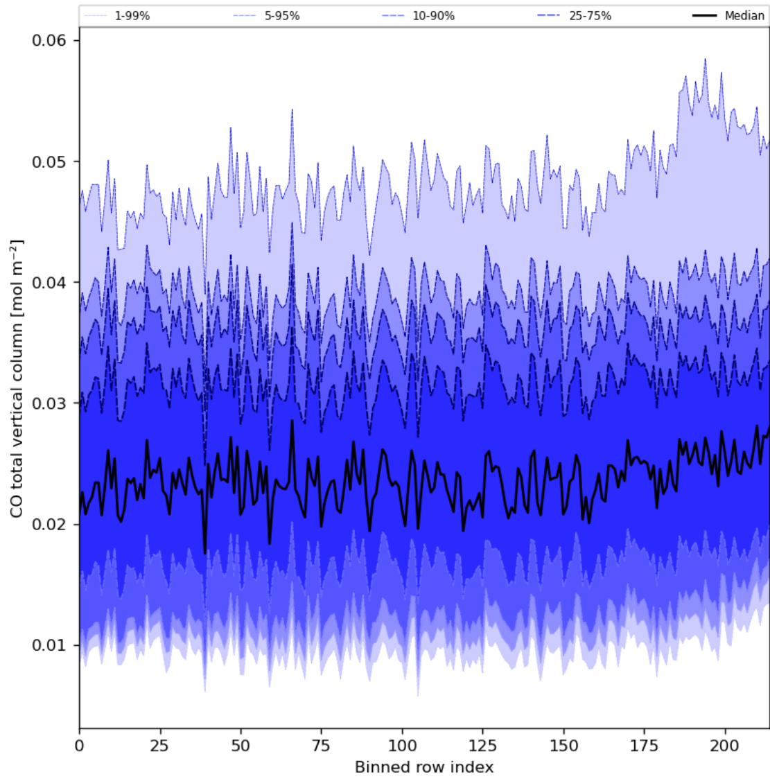
Figure 26: Along track statistics of “CO total vertical column” for 2023-11-25 to 2023-11-27
