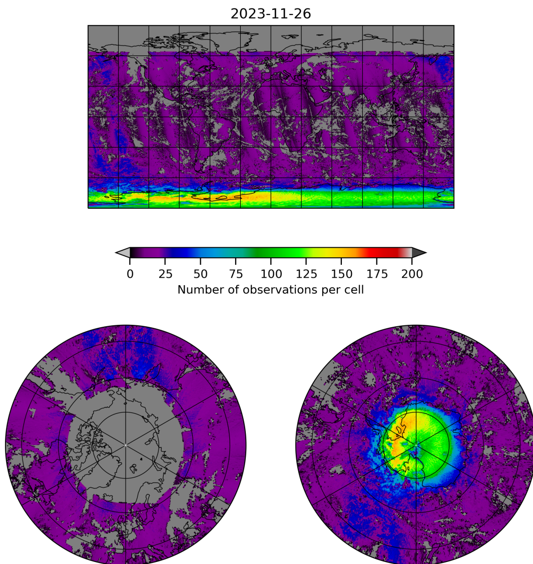
Figure 8: Map of the number of observations for 2023-11-25 to 2023-11-27
