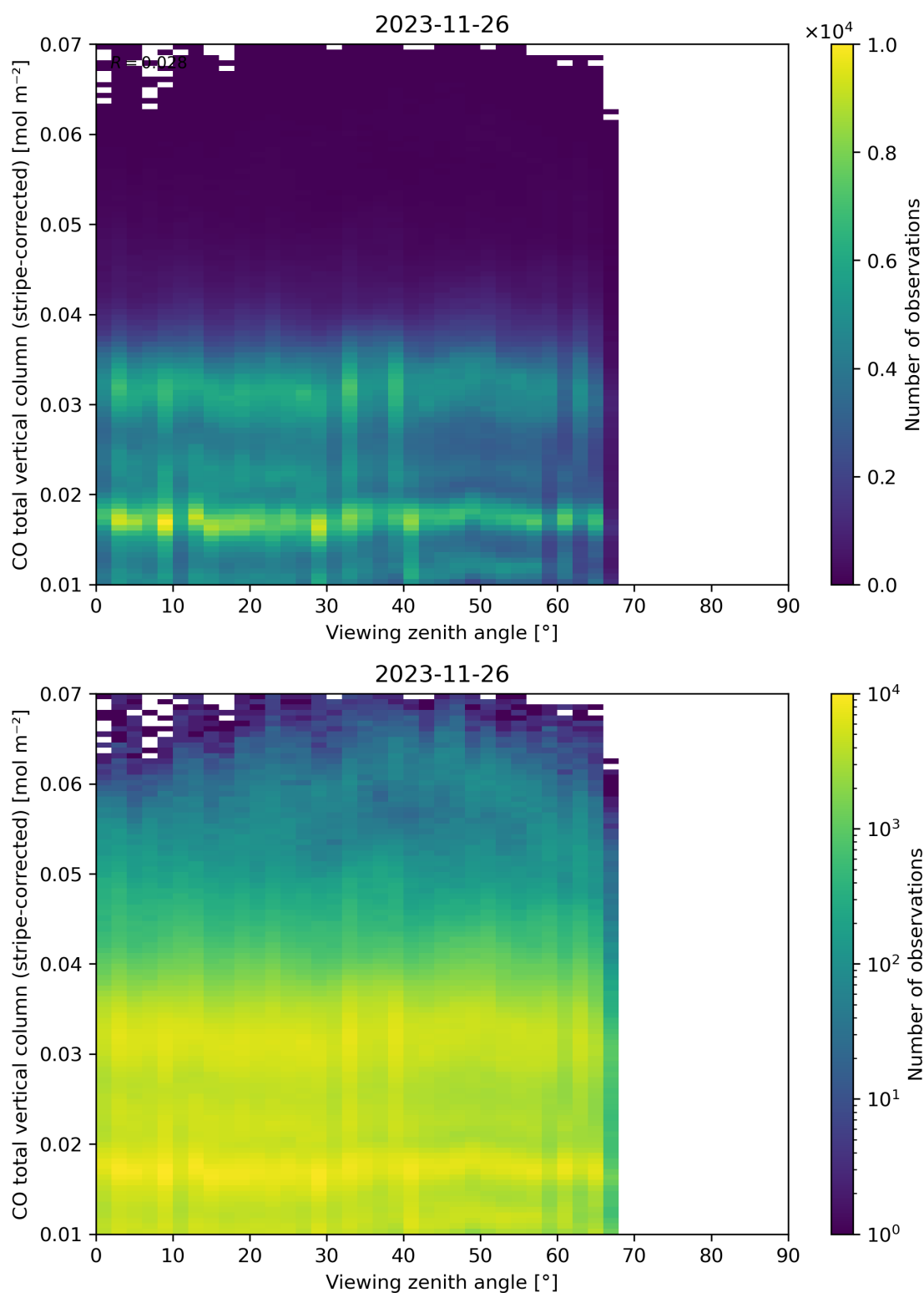
Figure 70: Scatter density plot of “Viewing zenith angle” against “CO total vertical column (stripe-corrected)” for 2023-11-25 to 2023-11-27.
