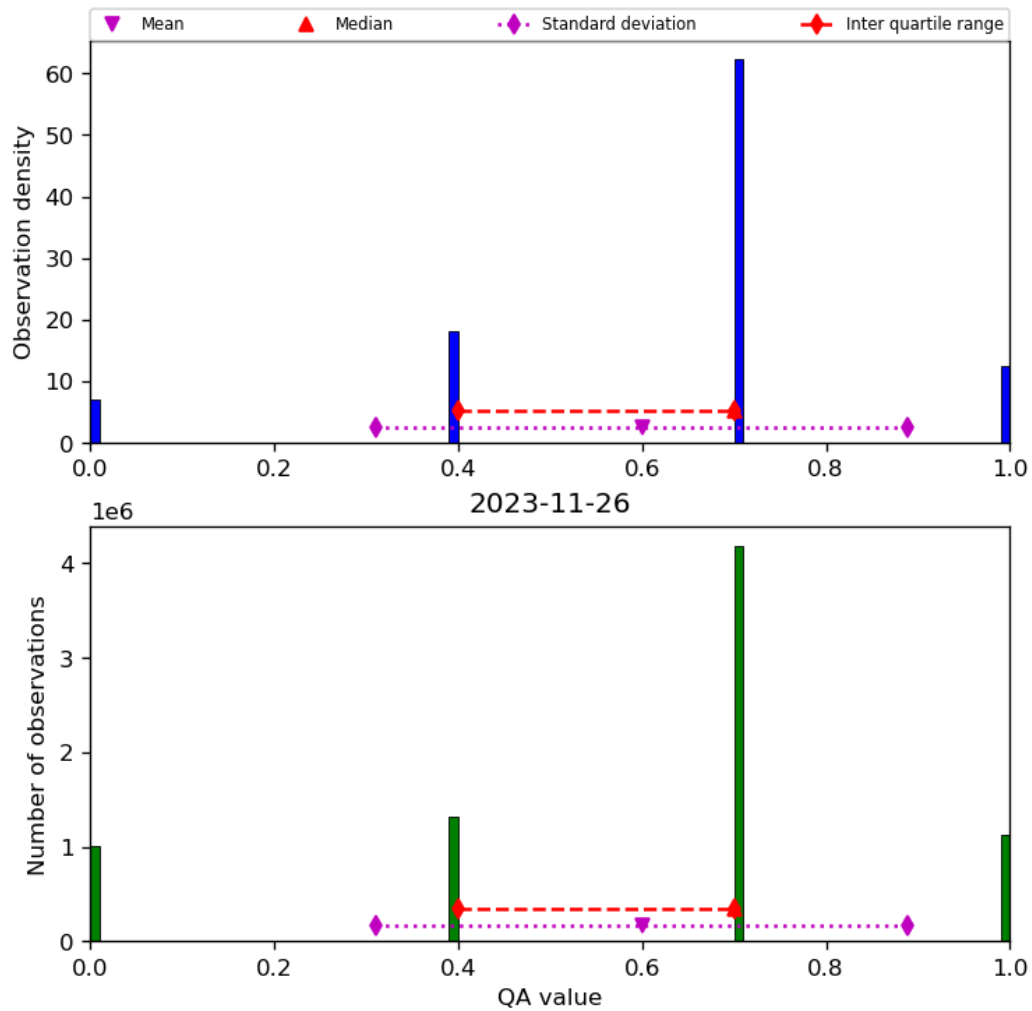
Figure 17: Histogram of “QA value” for 2023-11-25 to 2023-11-27
