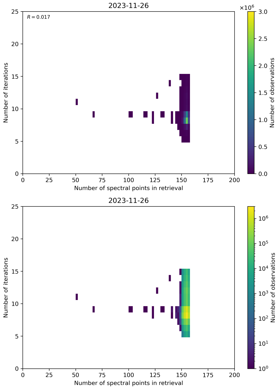
Figure 60: Scatter density plot of “Number of spectral points in retrieval” against “Number of iterations” for 2023-11-25 to 2023-11-27.
