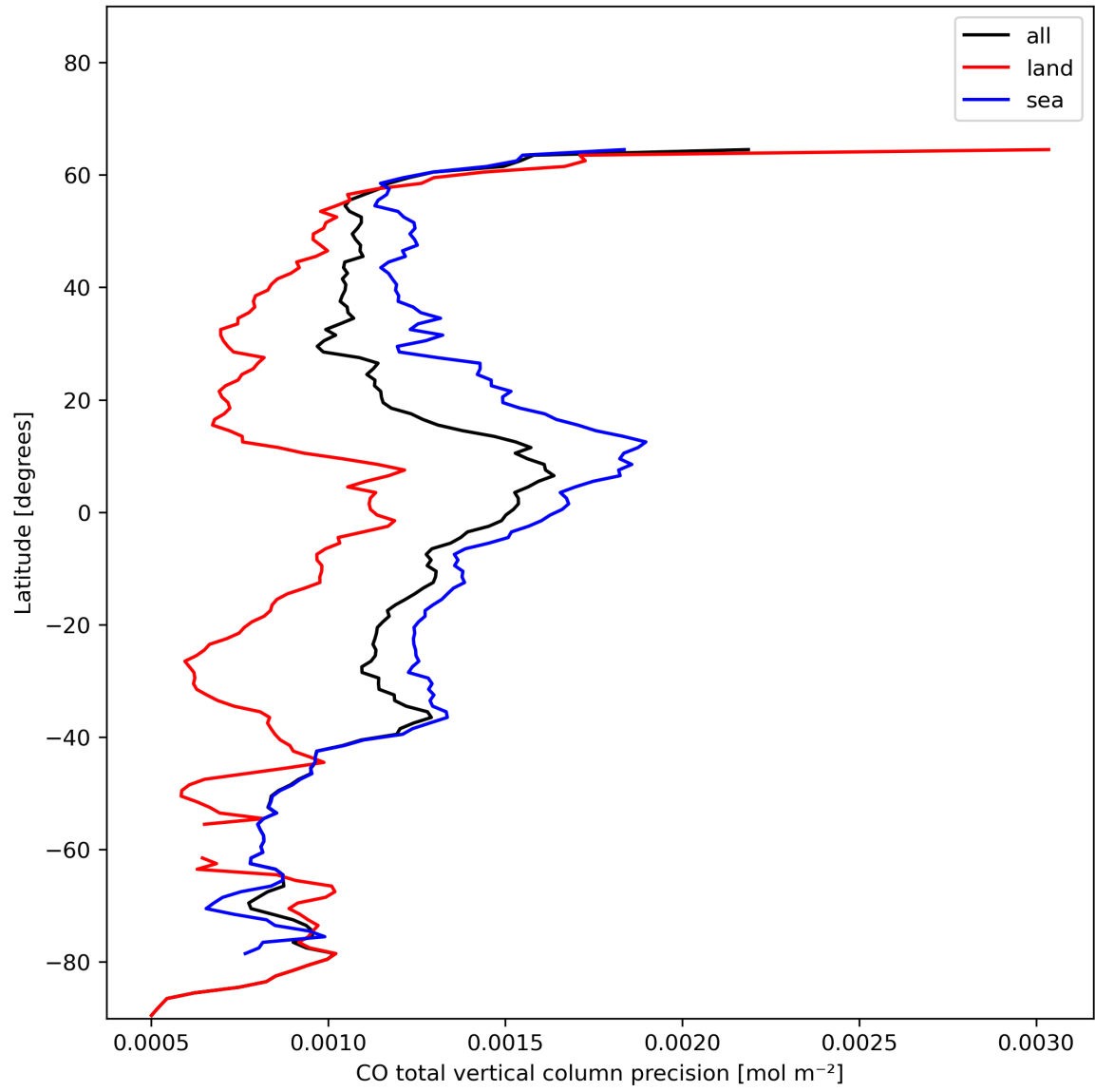
Figure 12: Zonal average of "CO total vertical column precision" for 2023-11-25 to 2023-11-27.
