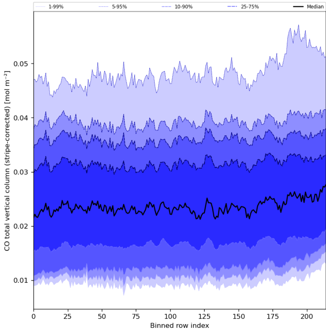
Figure 27: Along track statistics of “CO total vertical column (stripe-corrected)” for 2023-11-25 to 2023-11-27
