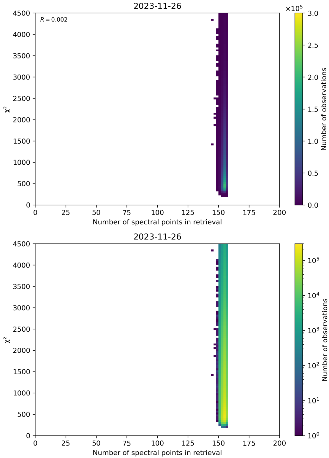
Figure 58: Scatter density plot of “Number of spectral points in retrieval” against “ \chi^2 ” for 2023-11-25 to 2023-11-27.
