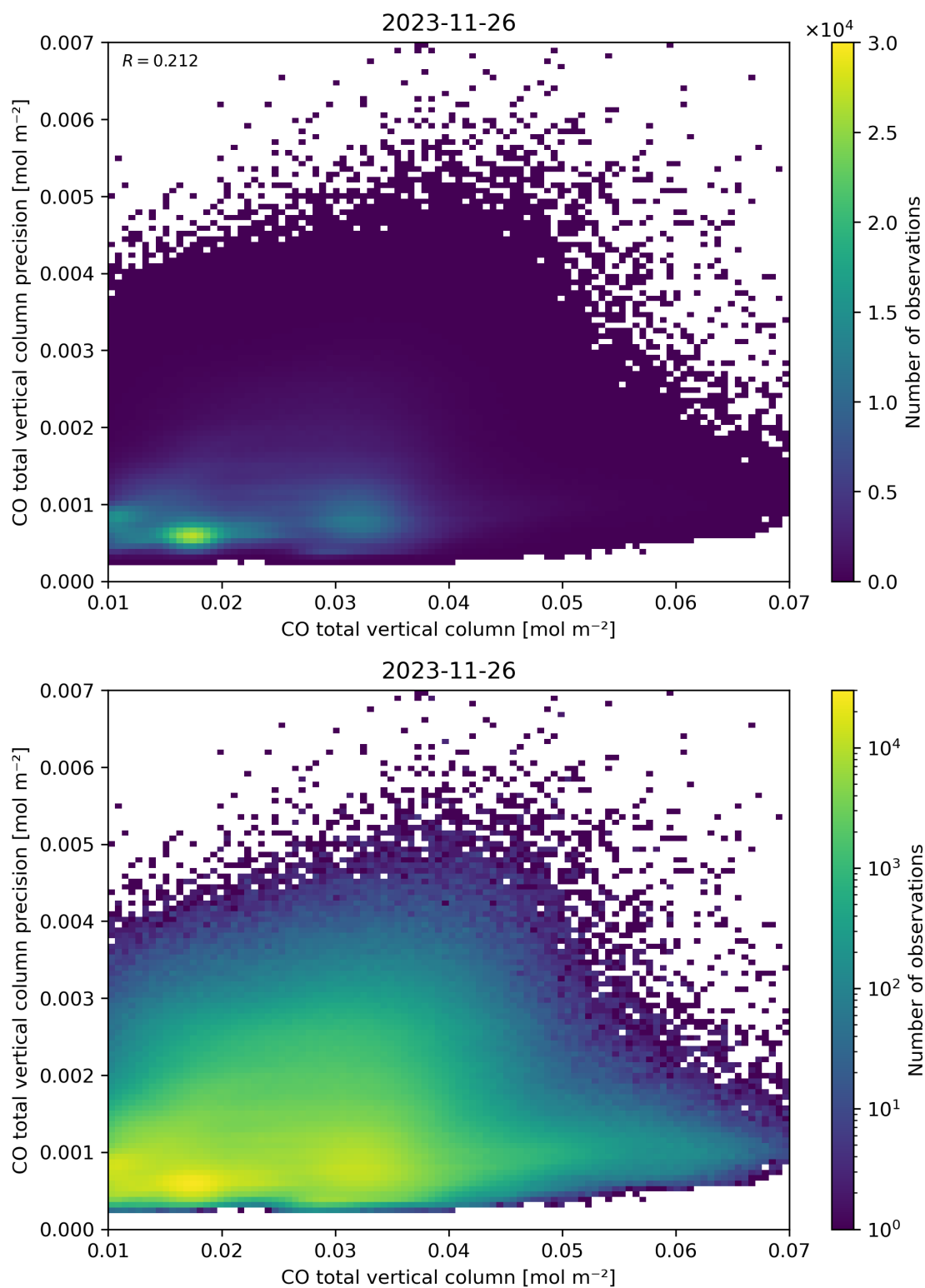
Figure 34: Scatter density plot of “CO total vertical column” against “CO total vertical column precision” for 2023-11-25 to 2023-11-27.
