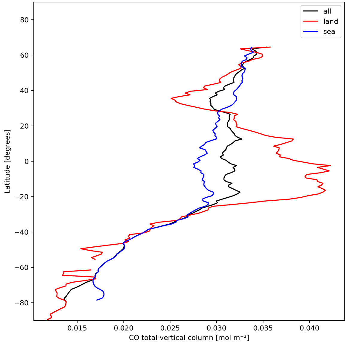
Figure 10: Zonal average of “CO total vertical column” for 2023-11-25 to 2023-11-27.
