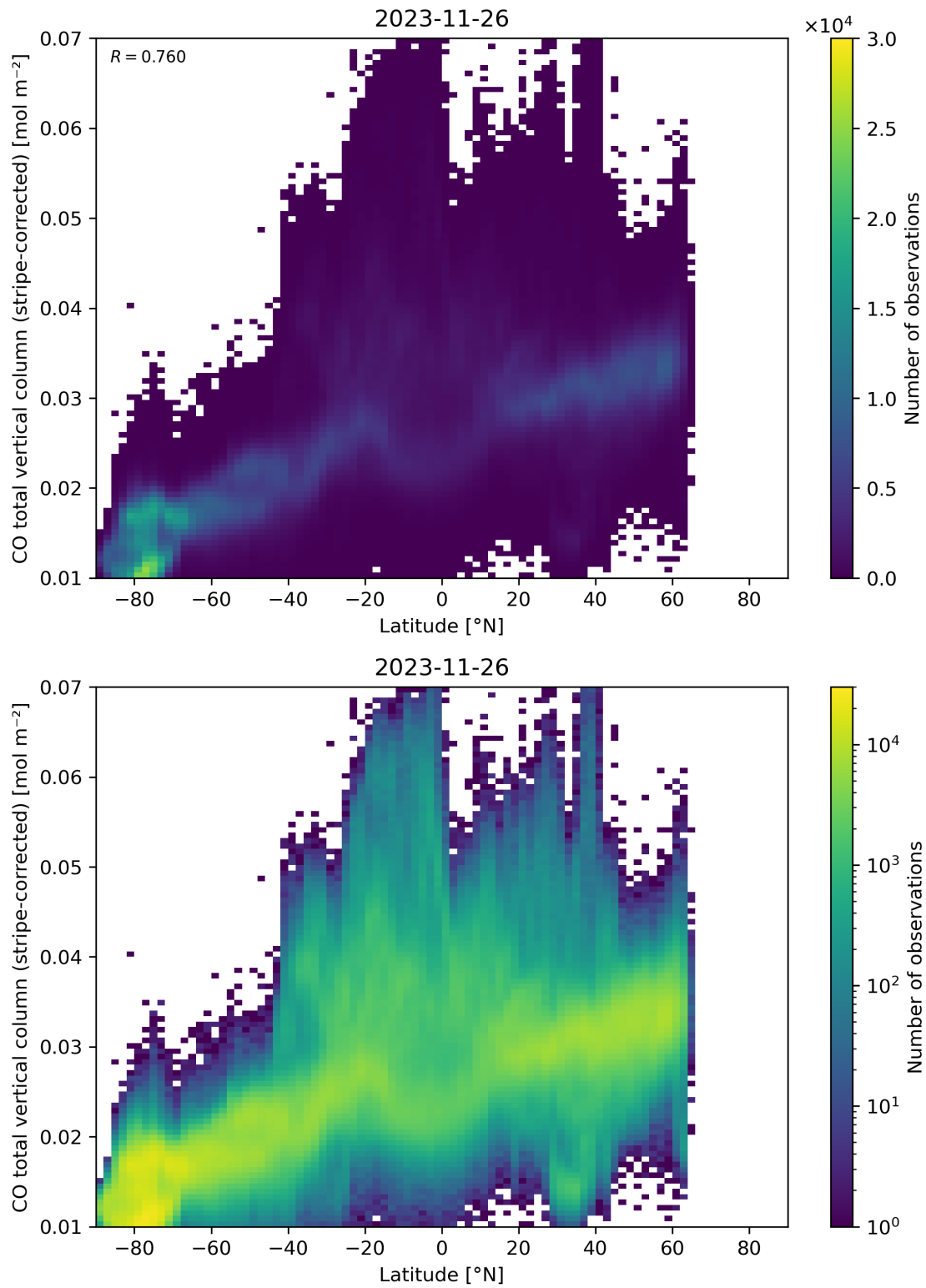
Figure 52: Scatter density plot of “Latitude” against “CO total vertical column (stripe-corrected)” for 2023-11-25 to 2023-11-27.
