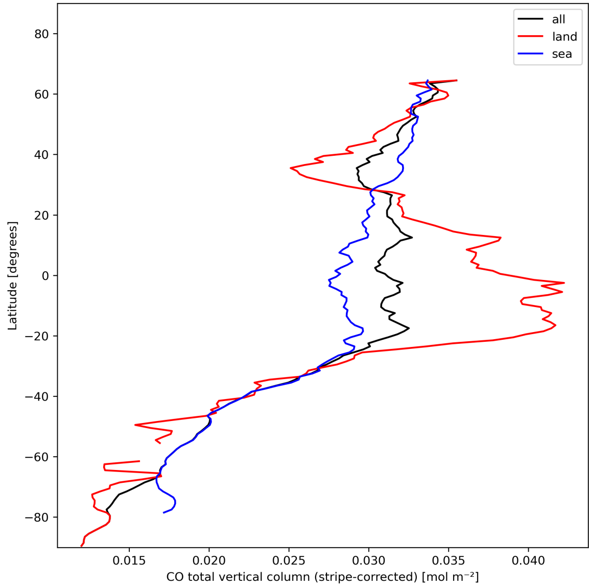
Figure 11: Zonal average of “CO total vertical column (stripe-corrected)” for 2023-11-25 to 2023-11-27.
