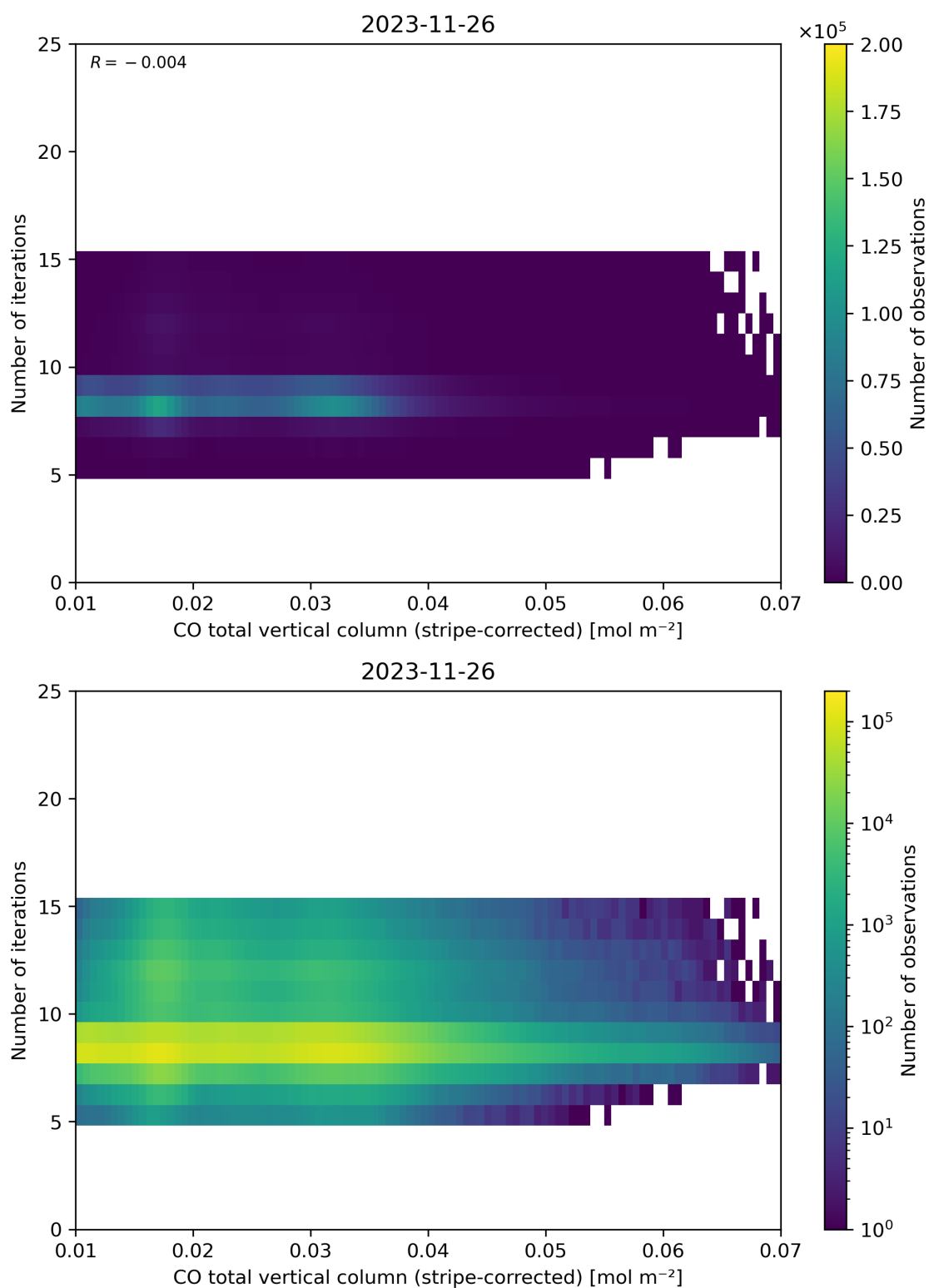
Figure 39: Scatter density plot of “CO total vertical column (stripe-corrected)” against “Number of iterations” for 2023-11-25 to 2023-11-27.
