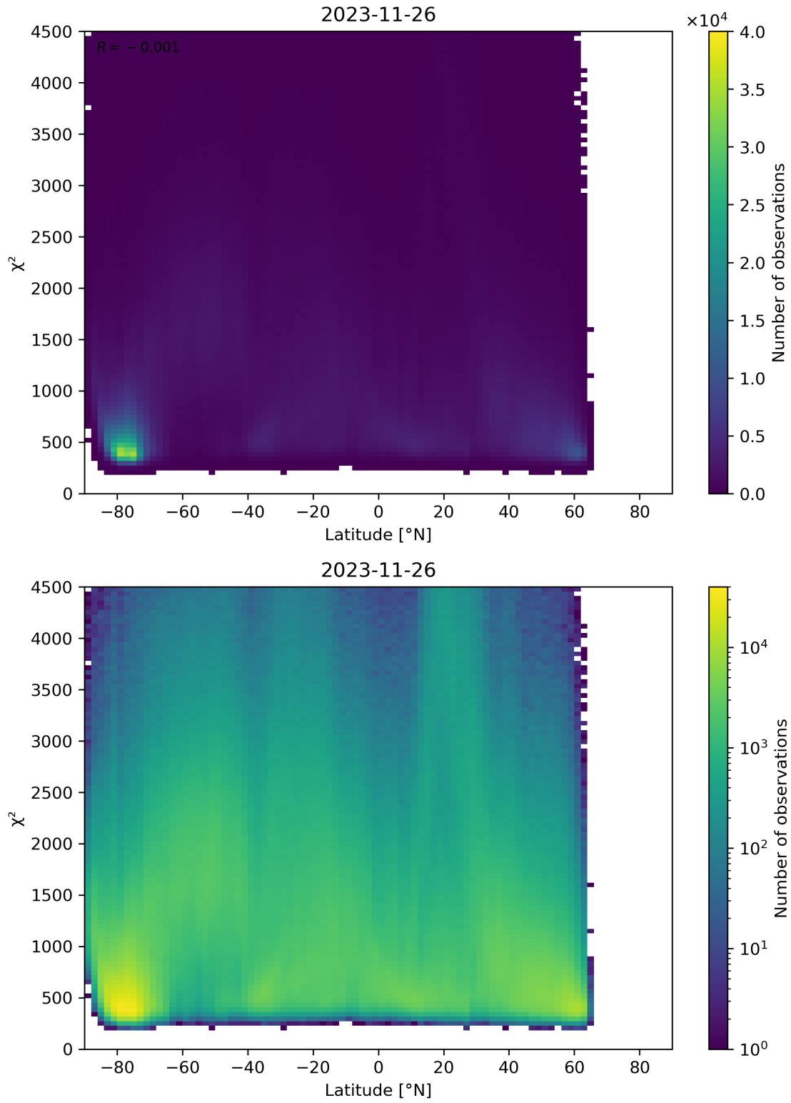
Figure 54: Scatter density plot of “Latitude” against “ \chi^2 ” for 2023-11-25 to 2023-11-27.
