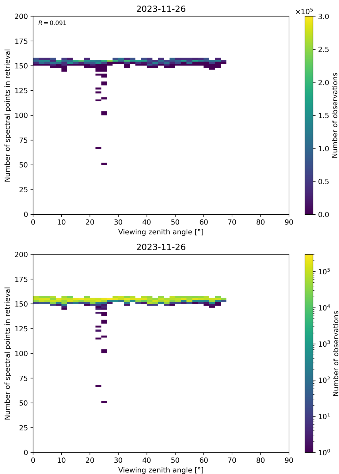
Figure 76: Scatter density plot of “Viewing zenith angle” against “Number of spectral points in retrieval” for 2023-11-25 to 2023-11-27.
