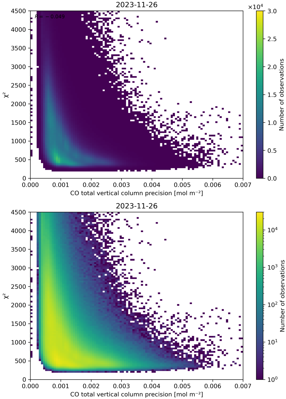
Figure 44: Scatter density plot of “CO total vertical column precision” against “ \chi^2 ” for 2023-11-25 to 2023-11-27.
