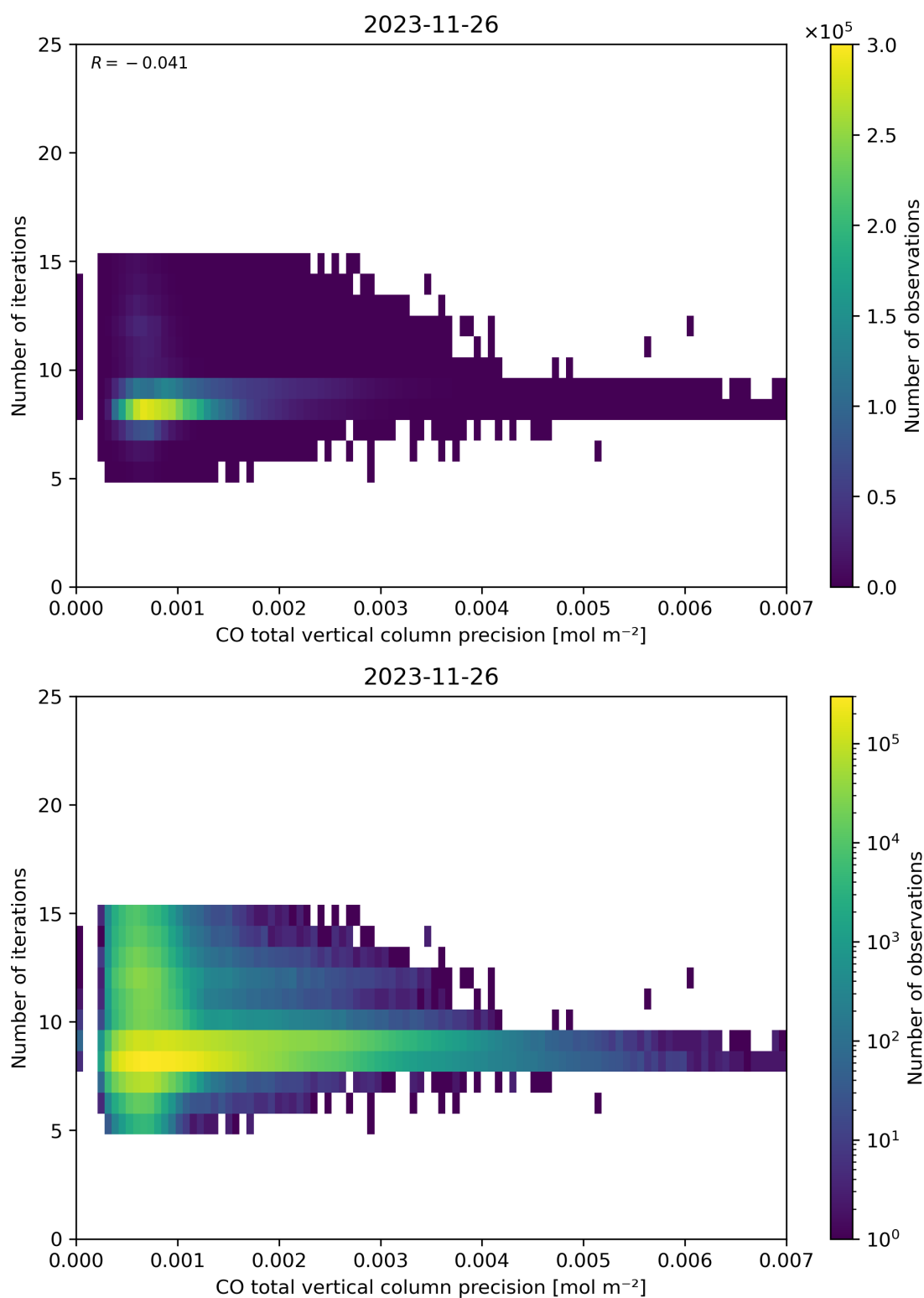
Figure 46: Scatter density plot of “CO total vertical column precision” against “Number of iterations” for 2023-11-25 to 2023-11-27.
