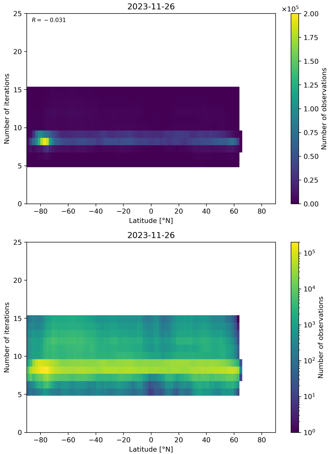
Figure 56: Scatter density plot of “Latitude” against “Number of iterations” for 2023-11-25 to 2023-11-27.
