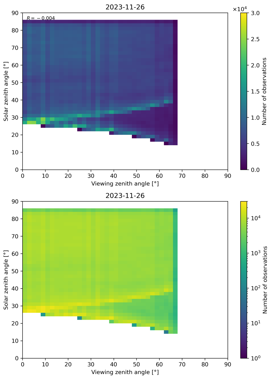
Figure 77: Scatter density plot of “Viewing zenith angle” against “Solar zenith angle” for 2023-11-25 to 2023-11-27.
