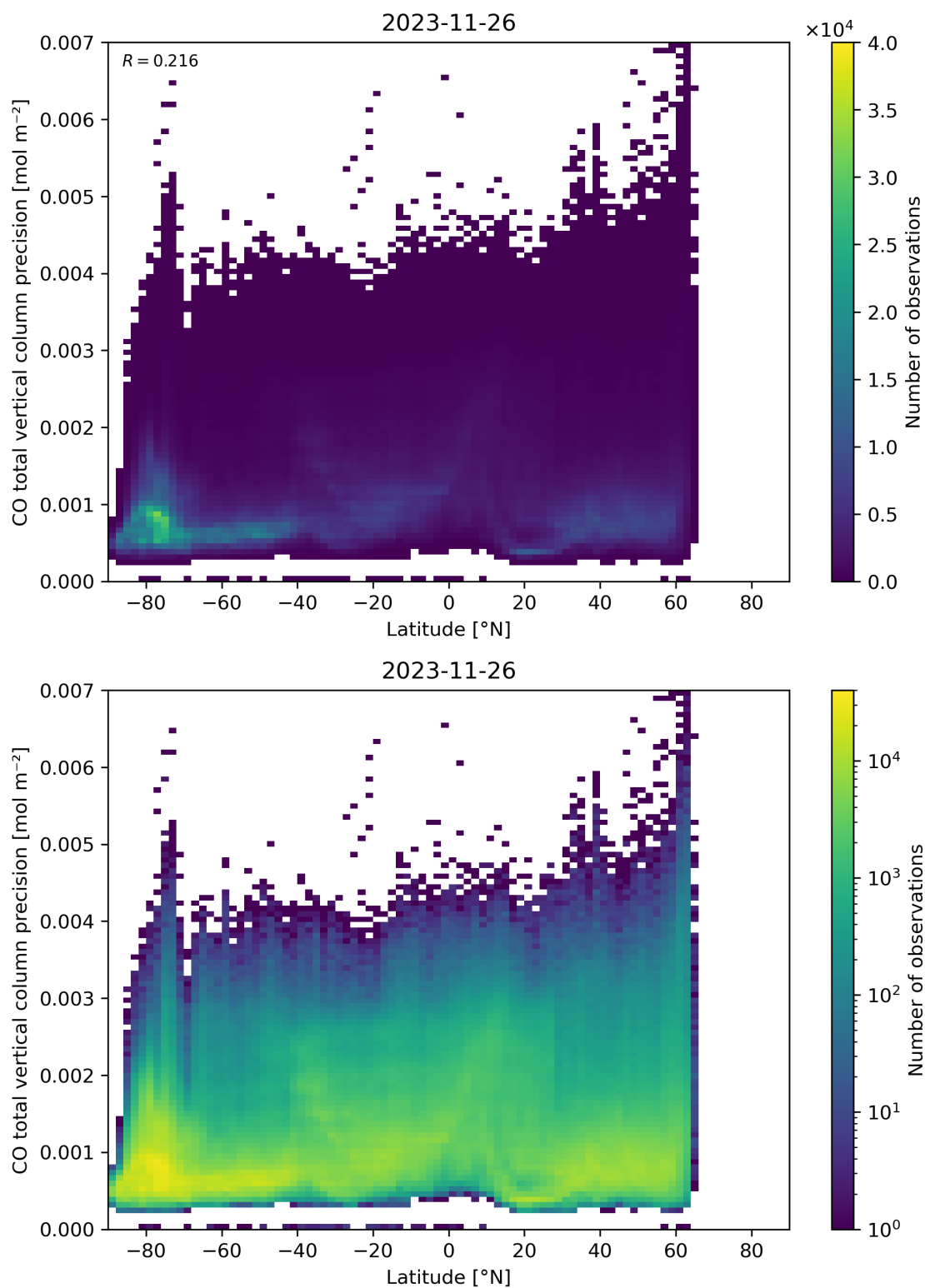
Figure 53: Scatter density plot of “Latitude” against “CO total vertical column precision” for 2023-11-25 to 2023-11-27.
