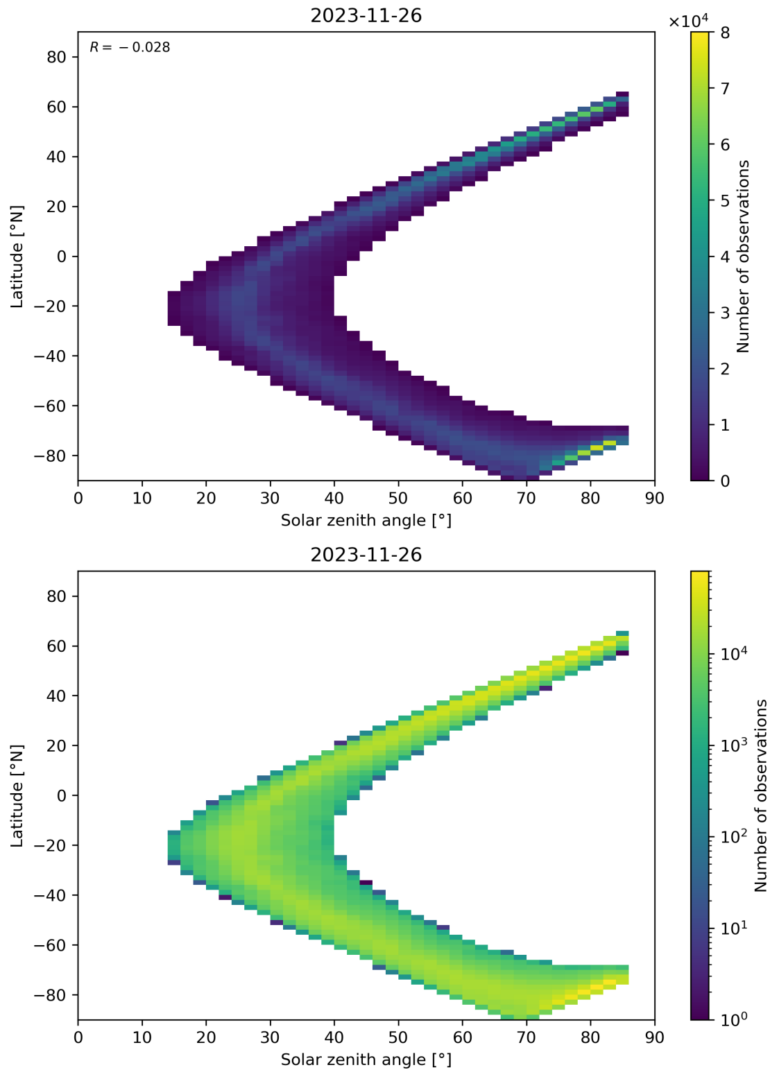
Figure 66: Scatter density plot of “Solar zenith angle” against “Latitude” for 2023-11-25 to 2023-11-27.
