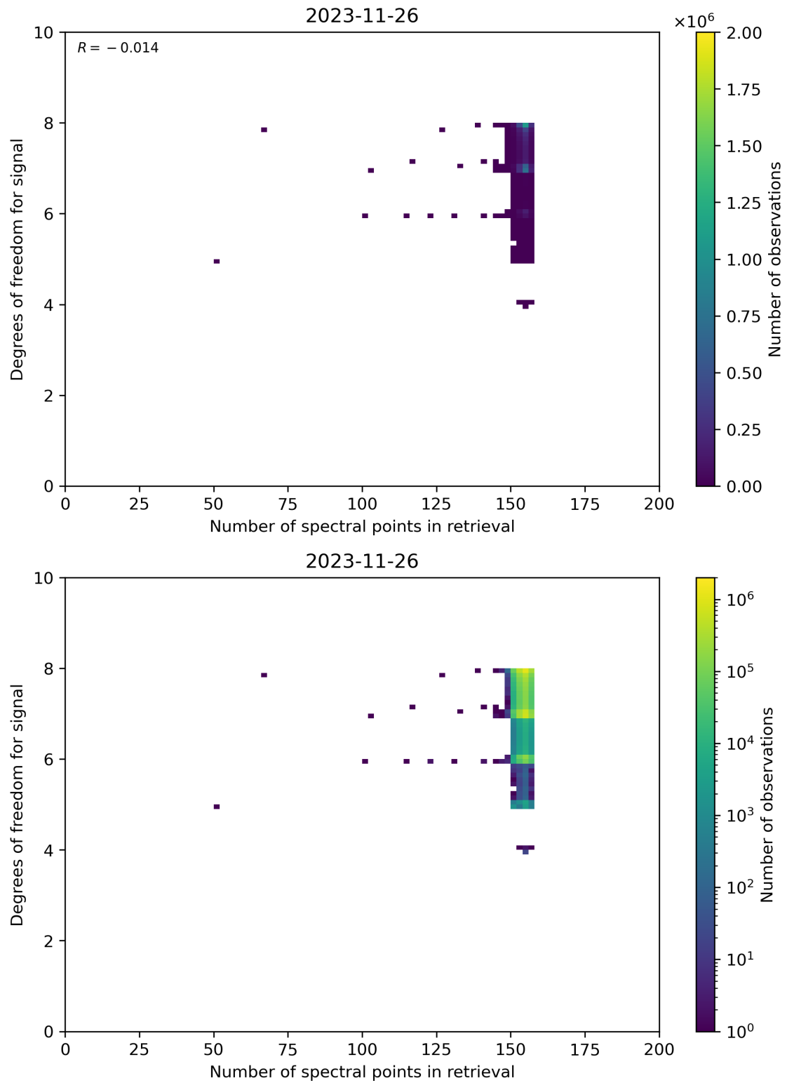
Figure 59: Scatter density plot of “Number of spectral points in retrieval” against “Degrees of freedom for signal” for 2023-11-25 to 2023-11-27.
