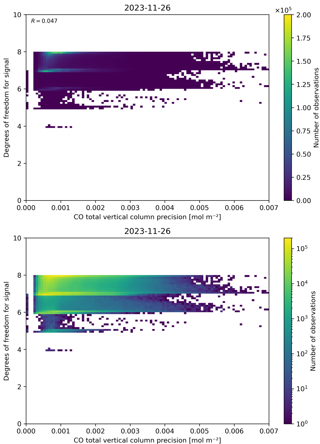
Figure 45: Scatter density plot of “CO total vertical column precision” against “Degrees of freedom for signal” for 2023-11-25 to 2023-11-27.
