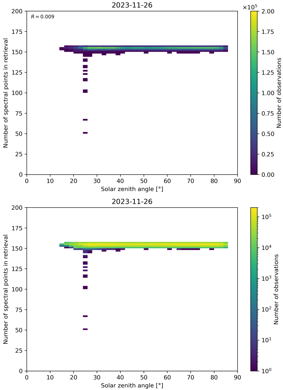
Figure 68: Scatter density plot of “Solar zenith angle” against “Number of spectral points in retrieval” for 2023-11-25 to 2023-11-27.
