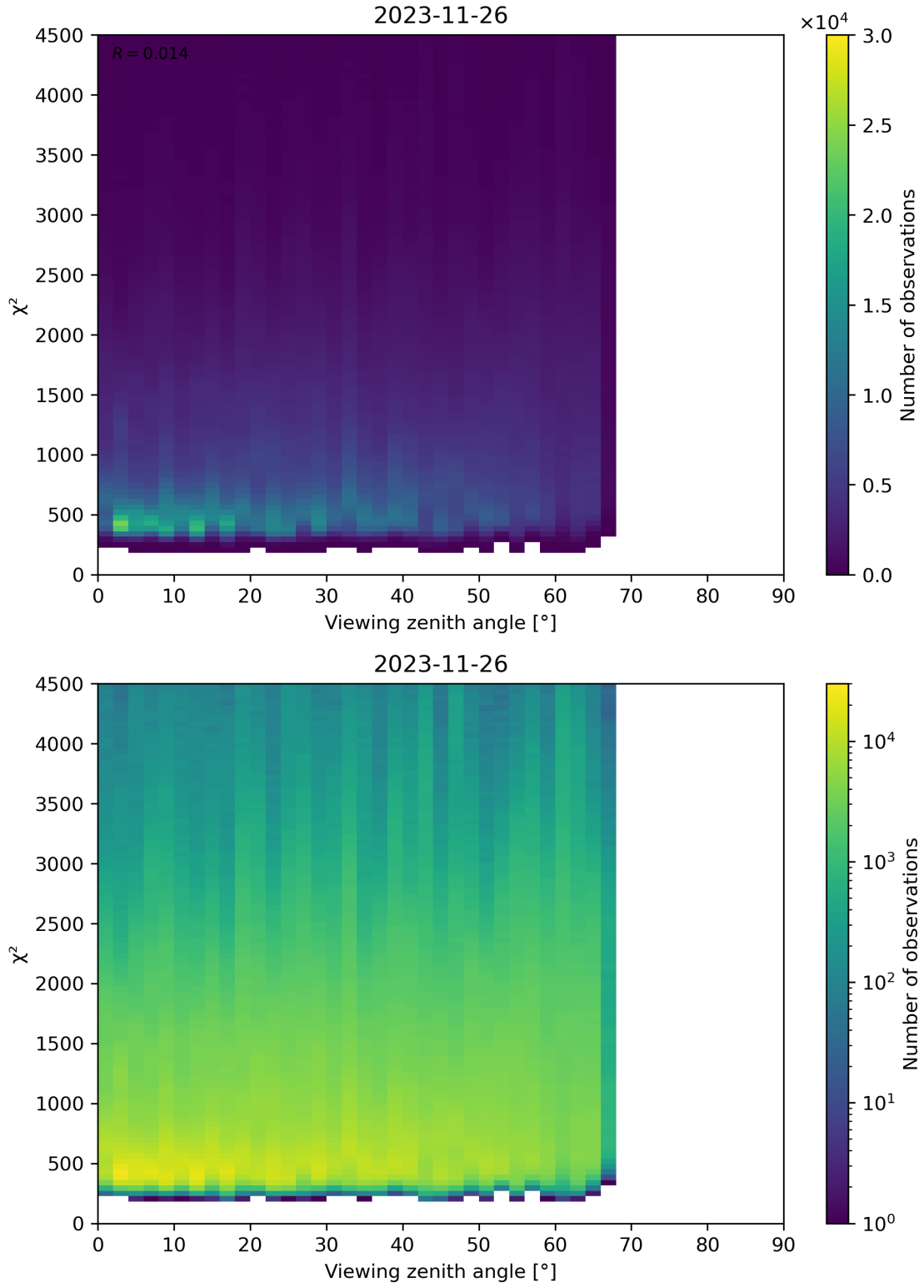
Figure 72: Scatter density plot of “Viewing zenith angle” against “ \chi^2 ” for 2023-11-25 to 2023-11-27.
