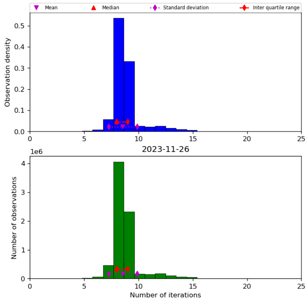
Figure 24: Histogram of “Number of iterations” for 2023-11-25 to 2023-11-27
