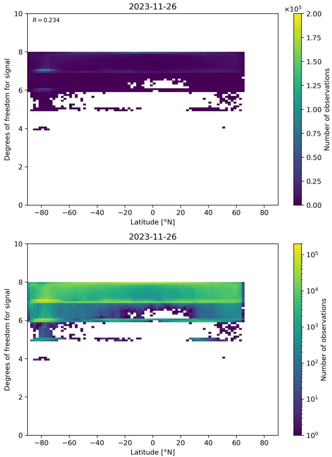
Figure 55: Scatter density plot of “Latitude” against “Degrees of freedom for signal” for 2023-11-25 to 2023-11-27.
