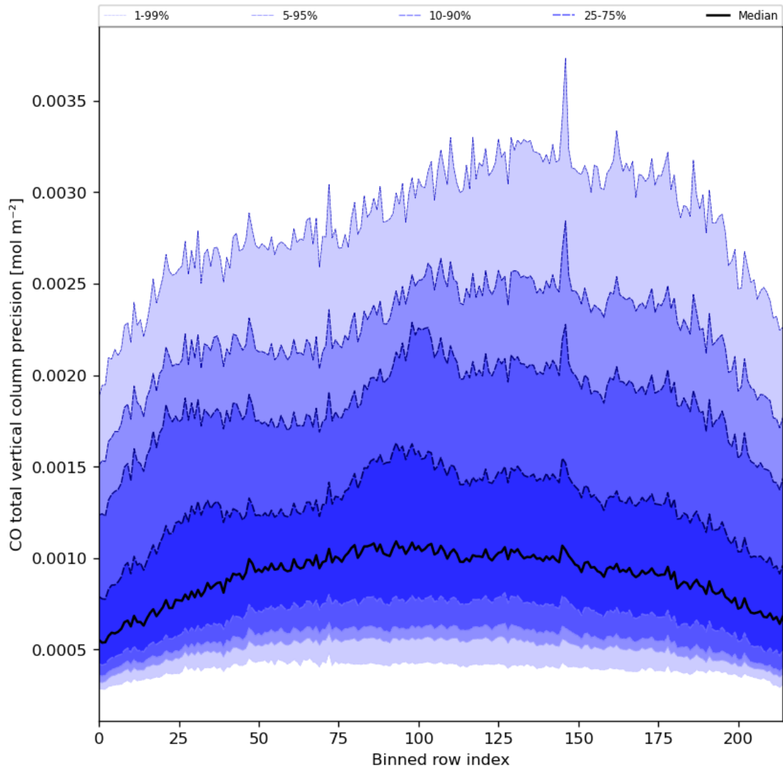
Figure 28: Along track statistics of “CO total vertical column precision” for 2023-11-25 to 2023-11-27
