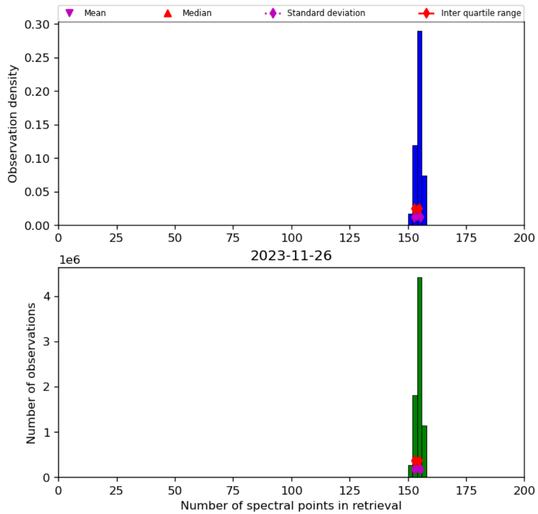
Figure 21: Histogram of “Number of spectral points in retrieval” for 2023-11-25 to 2023-11-27
