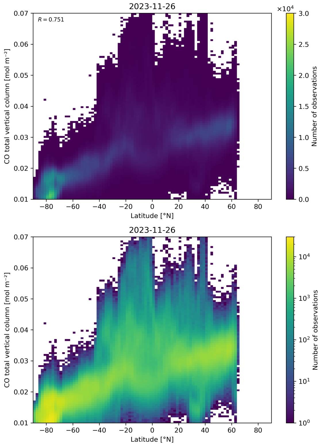
Figure 51: Scatter density plot of “Latitude” against “CO total vertical column” for 2023-11-25 to 2023-11-27.
