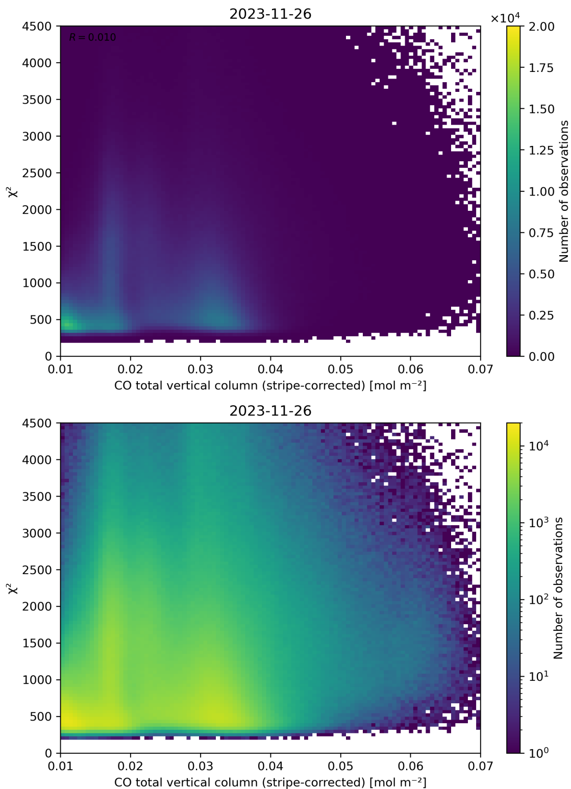
Figure 37: Scatter density plot of “CO total vertical column (stripe-corrected)” against “ \chi^2 ” for 2023-11-25 to 2023-11-27.
