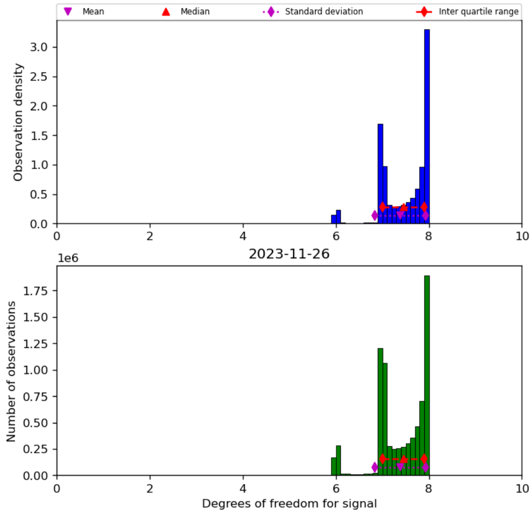
Figure 23: Histogram of “Degrees of freedom for signal” for 2023-11-25 to 2023-11-27
