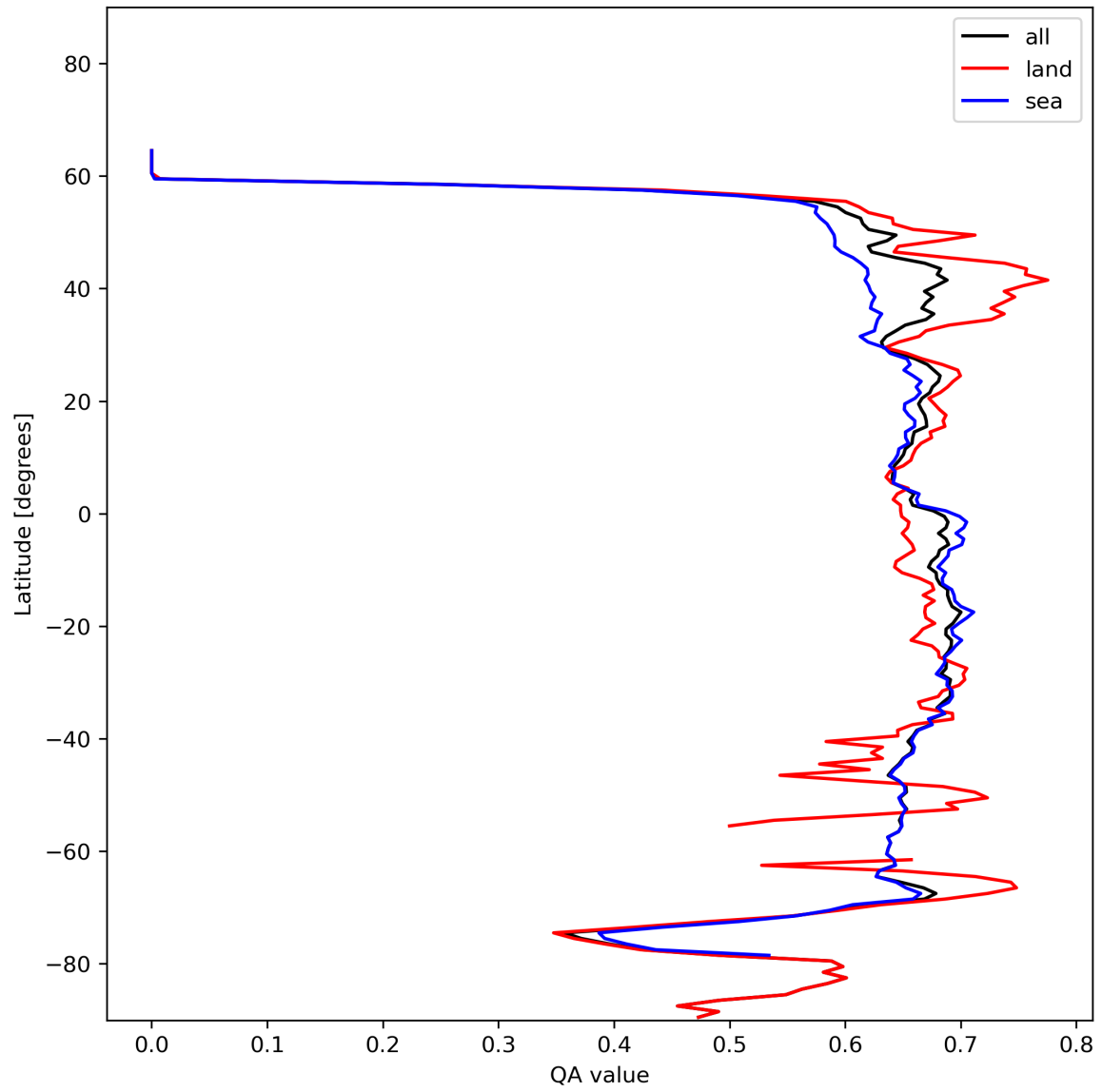
Figure 9: Zonal average of “QA value” for 2023-11-25 to 2023-11-27.
