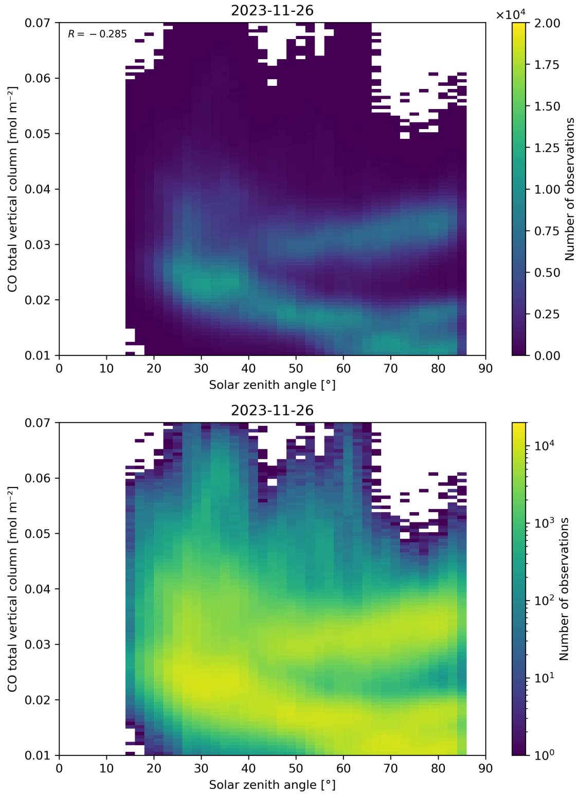
Figure 61: Scatter density plot of “Solar zenith angle” against “CO total vertical column” for 2023-11-25 to 2023-11-27.
