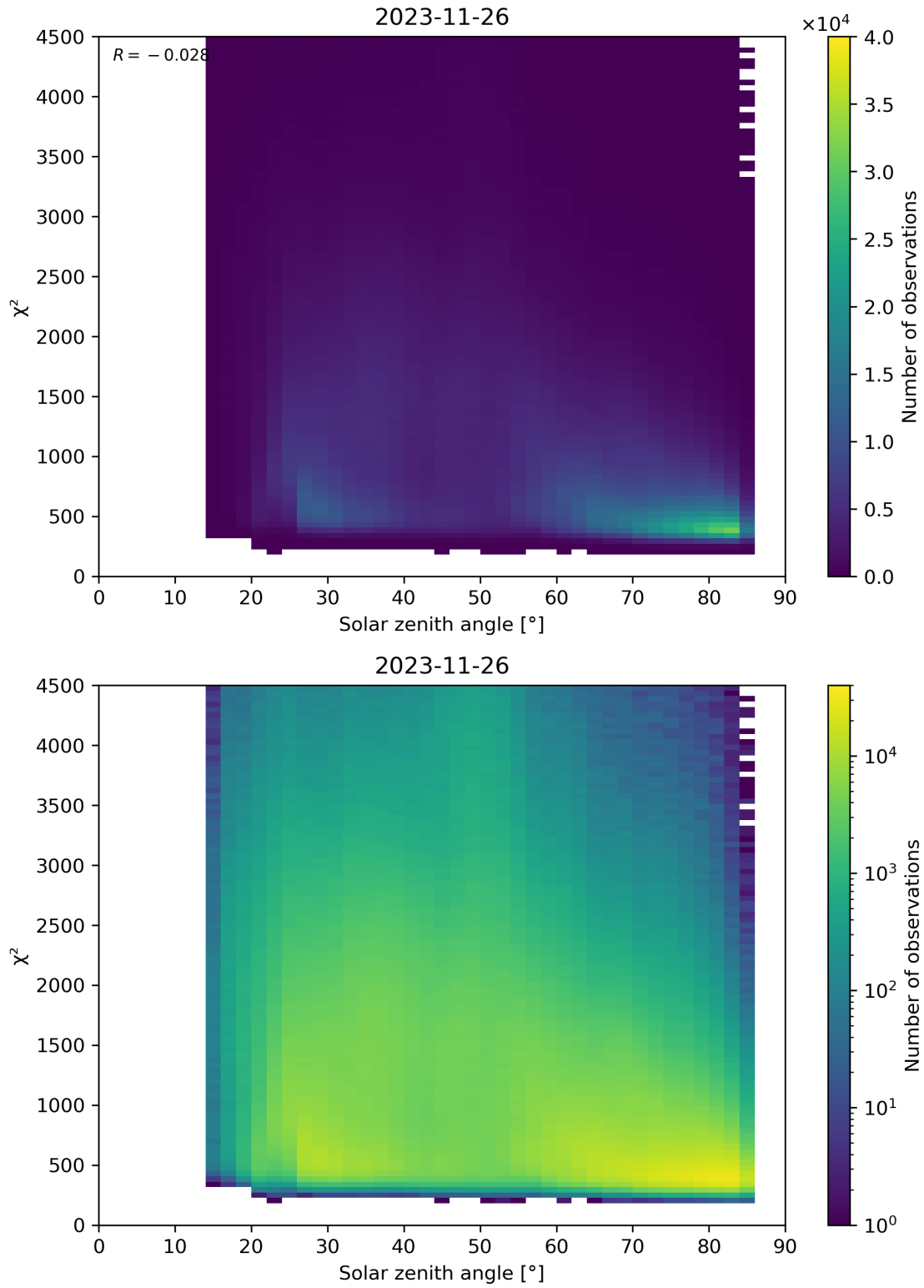
Figure 64: Scatter density plot of “Solar zenith angle” against “ \chi^2 ” for 2023-11-25 to 2023-11-27.
