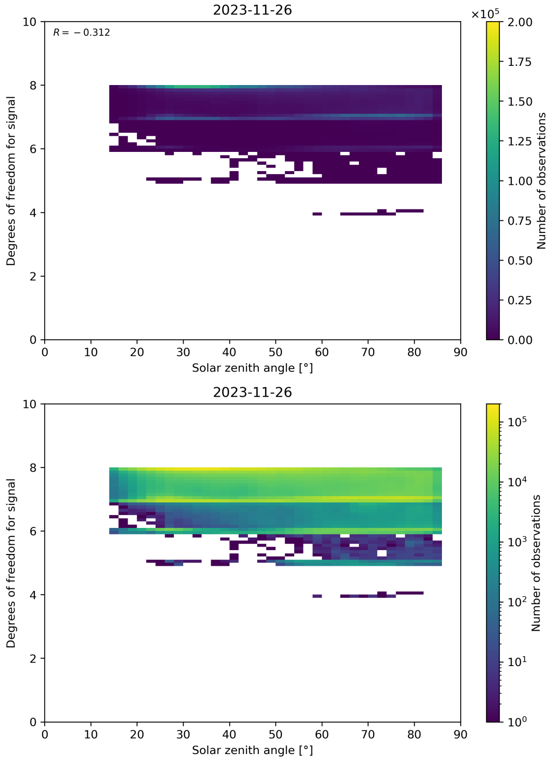
Figure 65: Scatter density plot of “Solar zenith angle” against “Degrees of freedom for signal” for 2023-11-25 to 2023-11-27.
