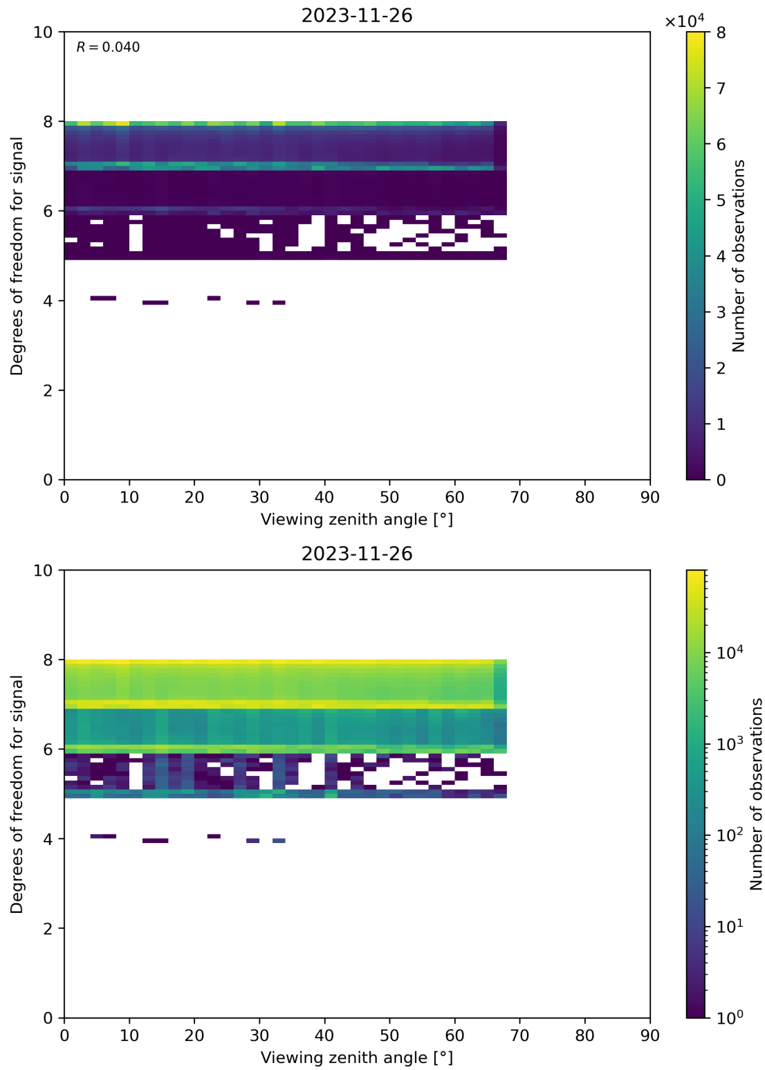
Figure 73: Scatter density plot of “Viewing zenith angle” against “Degrees of freedom for signal” for 2023-11-25 to 2023-11-27.
