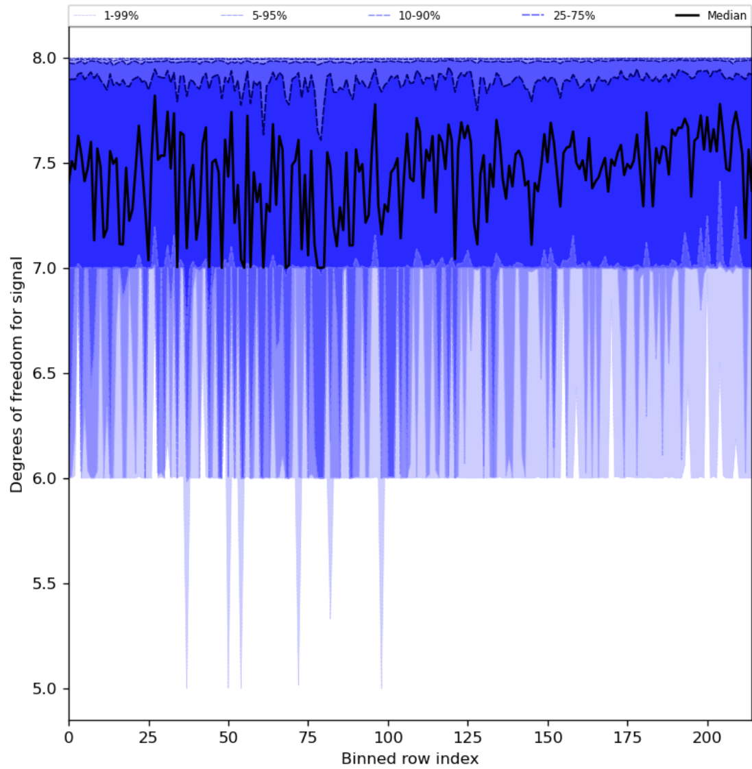
Figure 31: Along track statistics of “Degrees of freedom for signal” for 2023-11-25 to 2023-11-27
