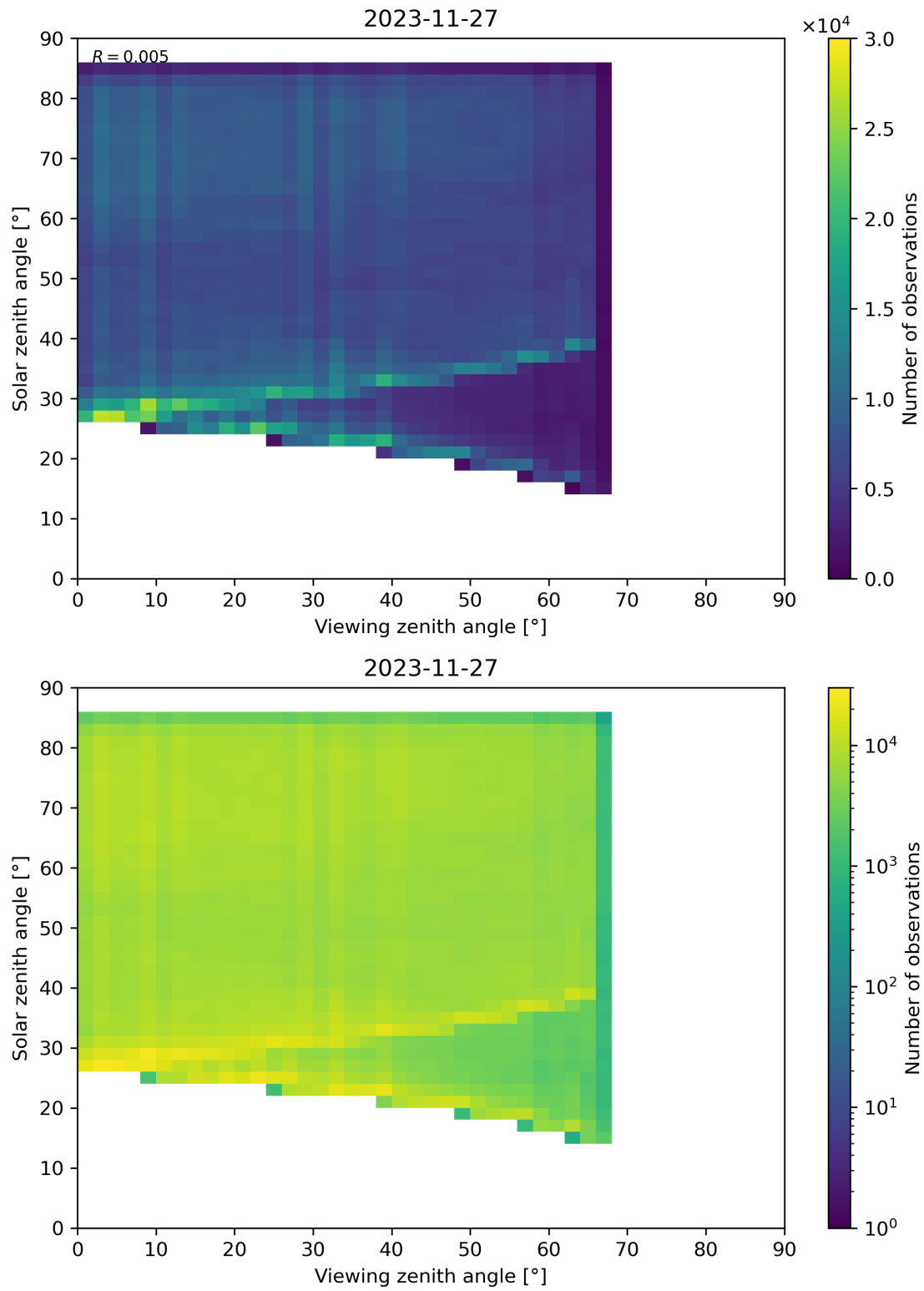
Figure 77: Scatter density plot of “Viewing zenith angle” against “Solar zenith angle” for 2023-11-26 to 2023-11-28.
