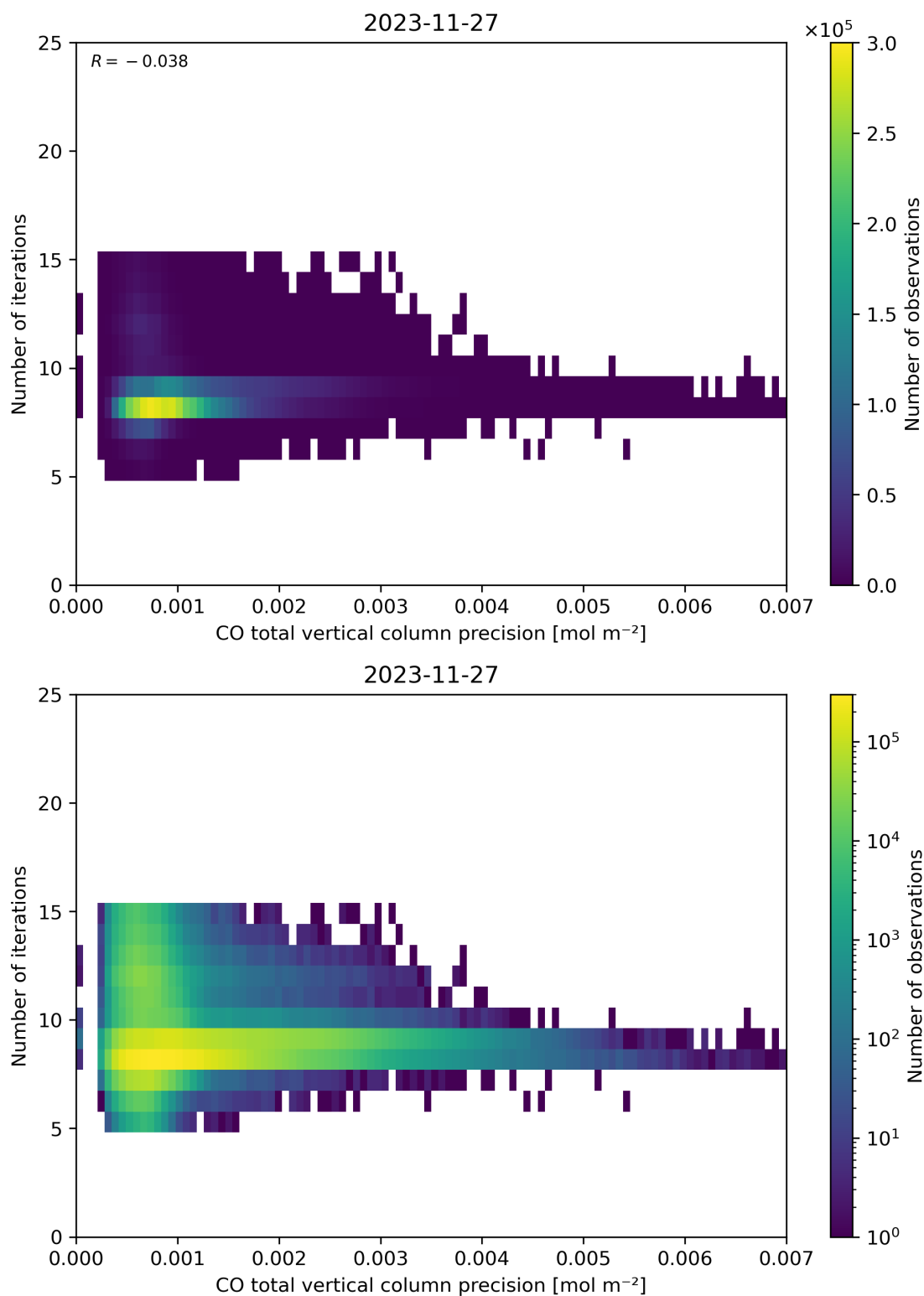
Figure 46: Scatter density plot of “CO total vertical column precision” against “Number of iterations” for 2023-11-26 to 2023-11-28.
