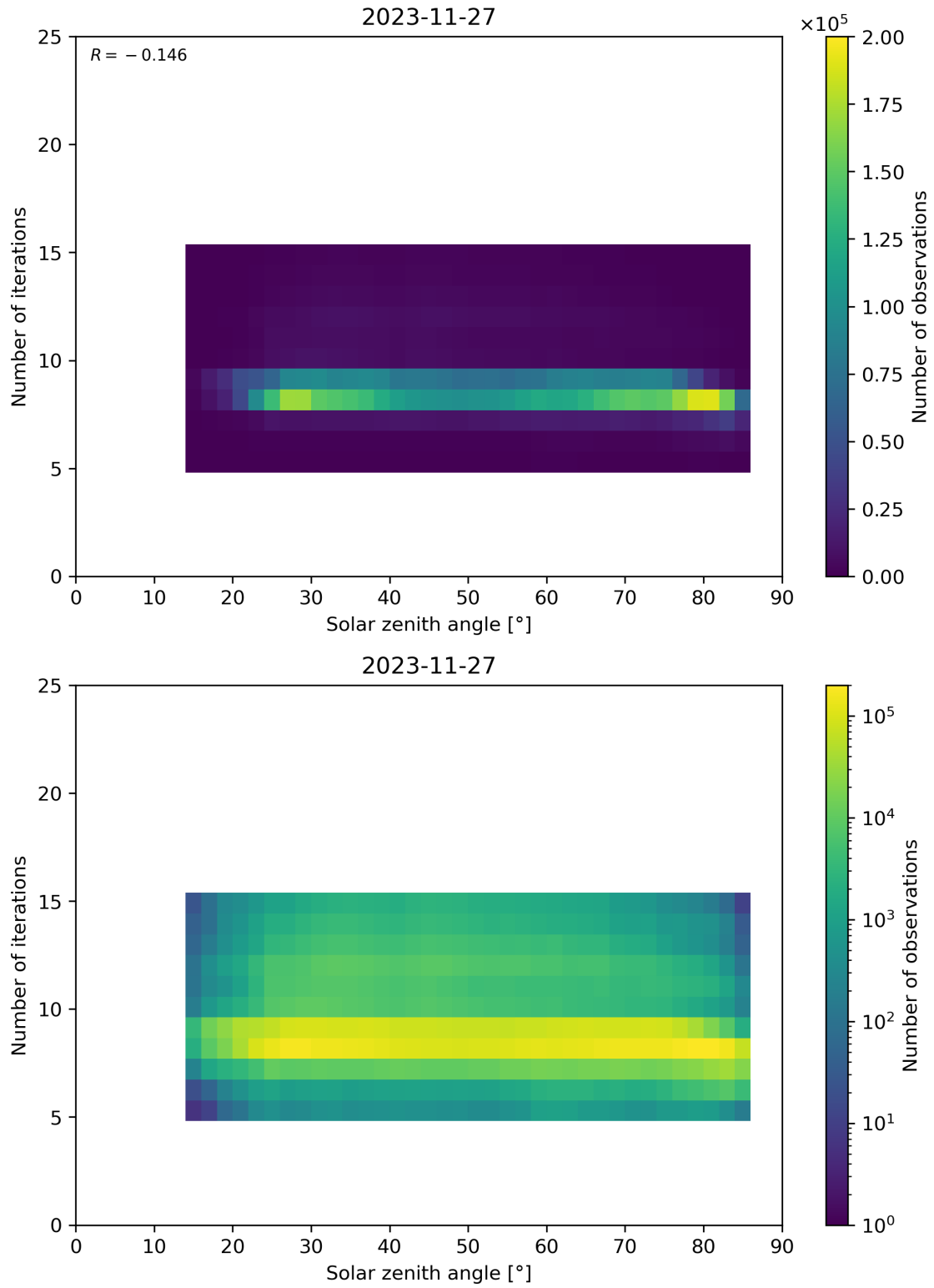
Figure 67: Scatter density plot of “Solar zenith angle” against “Number of iterations” for 2023-11-26 to 2023-11-28.
