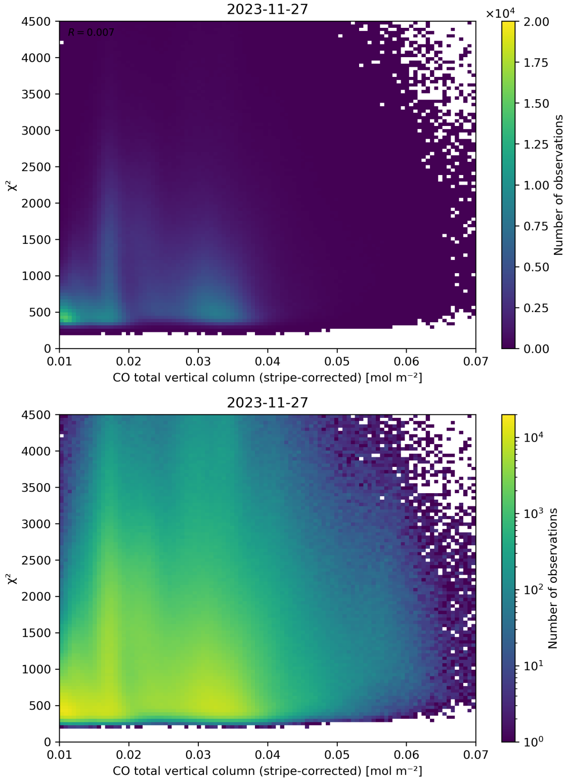
Figure 37: Scatter density plot of “CO total vertical column (stripe-corrected)” against “ \chi^2 ” for 2023-11-26 to 2023-11-28.
