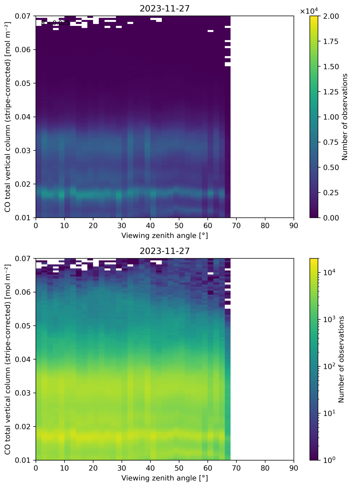
Figure 70: Scatter density plot of “Viewing zenith angle” against “CO total vertical column (stripe-corrected)” for 2023-11-26 to 2023-11-28.
