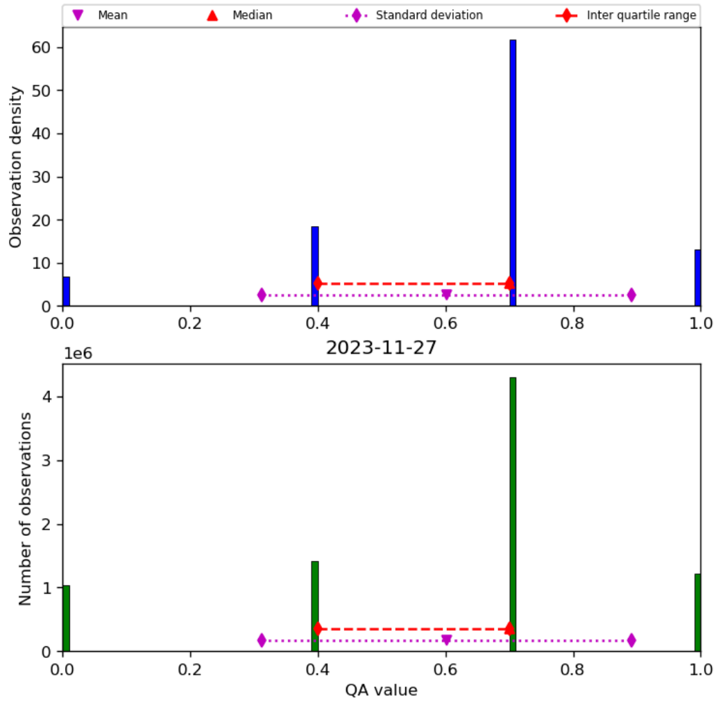
Figure 17: Histogram of “QA value” for 2023-11-26 to 2023-11-28
