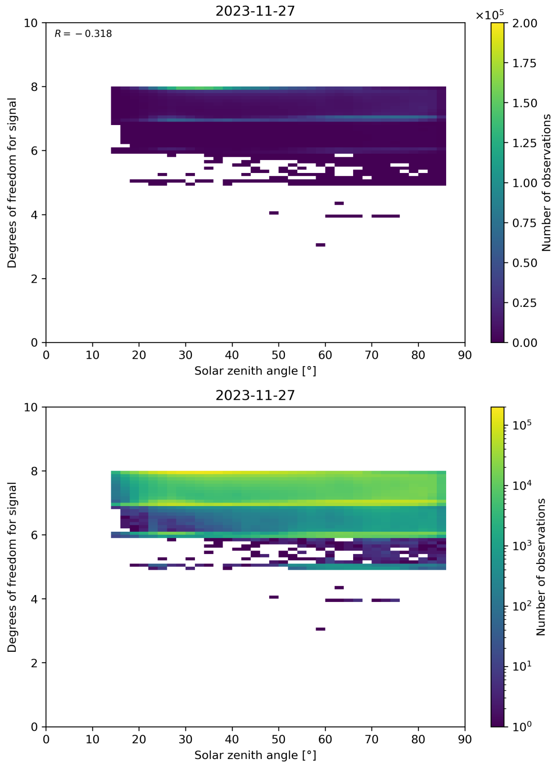
Figure 65: Scatter density plot of “Solar zenith angle” against “Degrees of freedom for signal” for 2023-11-26 to 2023-11-28.
