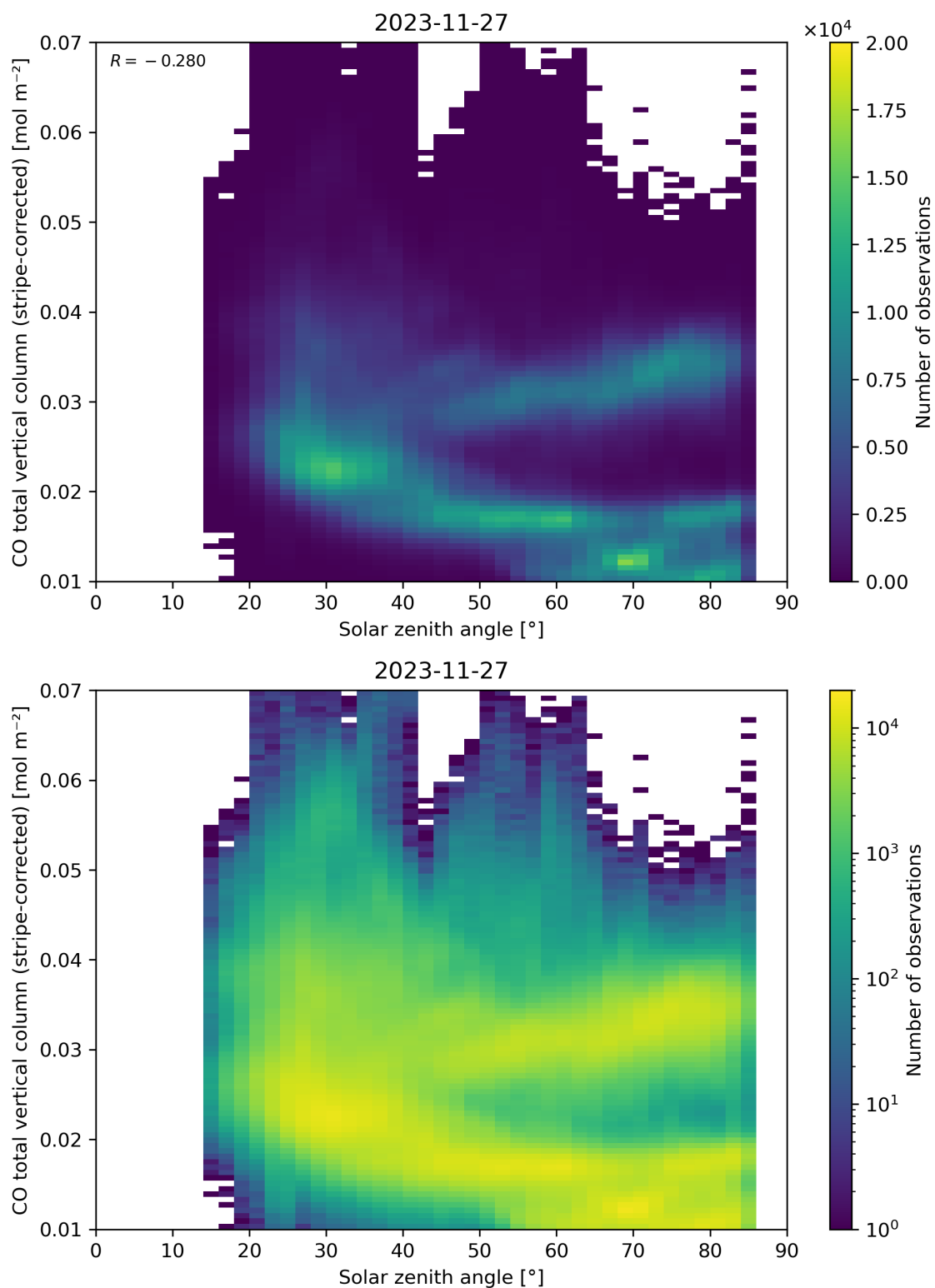
Figure 62: Scatter density plot of “Solar zenith angle” against “CO total vertical column (stripe-corrected)” for 2023-11-26 to 2023-11-28.
