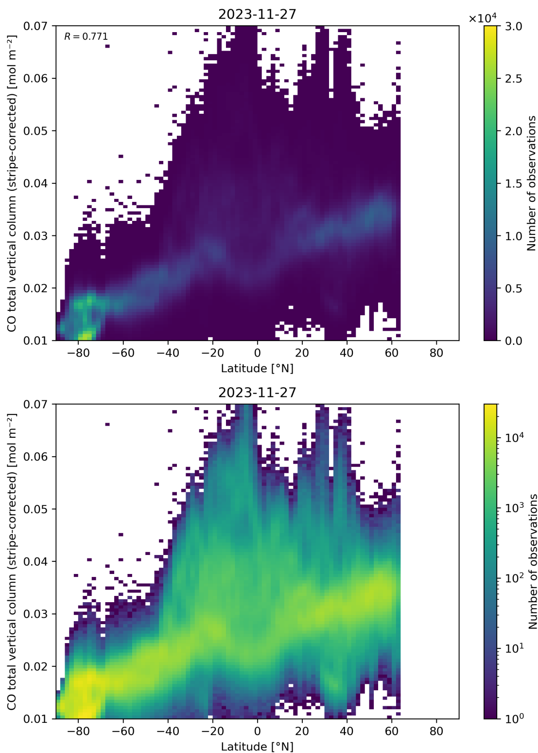
Figure 52: Scatter density plot of “Latitude” against “CO total vertical column (stripe-corrected)” for 2023-11-26 to 2023-11-28.
