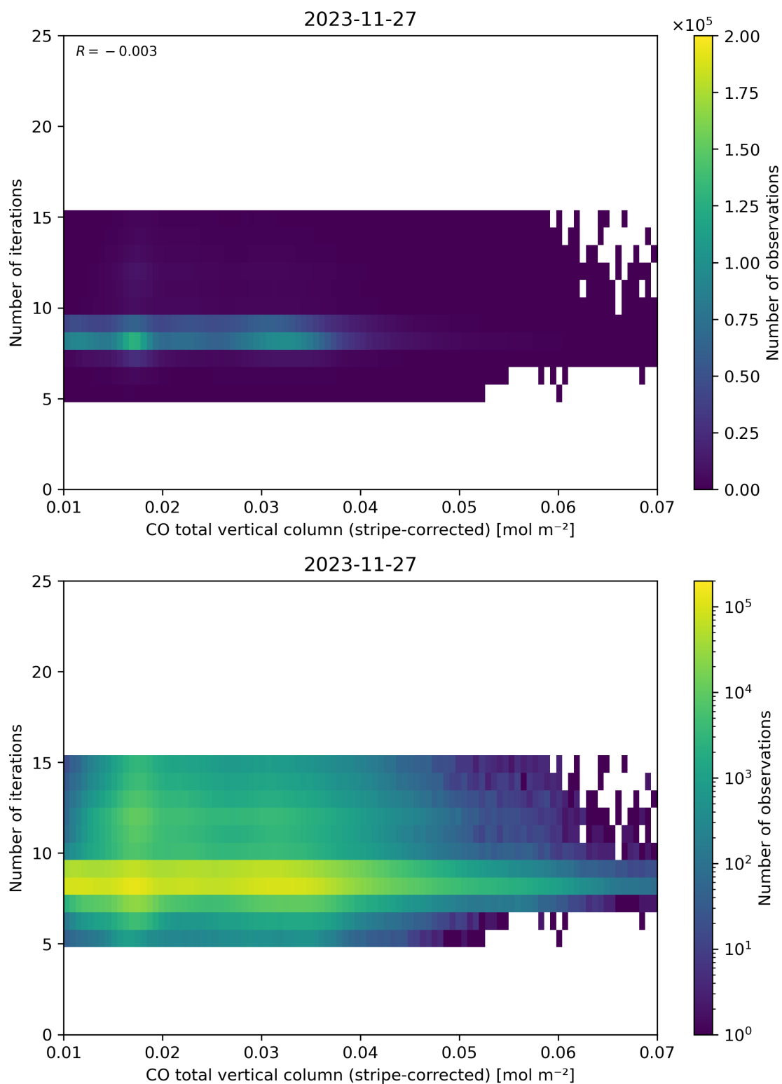
Figure 39: Scatter density plot of “CO total vertical column (stripe-corrected)” against “Number of iterations” for 2023-11-26 to 2023-11-28.
