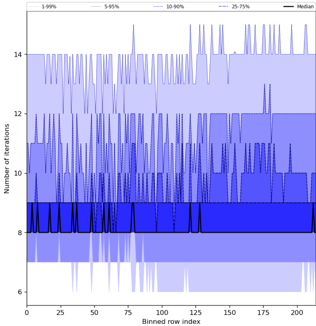
Figure 32: Along track statistics of “Number of iterations” for 2023-11-26 to 2023-11-28
