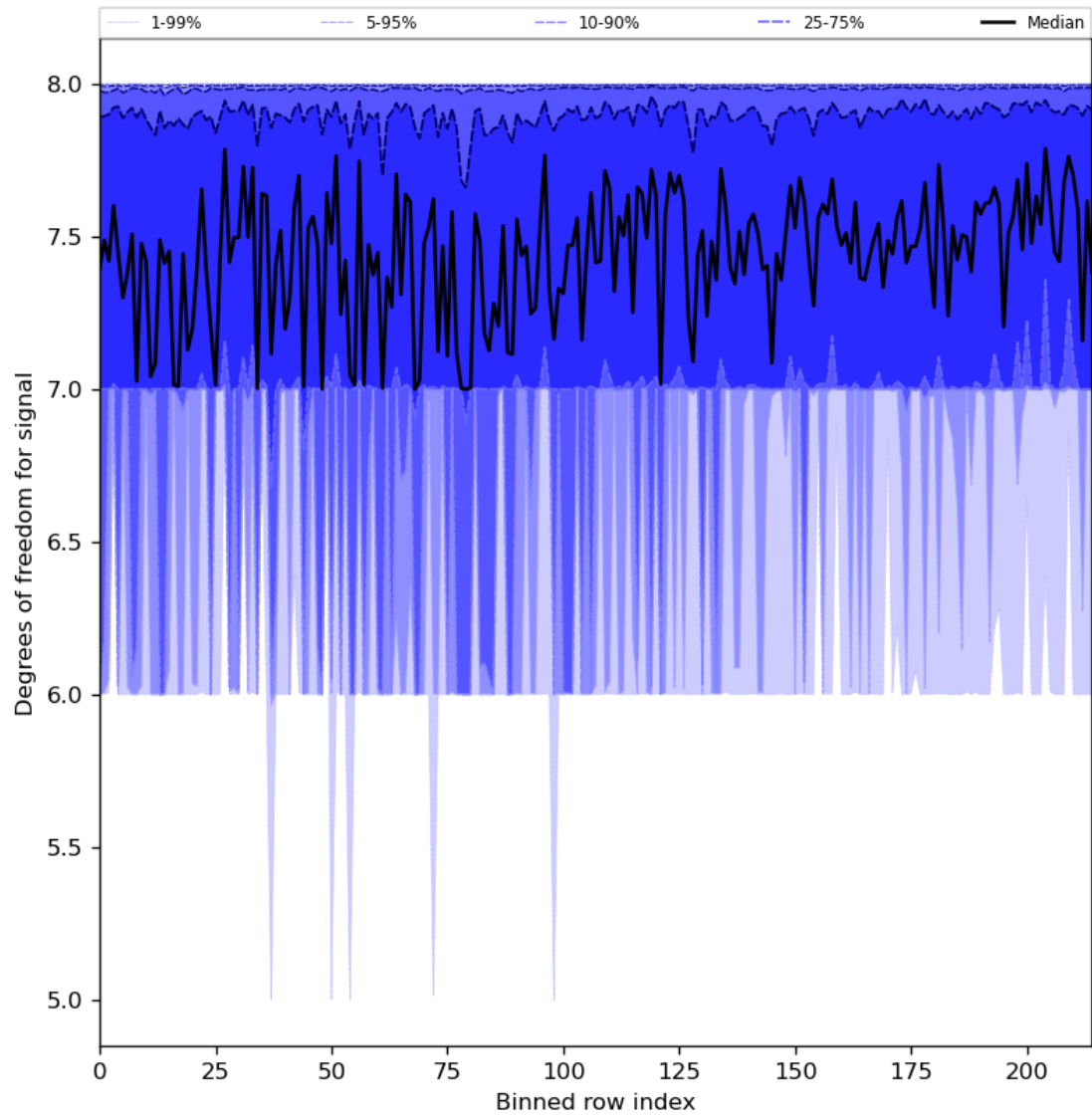
Figure 31: Along track statistics of “Degrees of freedom for signal” for 2023-11-26 to 2023-11-28
