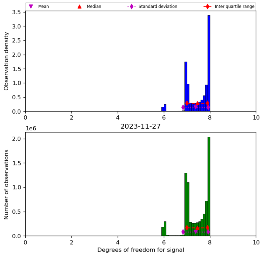
Figure 23: Histogram of “Degrees of freedom for signal” for 2023-11-26 to 2023-11-28
