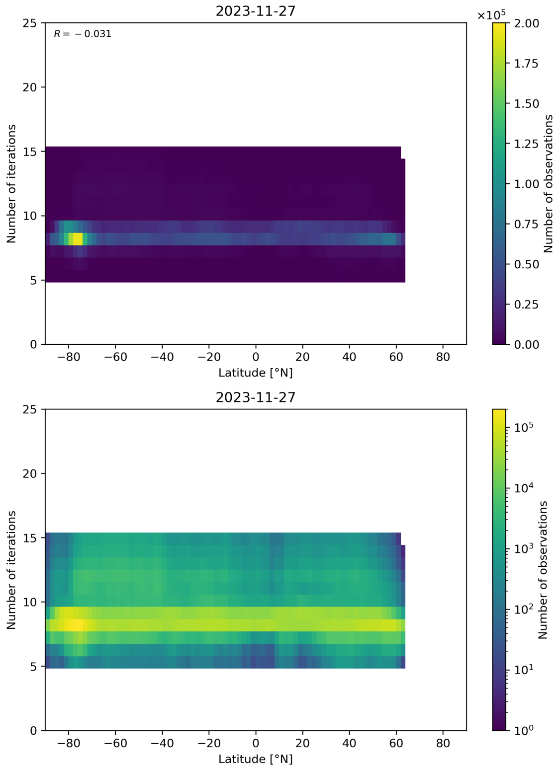
Figure 56: Scatter density plot of “Latitude” against “Number of iterations” for 2023-11-26 to 2023-11-28.
