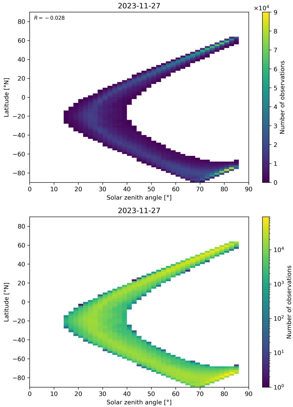
Figure 66: Scatter density plot of “Solar zenith angle” against “Latitude” for 2023-11-26 to 2023-11-28.
