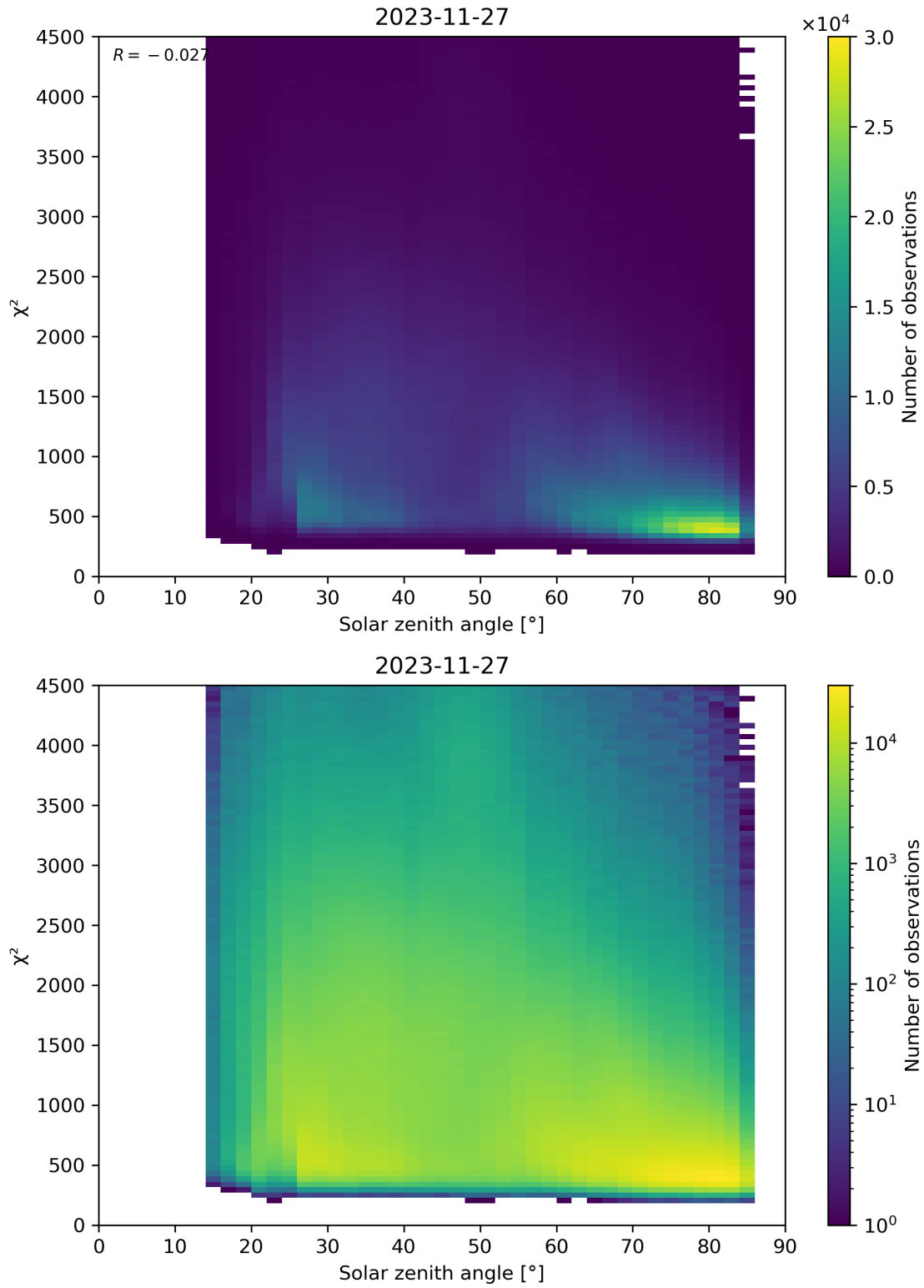
Figure 64: Scatter density plot of “Solar zenith angle” against “ \chi^2 ” for 2023-11-26 to 2023-11-28.
