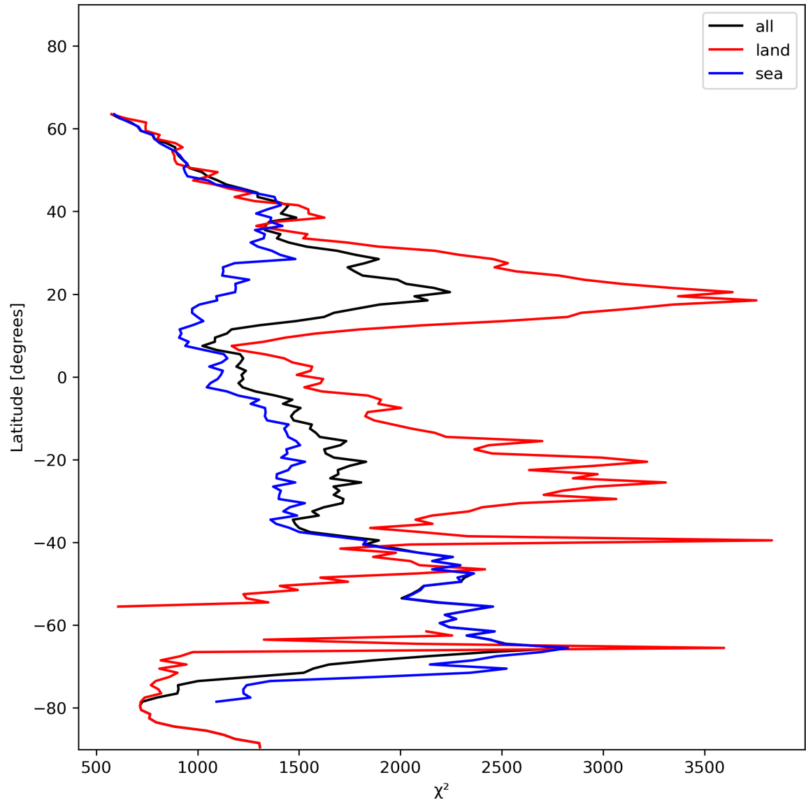
Figure 14: Zonal average of “ \chi^2 ” for 2023-11-26 to 2023-11-28.
