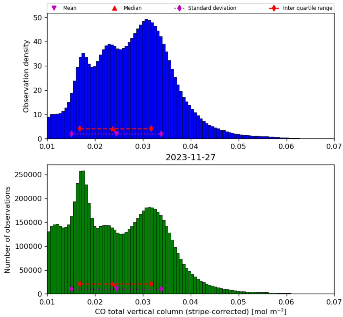
Figure 19: Histogram of “CO total vertical column (stripe-corrected)” for 2023-11-26 to 2023-11-28
