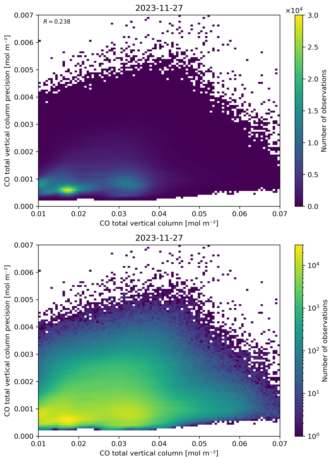
Figure 34: Scatter density plot of “CO total vertical column” against “CO total vertical column precision” for 2023-11-26 to 2023-11-28.
