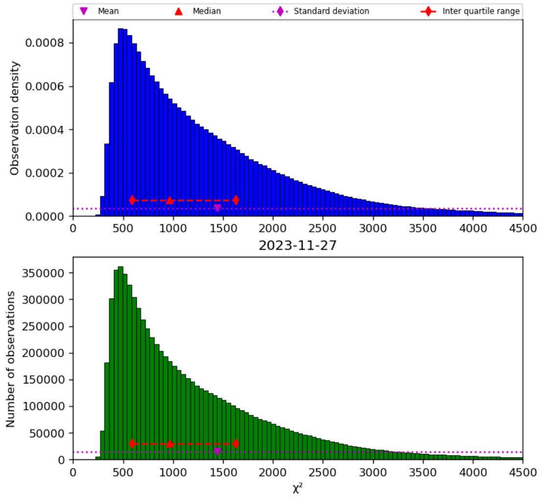
Figure 22: Histogram of “ \chi^2 ” for 2023-11-26 to 2023-11-28
