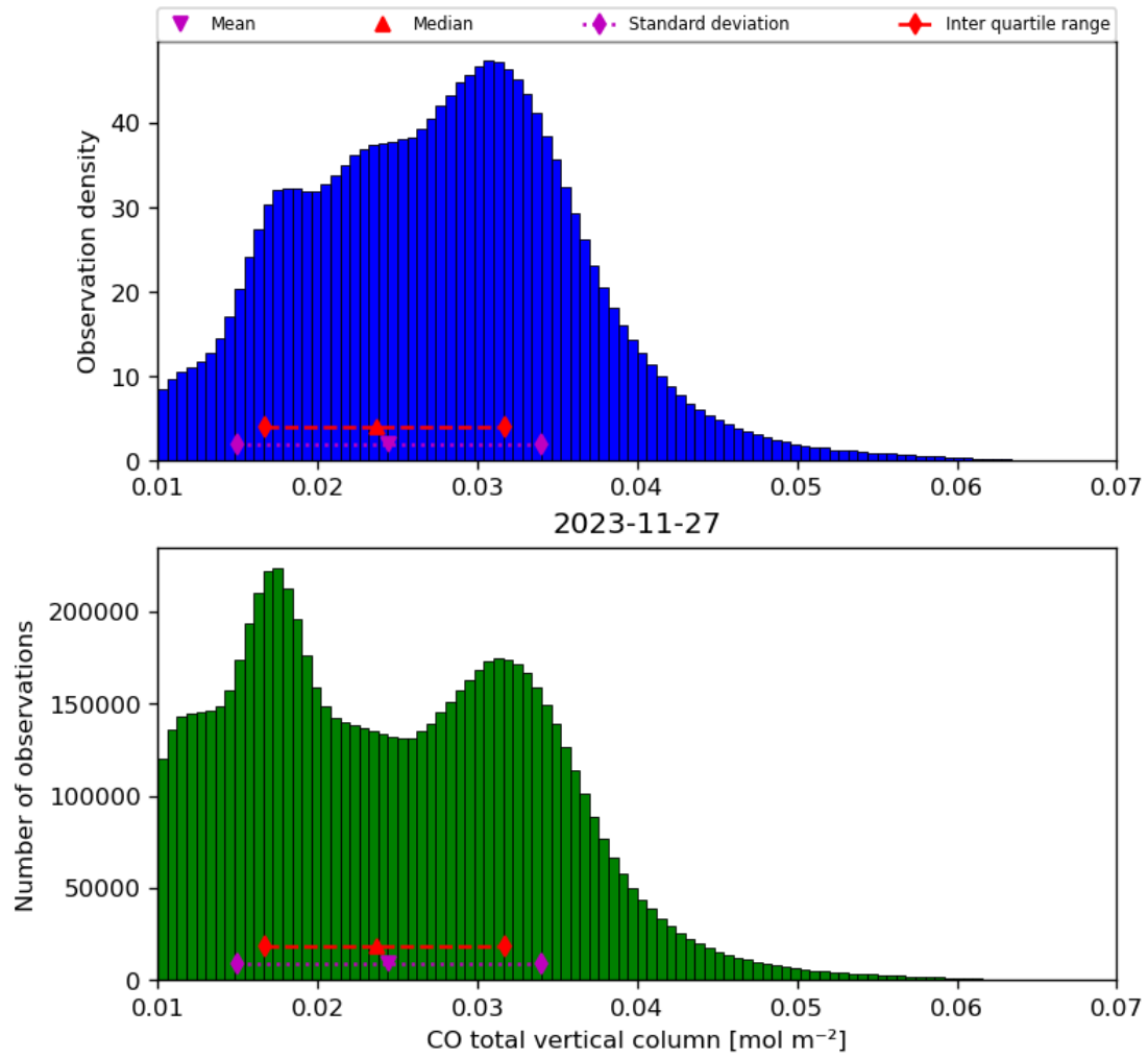
Figure 18: Histogram of “CO total vertical column” for 2023-11-26 to 2023-11-28
