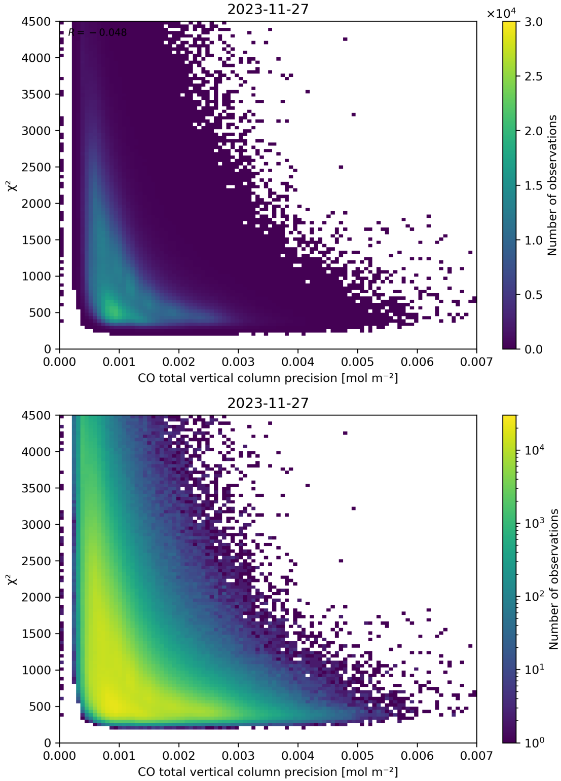
Figure 44: Scatter density plot of “CO total vertical column precision” against “ \chi^2 ” for 2023-11-26 to 2023-11-28.
