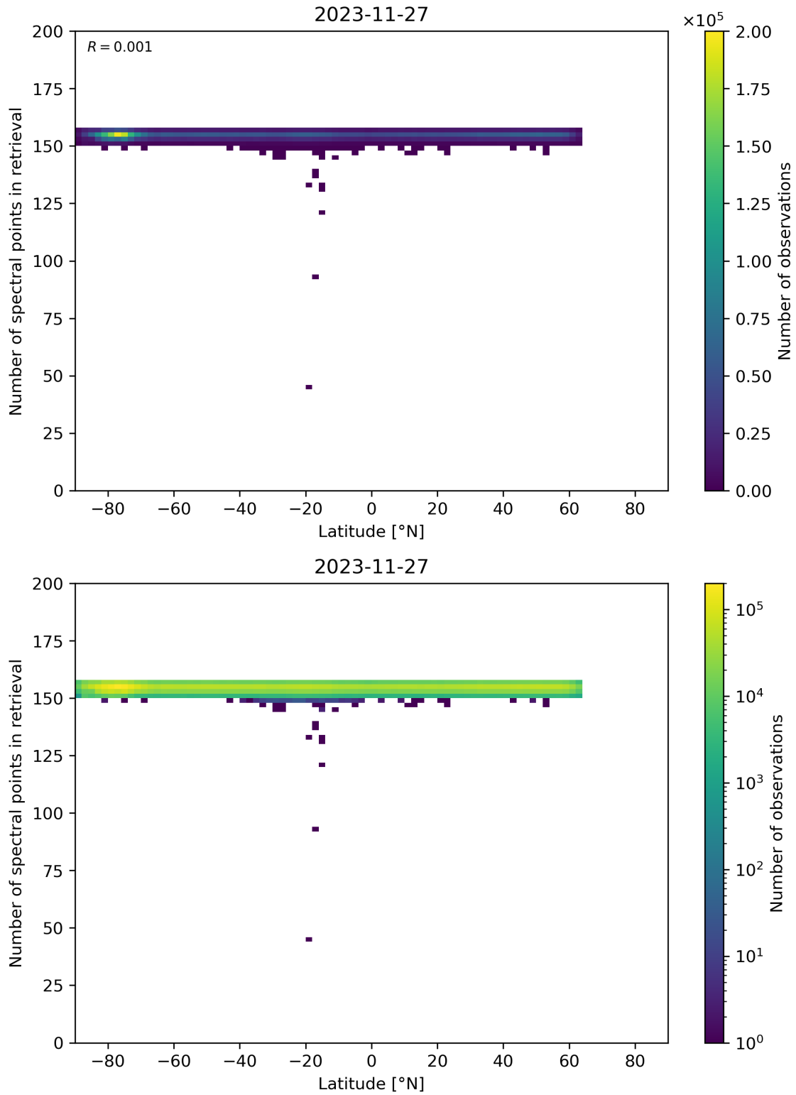
Figure 57: Scatter density plot of “Latitude” against “Number of spectral points in retrieval” for 2023-11-26 to 2023-11-28.
