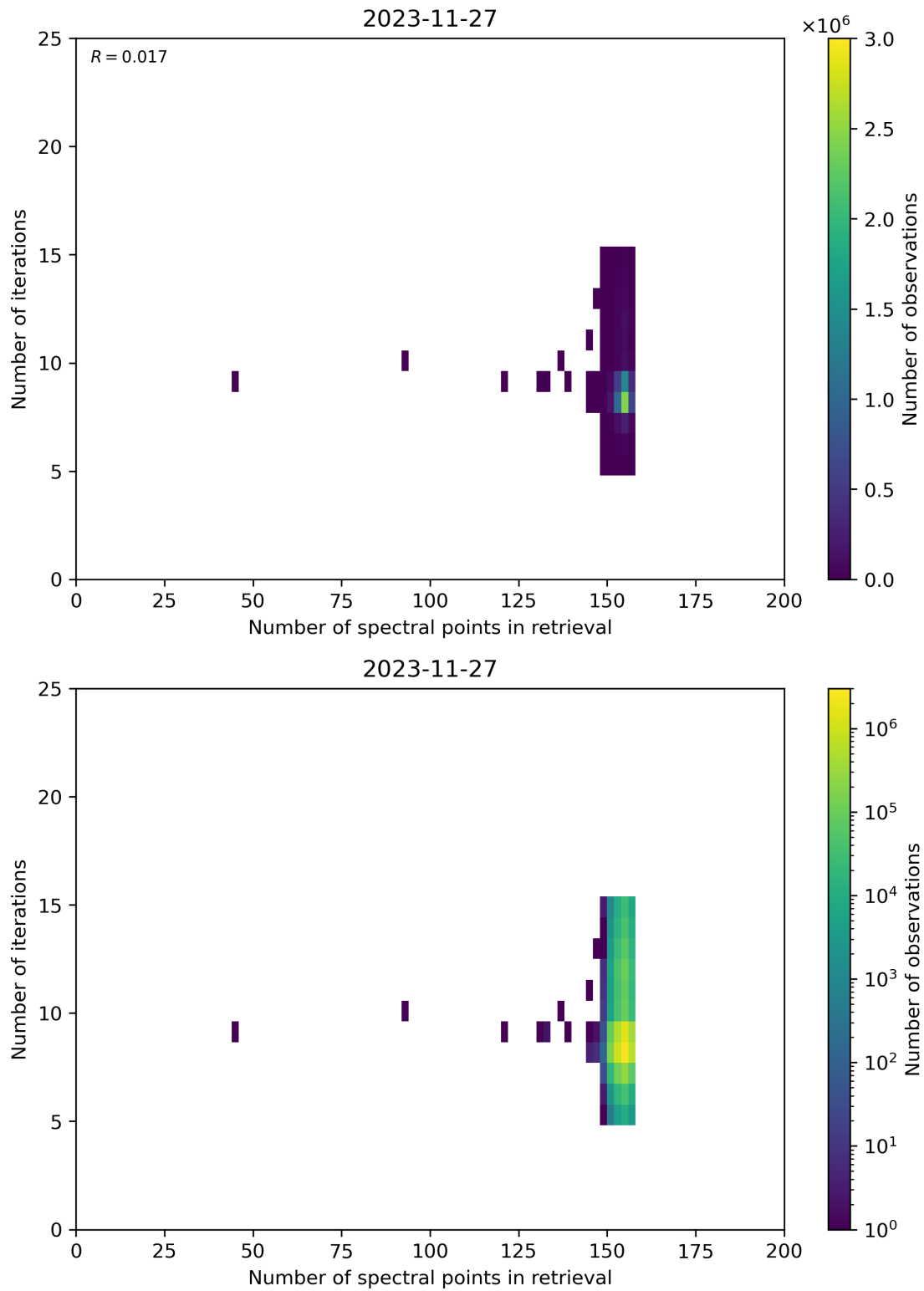
Figure 60: Scatter density plot of “Number of spectral points in retrieval” against “Number of iterations” for 2023-11-26 to 2023-11-28.
