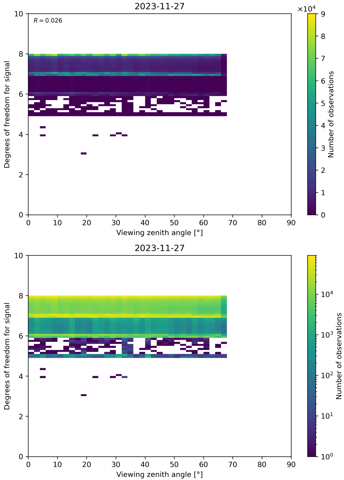
Figure 73: Scatter density plot of “Viewing zenith angle” against “Degrees of freedom for signal” for 2023-11-26 to 2023-11-28.
