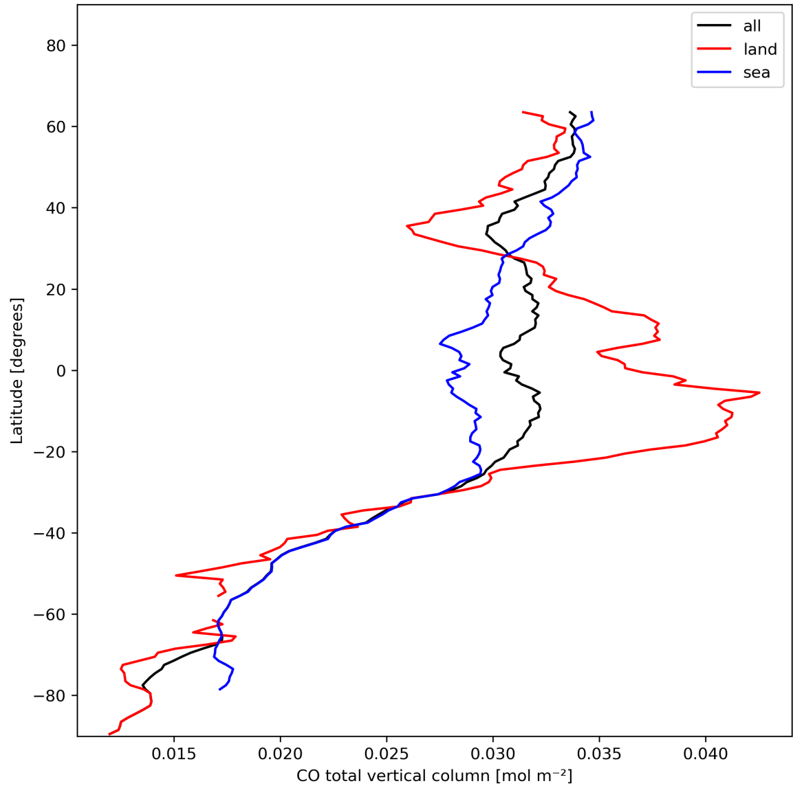
Figure 10: Zonal average of “CO total vertical column” for 2023-11-26 to 2023-11-28.
