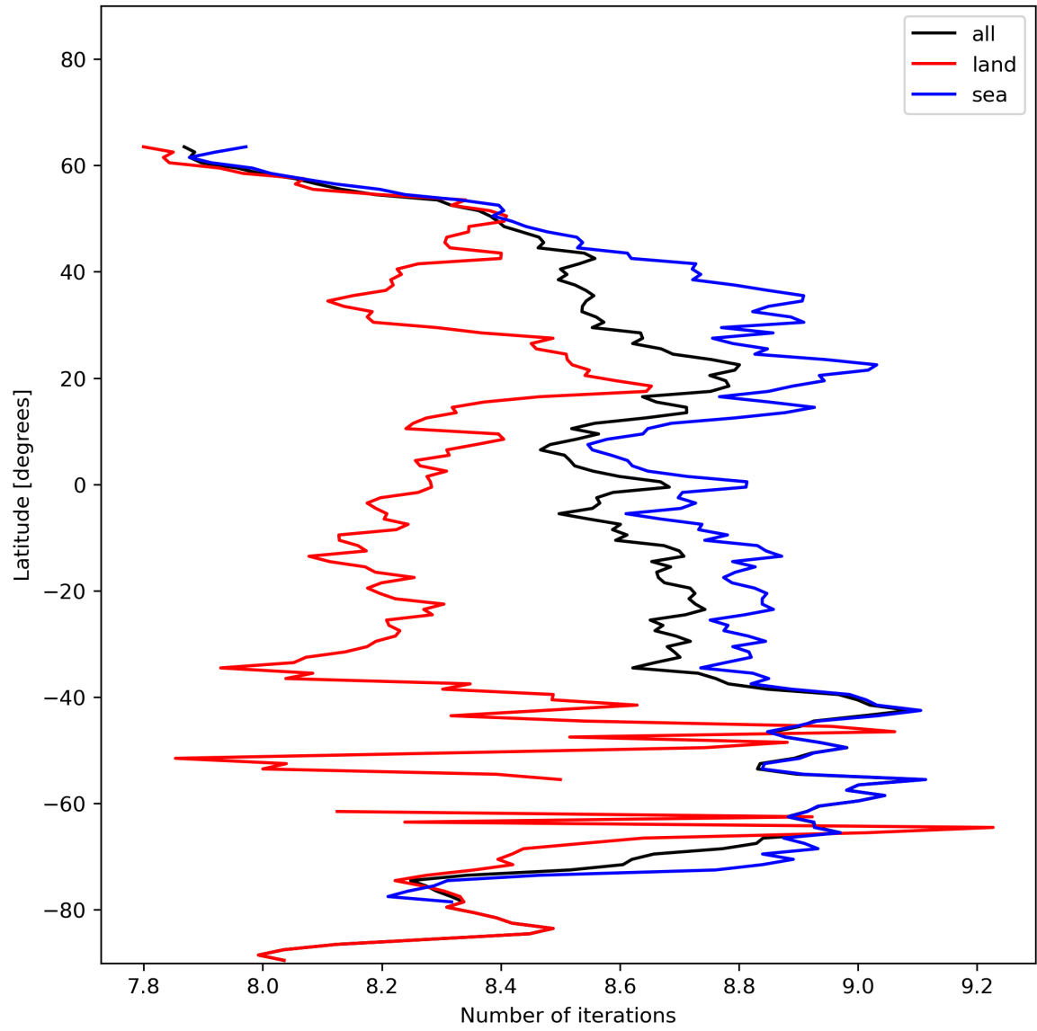
Figure 16: Zonal average of “Number of iterations” for 2023-11-26 to 2023-11-28.
