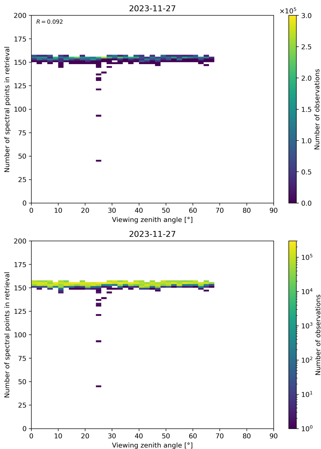
Figure 76: Scatter density plot of “Viewing zenith angle” against “Number of spectral points in retrieval” for 2023-11-26 to 2023-11-28.
