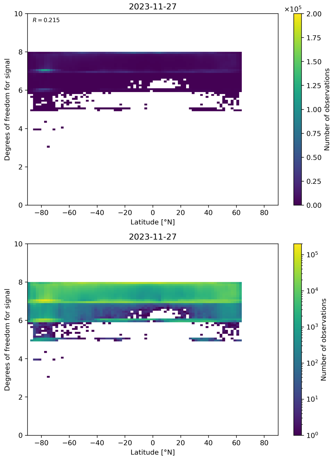
Figure 55: Scatter density plot of “Latitude” against “Degrees of freedom for signal” for 2023-11-26 to 2023-11-28.
