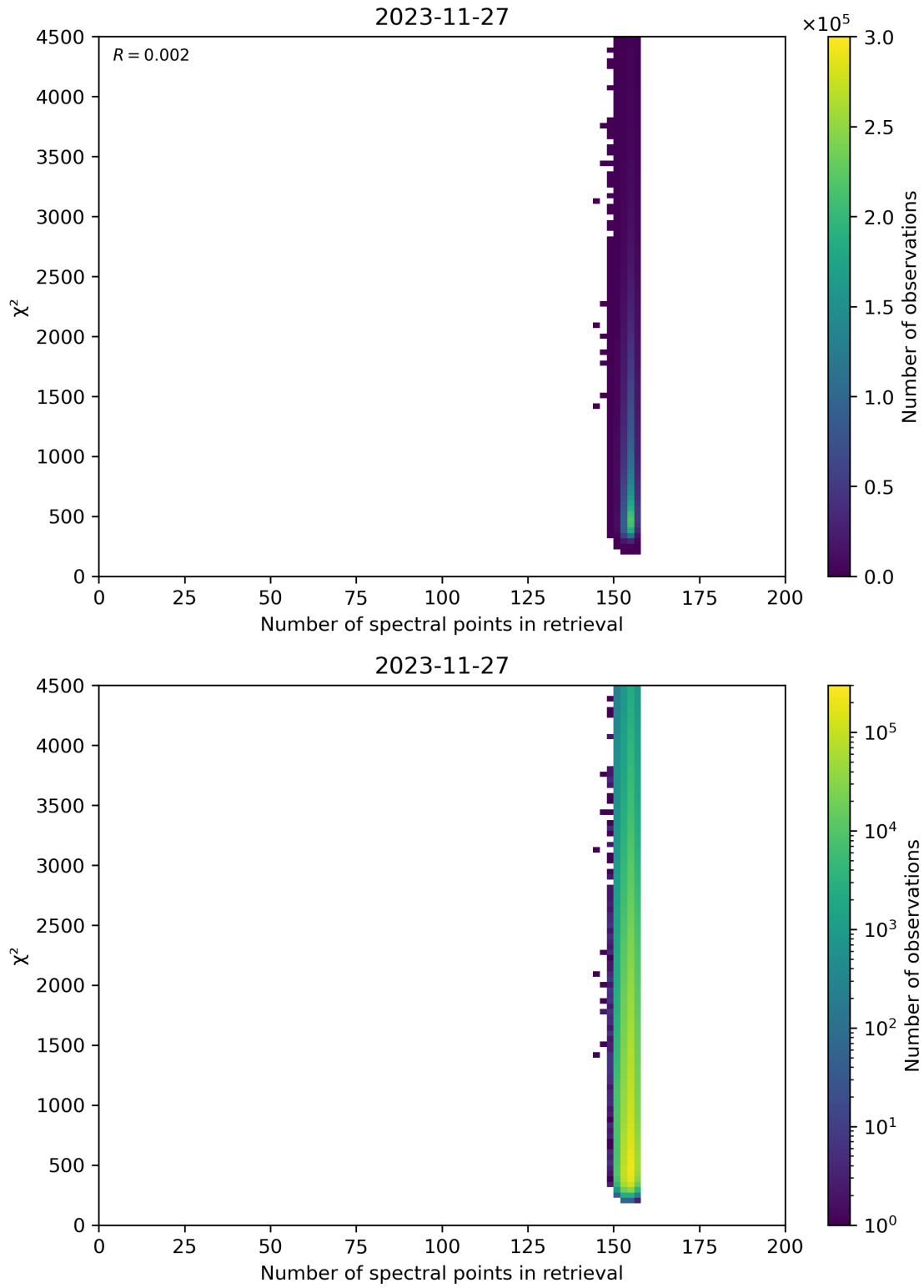
Figure 58: Scatter density plot of “Number of spectral points in retrieval” against “ \chi^2 ” for 2023-11-26 to 2023-11-28.
