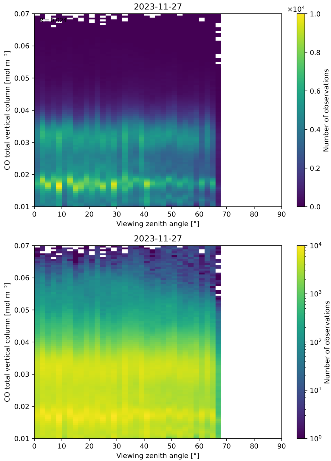
Figure 69: Scatter density plot of “Viewing zenith angle” against “CO total vertical column” for 2023-11-26 to 2023-11-28.
