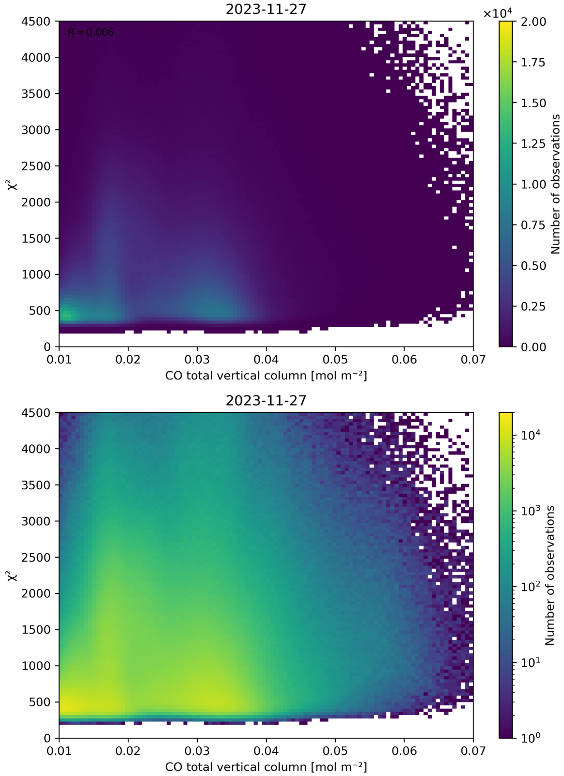
Figure 35: Scatter density plot of “CO total vertical column” against “ \chi^2 ” for 2023-11-26 to 2023-11-28.
