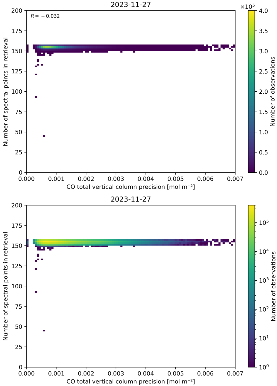
Figure 47: Scatter density plot of “CO total vertical column precision” against “Number of spectral points in retrieval” for 2023-11-26 to 2023-11-28.
