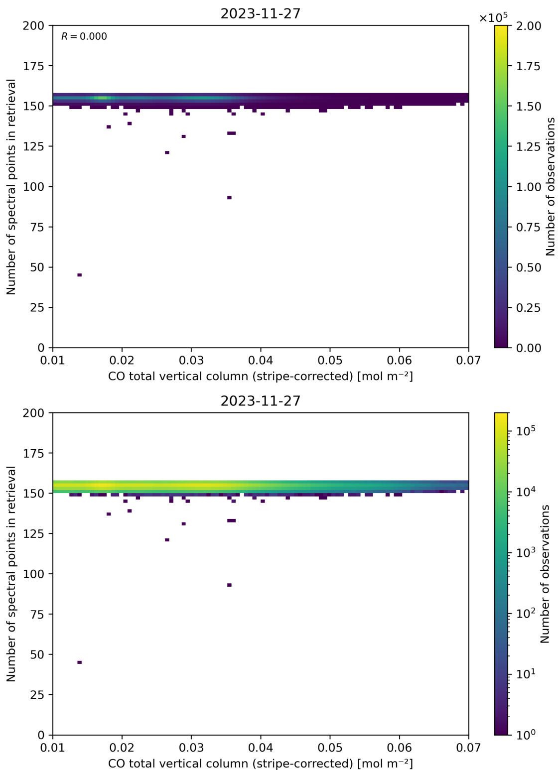
Figure 40: Scatter density plot of “CO total vertical column (stripe-corrected)” against “Number of spectral points in retrieval” for 2023-11-26 to 2023-11-28.
