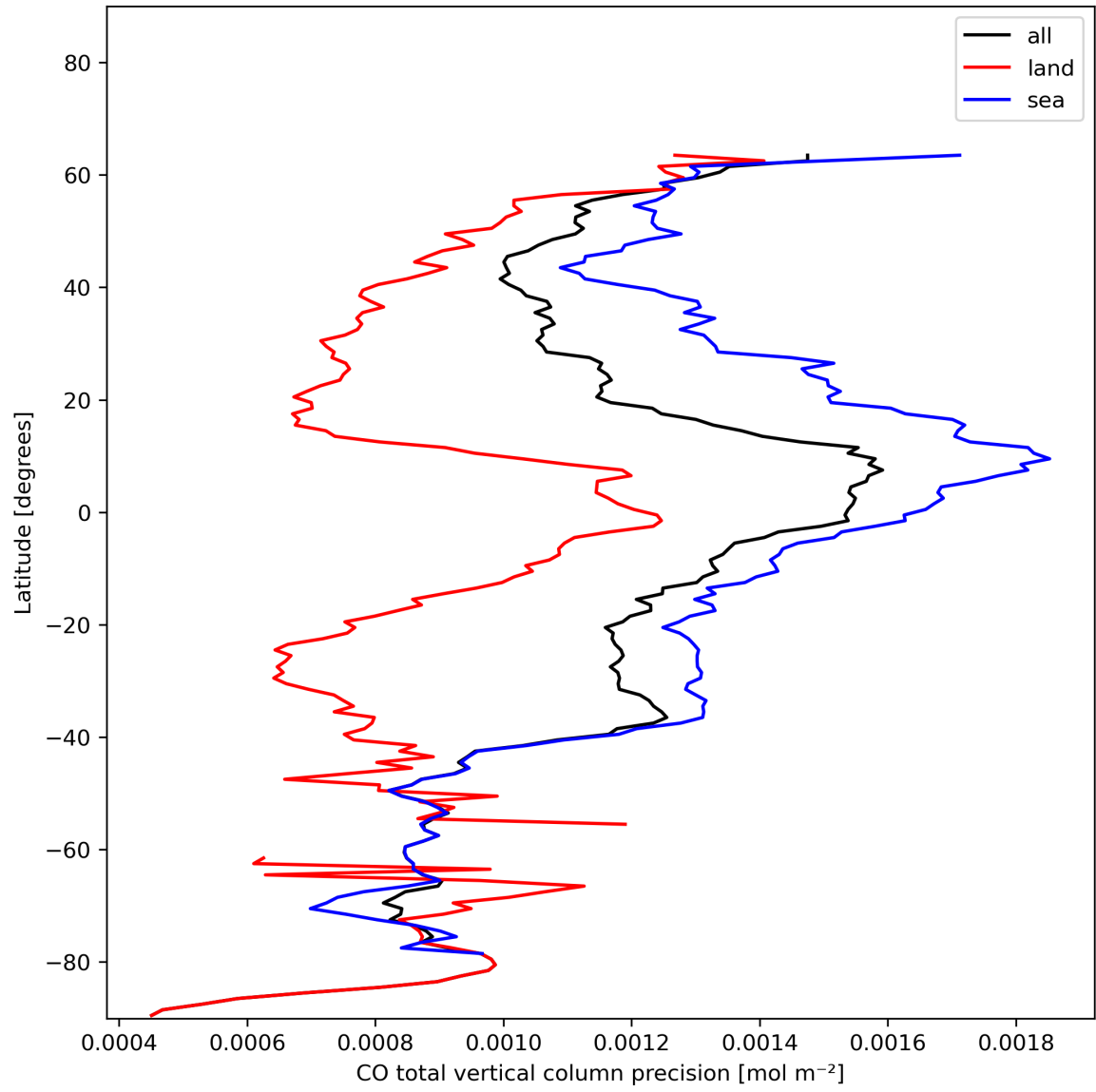
Figure 12: Zonal average of “CO total vertical column precision” for 2023-11-26 to 2023-11-28.
