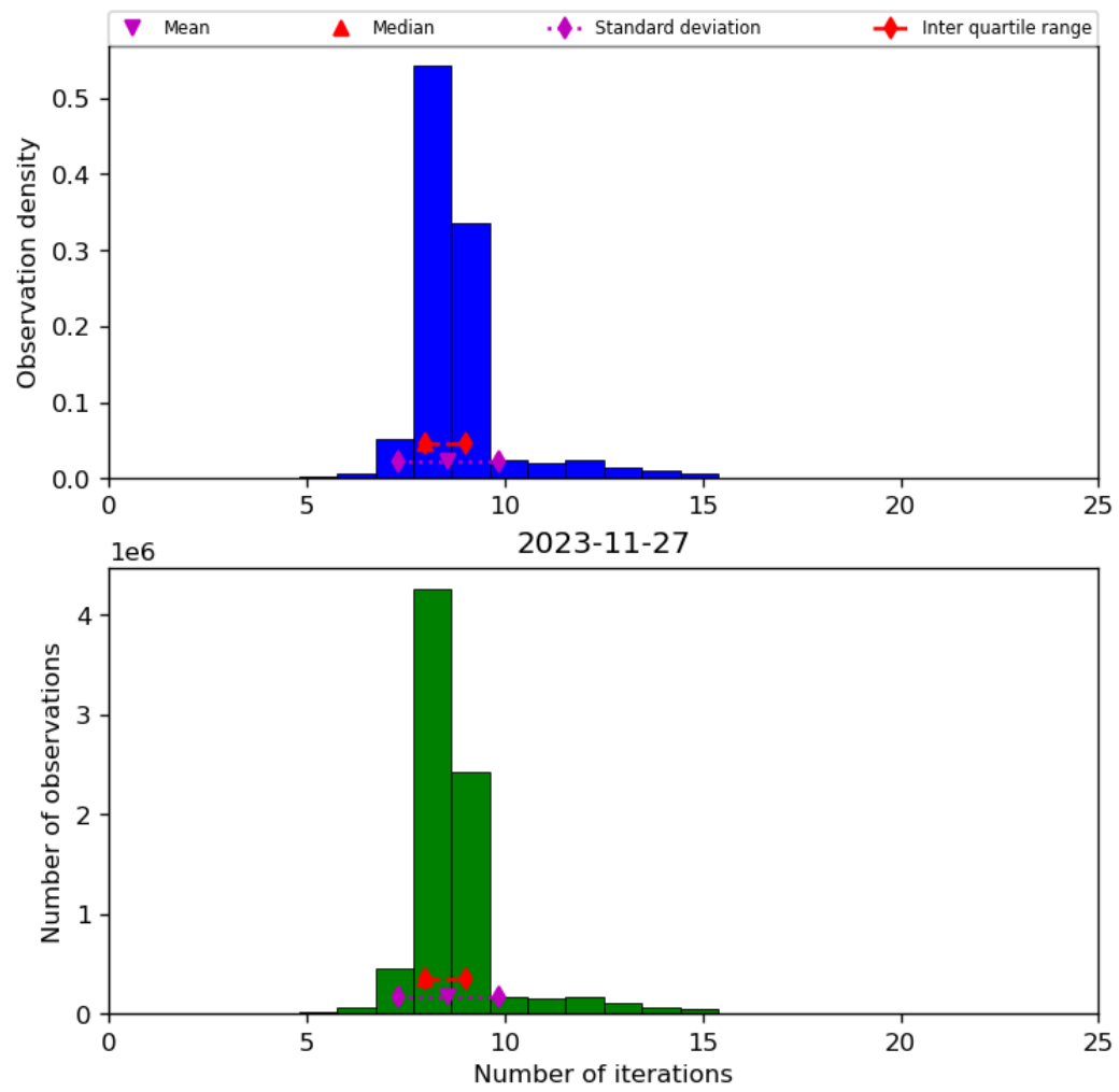
Figure 24: Histogram of “Number of iterations” for 2023-11-26 to 2023-11-28
