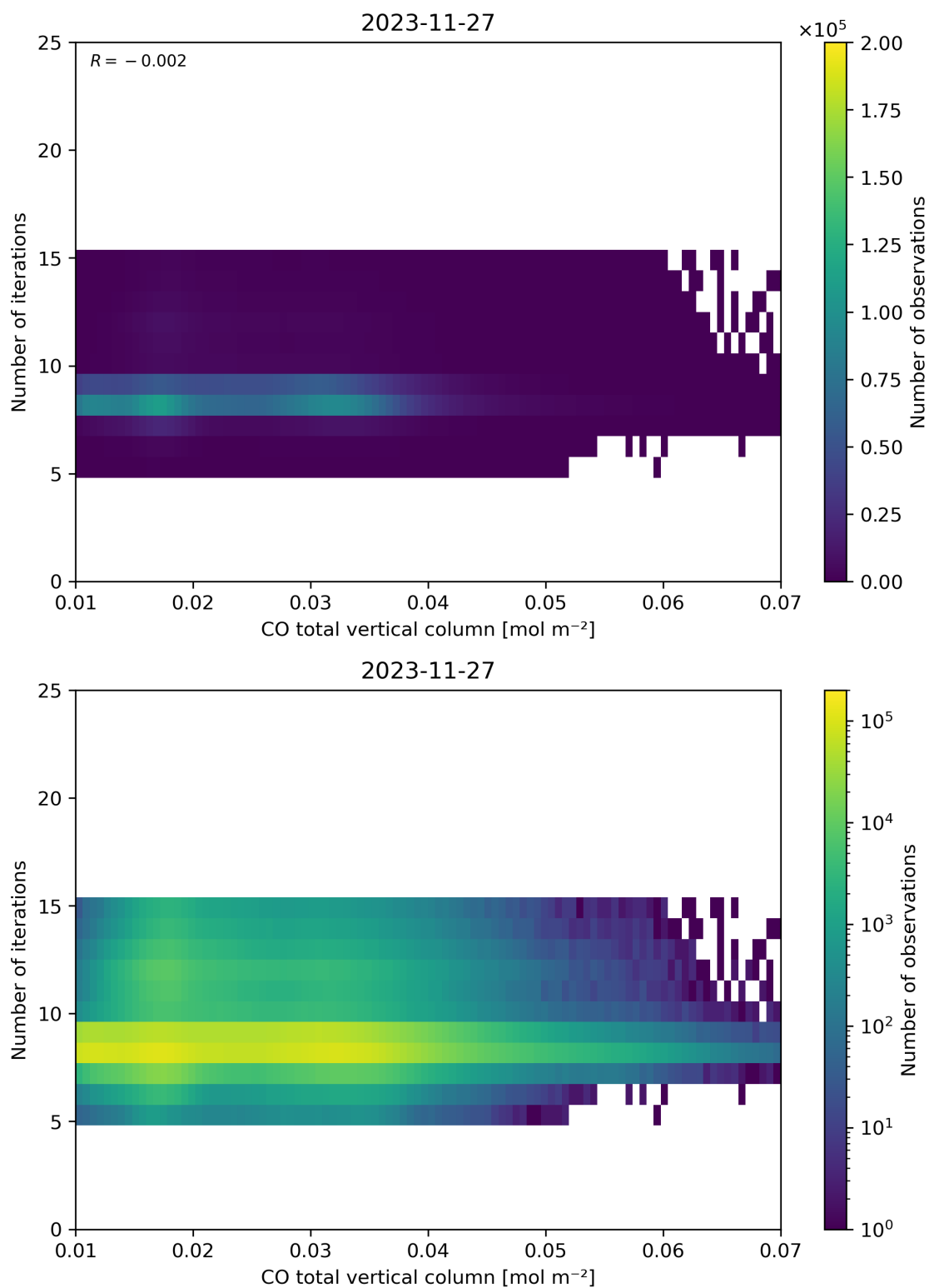
Figure 42: Scatter density plot of “CO total vertical column” against “Number of iterations” for 2023-11-26 to 2023-11-28.
