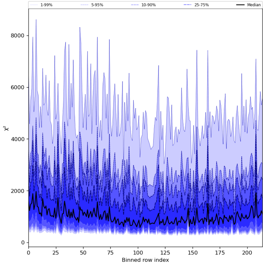
Figure 30: Along track statistics of “ \chi^2 ” for 2023-11-26 to 2023-11-28
