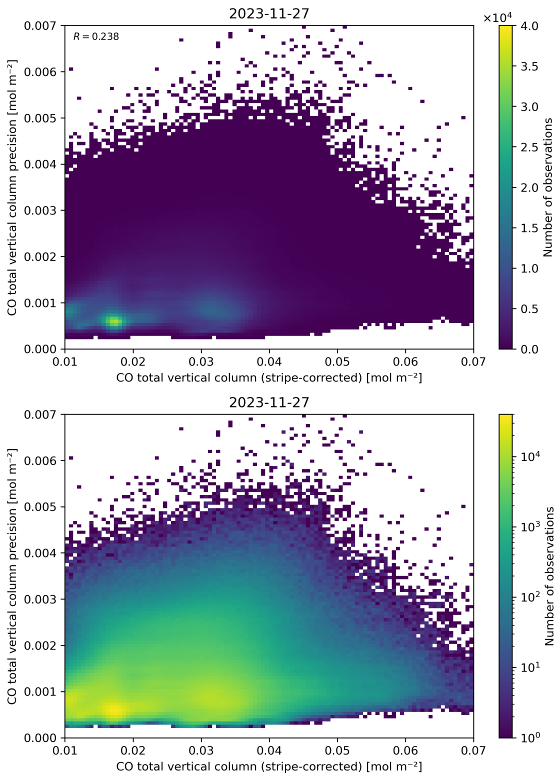
Figure 36: Scatter density plot of “CO total vertical column (stripe-corrected)” against “CO total vertical column precision” for 2023-11-26 to 2023-11-28.
