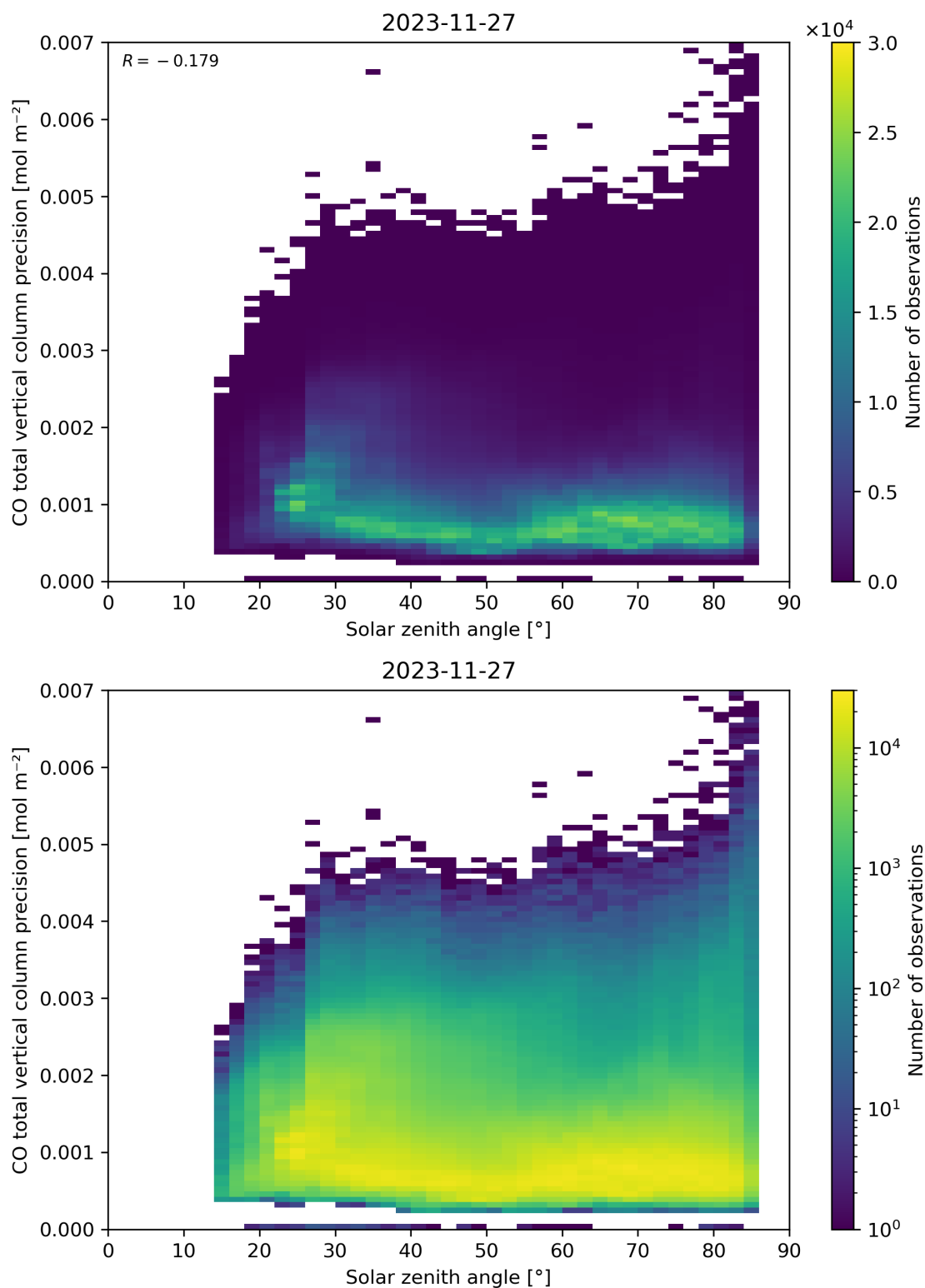
Figure 63: Scatter density plot of “Solar zenith angle” against “CO total vertical column precision” for 2023-11-26 to 2023-11-28.
