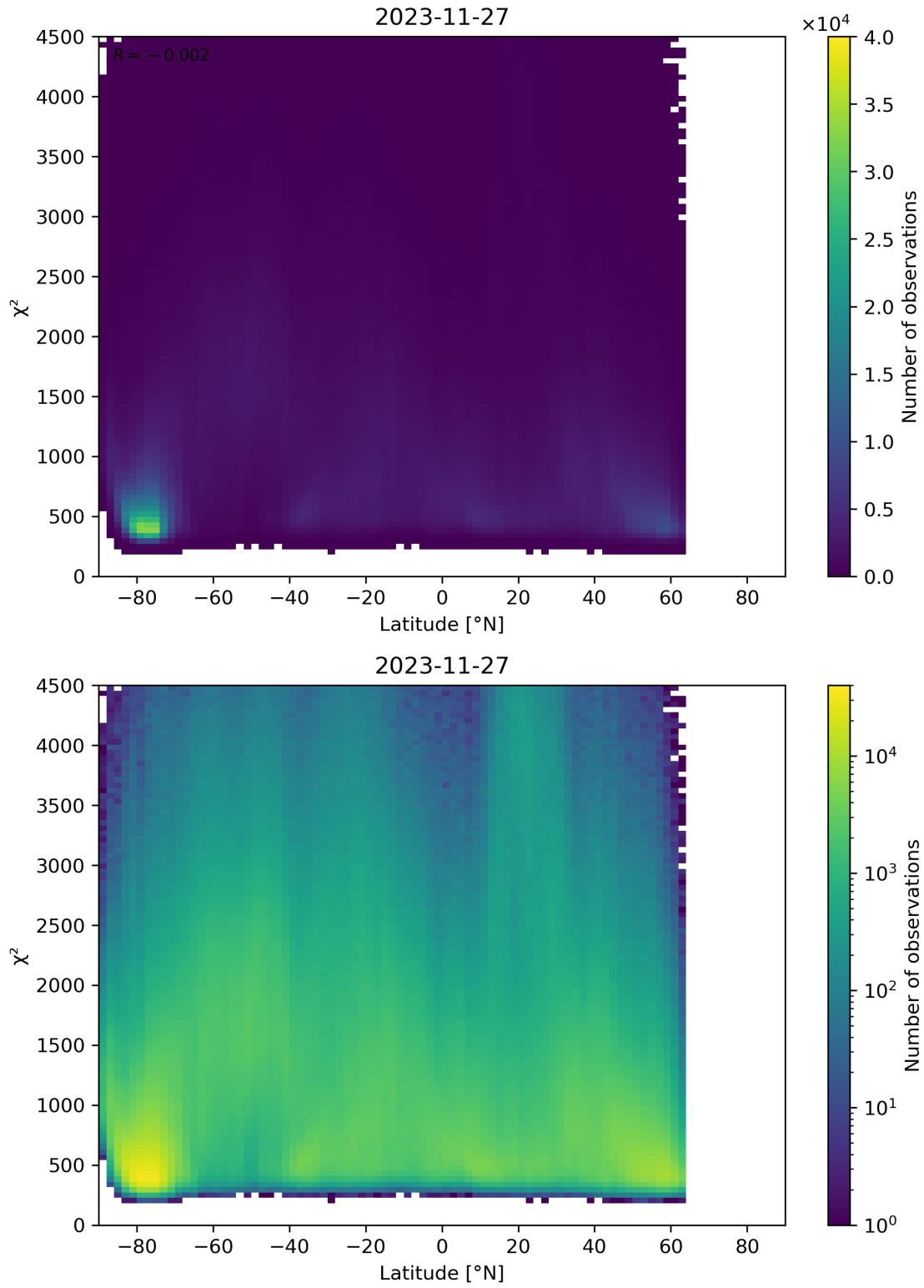
Figure 54: Scatter density plot of “Latitude” against “ \chi^2 ” for 2023-11-26 to 2023-11-28.
