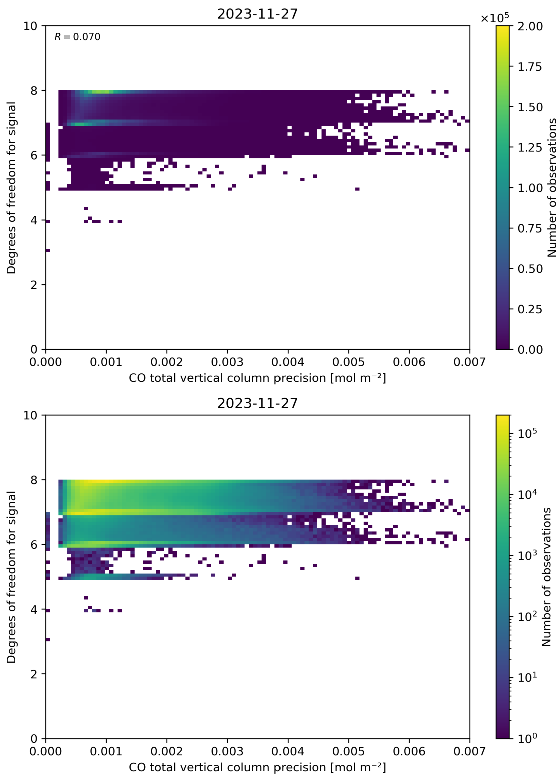
Figure 45: Scatter density plot of “CO total vertical column precision” against “Degrees of freedom for signal” for 2023-11-26 to 2023-11-28.
