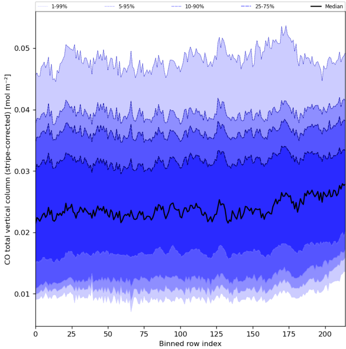
Figure 27: Along track statistics of “CO total vertical column (stripe-corrected)” for 2023-11-26 to 2023-11-28
