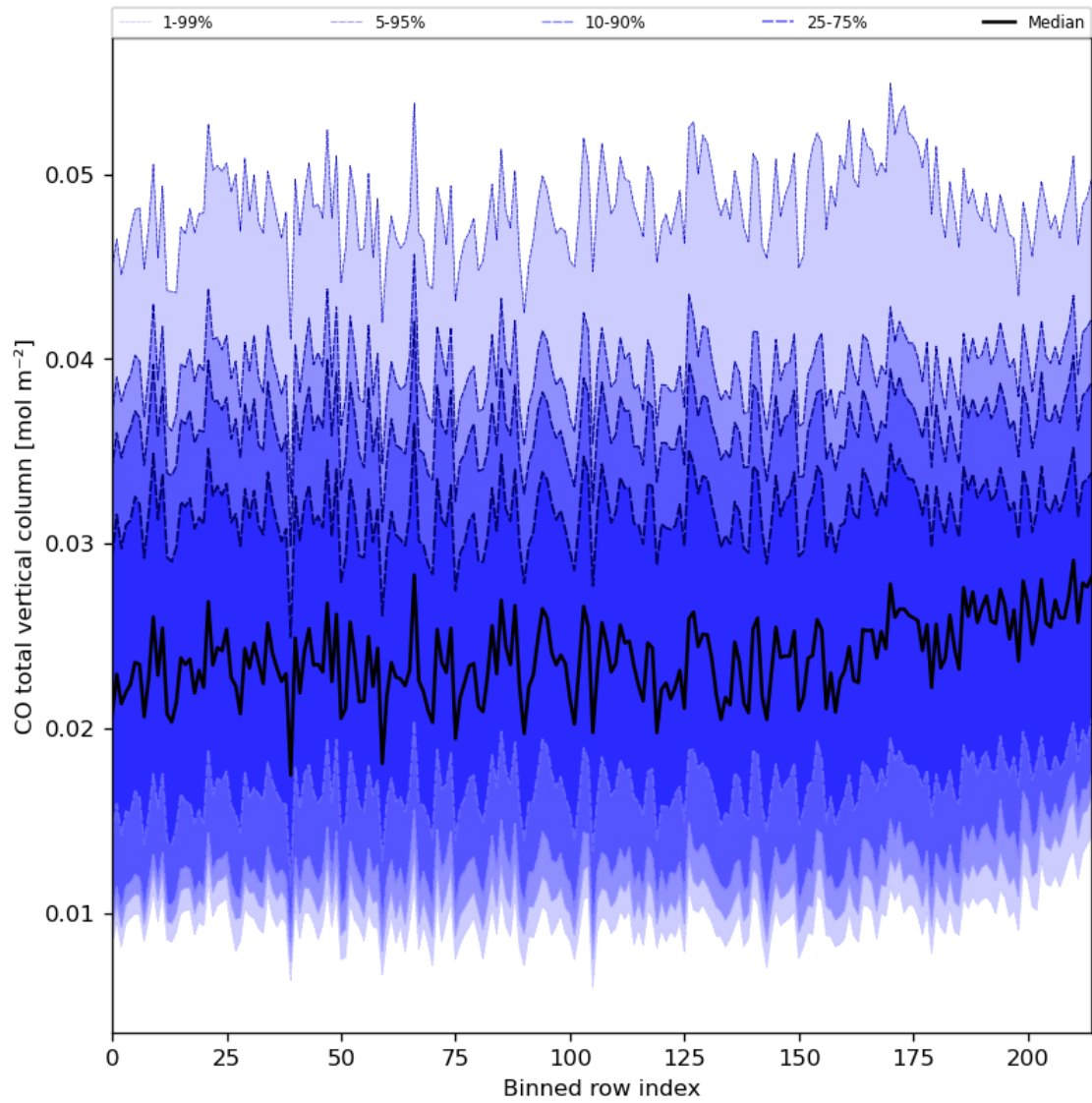
Figure 26: Along track statistics of “CO total vertical column” for 2023-11-26 to 2023-11-28
