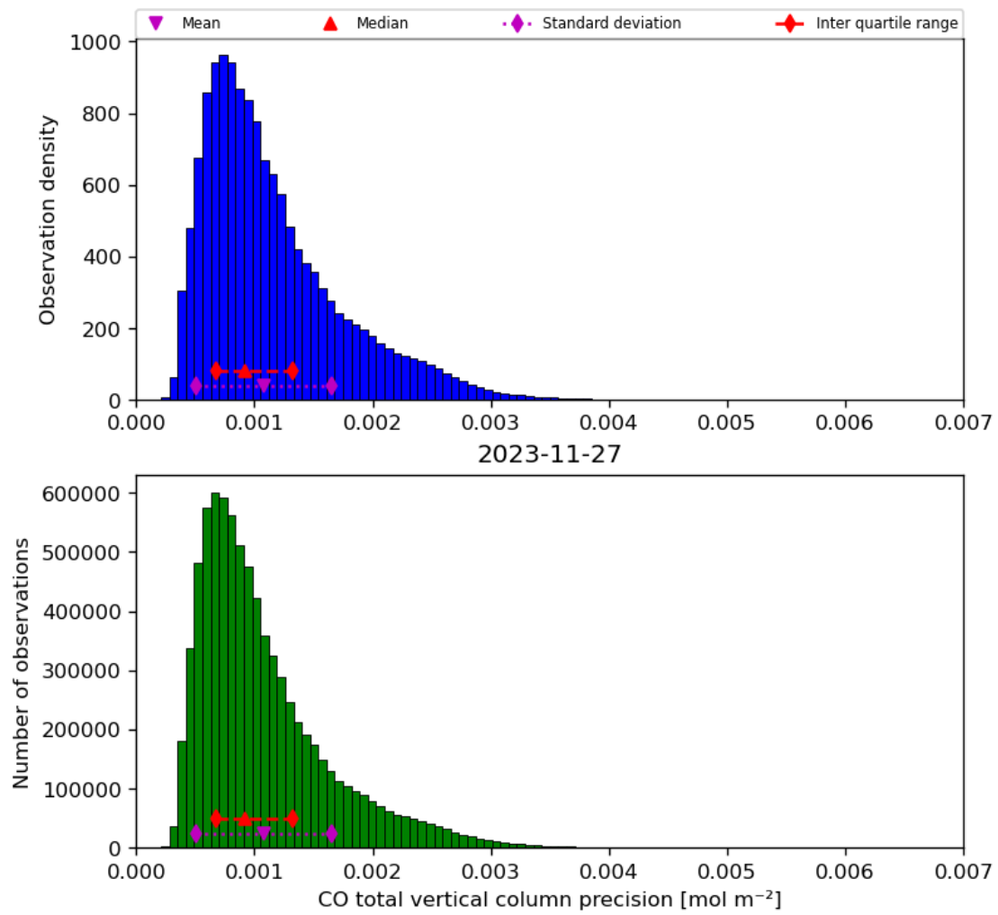
Figure 20: Histogram of “CO total vertical column precision” for 2023-11-26 to 2023-11-28
