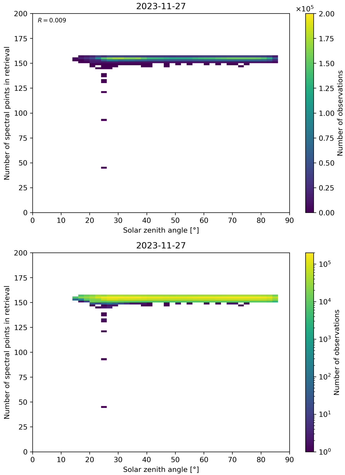
Figure 68: Scatter density plot of “Solar zenith angle” against “Number of spectral points in retrieval” for 2023-11-26 to 2023-11-28.
