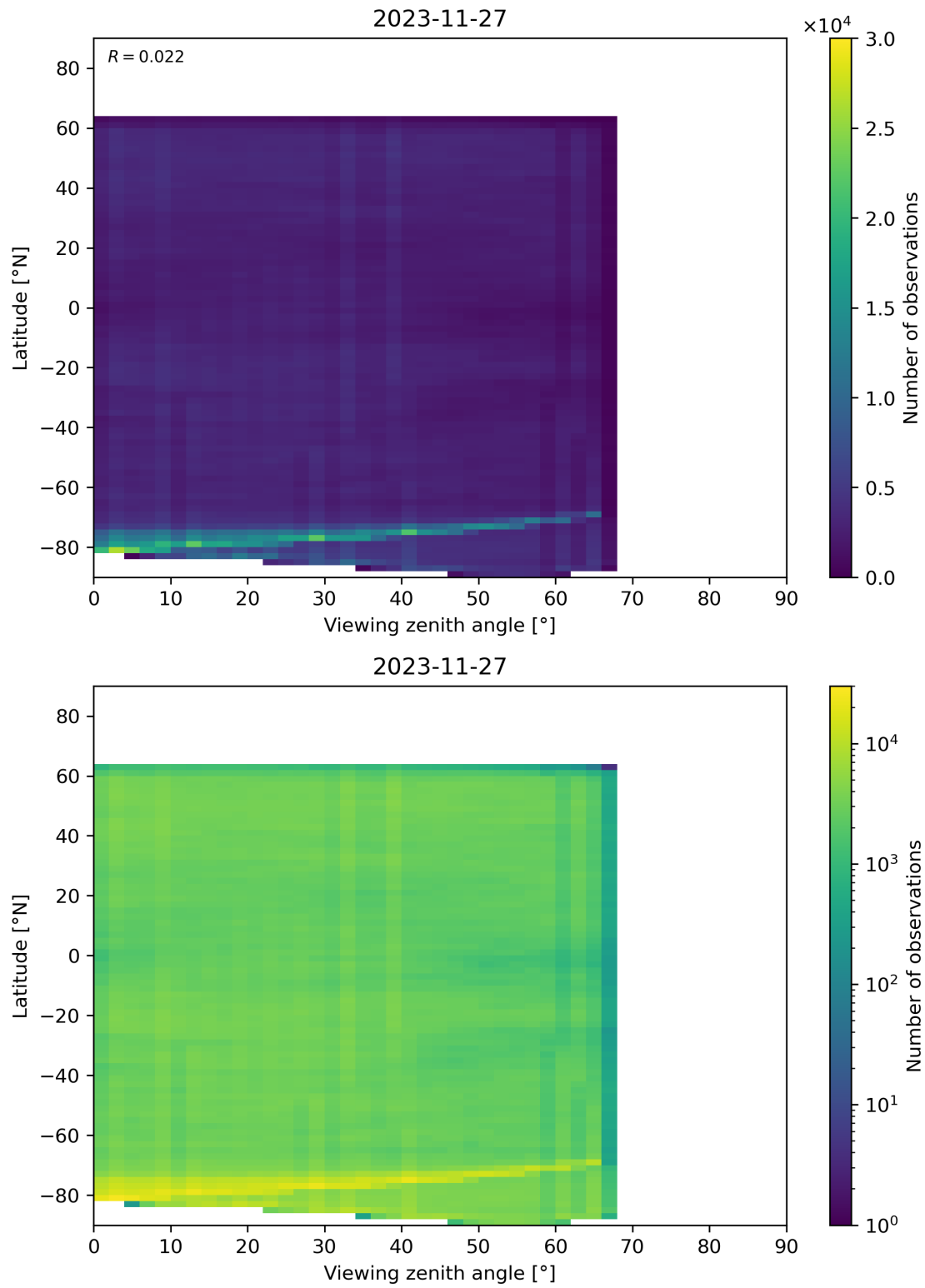
Figure 74: Scatter density plot of “Viewing zenith angle” against “Latitude” for 2023-11-26 to 2023-11-28.
