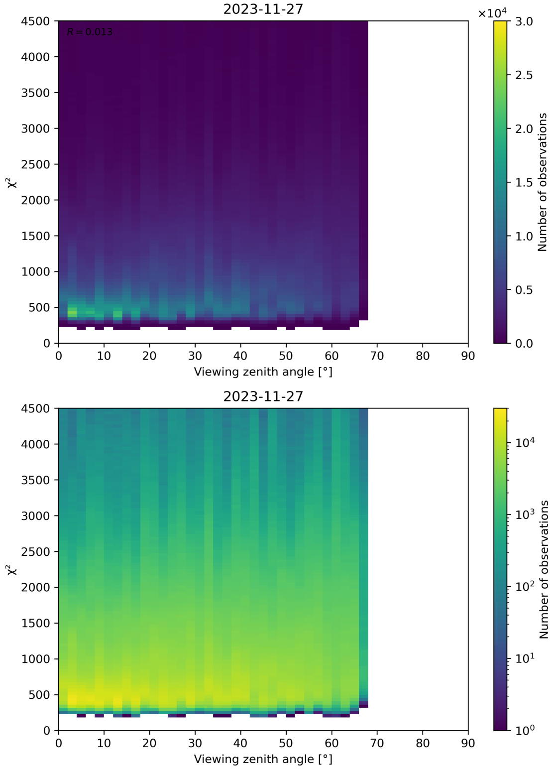
Figure 72: Scatter density plot of “Viewing zenith angle” against “ \chi^2 ” for 2023-11-26 to 2023-11-28.
