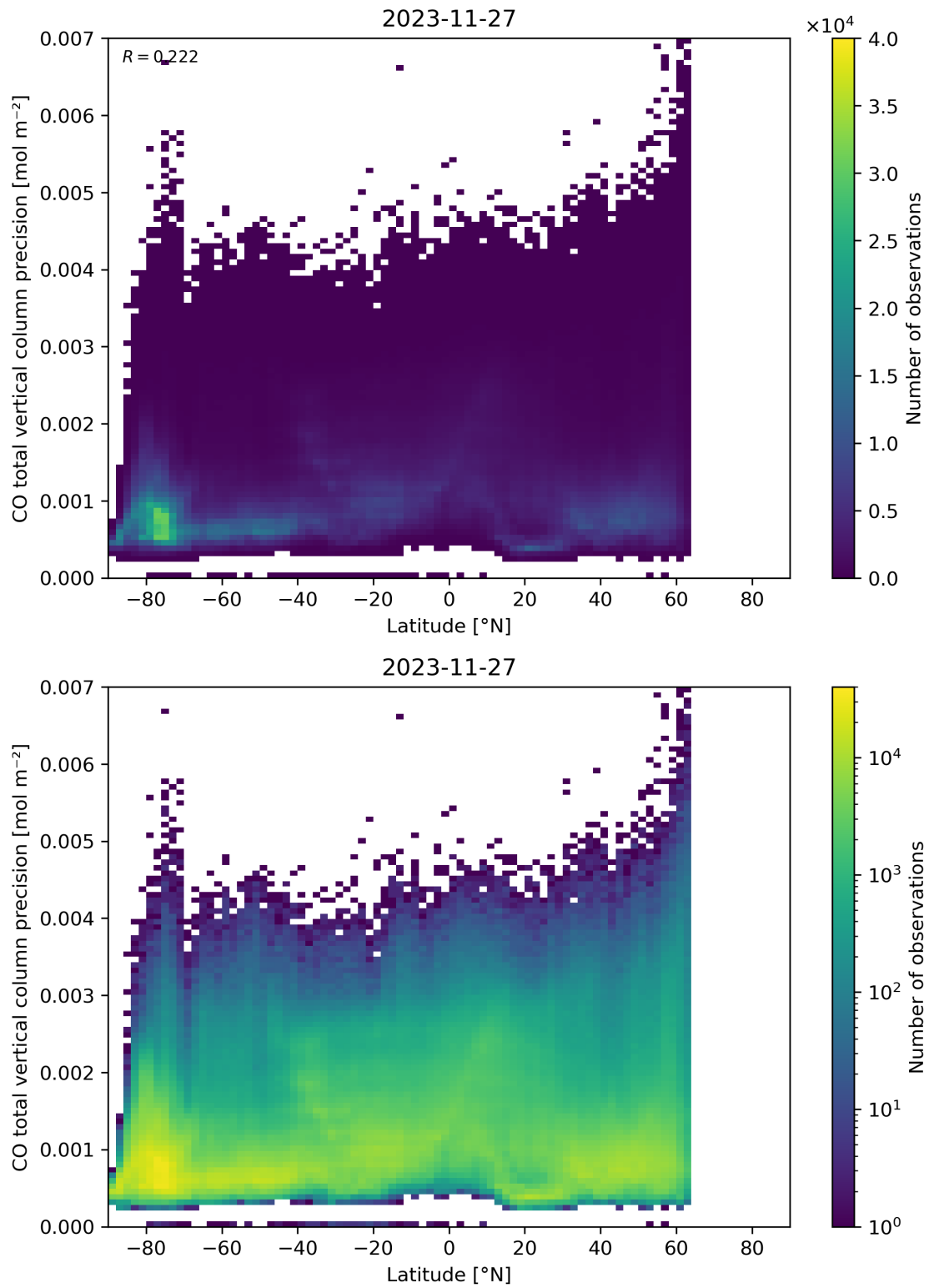
Figure 53: Scatter density plot of “Latitude” against “CO total vertical column precision” for 2023-11-26 to 2023-11-28.
