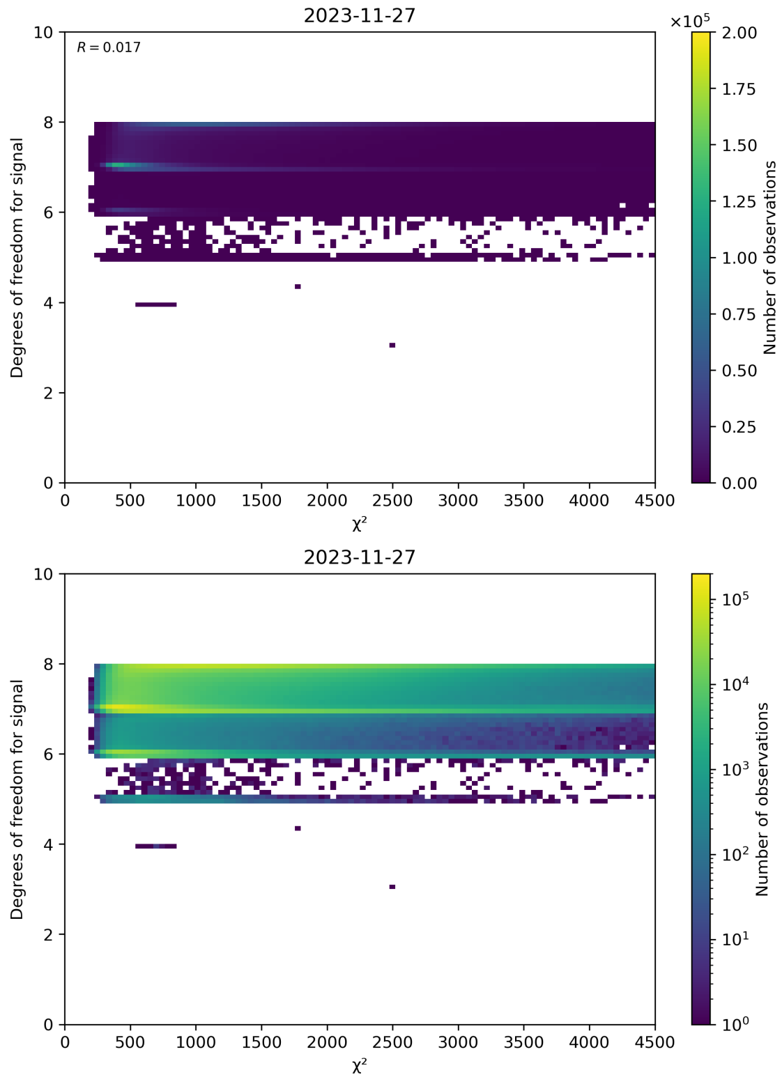
Figure 48: Scatter density plot of “ \chi^2 ” against “Degrees of freedom for signal” for 2023-11-26 to 2023-11-28.
