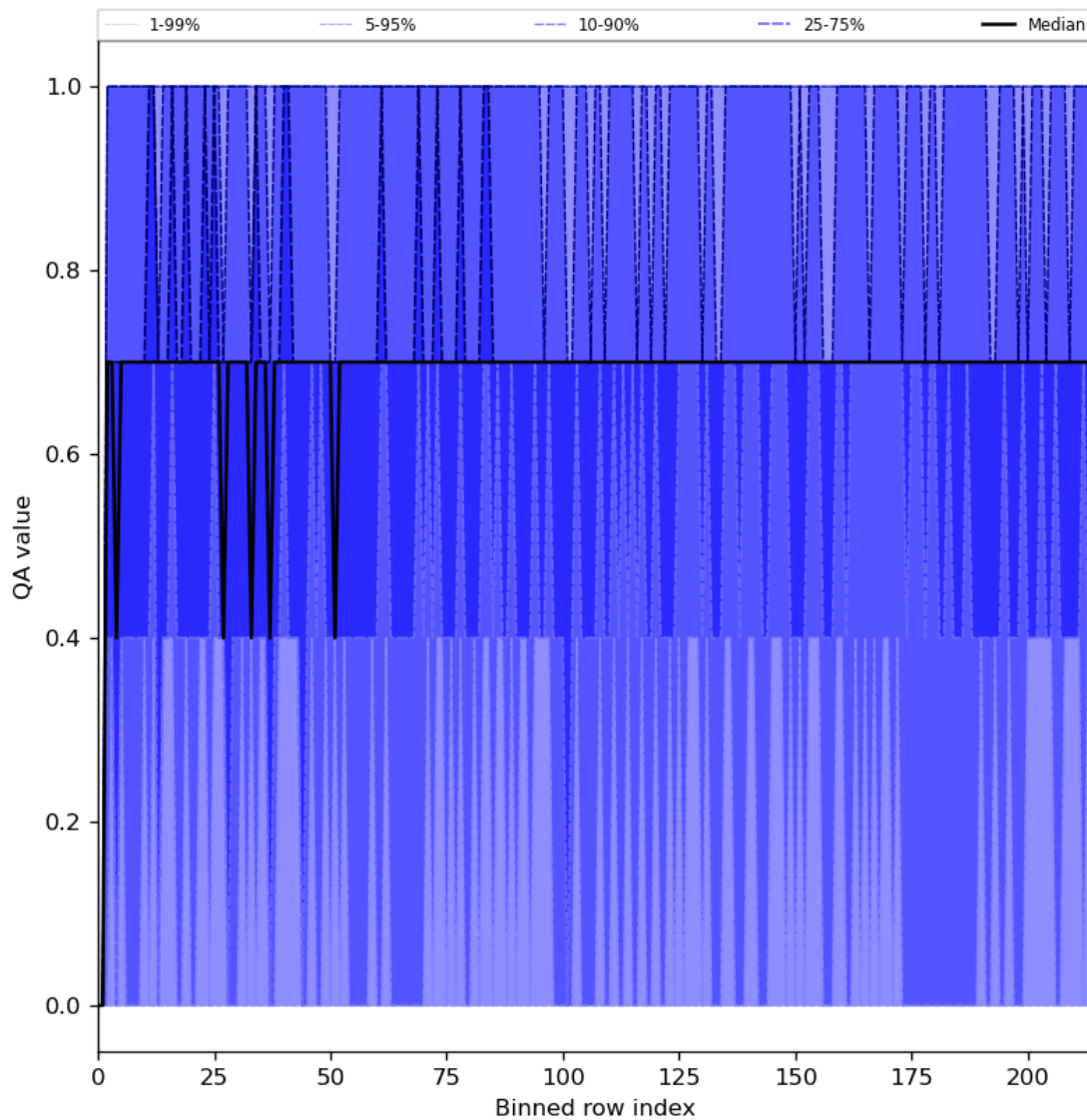
Figure 25: Along track statistics of “QA value” for 2023-11-26 to 2023-11-28
