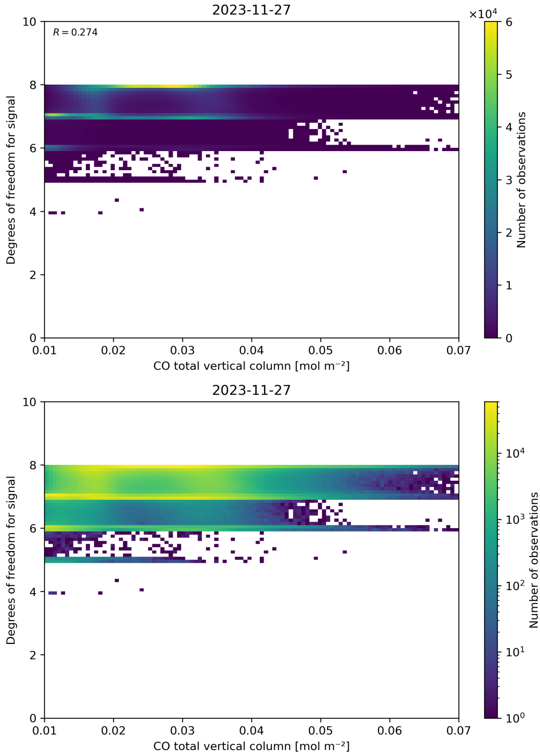
Figure 41: Scatter density plot of “CO total vertical column” against “Degrees of freedom for signal” for 2023-11-26 to 2023-11-28.
