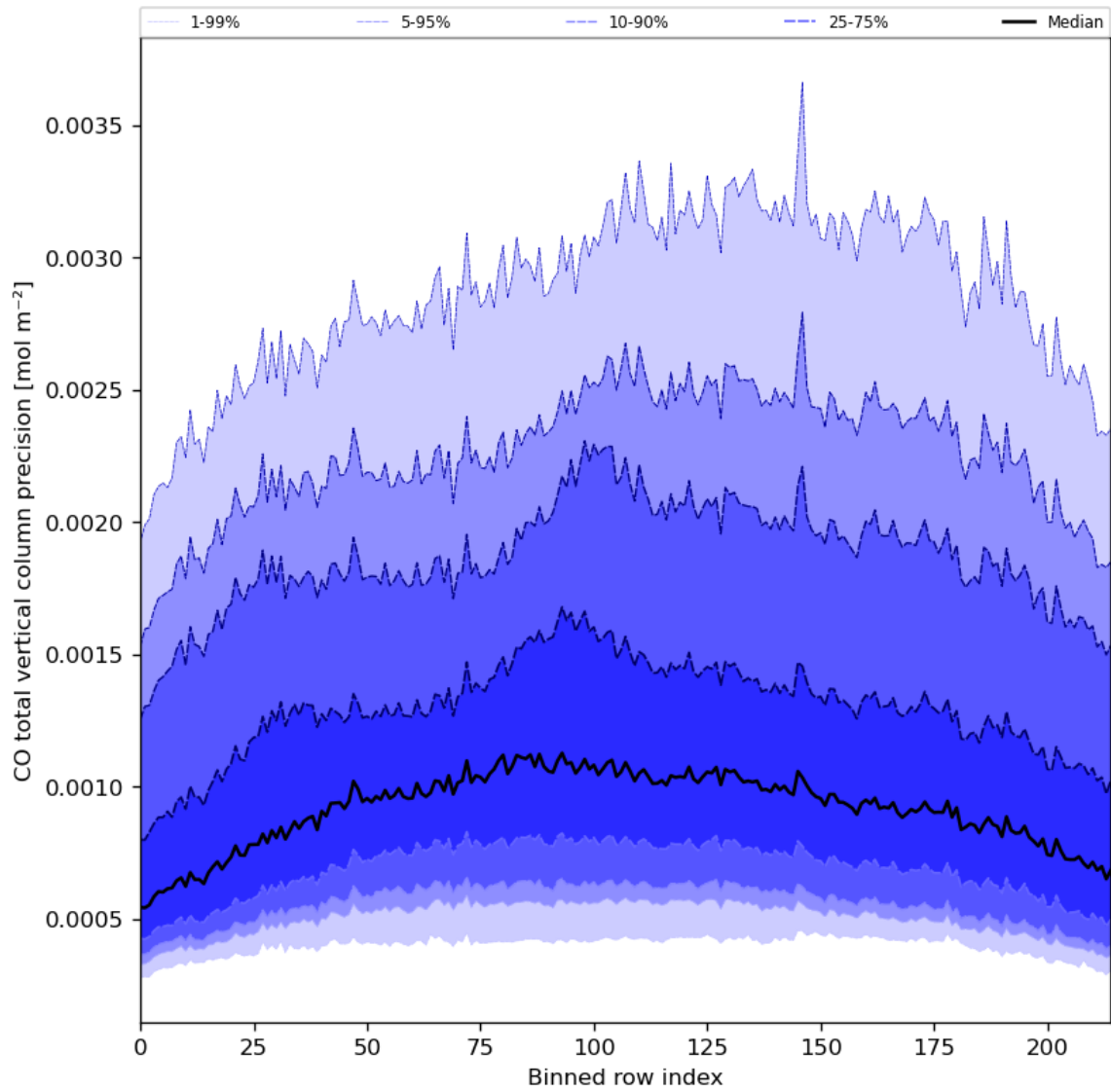
Figure 28: Along track statistics of “CO total vertical column precision” for 2023-11-26 to 2023-11-28
