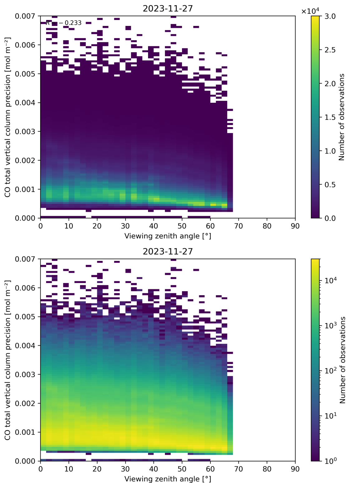
Figure 71: Scatter density plot of “Viewing zenith angle” against “CO total vertical column precision” for 2023-11-26 to 2023-11-28.
