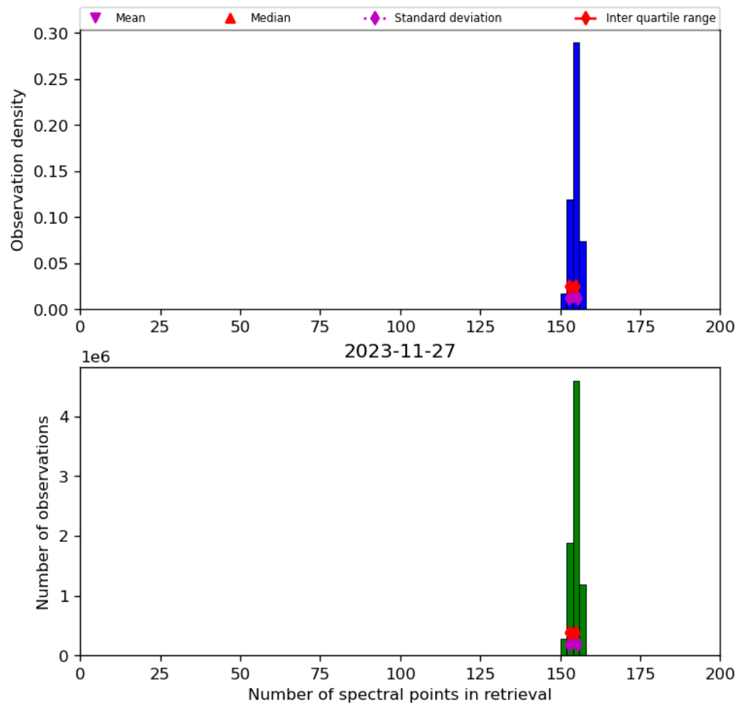
Figure 21: Histogram of “Number of spectral points in retrieval” for 2023-11-26 to 2023-11-28
