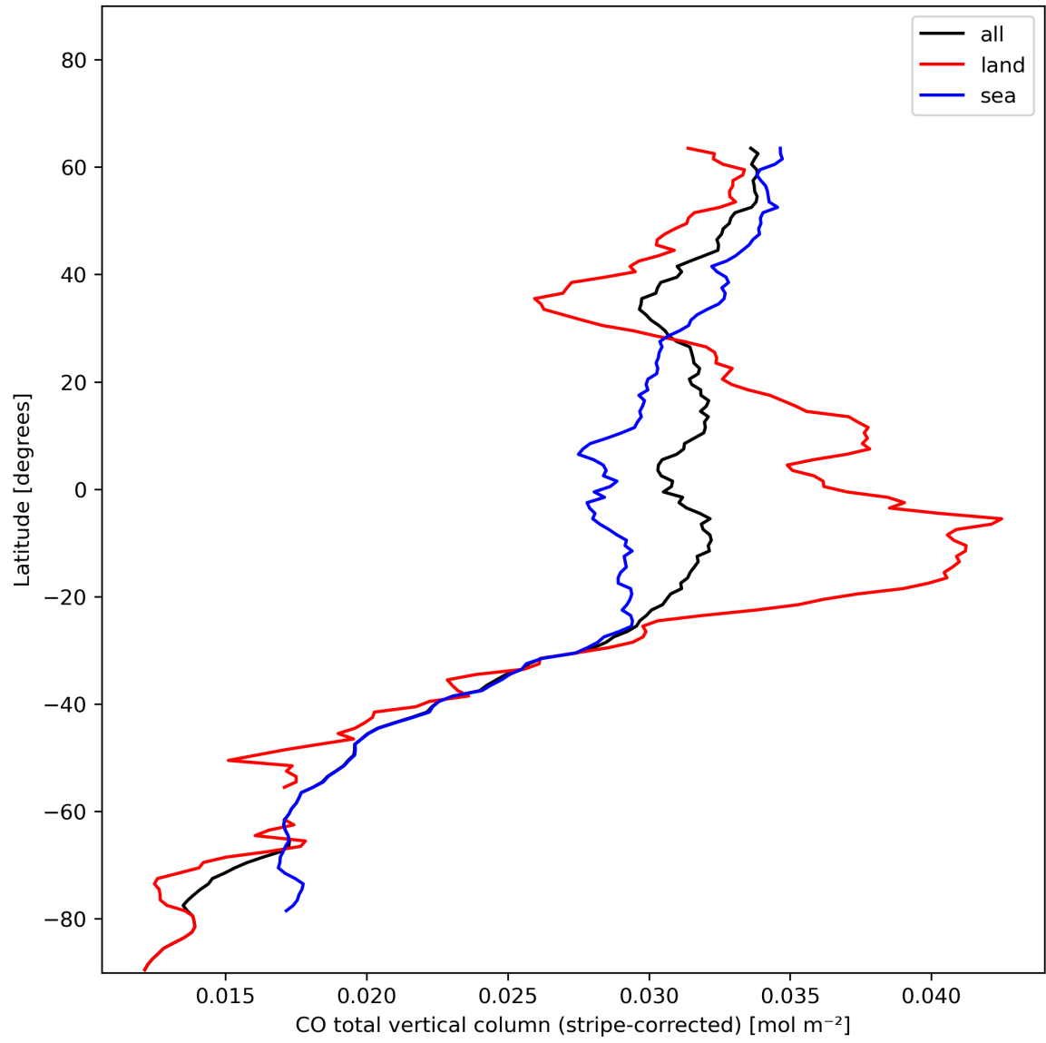
Figure 11: Zonal average of “CO total vertical column (stripe-corrected)” for 2023-11-26 to 2023-11-28.
