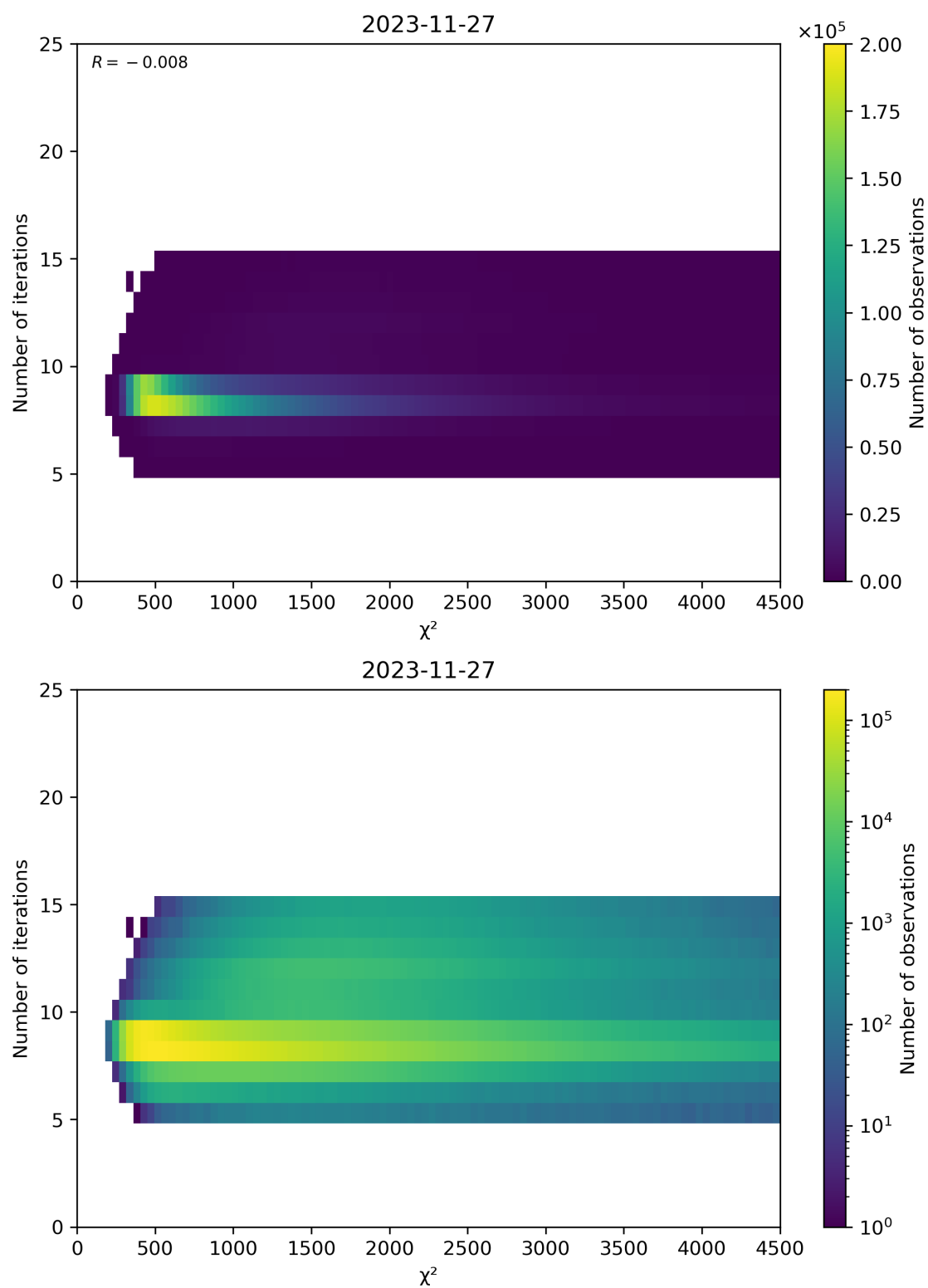
Figure 49: Scatter density plot of “ \chi^2 ” against “Number of iterations” for 2023-11-26 to 2023-11-28.
