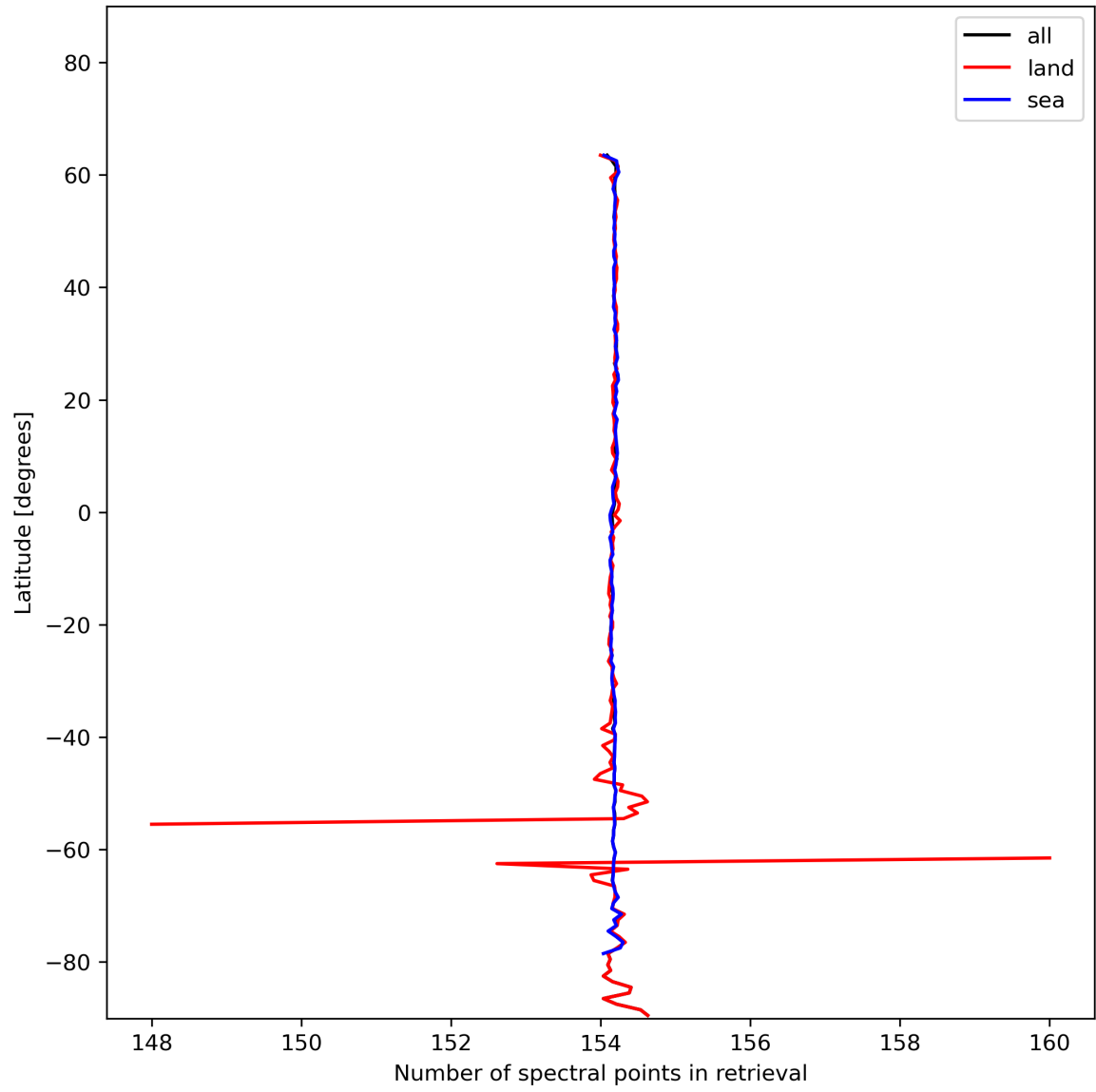
Figure 13: Zonal average of “Number of spectral points in retrieval” for 2023-11-26 to 2023-11-28.
