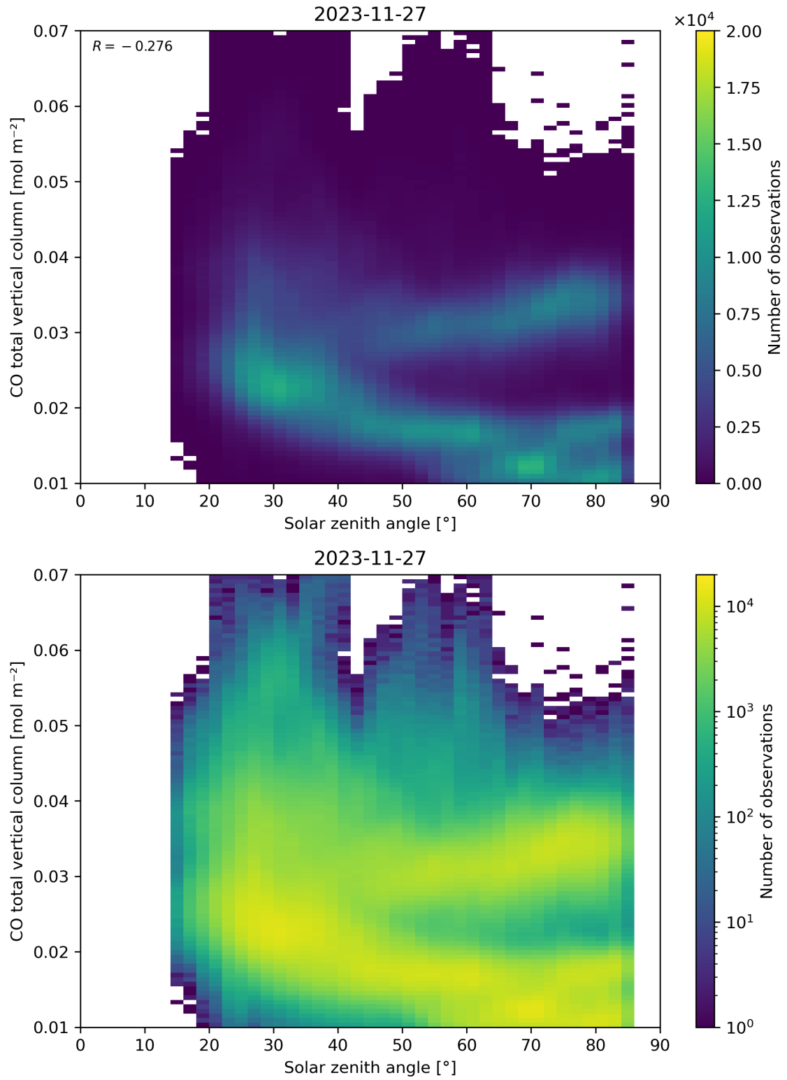
Figure 61: Scatter density plot of “Solar zenith angle” against “CO total vertical column” for 2023-11-26 to 2023-11-28.
