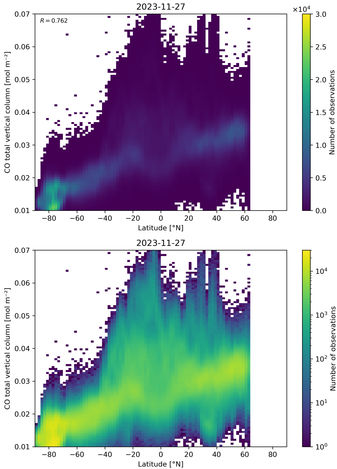
Figure 51: Scatter density plot of “Latitude” against “CO total vertical column” for 2023-11-26 to 2023-11-28.
