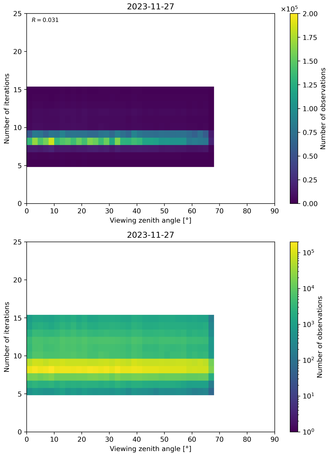
Figure 75: Scatter density plot of “Viewing zenith angle” against “Number of iterations” for 2023-11-26 to 2023-11-28.
