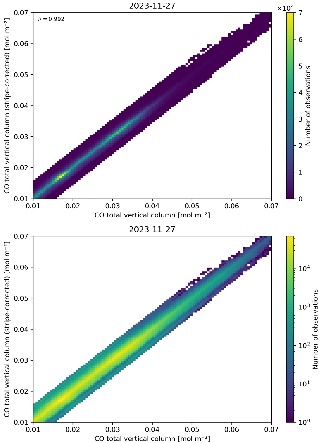
Figure 33: Scatter density plot of “CO total vertical column” against “CO total vertical column (stripe-corrected)” for 2023-11-26 to 2023-11-28.
