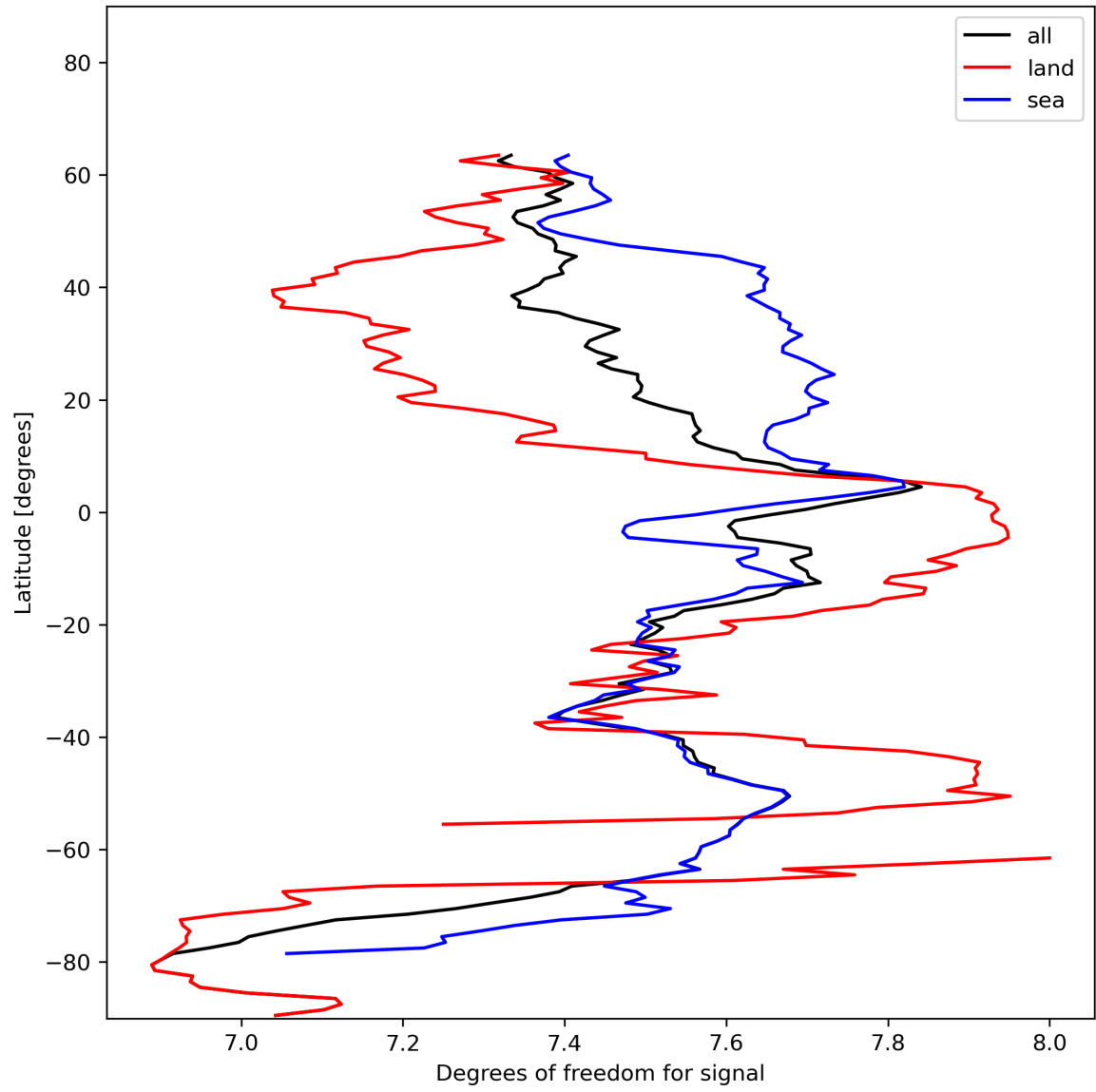
Figure 15: Zonal average of “Degrees of freedom for signal” for 2023-11-26 to 2023-11-28.
