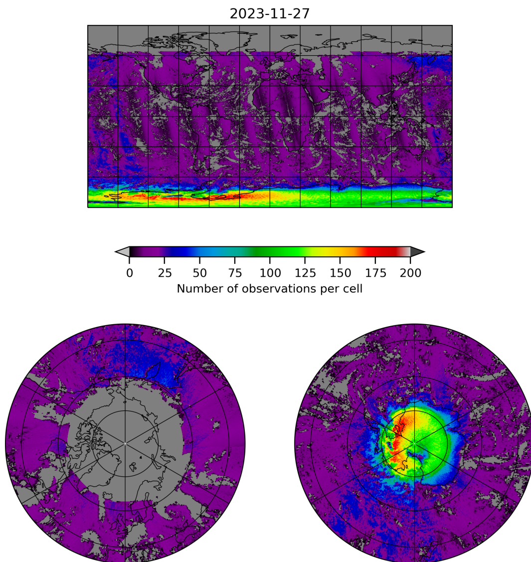
Figure 8: Map of the number of observations for 2023-11-26 to 2023-11-28
