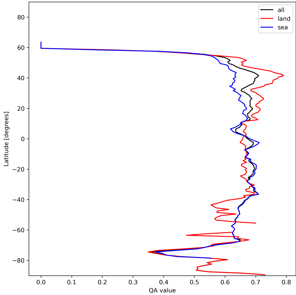
Figure 9: Zonal average of “QA value” for 2023-11-26 to 2023-11-28.
