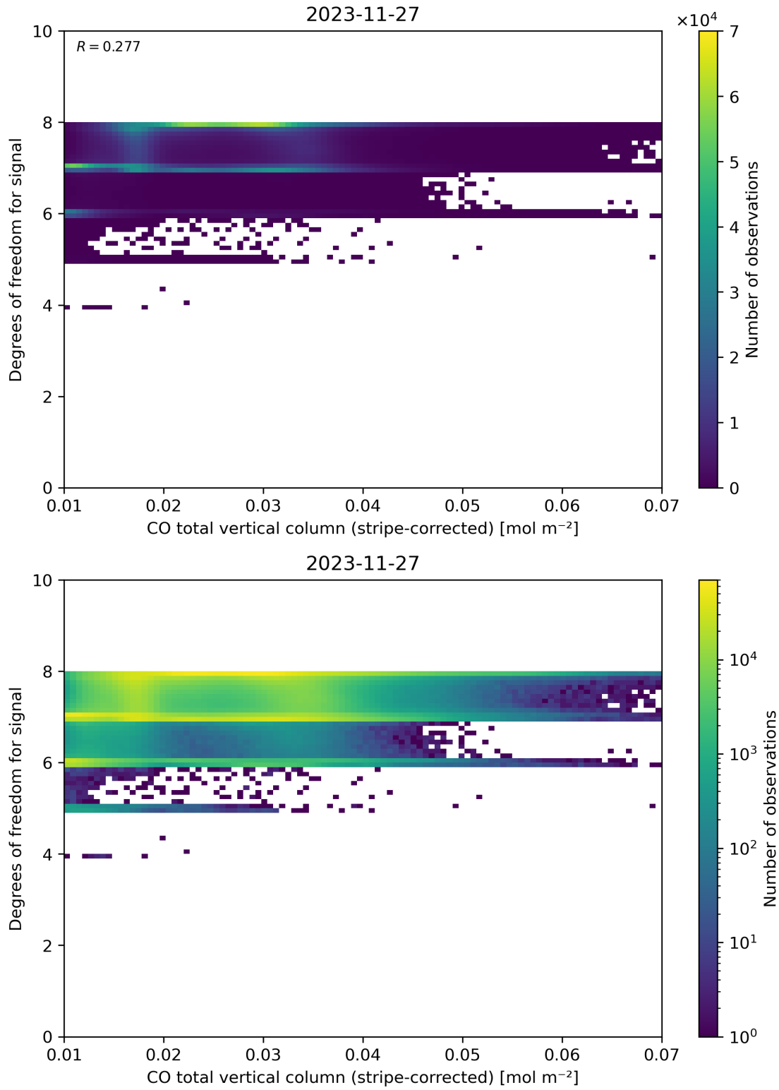
Figure 38: Scatter density plot of “CO total vertical column (stripe-corrected)” against “Degrees of freedom for signal” for 2023-11-26 to 2023-11-28.
