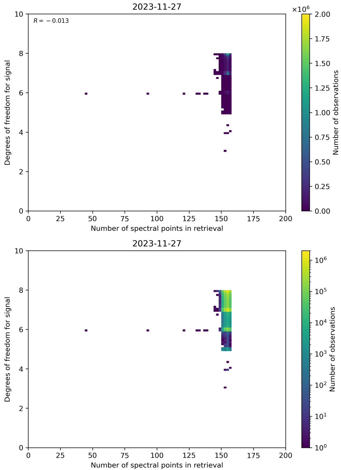
Figure 59: Scatter density plot of “Number of spectral points in retrieval” against “Degrees of freedom for signal” for 2023-11-26 to 2023-11-28.
