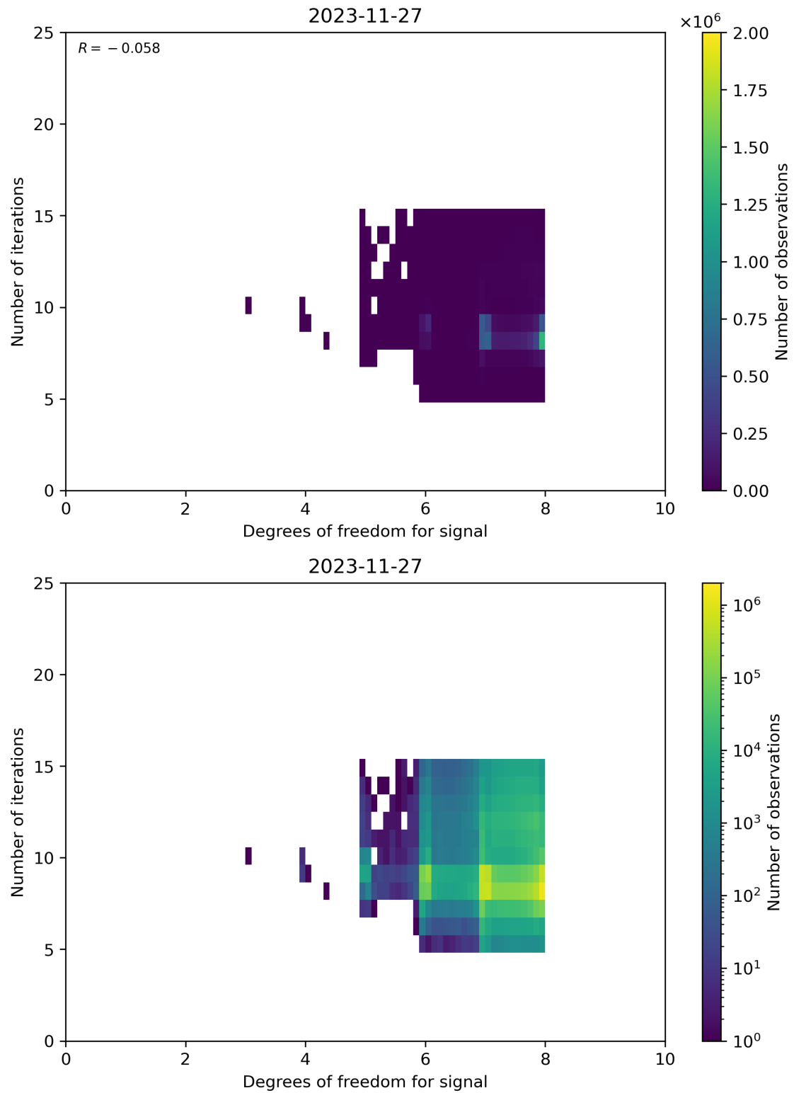
Figure 50: Scatter density plot of “Degrees of freedom for signal” against “Number of iterations” for 2023-11-26 to 2023-11-28.
