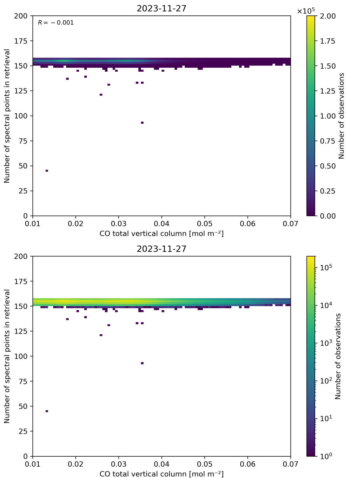
Figure 43: Scatter density plot of “CO total vertical column” against “Number of spectral points in retrieval” for 2023-11-26 to 2023-11-28.
