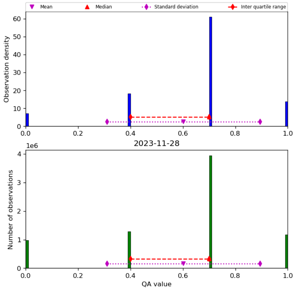
Figure 17: Histogram of “QA value” for 2023-11-28 to 2023-11-29
