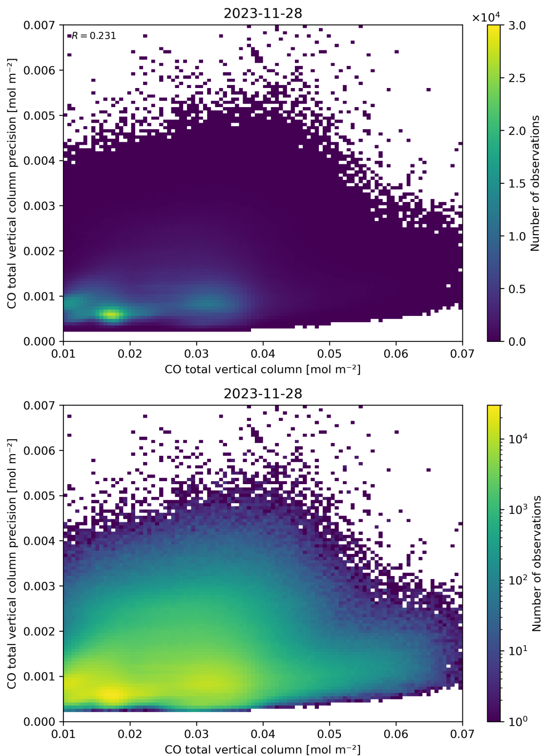
Figure 34: Scatter density plot of “CO total vertical column” against “CO total vertical column precision” for 2023-11-28 to 2023-11-29.
