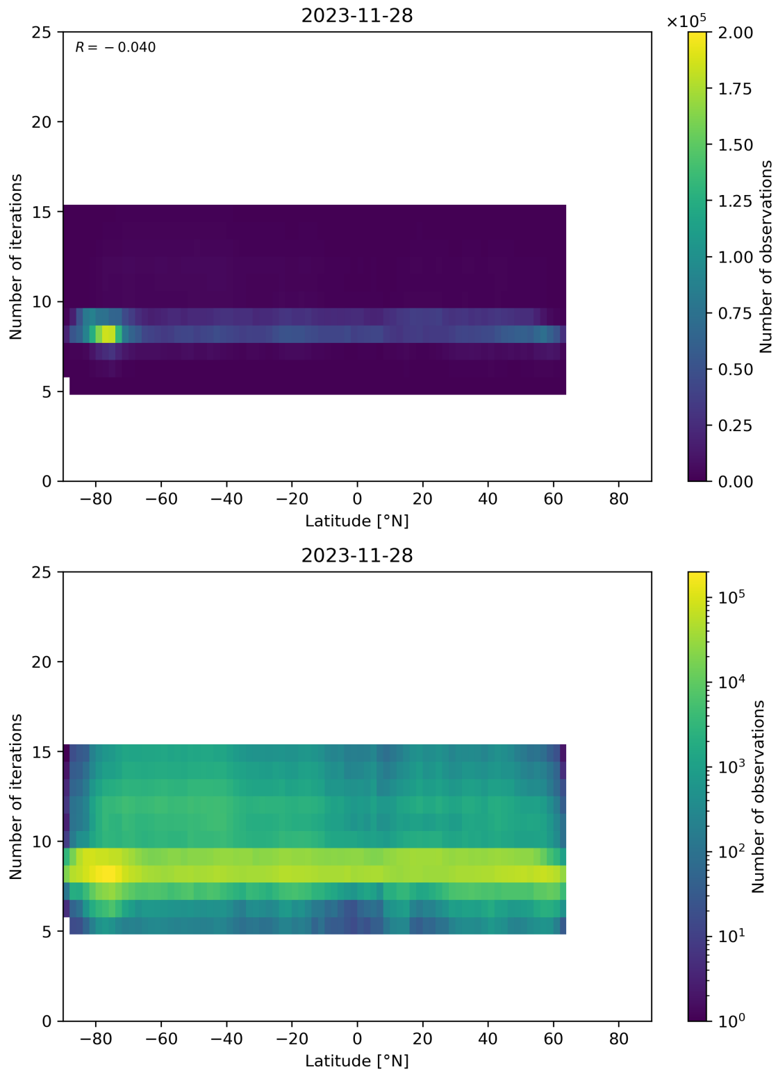
Figure 56: Scatter density plot of “Latitude” against “Number of iterations” for 2023-11-28 to 2023-11-29.
