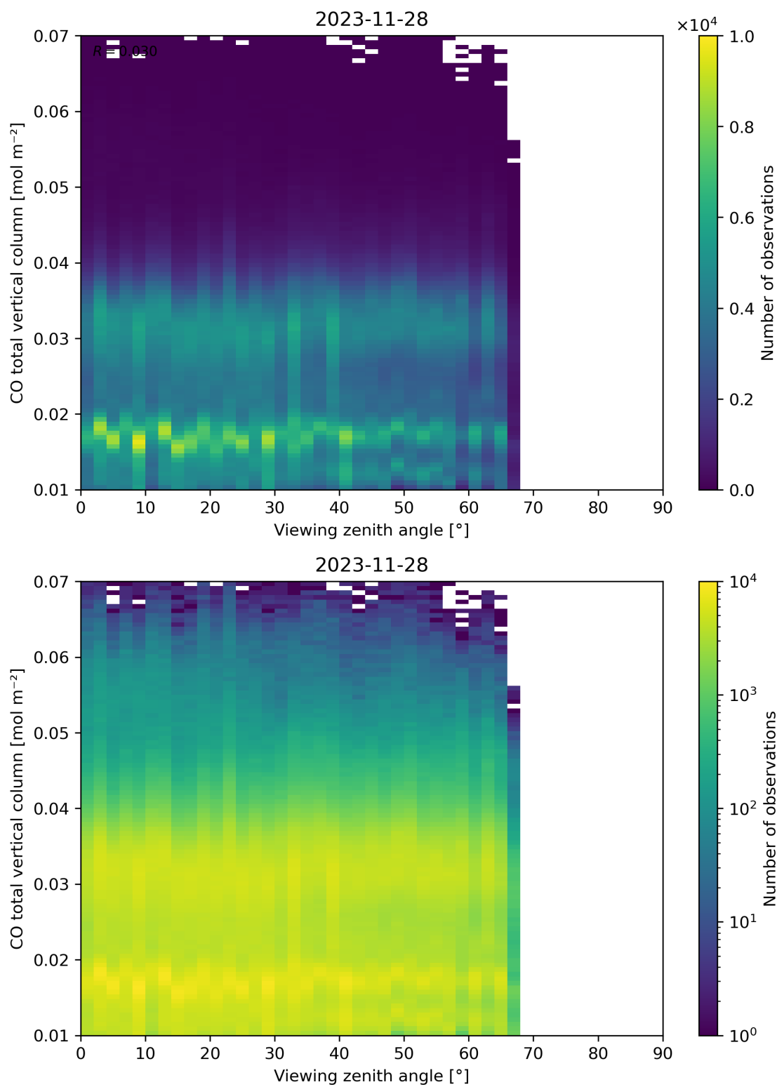
Figure 69: Scatter density plot of “Viewing zenith angle” against “CO total vertical column” for 2023-11-28 to 2023-11-29.
