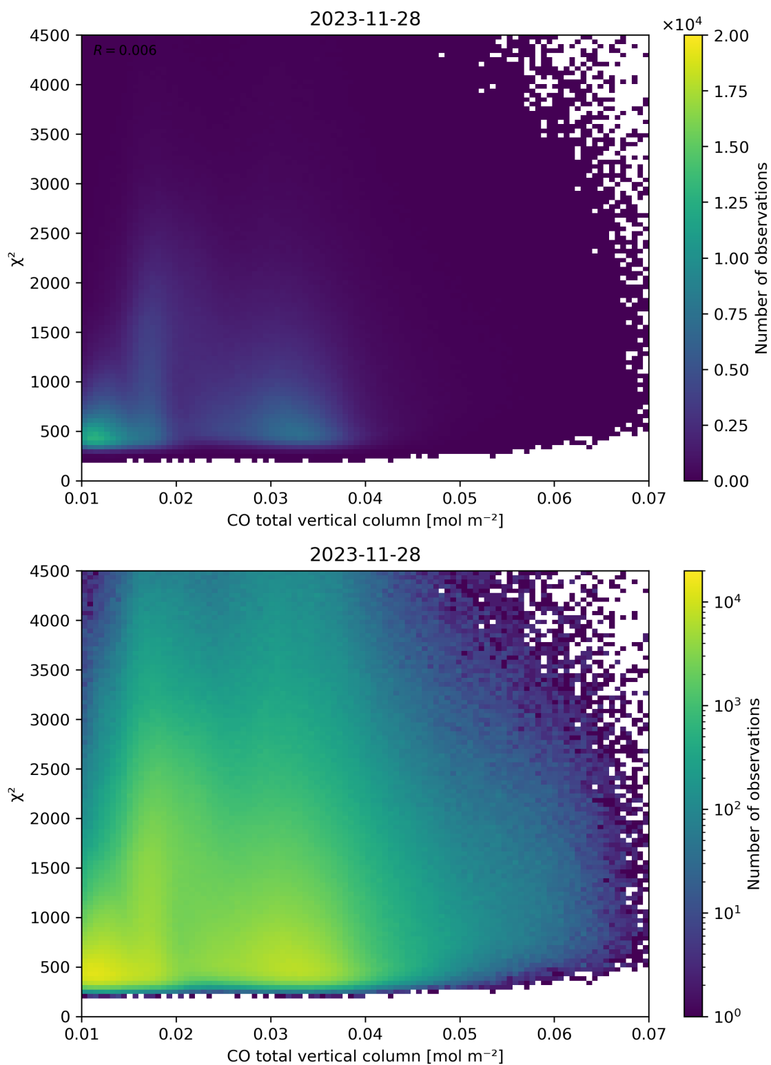
Figure 35: Scatter density plot of “CO total vertical column” against “ \chi^2 ” for 2023-11-28 to 2023-11-29.
