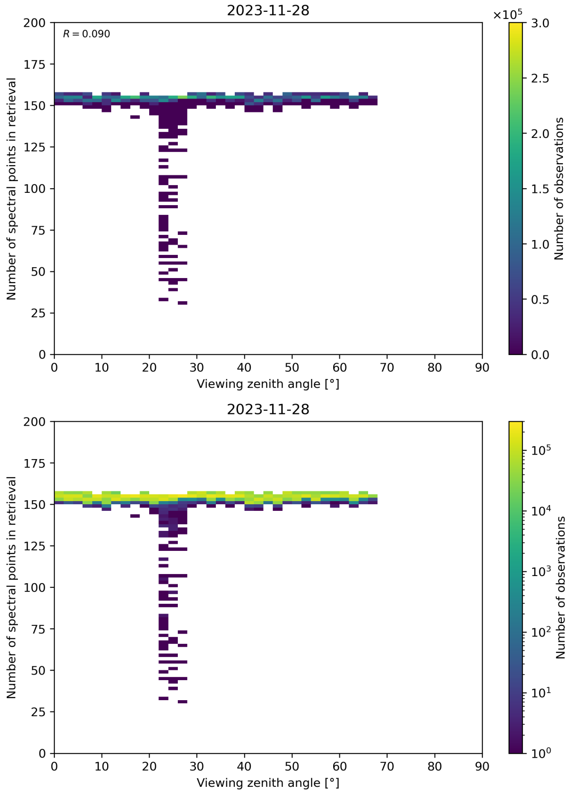
Figure 76: Scatter density plot of “Viewing zenith angle” against “Number of spectral points in retrieval” for 2023-11-28 to 2023-11-29.
