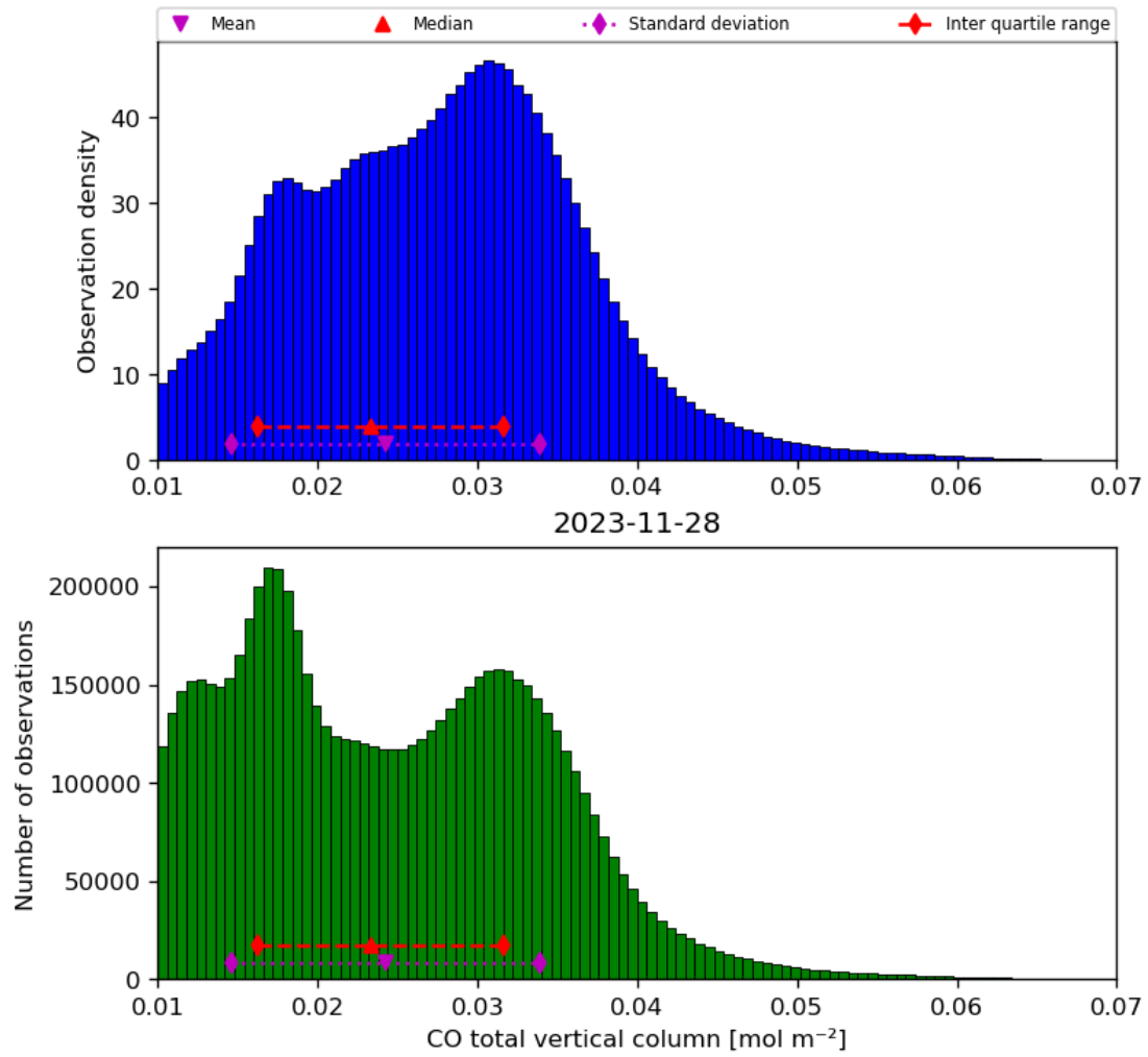
Figure 18: Histogram of “CO total vertical column” for 2023-11-28 to 2023-11-29
