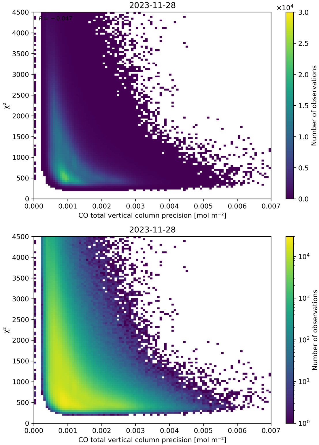
Figure 44: Scatter density plot of “CO total vertical column precision” against “ \chi^2 ” for 2023-11-28 to 2023-11-29.
