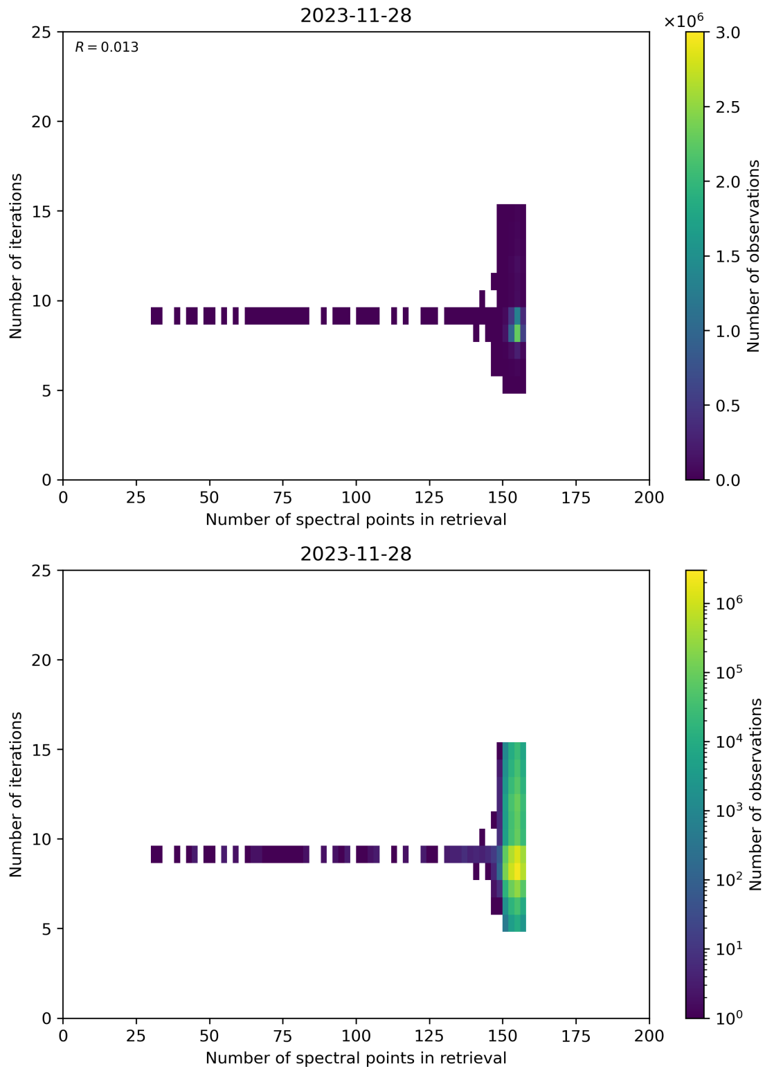
Figure 60: Scatter density plot of “Number of spectral points in retrieval” against “Number of iterations” for 2023-11-28 to 2023-11-29.
