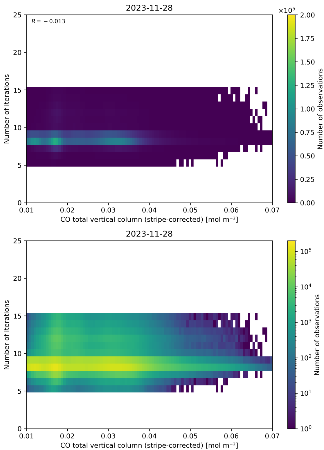
Figure 39: Scatter density plot of “CO total vertical column (stripe-corrected)” against “Number of iterations” for 2023-11-28 to 2023-11-29.
