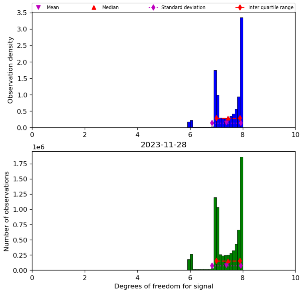
Figure 23: Histogram of “Degrees of freedom for signal” for 2023-11-28 to 2023-11-29
