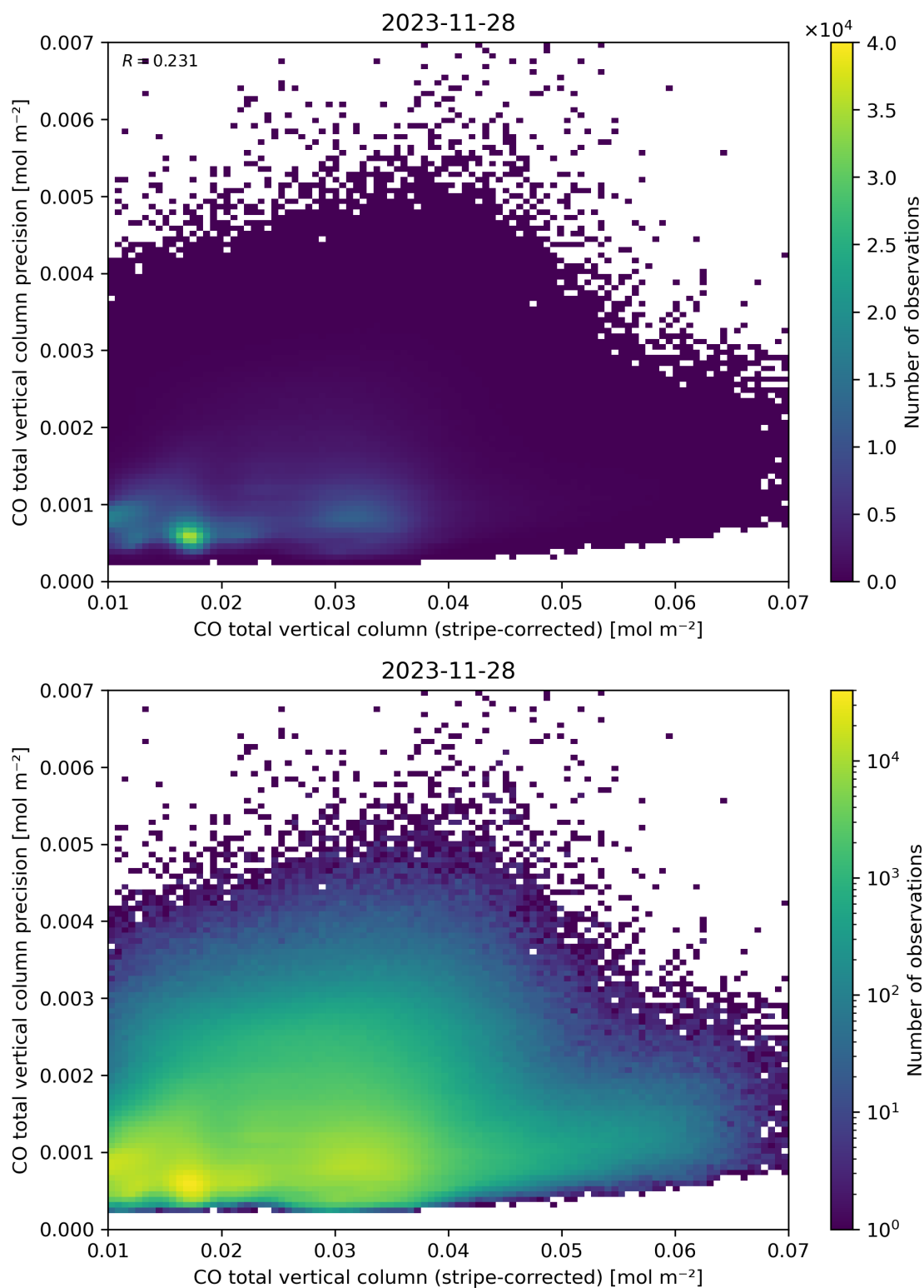
Figure 36: Scatter density plot of “CO total vertical column (stripe-corrected)” against “CO total vertical column precision” for 2023-11-28 to 2023-11-29.
