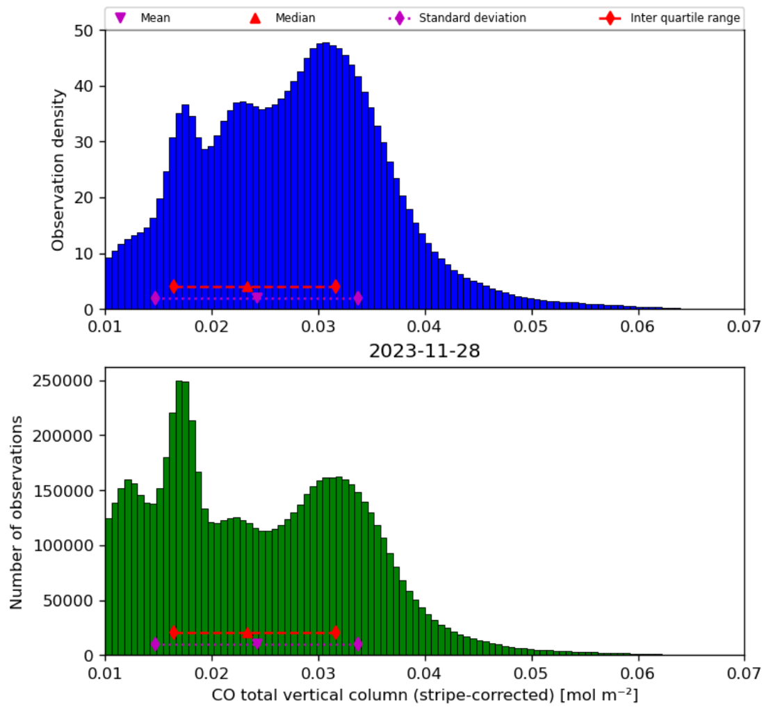
Figure 19: Histogram of “CO total vertical column (stripe-corrected)” for 2023-11-28 to 2023-11-29
