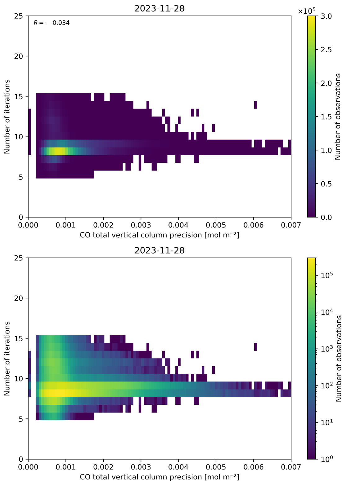
Figure 46: Scatter density plot of “CO total vertical column precision” against “Number of iterations” for 2023-11-28 to 2023-11-29.
