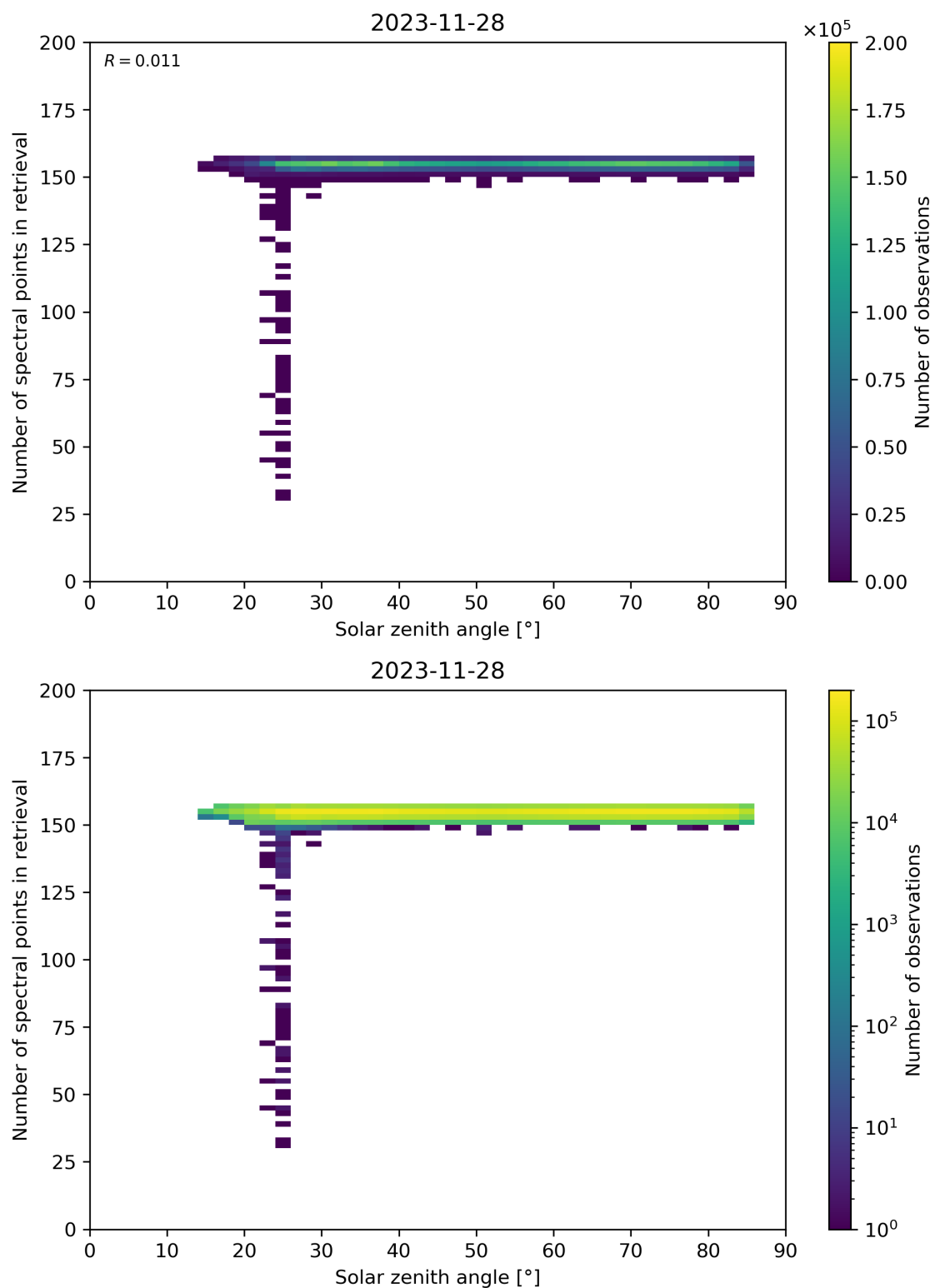
Figure 68: Scatter density plot of “Solar zenith angle” against “Number of spectral points in retrieval” for 2023-11-28 to 2023-11-29.
