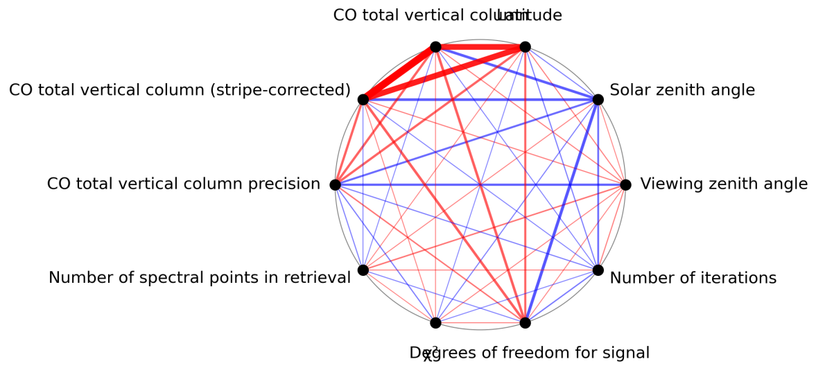
Figure 1: Map of correlation graph for 2023-11-28 to 2023-11-29.
