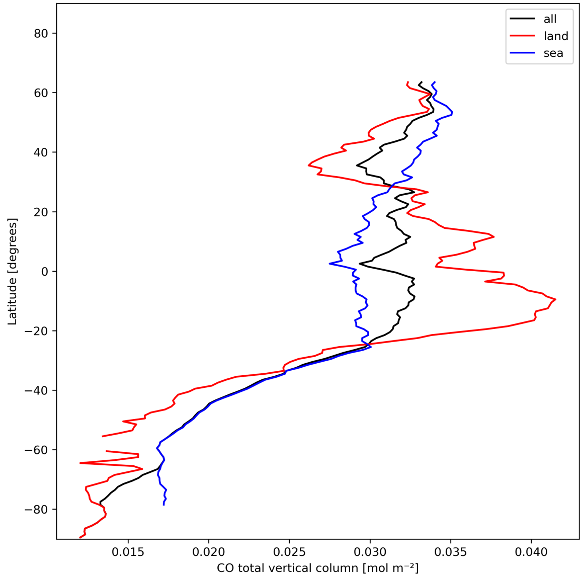
Figure 10: Zonal average of “CO total vertical column” for 2023-11-28 to 2023-11-29.
