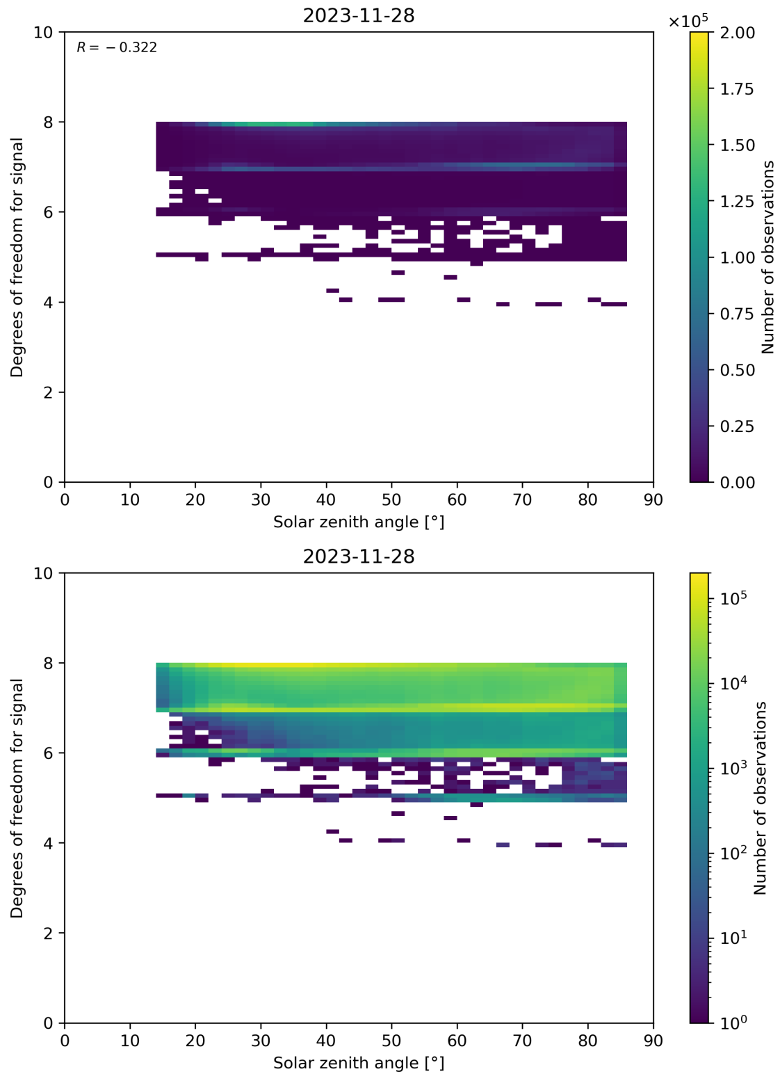
Figure 65: Scatter density plot of “Solar zenith angle” against “Degrees of freedom for signal” for 2023-11-28 to 2023-11-29.
