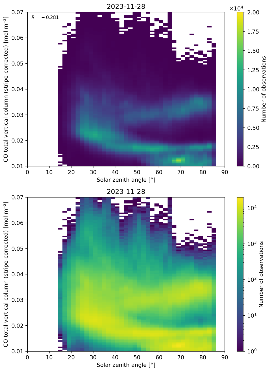
Figure 62: Scatter density plot of “Solar zenith angle” against “CO total vertical column (stripe-corrected)” for 2023-11-28 to 2023-11-29.
