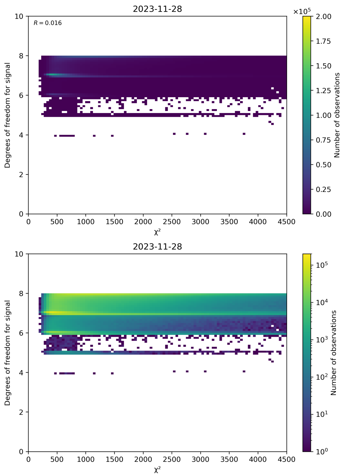
Figure 48: Scatter density plot of “ \chi^2 ” against “Degrees of freedom for signal” for 2023-11-28 to 2023-11-29.
