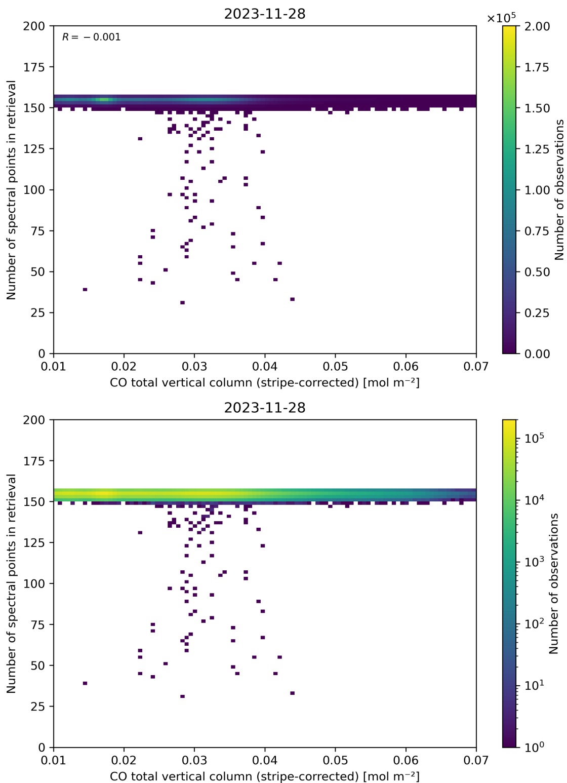
Figure 40: Scatter density plot of “CO total vertical column (stripe-corrected)” against “Number of spectral points in retrieval” for 2023-11-28 to 2023-11-29.
