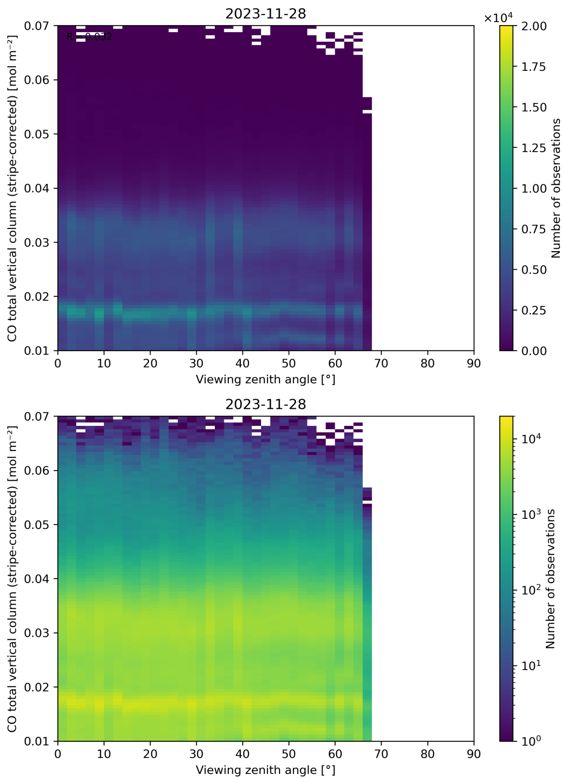
Figure 70: Scatter density plot of “Viewing zenith angle” against “CO total vertical column (stripe-corrected)” for 2023-11-28 to 2023-11-29.
