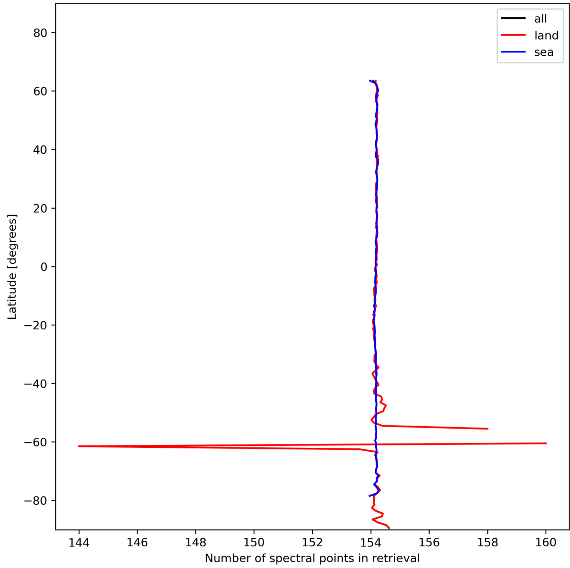
Figure 13: Zonal average of “Number of spectral points in retrieval” for 2023-11-28 to 2023-11-29.
