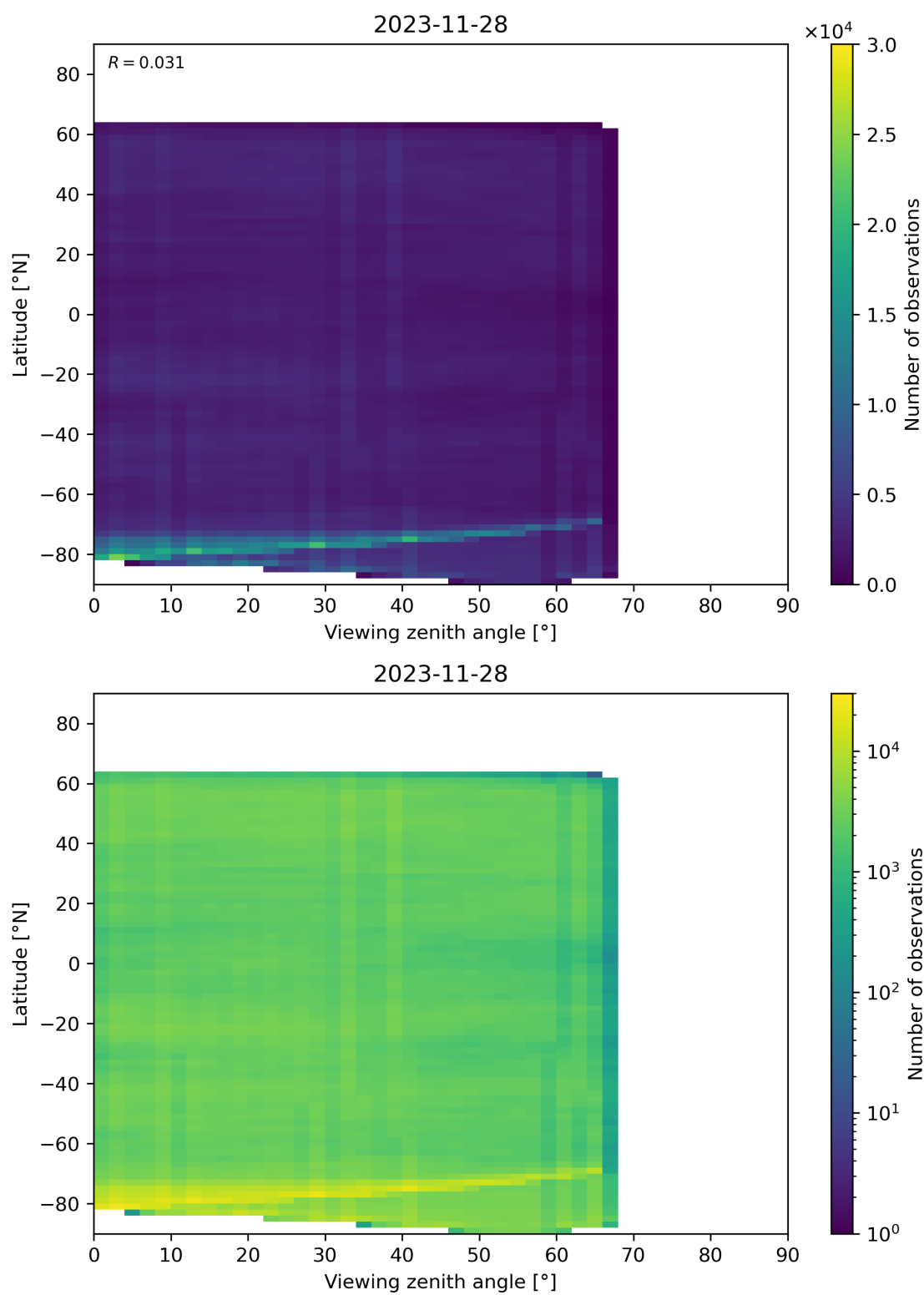
Figure 74: Scatter density plot of “Viewing zenith angle” against “Latitude” for 2023-11-28 to 2023-11-29.
