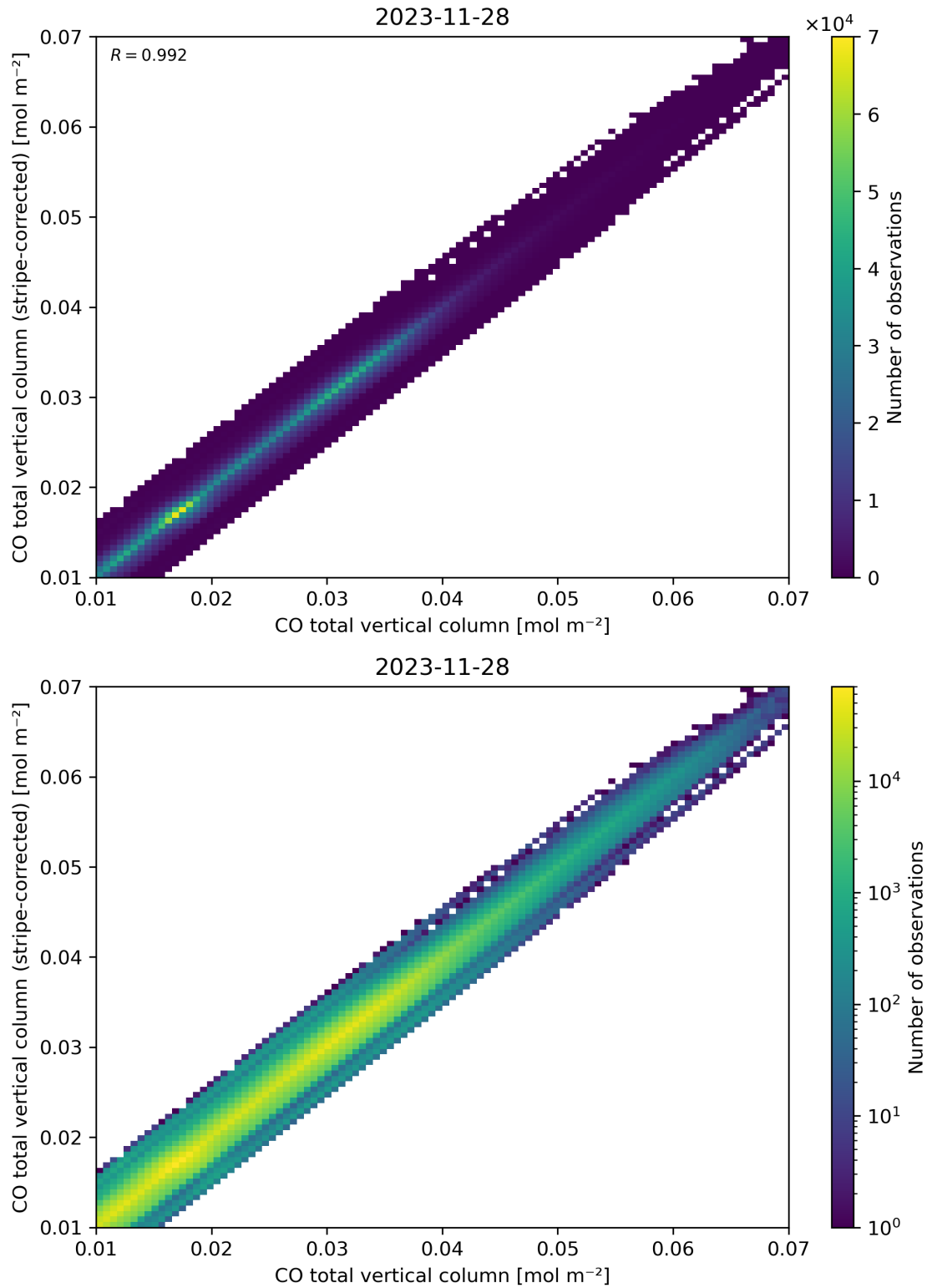
Figure 33: Scatter density plot of “CO total vertical column” against “CO total vertical column (stripe-corrected)” for 2023-11-28 to 2023-11-29.
