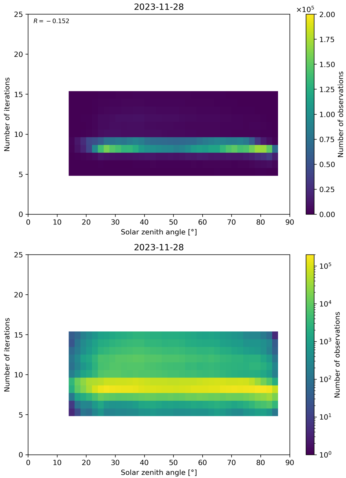
Figure 67: Scatter density plot of “Solar zenith angle” against “Number of iterations” for 2023-11-28 to 2023-11-29.
