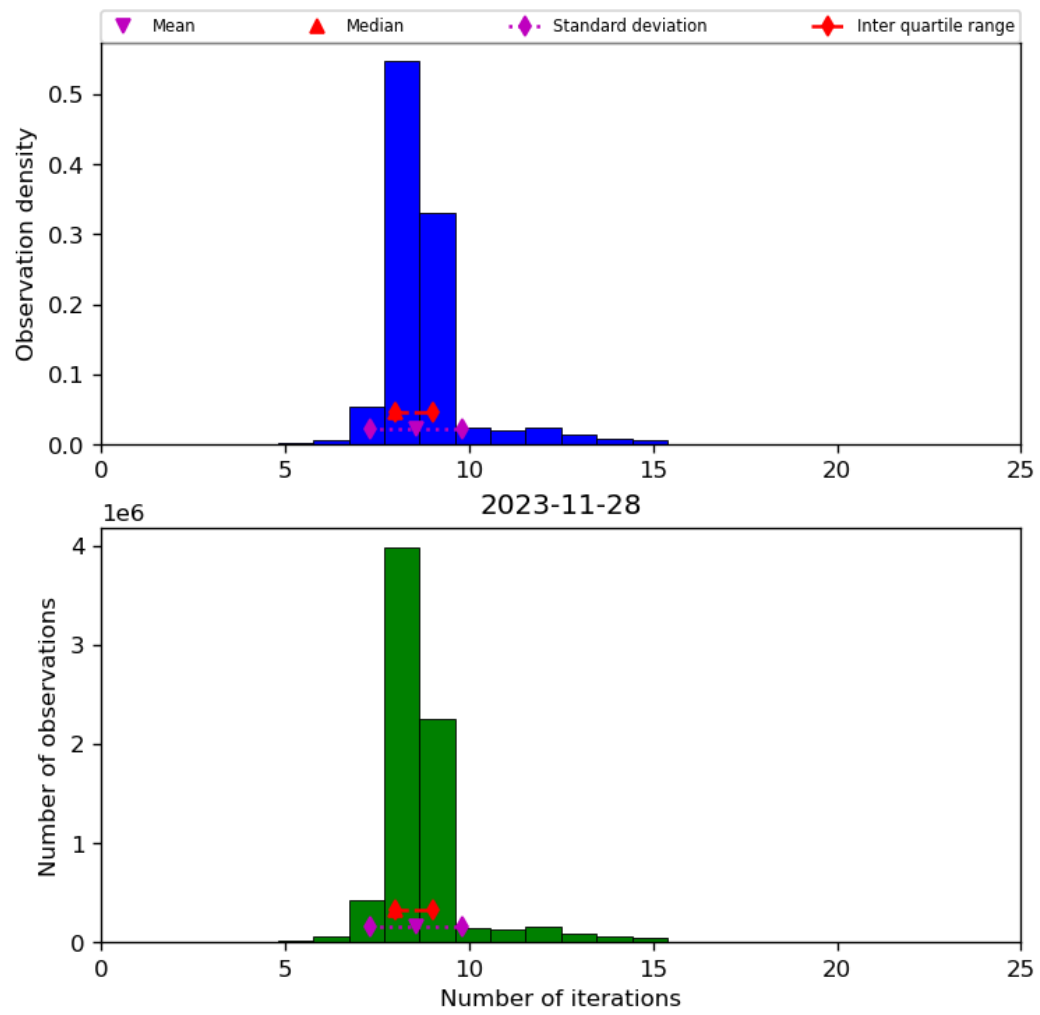
Figure 24: Histogram of “Number of iterations” for 2023-11-28 to 2023-11-29
