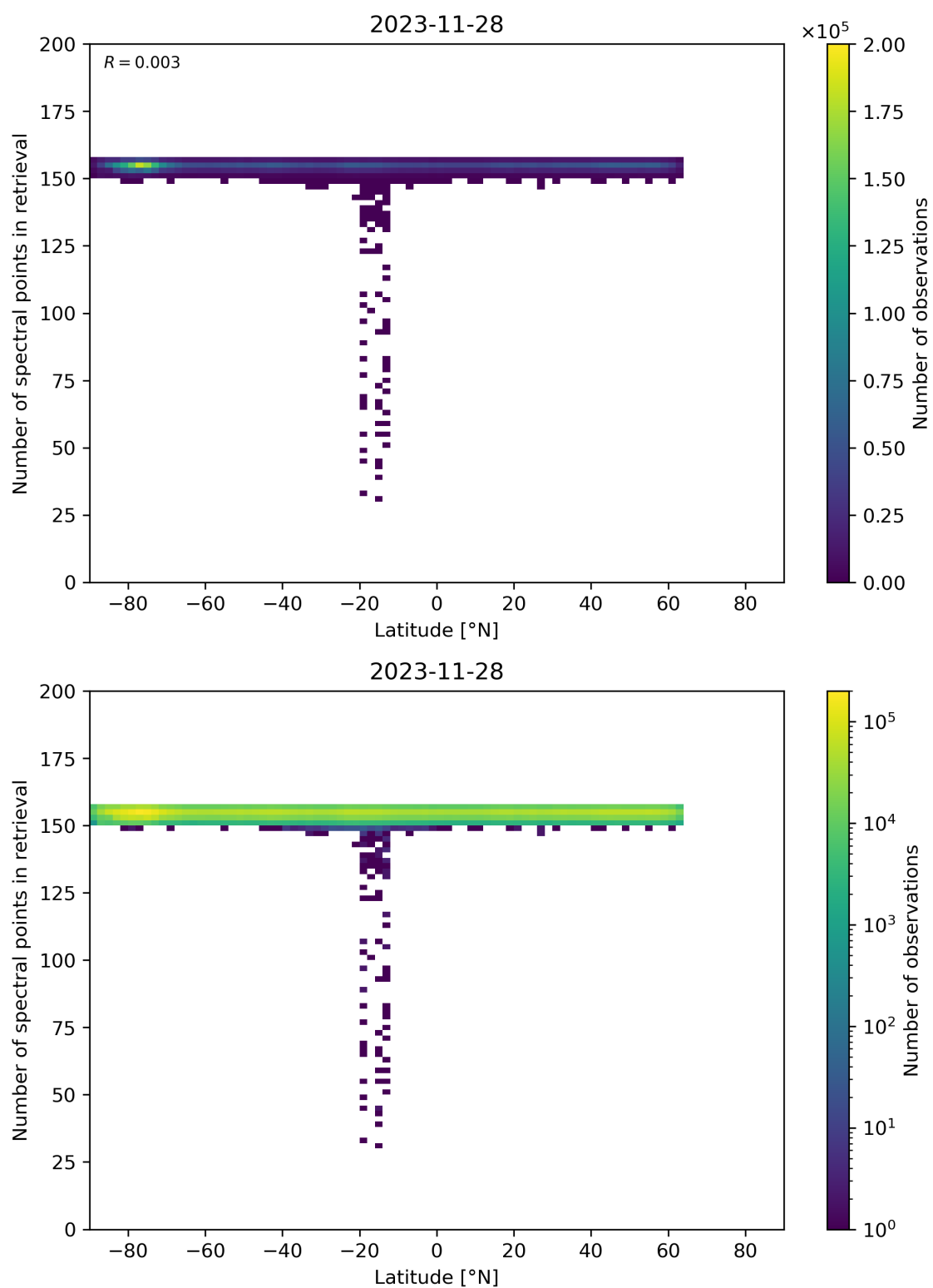
Figure 57: Scatter density plot of “Latitude” against “Number of spectral points in retrieval” for 2023-11-28 to 2023-11-29.
