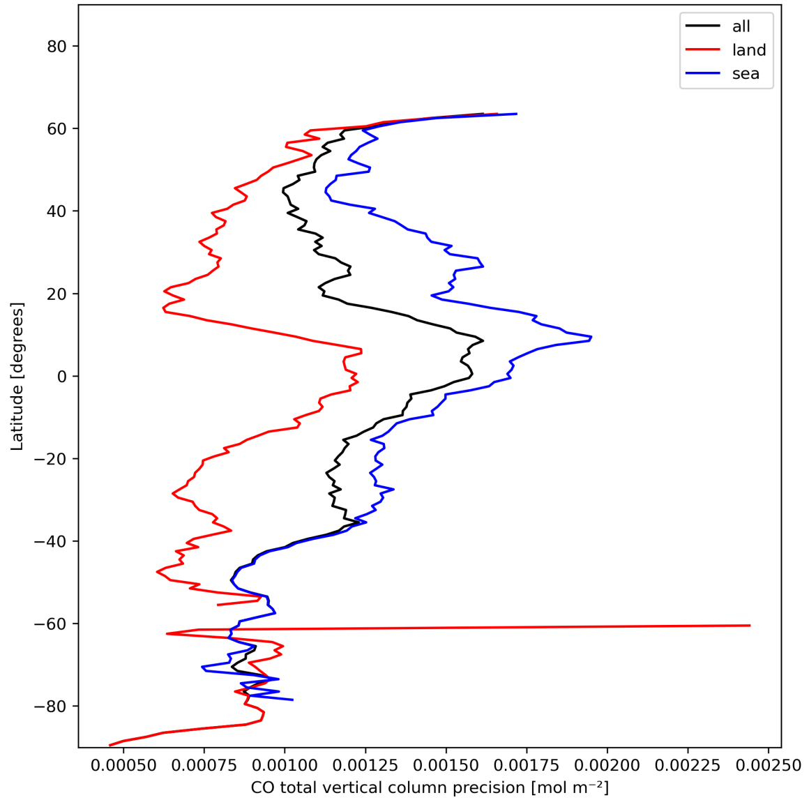
Figure 12: Zonal average of “CO total vertical column precision” for 2023-11-28 to 2023-11-29.
