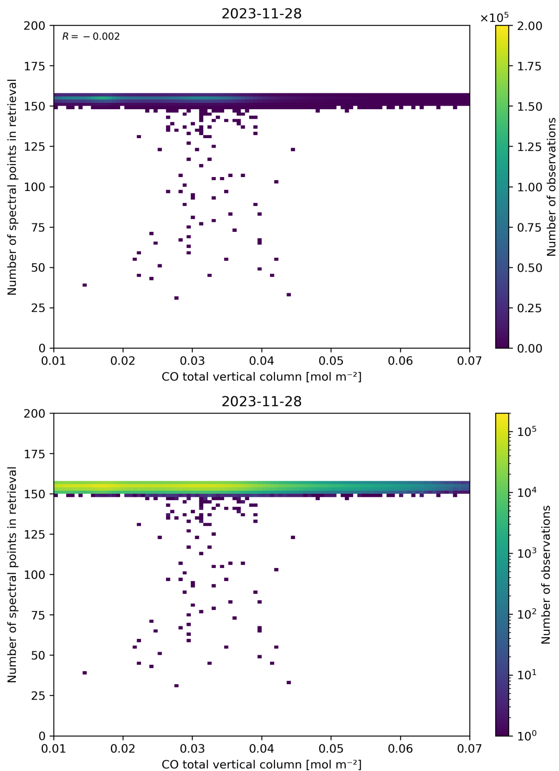
Figure 43: Scatter density plot of “CO total vertical column” against “Number of spectral points in retrieval” for 2023-11-28 to 2023-11-29.
