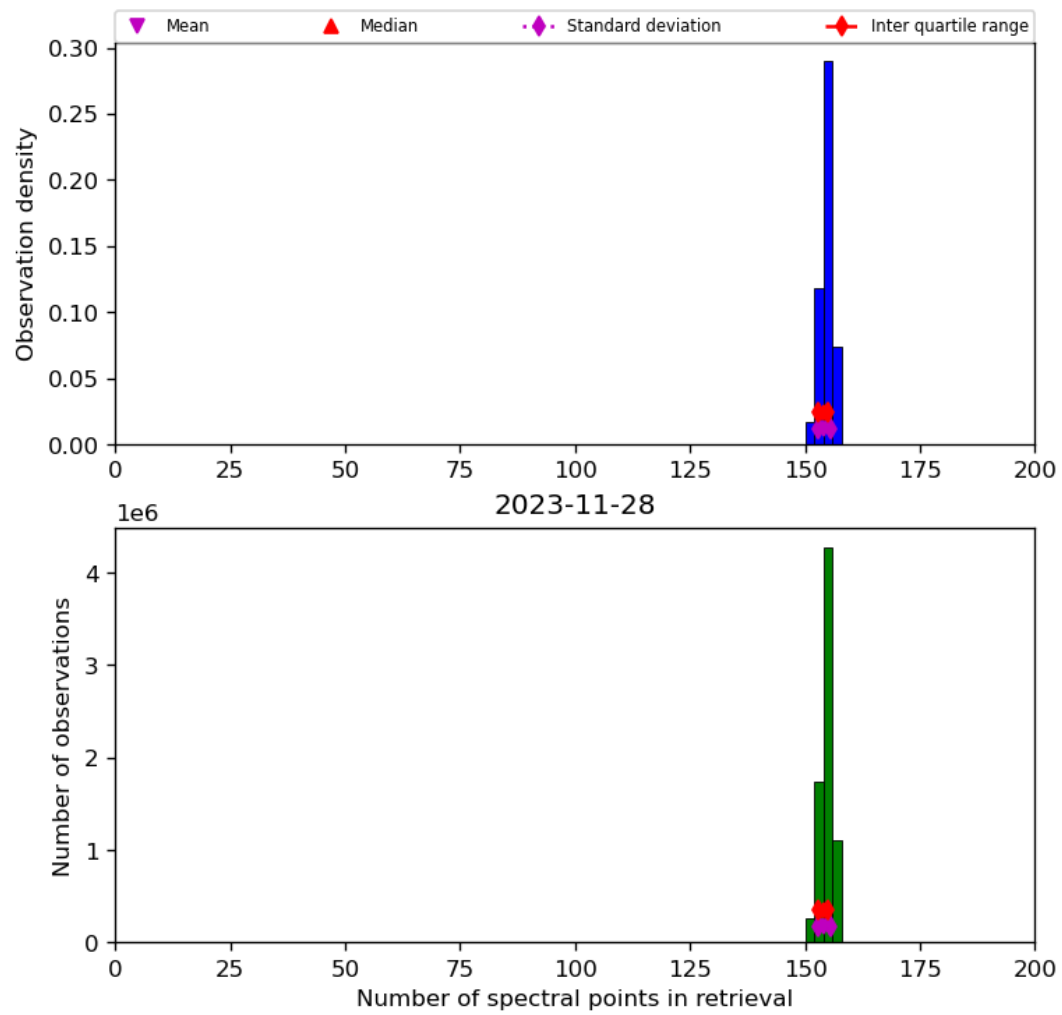
Figure 21: Histogram of “Number of spectral points in retrieval” for 2023-11-28 to 2023-11-29
