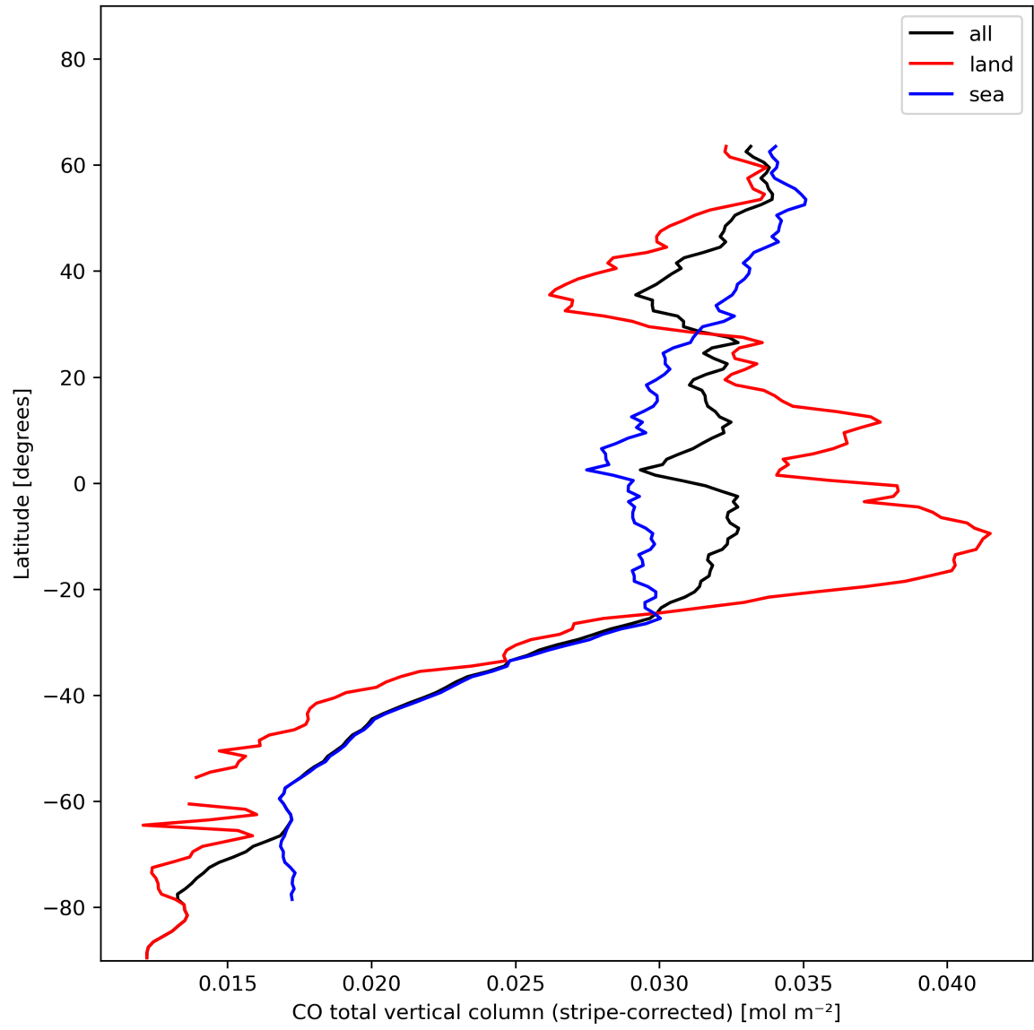
Figure 11: Zonal average of “CO total vertical column (stripe-corrected)” for 2023-11-28 to 2023-11-29.
