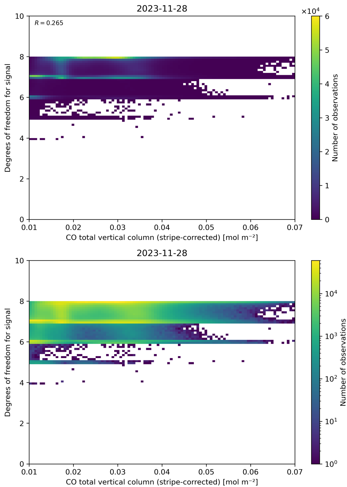
Figure 38: Scatter density plot of “CO total vertical column (stripe-corrected)” against “Degrees of freedom for signal” for 2023-11-28 to 2023-11-29.
