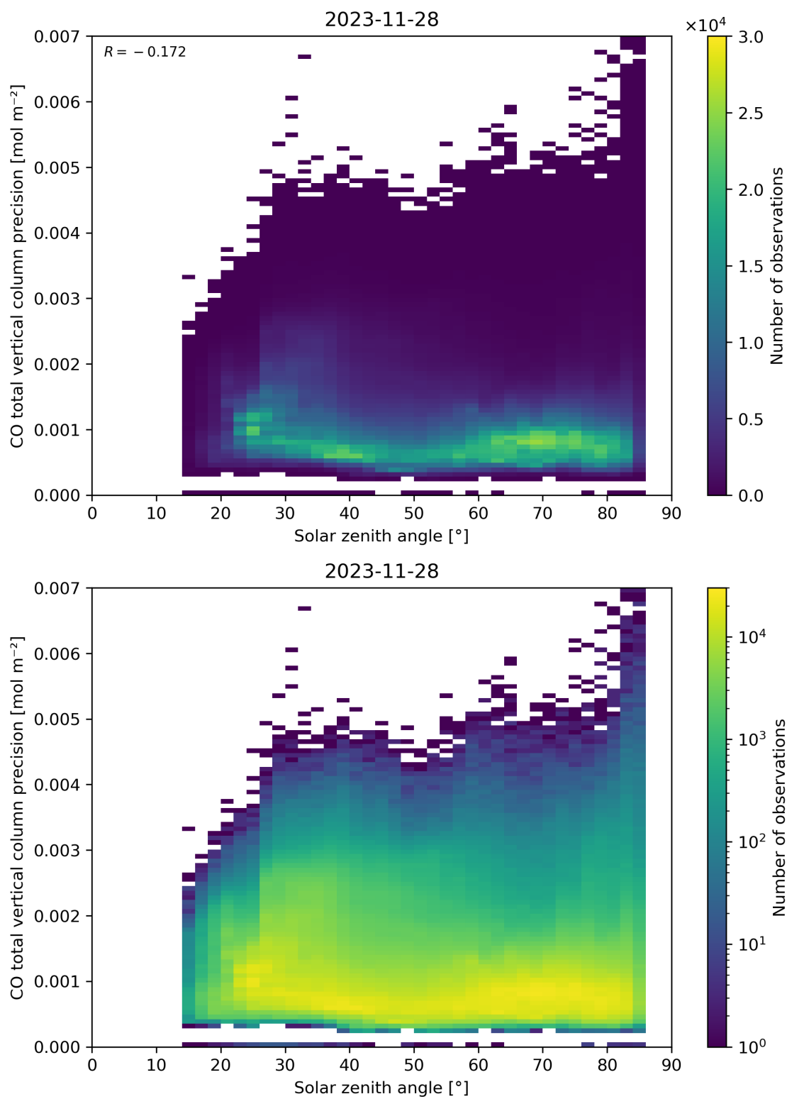
Figure 63: Scatter density plot of “Solar zenith angle” against “CO total vertical column precision” for 2023-11-28 to 2023-11-29.
