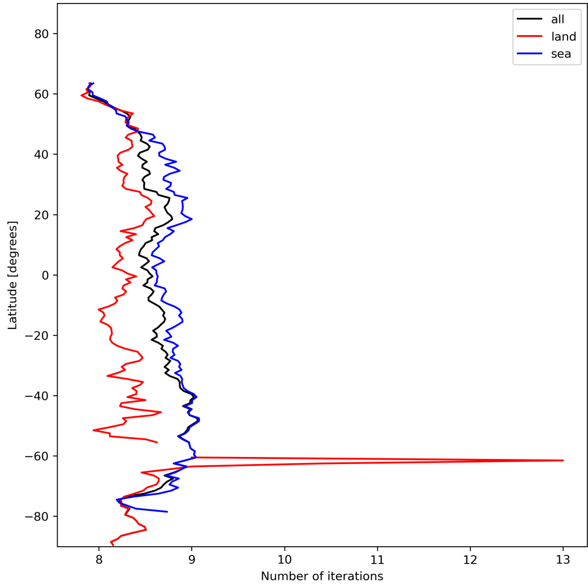
Figure 16: Zonal average of “Number of iterations” for 2023-11-28 to 2023-11-29.
