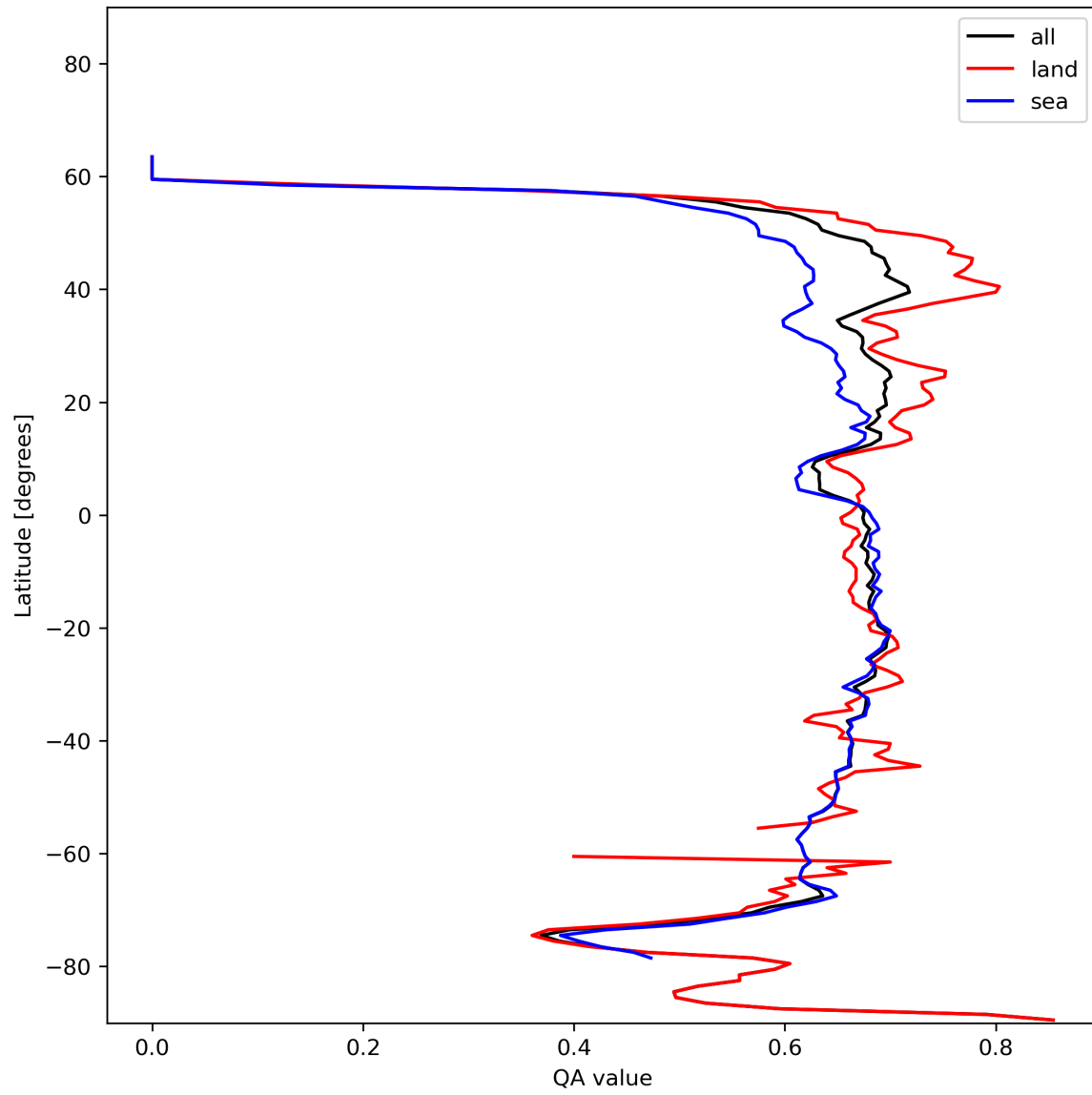
Figure 9: Zonal average of “QA value” for 2023-11-28 to 2023-11-29.
