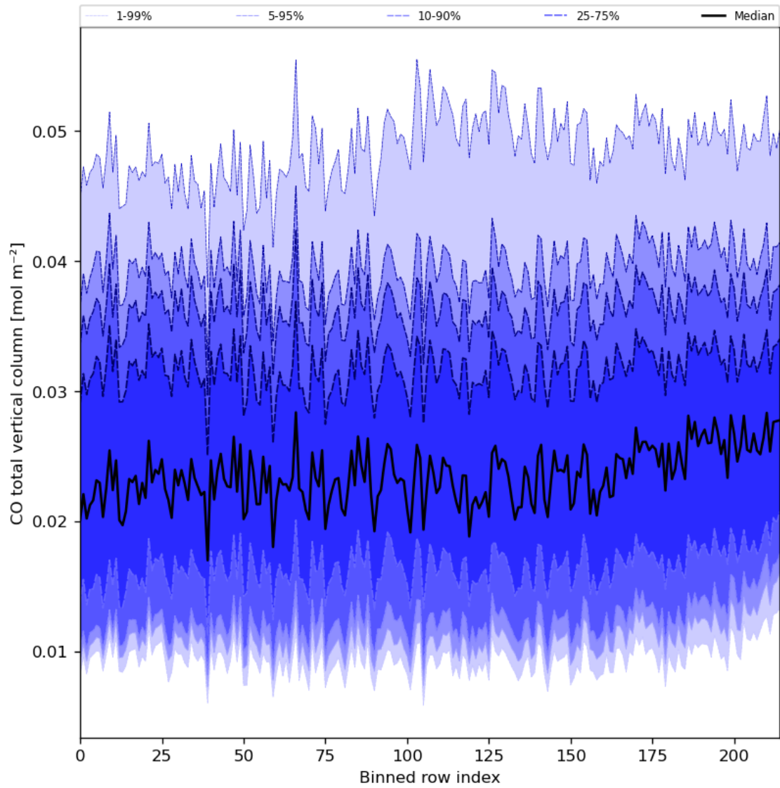
Figure 26: Along track statistics of “CO total vertical column” for 2023-11-28 to 2023-11-29
