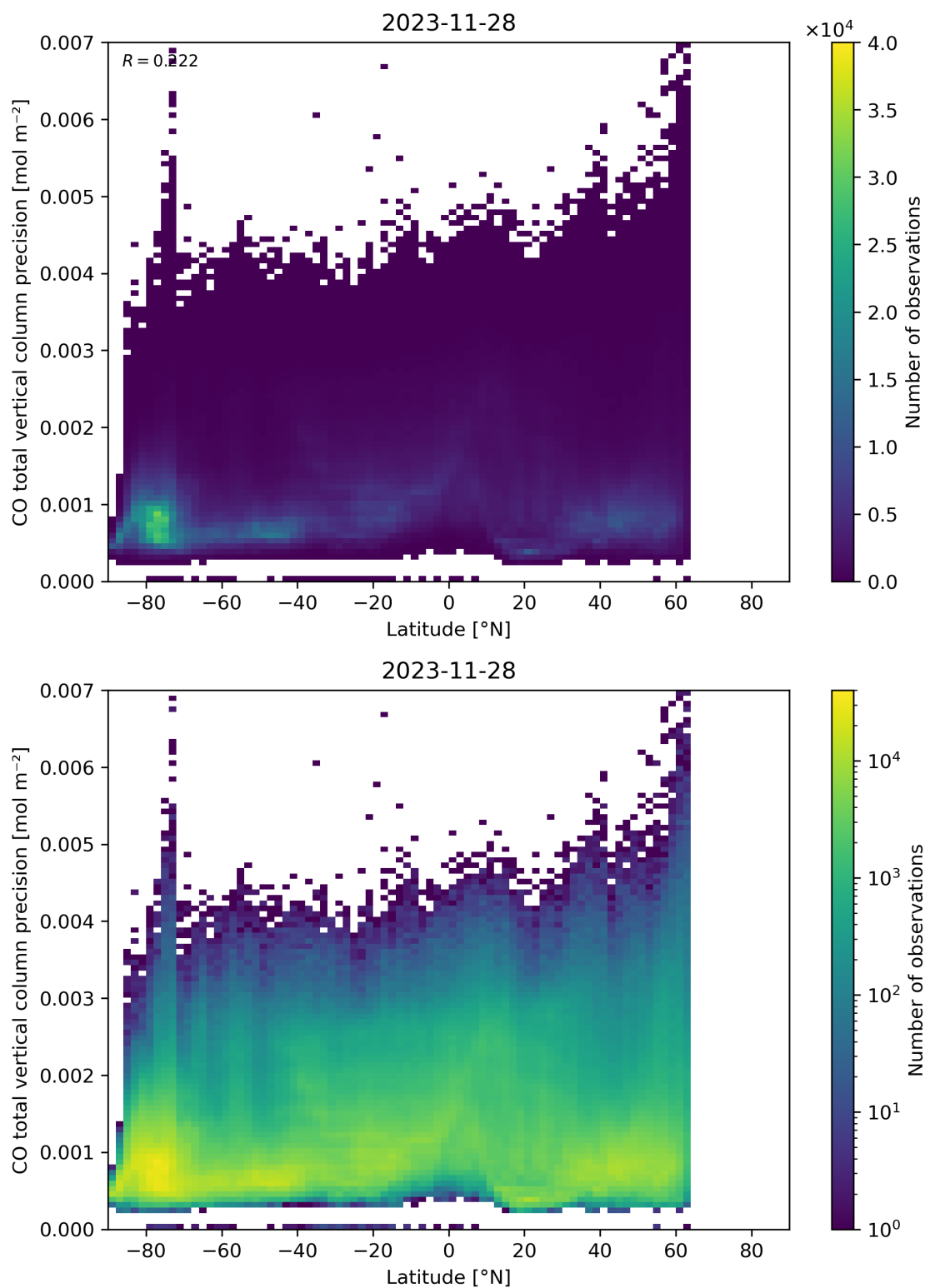
Figure 53: Scatter density plot of “Latitude” against “CO total vertical column precision” for 2023-11-28 to 2023-11-29.
