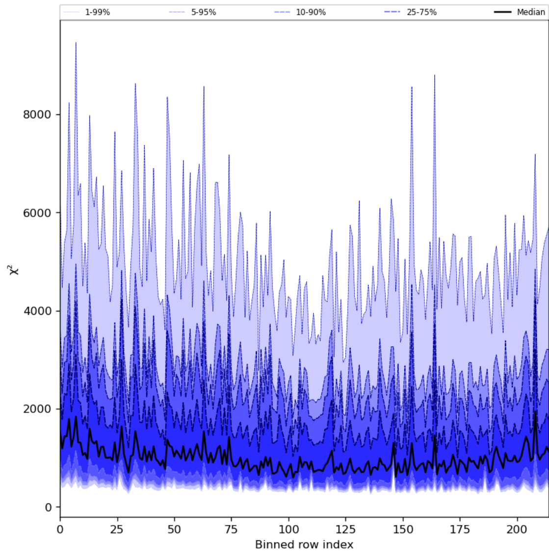
Figure 30: Along track statistics of “ \chi^2 ” for 2023-11-28 to 2023-11-29
