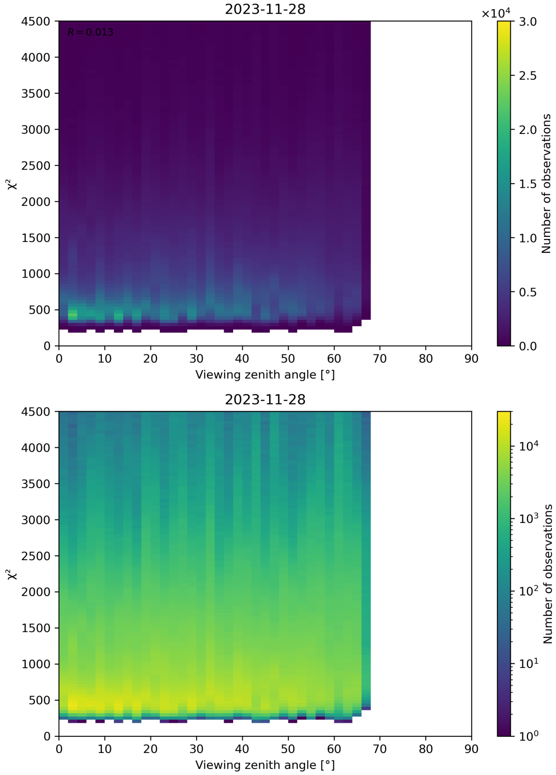
Figure 72: Scatter density plot of “Viewing zenith angle” against “ \chi^2 ” for 2023-11-28 to 2023-11-29.
