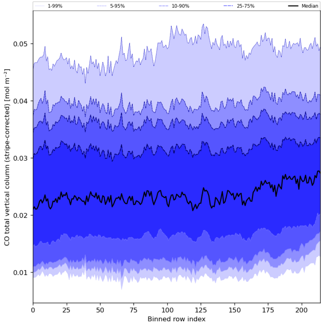
Figure 27: Along track statistics of “CO total vertical column (stripe-corrected)” for 2023-11-28 to 2023-11-29
