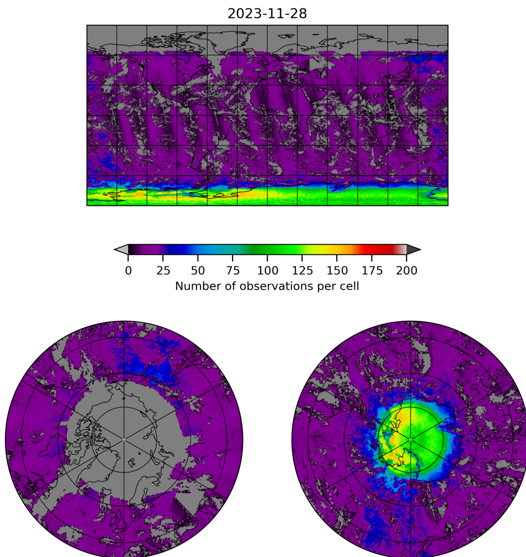
Figure 8: Map of the number of observations for 2023-11-28 to 2023-11-29
