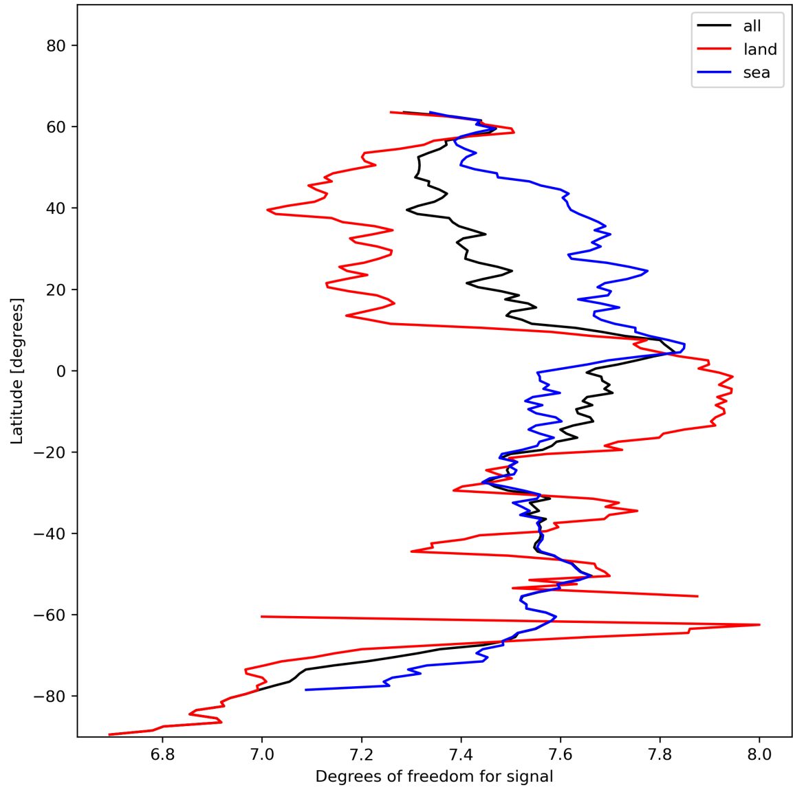
Figure 15: Zonal average of “Degrees of freedom for signal” for 2023-11-28 to 2023-11-29.
