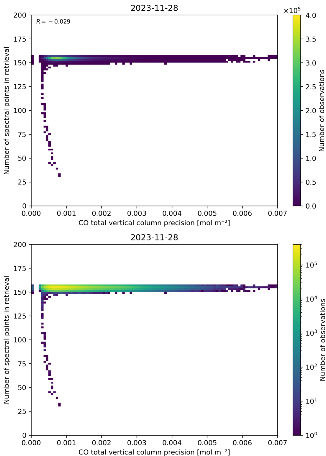
Figure 47: Scatter density plot of “CO total vertical column precision” against “Number of spectral points in retrieval” for 2023-11-28 to 2023-11-29.
