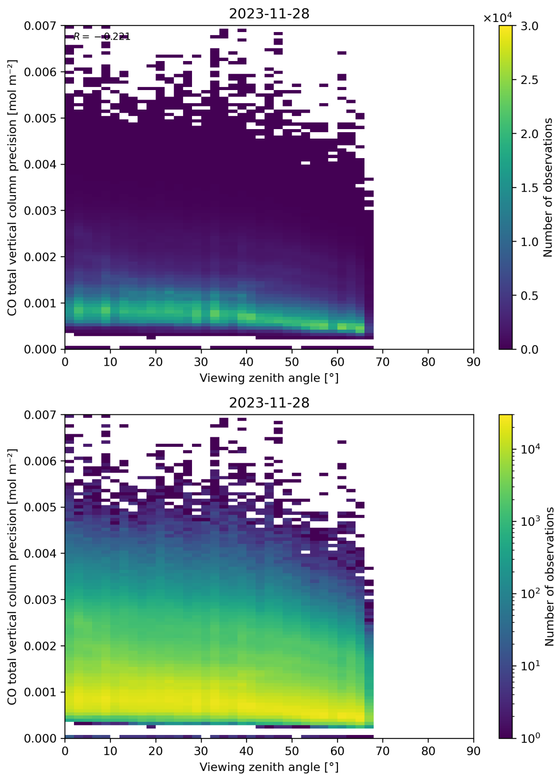
Figure 71: Scatter density plot of “Viewing zenith angle” against “CO total vertical column precision” for 2023-11-28 to 2023-11-29.
