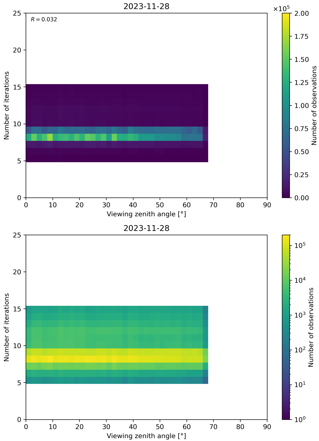
Figure 75: Scatter density plot of “Viewing zenith angle” against “Number of iterations” for 2023-11-28 to 2023-11-29.
