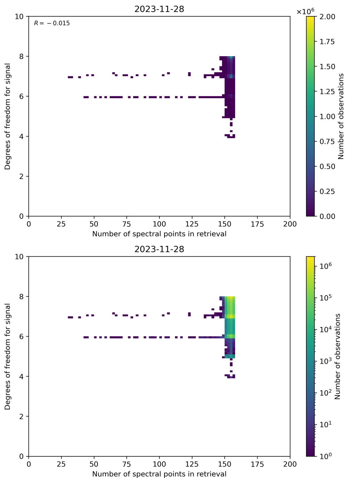
Figure 59: Scatter density plot of “Number of spectral points in retrieval” against “Degrees of freedom for signal” for 2023-11-28 to 2023-11-29.
