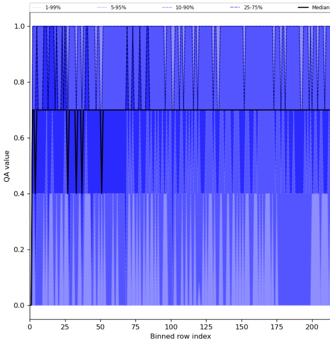
Figure 25: Along track statistics of “QA value” for 2023-11-28 to 2023-11-29
