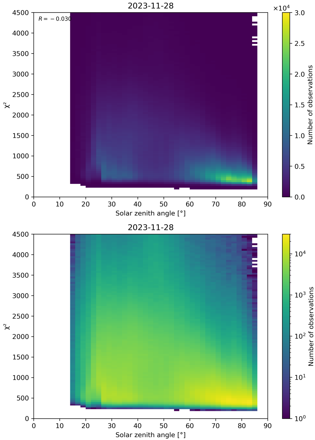
Figure 64: Scatter density plot of “Solar zenith angle” against “ \chi^2 ” for 2023-11-28 to 2023-11-29.
