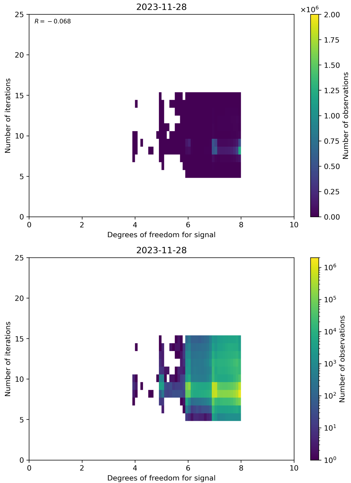
Figure 50: Scatter density plot of “Degrees of freedom for signal” against “Number of iterations” for 2023-11-28 to 2023-11-29.
