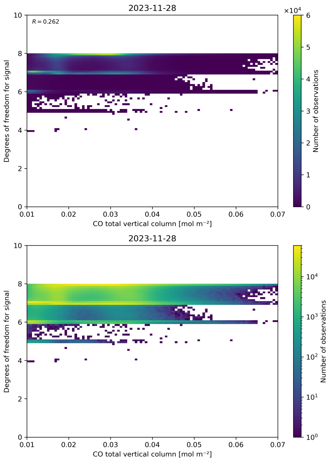
Figure 41: Scatter density plot of “CO total vertical column” against “Degrees of freedom for signal” for 2023-11-28 to 2023-11-29.
