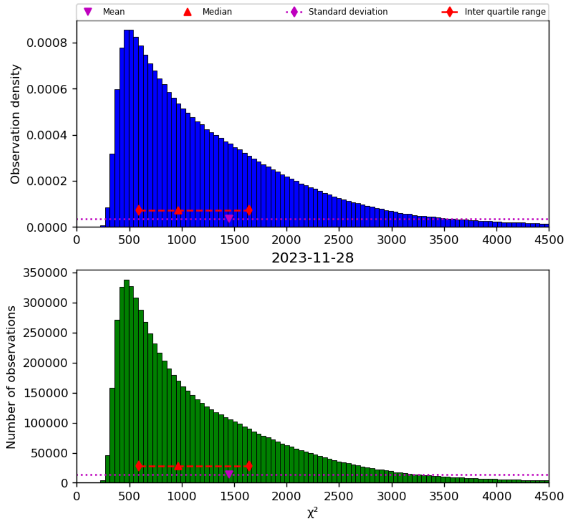
Figure 22: Histogram of “ \chi^2 ” for 2023-11-28 to 2023-11-29
