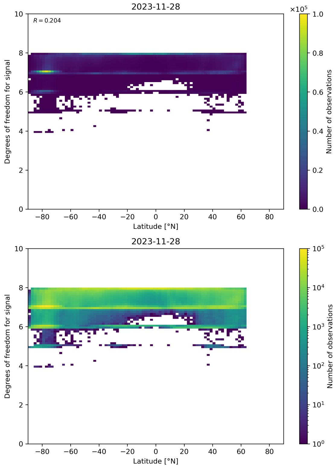
Figure 55: Scatter density plot of “Latitude” against “Degrees of freedom for signal” for 2023-11-28 to 2023-11-29.
