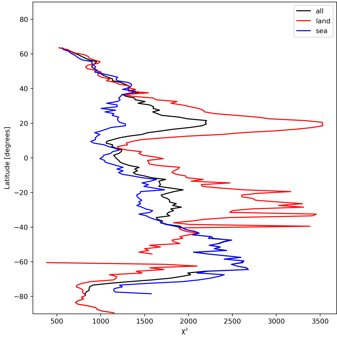
Figure 14: Zonal average of “ \chi^2 ” for 2023-11-28 to 2023-11-29.
