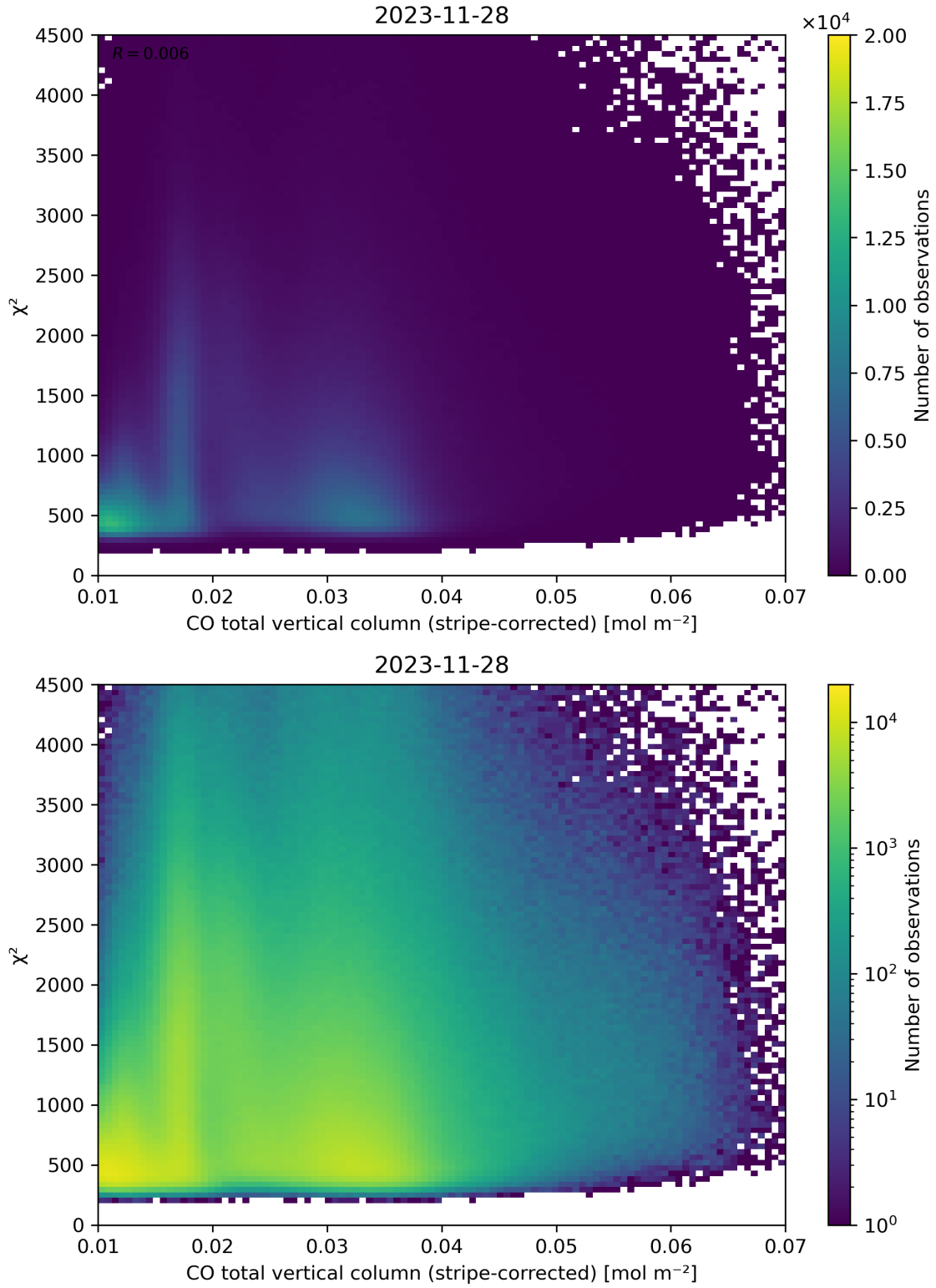
Figure 37: Scatter density plot of “CO total vertical column (stripe-corrected)” against “ \chi^2 ” for 2023-11-28 to 2023-11-29.
