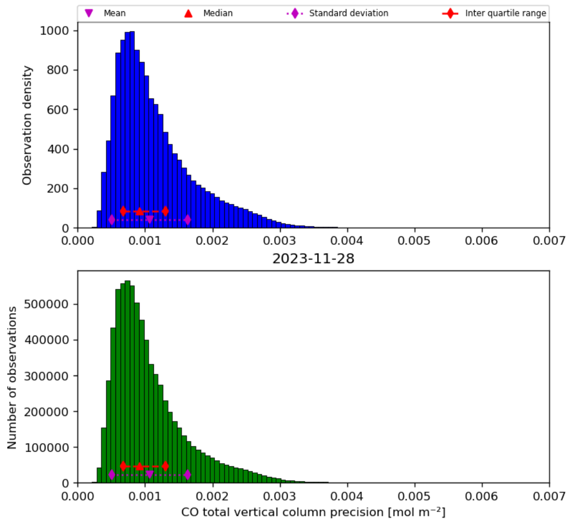
Figure 20: Histogram of “CO total vertical column precision” for 2023-11-28 to 2023-11-29
