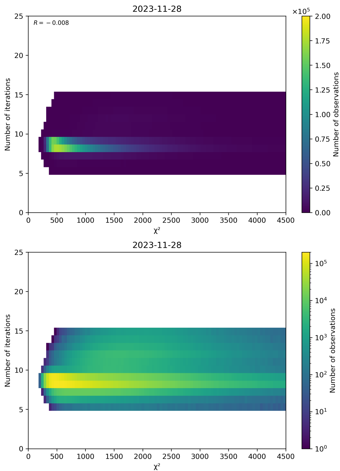
Figure 49: Scatter density plot of “ \chi^2 ” against “Number of iterations” for 2023-11-28 to 2023-11-29.
