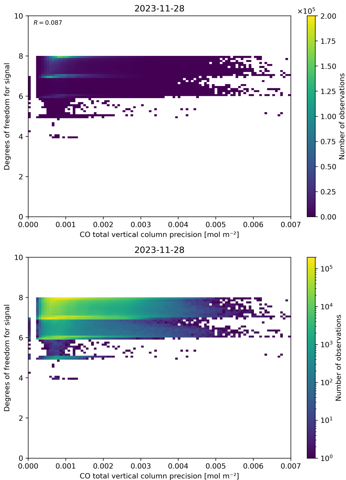
Figure 45: Scatter density plot of “CO total vertical column precision” against “Degrees of freedom for signal” for 2023-11-28 to 2023-11-29.
