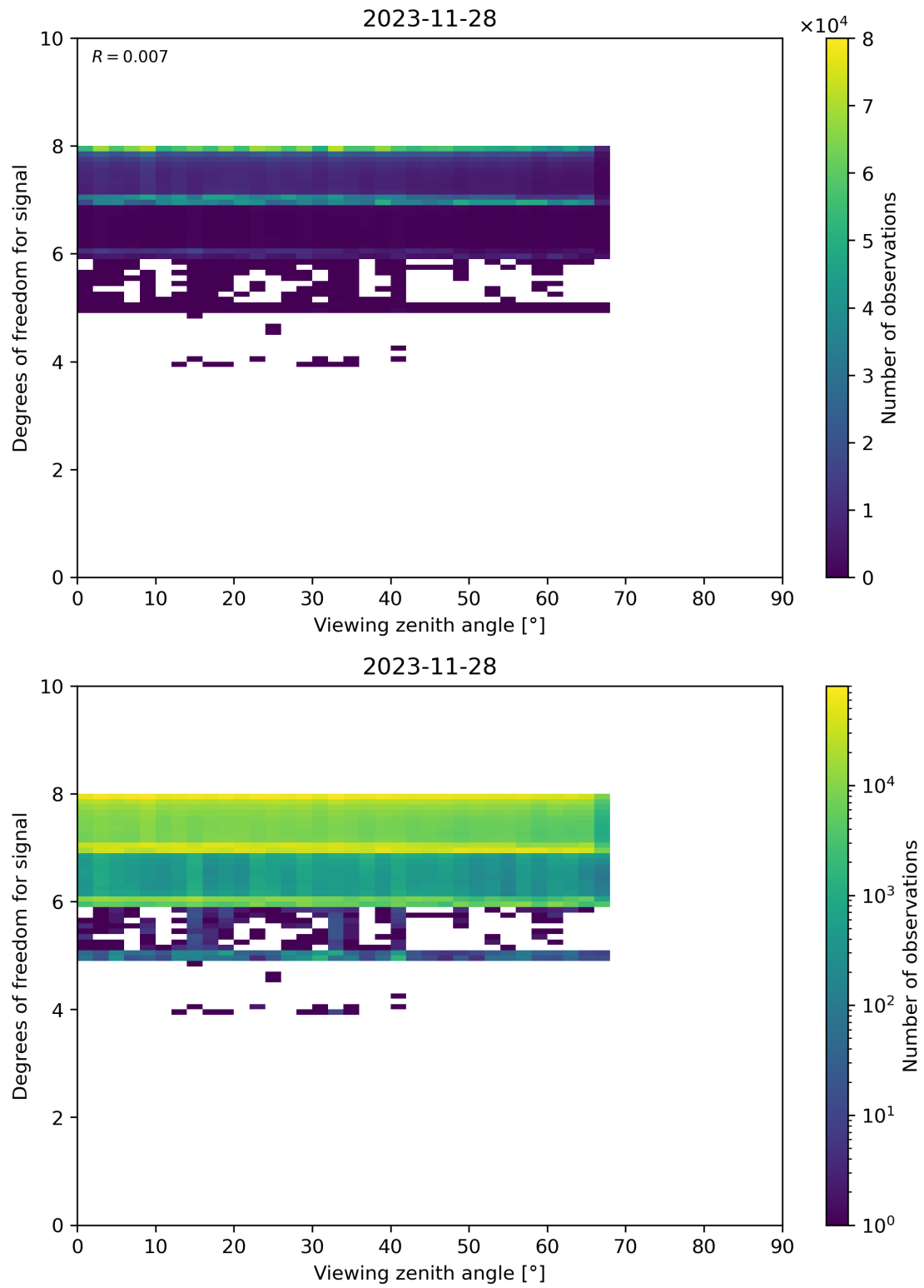
Figure 73: Scatter density plot of “Viewing zenith angle” against “Degrees of freedom for signal” for 2023-11-28 to 2023-11-29.
