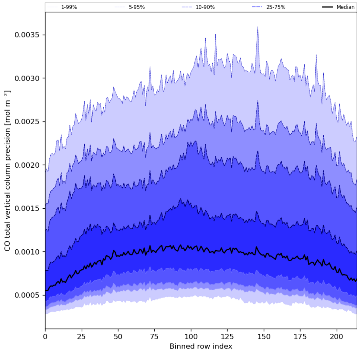
Figure 28: Along track statistics of “CO total vertical column precision” for 2023-11-28 to 2023-11-29
