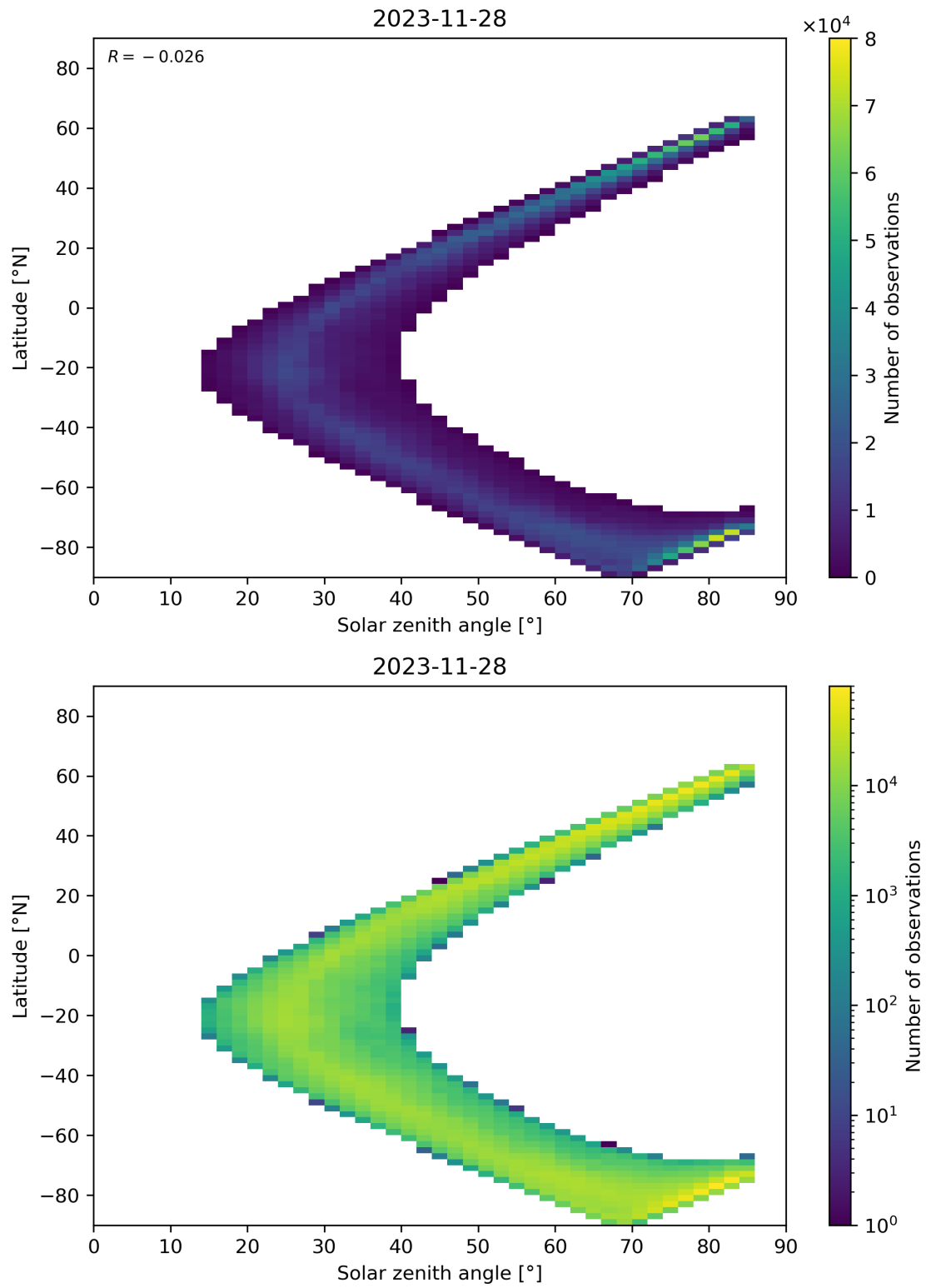
Figure 66: Scatter density plot of “Solar zenith angle” against “Latitude” for 2023-11-28 to 2023-11-29.
