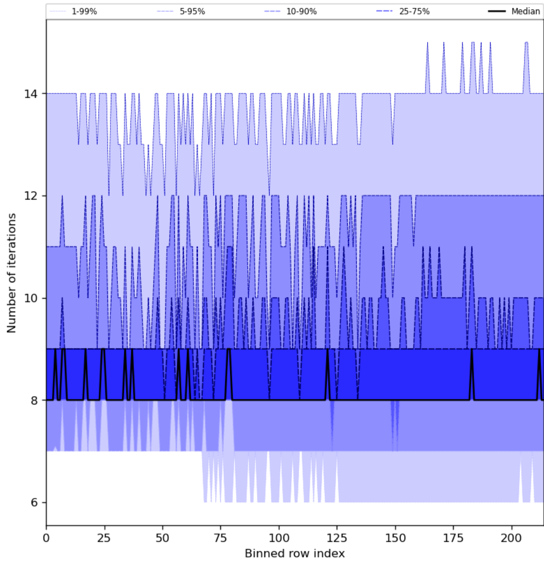
Figure 32: Along track statistics of “Number of iterations” for 2023-11-28 to 2023-11-29
