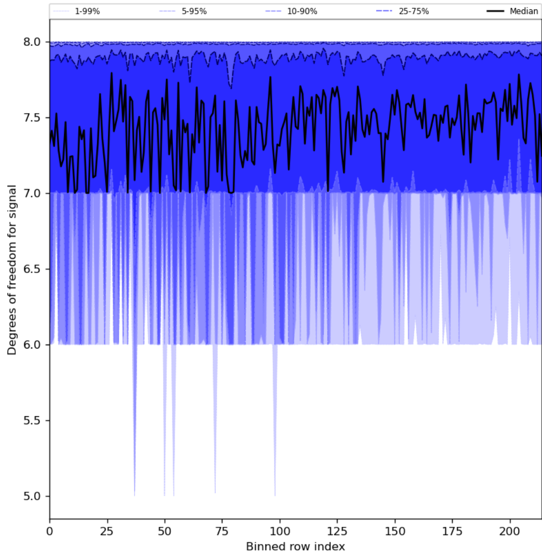
Figure 31: Along track statistics of “Degrees of freedom for signal” for 2023-11-28 to 2023-11-29
