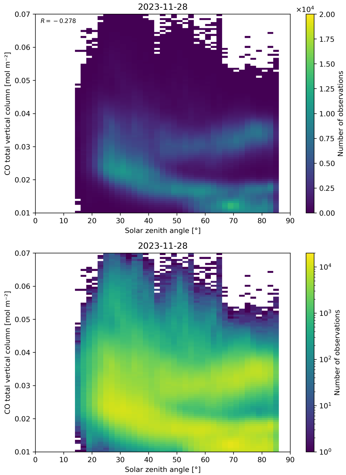
Figure 61: Scatter density plot of “Solar zenith angle” against “CO total vertical column” for 2023-11-28 to 2023-11-29.
