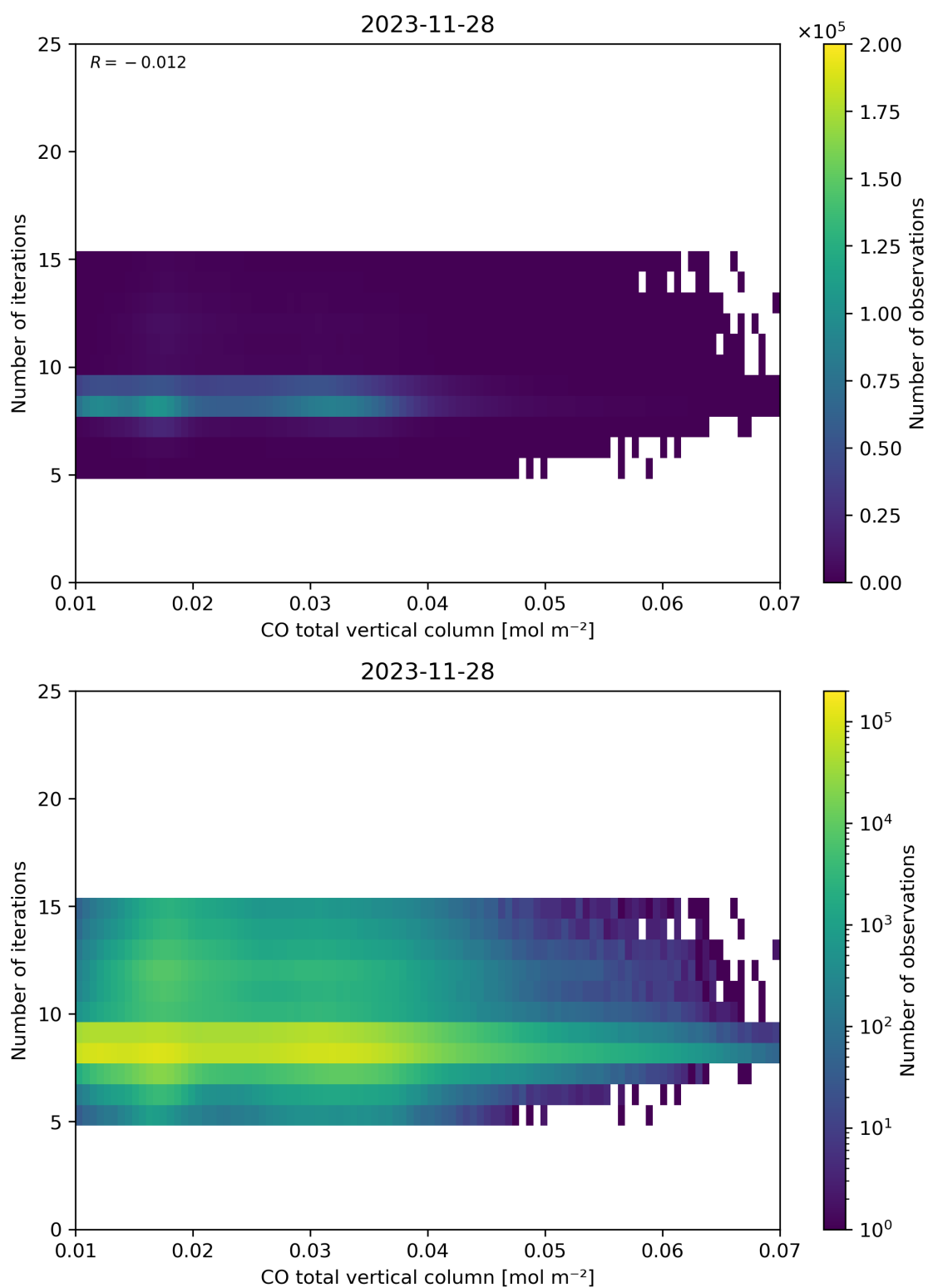
Figure 42: Scatter density plot of “CO total vertical column” against “Number of iterations” for 2023-11-28 to 2023-11-29.
