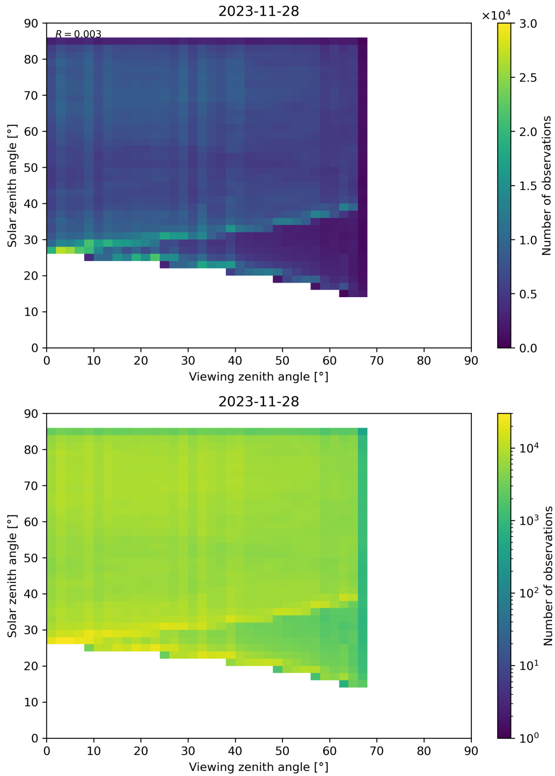
Figure 77: Scatter density plot of “Viewing zenith angle” against “Solar zenith angle” for 2023-11-28 to 2023-11-29.
