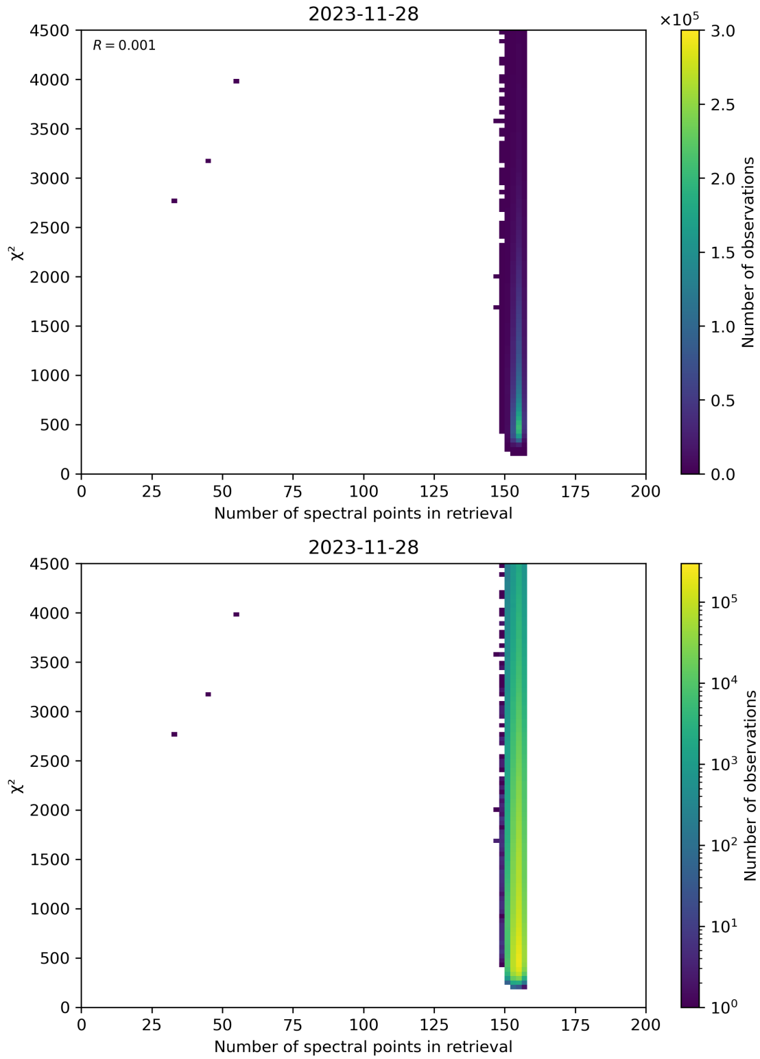
Figure 58: Scatter density plot of “Number of spectral points in retrieval” against “ \chi^2 ” for 2023-11-28 to 2023-11-29.
