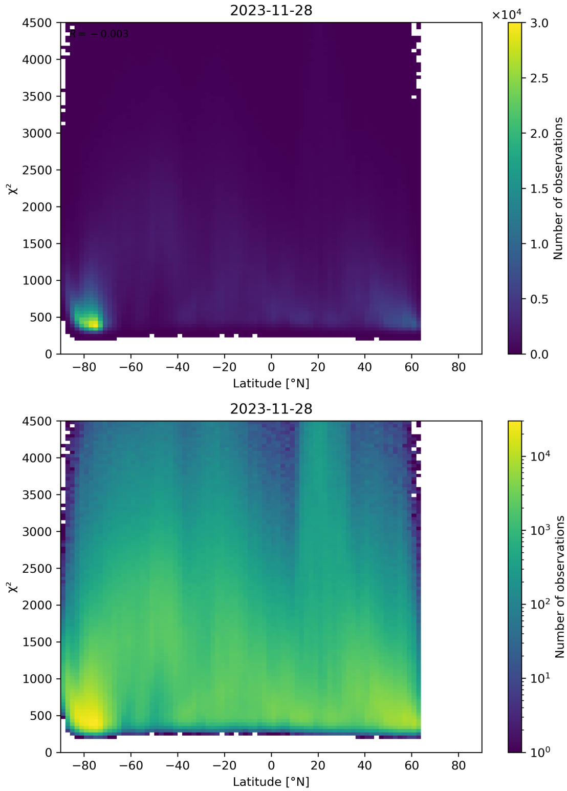
Figure 54: Scatter density plot of “Latitude” against “ \chi^2 ” for 2023-11-28 to 2023-11-29.
