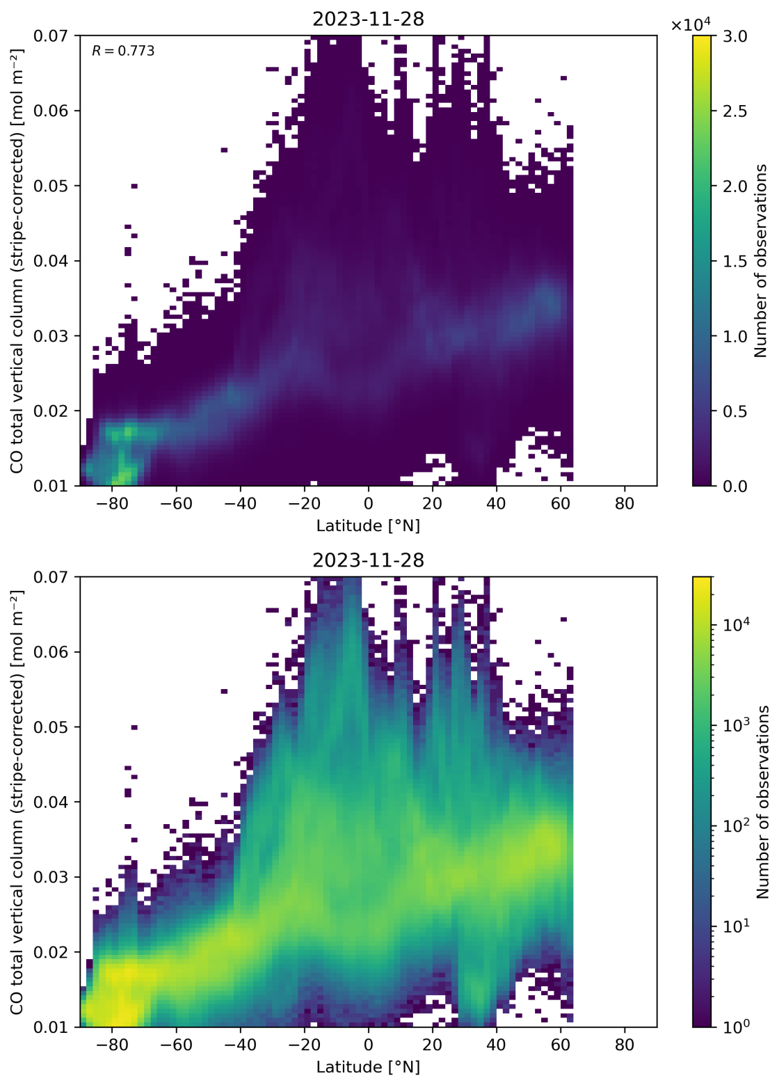
Figure 52: Scatter density plot of “Latitude” against “CO total vertical column (stripe-corrected)” for 2023-11-28 to 2023-11-29.
