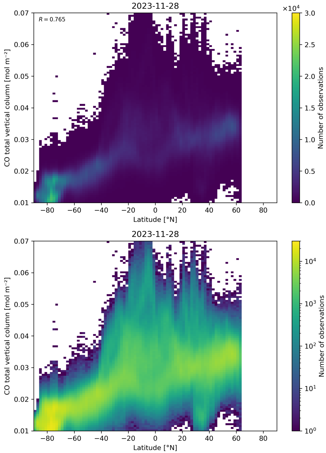
Figure 51: Scatter density plot of “Latitude” against “CO total vertical column” for 2023-11-28 to 2023-11-29.
