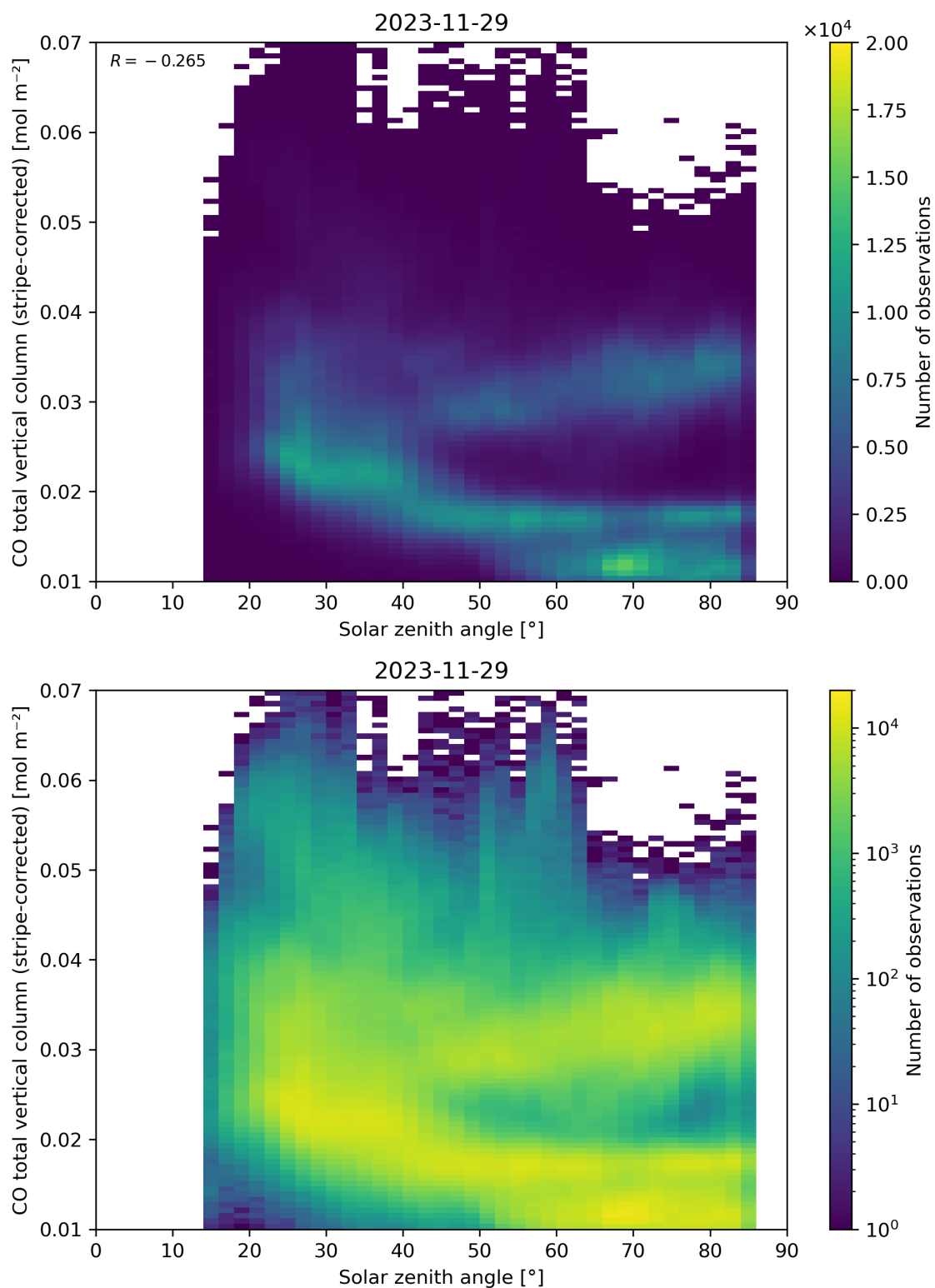
Figure 62: Scatter density plot of “Solar zenith angle” against “CO total vertical column (stripe-corrected)” for 2023-11-28 to 2023-11-30.
