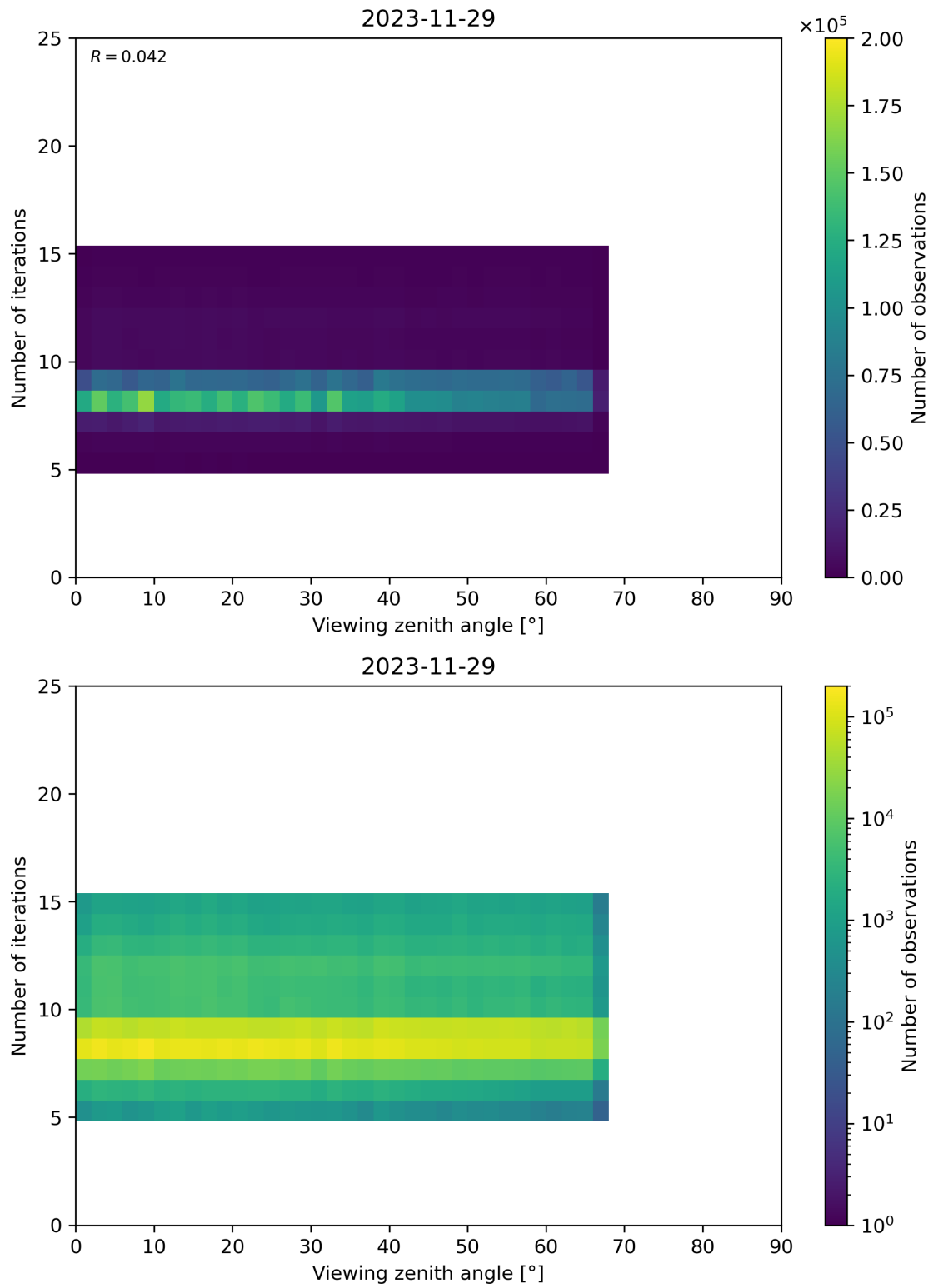
Figure 75: Scatter density plot of “Viewing zenith angle” against “Number of iterations” for 2023-11-28 to 2023-11-30.
