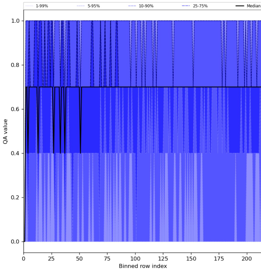
Figure 25: Along track statistics of “QA value” for 2023-11-28 to 2023-11-30
