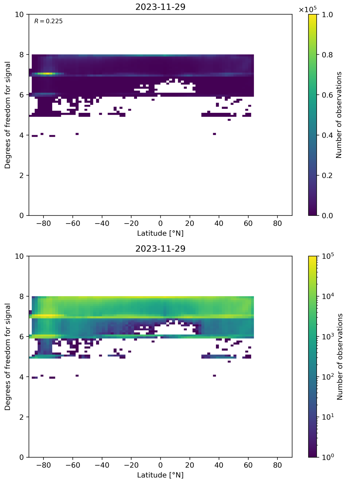
Figure 55: Scatter density plot of “Latitude” against “Degrees of freedom for signal” for 2023-11-28 to 2023-11-30.
