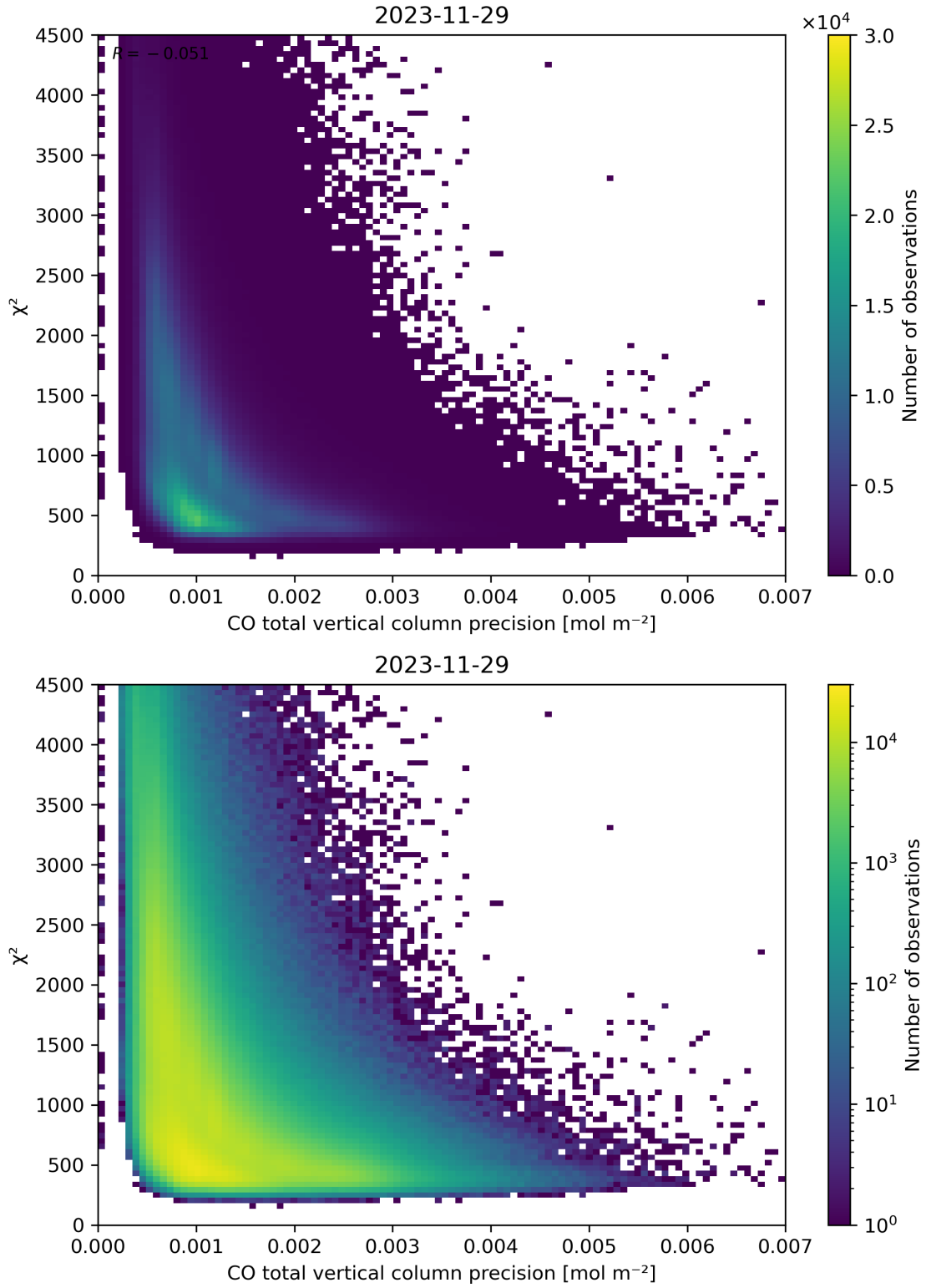
Figure 44: Scatter density plot of “CO total vertical column precision” against “ \chi^2 ” for 2023-11-28 to 2023-11-30.
