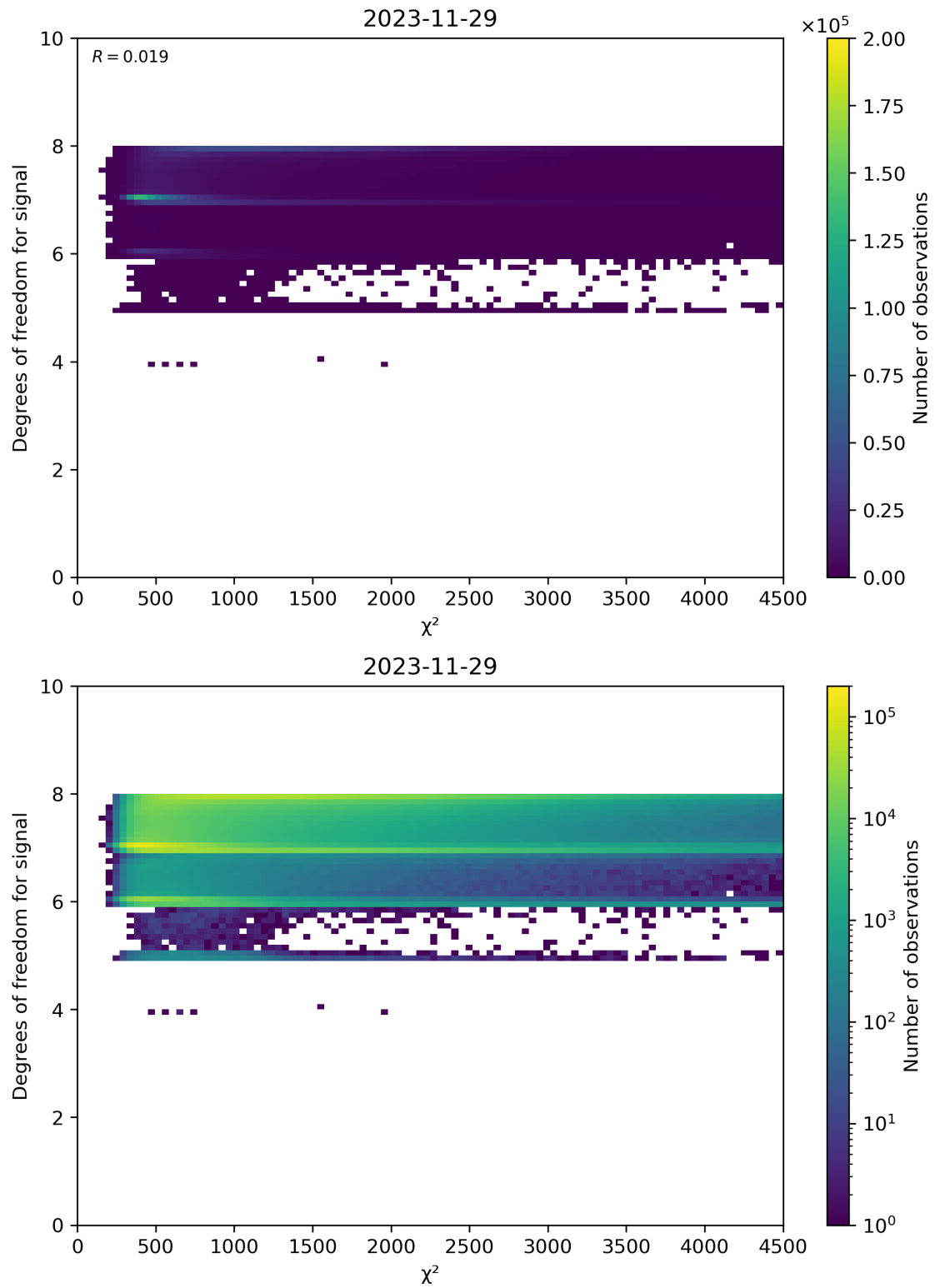
Figure 48: Scatter density plot of “ \chi^2 ” against “Degrees of freedom for signal” for 2023-11-28 to 2023-11-30.
