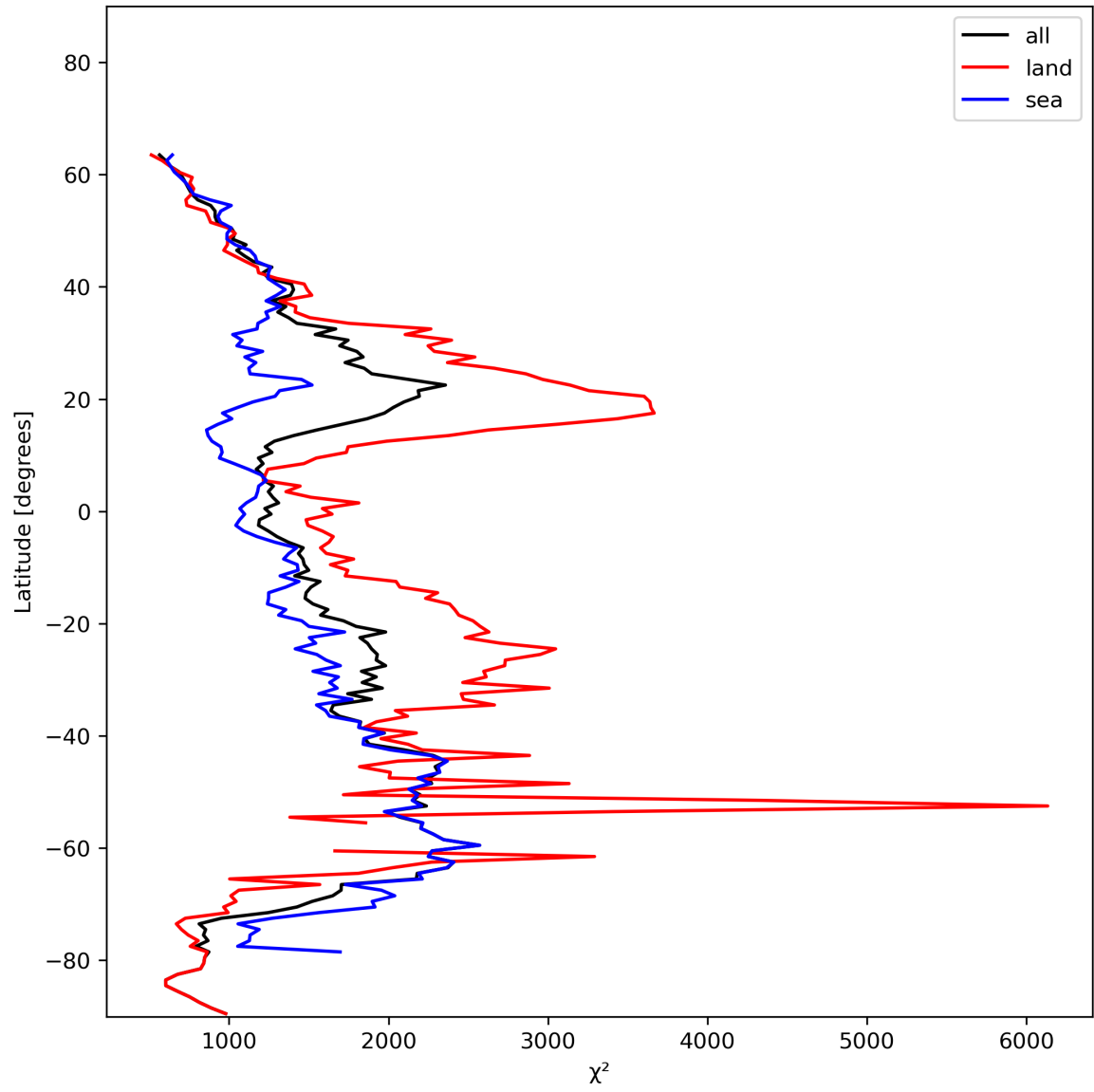
Figure 14: Zonal average of “ \chi^2 ” for 2023-11-28 to 2023-11-30.
