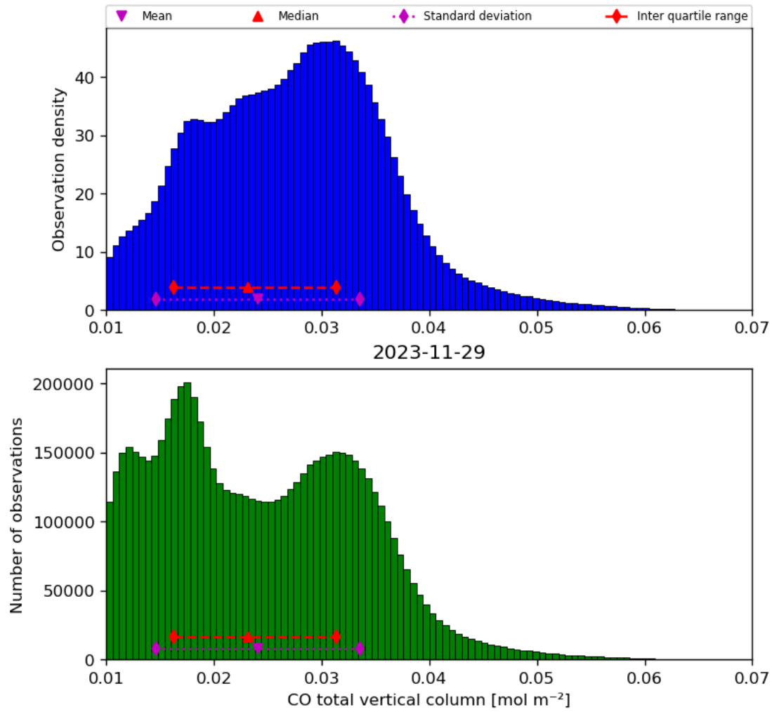
Figure 18: Histogram of “CO total vertical column” for 2023-11-28 to 2023-11-30
