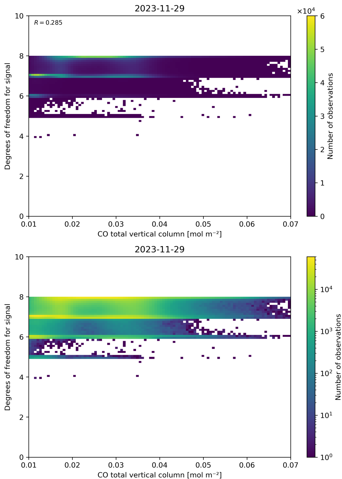
Figure 41: Scatter density plot of “CO total vertical column” against “Degrees of freedom for signal” for 2023-11-28 to 2023-11-30.
