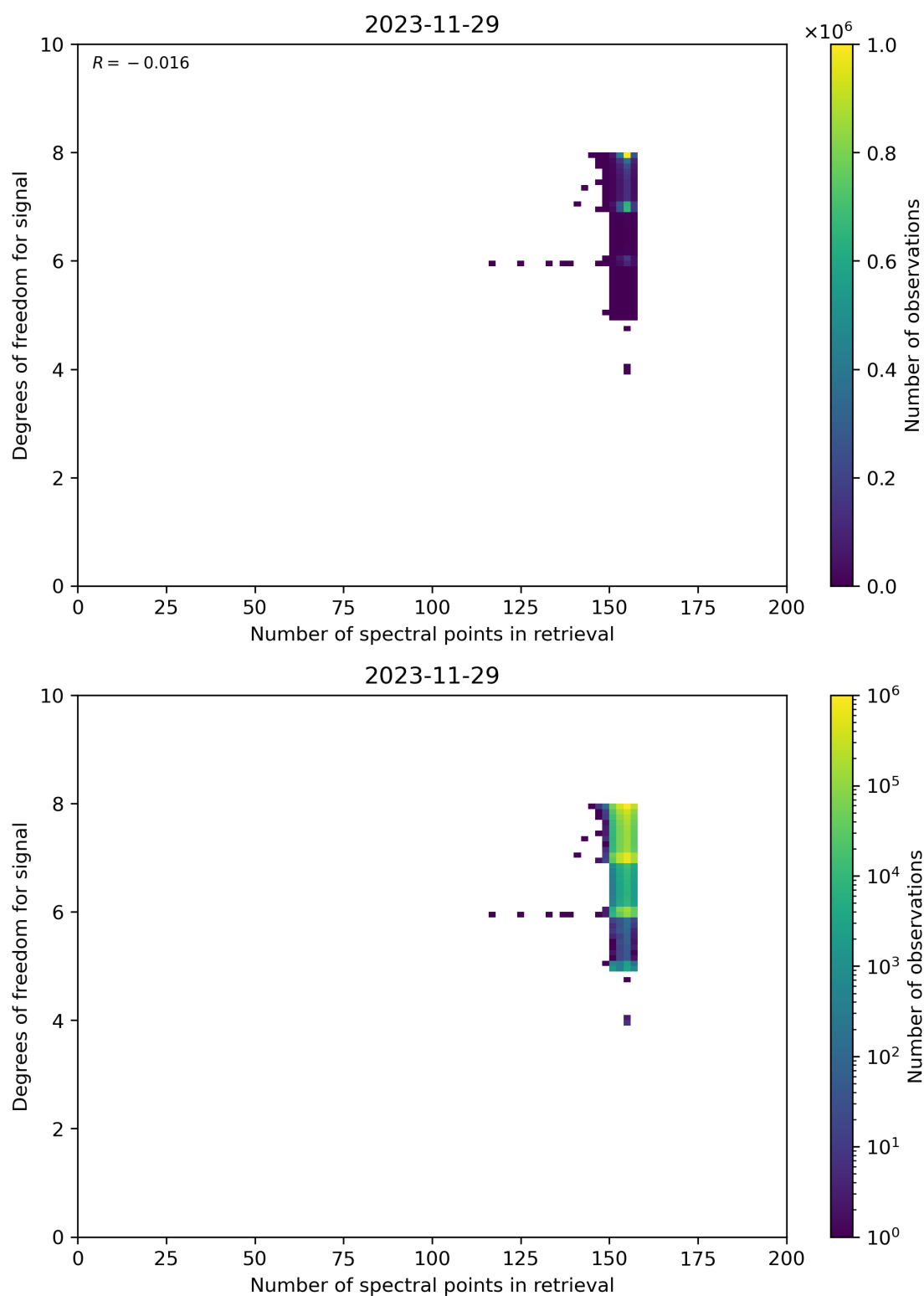
Figure 59: Scatter density plot of “Number of spectral points in retrieval” against “Degrees of freedom for signal” for 2023-11-28 to 2023-11-30.
