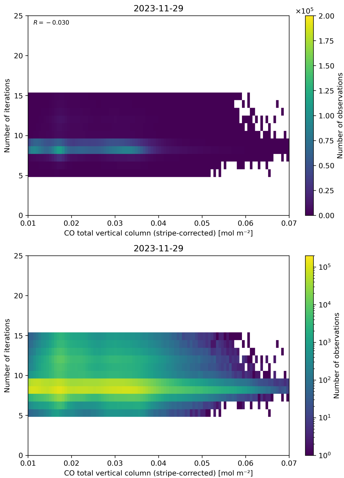
Figure 39: Scatter density plot of “CO total vertical column (stripe-corrected)” against “Number of iterations” for 2023-11-28 to 2023-11-30.
