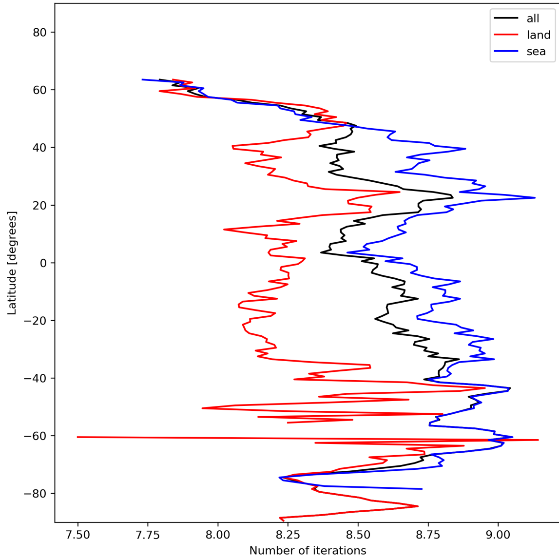
Figure 16: Zonal average of “Number of iterations” for 2023-11-28 to 2023-11-30.
