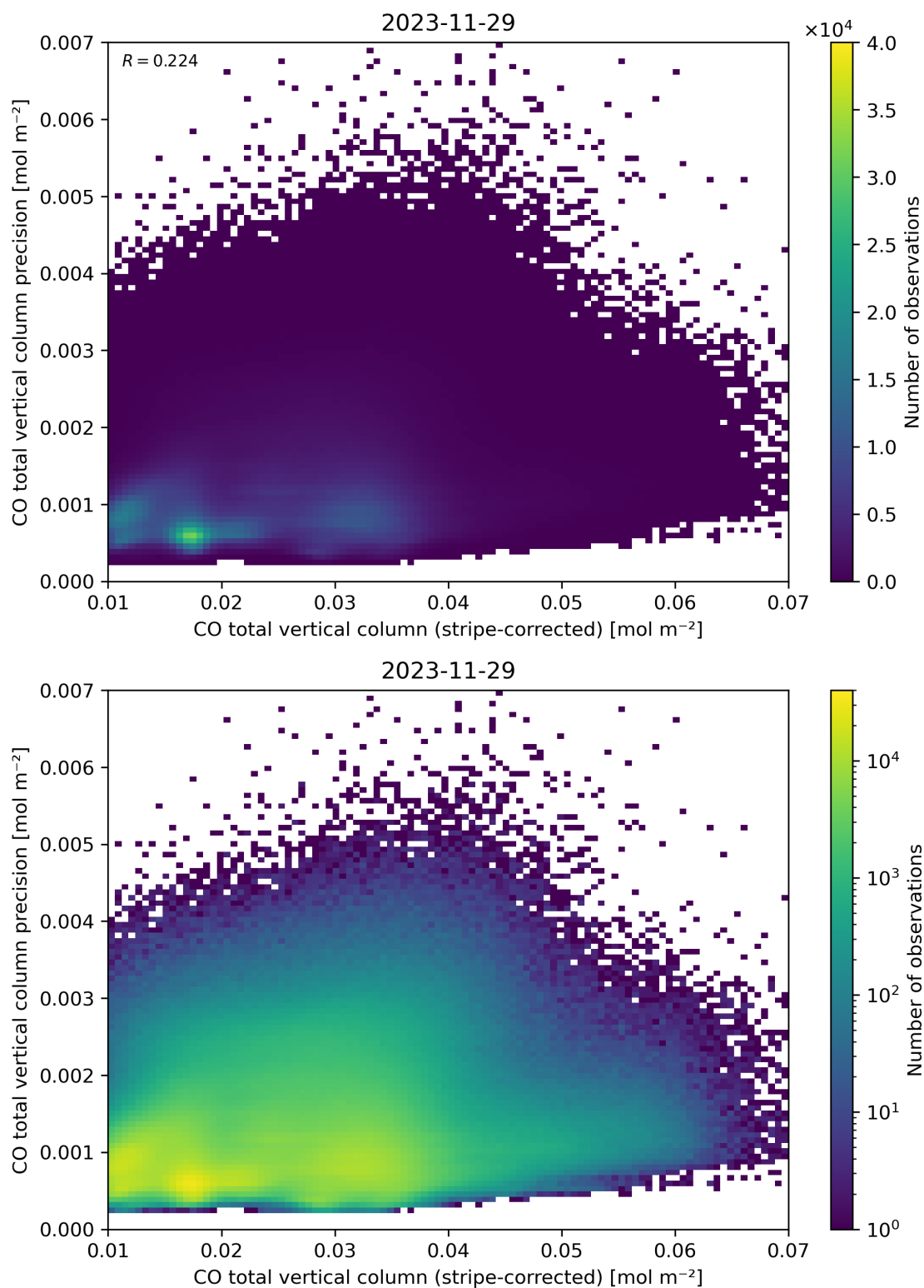
Figure 36: Scatter density plot of “CO total vertical column (stripe-corrected)” against “CO total vertical column precision” for 2023-11-28 to 2023-11-30.
