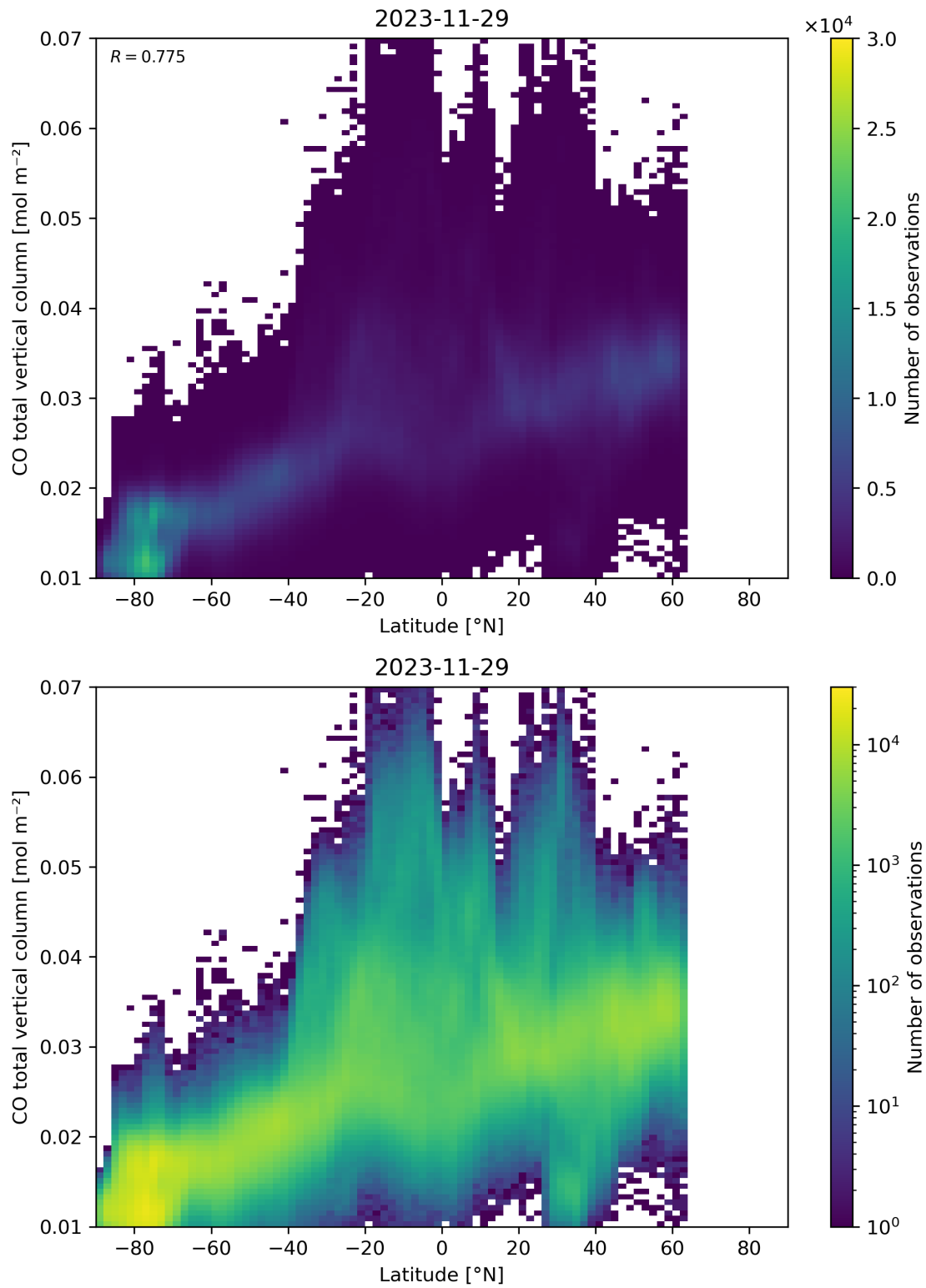
Figure 51: Scatter density plot of “Latitude” against “CO total vertical column” for 2023-11-28 to 2023-11-30.
