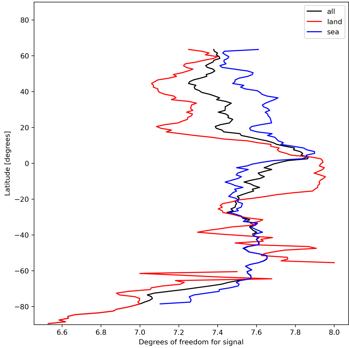
Figure 15: Zonal average of “Degrees of freedom for signal” for 2023-11-28 to 2023-11-30.
