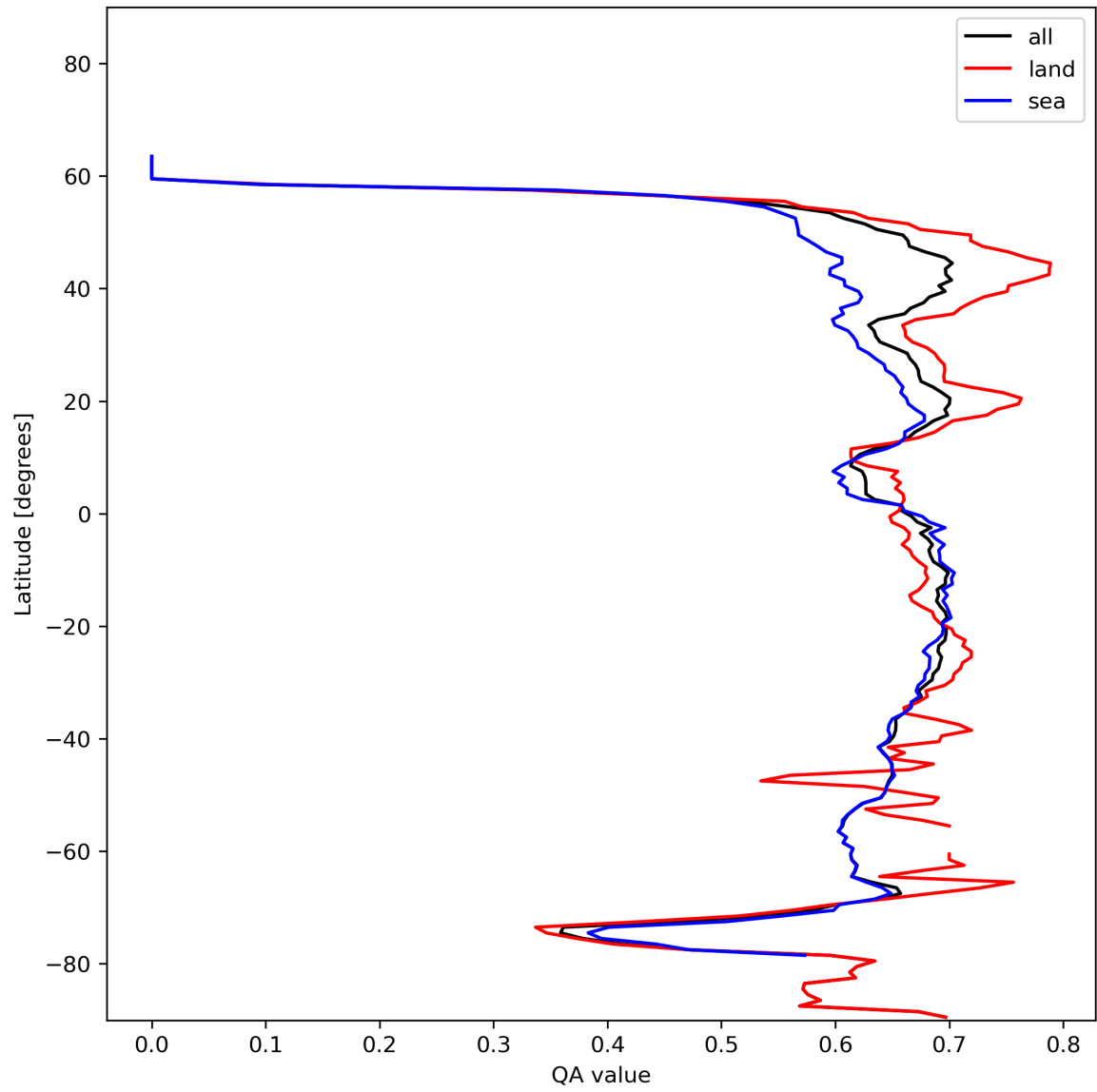
Figure 9: Zonal average of “QA value” for 2023-11-28 to 2023-11-30.
