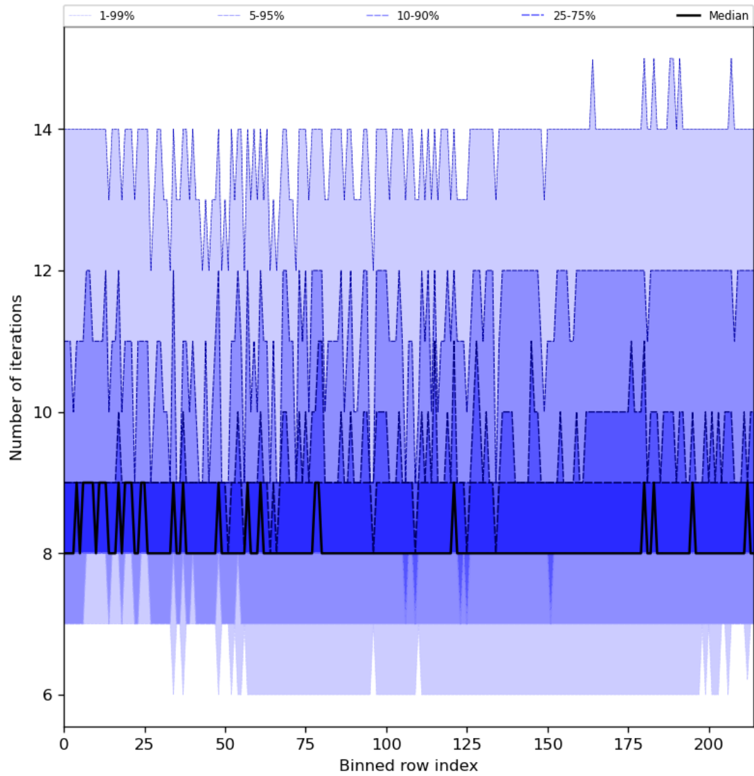
Figure 32: Along track statistics of “Number of iterations” for 2023-11-28 to 2023-11-30
