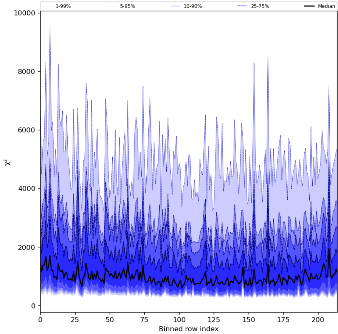
Figure 30: Along track statistics of “ \chi^2 ” for 2023-11-28 to 2023-11-30
