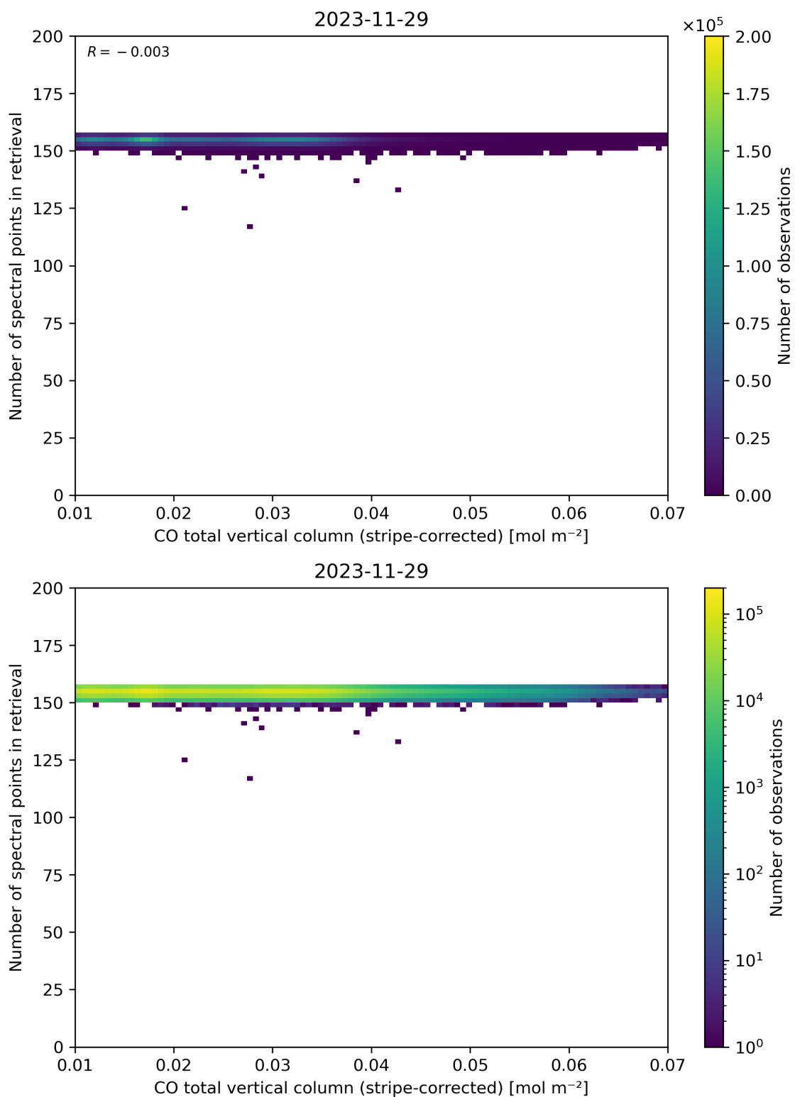
Figure 40: Scatter density plot of “CO total vertical column (stripe-corrected)” against “Number of spectral points in retrieval” for 2023-11-28 to 2023-11-30.
