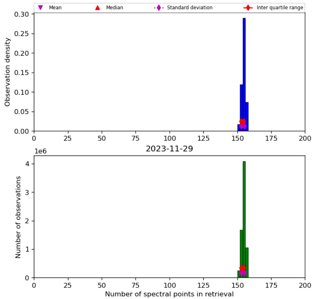
Figure 21: Histogram of “Number of spectral points in retrieval” for 2023-11-28 to 2023-11-30
