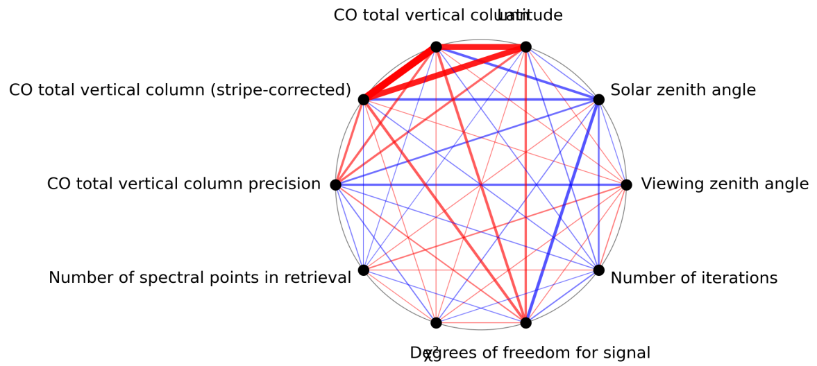
Figure 1: Map of correlation graph for 2023-11-28 to 2023-11-30.
