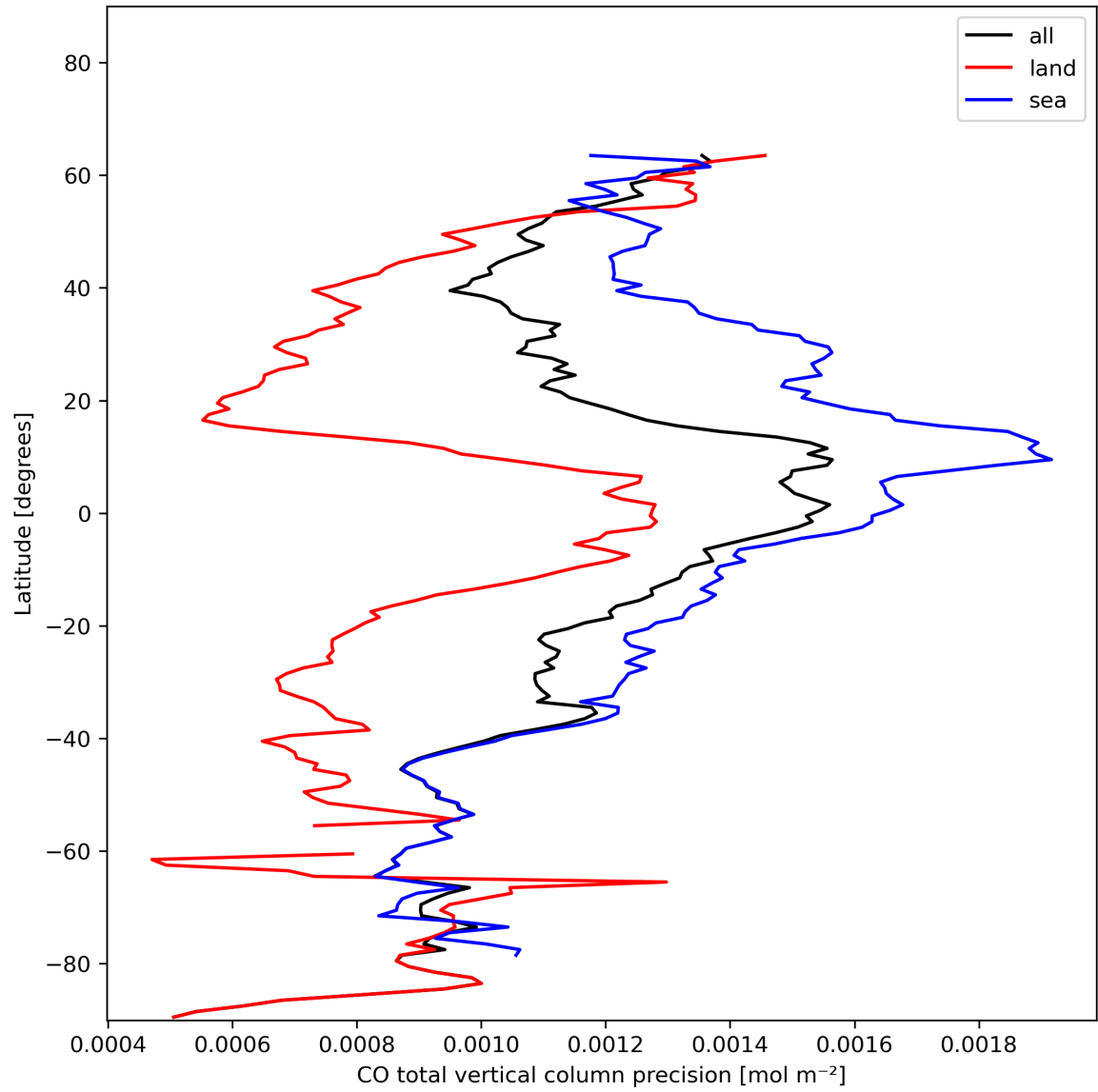
Figure 12: Zonal average of “CO total vertical column precision” for 2023-11-28 to 2023-11-30.
