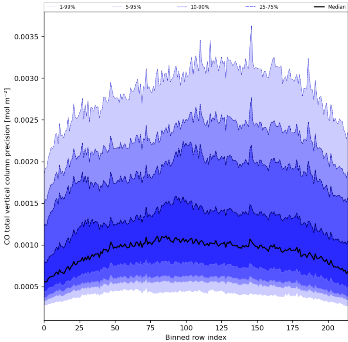
Figure 28: Along track statistics of “CO total vertical column precision” for 2023-11-28 to 2023-11-30
