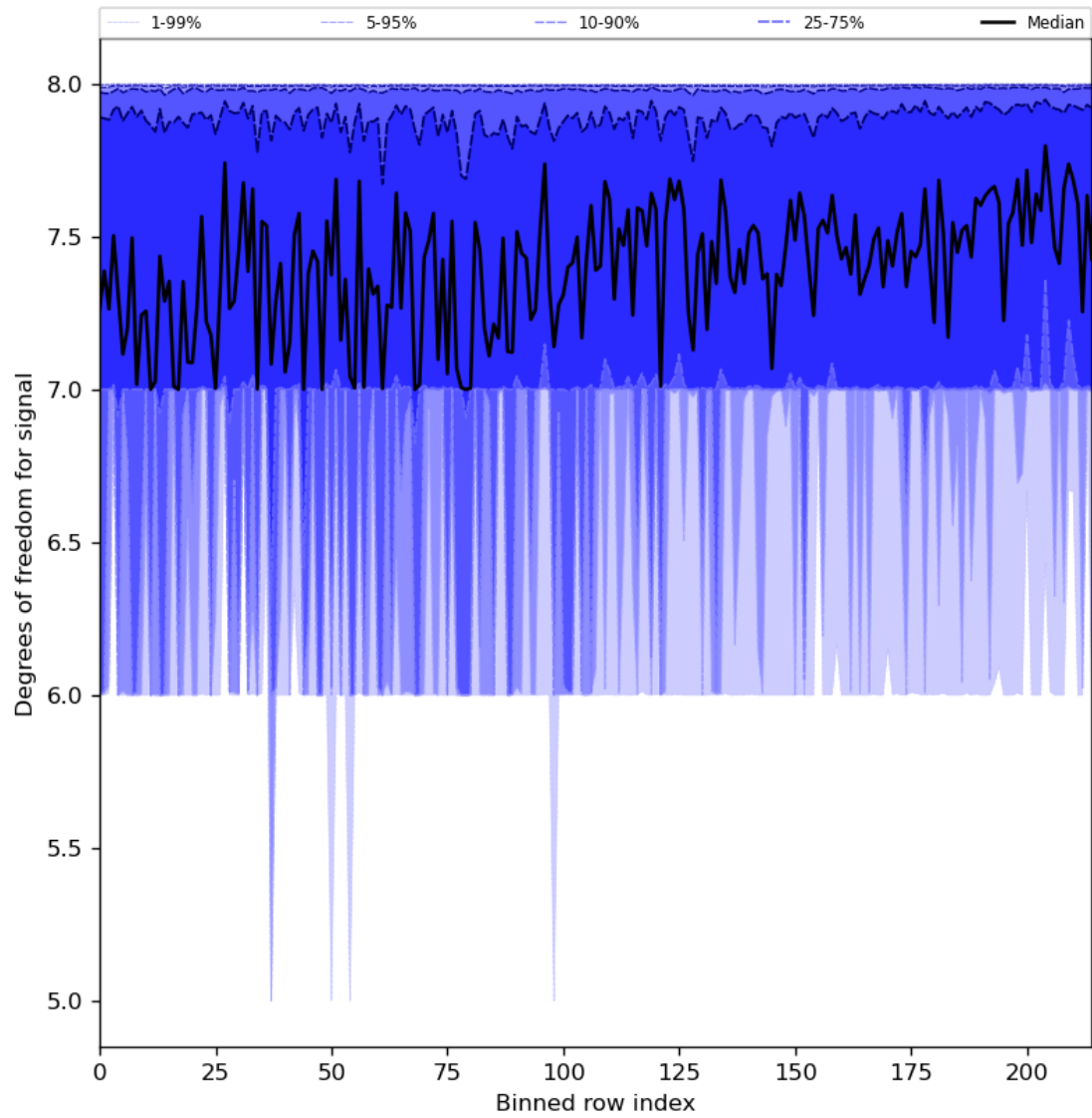
Figure 31: Along track statistics of “Degrees of freedom for signal” for 2023-11-28 to 2023-11-30
