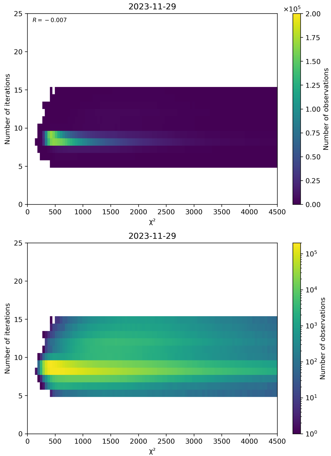
Figure 49: Scatter density plot of “ \chi^2 ” against “Number of iterations” for 2023-11-28 to 2023-11-30.
