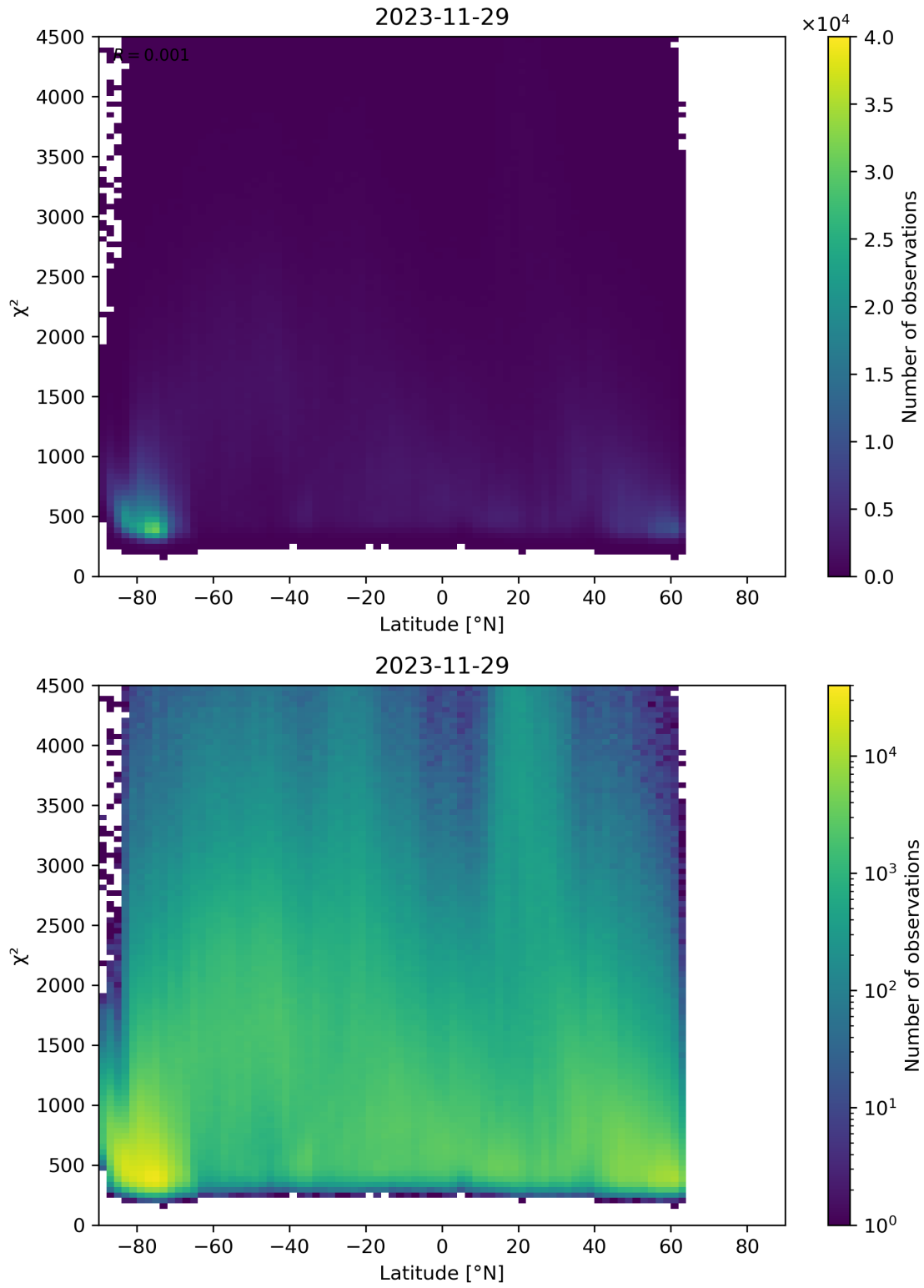
Figure 54: Scatter density plot of “Latitude” against “ \chi^2 ” for 2023-11-28 to 2023-11-30.
