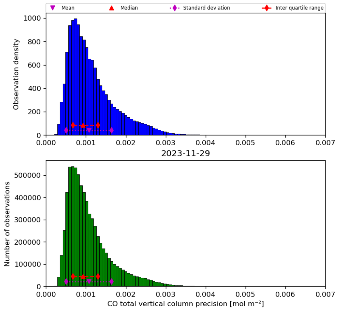
Figure 20: Histogram of “CO total vertical column precision” for 2023-11-28 to 2023-11-30
