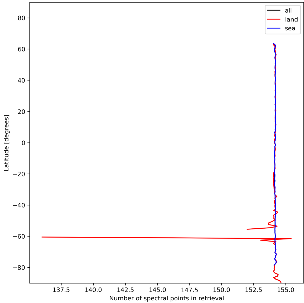
Figure 13: Zonal average of “Number of spectral points in retrieval” for 2023-11-28 to 2023-11-30.
