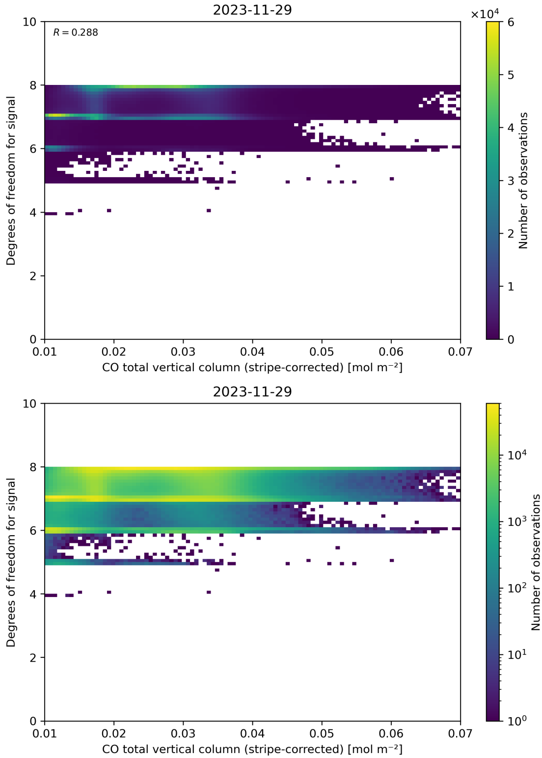
Figure 38: Scatter density plot of “CO total vertical column (stripe-corrected)” against “Degrees of freedom for signal” for 2023-11-28 to 2023-11-30.
