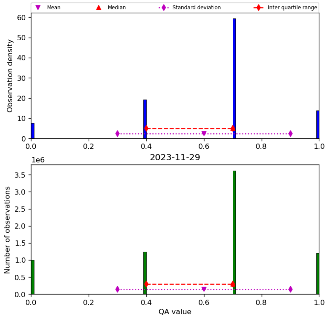
Figure 17: Histogram of “QA value” for 2023-11-28 to 2023-11-30
