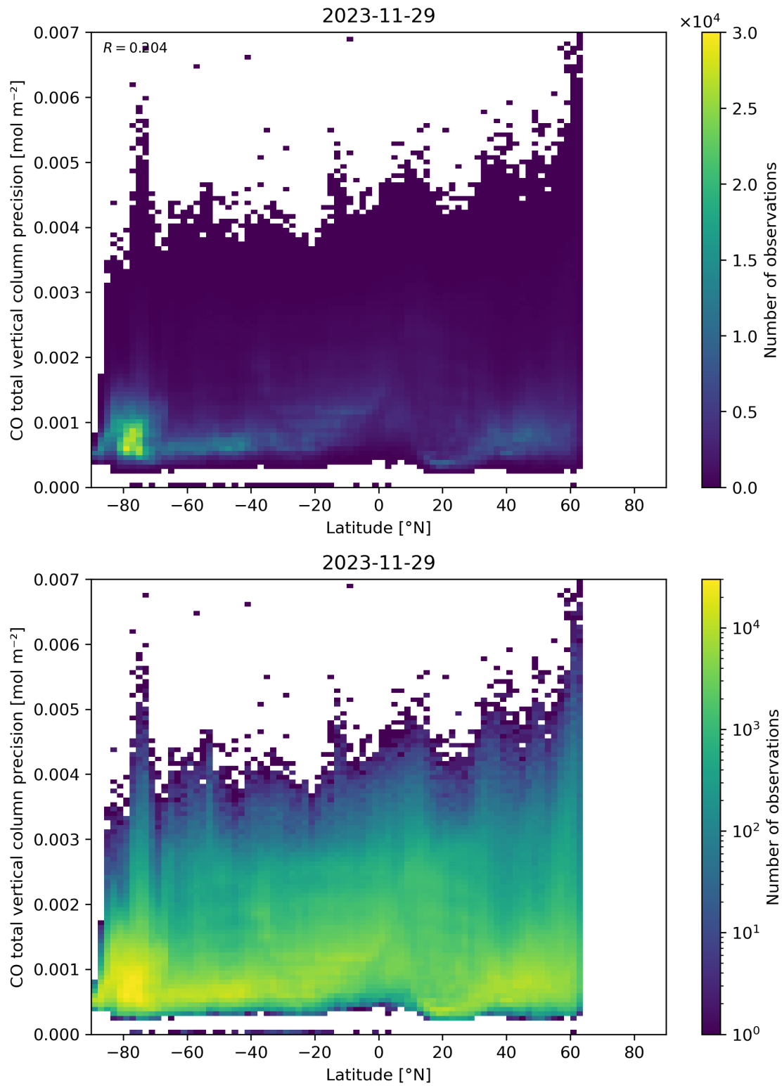
Figure 53: Scatter density plot of “Latitude” against “CO total vertical column precision” for 2023-11-28 to 2023-11-30.
