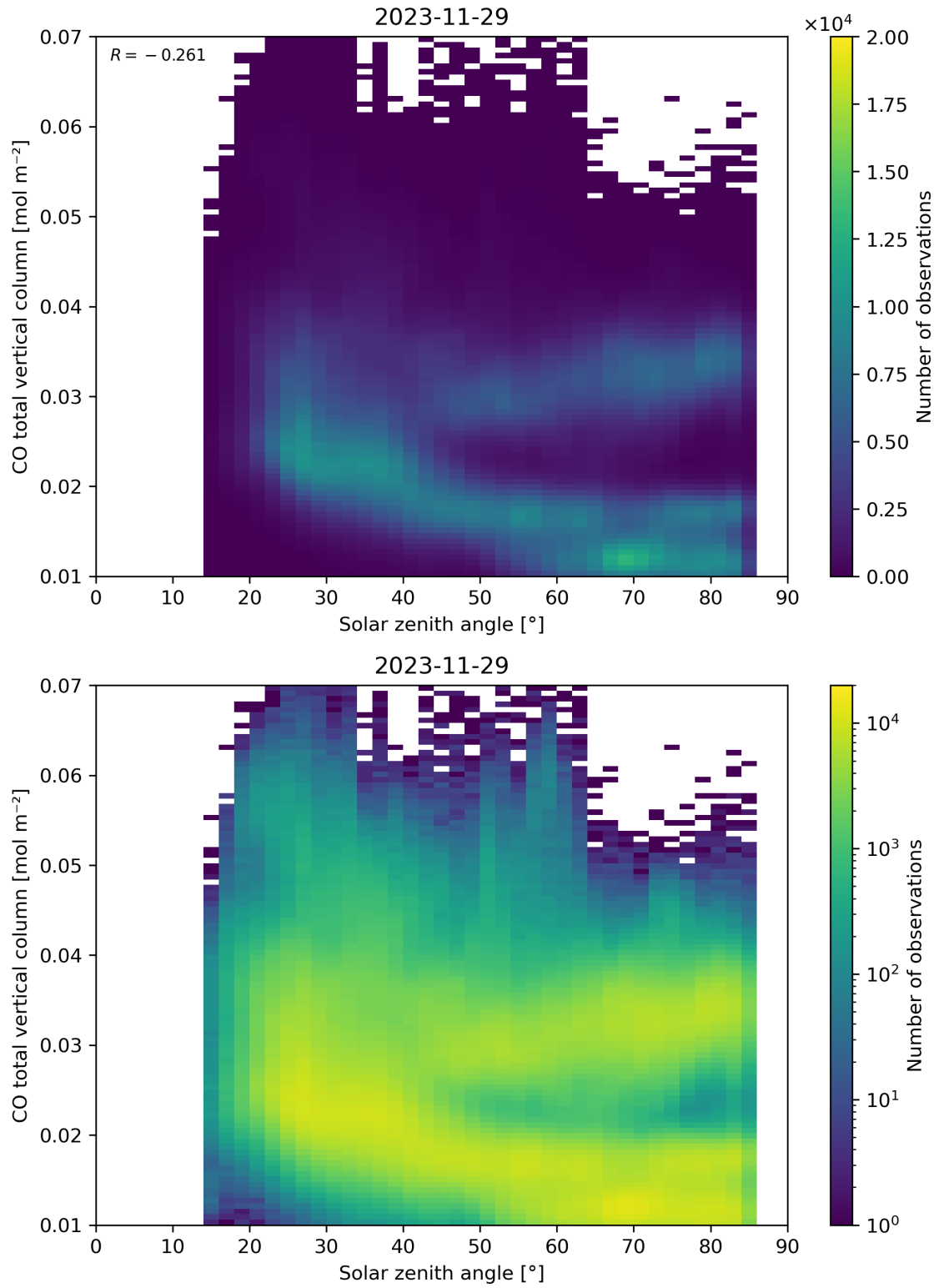
Figure 61: Scatter density plot of “Solar zenith angle” against “CO total vertical column” for 2023-11-28 to 2023-11-30.
