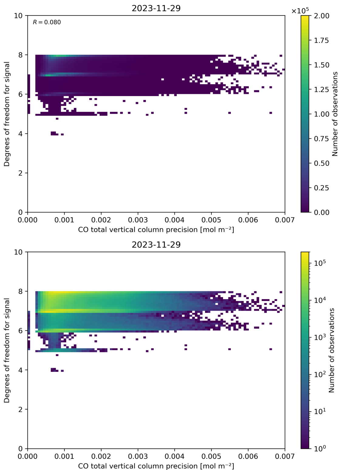
Figure 45: Scatter density plot of “CO total vertical column precision” against “Degrees of freedom for signal” for 2023-11-28 to 2023-11-30.
