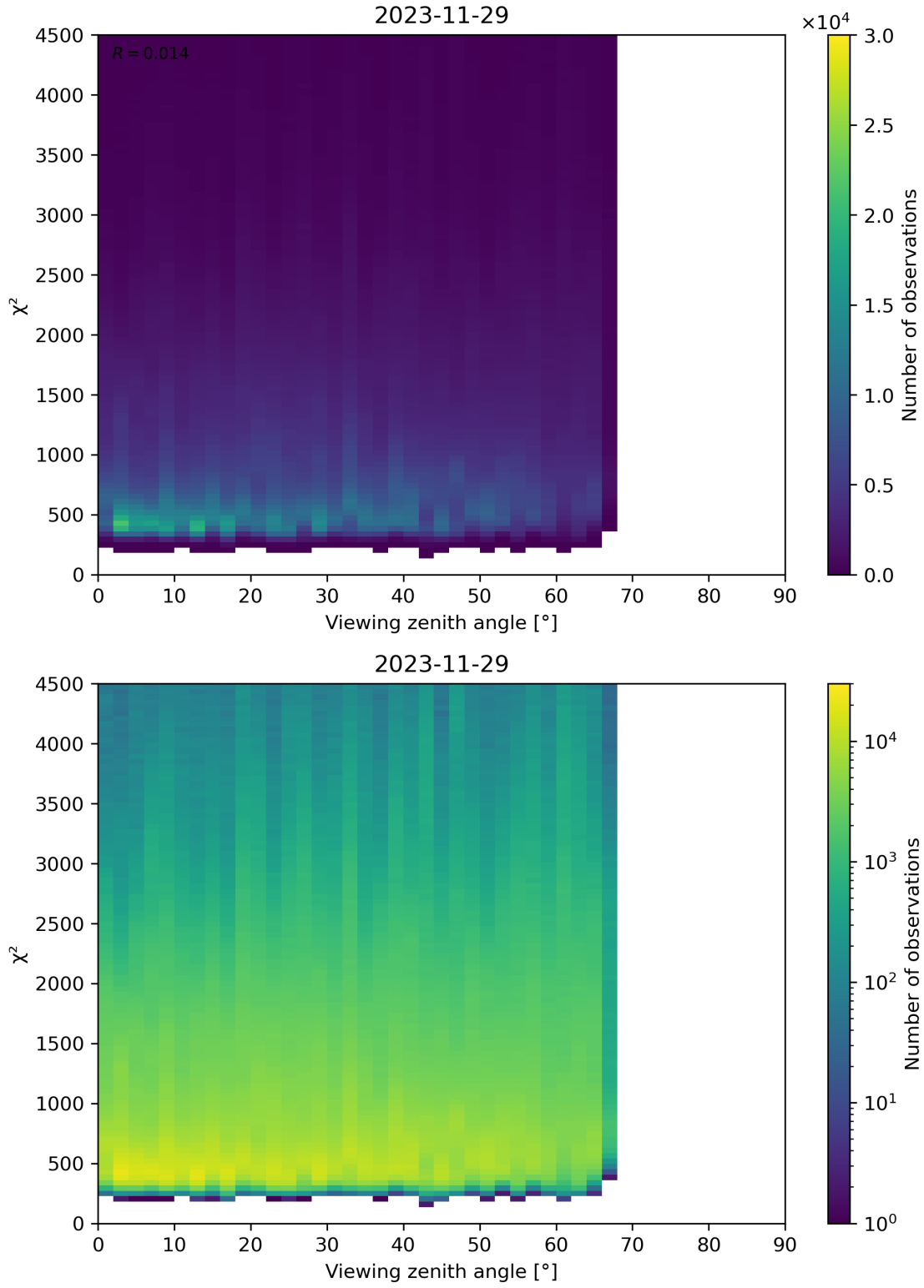
Figure 72: Scatter density plot of “Viewing zenith angle” against “ \chi^2 ” for 2023-11-28 to 2023-11-30.
