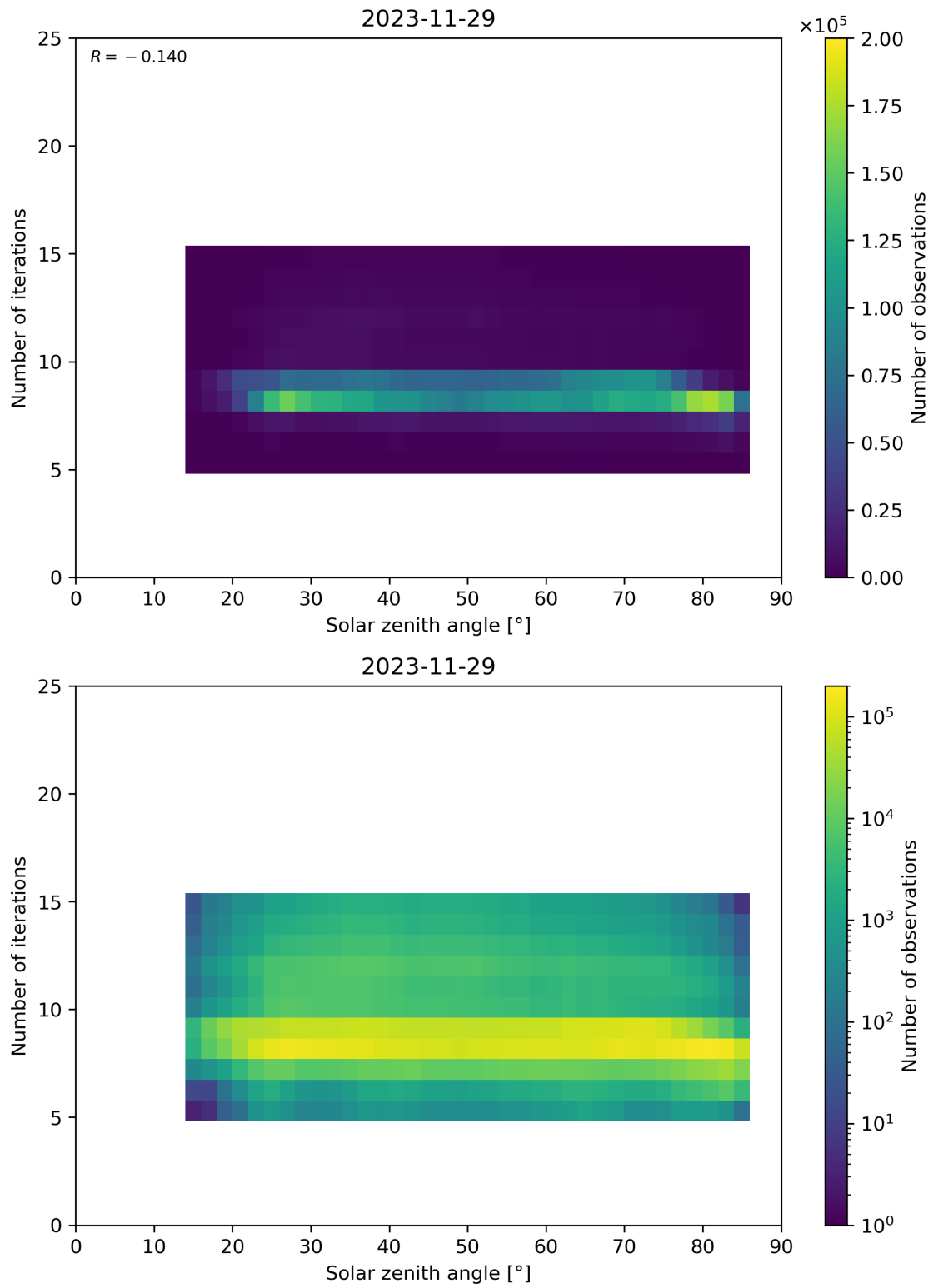
Figure 67: Scatter density plot of “Solar zenith angle” against “Number of iterations” for 2023-11-28 to 2023-11-30.
