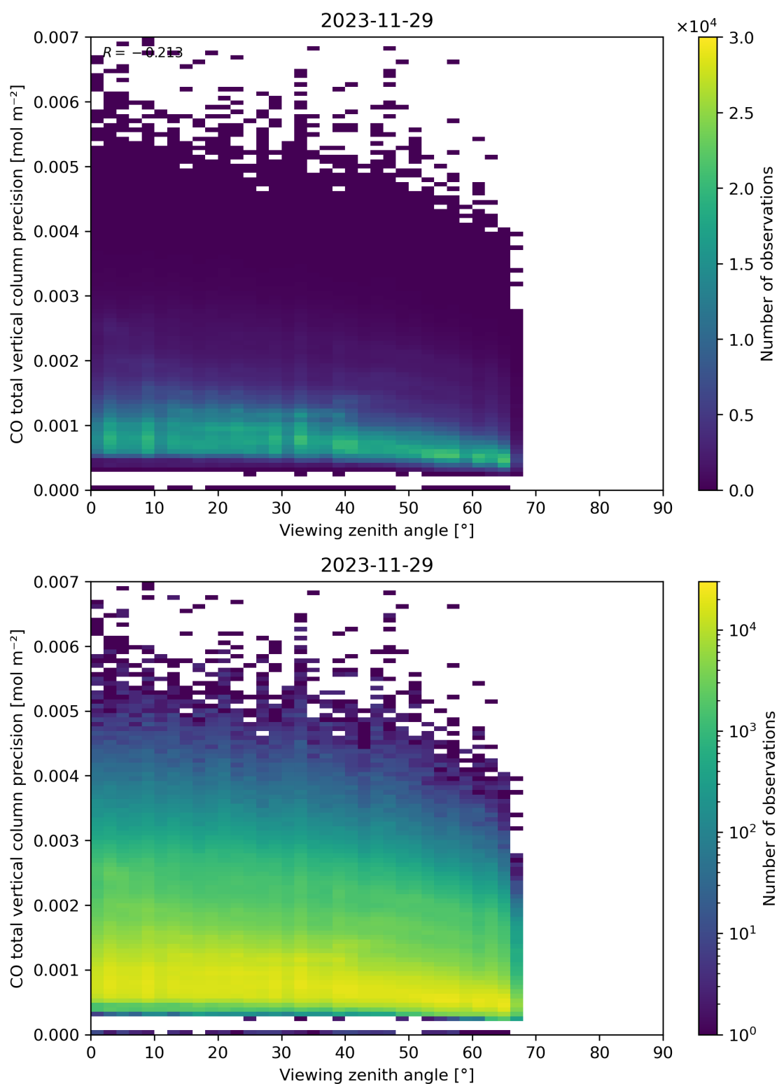
Figure 71: Scatter density plot of “Viewing zenith angle” against “CO total vertical column precision” for 2023-11-28 to 2023-11-30.
