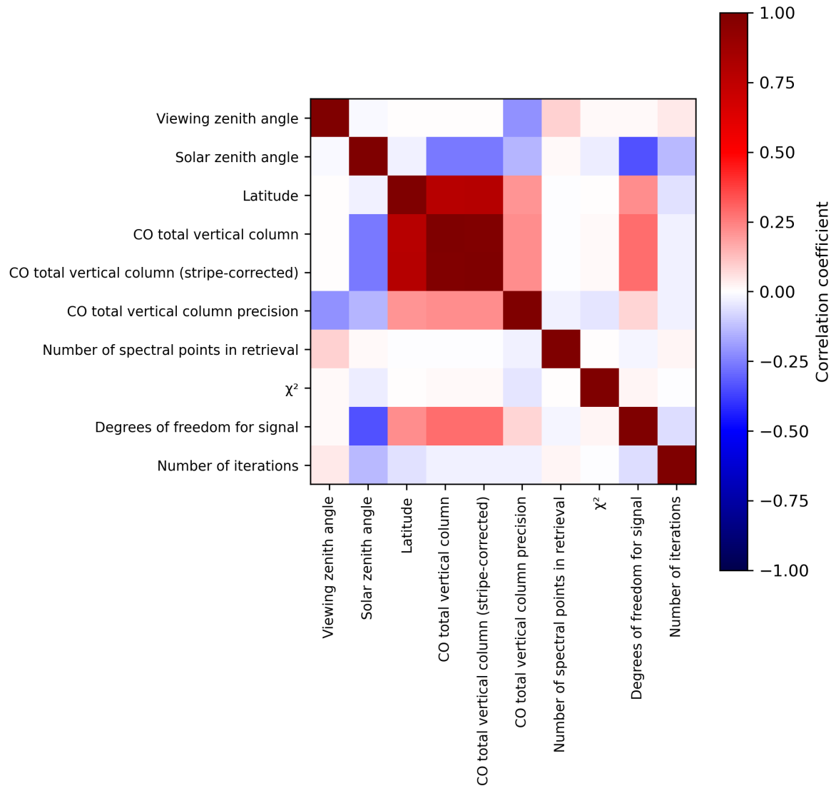
Figure 2: Map of correlation matrix for 2023-11-28 to 2023-11-30.
