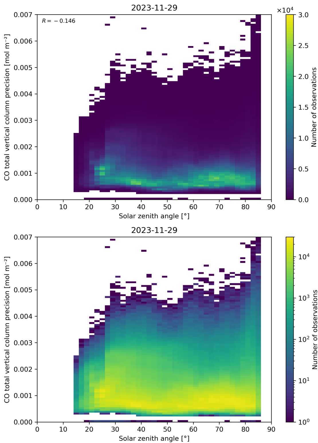
Figure 63: Scatter density plot of “Solar zenith angle” against “CO total vertical column precision” for 2023-11-28 to 2023-11-30.
