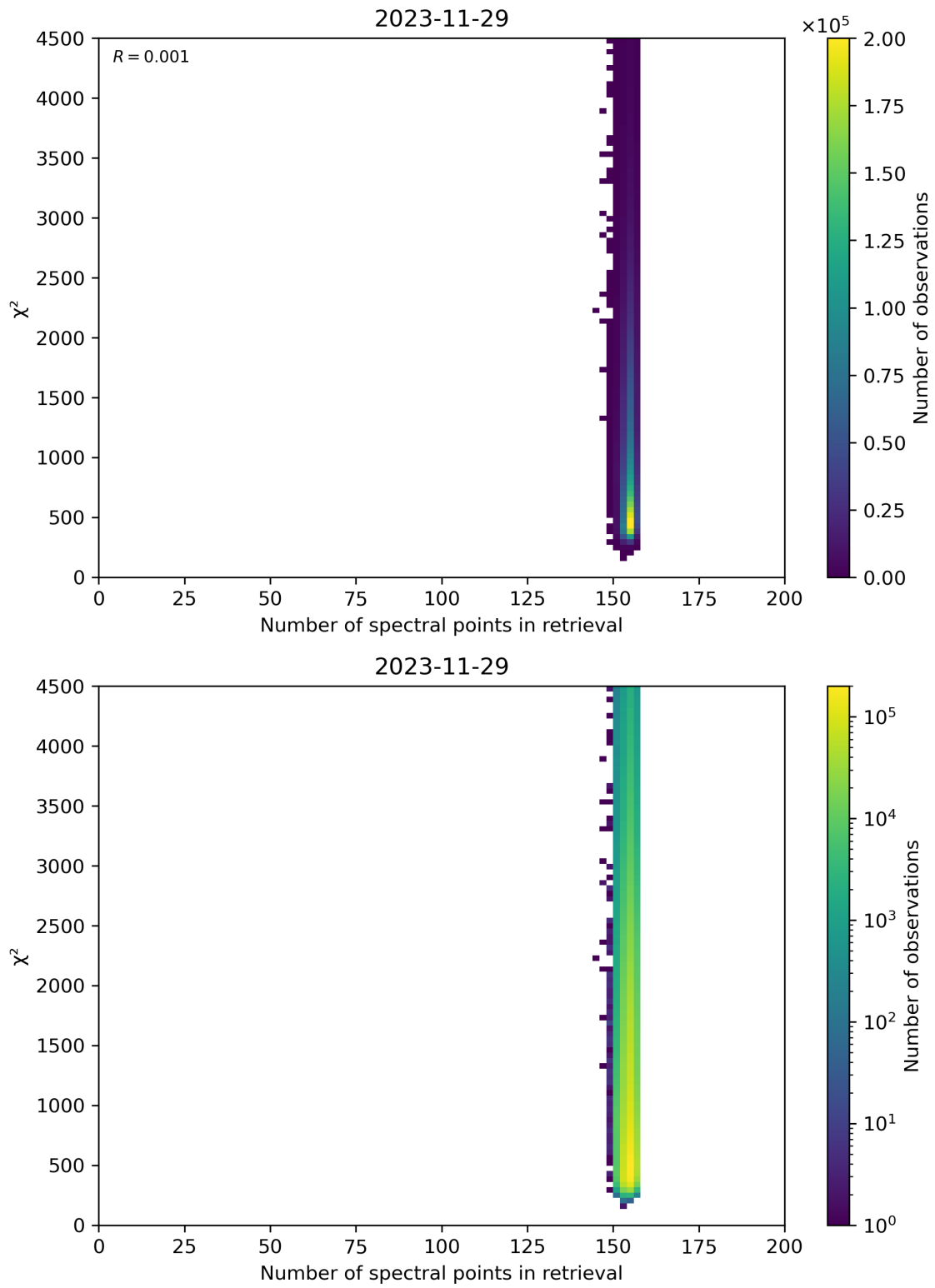
Figure 58: Scatter density plot of “Number of spectral points in retrieval” against “ \chi^2 ” for 2023-11-28 to 2023-11-30.
