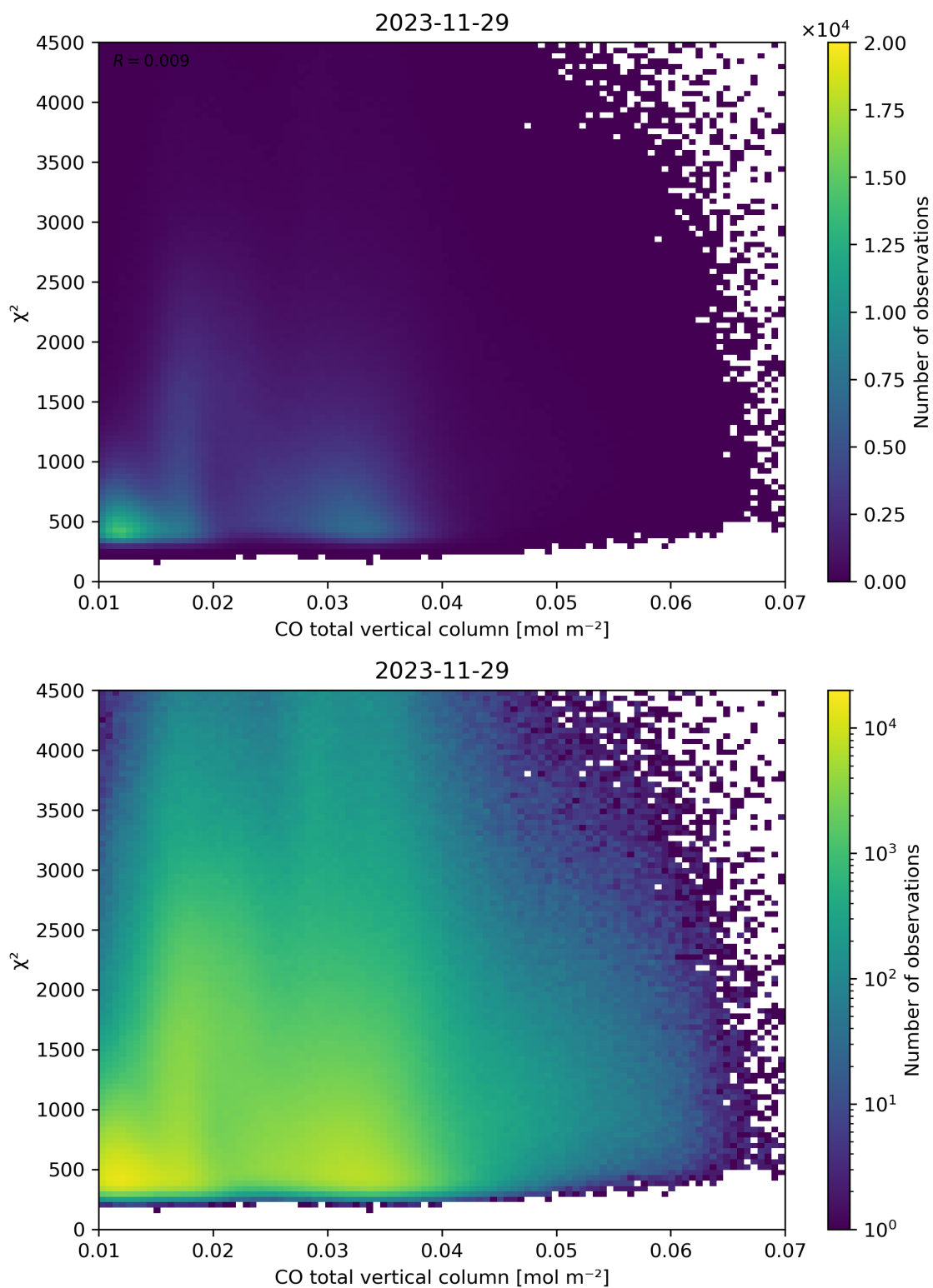
Figure 35: Scatter density plot of “CO total vertical column” against “ \chi^2 ” for 2023-11-28 to 2023-11-30.
