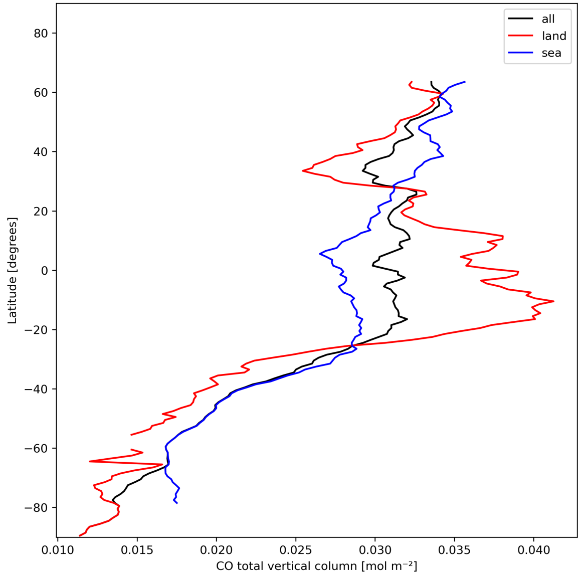
Figure 10: Zonal average of “CO total vertical column” for 2023-11-28 to 2023-11-30.
