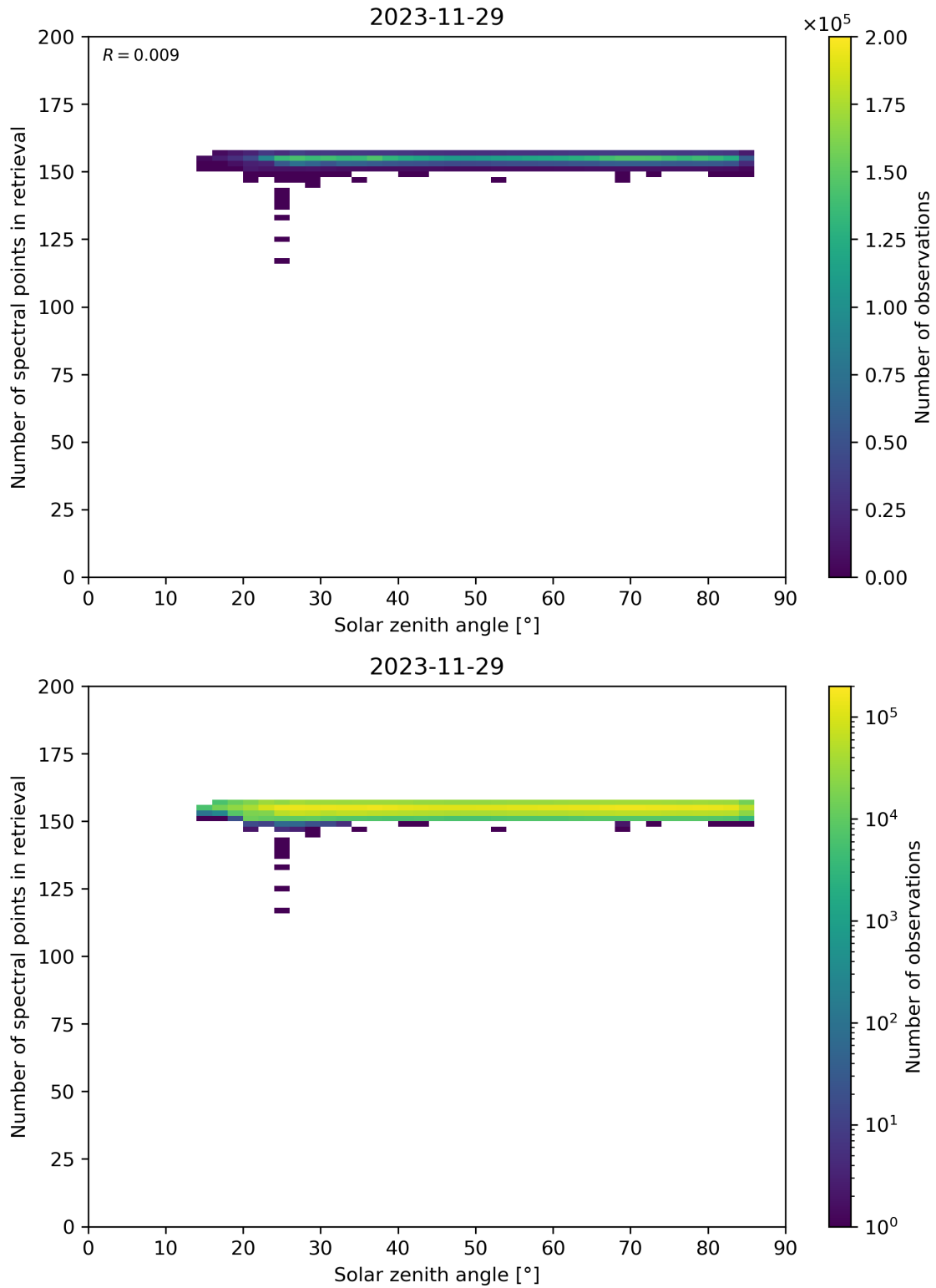
Figure 68: Scatter density plot of “Solar zenith angle” against “Number of spectral points in retrieval” for 2023-11-28 to 2023-11-30.
