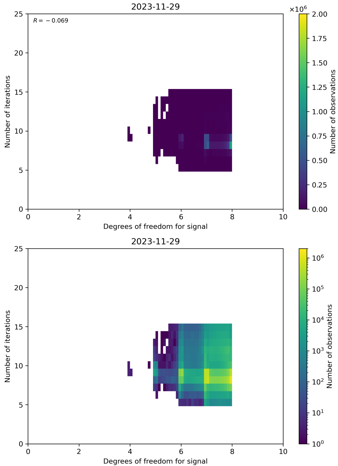
Figure 50: Scatter density plot of “Degrees of freedom for signal” against “Number of iterations” for 2023-11-28 to 2023-11-30.
