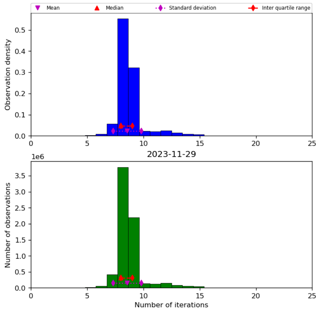
Figure 24: Histogram of “Number of iterations” for 2023-11-28 to 2023-11-30
