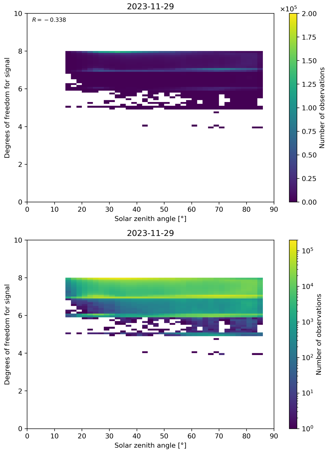
Figure 65: Scatter density plot of “Solar zenith angle” against “Degrees of freedom for signal” for 2023-11-28 to 2023-11-30.
