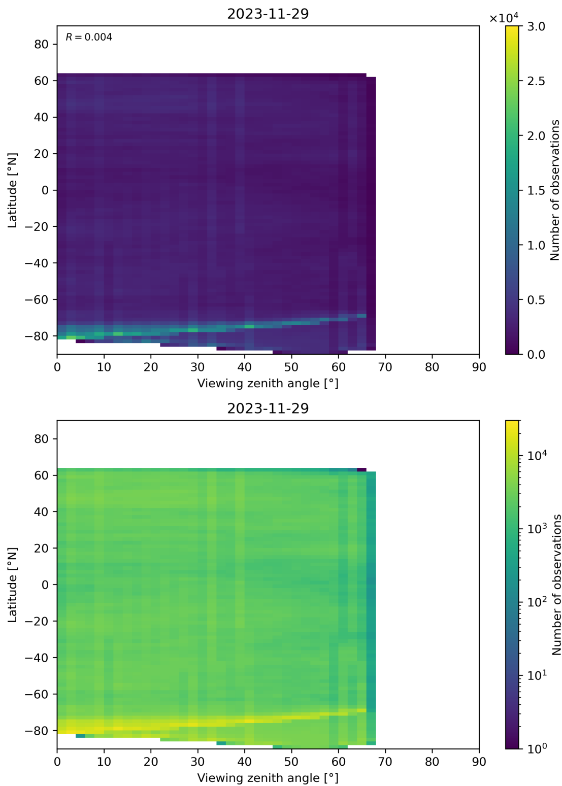
Figure 74: Scatter density plot of “Viewing zenith angle” against “Latitude” for 2023-11-28 to 2023-11-30.
