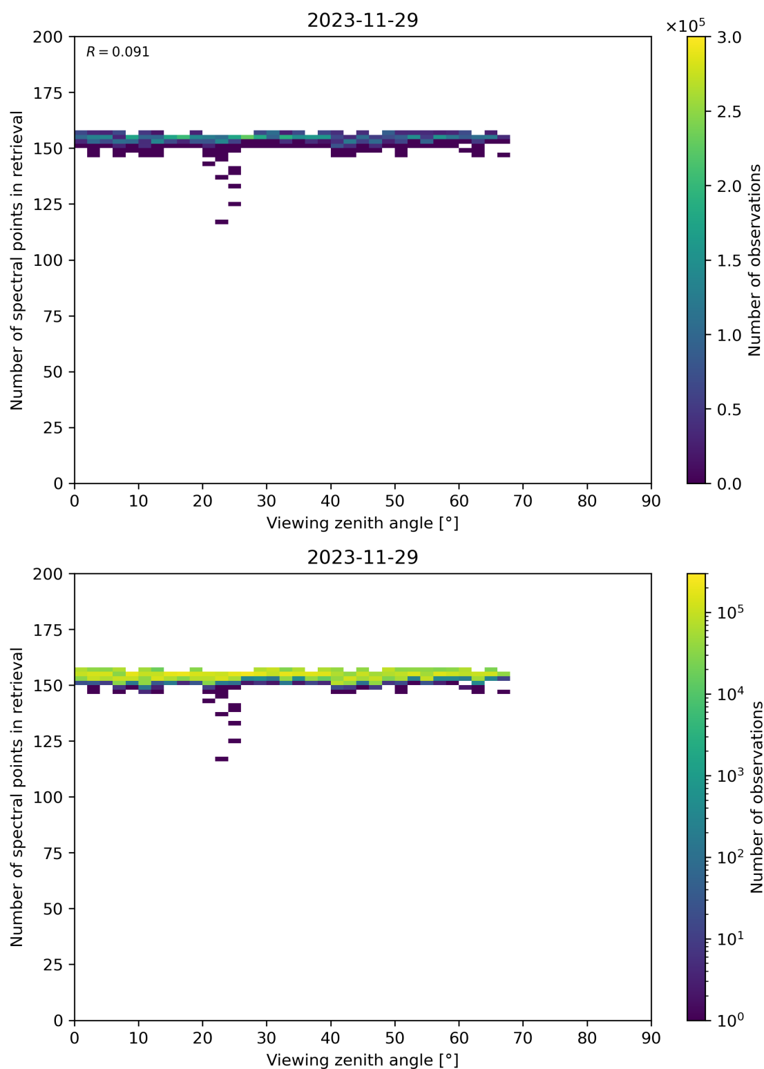
Figure 76: Scatter density plot of “Viewing zenith angle” against “Number of spectral points in retrieval” for 2023-11-28 to 2023-11-30.
