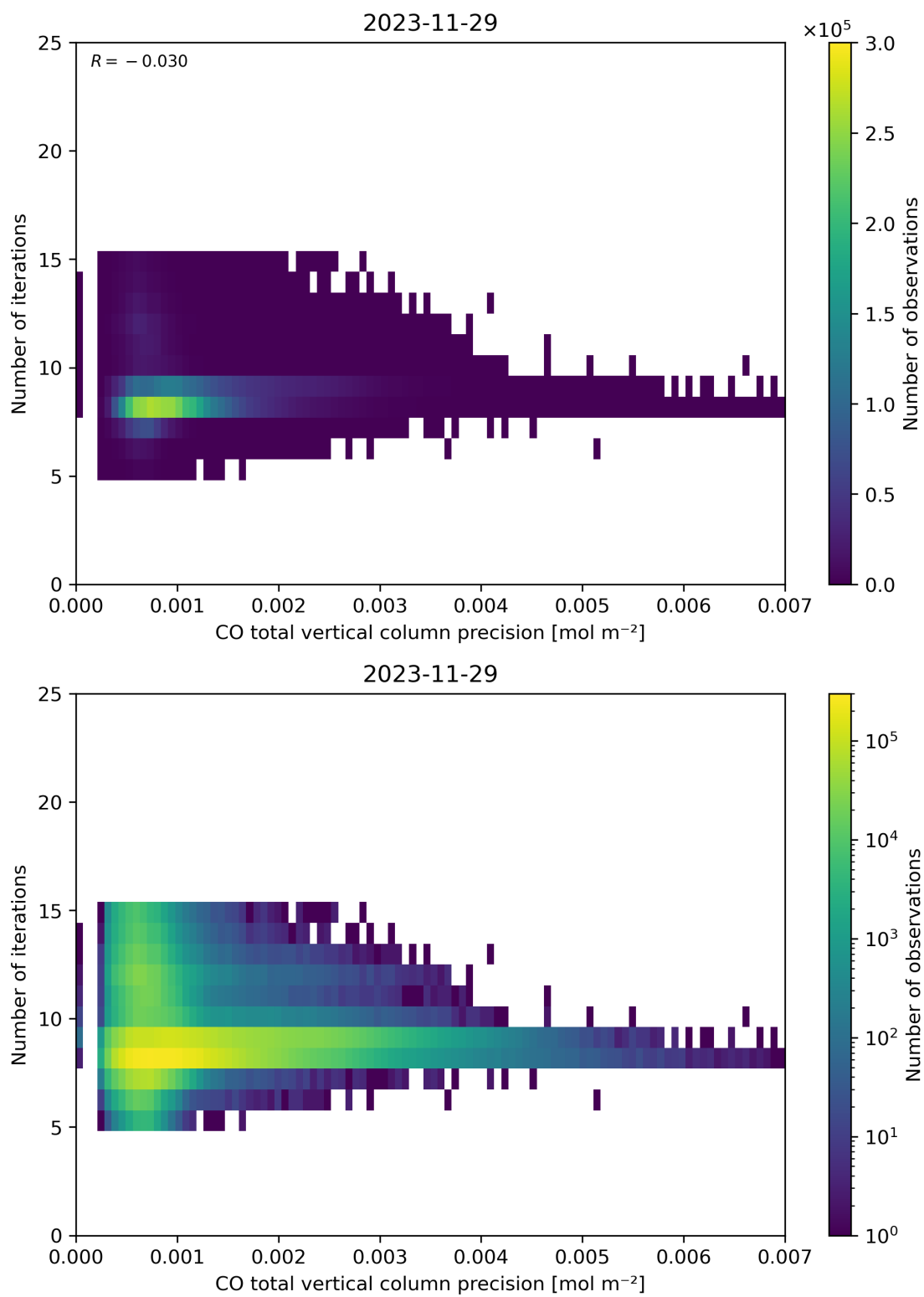
Figure 46: Scatter density plot of “CO total vertical column precision” against “Number of iterations” for 2023-11-28 to 2023-11-30.
