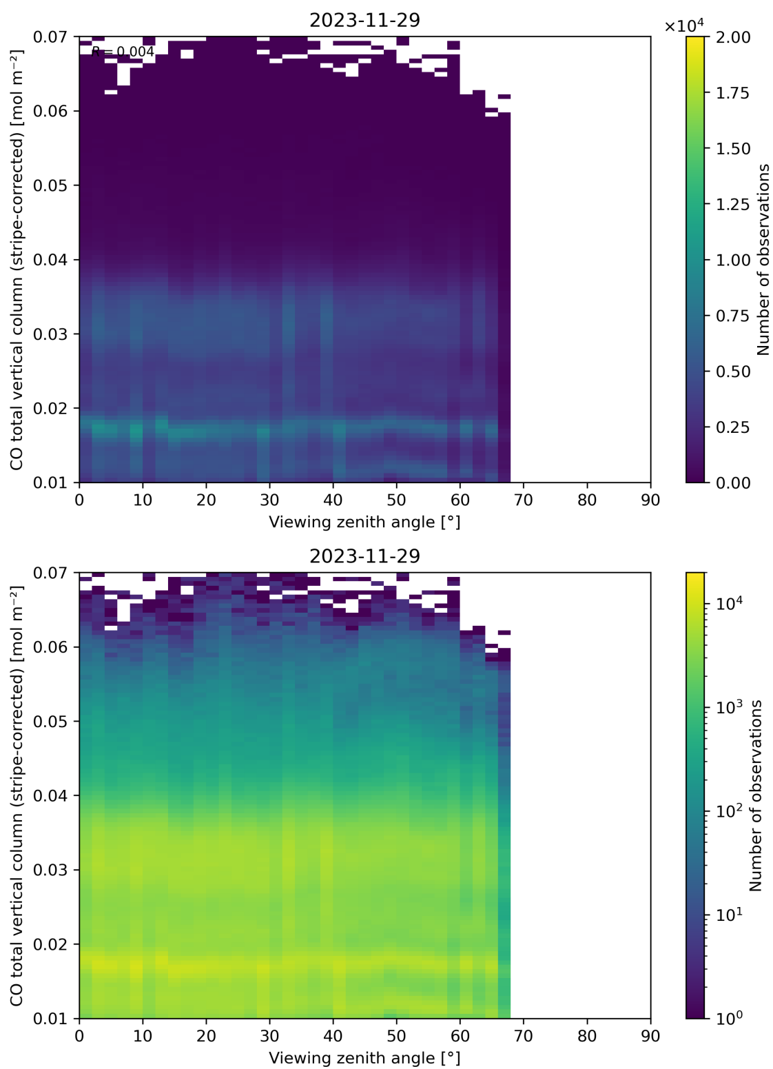
Figure 70: Scatter density plot of “Viewing zenith angle” against “CO total vertical column (stripe-corrected)” for 2023-11-28 to 2023-11-30.
