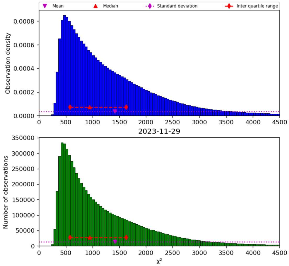
Figure 22: Histogram of “ \chi^2 ” for 2023-11-28 to 2023-11-30
