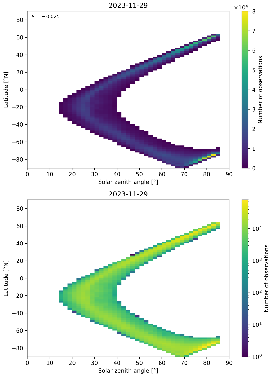
Figure 66: Scatter density plot of “Solar zenith angle” against “Latitude” for 2023-11-28 to 2023-11-30.
