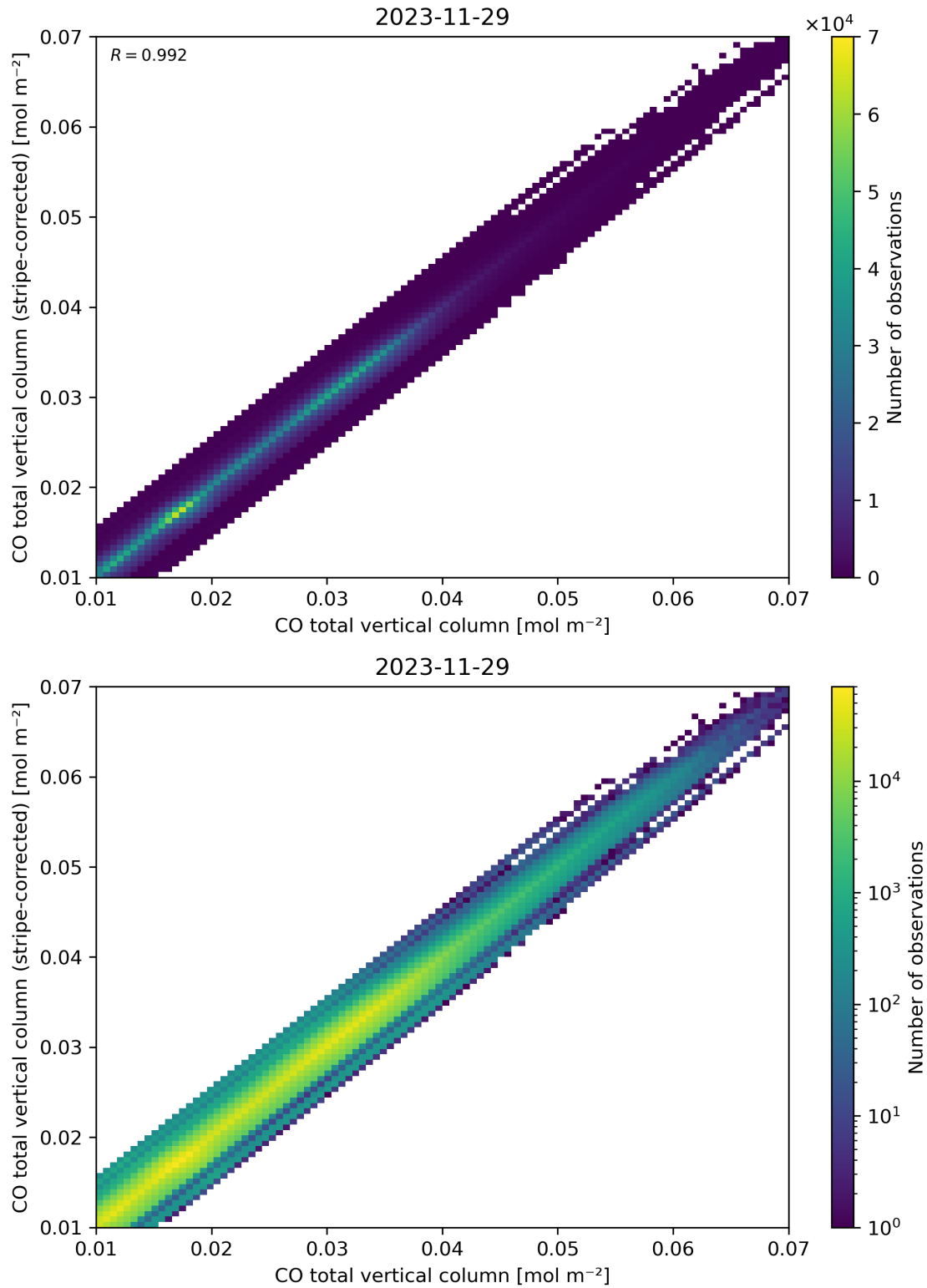
Figure 33: Scatter density plot of “CO total vertical column” against “CO total vertical column (stripe-corrected)” for 2023-11-28 to 2023-11-30.
