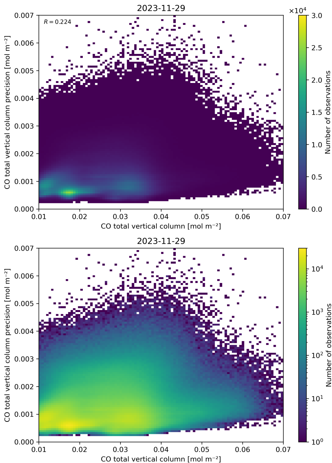
Figure 34: Scatter density plot of “CO total vertical column” against “CO total vertical column precision” for 2023-11-28 to 2023-11-30.
