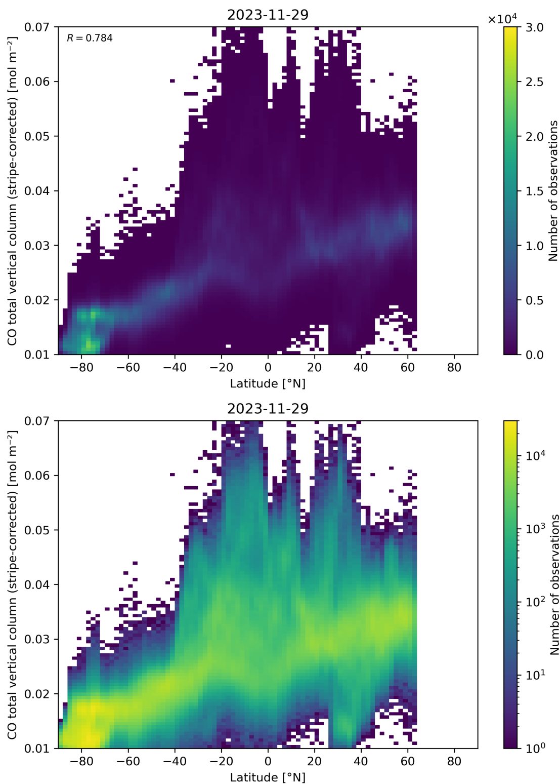
Figure 52: Scatter density plot of “Latitude” against “CO total vertical column (stripe-corrected)” for 2023-11-28 to 2023-11-30.
