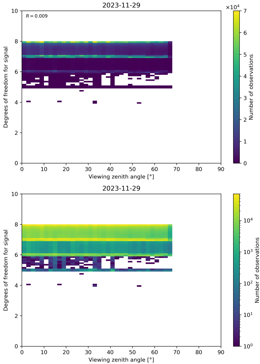
Figure 73: Scatter density plot of “Viewing zenith angle” against “Degrees of freedom for signal” for 2023-11-28 to 2023-11-30.
