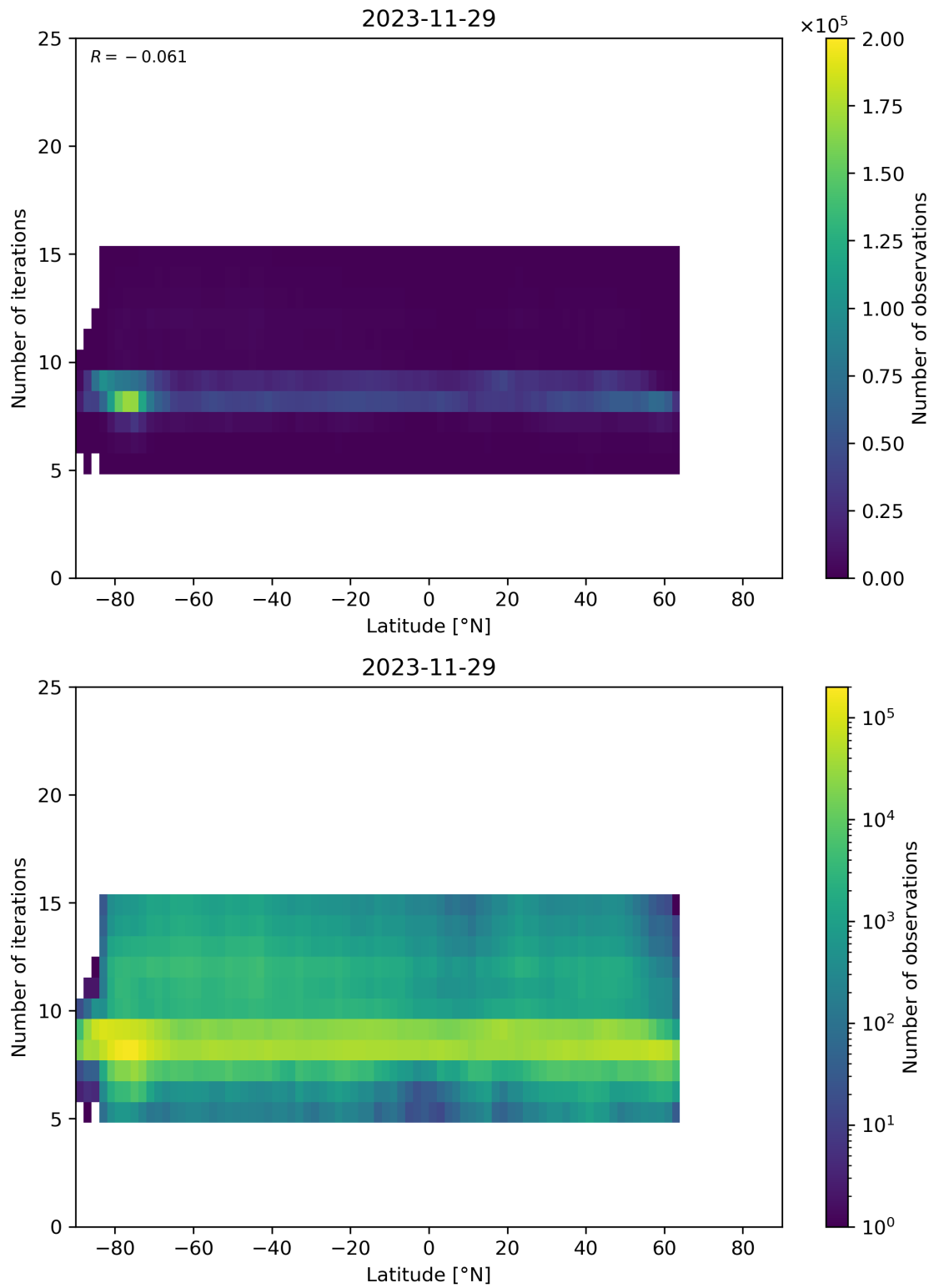
Figure 56: Scatter density plot of “Latitude” against “Number of iterations” for 2023-11-28 to 2023-11-30.
