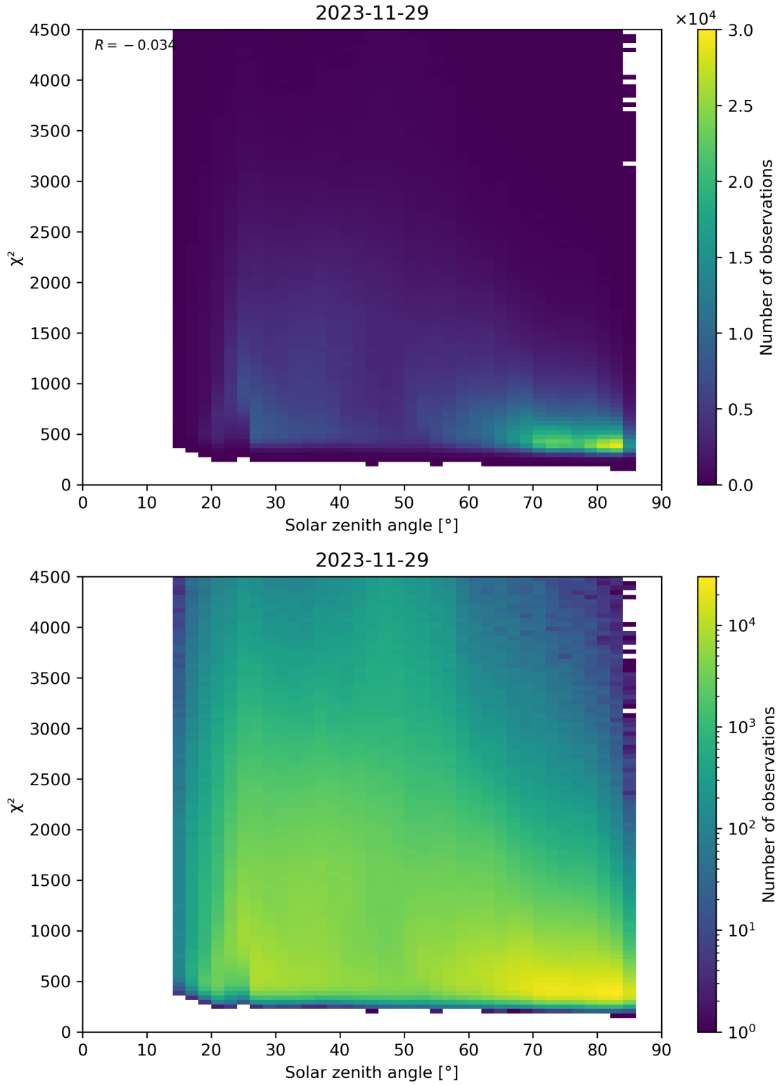
Figure 64: Scatter density plot of “Solar zenith angle” against “ \chi^2 ” for 2023-11-28 to 2023-11-30.
