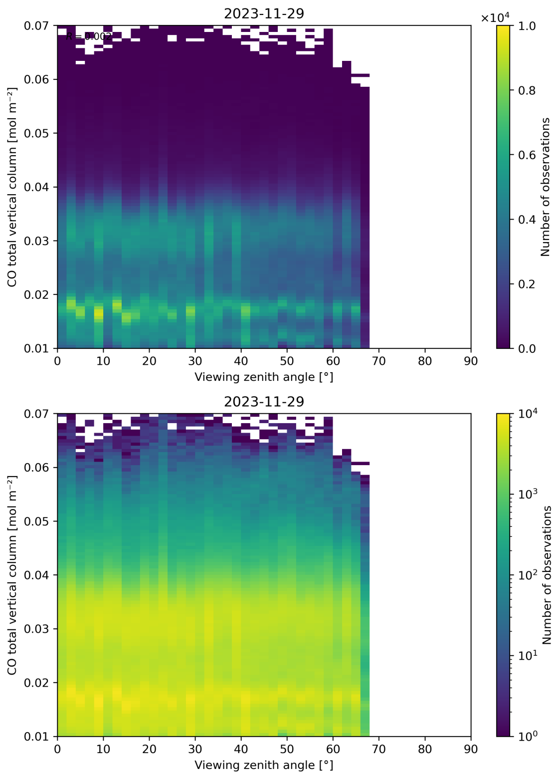
Figure 69: Scatter density plot of “Viewing zenith angle” against “CO total vertical column” for 2023-11-28 to 2023-11-30.
