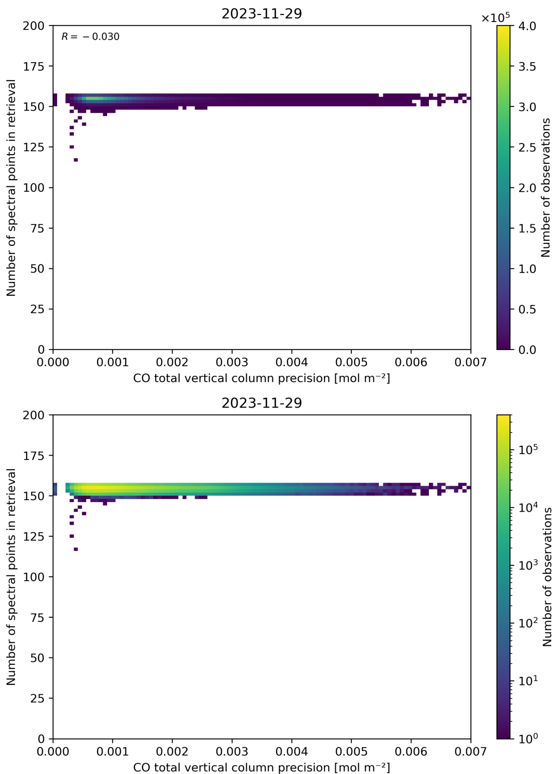
Figure 47: Scatter density plot of “CO total vertical column precision” against “Number of spectral points in retrieval” for 2023-11-28 to 2023-11-30.
