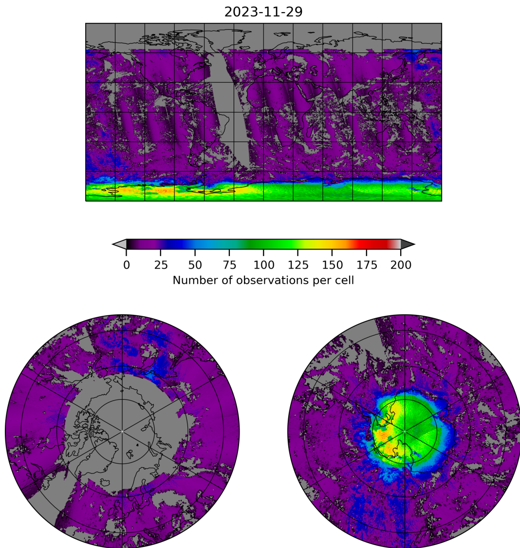
Figure 8: Map of the number of observations for 2023-11-28 to 2023-11-30
