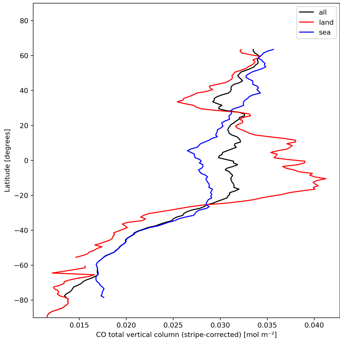
Figure 11: Zonal average of “CO total vertical column (stripe-corrected)” for 2023-11-28 to 2023-11-30.
