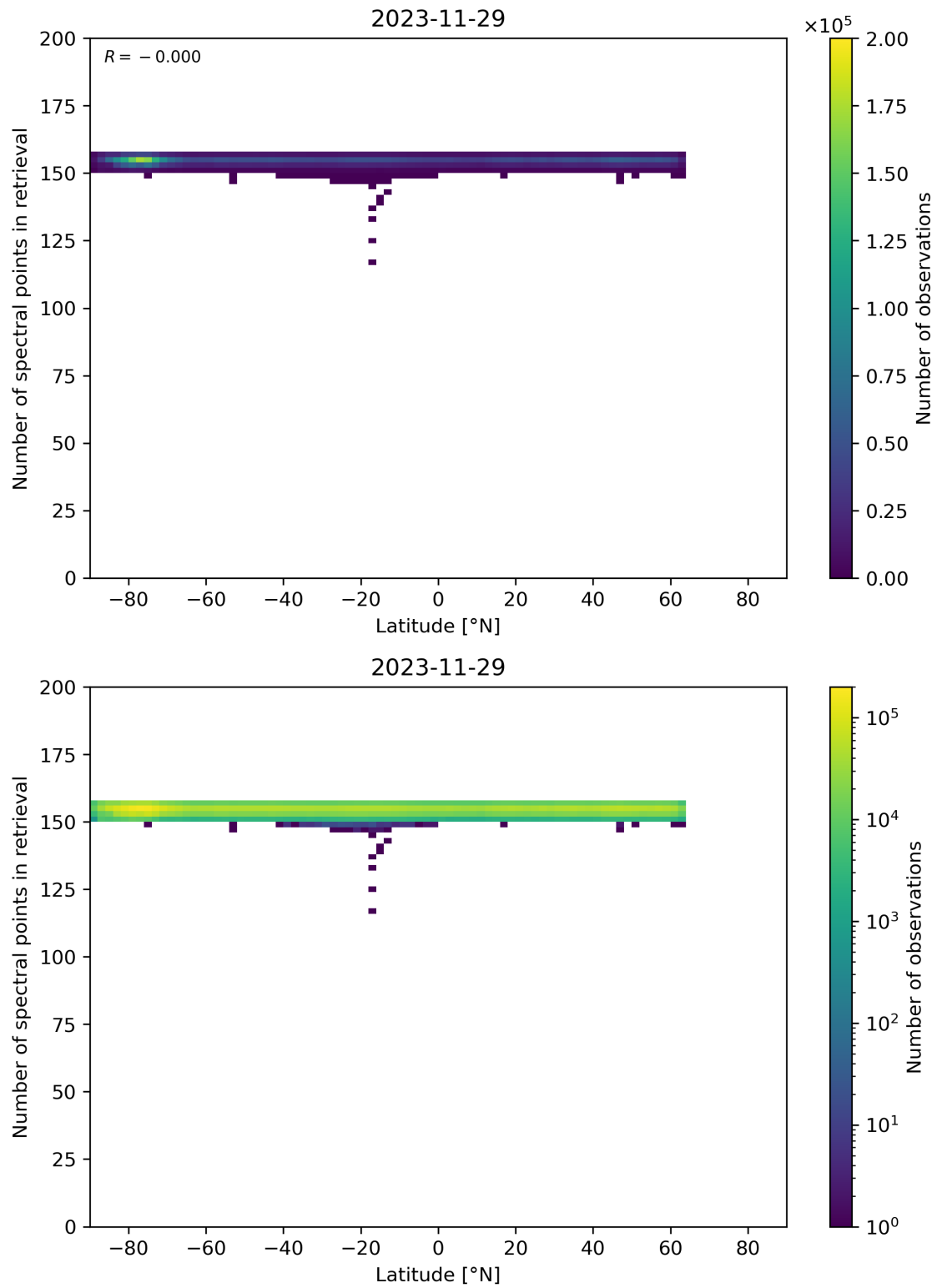
Figure 57: Scatter density plot of “Latitude” against “Number of spectral points in retrieval” for 2023-11-28 to 2023-11-30.
