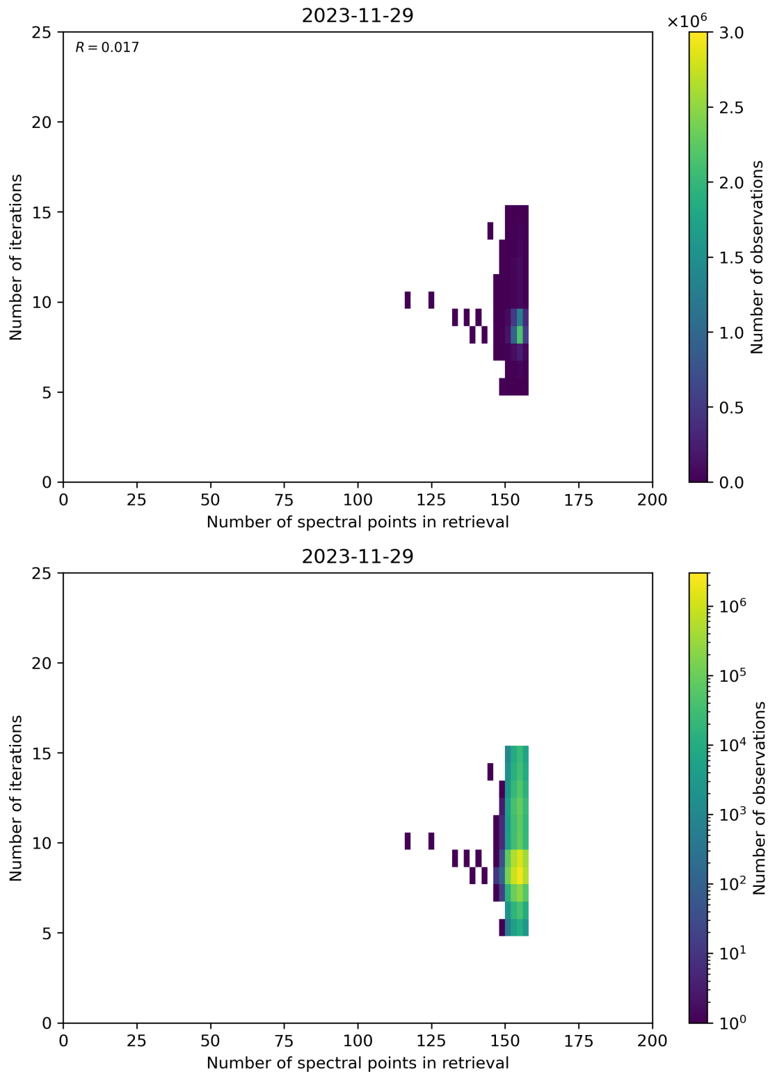
Figure 60: Scatter density plot of “Number of spectral points in retrieval” against “Number of iterations” for 2023-11-28 to 2023-11-30.
