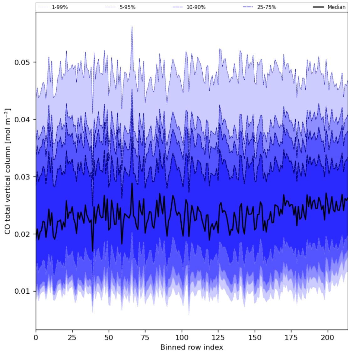
Figure 26: Along track statistics of “CO total vertical column” for 2023-11-28 to 2023-11-30
