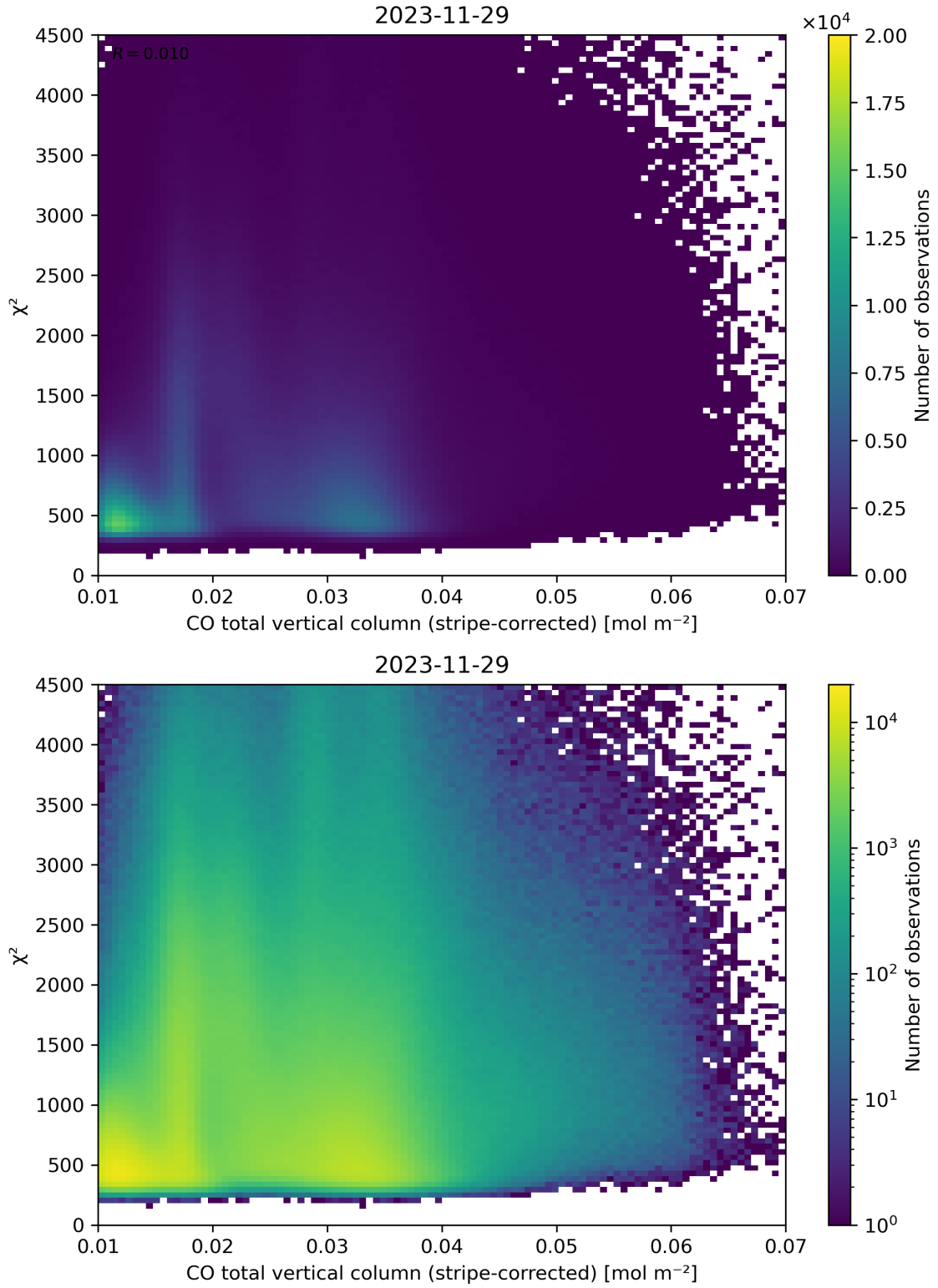
Figure 37: Scatter density plot of “CO total vertical column (stripe-corrected)” against “ \chi^2 ” for 2023-11-28 to 2023-11-30.
