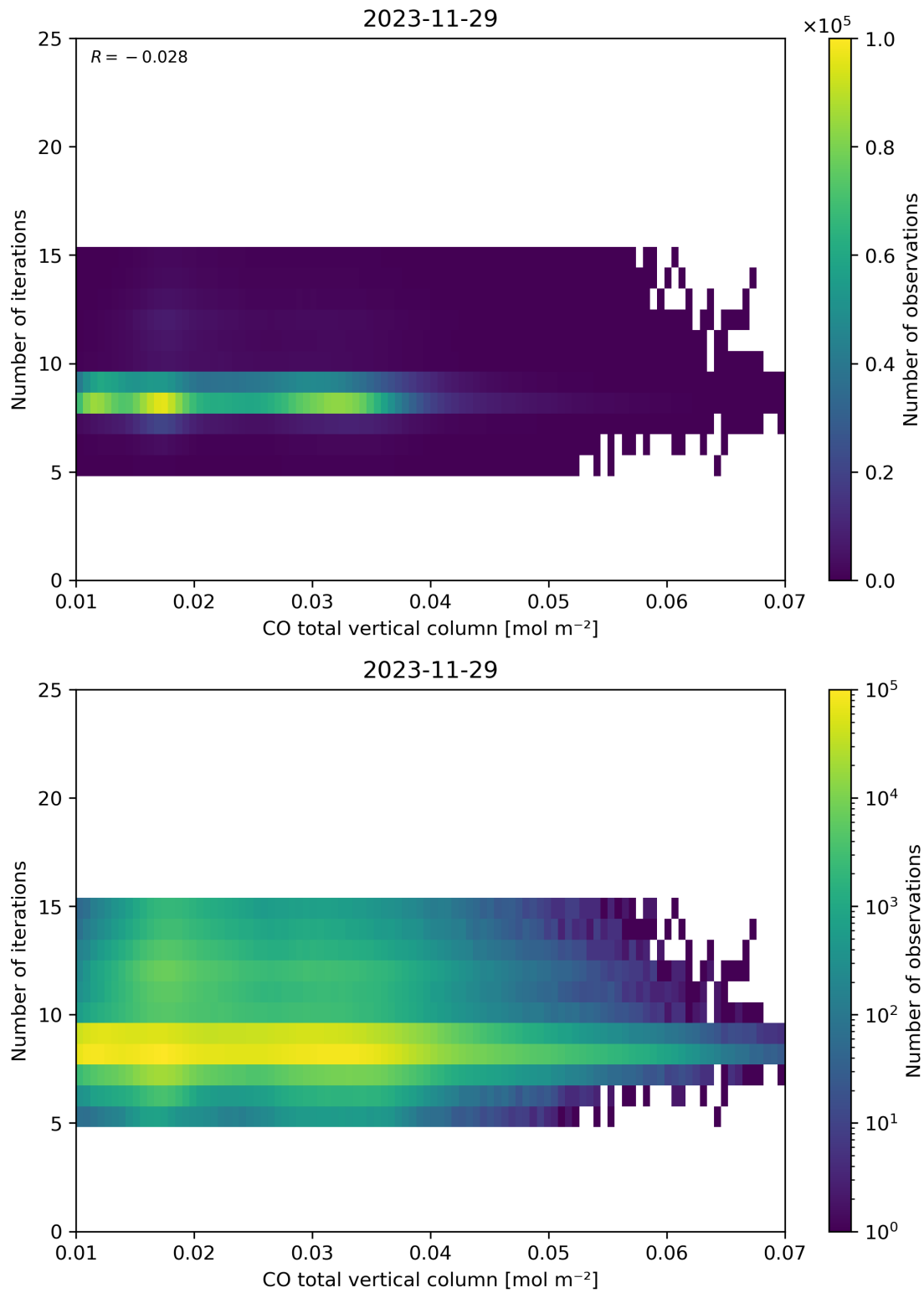
Figure 42: Scatter density plot of “CO total vertical column” against “Number of iterations” for 2023-11-28 to 2023-11-30.
