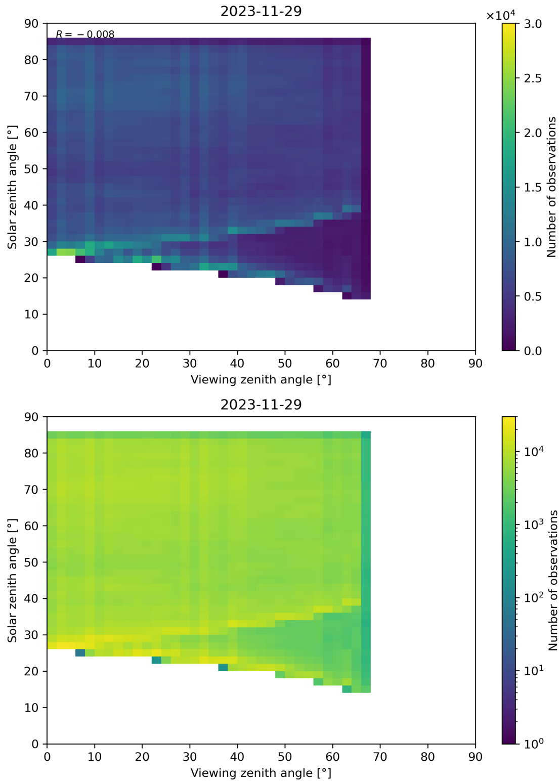
Figure 77: Scatter density plot of “Viewing zenith angle” against “Solar zenith angle” for 2023-11-28 to 2023-11-30.
