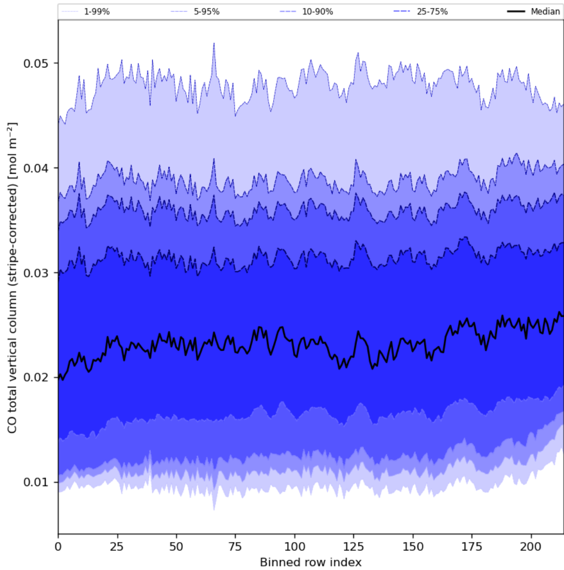
Figure 27: Along track statistics of “CO total vertical column (stripe-corrected)” for 2023-11-28 to 2023-11-30
