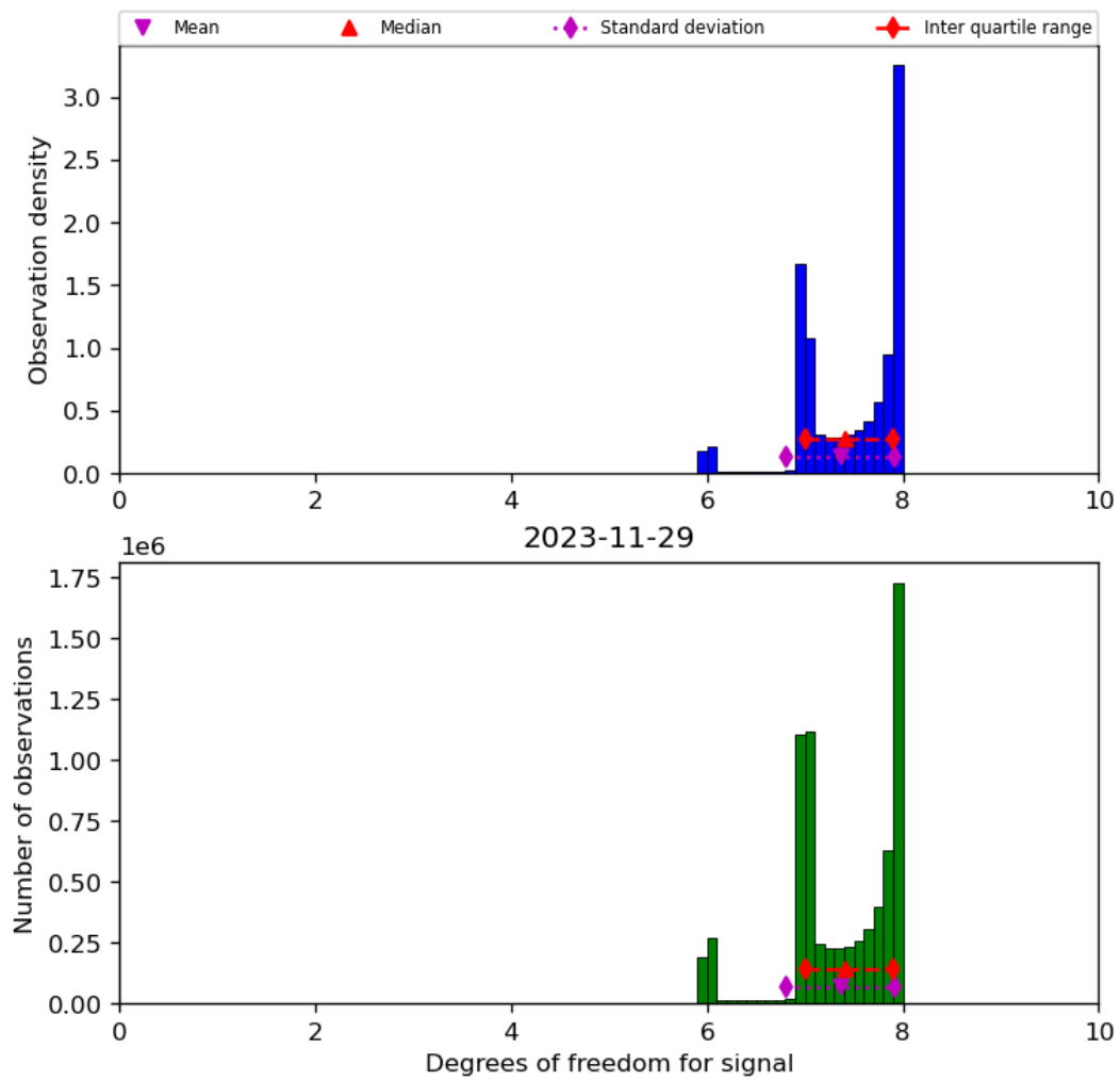
Figure 23: Histogram of “Degrees of freedom for signal” for 2023-11-28 to 2023-11-30
