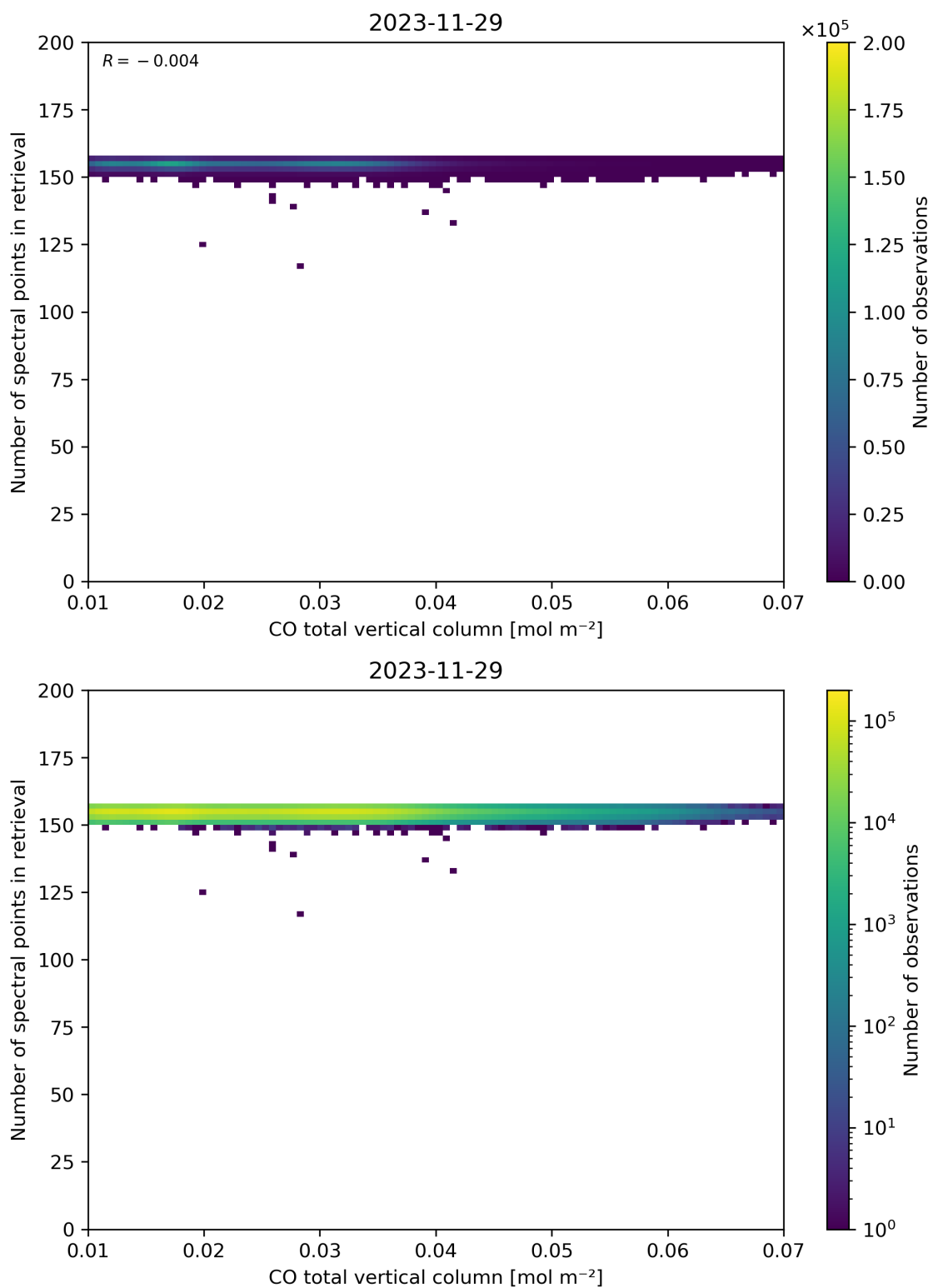
Figure 43: Scatter density plot of “CO total vertical column” against “Number of spectral points in retrieval” for 2023-11-28 to 2023-11-30.
