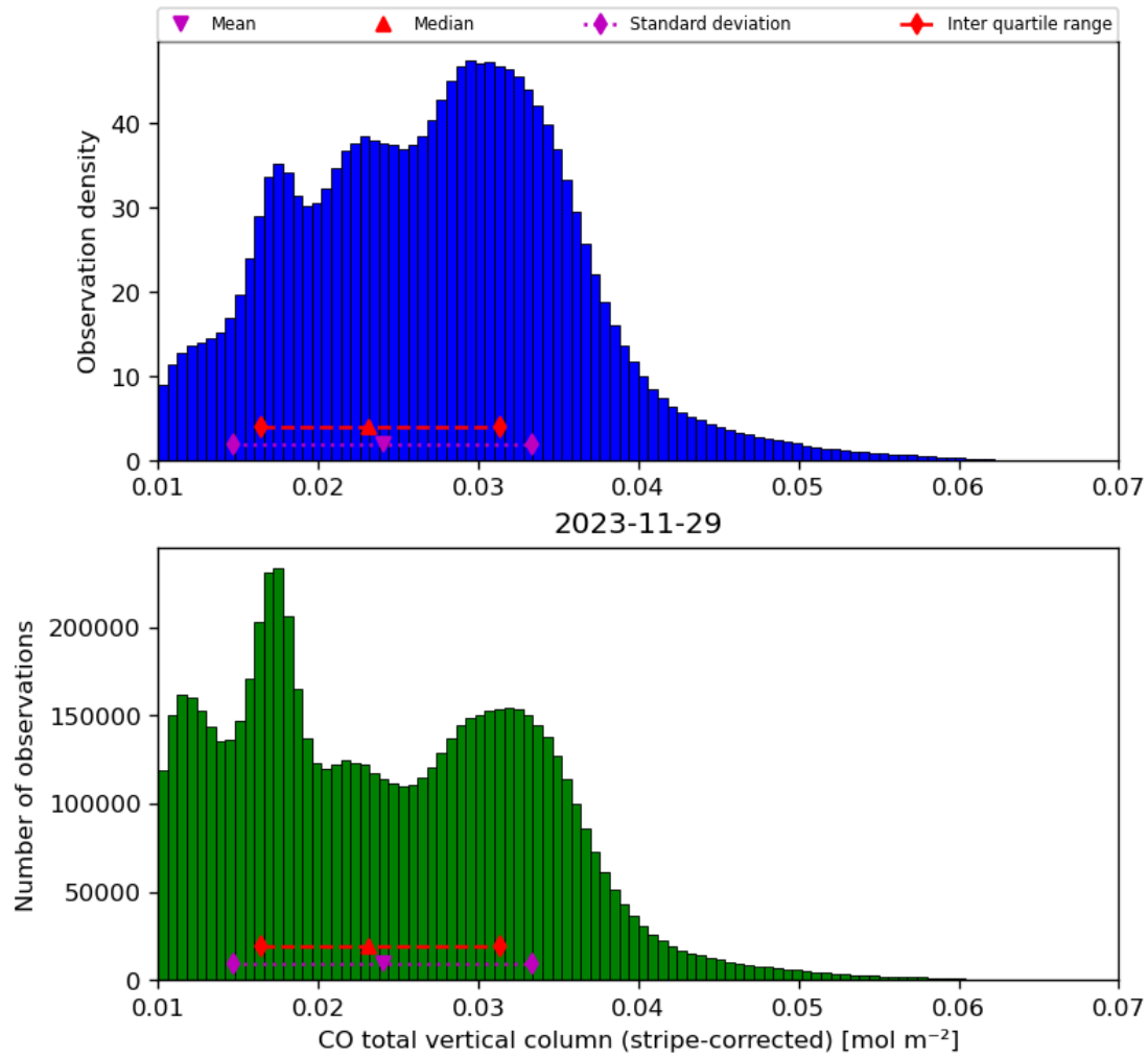
Figure 19: Histogram of “CO total vertical column (stripe-corrected)” for 2023-11-28 to 2023-11-30
