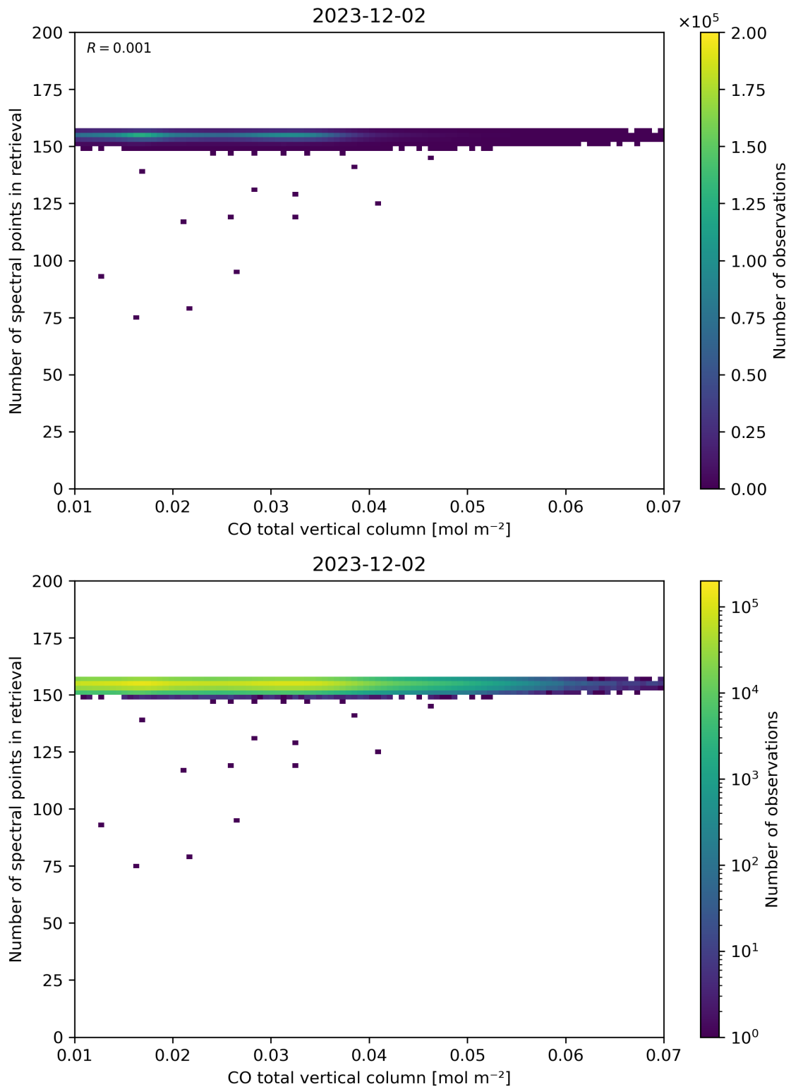
Figure 43: Scatter density plot of “CO total vertical column” against “Number of spectral points in retrieval” for 2023-12-01 to 2023-12-03.
