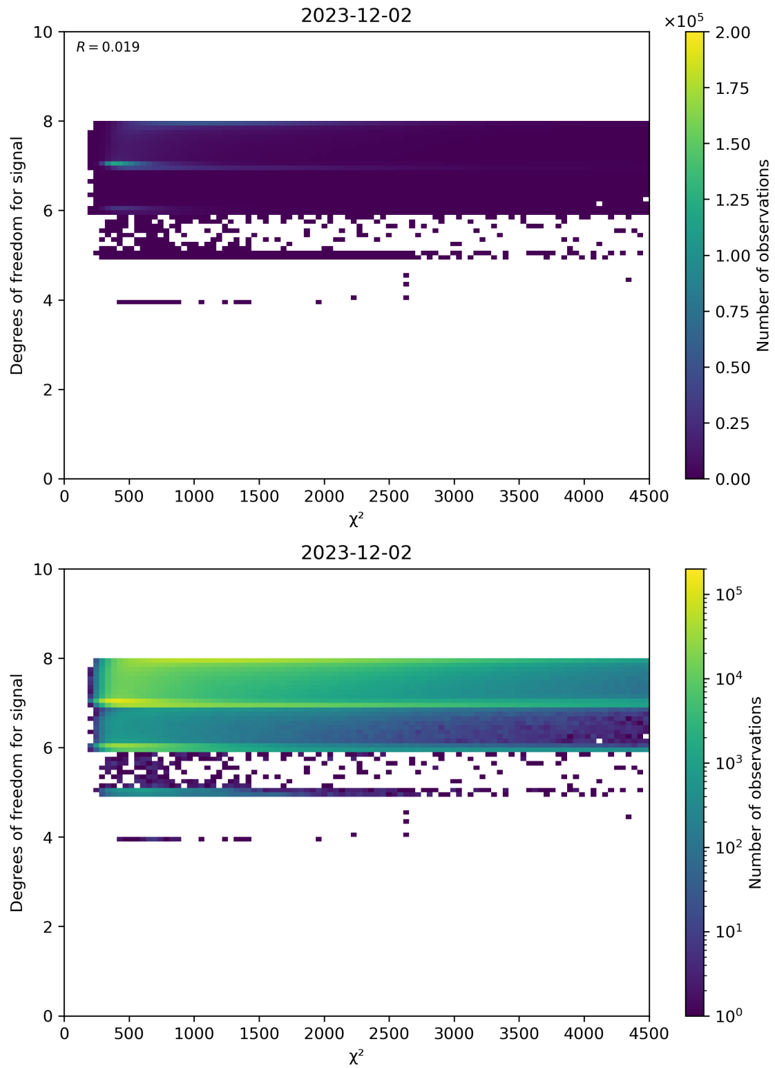
Figure 48: Scatter density plot of “ \chi^2 ” against “Degrees of freedom for signal” for 2023-12-01 to 2023-12-03.
