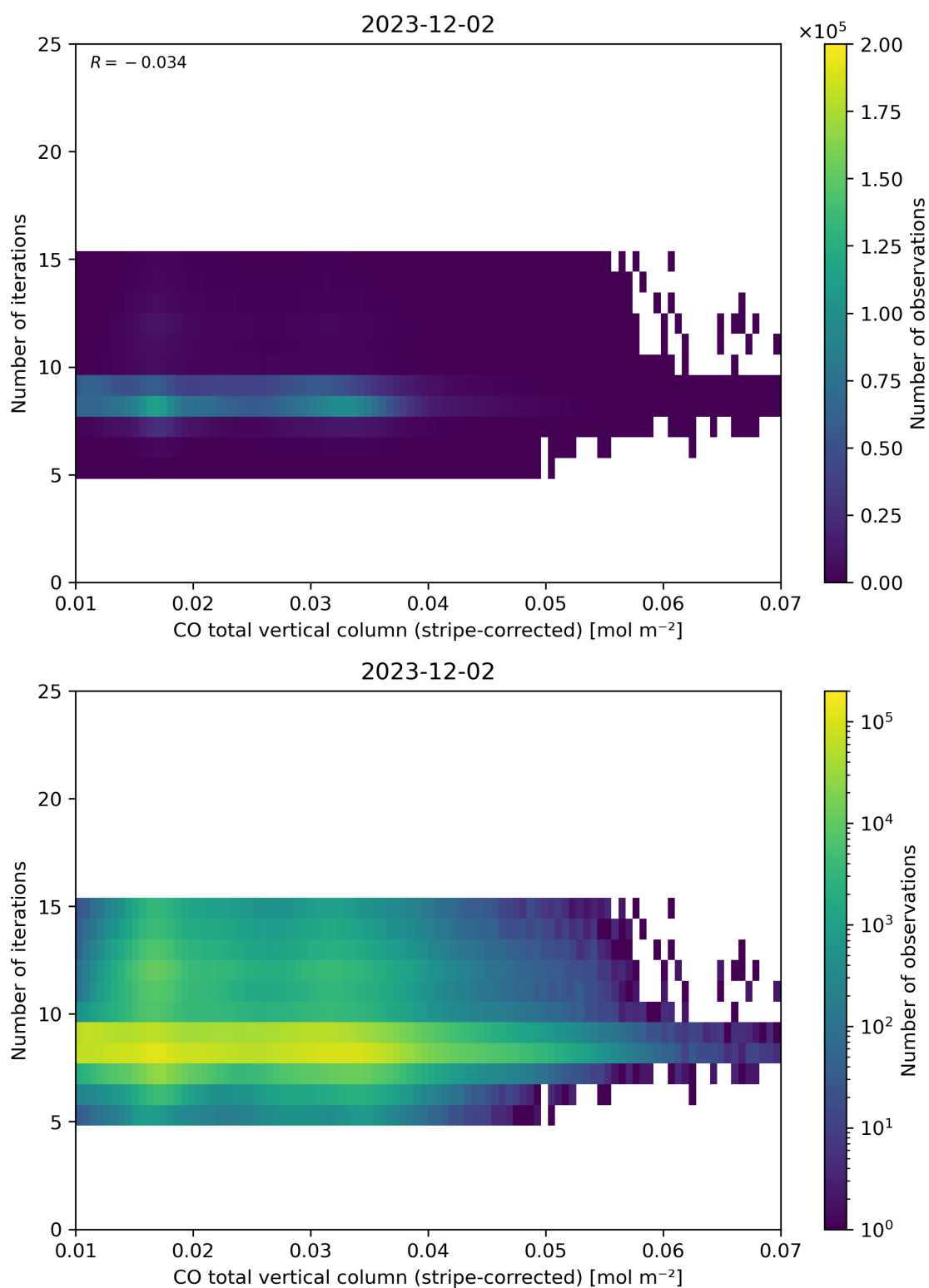
Figure 39: Scatter density plot of “CO total vertical column (stripe-corrected)” against “Number of iterations” for 2023-12-01 to 2023-12-03.
