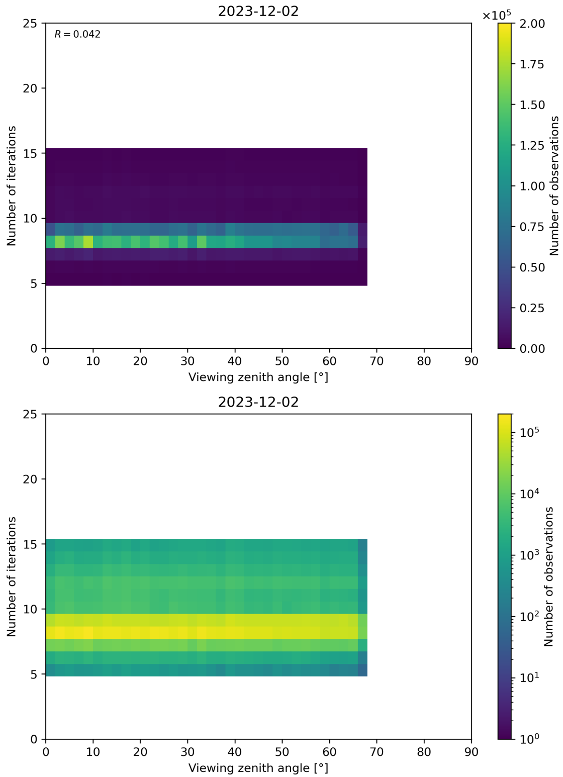
Figure 75: Scatter density plot of “Viewing zenith angle” against “Number of iterations” for 2023-12-01 to 2023-12-03.
