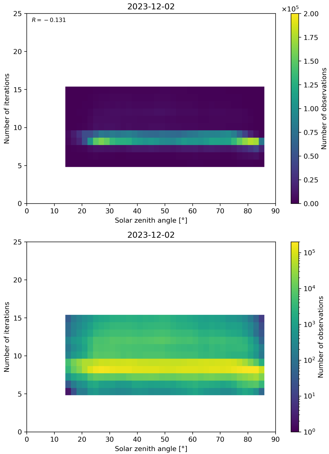
Figure 67: Scatter density plot of “Solar zenith angle” against “Number of iterations” for 2023-12-01 to 2023-12-03.
