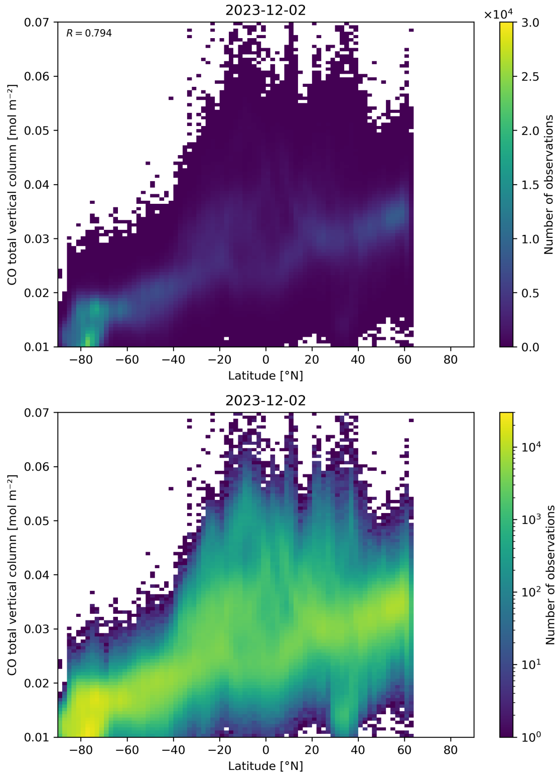
Figure 51: Scatter density plot of “Latitude” against “CO total vertical column” for 2023-12-01 to 2023-12-03.
