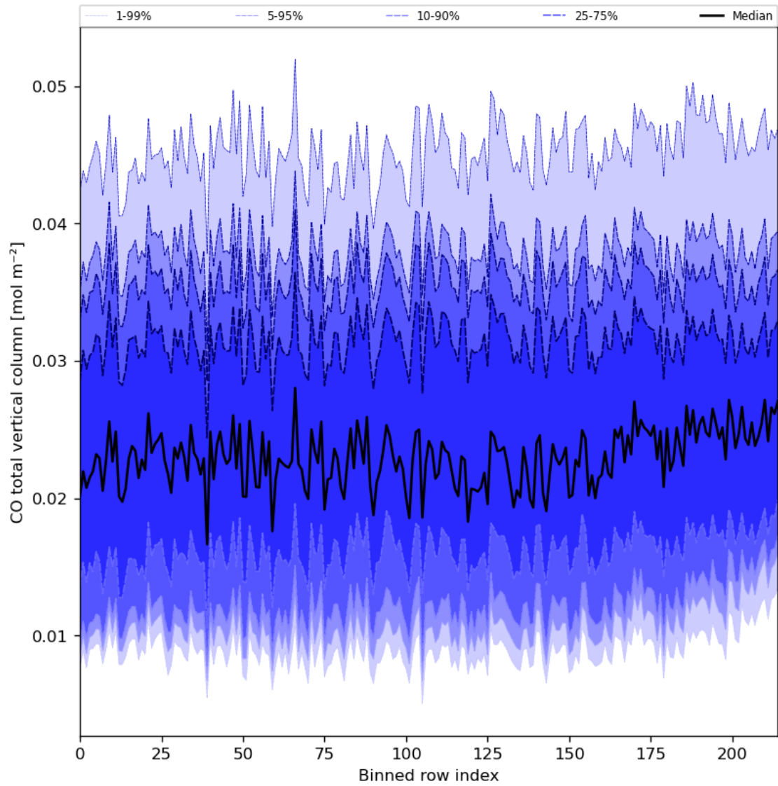
Figure 26: Along track statistics of “CO total vertical column” for 2023-12-01 to 2023-12-03
