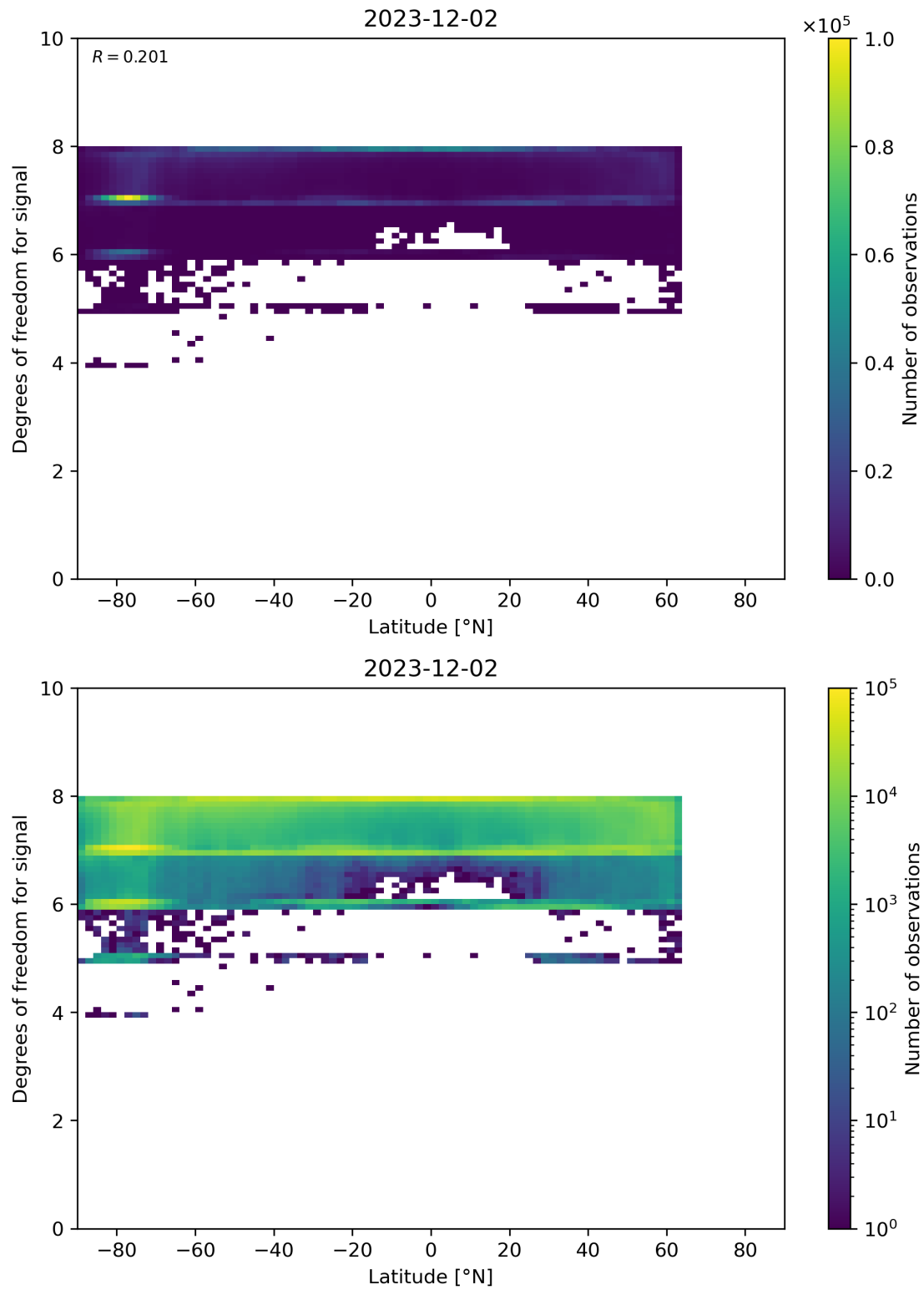
Figure 55: Scatter density plot of “Latitude” against “Degrees of freedom for signal” for 2023-12-01 to 2023-12-03.
