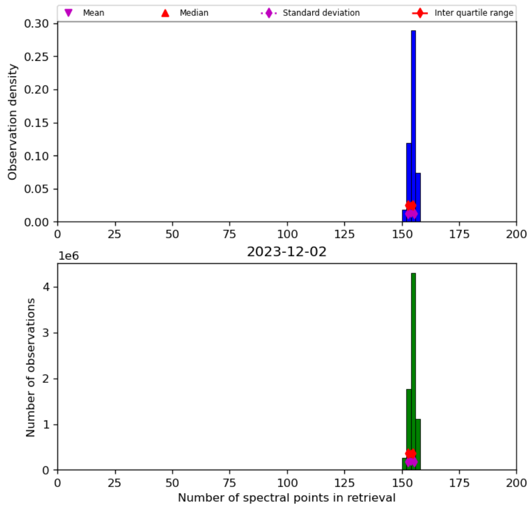
Figure 21: Histogram of “Number of spectral points in retrieval” for 2023-12-01 to 2023-12-03
