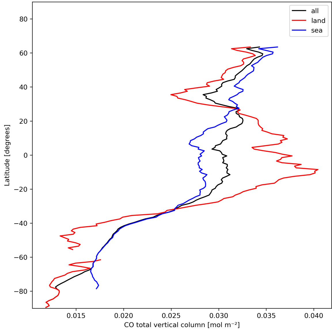
Figure 10: Zonal average of “CO total vertical column” for 2023-12-01 to 2023-12-03.
