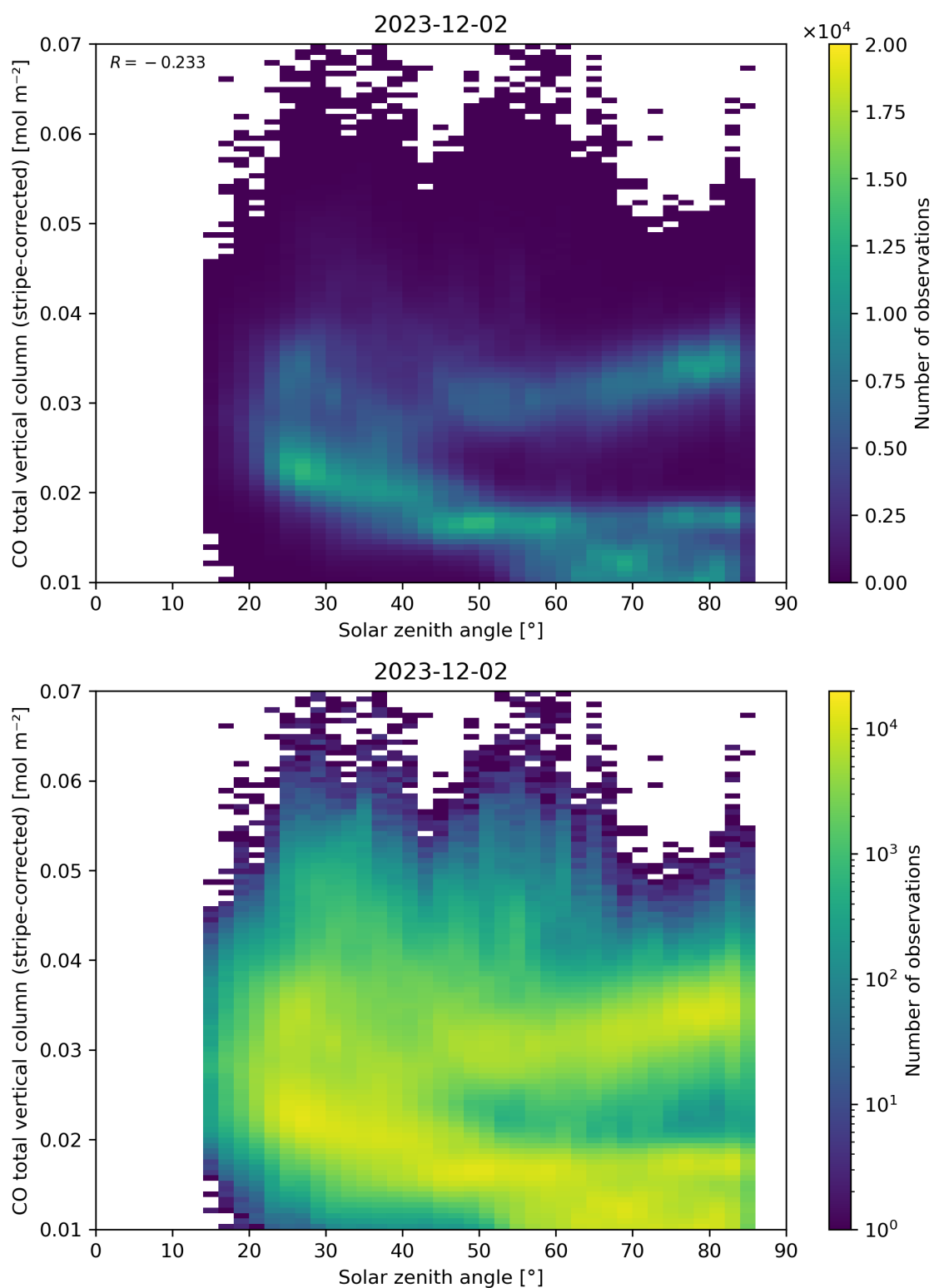
Figure 62: Scatter density plot of “Solar zenith angle” against “CO total vertical column (stripe-corrected)” for 2023-12-01 to 2023-12-03.
