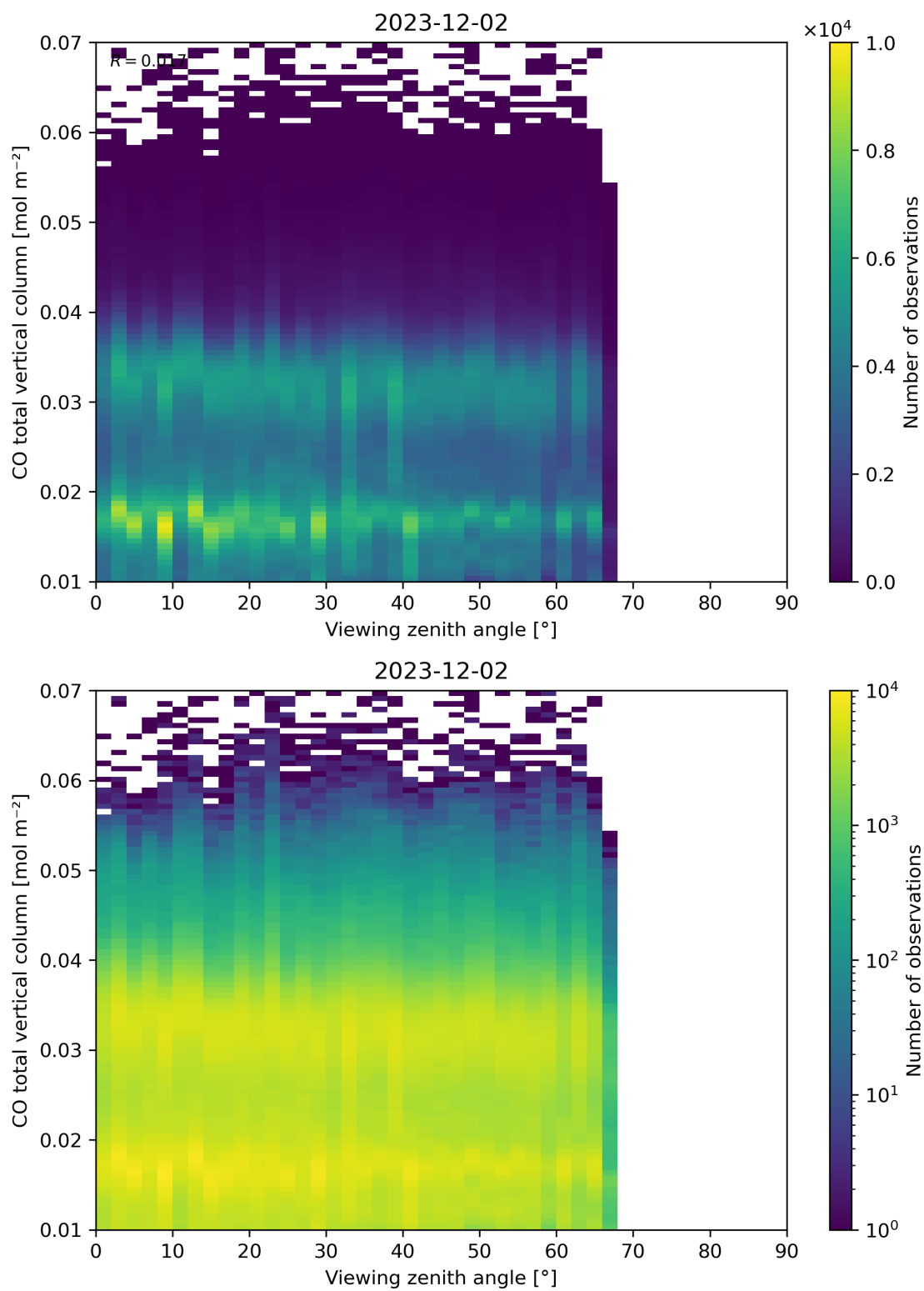
Figure 69: Scatter density plot of “Viewing zenith angle” against “CO total vertical column” for 2023-12-01 to 2023-12-03.
