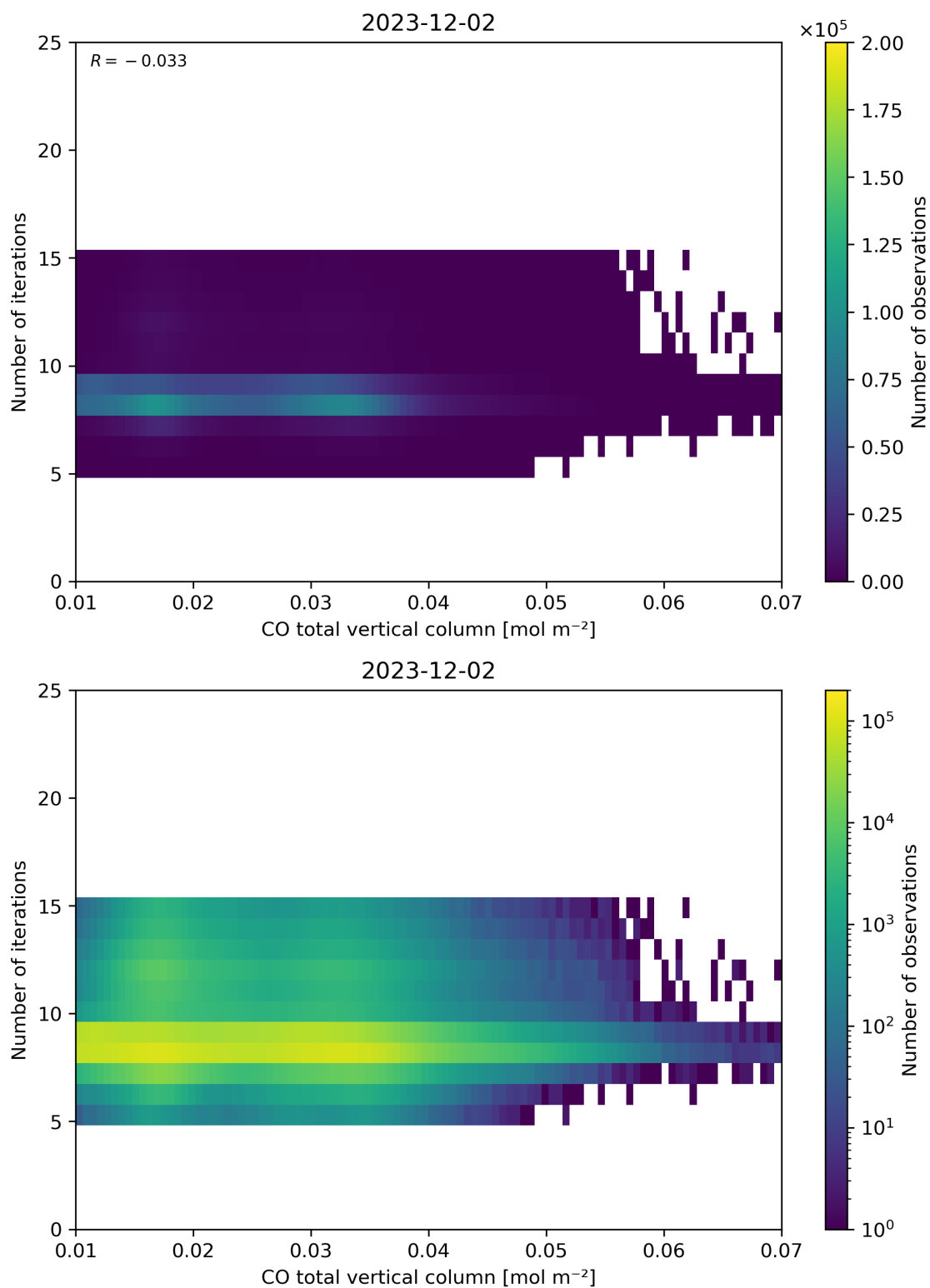
Figure 42: Scatter density plot of “CO total vertical column” against “Number of iterations” for 2023-12-01 to 2023-12-03.
