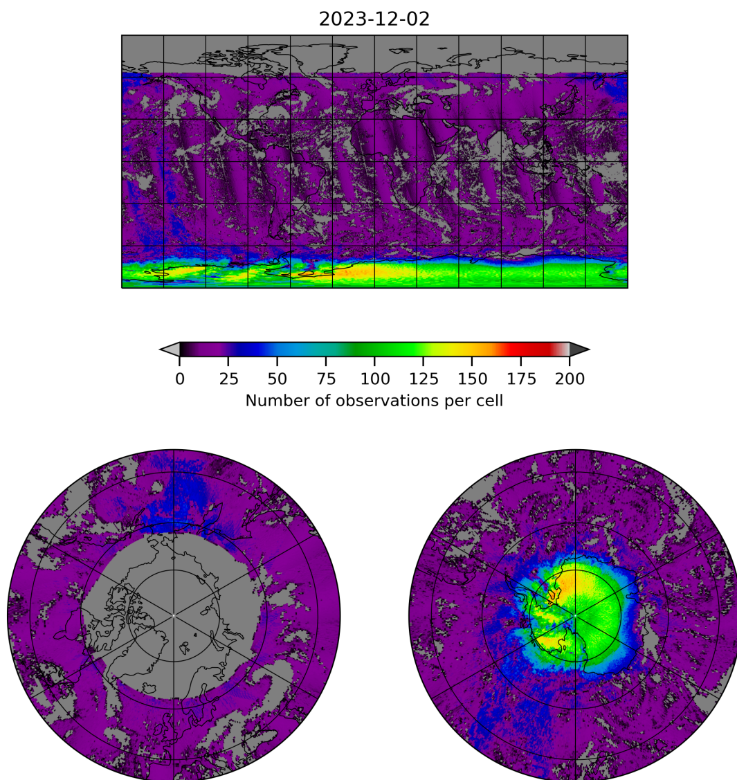
Figure 8: Map of the number of observations for 2023-12-01 to 2023-12-03
