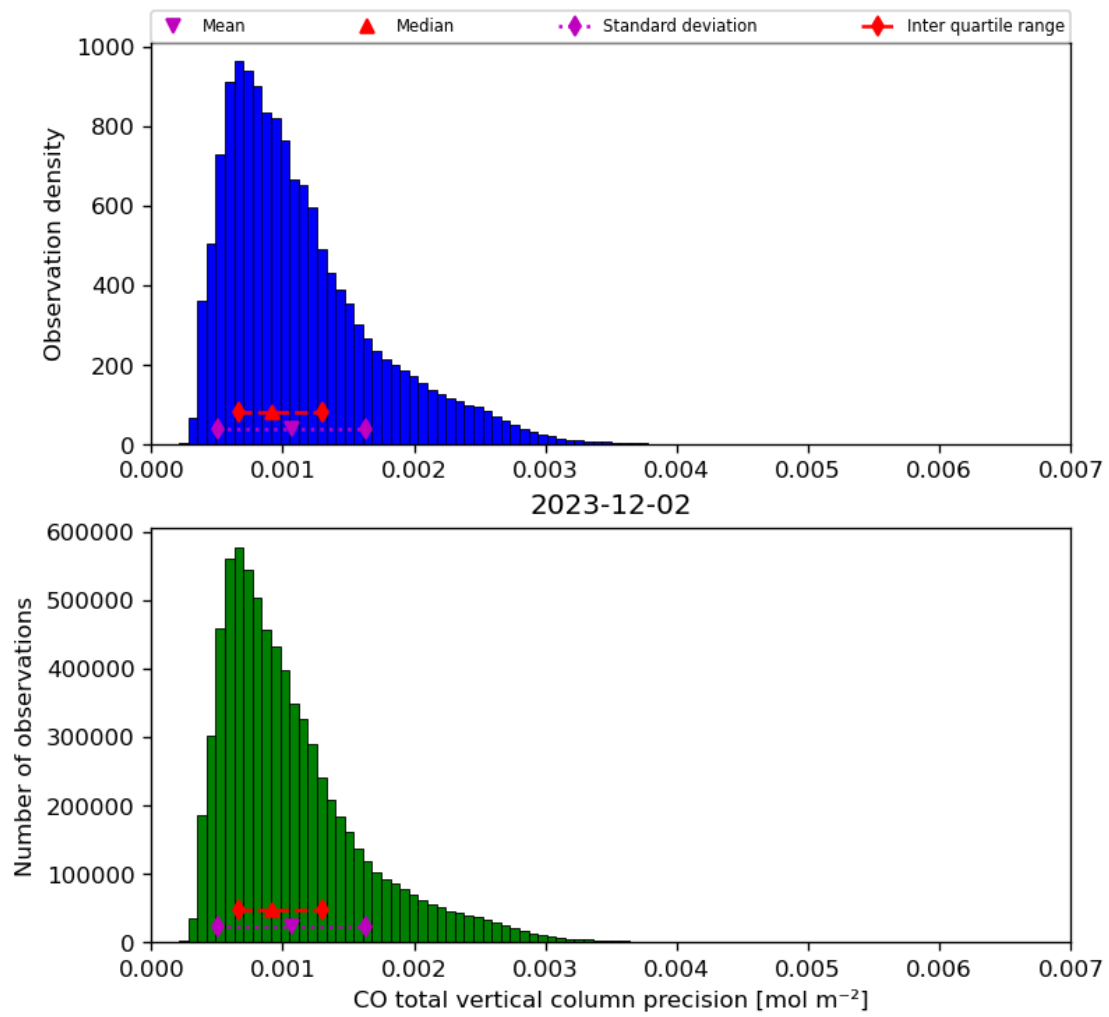
Figure 20: Histogram of “CO total vertical column precision” for 2023-12-01 to 2023-12-03
