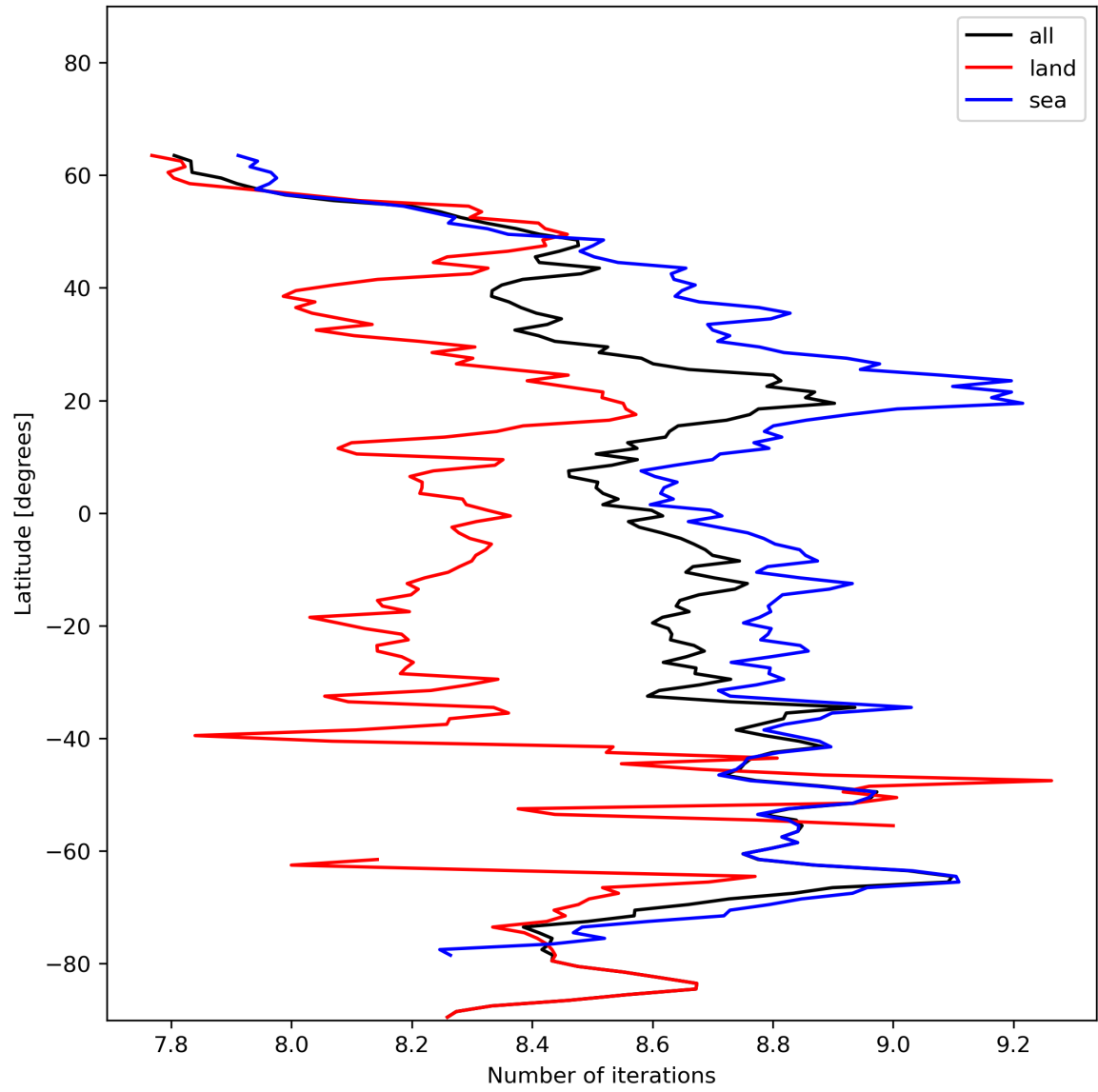
Figure 16: Zonal average of “Number of iterations” for 2023-12-01 to 2023-12-03.
