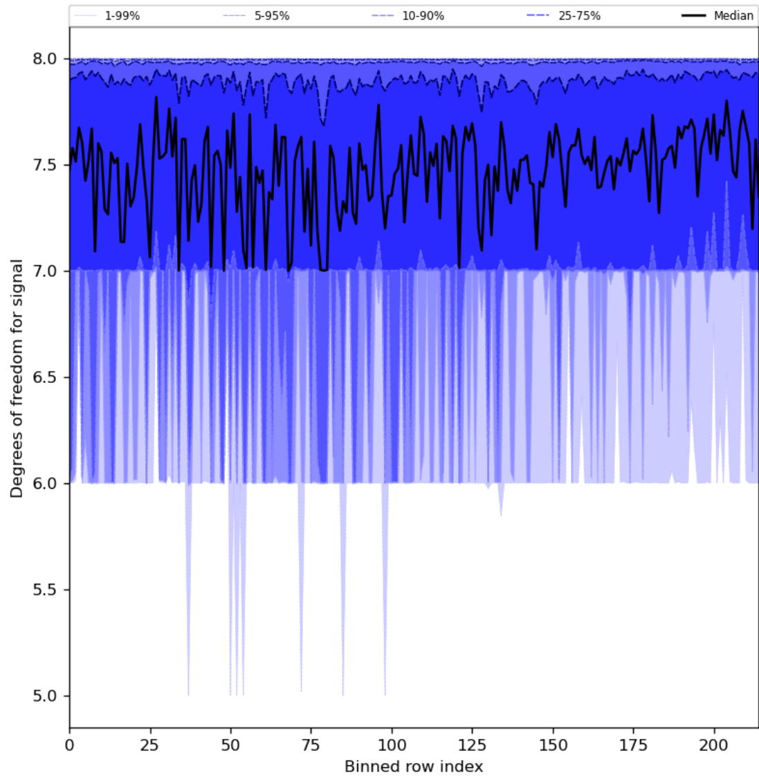
Figure 31: Along track statistics of “Degrees of freedom for signal” for 2023-12-01 to 2023-12-03
