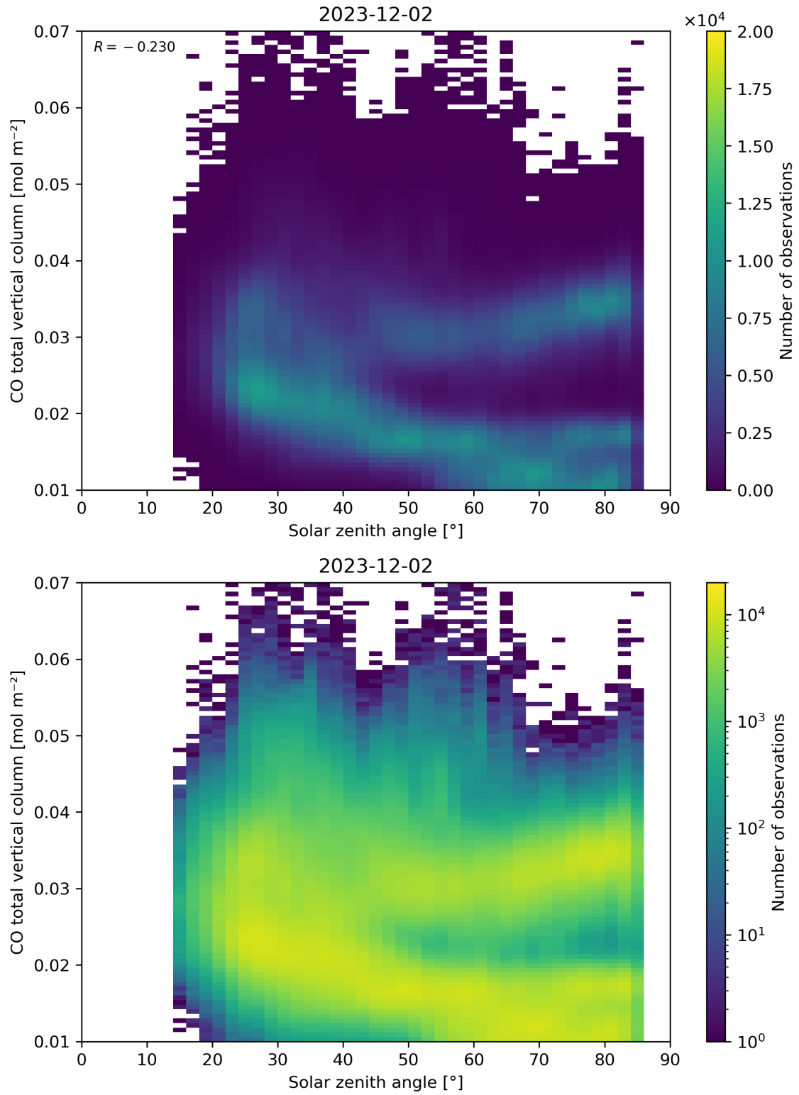
Figure 61: Scatter density plot of “Solar zenith angle” against “CO total vertical column” for 2023-12-01 to 2023-12-03.
