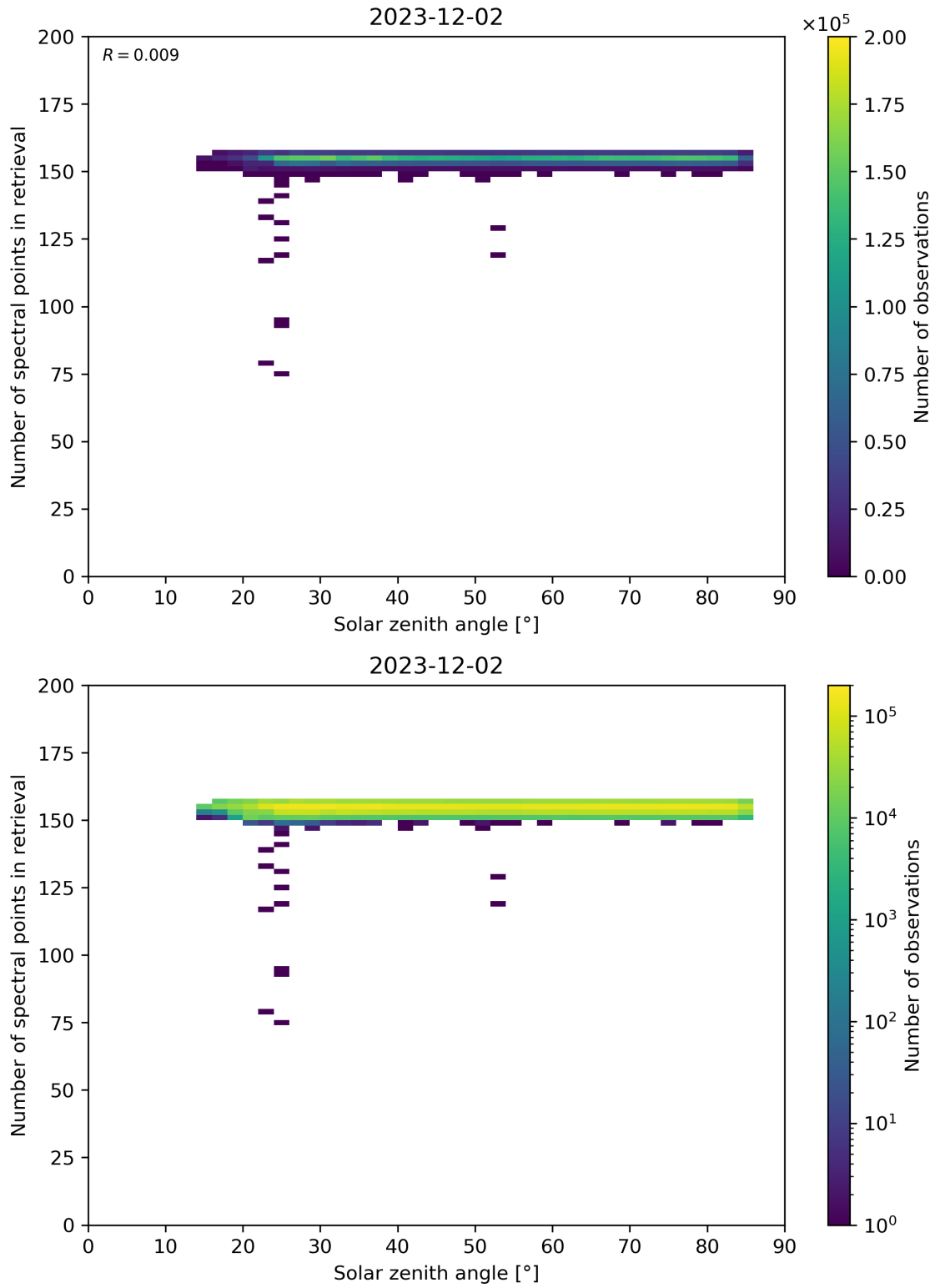
Figure 68: Scatter density plot of “Solar zenith angle” against “Number of spectral points in retrieval” for 2023-12-01 to 2023-12-03.
