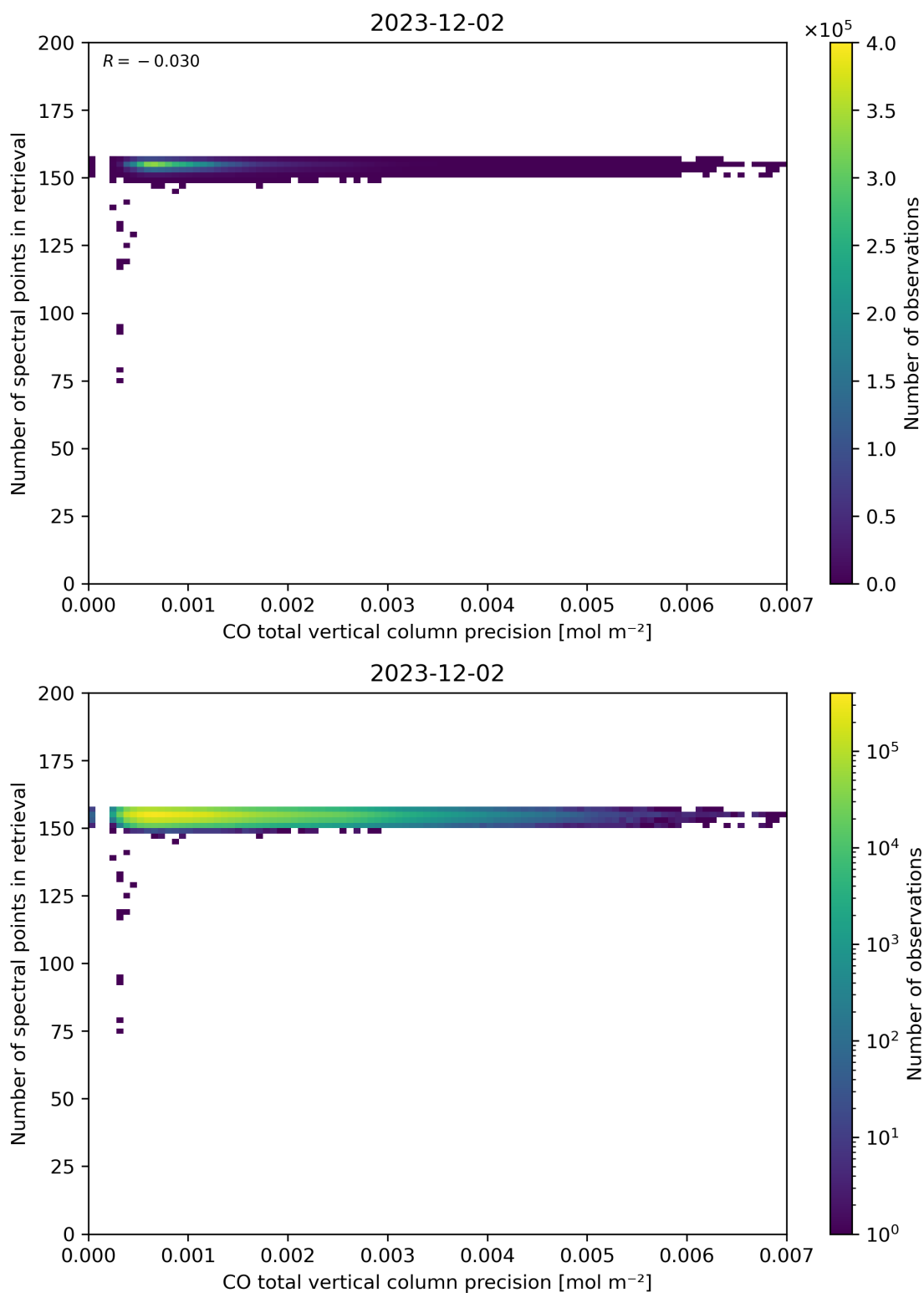
Figure 47: Scatter density plot of “CO total vertical column precision” against “Number of spectral points in retrieval” for 2023-12-01 to 2023-12-03.
