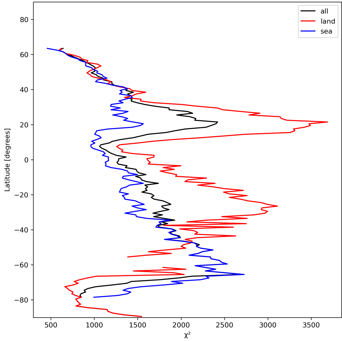
Figure 14: Zonal average of “ \chi^2 ” for 2023-12-01 to 2023-12-03.
