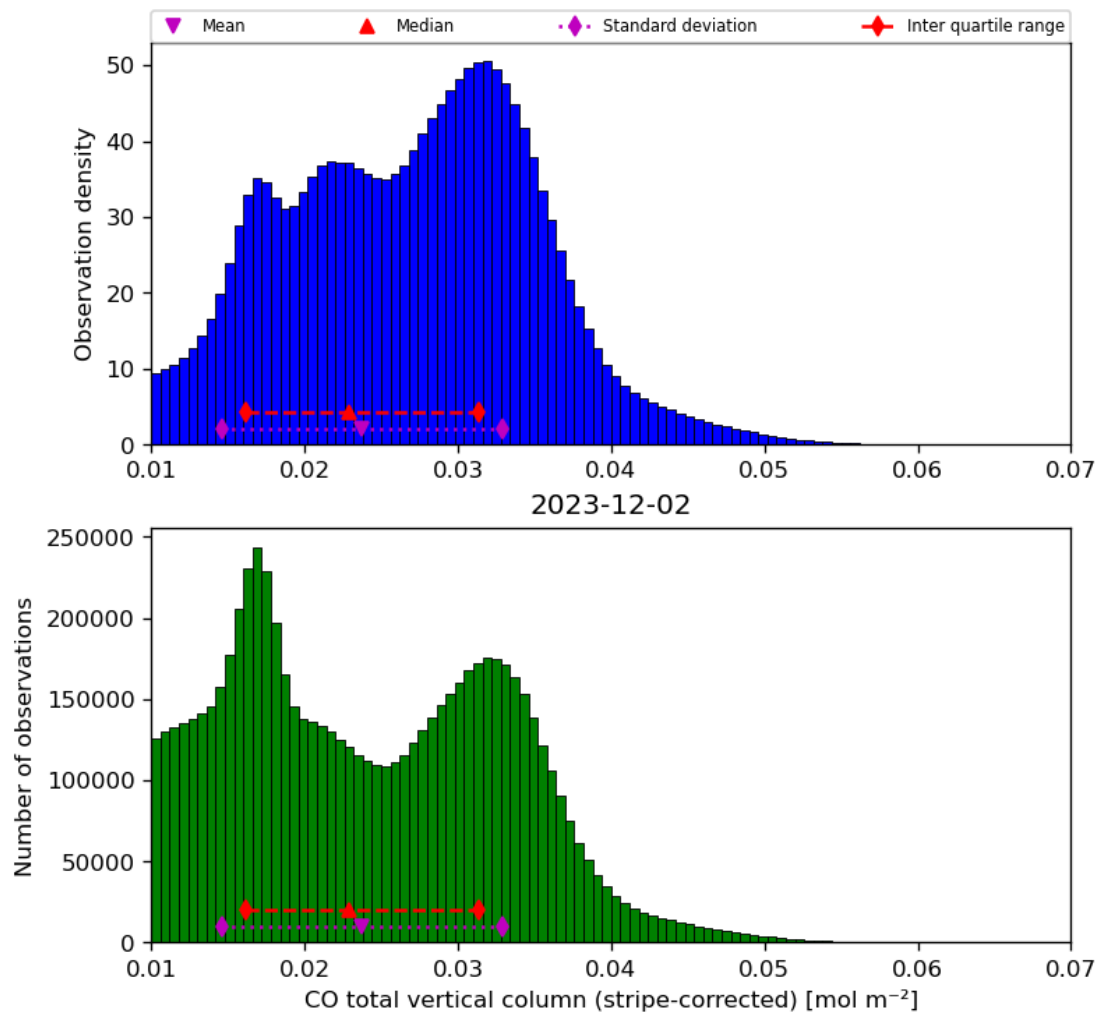
Figure 19: Histogram of “CO total vertical column (stripe-corrected)” for 2023-12-01 to 2023-12-03
