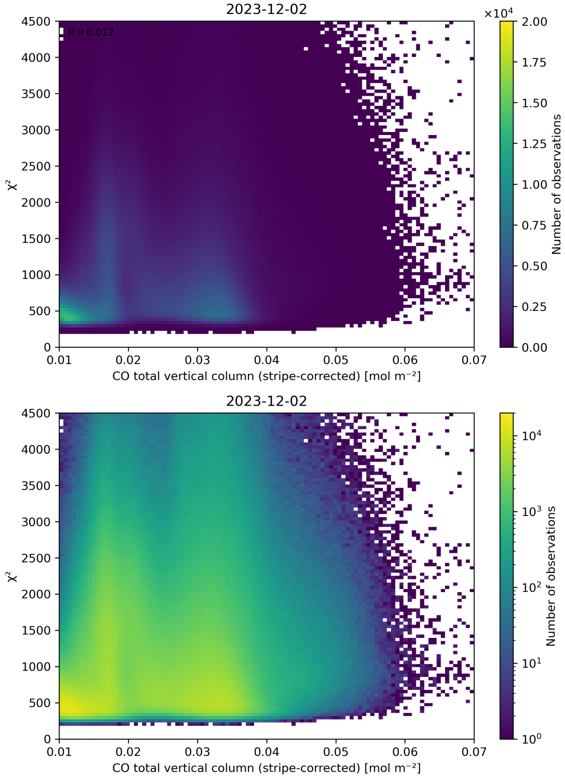
Figure 37: Scatter density plot of “CO total vertical column (stripe-corrected)” against “ \chi^2 ” for 2023-12-01 to 2023-12-03.
