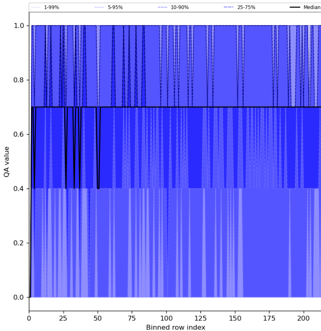
Figure 25: Along track statistics of “QA value” for 2023-12-01 to 2023-12-03
