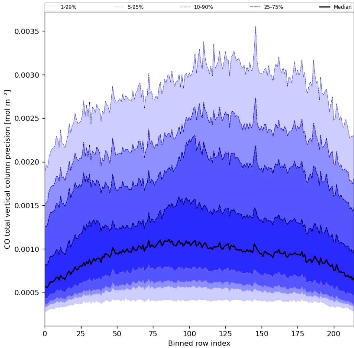
Figure 28: Along track statistics of “CO total vertical column precision” for 2023-12-01 to 2023-12-03
