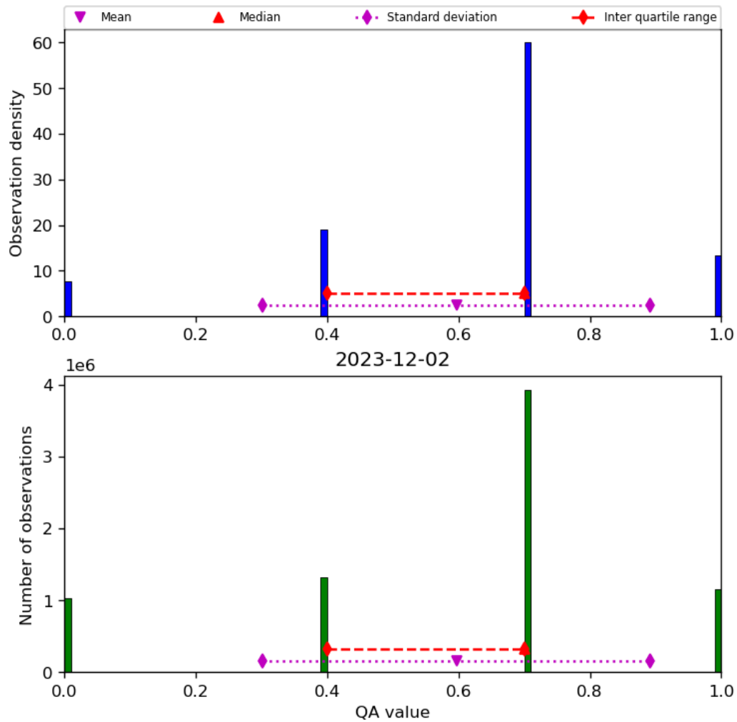
Figure 17: Histogram of “QA value” for 2023-12-01 to 2023-12-03
