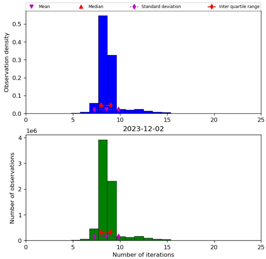
Figure 24: Histogram of “Number of iterations” for 2023-12-01 to 2023-12-03
