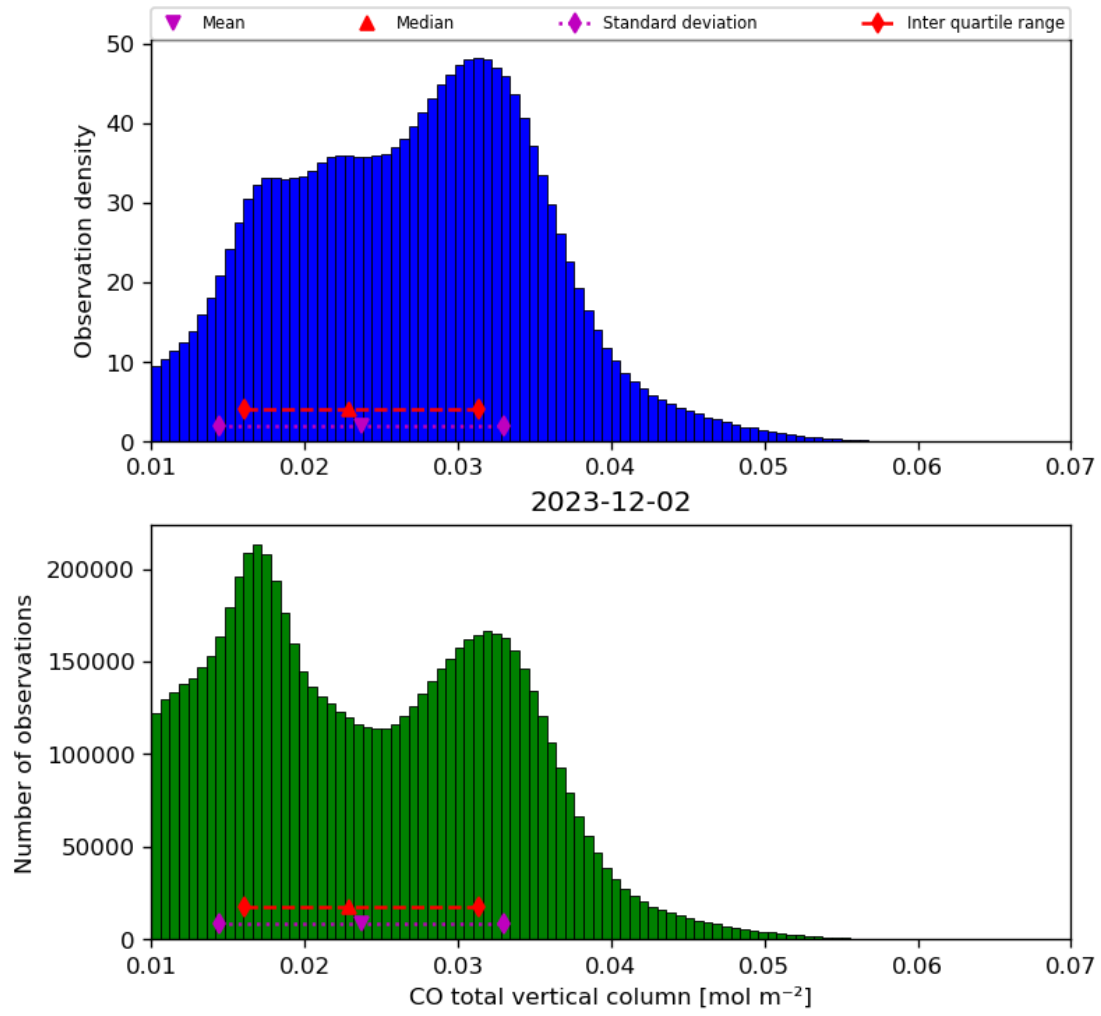
Figure 18: Histogram of “CO total vertical column” for 2023-12-01 to 2023-12-03
