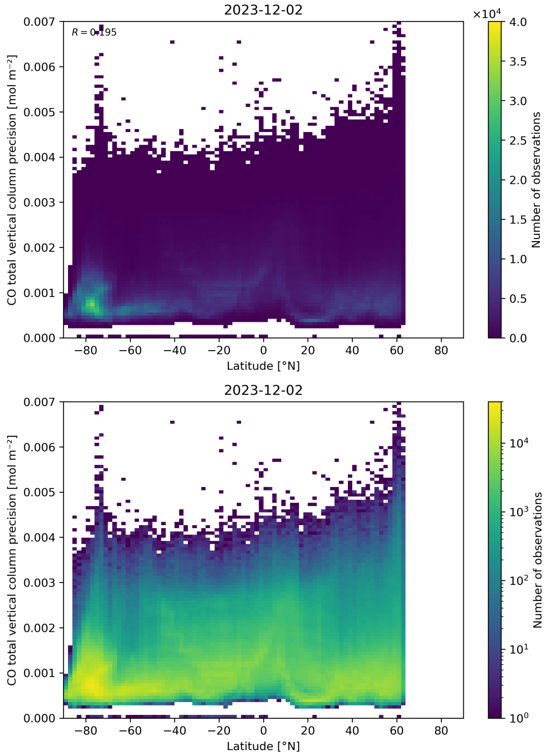
Figure 53: Scatter density plot of “Latitude” against “CO total vertical column precision” for 2023-12-01 to 2023-12-03.
