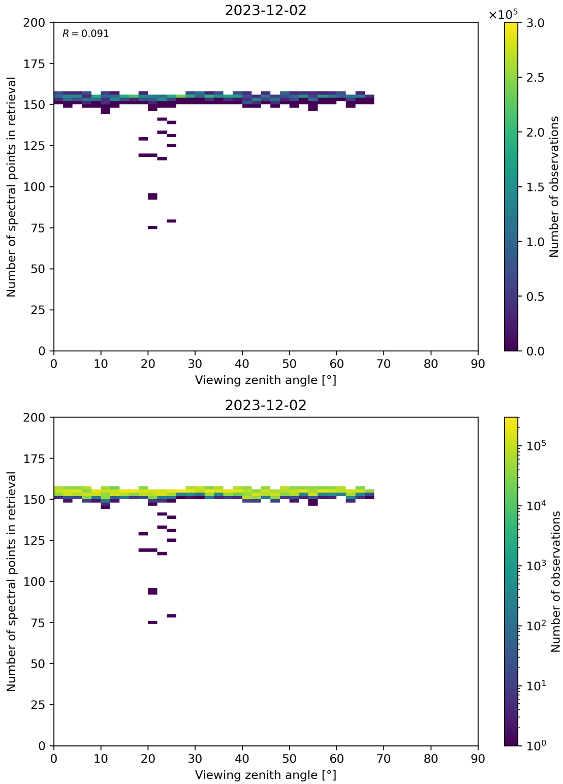
Figure 76: Scatter density plot of “Viewing zenith angle” against “Number of spectral points in retrieval” for 2023-12-01 to 2023-12-03.
