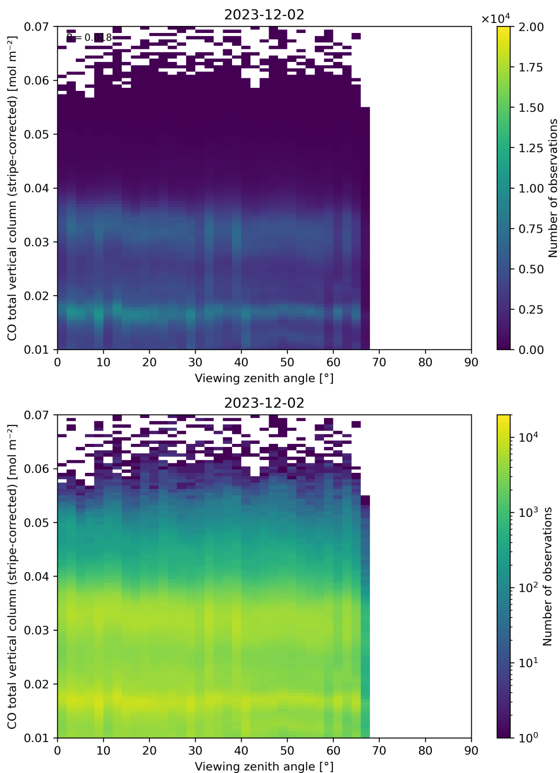
Figure 70: Scatter density plot of “Viewing zenith angle” against “CO total vertical column (stripe-corrected)” for 2023-12-01 to 2023-12-03.
