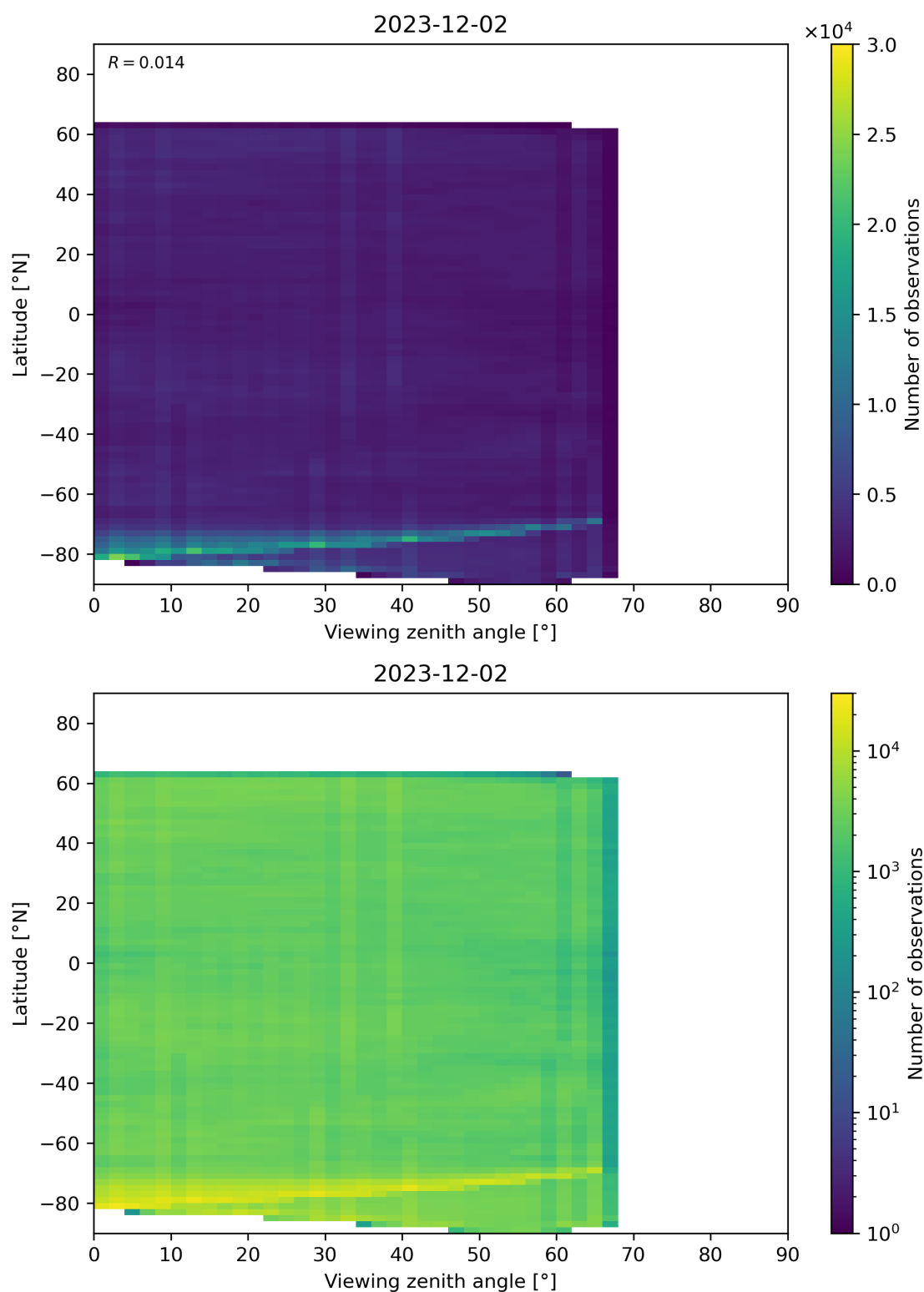
Figure 74: Scatter density plot of “Viewing zenith angle” against “Latitude” for 2023-12-01 to 2023-12-03.
