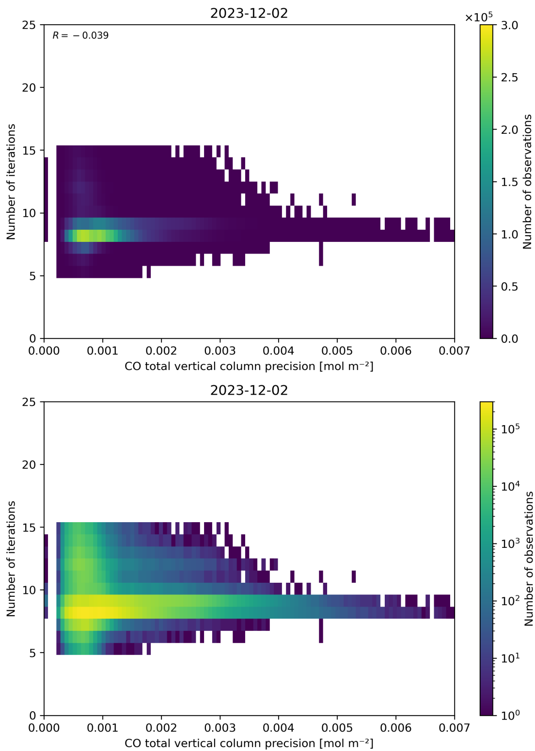
Figure 46: Scatter density plot of “CO total vertical column precision” against “Number of iterations” for 2023-12-01 to 2023-12-03.
