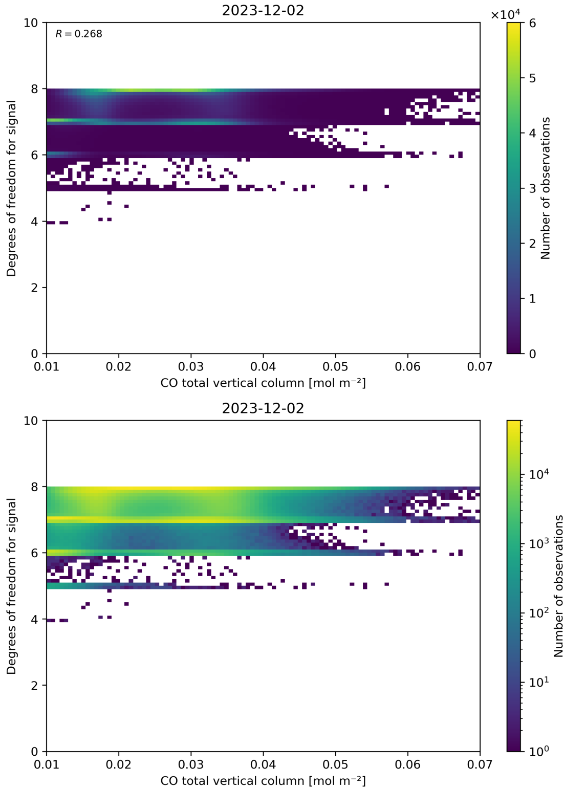
Figure 41: Scatter density plot of “CO total vertical column” against “Degrees of freedom for signal” for 2023-12-01 to 2023-12-03.
