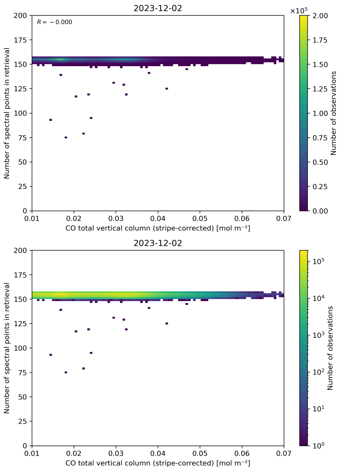
Figure 40: Scatter density plot of “CO total vertical column (stripe-corrected)” against “Number of spectral points in retrieval” for 2023-12-01 to 2023-12-03.
