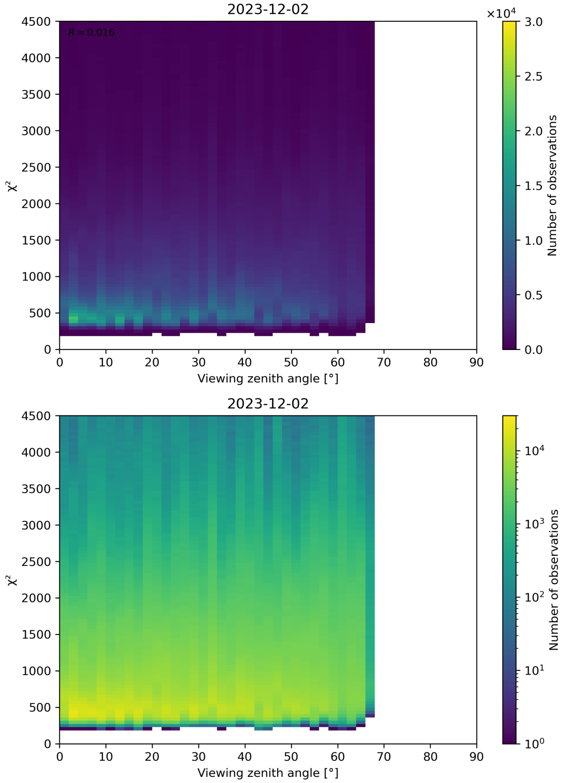
Figure 72: Scatter density plot of “Viewing zenith angle” against “ \chi^2 ” for 2023-12-01 to 2023-12-03.
