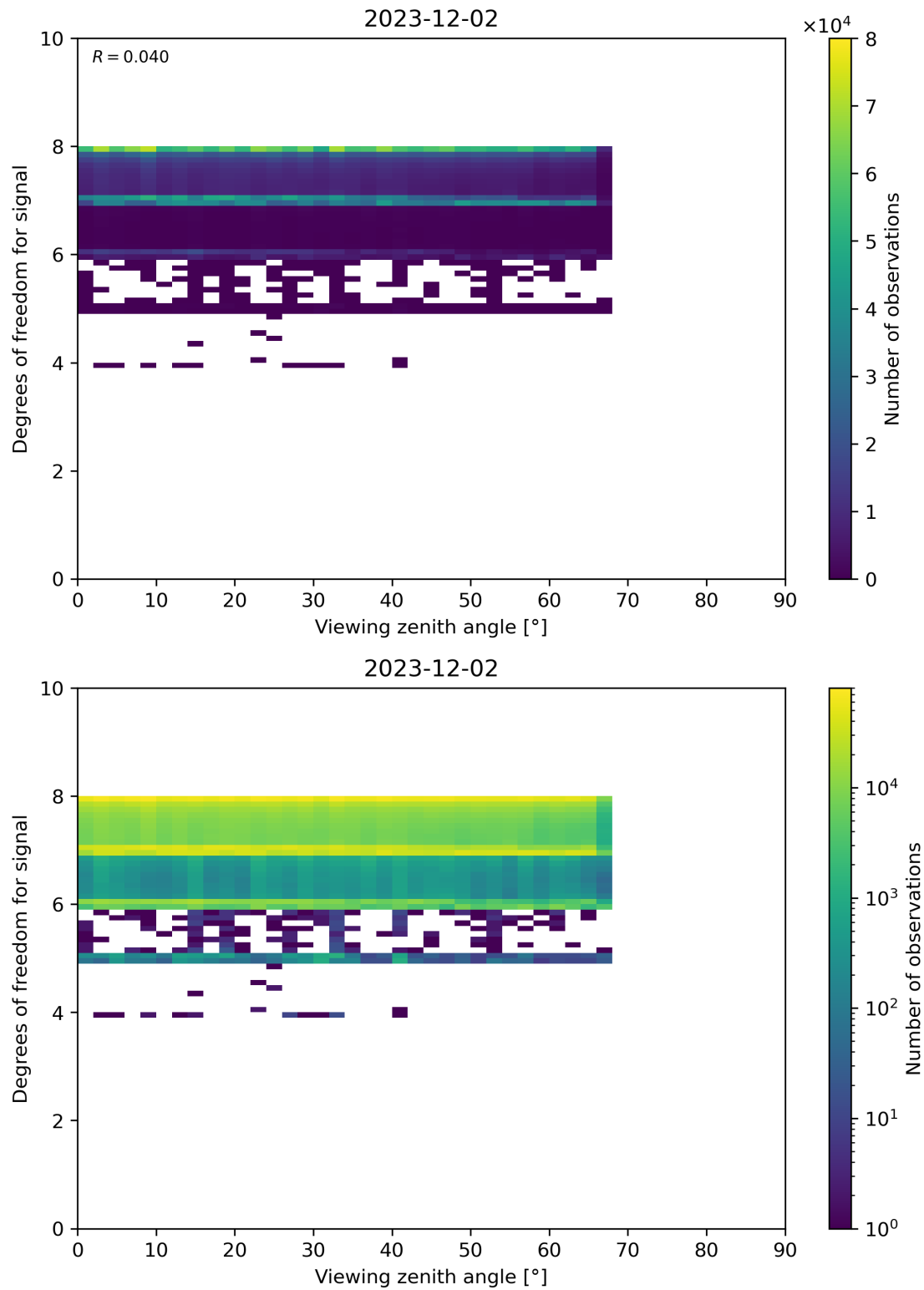
Figure 73: Scatter density plot of “Viewing zenith angle” against “Degrees of freedom for signal” for 2023-12-01 to 2023-12-03.
