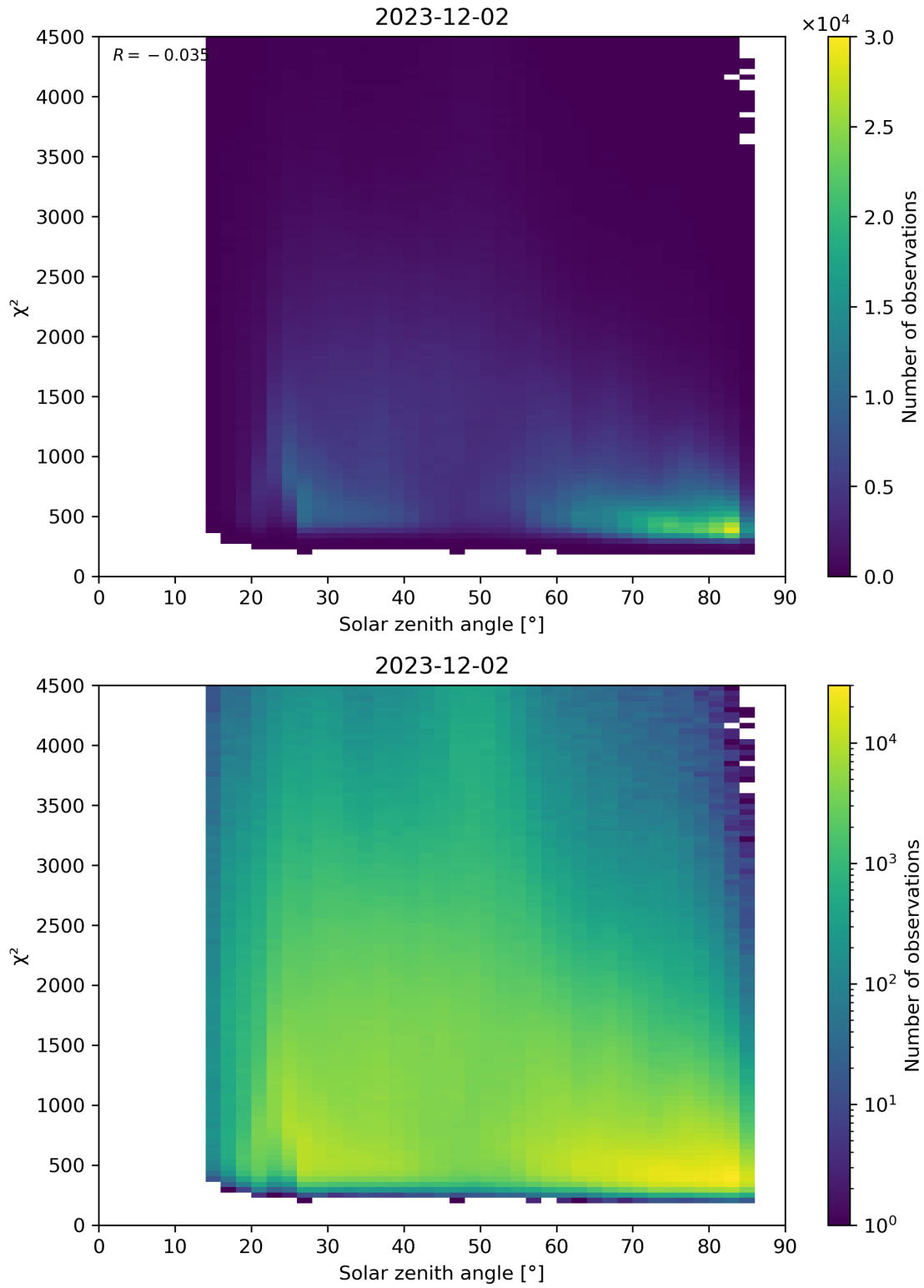
Figure 64: Scatter density plot of “Solar zenith angle” against “ \chi^2 ” for 2023-12-01 to 2023-12-03.
