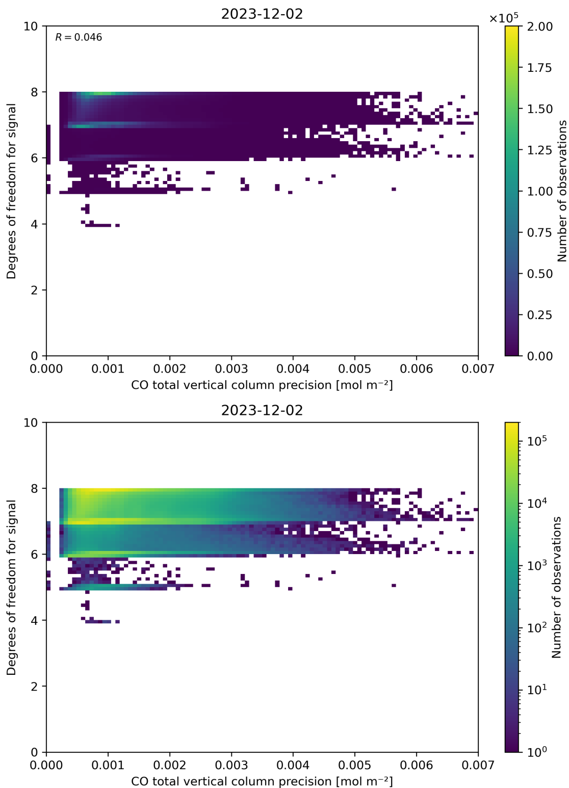
Figure 45: Scatter density plot of “CO total vertical column precision” against “Degrees of freedom for signal” for 2023-12-01 to 2023-12-03.
