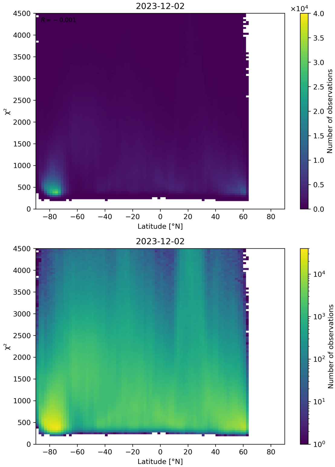
Figure 54: Scatter density plot of “Latitude” against “ \chi^2 ” for 2023-12-01 to 2023-12-03.
