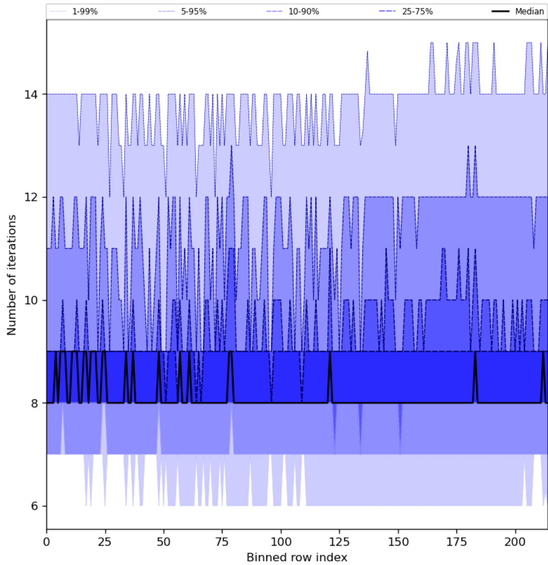
Figure 32: Along track statistics of “Number of iterations” for 2023-12-01 to 2023-12-03
