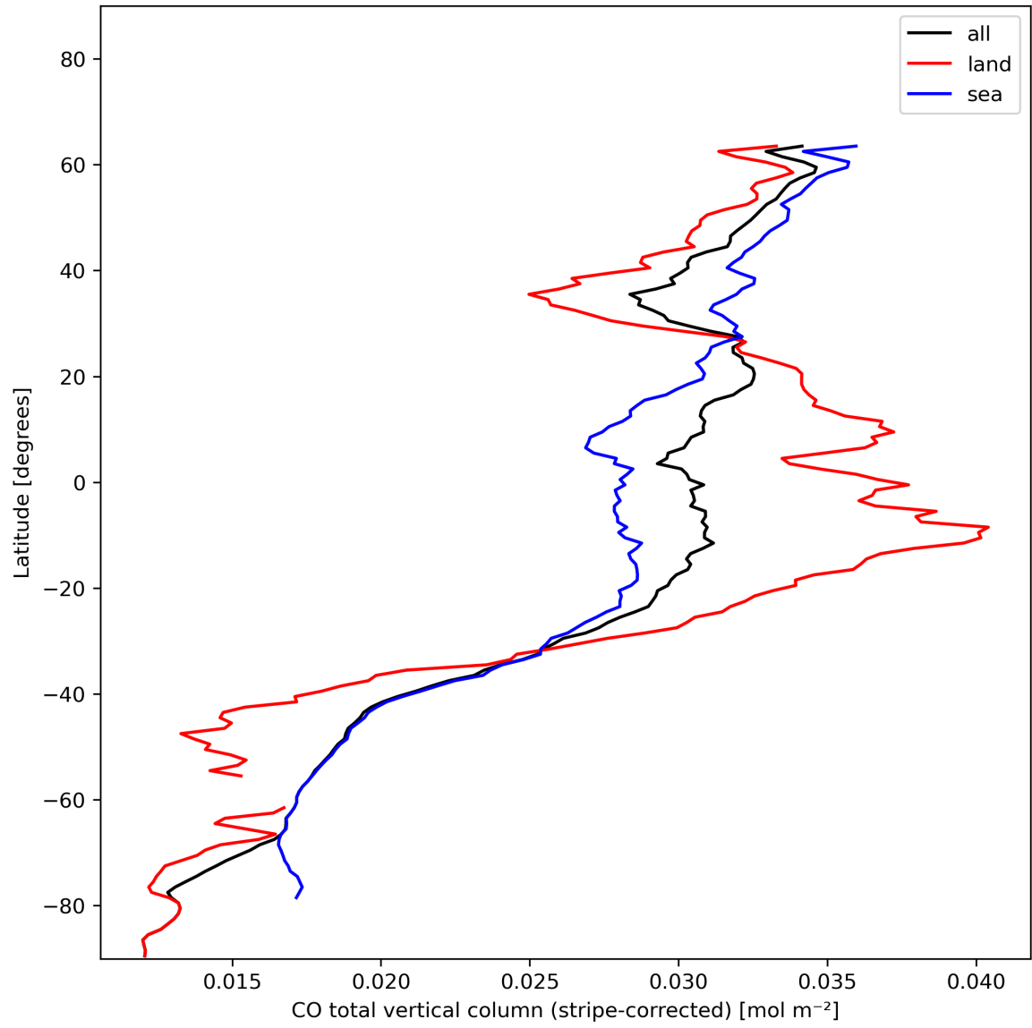
Figure 11: Zonal average of “CO total vertical column (stripe-corrected)” for 2023-12-01 to 2023-12-03.
