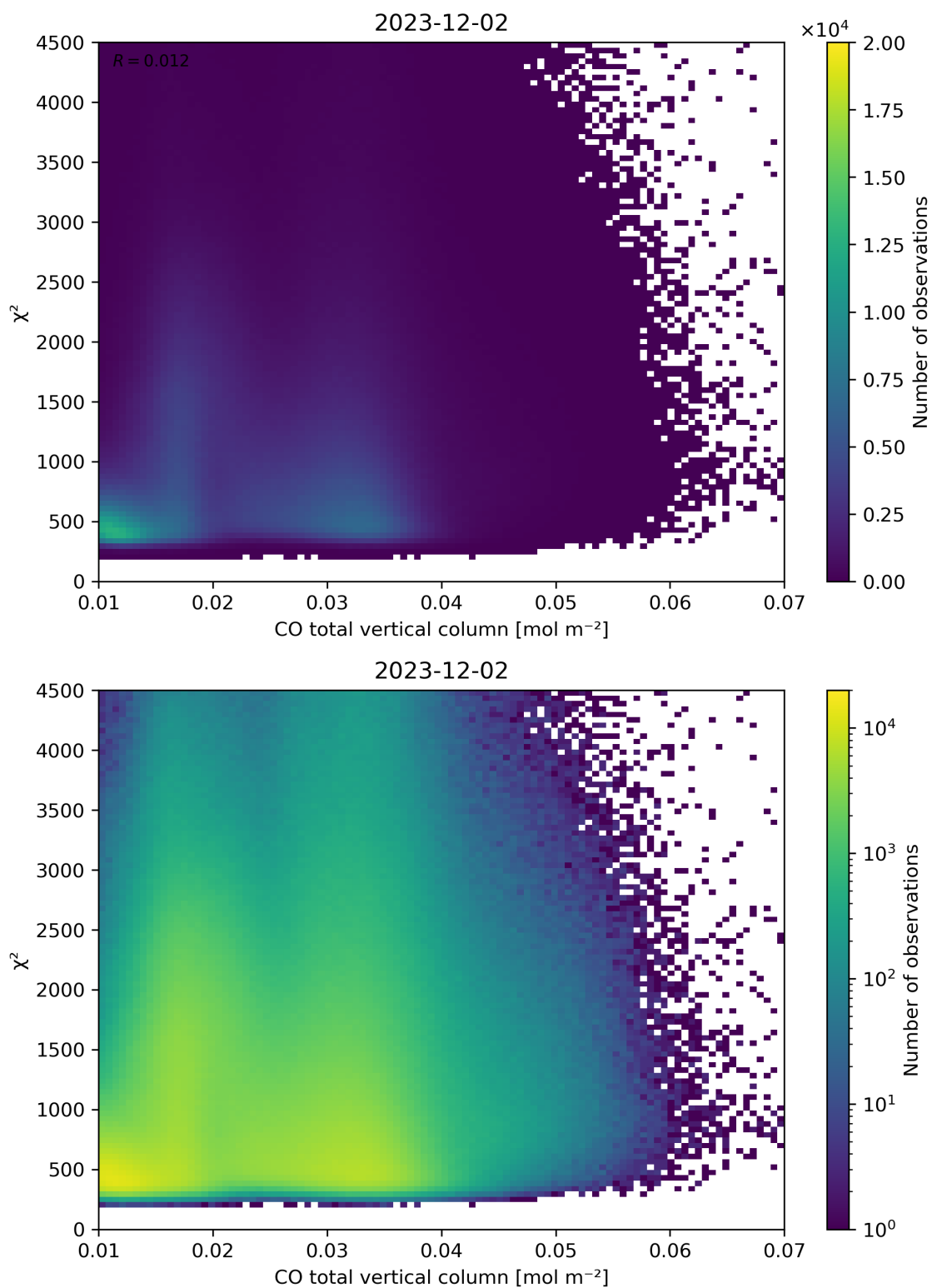
Figure 35: Scatter density plot of “CO total vertical column” against “ \chi^2 ” for 2023-12-01 to 2023-12-03.
