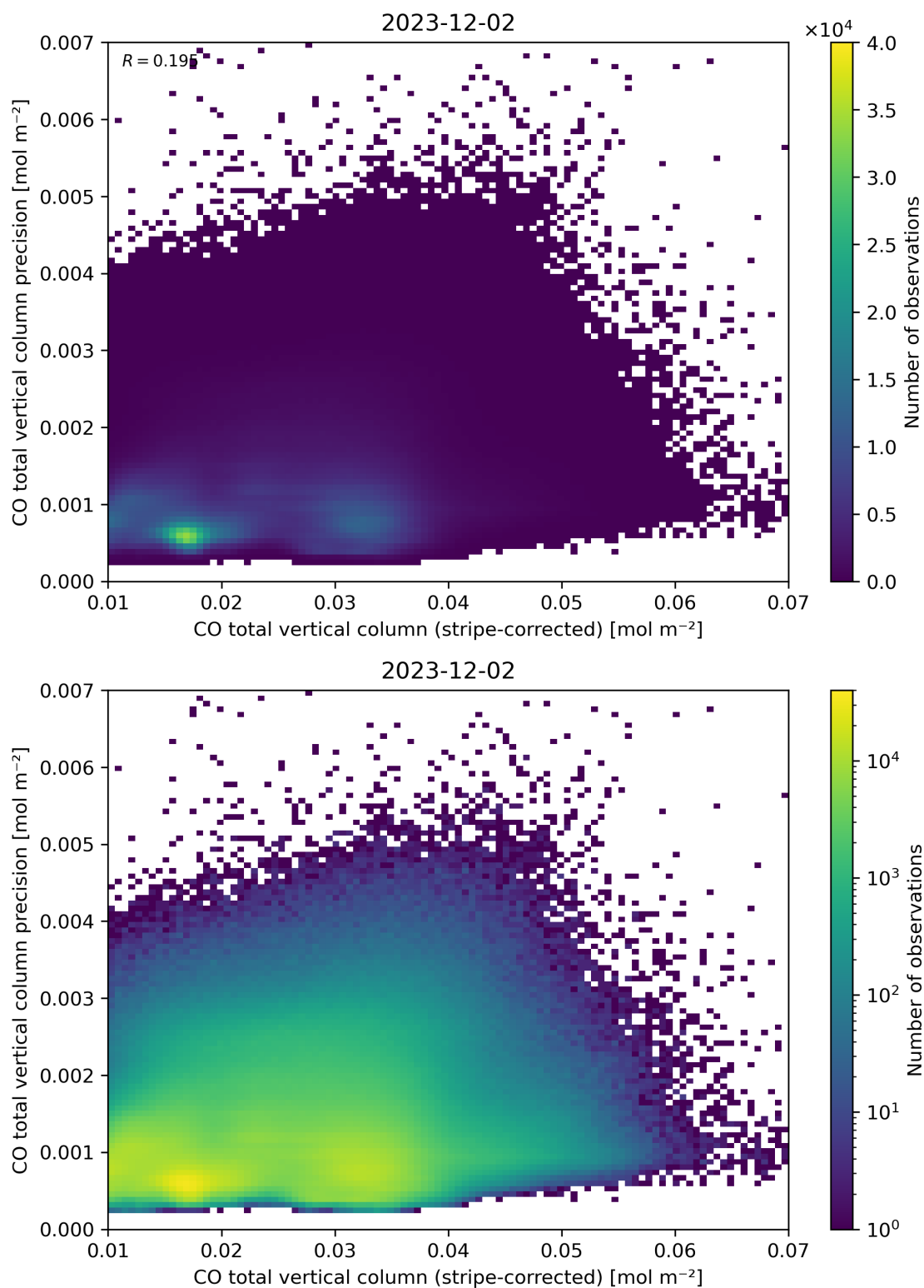
Figure 36: Scatter density plot of “CO total vertical column (stripe-corrected)” against “CO total vertical column precision” for 2023-12-01 to 2023-12-03.
