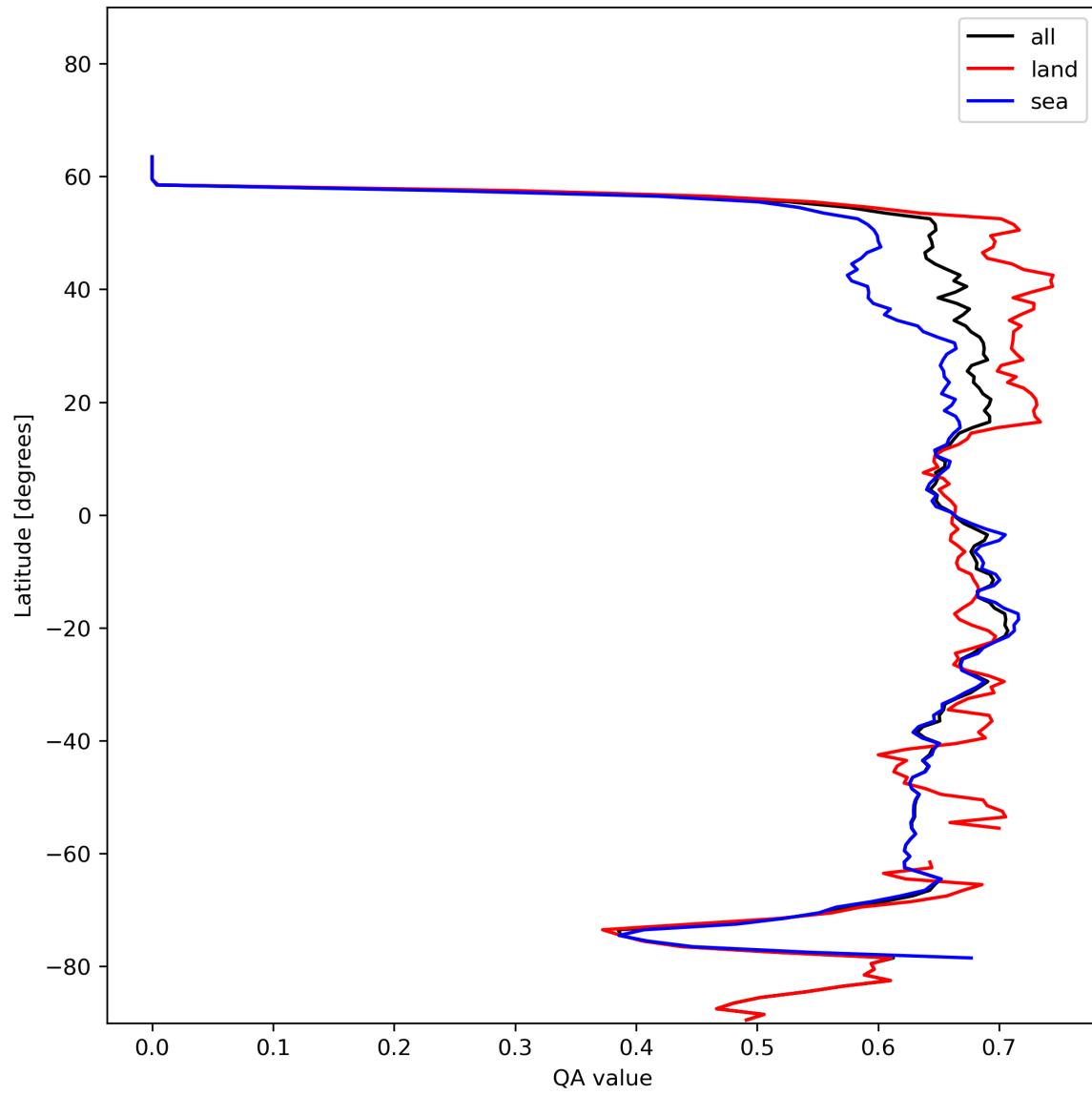
Figure 9: Zonal average of “QA value” for 2023-12-01 to 2023-12-03.
