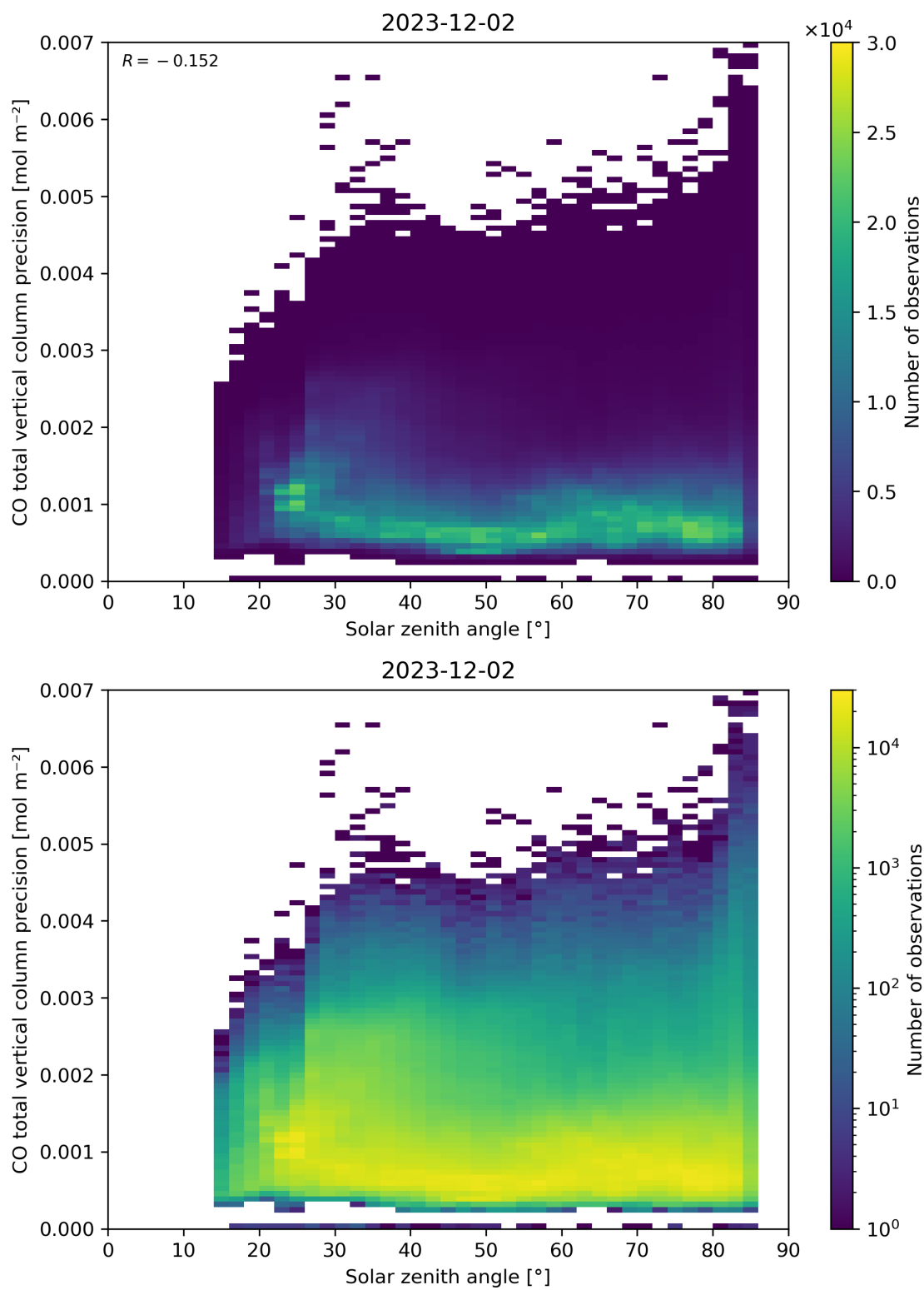
Figure 63: Scatter density plot of “Solar zenith angle” against “CO total vertical column precision” for 2023-12-01 to 2023-12-03.
