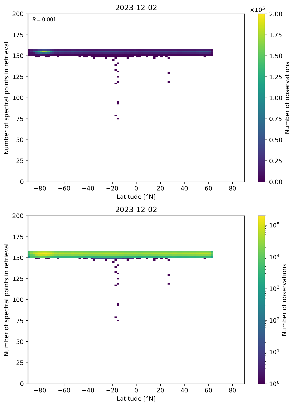
Figure 57: Scatter density plot of “Latitude” against “Number of spectral points in retrieval” for 2023-12-01 to 2023-12-03.
