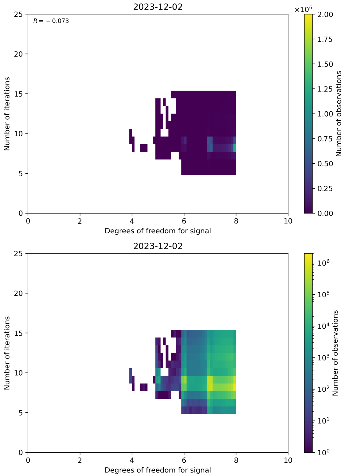
Figure 50: Scatter density plot of “Degrees of freedom for signal” against “Number of iterations” for 2023-12-01 to 2023-12-03.
