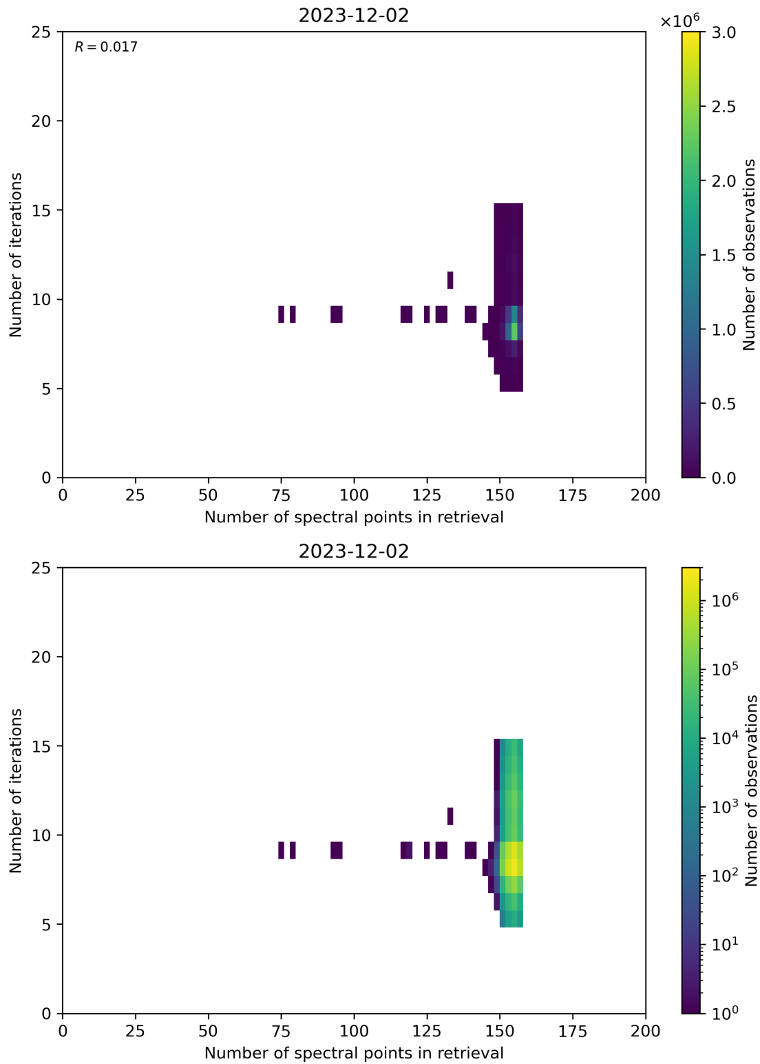
Figure 60: Scatter density plot of “Number of spectral points in retrieval” against “Number of iterations” for 2023-12-01 to 2023-12-03.
