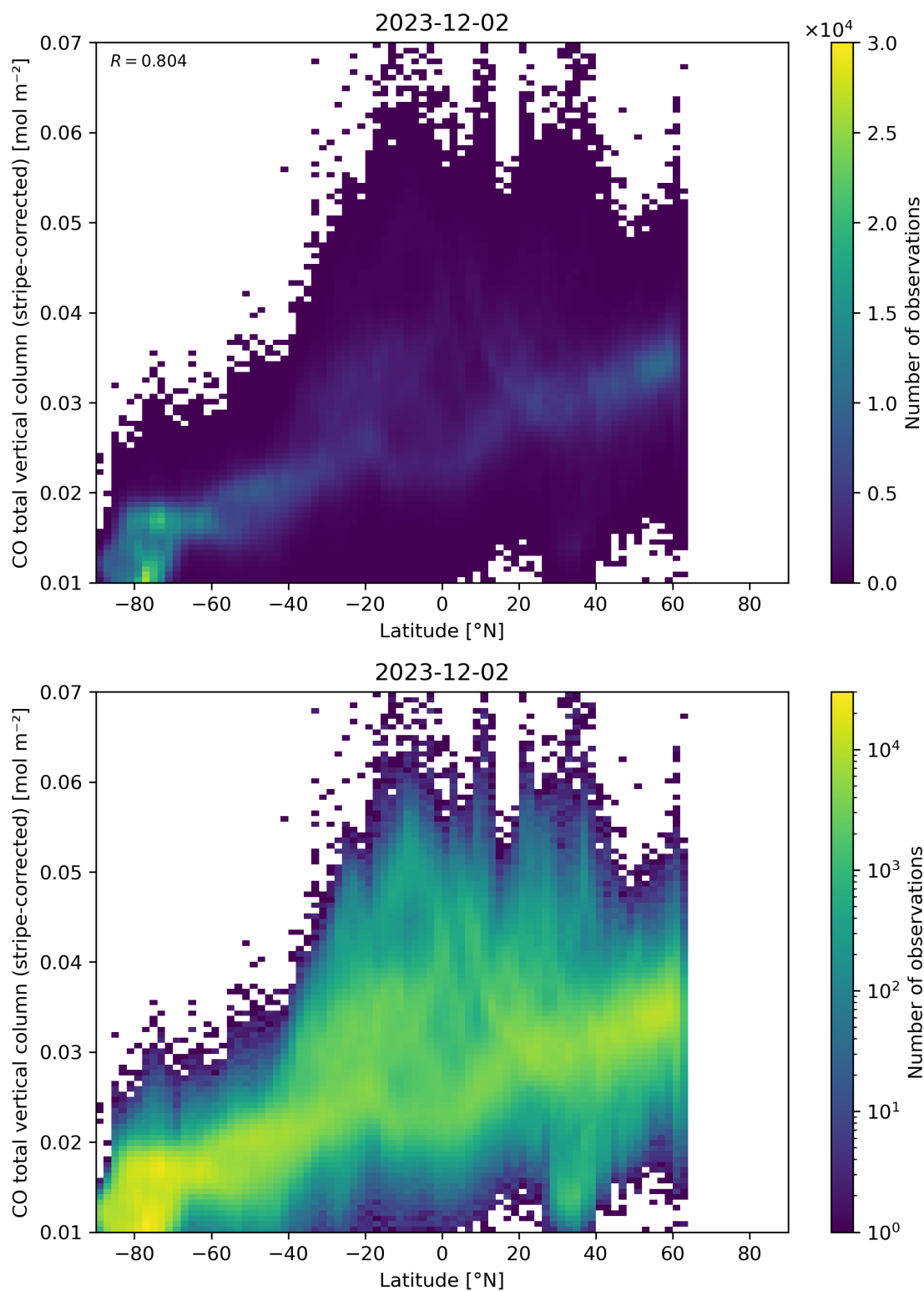
Figure 52: Scatter density plot of “Latitude” against “CO total vertical column (stripe-corrected)” for 2023-12-01 to 2023-12-03.
