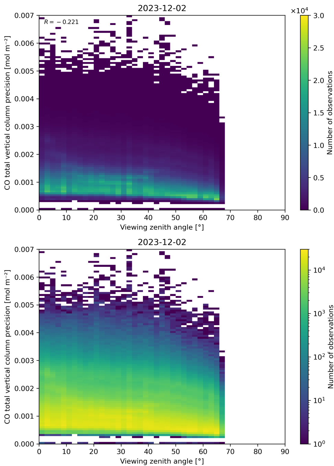
Figure 71: Scatter density plot of “Viewing zenith angle” against “CO total vertical column precision” for 2023-12-01 to 2023-12-03.
