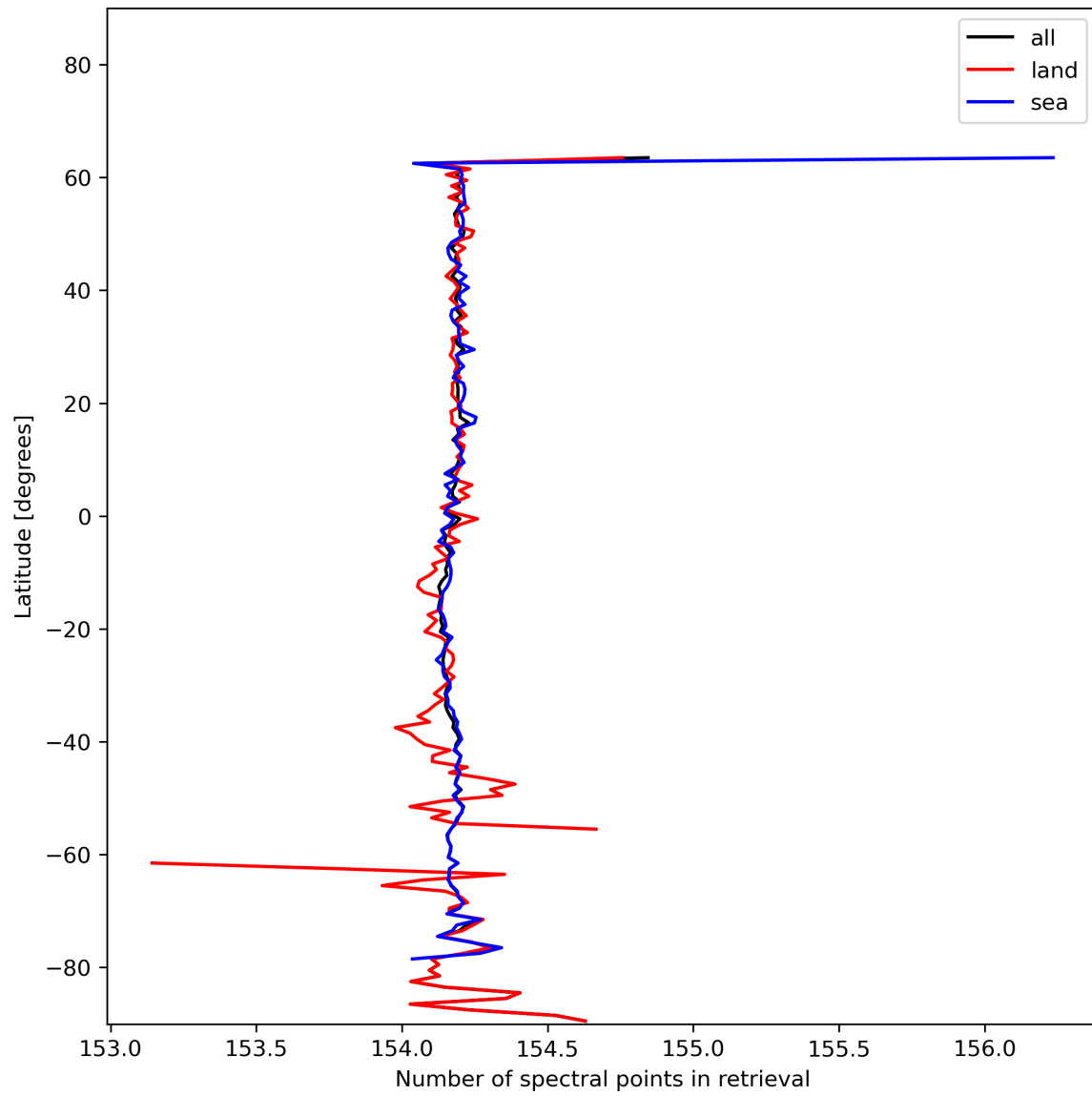
Figure 13: Zonal average of “Number of spectral points in retrieval” for 2023-12-01 to 2023-12-03.
