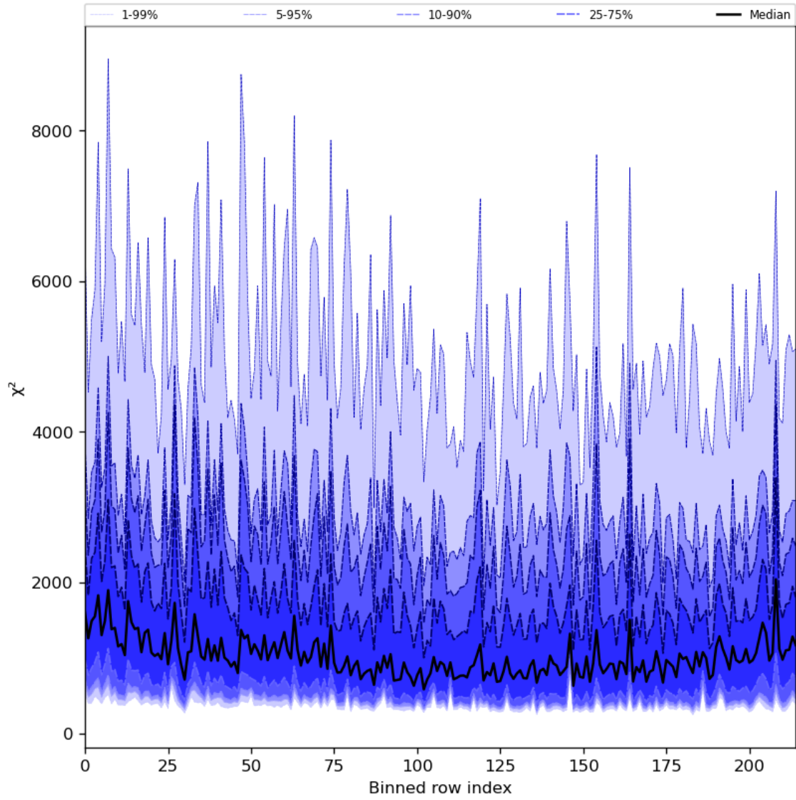
Figure 30: Along track statistics of “ \chi^2 ” for 2023-12-01 to 2023-12-03
