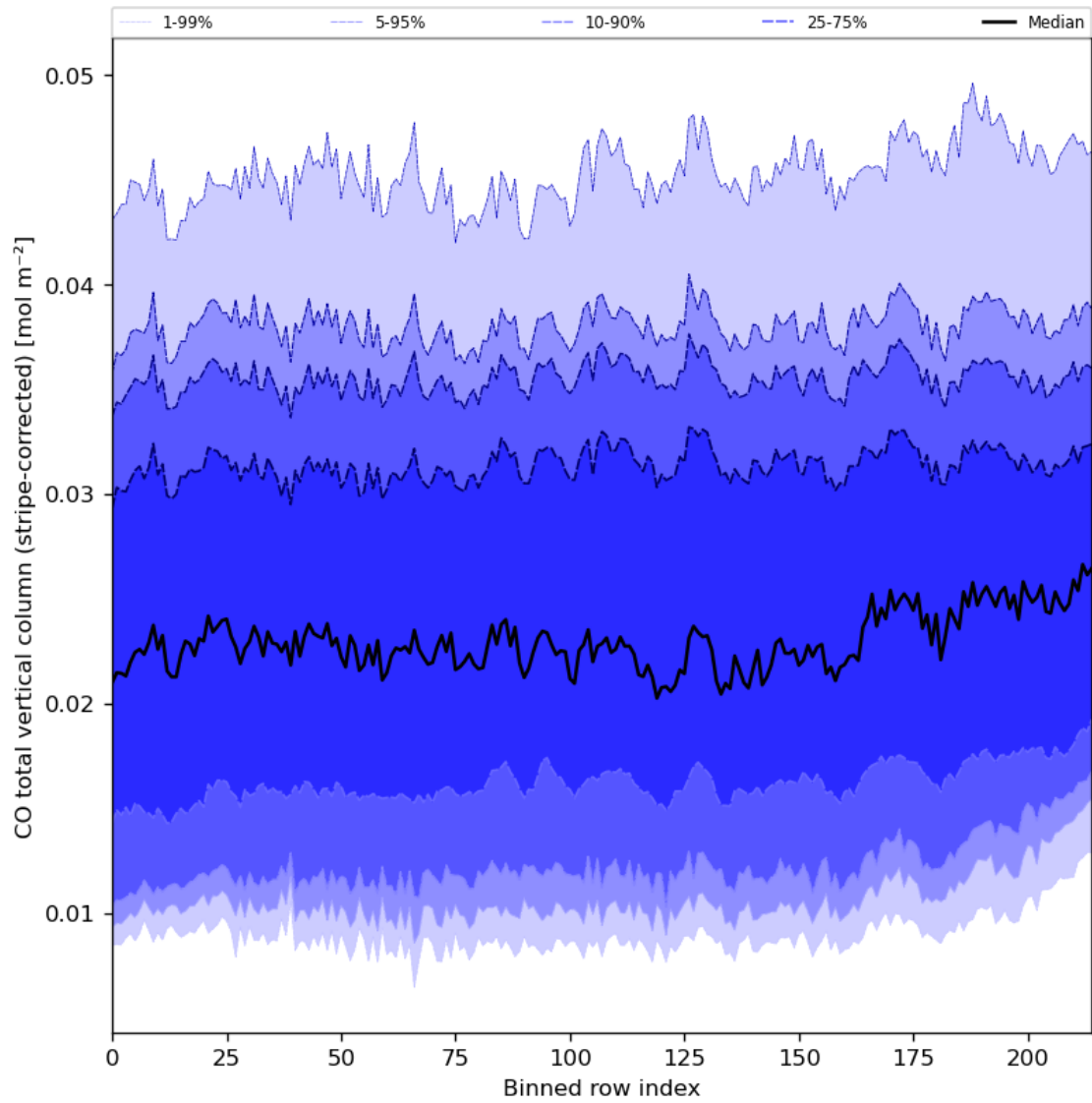
Figure 27: Along track statistics of “CO total vertical column (stripe-corrected)” for 2023-12-01 to 2023-12-03
