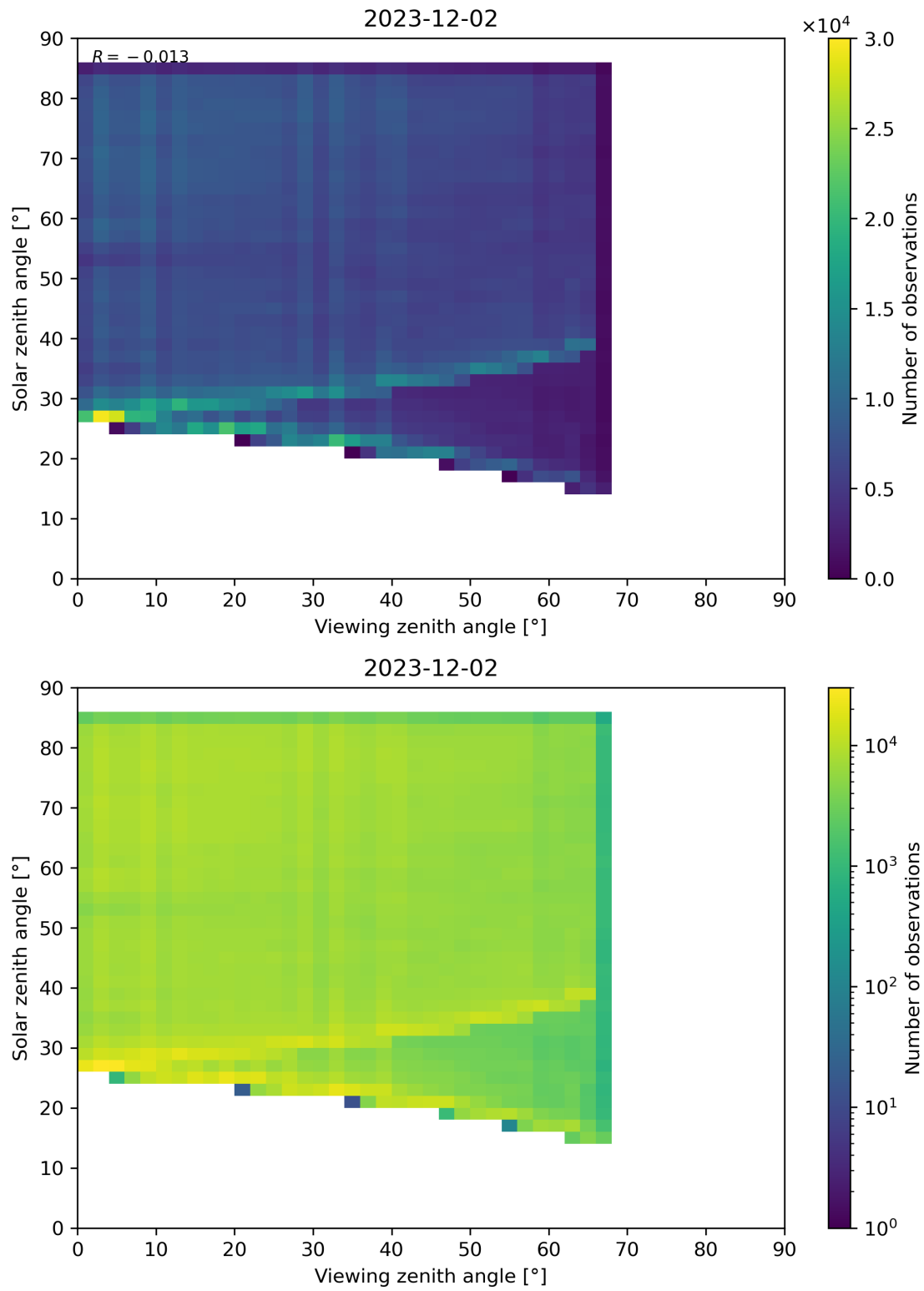
Figure 77: Scatter density plot of “Viewing zenith angle” against “Solar zenith angle” for 2023-12-01 to 2023-12-03.
