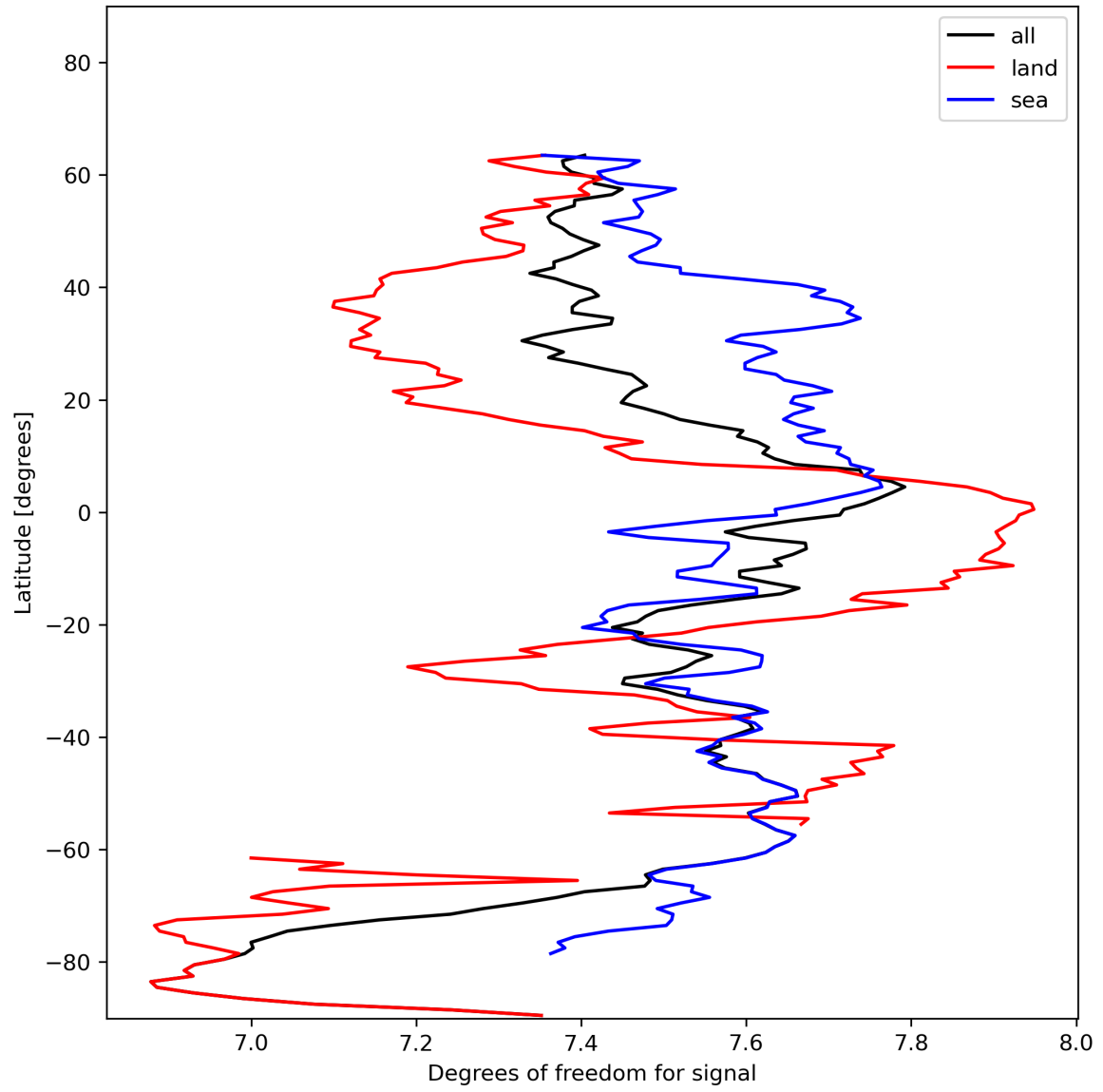
Figure 15: Zonal average of “Degrees of freedom for signal” for 2023-12-01 to 2023-12-03.
