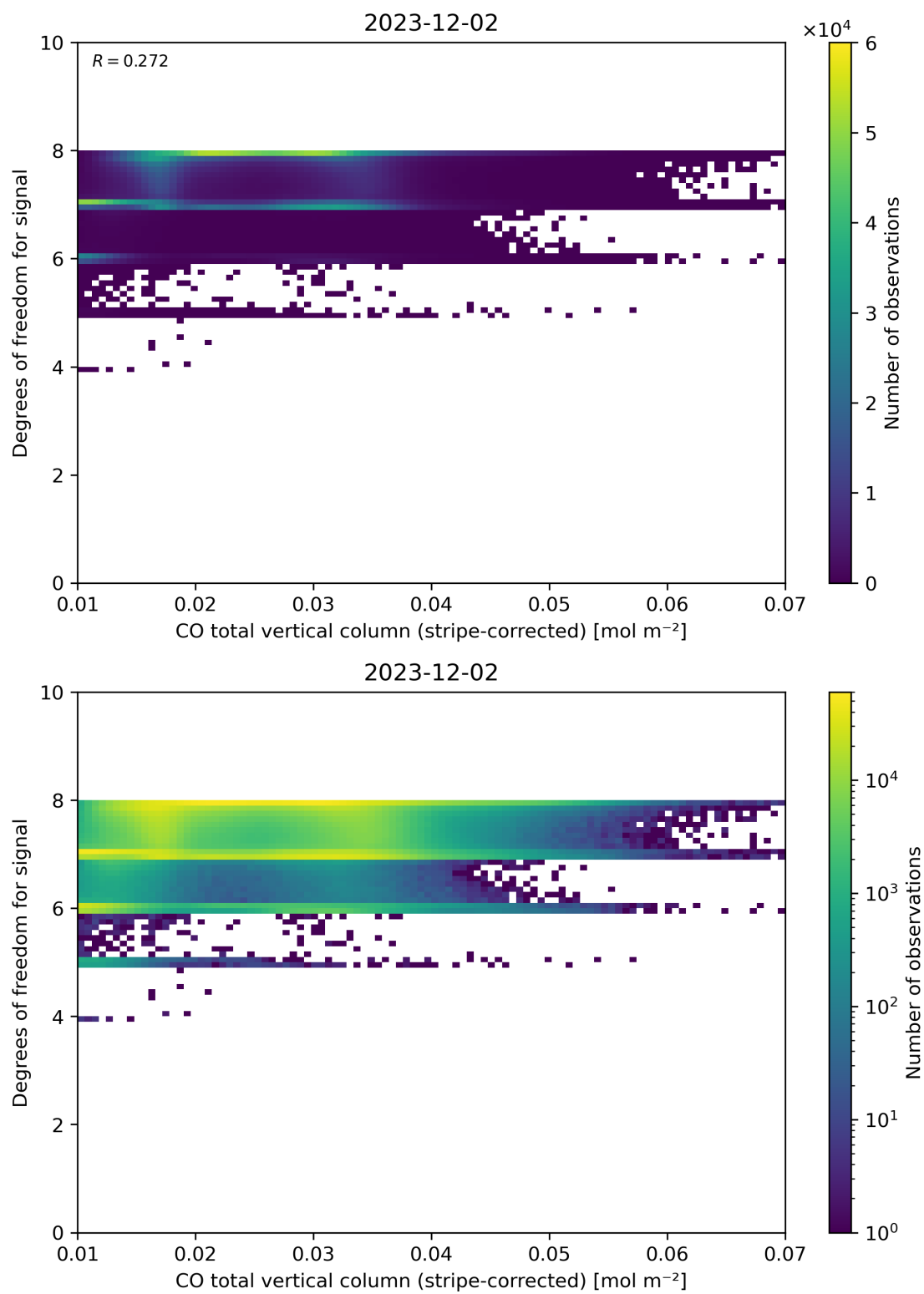
Figure 38: Scatter density plot of “CO total vertical column (stripe-corrected)” against “Degrees of freedom for signal” for 2023-12-01 to 2023-12-03.
