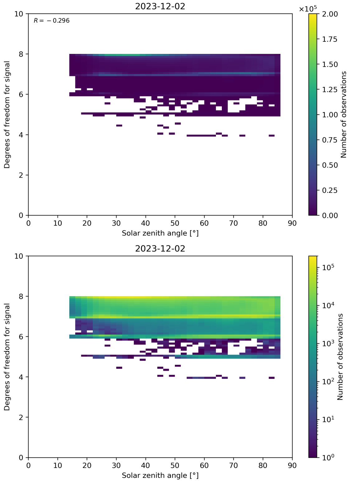
Figure 65: Scatter density plot of “Solar zenith angle” against “Degrees of freedom for signal” for 2023-12-01 to 2023-12-03.
