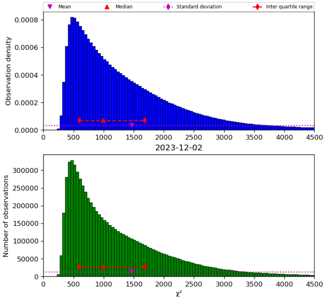
Figure 22: Histogram of “ \chi^2 ” for 2023-12-01 to 2023-12-03
