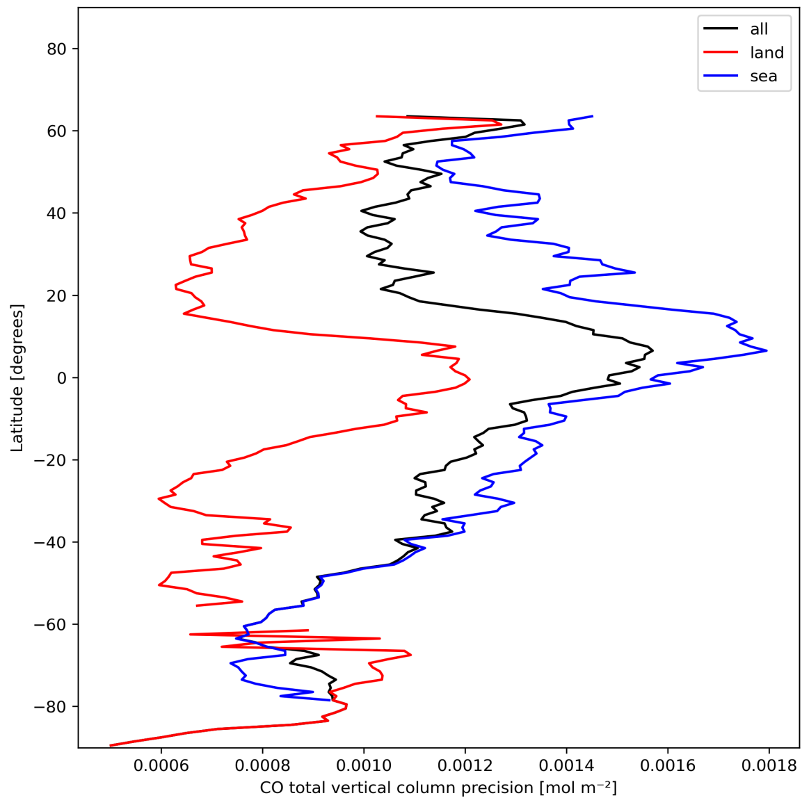
Figure 12: Zonal average of “CO total vertical column precision” for 2023-12-01 to 2023-12-03.
