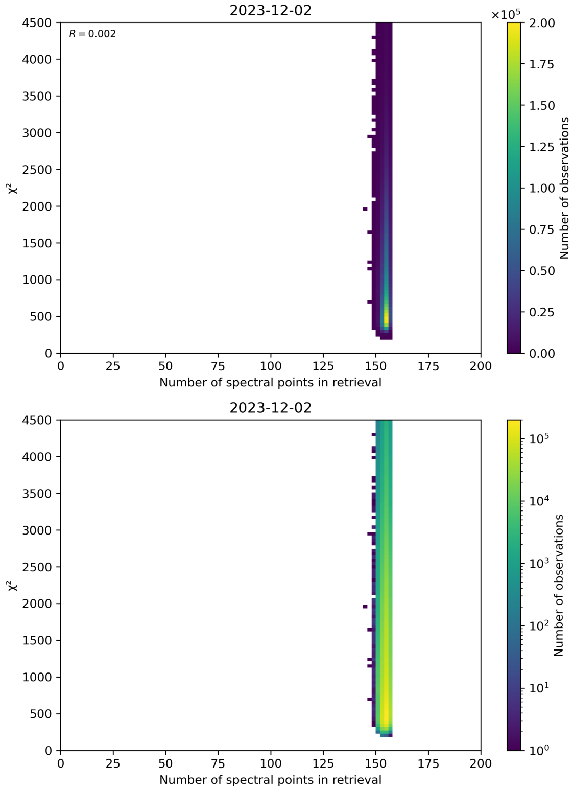
Figure 58: Scatter density plot of “Number of spectral points in retrieval” against “ \chi^2 ” for 2023-12-01 to 2023-12-03.
