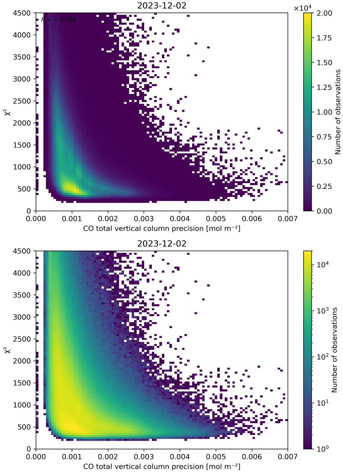
Figure 44: Scatter density plot of “CO total vertical column precision” against “ \chi^2 ” for 2023-12-01 to 2023-12-03.
