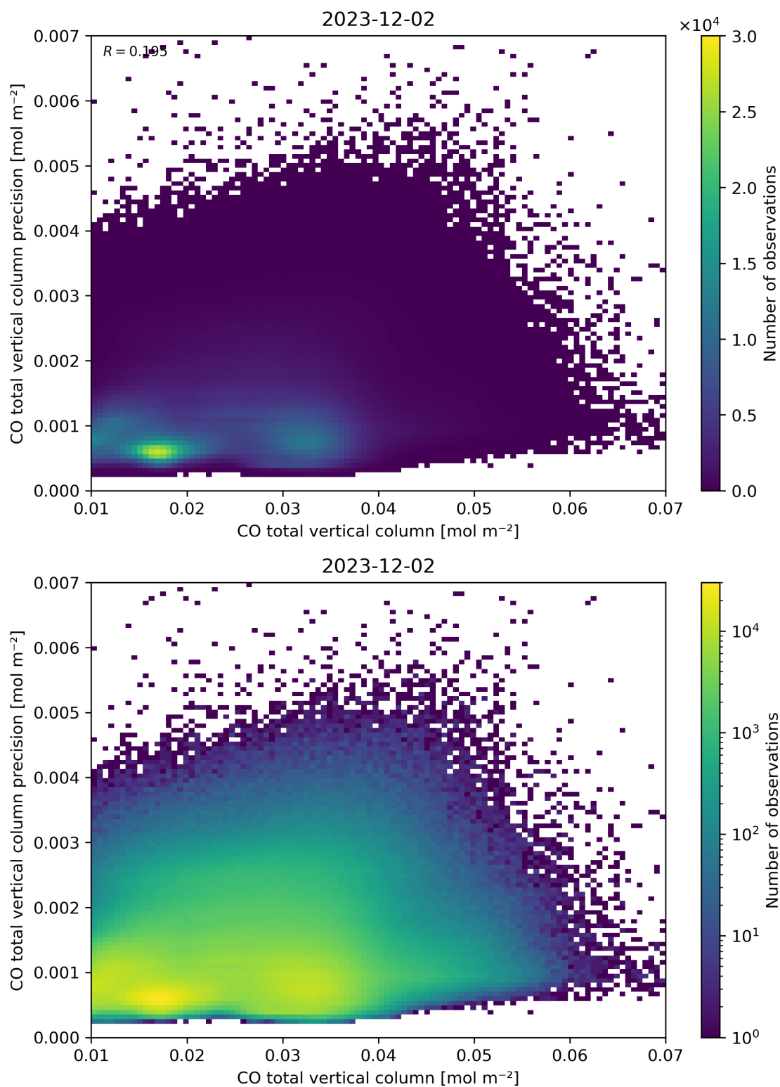
Figure 34: Scatter density plot of “CO total vertical column” against “CO total vertical column precision” for 2023-12-01 to 2023-12-03.
