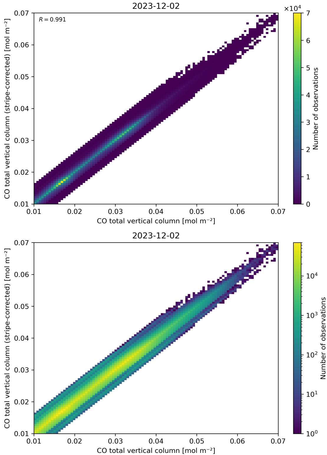
Figure 33: Scatter density plot of “CO total vertical column” against “CO total vertical column (stripe-corrected)” for 2023-12-01 to 2023-12-03.
