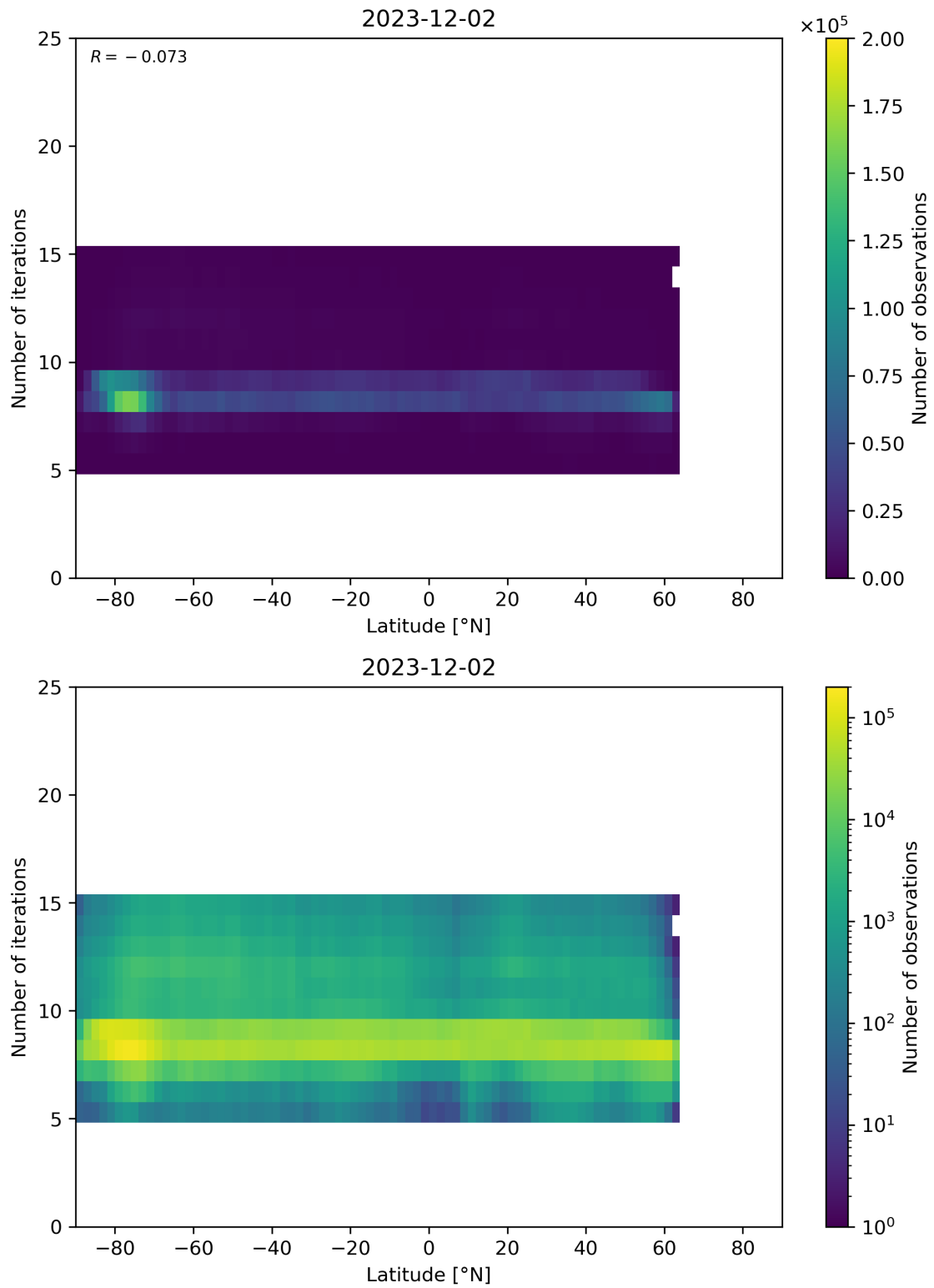
Figure 56: Scatter density plot of “Latitude” against “Number of iterations” for 2023-12-01 to 2023-12-03.
