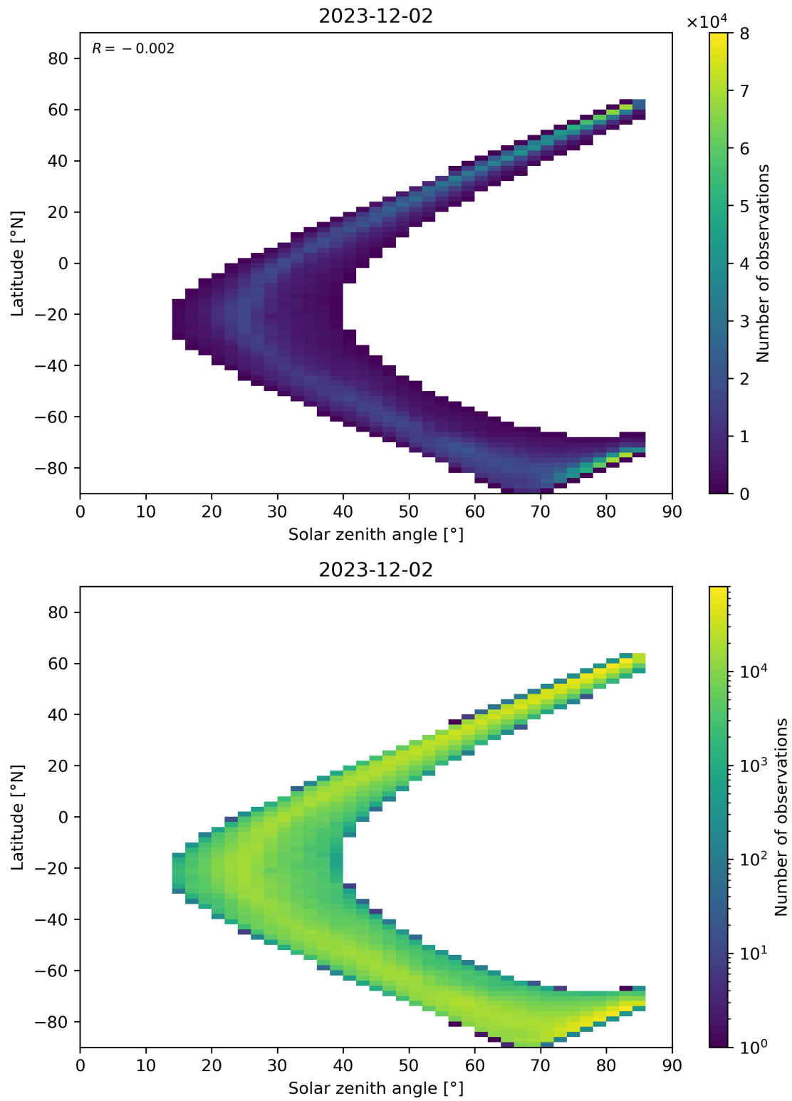
Figure 66: Scatter density plot of “Solar zenith angle” against “Latitude” for 2023-12-01 to 2023-12-03.
