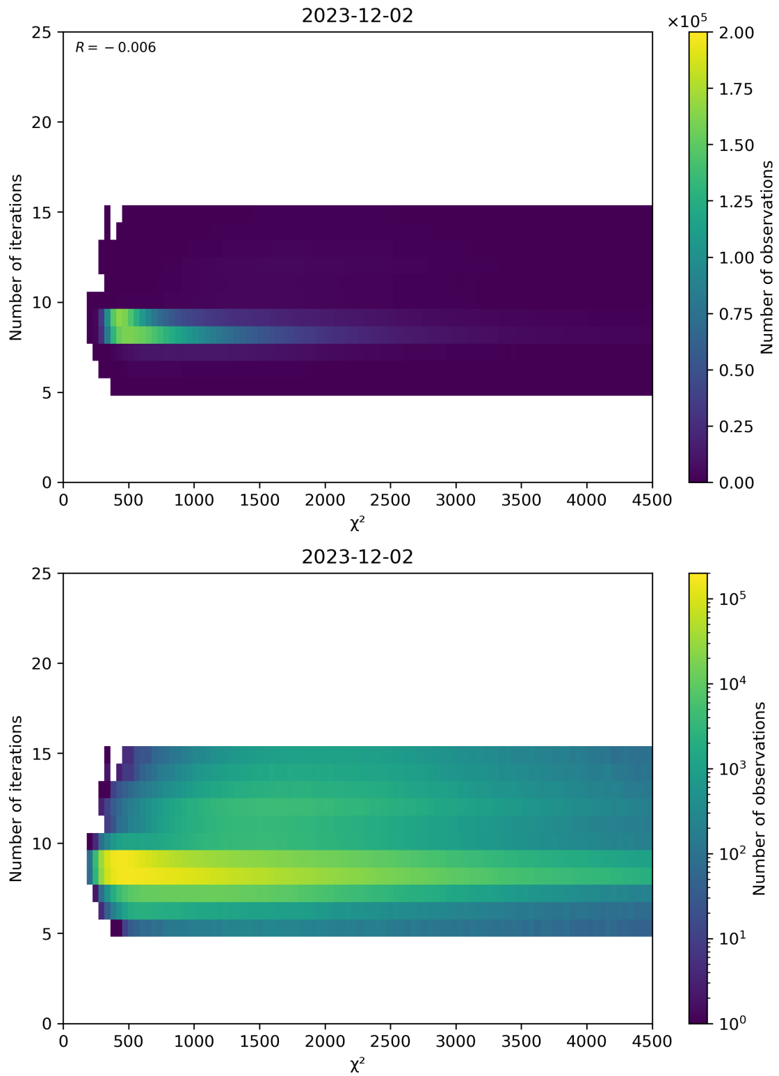
Figure 49: Scatter density plot of “ \chi^2 ” against “Number of iterations” for 2023-12-01 to 2023-12-03.
