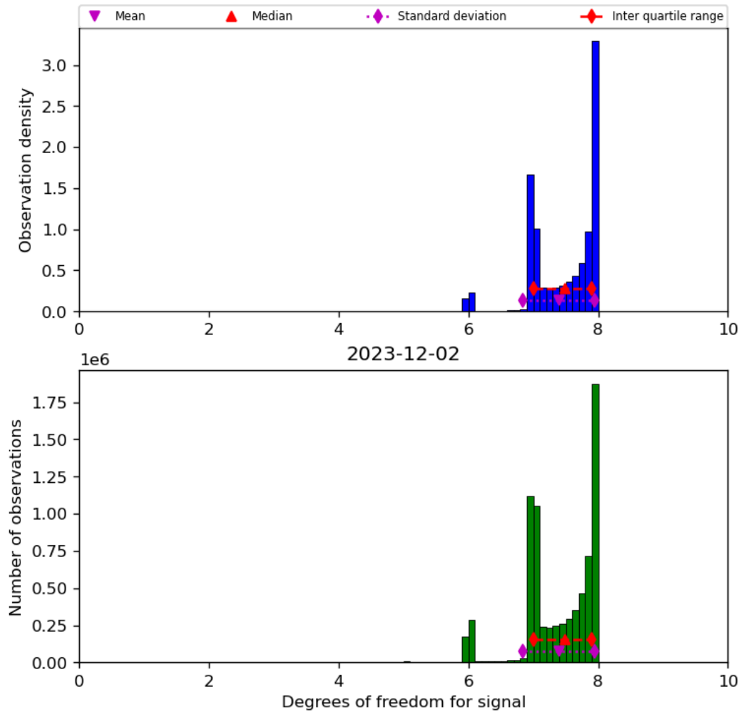
Figure 23: Histogram of “Degrees of freedom for signal” for 2023-12-01 to 2023-12-03
